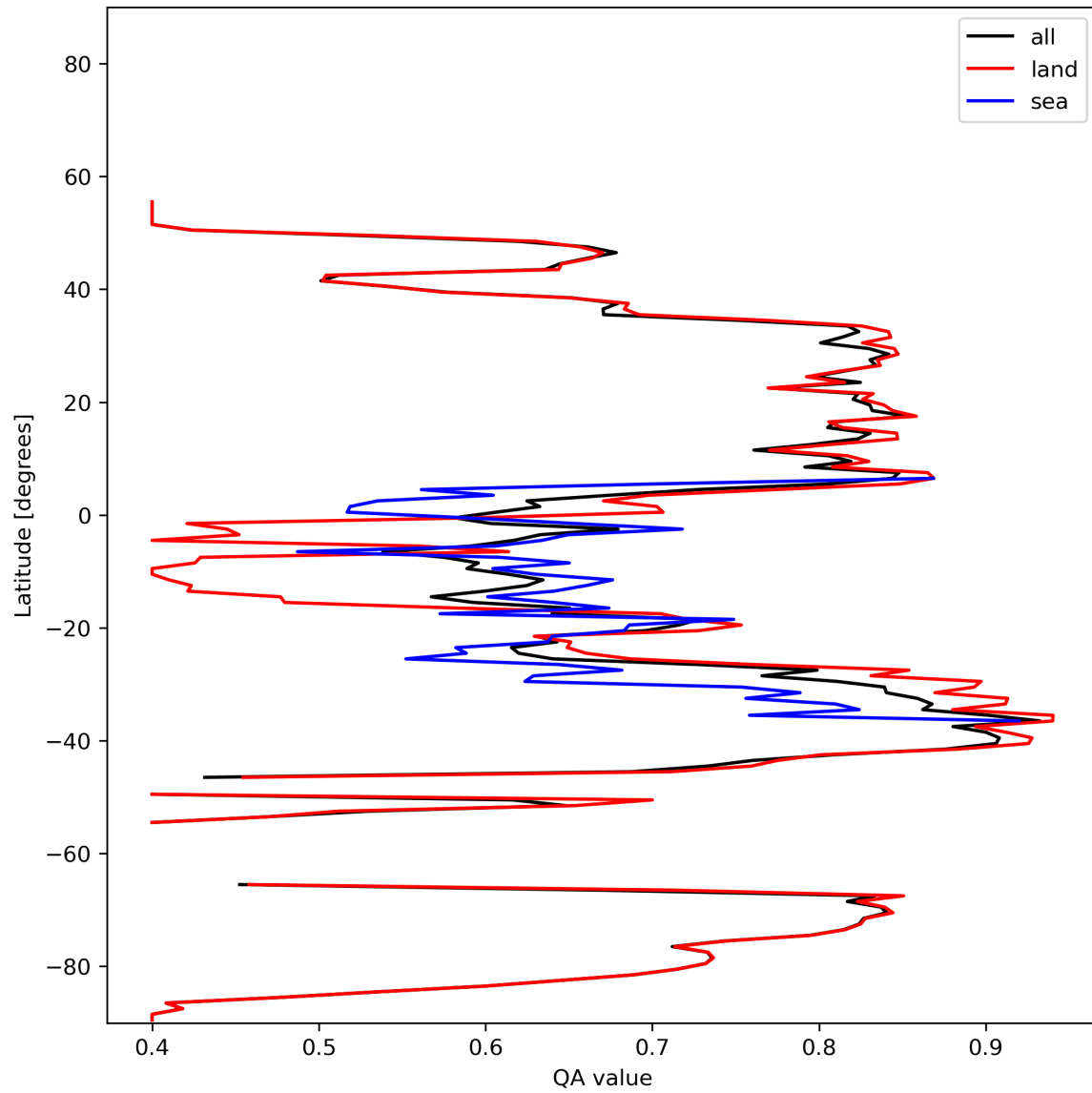
Figure 11: Zonal average of “QA value” for 2024-01-22 to 2024-01-24.
