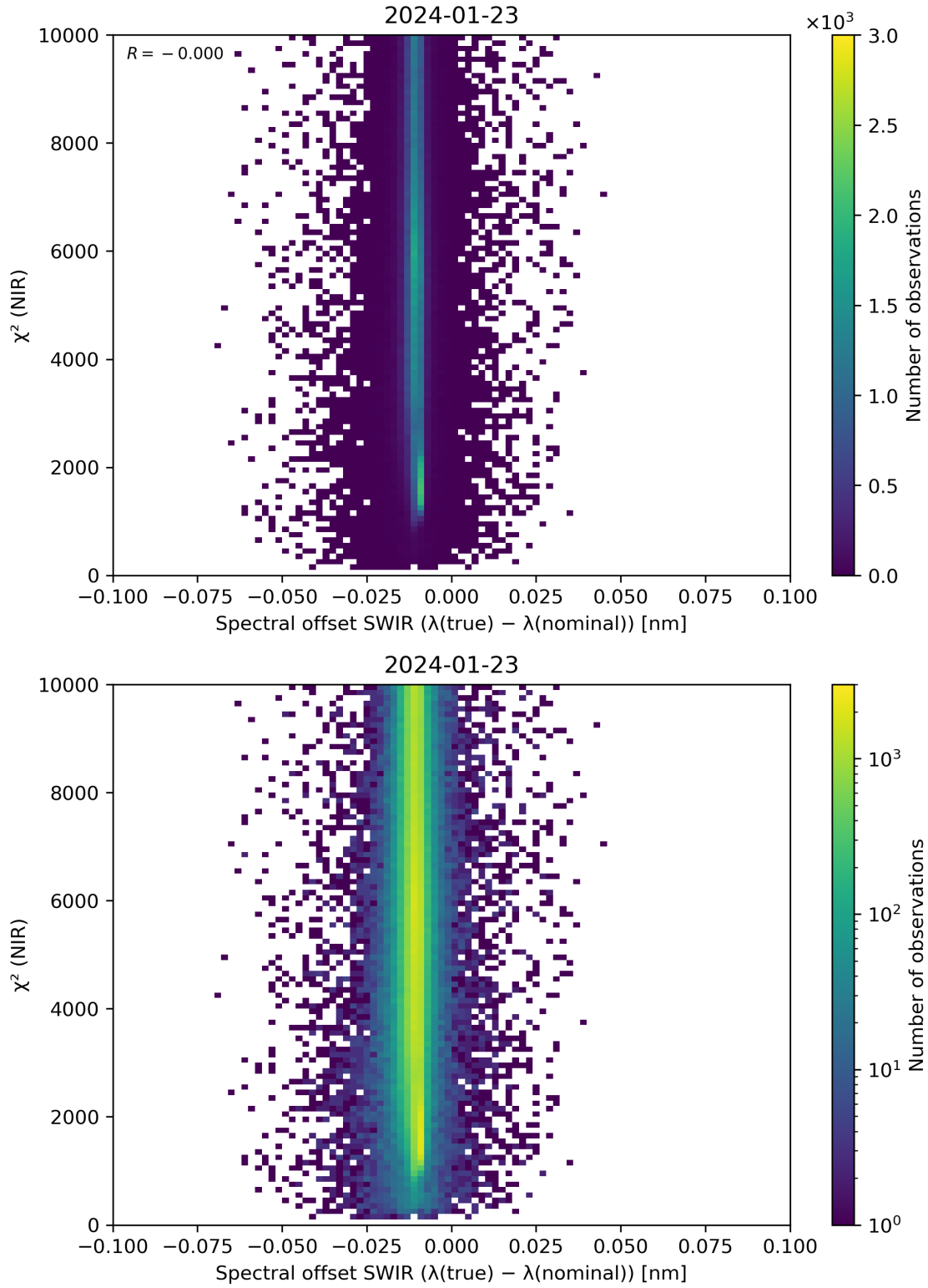
Figure 117: Scatter density plot of “Spectral offset SWIR ( \lambda(\text{true}) - \lambda(\text{nominal}) )” against “ \chi^2 (NIR)” for 2024-01-22 to 2024-01-24.
