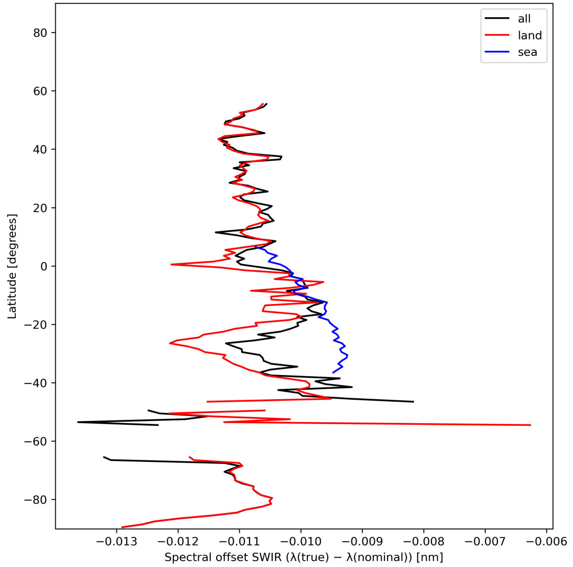
Figure 16: Zonal average of “Spectral offset SWIR ( \lambda(\text{true}) - \lambda(\text{nominal}) )” for 2024-01-22 to 2024-01-24.
