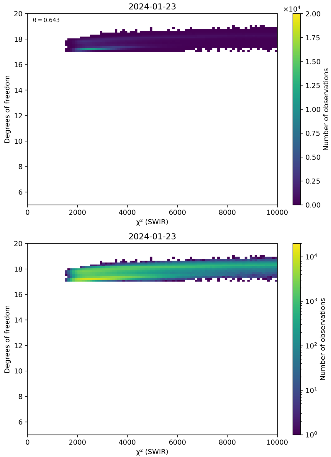
Figure 48: Scatter density plot of “ \chi^2 (SWIR)” against “Degrees of freedom” for 2024-01-22 to 2024-01-24.
