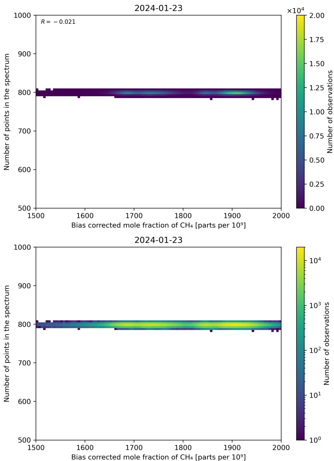
Figure 68: Scatter density plot of “Bias corrected mole fraction of CH 4 ” against “Number of points in the spectrum” for 2024-01-22 to 2024-01-24.
