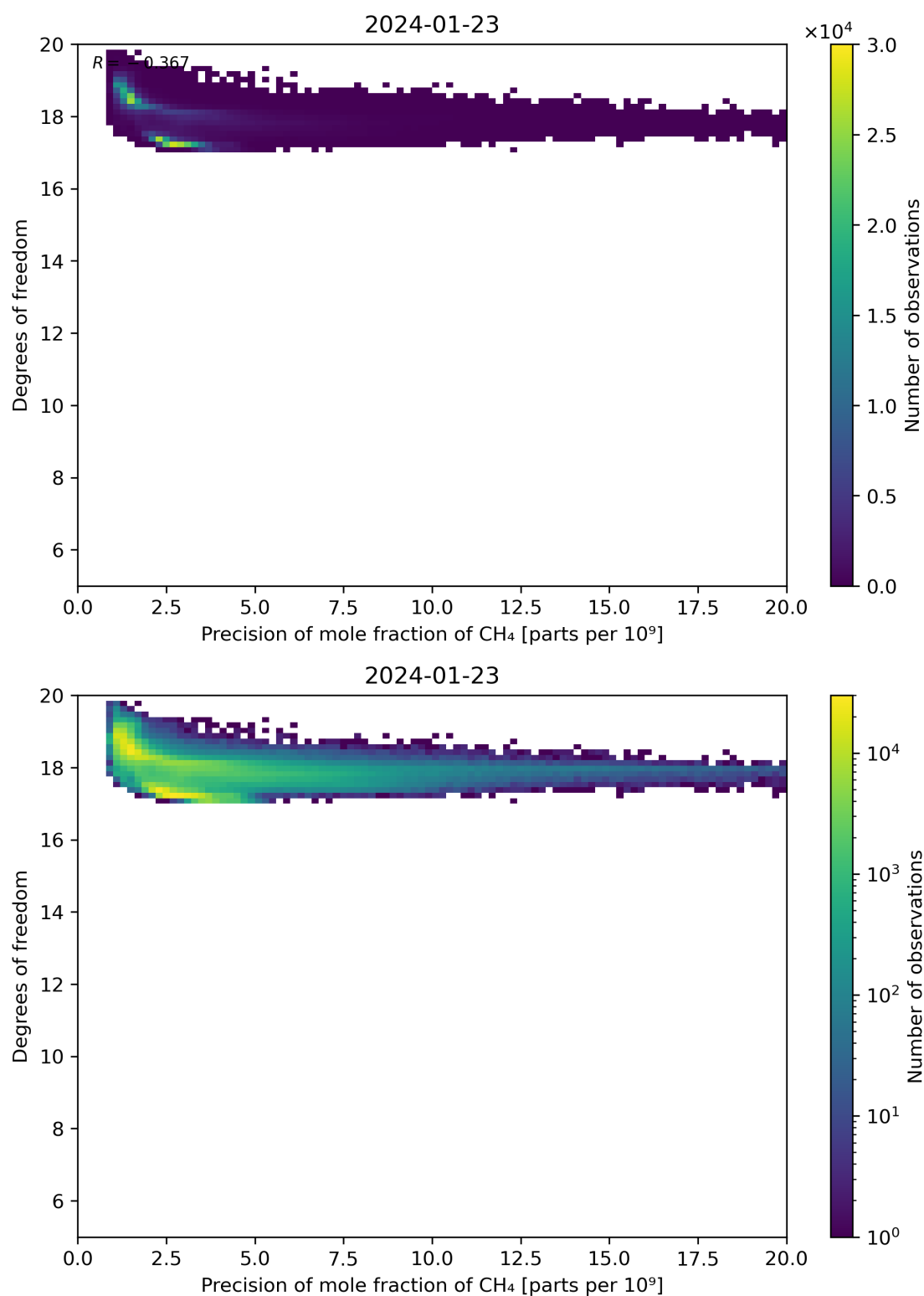
Figure 80: Scatter density plot of “Precision of mole fraction of CH 4 ” against “Degrees of freedom” for 2024-01-22 to 2024-01-24.
