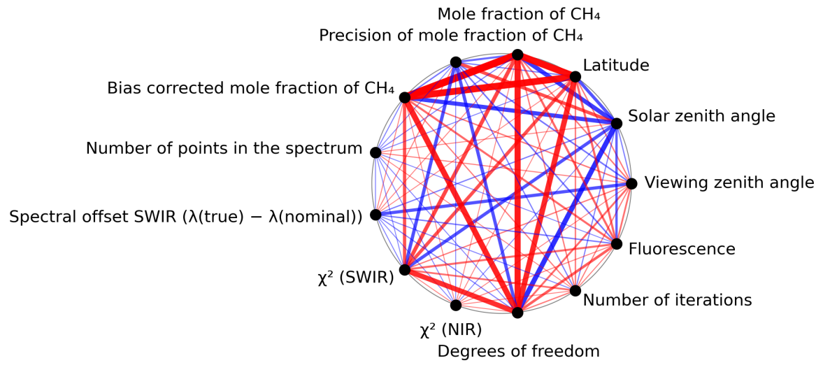
Figure 1: Map of correlation graph for 2024-01-22 to 2024-01-24.
