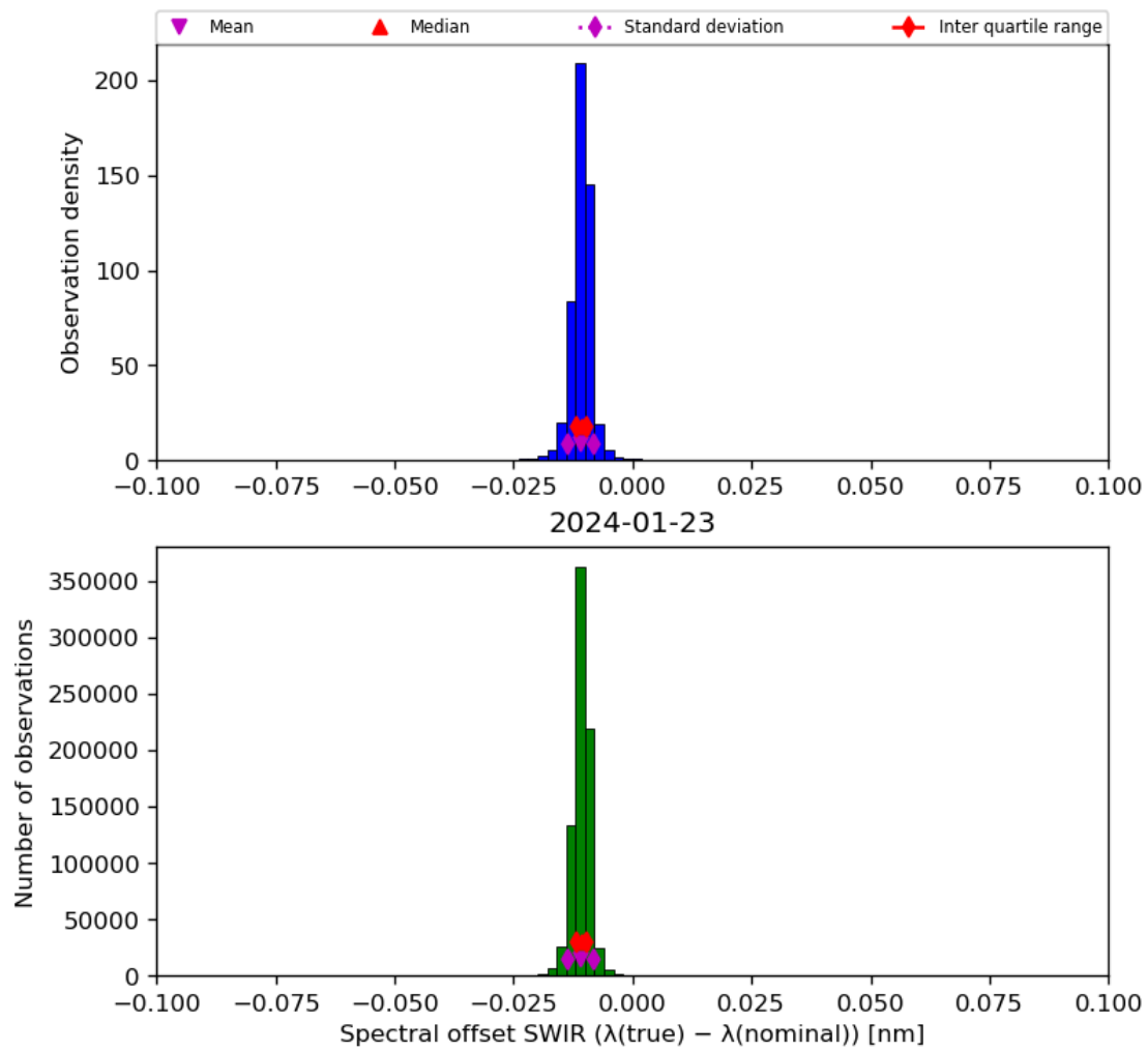
Figure 27: Histogram of “Spectral offset SWIR ( \lambda(\text{true}) - \lambda(\text{nominal}) )” for 2024-01-22 to 2024-01-24
