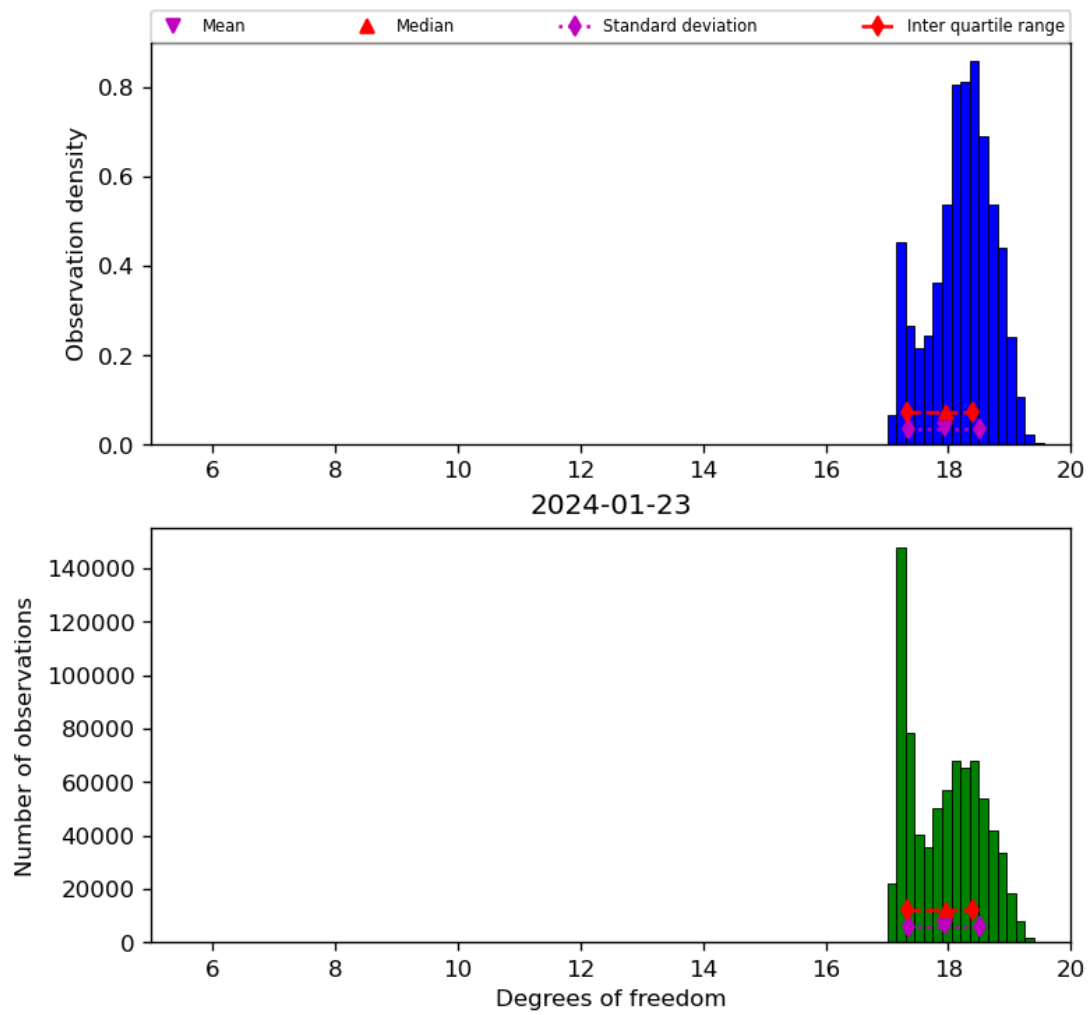
Figure 30: Histogram of “Degrees of freedom” for 2024-01-22 to 2024-01-24
