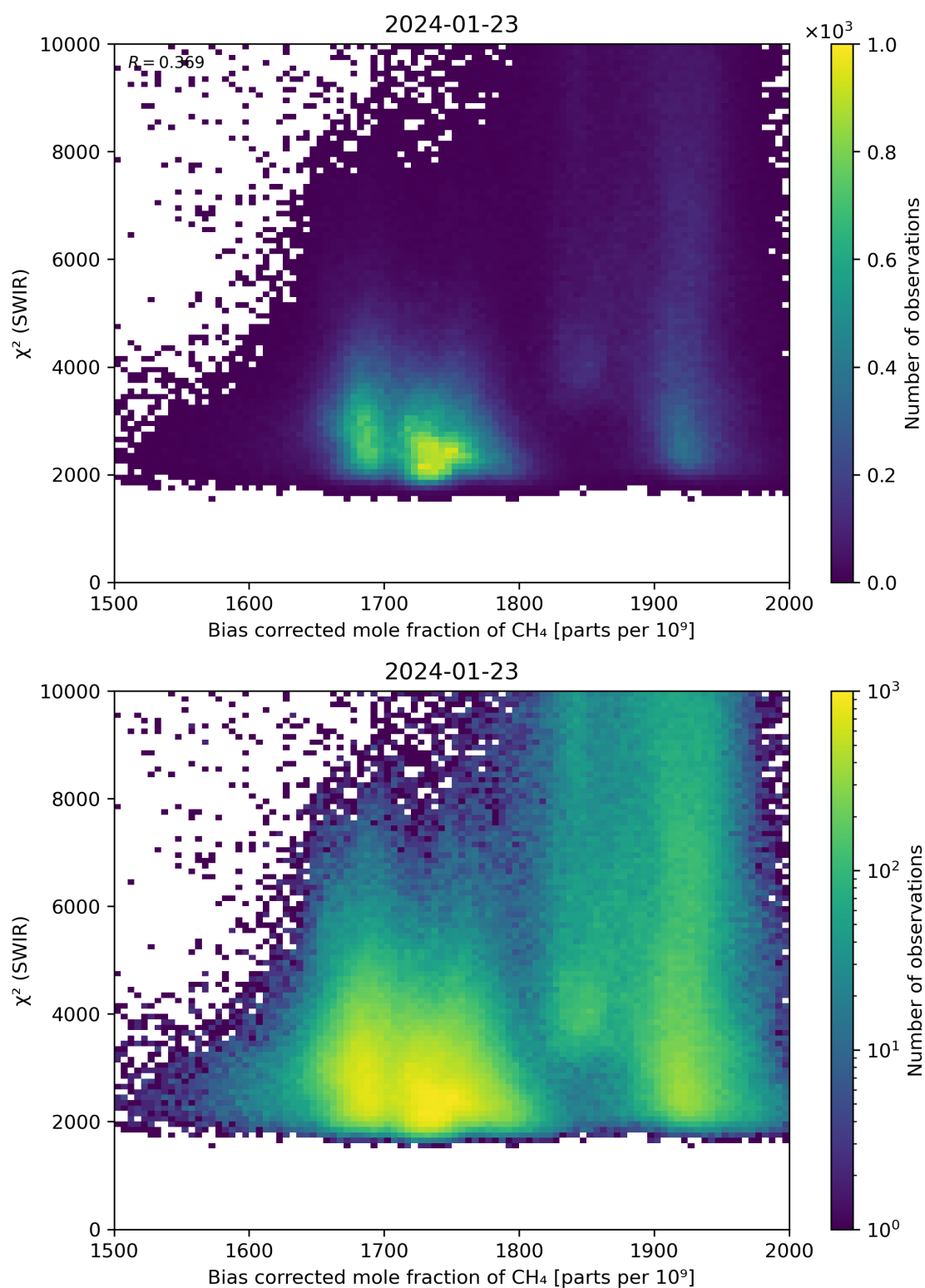
Figure 64: Scatter density plot of “Bias corrected mole fraction of \text{CH}_4 ” against “ \chi^2 (SWIR)” for 2024-01-22 to 2024-01-24.
