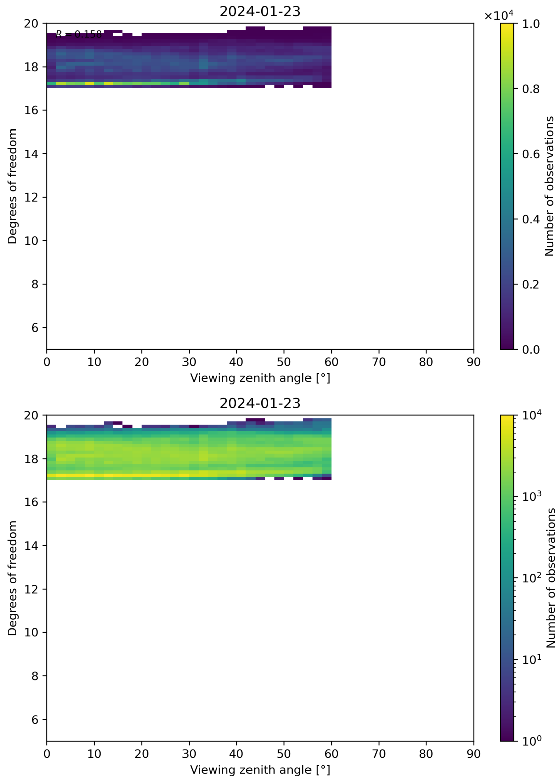
Figure 107: Scatter density plot of “Viewing zenith angle” against “Degrees of freedom” for 2024-01-22 to 2024-01-24.
