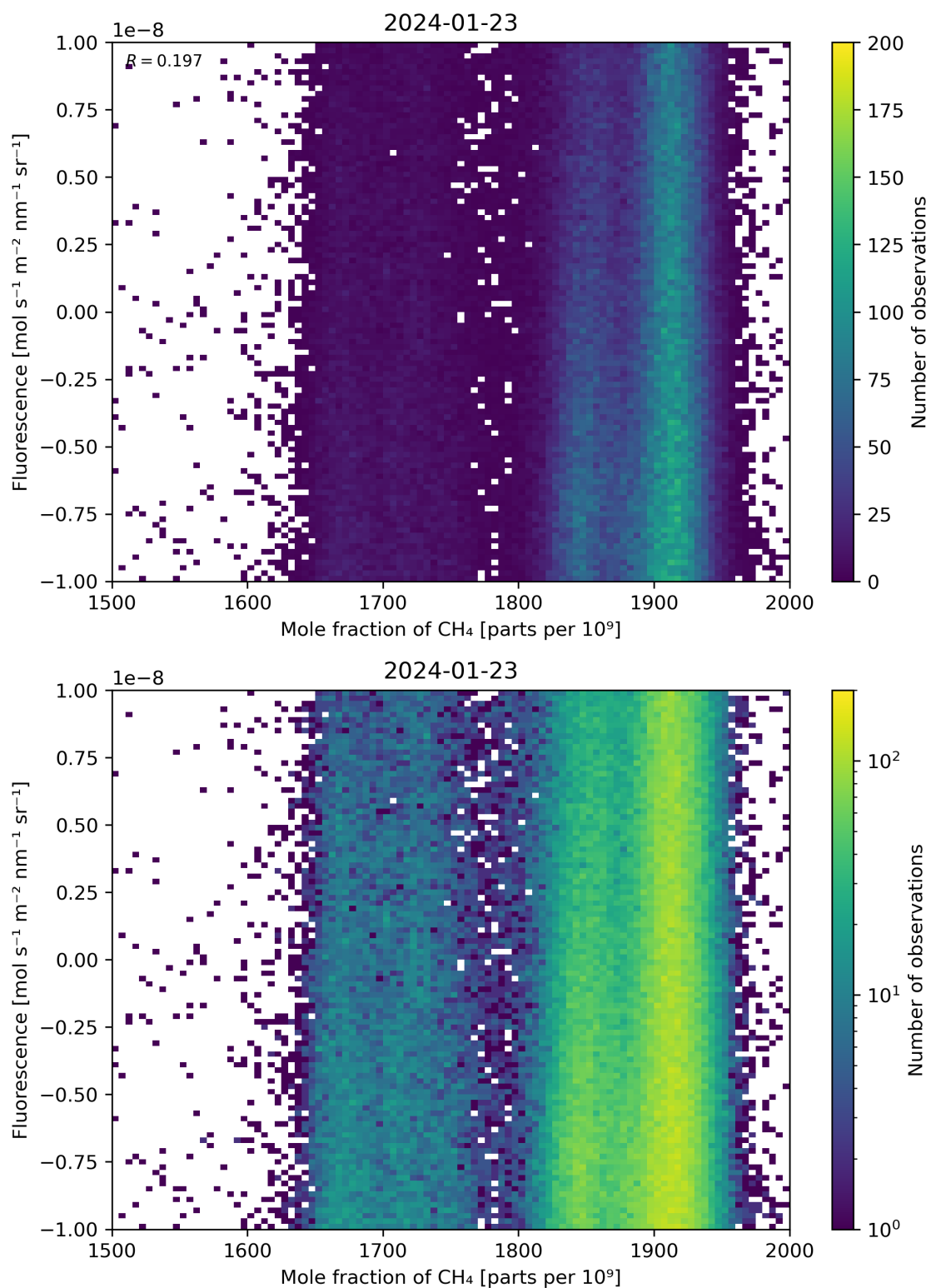
Figure 73: Scatter density plot of “Mole fraction of \text{CH}_4 ” against “Fluorescence” for 2024-01-22 to 2024-01-24.
