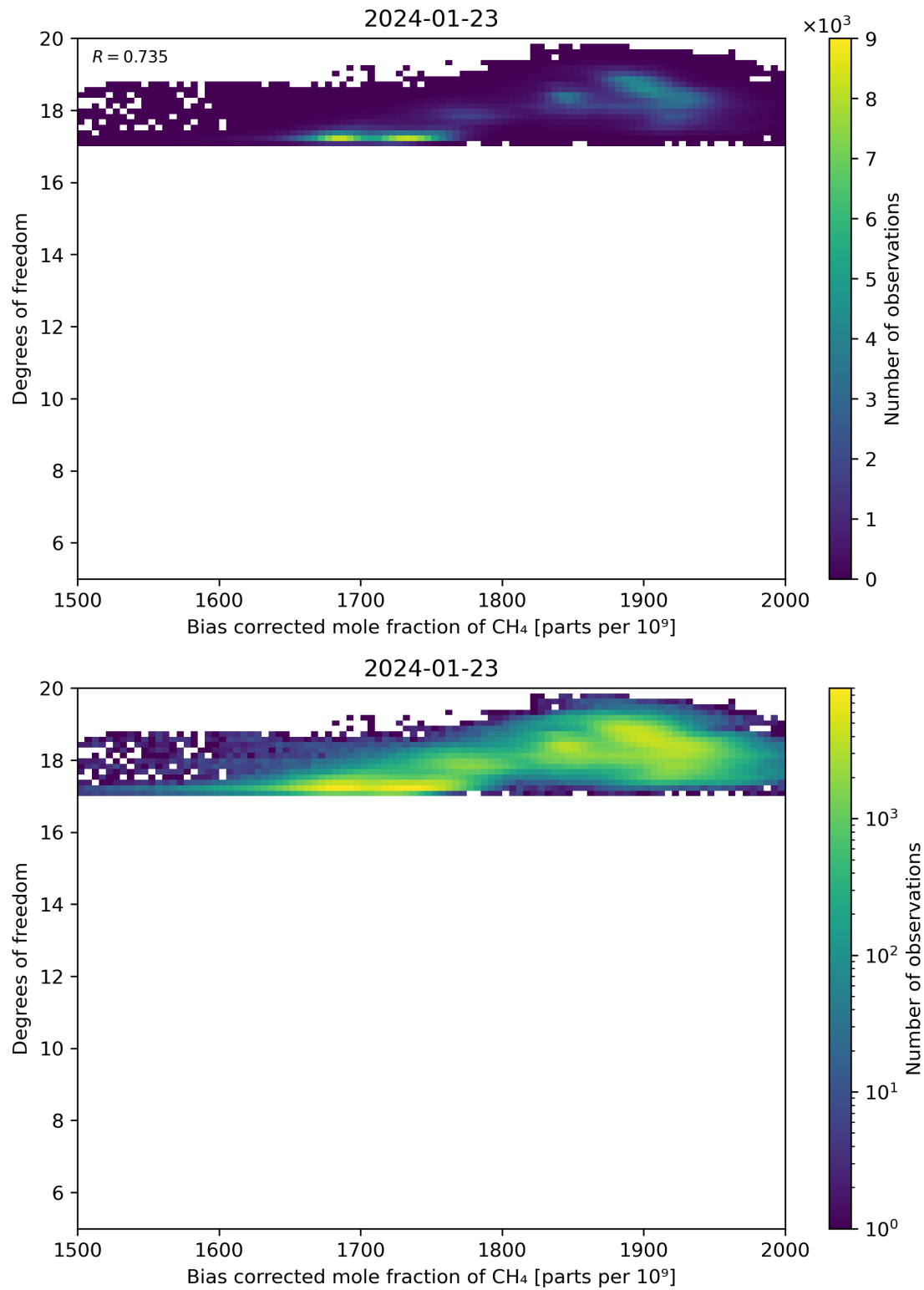
Figure 65: Scatter density plot of “Bias corrected mole fraction of CH 4 ” against “Degrees of freedom” for 2024-01-22 to 2024-01-24.
