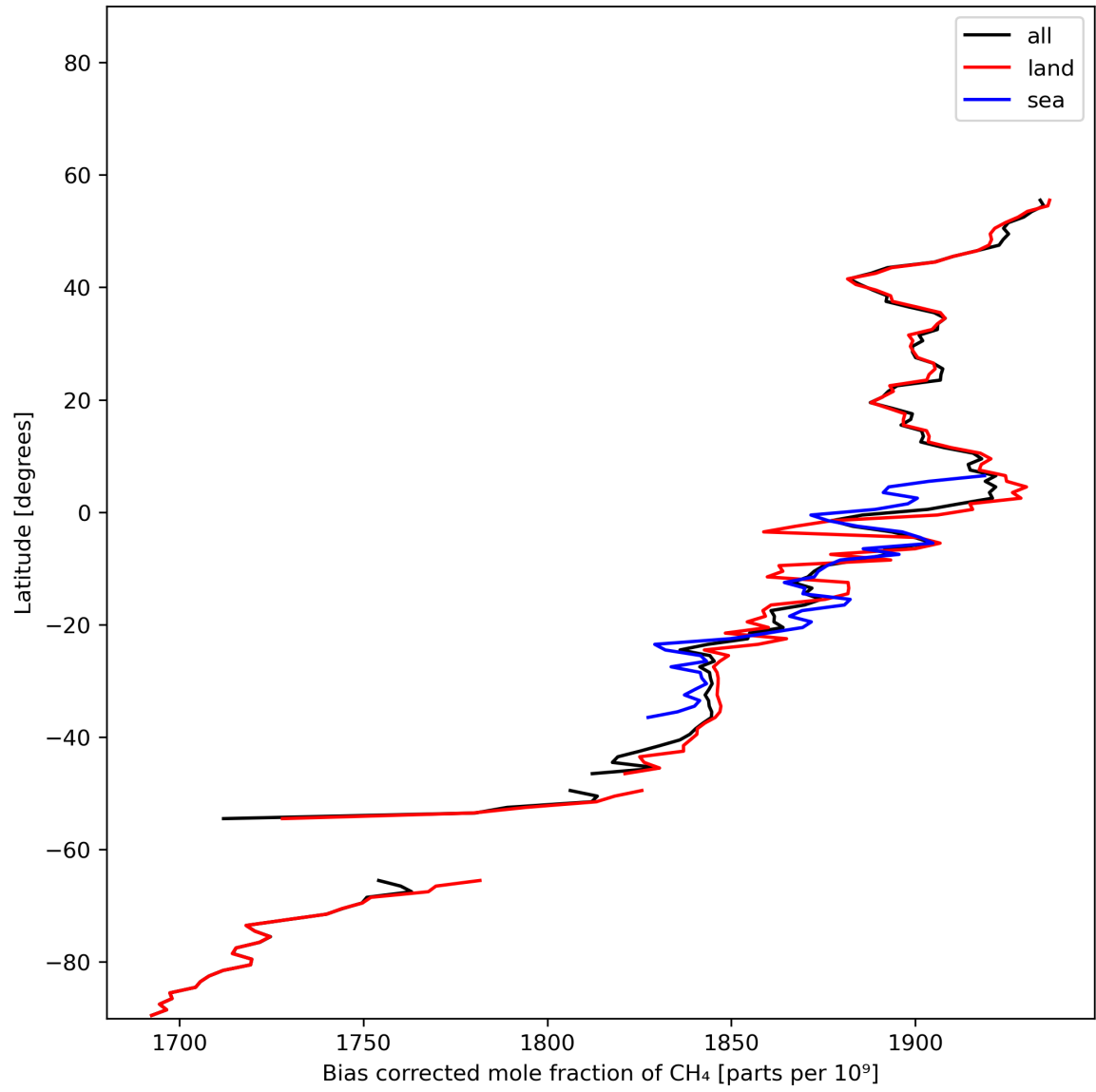
Figure 14: Zonal average of “Bias corrected mole fraction of \text{CH}_4 ” for 2024-01-22 to 2024-01-24.
