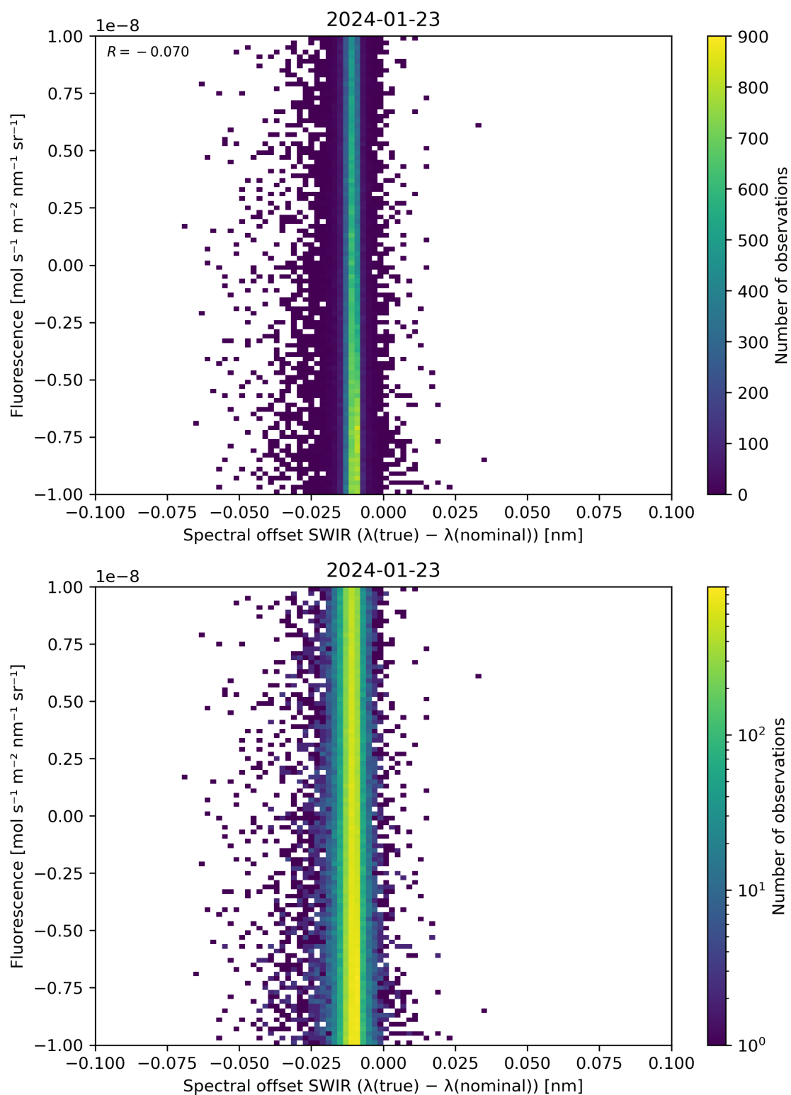
Figure 120: Scatter density plot of “Spectral offset SWIR ( \lambda(\text{true}) - \lambda(\text{nominal}) )” against “Fluorescence” for 2024-01-22 to 2024-01-24.
