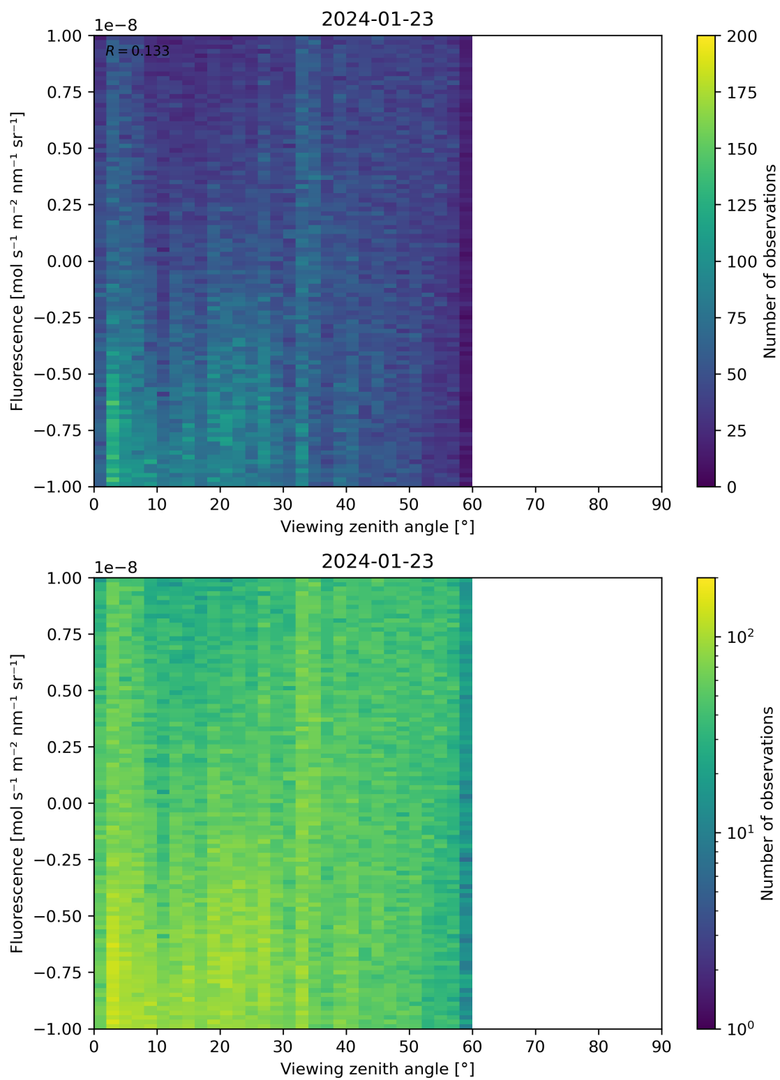
Figure 108: Scatter density plot of “Viewing zenith angle” against “Fluorescence” for 2024-01-22 to 2024-01-24.
