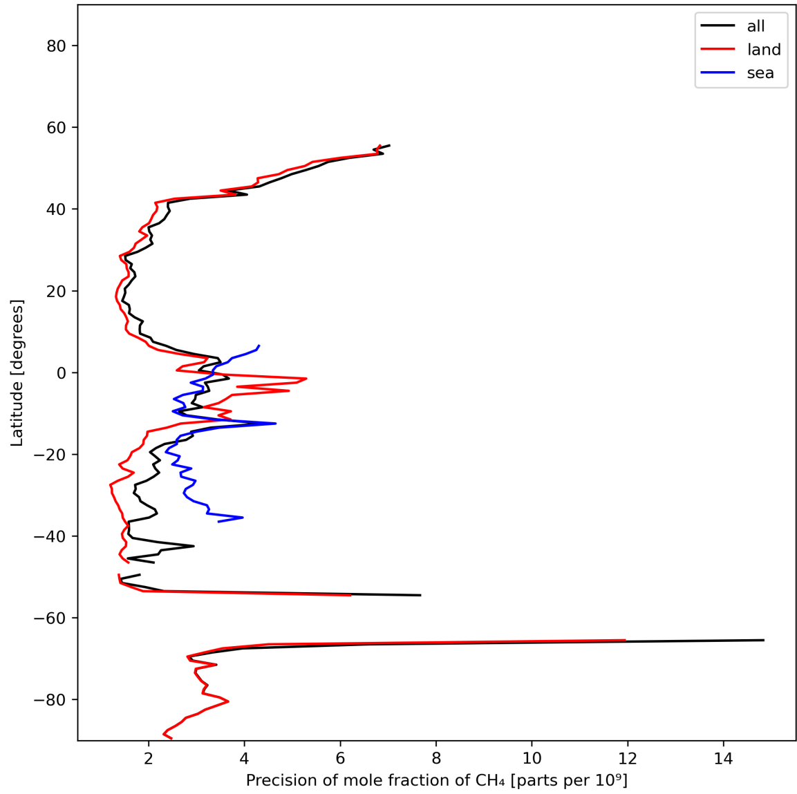
Figure 13: Zonal average of “Precision of mole fraction of CH 4 ” for 2024-01-22 to 2024-01-24.
