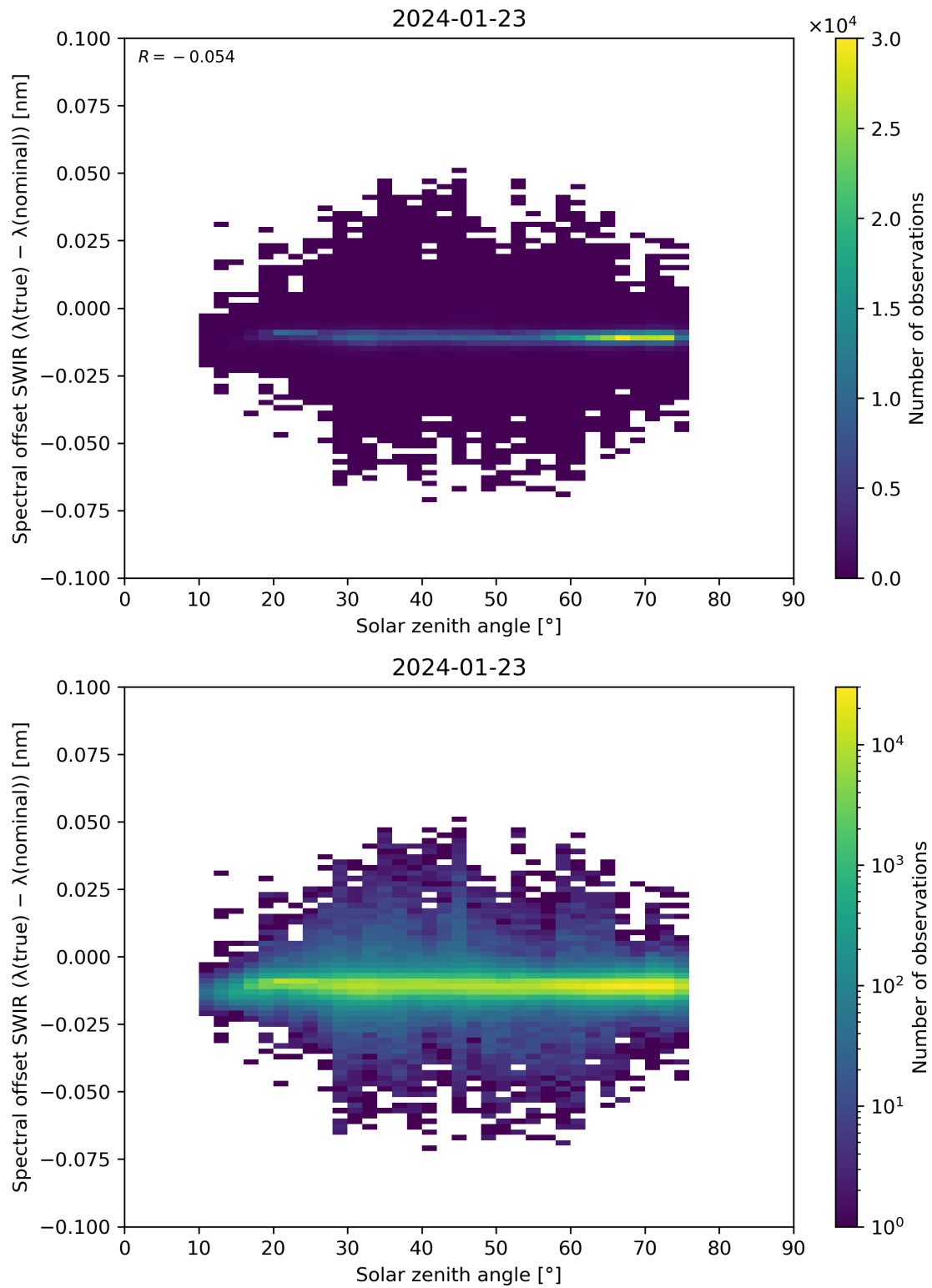
Figure 104: Scatter density plot of “Solar zenith angle” against “Spectral offset SWIR ( \lambda(\text{true}) - \lambda(\text{nominal}) )” for 2024-01-22 to 2024-01-24.
