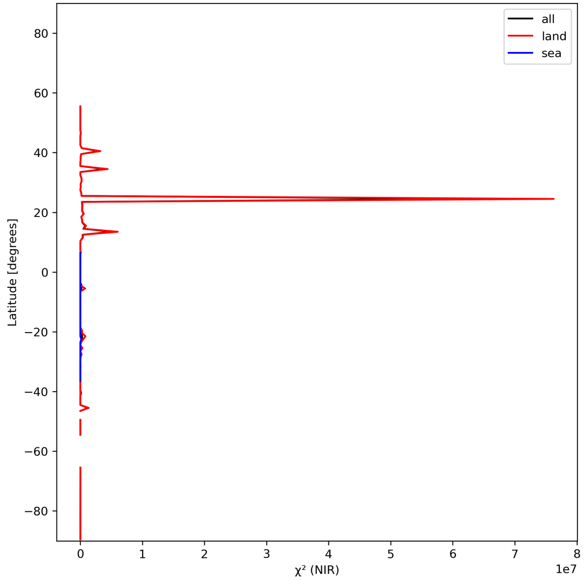
Figure 18: Zonal average of “ \chi^2 (NIR)” for 2024-01-22 to 2024-01-24.
