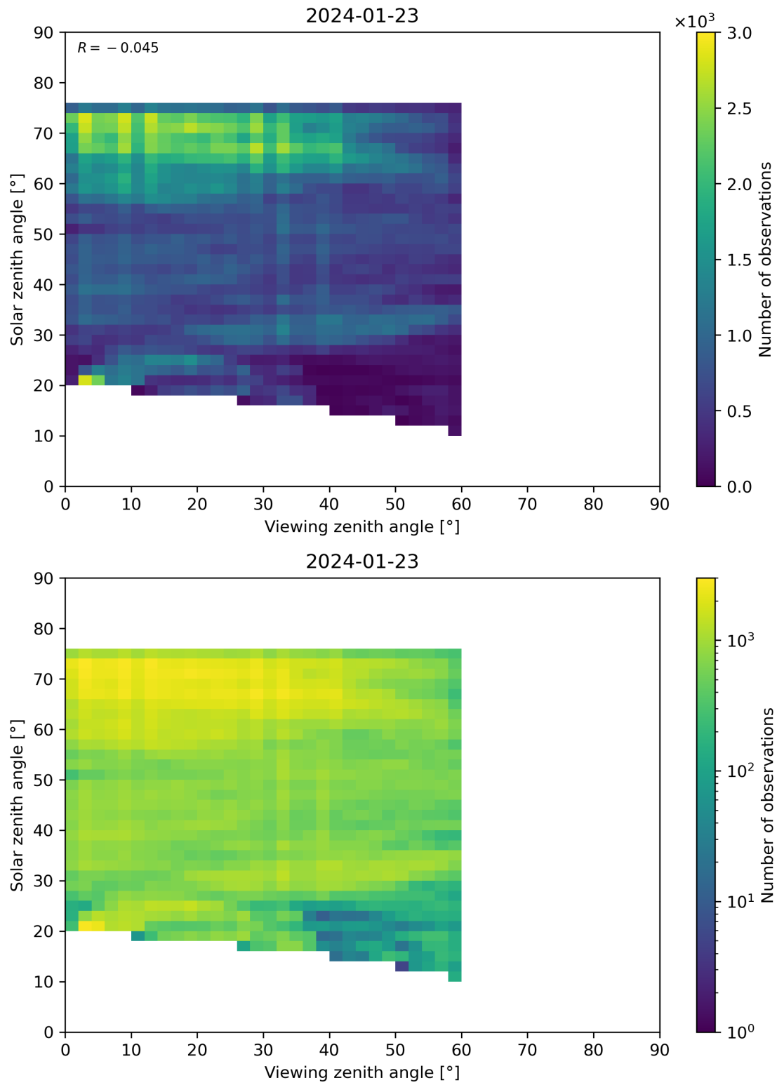
Figure 115: Scatter density plot of “Viewing zenith angle” against “Solar zenith angle” for 2024-01-22 to 2024-01-24.
