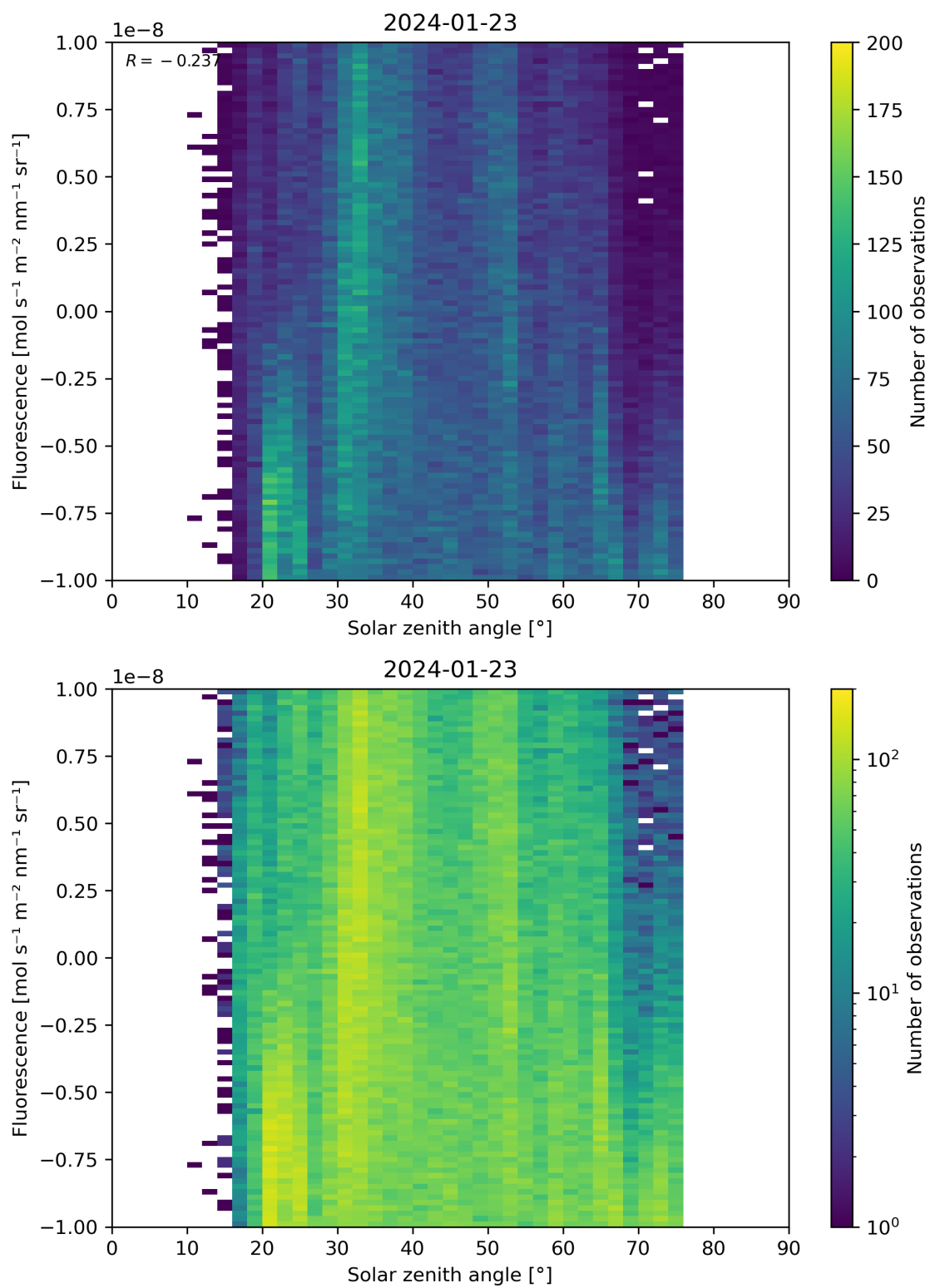
Figure 97: Scatter density plot of “Solar zenith angle” against “Fluorescence” for 2024-01-22 to 2024-01-24.
