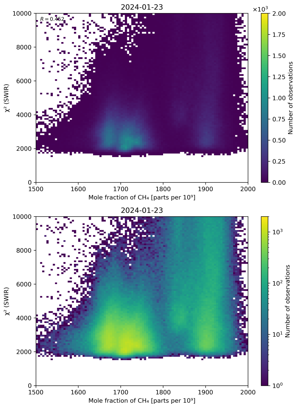
Figure 71: Scatter density plot of “Mole fraction of \text{CH}_4 ” against “ \chi^2 (SWIR)” for 2024-01-22 to 2024-01-24.
