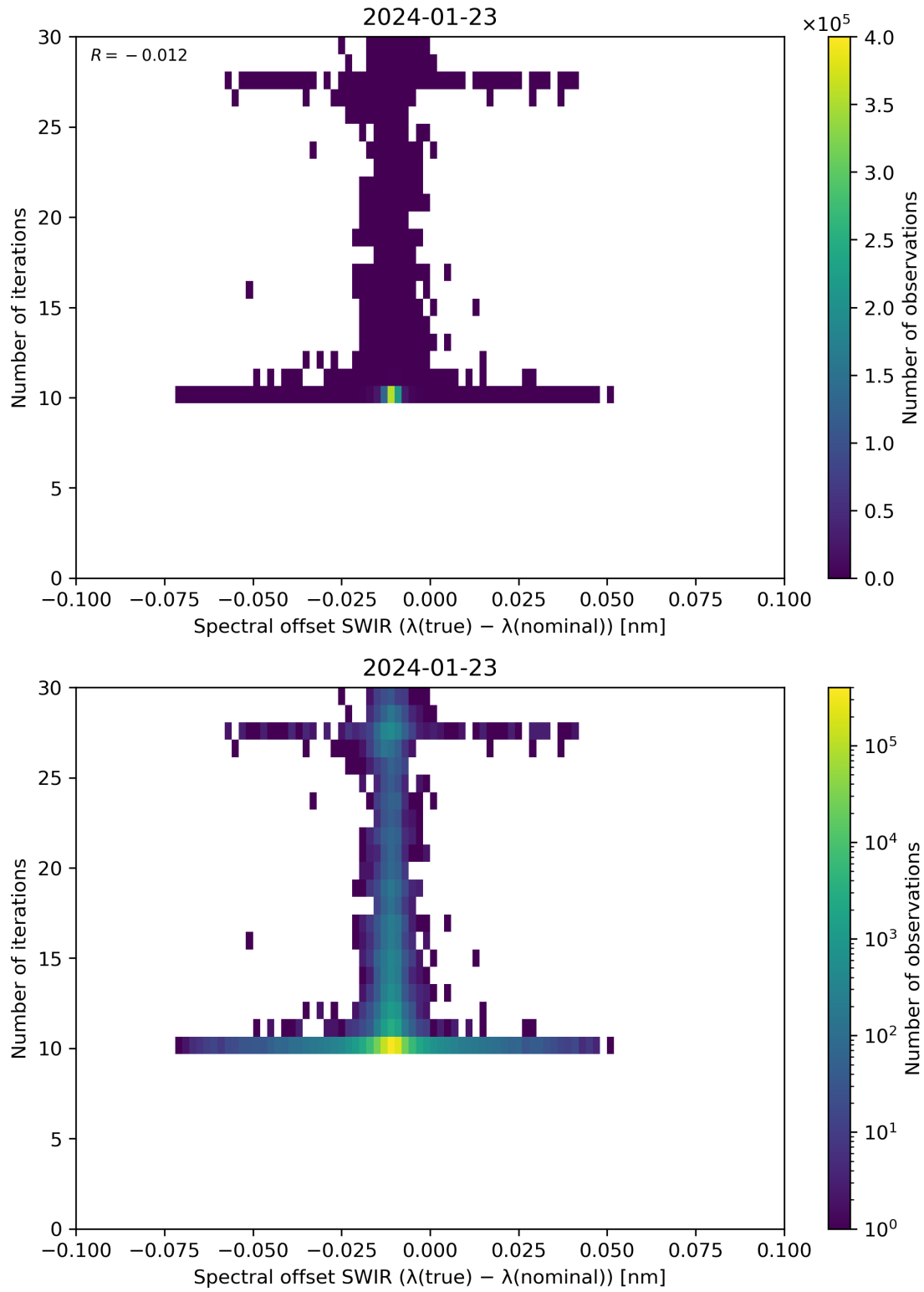
Figure 121: Scatter density plot of “Spectral offset SWIR ( \lambda(\text{true}) - \lambda(\text{nominal}) )” against “Number of iterations” for 2024-01-22 to 2024-01-24.
