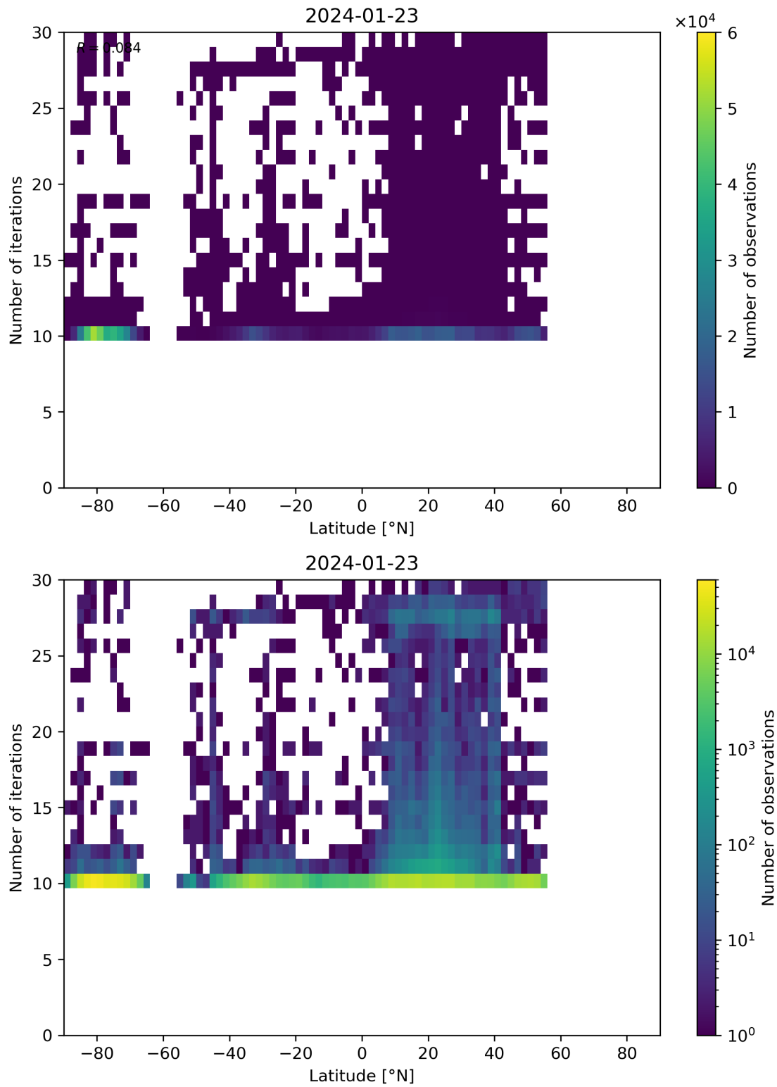
Figure 60: Scatter density plot of “Latitude” against “Number of iterations” for 2024-01-22 to 2024-01-24.
