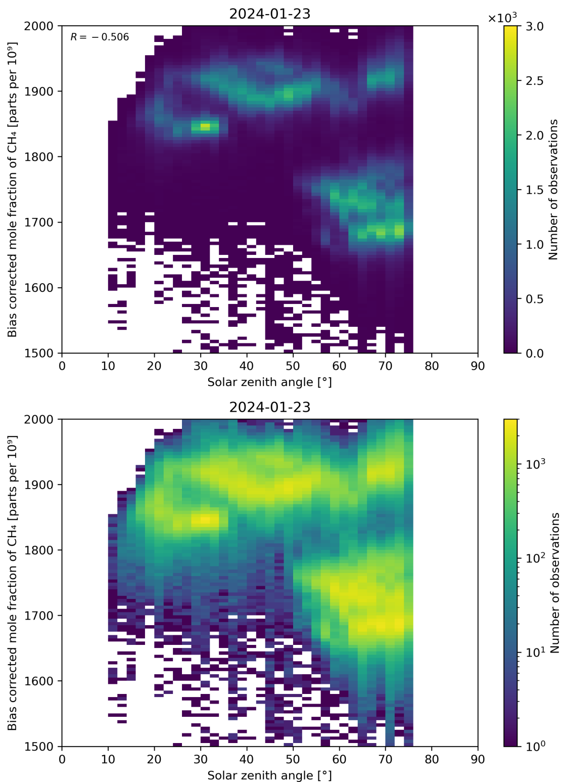
Figure 100: Scatter density plot of “Solar zenith angle” against “Bias corrected mole fraction of CH 4 ” for 2024-01-22 to 2024-01-24.
