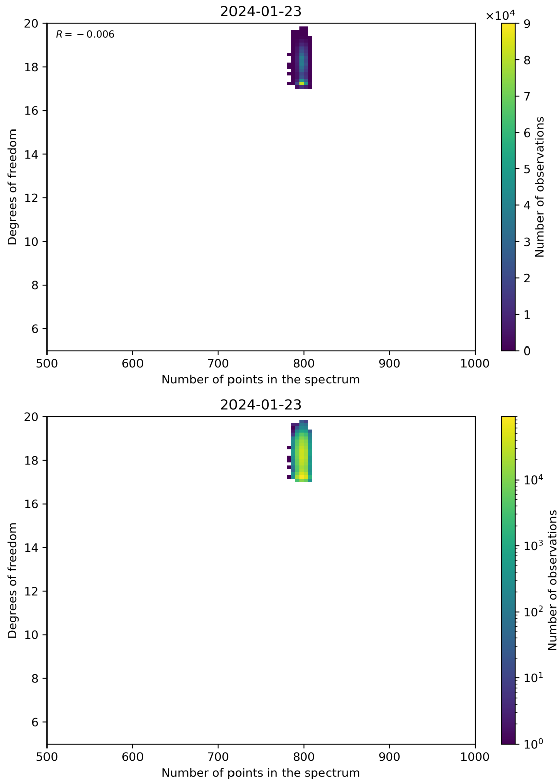
Figure 90: Scatter density plot of “Number of points in the spectrum” against “Degrees of freedom” for 2024-01-22 to 2024-01-24.
