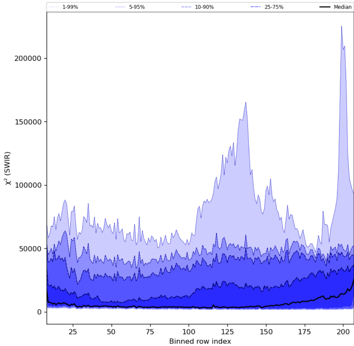
Figure 39: Along track statistics of “ \chi^2 (SWIR)” for 2024-01-22 to 2024-01-24
