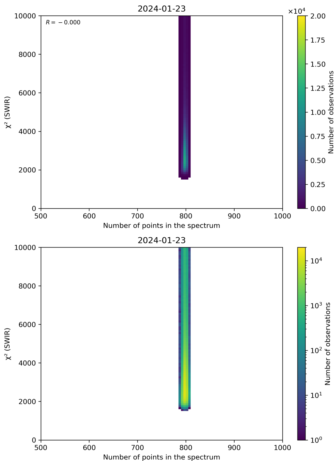
Figure 89: Scatter density plot of “Number of points in the spectrum” against “ \chi^2 (SWIR)” for 2024-01-22 to 2024-01-24.
