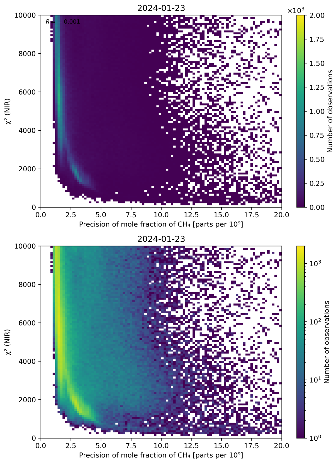
Figure 78: Scatter density plot of “Precision of mole fraction of CH 4 ” against “ \chi^2 (NIR)” for 2024-01-22 to 2024-01-24.
