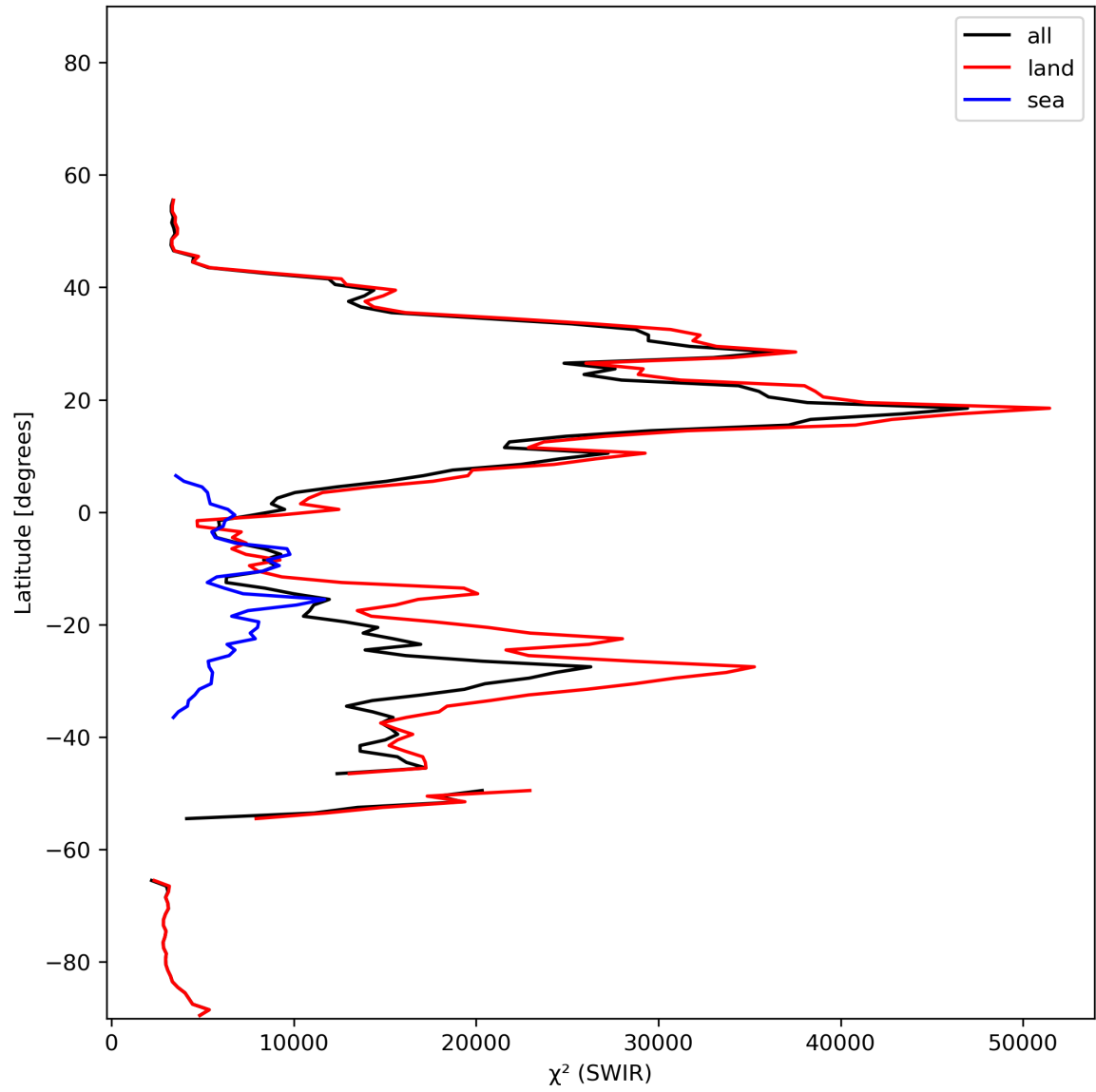
Figure 17: Zonal average of “ \chi^2 (SWIR)” for 2024-01-22 to 2024-01-24.
