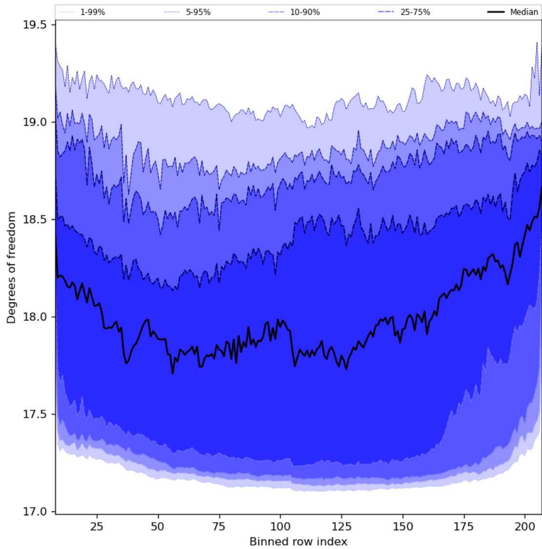
Figure 41: Along track statistics of “Degrees of freedom” for 2024-01-22 to 2024-01-24
