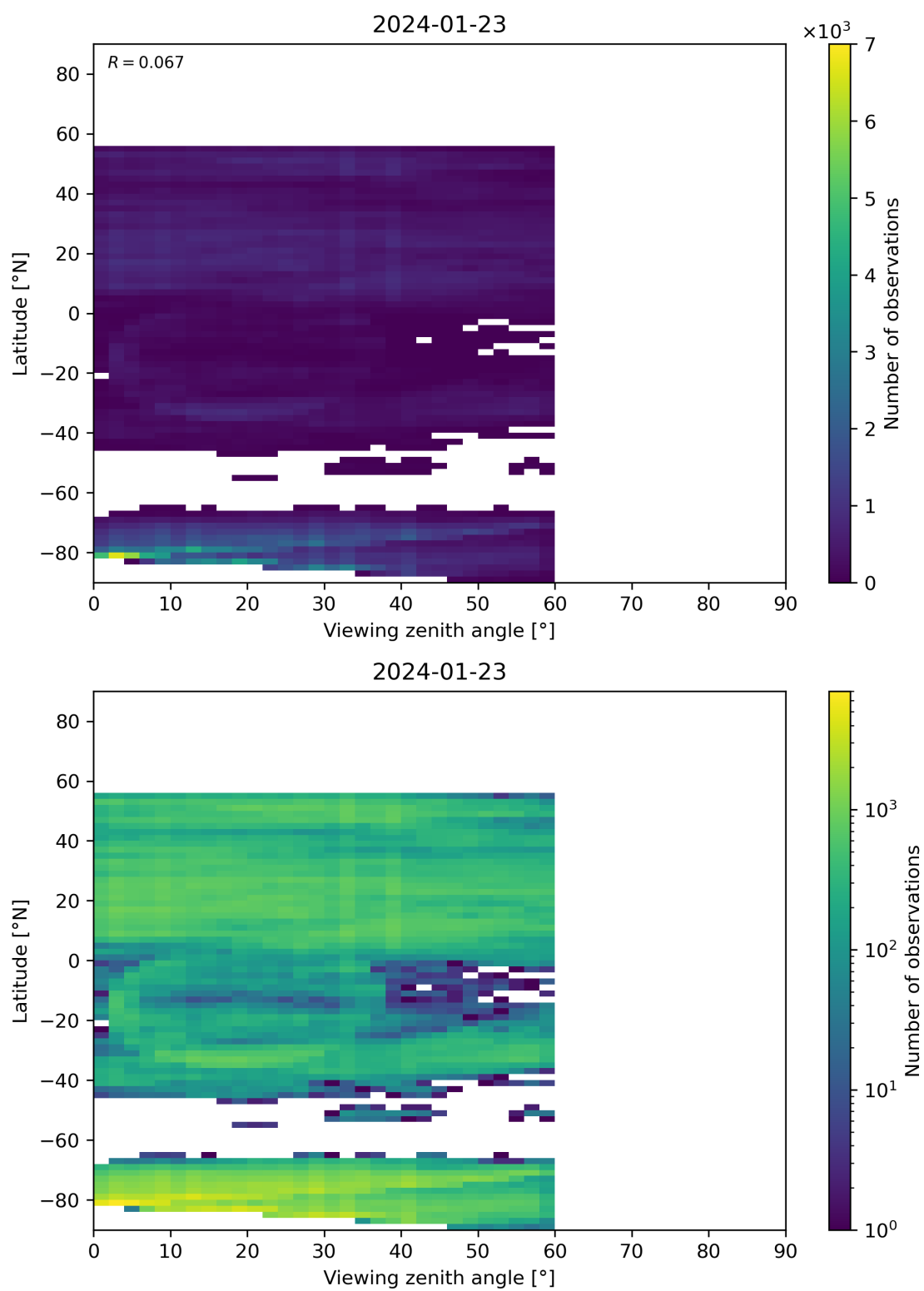
Figure 109: Scatter density plot of “Viewing zenith angle” against “Latitude” for 2024-01-22 to 2024-01-24.
