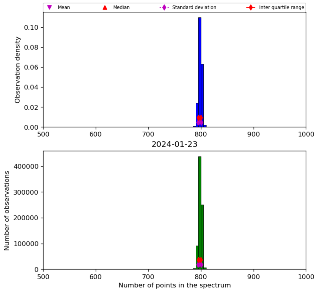
Figure 26: Histogram of “Number of points in the spectrum” for 2024-01-22 to 2024-01-24
