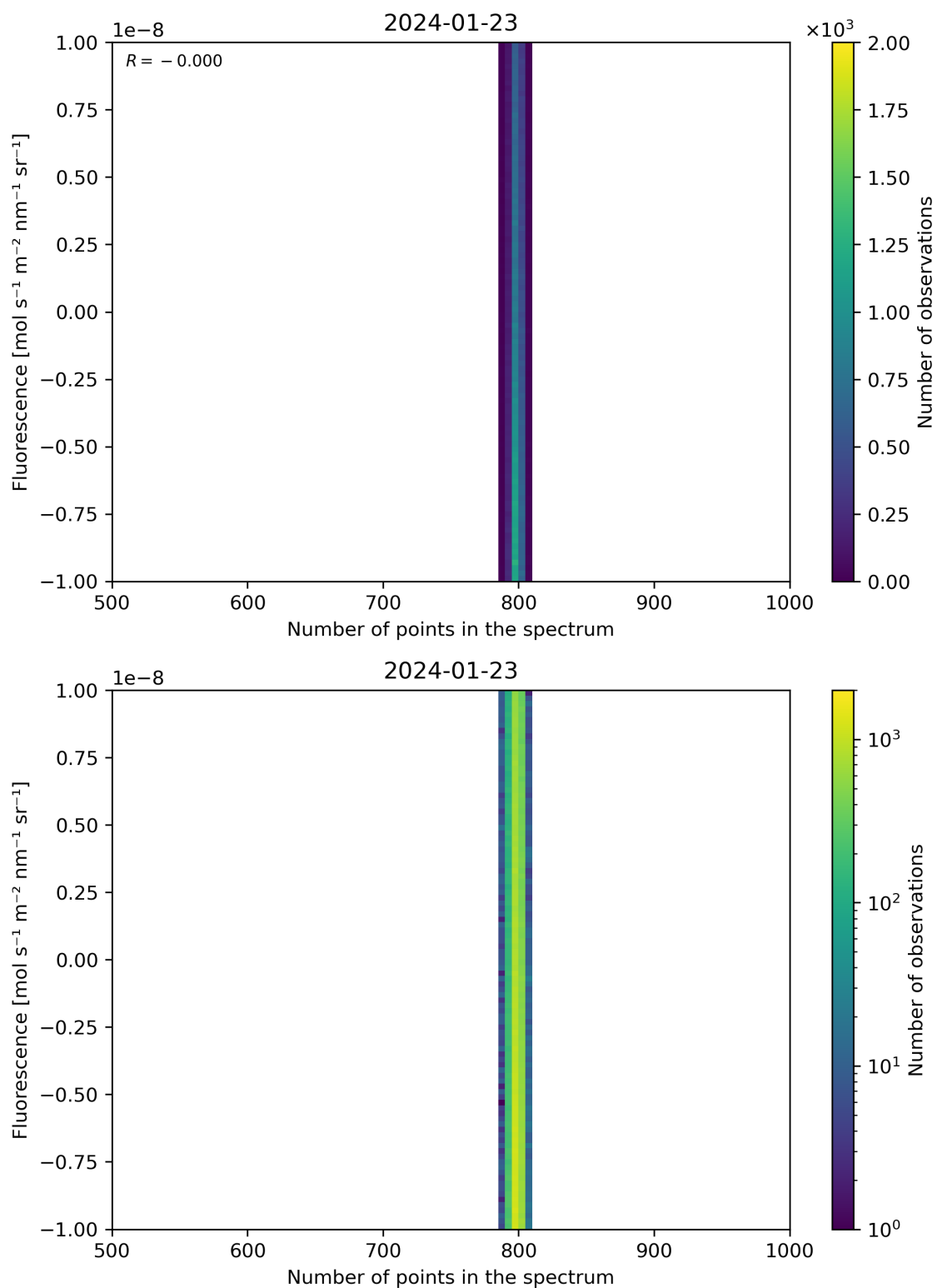
Figure 91: Scatter density plot of “Number of points in the spectrum” against “Fluorescence” for 2024-01-22 to 2024-01-24.
