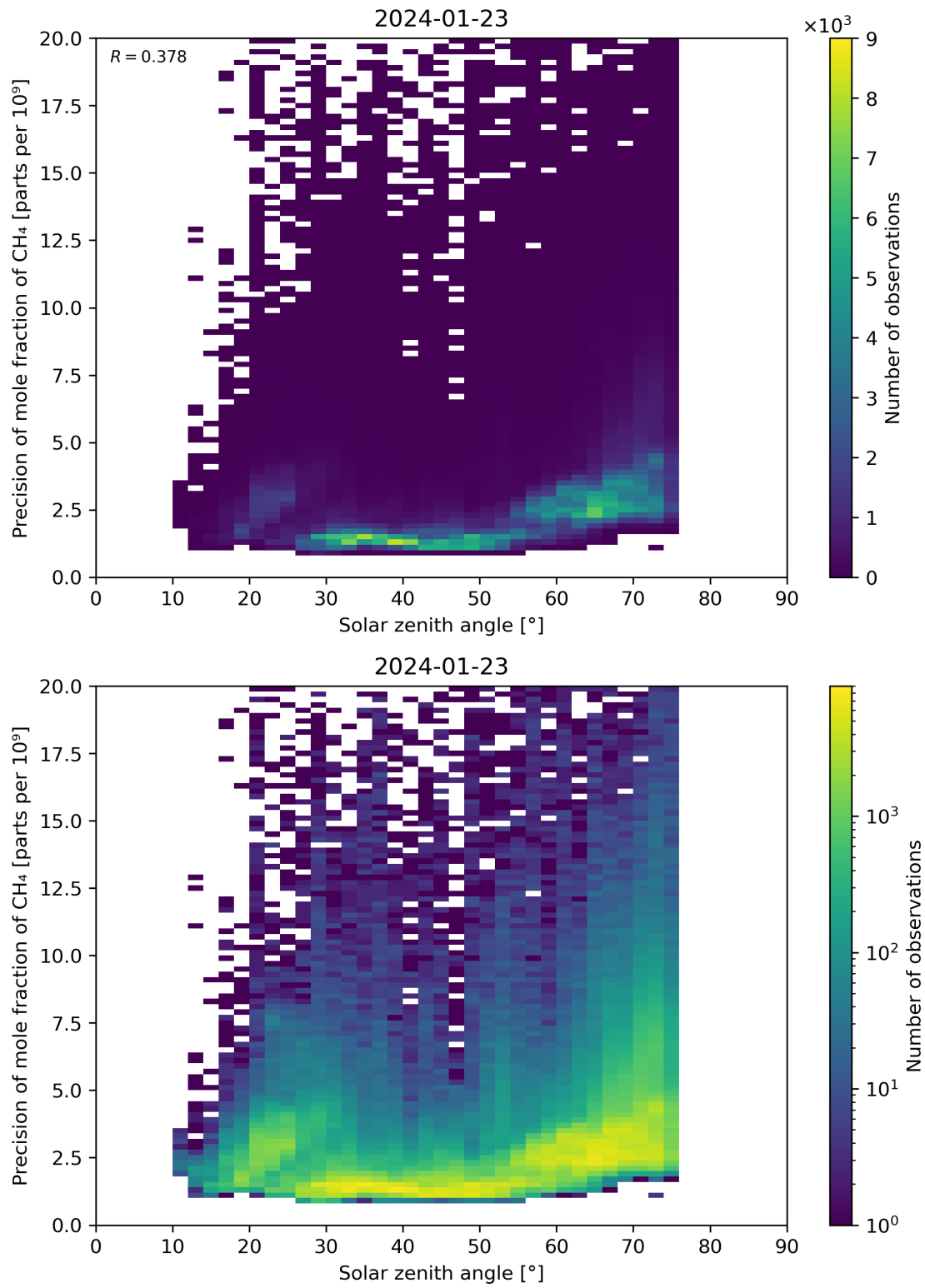
Figure 101: Scatter density plot of “Solar zenith angle” against “Precision of mole fraction of \text{CH}_4 ” for 2024-01-22 to 2024-01-24.
