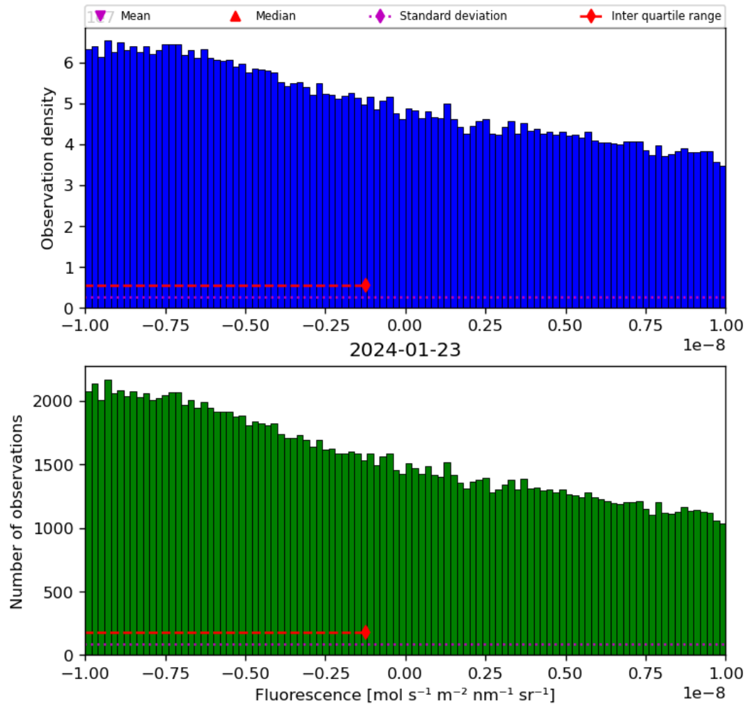
Figure 32: Histogram of “Fluorescence” for 2024-01-22 to 2024-01-24
