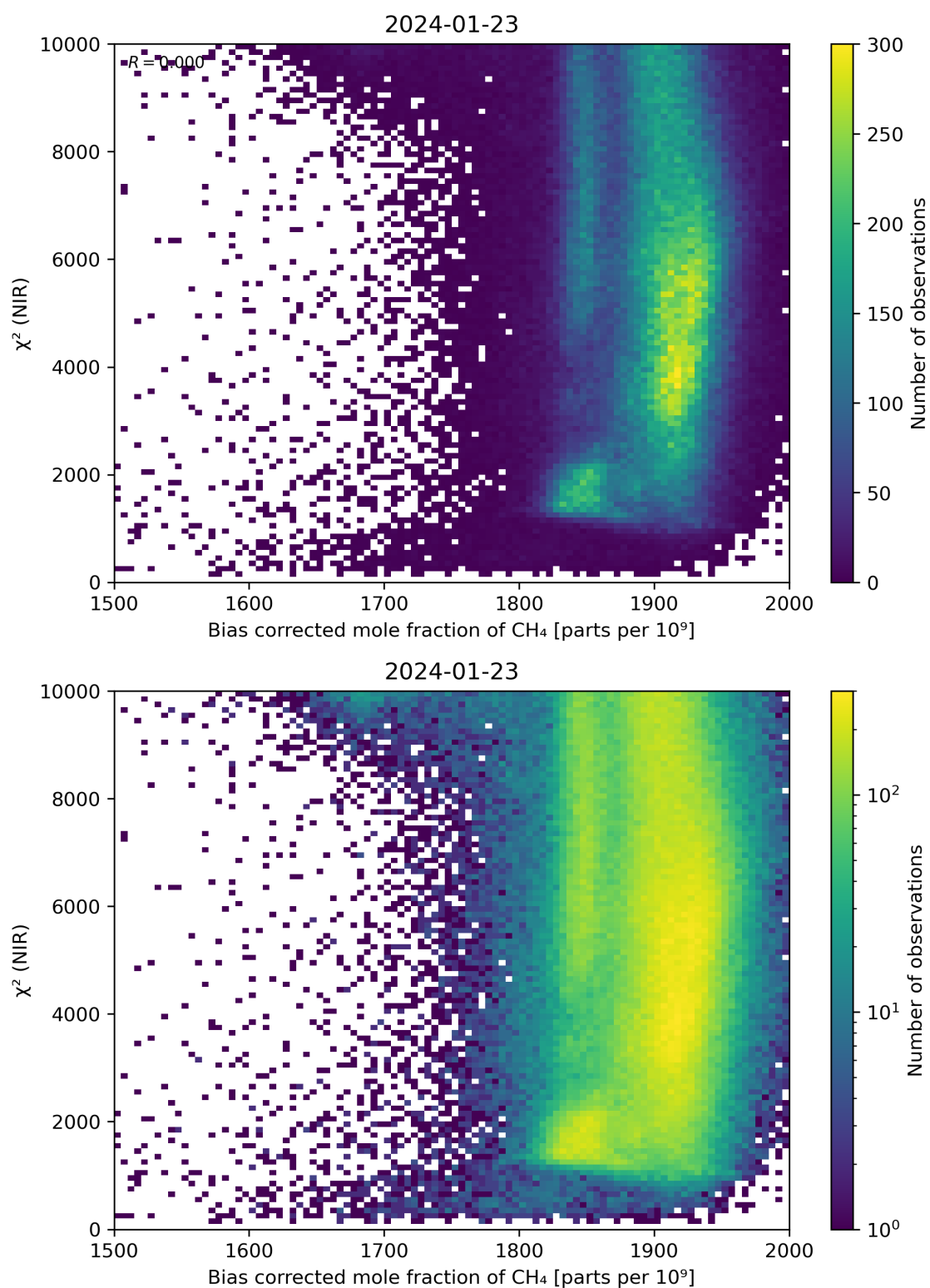
Figure 63: Scatter density plot of “Bias corrected mole fraction of CH 4 ” against “ \chi^2 (NIR)” for 2024-01-22 to 2024-01-24.
