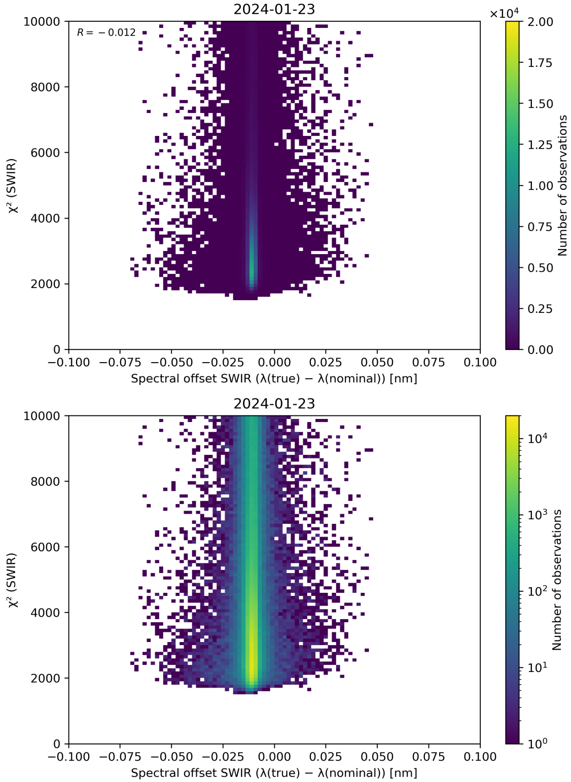
Figure 118: Scatter density plot of “Spectral offset SWIR ( \lambda(\text{true}) - \lambda(\text{nominal}) )” against “ \chi^2 (SWIR)” for 2024-01-22 to 2024-01-24.
