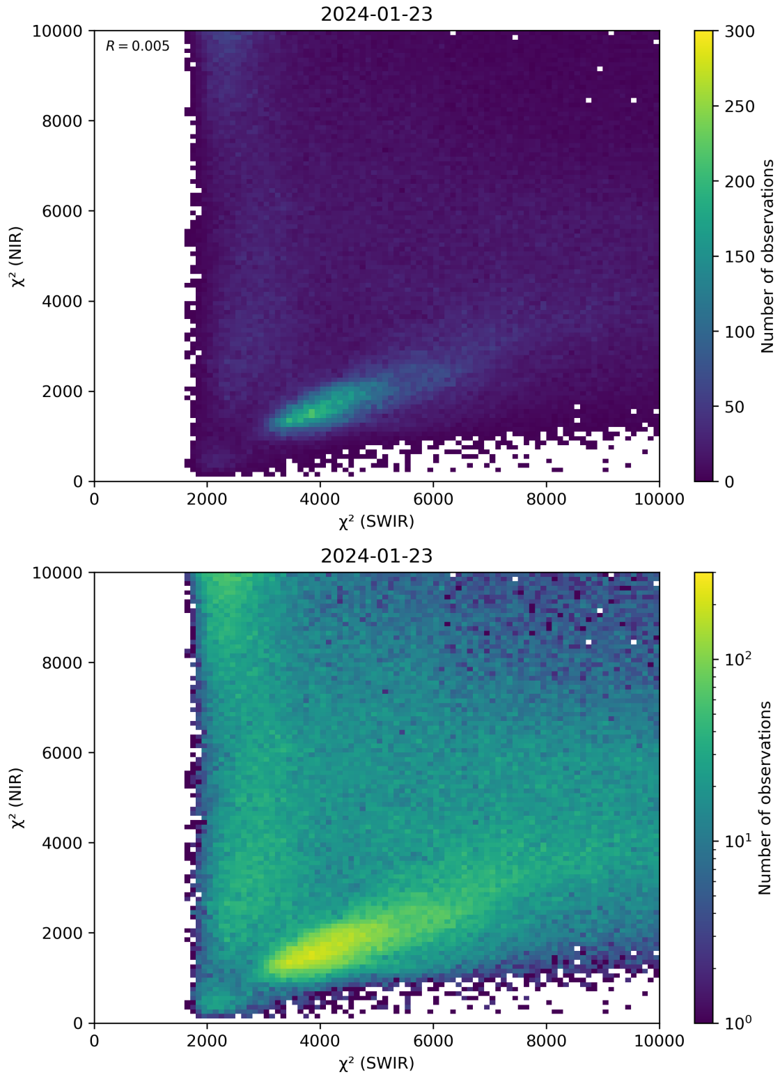
Figure 47: Scatter density plot of “ \chi^2 (SWIR)” against “ \chi^2 (NIR)” for 2024-01-22 to 2024-01-24.
