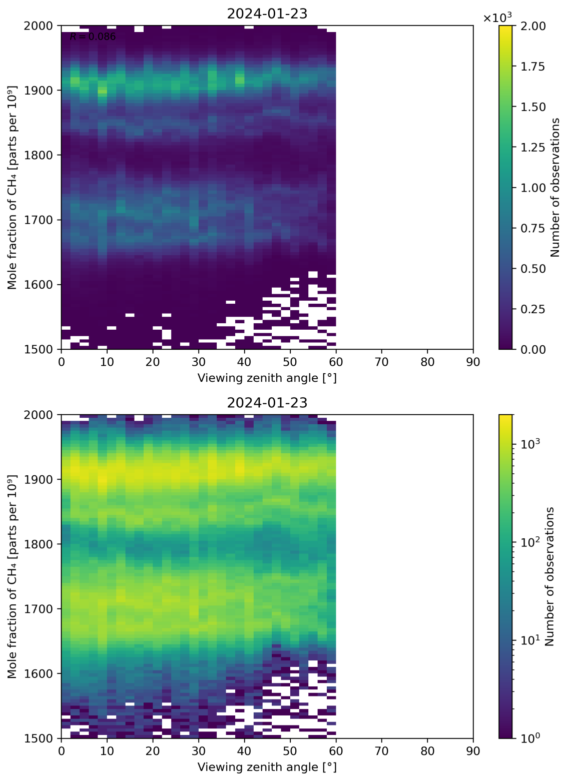
Figure 110: Scatter density plot of “Viewing zenith angle” against “Mole fraction of CH 4 ” for 2024-01-22 to 2024-01-24.
