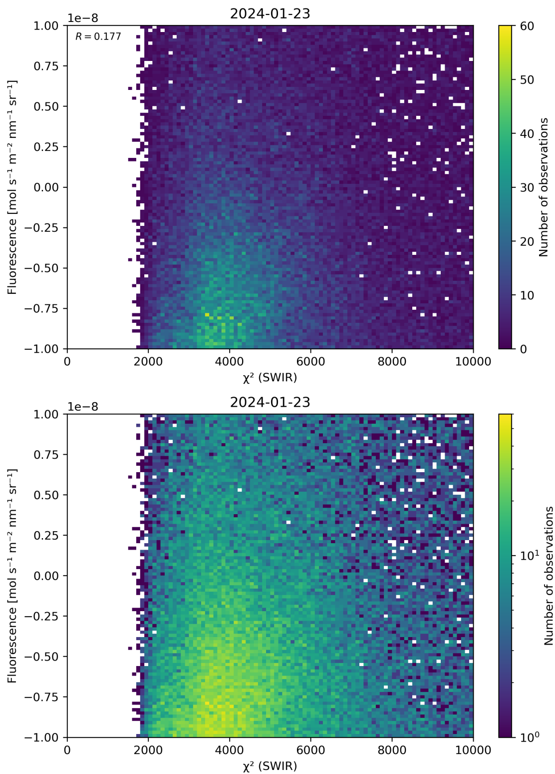
Figure 49: Scatter density plot of “ \chi^2 (SWIR)” against “Fluorescence” for 2024-01-22 to 2024-01-24.
