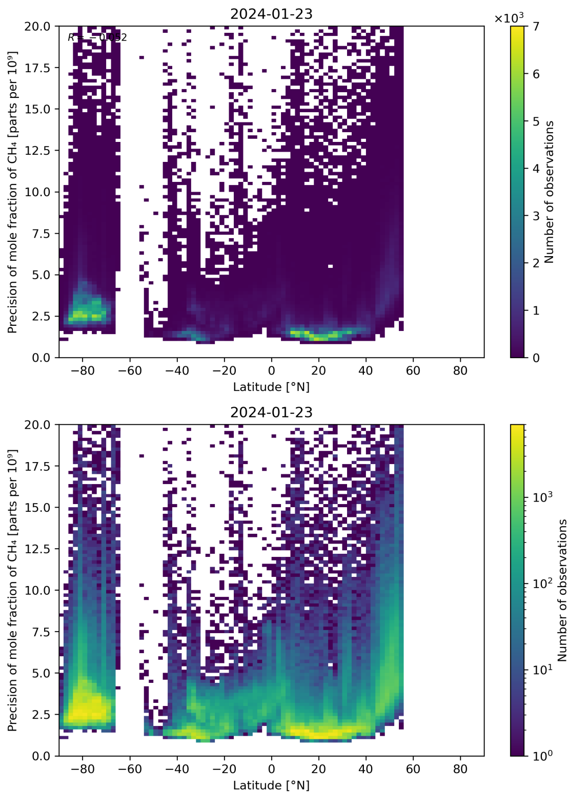
Figure 59: Scatter density plot of “Latitude” against “Precision of mole fraction of CH 4 ” for 2024-01-22 to 2024-01-24.
