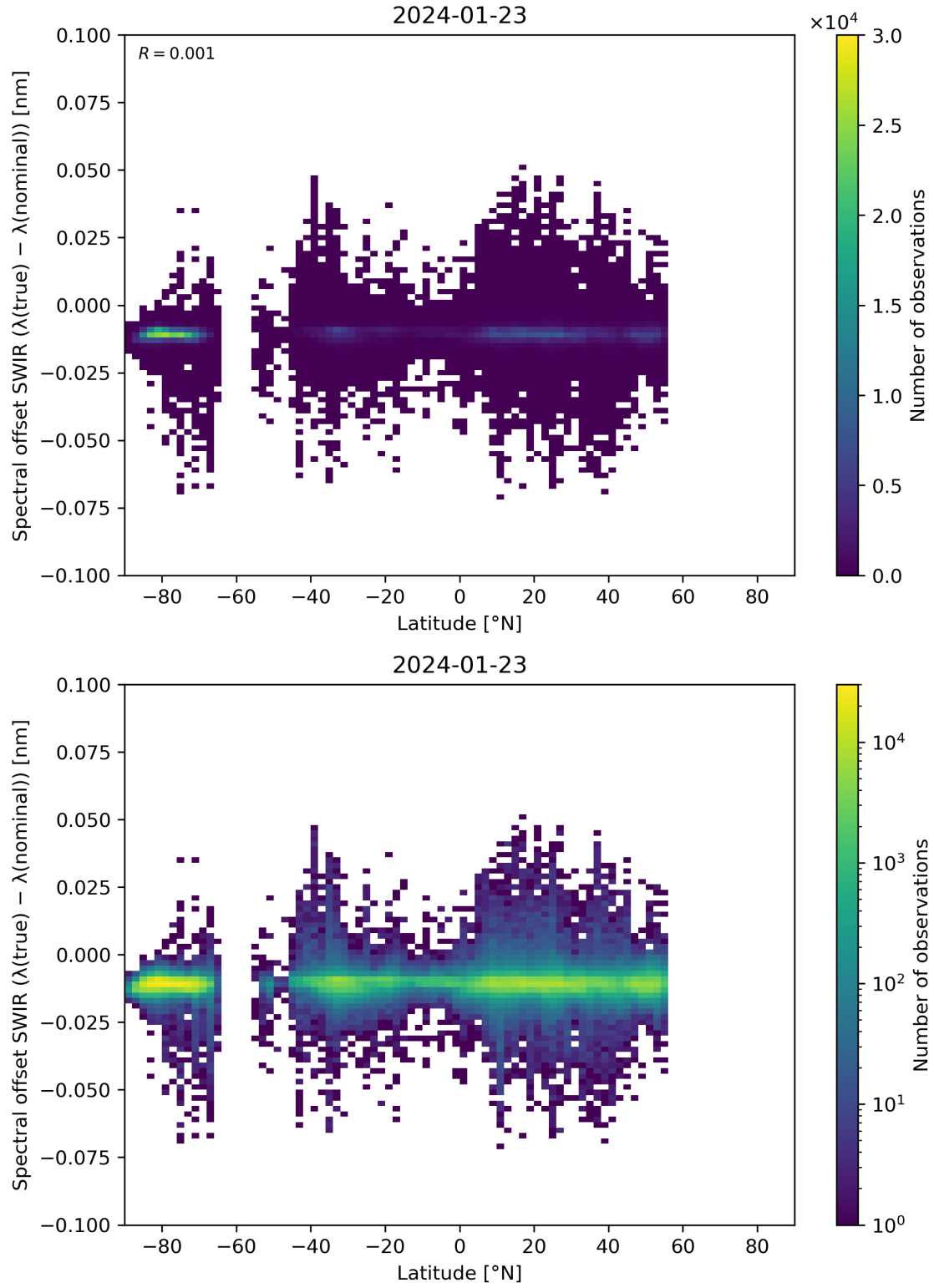
Figure 62: Scatter density plot of “Latitude” against “Spectral offset SWIR ( \lambda(\text{true}) - \lambda(\text{nominal}) )” for 2024-01-22 to 2024-01-24.
