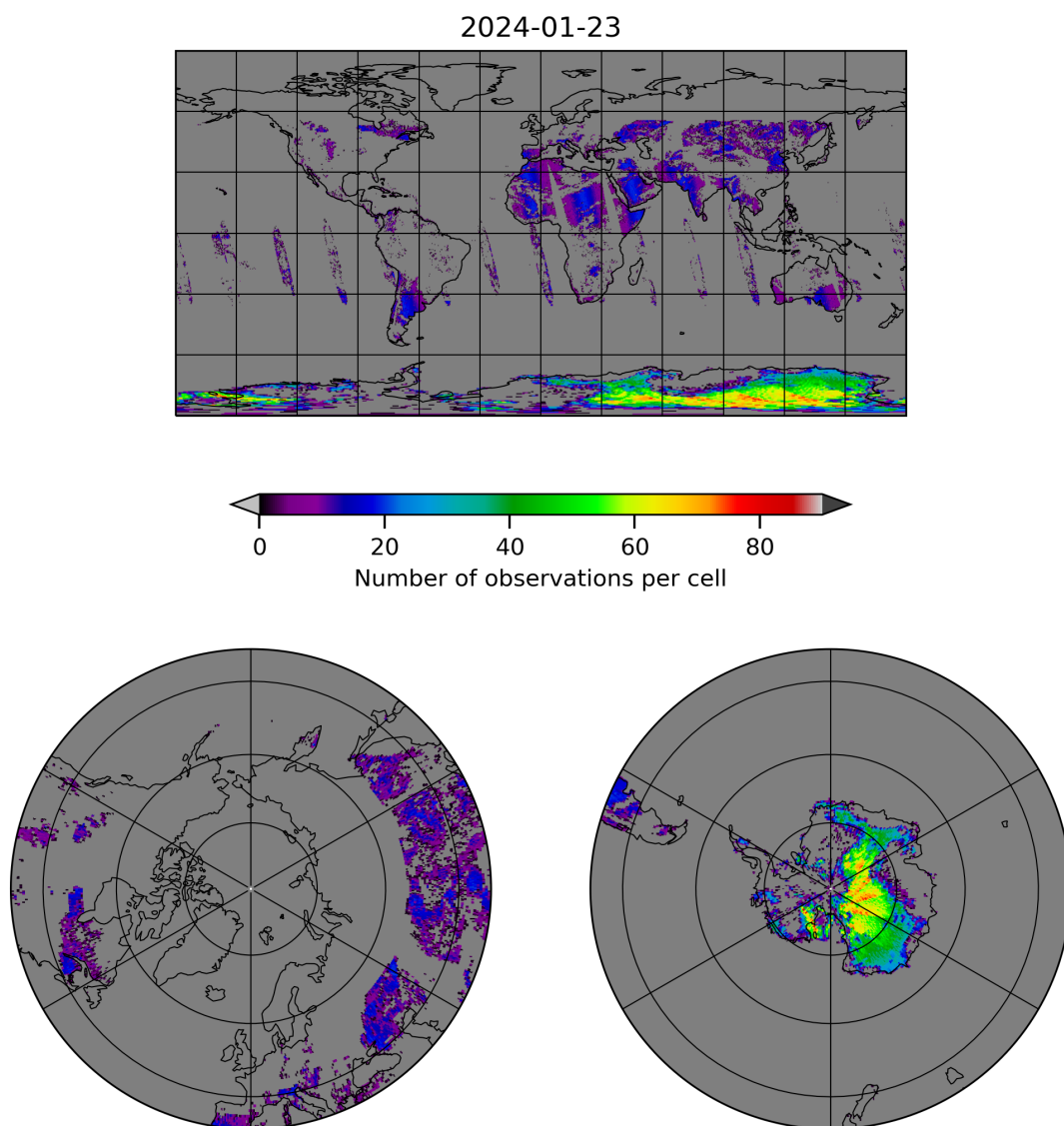
Figure 10: Map of the number of observations for 2024-01-22 to 2024-01-24
