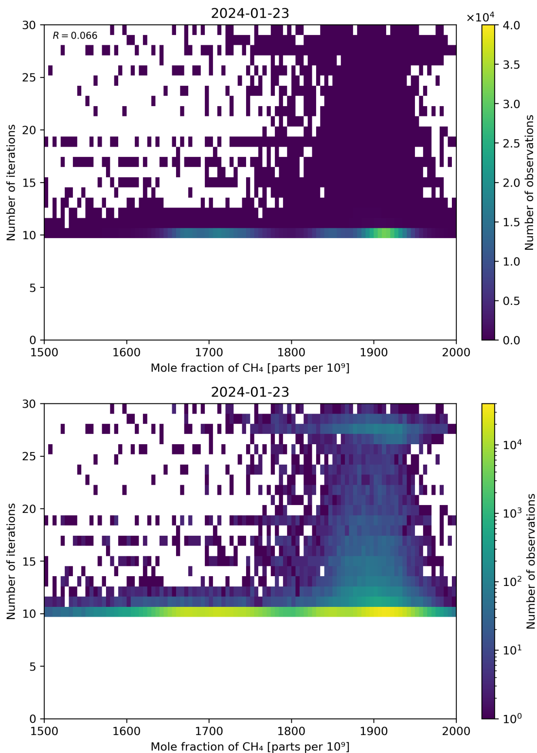
Figure 76: Scatter density plot of “Mole fraction of CH 4 ” against “Number of iterations” for 2024-01-22 to 2024-01-24.
