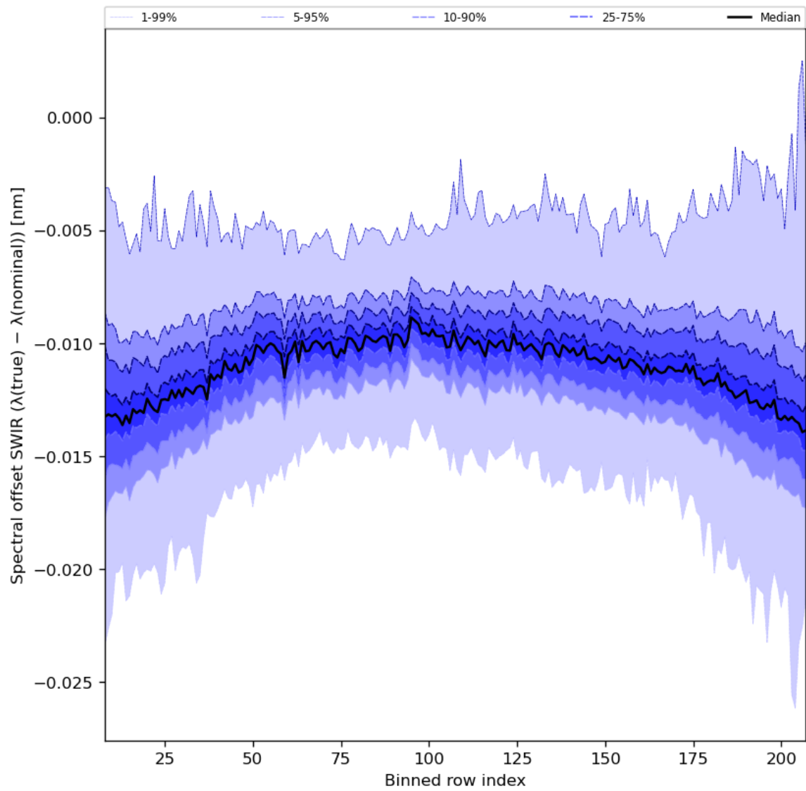
Figure 38: Along track statistics of “Spectral offset SWIR ( \lambda(\text{true}) - \lambda(\text{nominal}) )” for 2024-01-22 to 2024-01-24
