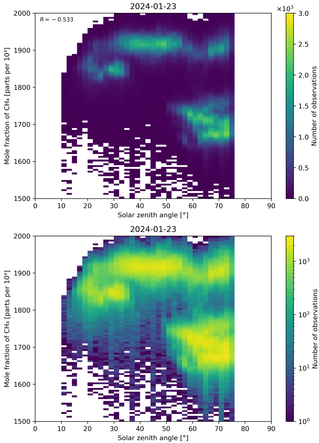
Figure 99: Scatter density plot of “Solar zenith angle” against “Mole fraction of CH 4 ” for 2024-01-22 to 2024-01-24.
