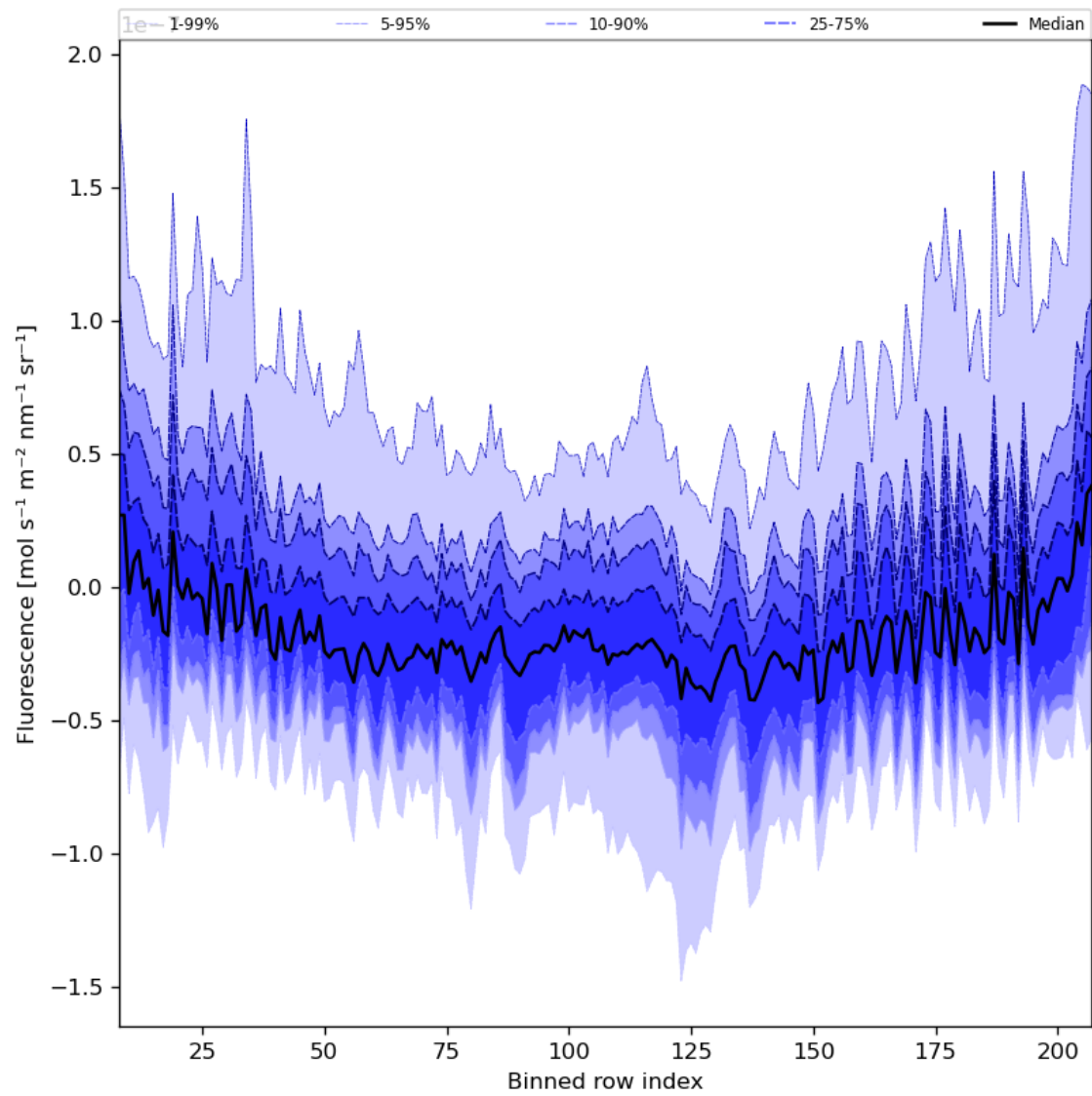
Figure 43: Along track statistics of “Fluorescence” for 2024-01-22 to 2024-01-24
