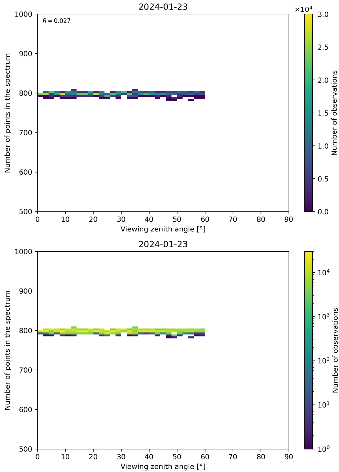
Figure 114: Scatter density plot of “Viewing zenith angle” against “Number of points in the spectrum” for 2024-01-22 to 2024-01-24.
