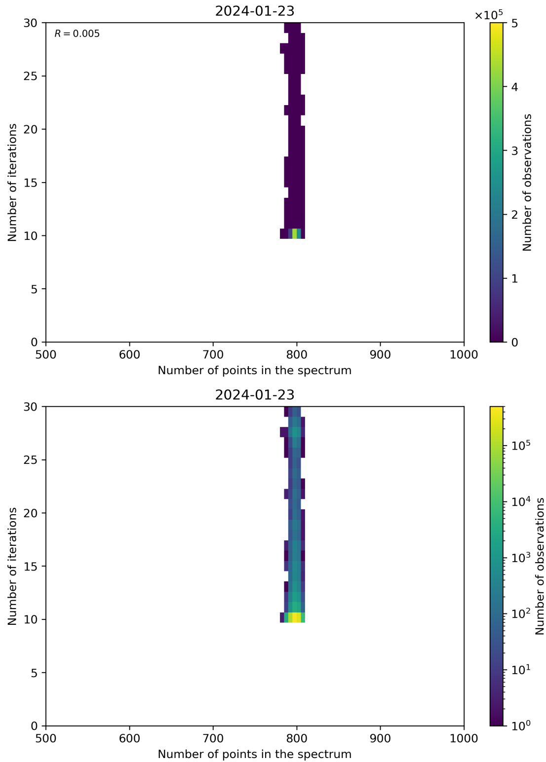
Figure 92: Scatter density plot of “Number of points in the spectrum” against “Number of iterations” for 2024-01-22 to 2024-01-24.
