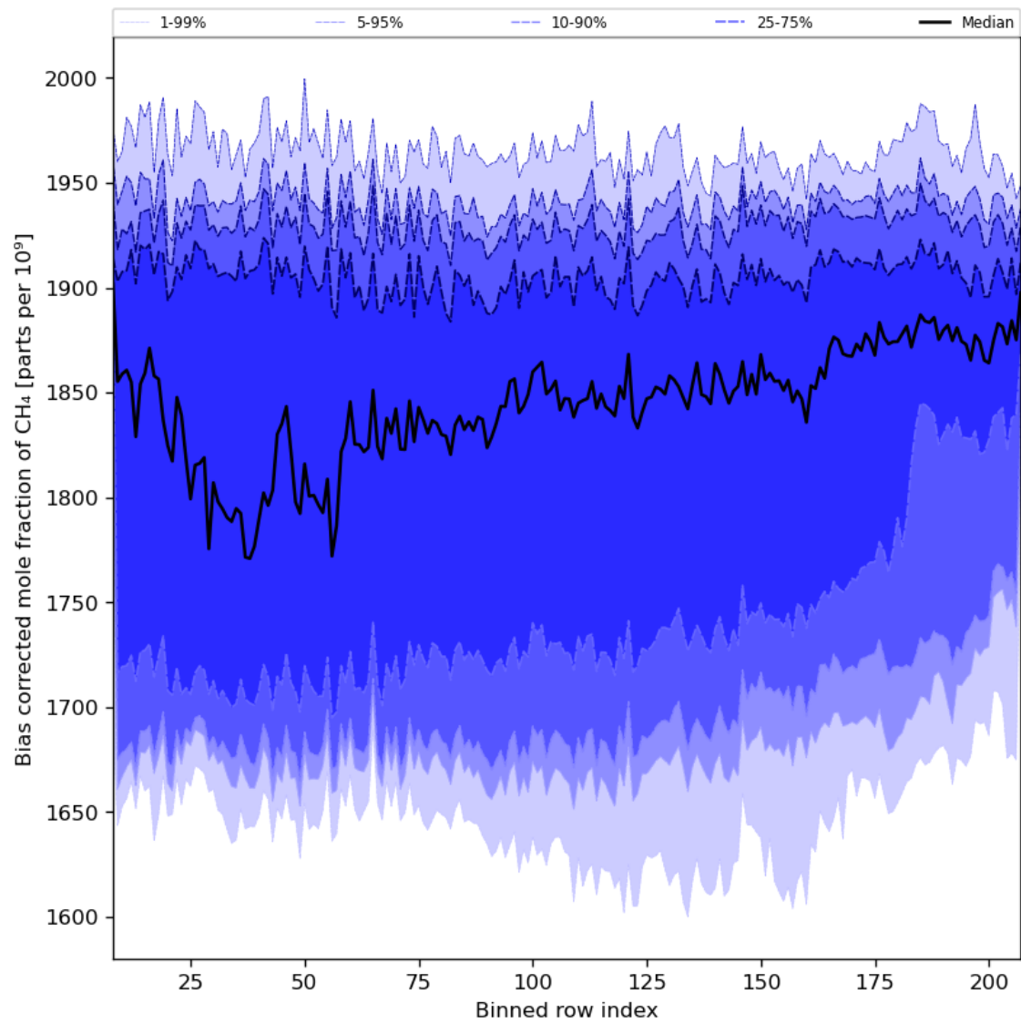
Figure 36: Along track statistics of “Bias corrected mole fraction of CH 4 ” for 2024-01-22 to 2024-01-24
