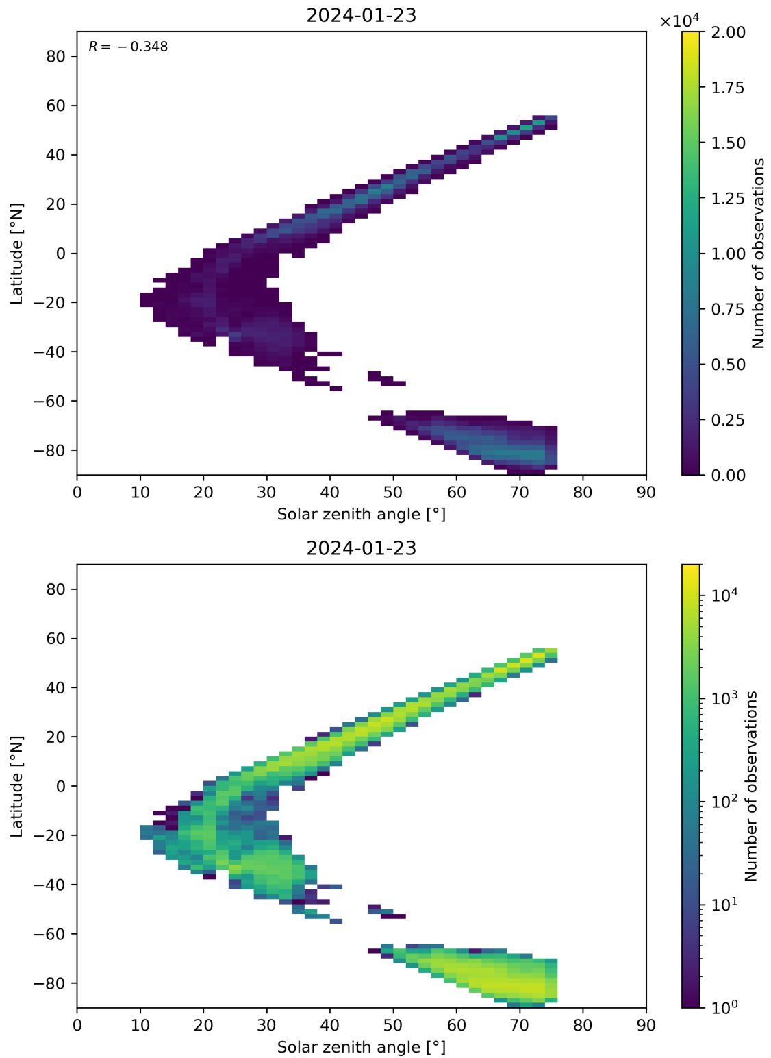
Figure 98: Scatter density plot of “Solar zenith angle” against “Latitude” for 2024-01-22 to 2024-01-24.
