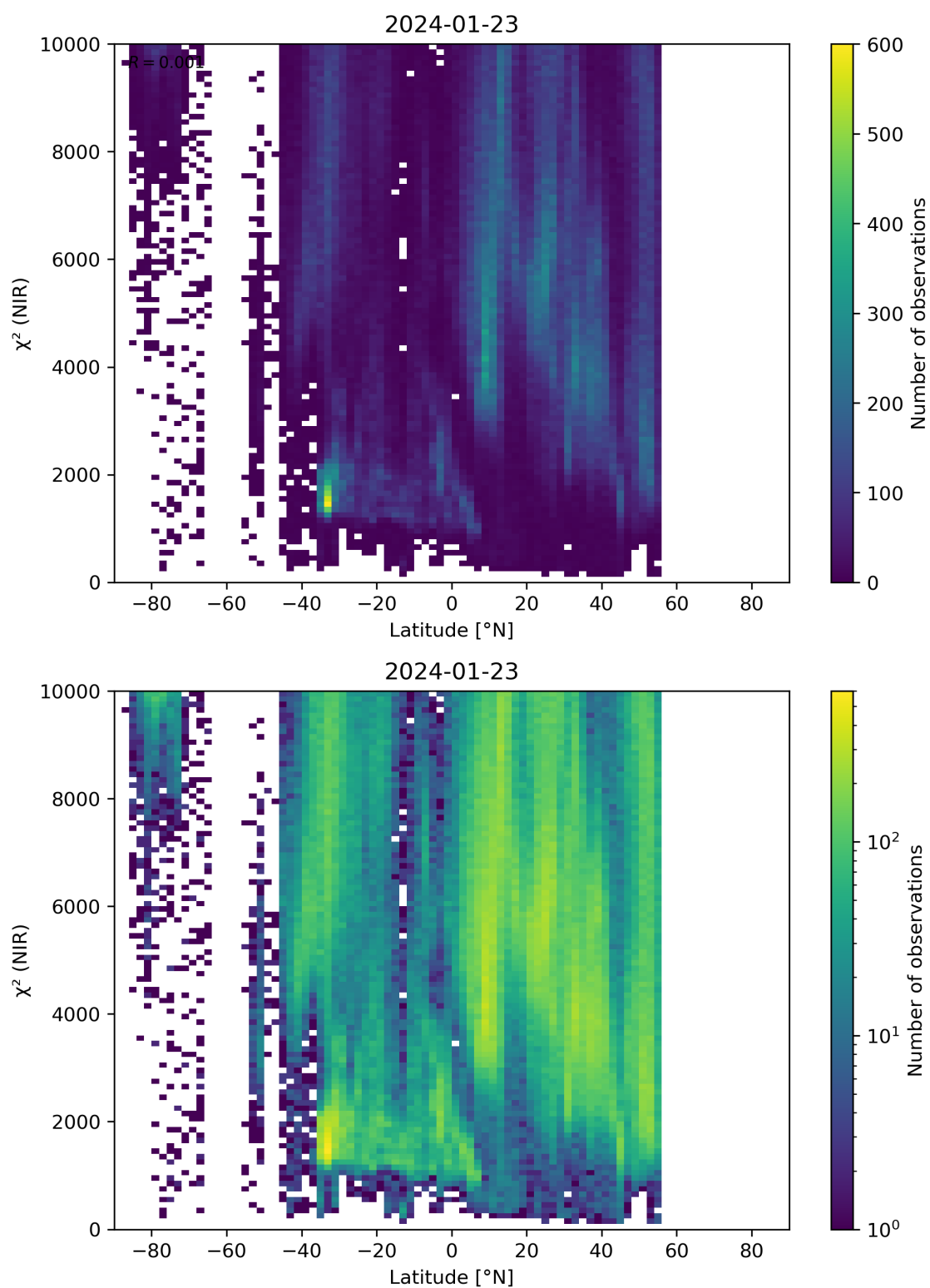
Figure 53: Scatter density plot of “Latitude” against “ \chi^2 (NIR)” for 2024-01-22 to 2024-01-24.
