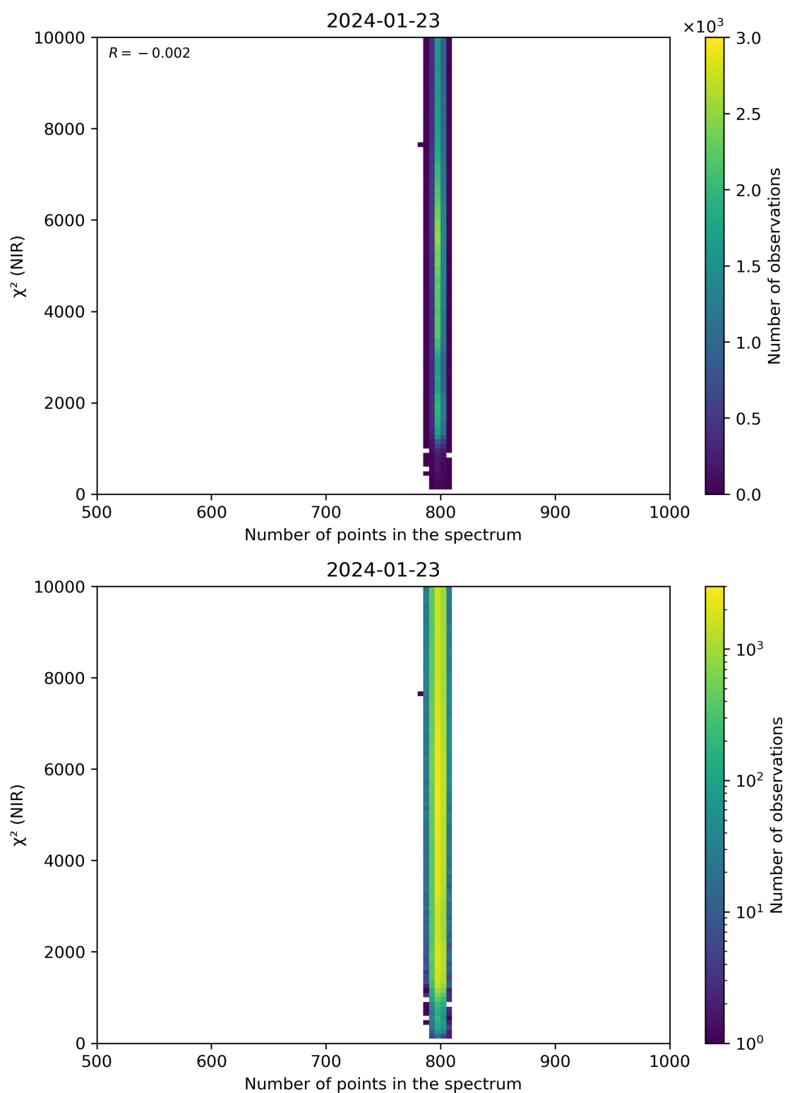
Figure 88: Scatter density plot of “Number of points in the spectrum” against “ \chi^2 (NIR)” for 2024-01-22 to 2024-01-24.
