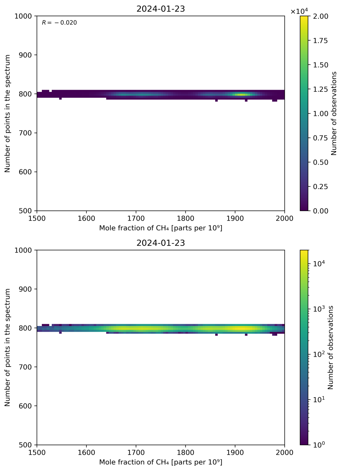
Figure 77: Scatter density plot of “Mole fraction of CH 4 ” against “Number of points in the spectrum” for 2024-01-22 to 2024-01-24.
