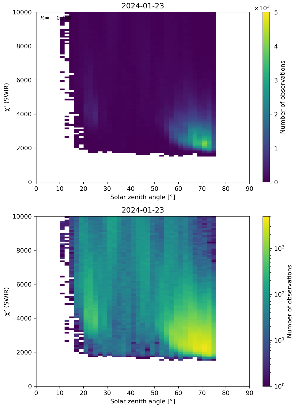
Figure 95: Scatter density plot of “Solar zenith angle” against “ \chi^2 (SWIR)” for 2024-01-22 to 2024-01-24.
