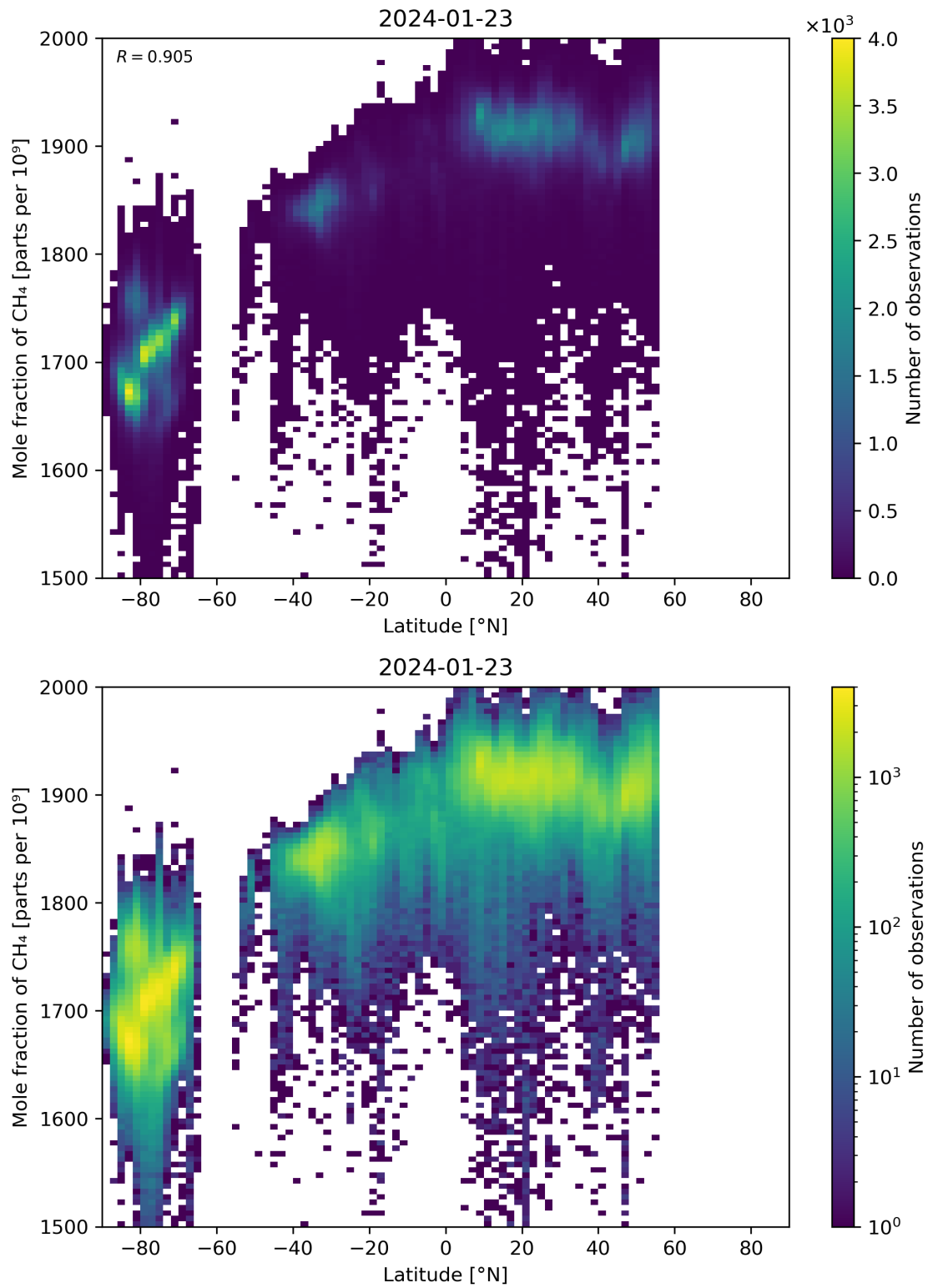
Figure 57: Scatter density plot of “Latitude” against “Mole fraction of \text{CH}_4 ” for 2024-01-22 to 2024-01-24.
