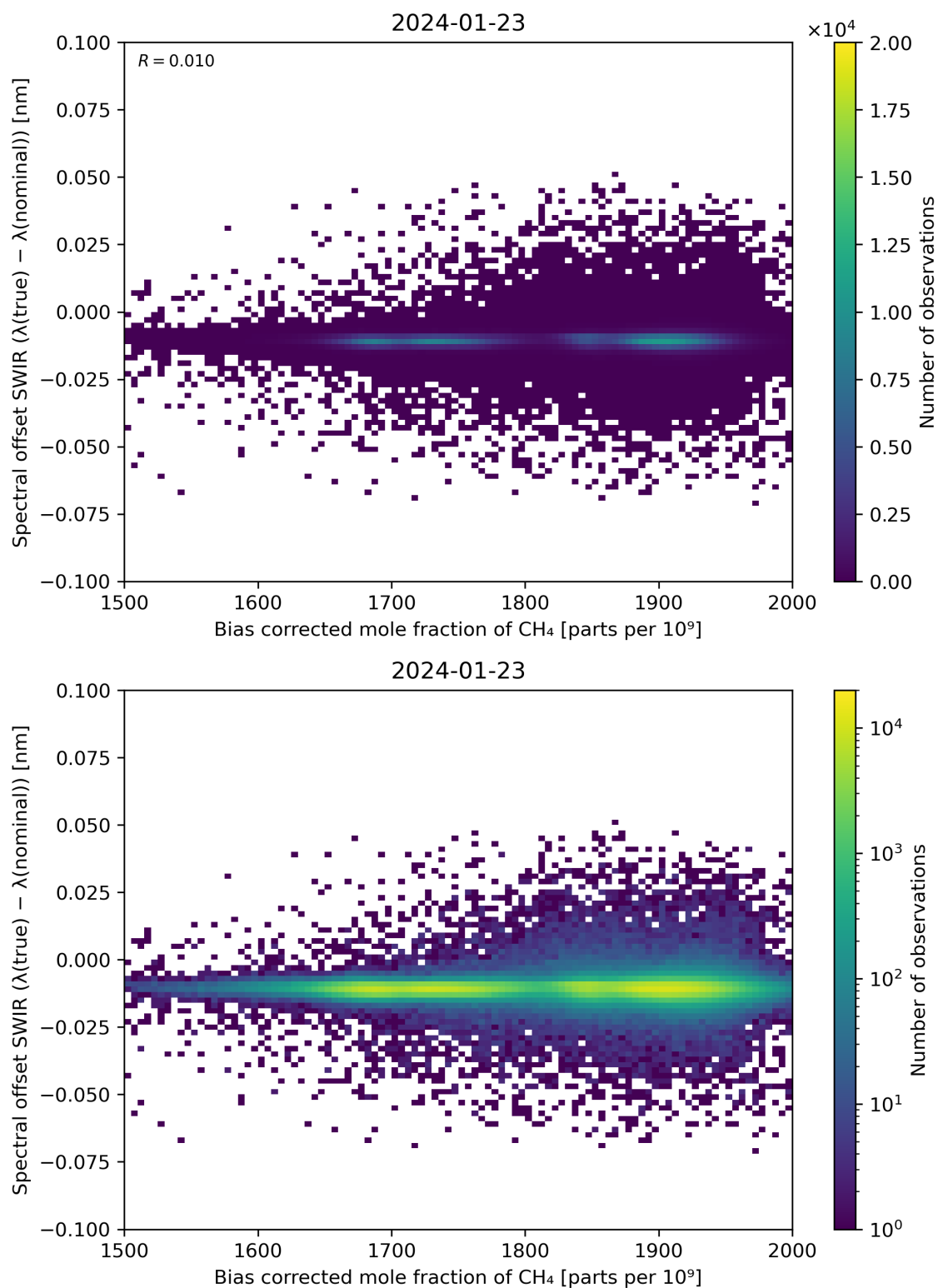
Figure 69: Scatter density plot of “Bias corrected mole fraction of \text{CH}_4 ” against “Spectral offset SWIR ( \lambda(\text{true}) - \lambda(\text{nominal}) )” for 2024-01-22 to 2024-01-24.
