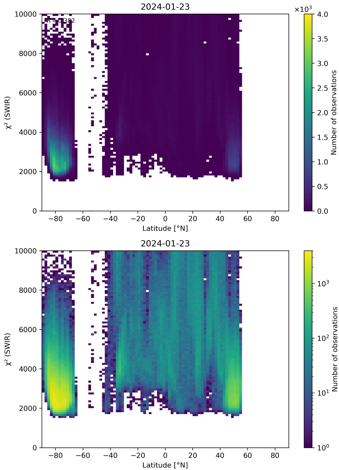
Figure 54: Scatter density plot of “Latitude” against “ \chi^2 (SWIR)” for 2024-01-22 to 2024-01-24.
