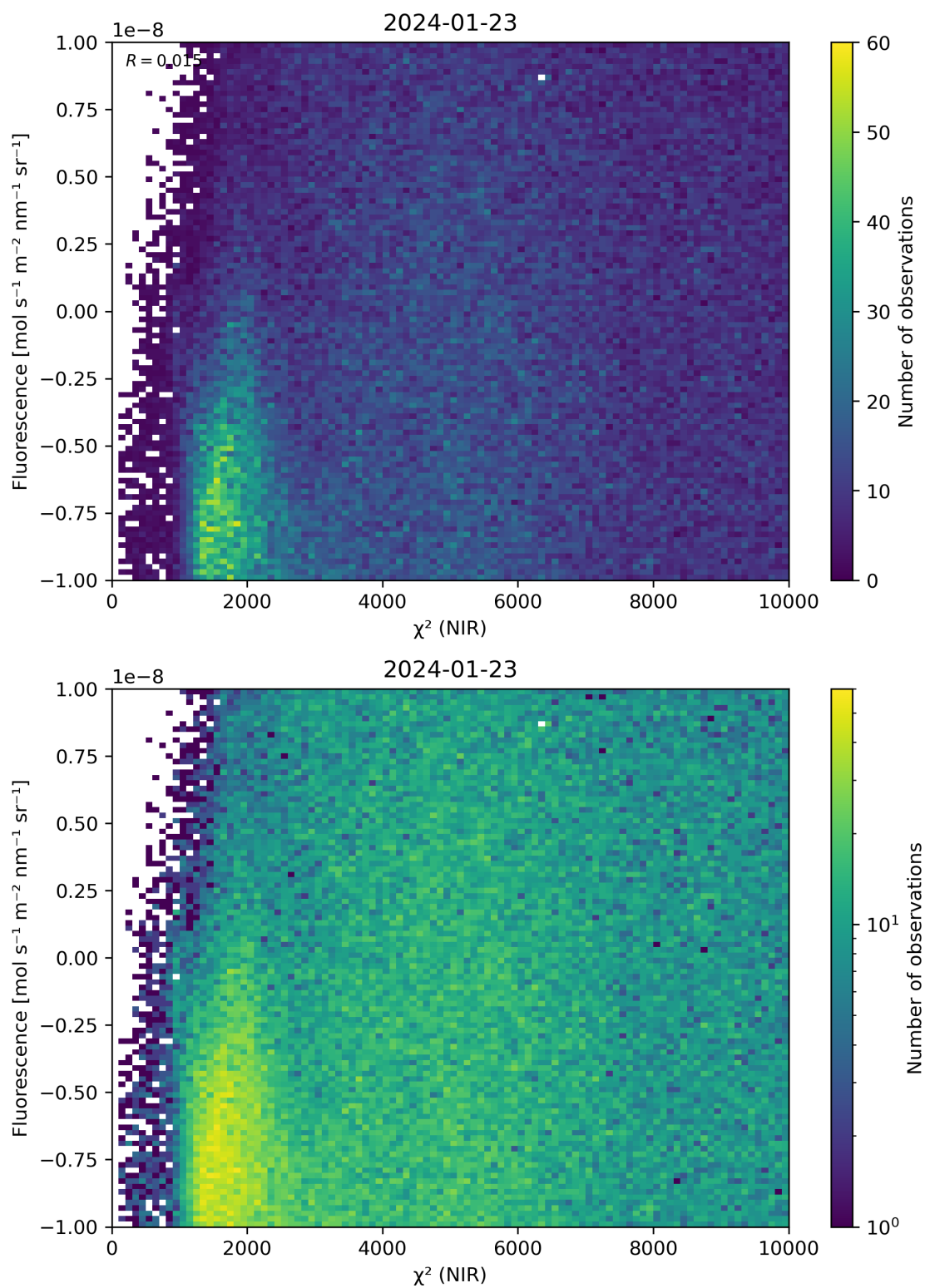
Figure 45: Scatter density plot of “ \chi^2 (NIR)” against “Fluorescence” for 2024-01-22 to 2024-01-24.
