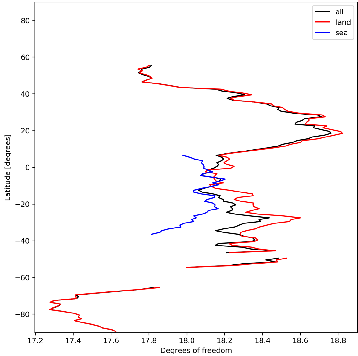
Figure 19: Zonal average of “Degrees of freedom” for 2024-01-22 to 2024-01-24.
