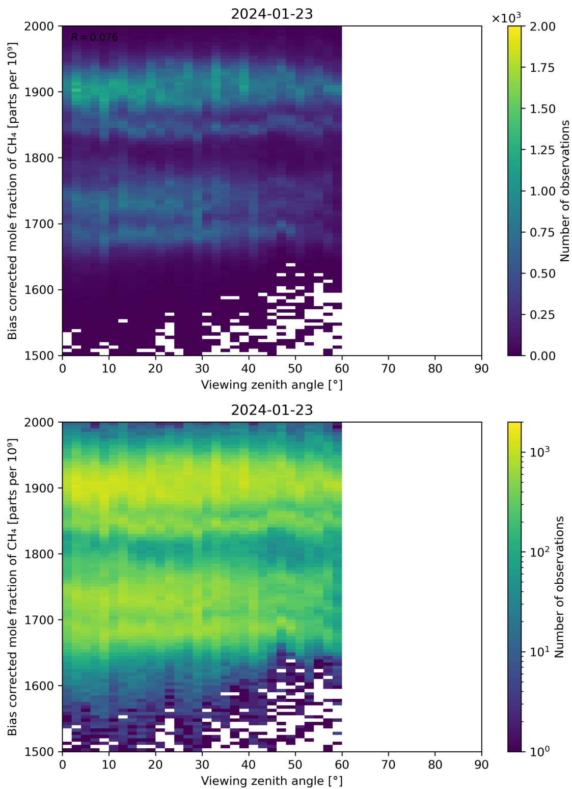
Figure 111: Scatter density plot of “Viewing zenith angle” against “Bias corrected mole fraction of CH 4 ” for 2024-01-22 to 2024-01-24.
