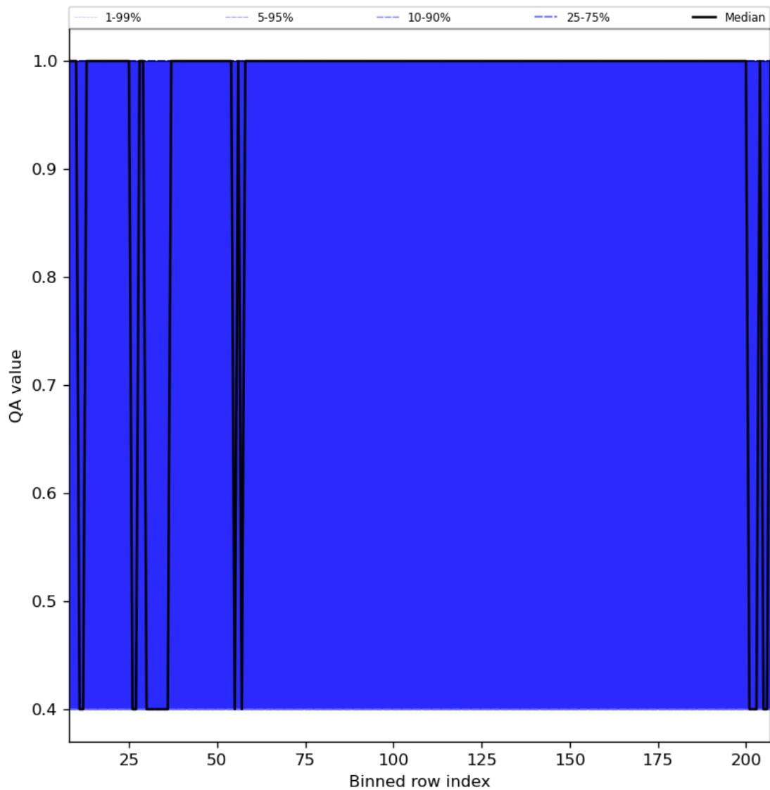
Figure 33: Along track statistics of “QA value” for 2024-01-22 to 2024-01-24
