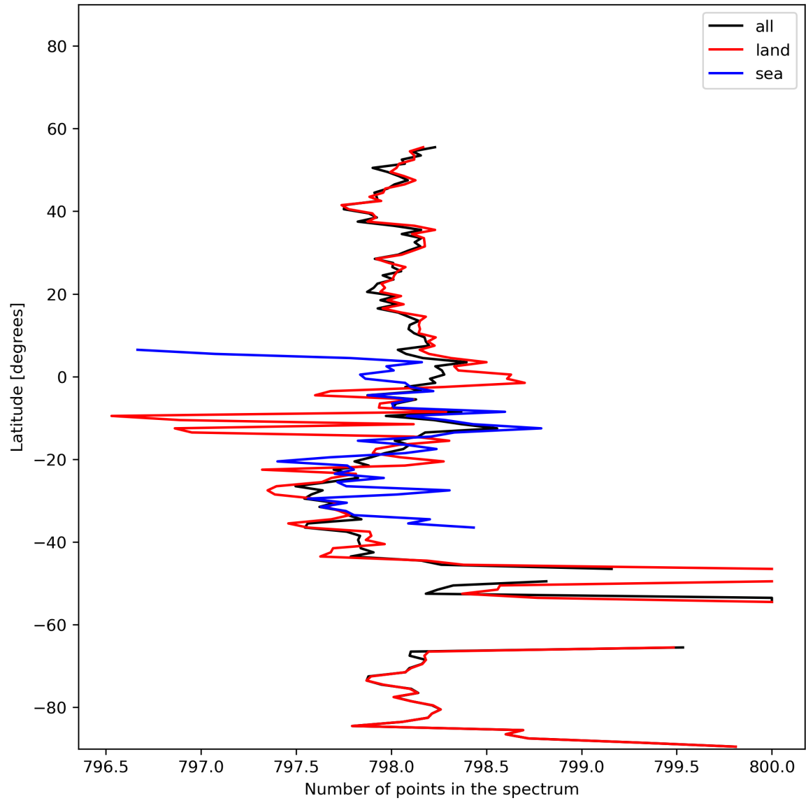
Figure 15: Zonal average of “Number of points in the spectrum” for 2024-01-22 to 2024-01-24.
