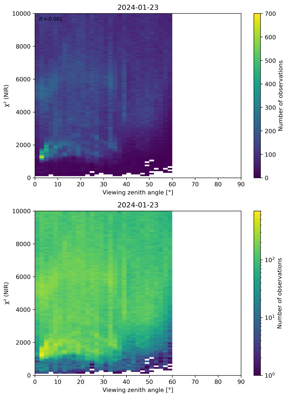
Figure 105: Scatter density plot of “Viewing zenith angle” against “ \chi^2 (NIR)” for 2024-01-22 to 2024-01-24.
