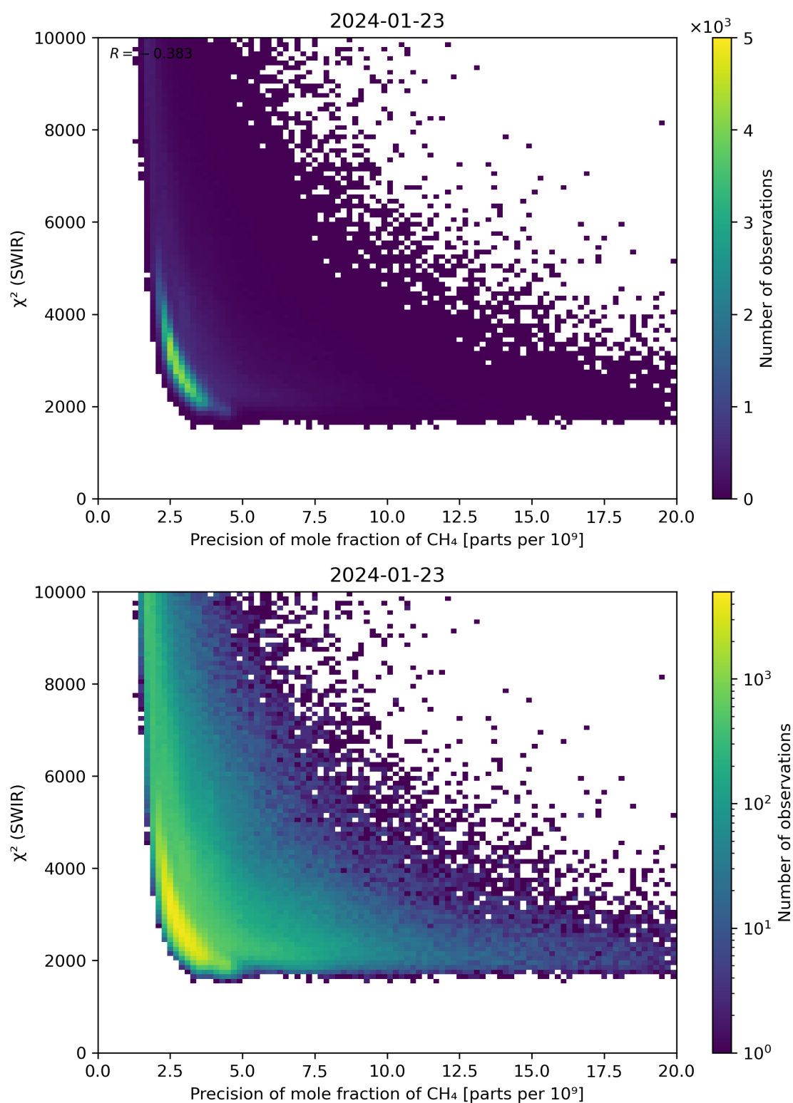
Figure 79: Scatter density plot of “Precision of mole fraction of CH 4 ” against “ \chi^2 (SWIR)” for 2024-01-22 to 2024-01-24.
