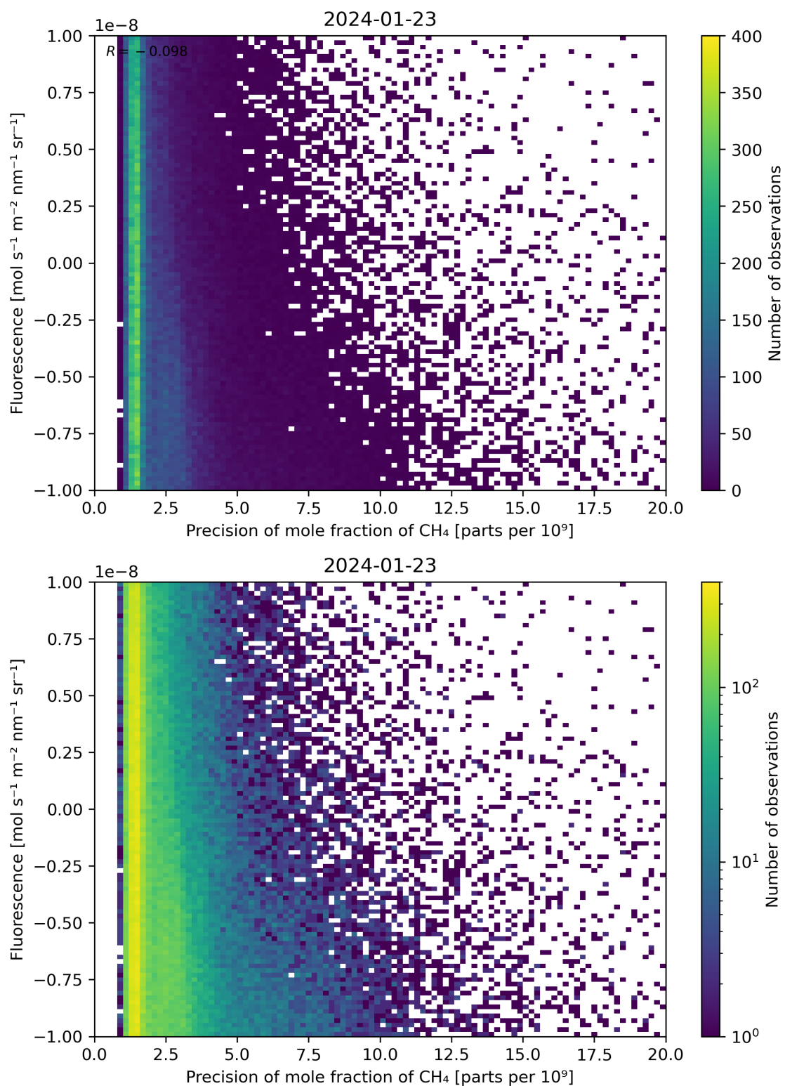
Figure 81: Scatter density plot of “Precision of mole fraction of \text{CH}_4 ” against “Fluorescence” for 2024-01-22 to 2024-01-24.
