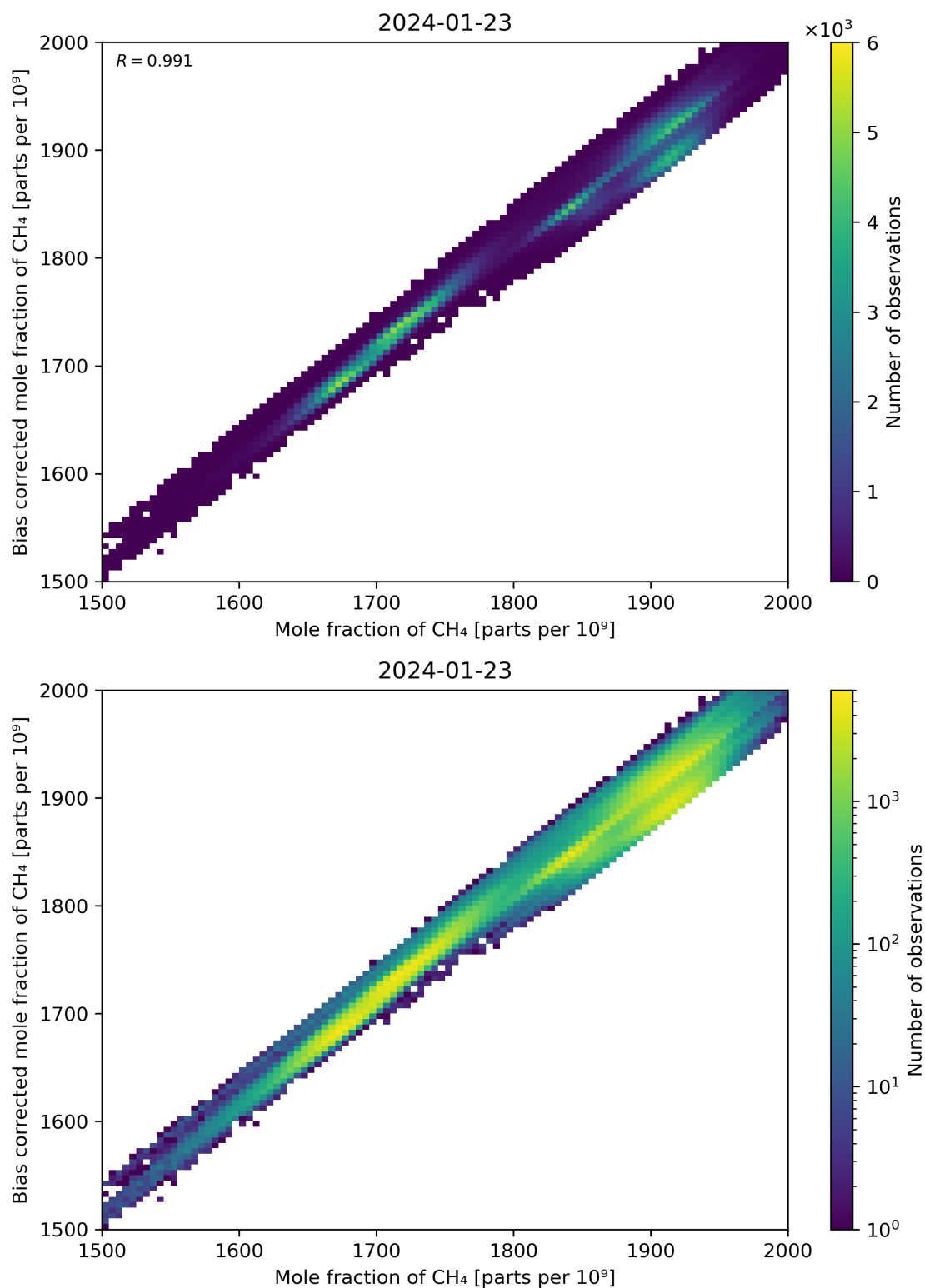
Figure 74: Scatter density plot of “Mole fraction of CH 4 ” against “Bias corrected mole fraction of CH 4 ” for 2024-01-22 to 2024-01-24.
