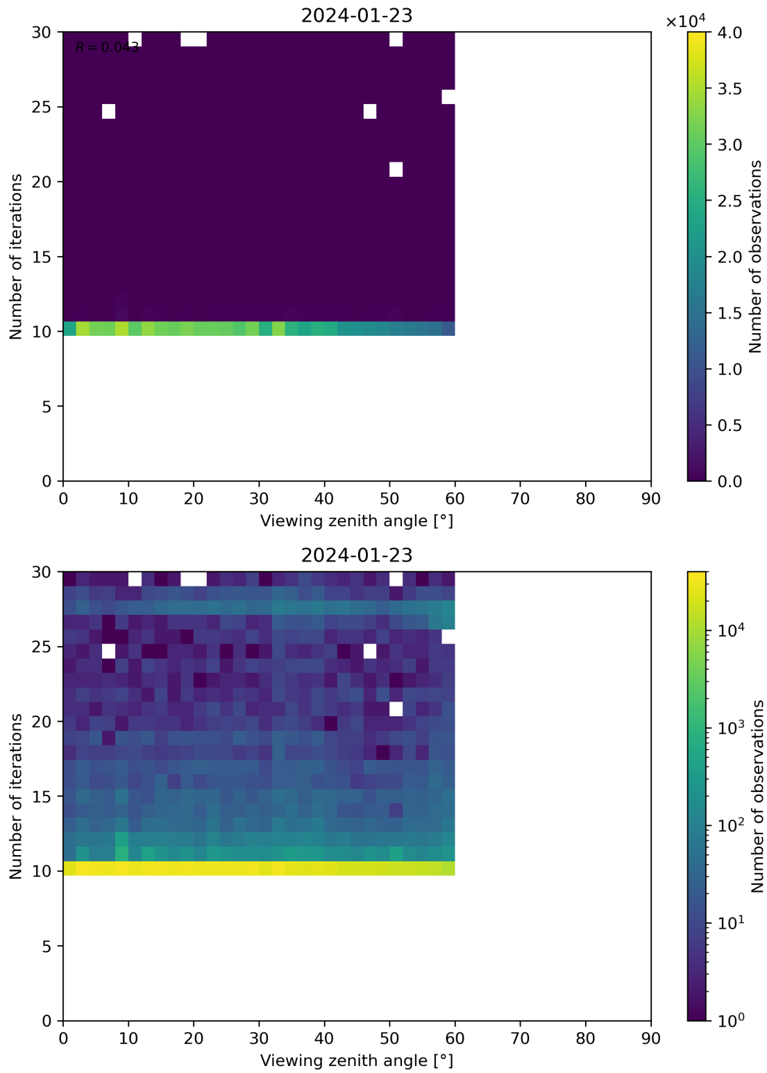
Figure 113: Scatter density plot of “Viewing zenith angle” against “Number of iterations” for 2024-01-22 to 2024-01-24.
