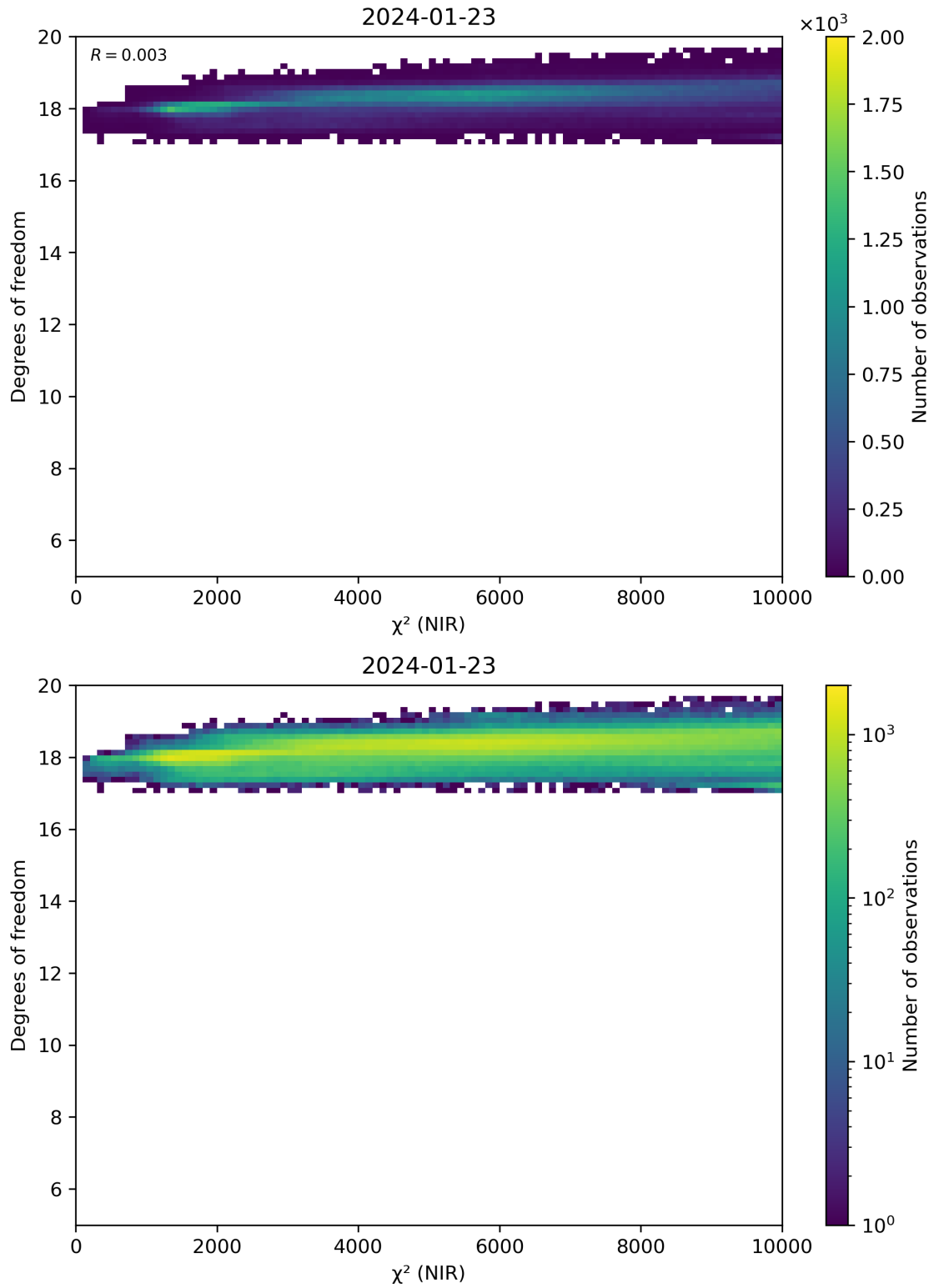
Figure 44: Scatter density plot of “ \chi^2 (NIR)” against “Degrees of freedom” for 2024-01-22 to 2024-01-24.
