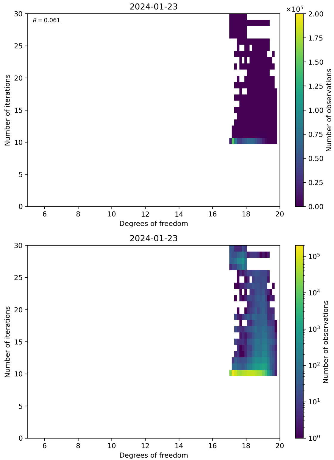
Figure 52: Scatter density plot of “Degrees of freedom” against “Number of iterations” for 2024-01-22 to 2024-01-24.
