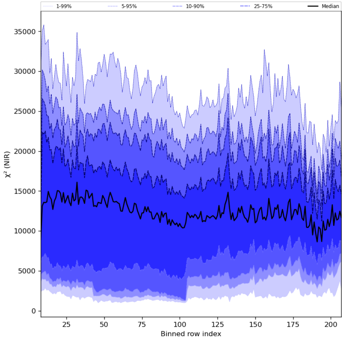
Figure 40: Along track statistics of “ \chi^2 (NIR)” for 2024-01-22 to 2024-01-24
