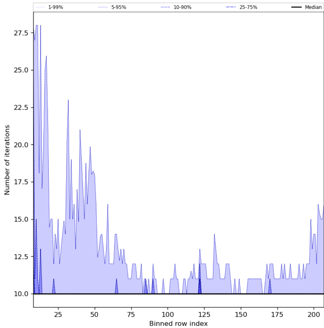
Figure 42: Along track statistics of “Number of iterations” for 2024-01-22 to 2024-01-24
