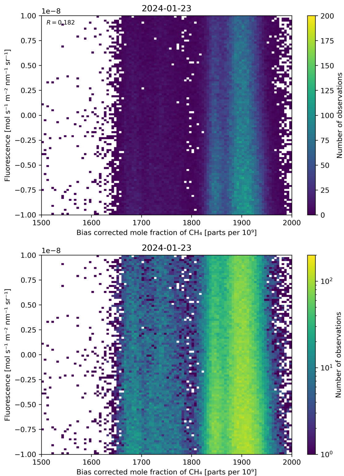
Figure 66: Scatter density plot of “Bias corrected mole fraction of \text{CH}_4 ” against “Fluorescence” for 2024-01-22 to 2024-01-24.
