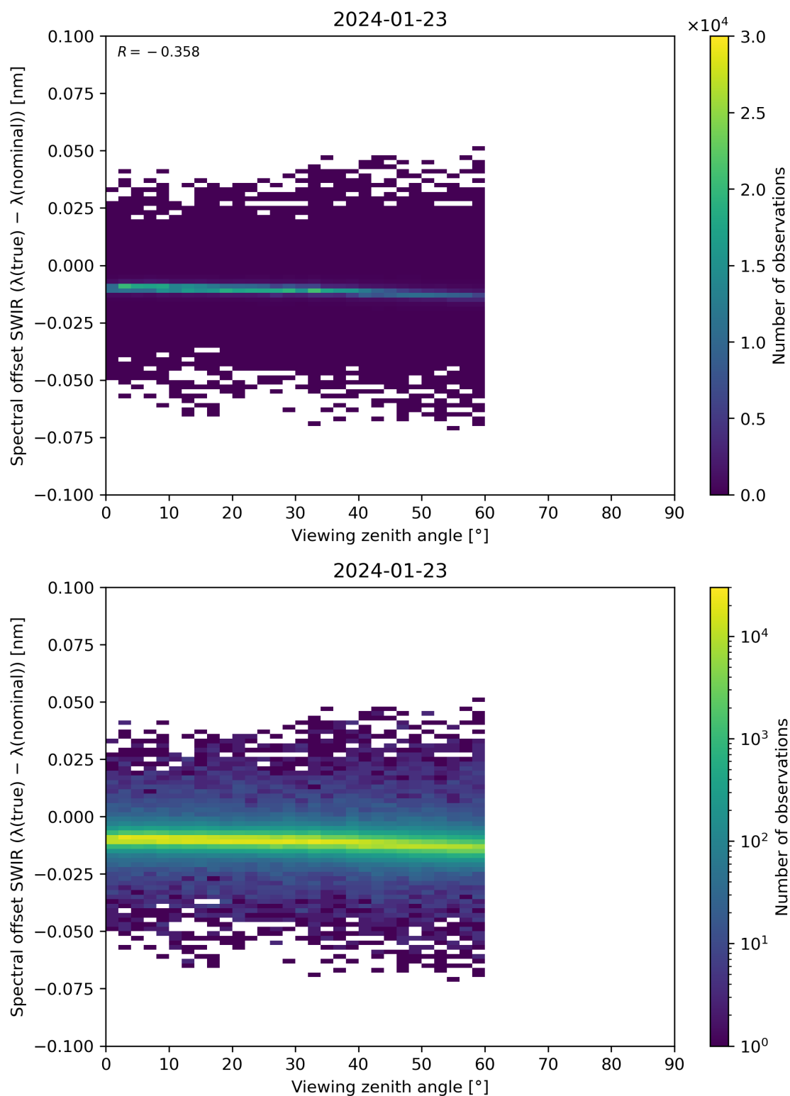
Figure 116: Scatter density plot of “Viewing zenith angle” against “Spectral offset SWIR ( \lambda(\text{true}) - \lambda(\text{nominal}) )” for 2024-01-22 to 2024-01-24.
