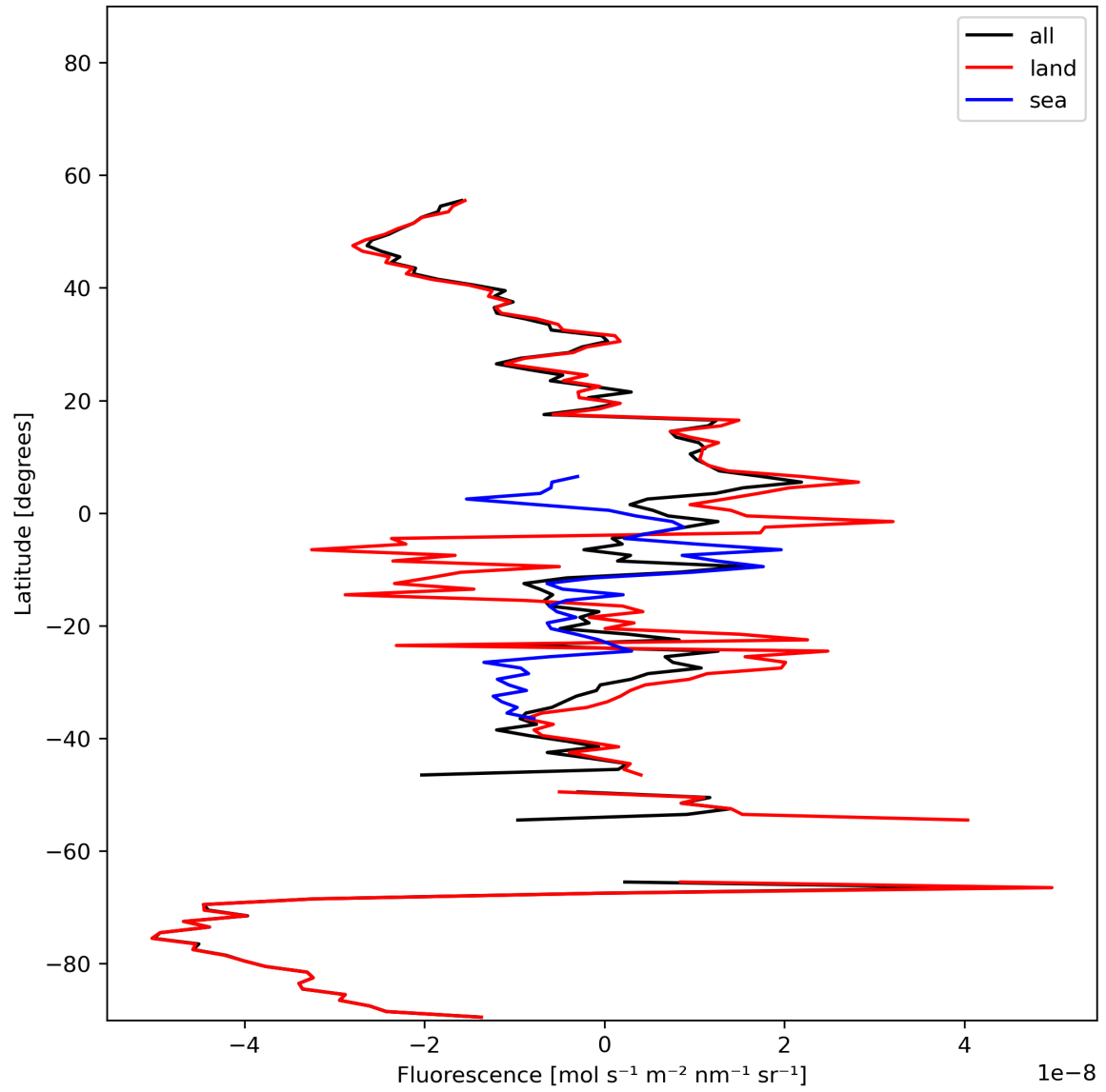
Figure 21: Zonal average of “Fluorescence” for 2024-01-22 to 2024-01-24.
