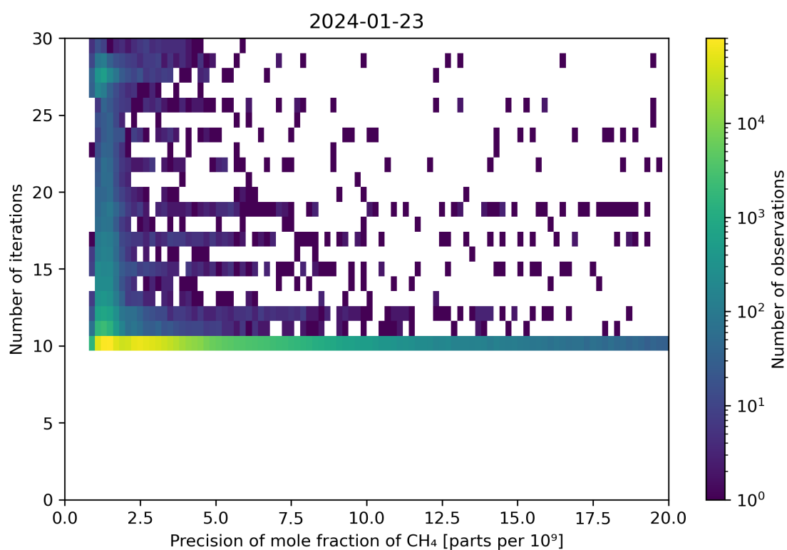
Figure 83: Scatter density plot of “Precision of mole fraction of CH 4 ” against “Number of iterations” for 2024-01-22 to 2024-01-24.
