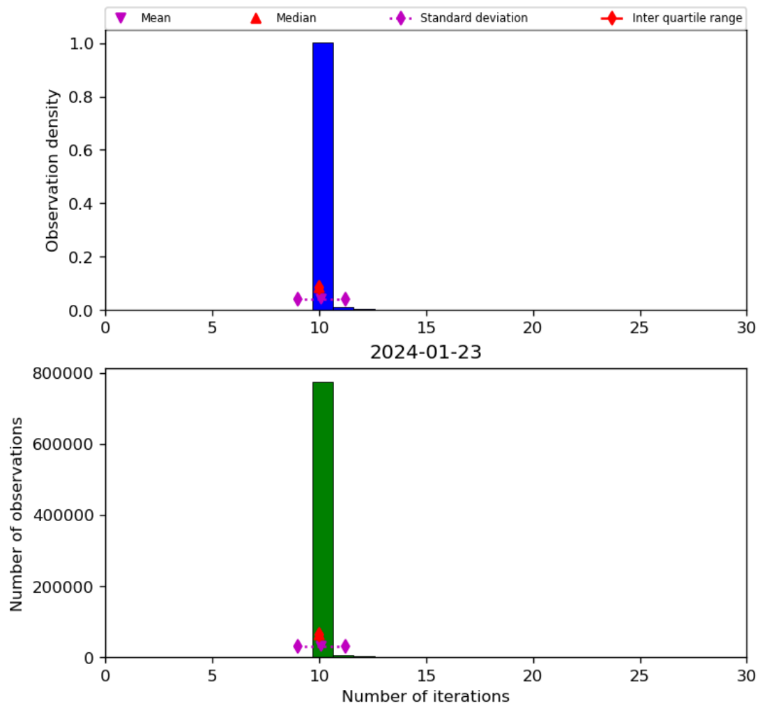
Figure 31: Histogram of “Number of iterations” for 2024-01-22 to 2024-01-24
