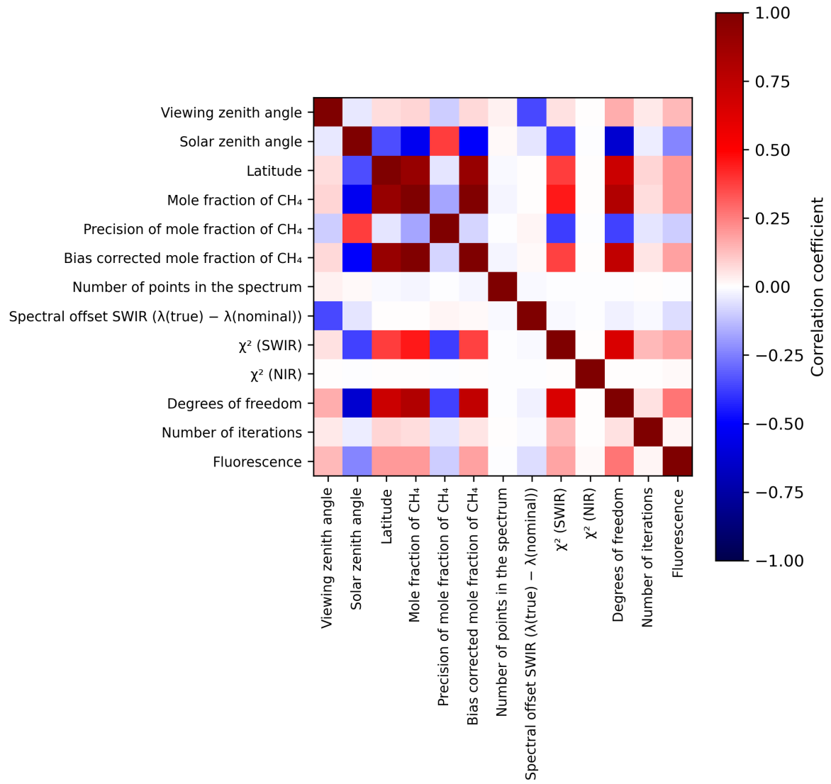
Figure 2: Map of correlation matrix for 2024-01-22 to 2024-01-24.
