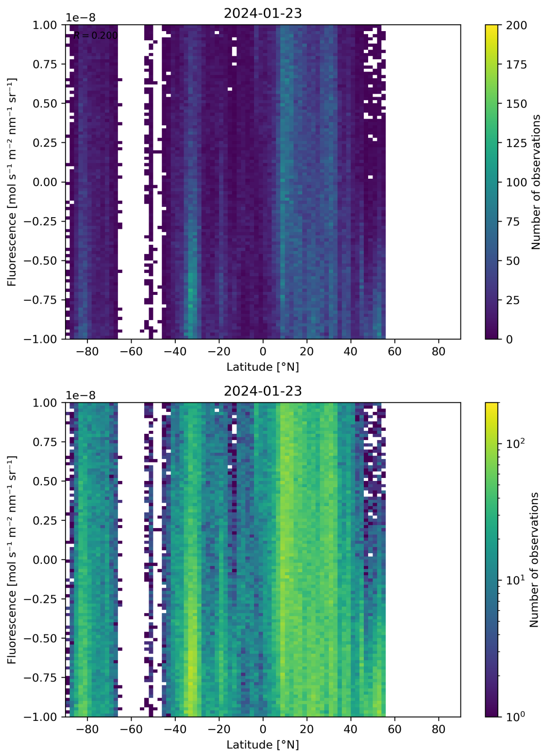
Figure 56: Scatter density plot of “Latitude” against “Fluorescence” for 2024-01-22 to 2024-01-24.
