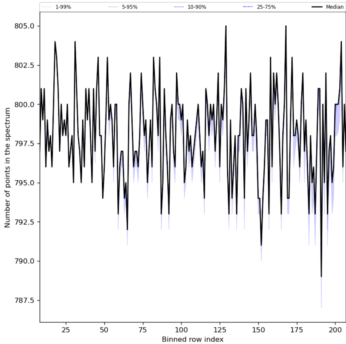
Figure 37: Along track statistics of “Number of points in the spectrum” for 2024-01-22 to 2024-01-24
