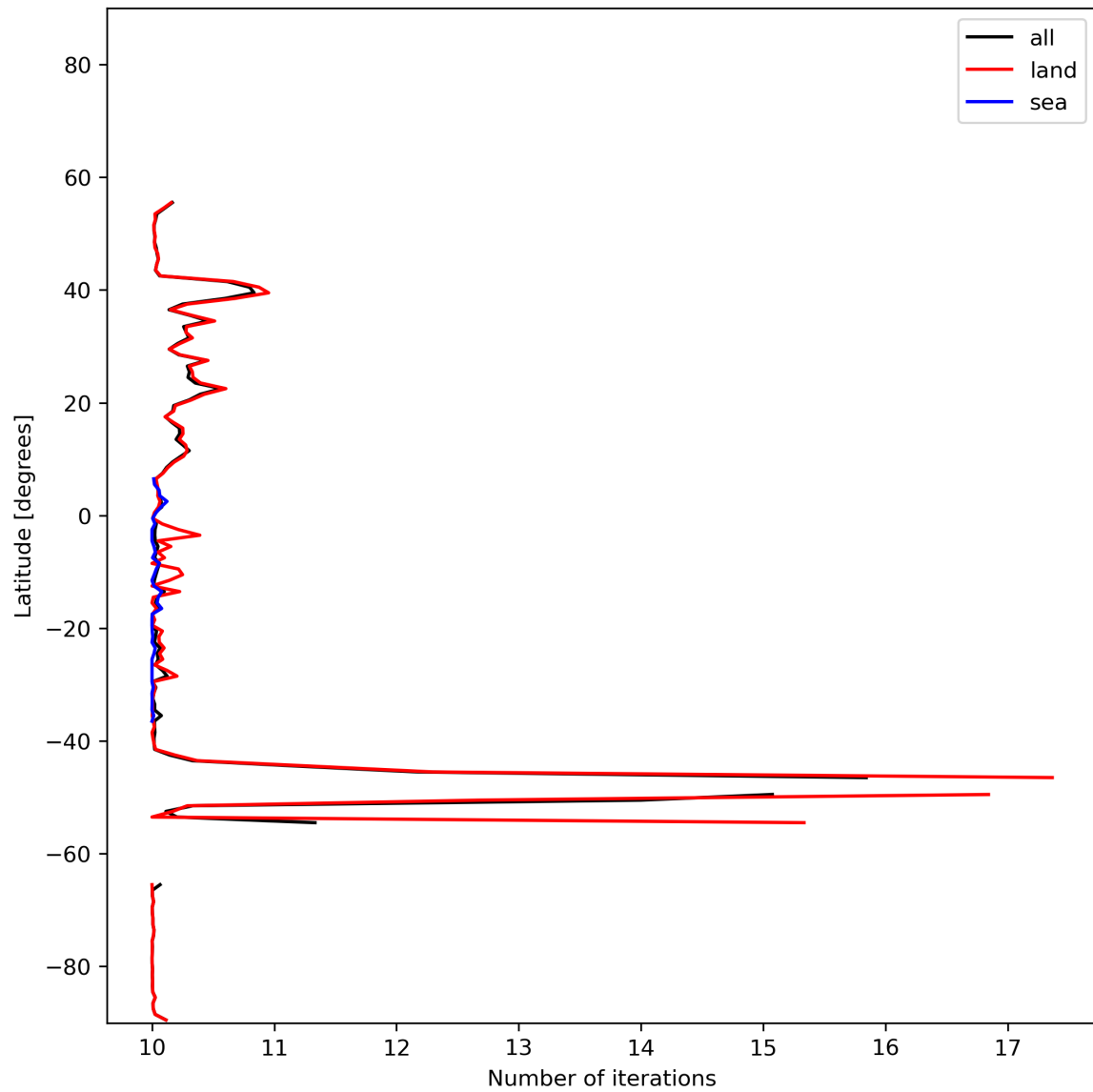
Figure 20: Zonal average of “Number of iterations” for 2024-01-22 to 2024-01-24.
