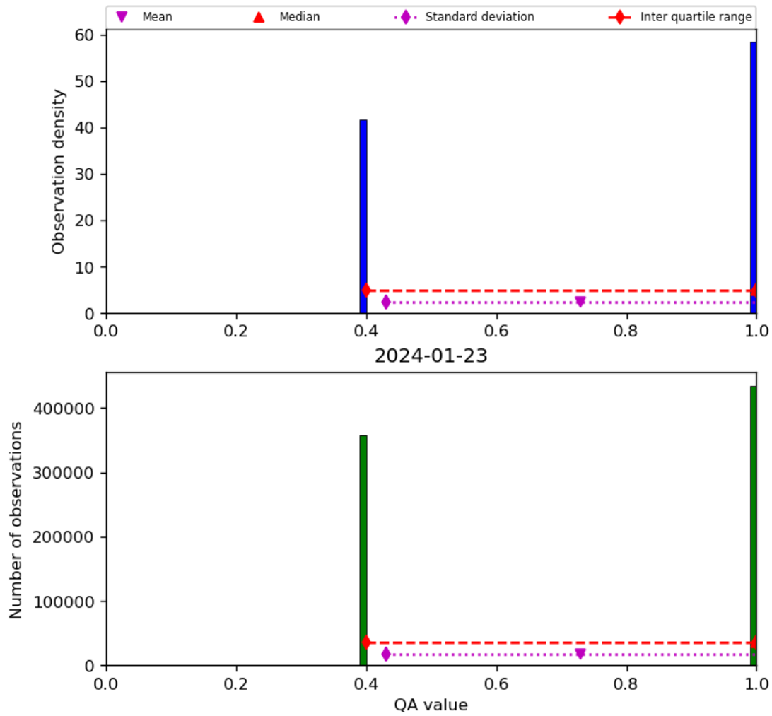
Figure 22: Histogram of “QA value” for 2024-01-22 to 2024-01-24
