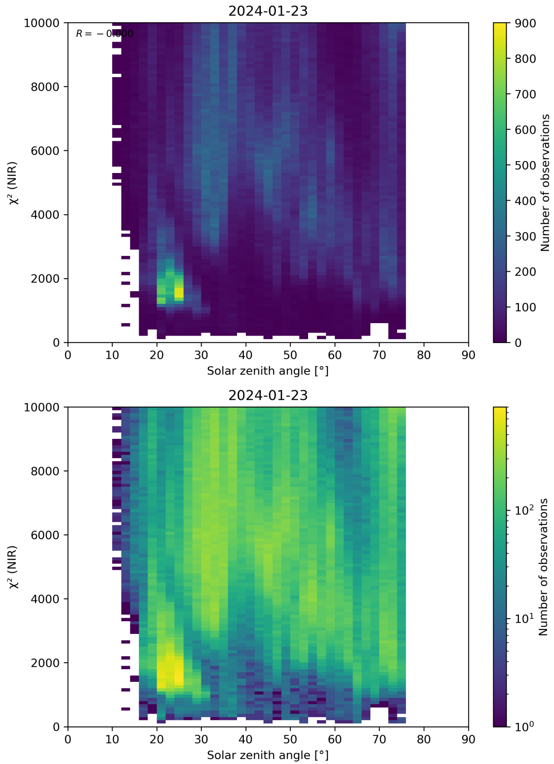
Figure 94: Scatter density plot of “Solar zenith angle” against “ \chi^2 (NIR)” for 2024-01-22 to 2024-01-24.
