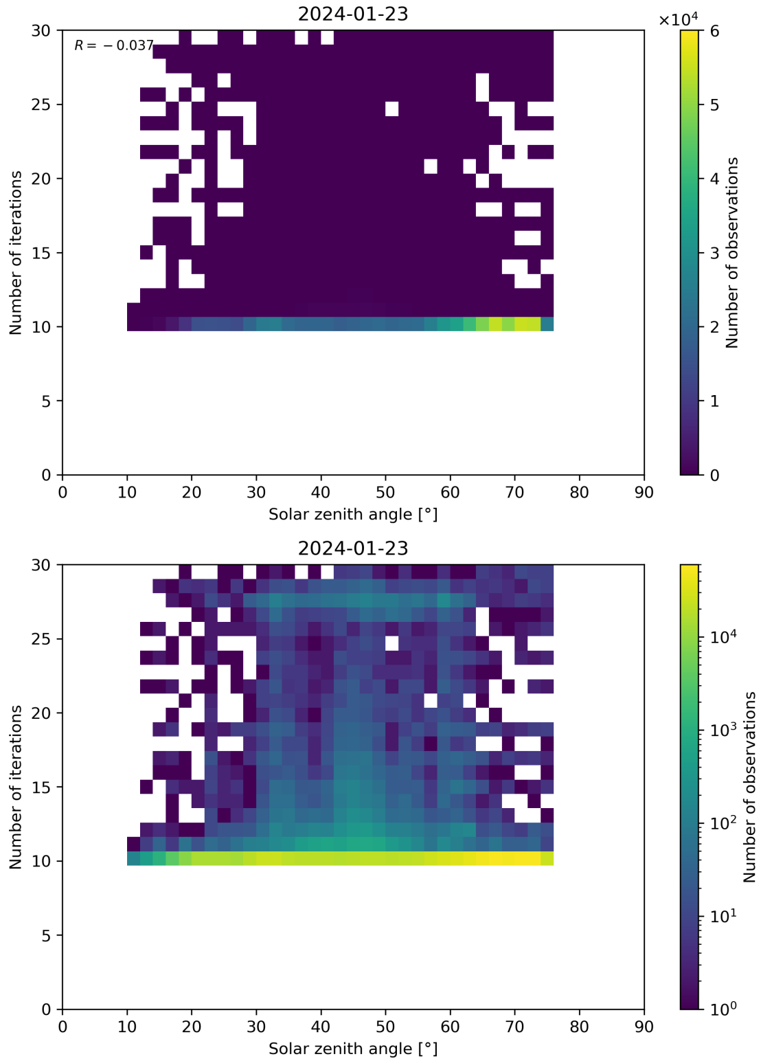
Figure 102: Scatter density plot of “Solar zenith angle” against “Number of iterations” for 2024-01-22 to 2024-01-24.
