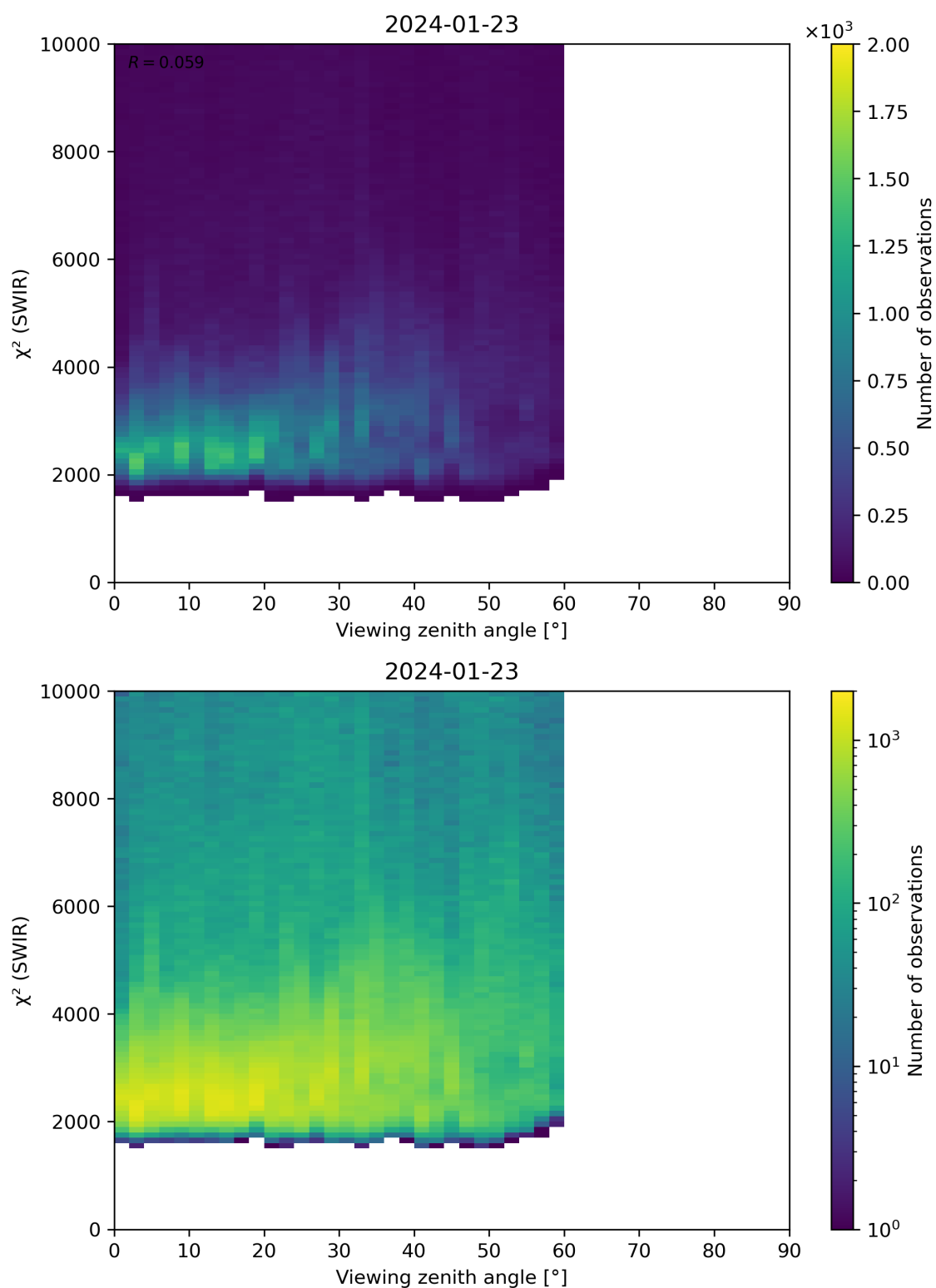
Figure 106: Scatter density plot of “Viewing zenith angle” against “ \chi^2 (SWIR)” for 2024-01-22 to 2024-01-24.
