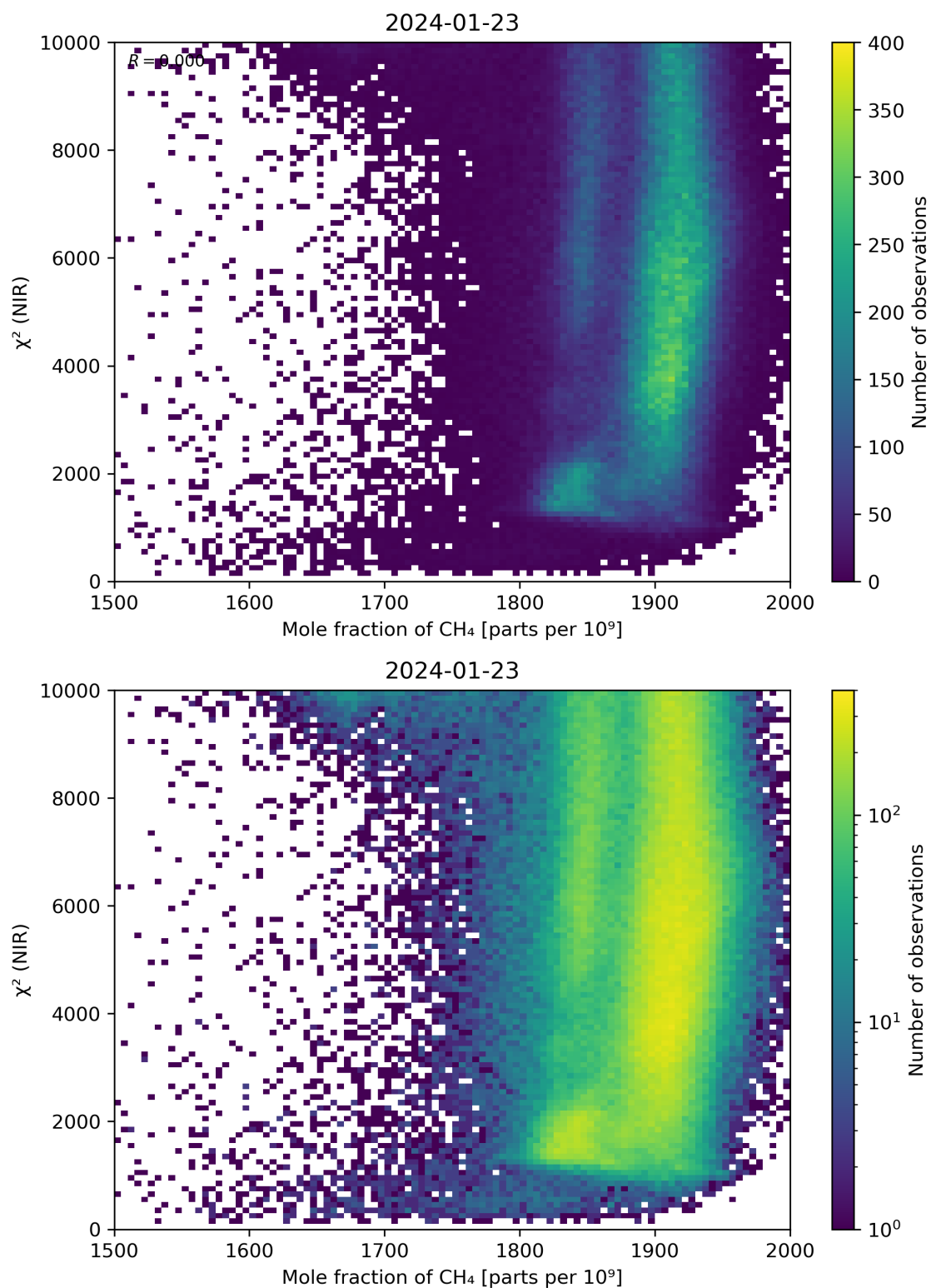
Figure 70: Scatter density plot of “Mole fraction of \text{CH}_4 ” against “ \chi^2 (NIR)” for 2024-01-22 to 2024-01-24.
