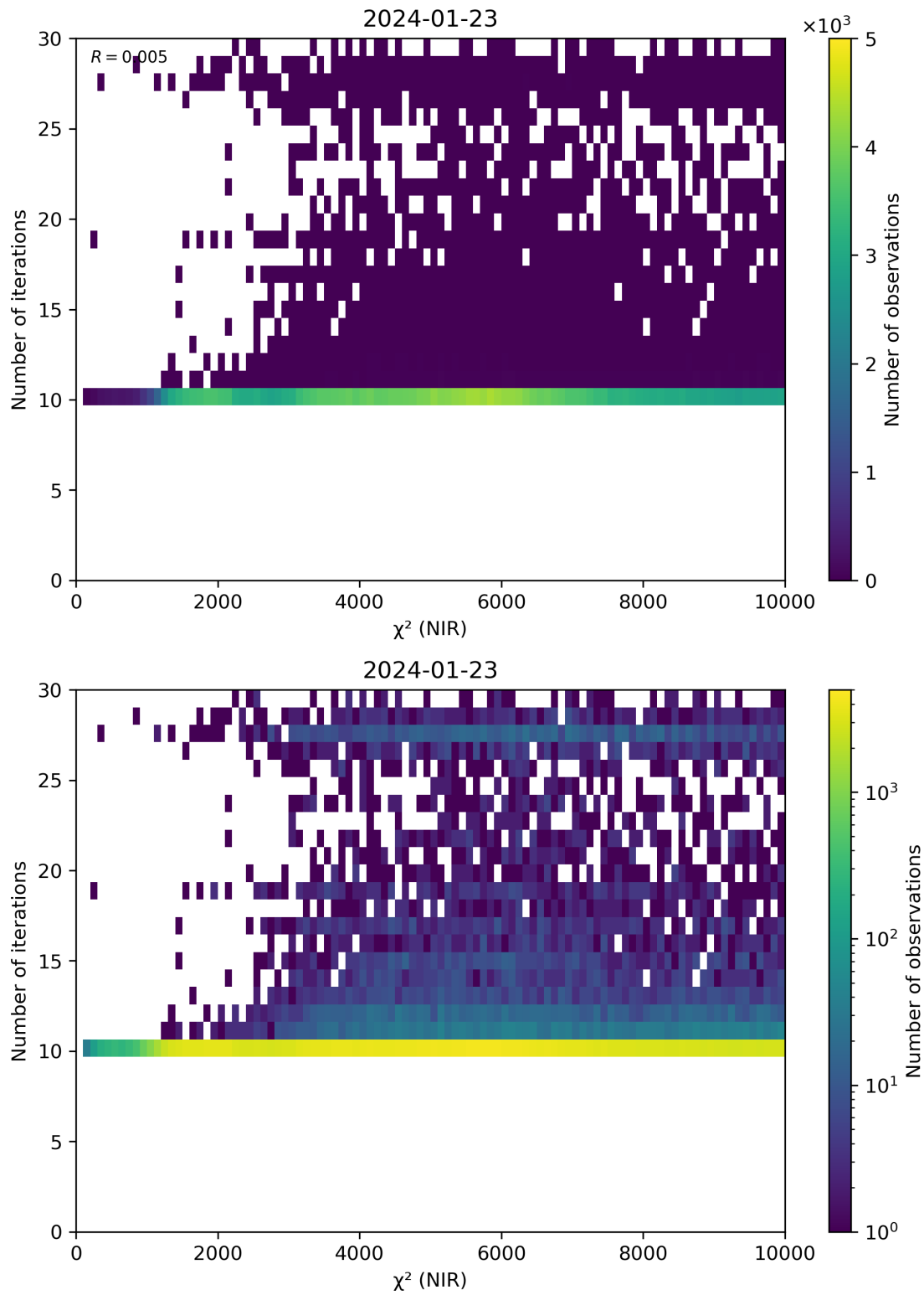
Figure 46: Scatter density plot of “ \chi^2 (NIR)” against “Number of iterations” for 2024-01-22 to 2024-01-24.
