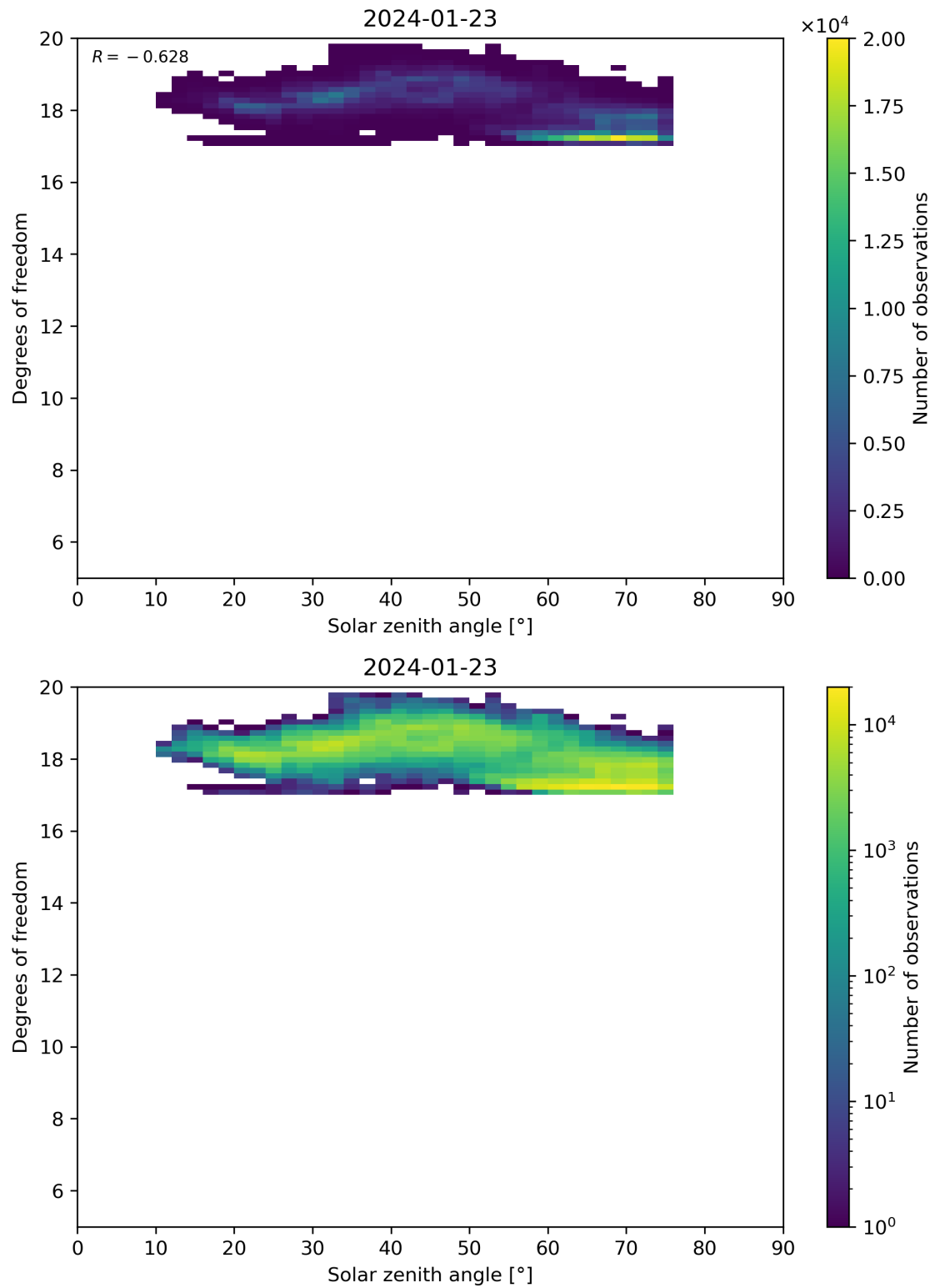
Figure 96: Scatter density plot of “Solar zenith angle” against “Degrees of freedom” for 2024-01-22 to 2024-01-24.
