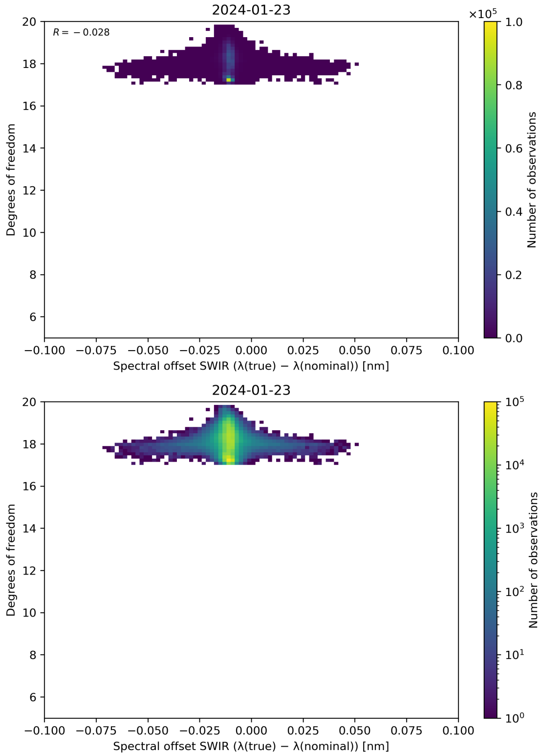
Figure 119: Scatter density plot of “Spectral offset SWIR ( \lambda(\text{true}) - \lambda(\text{nominal}) )” against “Degrees of freedom” for 2024-01-22 to 2024-01-24.
