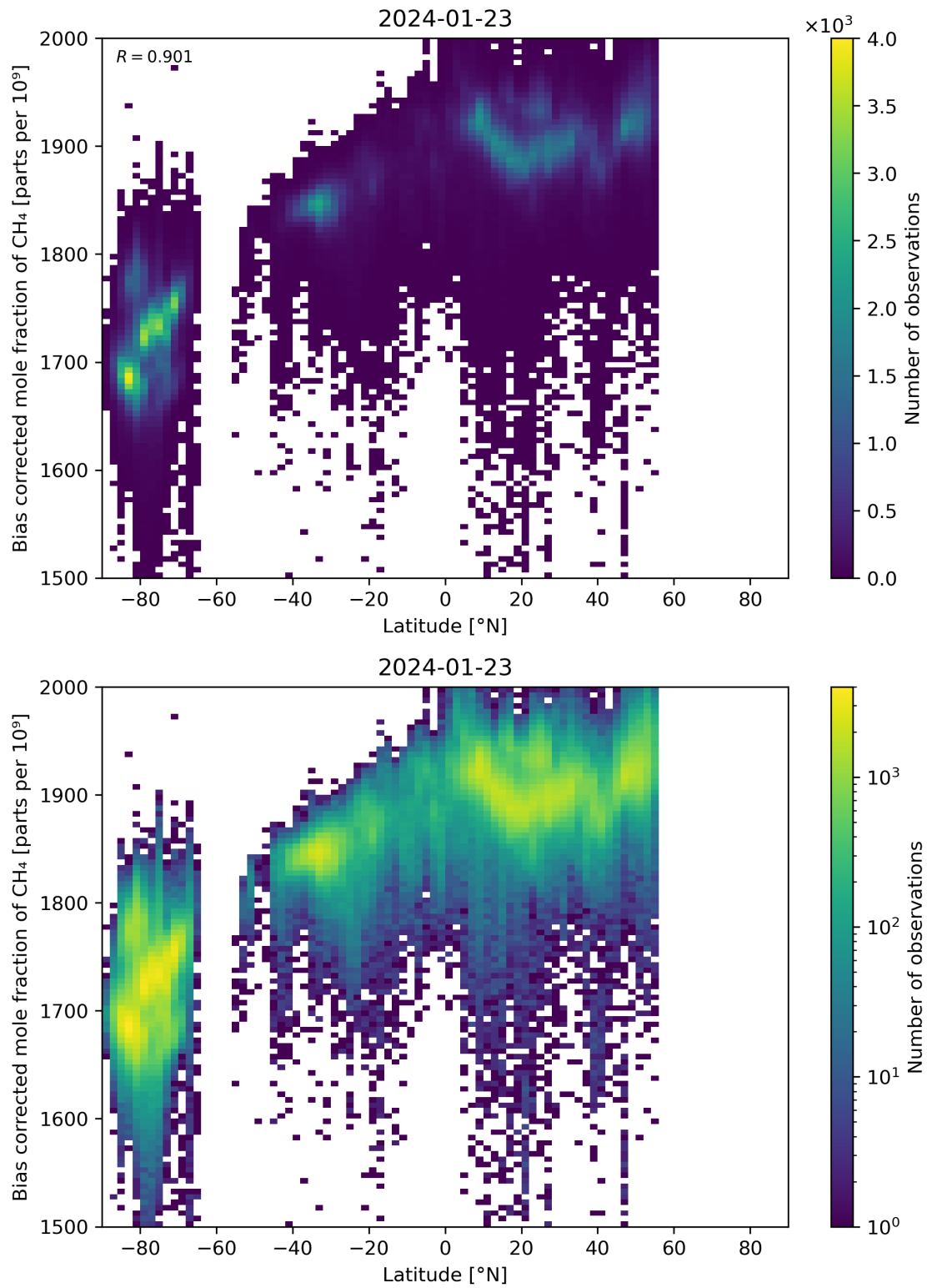
Figure 58: Scatter density plot of “Latitude” against “Bias corrected mole fraction of CH 4 ” for 2024-01-22 to 2024-01-24.
