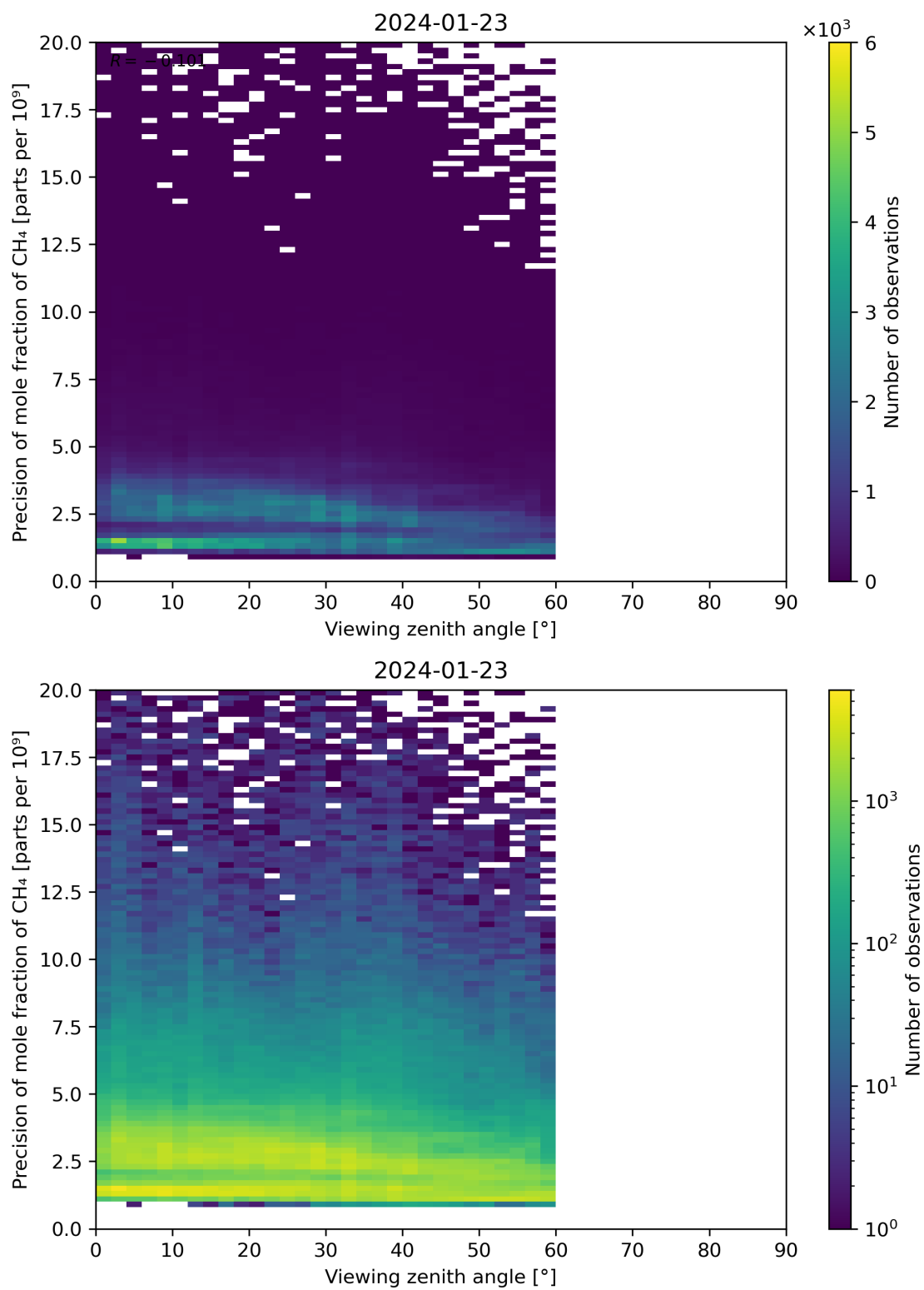
Figure 112: Scatter density plot of “Viewing zenith angle” against “Precision of mole fraction of CH 4 ” for 2024-01-22 to 2024-01-24.
