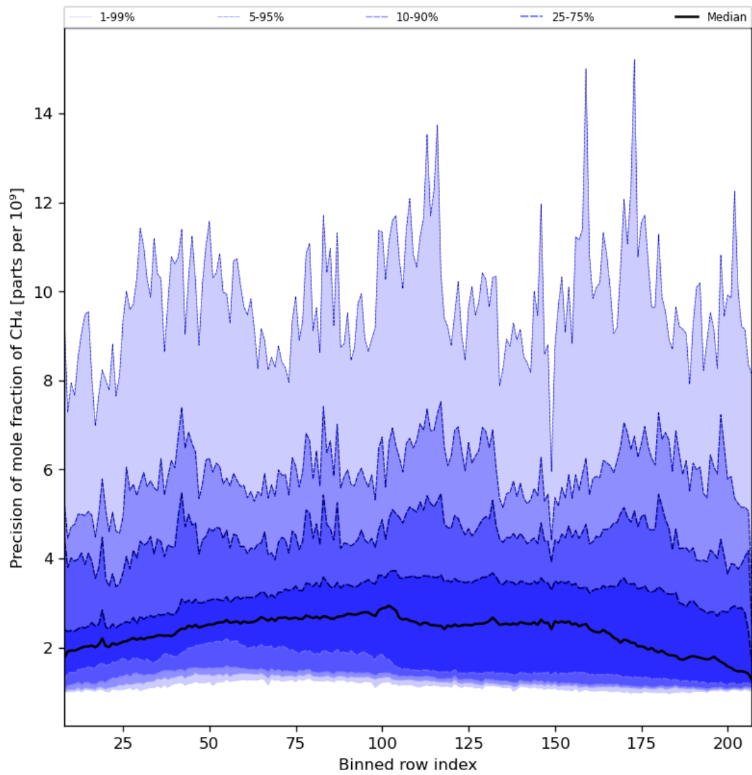
Figure 35: Along track statistics of “Precision of mole fraction of CH 4 ” for 2024-01-22 to 2024-01-24
