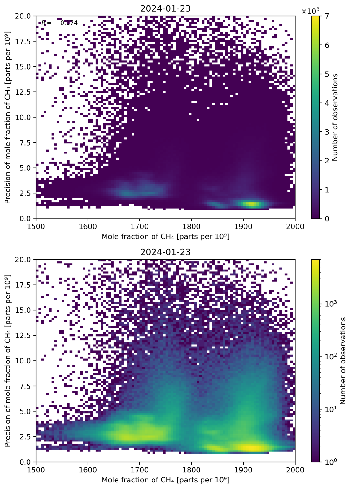
Figure 75: Scatter density plot of “Mole fraction of CH 4 ” against “Precision of mole fraction of CH 4 ” for 2024-01-22 to 2024-01-24.
