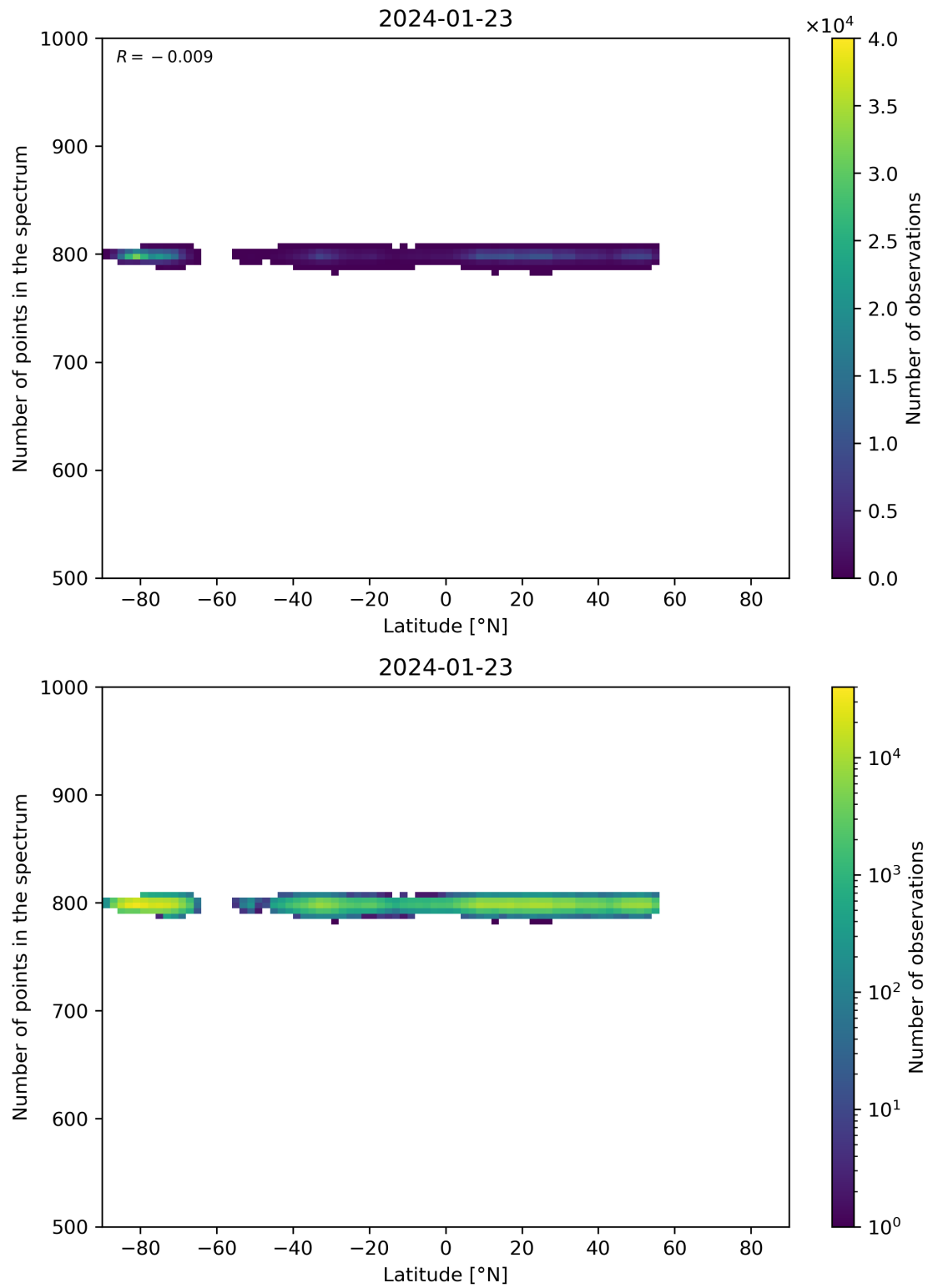
Figure 61: Scatter density plot of “Latitude” against “Number of points in the spectrum” for 2024-01-22 to 2024-01-24.
