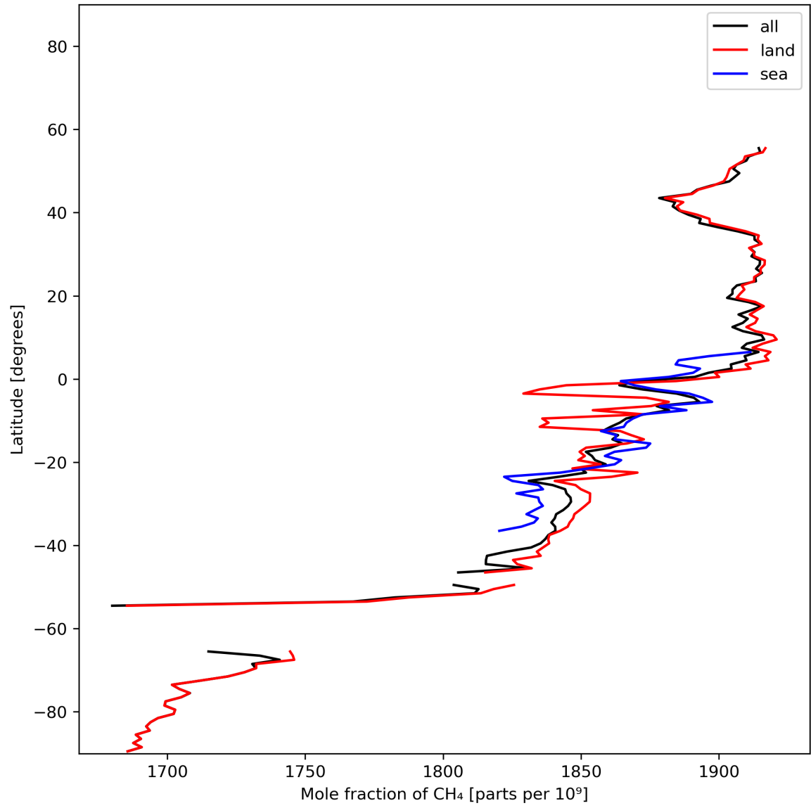
Figure 12: Zonal average of “Mole fraction of \text{CH}_4 ” for 2024-01-22 to 2024-01-24.
