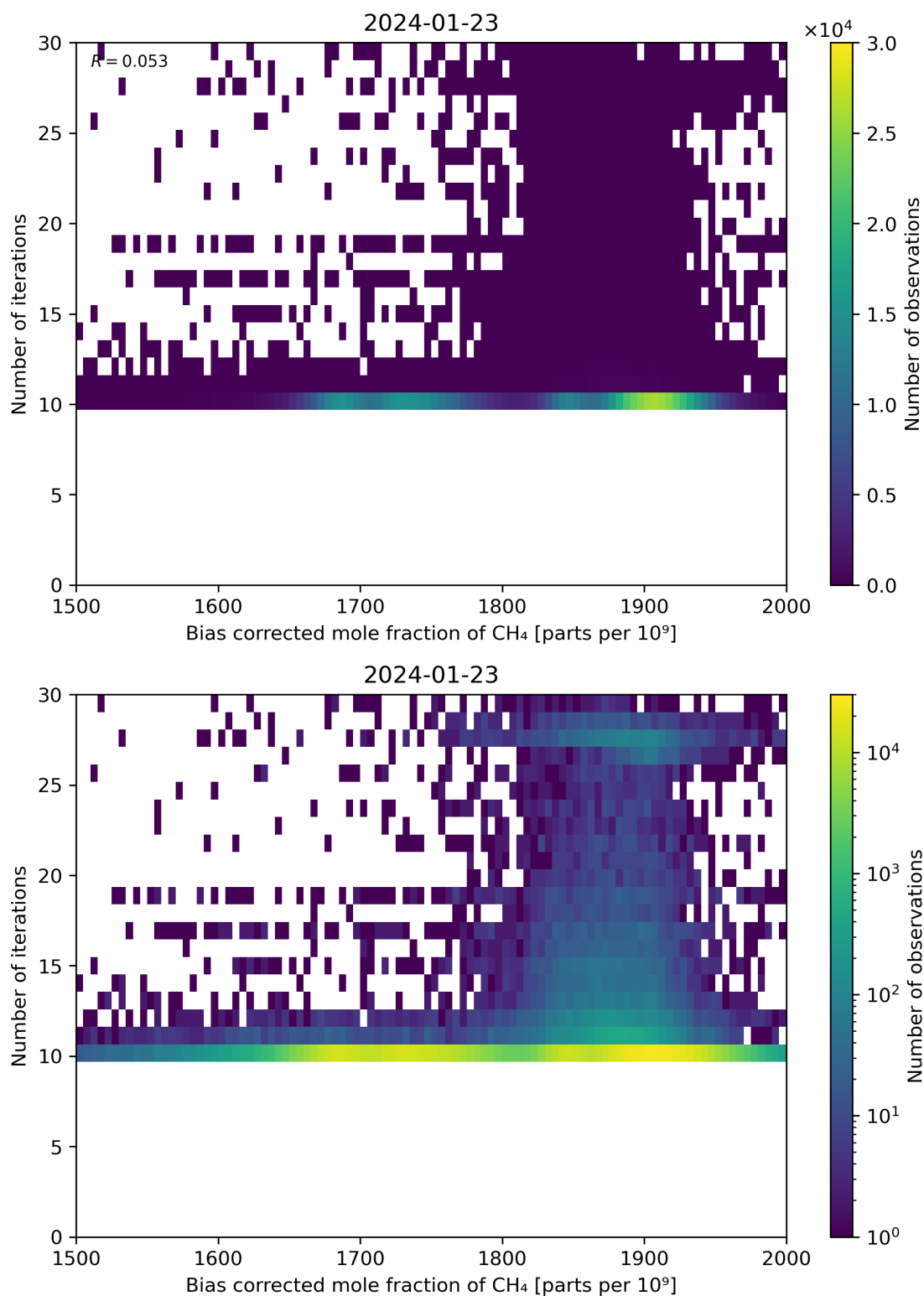
Figure 67: Scatter density plot of “Bias corrected mole fraction of \text{CH}_4 ” against “Number of iterations” for 2024-01-22 to 2024-01-24.
