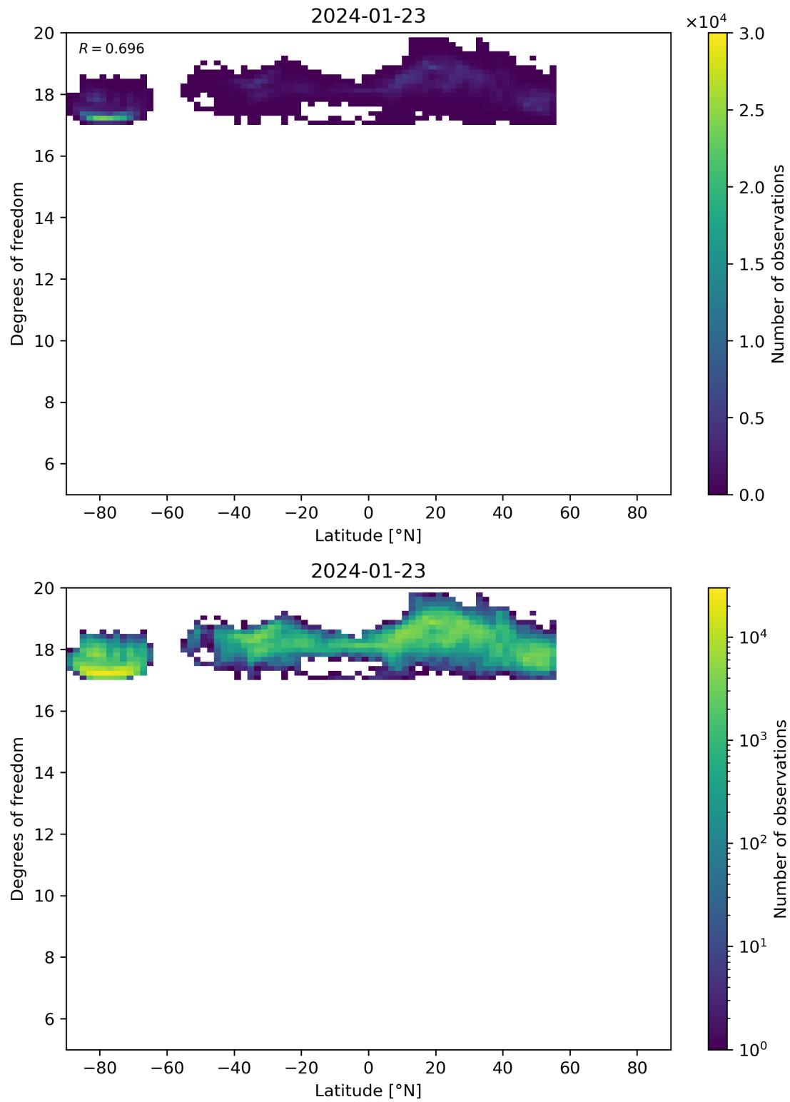
Figure 55: Scatter density plot of “Latitude” against “Degrees of freedom” for 2024-01-22 to 2024-01-24.
