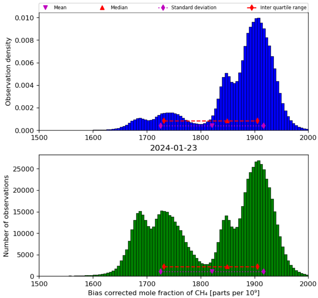
Figure 25: Histogram of “Bias corrected mole fraction of CH 4 ” for 2024-01-22 to 2024-01-24
