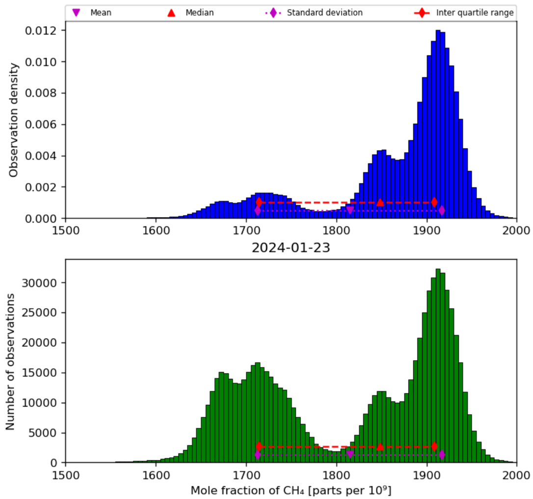
Figure 23: Histogram of “Mole fraction of CH 4 ” for 2024-01-22 to 2024-01-24
