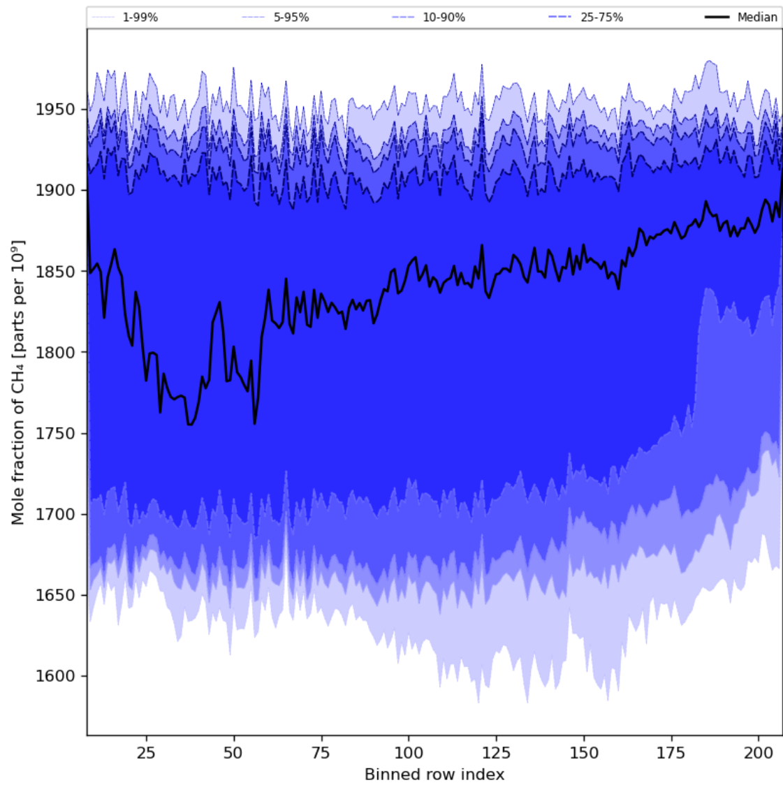
Figure 34: Along track statistics of “Mole fraction of CH 4 ” for 2024-01-22 to 2024-01-24
