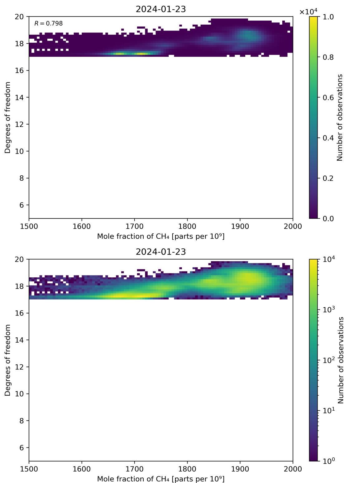
Figure 72: Scatter density plot of “Mole fraction of CH 4 ” against “Degrees of freedom” for 2024-01-22 to 2024-01-24.
