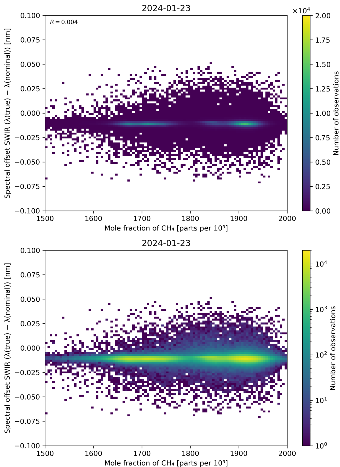
Figure 86: Scatter density plot of “Mole fraction of CH 4 ” against “Spectral offset SWIR ( \lambda(\text{true}) - \lambda(\text{nominal}) )” for 2024-01-22 to 2024-01-24.
