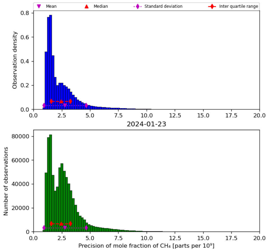
Figure 24: Histogram of “Precision of mole fraction of CH 4 ” for 2024-01-22 to 2024-01-24
