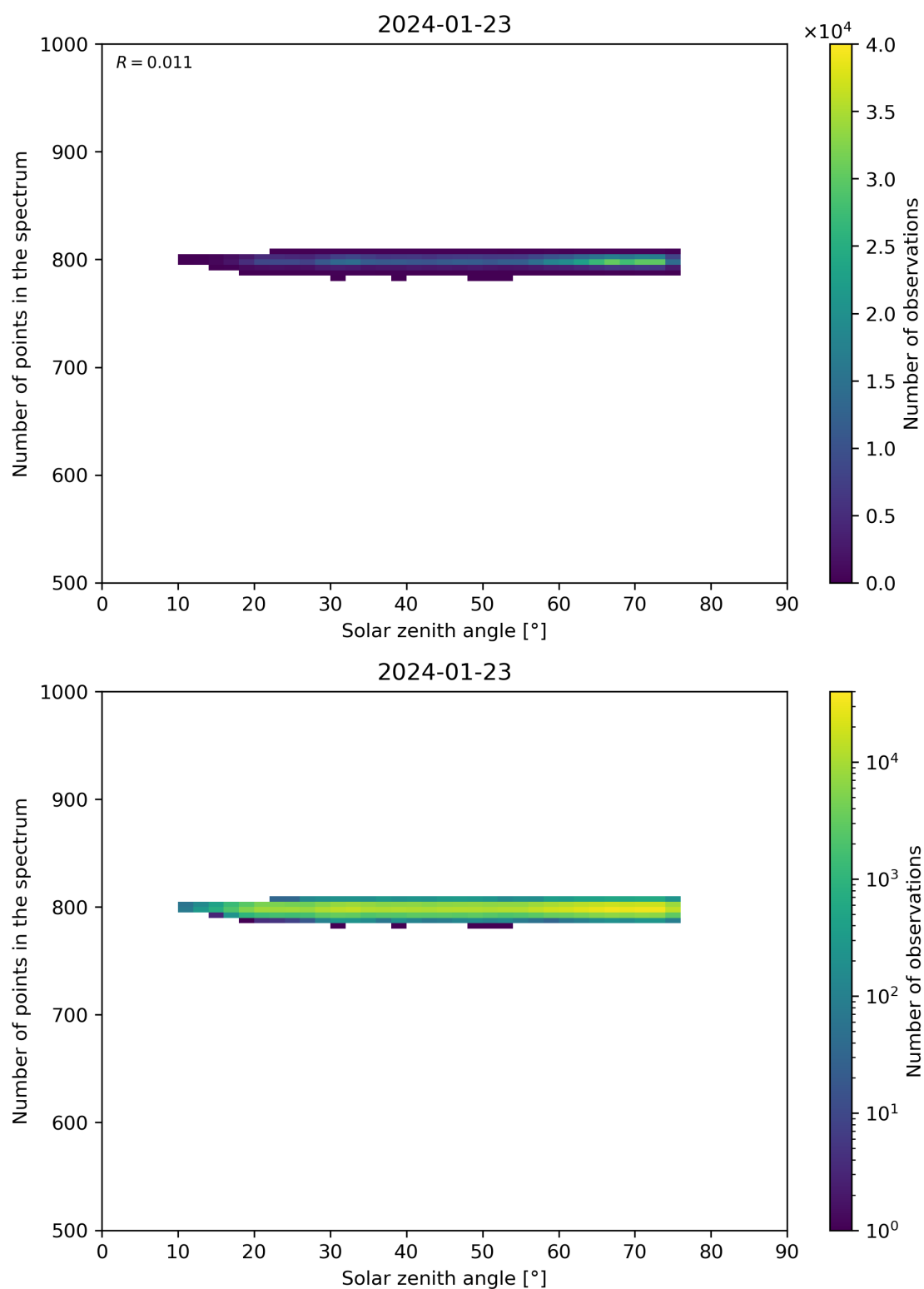
Figure 103: Scatter density plot of “Solar zenith angle” against “Number of points in the spectrum” for 2024-01-22 to 2024-01-24.
