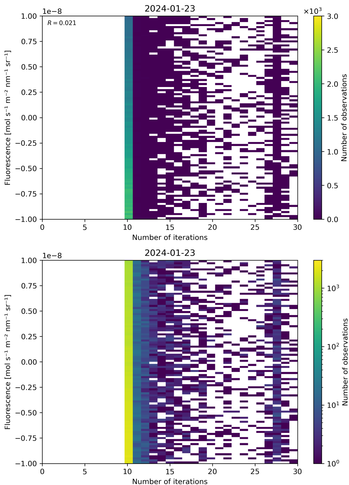
Figure 87: Scatter density plot of “Number of iterations” against “Fluorescence” for 2024-01-22 to 2024-01-24.
