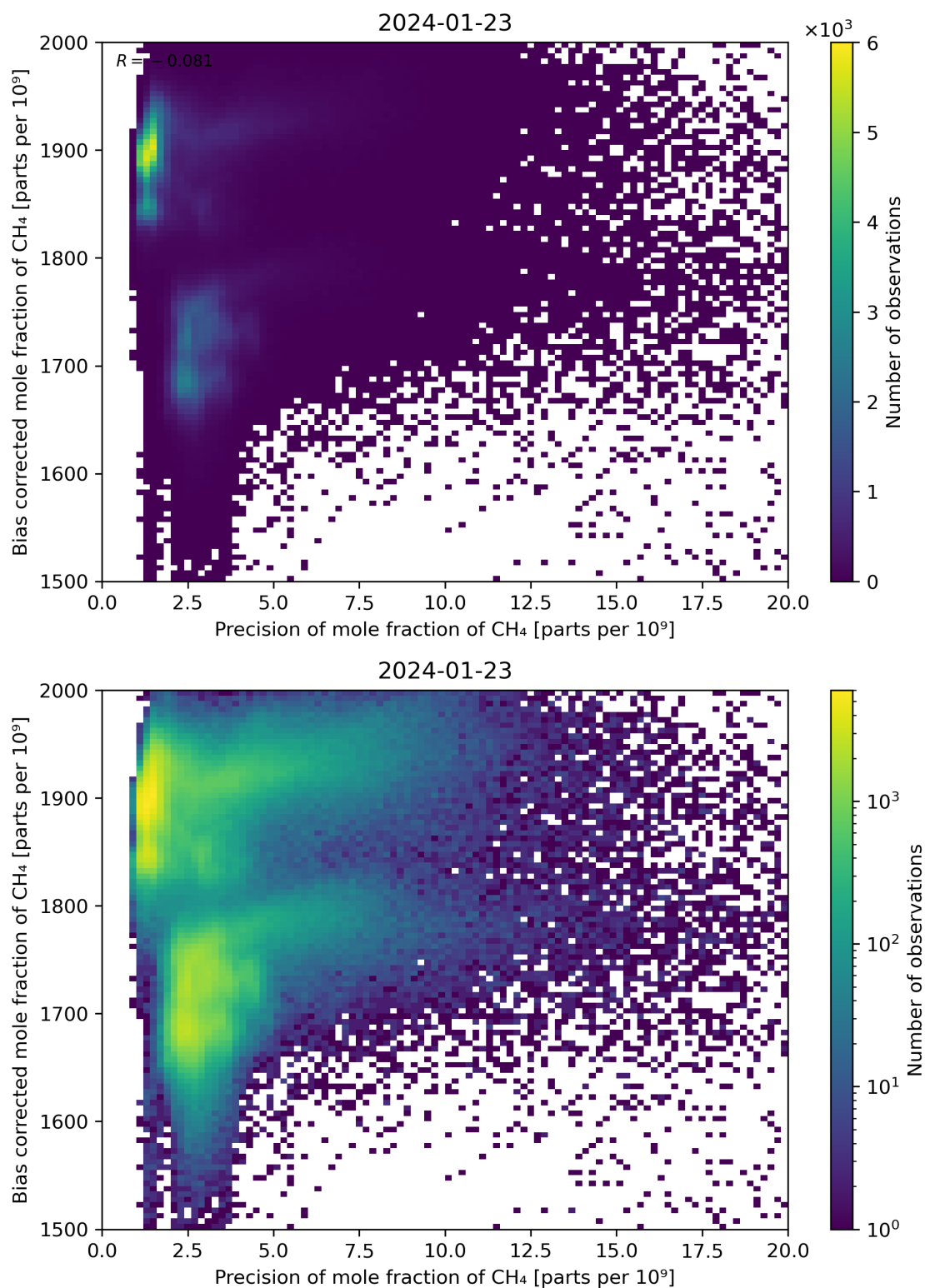
Figure 82: Scatter density plot of “Precision of mole fraction of \text{CH}_4 ” against “Bias corrected mole fraction of \text{CH}_4 ” for 2024-01-22 to 2024-01-24.
