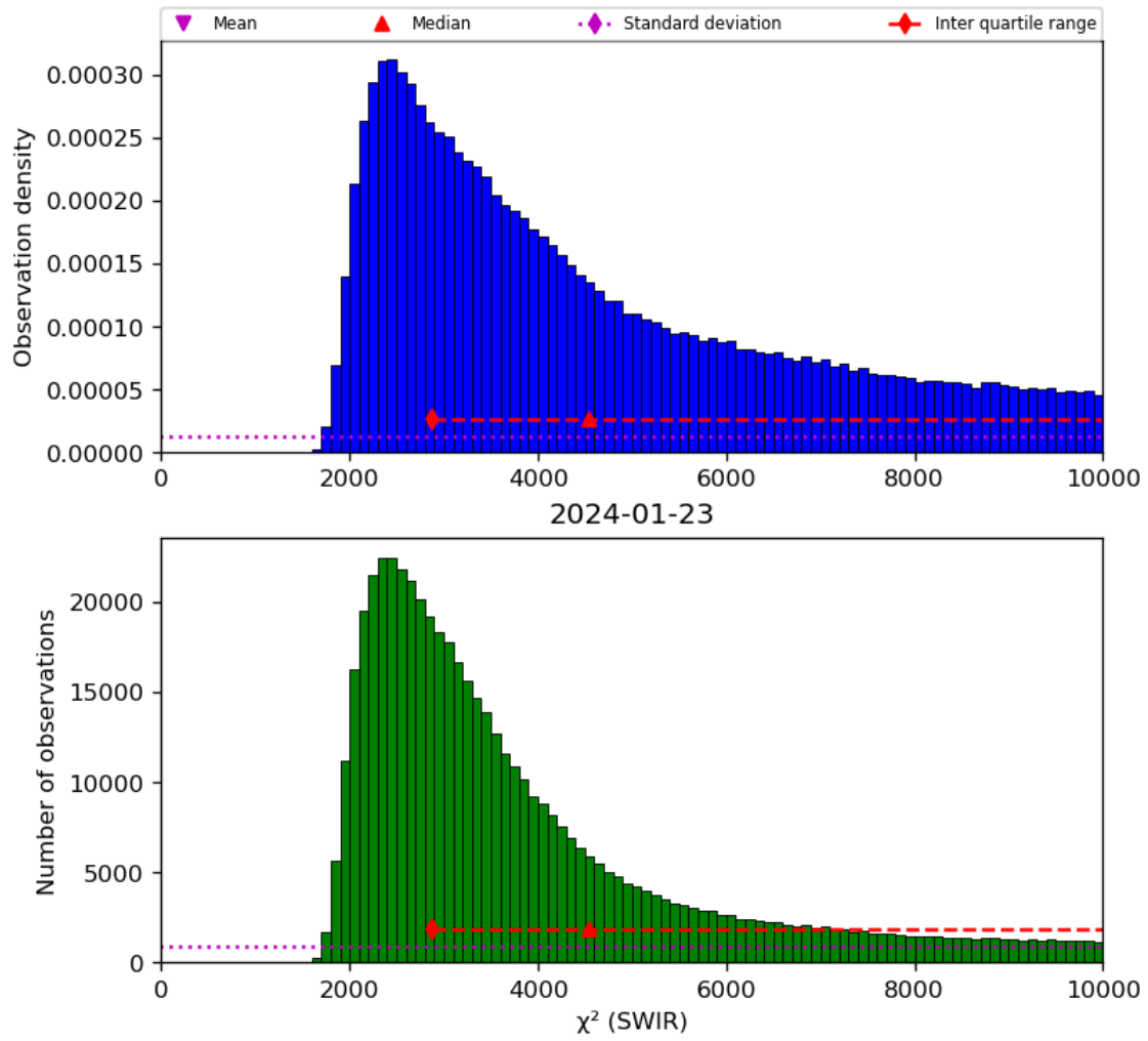
Figure 28: Histogram of “ \chi^2 (SWIR)” for 2024-01-22 to 2024-01-24
