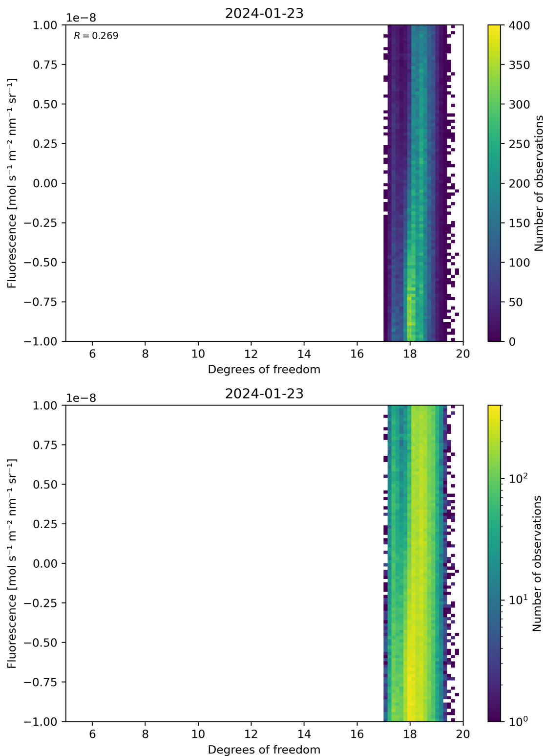
Figure 51: Scatter density plot of “Degrees of freedom” against “Fluorescence” for 2024-01-22 to 2024-01-24.
