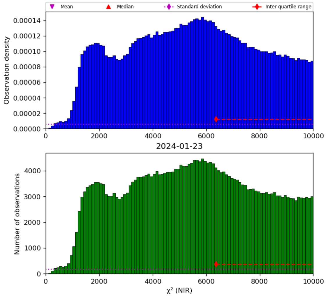
Figure 29: Histogram of " \chi^2 (NIR)" for 2024-01-22 to 2024-01-24
