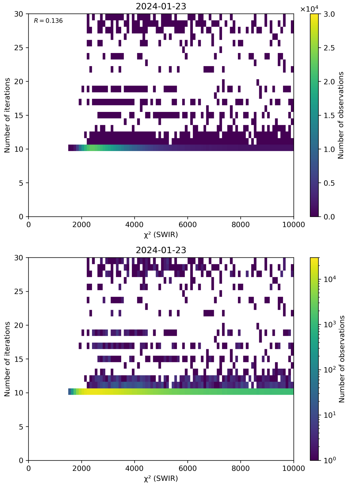
Figure 50: Scatter density plot of “ \chi^2 (SWIR)” against “Number of iterations” for 2024-01-22 to 2024-01-24.
