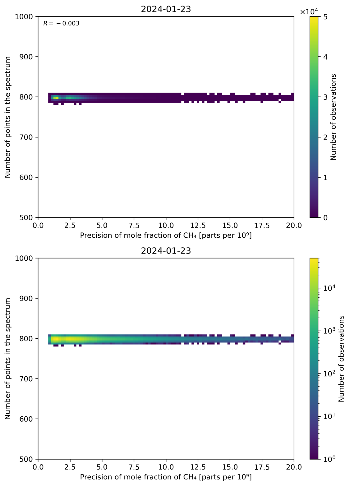
Figure 84: Scatter density plot of “Precision of mole fraction of CH 4 ” against “Number of points in the spectrum” for 2024-01-22 to 2024-01-24.
