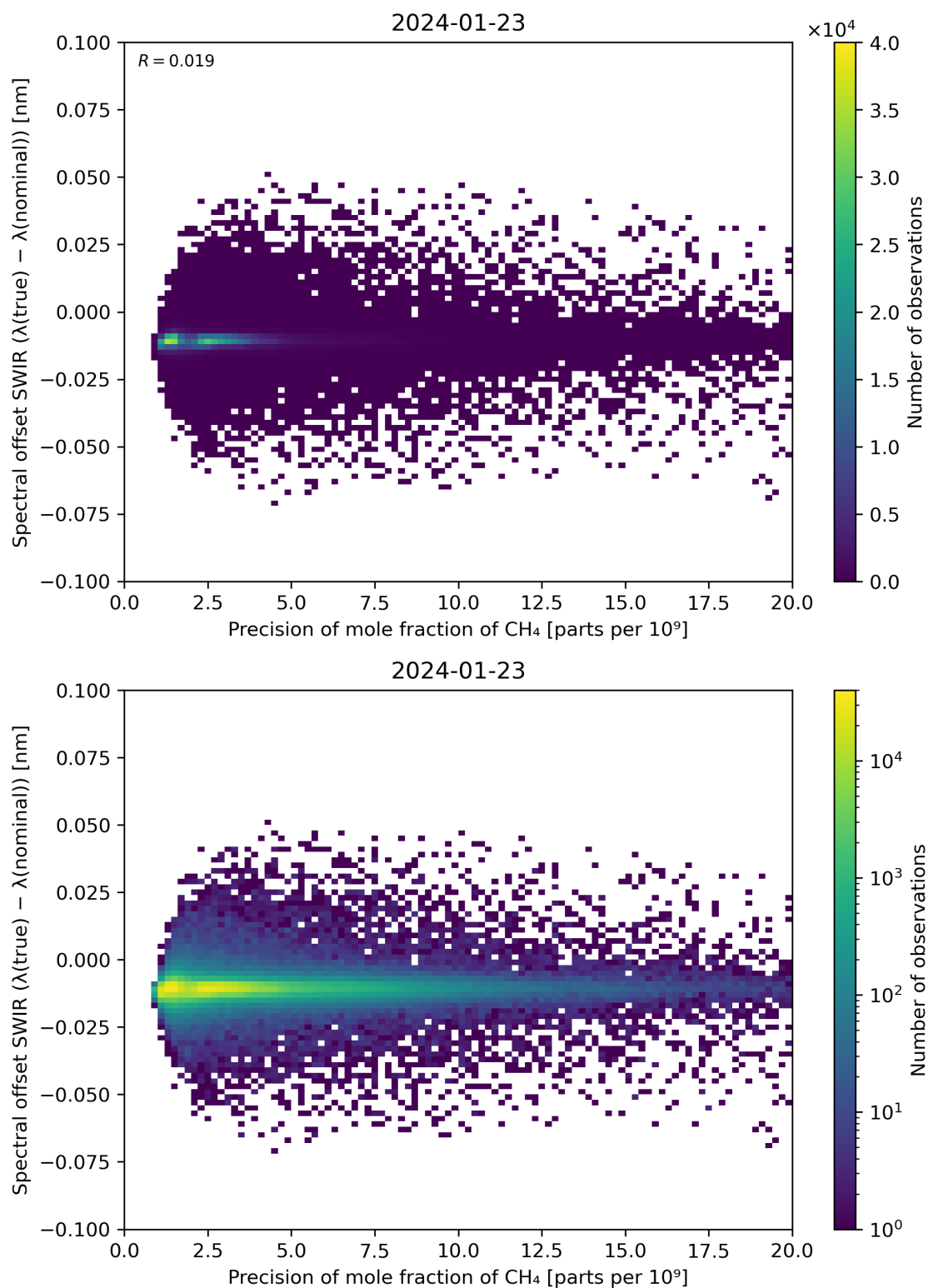
Figure 85: Scatter density plot of “Precision of mole fraction of \text{CH}_4 ” against “Spectral offset SWIR ( \lambda(\text{true}) - \lambda(\text{nominal}) )” for 2024-01-22 to 2024-01-24.
