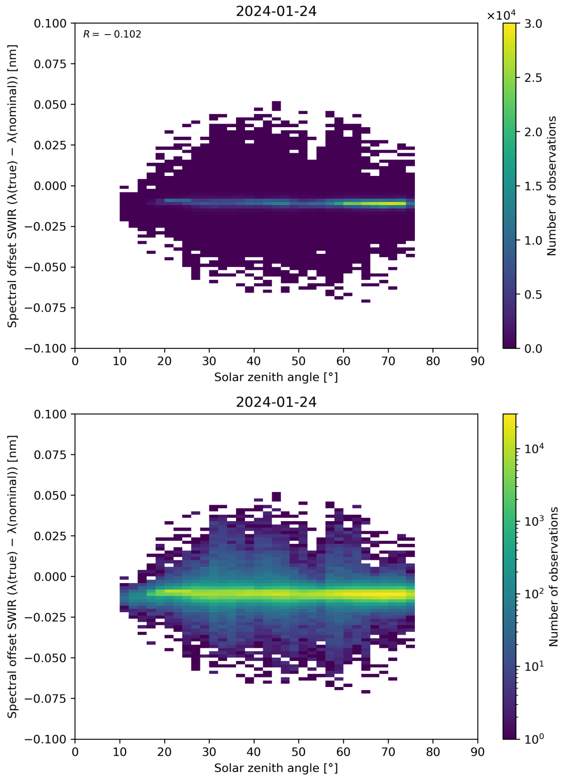
Figure 104: Scatter density plot of “Solar zenith angle” against “Spectral offset SWIR ( \lambda(\text{true}) - \lambda(\text{nominal}) )” for 2024-01-23 to 2024-01-25.
