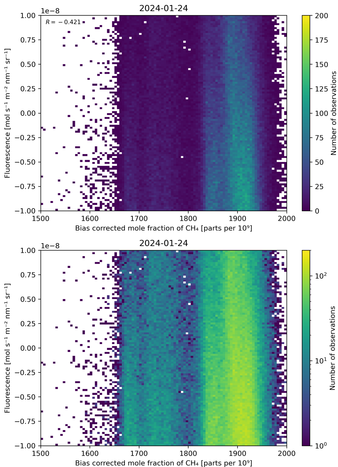
Figure 66: Scatter density plot of “Bias corrected mole fraction of CH 4 ” against “Fluorescence” for 2024-01-23 to 2024-01-25.
