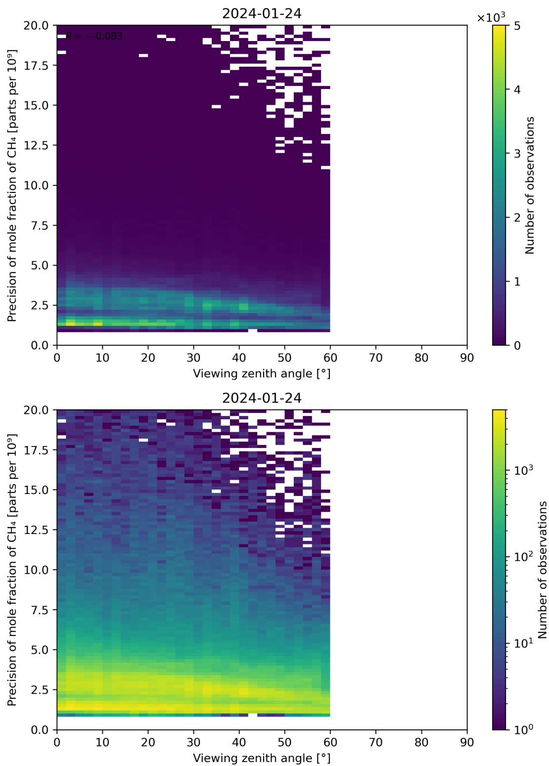
Figure 112: Scatter density plot of “Viewing zenith angle” against “Precision of mole fraction of CH 4 ” for 2024-01-23 to 2024-01-25.
