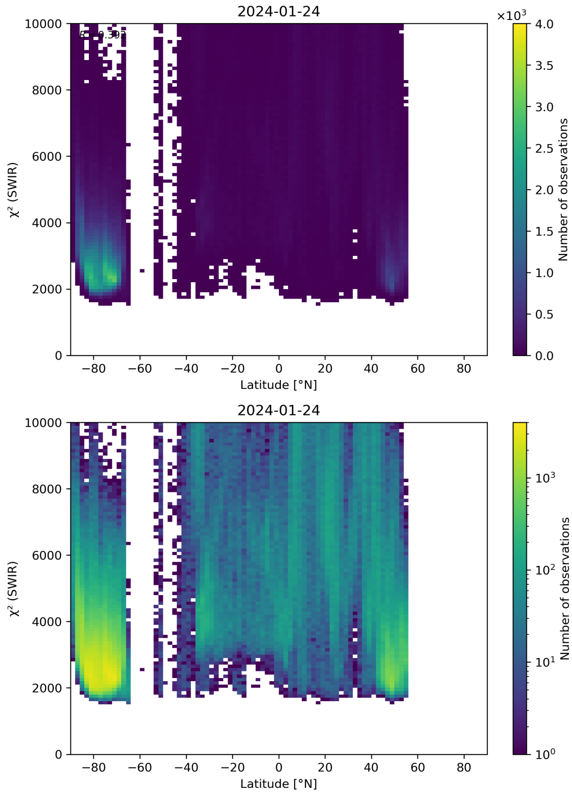
Figure 54: Scatter density plot of “Latitude” against “ \chi^2 (SWIR)” for 2024-01-23 to 2024-01-25.
