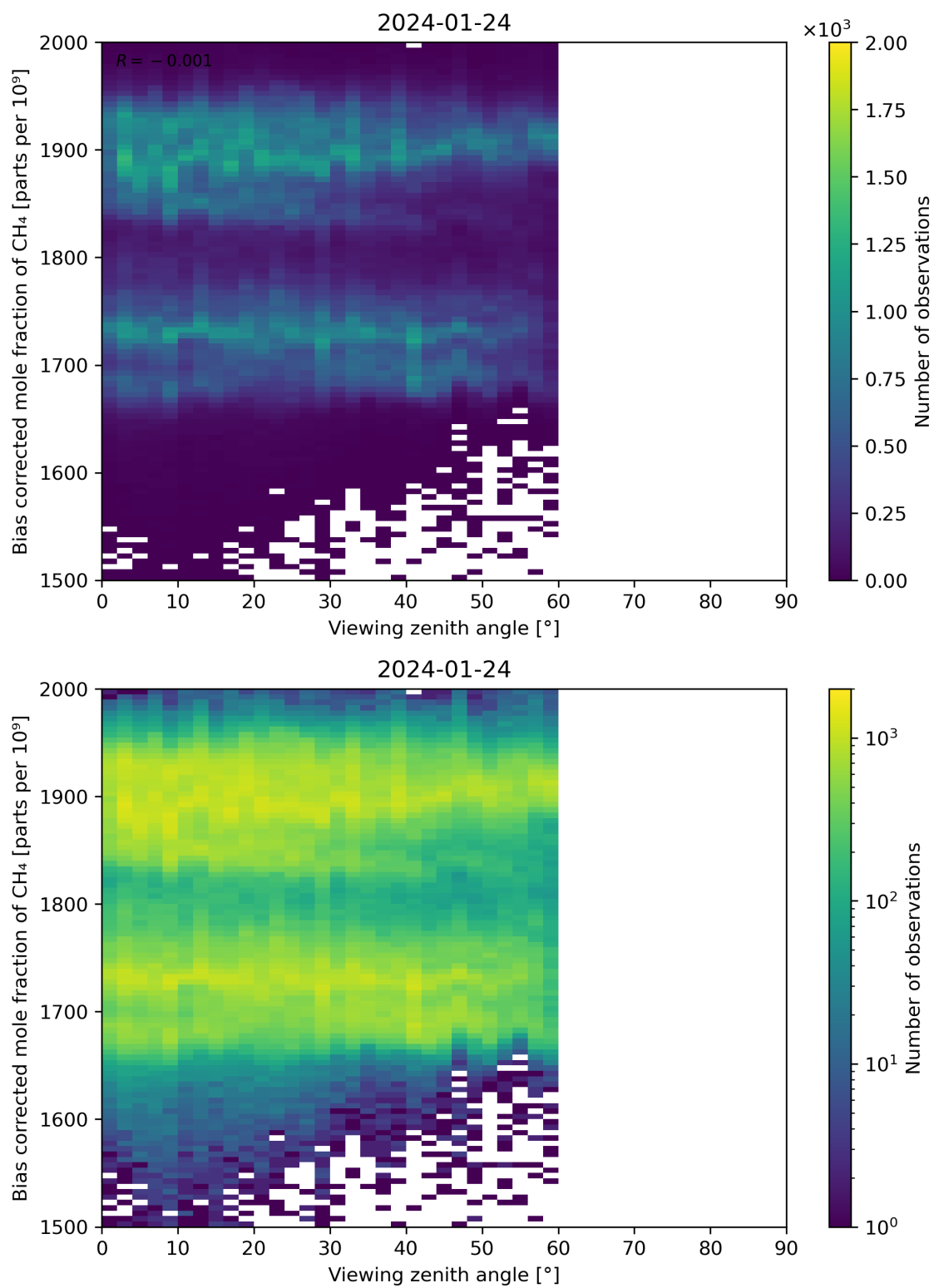
Figure 111: Scatter density plot of “Viewing zenith angle” against “Bias corrected mole fraction of CH 4 ” for 2024-01-23 to 2024-01-25.
