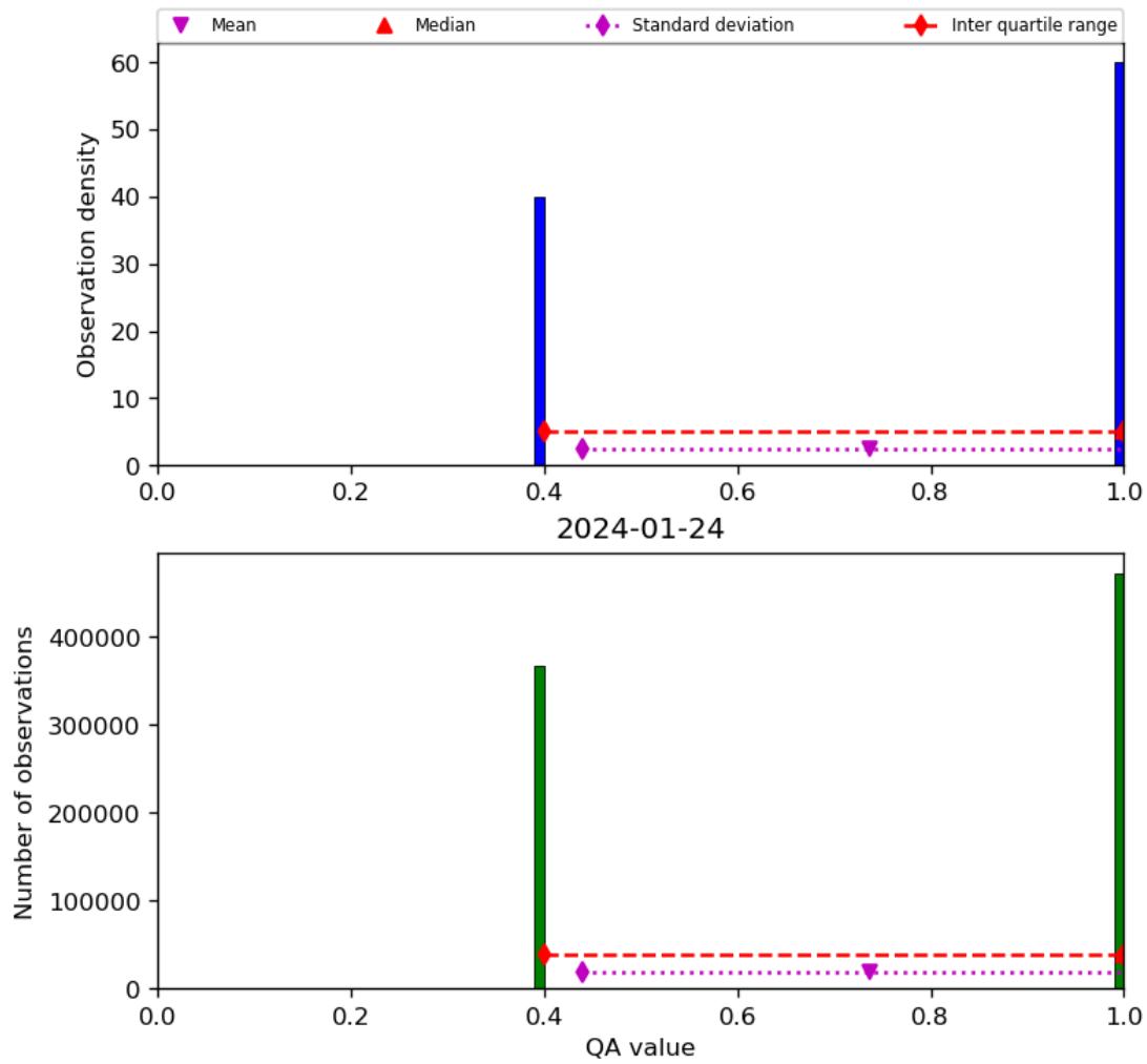
Figure 22: Histogram of “QA value” for 2024-01-23 to 2024-01-25
