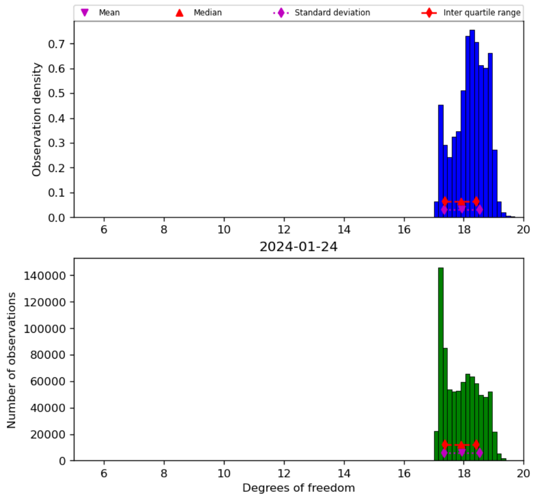
Figure 30: Histogram of “Degrees of freedom” for 2024-01-23 to 2024-01-25
