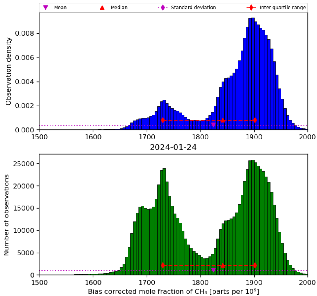
Figure 25: Histogram of “Bias corrected mole fraction of CH 4 ” for 2024-01-23 to 2024-01-25
