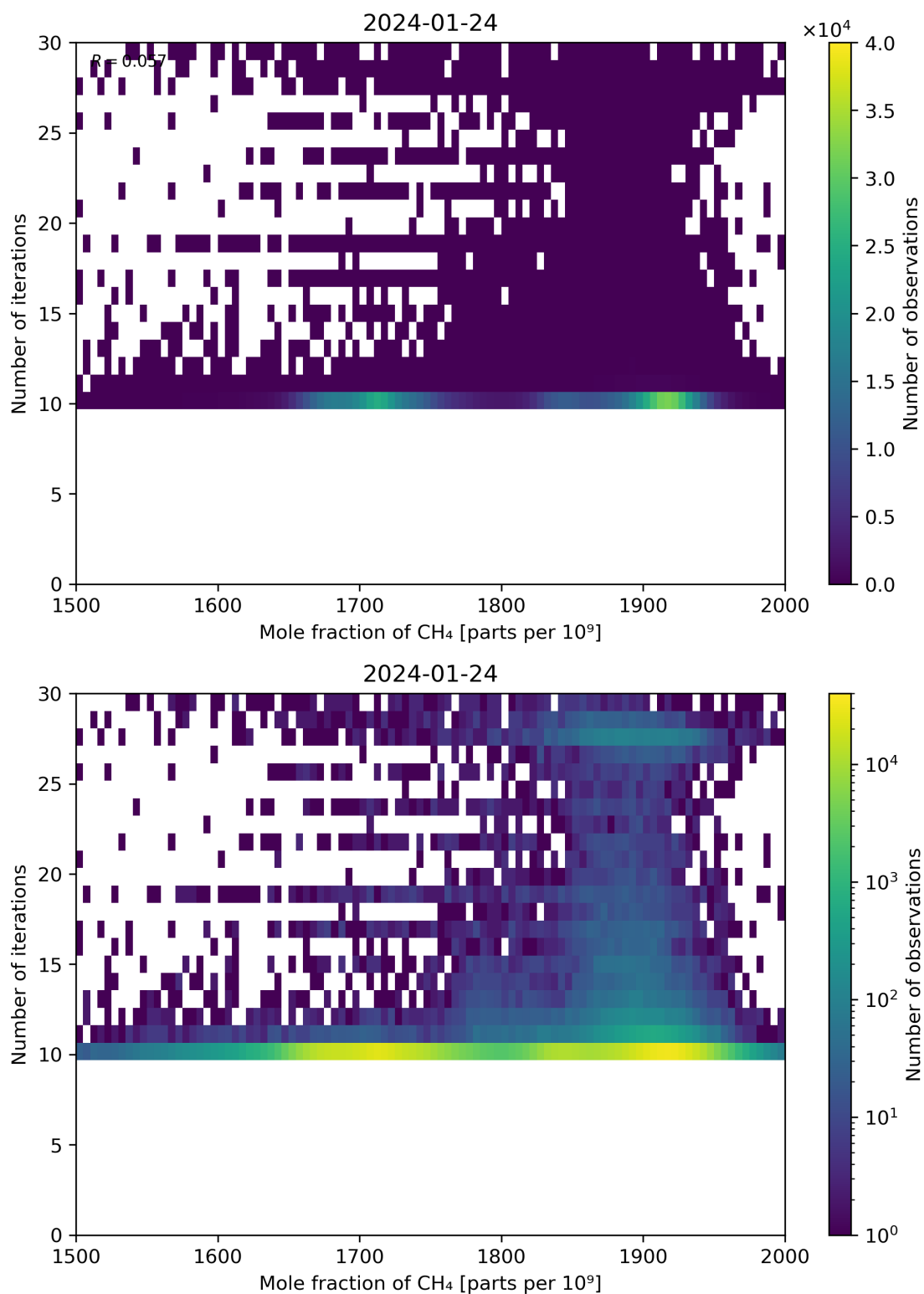
Figure 76: Scatter density plot of “Mole fraction of CH 4 ” against “Number of iterations” for 2024-01-23 to 2024-01-25.
