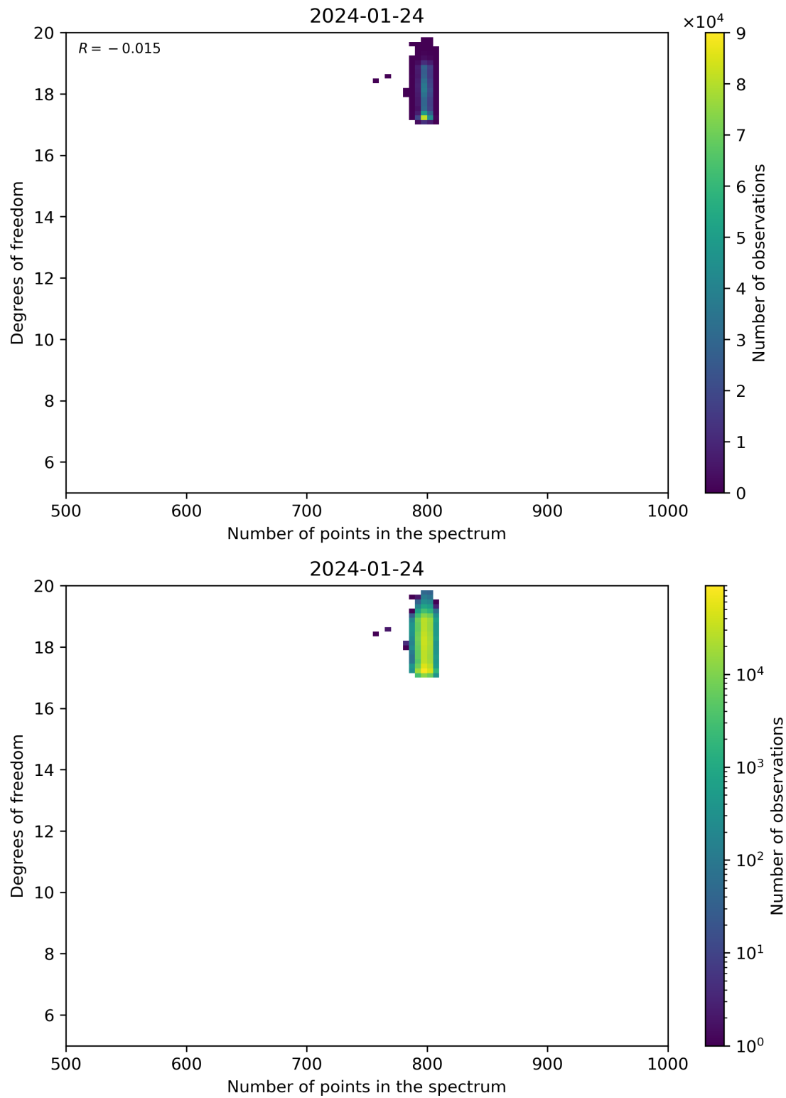
Figure 90: Scatter density plot of “Number of points in the spectrum” against “Degrees of freedom” for 2024-01-23 to 2024-01-25.
