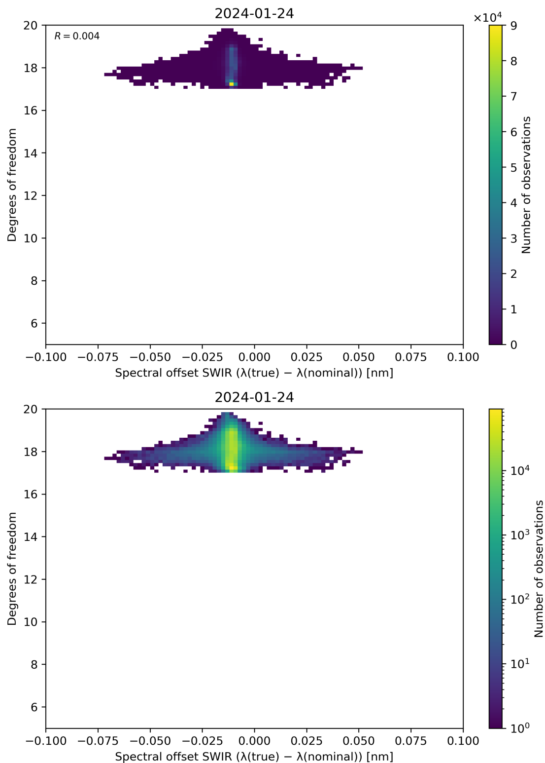
Figure 119: Scatter density plot of “Spectral offset SWIR ( \lambda(\text{true}) - \lambda(\text{nominal}) )” against “Degrees of freedom” for 2024-01-23 to 2024-01-25.
