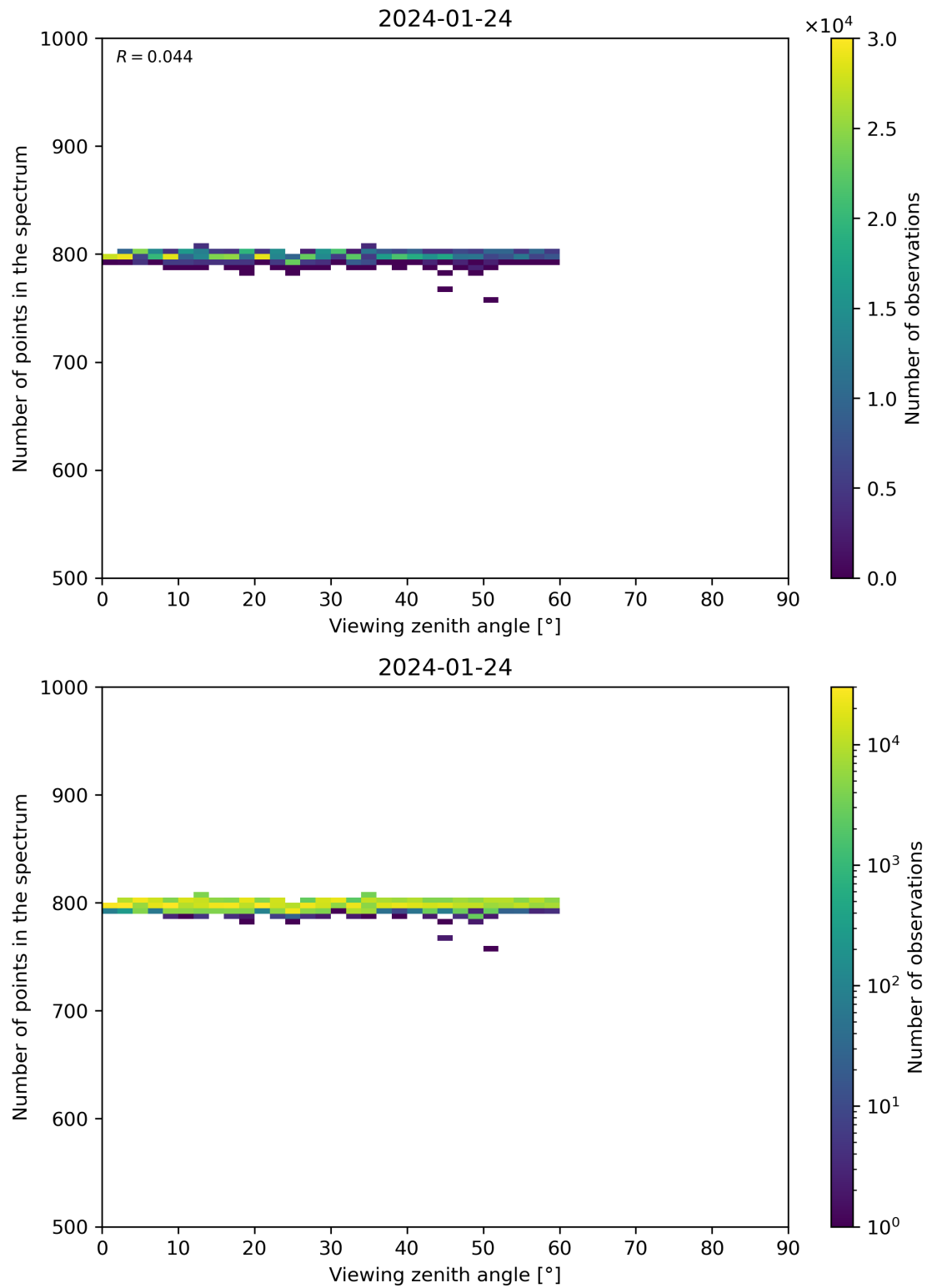
Figure 114: Scatter density plot of “Viewing zenith angle” against “Number of points in the spectrum” for 2024-01-23 to 2024-01-25.
