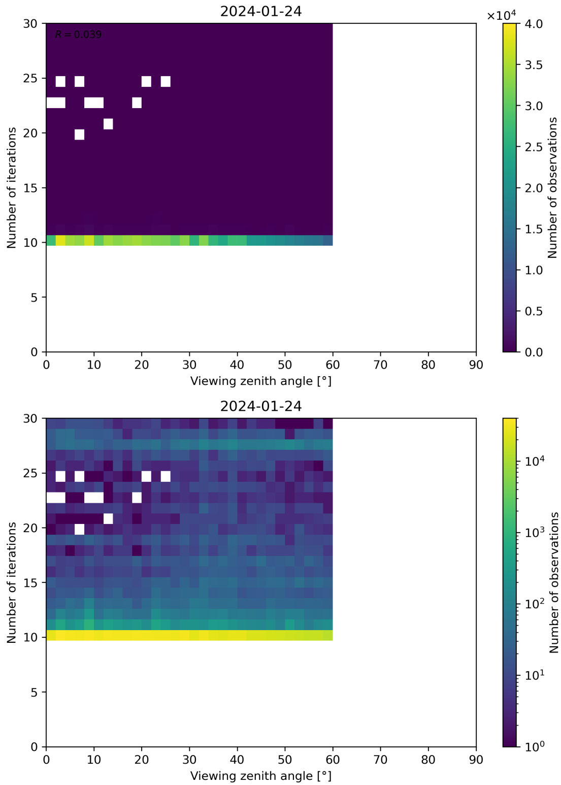
Figure 113: Scatter density plot of “Viewing zenith angle” against “Number of iterations” for 2024-01-23 to 2024-01-25.
