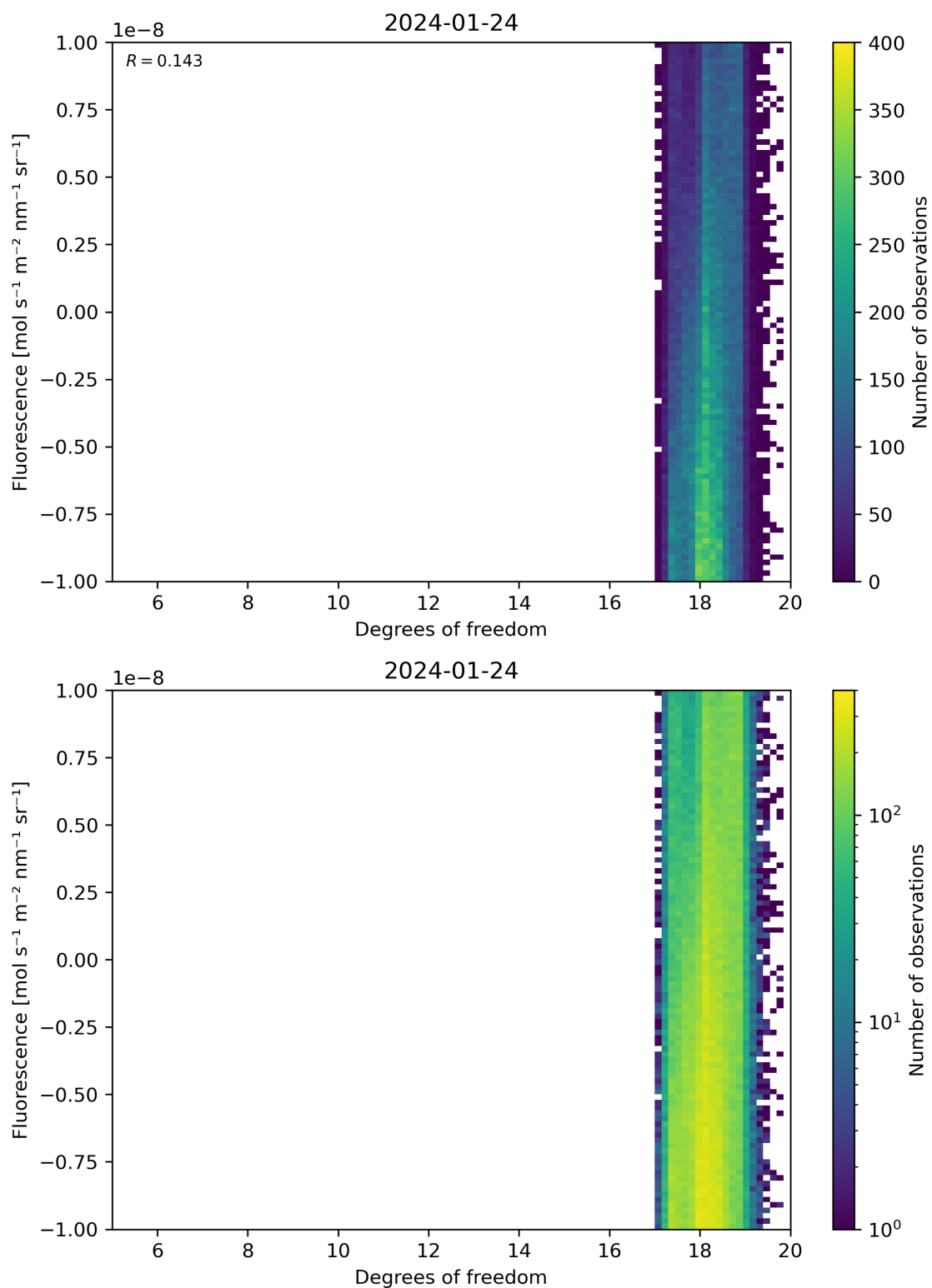
Figure 51: Scatter density plot of “Degrees of freedom” against “Fluorescence” for 2024-01-23 to 2024-01-25.
