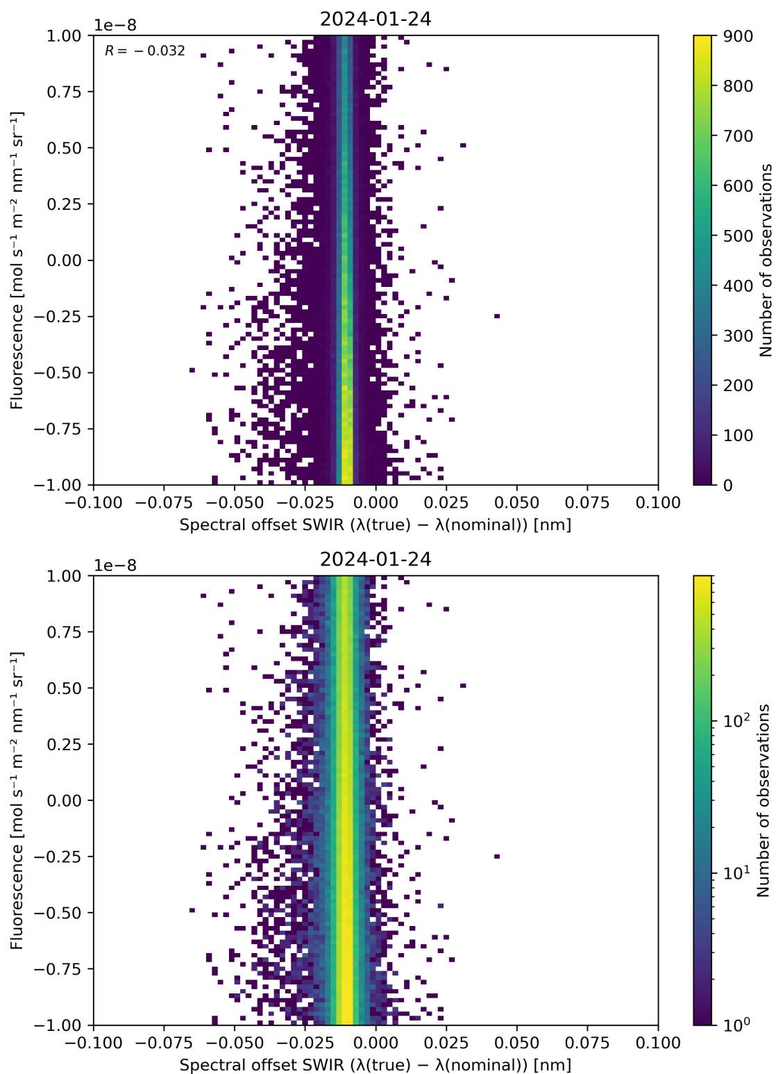
Figure 120: Scatter density plot of “Spectral offset SWIR ( \lambda(\text{true}) - \lambda(\text{nominal}) )” against “Fluorescence” for 2024-01-23 to 2024-01-25.
