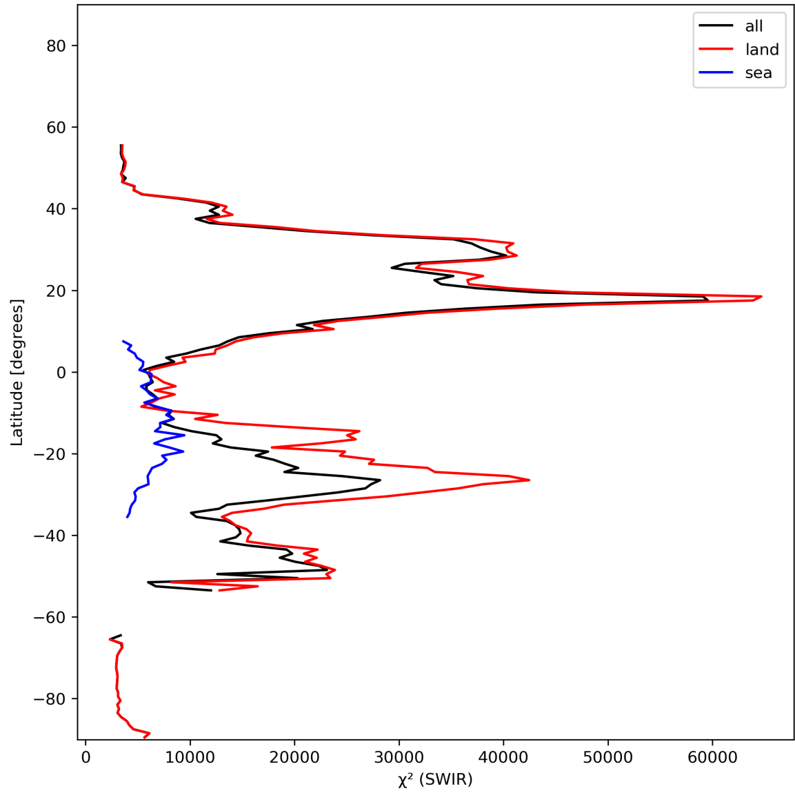
Figure 17: Zonal average of “ \chi^2 (SWIR)” for 2024-01-23 to 2024-01-25.
