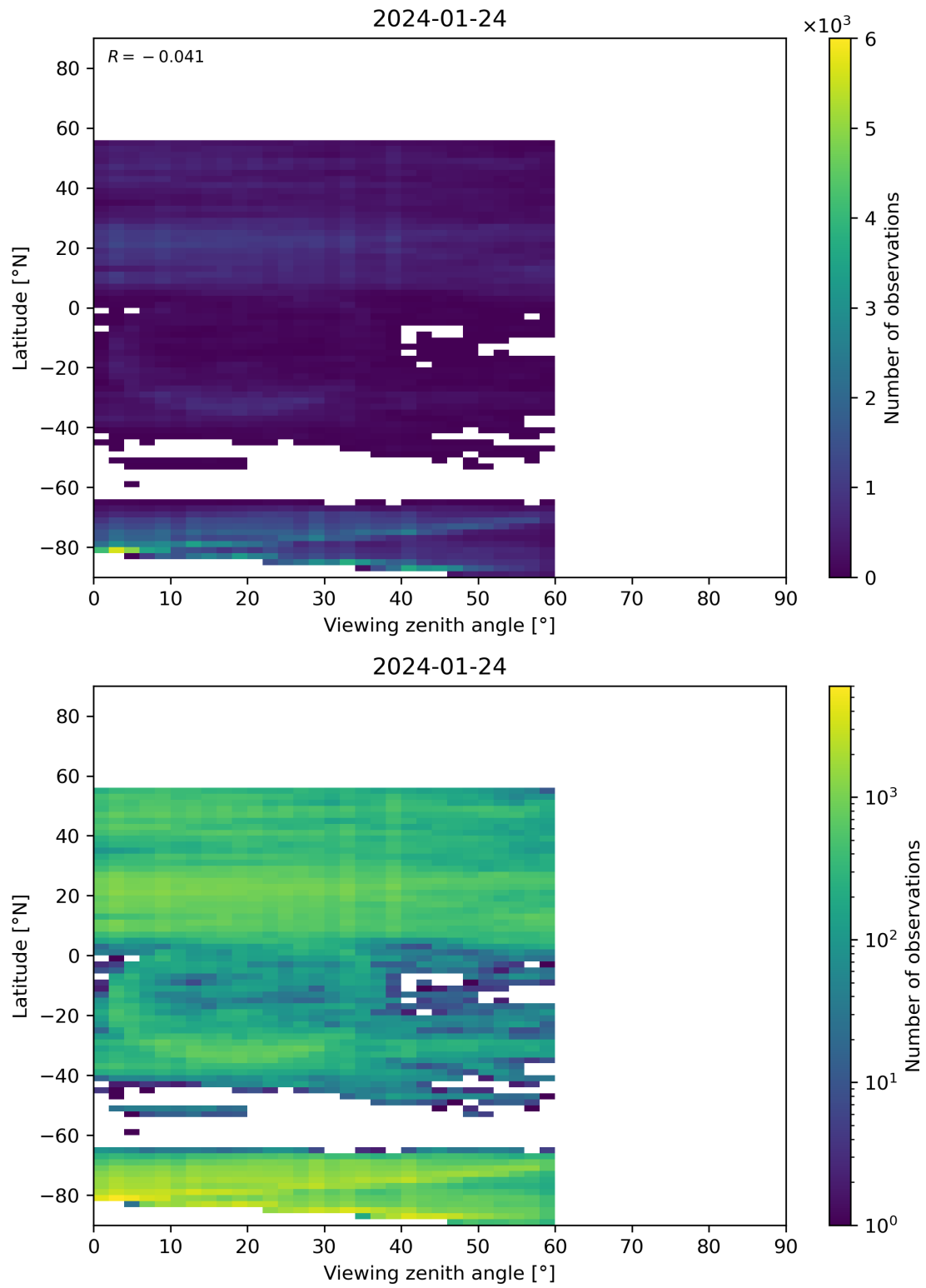
Figure 109: Scatter density plot of “Viewing zenith angle” against “Latitude” for 2024-01-23 to 2024-01-25.
