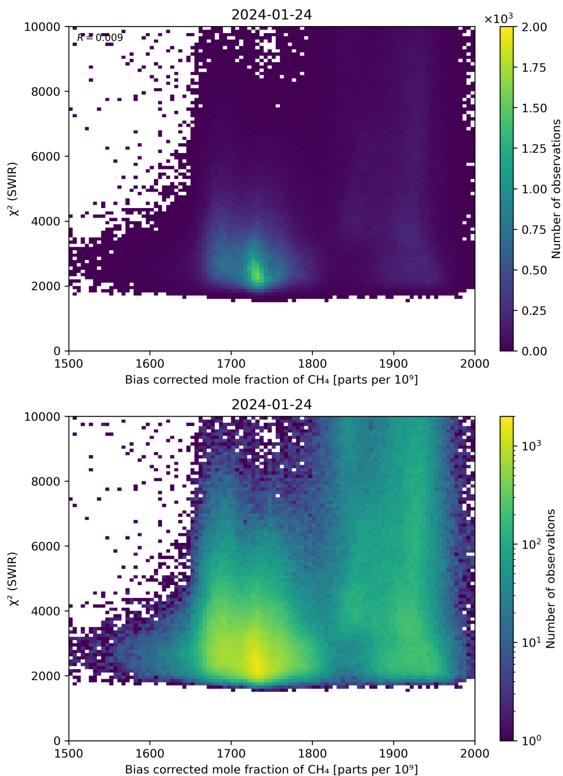
Figure 64: Scatter density plot of “Bias corrected mole fraction of CH 4 ” against “ \chi^2 (SWIR)” for 2024-01-23 to 2024-01-25.
