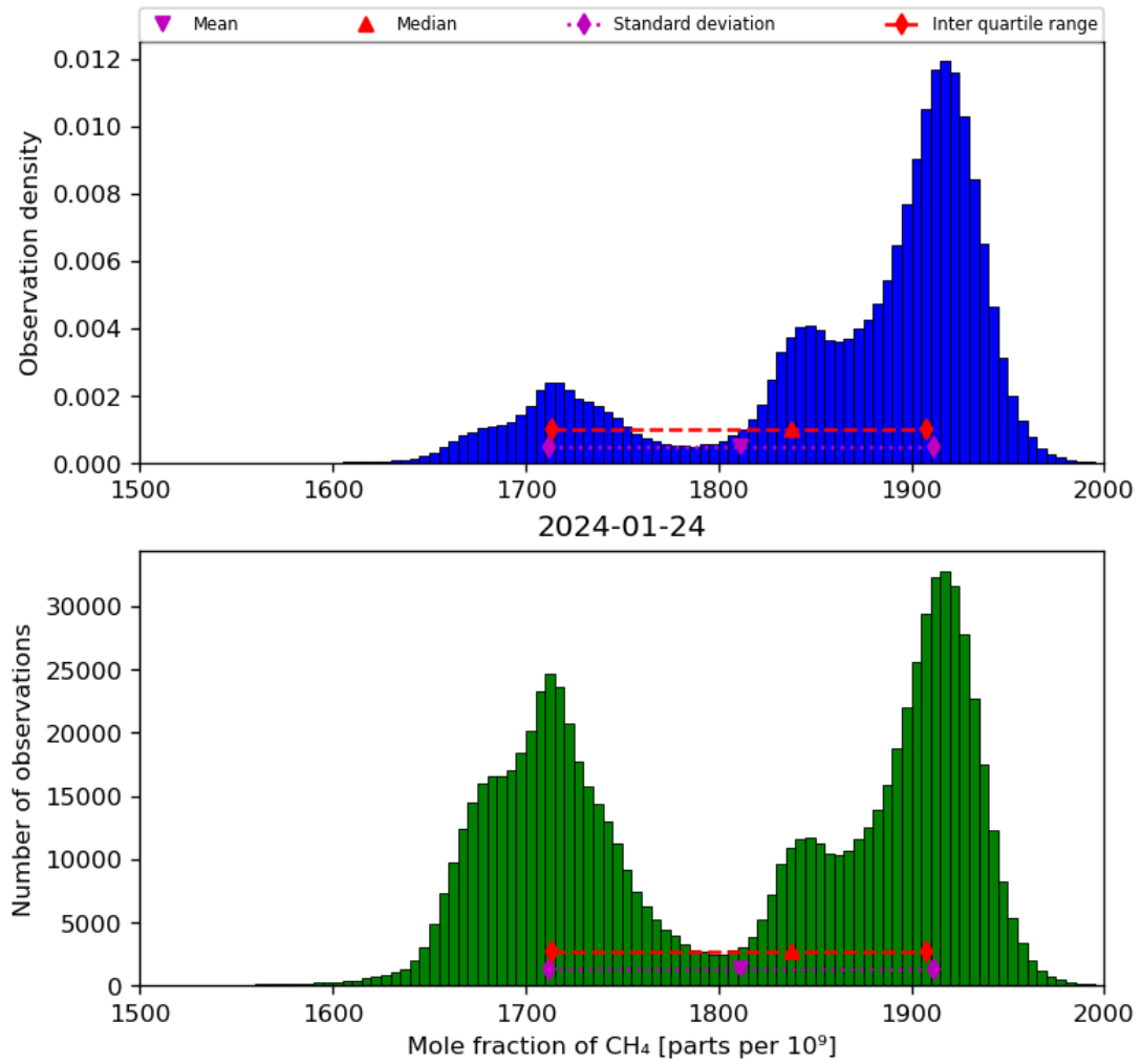
Figure 23: Histogram of “Mole fraction of CH 4 ” for 2024-01-23 to 2024-01-25
