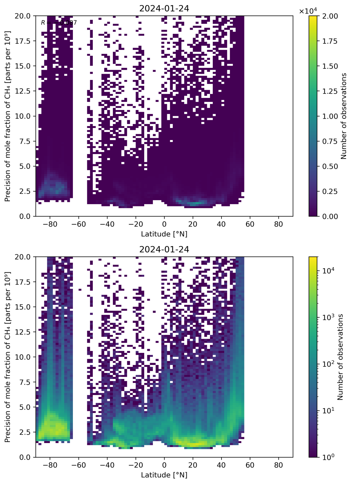
Figure 59: Scatter density plot of “Latitude” against “Precision of mole fraction of CH 4 ” for 2024-01-23 to 2024-01-25.
