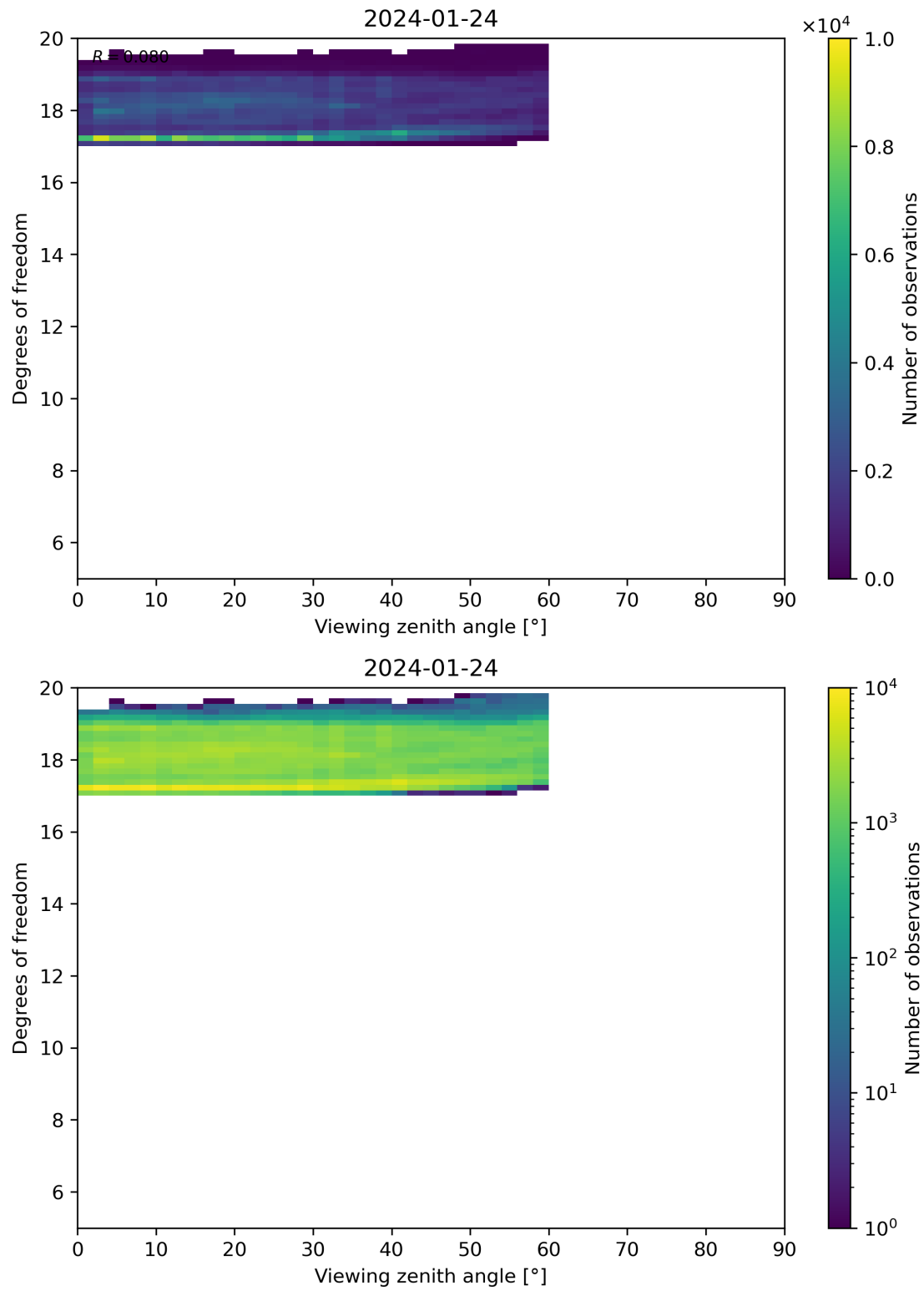
Figure 107: Scatter density plot of “Viewing zenith angle” against “Degrees of freedom” for 2024-01-23 to 2024-01-25.
