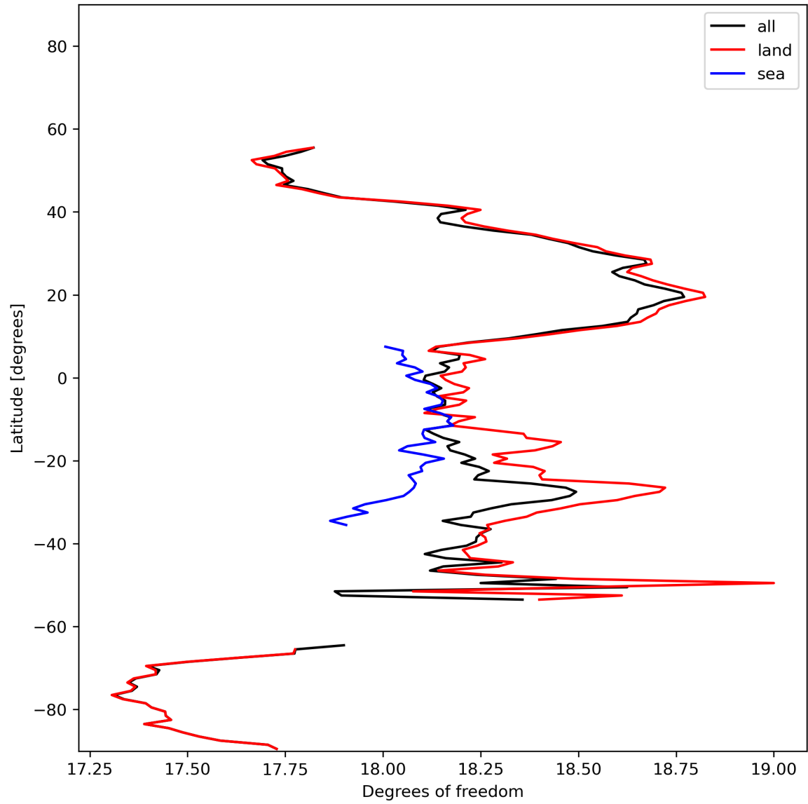
Figure 19: Zonal average of “Degrees of freedom” for 2024-01-23 to 2024-01-25.
