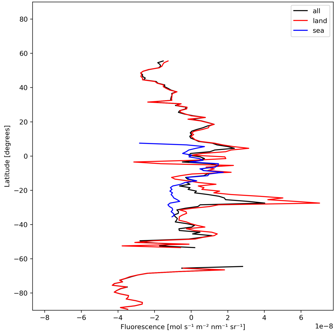
Figure 21: Zonal average of “Fluorescence” for 2024-01-23 to 2024-01-25.
