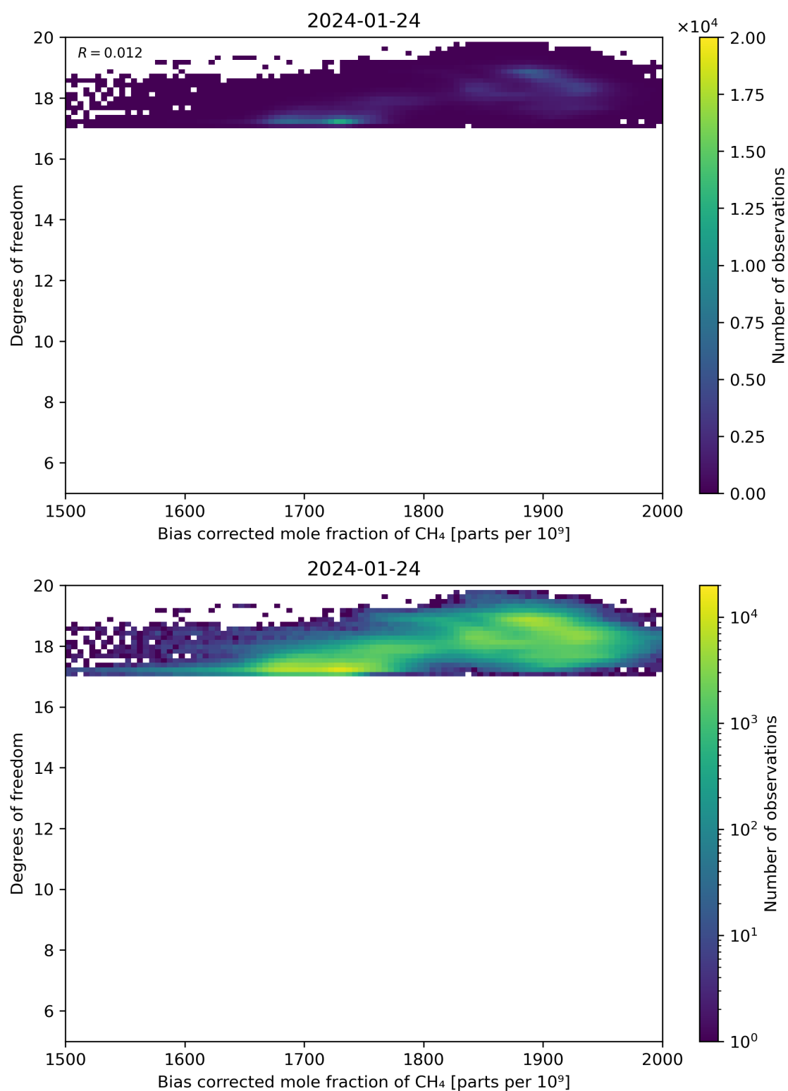
Figure 65: Scatter density plot of “Bias corrected mole fraction of CH 4 ” against “Degrees of freedom” for 2024-01-23 to 2024-01-25.
