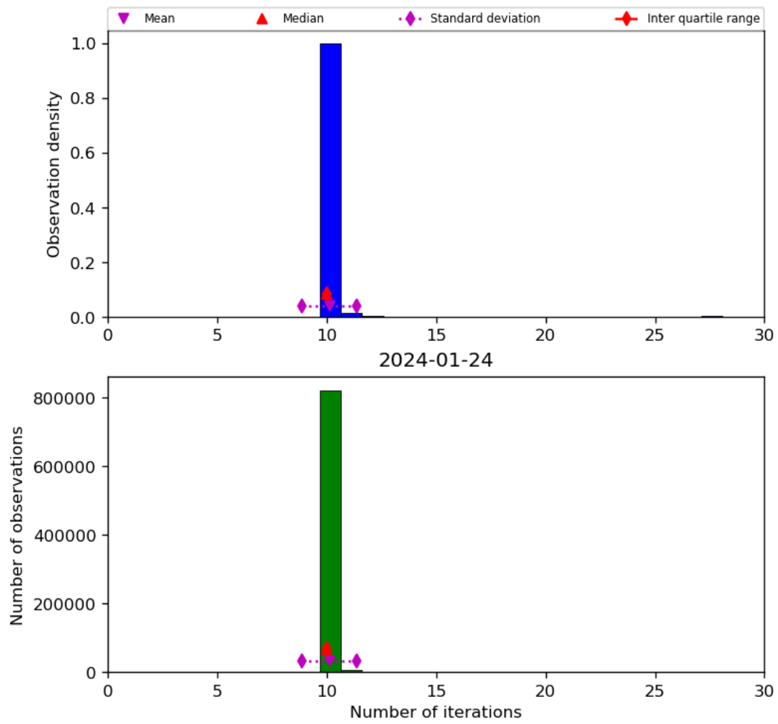
Figure 31: Histogram of “Number of iterations” for 2024-01-23 to 2024-01-25
