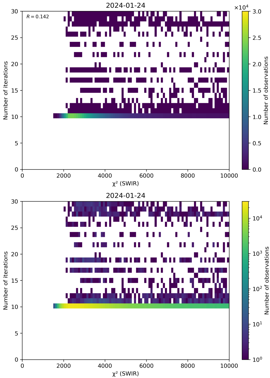
Figure 50: Scatter density plot of “ \chi^2 (SWIR)” against “Number of iterations” for 2024-01-23 to 2024-01-25.
