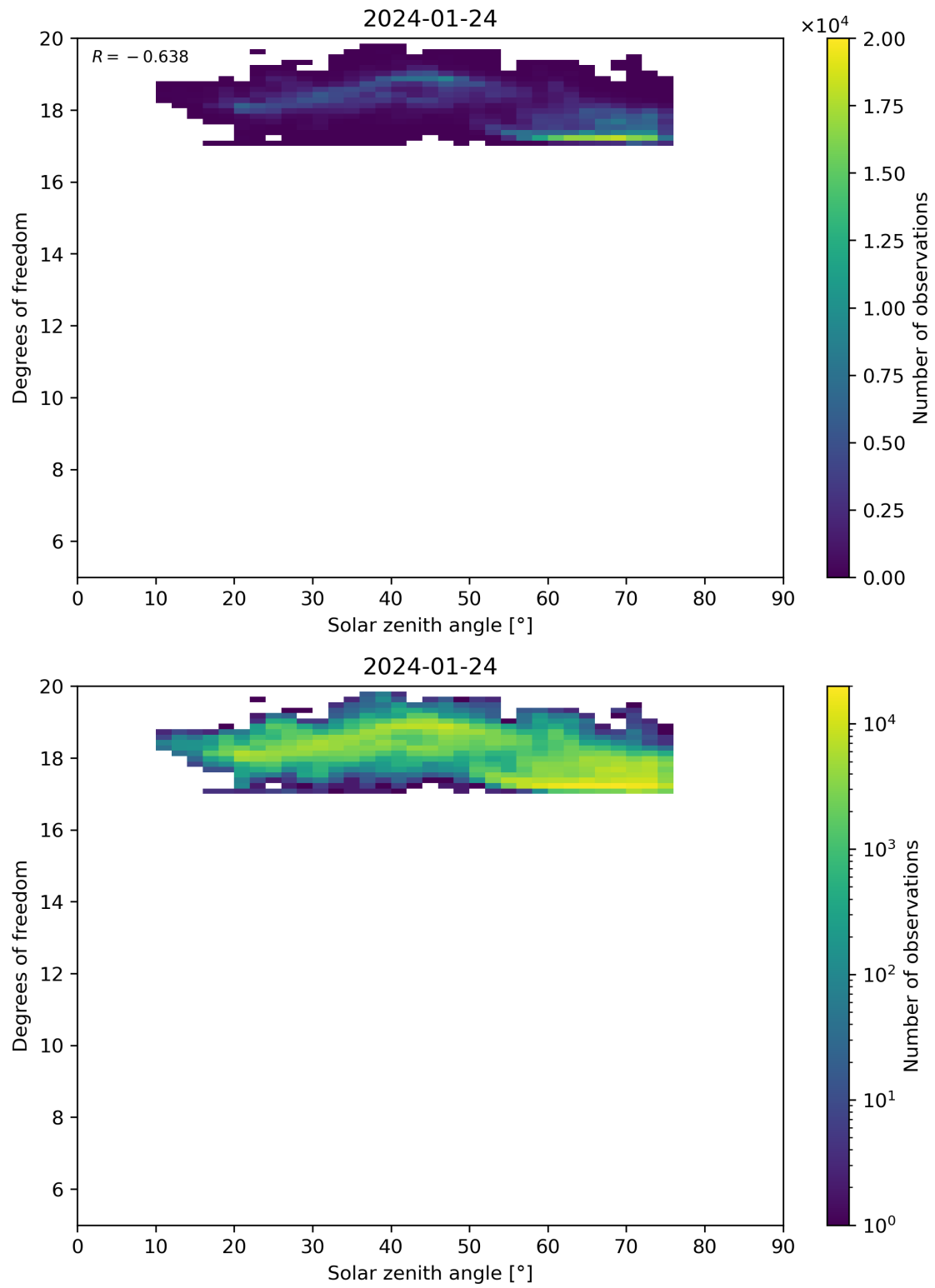
Figure 96: Scatter density plot of “Solar zenith angle” against “Degrees of freedom” for 2024-01-23 to 2024-01-25.
