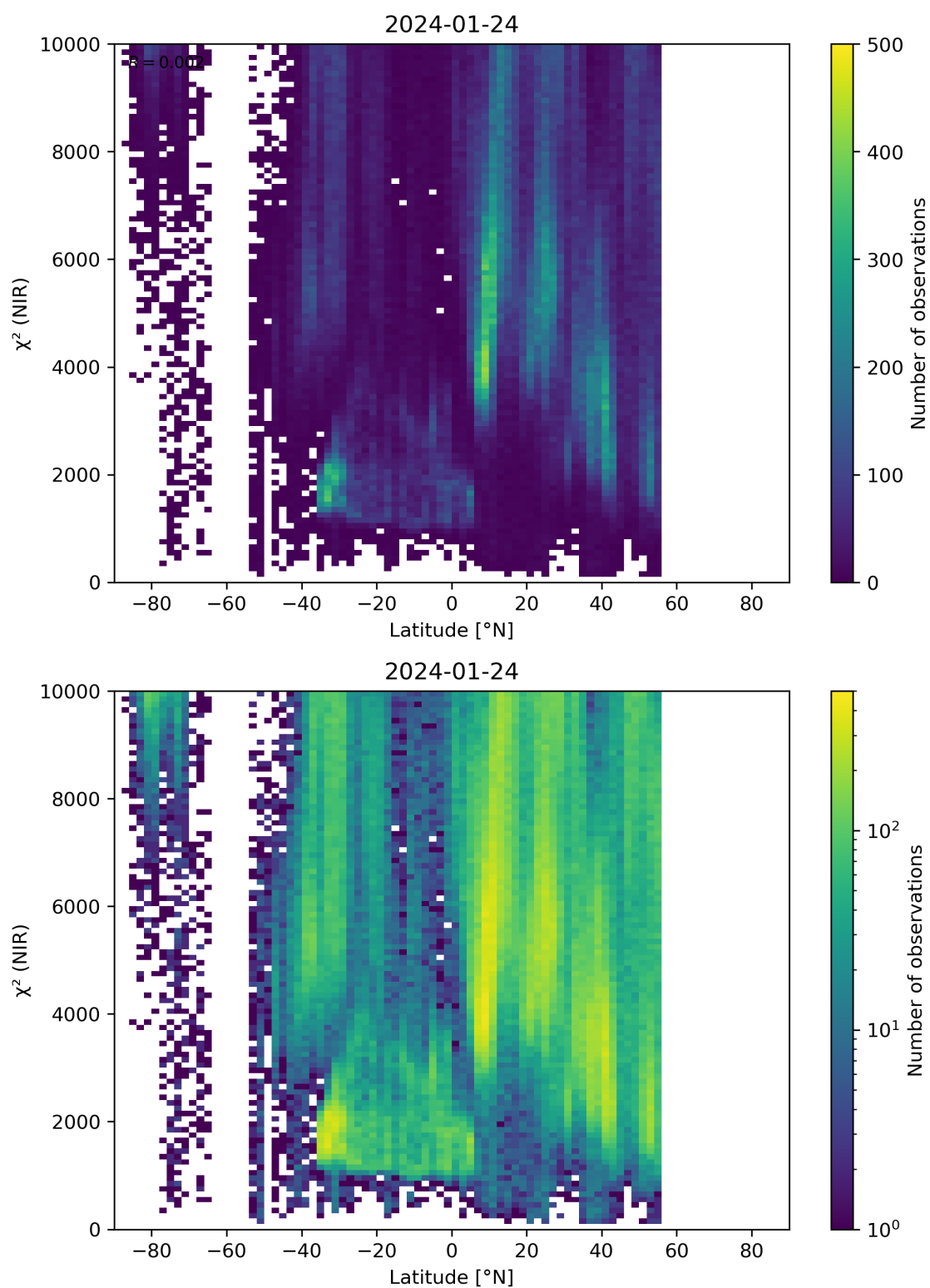
Figure 53: Scatter density plot of “Latitude” against “ \chi^2 (NIR)” for 2024-01-23 to 2024-01-25.
