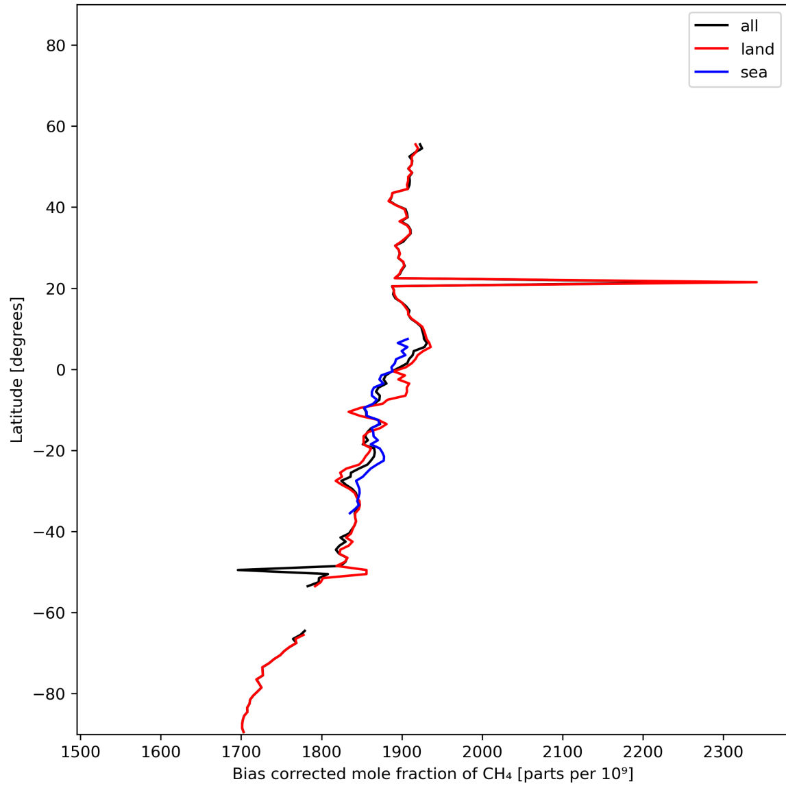
Figure 14: Zonal average of “Bias corrected mole fraction of CH 4 ” for 2024-01-23 to 2024-01-25.
