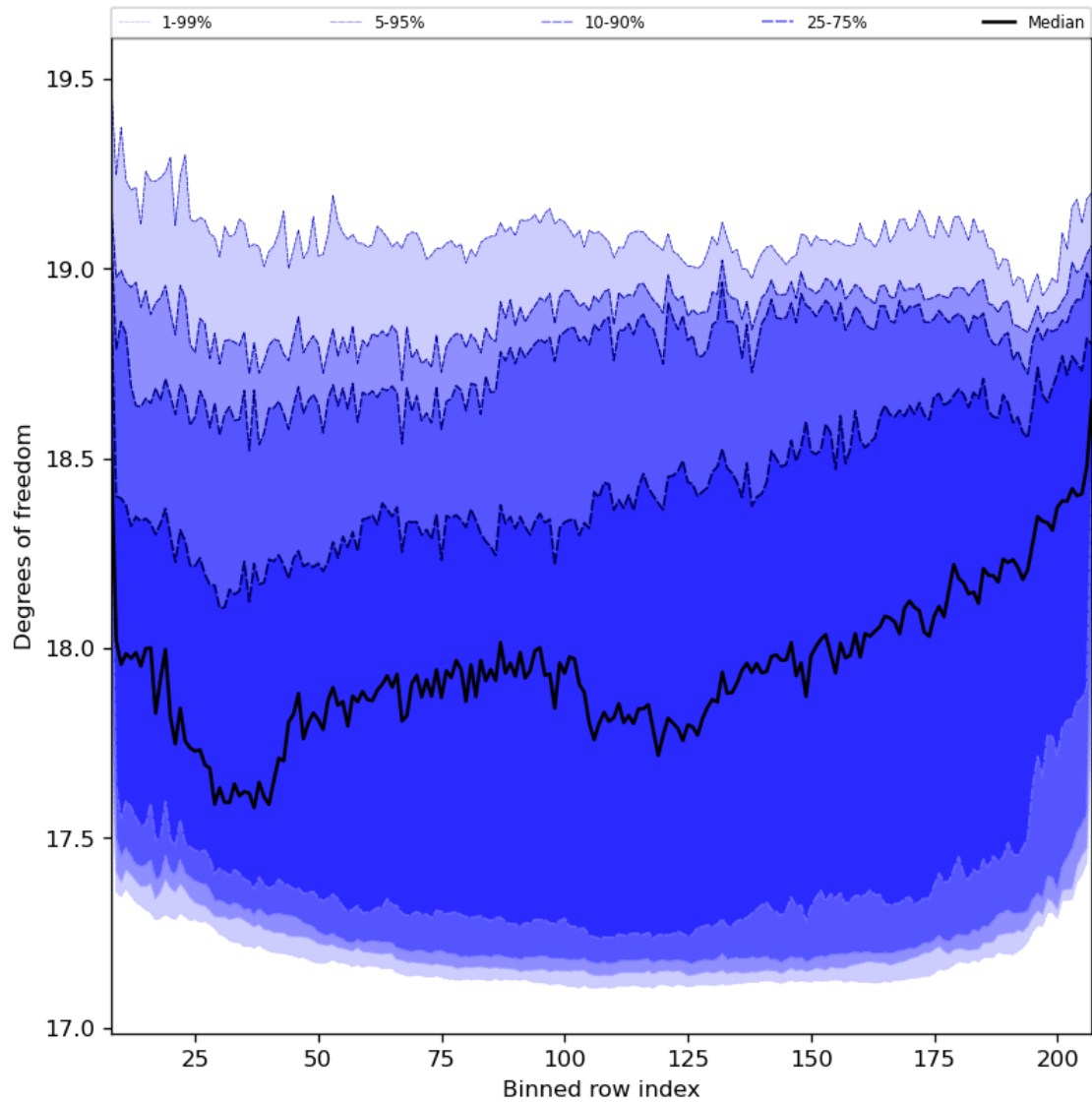
Figure 41: Along track statistics of “Degrees of freedom” for 2024-01-23 to 2024-01-25
