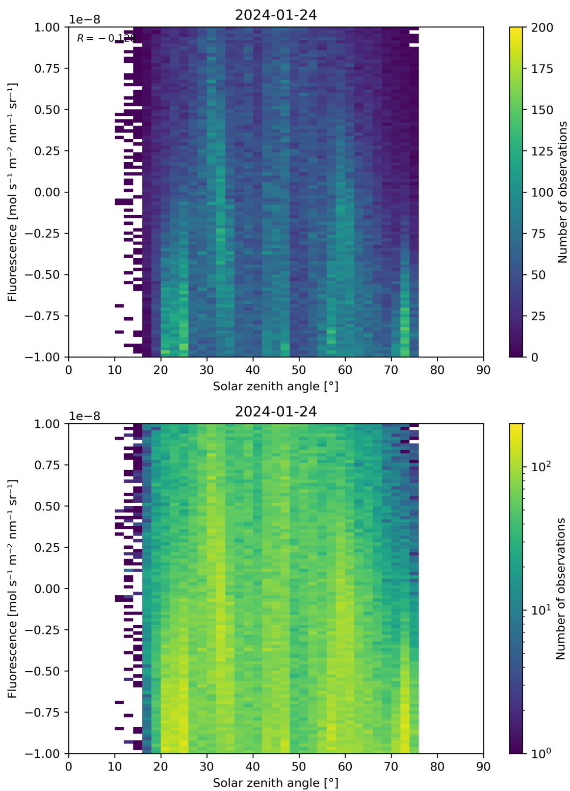
Figure 97: Scatter density plot of “Solar zenith angle” against “Fluorescence” for 2024-01-23 to 2024-01-25.
