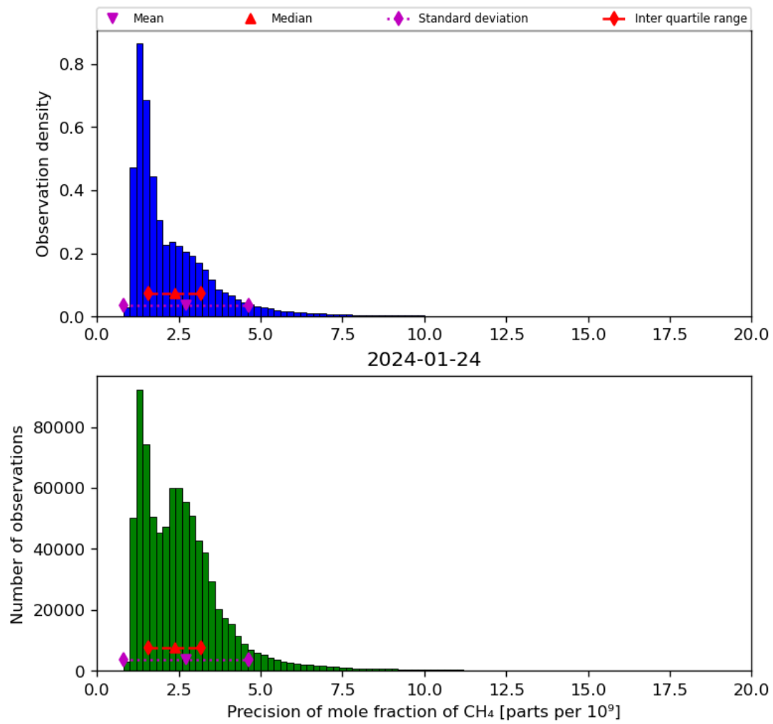
Figure 24: Histogram of “Precision of mole fraction of CH 4 ” for 2024-01-23 to 2024-01-25
