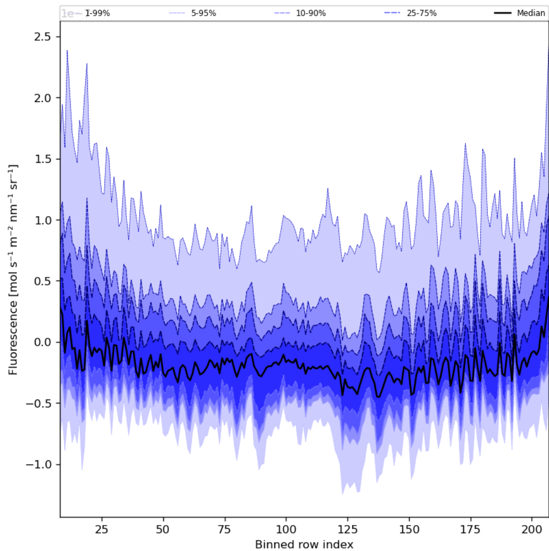
Figure 43: Along track statistics of “Fluorescence” for 2024-01-23 to 2024-01-25
