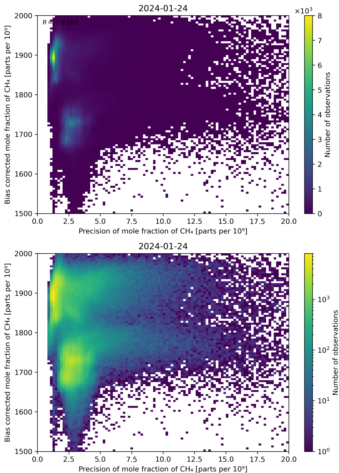
Figure 82: Scatter density plot of “Precision of mole fraction of CH 4 ” against “Bias corrected mole fraction of CH 4 ” for 2024-01-23 to 2024-01-25.
