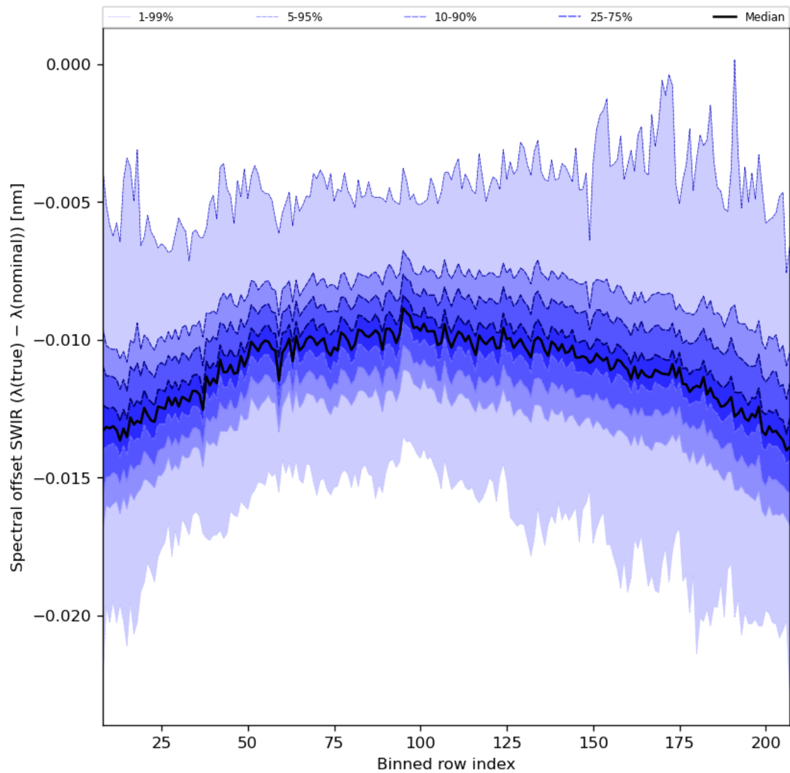
Figure 38: Along track statistics of “Spectral offset SWIR ( \lambda(\text{true}) - \lambda(\text{nominal}) )” for 2024-01-23 to 2024-01-25
