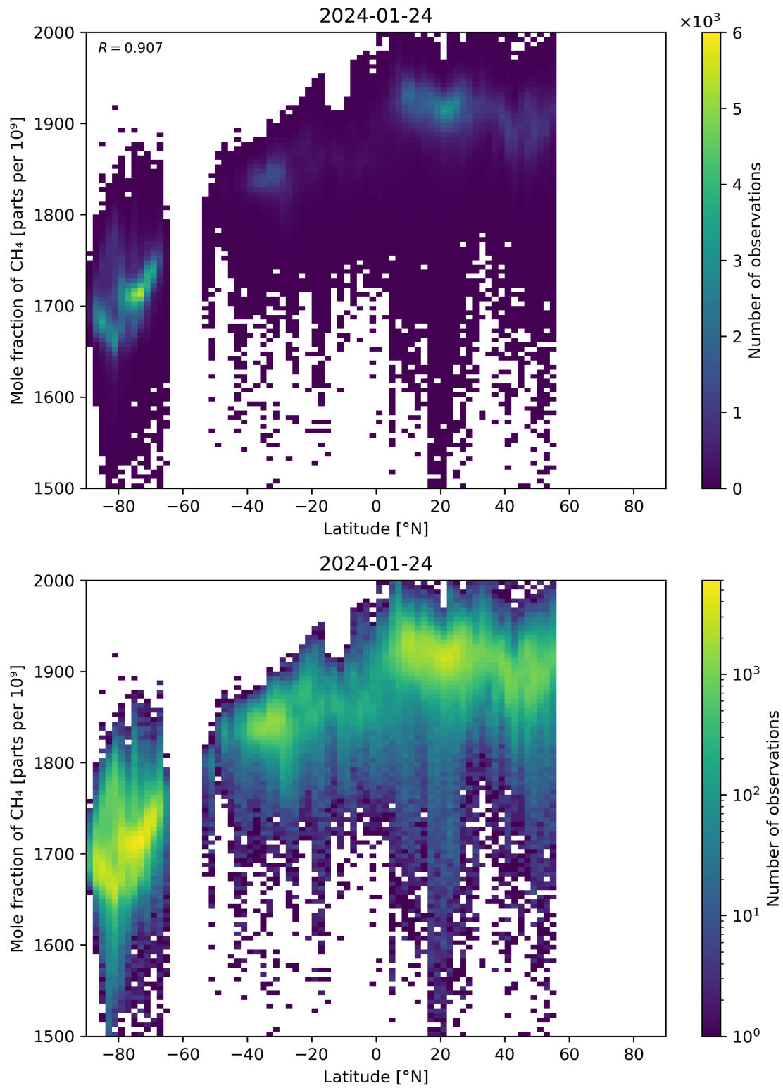
Figure 57: Scatter density plot of “Latitude” against “Mole fraction of CH 4 ” for 2024-01-23 to 2024-01-25.
