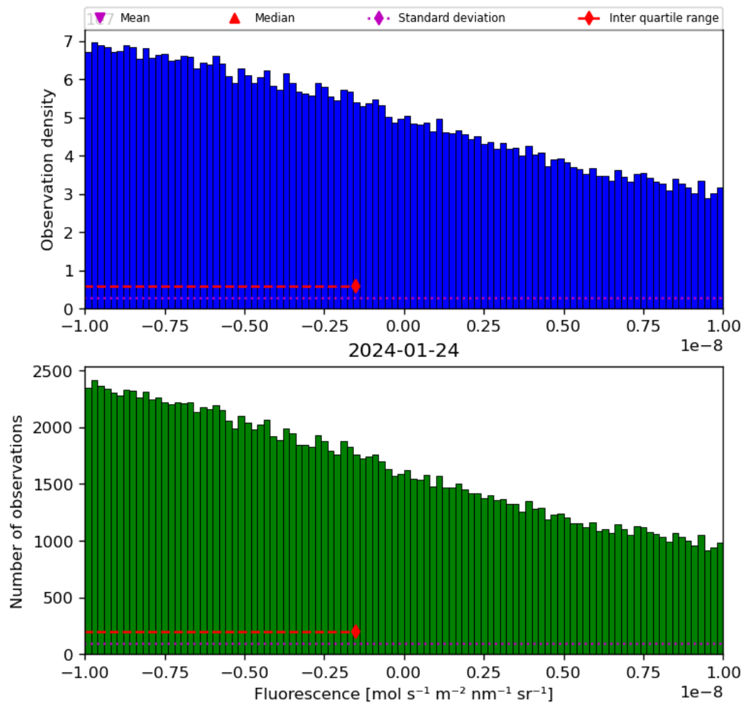
Figure 32: Histogram of “Fluorescence” for 2024-01-23 to 2024-01-25
