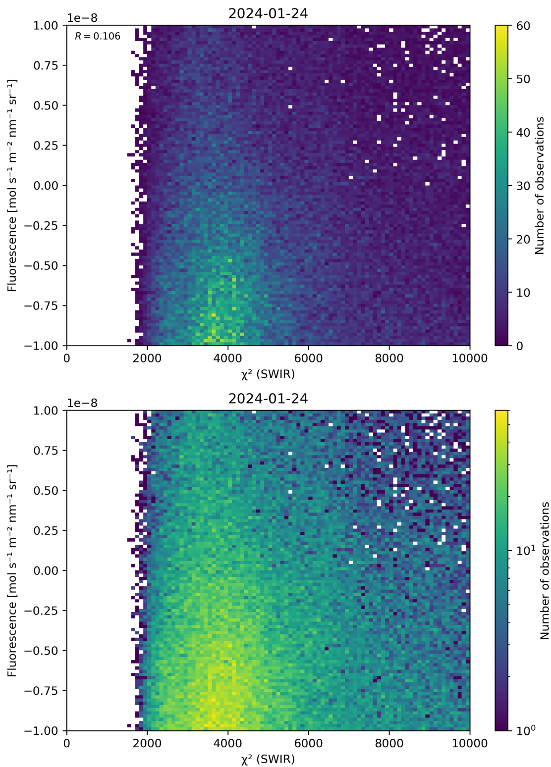
Figure 49: Scatter density plot of “ \chi^2 (SWIR)” against “Fluorescence” for 2024-01-23 to 2024-01-25.
