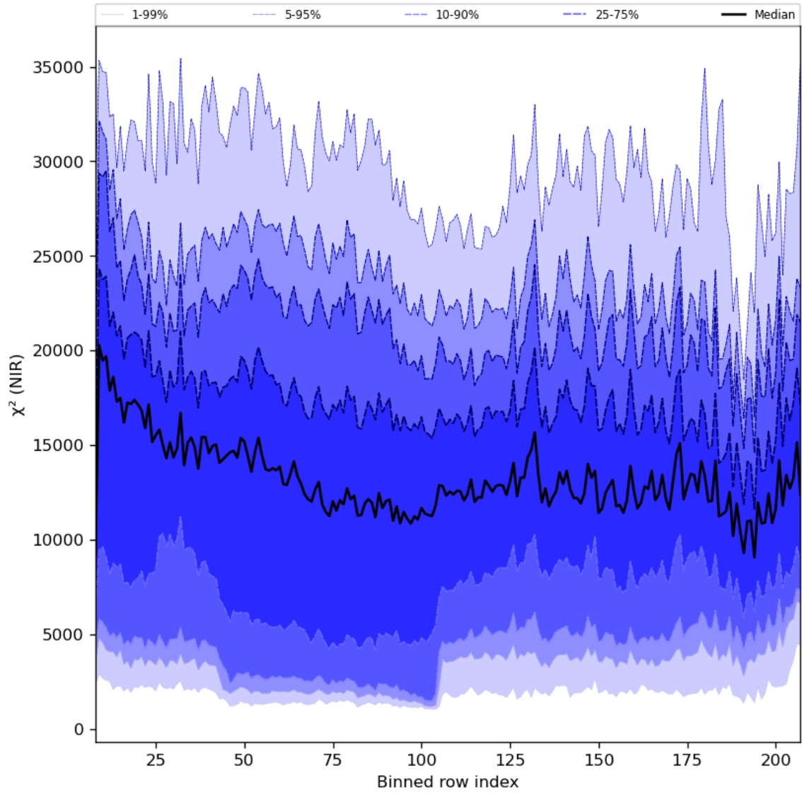
Figure 40: Along track statistics of “ \chi^2 (NIR)” for 2024-01-23 to 2024-01-25
