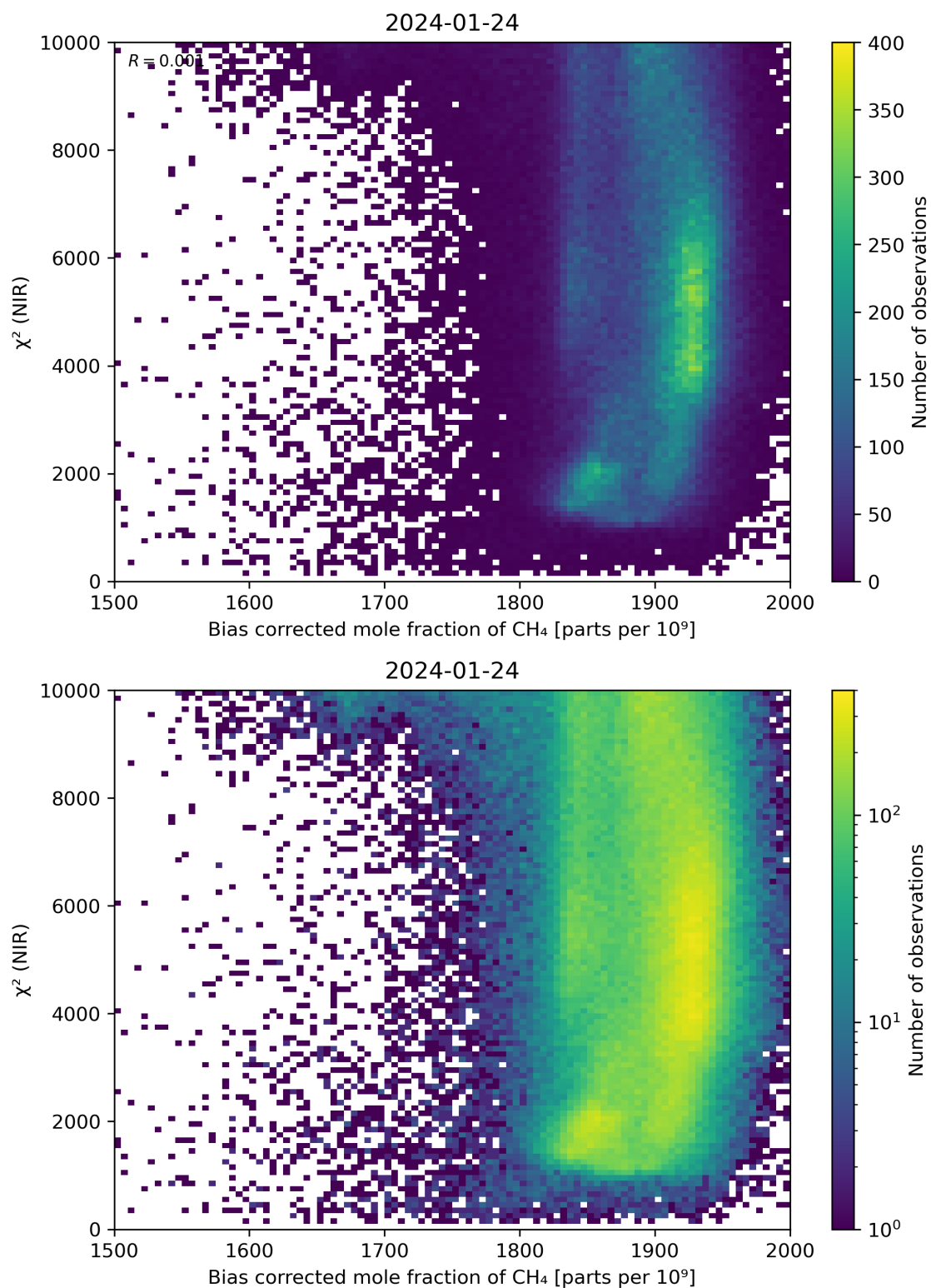
Figure 63: Scatter density plot of “Bias corrected mole fraction of CH 4 ” against “ \chi^2 (NIR)” for 2024-01-23 to 2024-01-25.
