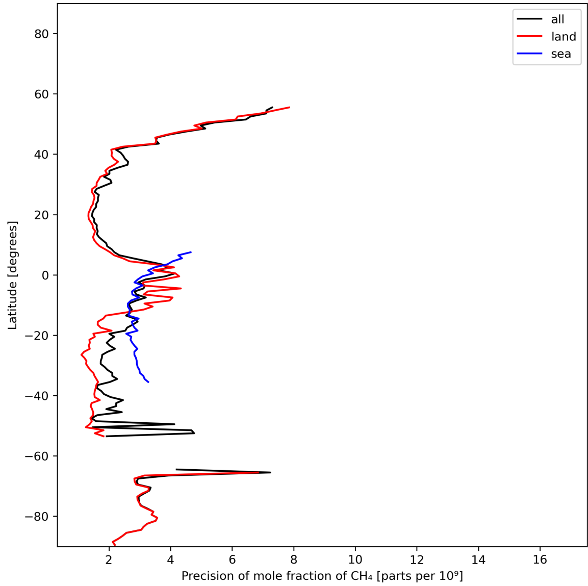
Figure 13: Zonal average of “Precision of mole fraction of CH 4 ” for 2024-01-23 to 2024-01-25.
