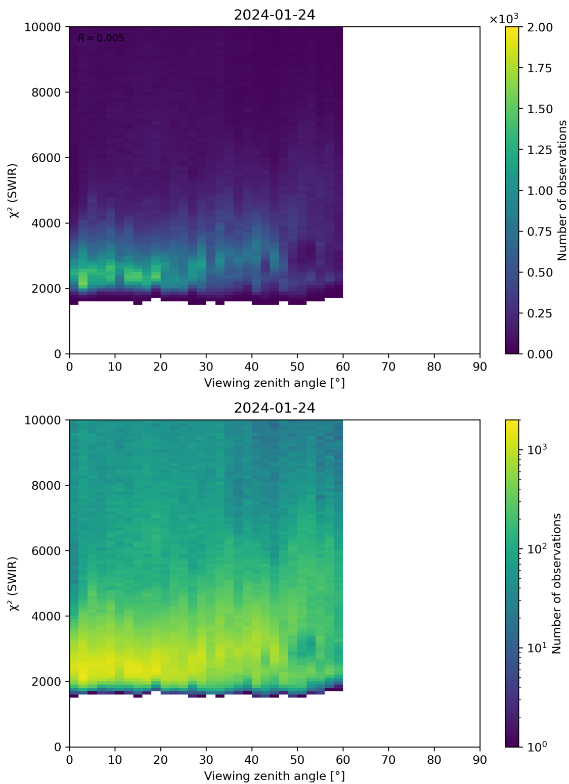
Figure 106: Scatter density plot of “Viewing zenith angle” against “ \chi^2 (SWIR)” for 2024-01-23 to 2024-01-25.
