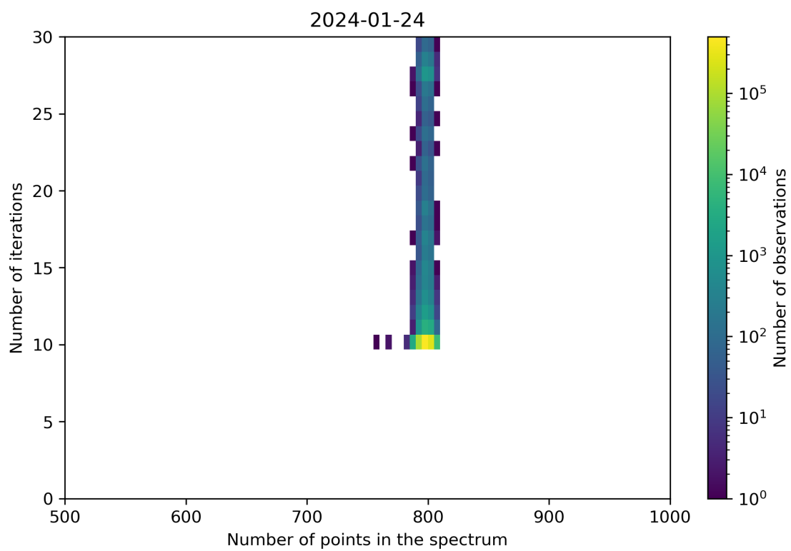
Figure 92: Scatter density plot of “Number of points in the spectrum” against “Number of iterations” for 2024-01-23 to 2024-01-25.
