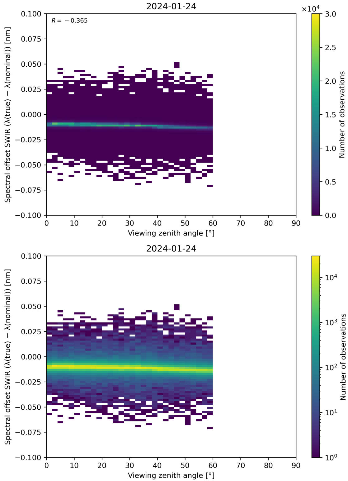
Figure 116: Scatter density plot of “Viewing zenith angle” against “Spectral offset SWIR ( \lambda(\text{true}) - \lambda(\text{nominal}) )” for 2024-01-23 to 2024-01-25.
