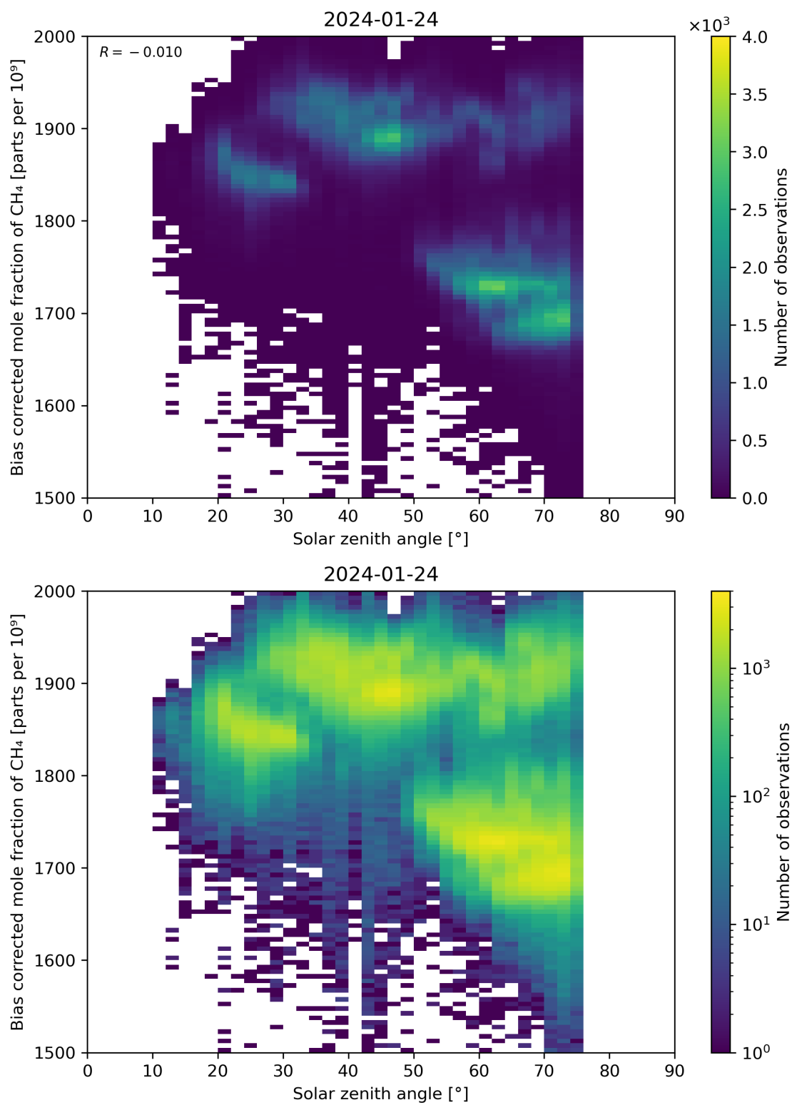
Figure 100: Scatter density plot of “Solar zenith angle” against “Bias corrected mole fraction of \text{CH}_4 ” for 2024-01-23 to 2024-01-25.
