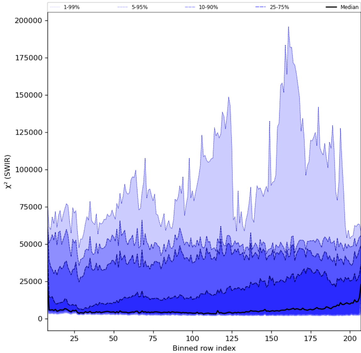
Figure 39: Along track statistics of “ \chi^2 (SWIR)” for 2024-01-23 to 2024-01-25
