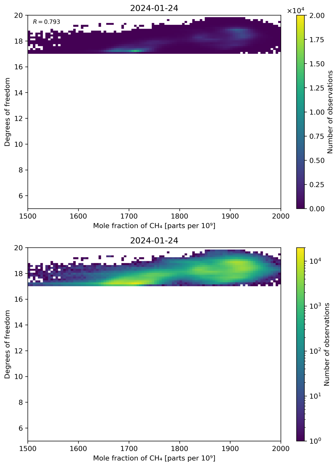
Figure 72: Scatter density plot of “Mole fraction of CH 4 ” against “Degrees of freedom” for 2024-01-23 to 2024-01-25.
