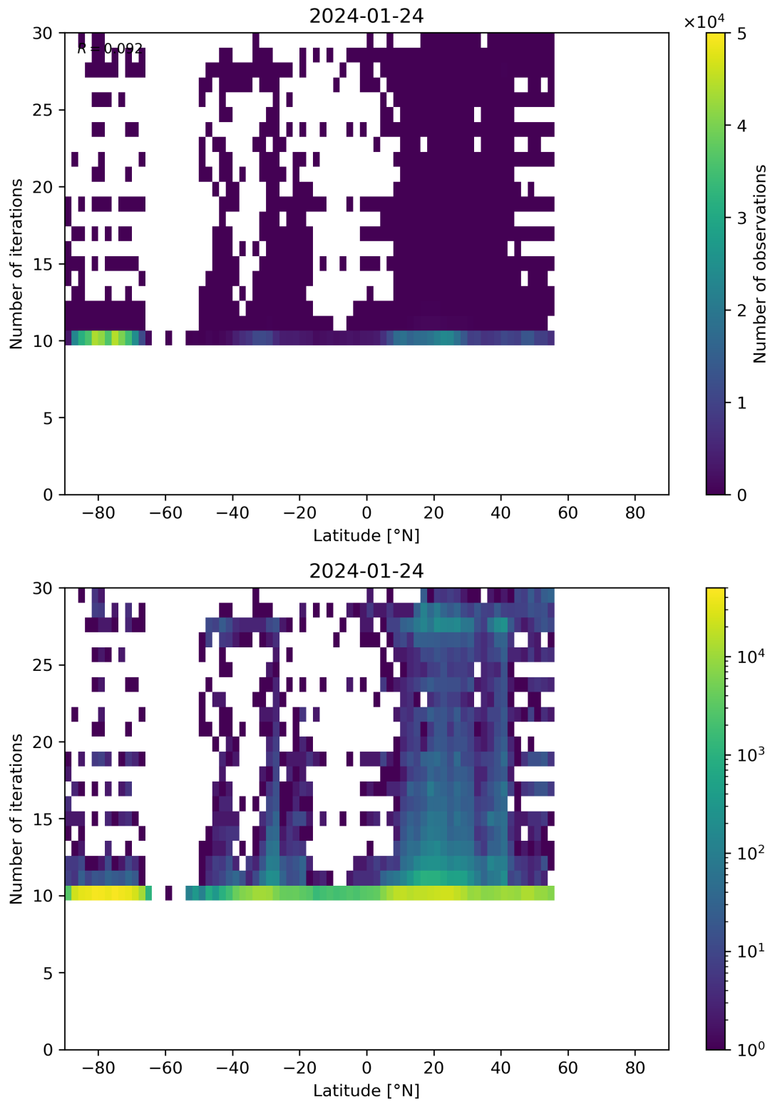
Figure 60: Scatter density plot of “Latitude” against “Number of iterations” for 2024-01-23 to 2024-01-25.
