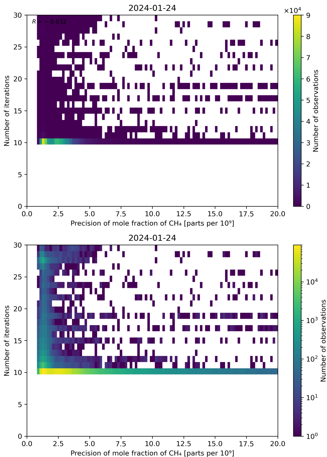
Figure 83: Scatter density plot of “Precision of mole fraction of CH 4 ” against “Number of iterations” for 2024-01-23 to 2024-01-25.
