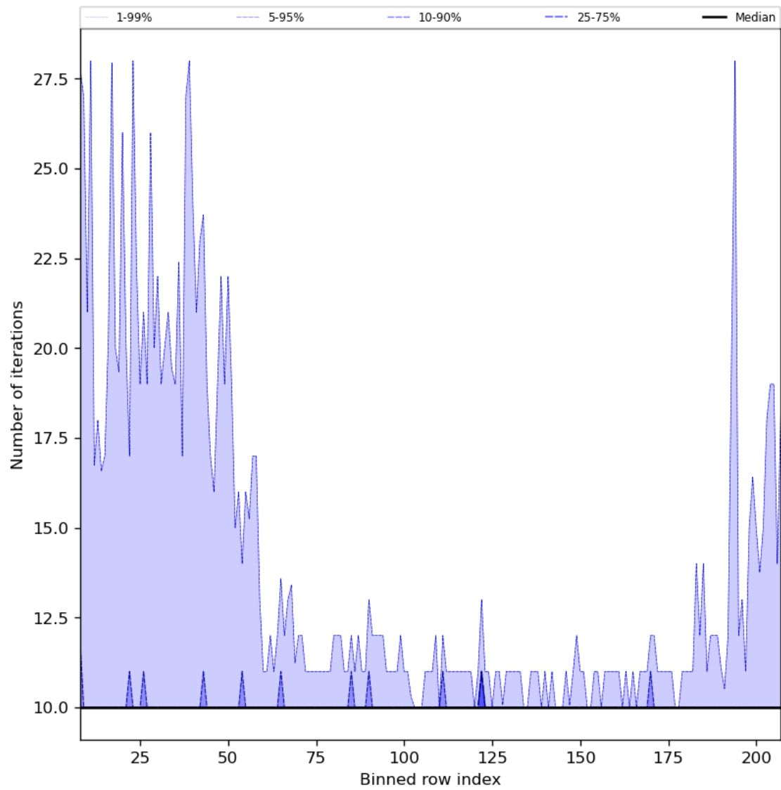
Figure 42: Along track statistics of “Number of iterations” for 2024-01-23 to 2024-01-25
