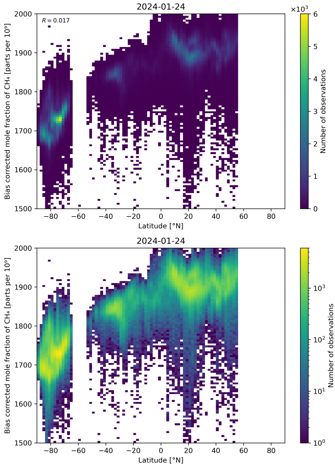
Figure 58: Scatter density plot of “Latitude” against “Bias corrected mole fraction of CH 4 ” for 2024-01-23 to 2024-01-25.
