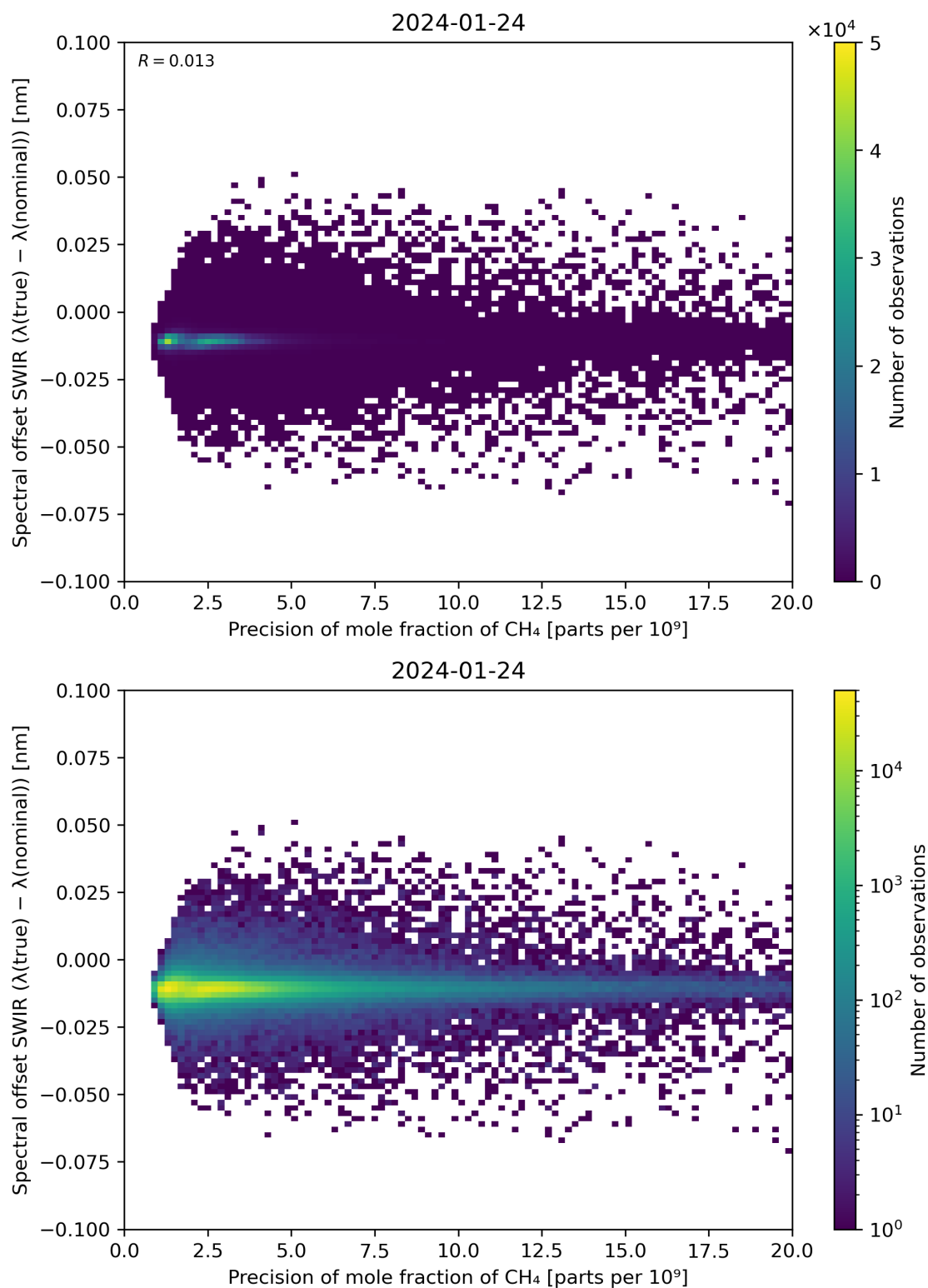
Figure 85: Scatter density plot of “Precision of mole fraction of CH 4 ” against “Spectral offset SWIR ( \lambda(\text{true}) - \lambda(\text{nominal}) )” for 2024-01-23 to 2024-01-25.
