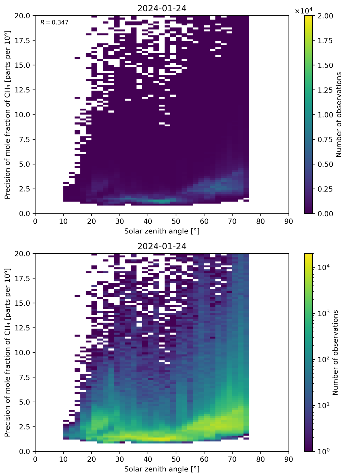
Figure 101: Scatter density plot of “Solar zenith angle” against “Precision of mole fraction of CH 4 ” for 2024-01-23 to 2024-01-25.
