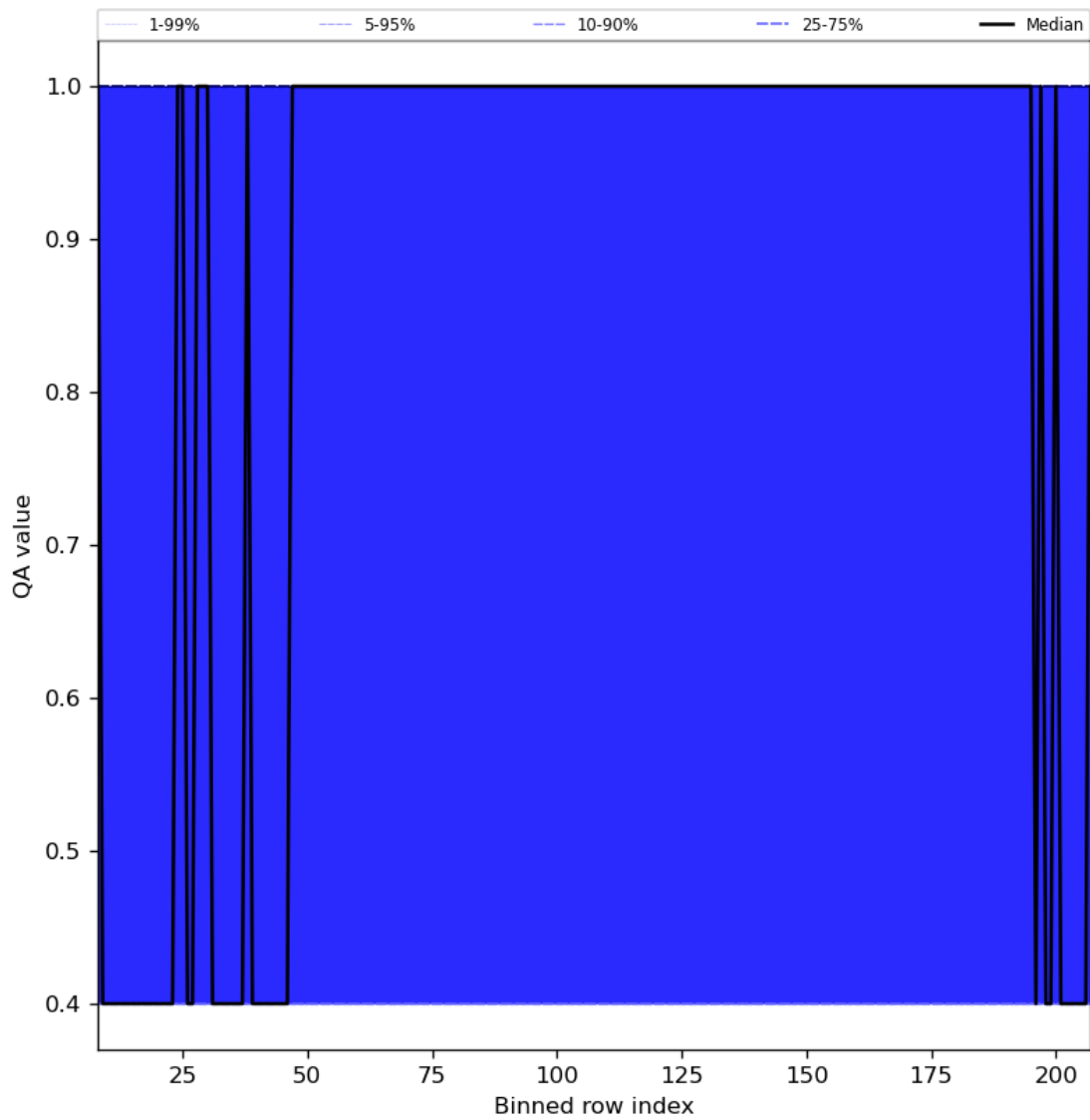
Figure 33: Along track statistics of “QA value” for 2024-01-23 to 2024-01-25
