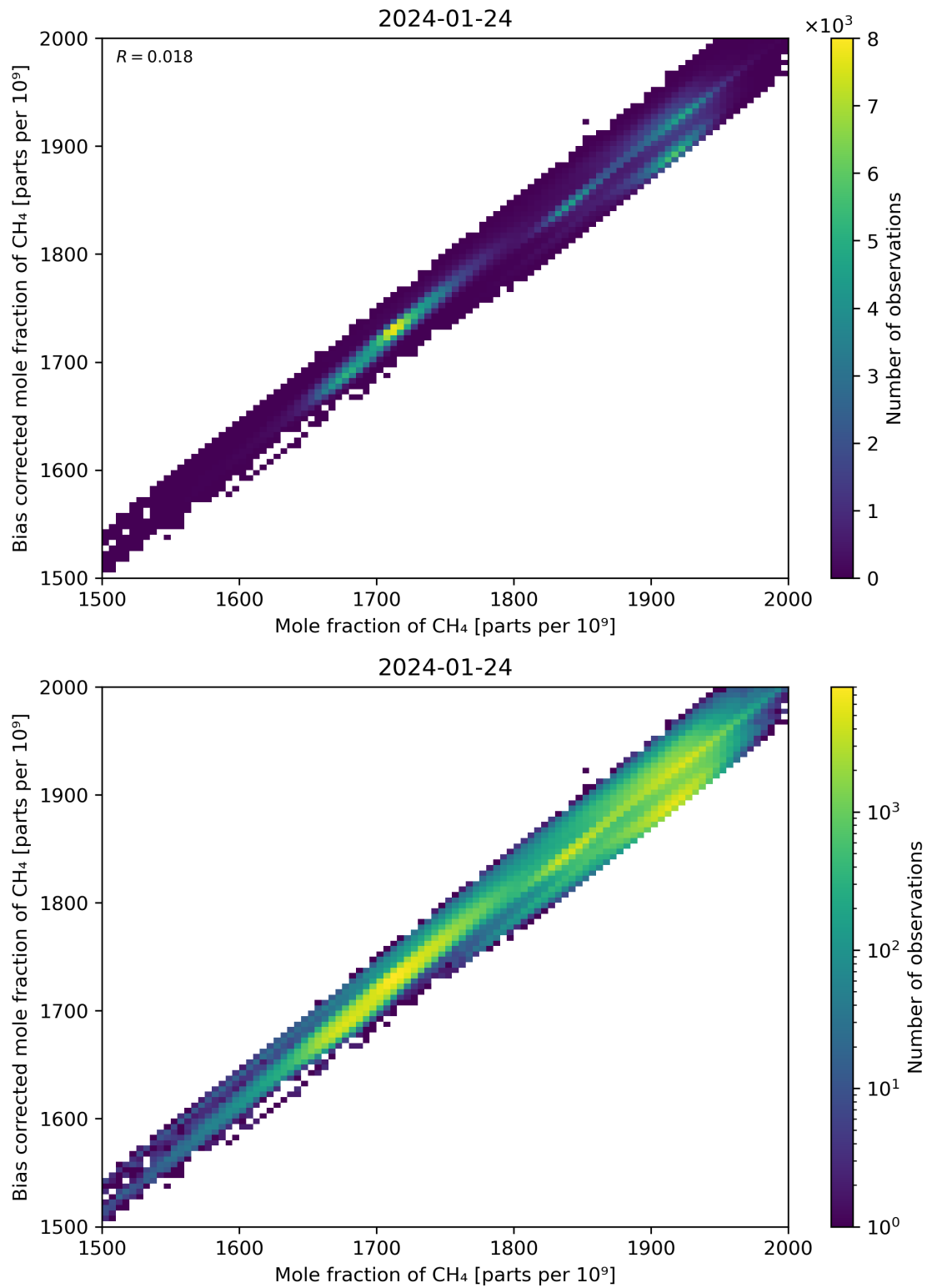
Figure 74: Scatter density plot of “Mole fraction of CH 4 ” against “Bias corrected mole fraction of CH 4 ” for 2024-01-23 to 2024-01-25.
