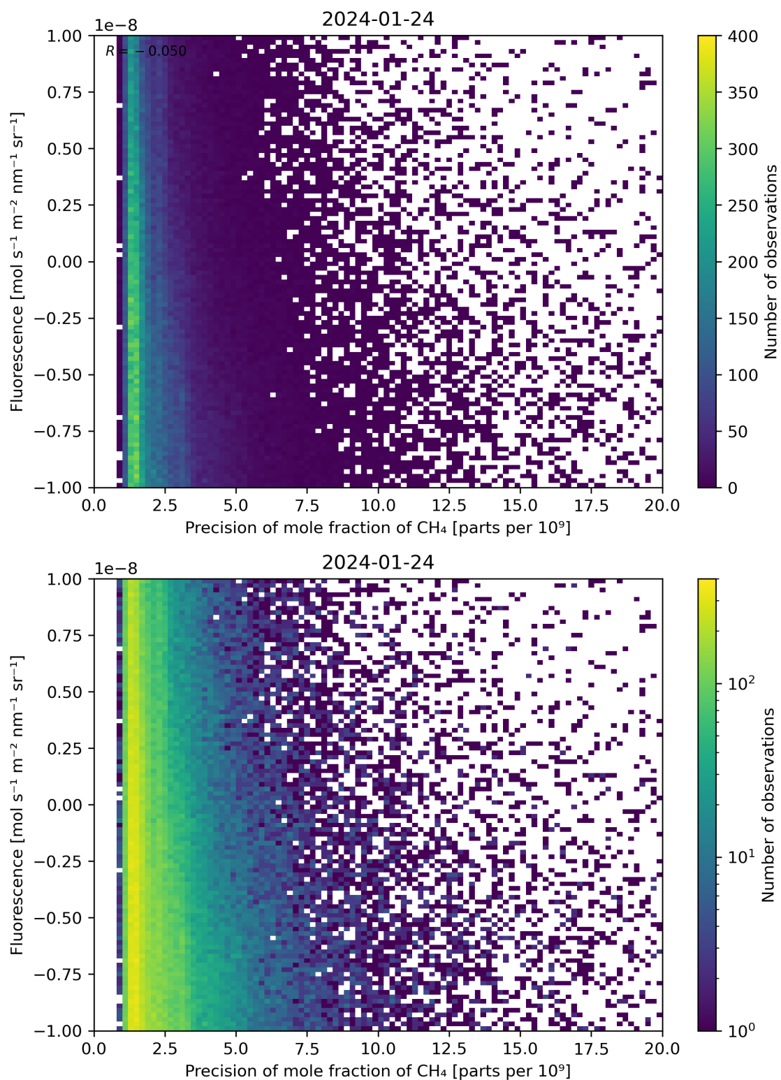
Figure 81: Scatter density plot of “Precision of mole fraction of \text{CH}_4 ” against “Fluorescence” for 2024-01-23 to 2024-01-25.
