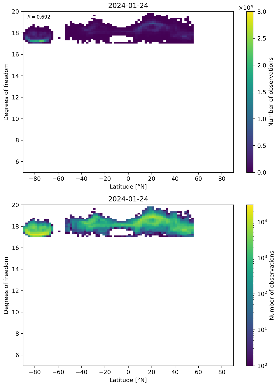
Figure 55: Scatter density plot of “Latitude” against “Degrees of freedom” for 2024-01-23 to 2024-01-25.
