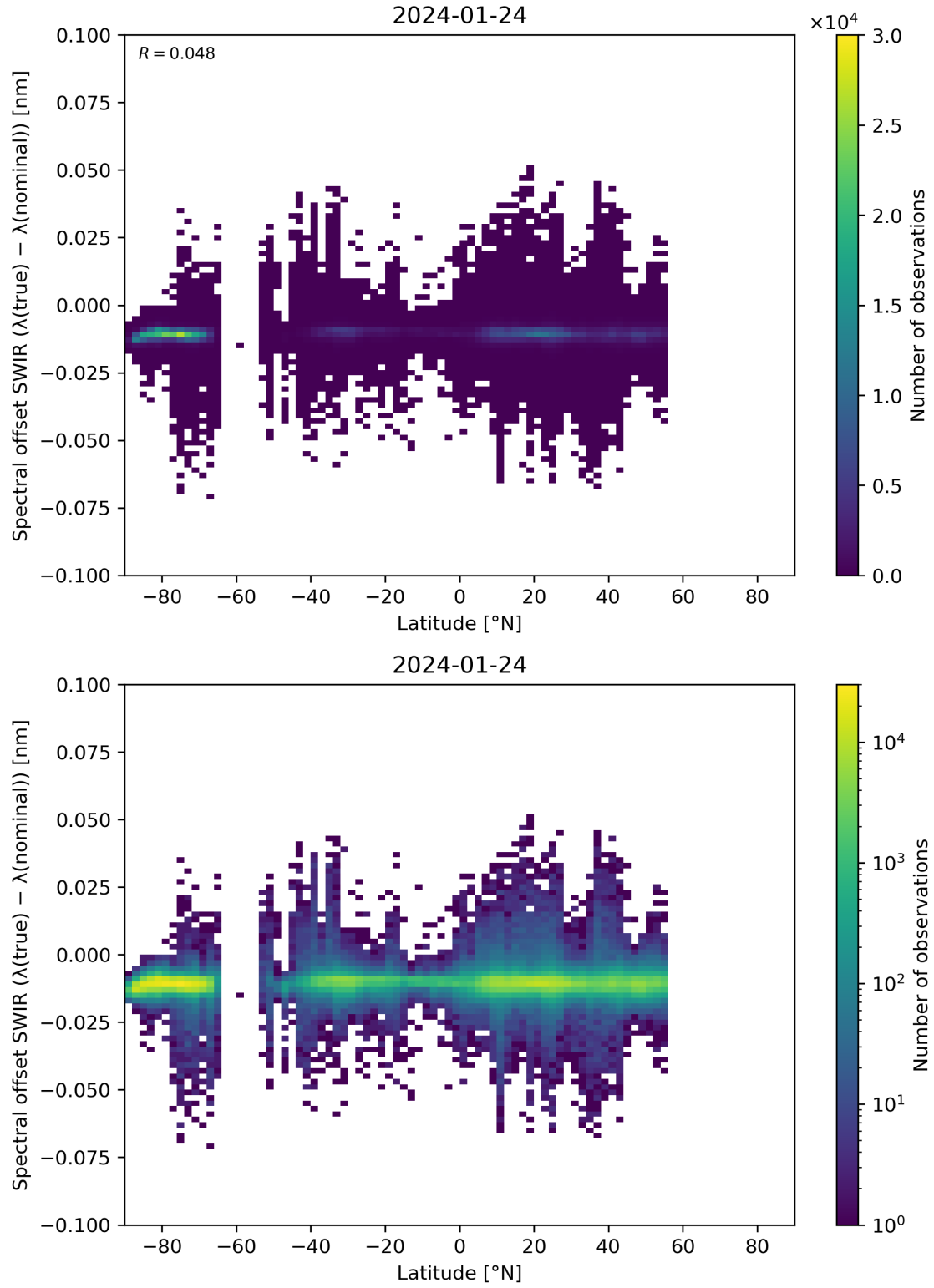
Figure 62: Scatter density plot of “Latitude” against “Spectral offset SWIR ( \lambda(\text{true}) - \lambda(\text{nominal}) )” for 2024-01-23 to 2024-01-25.
