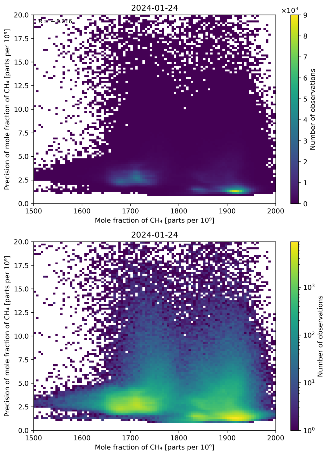
Figure 75: Scatter density plot of “Mole fraction of CH 4 ” against “Precision of mole fraction of CH 4 ” for 2024-01-23 to 2024-01-25.
