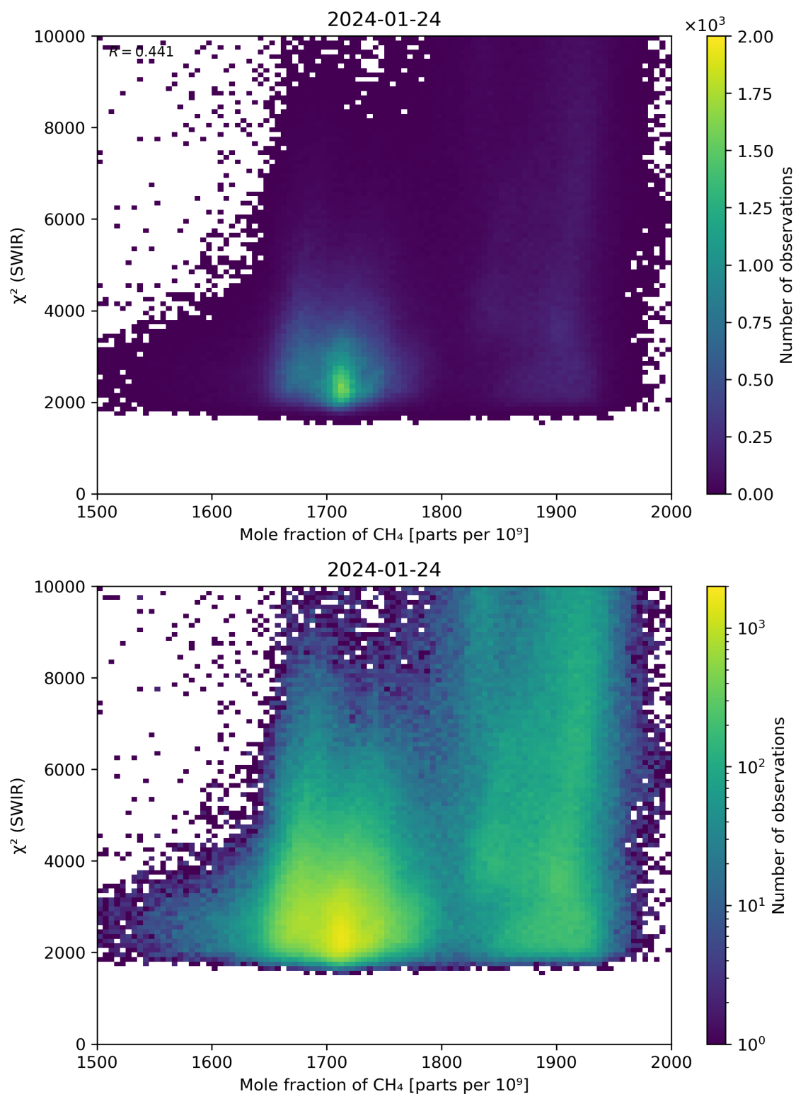
Figure 71: Scatter density plot of “Mole fraction of \text{CH}_4 ” against “ \chi^2 (SWIR)” for 2024-01-23 to 2024-01-25.
