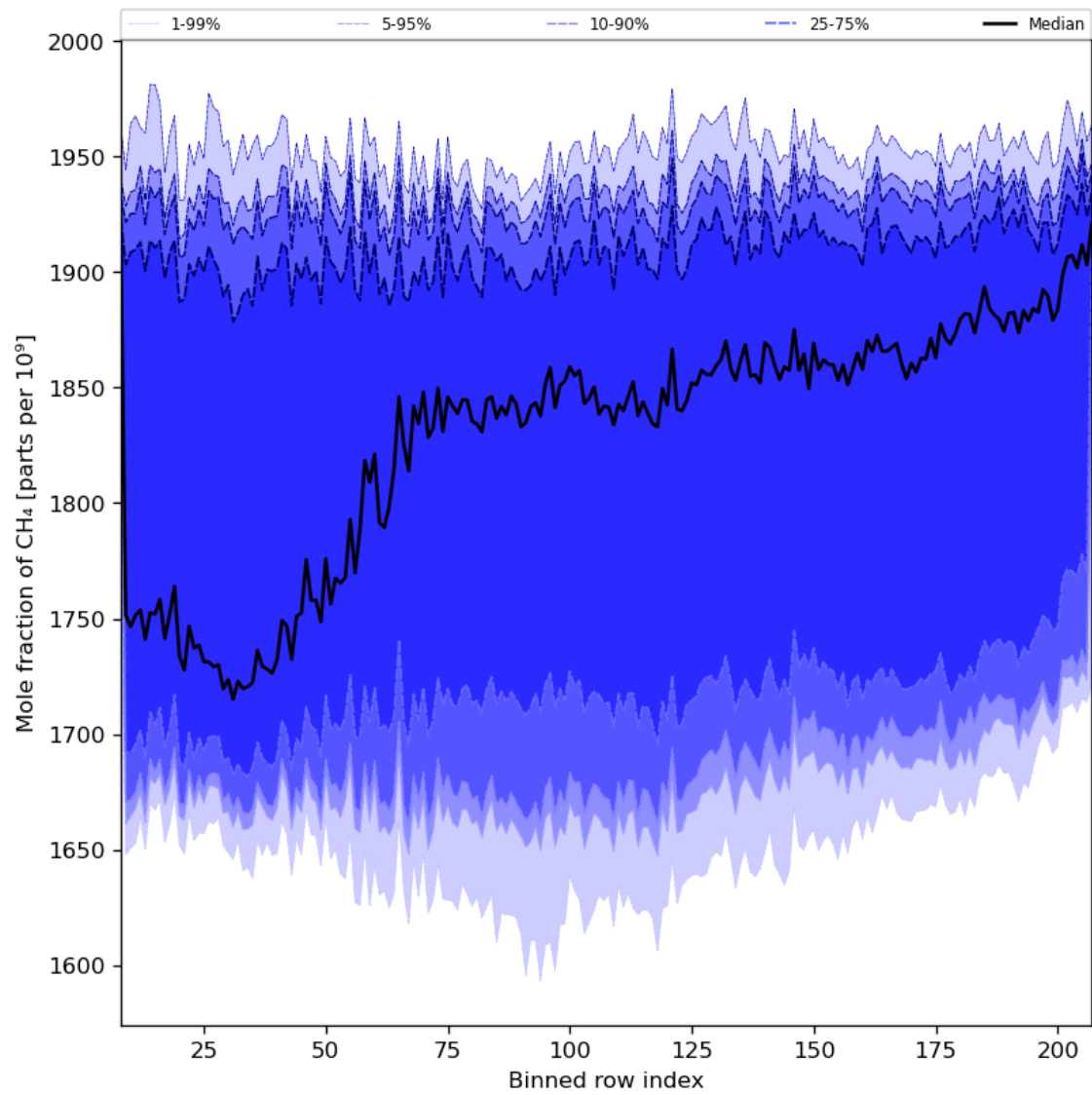
Figure 34: Along track statistics of “Mole fraction of CH 4 ” for 2024-01-23 to 2024-01-25
