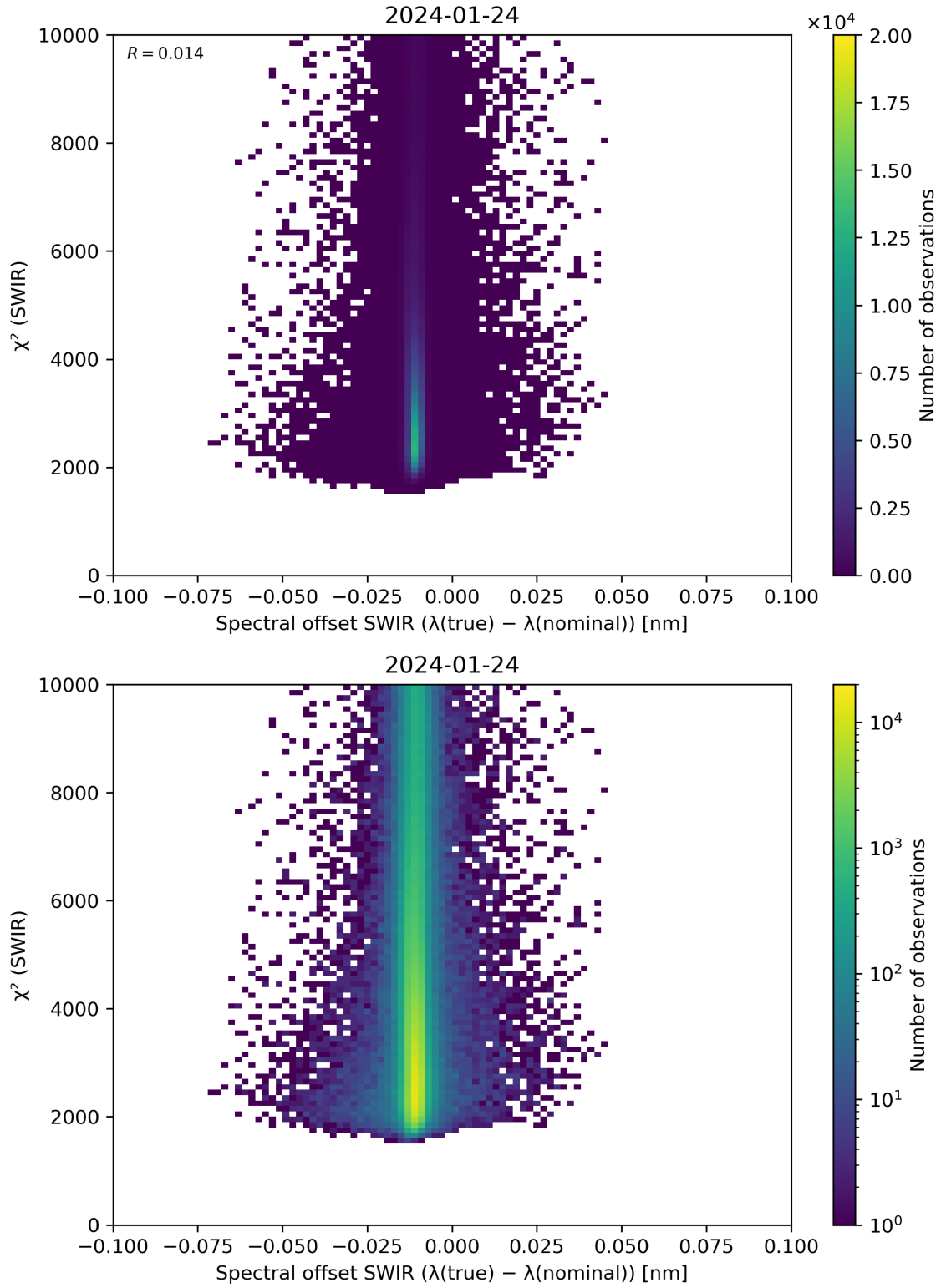
Figure 118: Scatter density plot of “Spectral offset SWIR ( \lambda(\text{true}) - \lambda(\text{nominal}) )” against “ \chi^2 (SWIR)” for 2024-01-23 to 2024-01-25.
