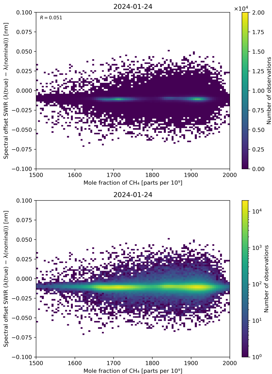
Figure 86: Scatter density plot of “Mole fraction of CH 4 ” against “Spectral offset SWIR ( \lambda(\text{true}) - \lambda(\text{nominal}) )” for 2024-01-23 to 2024-01-25.
