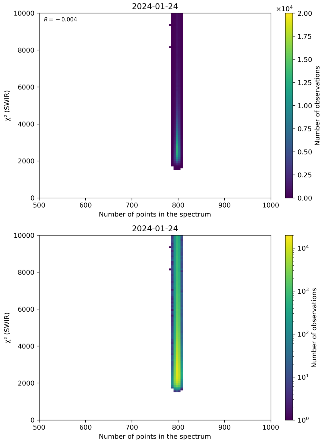
Figure 89: Scatter density plot of “Number of points in the spectrum” against “ \chi^2 (SWIR)” for 2024-01-23 to 2024-01-25.
