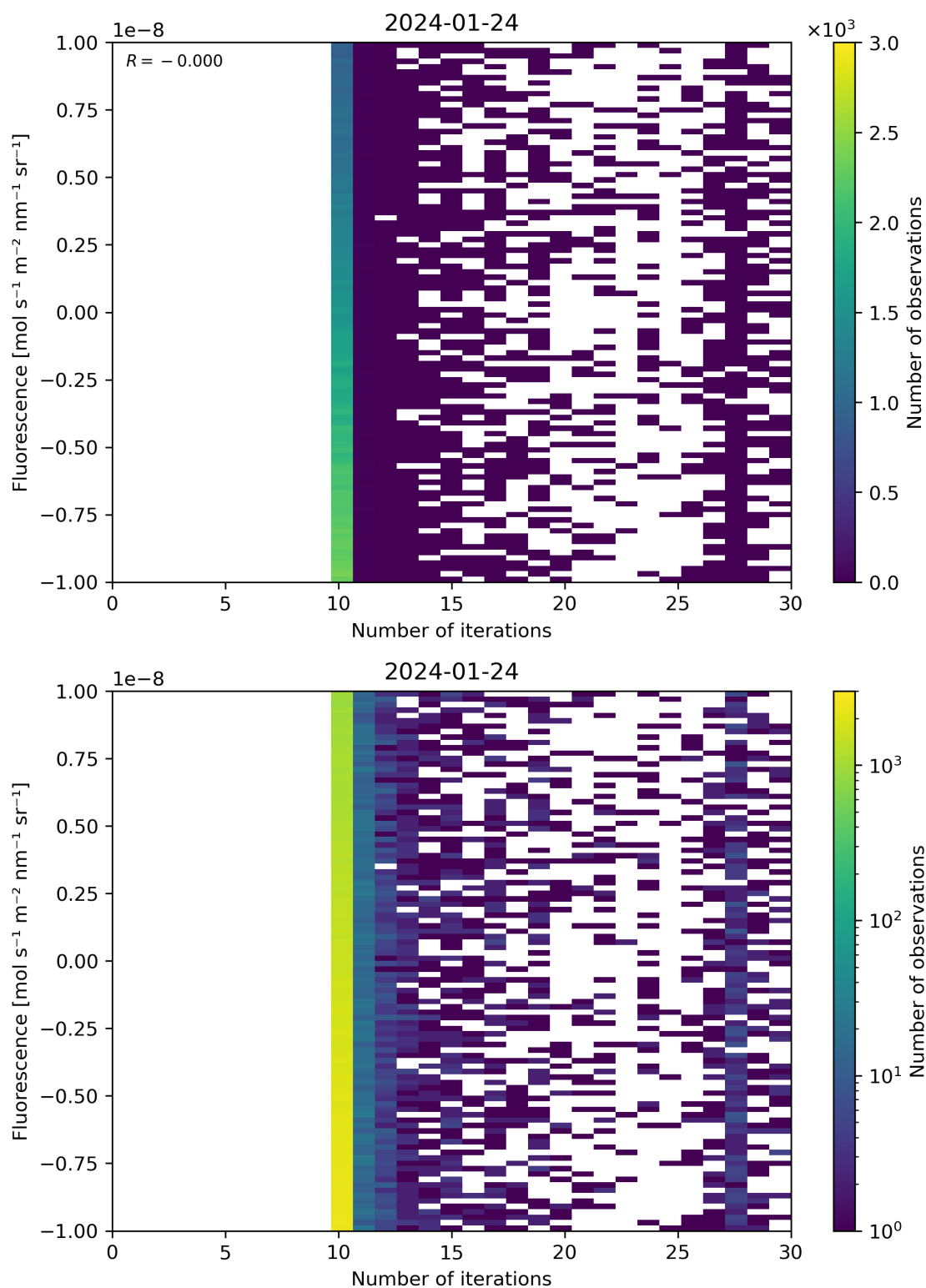
Figure 87: Scatter density plot of “Number of iterations” against “Fluorescence” for 2024-01-23 to 2024-01-25.
