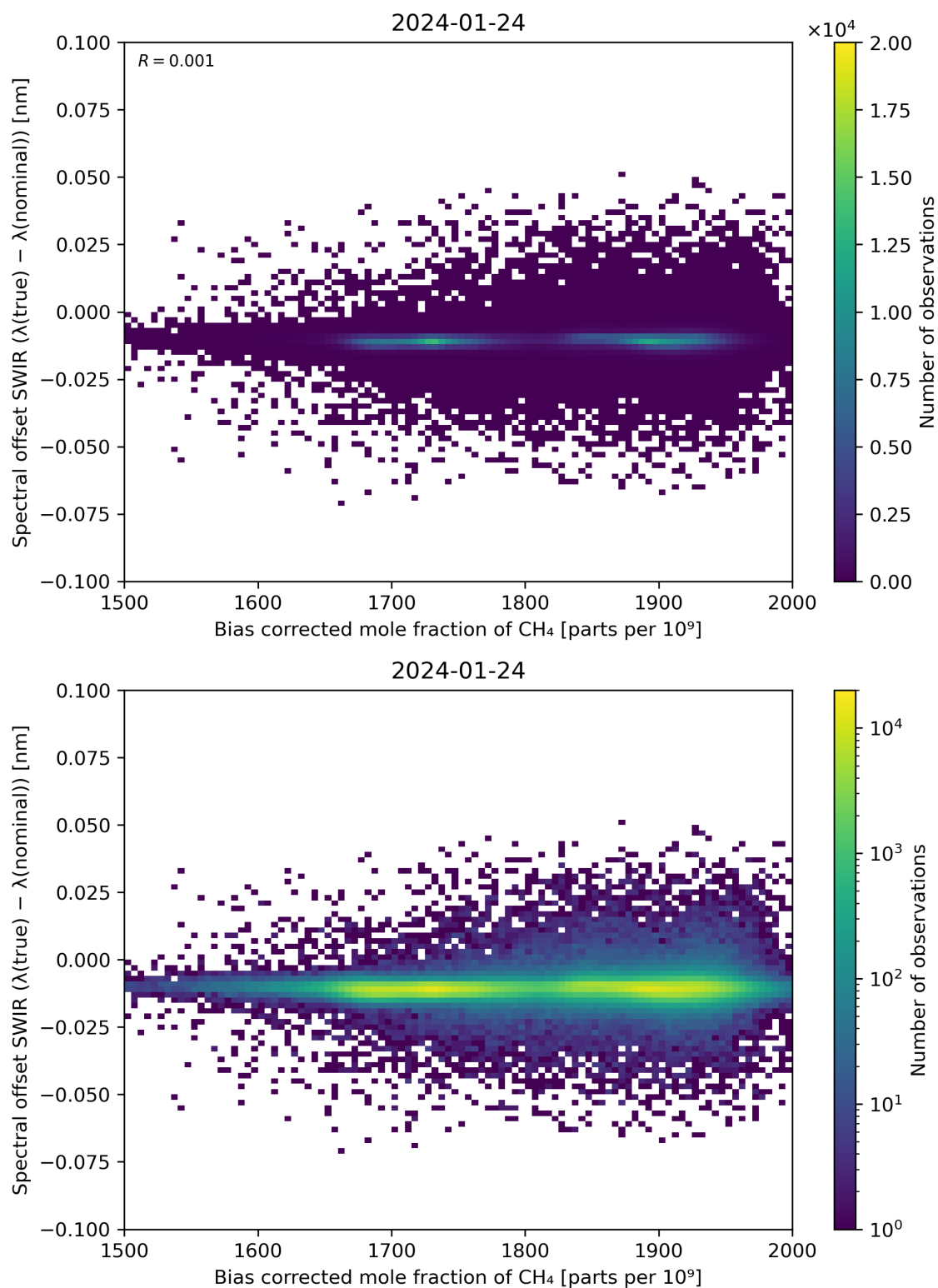
Figure 69: Scatter density plot of “Bias corrected mole fraction of \text{CH}_4 ” against “Spectral offset SWIR ( \lambda(\text{true}) - \lambda(\text{nominal}) )” for 2024-01-23 to 2024-01-25.
