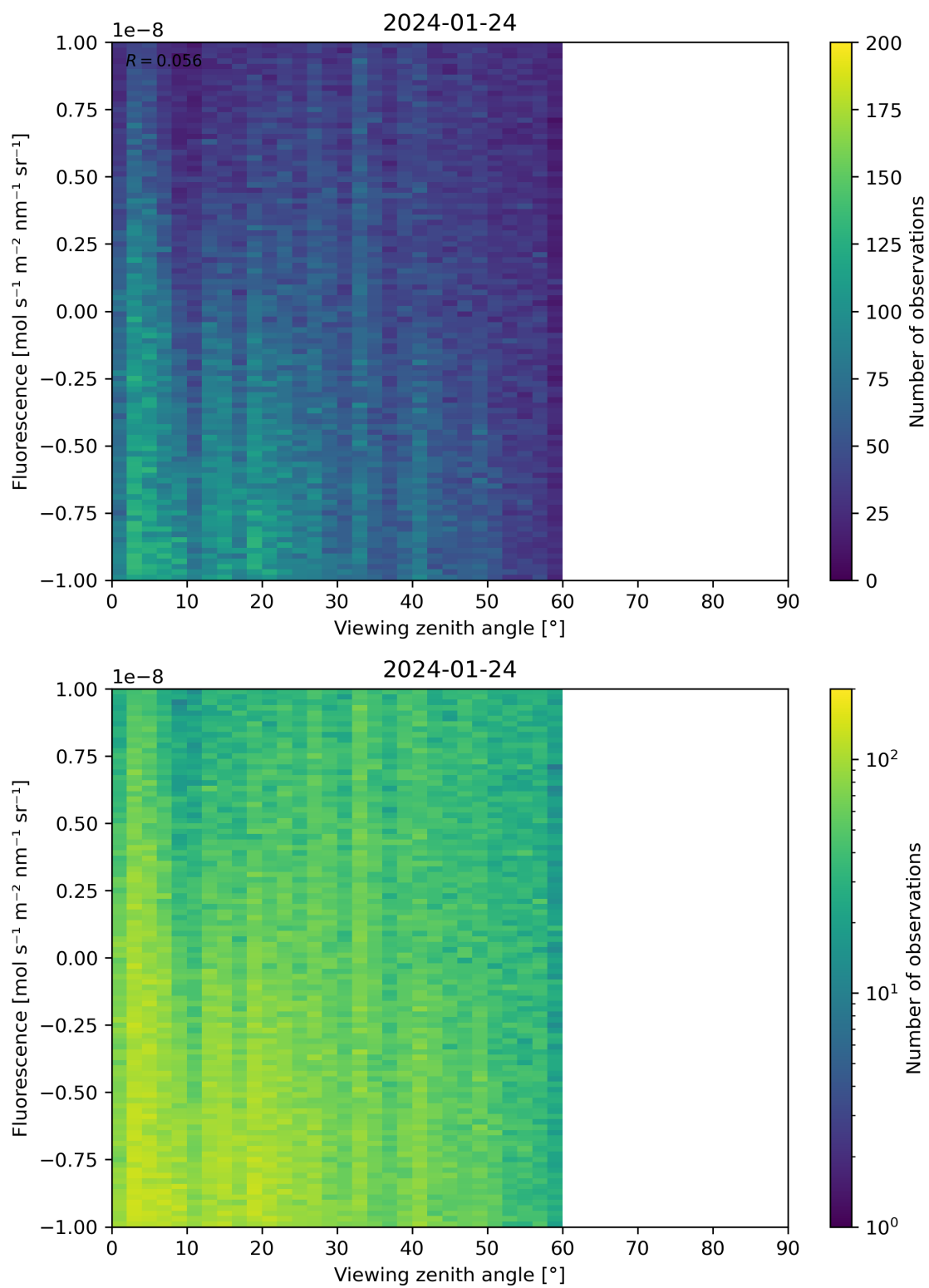
Figure 108: Scatter density plot of “Viewing zenith angle” against “Fluorescence” for 2024-01-23 to 2024-01-25.
