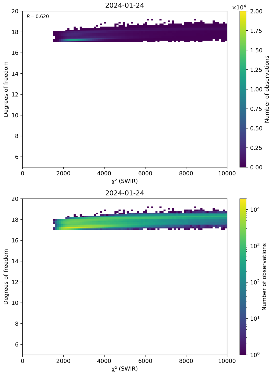
Figure 48: Scatter density plot of “ \chi^2 (SWIR)” against “Degrees of freedom” for 2024-01-23 to 2024-01-25.
