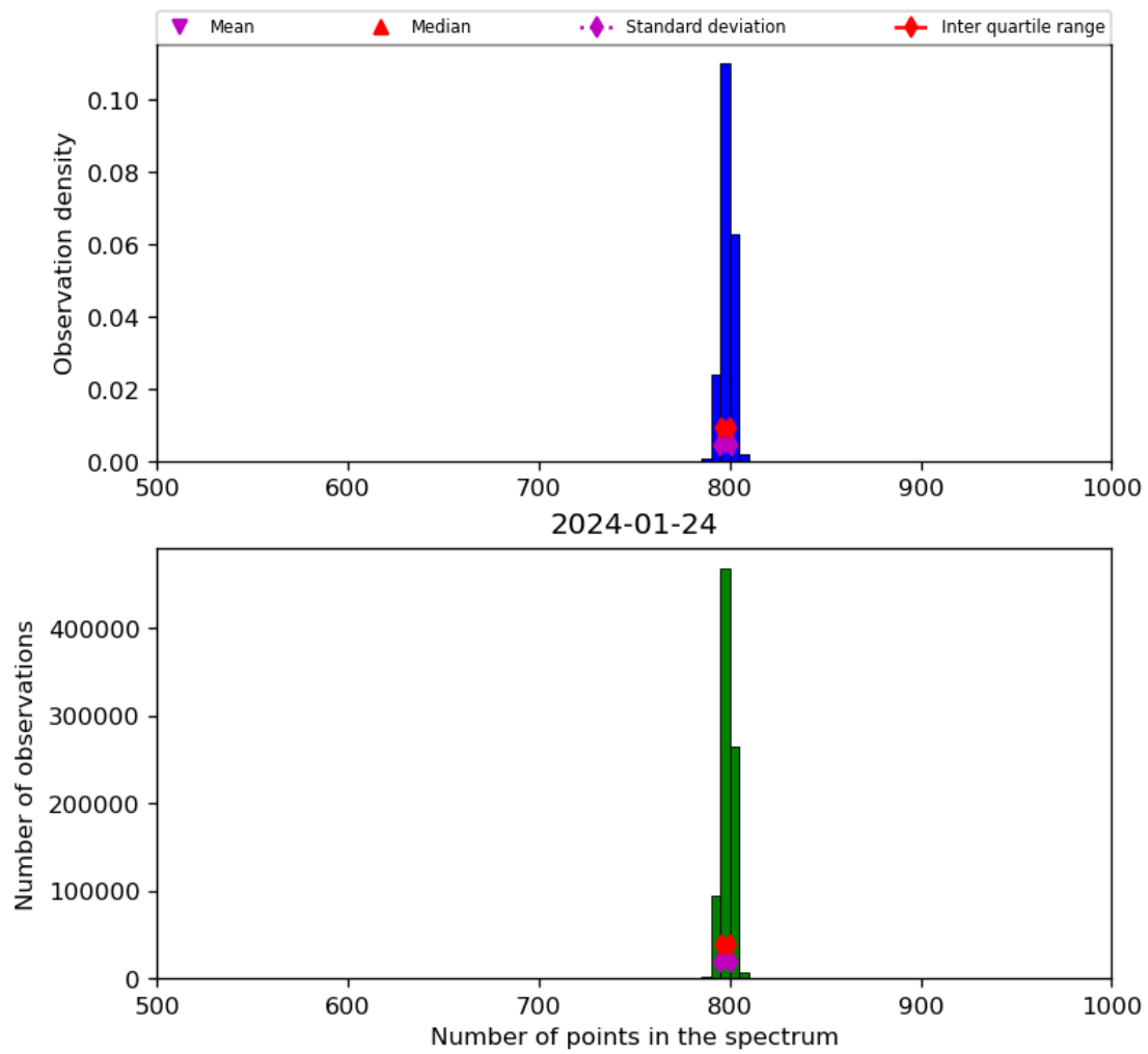
Figure 26: Histogram of “Number of points in the spectrum” for 2024-01-23 to 2024-01-25
