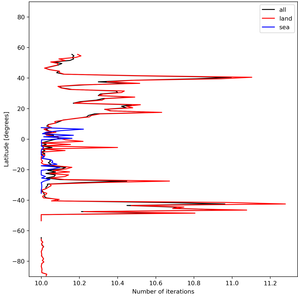
Figure 20: Zonal average of “Number of iterations” for 2024-01-23 to 2024-01-25.
