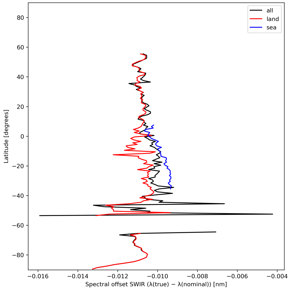
Figure 16: Zonal average of “Spectral offset SWIR ( \lambda(\text{true}) - \lambda(\text{nominal}) )” for 2024-01-23 to 2024-01-25.
