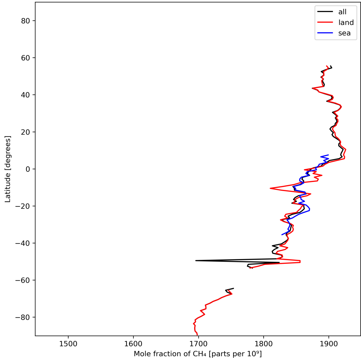
Figure 12: Zonal average of “Mole fraction of \text{CH}_4 ” for 2024-01-23 to 2024-01-25.
