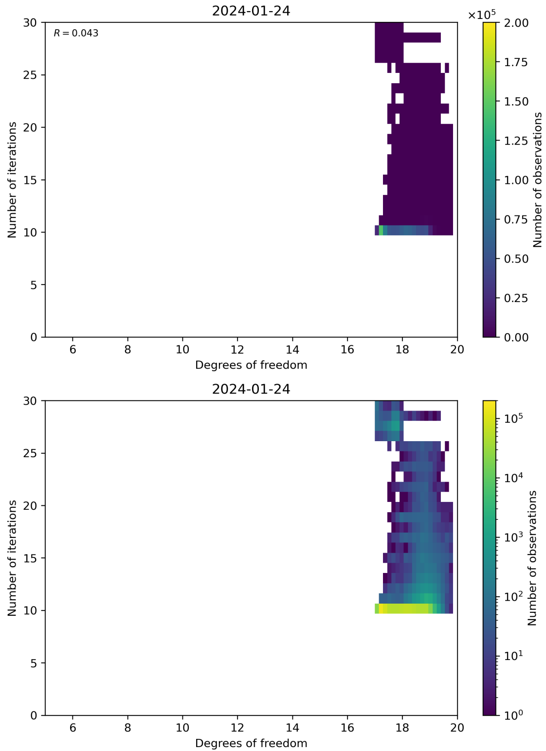
Figure 52: Scatter density plot of “Degrees of freedom” against “Number of iterations” for 2024-01-23 to 2024-01-25.
