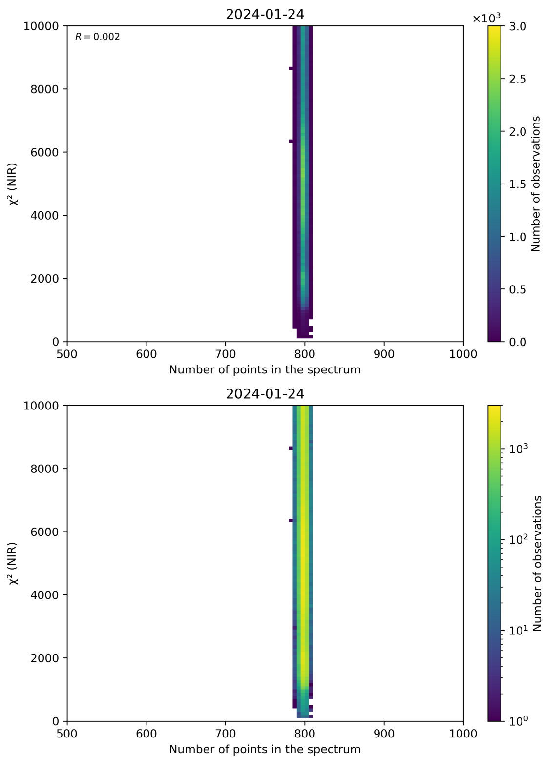
Figure 88: Scatter density plot of “Number of points in the spectrum” against “ \chi^2 (NIR)” for 2024-01-23 to 2024-01-25.
