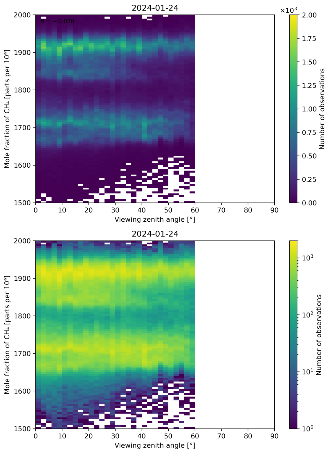
Figure 110: Scatter density plot of “Viewing zenith angle” against “Mole fraction of \text{CH}_4 ” for 2024-01-23 to 2024-01-25.
