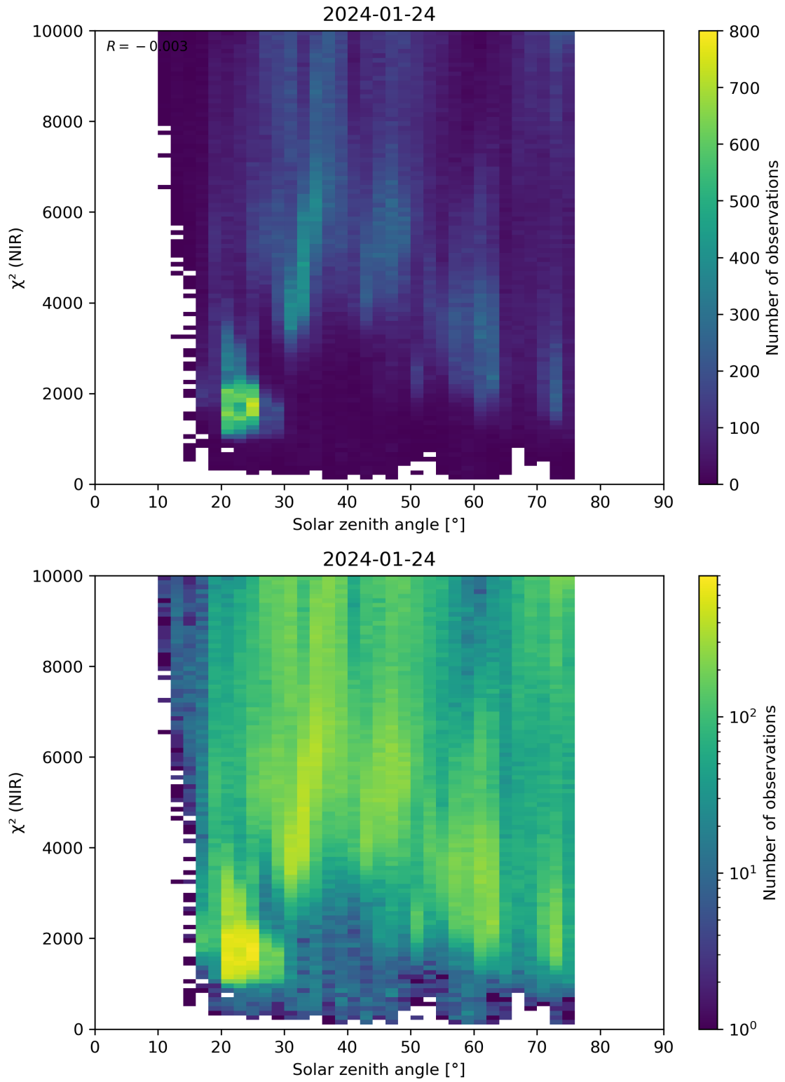
Figure 94: Scatter density plot of “Solar zenith angle” against “ \chi^2 (NIR)” for 2024-01-23 to 2024-01-25.
