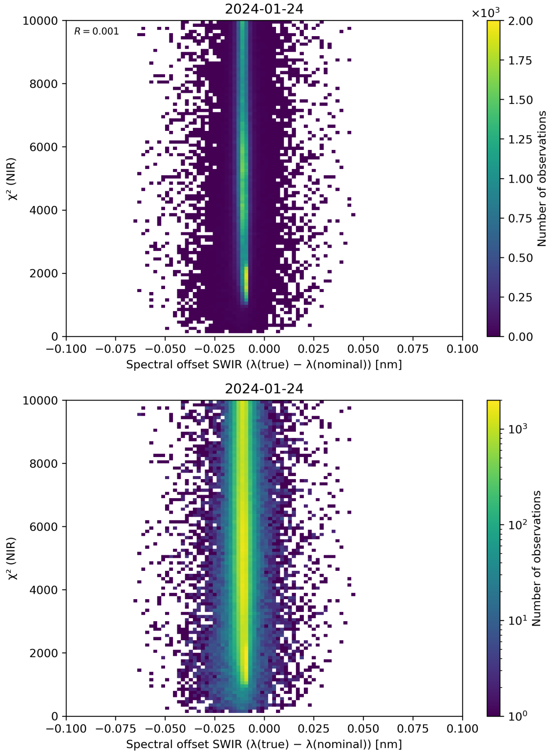
Figure 117: Scatter density plot of “Spectral offset SWIR ( \lambda(\text{true}) - \lambda(\text{nominal}) )” against “ \chi^2 (NIR)” for 2024-01-23 to 2024-01-25.
