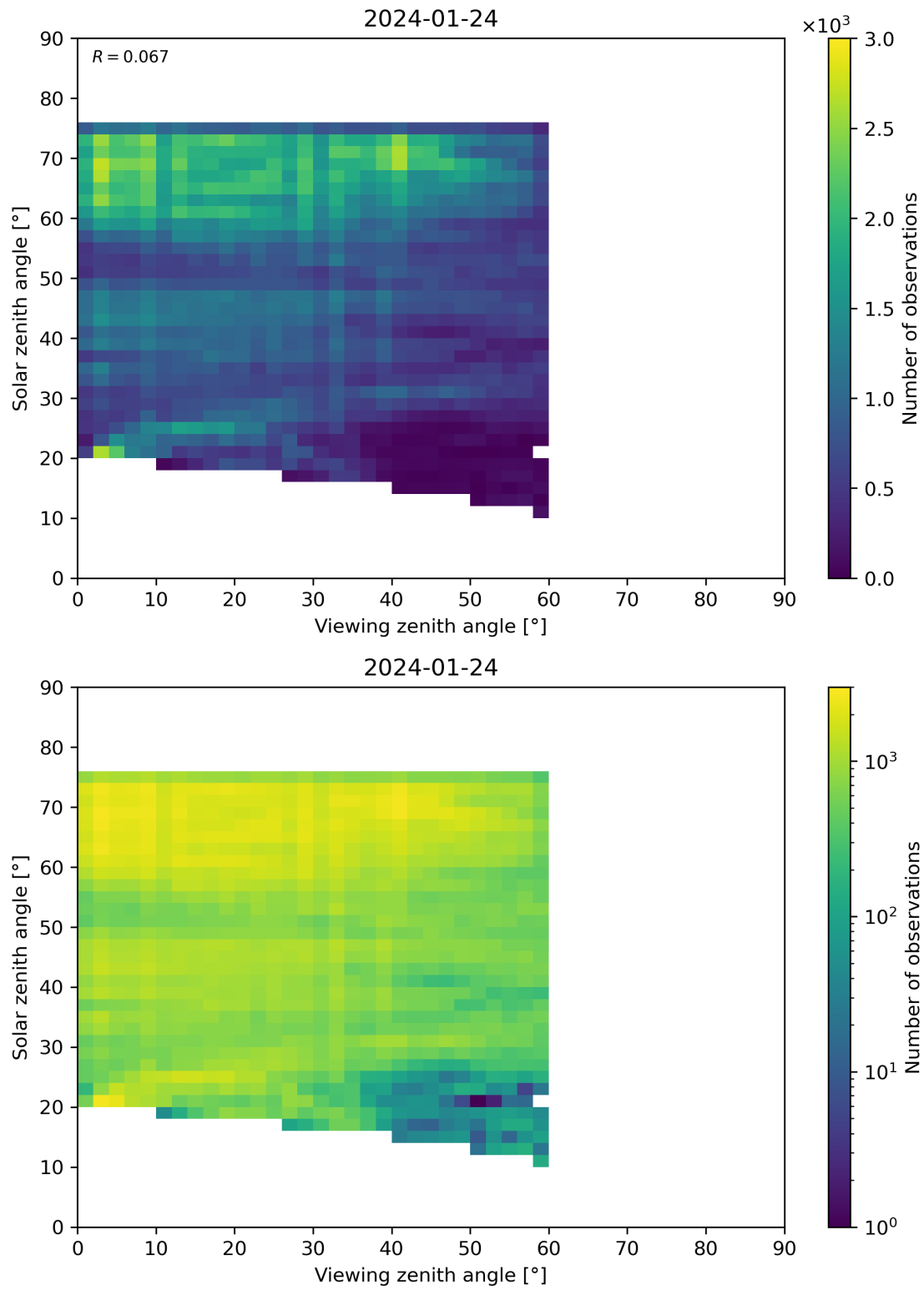
Figure 115: Scatter density plot of “Viewing zenith angle” against “Solar zenith angle” for 2024-01-23 to 2024-01-25.
