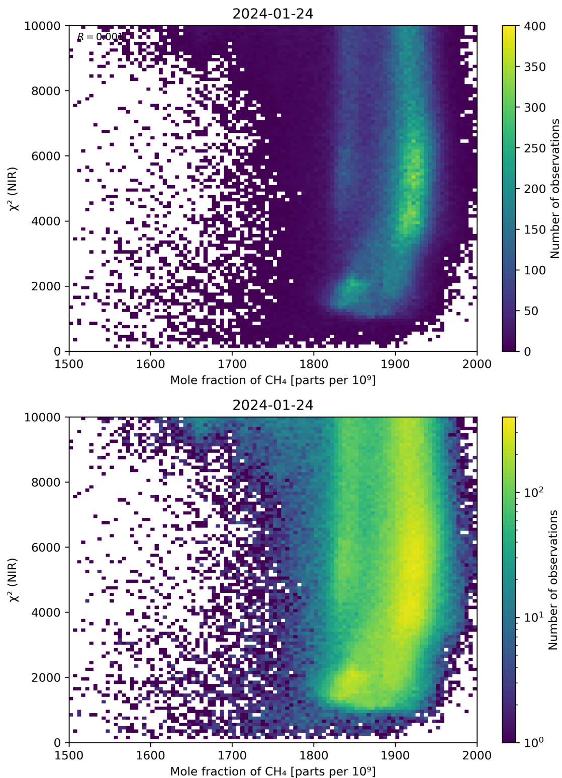
Figure 70: Scatter density plot of “Mole fraction of \text{CH}_4 ” against “ \chi^2 (NIR)” for 2024-01-23 to 2024-01-25.
