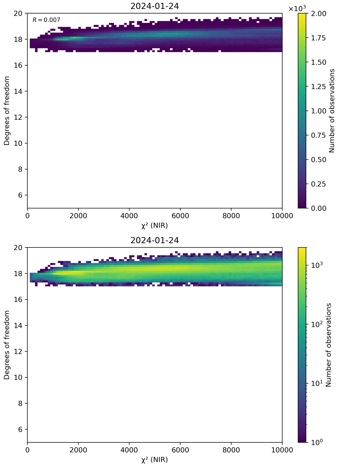
Figure 44: Scatter density plot of “ \chi^2 (NIR)” against “Degrees of freedom” for 2024-01-23 to 2024-01-25.
