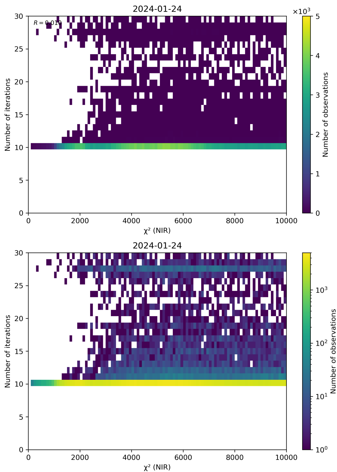
Figure 46: Scatter density plot of “ \chi^2 (NIR)” against “Number of iterations” for 2024-01-23 to 2024-01-25.
