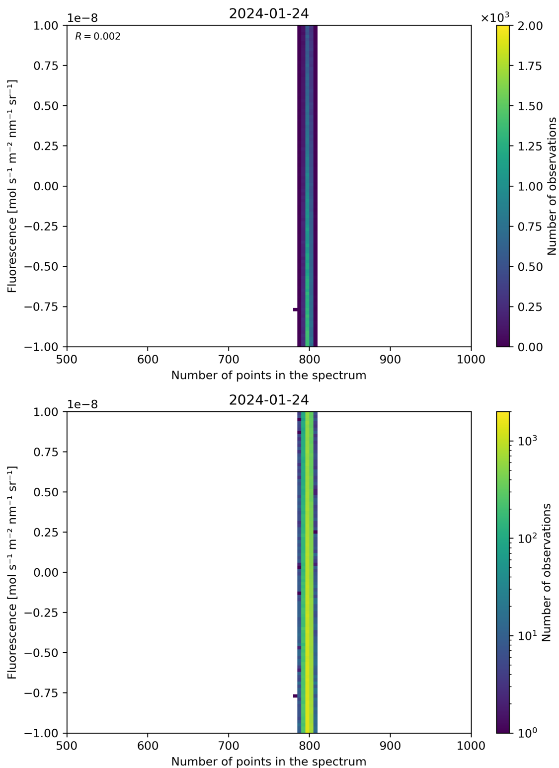
Figure 91: Scatter density plot of “Number of points in the spectrum” against “Fluorescence” for 2024-01-23 to 2024-01-25.
