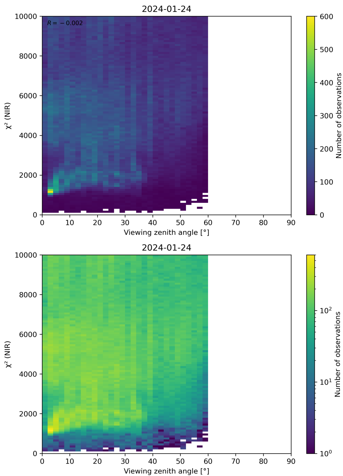
Figure 105: Scatter density plot of “Viewing zenith angle” against “ \chi^2 (NIR)” for 2024-01-23 to 2024-01-25.
