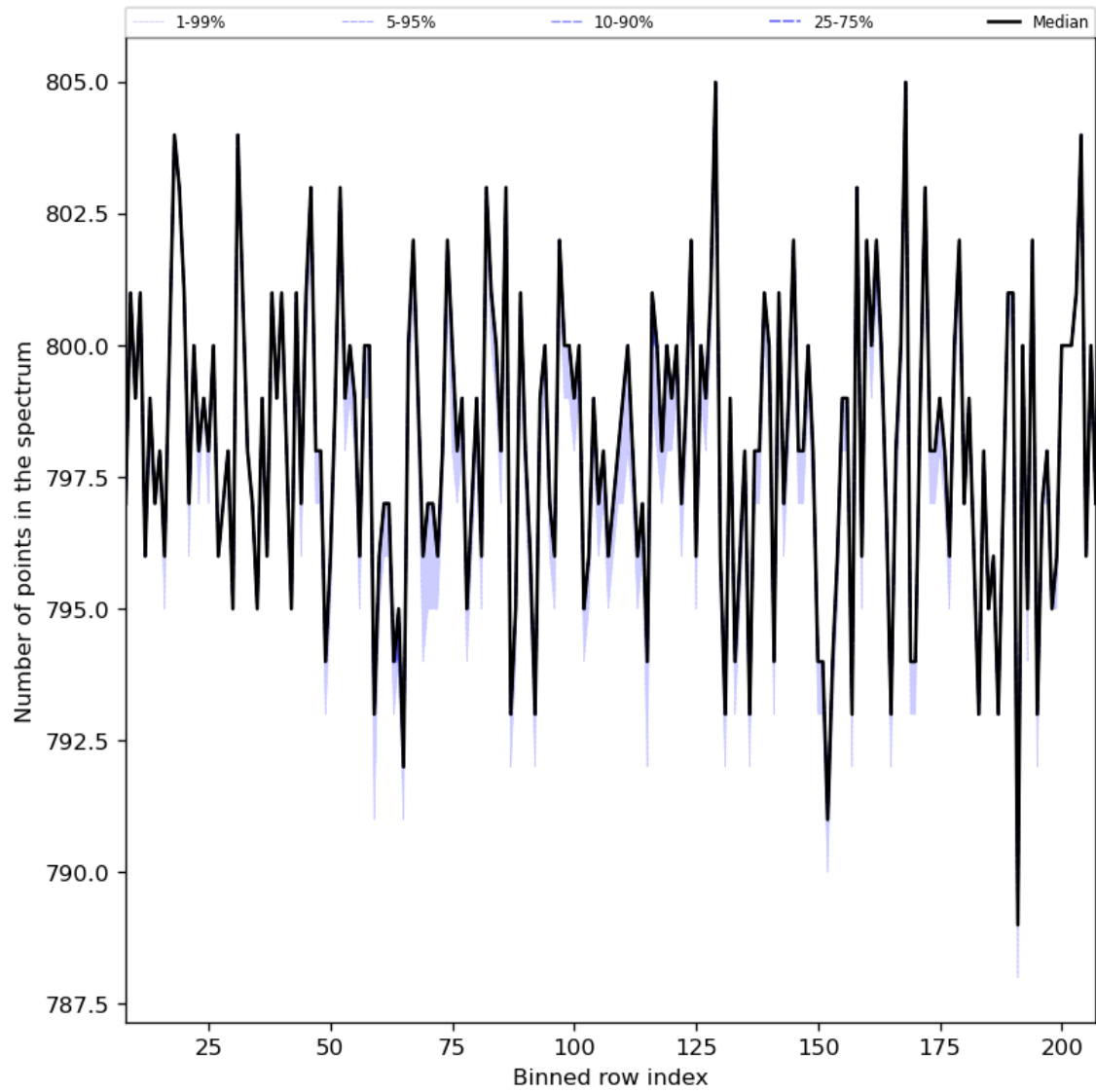
Figure 37: Along track statistics of “Number of points in the spectrum” for 2024-01-23 to 2024-01-25
