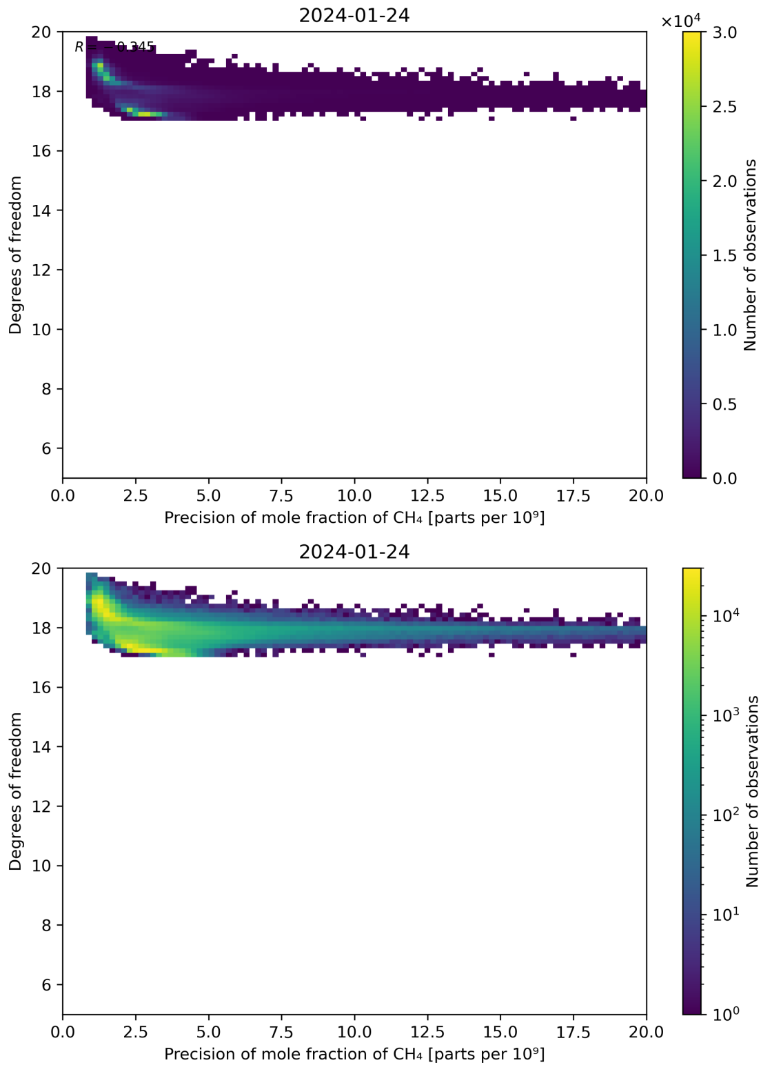
Figure 80: Scatter density plot of “Precision of mole fraction of CH 4 ” against “Degrees of freedom” for 2024-01-23 to 2024-01-25.
