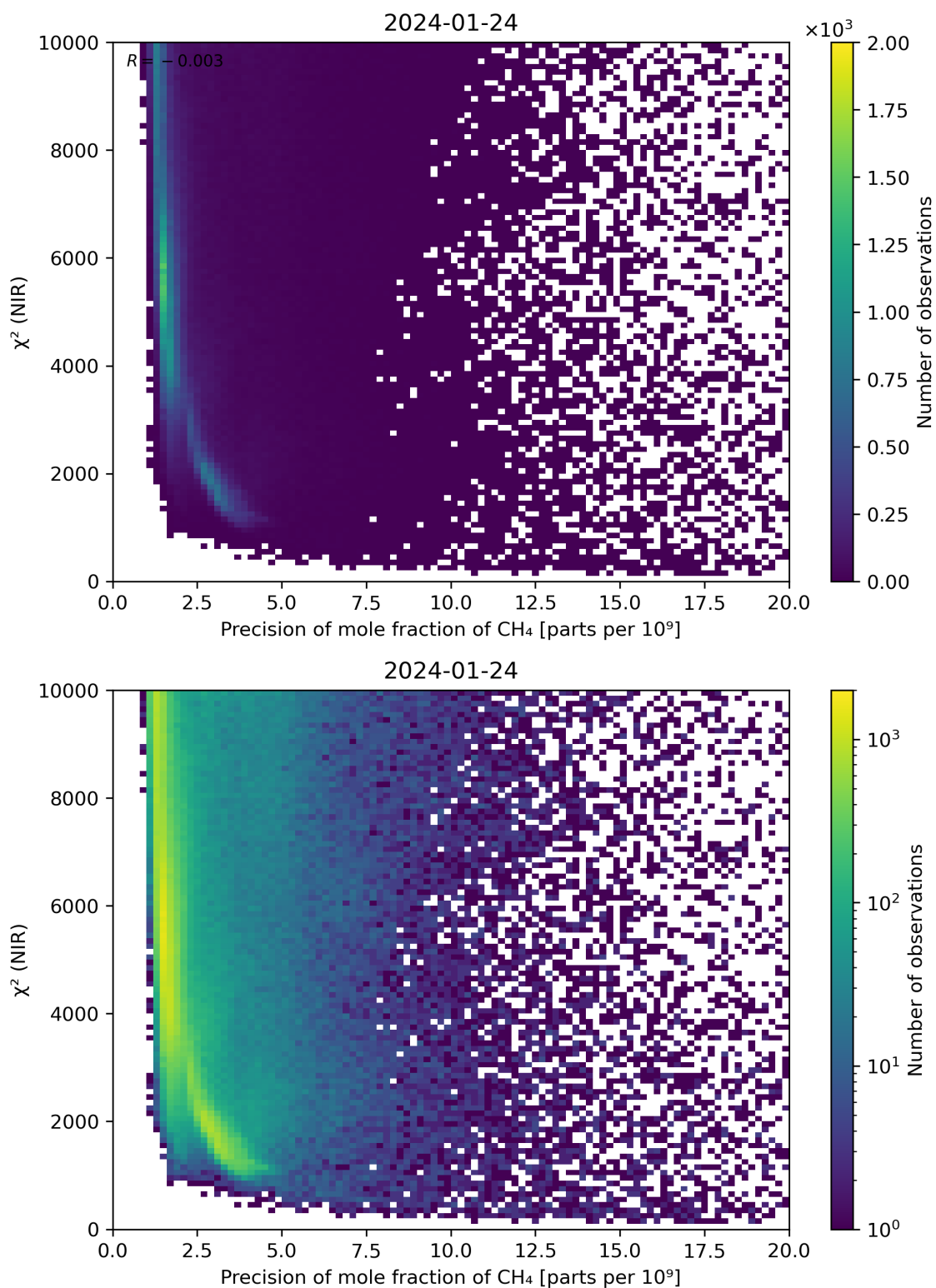
Figure 78: Scatter density plot of “Precision of mole fraction of CH 4 ” against “ \chi^2 (NIR)” for 2024-01-23 to 2024-01-25.
