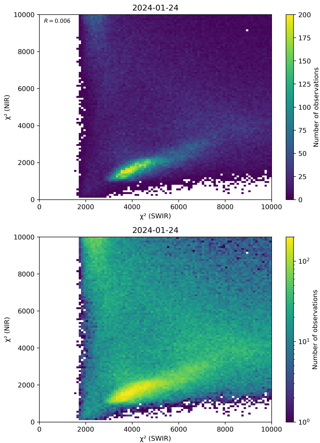
Figure 47: Scatter density plot of “ \chi^2 (SWIR)” against “ \chi^2 (NIR)” for 2024-01-23 to 2024-01-25.
