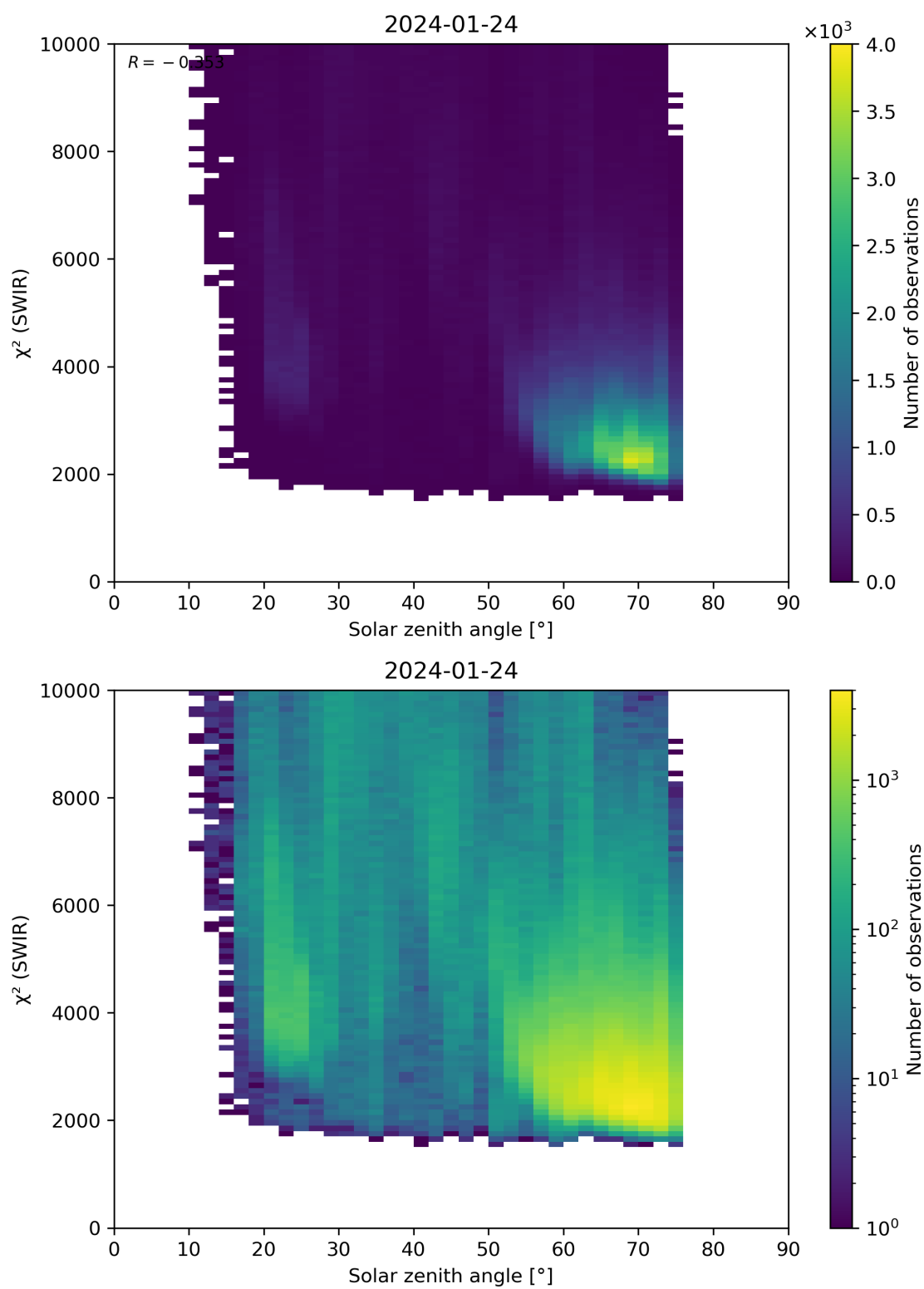
Figure 95: Scatter density plot of “Solar zenith angle” against “ \chi^2 (SWIR)” for 2024-01-23 to 2024-01-25.
