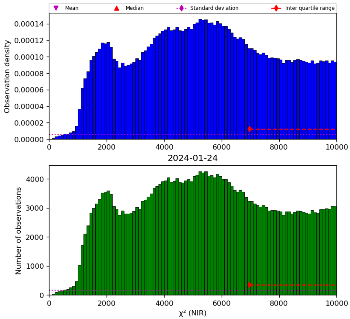
Figure 29: Histogram of “ \chi^2 (NIR)” for 2024-01-23 to 2024-01-25
