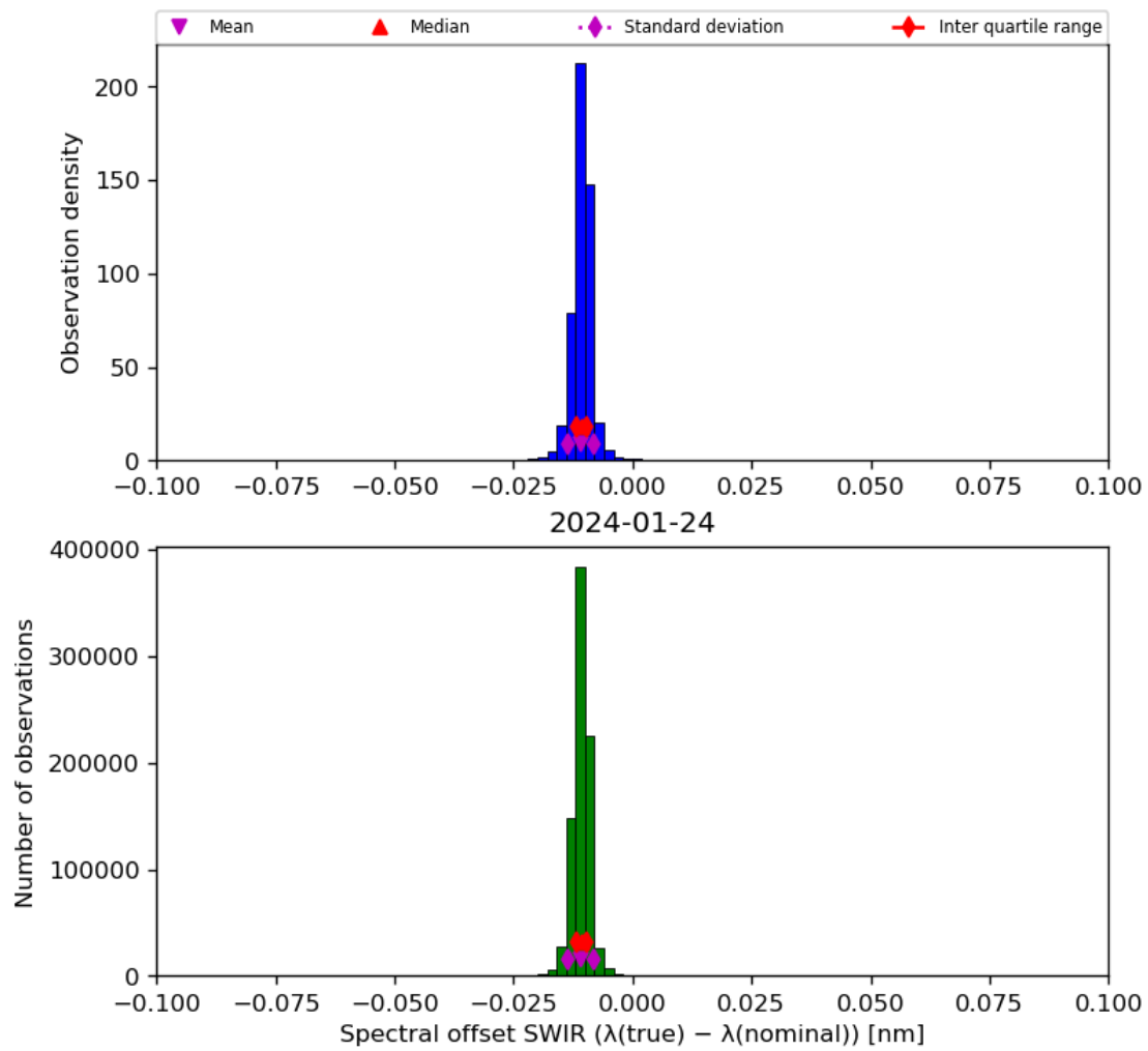
Figure 27: Histogram of “Spectral offset SWIR ( \lambda(\text{true}) - \lambda(\text{nominal}) )” for 2024-01-23 to 2024-01-25
