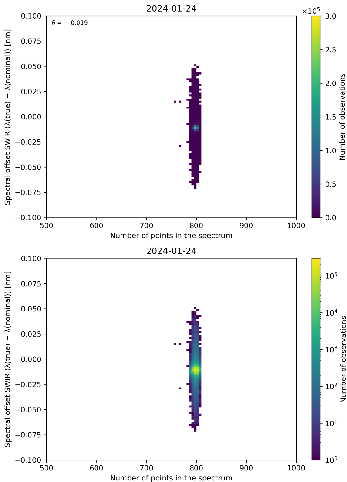
Figure 93: Scatter density plot of “Number of points in the spectrum” against “Spectral offset SWIR ( \lambda(\text{true}) - \lambda(\text{nominal}) )” for 2024-01-23 to 2024-01-25.
