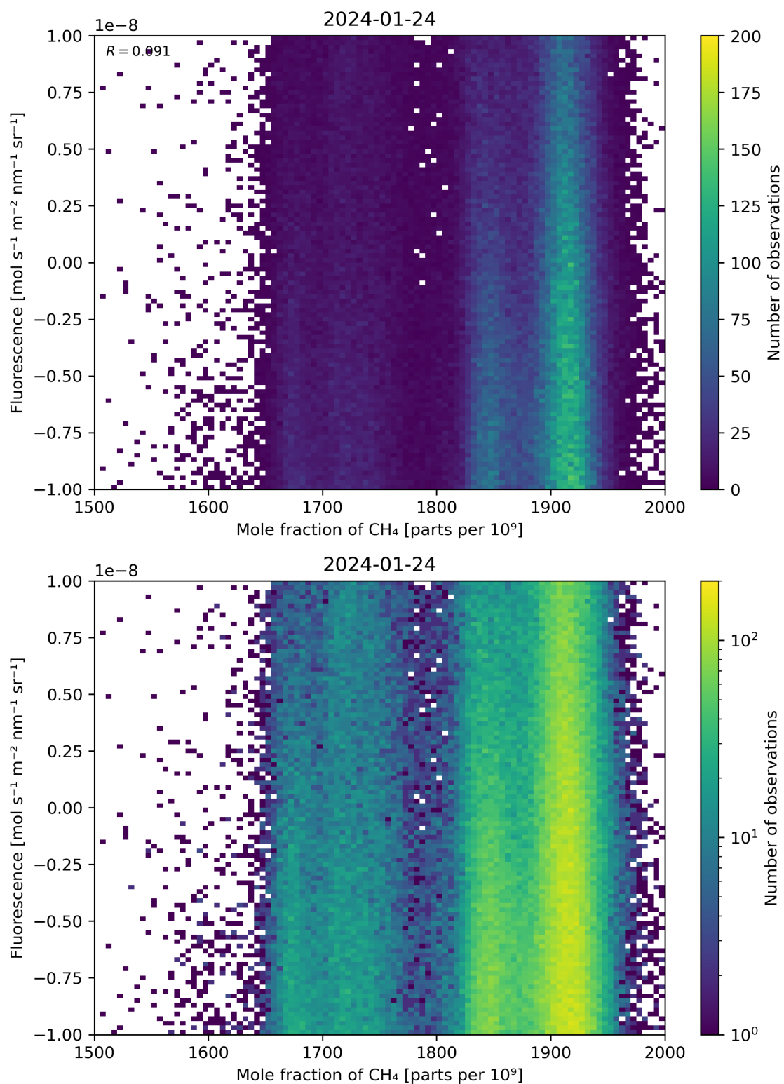
Figure 73: Scatter density plot of “Mole fraction of \text{CH}_4 ” against “Fluorescence” for 2024-01-23 to 2024-01-25.
