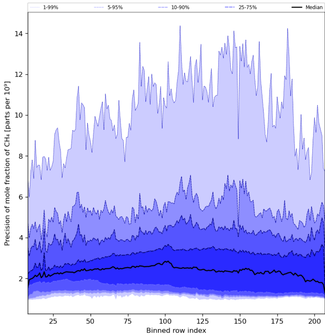
Figure 35: Along track statistics of “Precision of mole fraction of CH 4 ” for 2024-01-23 to 2024-01-25
