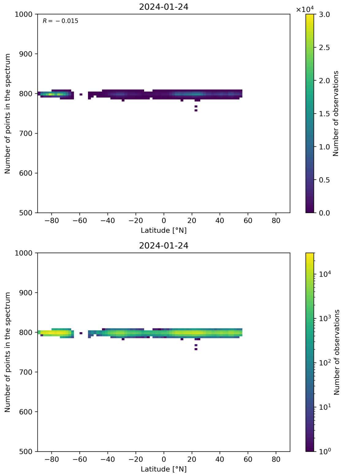
Figure 61: Scatter density plot of “Latitude” against “Number of points in the spectrum” for 2024-01-23 to 2024-01-25.
