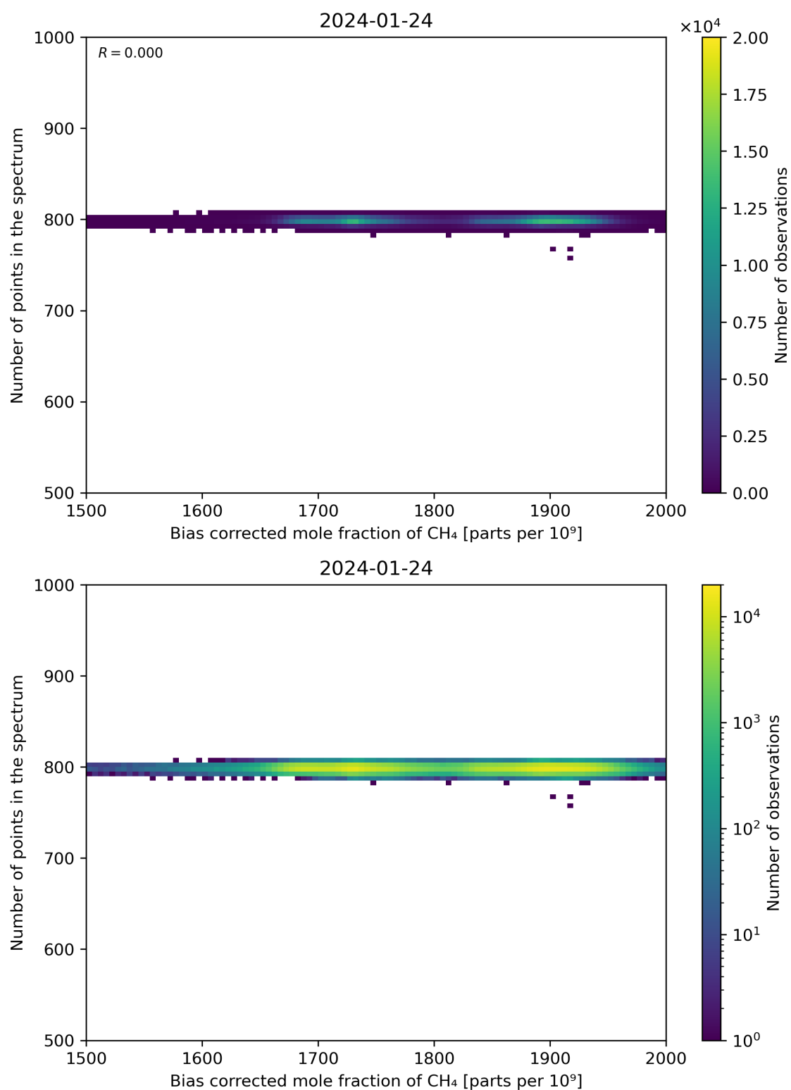
Figure 68: Scatter density plot of “Bias corrected mole fraction of CH 4 ” against “Number of points in the spectrum” for 2024-01-23 to 2024-01-25.
