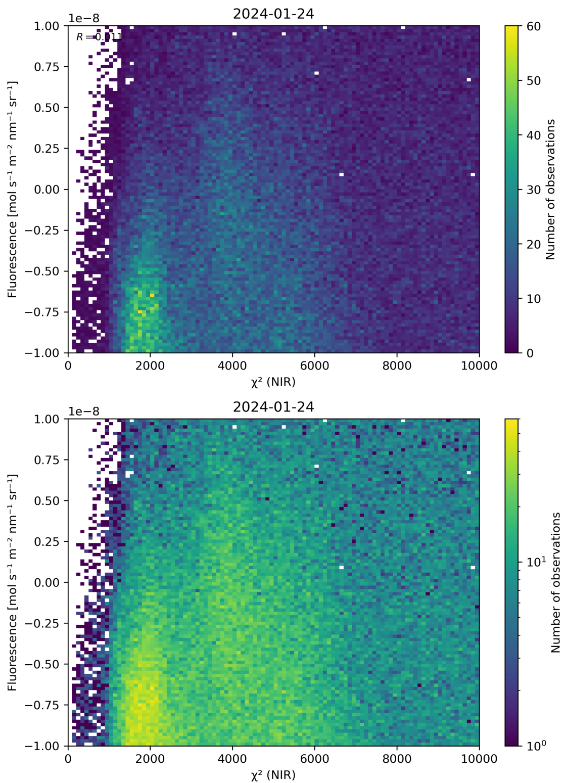
Figure 45: Scatter density plot of “ \chi^2 (NIR)” against “Fluorescence” for 2024-01-23 to 2024-01-25.
