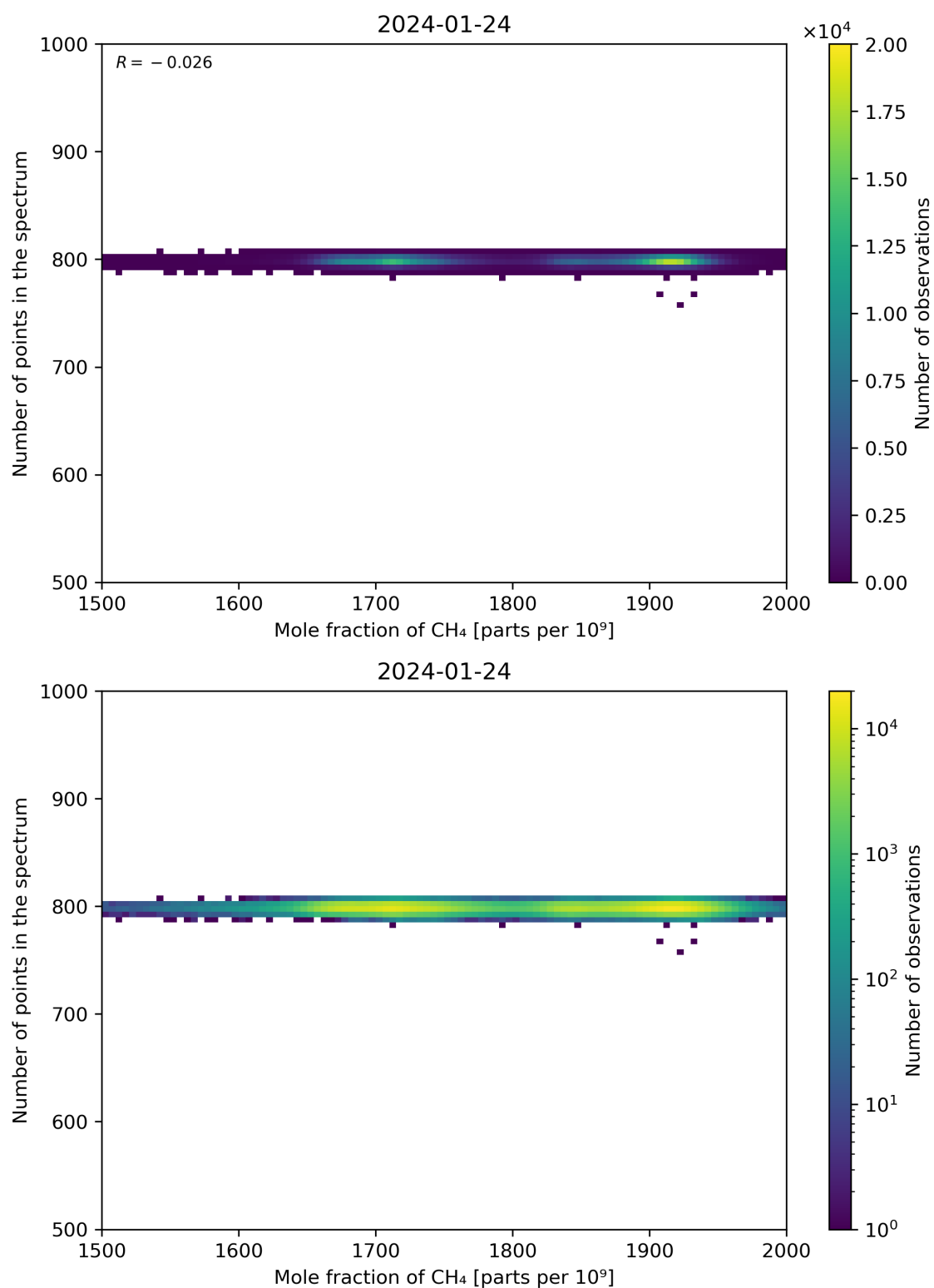
Figure 77: Scatter density plot of “Mole fraction of CH 4 ” against “Number of points in the spectrum” for 2024-01-23 to 2024-01-25.
