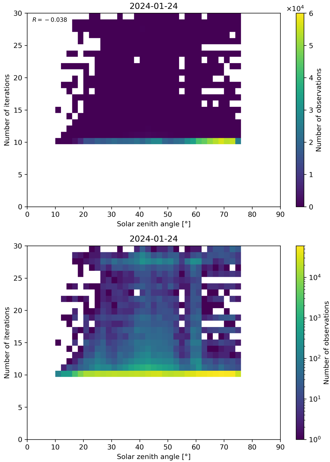
Figure 102: Scatter density plot of “Solar zenith angle” against “Number of iterations” for 2024-01-23 to 2024-01-25.
