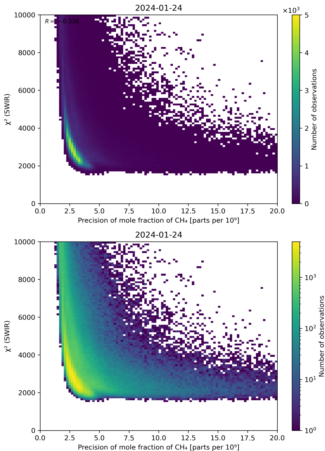
Figure 79: Scatter density plot of “Precision of mole fraction of CH 4 ” against “ \chi^2 (SWIR)” for 2024-01-23 to 2024-01-25.
