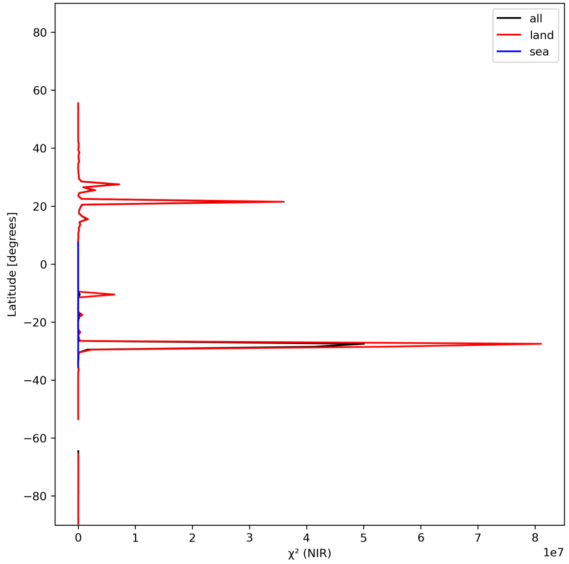
Figure 18: Zonal average of “ \chi^2 (NIR)” for 2024-01-23 to 2024-01-25.
