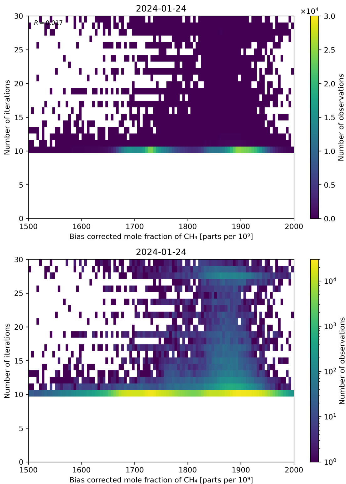
Figure 67: Scatter density plot of “Bias corrected mole fraction of \text{CH}_4 ” against “Number of iterations” for 2024-01-23 to 2024-01-25.
