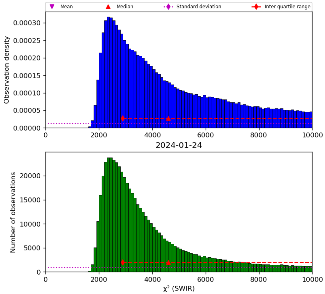
Figure 28: Histogram of “ \chi^2 (SWIR)” for 2024-01-23 to 2024-01-25
