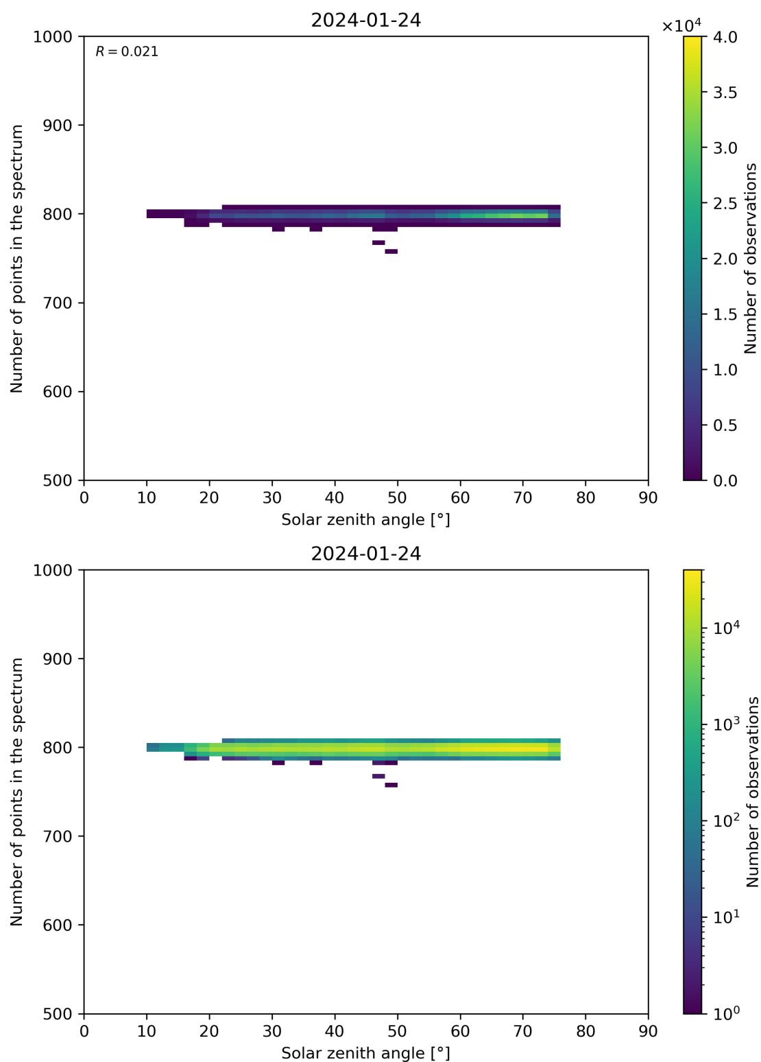
Figure 103: Scatter density plot of “Solar zenith angle” against “Number of points in the spectrum” for 2024-01-23 to 2024-01-25.
