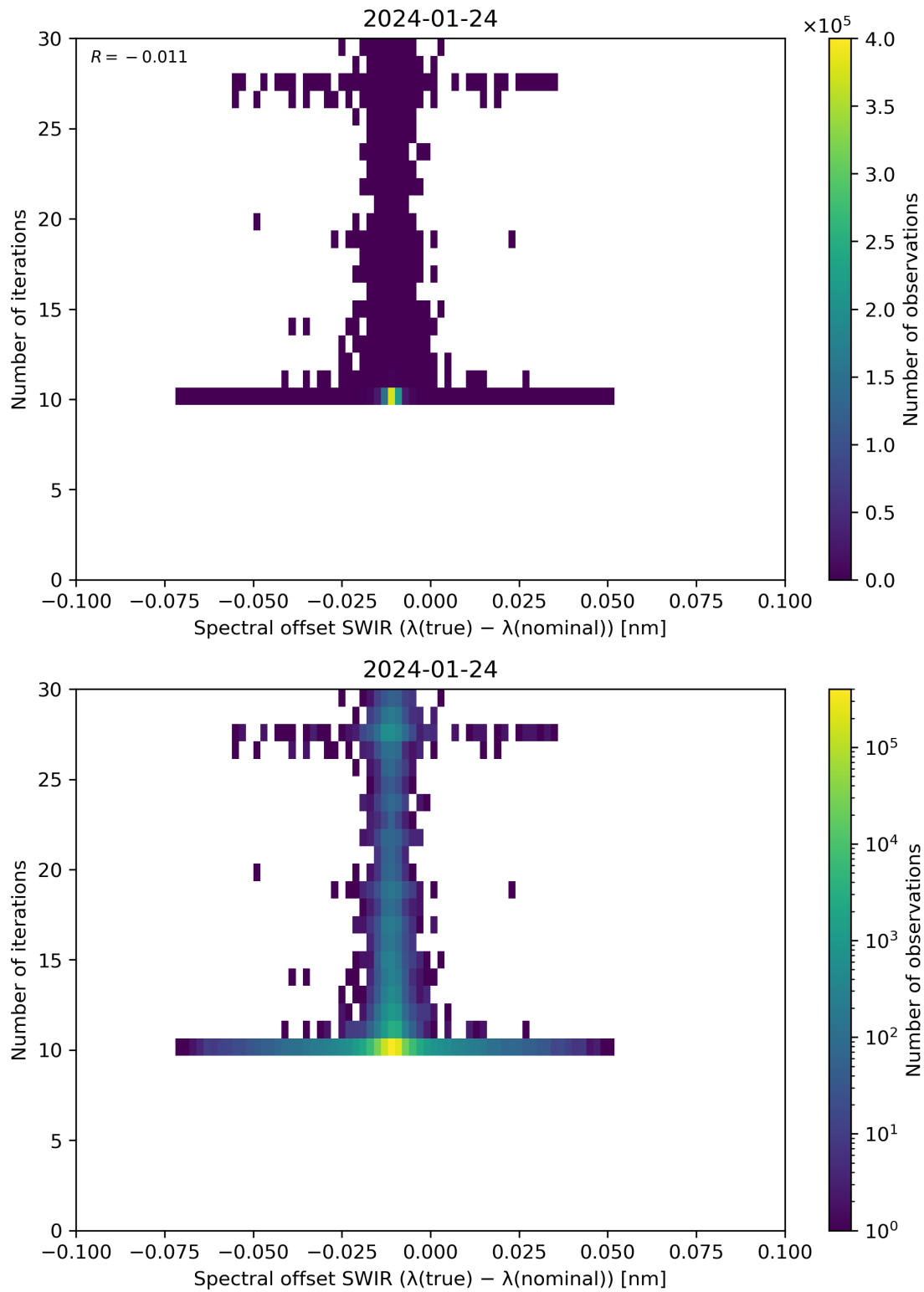
Figure 121: Scatter density plot of “Spectral offset SWIR ( \lambda(\text{true}) - \lambda(\text{nominal}) )” against “Number of iterations” for 2024-01-23 to 2024-01-25.
