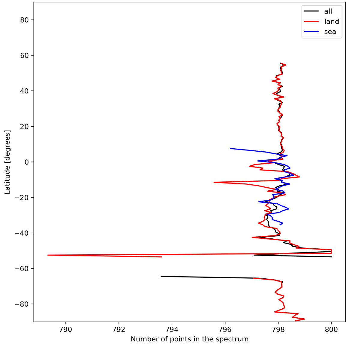
Figure 15: Zonal average of “Number of points in the spectrum” for 2024-01-23 to 2024-01-25.
