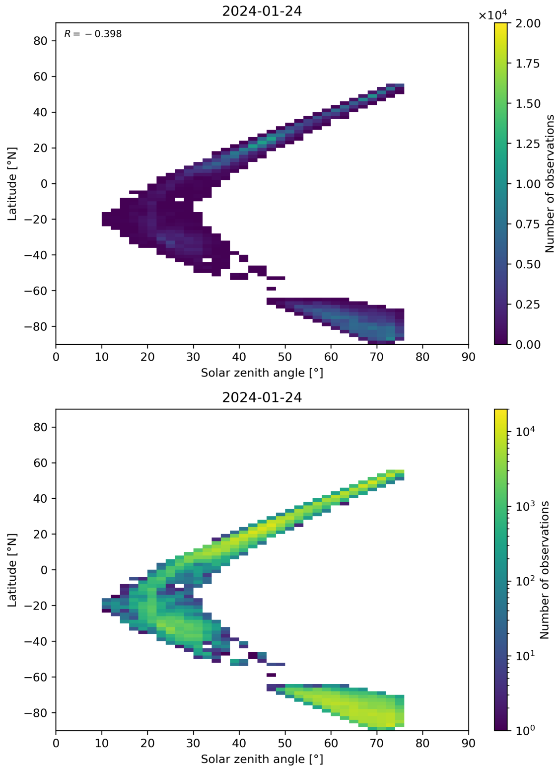
Figure 98: Scatter density plot of “Solar zenith angle” against “Latitude” for 2024-01-23 to 2024-01-25.
