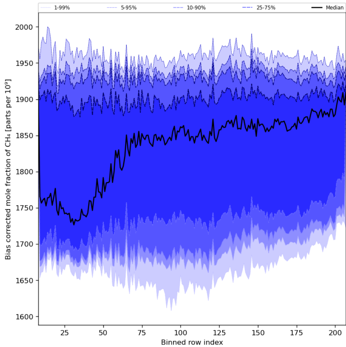
Figure 36: Along track statistics of “Bias corrected mole fraction of CH 4 ” for 2024-01-23 to 2024-01-25
