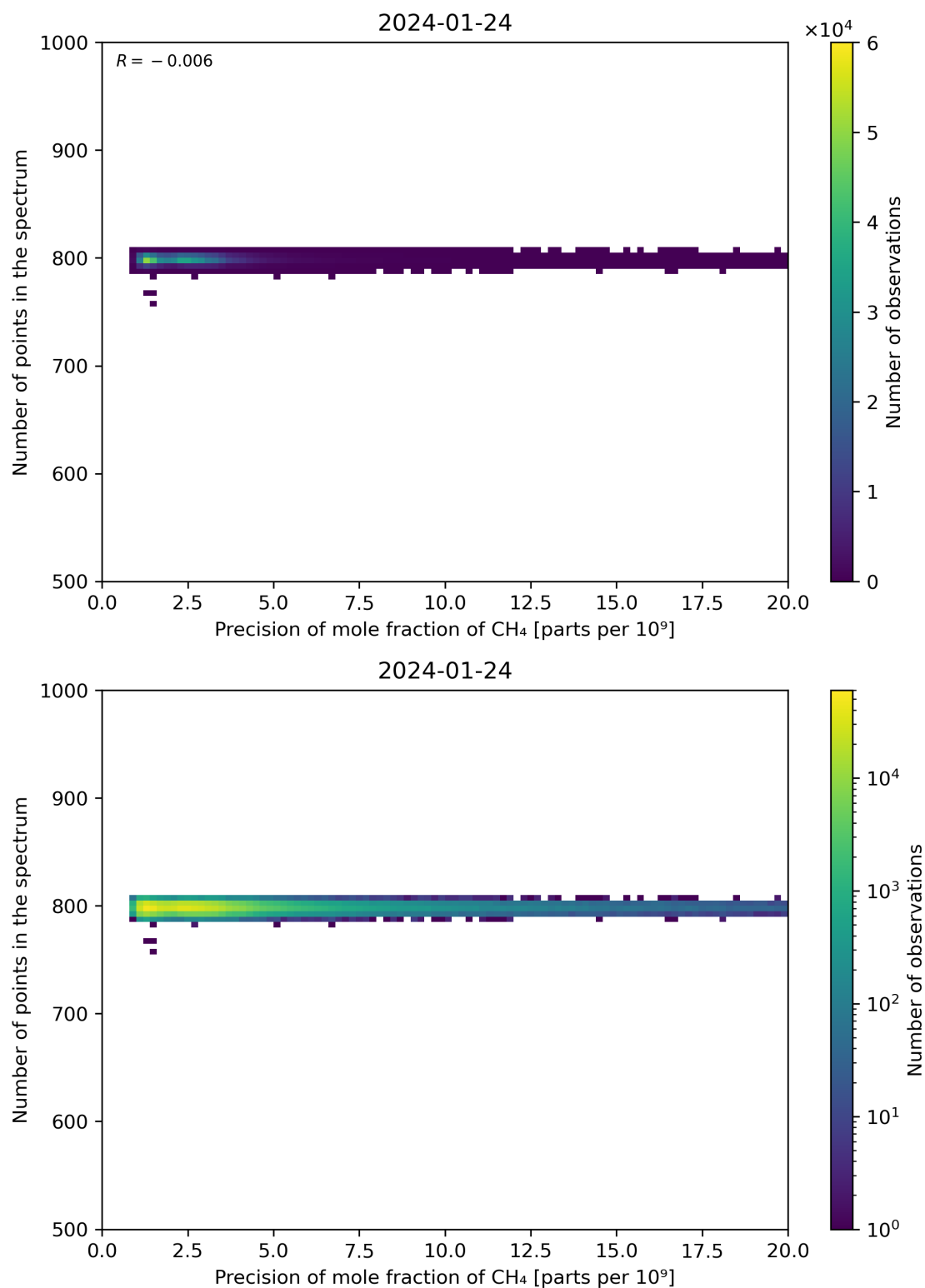
Figure 84: Scatter density plot of “Precision of mole fraction of CH 4 ” against “Number of points in the spectrum” for 2024-01-23 to 2024-01-25.
