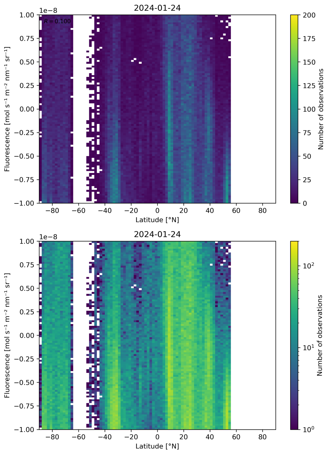
Figure 56: Scatter density plot of “Latitude” against “Fluorescence” for 2024-01-23 to 2024-01-25.
