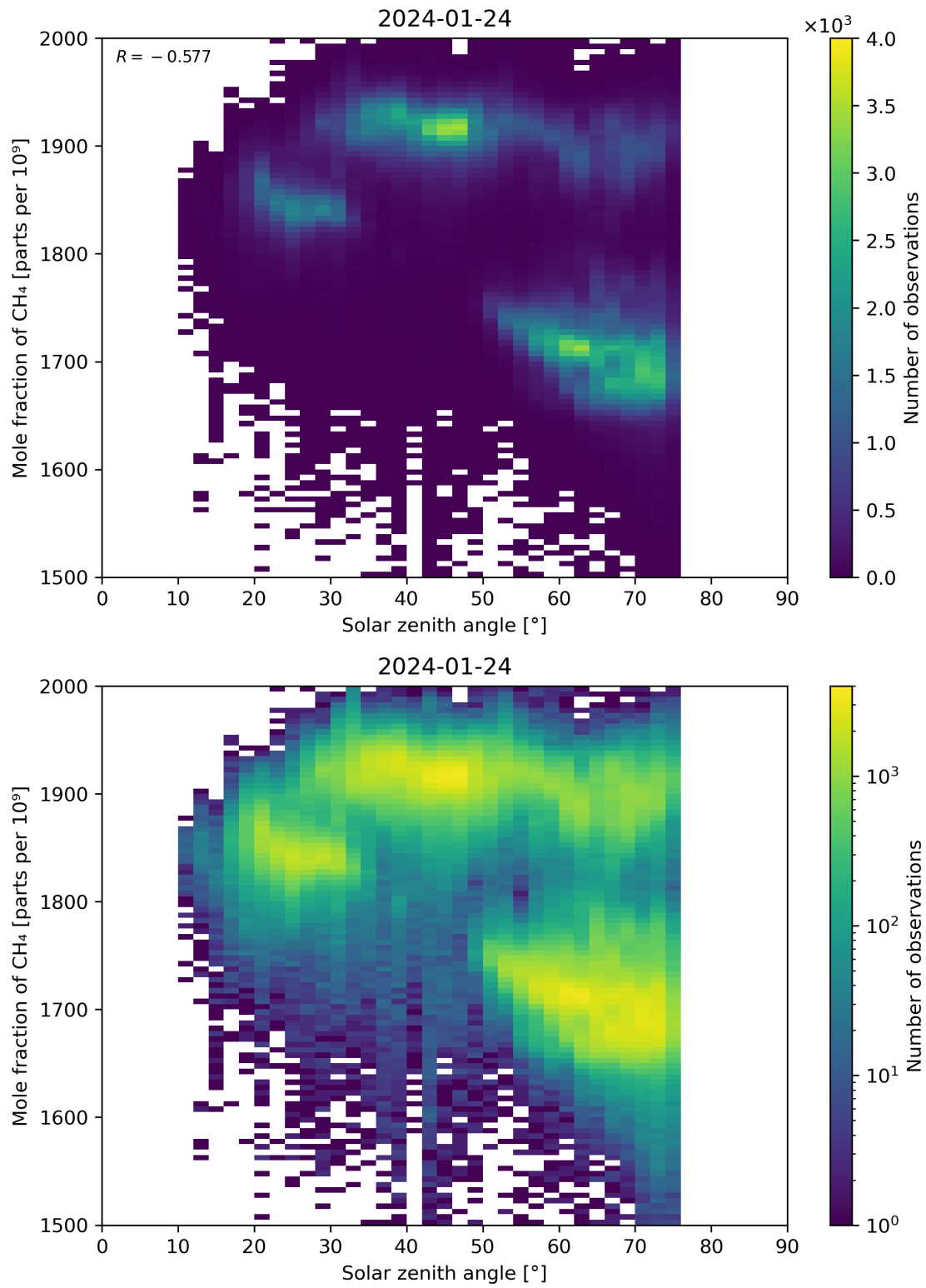
Figure 99: Scatter density plot of “Solar zenith angle” against “Mole fraction of CH 4 ” for 2024-01-23 to 2024-01-25.
