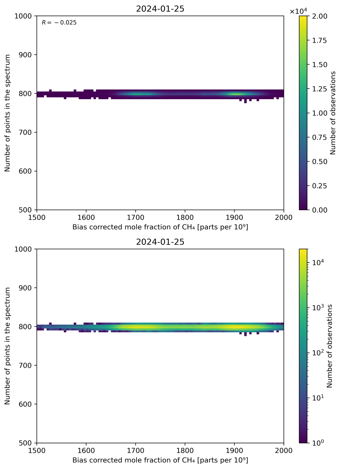
Figure 68: Scatter density plot of “Bias corrected mole fraction of CH 4 ” against “Number of points in the spectrum” for 2024-01-24 to 2024-01-26.
