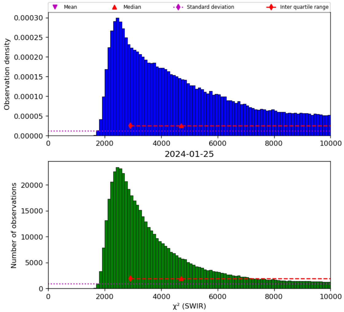
Figure 28: Histogram of “ \chi^2 (SWIR)” for 2024-01-24 to 2024-01-26
