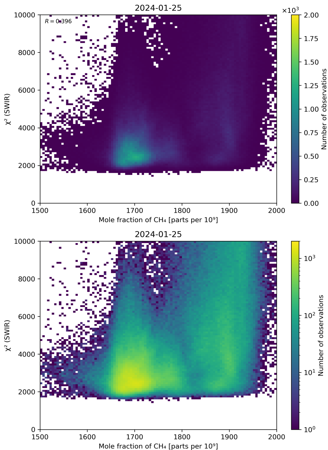
Figure 71: Scatter density plot of “Mole fraction of \text{CH}_4 ” against “ \chi^2 (SWIR)” for 2024-01-24 to 2024-01-26.
