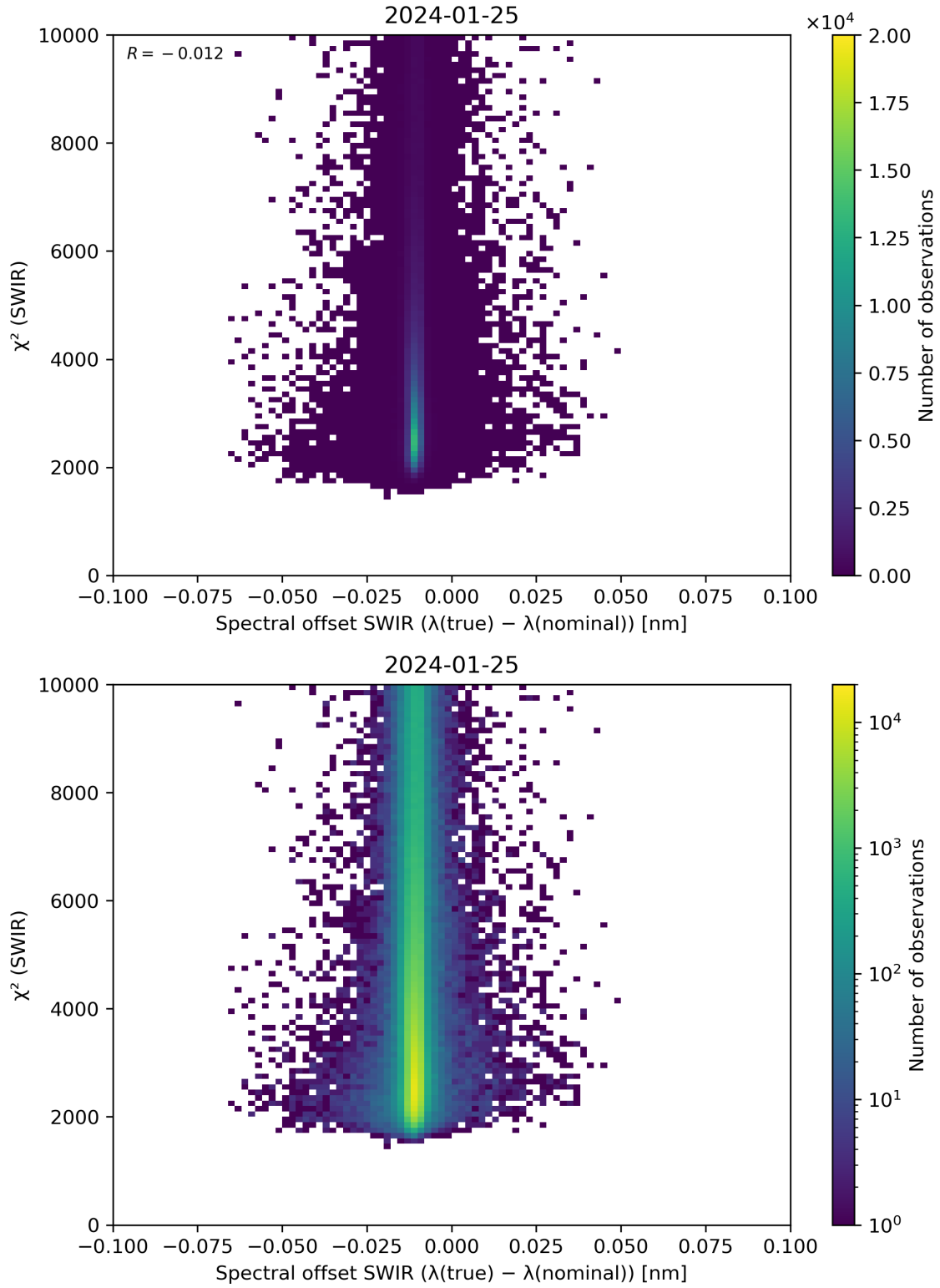
Figure 118: Scatter density plot of “Spectral offset SWIR ( \lambda(\text{true}) - \lambda(\text{nominal}) )” against “ \chi^2 (SWIR)” for 2024-01-24 to 2024-01-26.
