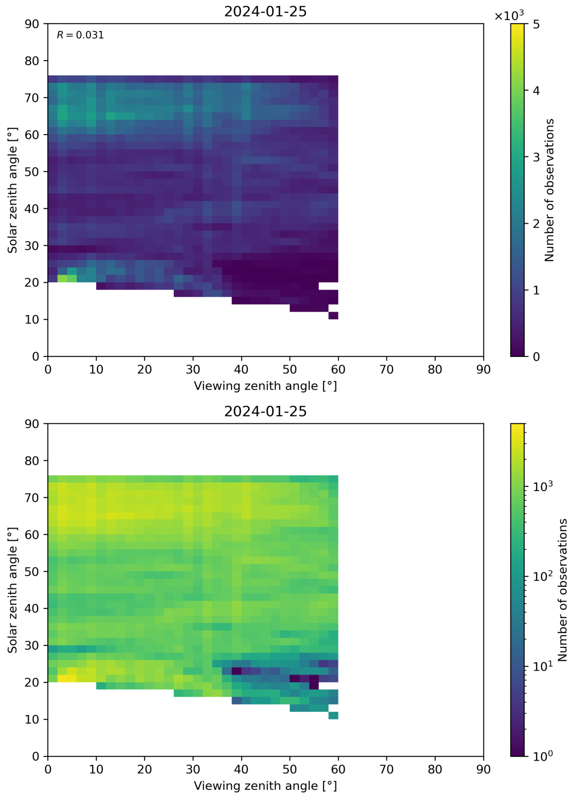
Figure 115: Scatter density plot of “Viewing zenith angle” against “Solar zenith angle” for 2024-01-24 to 2024-01-26.
