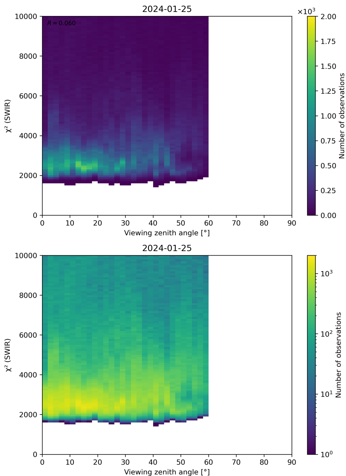
Figure 106: Scatter density plot of “Viewing zenith angle” against “ \chi^2 (SWIR)” for 2024-01-24 to 2024-01-26.
