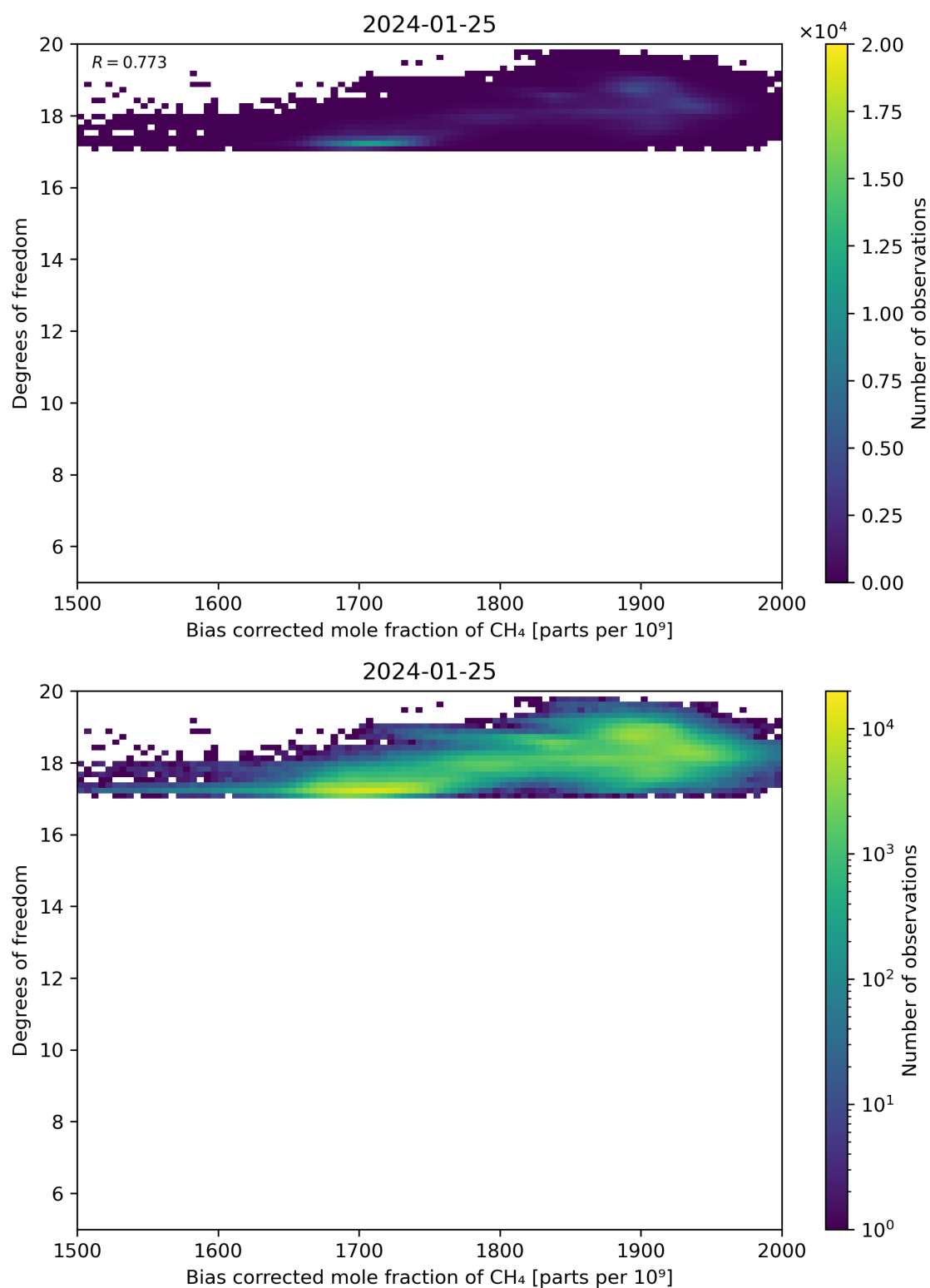
Figure 65: Scatter density plot of “Bias corrected mole fraction of CH 4 ” against “Degrees of freedom” for 2024-01-24 to 2024-01-26.
