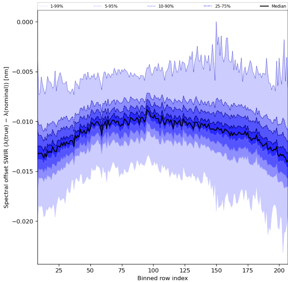
Figure 38: Along track statistics of “Spectral offset SWIR ( \lambda(\text{true}) - \lambda(\text{nominal}) )” for 2024-01-24 to 2024-01-26
