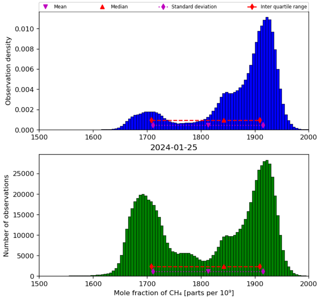
Figure 23: Histogram of “Mole fraction of CH 4 ” for 2024-01-24 to 2024-01-26
