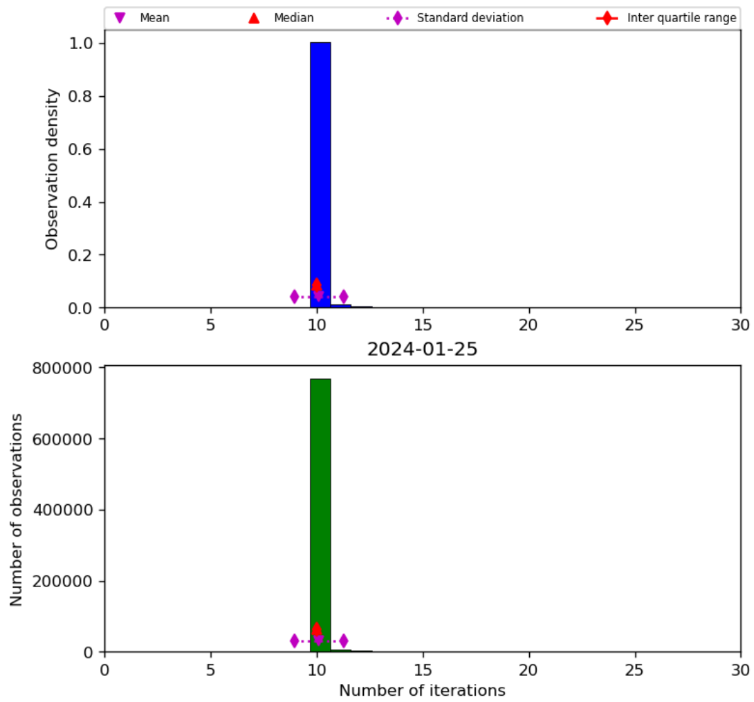
Figure 31: Histogram of “Number of iterations” for 2024-01-24 to 2024-01-26
