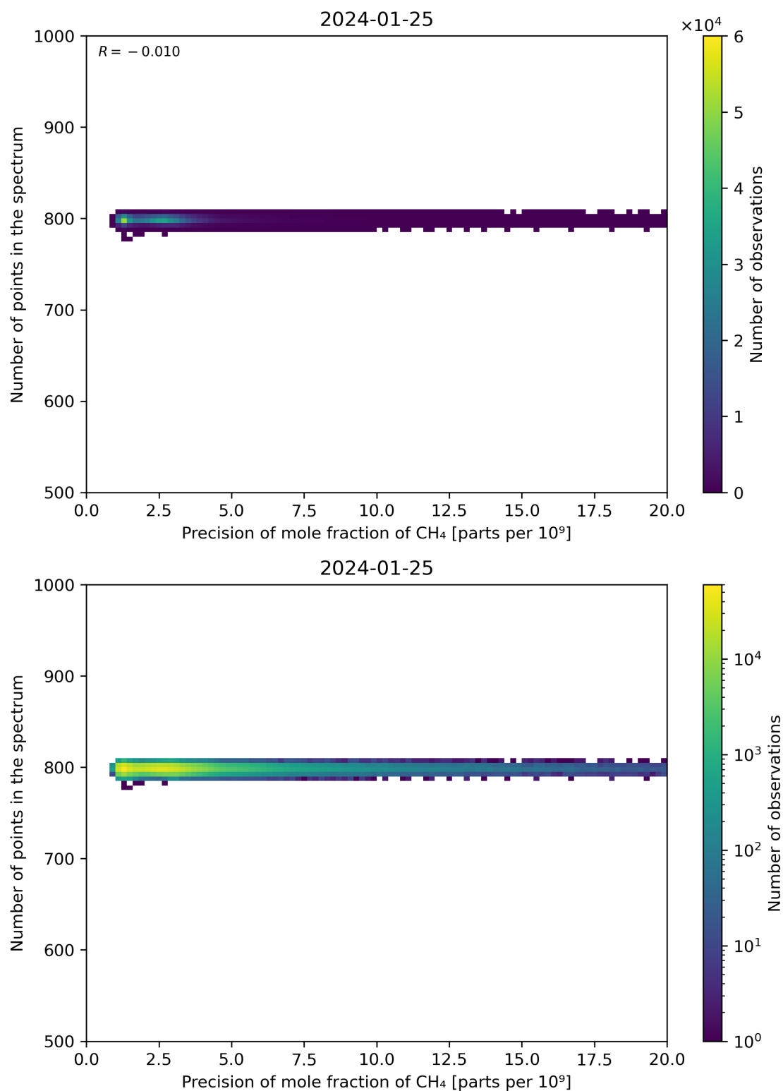
Figure 84: Scatter density plot of “Precision of mole fraction of CH 4 ” against “Number of points in the spectrum” for 2024-01-24 to 2024-01-26.
