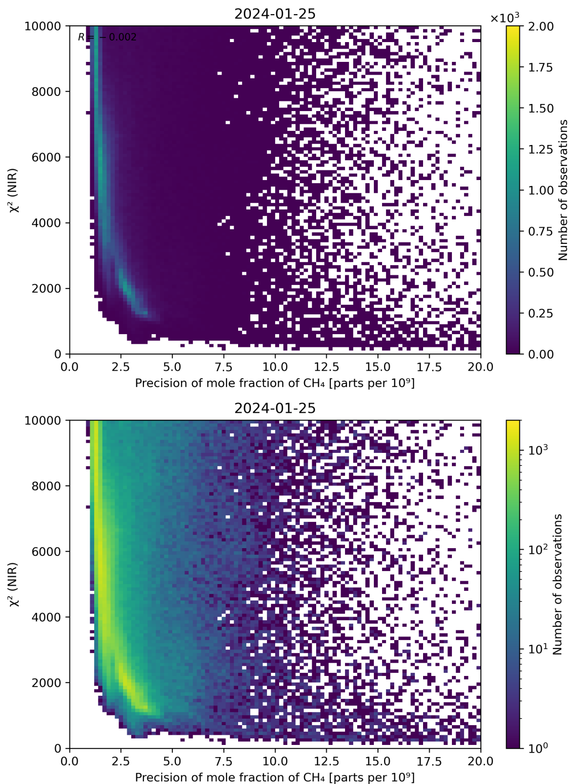
Figure 78: Scatter density plot of “Precision of mole fraction of CH 4 ” against “ \chi^2 (NIR)” for 2024-01-24 to 2024-01-26.
