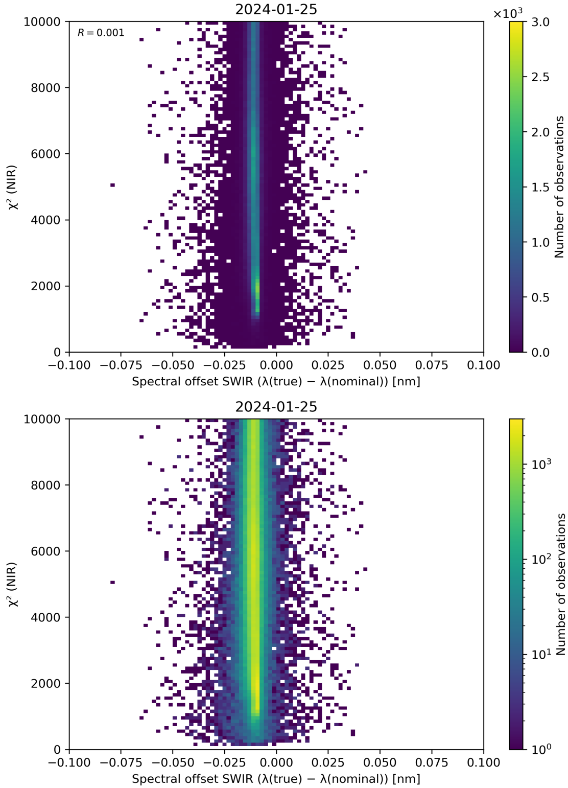
Figure 117: Scatter density plot of “Spectral offset SWIR ( \lambda(\text{true}) - \lambda(\text{nominal}) )” against “ \chi^2 (NIR)” for 2024-01-24 to 2024-01-26.
