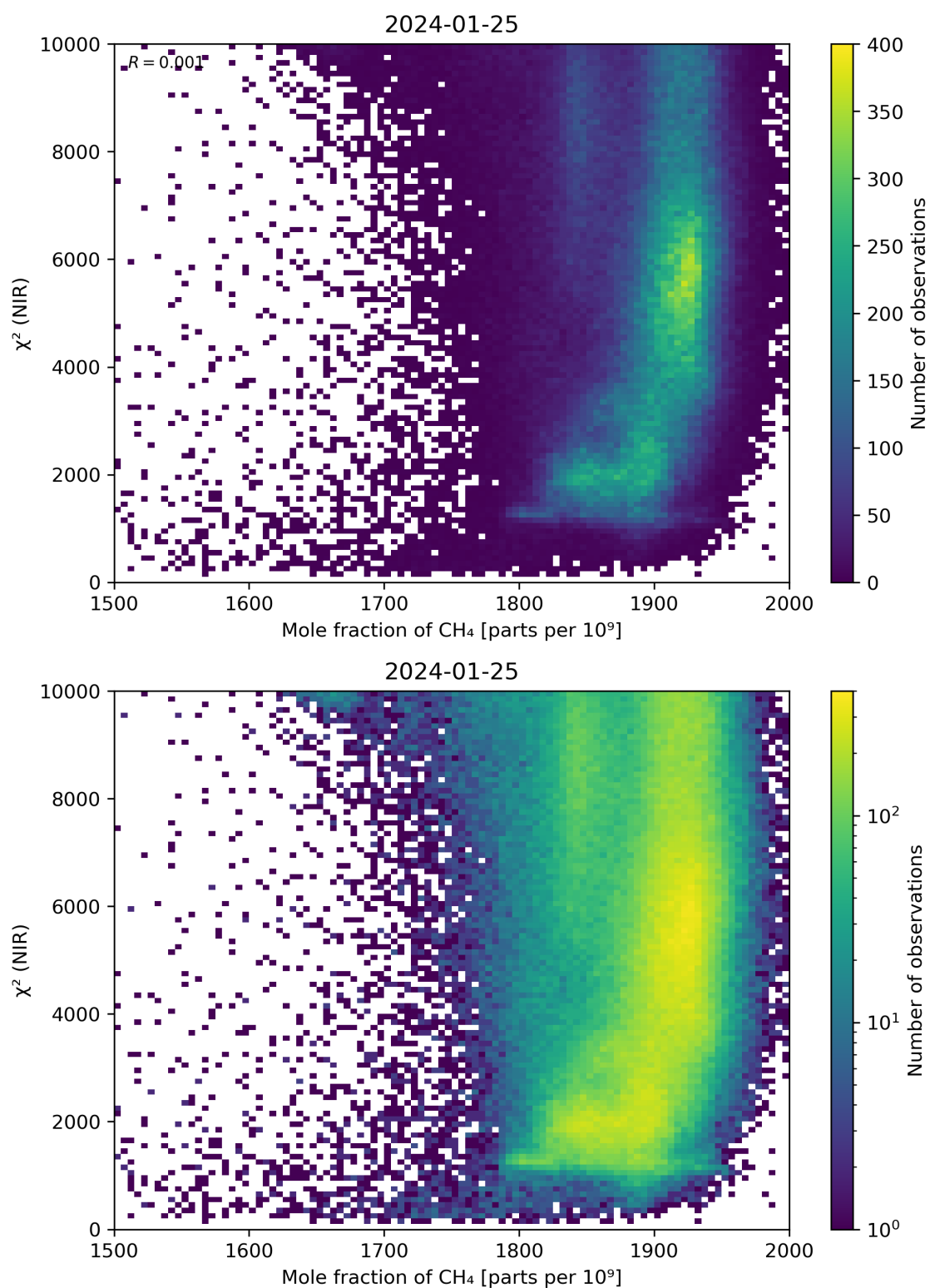
Figure 70: Scatter density plot of “Mole fraction of \text{CH}_4 ” against “ \chi^2 (NIR)” for 2024-01-24 to 2024-01-26.
