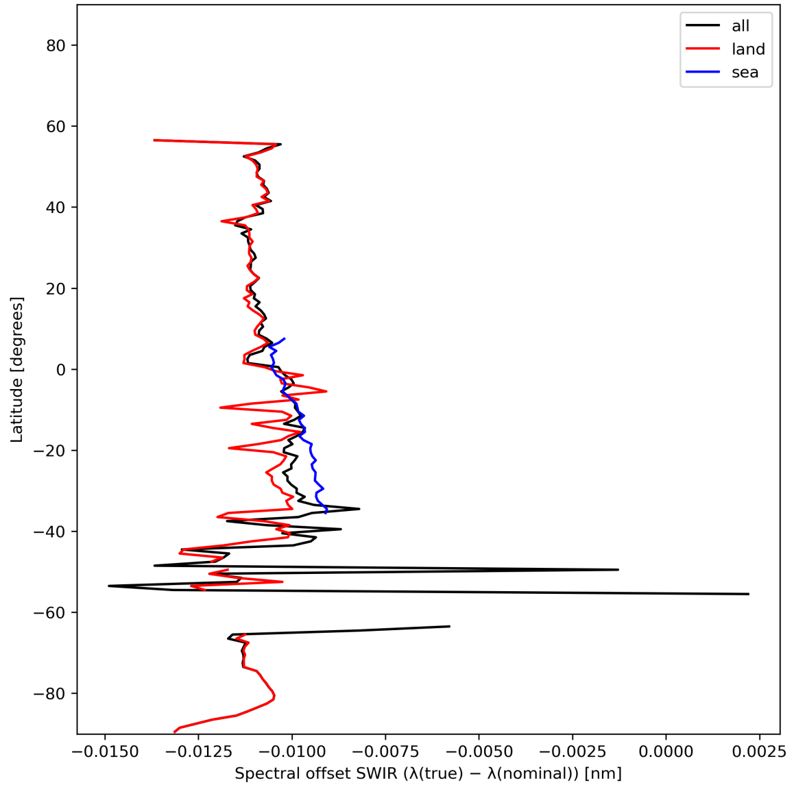
Figure 16: Zonal average of “Spectral offset SWIR ( \lambda(\text{true}) - \lambda(\text{nominal}) )” for 2024-01-24 to 2024-01-26.
