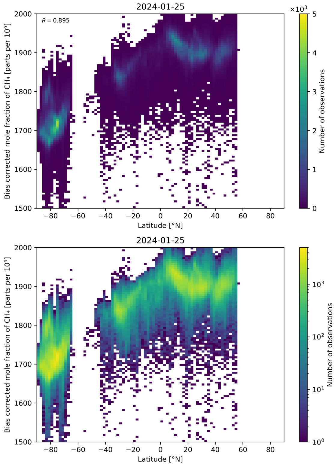
Figure 58: Scatter density plot of “Latitude” against “Bias corrected mole fraction of \text{CH}_4 ” for 2024-01-24 to 2024-01-26.
