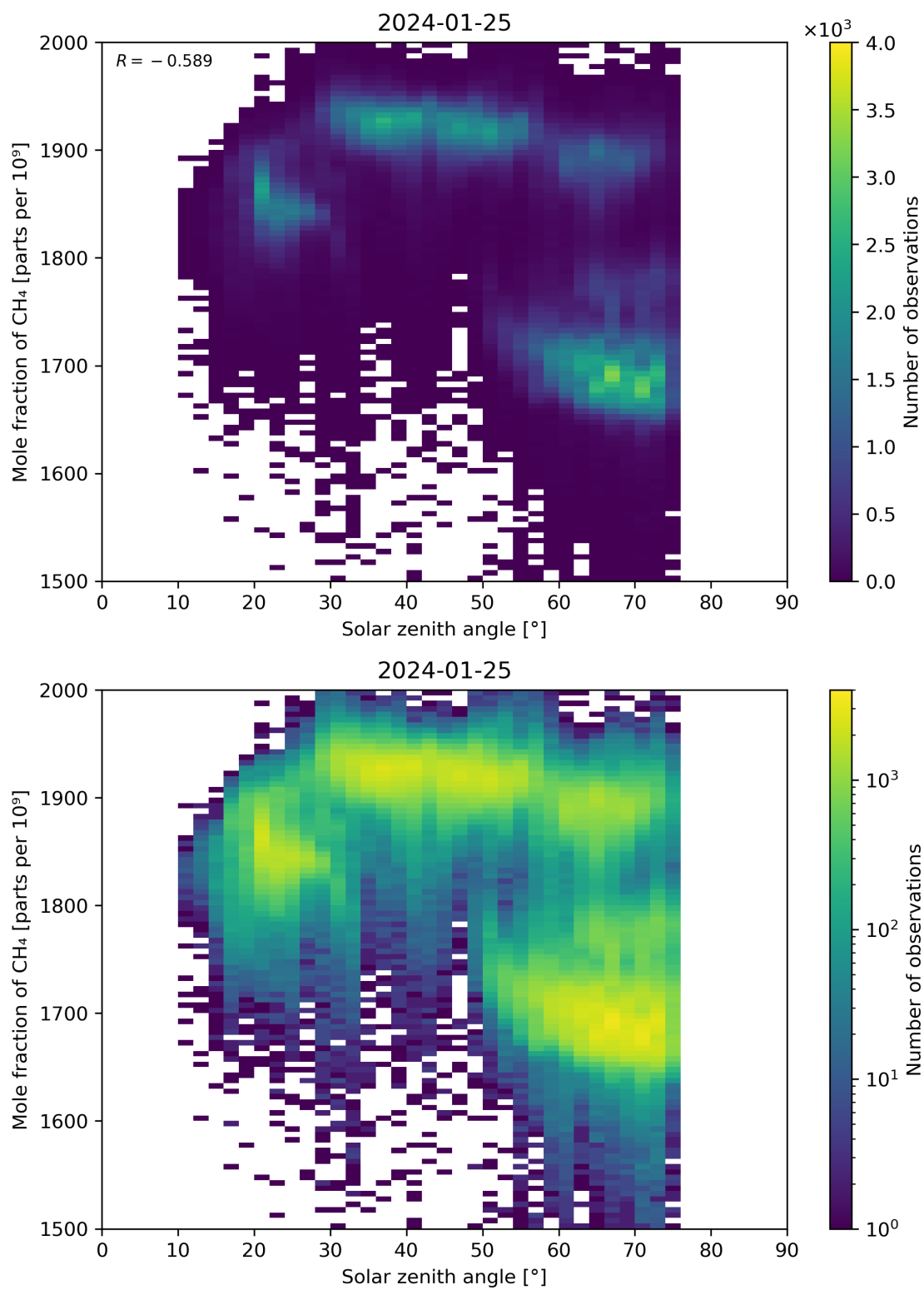
Figure 99: Scatter density plot of “Solar zenith angle” against “Mole fraction of CH 4 ” for 2024-01-24 to 2024-01-26.
