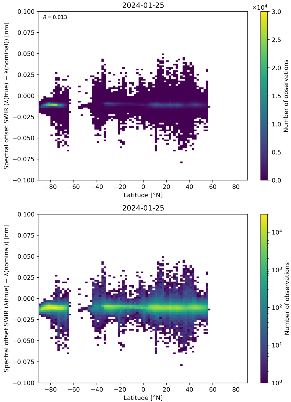
Figure 62: Scatter density plot of “Latitude” against “Spectral offset SWIR ( \lambda(\text{true}) - \lambda(\text{nominal}) )” for 2024-01-24 to 2024-01-26.
