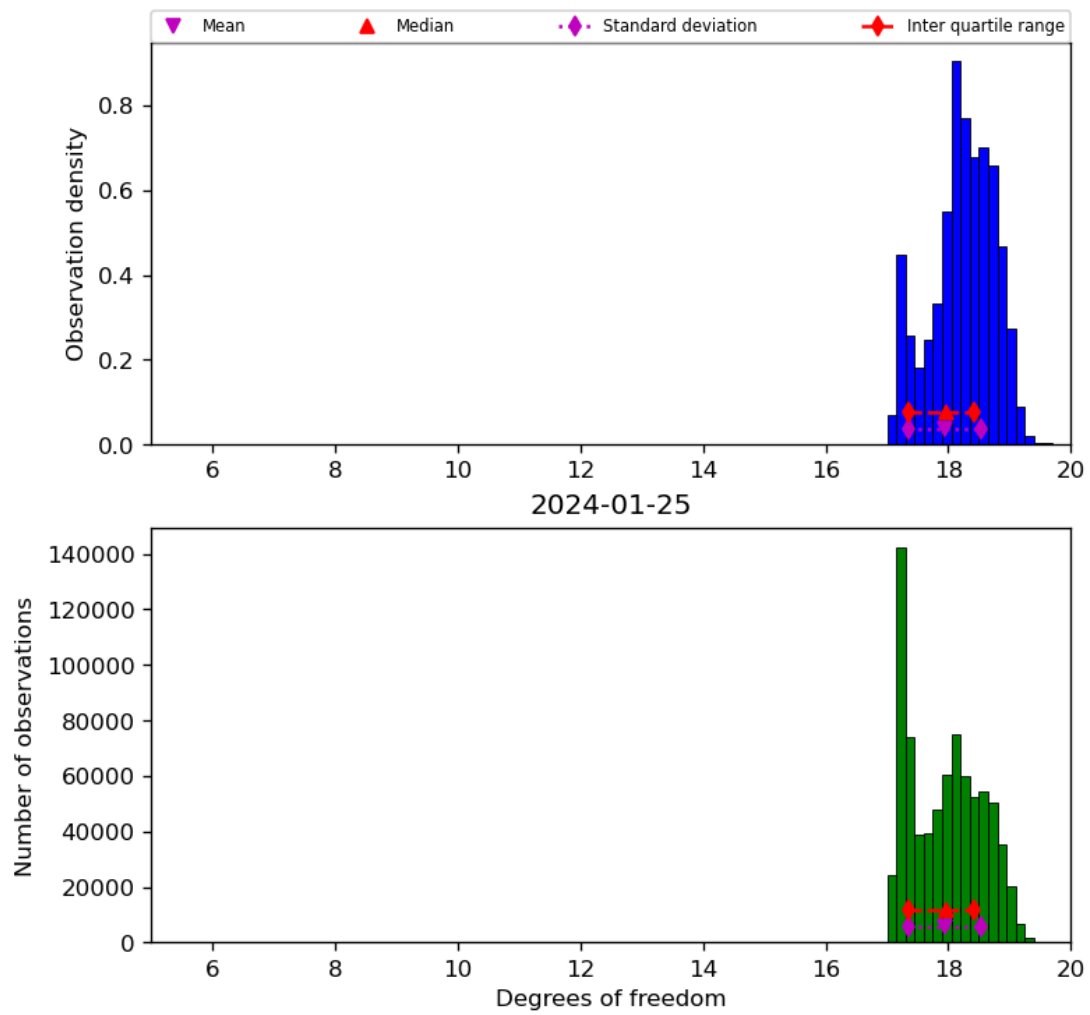
Figure 30: Histogram of “Degrees of freedom” for 2024-01-24 to 2024-01-26
