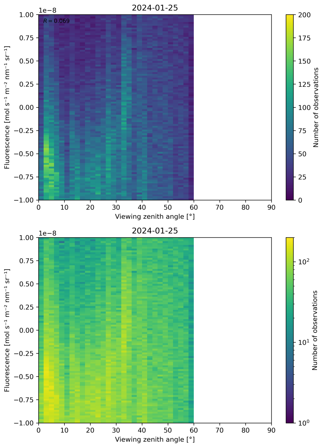
Figure 108: Scatter density plot of “Viewing zenith angle” against “Fluorescence” for 2024-01-24 to 2024-01-26.
