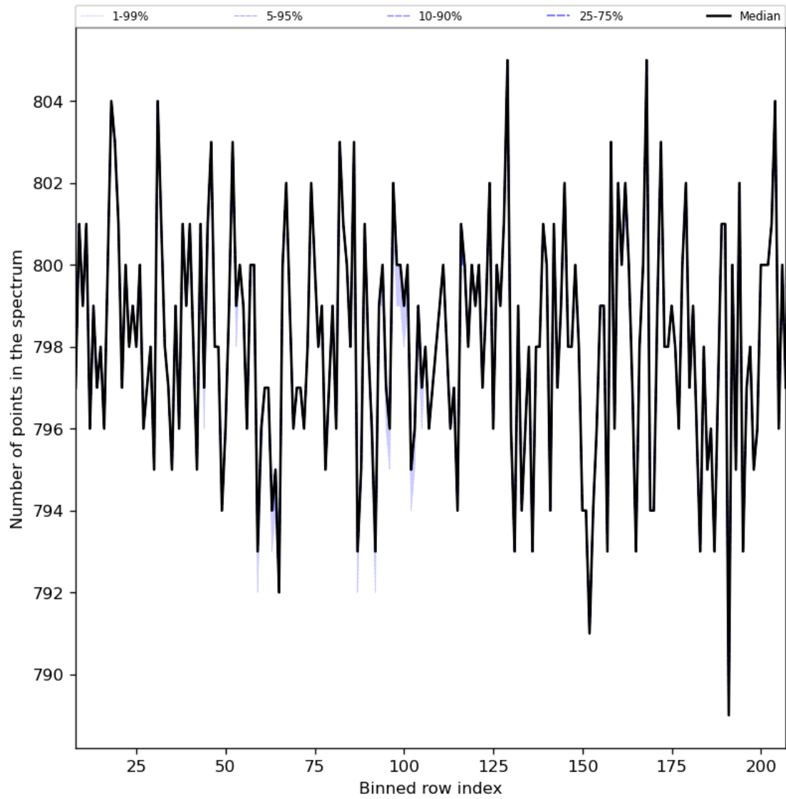
Figure 37: Along track statistics of “Number of points in the spectrum” for 2024-01-24 to 2024-01-26
