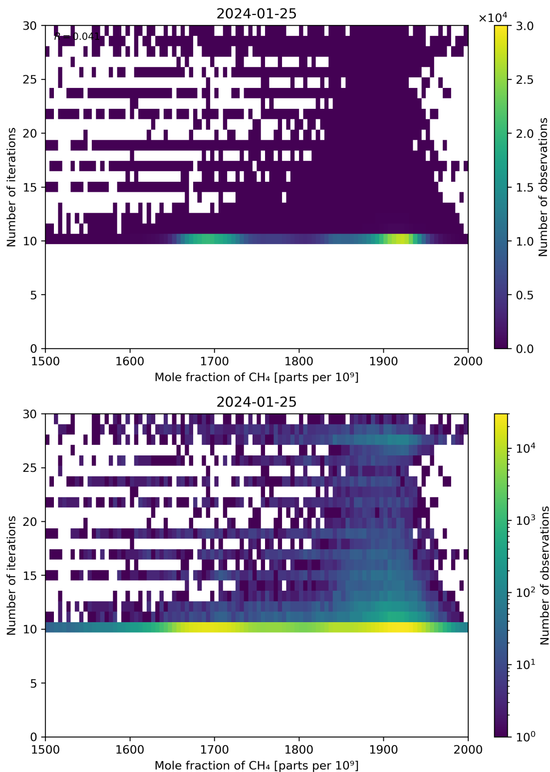
Figure 76: Scatter density plot of “Mole fraction of CH 4 ” against “Number of iterations” for 2024-01-24 to 2024-01-26.
