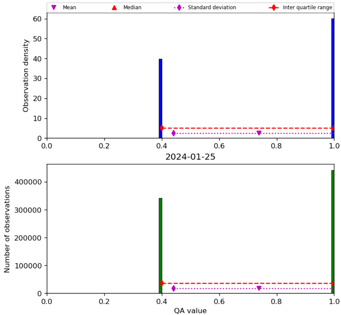
Figure 22: Histogram of “QA value” for 2024-01-24 to 2024-01-26
