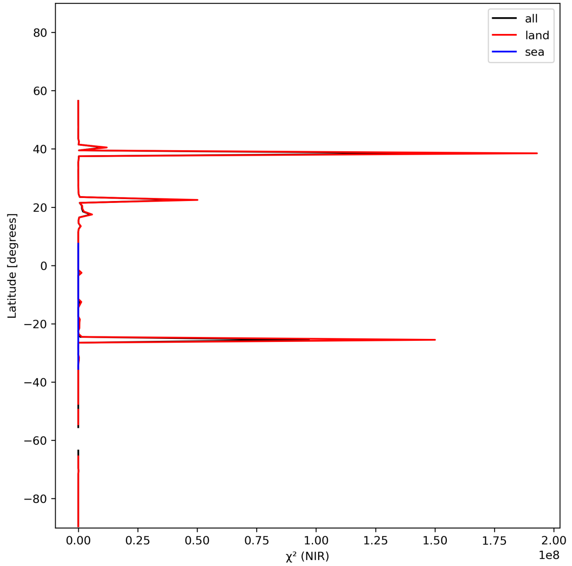
Figure 18: Zonal average of “ \chi^2 (NIR)” for 2024-01-24 to 2024-01-26.
