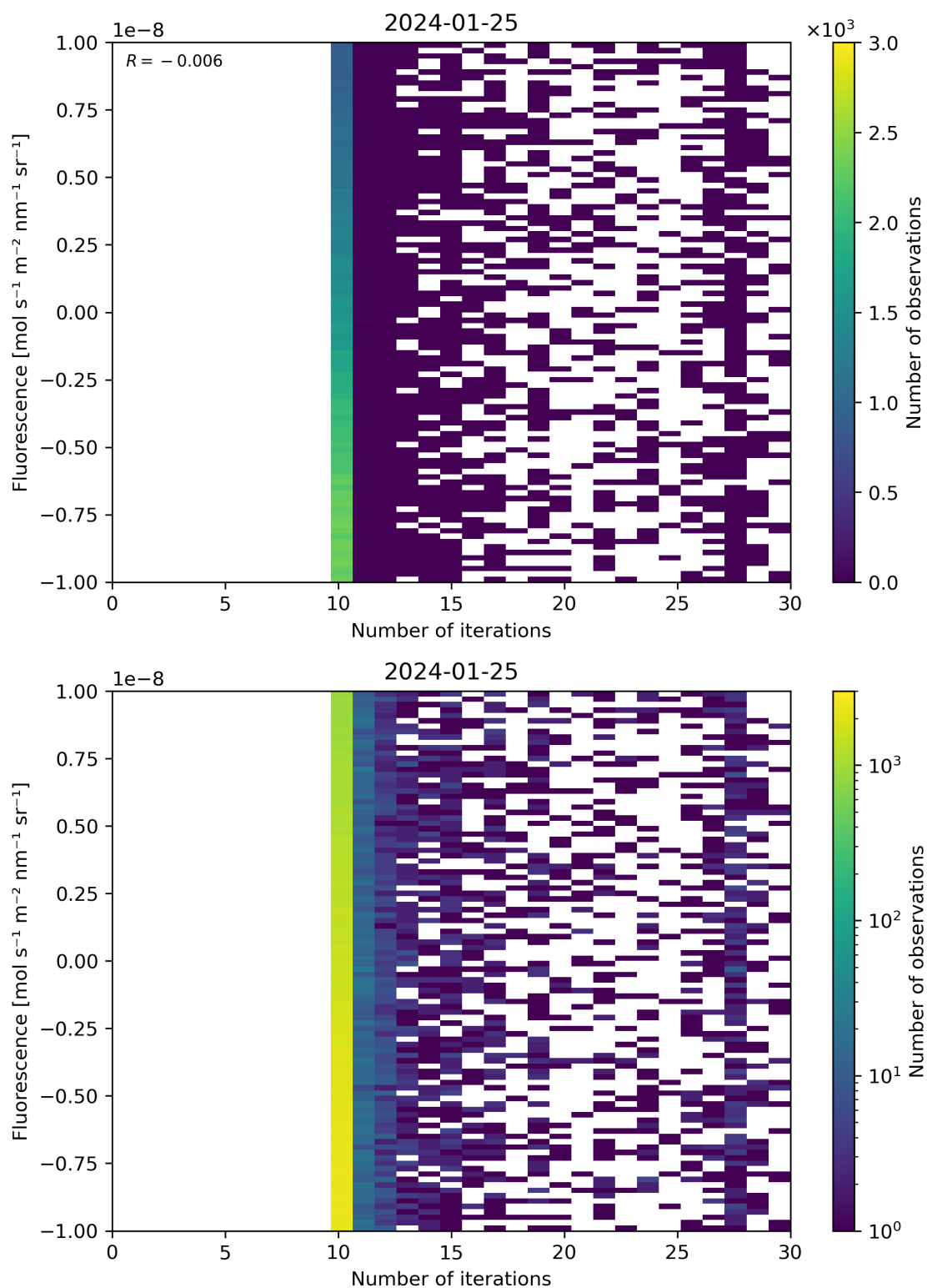
Figure 87: Scatter density plot of “Number of iterations” against “Fluorescence” for 2024-01-24 to 2024-01-26.
