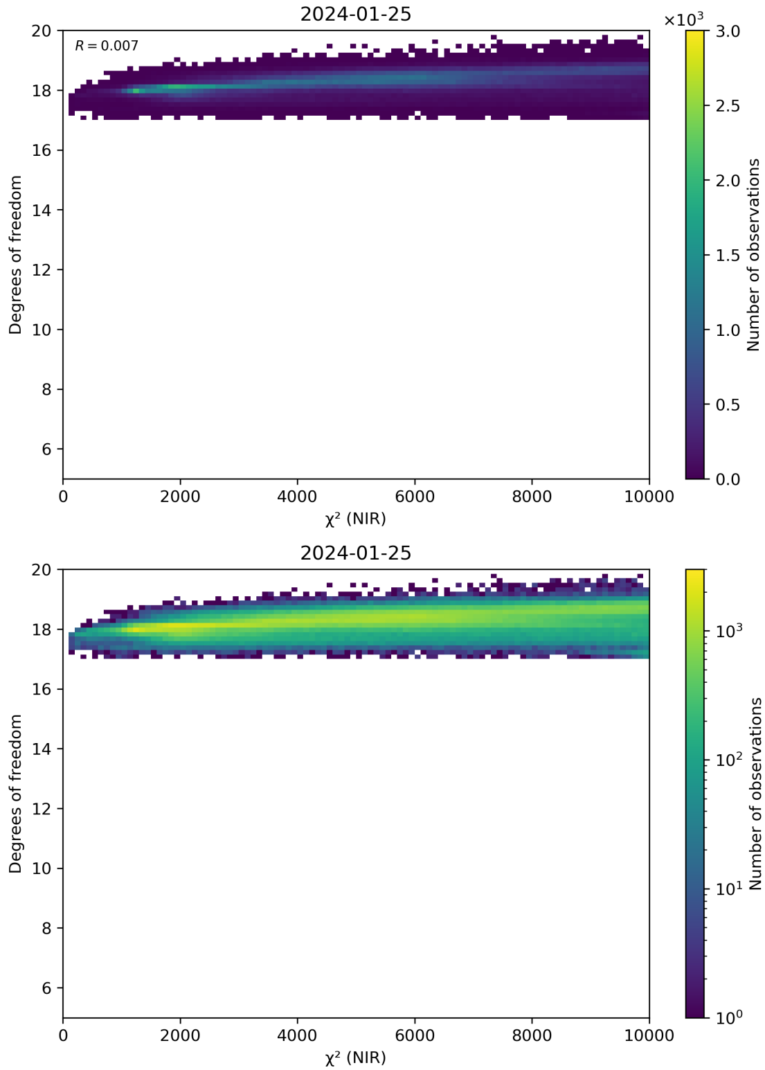
Figure 44: Scatter density plot of “ \chi^2 (NIR)” against “Degrees of freedom” for 2024-01-24 to 2024-01-26.
