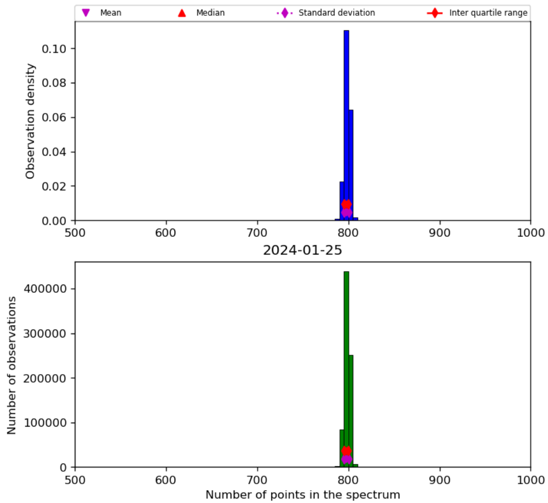
Figure 26: Histogram of “Number of points in the spectrum” for 2024-01-24 to 2024-01-26
