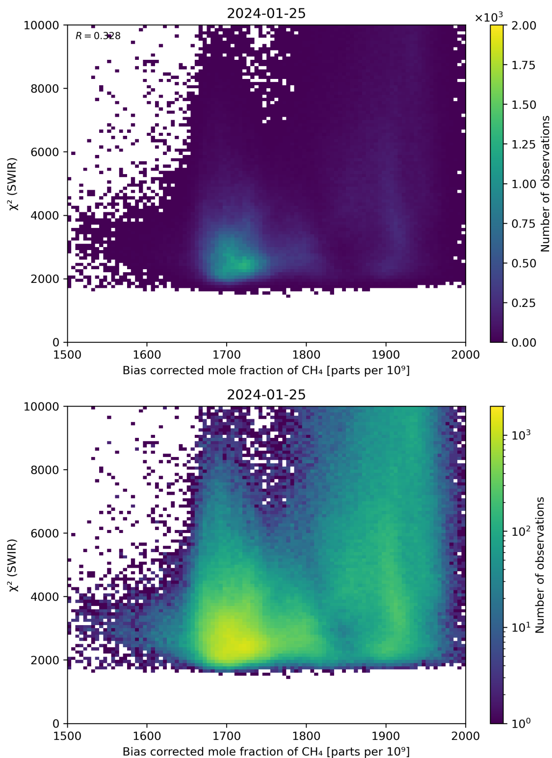
Figure 64: Scatter density plot of “Bias corrected mole fraction of \text{CH}_4 ” against “ \chi^2 (SWIR)” for 2024-01-24 to 2024-01-26.
