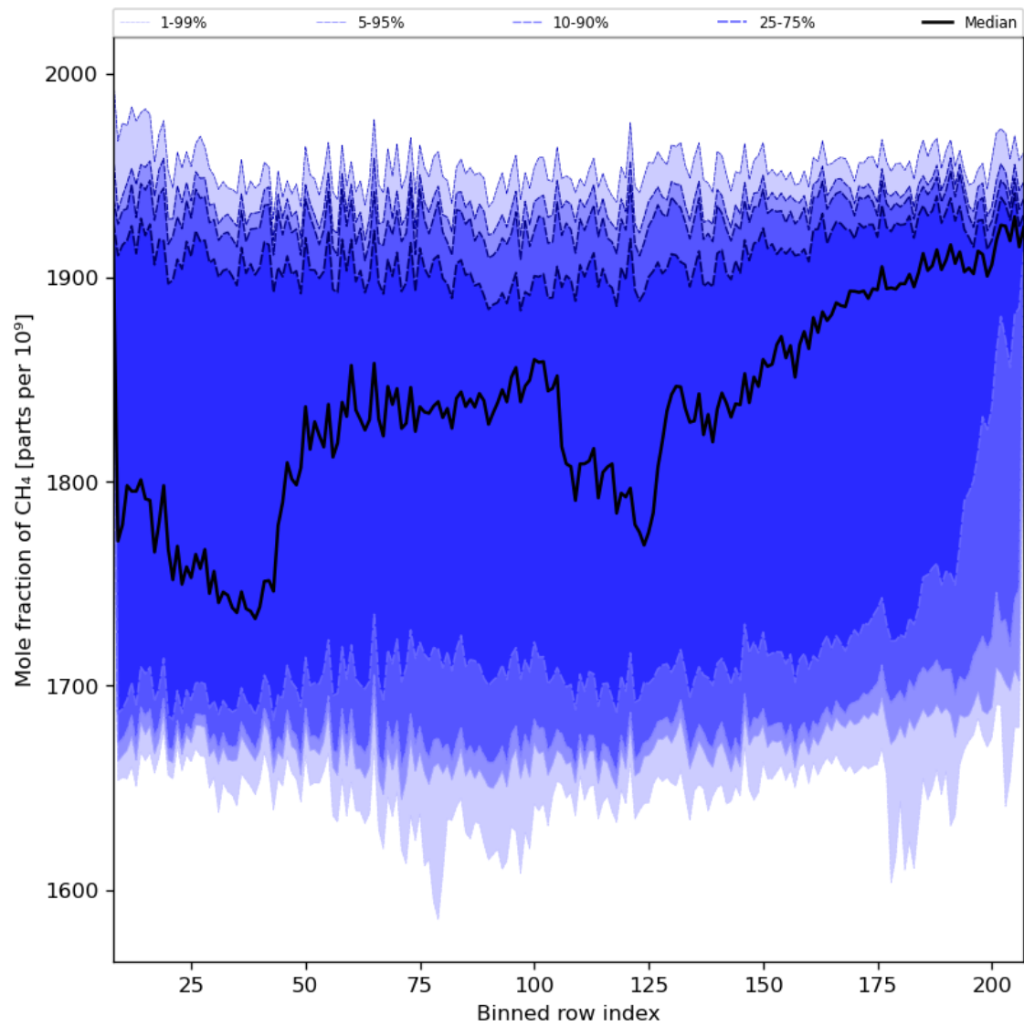
Figure 34: Along track statistics of “Mole fraction of CH 4 ” for 2024-01-24 to 2024-01-26
