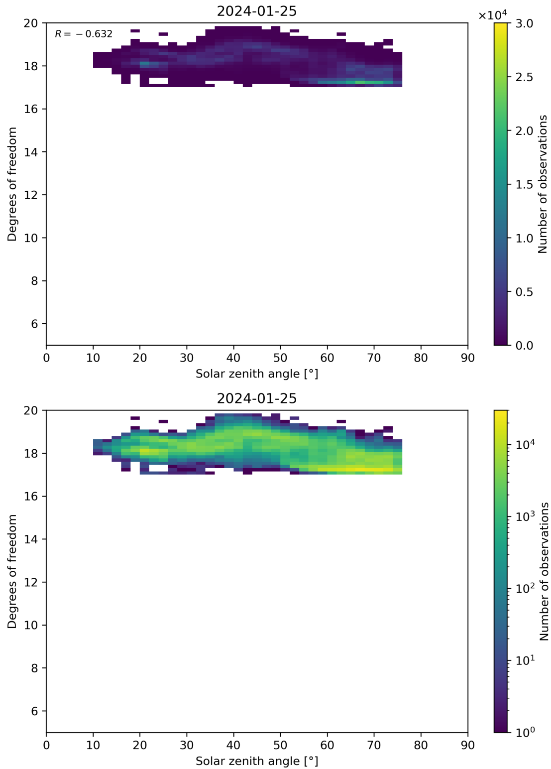
Figure 96: Scatter density plot of “Solar zenith angle” against “Degrees of freedom” for 2024-01-24 to 2024-01-26.
