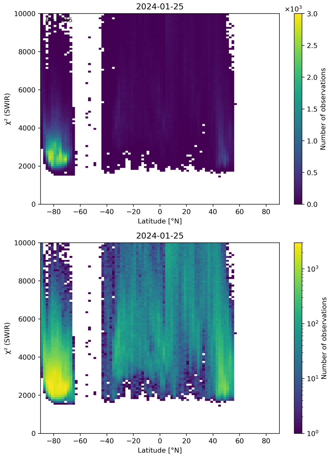
Figure 54: Scatter density plot of “Latitude” against “ \chi^2 (SWIR)” for 2024-01-24 to 2024-01-26.
