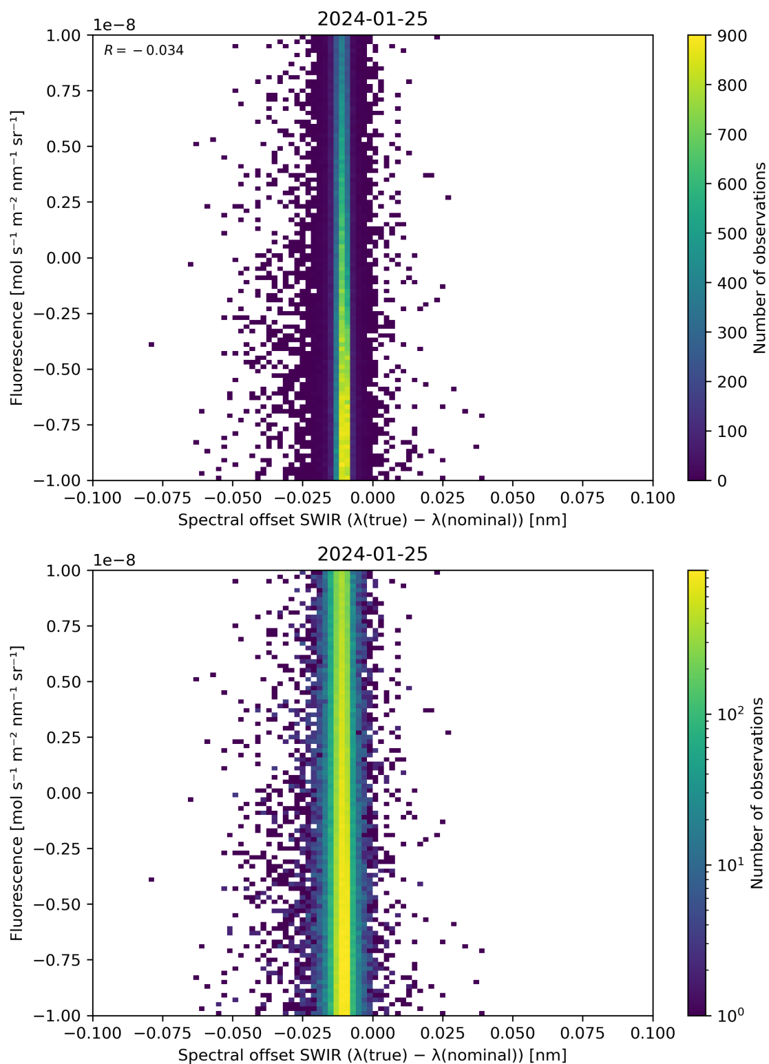
Figure 120: Scatter density plot of “Spectral offset SWIR ( \lambda(\text{true}) - \lambda(\text{nominal}) )” against “Fluorescence” for 2024-01-24 to 2024-01-26.
