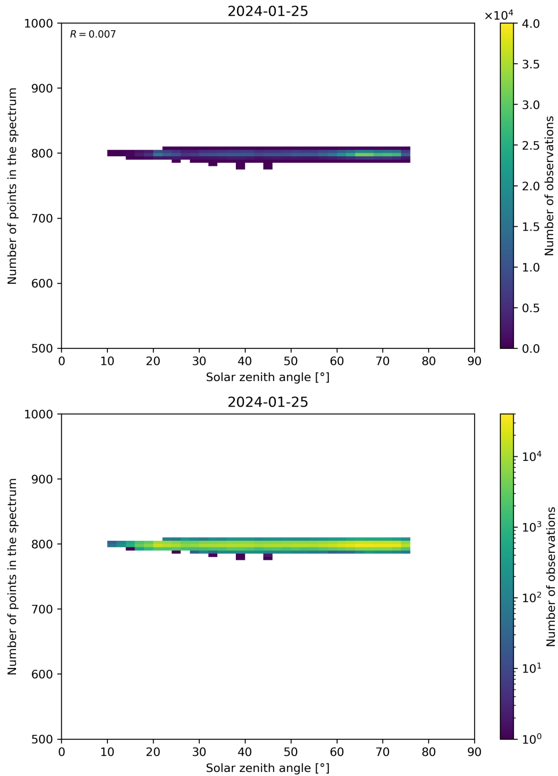
Figure 103: Scatter density plot of “Solar zenith angle” against “Number of points in the spectrum” for 2024-01-24 to 2024-01-26.
