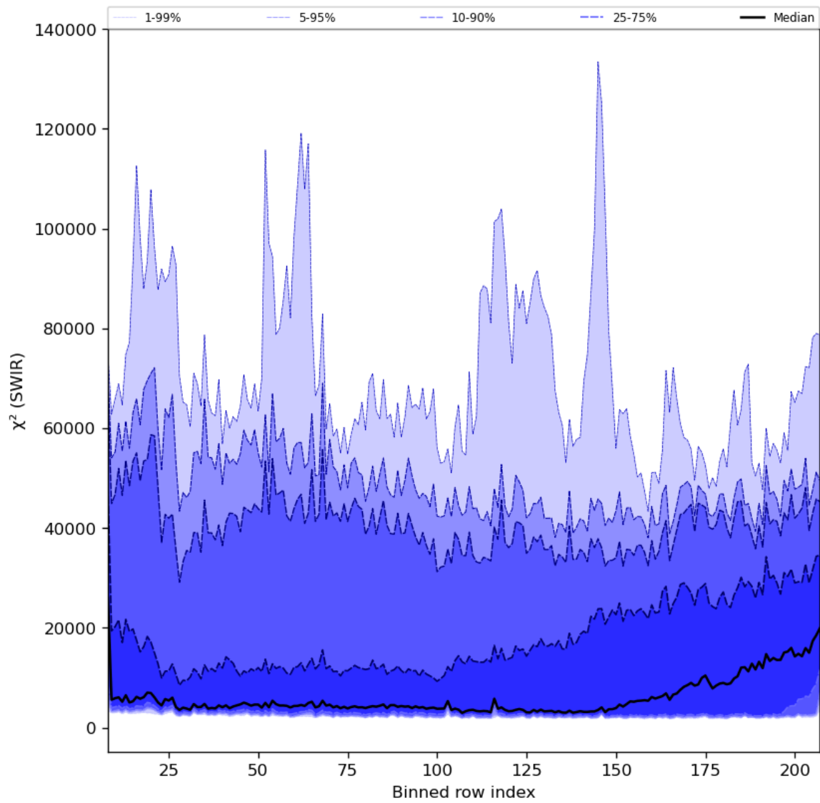
Figure 39: Along track statistics of " \chi^2 (SWIR)" for 2024-01-24 to 2024-01-26
