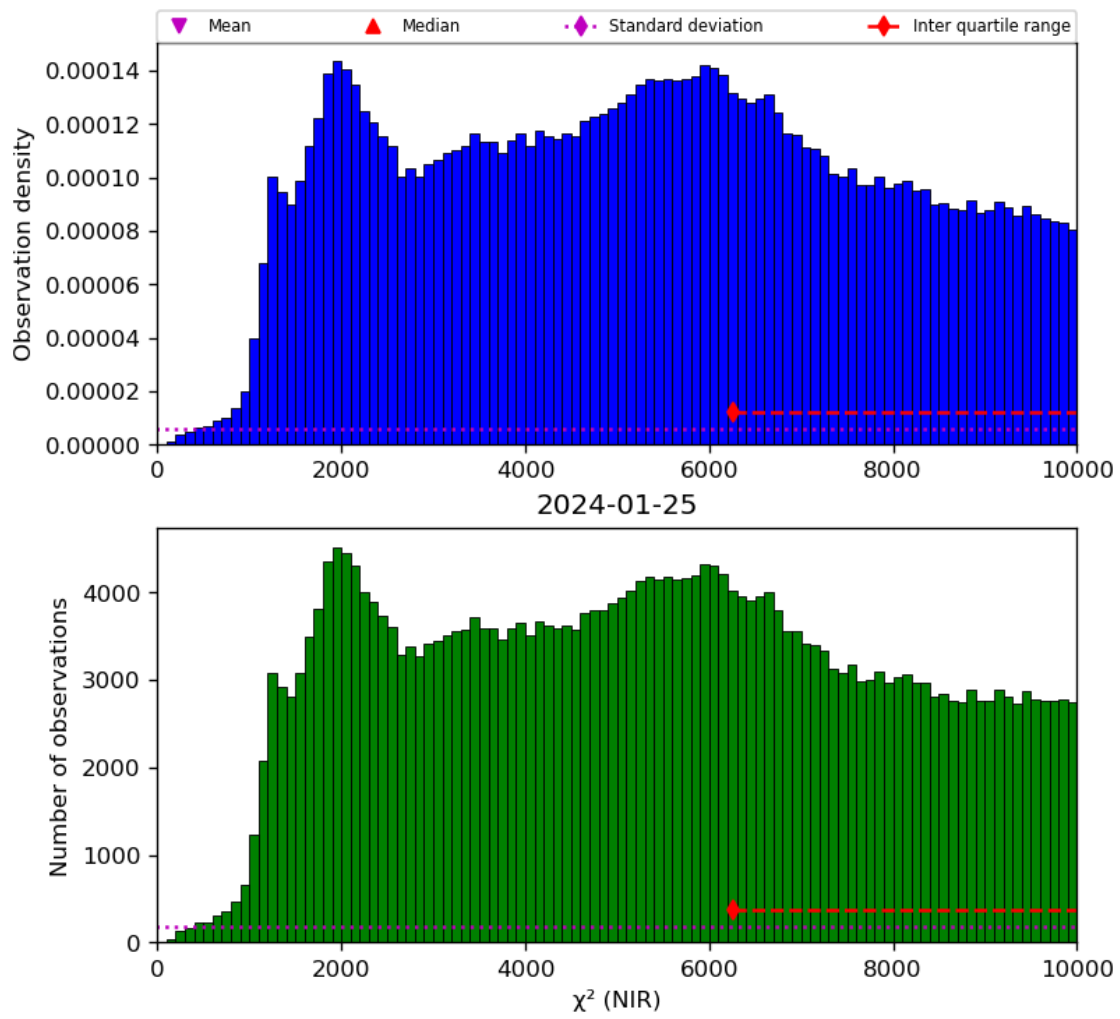
Figure 29: Histogram of “ \chi^2 (NIR)” for 2024-01-24 to 2024-01-26
