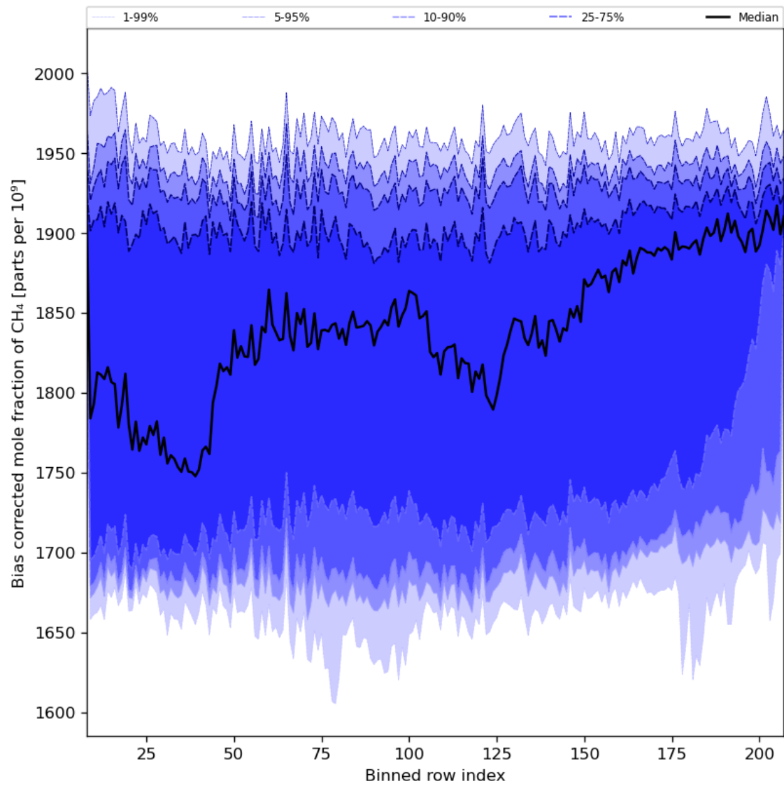
Figure 36: Along track statistics of “Bias corrected mole fraction of CH 4 ” for 2024-01-24 to 2024-01-26
