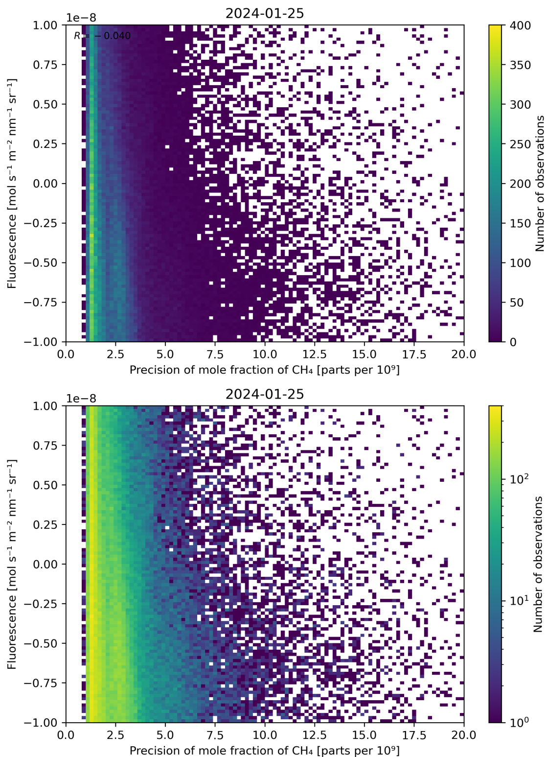
Figure 81: Scatter density plot of “Precision of mole fraction of \text{CH}_4 ” against “Fluorescence” for 2024-01-24 to 2024-01-26.
