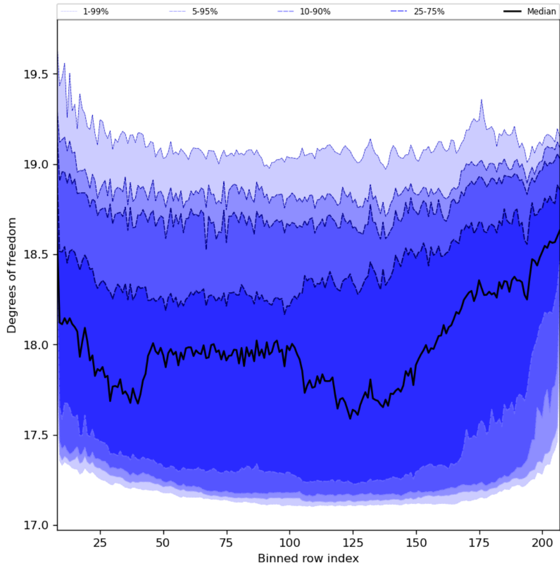
Figure 41: Along track statistics of “Degrees of freedom” for 2024-01-24 to 2024-01-26
