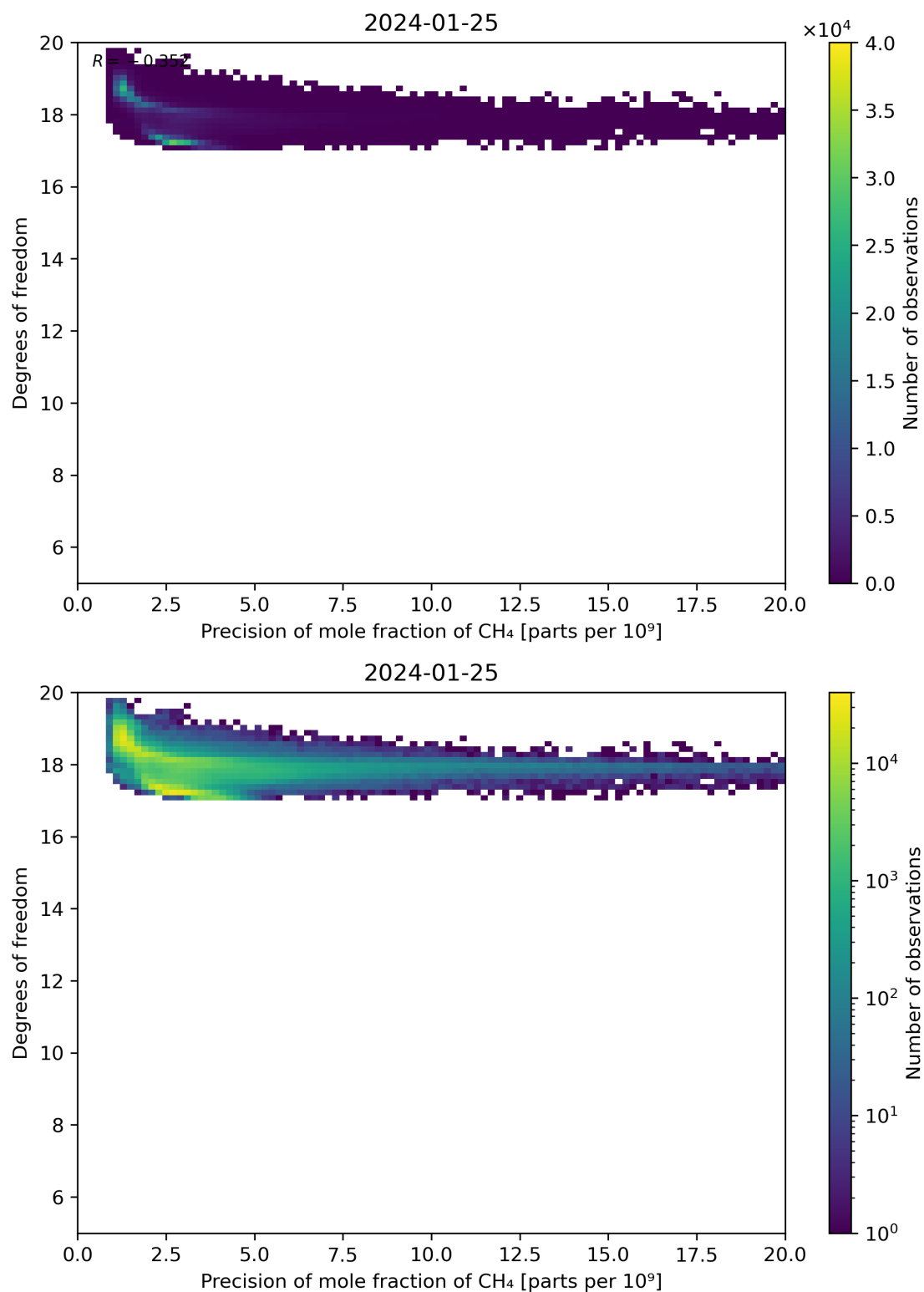
Figure 80: Scatter density plot of “Precision of mole fraction of CH 4 ” against “Degrees of freedom” for 2024-01-24 to 2024-01-26.
