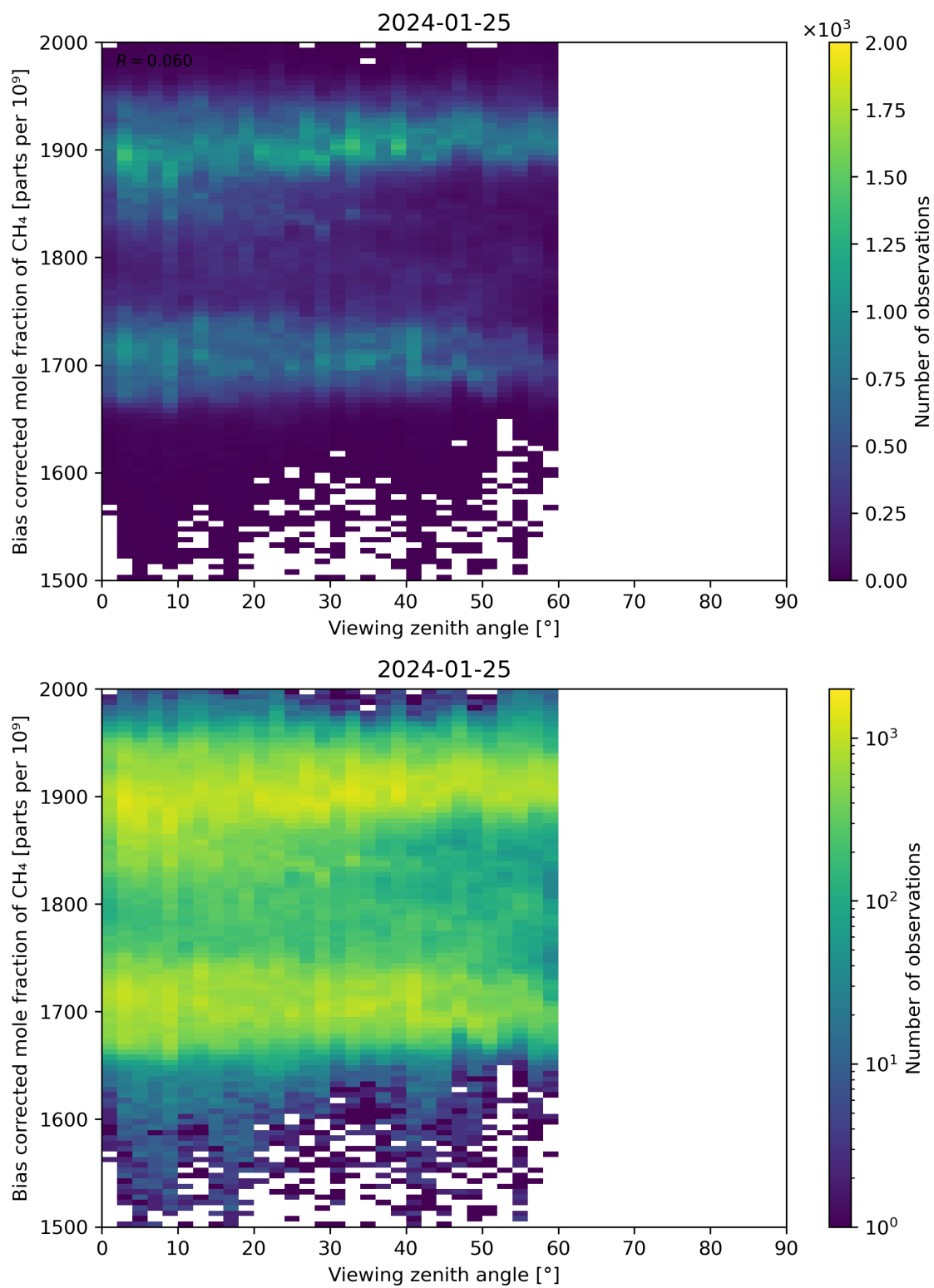
Figure 111: Scatter density plot of “Viewing zenith angle” against “Bias corrected mole fraction of CH 4 ” for 2024-01-24 to 2024-01-26.
