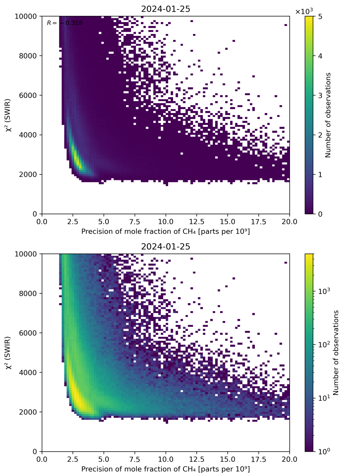
Figure 79: Scatter density plot of “Precision of mole fraction of \text{CH}_4 ” against “ \chi^2 (SWIR)” for 2024-01-24 to 2024-01-26.
