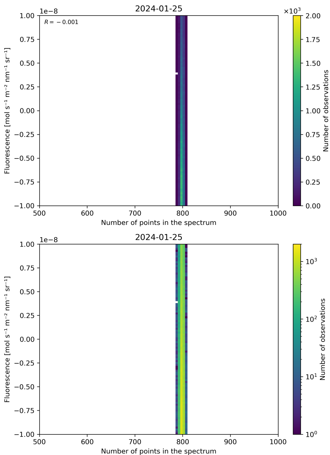
Figure 91: Scatter density plot of “Number of points in the spectrum” against “Fluorescence” for 2024-01-24 to 2024-01-26.
