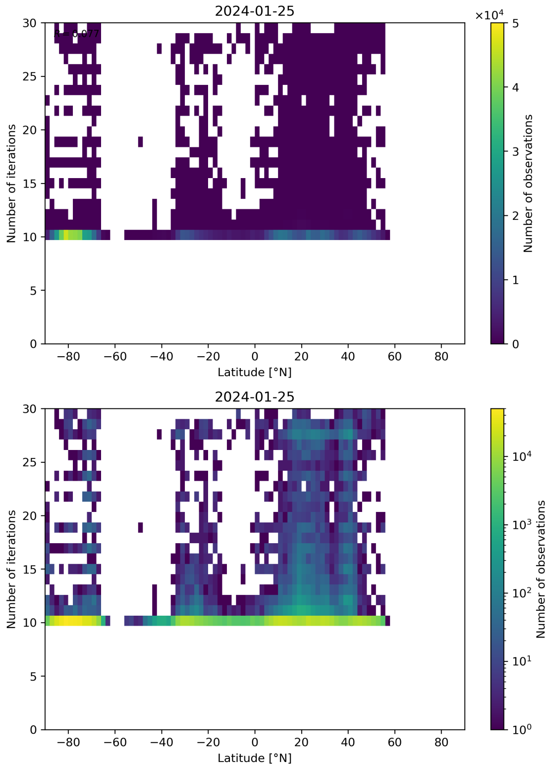
Figure 60: Scatter density plot of “Latitude” against “Number of iterations” for 2024-01-24 to 2024-01-26.
