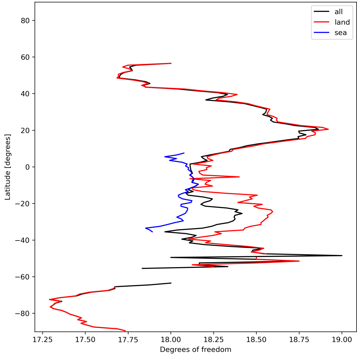
Figure 19: Zonal average of “Degrees of freedom” for 2024-01-24 to 2024-01-26.
