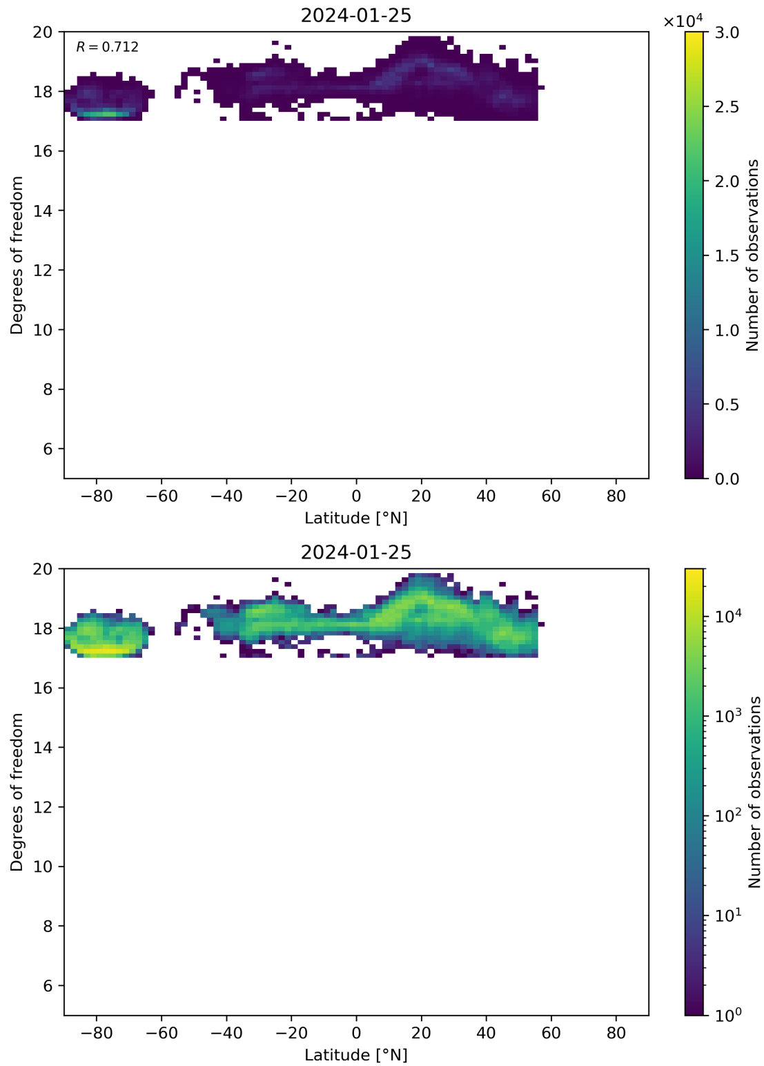
Figure 55: Scatter density plot of “Latitude” against “Degrees of freedom” for 2024-01-24 to 2024-01-26.
