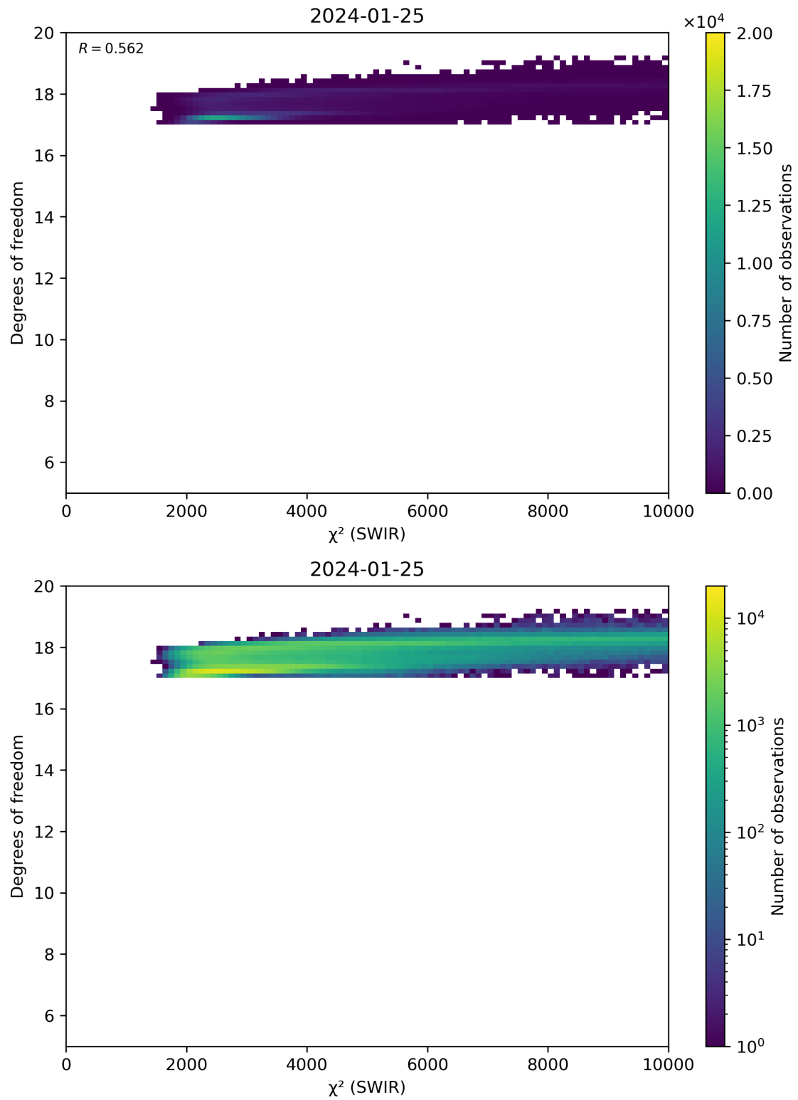
Figure 48: Scatter density plot of “ \chi^2 (SWIR)” against “Degrees of freedom” for 2024-01-24 to 2024-01-26.
