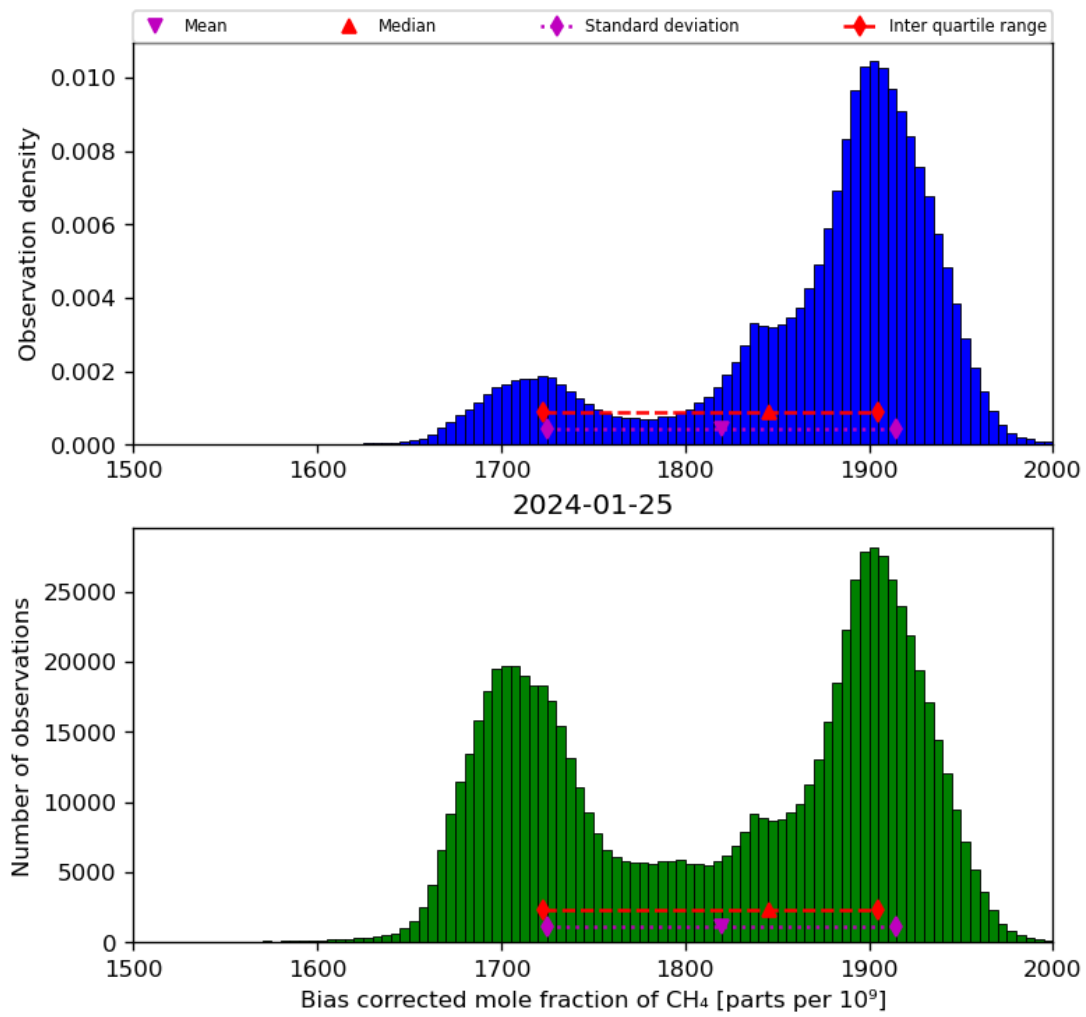
Figure 25: Histogram of “Bias corrected mole fraction of CH 4 ” for 2024-01-24 to 2024-01-26
