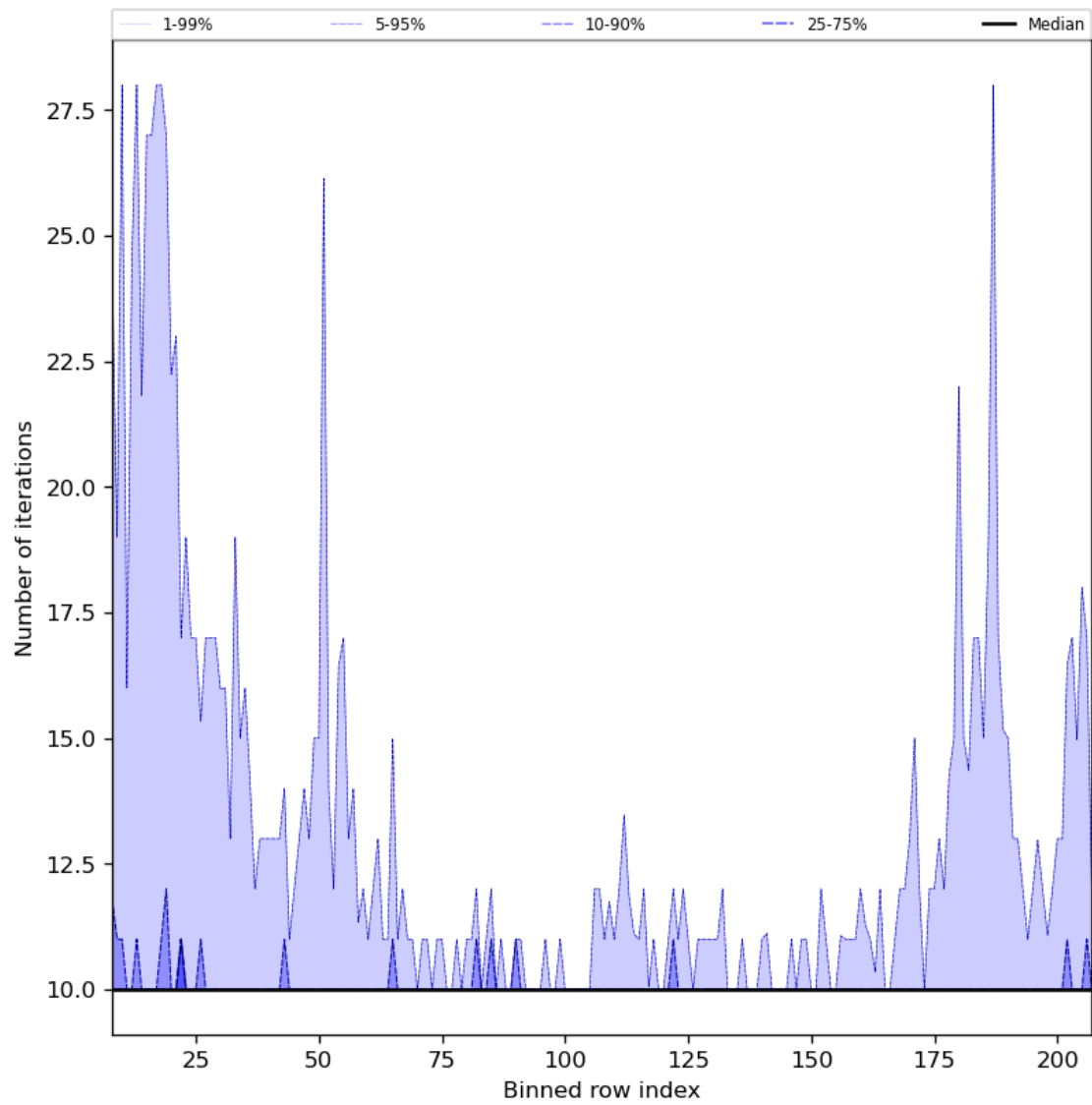
Figure 42: Along track statistics of “Number of iterations” for 2024-01-24 to 2024-01-26
