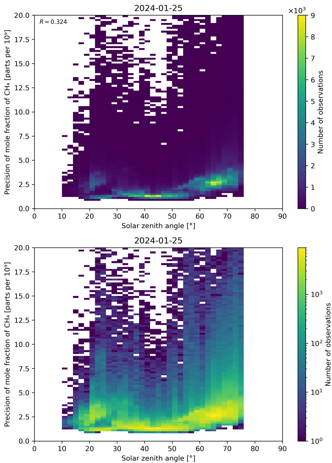
Figure 101: Scatter density plot of “Solar zenith angle” against “Precision of mole fraction of \text{CH}_4 ” for 2024-01-24 to 2024-01-26.
