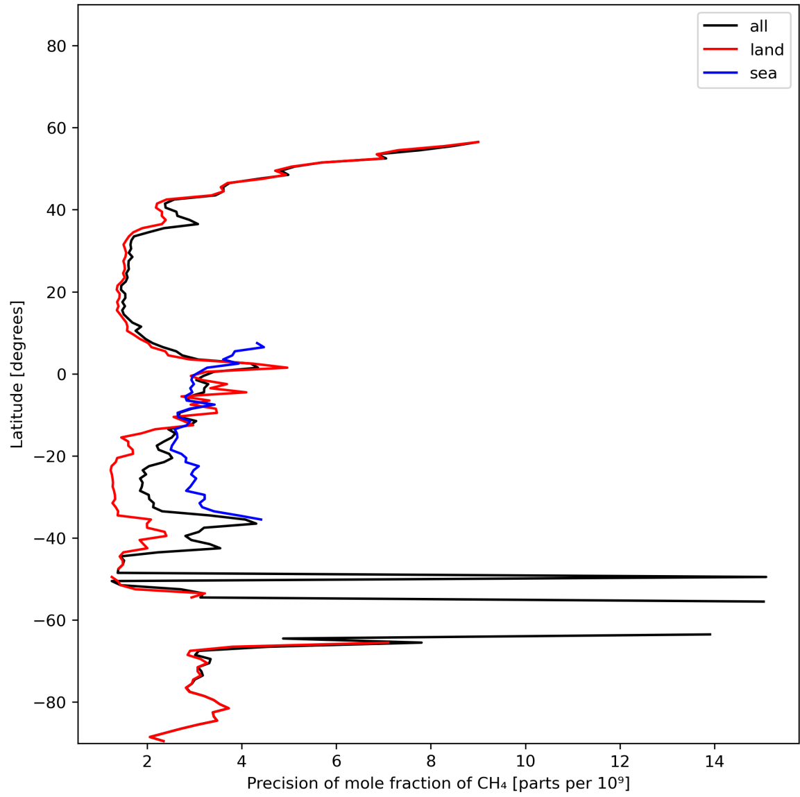
Figure 13: Zonal average of “Precision of mole fraction of CH 4 ” for 2024-01-24 to 2024-01-26.
