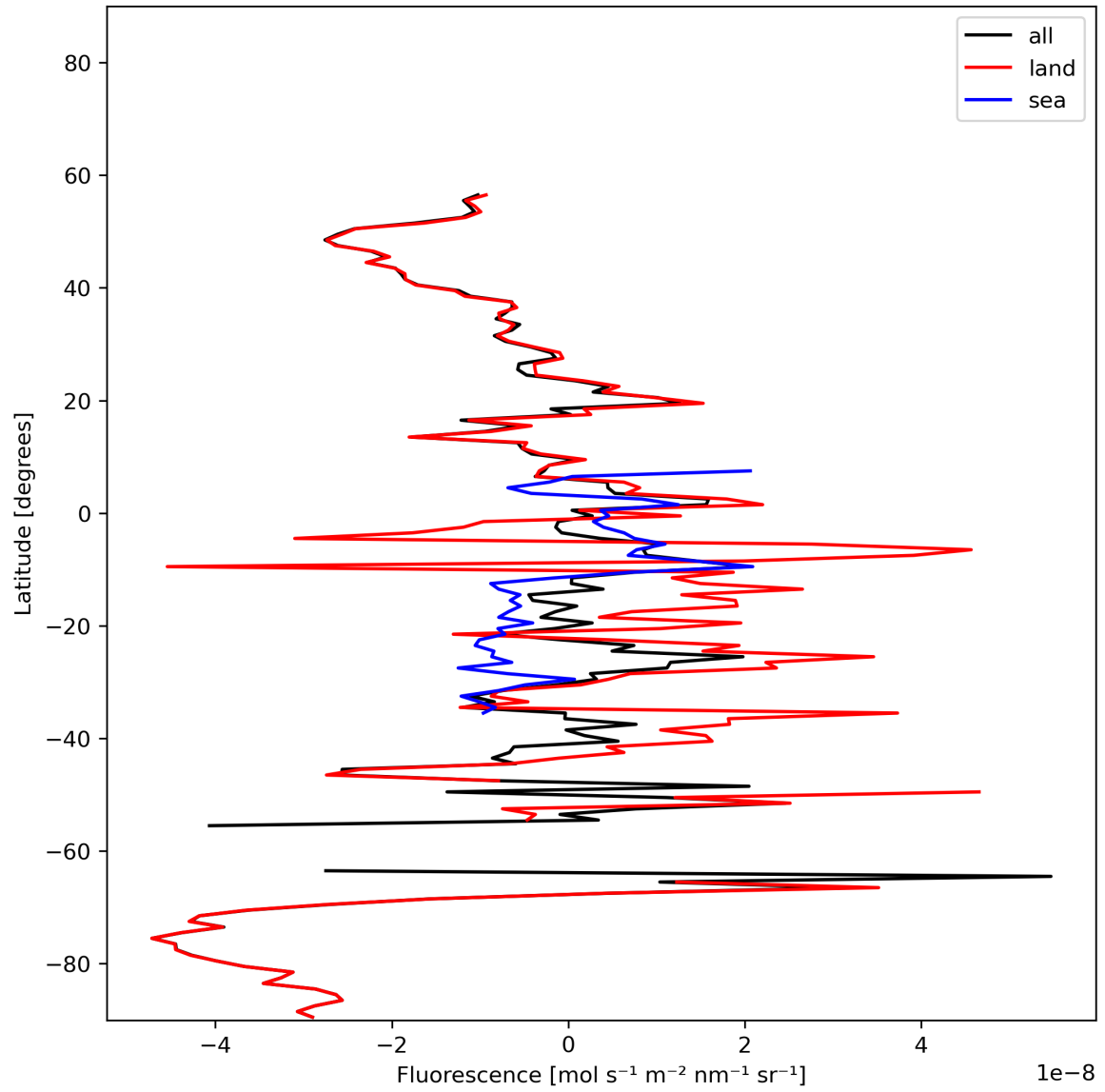
Figure 21: Zonal average of “Fluorescence” for 2024-01-24 to 2024-01-26.
