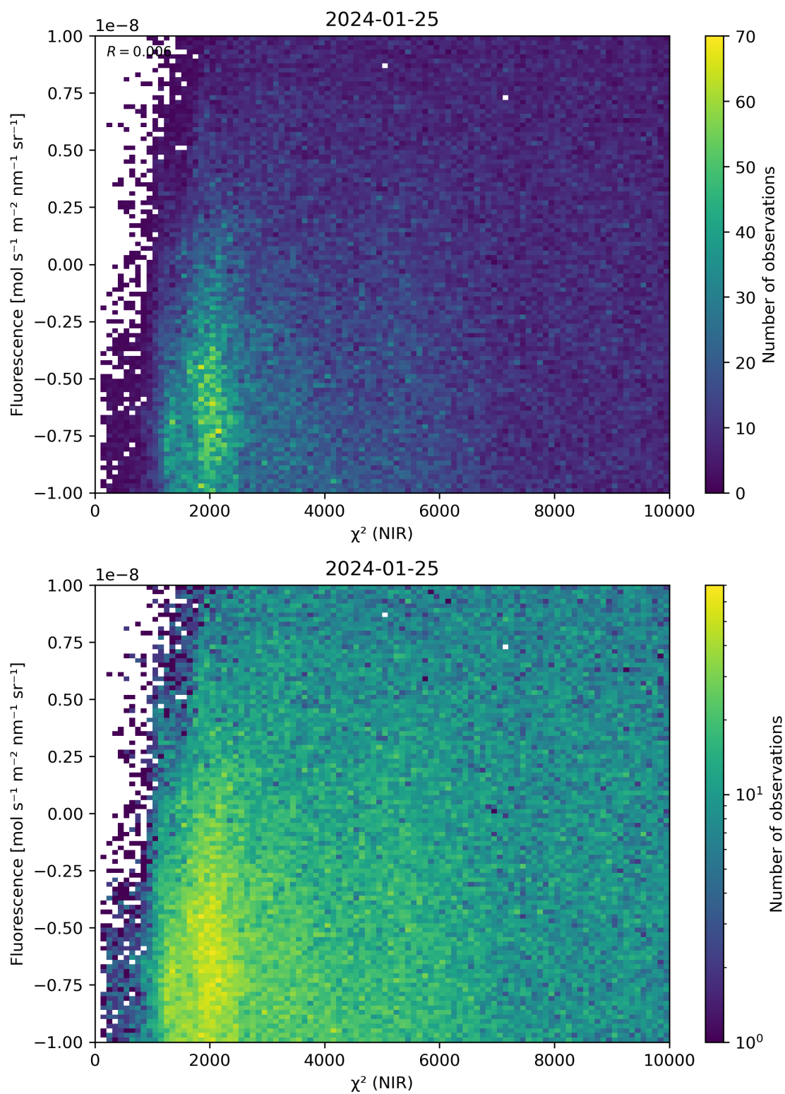
Figure 45: Scatter density plot of “ \chi^2 (NIR)” against “Fluorescence” for 2024-01-24 to 2024-01-26.
