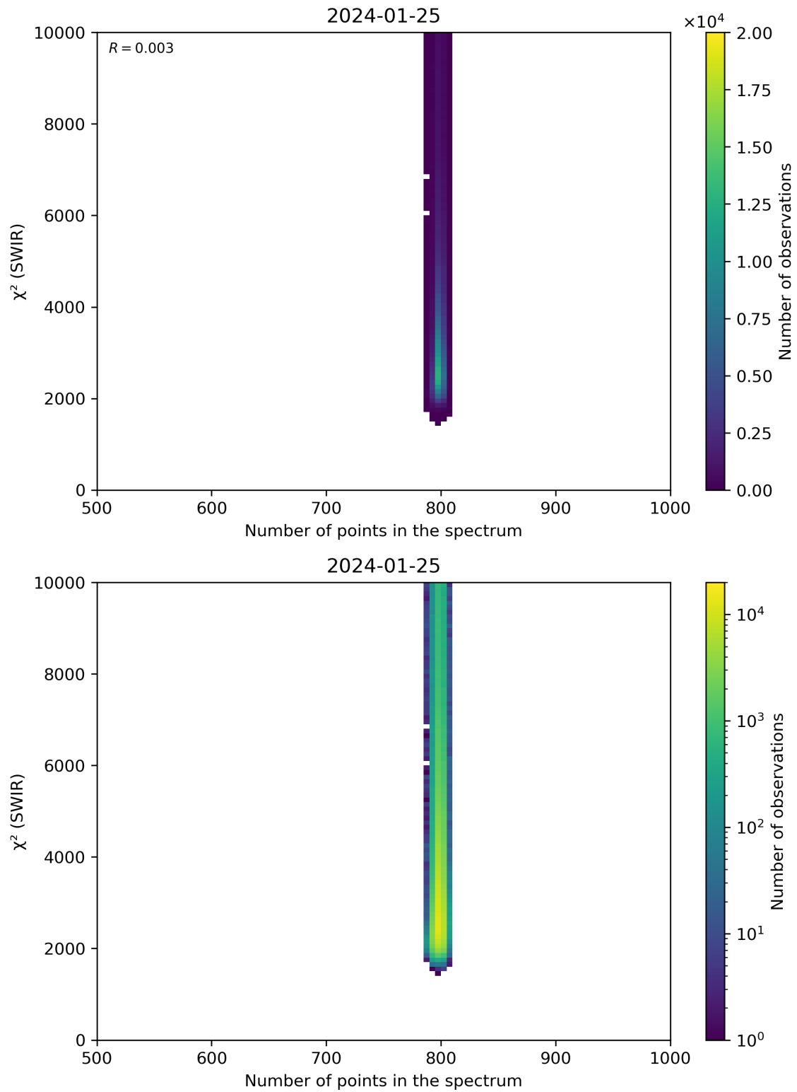
Figure 89: Scatter density plot of “Number of points in the spectrum” against “ \chi^2 (SWIR)” for 2024-01-24 to 2024-01-26.
