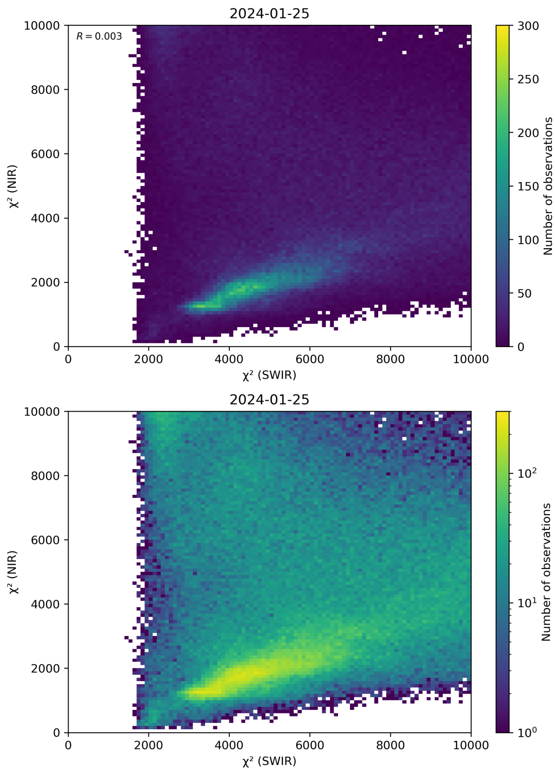
Figure 47: Scatter density plot of “ \chi^2 (SWIR)” against “ \chi^2 (NIR)” for 2024-01-24 to 2024-01-26.
