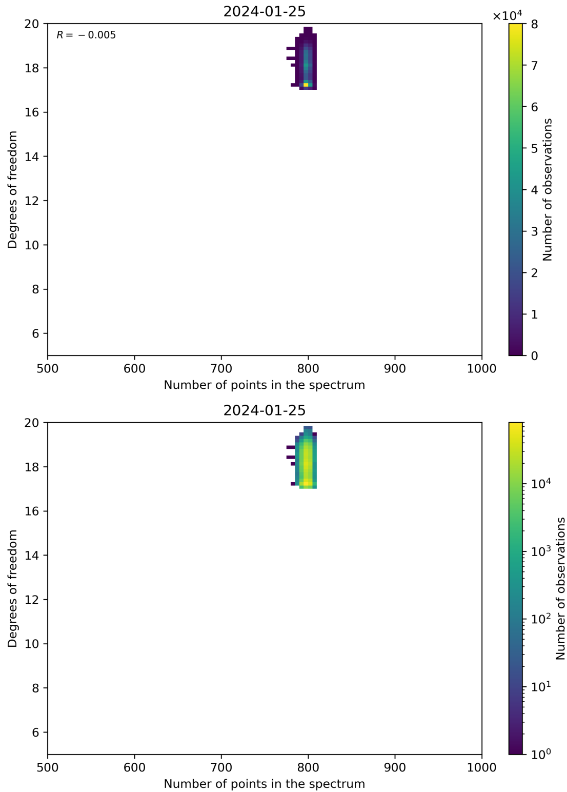
Figure 90: Scatter density plot of “Number of points in the spectrum” against “Degrees of freedom” for 2024-01-24 to 2024-01-26.
