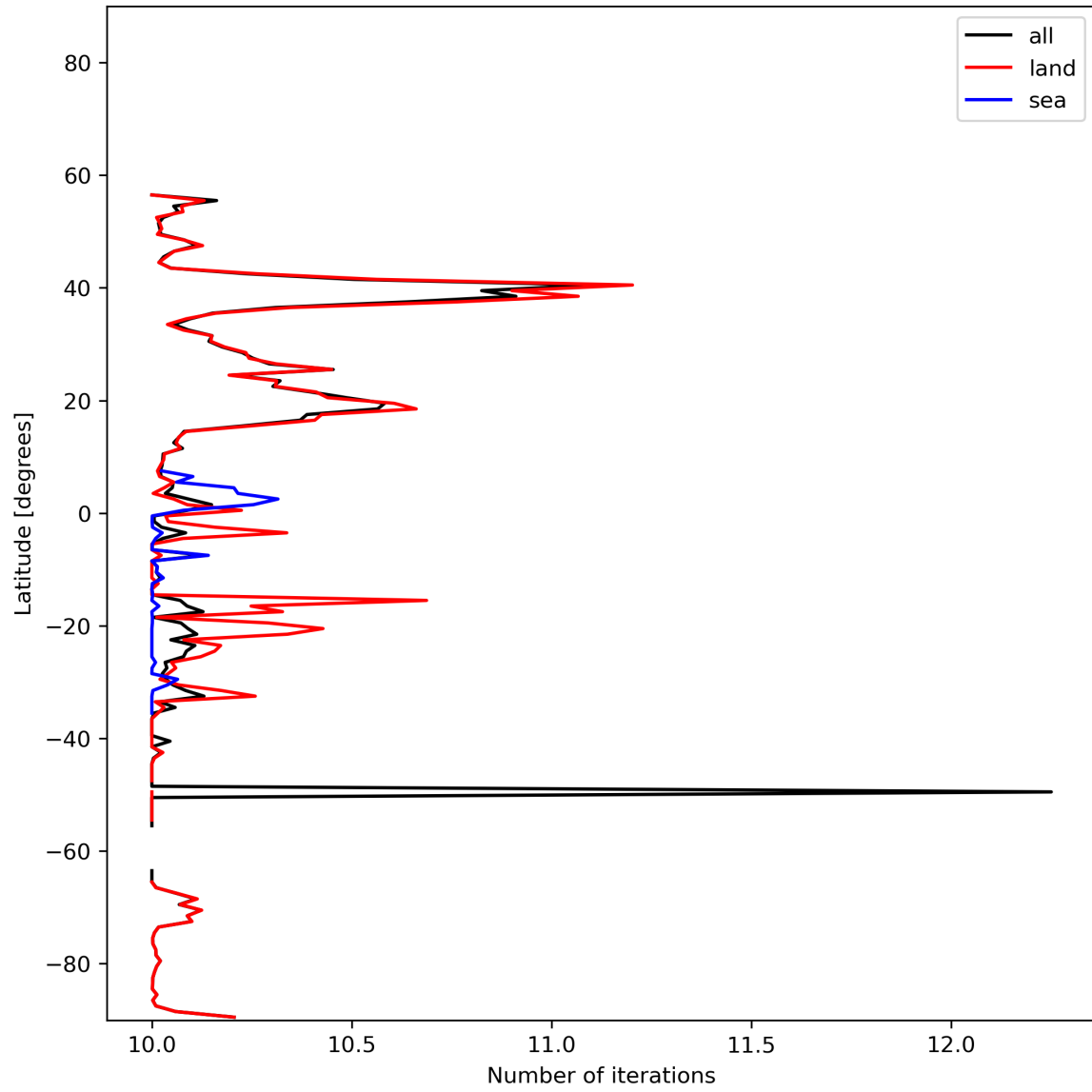
Figure 20: Zonal average of “Number of iterations” for 2024-01-24 to 2024-01-26.
