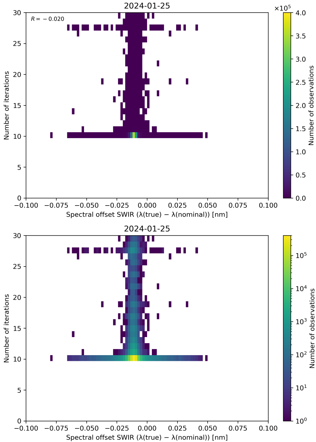
Figure 121: Scatter density plot of “Spectral offset SWIR ( \lambda(\text{true}) - \lambda(\text{nominal}) )” against “Number of iterations” for 2024-01-24 to 2024-01-26.
