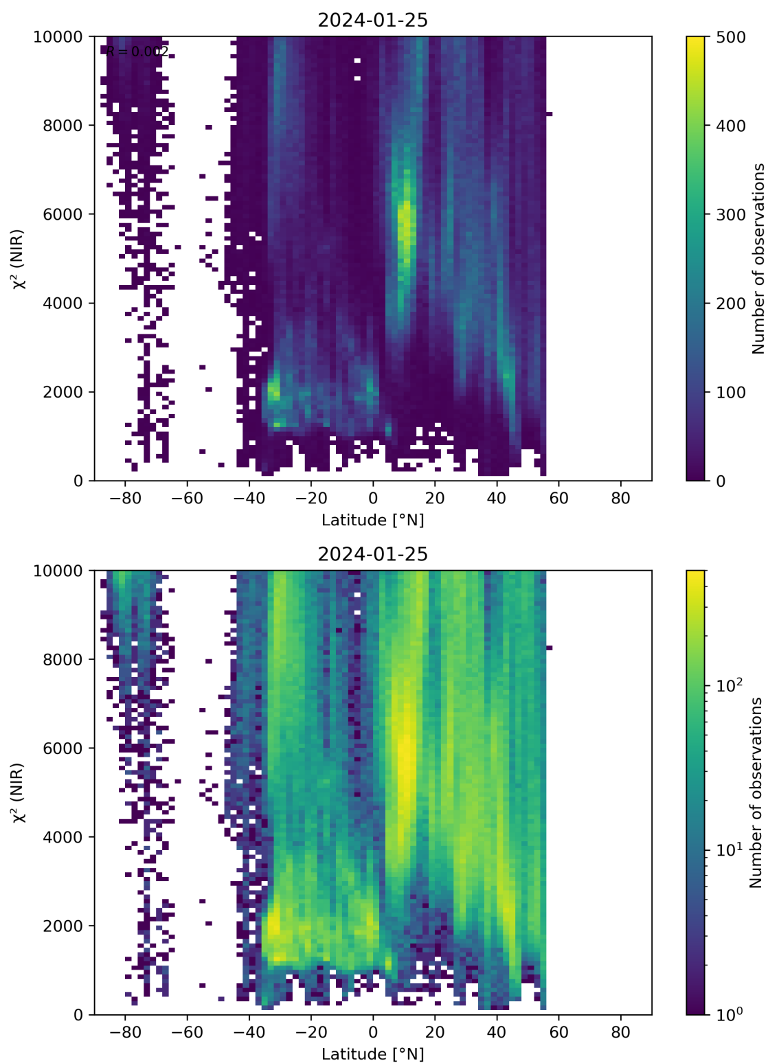
Figure 53: Scatter density plot of “Latitude” against “ \chi^2 (NIR)” for 2024-01-24 to 2024-01-26.
