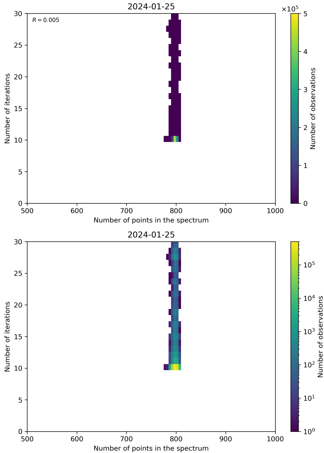
Figure 92: Scatter density plot of “Number of points in the spectrum” against “Number of iterations” for 2024-01-24 to 2024-01-26.
