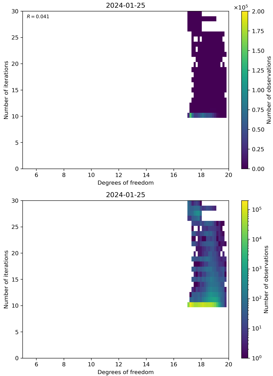
Figure 52: Scatter density plot of “Degrees of freedom” against “Number of iterations” for 2024-01-24 to 2024-01-26.
