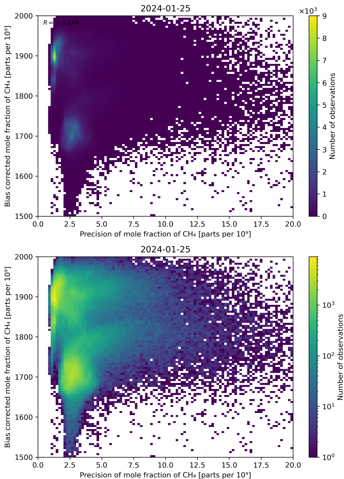
Figure 82: Scatter density plot of “Precision of mole fraction of CH 4 ” against “Bias corrected mole fraction of CH 4 ” for 2024-01-24 to 2024-01-26.
