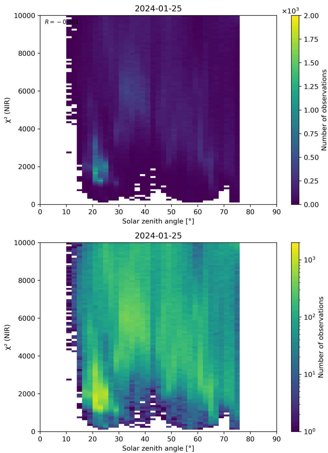
Figure 94: Scatter density plot of “Solar zenith angle” against “ \chi^2 (NIR)” for 2024-01-24 to 2024-01-26.
