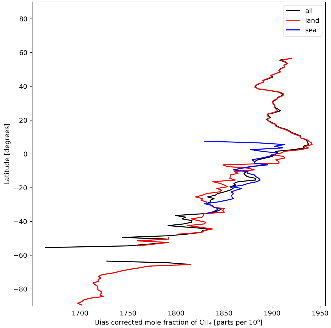
Figure 14: Zonal average of “Bias corrected mole fraction of \text{CH}_4 ” for 2024-01-24 to 2024-01-26.
