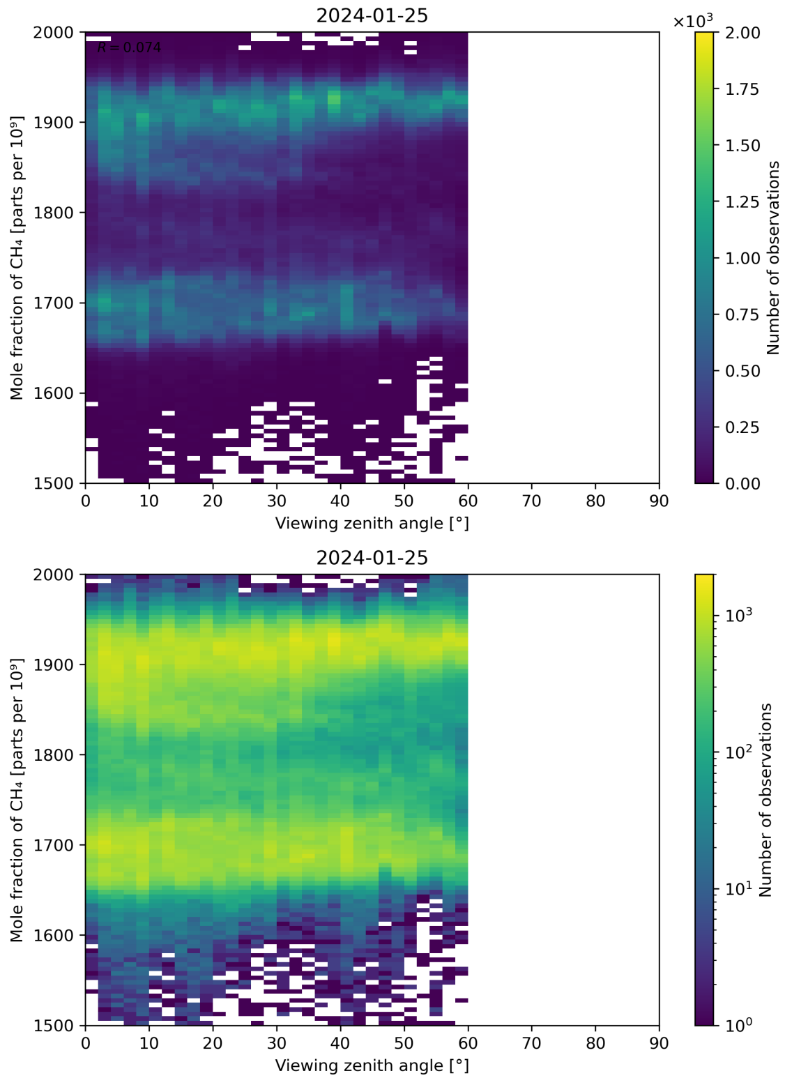
Figure 110: Scatter density plot of “Viewing zenith angle” against “Mole fraction of \text{CH}_4 ” for 2024-01-24 to 2024-01-26.
