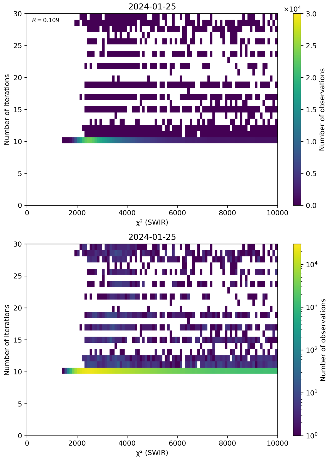
Figure 50: Scatter density plot of “ \chi^2 (SWIR)” against “Number of iterations” for 2024-01-24 to 2024-01-26.
