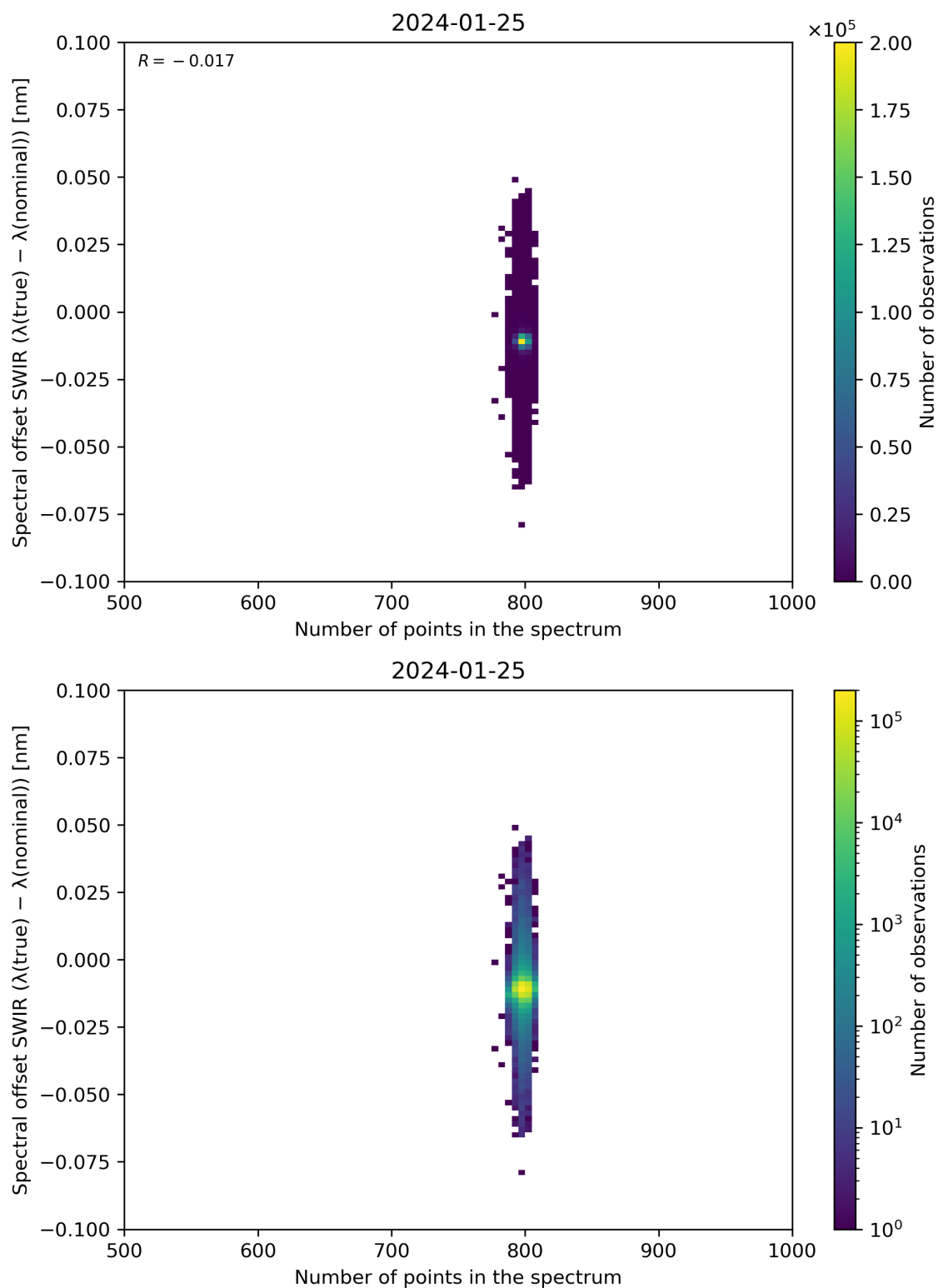
Figure 93: Scatter density plot of “Number of points in the spectrum” against “Spectral offset SWIR ( \lambda(\text{true}) - \lambda(\text{nominal}) )” for 2024-01-24 to 2024-01-26.
