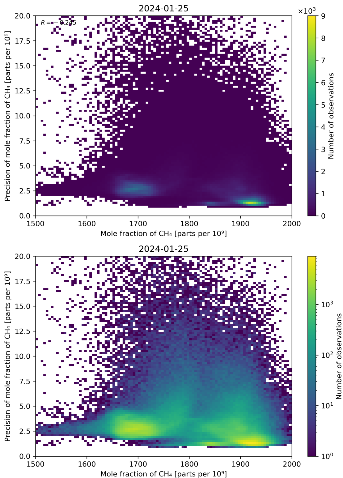
Figure 75: Scatter density plot of “Mole fraction of CH 4 ” against “Precision of mole fraction of CH 4 ” for 2024-01-24 to 2024-01-26.
