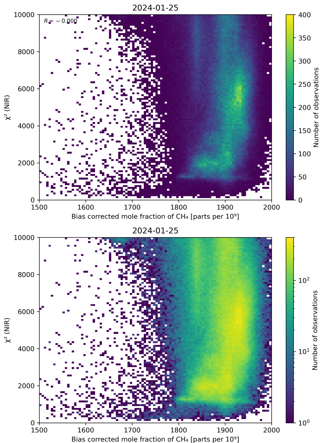
Figure 63: Scatter density plot of “Bias corrected mole fraction of CH 4 ” against “ \chi^2 (NIR)” for 2024-01-24 to 2024-01-26.
