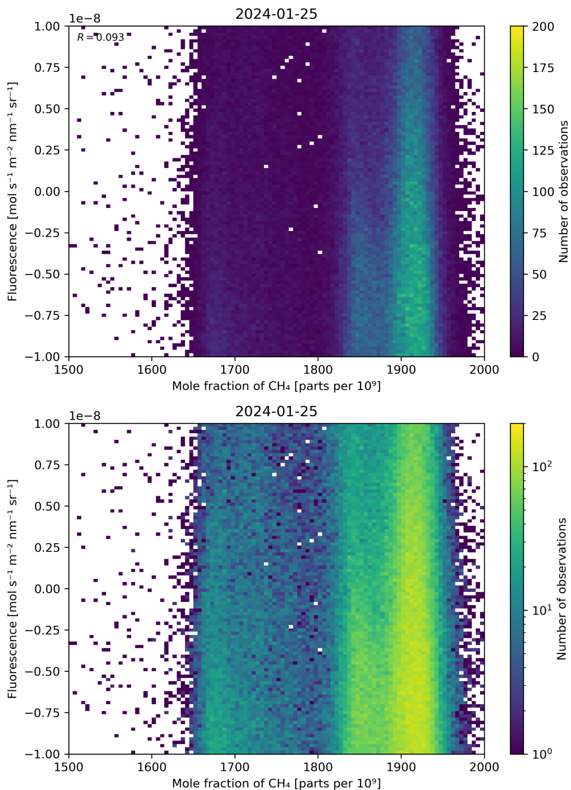
Figure 73: Scatter density plot of “Mole fraction of \text{CH}_4 ” against “Fluorescence” for 2024-01-24 to 2024-01-26.
