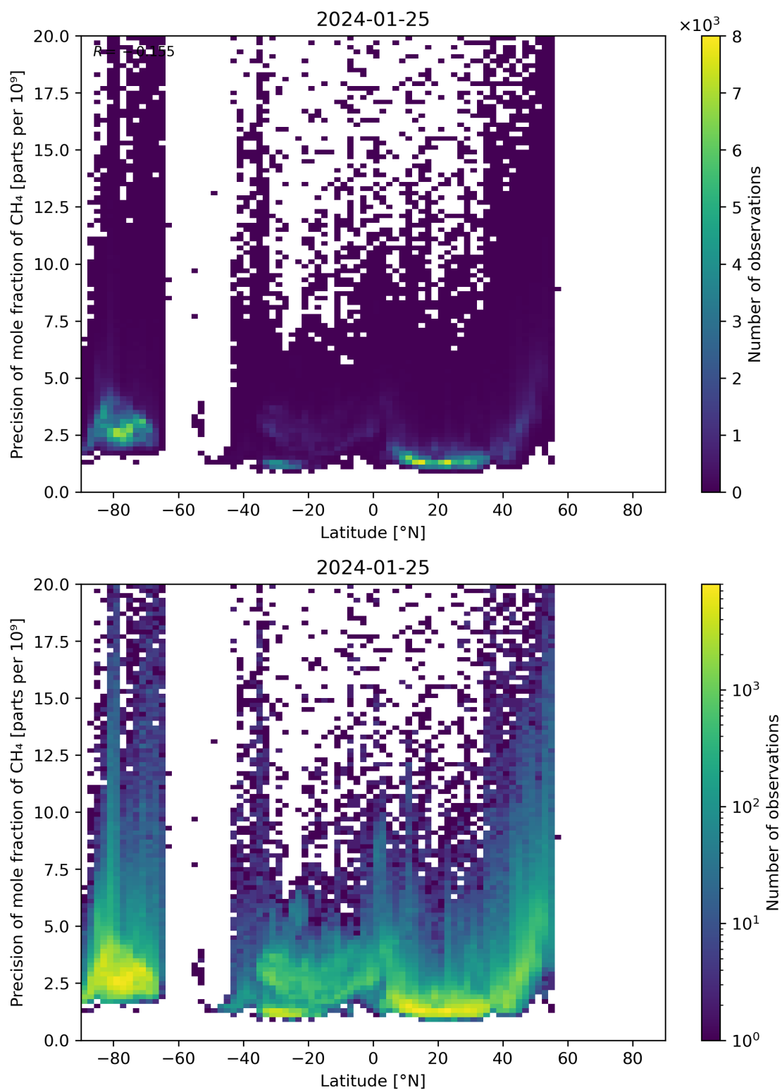
Figure 59: Scatter density plot of “Latitude” against “Precision of mole fraction of CH 4 ” for 2024-01-24 to 2024-01-26.
