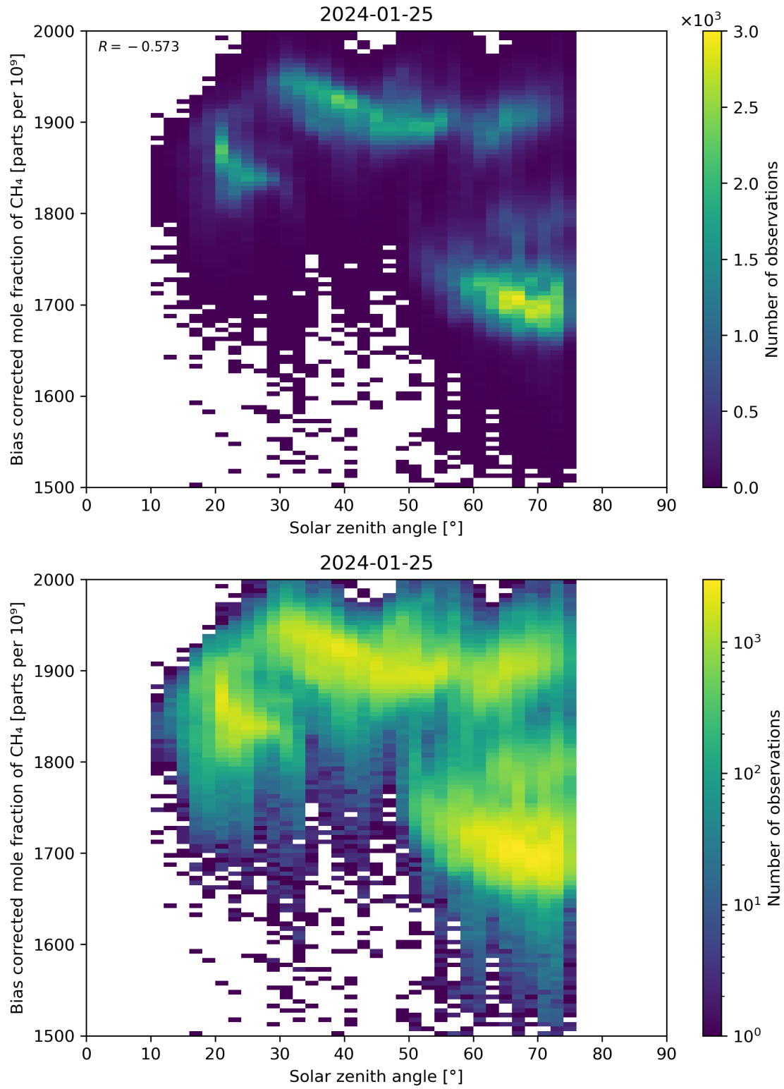
Figure 100: Scatter density plot of “Solar zenith angle” against “Bias corrected mole fraction of \text{CH}_4 ” for 2024-01-24 to 2024-01-26.
