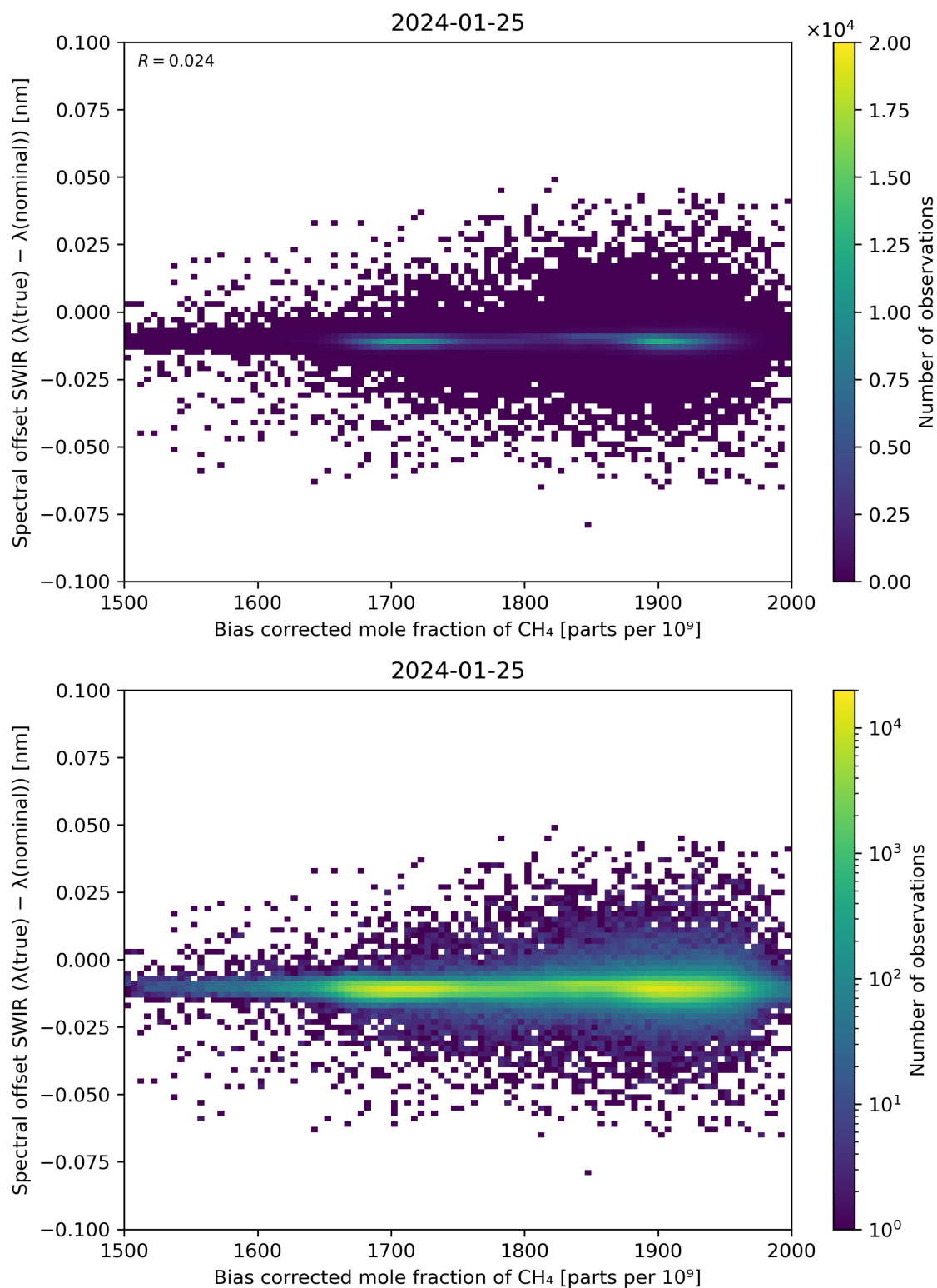
Figure 69: Scatter density plot of “Bias corrected mole fraction of \text{CH}_4 ” against “Spectral offset SWIR ( \lambda(\text{true}) - \lambda(\text{nominal}) )” for 2024-01-24 to 2024-01-26.
