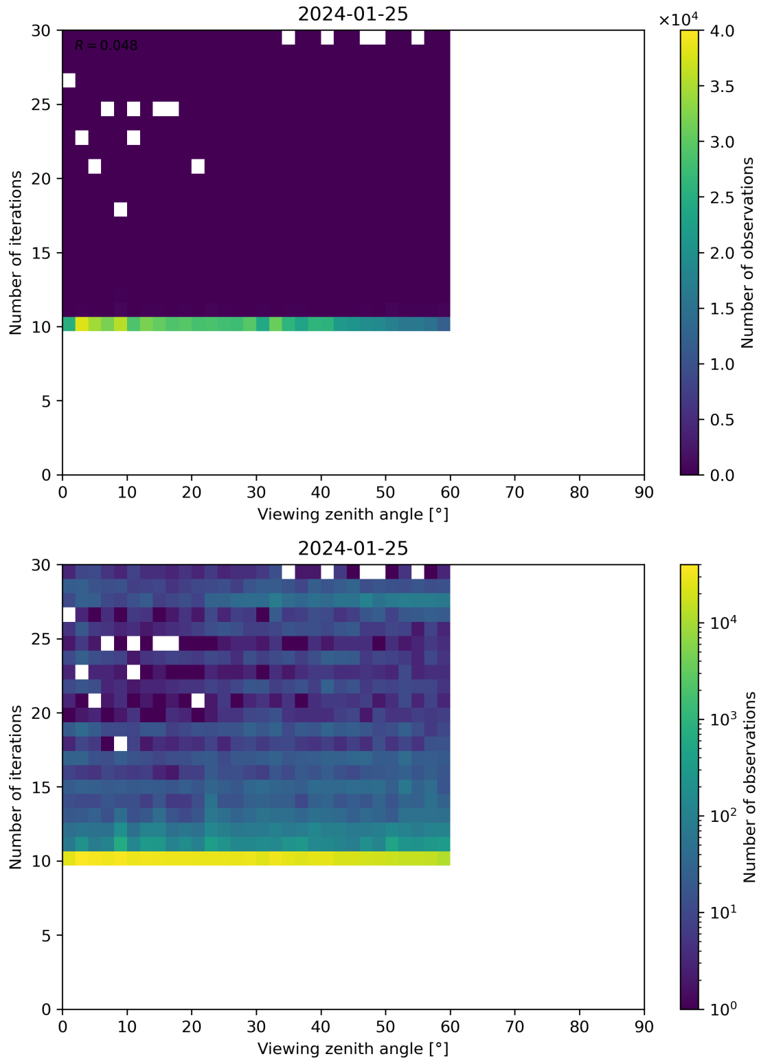
Figure 113: Scatter density plot of “Viewing zenith angle” against “Number of iterations” for 2024-01-24 to 2024-01-26.
