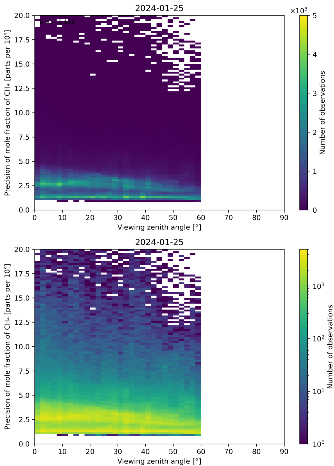
Figure 112: Scatter density plot of “Viewing zenith angle” against “Precision of mole fraction of CH 4 ” for 2024-01-24 to 2024-01-26.
