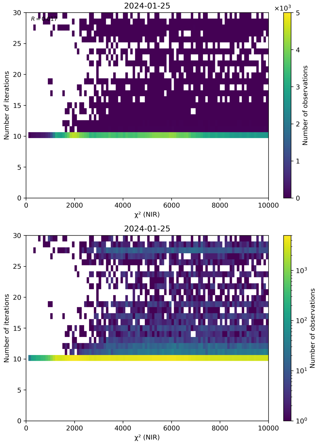
Figure 46: Scatter density plot of “ \chi^2 (NIR)” against “Number of iterations” for 2024-01-24 to 2024-01-26.
