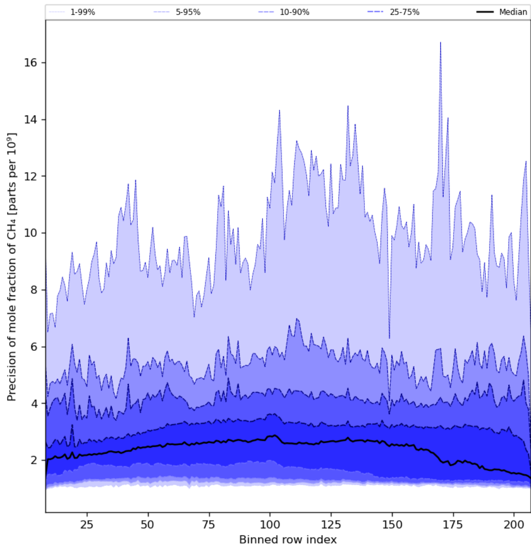
Figure 35: Along track statistics of “Precision of mole fraction of CH 4 ” for 2024-01-24 to 2024-01-26
