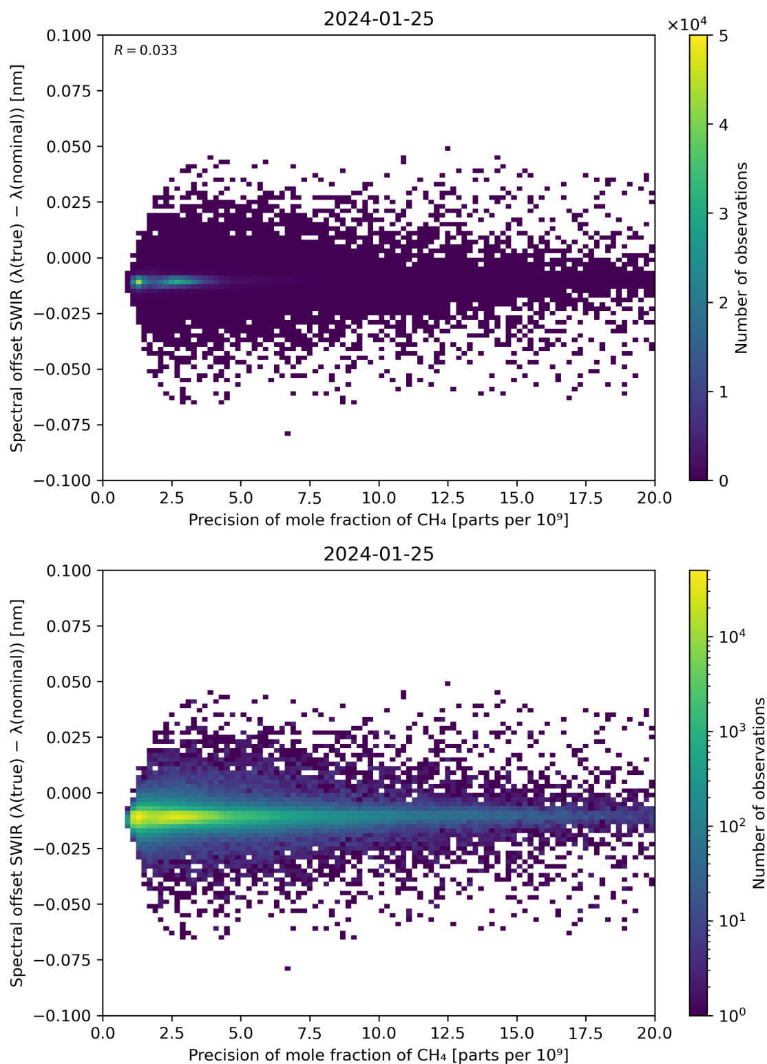
Figure 85: Scatter density plot of “Precision of mole fraction of CH 4 ” against “Spectral offset SWIR ( \lambda(\text{true}) - \lambda(\text{nominal}) )” for 2024-01-24 to 2024-01-26.
