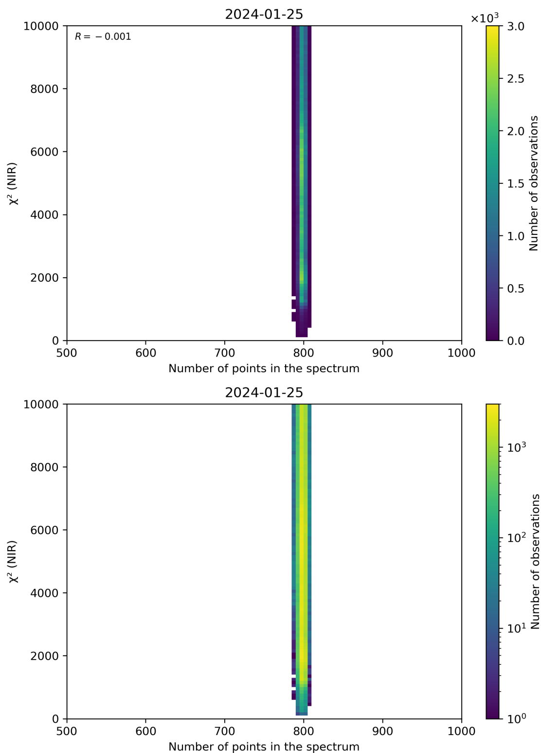
Figure 88: Scatter density plot of “Number of points in the spectrum” against “ \chi^2 (NIR)” for 2024-01-24 to 2024-01-26.
