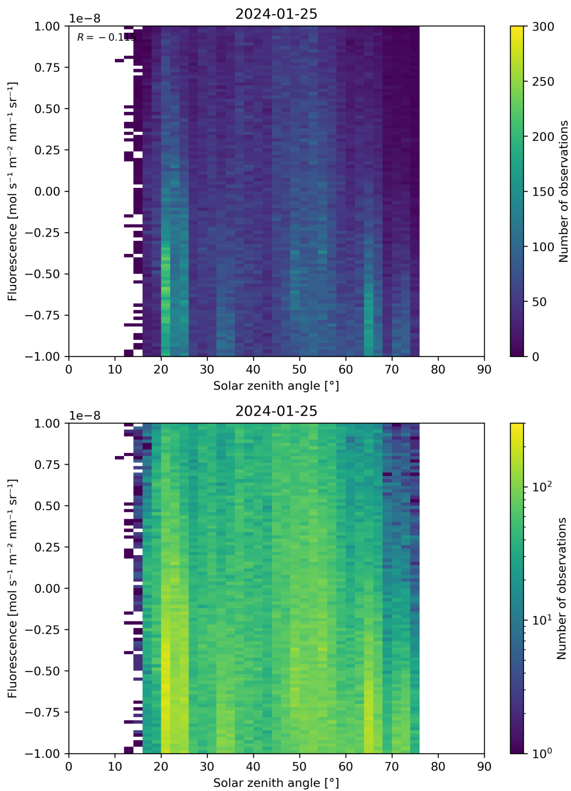
Figure 97: Scatter density plot of “Solar zenith angle” against “Fluorescence” for 2024-01-24 to 2024-01-26.
