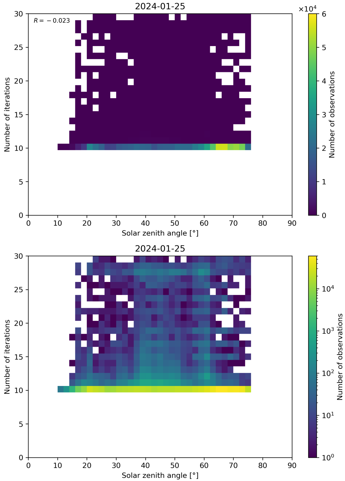
Figure 102: Scatter density plot of “Solar zenith angle” against “Number of iterations” for 2024-01-24 to 2024-01-26.
