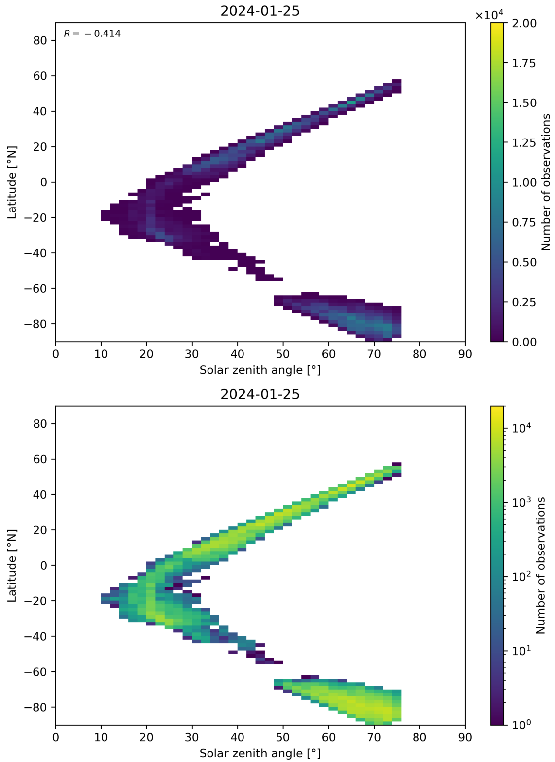
Figure 98: Scatter density plot of “Solar zenith angle” against “Latitude” for 2024-01-24 to 2024-01-26.
