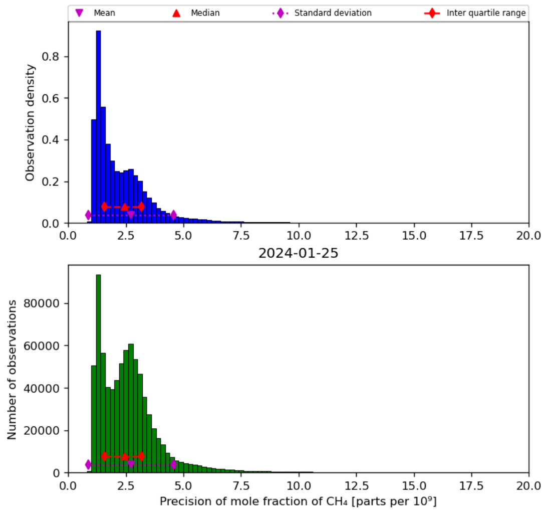
Figure 24: Histogram of “Precision of mole fraction of CH 4 ” for 2024-01-24 to 2024-01-26
