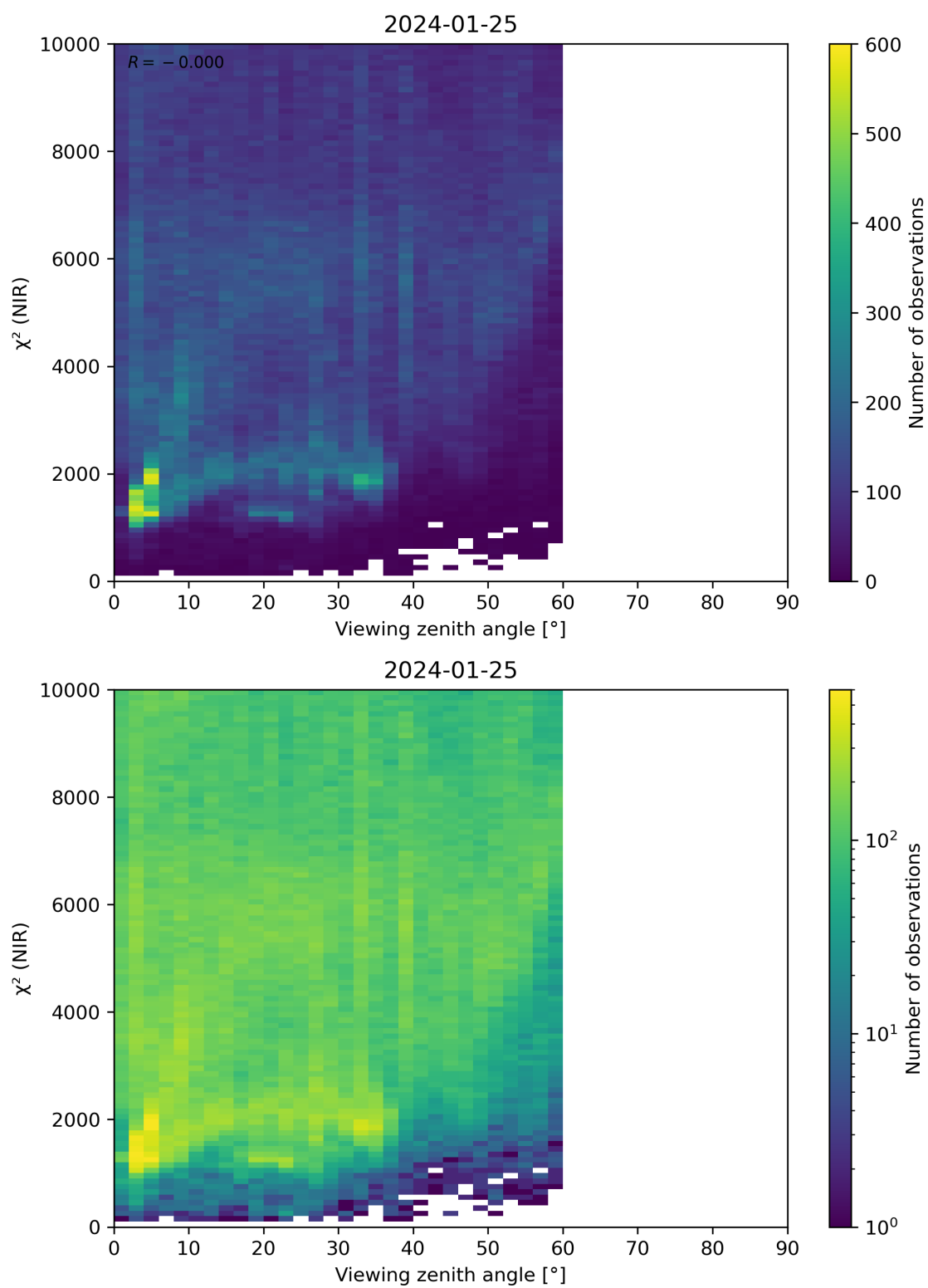
Figure 105: Scatter density plot of “Viewing zenith angle” against “ \chi^2 (NIR)” for 2024-01-24 to 2024-01-26.
