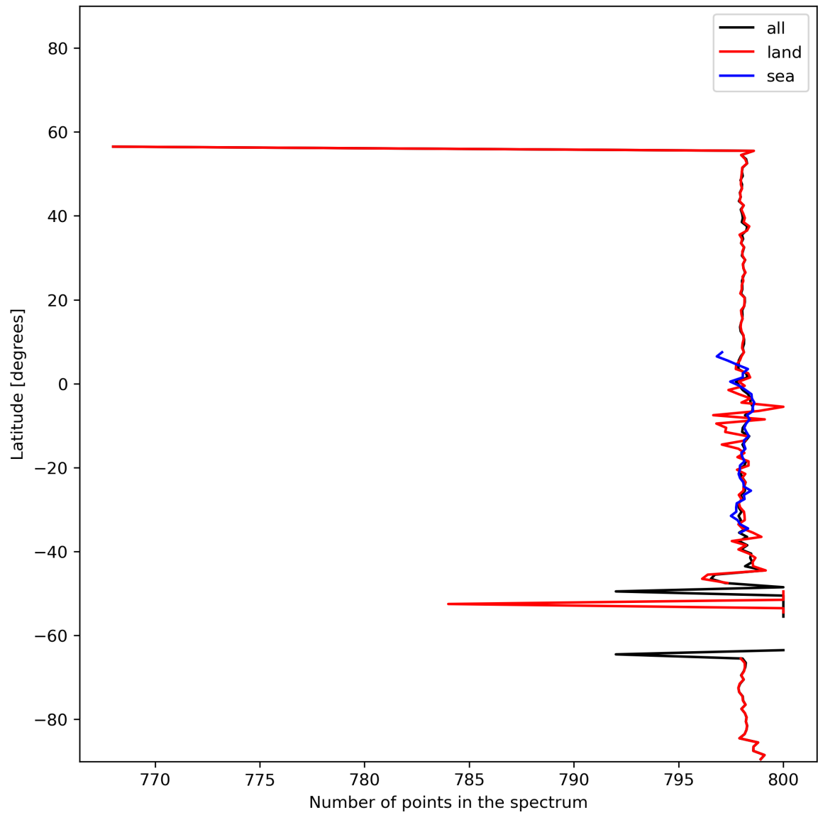
Figure 15: Zonal average of “Number of points in the spectrum” for 2024-01-24 to 2024-01-26.
