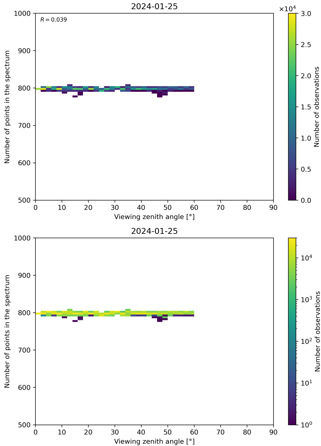
Figure 114: Scatter density plot of “Viewing zenith angle” against “Number of points in the spectrum” for 2024-01-24 to 2024-01-26.
