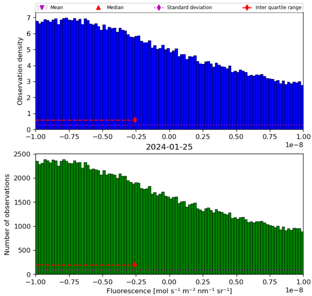
Figure 32: Histogram of “Fluorescence” for 2024-01-24 to 2024-01-26
