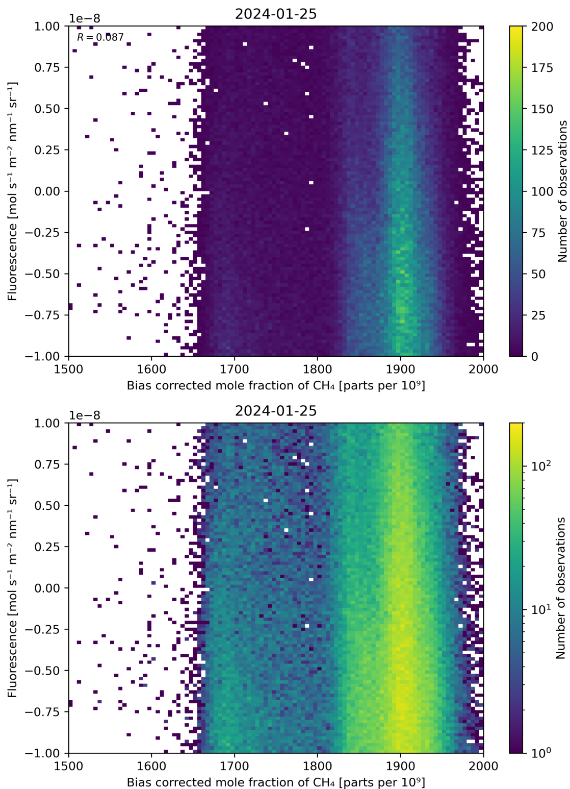
Figure 66: Scatter density plot of “Bias corrected mole fraction of \text{CH}_4 ” against “Fluorescence” for 2024-01-24 to 2024-01-26.
