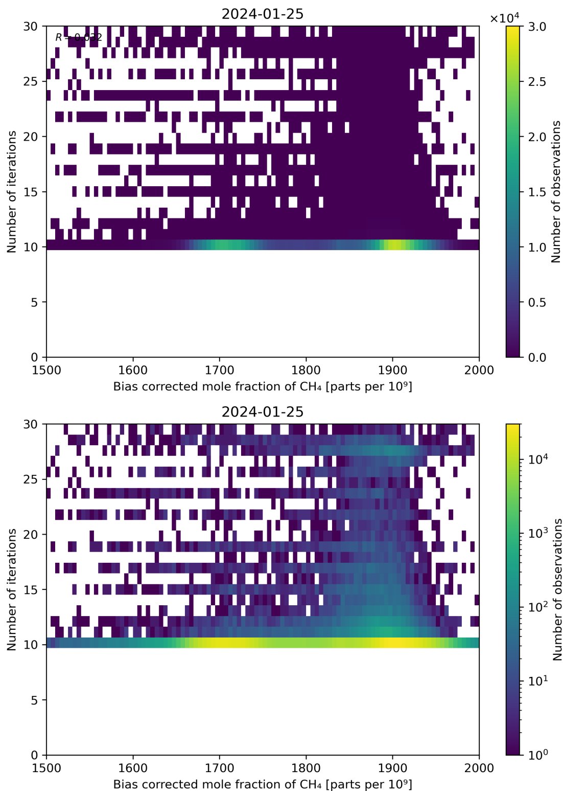
Figure 67: Scatter density plot of “Bias corrected mole fraction of \text{CH}_4 ” against “Number of iterations” for 2024-01-24 to 2024-01-26.
