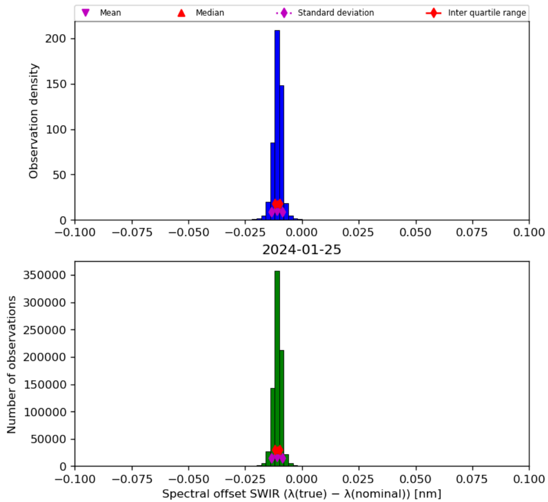
Figure 27: Histogram of “Spectral offset SWIR ( \lambda(\text{true}) - \lambda(\text{nominal}) )” for 2024-01-24 to 2024-01-26
