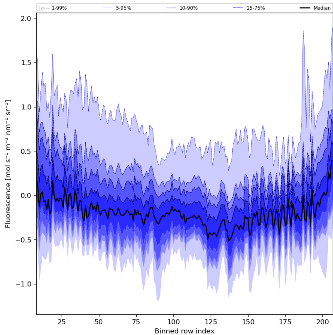
Figure 43: Along track statistics of “Fluorescence” for 2024-01-24 to 2024-01-26
