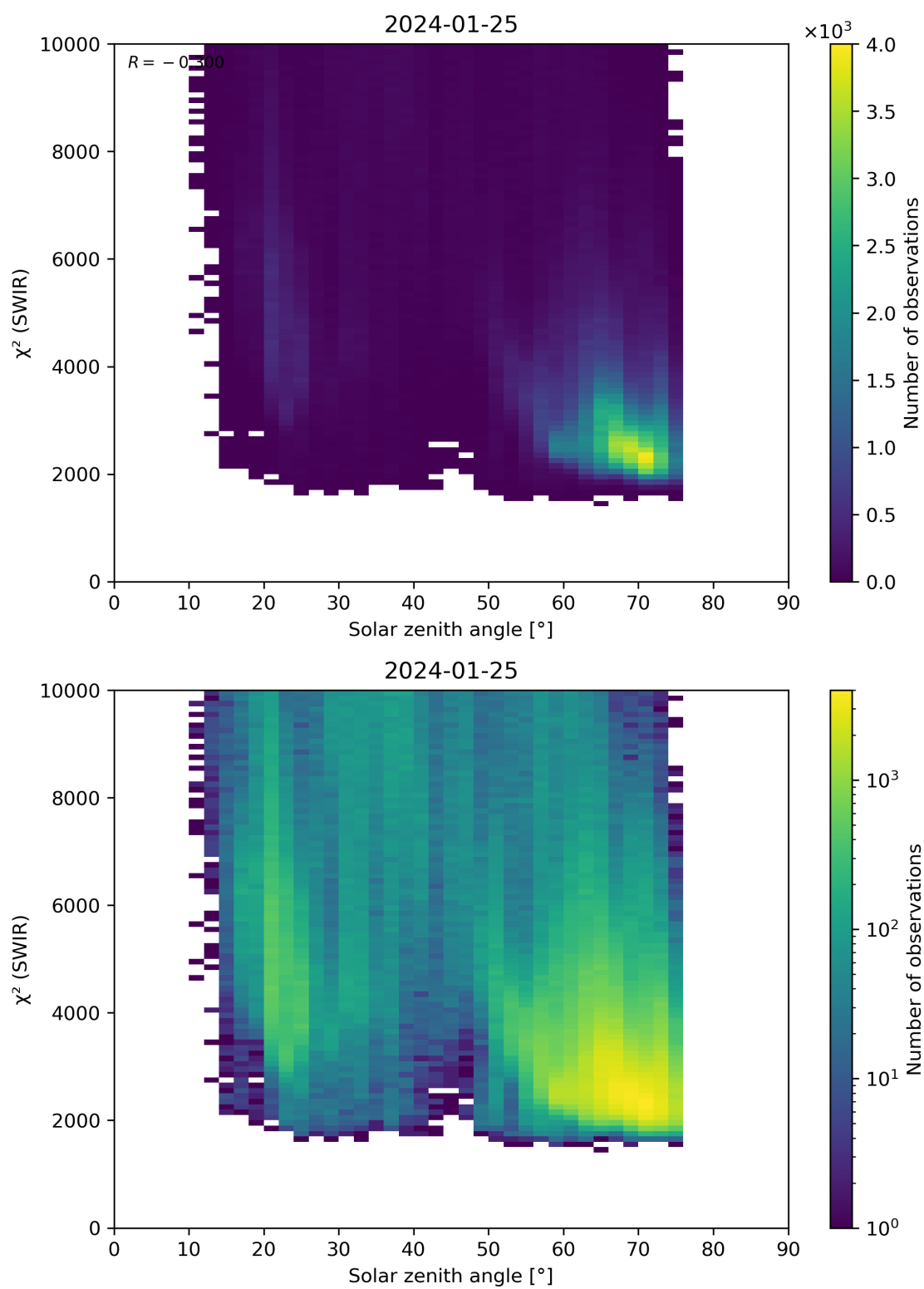
Figure 95: Scatter density plot of “Solar zenith angle” against “ \chi^2 (SWIR)” for 2024-01-24 to 2024-01-26.
