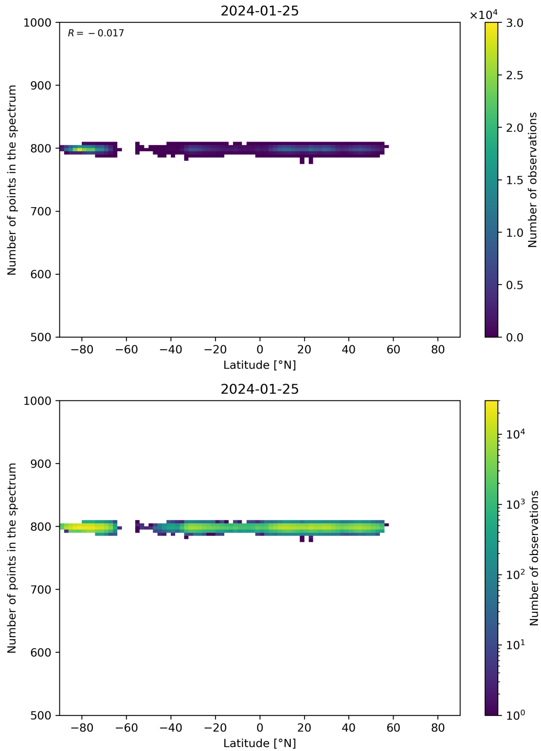
Figure 61: Scatter density plot of “Latitude” against “Number of points in the spectrum” for 2024-01-24 to 2024-01-26.
