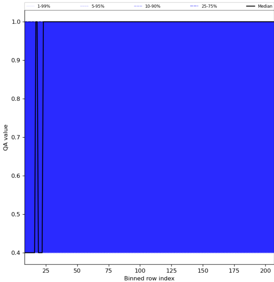
Figure 33: Along track statistics of “QA value” for 2024-01-24 to 2024-01-26
