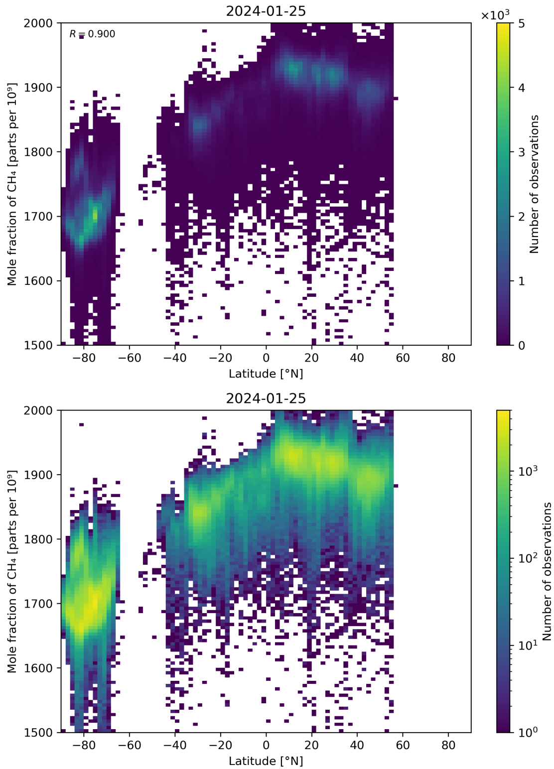
Figure 57: Scatter density plot of “Latitude” against “Mole fraction of CH 4 ” for 2024-01-24 to 2024-01-26.
