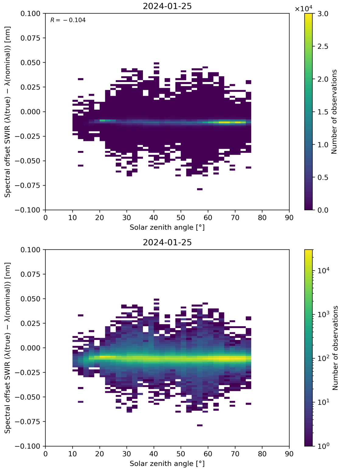
Figure 104: Scatter density plot of “Solar zenith angle” against “Spectral offset SWIR ( \lambda(\text{true}) - \lambda(\text{nominal}) )” for 2024-01-24 to 2024-01-26.
