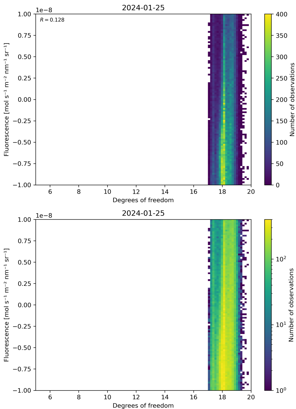
Figure 51: Scatter density plot of “Degrees of freedom” against “Fluorescence” for 2024-01-24 to 2024-01-26.
