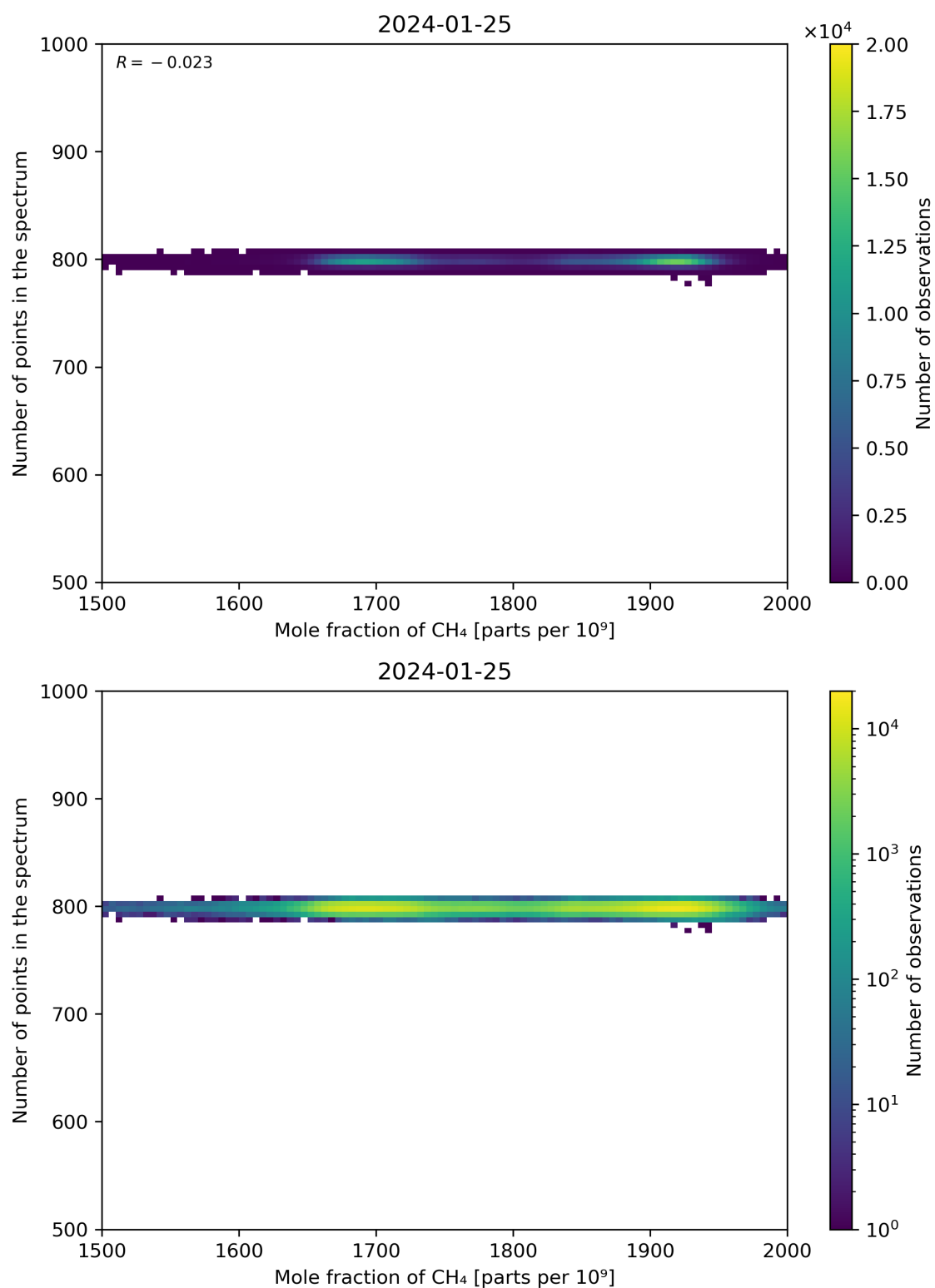
Figure 77: Scatter density plot of “Mole fraction of CH 4 ” against “Number of points in the spectrum” for 2024-01-24 to 2024-01-26.
