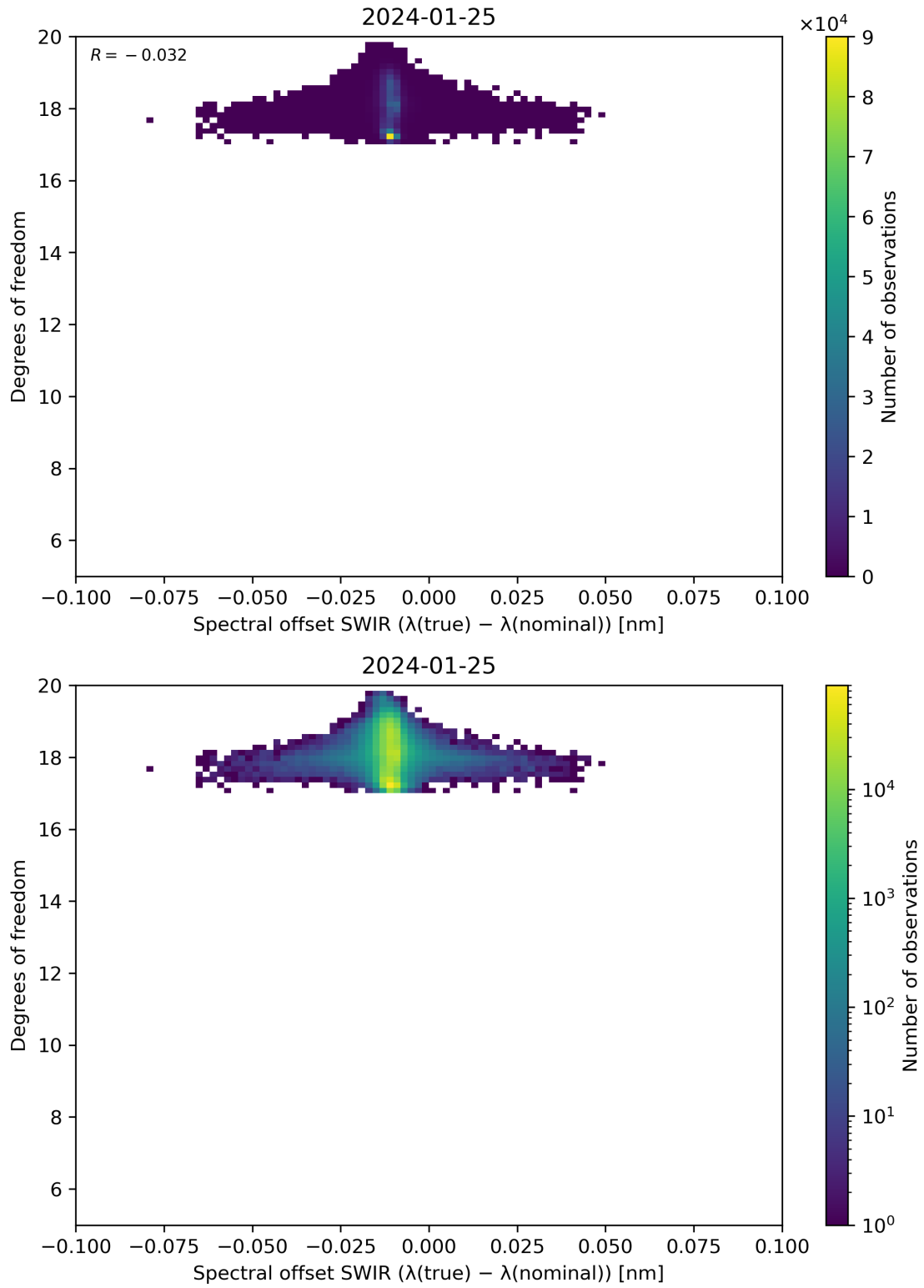
Figure 119: Scatter density plot of “Spectral offset SWIR ( \lambda(\text{true}) - \lambda(\text{nominal}) )” against “Degrees of freedom” for 2024-01-24 to 2024-01-26.
