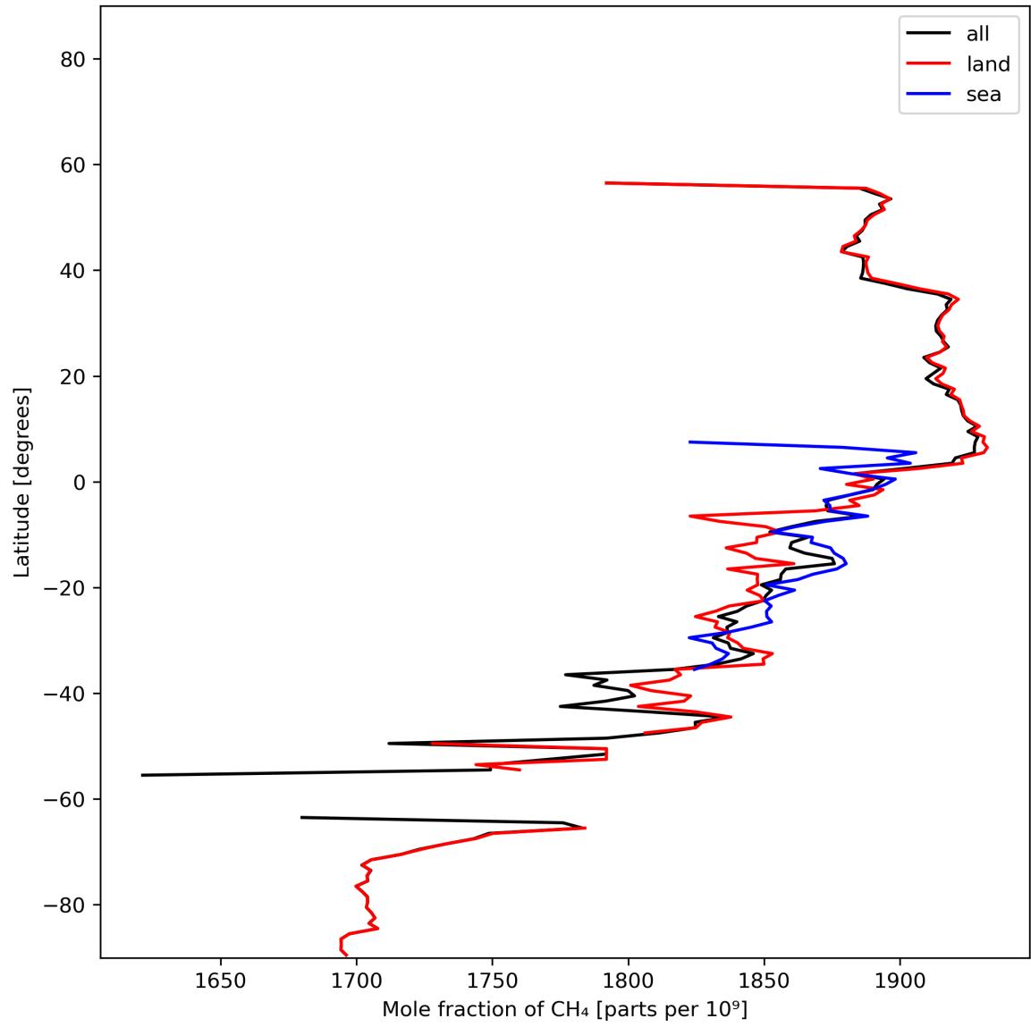
Figure 12: Zonal average of “Mole fraction of \text{CH}_4 ” for 2024-01-24 to 2024-01-26.
