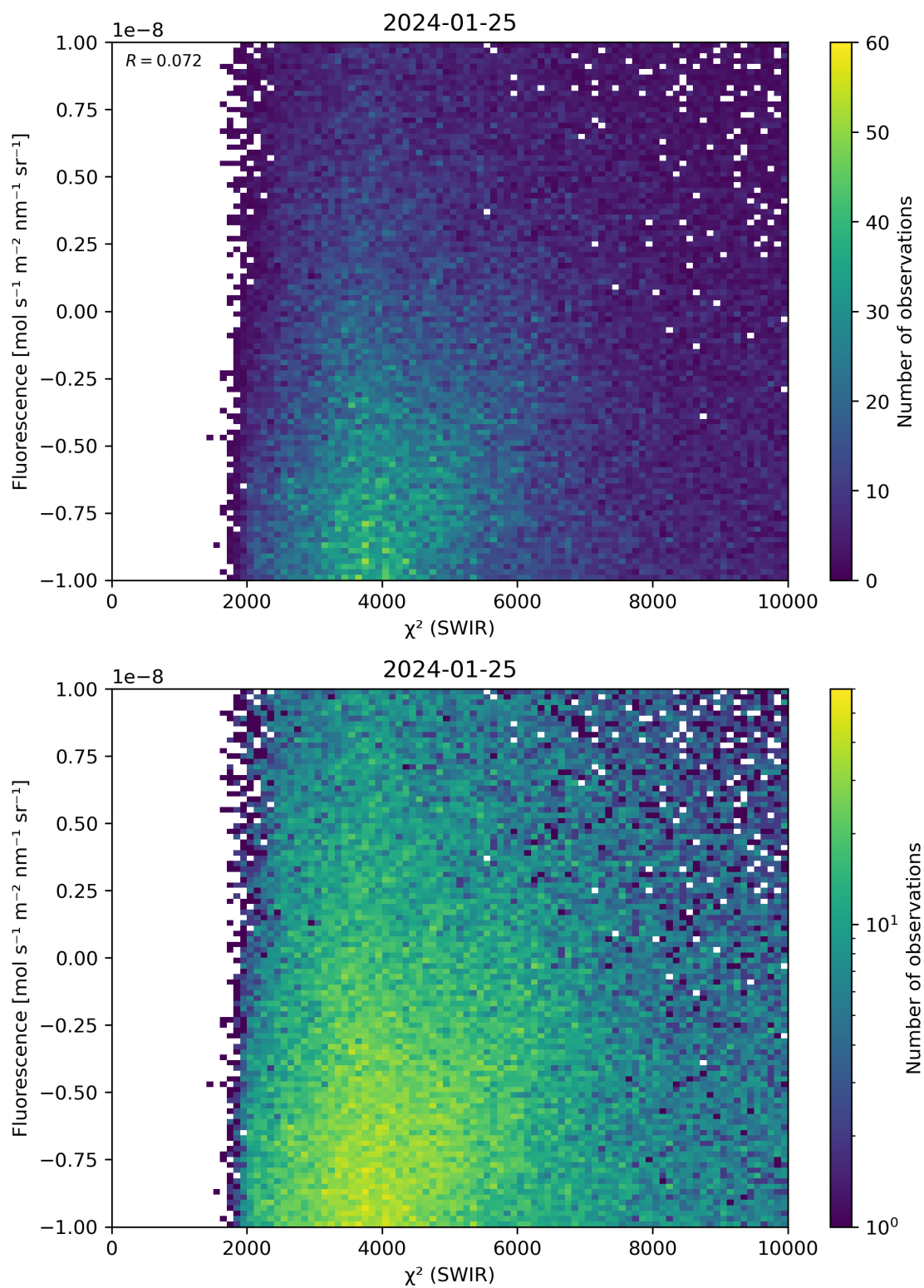
Figure 49: Scatter density plot of “ \chi^2 (SWIR)” against “Fluorescence” for 2024-01-24 to 2024-01-26.
