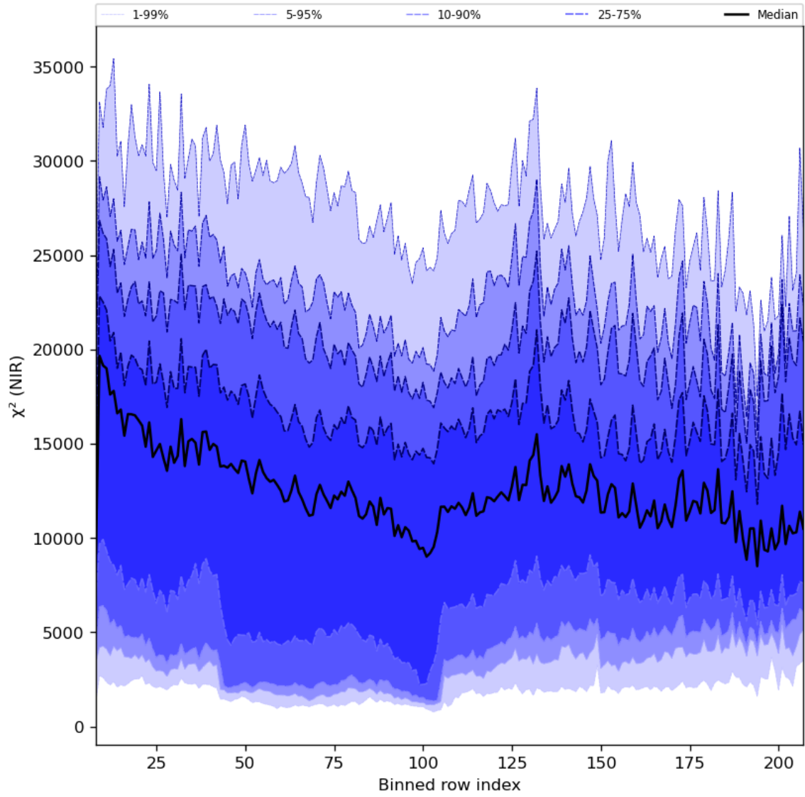
Figure 40: Along track statistics of “ \chi^2 (NIR)” for 2024-01-24 to 2024-01-26
