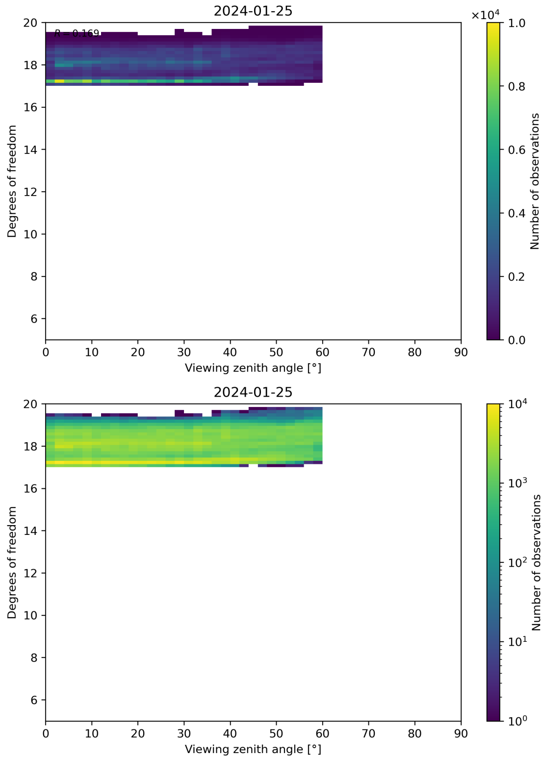
Figure 107: Scatter density plot of “Viewing zenith angle” against “Degrees of freedom” for 2024-01-24 to 2024-01-26.
