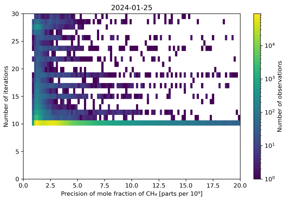
Figure 83: Scatter density plot of “Precision of mole fraction of \text{CH}_4 ” against “Number of iterations” for 2024-01-24 to 2024-01-26.
