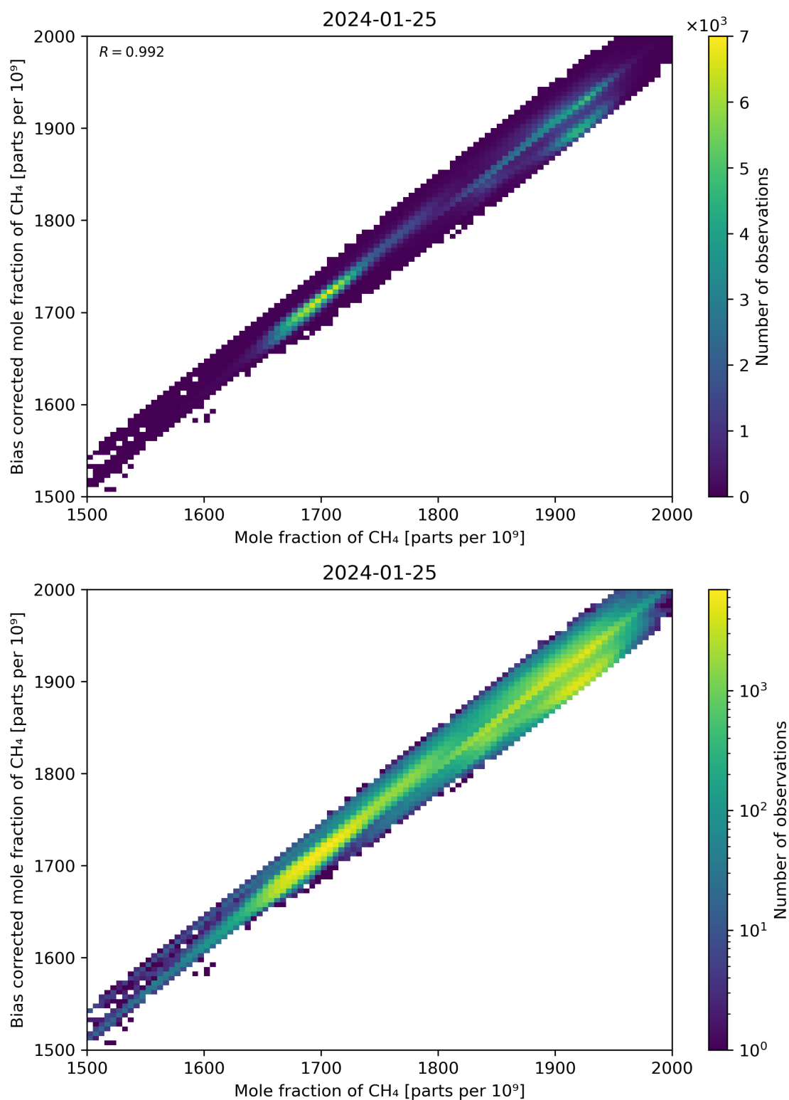
Figure 74: Scatter density plot of “Mole fraction of CH 4 ” against “Bias corrected mole fraction of CH 4 ” for 2024-01-24 to 2024-01-26.
