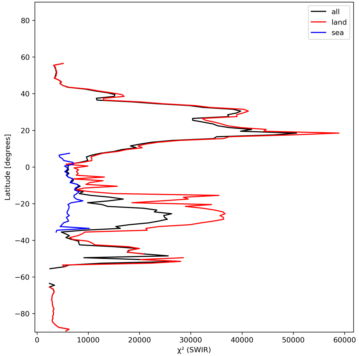
Figure 17: Zonal average of “ \chi^2 (SWIR)” for 2024-01-24 to 2024-01-26.
