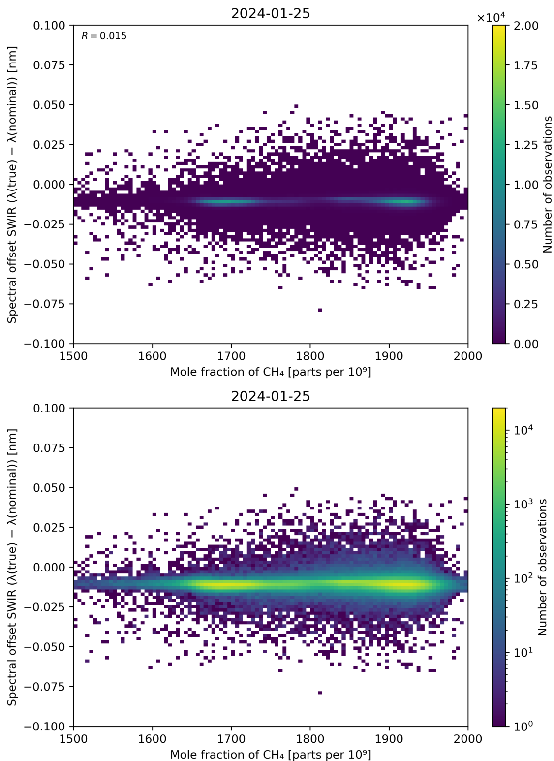
Figure 86: Scatter density plot of “Mole fraction of CH 4 ” against “Spectral offset SWIR ( \lambda(\text{true}) - \lambda(\text{nominal}) )” for 2024-01-24 to 2024-01-26.
