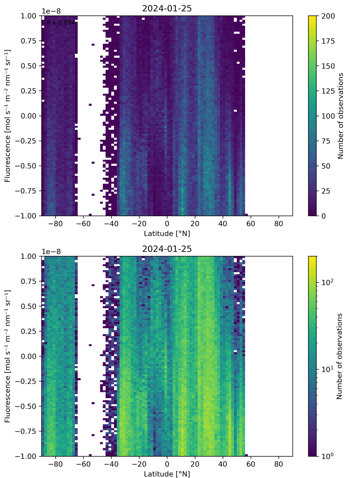
Figure 56: Scatter density plot of “Latitude” against “Fluorescence” for 2024-01-24 to 2024-01-26.
