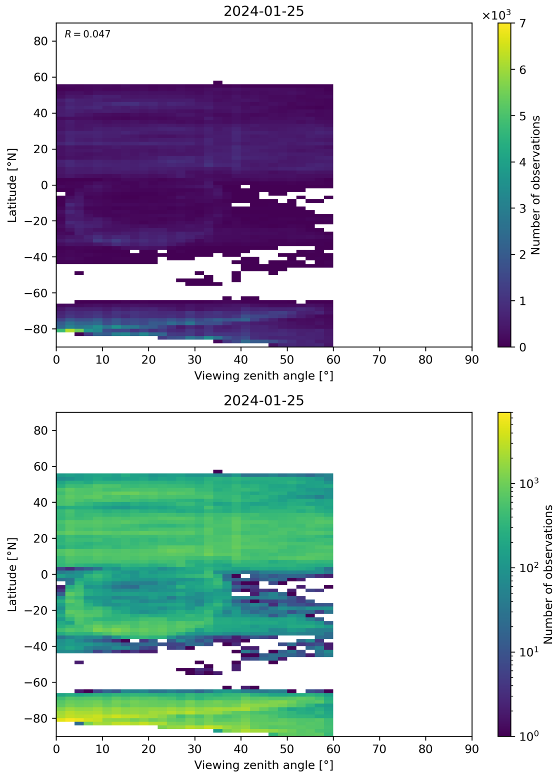
Figure 109: Scatter density plot of “Viewing zenith angle” against “Latitude” for 2024-01-24 to 2024-01-26.
