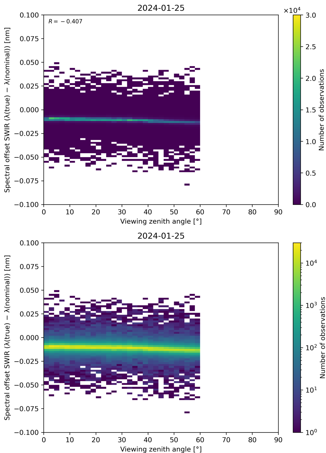
Figure 116: Scatter density plot of “Viewing zenith angle” against “Spectral offset SWIR ( \lambda(\text{true}) - \lambda(\text{nominal}) )” for 2024-01-24 to 2024-01-26.
