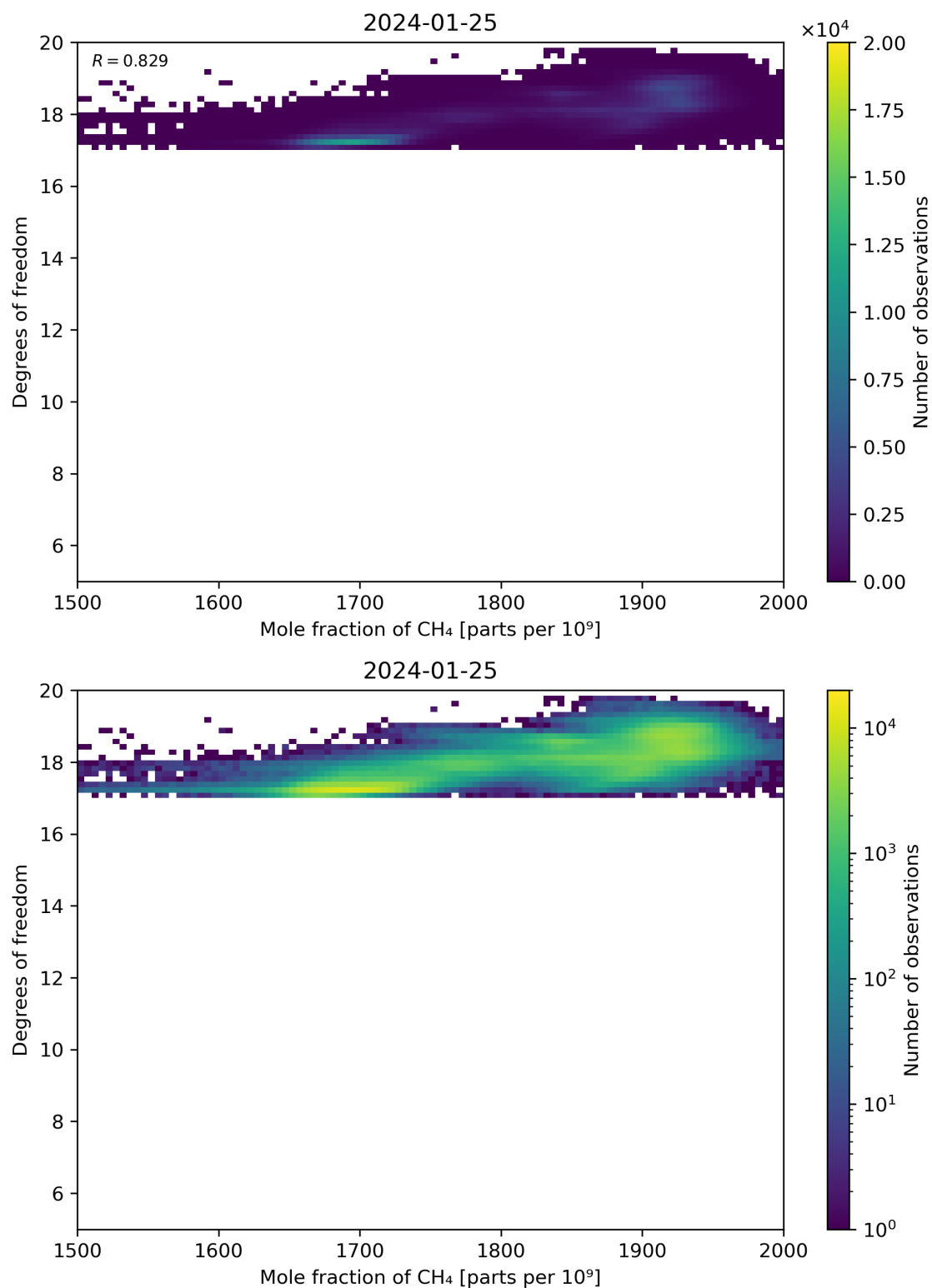
Figure 72: Scatter density plot of “Mole fraction of CH 4 ” against “Degrees of freedom” for 2024-01-24 to 2024-01-26.
