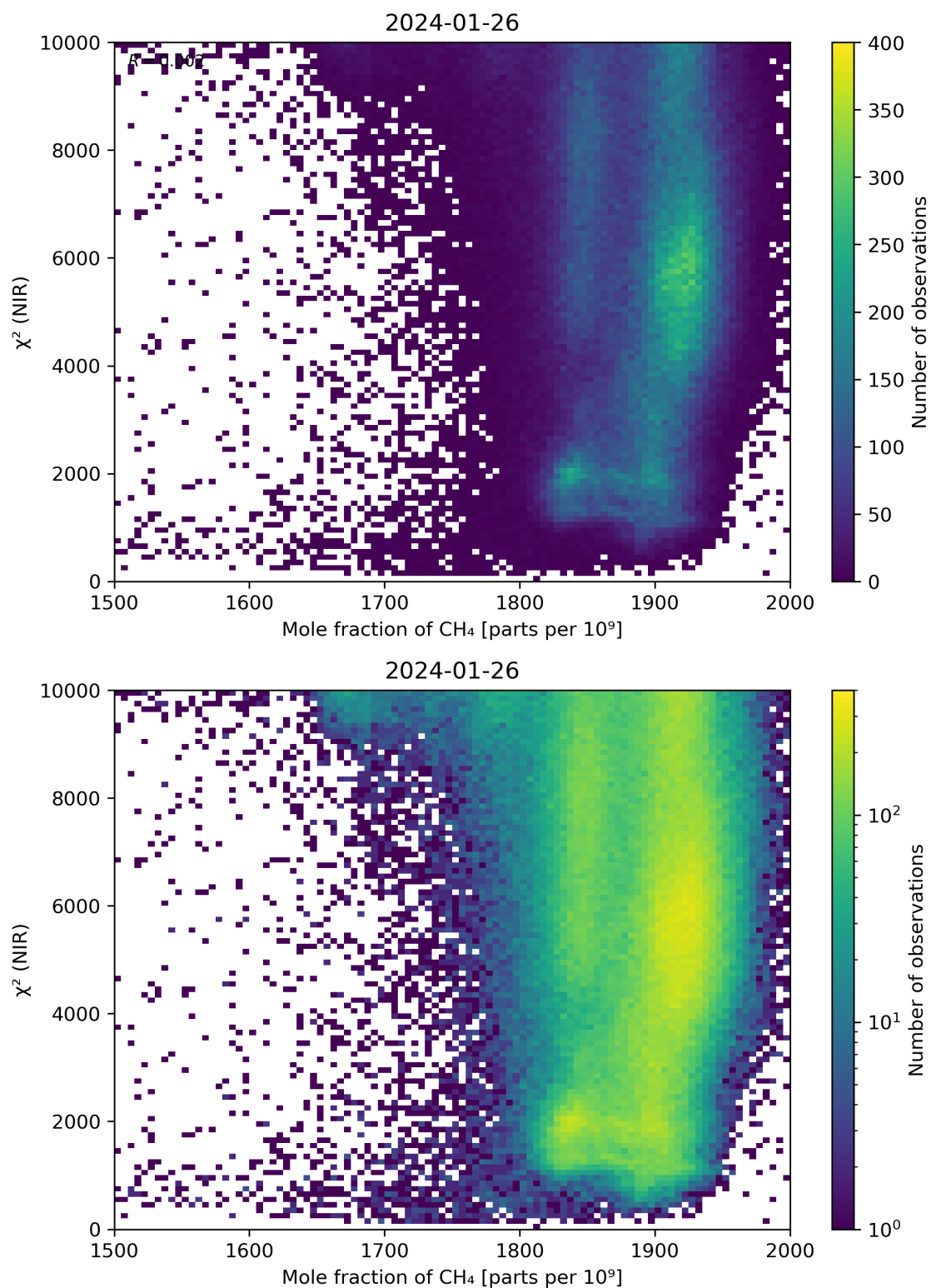
Figure 70: Scatter density plot of “Mole fraction of \text{CH}_4 ” against “ \chi^2 (NIR)” for 2024-01-26 to 2024-01-27.
