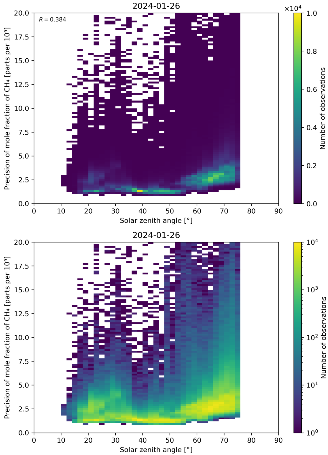
Figure 101: Scatter density plot of “Solar zenith angle” against “Precision of mole fraction of \text{CH}_4 ” for 2024-01-26 to 2024-01-27.
