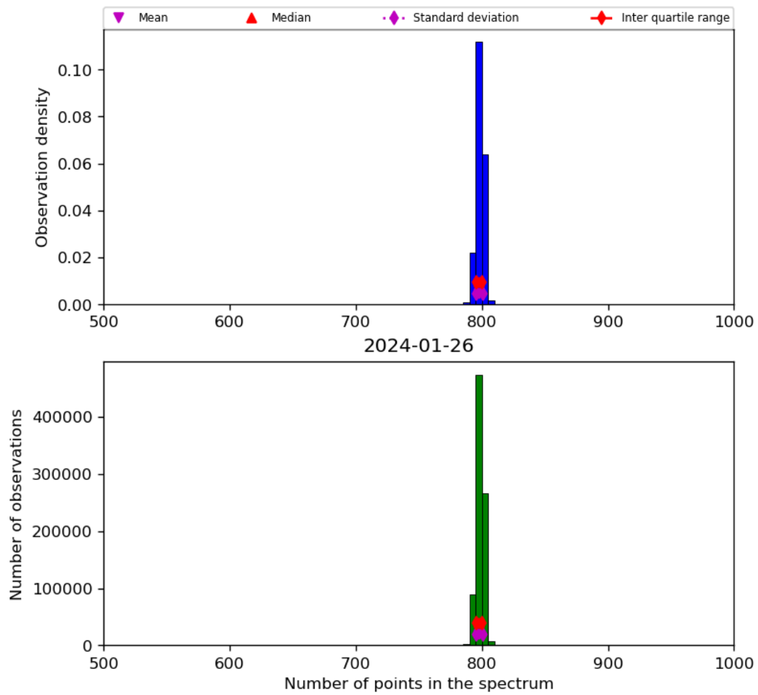
Figure 26: Histogram of “Number of points in the spectrum” for 2024-01-26 to 2024-01-27
