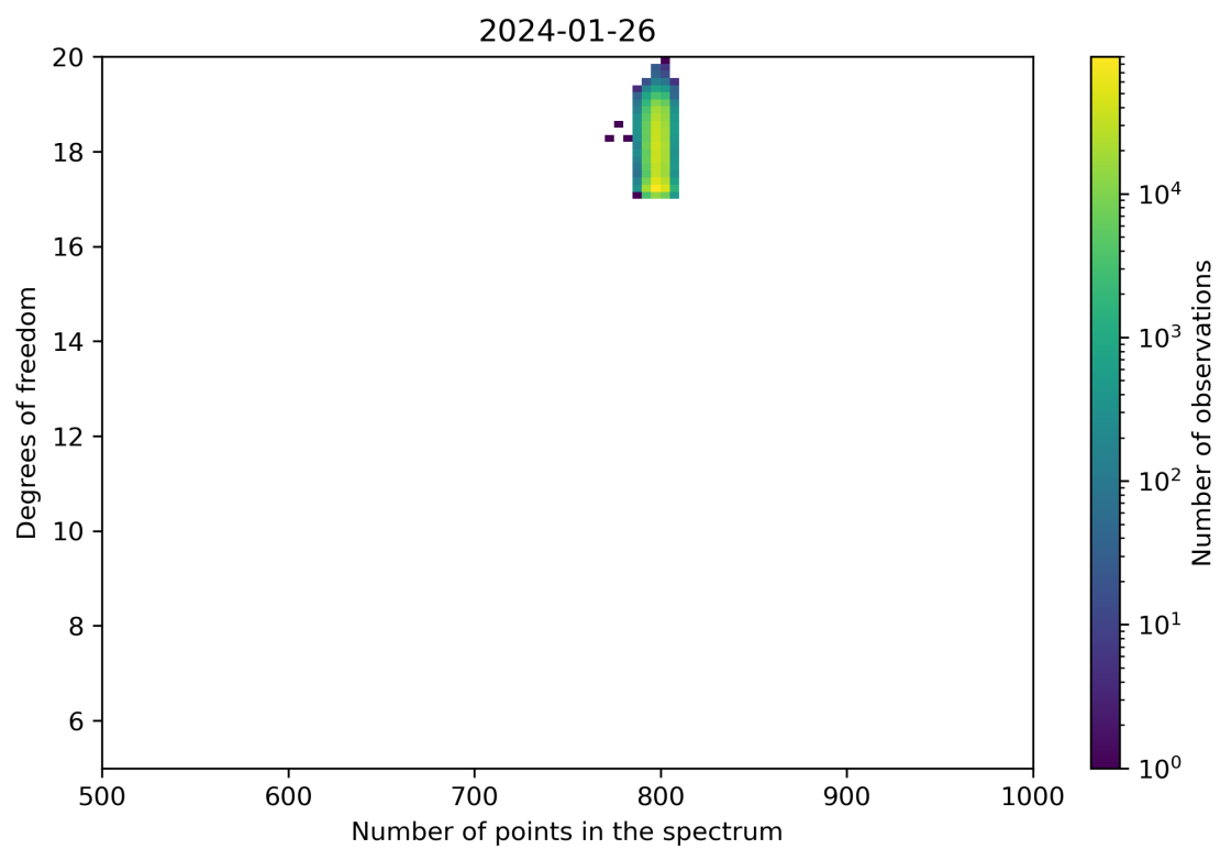
Figure 90: Scatter density plot of “Number of points in the spectrum” against “Degrees of freedom” for 2024-01-26 to 2024-01-27.
