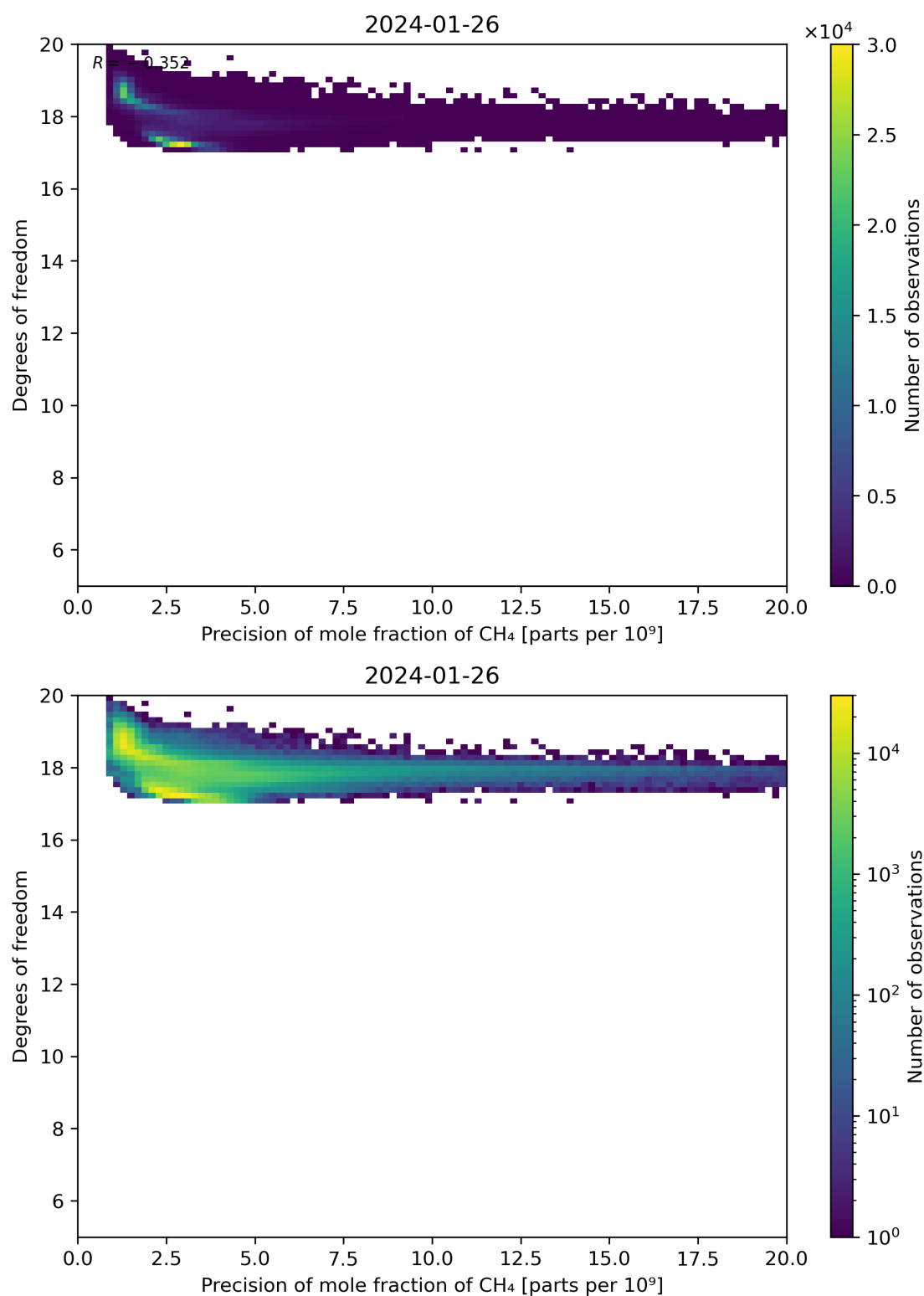
Figure 80: Scatter density plot of “Precision of mole fraction of CH 4 ” against “Degrees of freedom” for 2024-01-26 to 2024-01-27.
