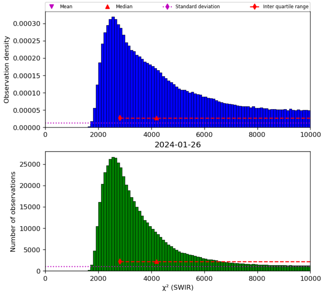
Figure 28: Histogram of “ \chi^2 (SWIR)” for 2024-01-26 to 2024-01-27
