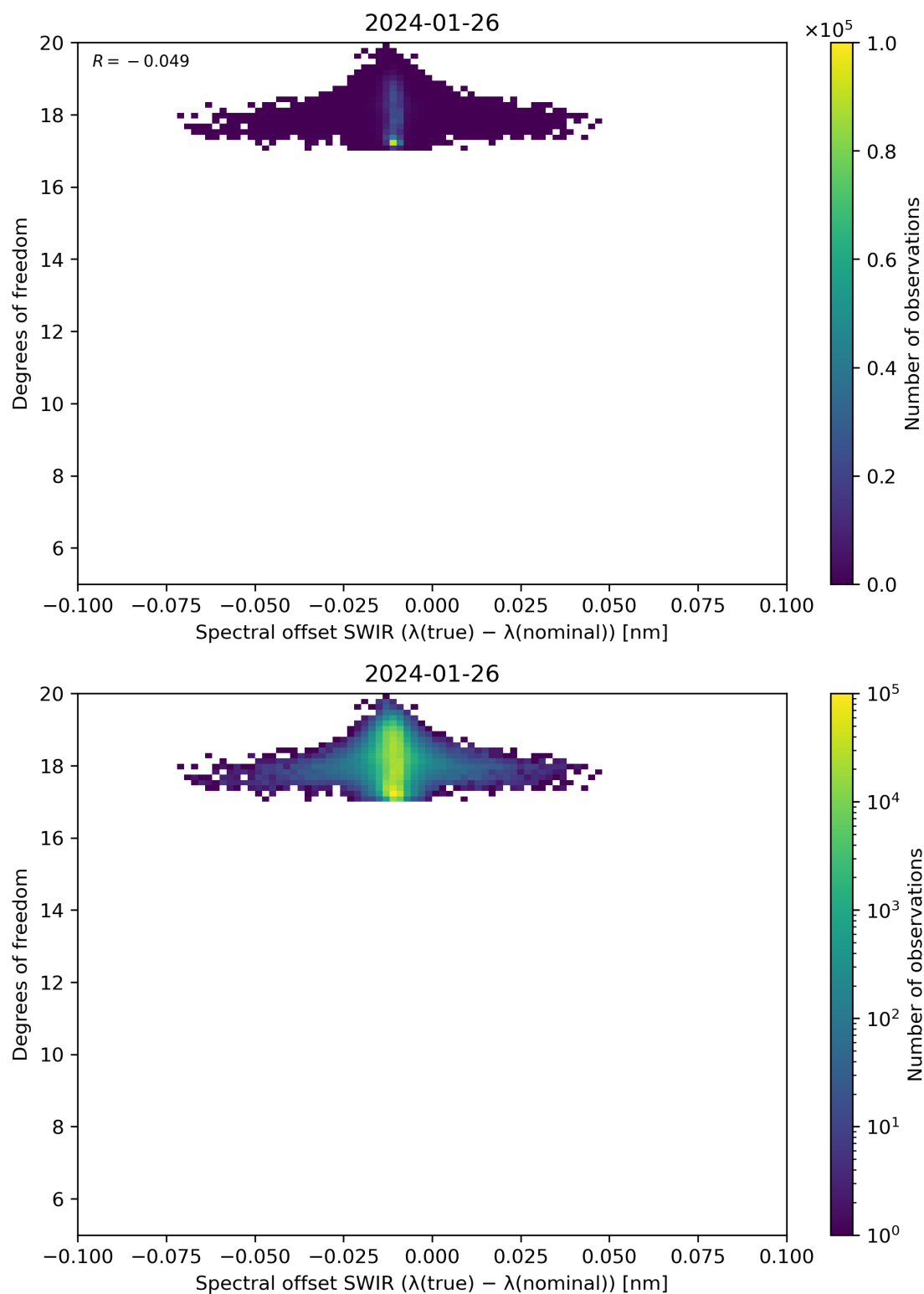
Figure 119: Scatter density plot of “Spectral offset SWIR ( \lambda(\text{true}) - \lambda(\text{nominal}) )” against “Degrees of freedom” for 2024-01-26 to 2024-01-27.
