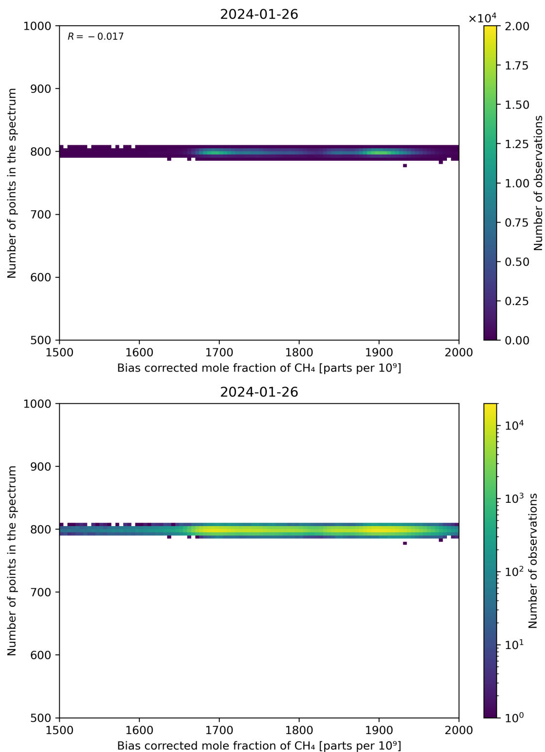
Figure 68: Scatter density plot of “Bias corrected mole fraction of CH 4 ” against “Number of points in the spectrum” for 2024-01-26 to 2024-01-27.
