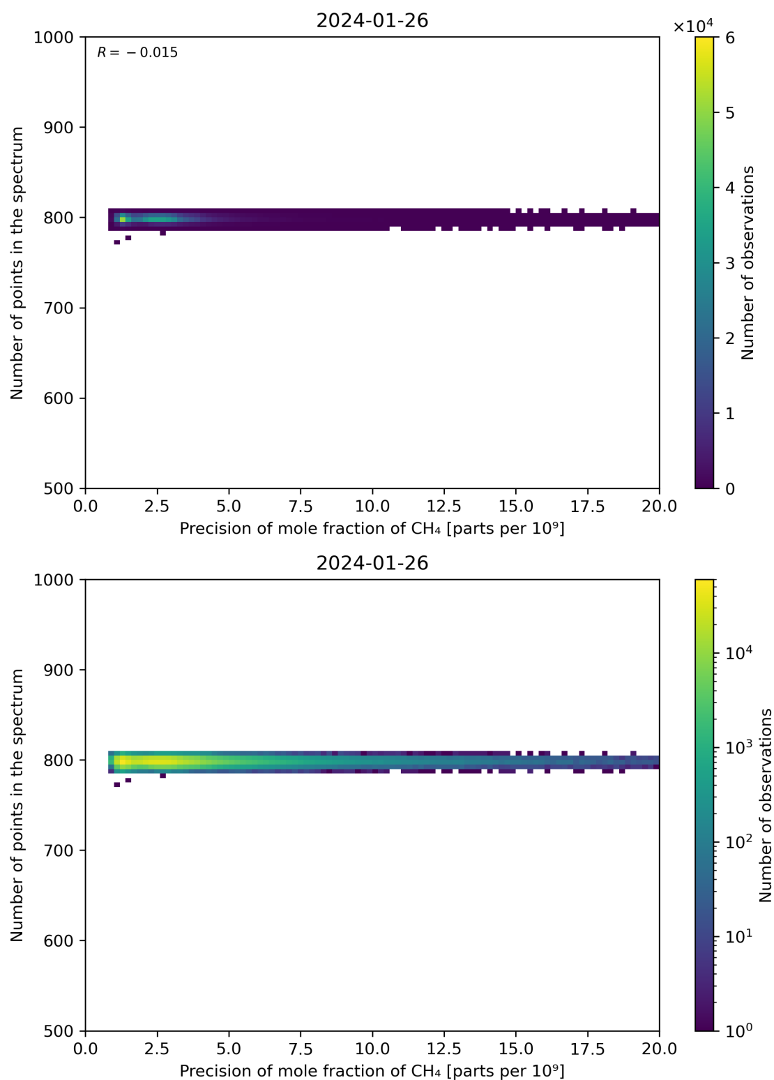
Figure 84: Scatter density plot of “Precision of mole fraction of CH 4 ” against “Number of points in the spectrum” for 2024-01-26 to 2024-01-27.
