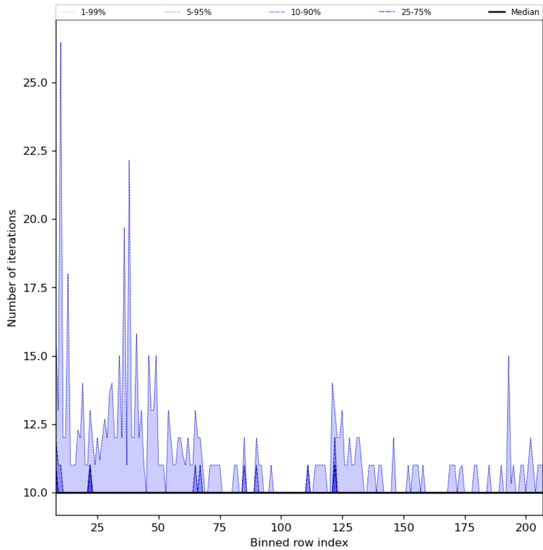
Figure 42: Along track statistics of “Number of iterations” for 2024-01-26 to 2024-01-27
