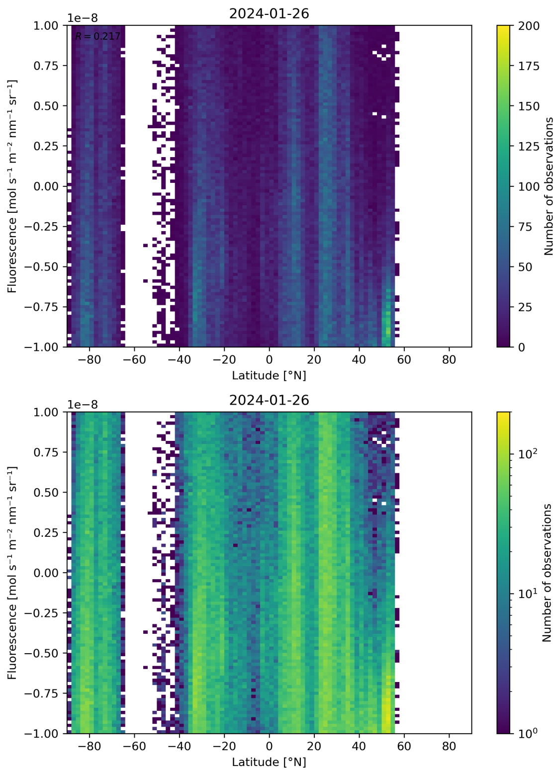
Figure 56: Scatter density plot of “Latitude” against “Fluorescence” for 2024-01-26 to 2024-01-27.
