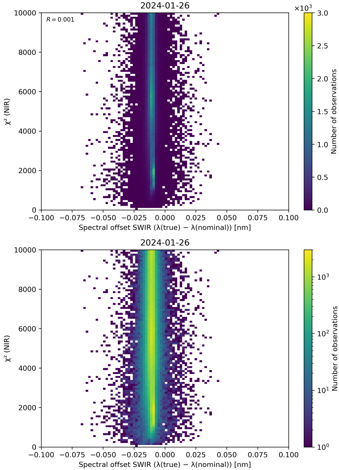
Figure 117: Scatter density plot of “Spectral offset SWIR ( \lambda(\text{true}) - \lambda(\text{nominal}) )” against “ \chi^2 (NIR)” for 2024-01-26 to 2024-01-27.
