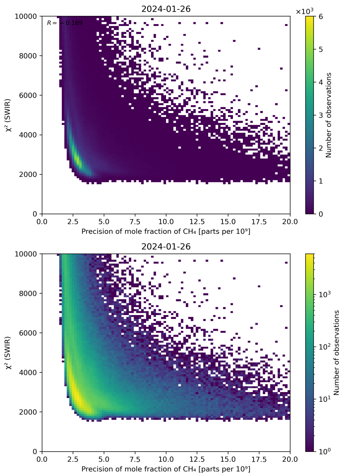
Figure 79: Scatter density plot of “Precision of mole fraction of \text{CH}_4 ” against “ \chi^2 (SWIR)” for 2024-01-26 to 2024-01-27.
