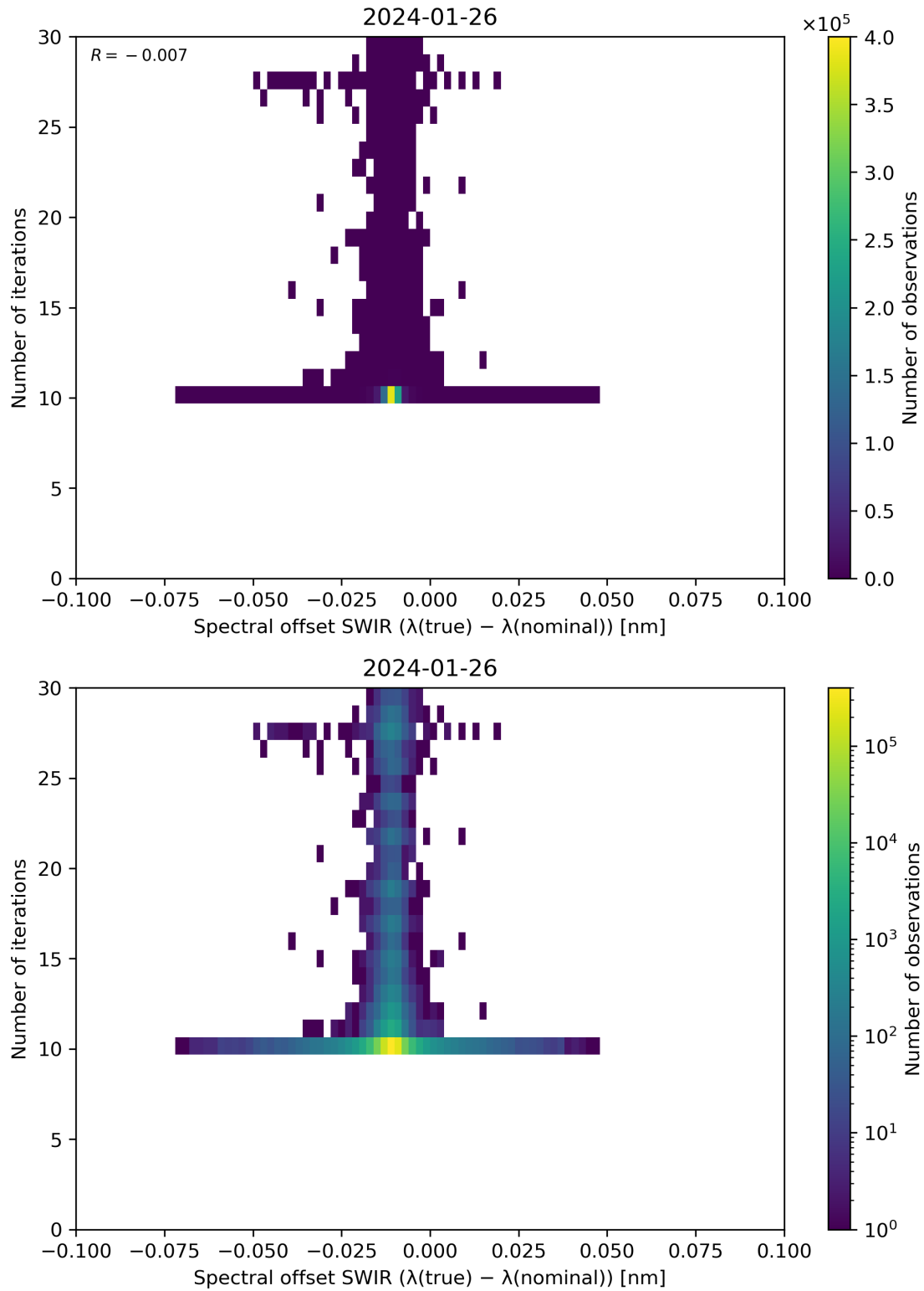
Figure 121: Scatter density plot of “Spectral offset SWIR ( \lambda(\text{true}) - \lambda(\text{nominal}) )” against “Number of iterations” for 2024-01-26 to 2024-01-27.
