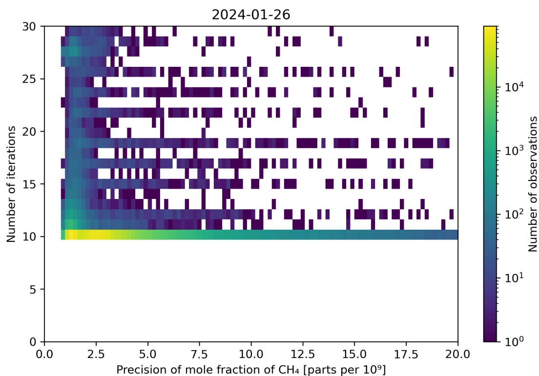
Figure 83: Scatter density plot of “Precision of mole fraction of CH 4 ” against “Number of iterations” for 2024-01-26 to 2024-01-27.
