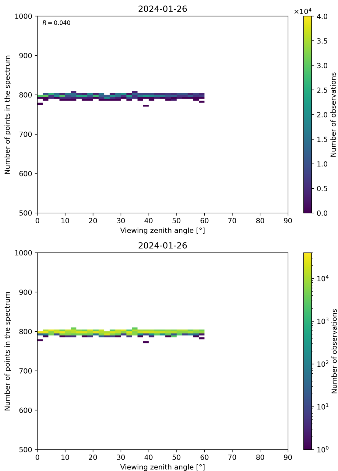
Figure 114: Scatter density plot of “Viewing zenith angle” against “Number of points in the spectrum” for 2024-01-26 to 2024-01-27.
