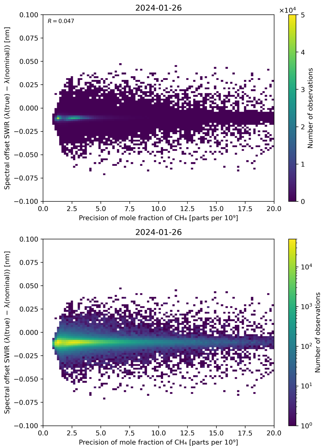
Figure 85: Scatter density plot of “Precision of mole fraction of CH 4 ” against “Spectral offset SWIR ( \lambda(\text{true}) - \lambda(\text{nominal}) )” for 2024-01-26 to 2024-01-27.
