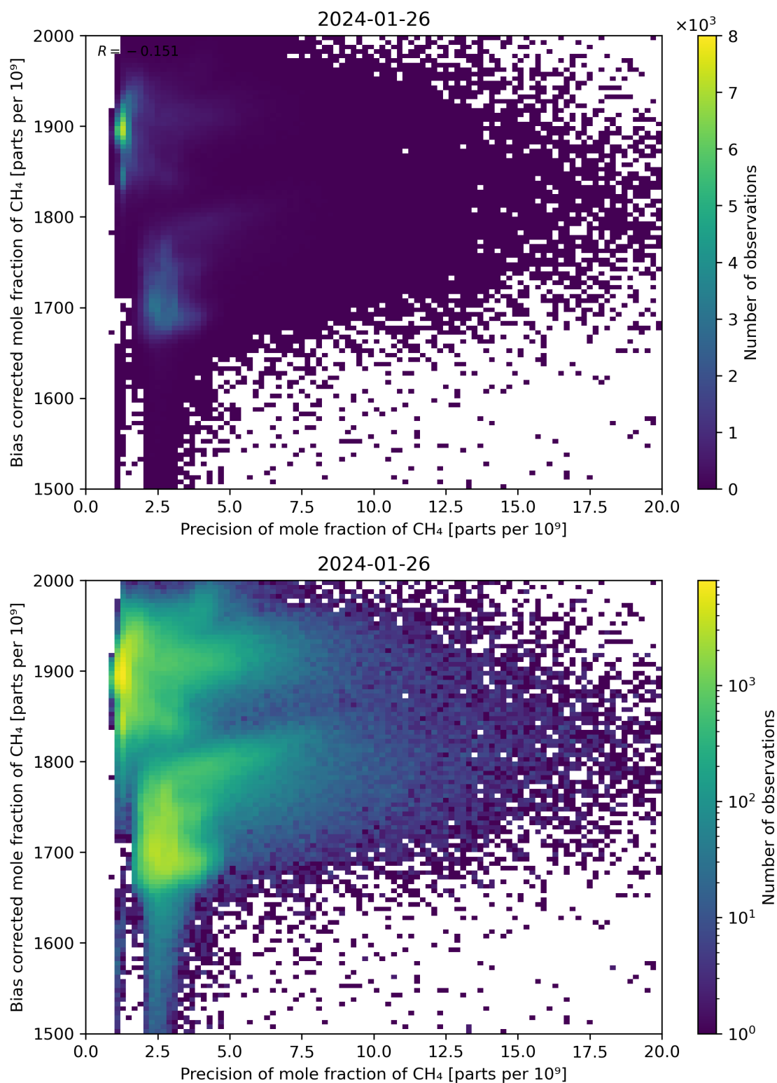
Figure 82: Scatter density plot of “Precision of mole fraction of CH 4 ” against “Bias corrected mole fraction of CH 4 ” for 2024-01-26 to 2024-01-27.
