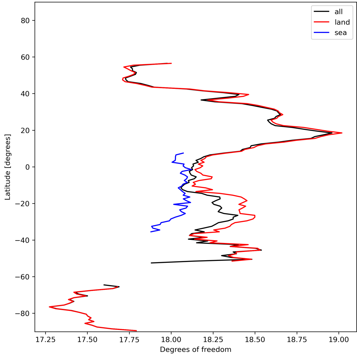
Figure 19: Zonal average of “Degrees of freedom” for 2024-01-26 to 2024-01-27.
