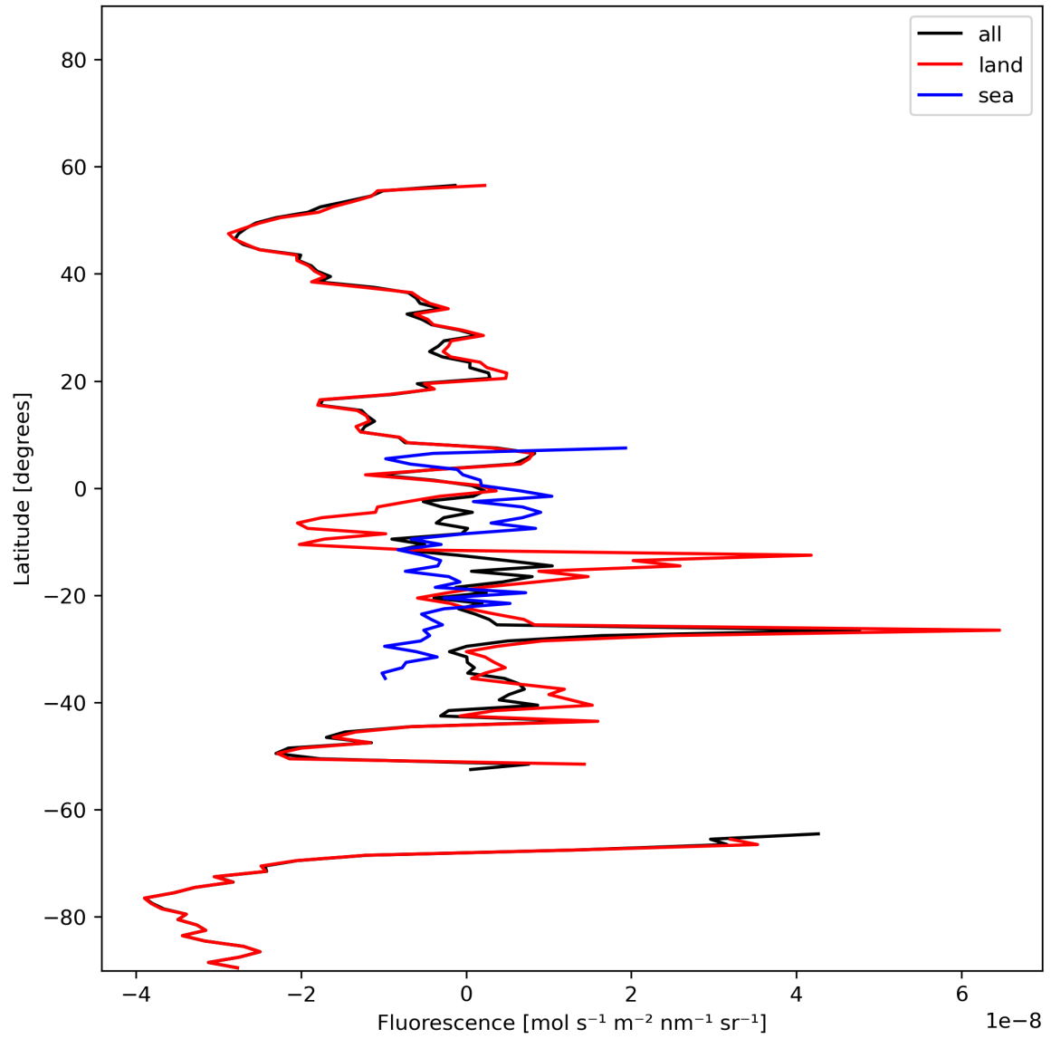
Figure 21: Zonal average of “Fluorescence” for 2024-01-26 to 2024-01-27.
