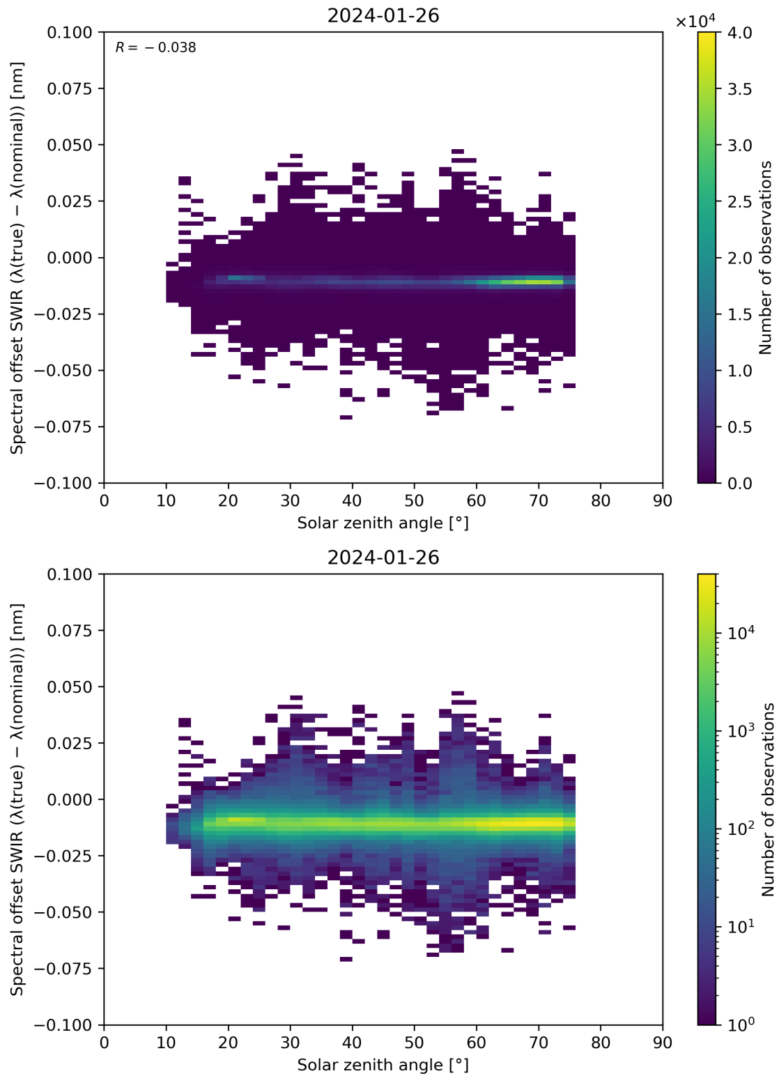
Figure 104: Scatter density plot of “Solar zenith angle” against “Spectral offset SWIR ( \lambda(\text{true}) - \lambda(\text{nominal}) )” for 2024-01-26 to 2024-01-27.
