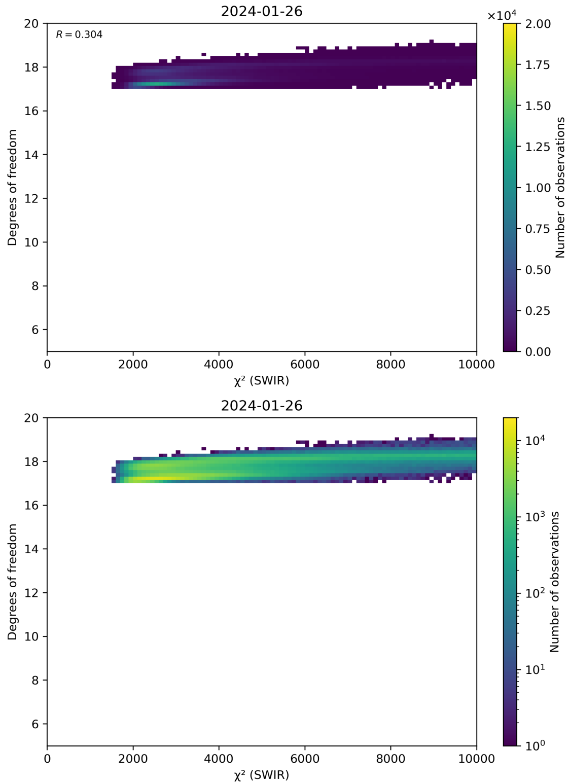
Figure 48: Scatter density plot of “ \chi^2 (SWIR)” against “Degrees of freedom” for 2024-01-26 to 2024-01-27.
