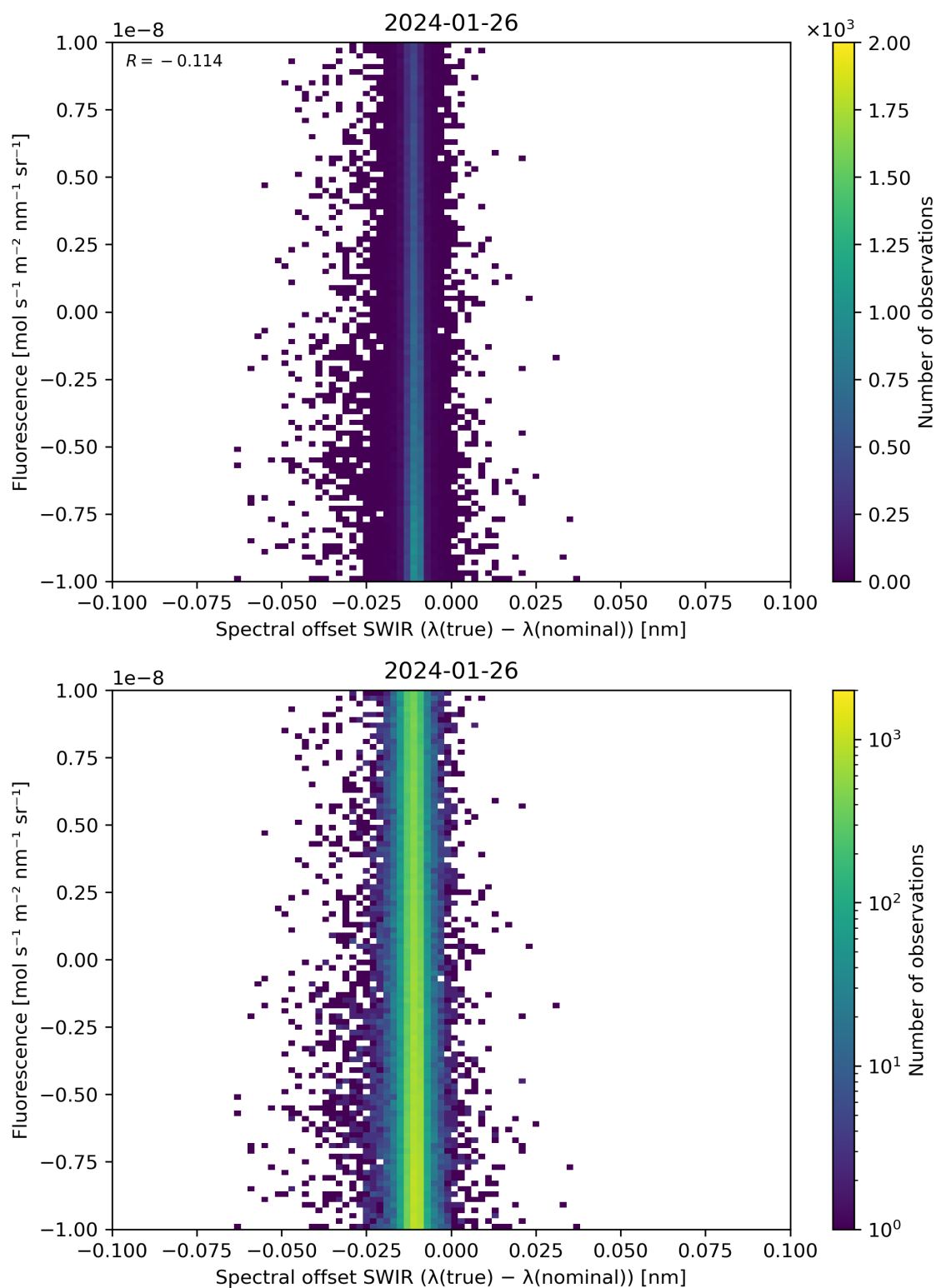
Figure 120: Scatter density plot of “Spectral offset SWIR ( \lambda(\text{true}) - \lambda(\text{nominal}) )” against “Fluorescence” for 2024-01-26 to 2024-01-27.
