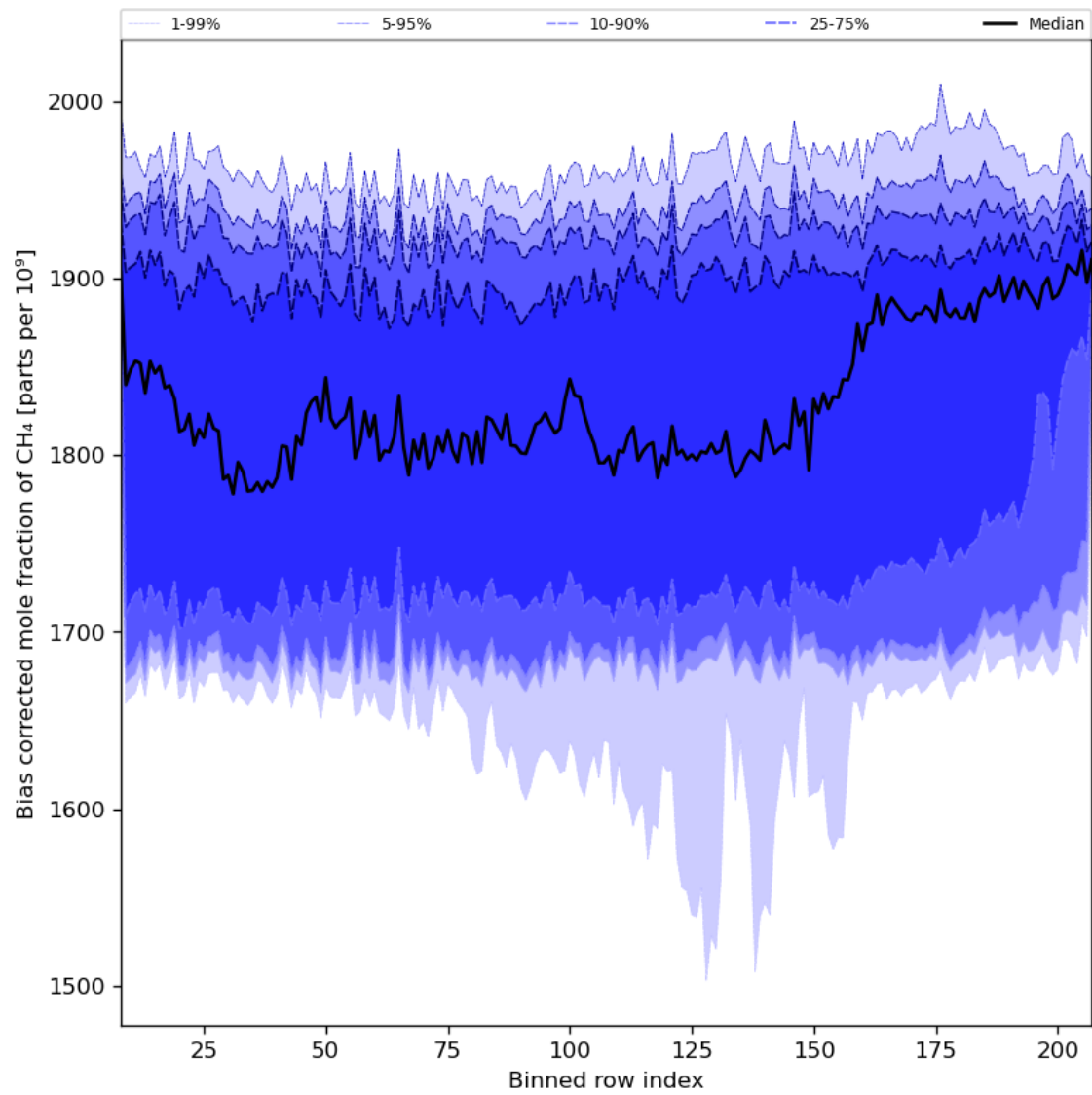
Figure 36: Along track statistics of “Bias corrected mole fraction of CH 4 ” for 2024-01-26 to 2024-01-27
