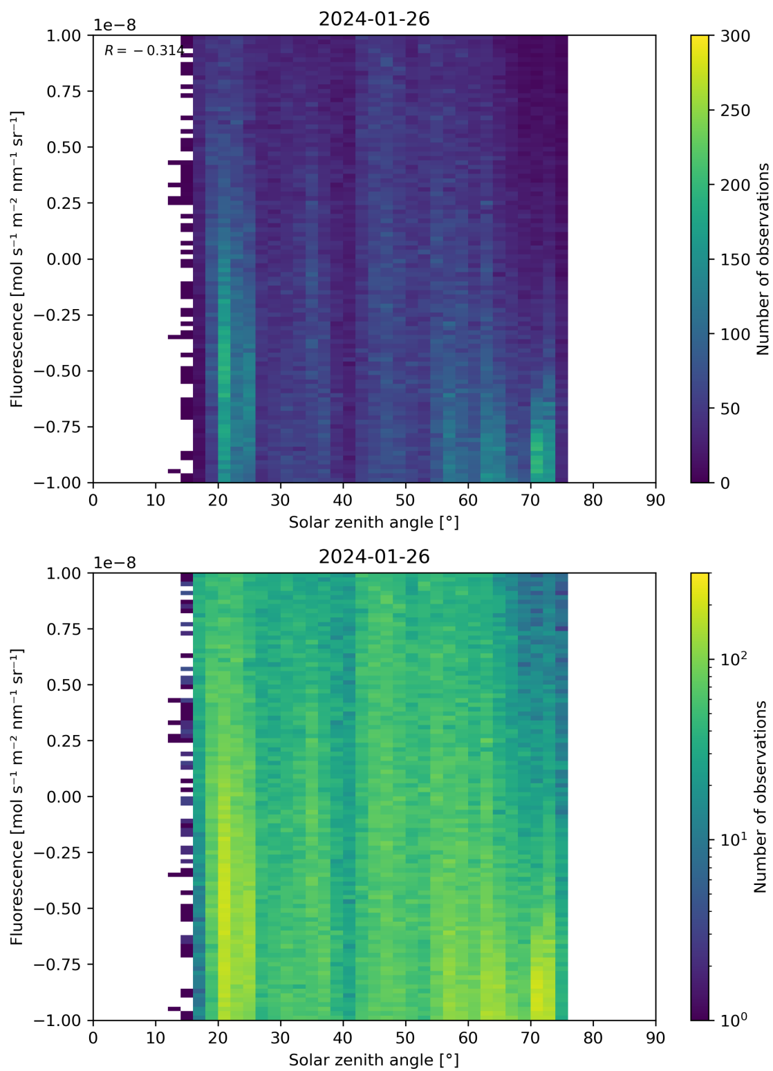
Figure 97: Scatter density plot of “Solar zenith angle” against “Fluorescence” for 2024-01-26 to 2024-01-27.
