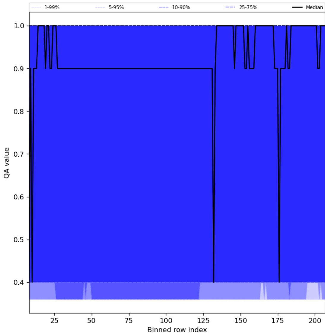
Figure 33: Along track statistics of “QA value” for 2024-01-26 to 2024-01-27
