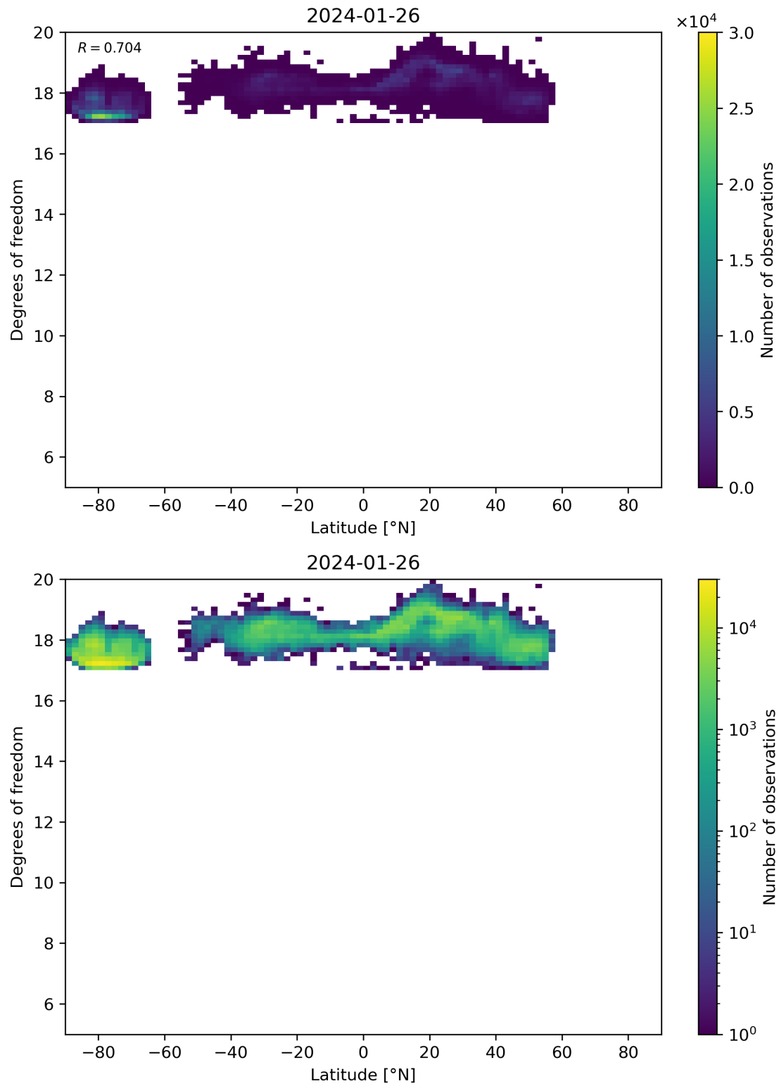
Figure 55: Scatter density plot of “Latitude” against “Degrees of freedom” for 2024-01-26 to 2024-01-27.
