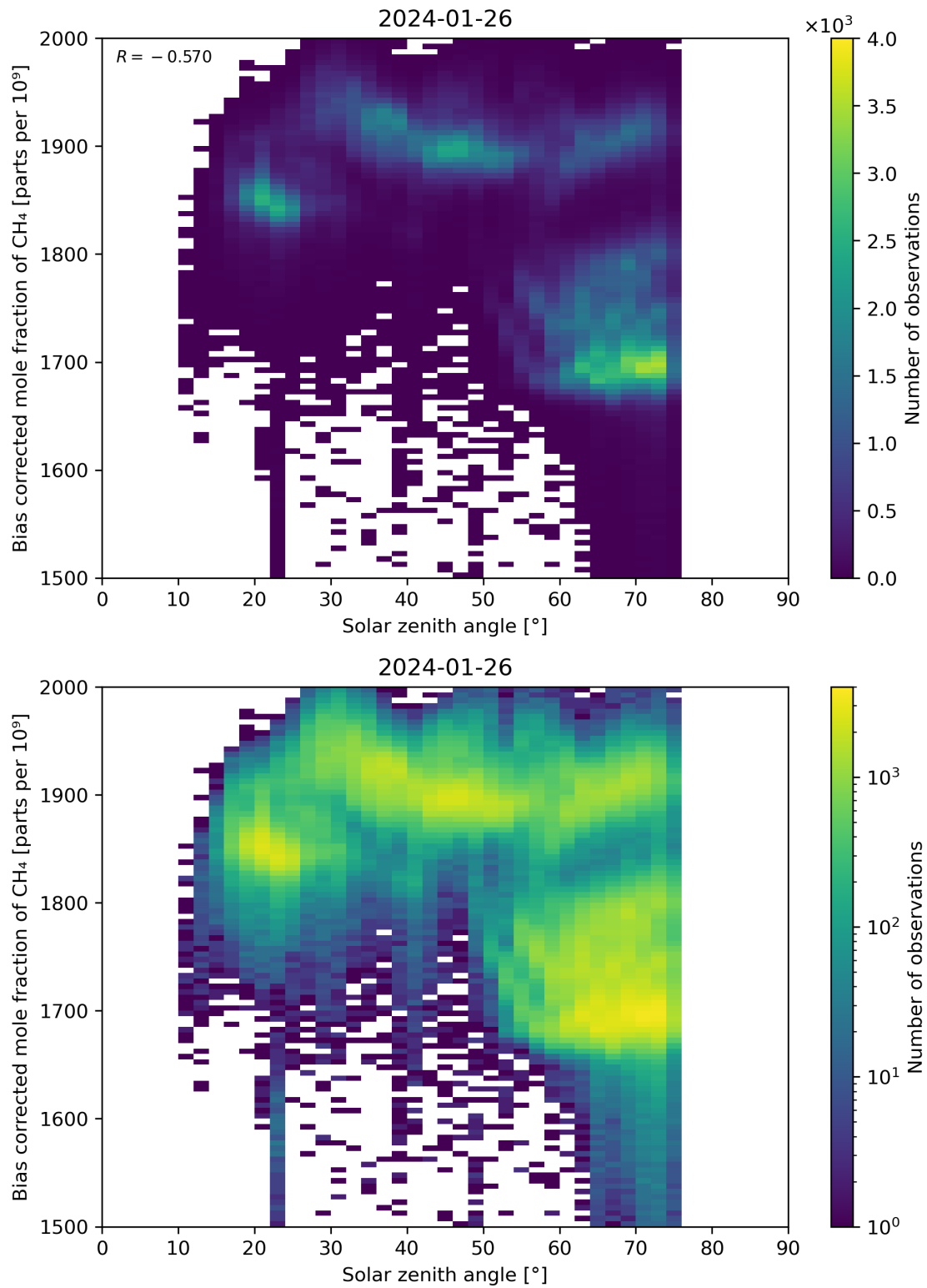
Figure 100: Scatter density plot of “Solar zenith angle” against “Bias corrected mole fraction of \text{CH}_4 ” for 2024-01-26 to 2024-01-27.
