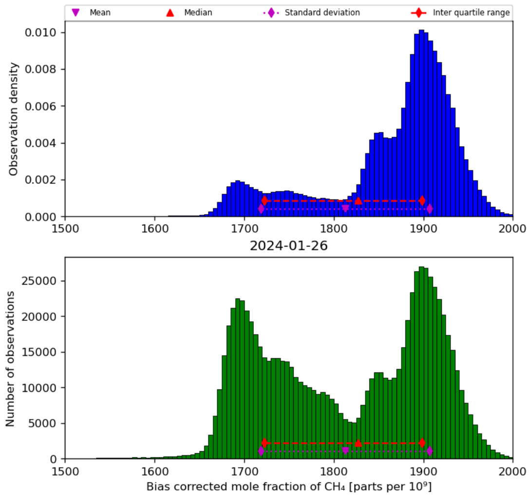
Figure 25: Histogram of “Bias corrected mole fraction of CH 4 ” for 2024-01-26 to 2024-01-27
