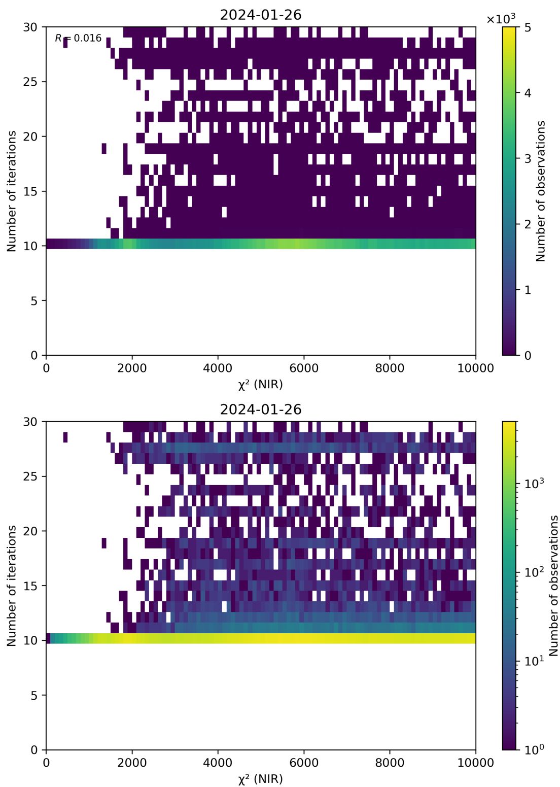
Figure 46: Scatter density plot of “ \chi^2 (NIR)” against “Number of iterations” for 2024-01-26 to 2024-01-27.
