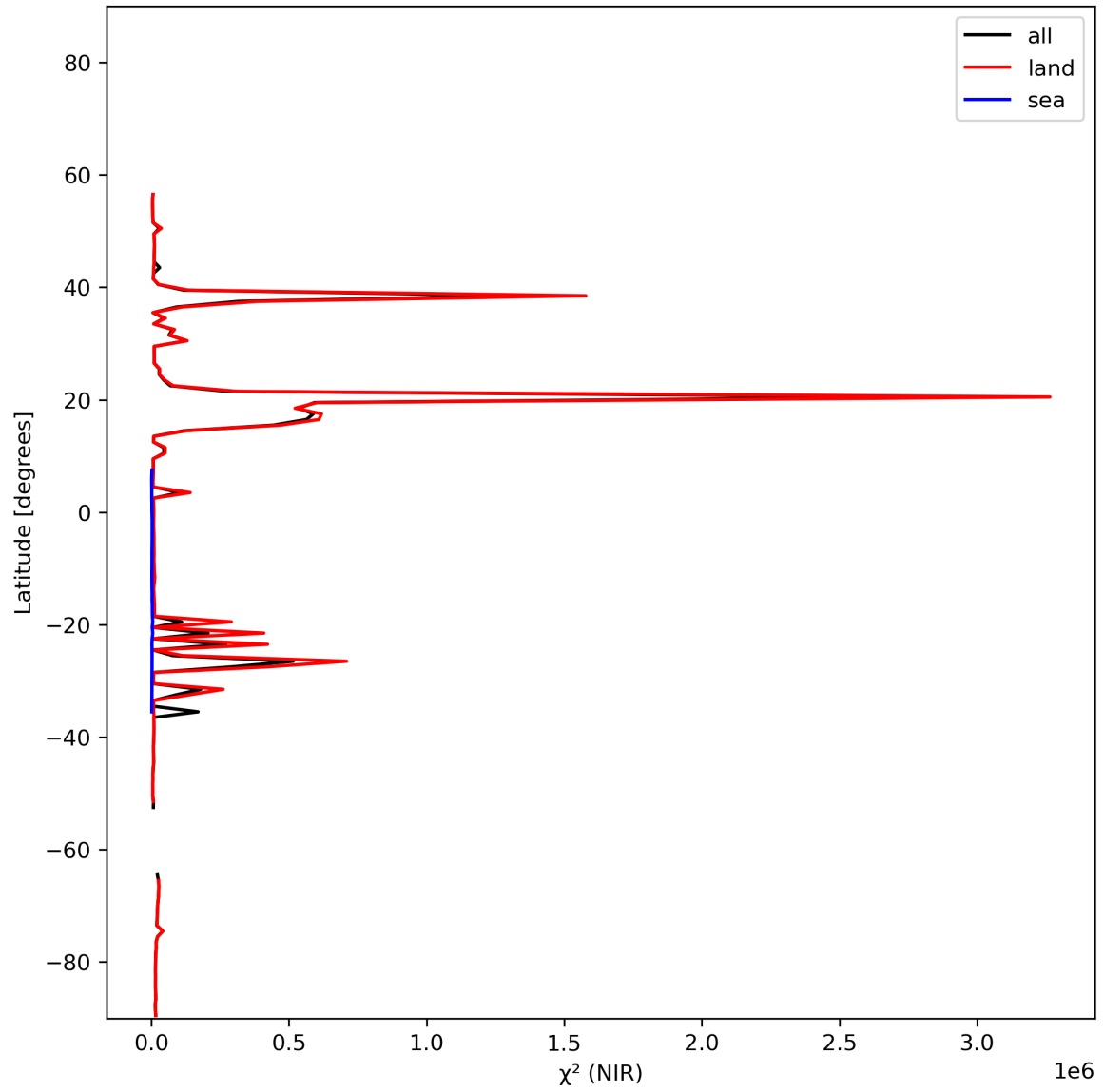
Figure 18: Zonal average of “ \chi^2 (NIR)” for 2024-01-26 to 2024-01-27.
