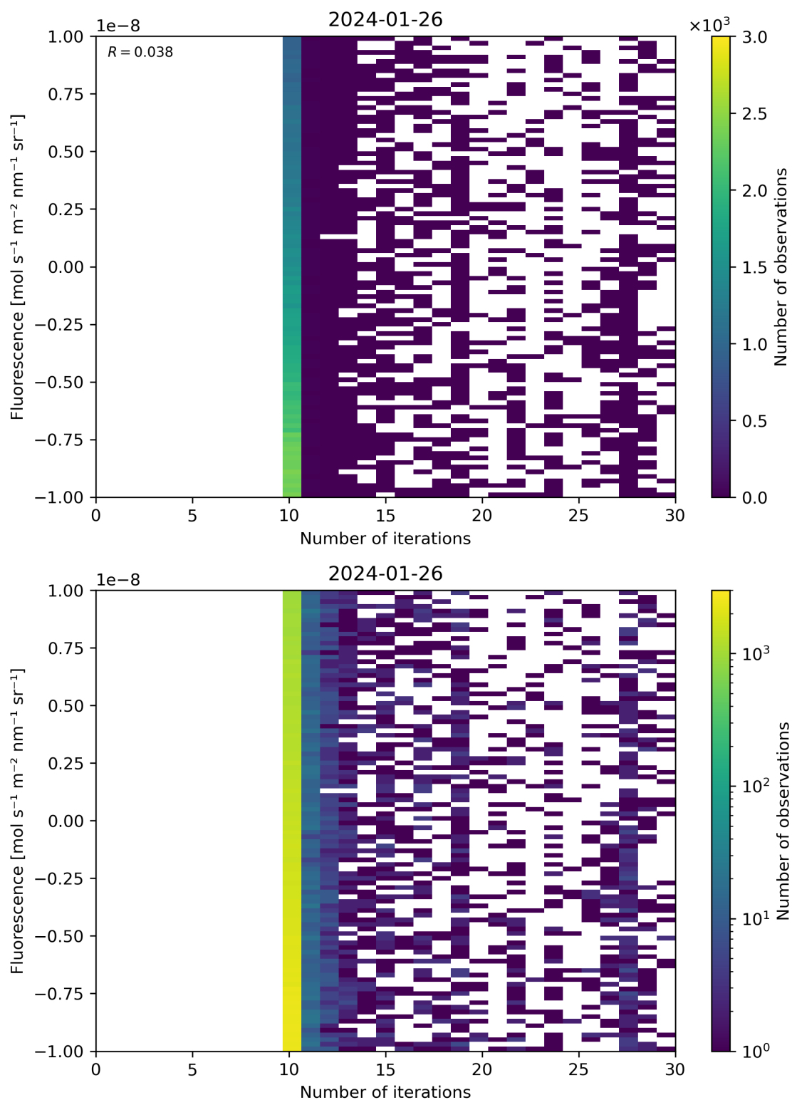
Figure 87: Scatter density plot of “Number of iterations” against “Fluorescence” for 2024-01-26 to 2024-01-27.
