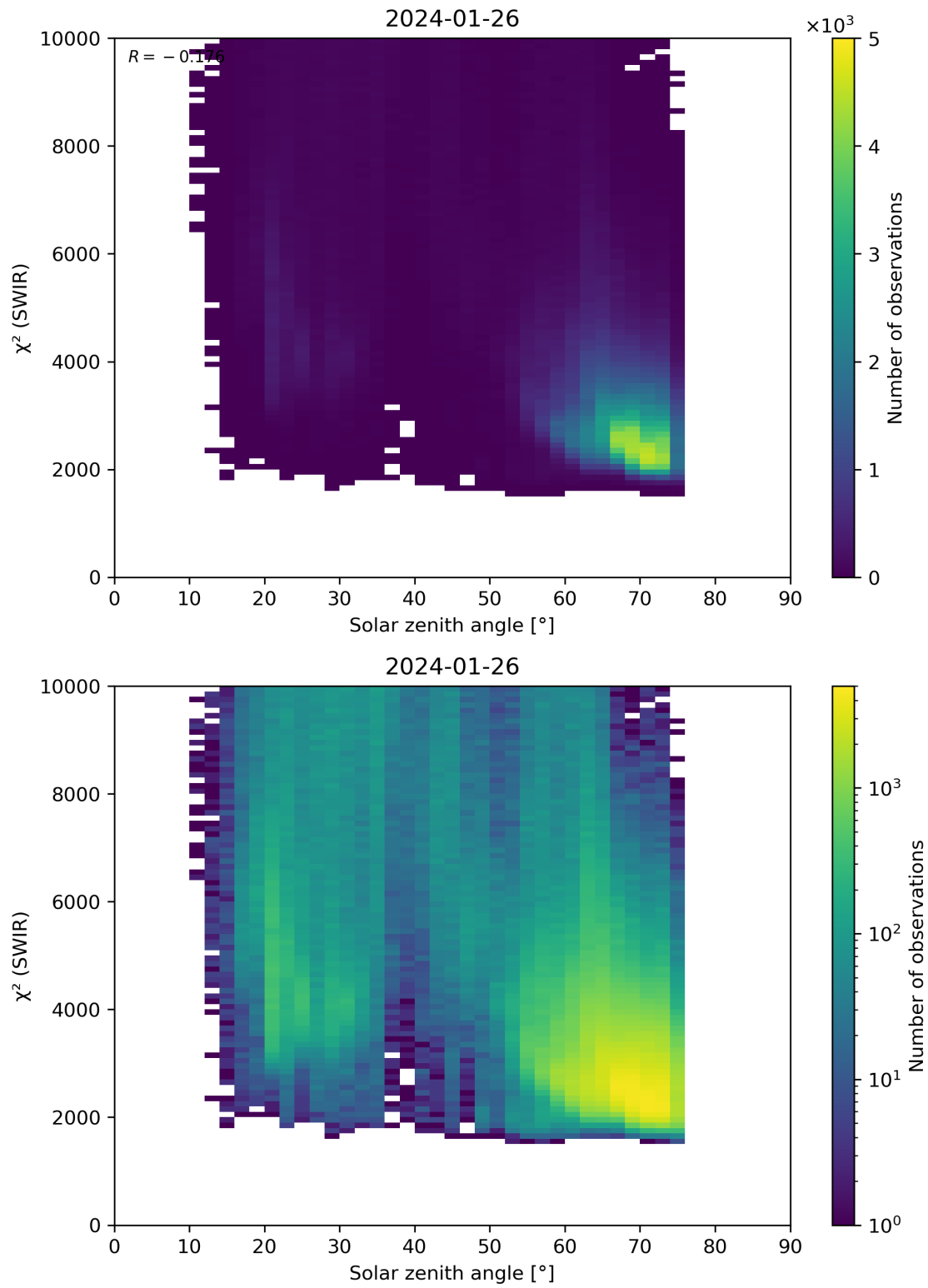
Figure 95: Scatter density plot of “Solar zenith angle” against “ \chi^2 (SWIR)” for 2024-01-26 to 2024-01-27.
