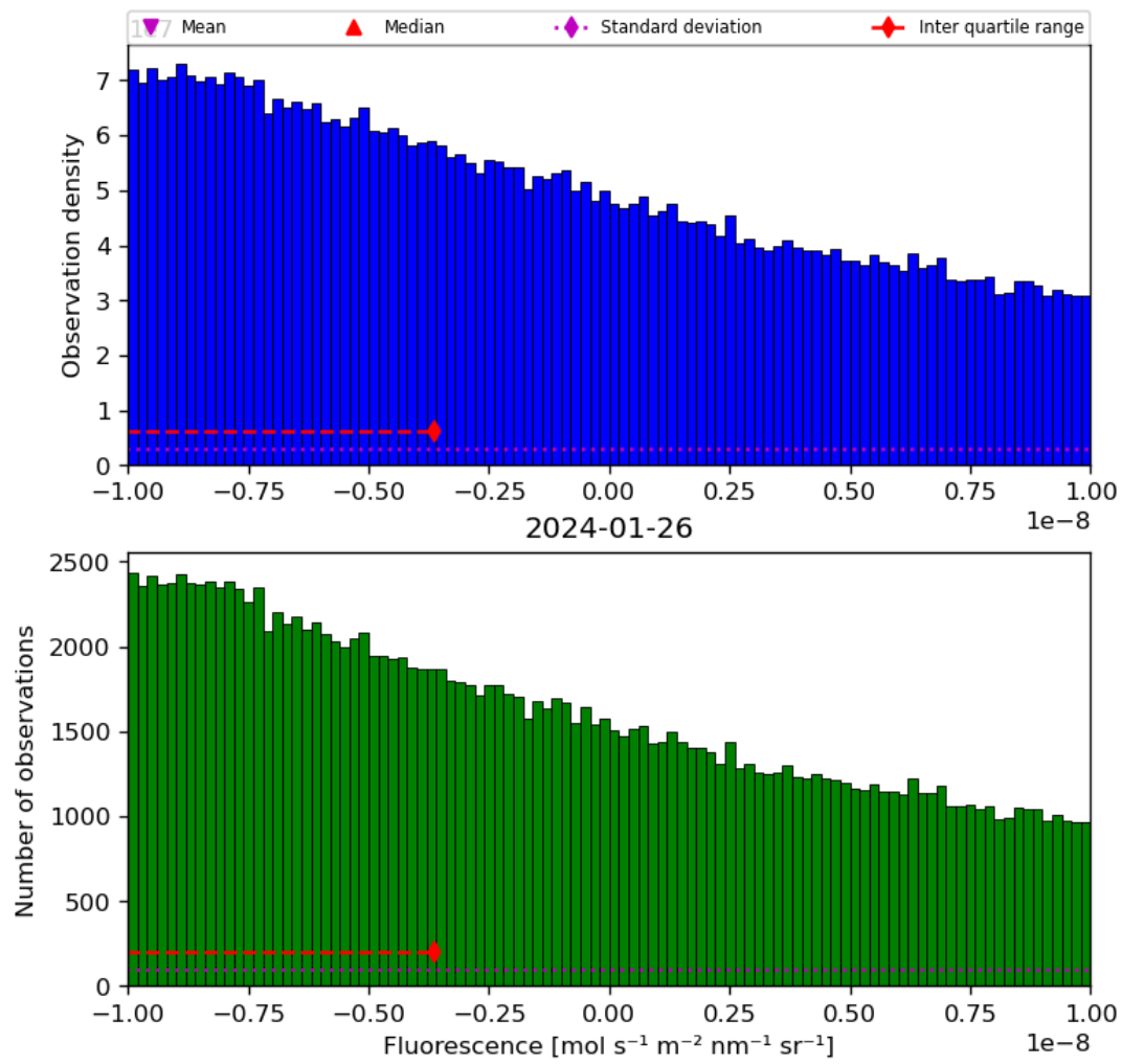
Figure 32: Histogram of “Fluorescence” for 2024-01-26 to 2024-01-27
