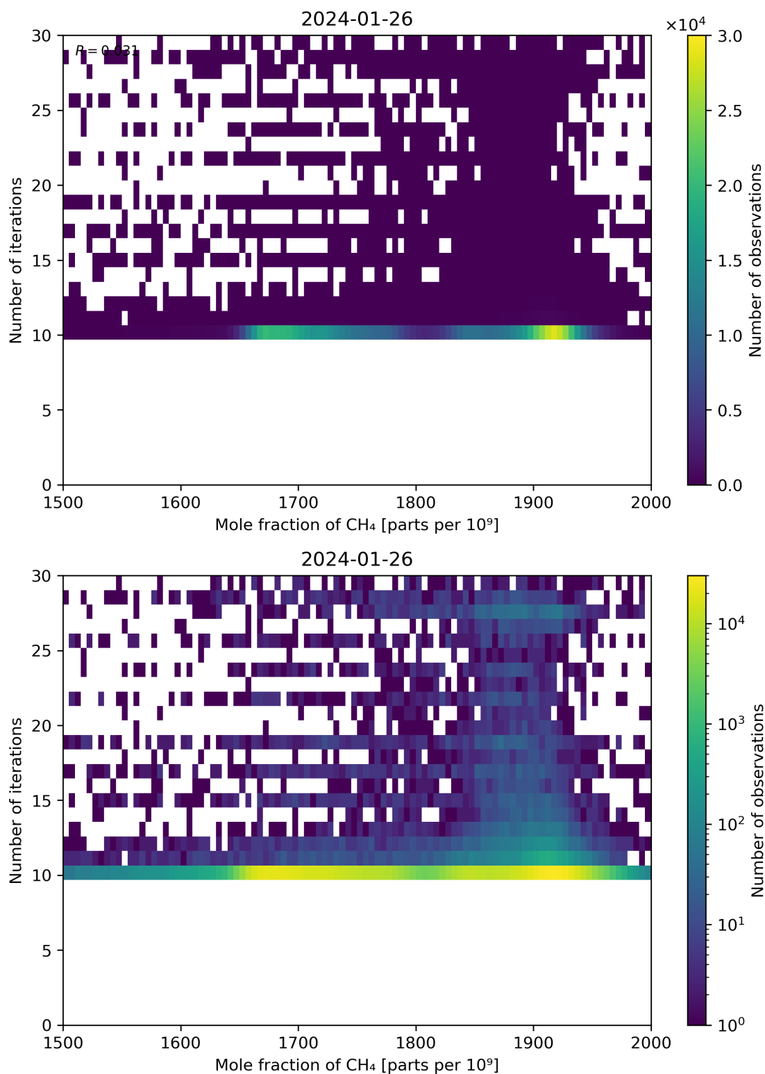
Figure 76: Scatter density plot of “Mole fraction of CH 4 ” against “Number of iterations” for 2024-01-26 to 2024-01-27.
