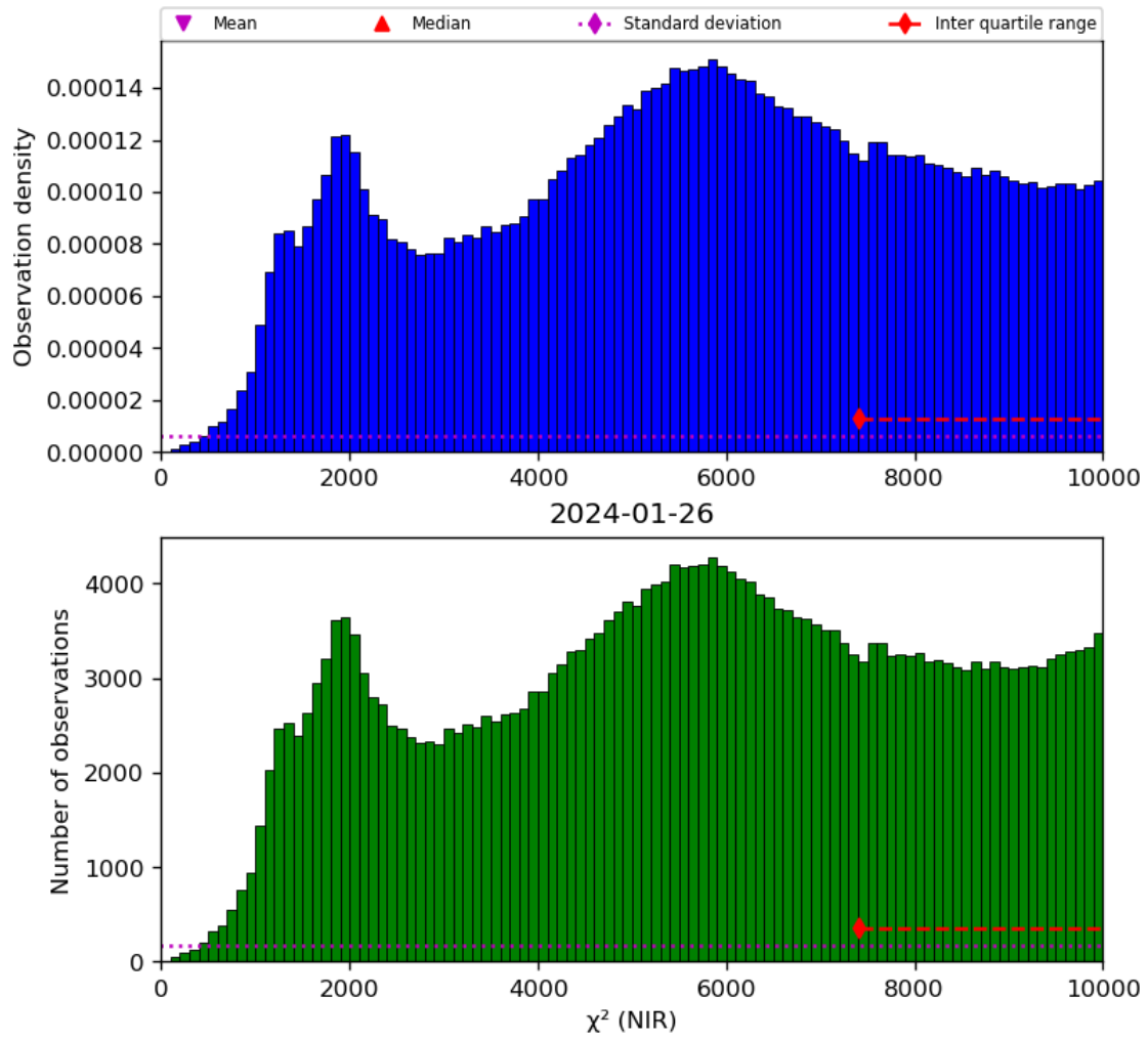
Figure 29: Histogram of “ \chi^2 (NIR)” for 2024-01-26 to 2024-01-27
