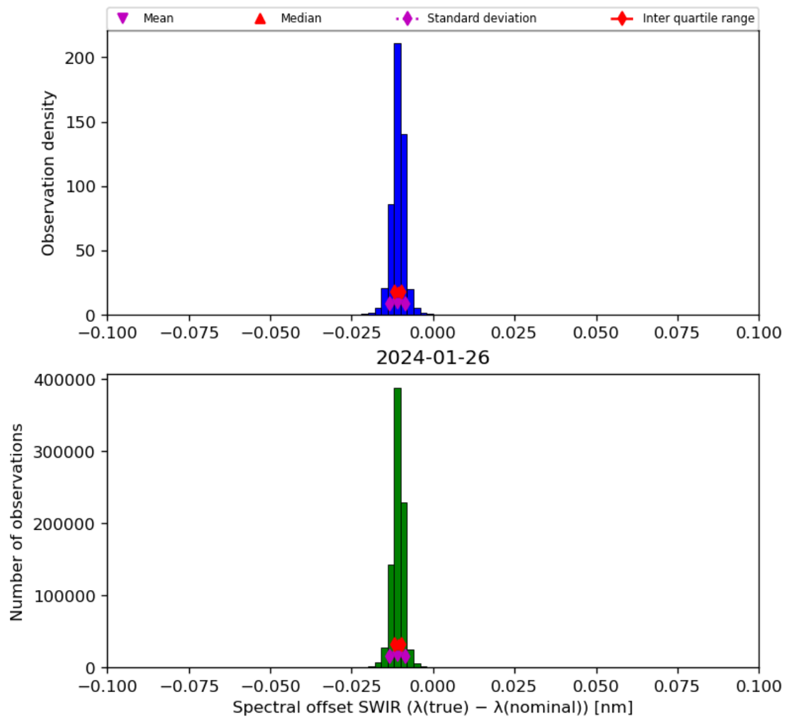
Figure 27: Histogram of “Spectral offset SWIR ( \lambda(\text{true}) - \lambda(\text{nominal}) )” for 2024-01-26 to 2024-01-27
