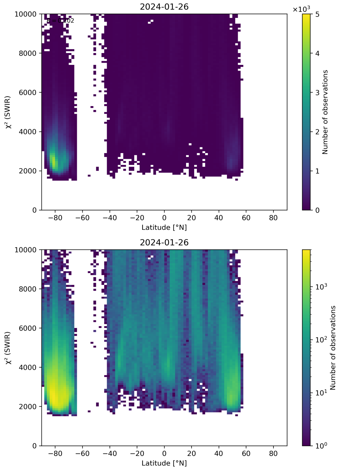
Figure 54: Scatter density plot of “Latitude” against “ \chi^2 (SWIR)” for 2024-01-26 to 2024-01-27.
