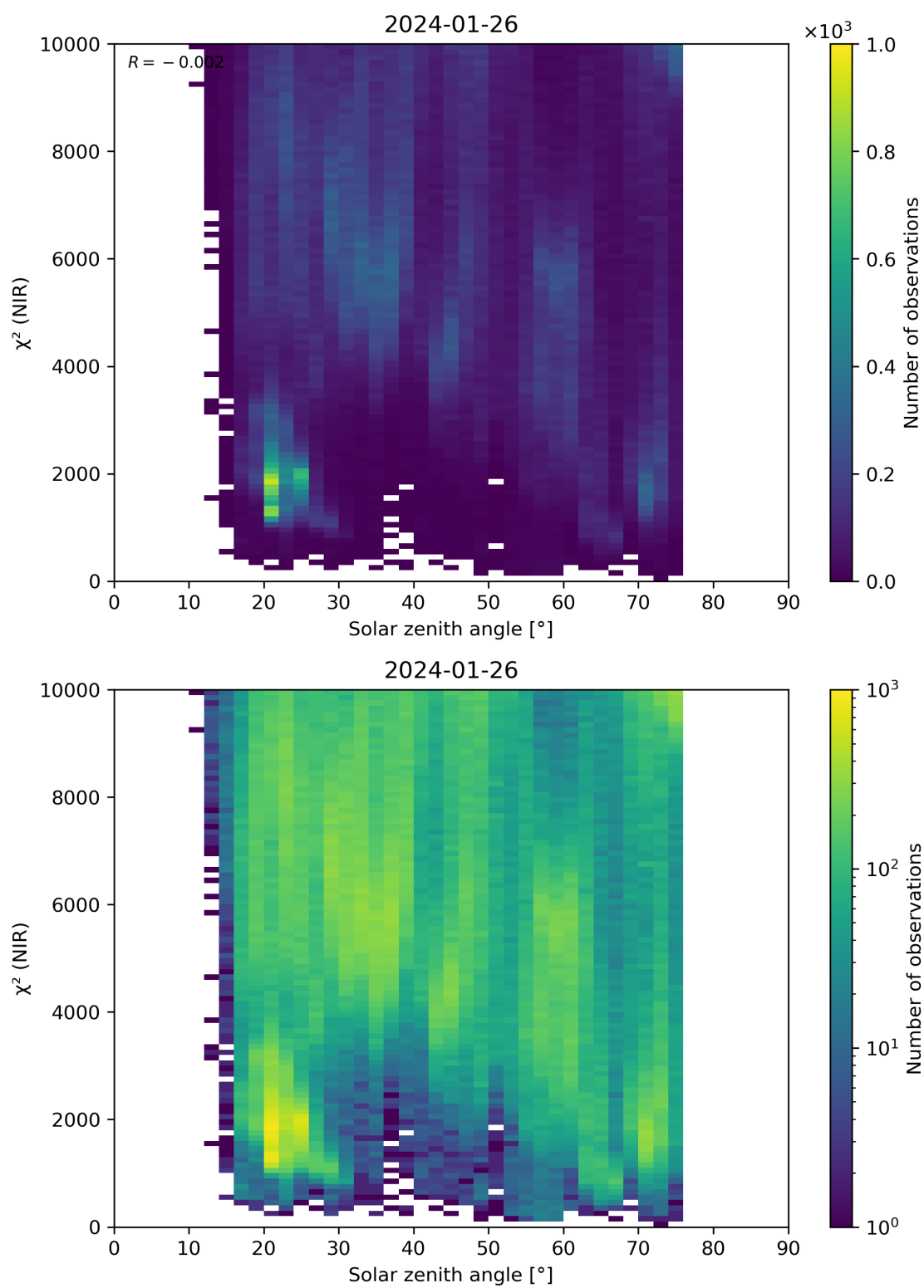
Figure 94: Scatter density plot of “Solar zenith angle” against “ \chi^2 (NIR)” for 2024-01-26 to 2024-01-27.
