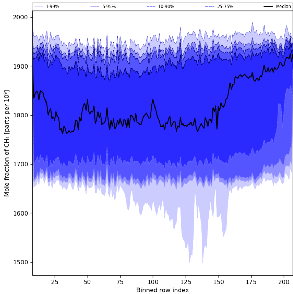
Figure 34: Along track statistics of “Mole fraction of CH 4 ” for 2024-01-26 to 2024-01-27
