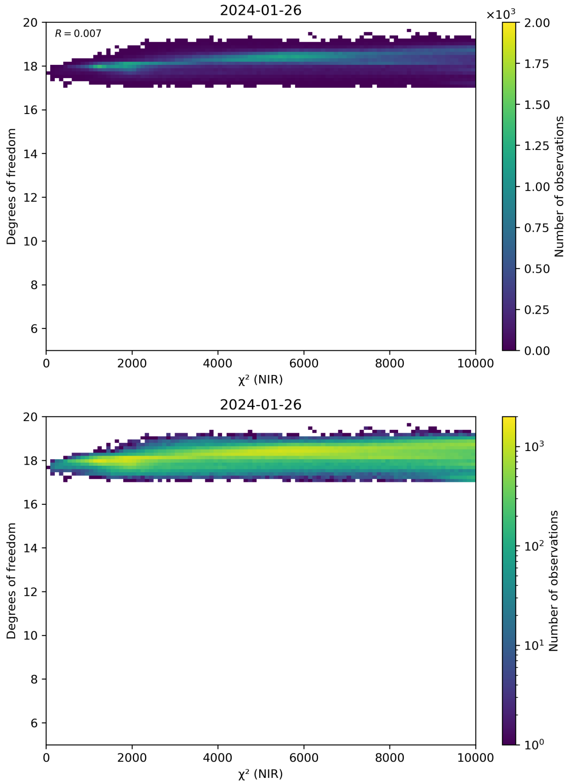
Figure 44: Scatter density plot of “ \chi^2 (NIR)” against “Degrees of freedom” for 2024-01-26 to 2024-01-27.
