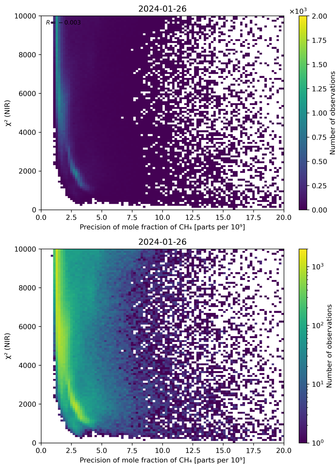
Figure 78: Scatter density plot of “Precision of mole fraction of CH 4 ” against “ \chi^2 (NIR)” for 2024-01-26 to 2024-01-27.
