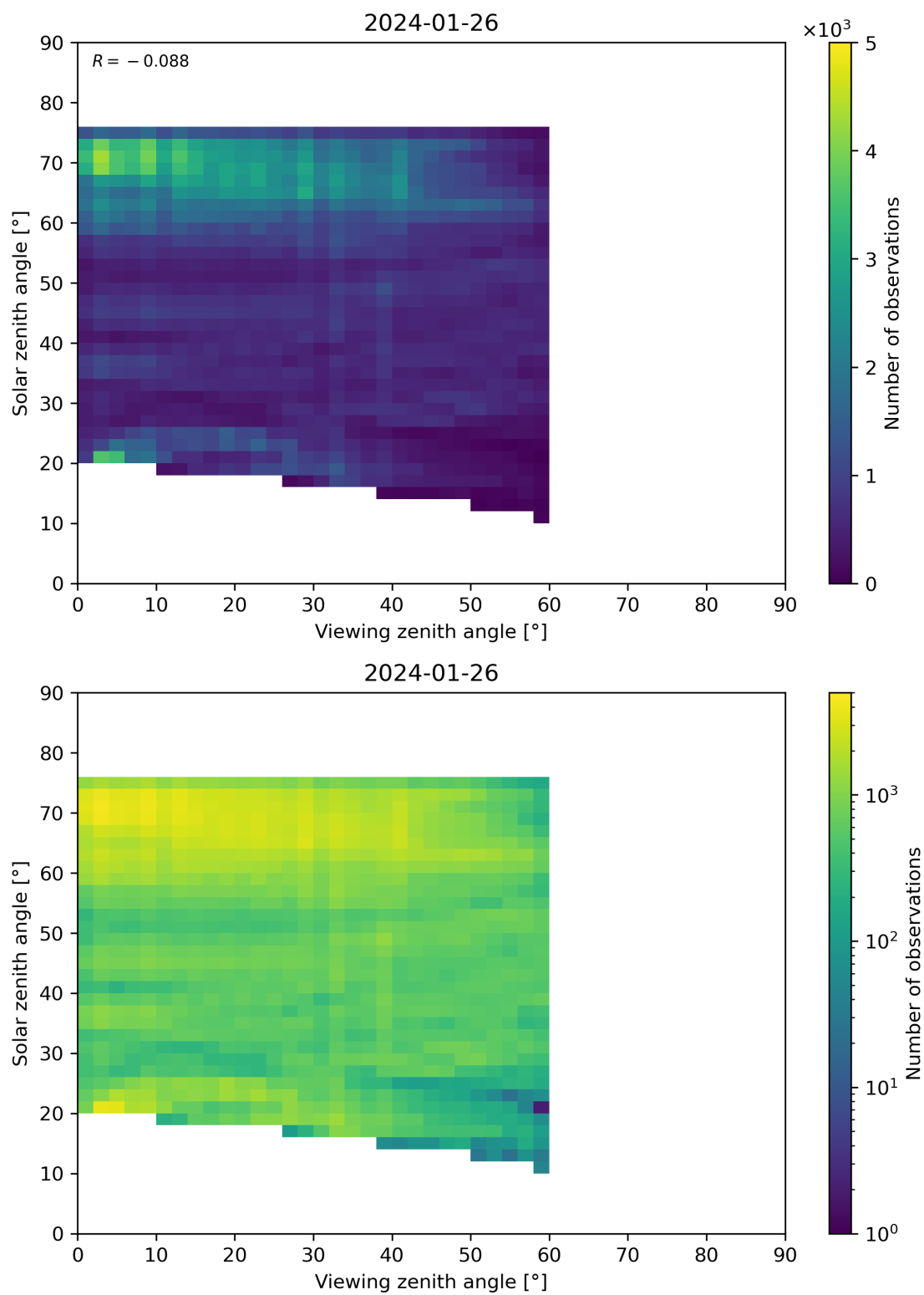
Figure 115: Scatter density plot of “Viewing zenith angle” against “Solar zenith angle” for 2024-01-26 to 2024-01-27.
