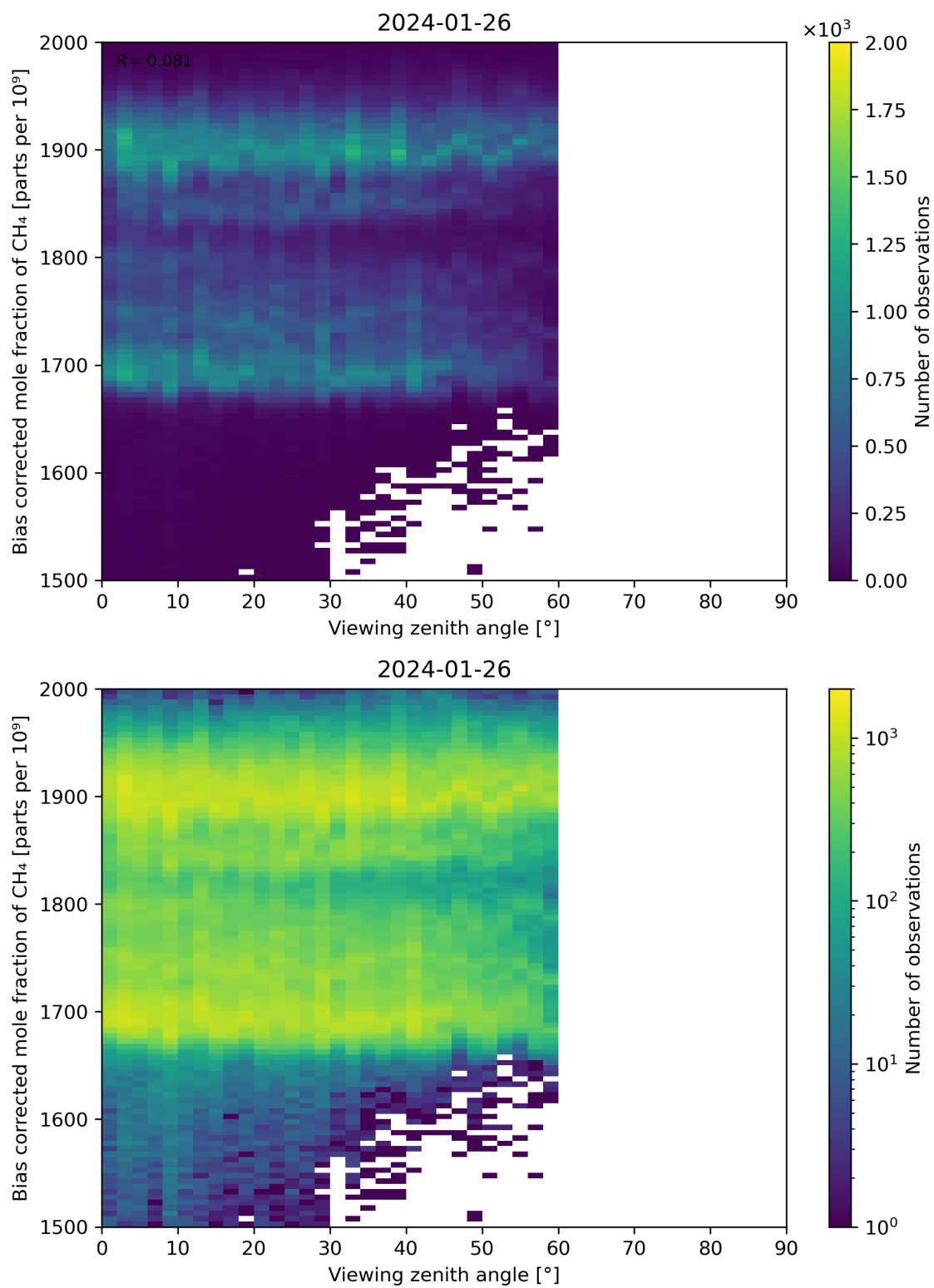
Figure 111: Scatter density plot of “Viewing zenith angle” against “Bias corrected mole fraction of CH 4 ” for 2024-01-26 to 2024-01-27.
