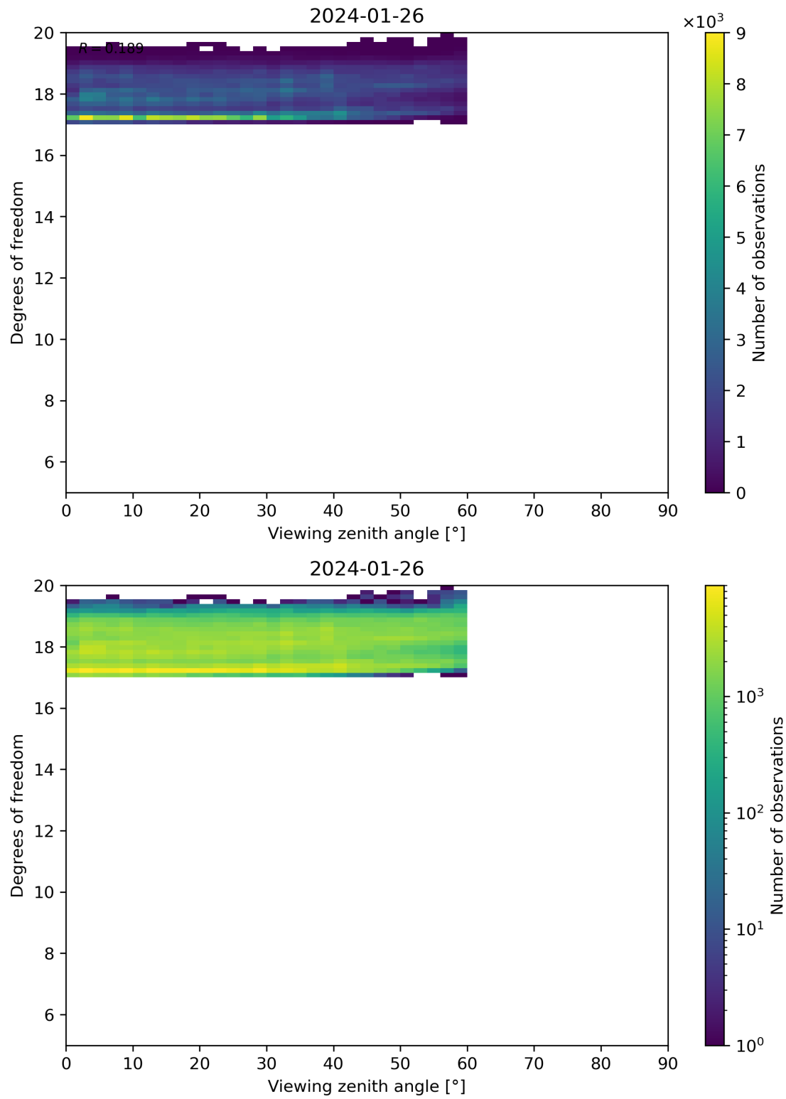
Figure 107: Scatter density plot of “Viewing zenith angle” against “Degrees of freedom” for 2024-01-26 to 2024-01-27.
