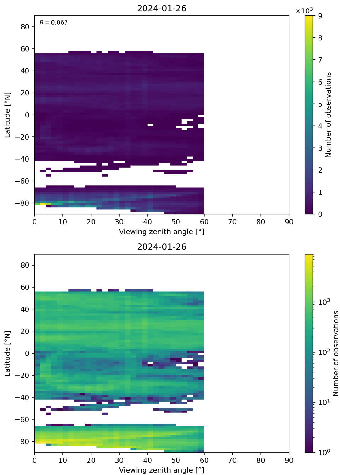
Figure 109: Scatter density plot of “Viewing zenith angle” against “Latitude” for 2024-01-26 to 2024-01-27.
