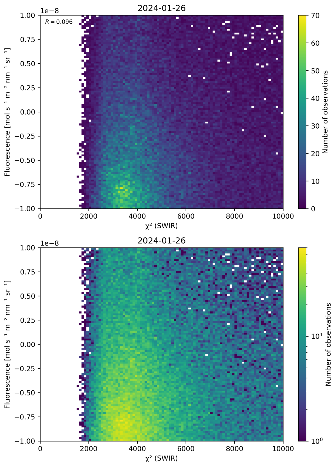
Figure 49: Scatter density plot of “ \chi^2 (SWIR)” against “Fluorescence” for 2024-01-26 to 2024-01-27.
