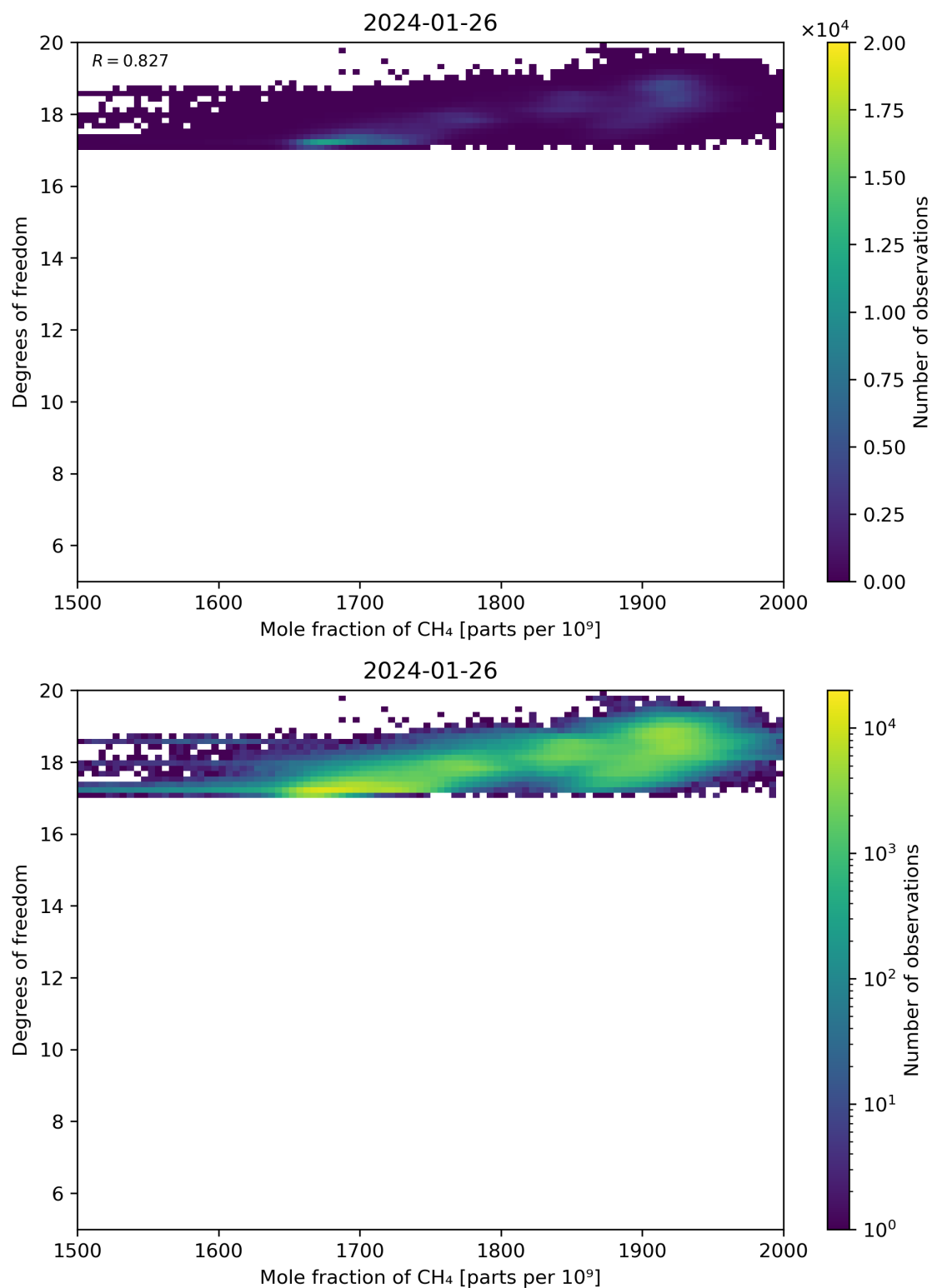
Figure 72: Scatter density plot of “Mole fraction of CH 4 ” against “Degrees of freedom” for 2024-01-26 to 2024-01-27.
