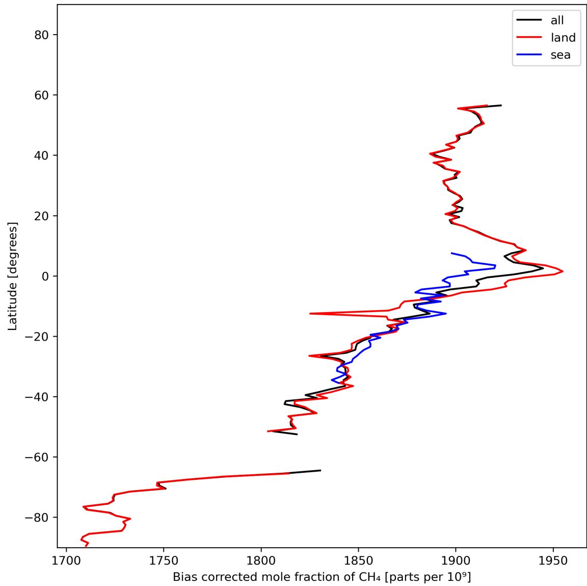
Figure 14: Zonal average of “Bias corrected mole fraction of CH 4 ” for 2024-01-26 to 2024-01-27.
