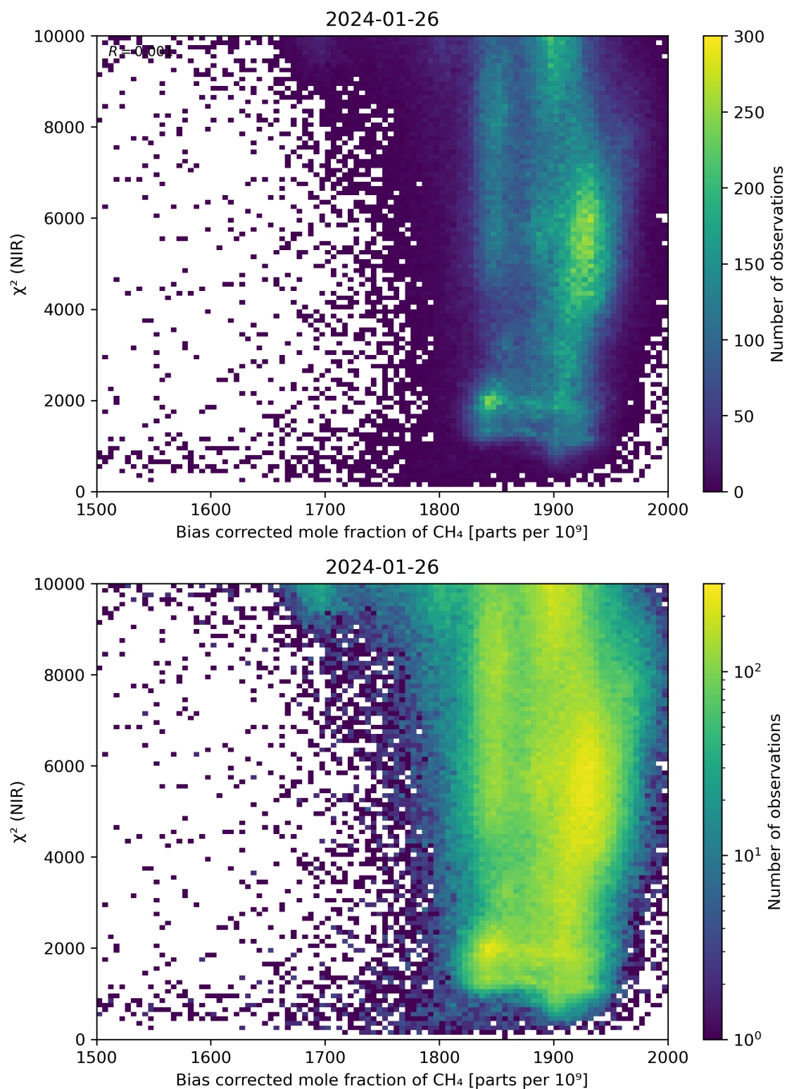
Figure 63: Scatter density plot of “Bias corrected mole fraction of \text{CH}_4 ” against “ \chi^2 (NIR)” for 2024-01-26 to 2024-01-27.
