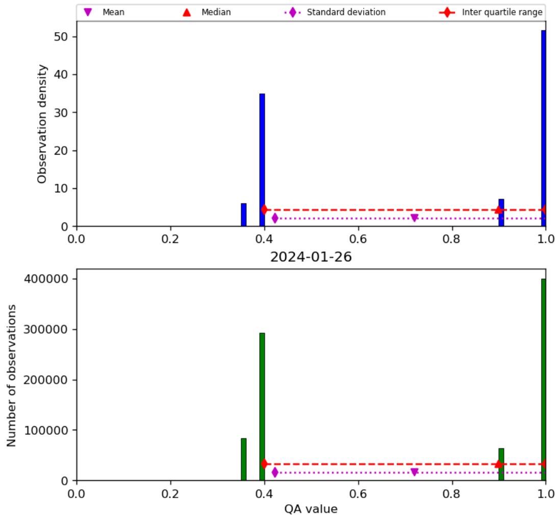
Figure 22: Histogram of “QA value” for 2024-01-26 to 2024-01-27
