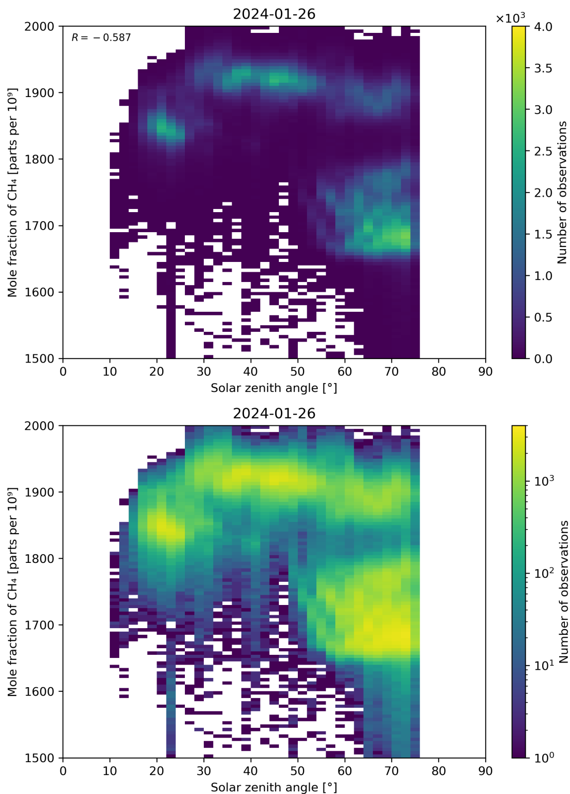
Figure 99: Scatter density plot of “Solar zenith angle” against “Mole fraction of \text{CH}_4 ” for 2024-01-26 to 2024-01-27.
