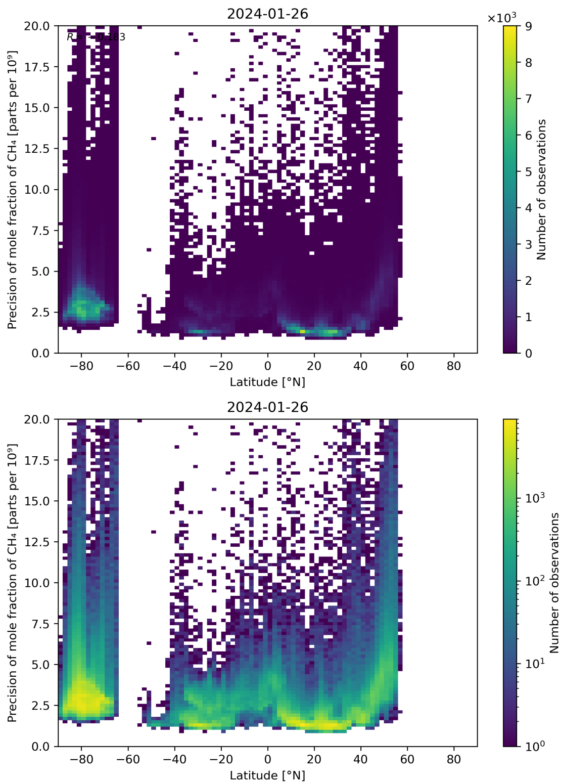
Figure 59: Scatter density plot of “Latitude” against “Precision of mole fraction of CH 4 ” for 2024-01-26 to 2024-01-27.
