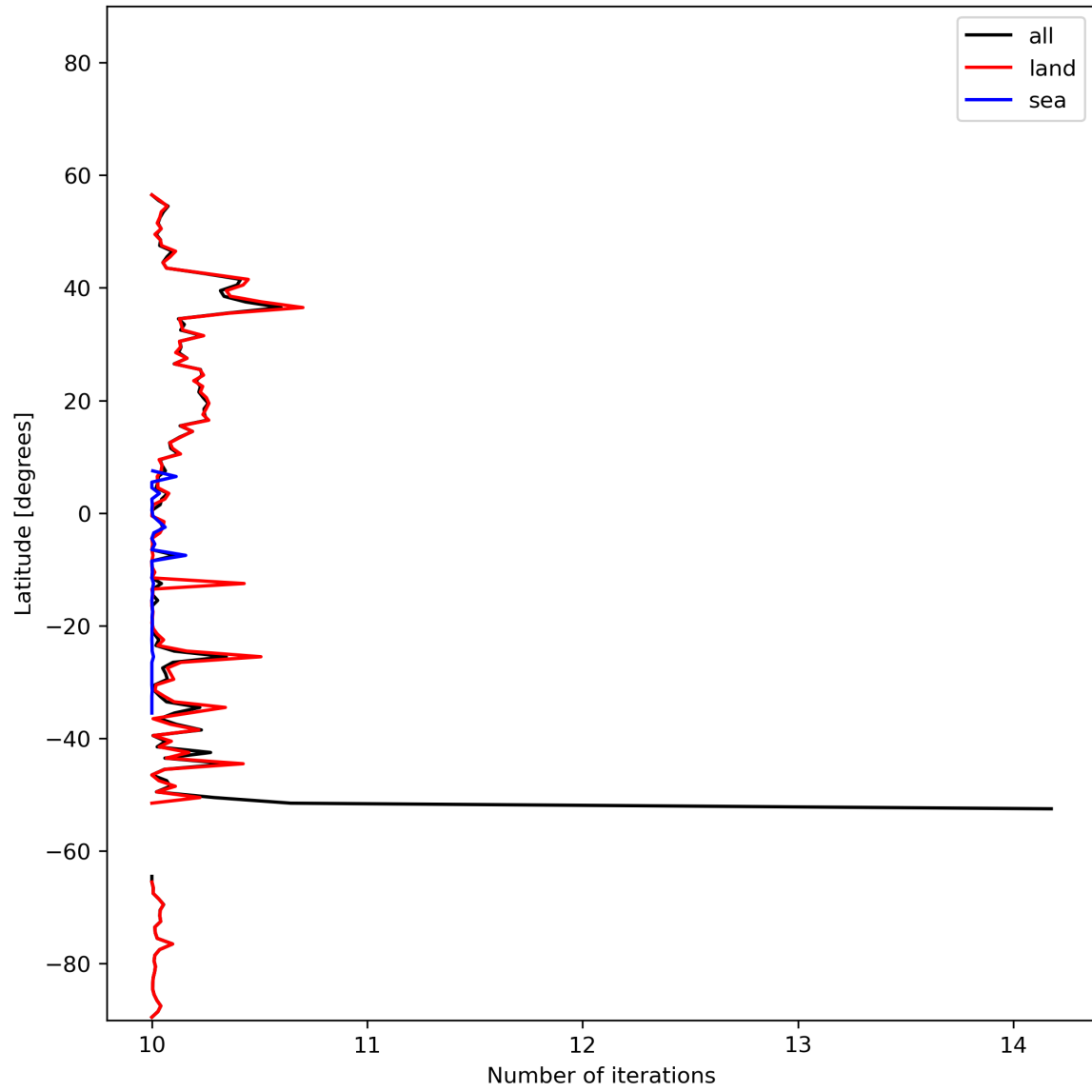
Figure 20: Zonal average of “Number of iterations” for 2024-01-26 to 2024-01-27.
