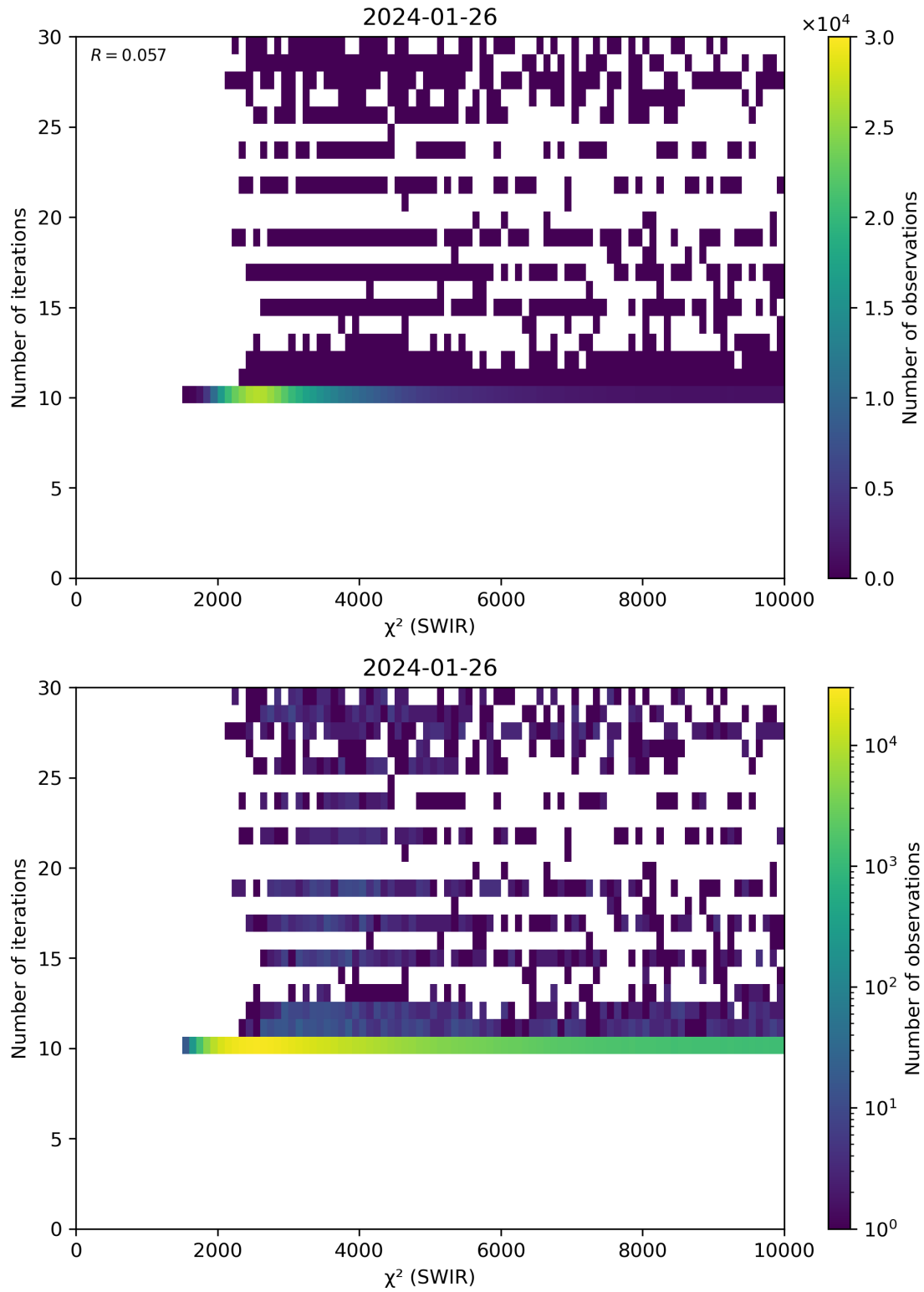
Figure 50: Scatter density plot of “ \chi^2 (SWIR)” against “Number of iterations” for 2024-01-26 to 2024-01-27.
