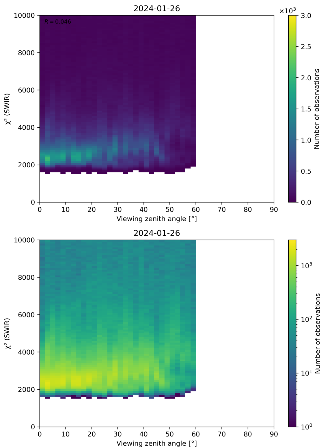
Figure 106: Scatter density plot of “Viewing zenith angle” against “ \chi^2 (SWIR)” for 2024-01-26 to 2024-01-27.
