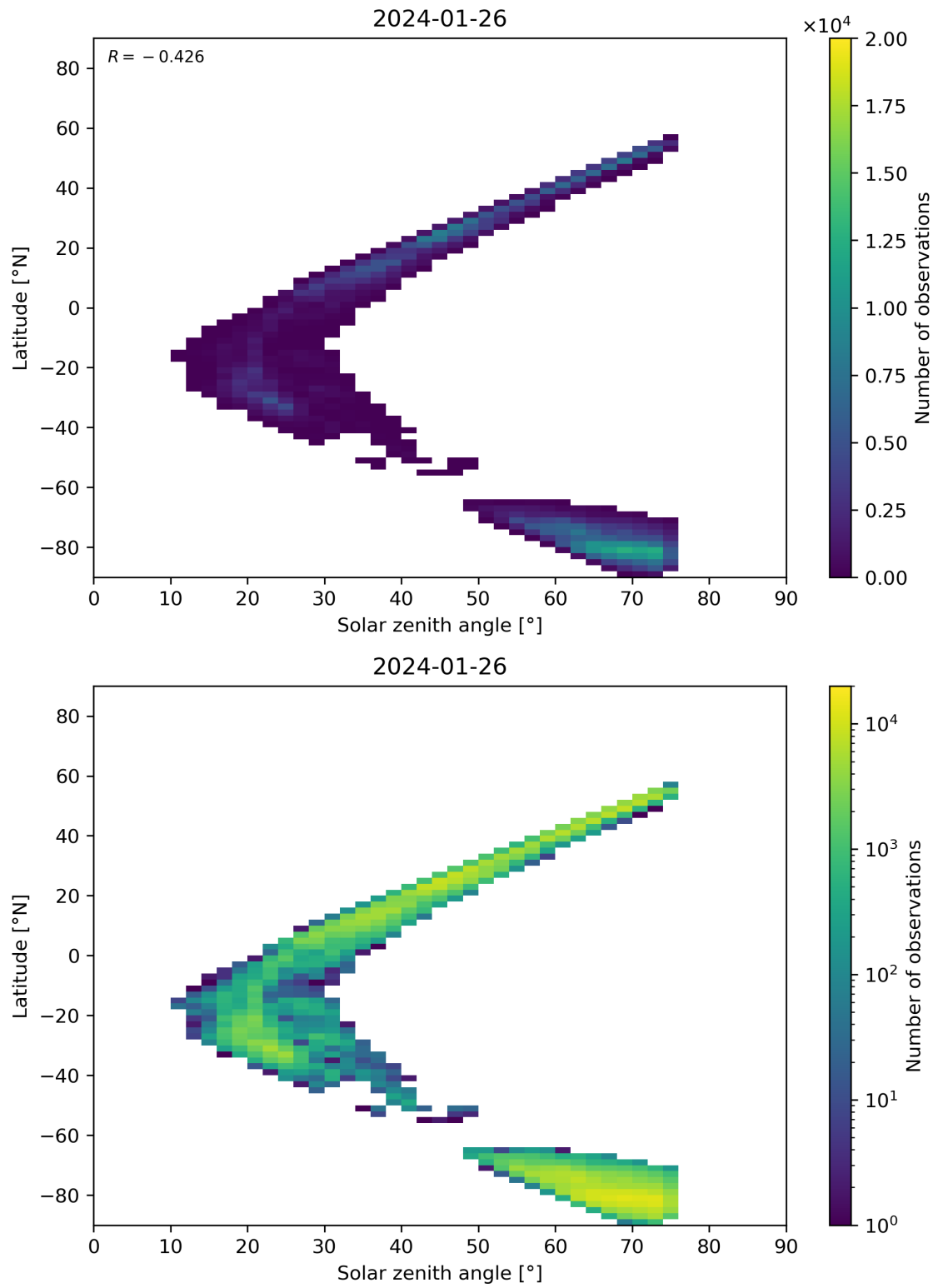
Figure 98: Scatter density plot of “Solar zenith angle” against “Latitude” for 2024-01-26 to 2024-01-27.
