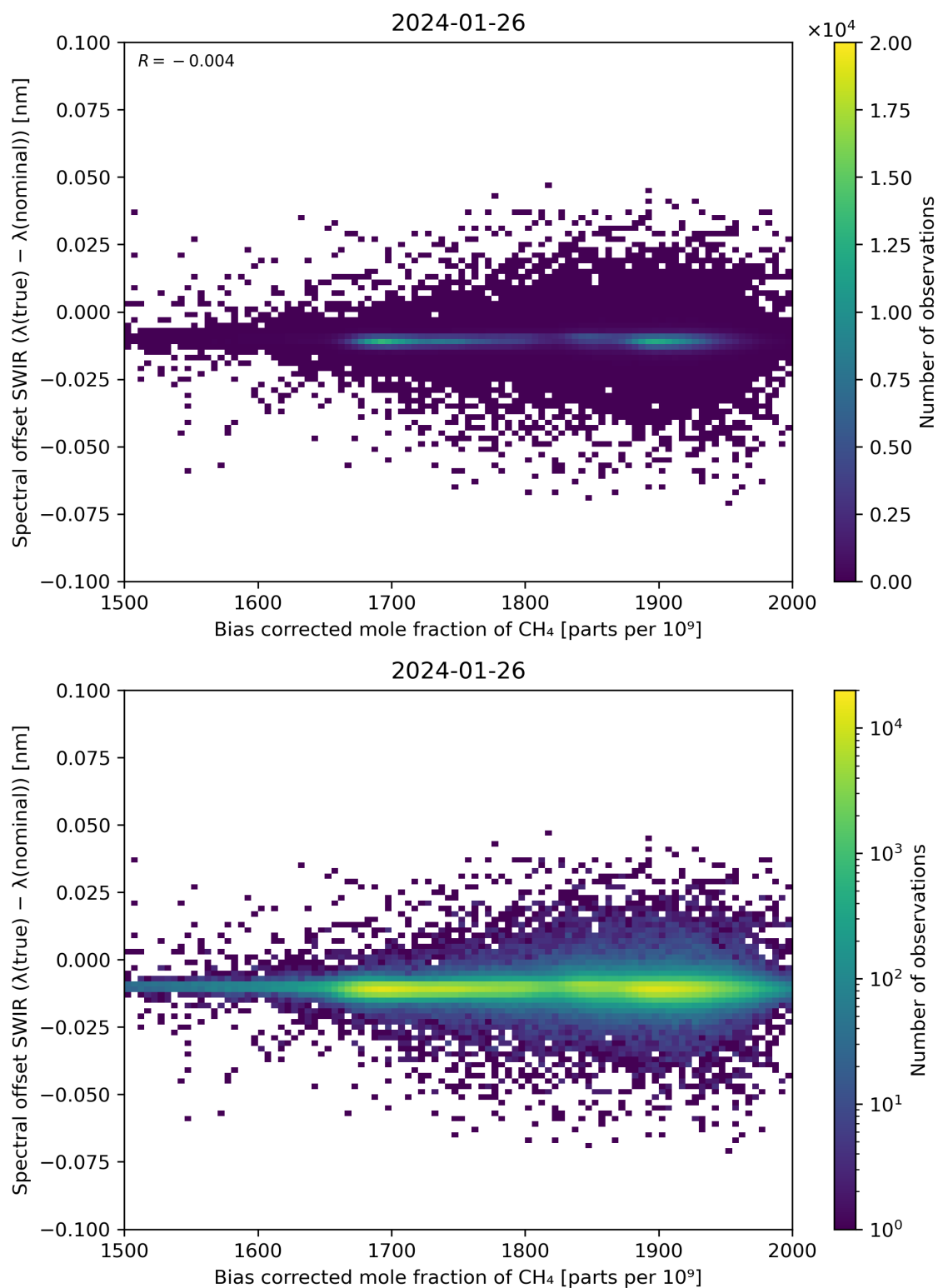
Figure 69: Scatter density plot of “Bias corrected mole fraction of \text{CH}_4 ” against “Spectral offset SWIR ( \lambda(\text{true}) - \lambda(\text{nominal}) )” for 2024-01-26 to 2024-01-27.
