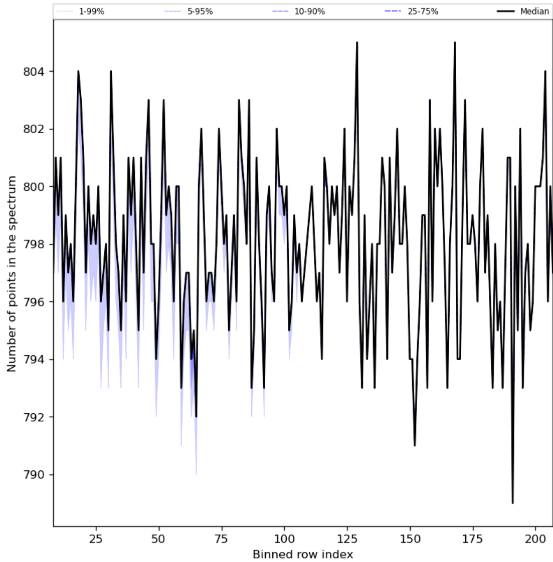
Figure 37: Along track statistics of “Number of points in the spectrum” for 2024-01-26 to 2024-01-27
