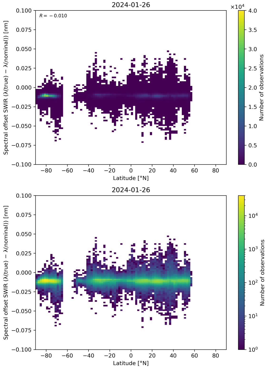
Figure 62: Scatter density plot of “Latitude” against “Spectral offset SWIR ( \lambda(\text{true}) - \lambda(\text{nominal}) )” for 2024-01-26 to 2024-01-27.
