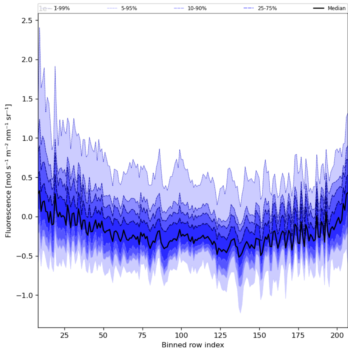
Figure 43: Along track statistics of “Fluorescence” for 2024-01-26 to 2024-01-27
