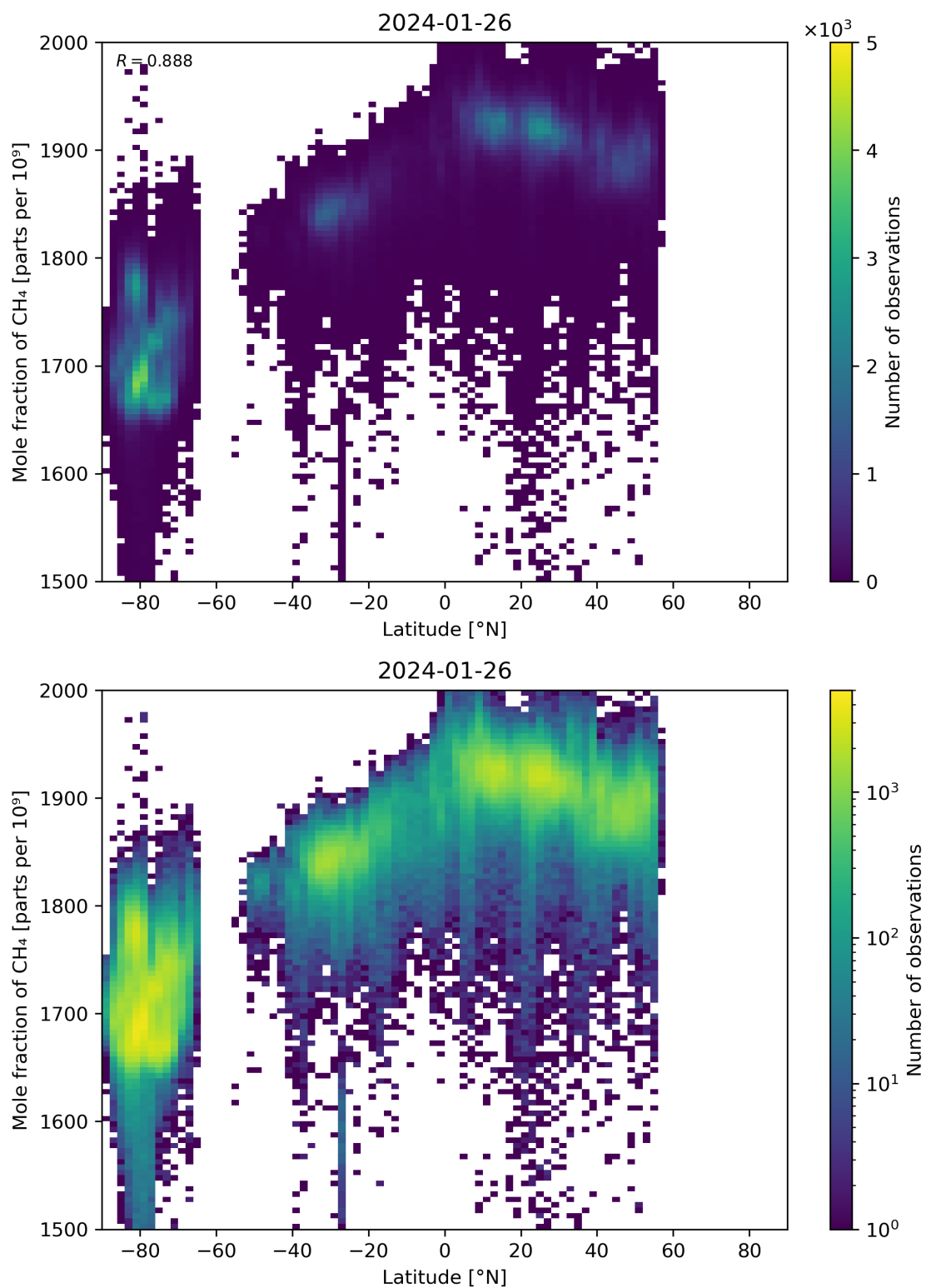
Figure 57: Scatter density plot of “Latitude” against “Mole fraction of CH 4 ” for 2024-01-26 to 2024-01-27.
