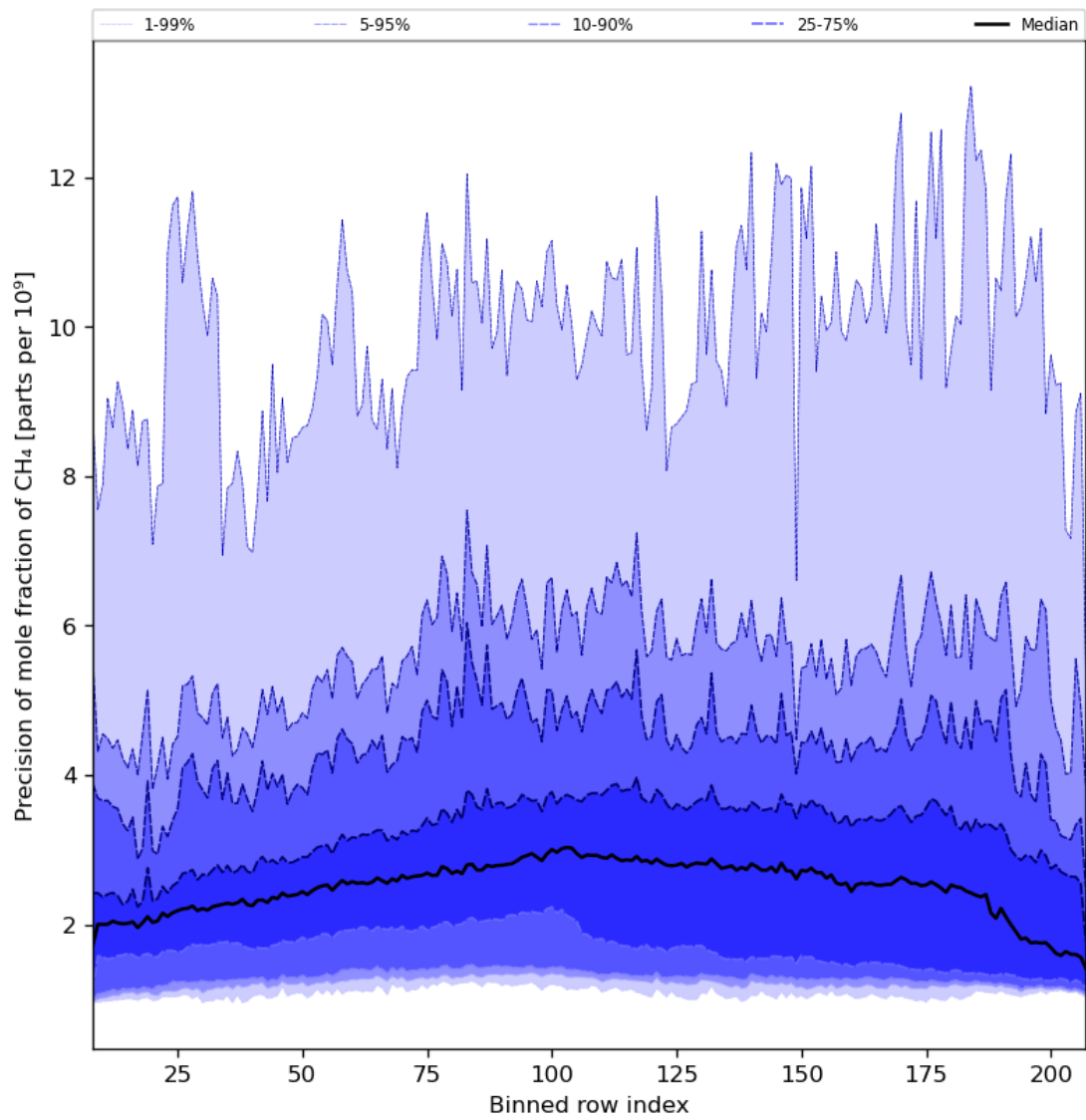
Figure 35: Along track statistics of “Precision of mole fraction of CH 4 ” for 2024-01-26 to 2024-01-27
