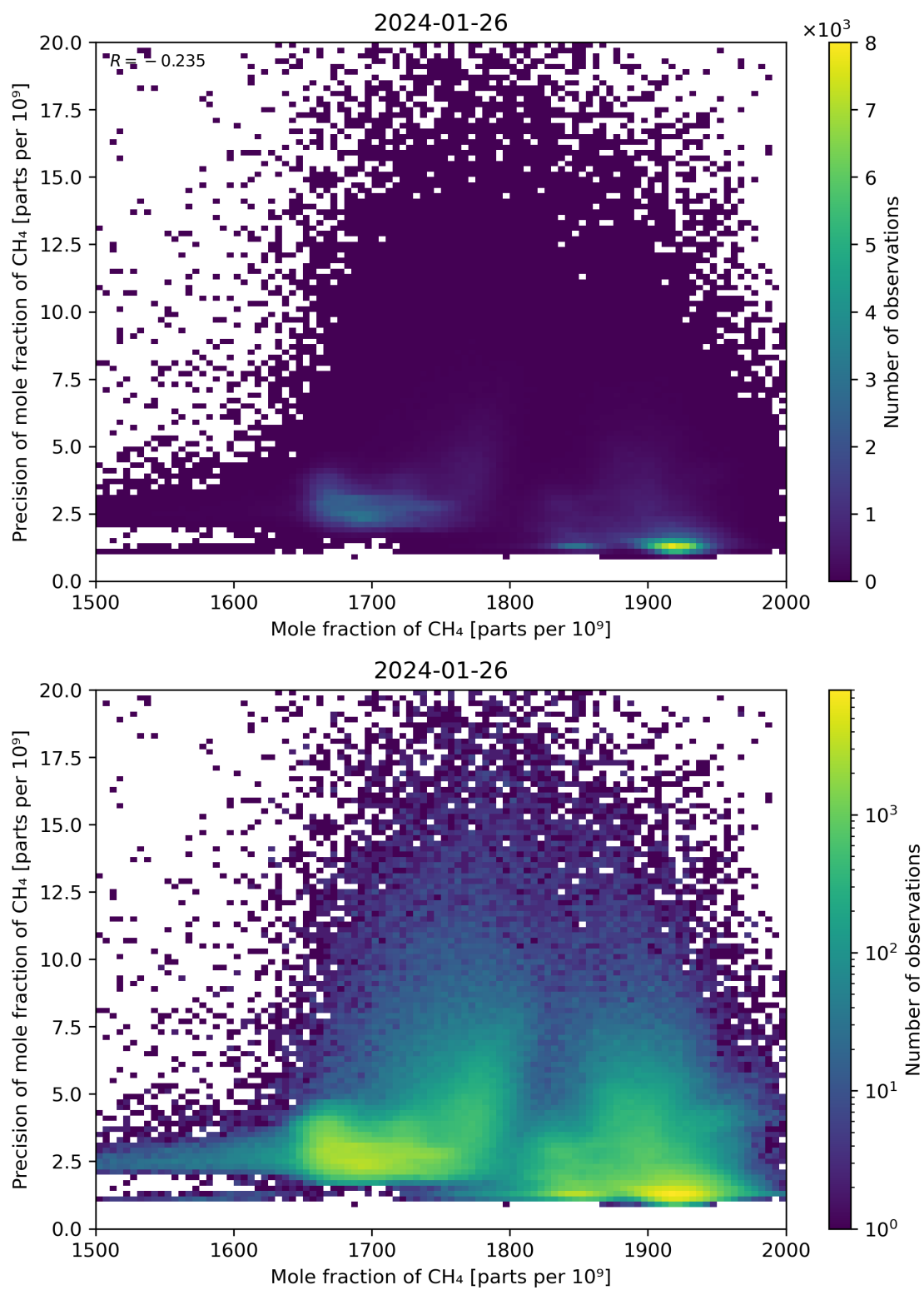
Figure 75: Scatter density plot of “Mole fraction of CH 4 ” against “Precision of mole fraction of CH 4 ” for 2024-01-26 to 2024-01-27.
