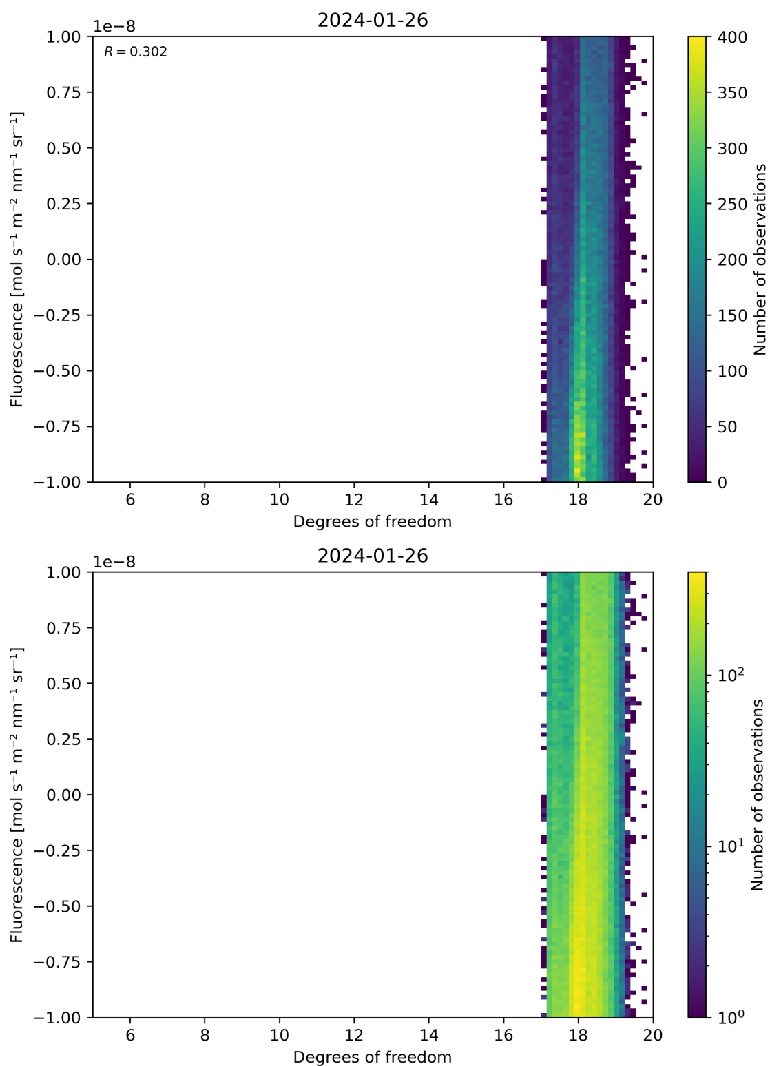
Figure 51: Scatter density plot of “Degrees of freedom” against “Fluorescence” for 2024-01-26 to 2024-01-27.
