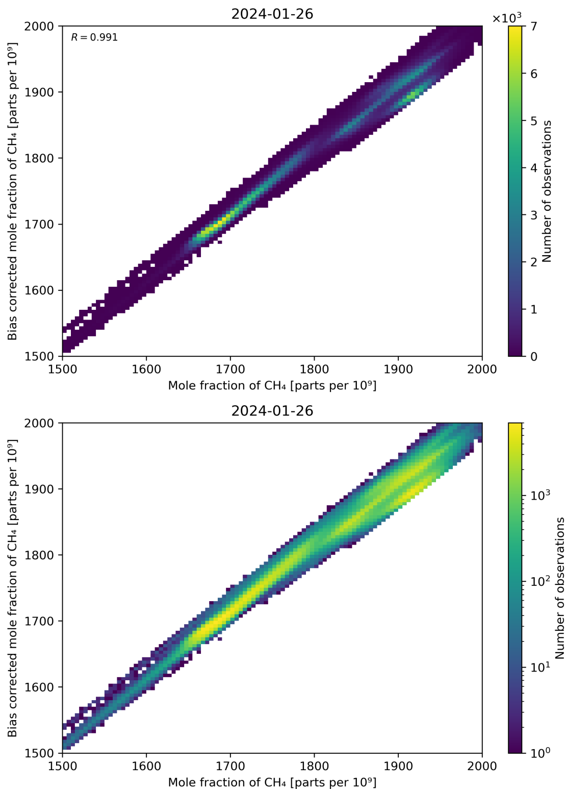
Figure 74: Scatter density plot of “Mole fraction of CH 4 ” against “Bias corrected mole fraction of CH 4 ” for 2024-01-26 to 2024-01-27.
