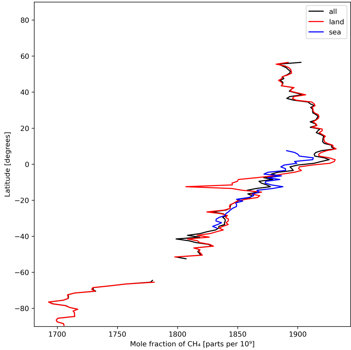
Figure 12: Zonal average of “Mole fraction of CH 4 ” for 2024-01-26 to 2024-01-27.
