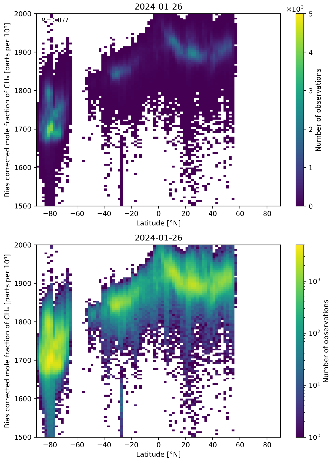
Figure 58: Scatter density plot of “Latitude” against “Bias corrected mole fraction of CH 4 ” for 2024-01-26 to 2024-01-27.
