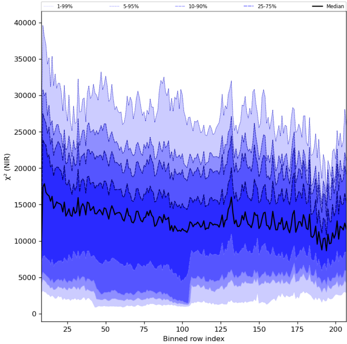
Figure 40: Along track statistics of “ \chi^2 (NIR)” for 2024-01-26 to 2024-01-27
