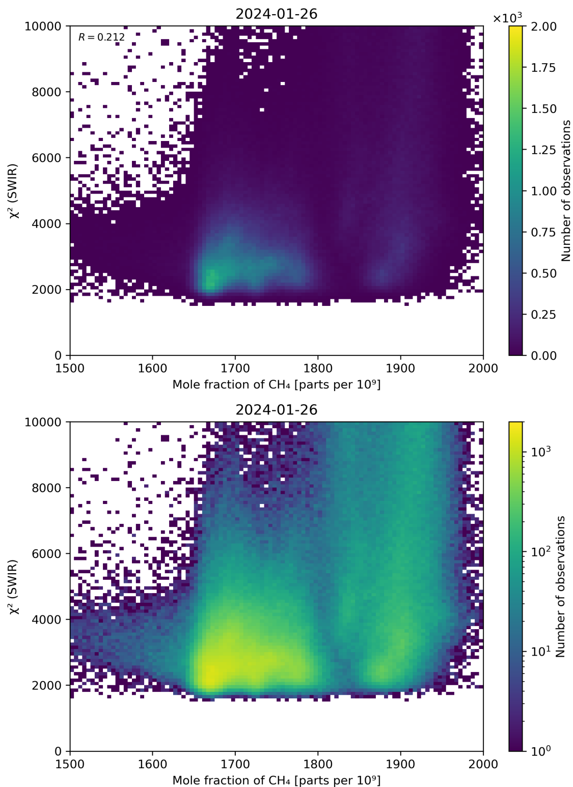
Figure 71: Scatter density plot of “Mole fraction of \text{CH}_4 ” against “ \chi^2 (SWIR)” for 2024-01-26 to 2024-01-27.
