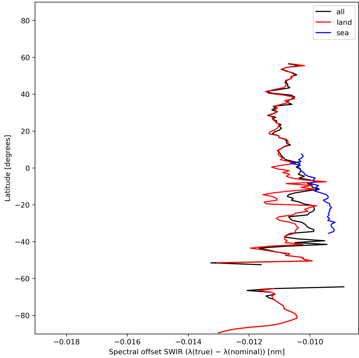
Figure 16: Zonal average of “Spectral offset SWIR ( \lambda(\text{true}) - \lambda(\text{nominal}) )” for 2024-01-26 to 2024-01-27.
