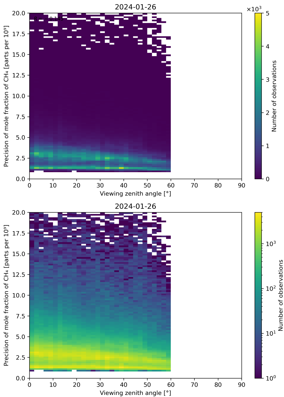
Figure 112: Scatter density plot of “Viewing zenith angle” against “Precision of mole fraction of CH 4 ” for 2024-01-26 to 2024-01-27.
