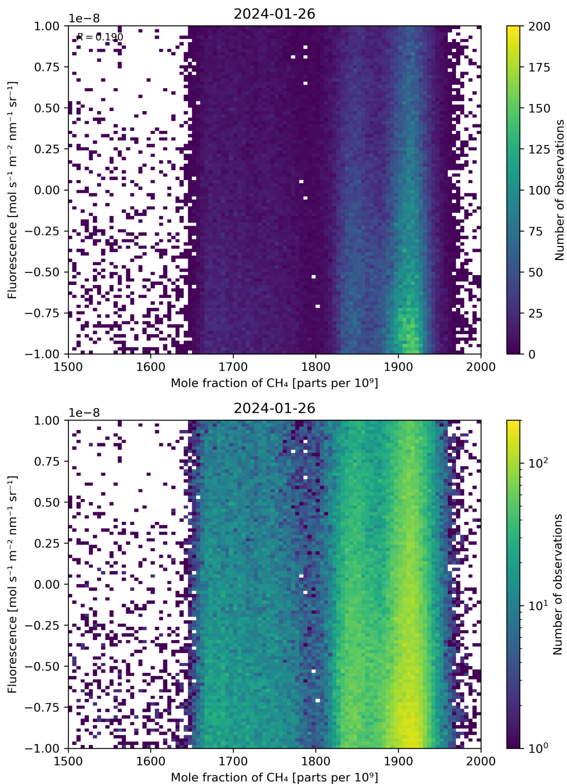
Figure 73: Scatter density plot of “Mole fraction of \text{CH}_4 ” against “Fluorescence” for 2024-01-26 to 2024-01-27.
