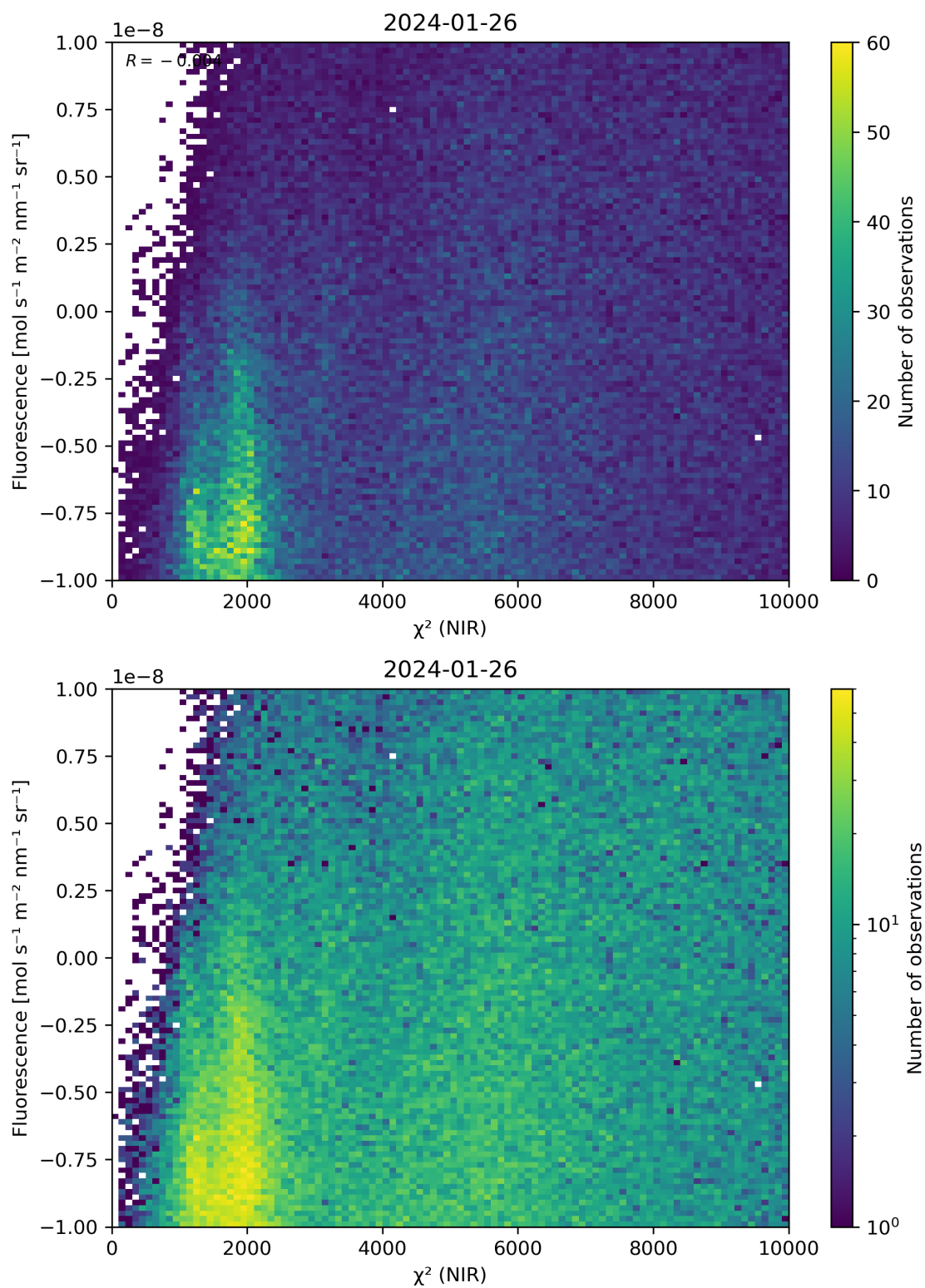
Figure 45: Scatter density plot of “ \chi^2 (NIR)” against “Fluorescence” for 2024-01-26 to 2024-01-27.
