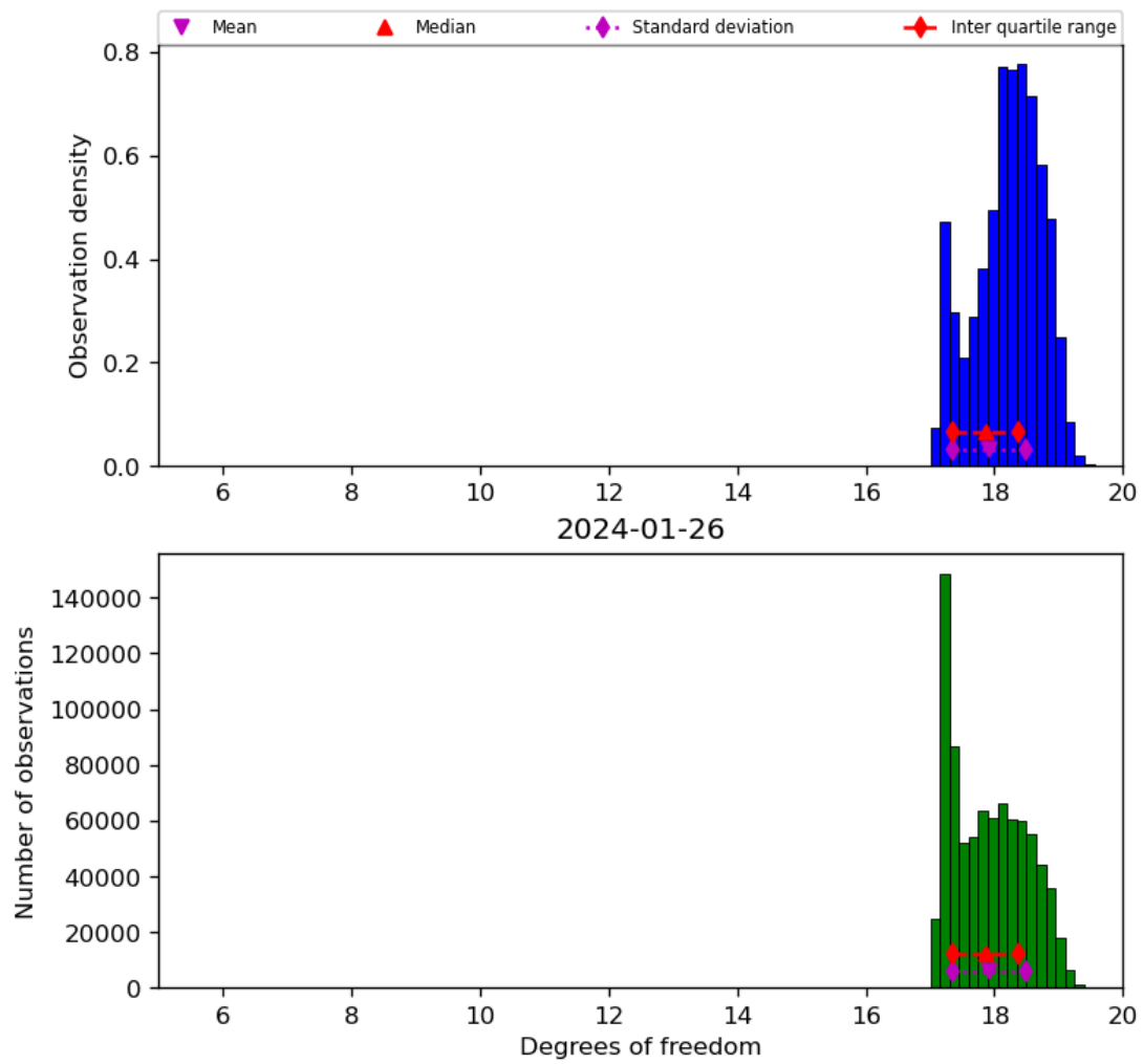
Figure 30: Histogram of “Degrees of freedom” for 2024-01-26 to 2024-01-27
