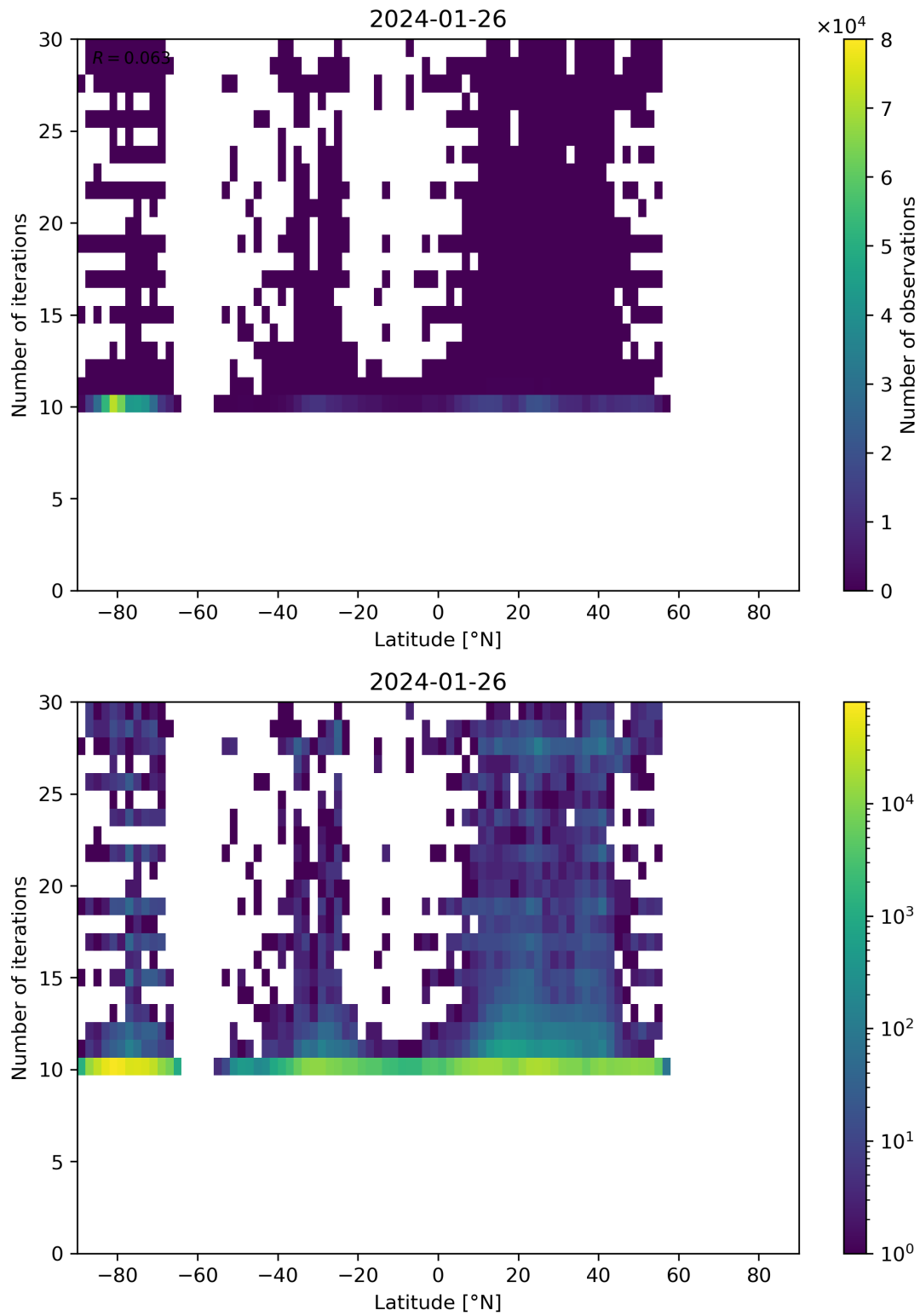
Figure 60: Scatter density plot of “Latitude” against “Number of iterations” for 2024-01-26 to 2024-01-27.
