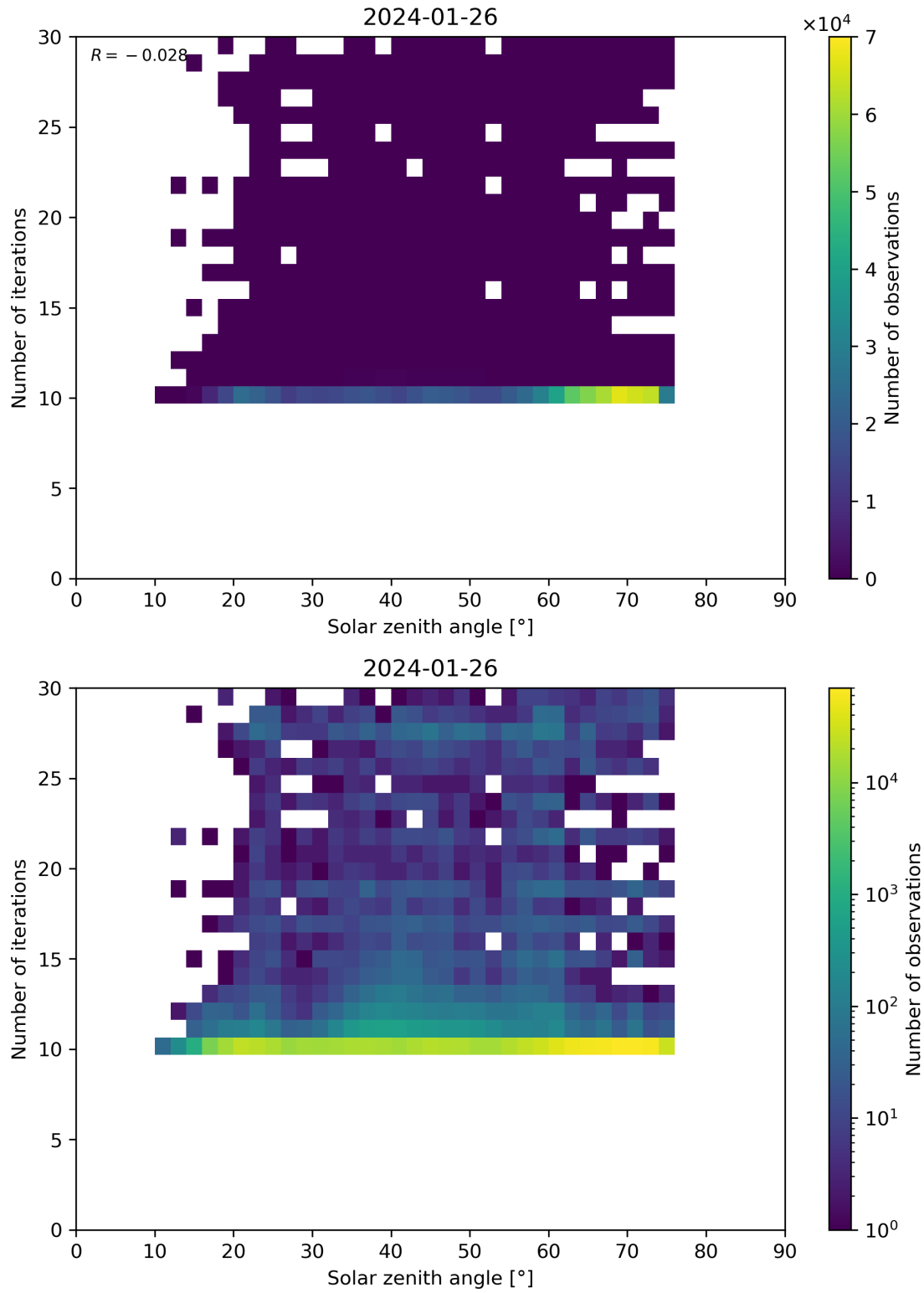
Figure 102: Scatter density plot of “Solar zenith angle” against “Number of iterations” for 2024-01-26 to 2024-01-27.
