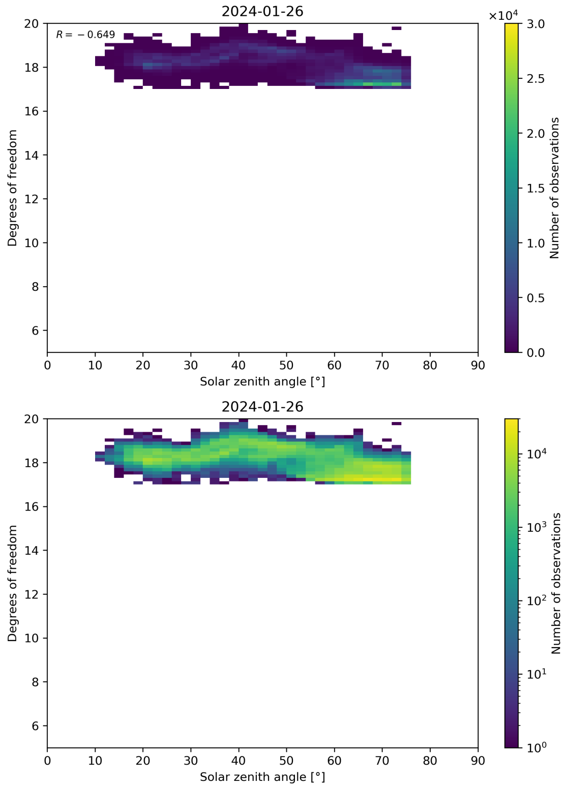
Figure 96: Scatter density plot of “Solar zenith angle” against “Degrees of freedom” for 2024-01-26 to 2024-01-27.
