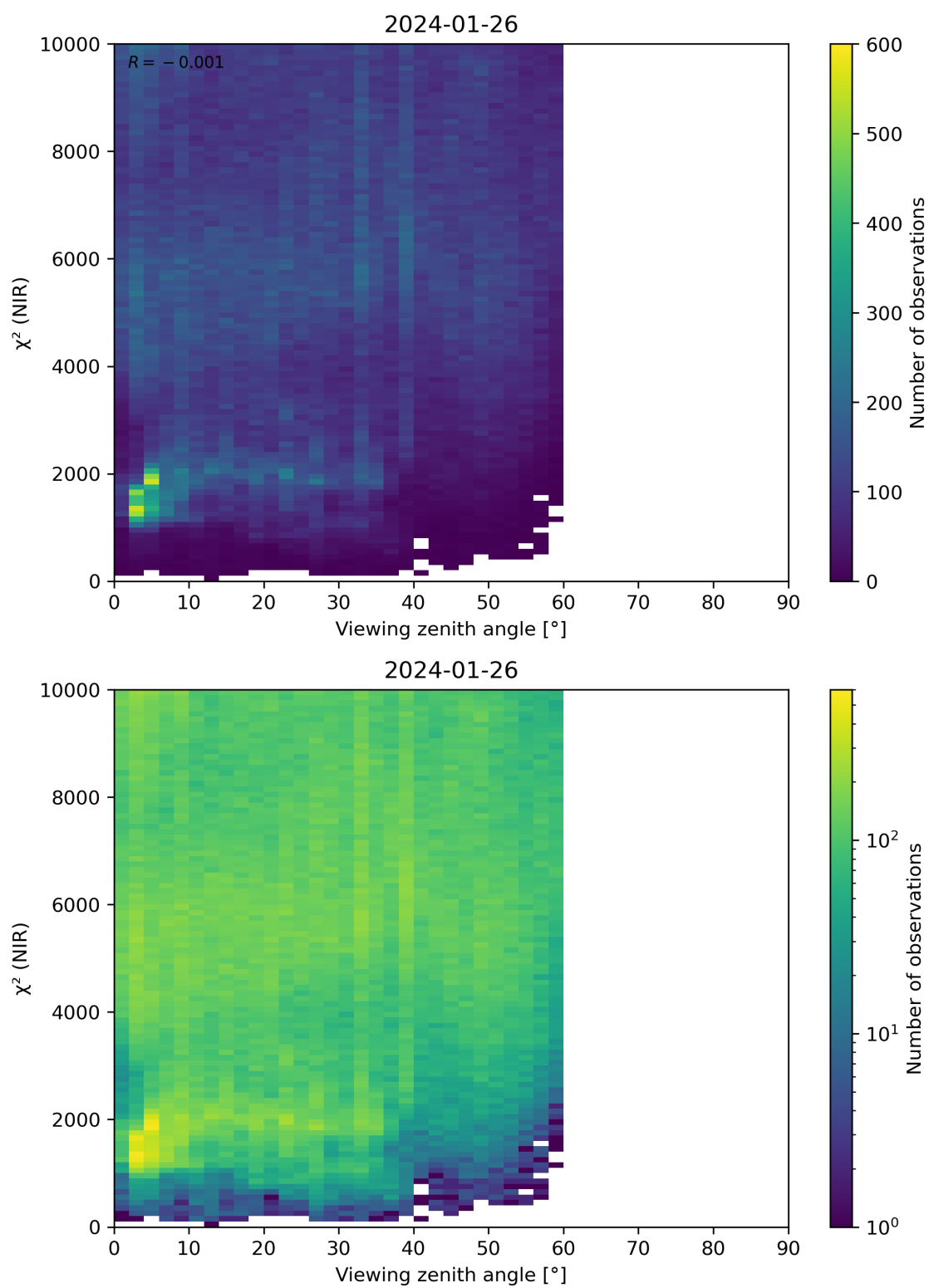
Figure 105: Scatter density plot of “Viewing zenith angle” against “ \chi^2 (NIR)” for 2024-01-26 to 2024-01-27.
