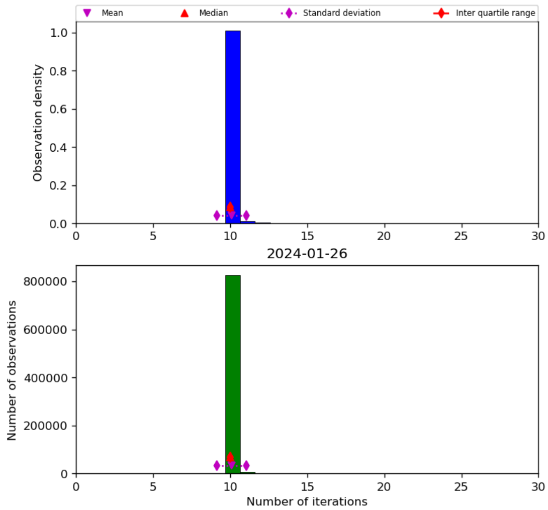
Figure 31: Histogram of “Number of iterations” for 2024-01-26 to 2024-01-27
