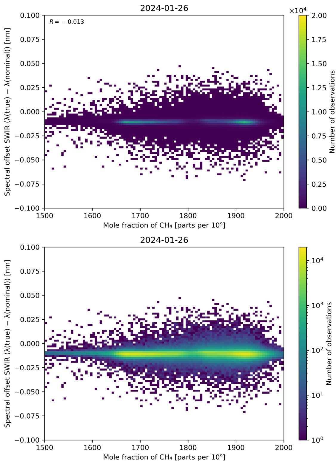
Figure 86: Scatter density plot of “Mole fraction of CH 4 ” against “Spectral offset SWIR ( \lambda(\text{true}) - \lambda(\text{nominal}) )” for 2024-01-26 to 2024-01-27.
