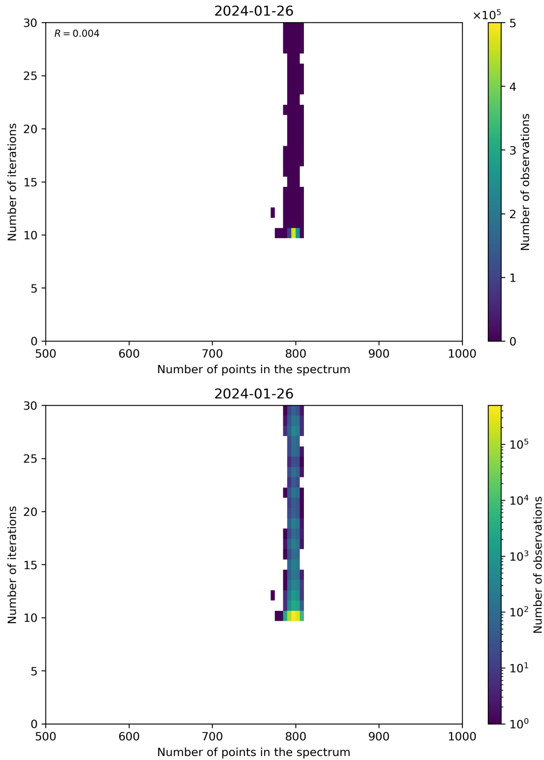
Figure 92: Scatter density plot of “Number of points in the spectrum” against “Number of iterations” for 2024-01-26 to 2024-01-27.
