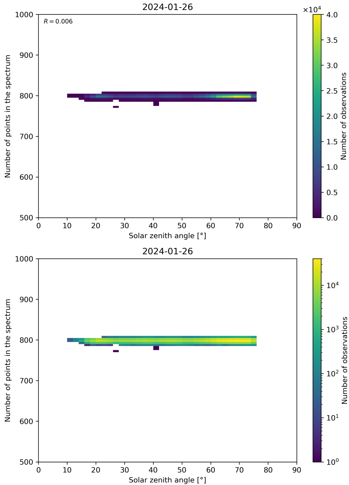
Figure 103: Scatter density plot of “Solar zenith angle” against “Number of points in the spectrum” for 2024-01-26 to 2024-01-27.
