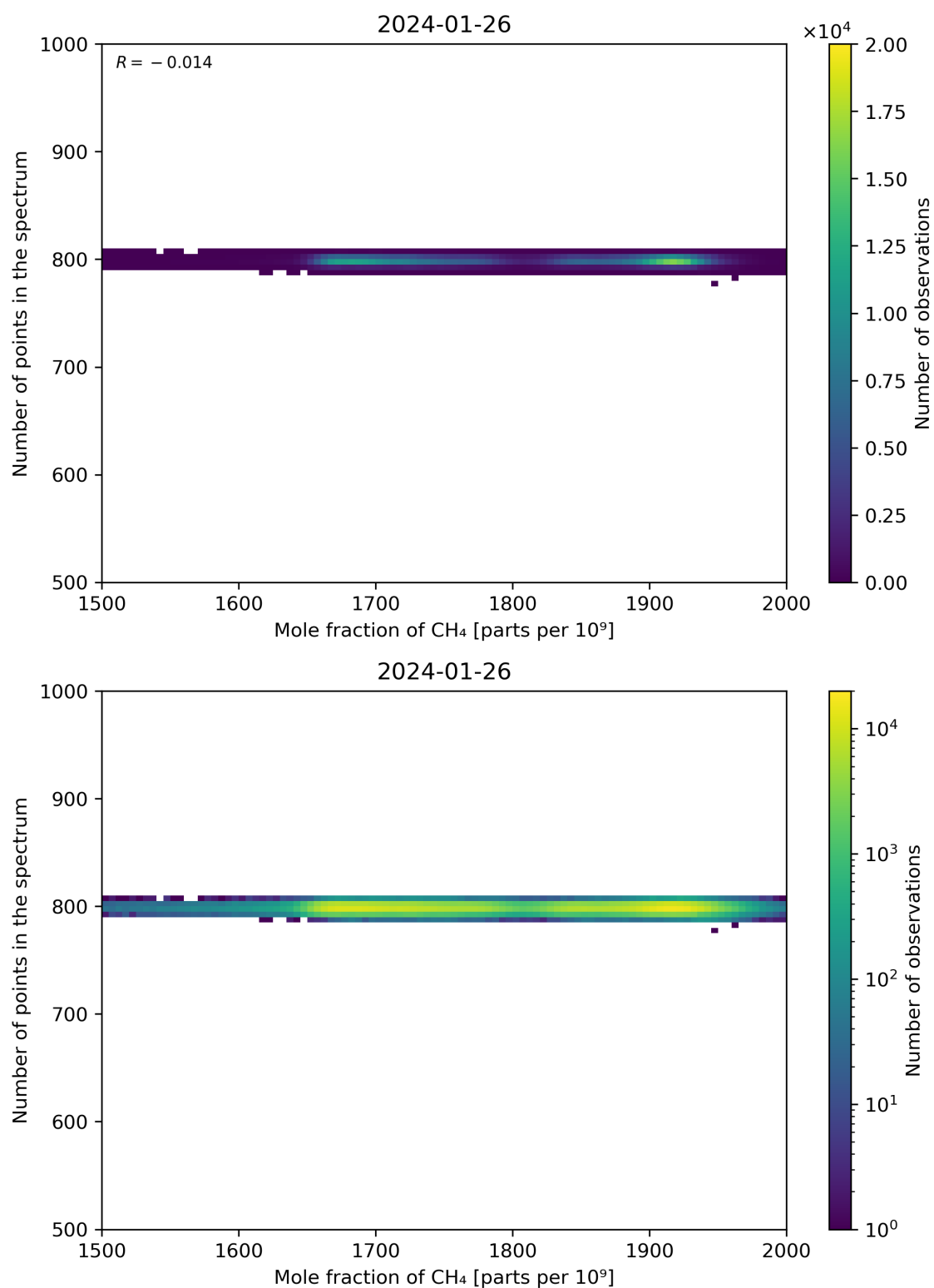
Figure 77: Scatter density plot of “Mole fraction of CH 4 ” against “Number of points in the spectrum” for 2024-01-26 to 2024-01-27.
