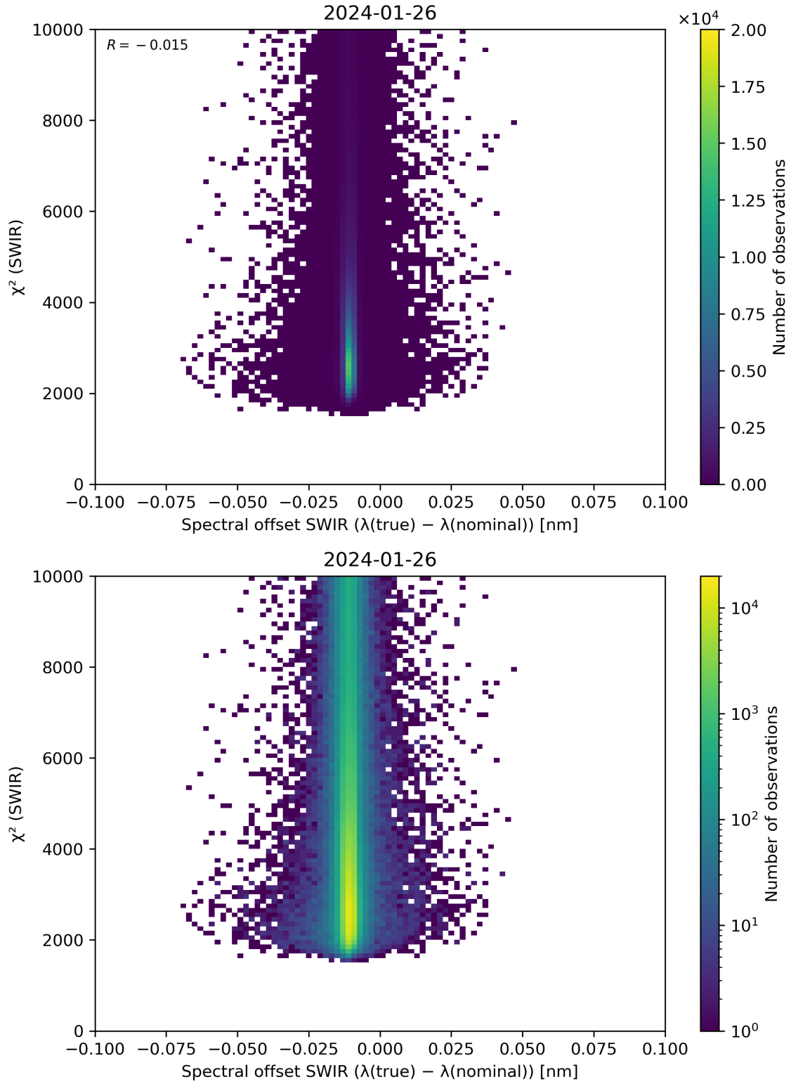
Figure 118: Scatter density plot of “Spectral offset SWIR ( \lambda(\text{true}) - \lambda(\text{nominal}) )” against “ \chi^2 (SWIR)” for 2024-01-26 to 2024-01-27.
