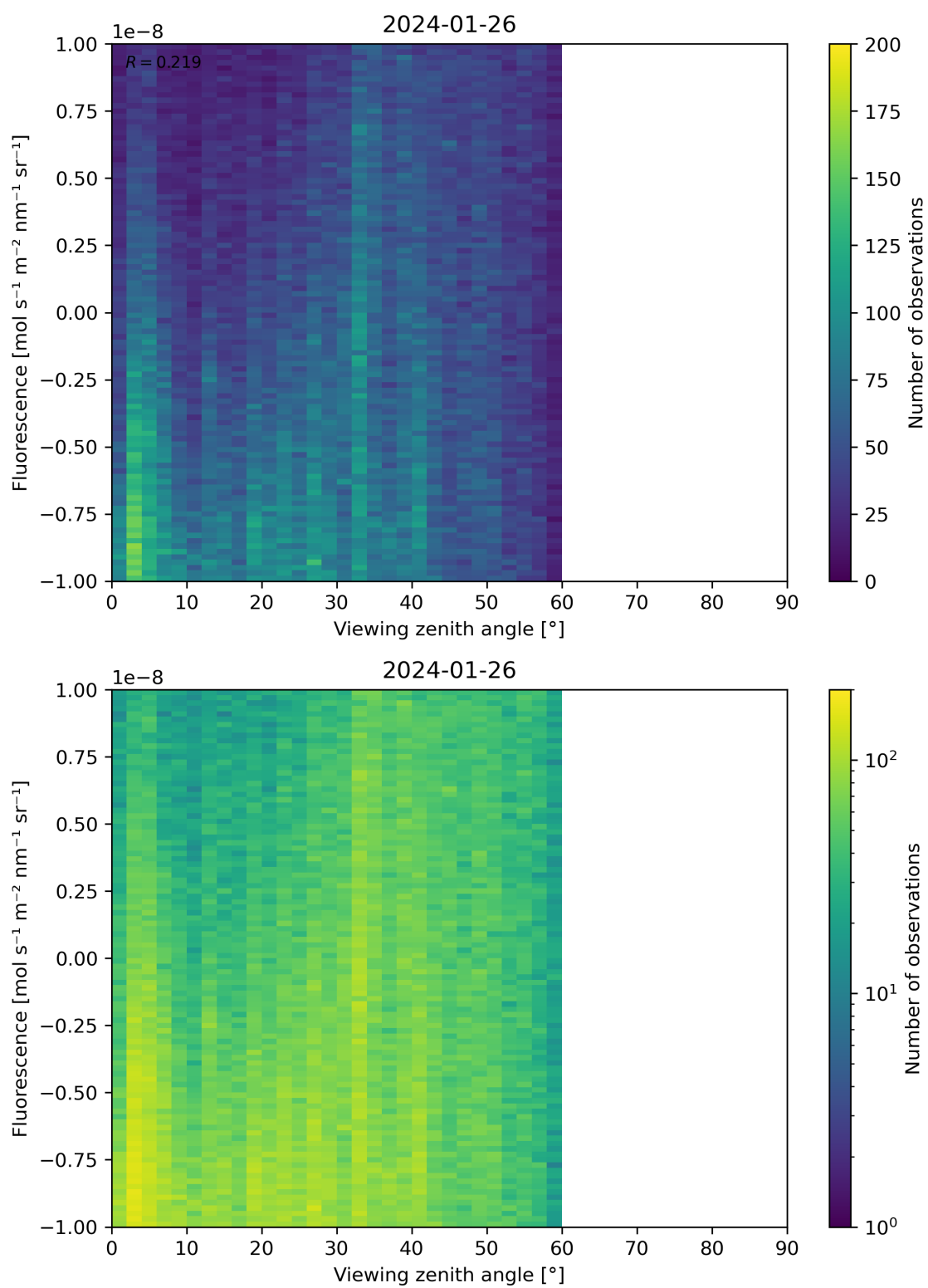
Figure 108: Scatter density plot of “Viewing zenith angle” against “Fluorescence” for 2024-01-26 to 2024-01-27.
