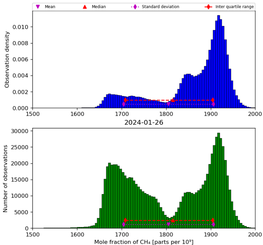
Figure 23: Histogram of “Mole fraction of CH 4 ” for 2024-01-26 to 2024-01-27
