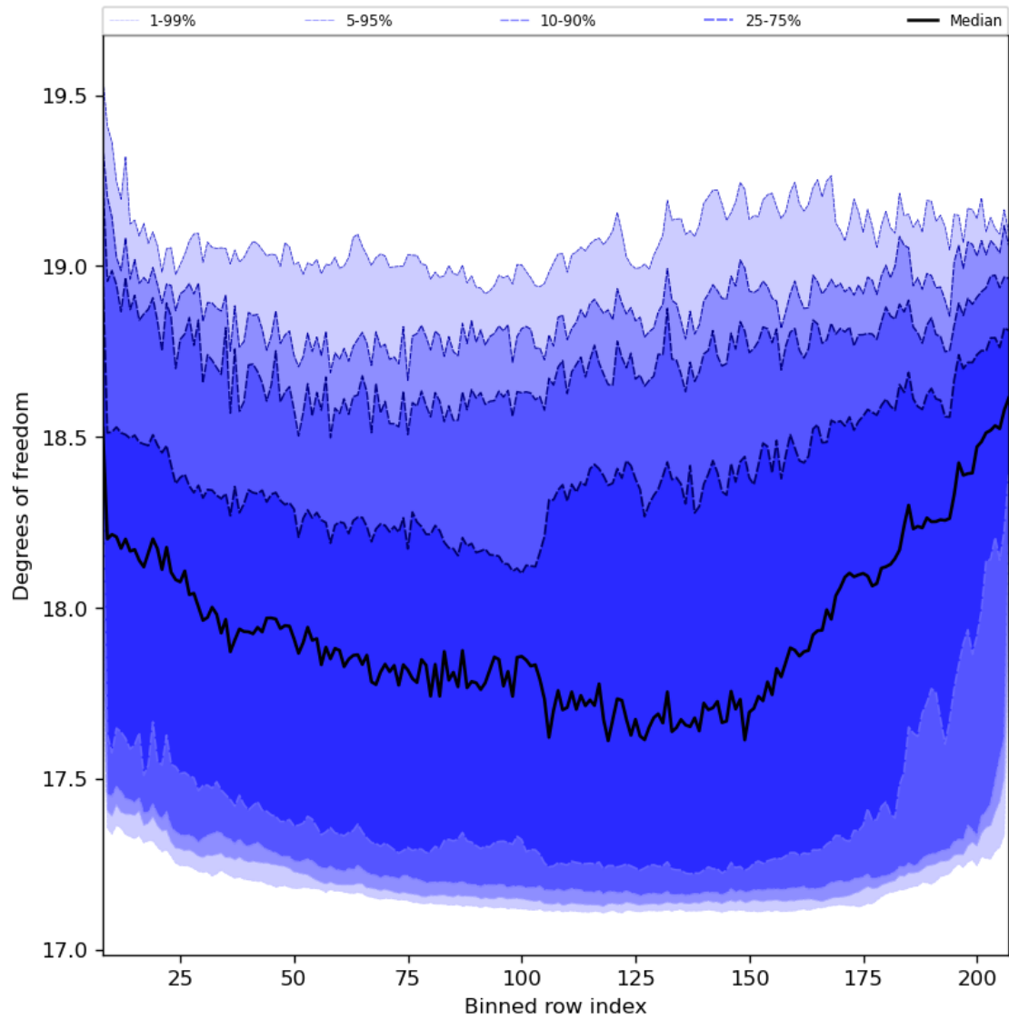
Figure 41: Along track statistics of “Degrees of freedom” for 2024-01-26 to 2024-01-27
