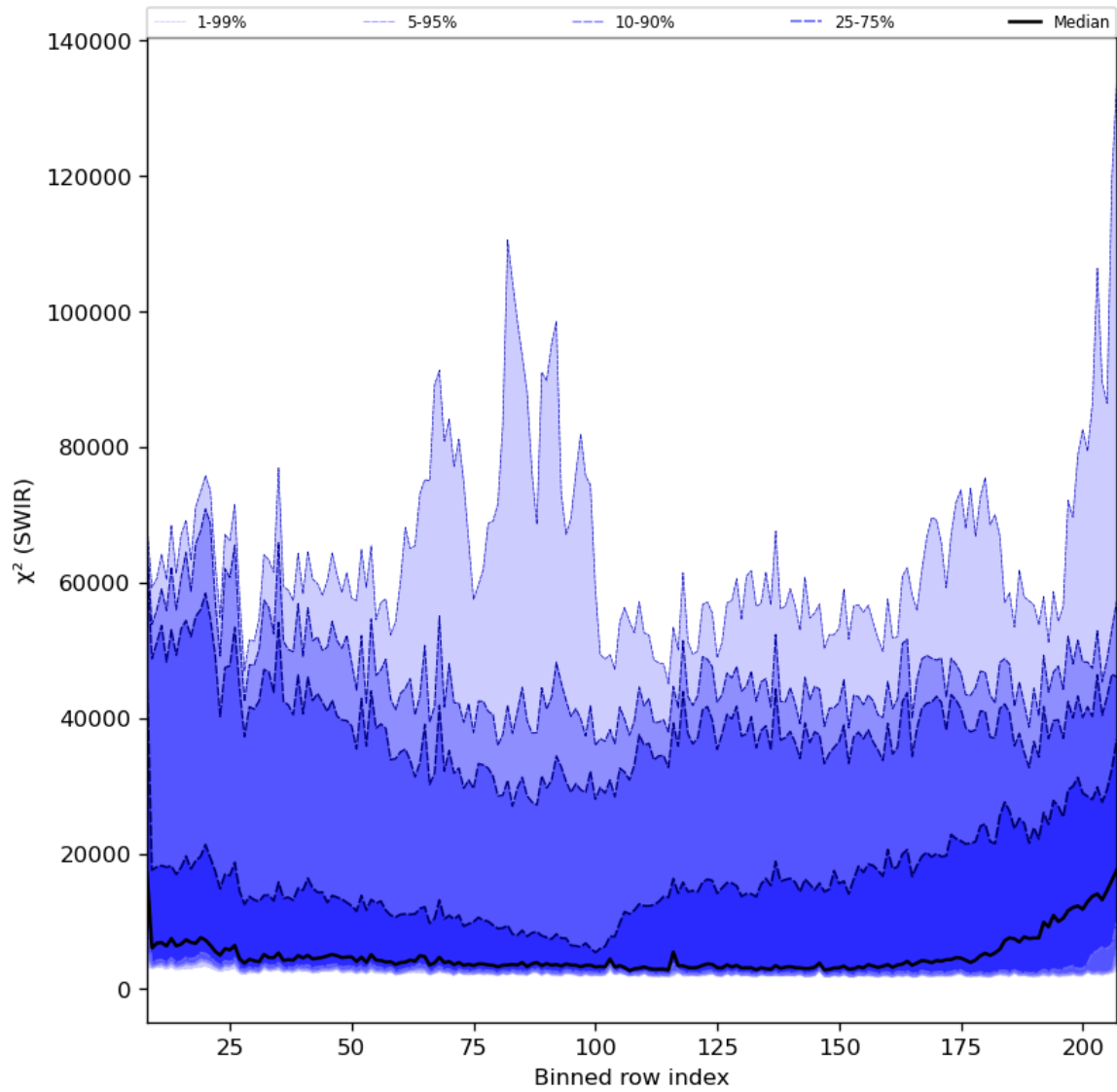
Figure 39: Along track statistics of “ \chi^2 (SWIR)” for 2024-01-26 to 2024-01-27
