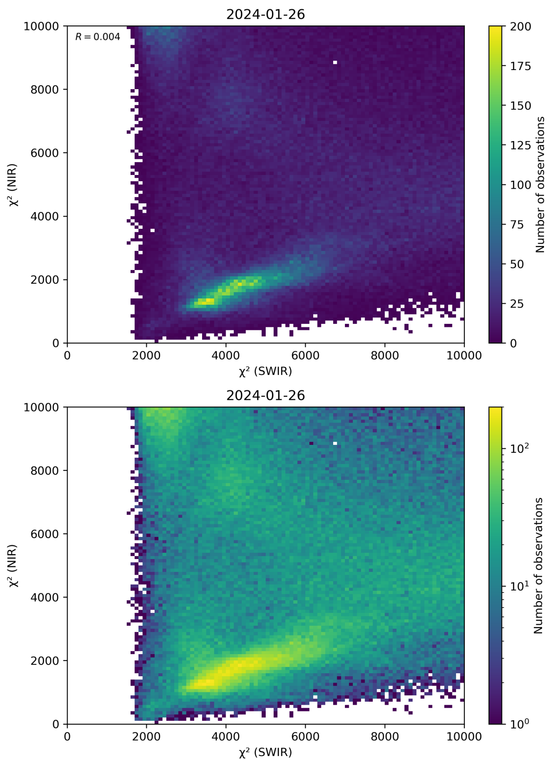
Figure 47: Scatter density plot of “ \chi^2 (SWIR)” against “ \chi^2 (NIR)” for 2024-01-26 to 2024-01-27.
