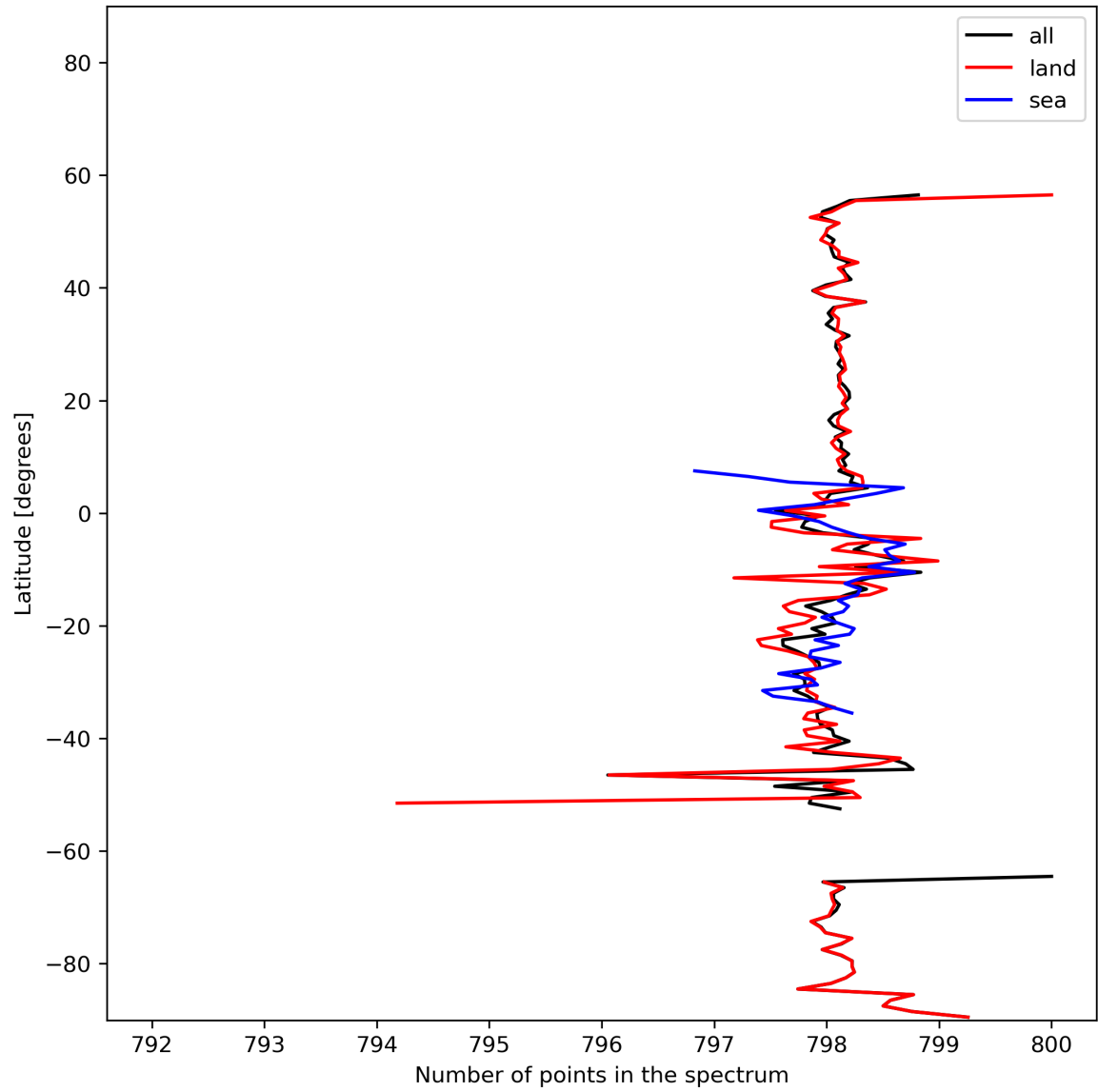
Figure 15: Zonal average of “Number of points in the spectrum” for 2024-01-26 to 2024-01-27.
