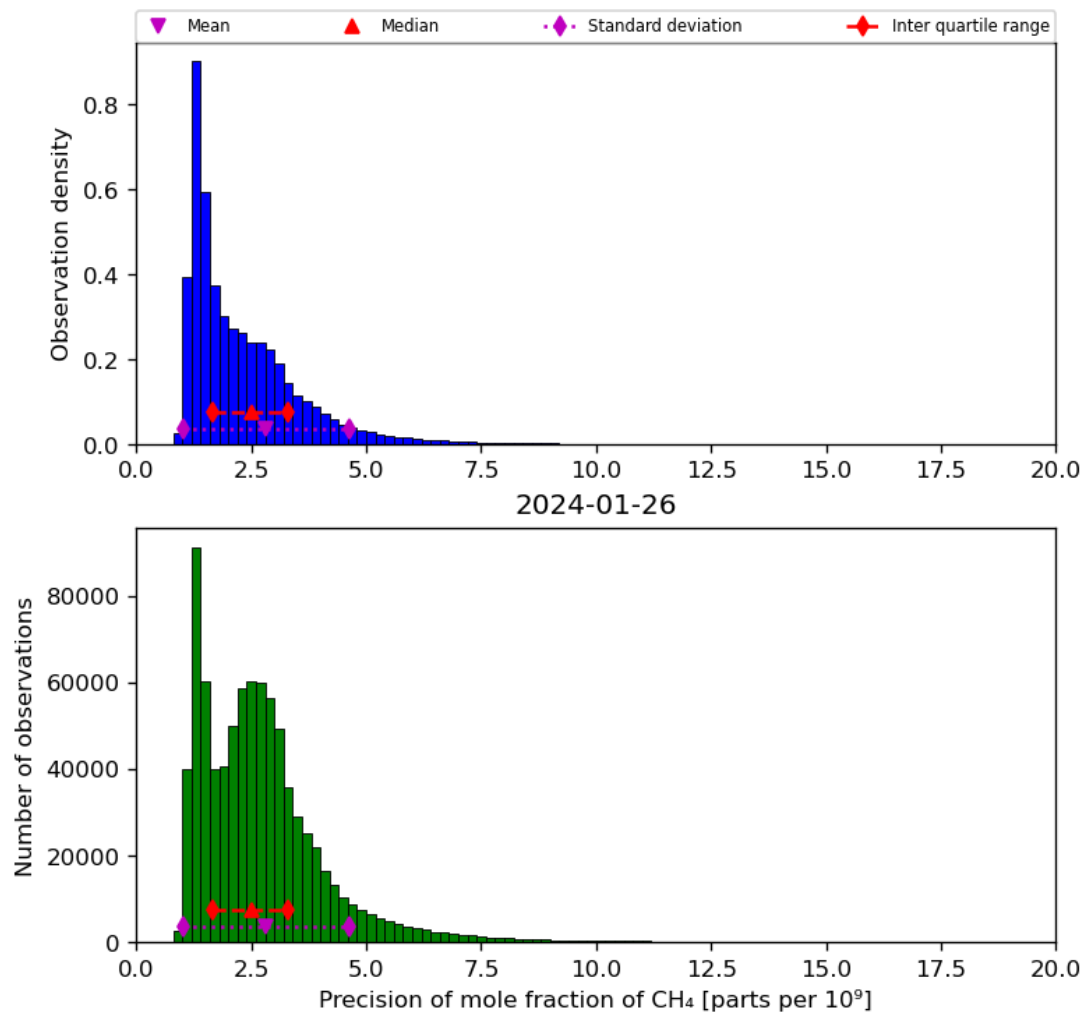
Figure 24: Histogram of “Precision of mole fraction of CH 4 ” for 2024-01-26 to 2024-01-27
