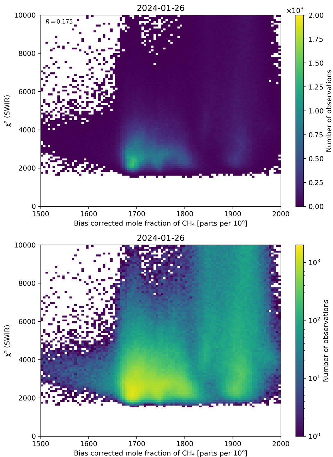
Figure 64: Scatter density plot of “Bias corrected mole fraction of \text{CH}_4 ” against “ \chi^2 (SWIR)” for 2024-01-26 to 2024-01-27.
