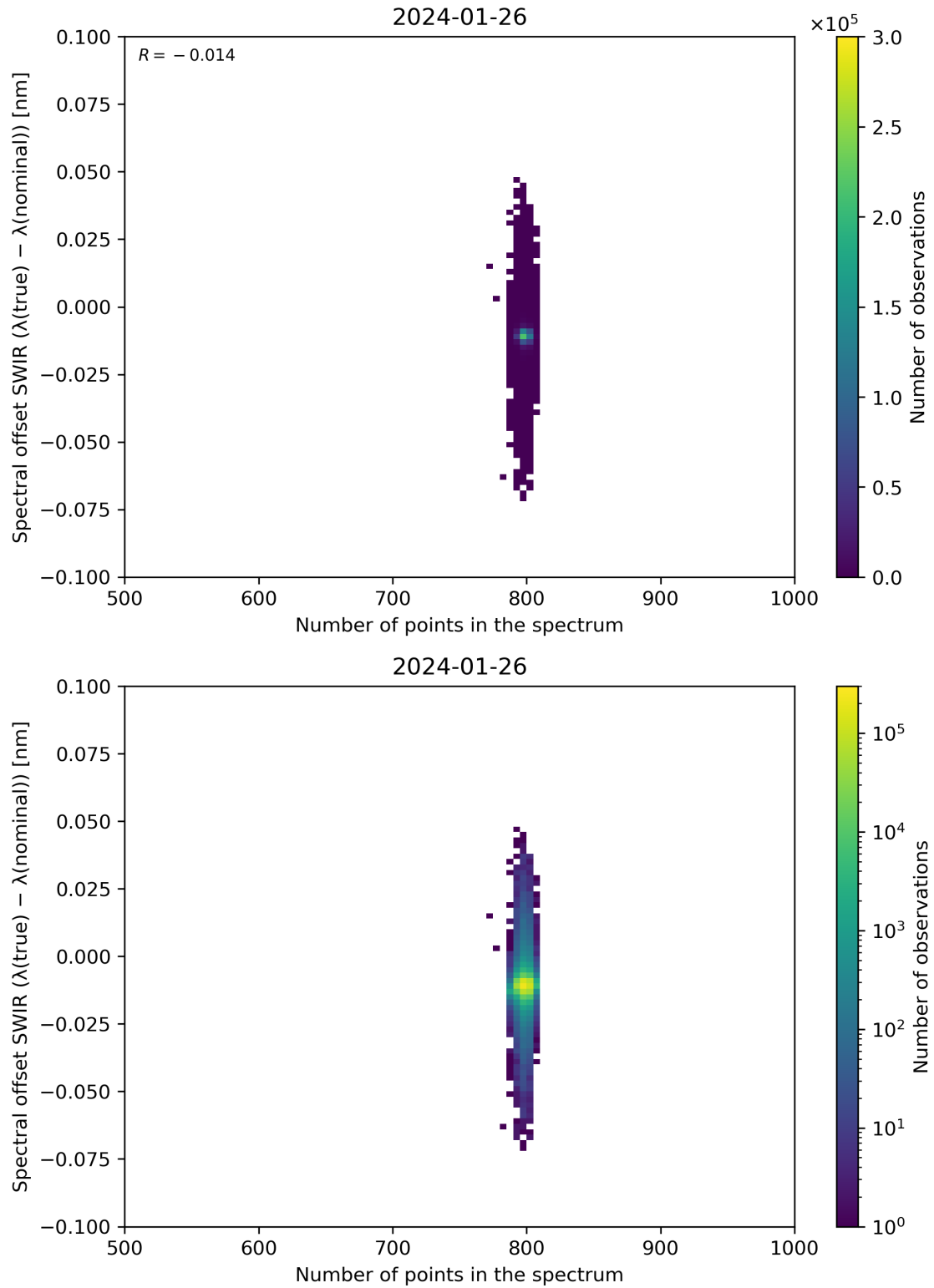
Figure 93: Scatter density plot of “Number of points in the spectrum” against “Spectral offset SWIR ( \lambda(\text{true}) - \lambda(\text{nominal}) )” for 2024-01-26 to 2024-01-27.
