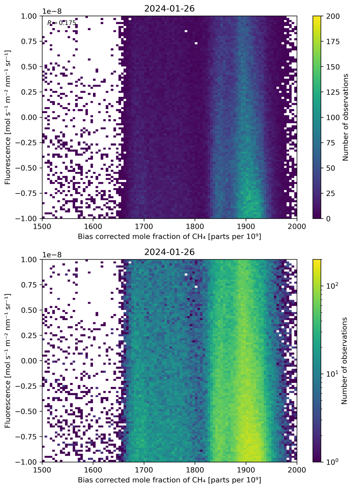
Figure 66: Scatter density plot of “Bias corrected mole fraction of \text{CH}_4 ” against “Fluorescence” for 2024-01-26 to 2024-01-27.
