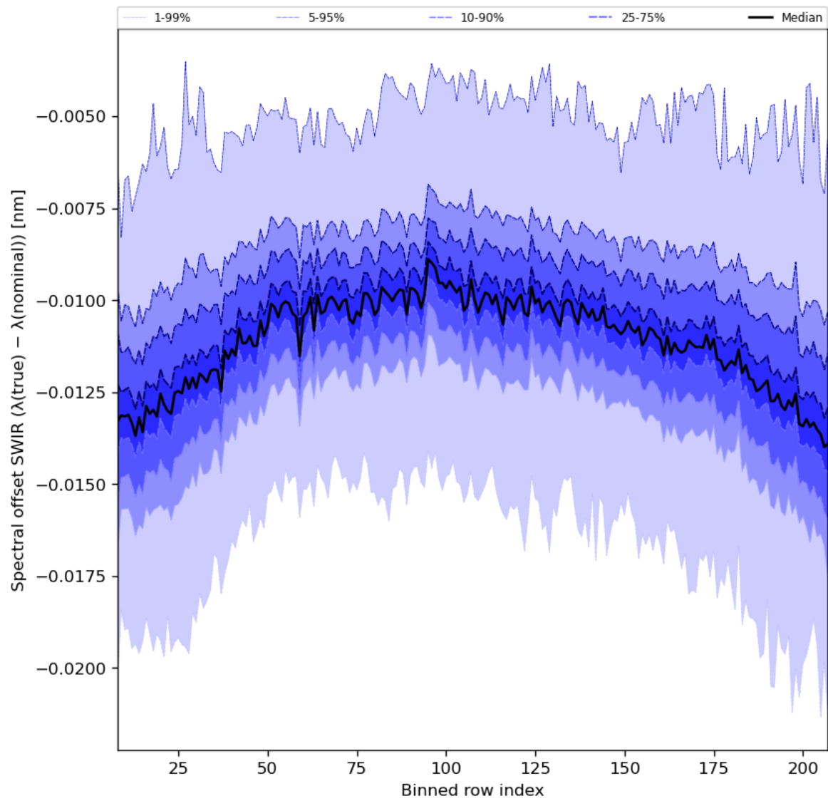
Figure 38: Along track statistics of “Spectral offset SWIR ( \lambda(\text{true}) - \lambda(\text{nominal}) )” for 2024-01-26 to 2024-01-27
