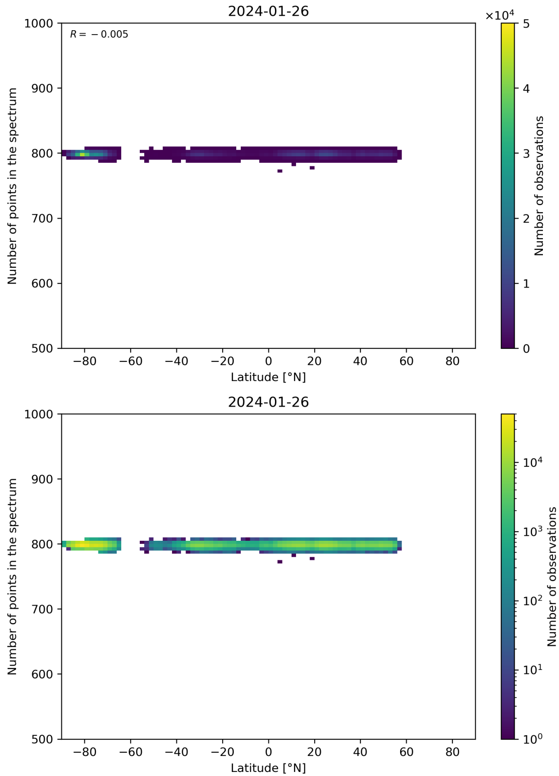
Figure 61: Scatter density plot of “Latitude” against “Number of points in the spectrum” for 2024-01-26 to 2024-01-27.
