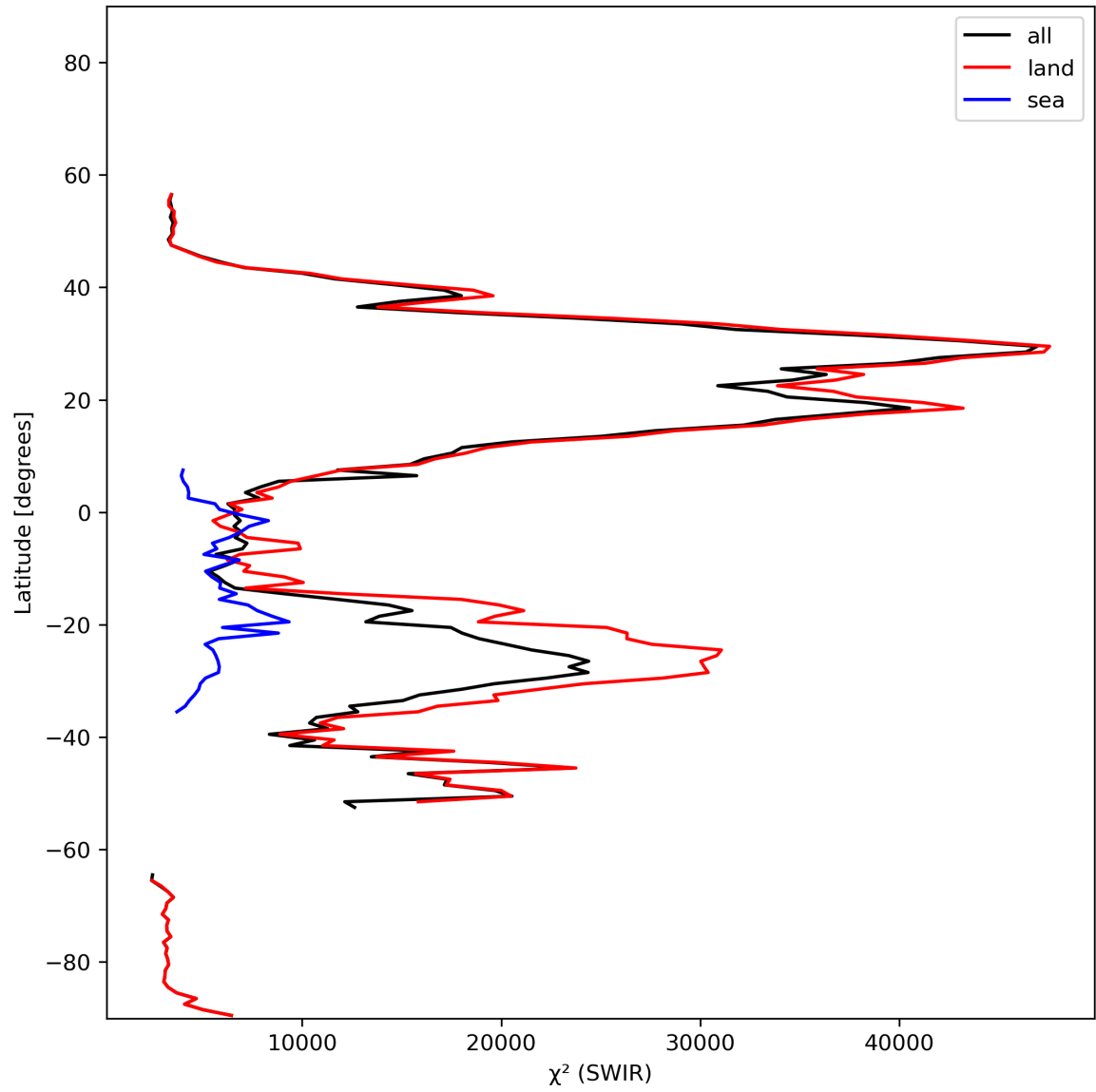
Figure 17: Zonal average of “ \chi^2 (SWIR)” for 2024-01-26 to 2024-01-27.
