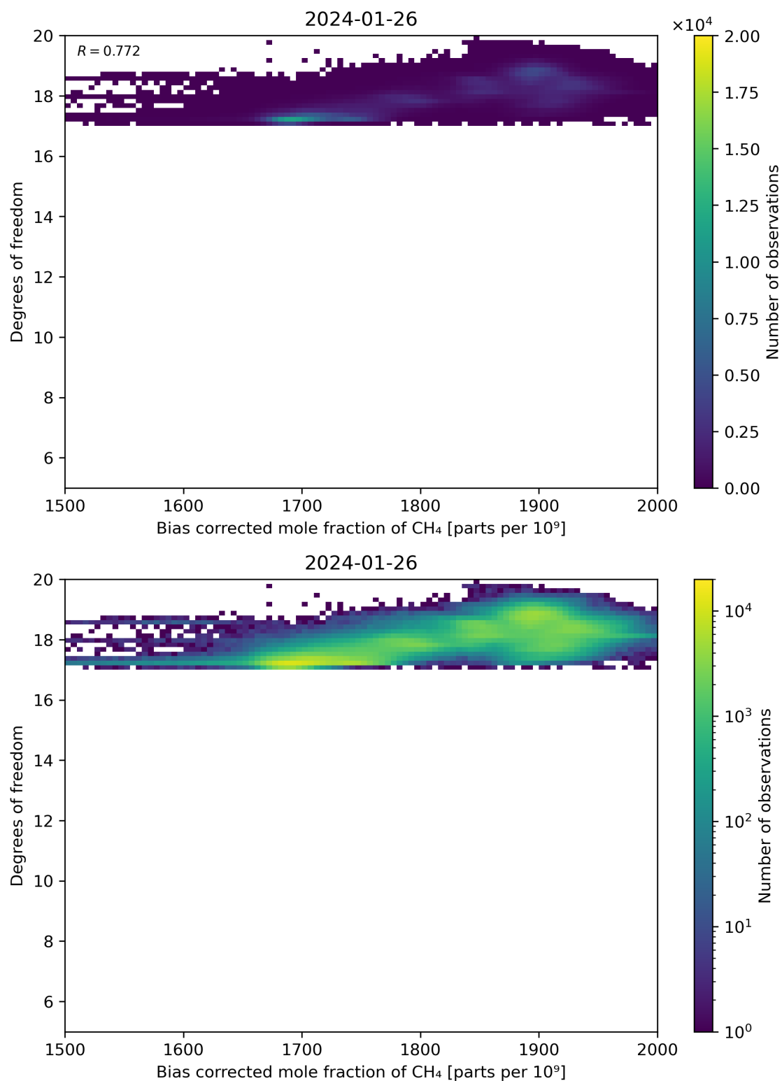
Figure 65: Scatter density plot of “Bias corrected mole fraction of CH 4 ” against “Degrees of freedom” for 2024-01-26 to 2024-01-27.
