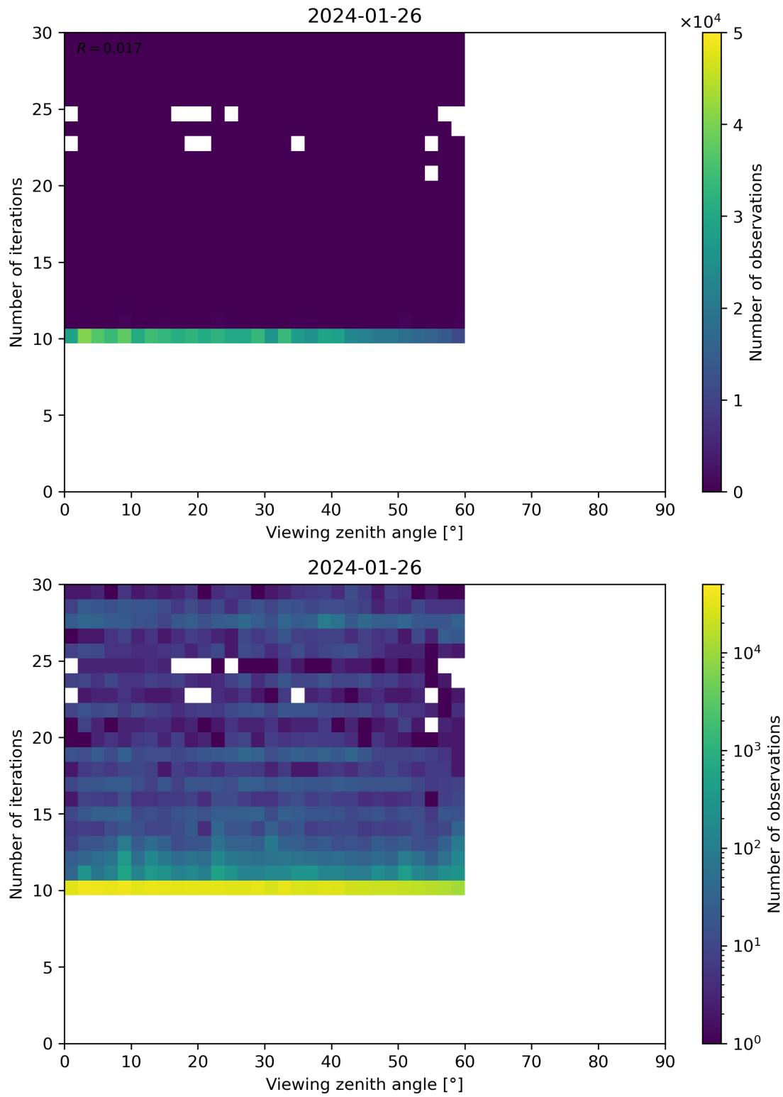
Figure 113: Scatter density plot of “Viewing zenith angle” against “Number of iterations” for 2024-01-26 to 2024-01-27.
