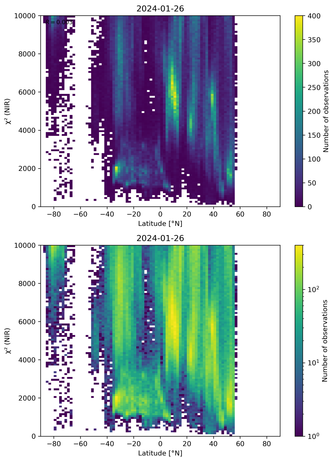
Figure 53: Scatter density plot of “Latitude” against “ \chi^2 (NIR)” for 2024-01-26 to 2024-01-27.
