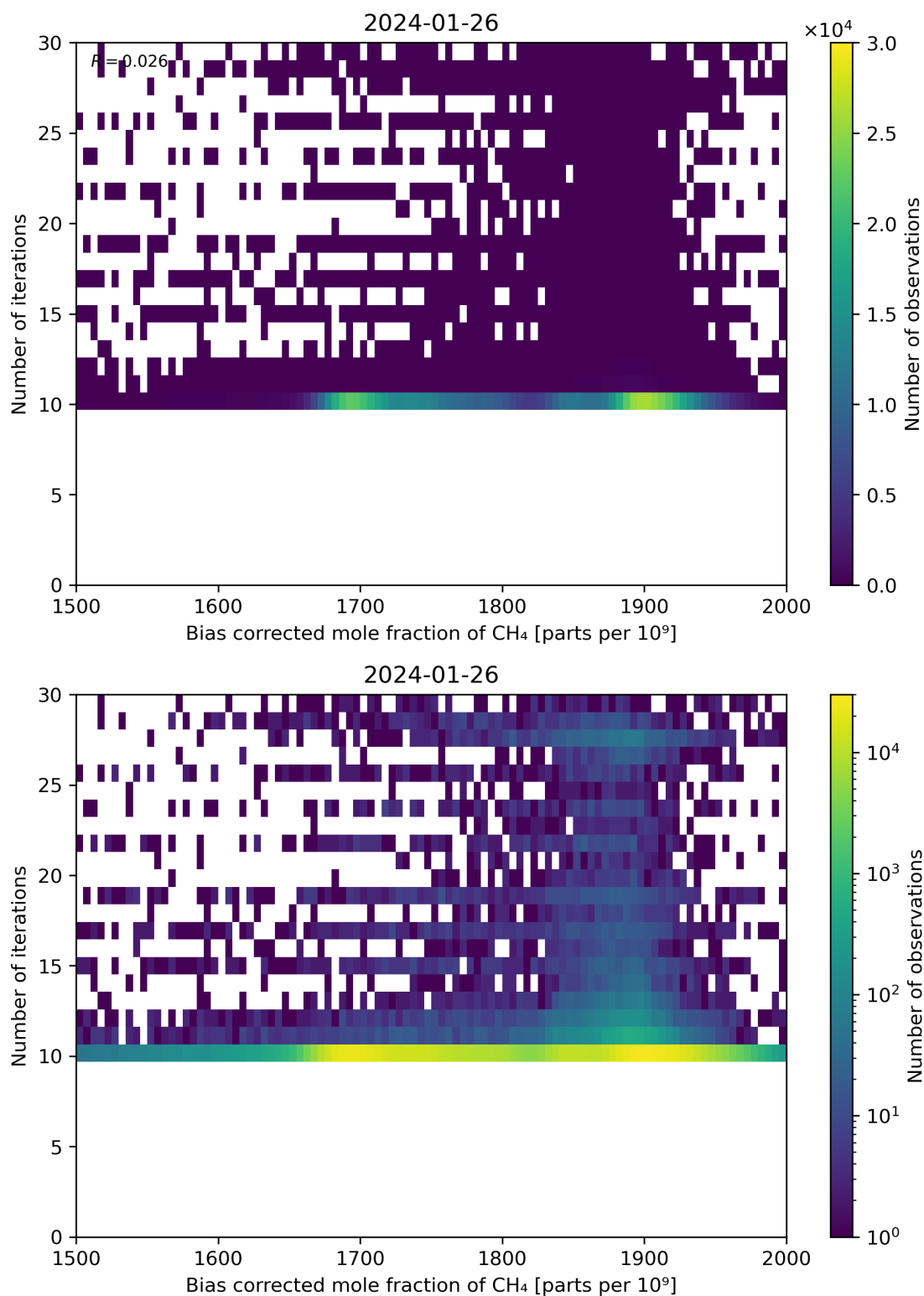
Figure 67: Scatter density plot of “Bias corrected mole fraction of CH 4 ” against “Number of iterations” for 2024-01-26 to 2024-01-27.
