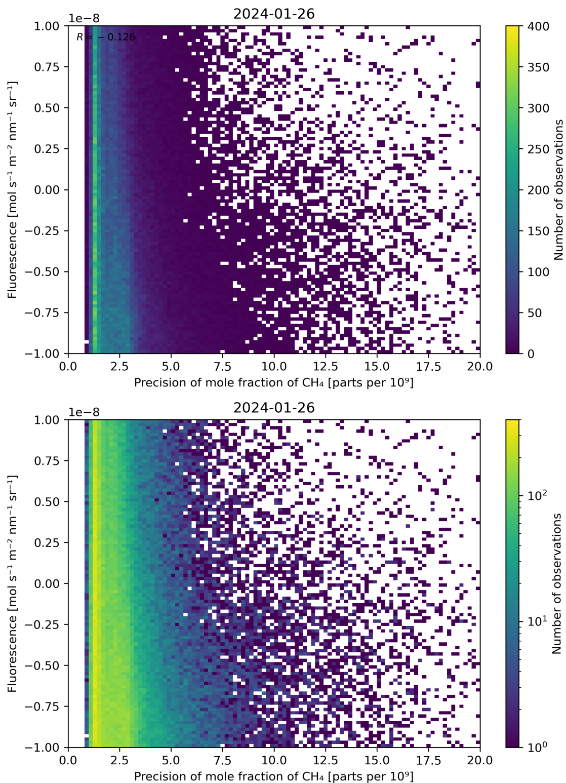
Figure 81: Scatter density plot of “Precision of mole fraction of \text{CH}_4 ” against “Fluorescence” for 2024-01-26 to 2024-01-27.
