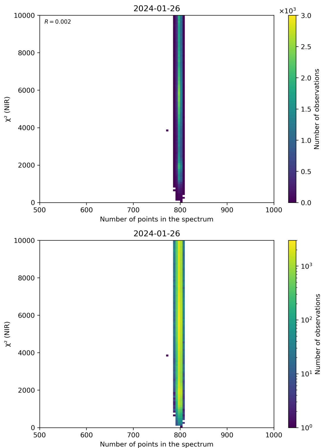
Figure 88: Scatter density plot of “Number of points in the spectrum” against “ \chi^2 (NIR)” for 2024-01-26 to 2024-01-27.
