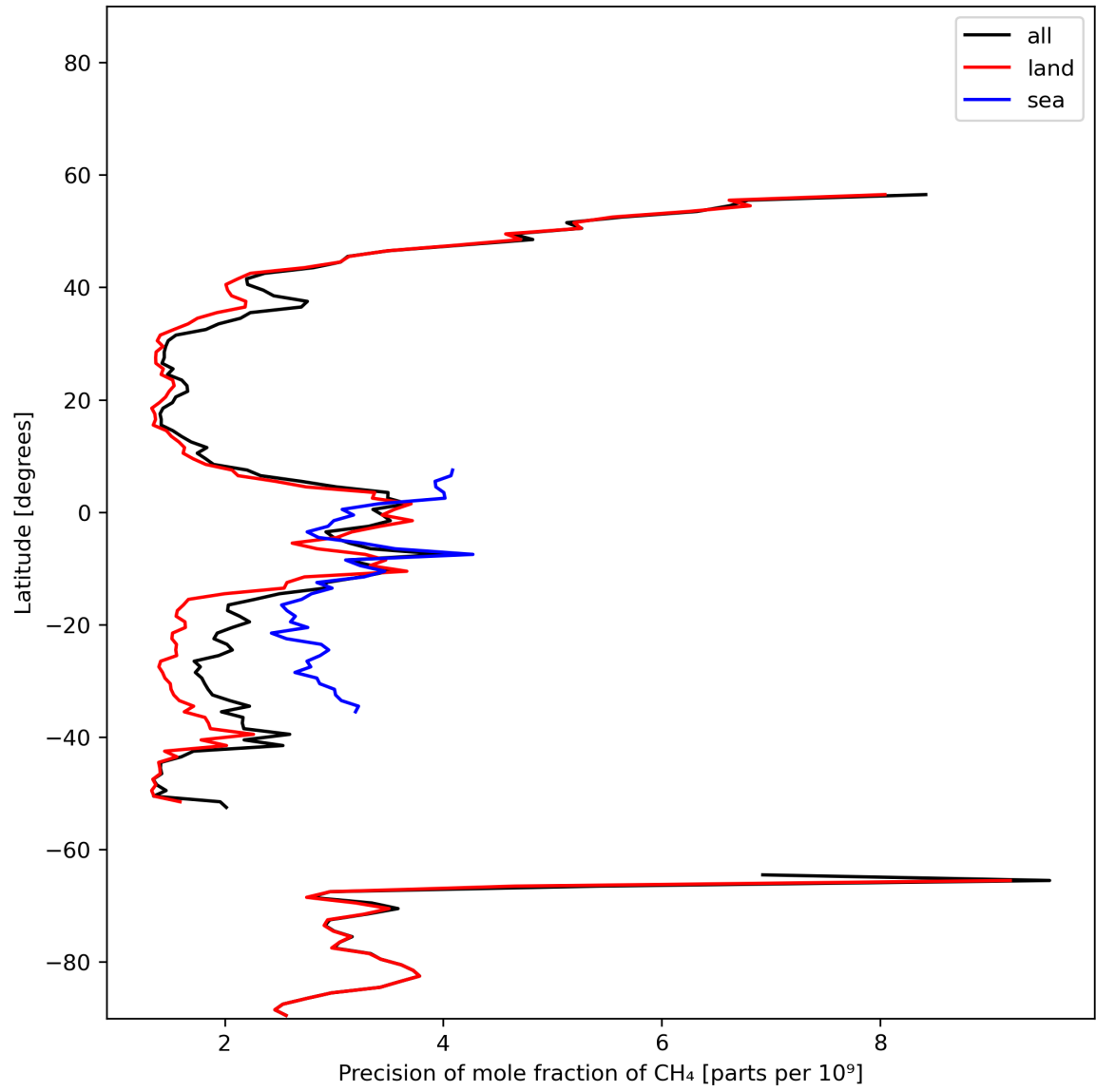
Figure 13: Zonal average of “Precision of mole fraction of CH 4 ” for 2024-01-26 to 2024-01-27.
