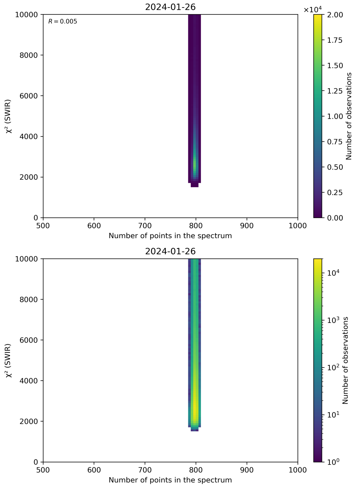
Figure 89: Scatter density plot of “Number of points in the spectrum” against “ \chi^2 (SWIR)” for 2024-01-26 to 2024-01-27.
