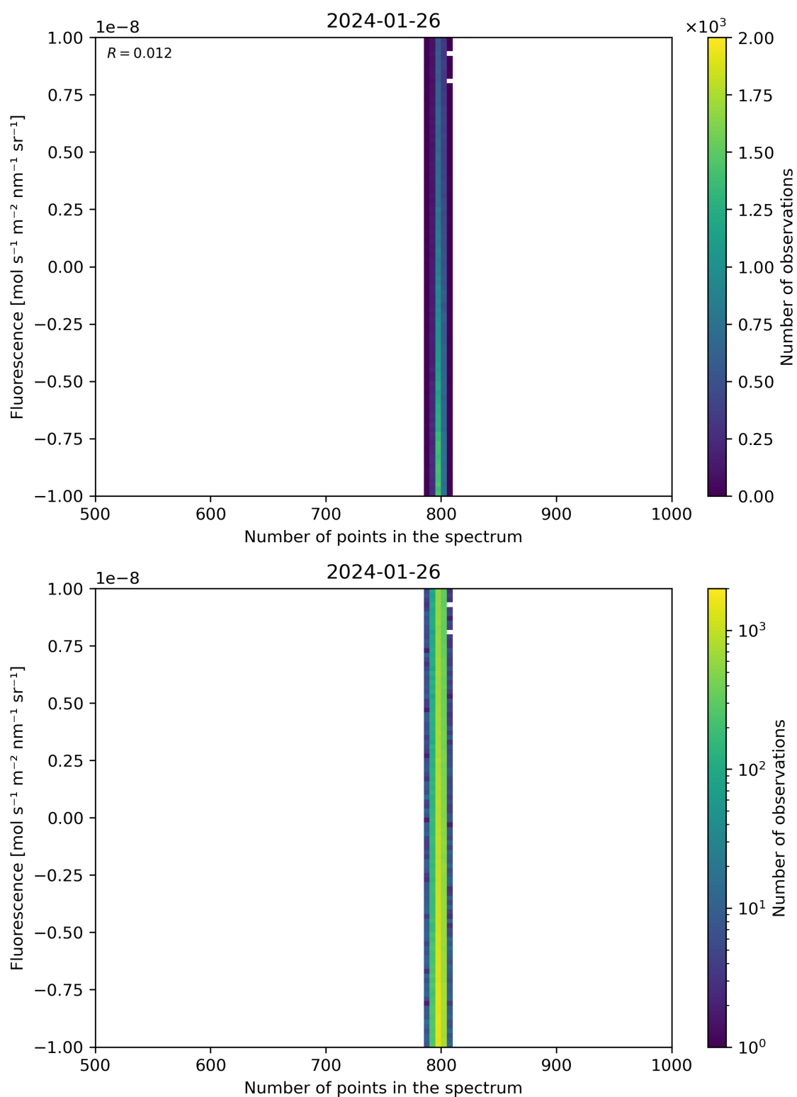
Figure 91: Scatter density plot of “Number of points in the spectrum” against “Fluorescence” for 2024-01-26 to 2024-01-27.
