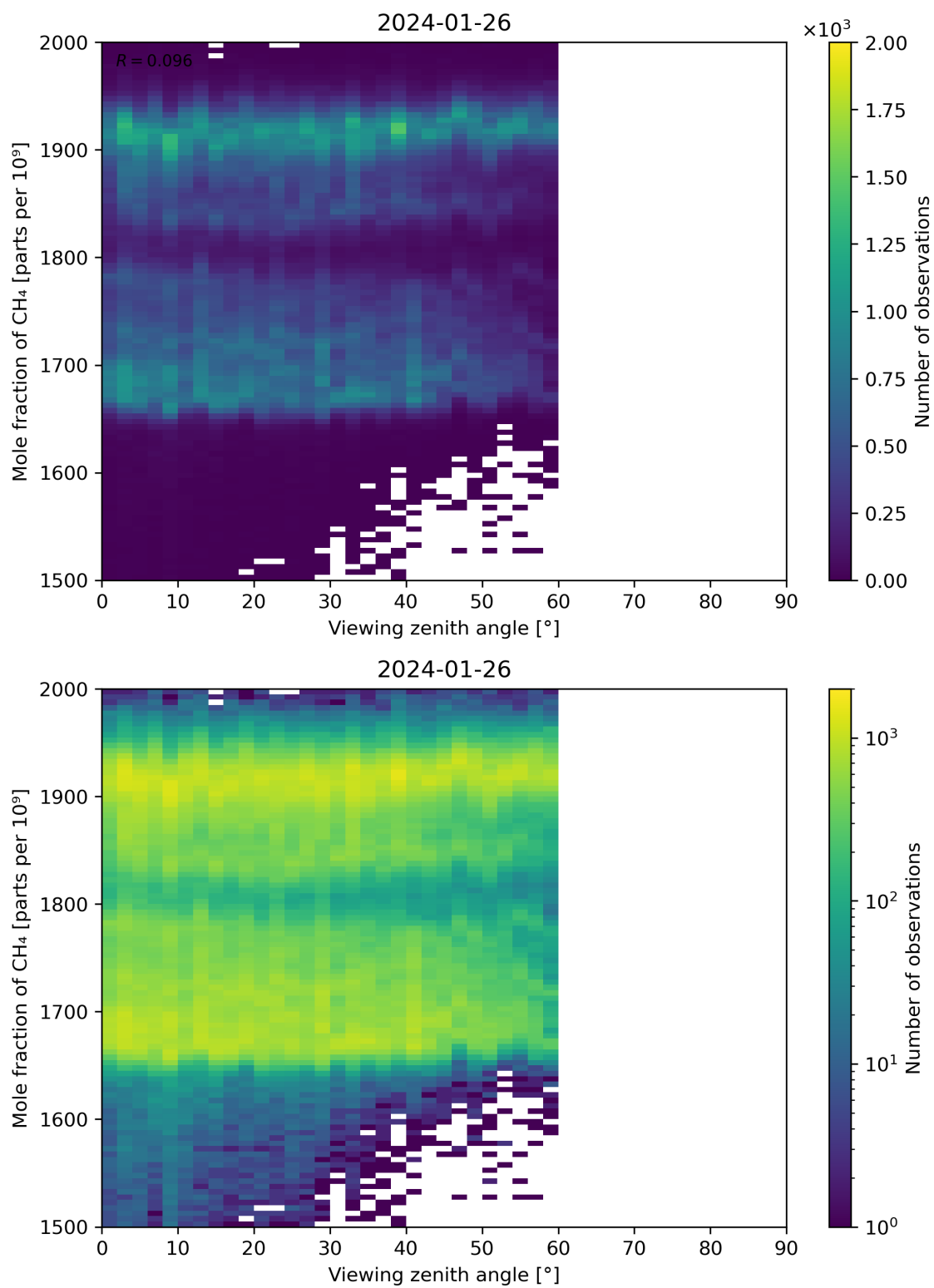
Figure 110: Scatter density plot of “Viewing zenith angle” against “Mole fraction of \text{CH}_4 ” for 2024-01-26 to 2024-01-27.
