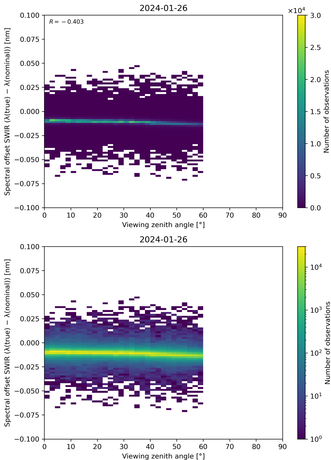
Figure 116: Scatter density plot of “Viewing zenith angle” against “Spectral offset SWIR ( \lambda(\text{true}) - \lambda(\text{nominal}) )” for 2024-01-26 to 2024-01-27.
