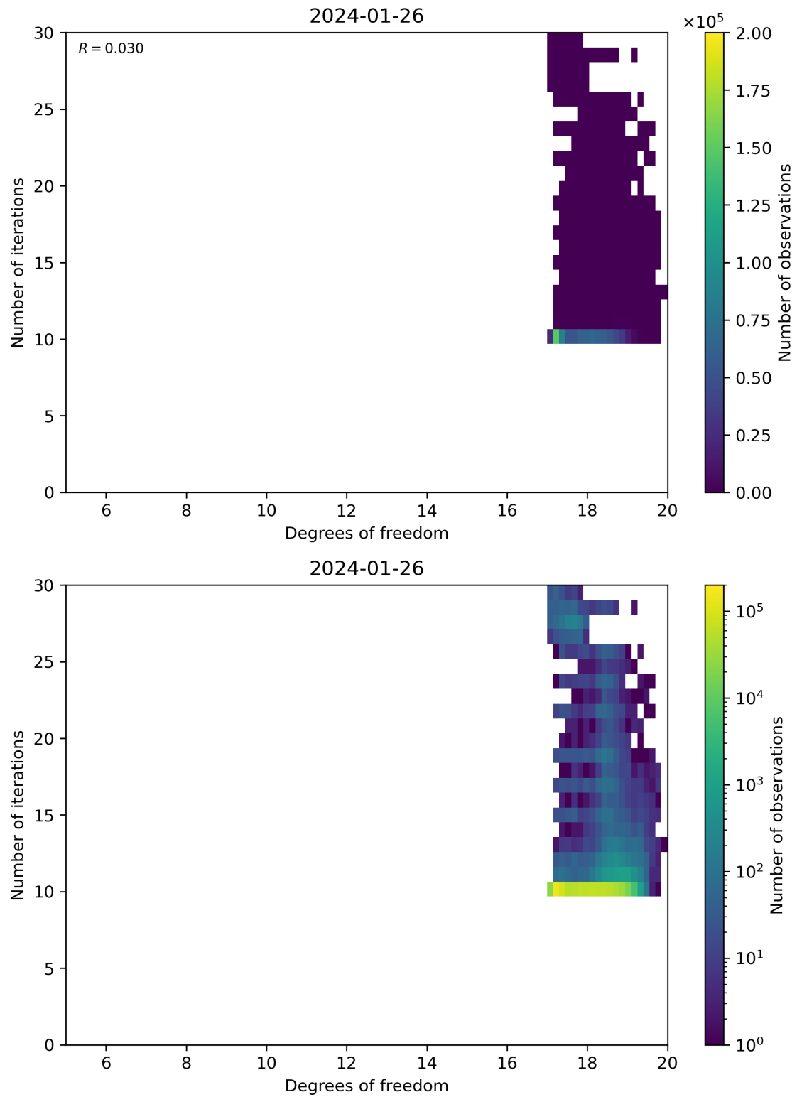
Figure 52: Scatter density plot of “Degrees of freedom” against “Number of iterations” for 2024-01-26 to 2024-01-27.
