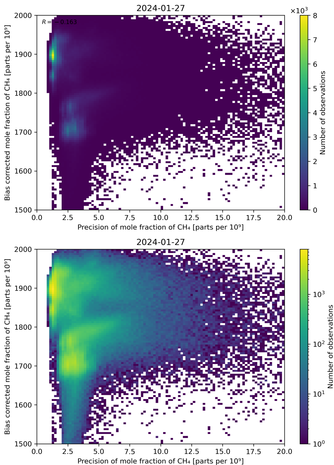
Figure 82: Scatter density plot of “Precision of mole fraction of \text{CH}_4 ” against “Bias corrected mole fraction of \text{CH}_4 ” for 2024-01-26 to 2024-01-28.
