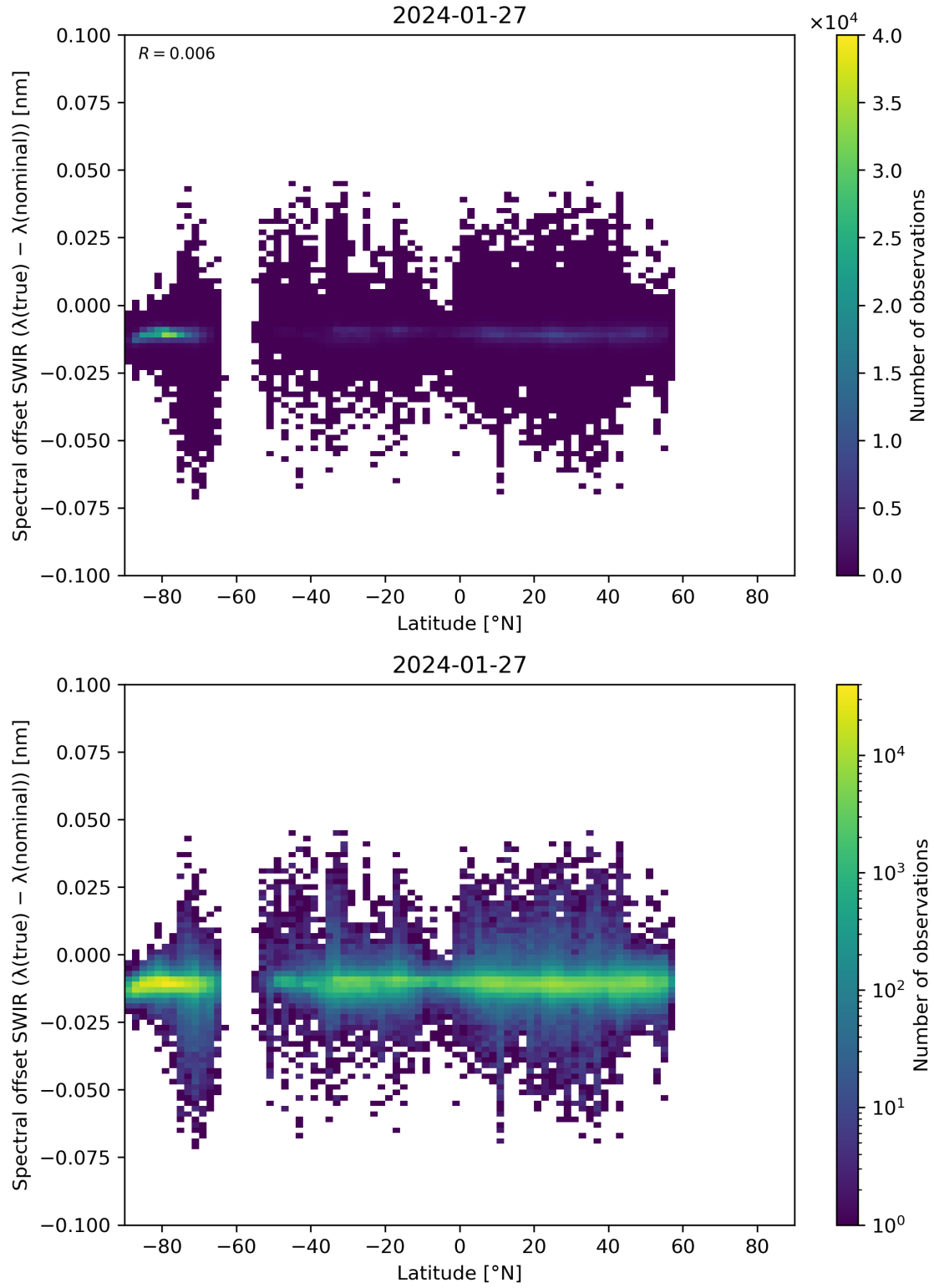
Figure 62: Scatter density plot of “Latitude” against “Spectral offset SWIR ( \lambda(\text{true}) - \lambda(\text{nominal}) )” for 2024-01-26 to 2024-01-28.
