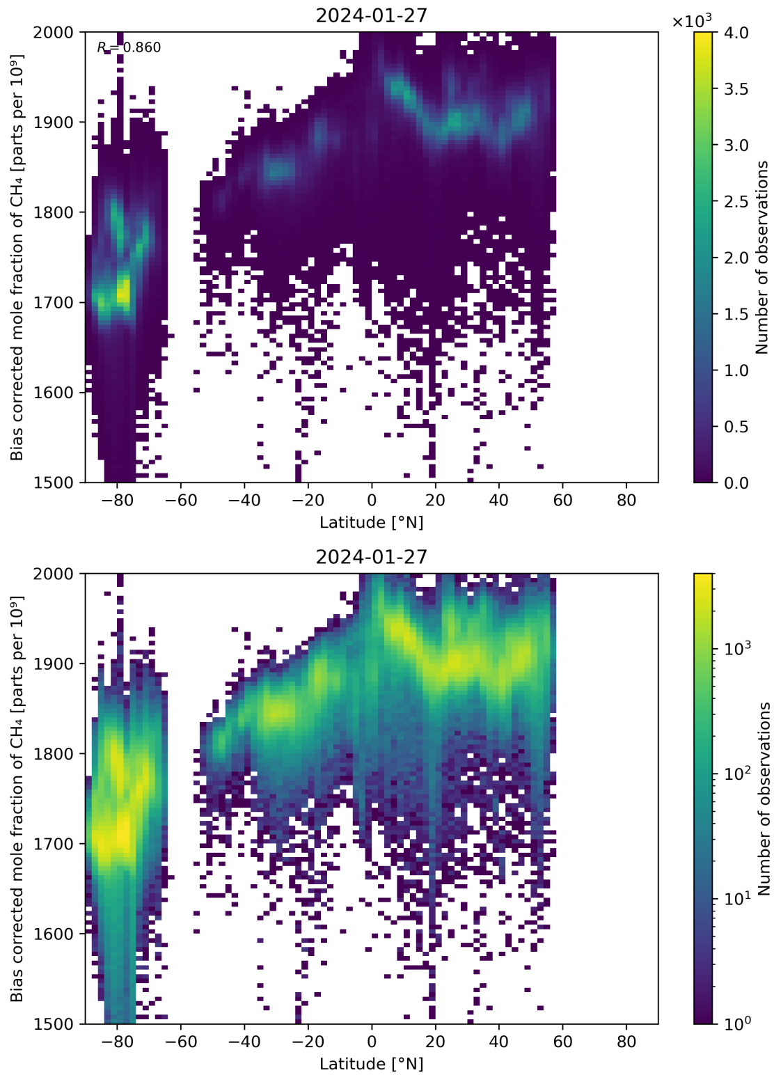
Figure 58: Scatter density plot of “Latitude” against “Bias corrected mole fraction of CH 4 ” for 2024-01-26 to 2024-01-28.
