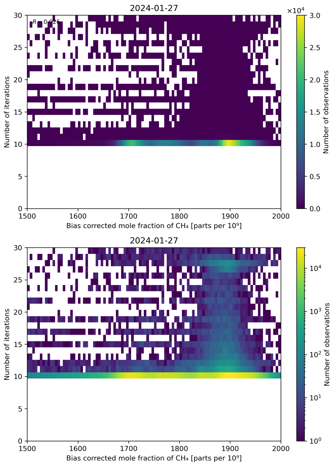
Figure 67: Scatter density plot of “Bias corrected mole fraction of \text{CH}_4 ” against “Number of iterations” for 2024-01-26 to 2024-01-28.
