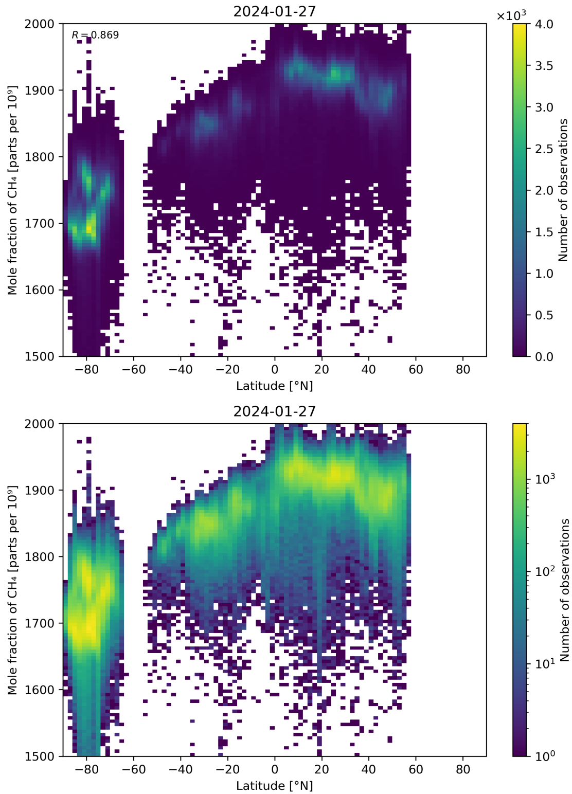
Figure 57: Scatter density plot of “Latitude” against “Mole fraction of CH 4 ” for 2024-01-26 to 2024-01-28.
