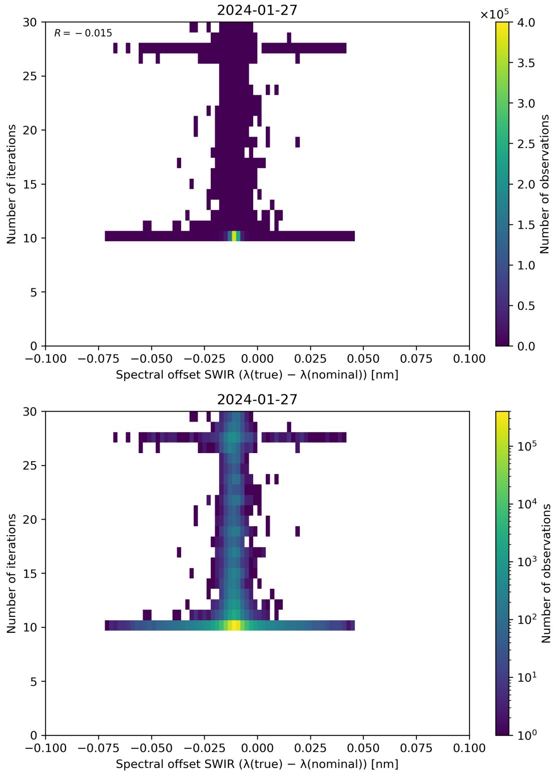
Figure 121: Scatter density plot of “Spectral offset SWIR ( \lambda(\text{true}) - \lambda(\text{nominal}) )” against “Number of iterations” for 2024-01-26 to 2024-01-28.
