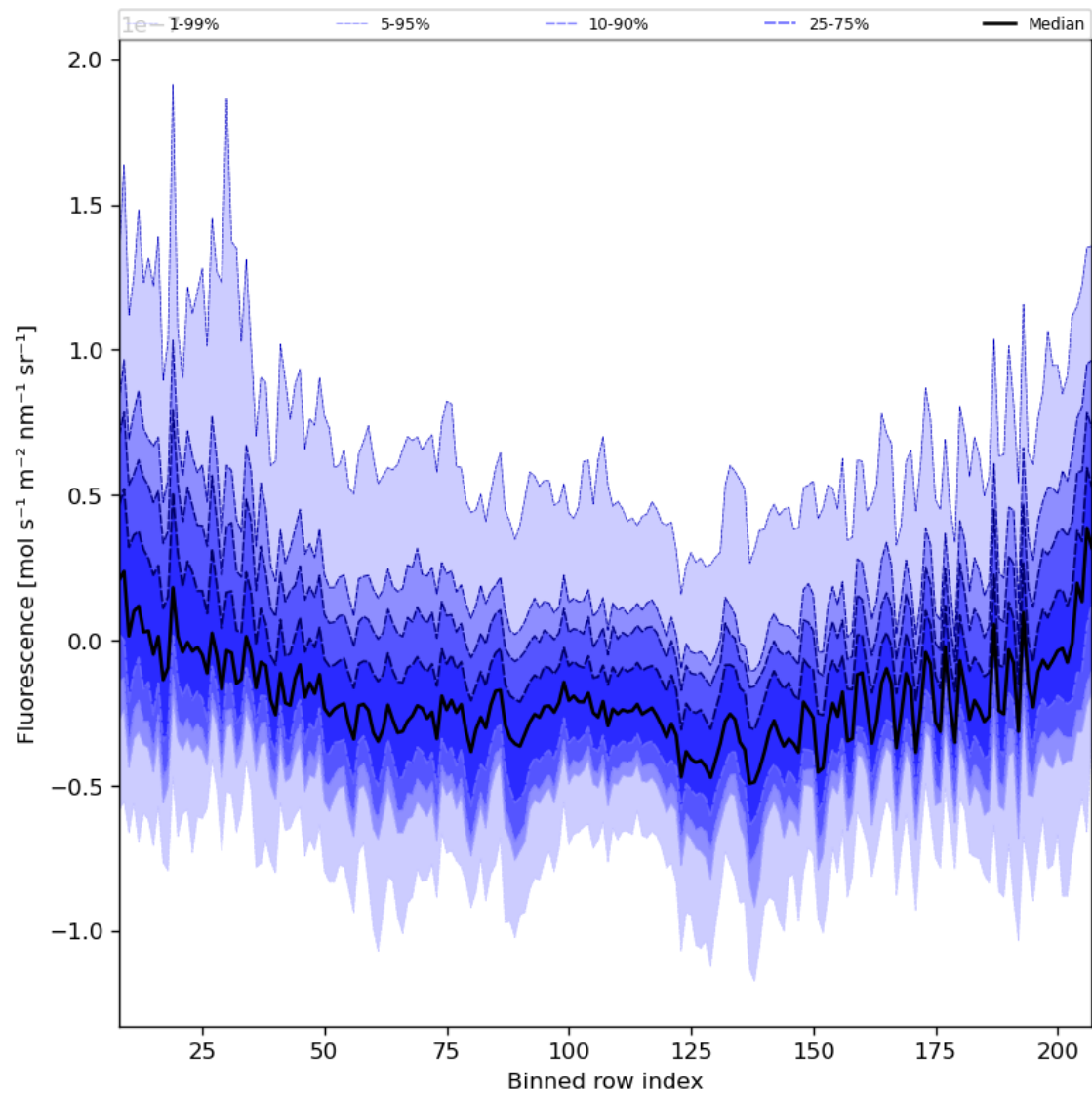
Figure 43: Along track statistics of “Fluorescence” for 2024-01-26 to 2024-01-28
