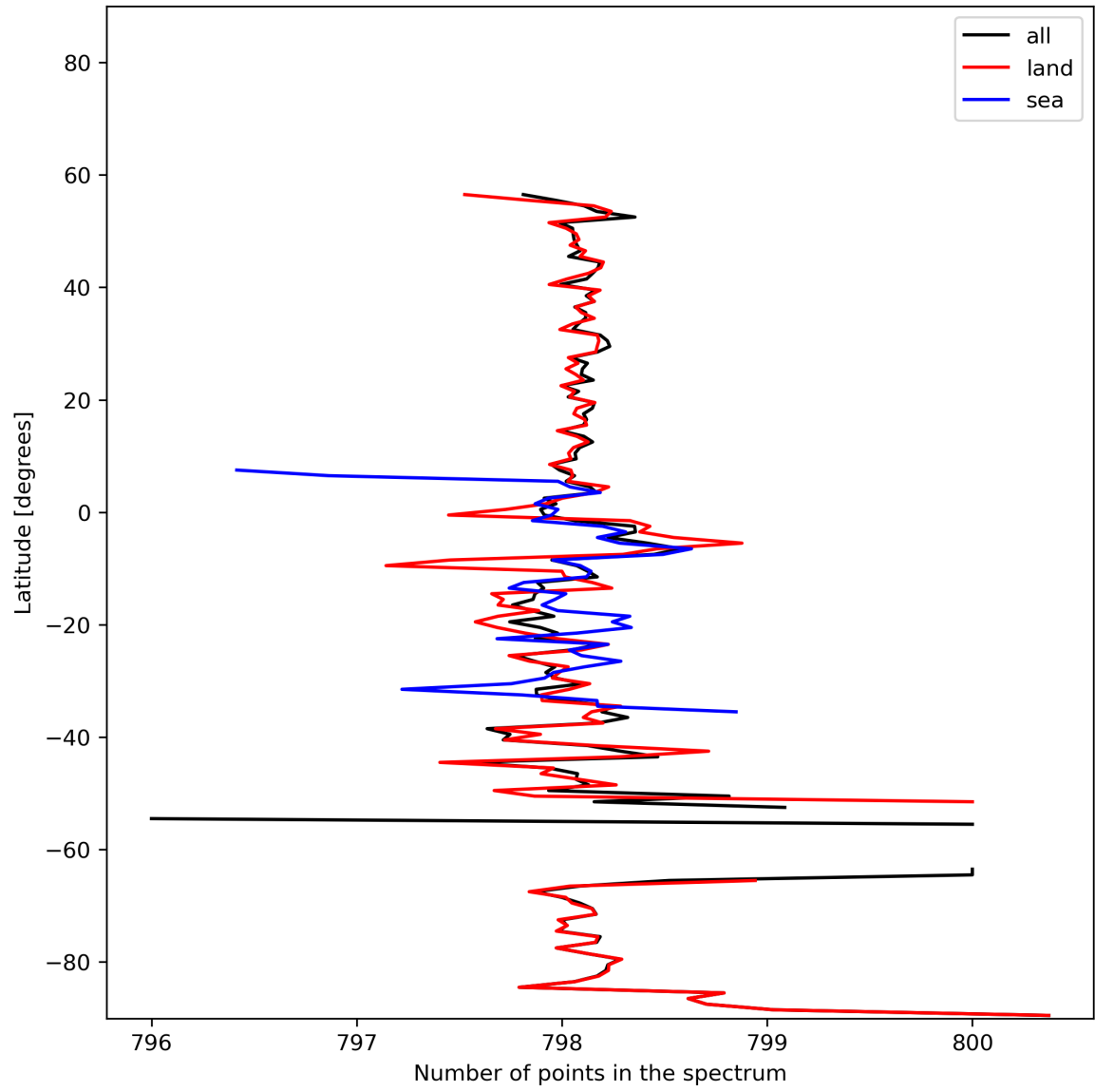
Figure 15: Zonal average of “Number of points in the spectrum” for 2024-01-26 to 2024-01-28.
