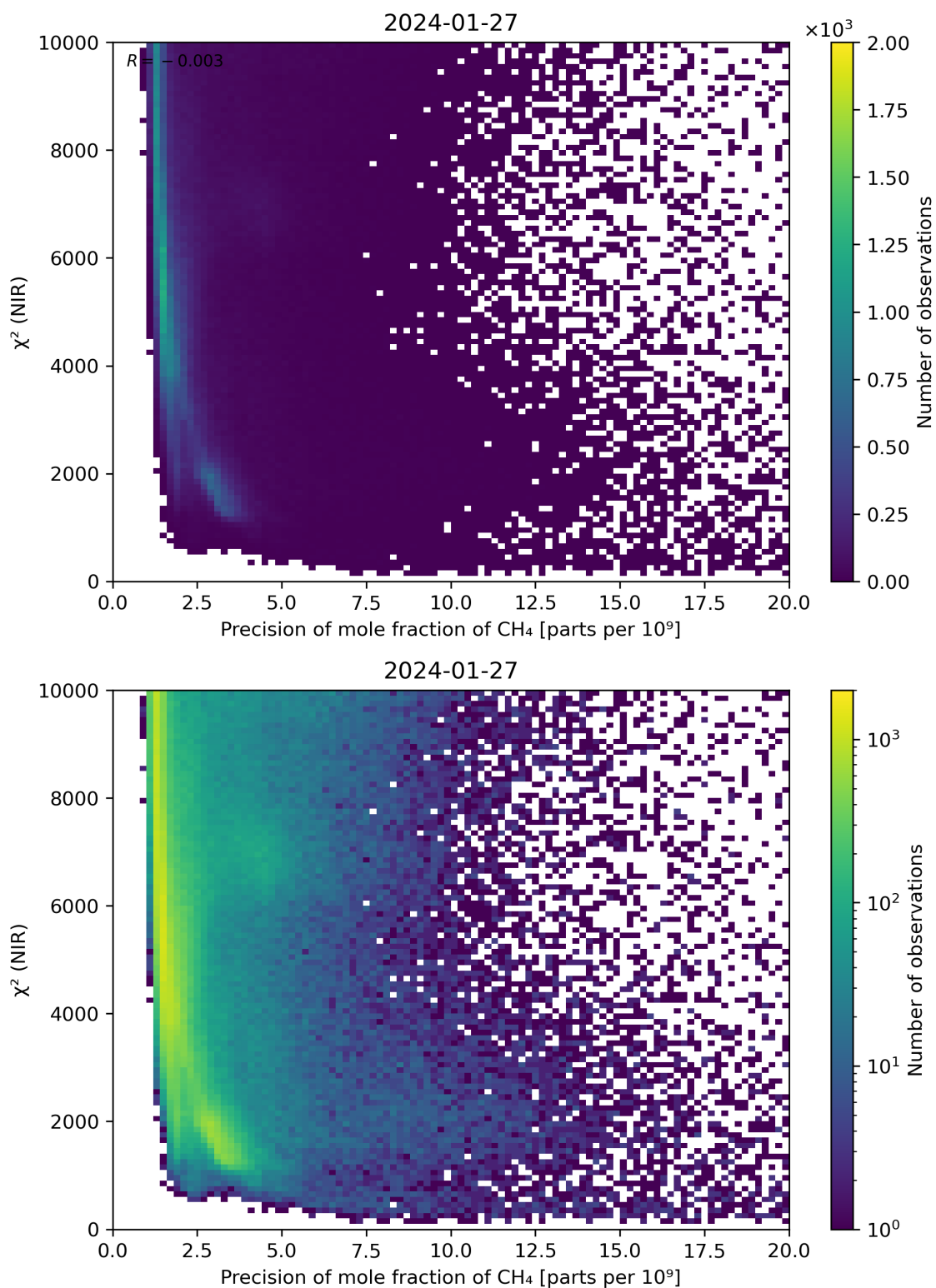
Figure 78: Scatter density plot of “Precision of mole fraction of CH 4 ” against “ \chi^2 (NIR)” for 2024-01-26 to 2024-01-28.
