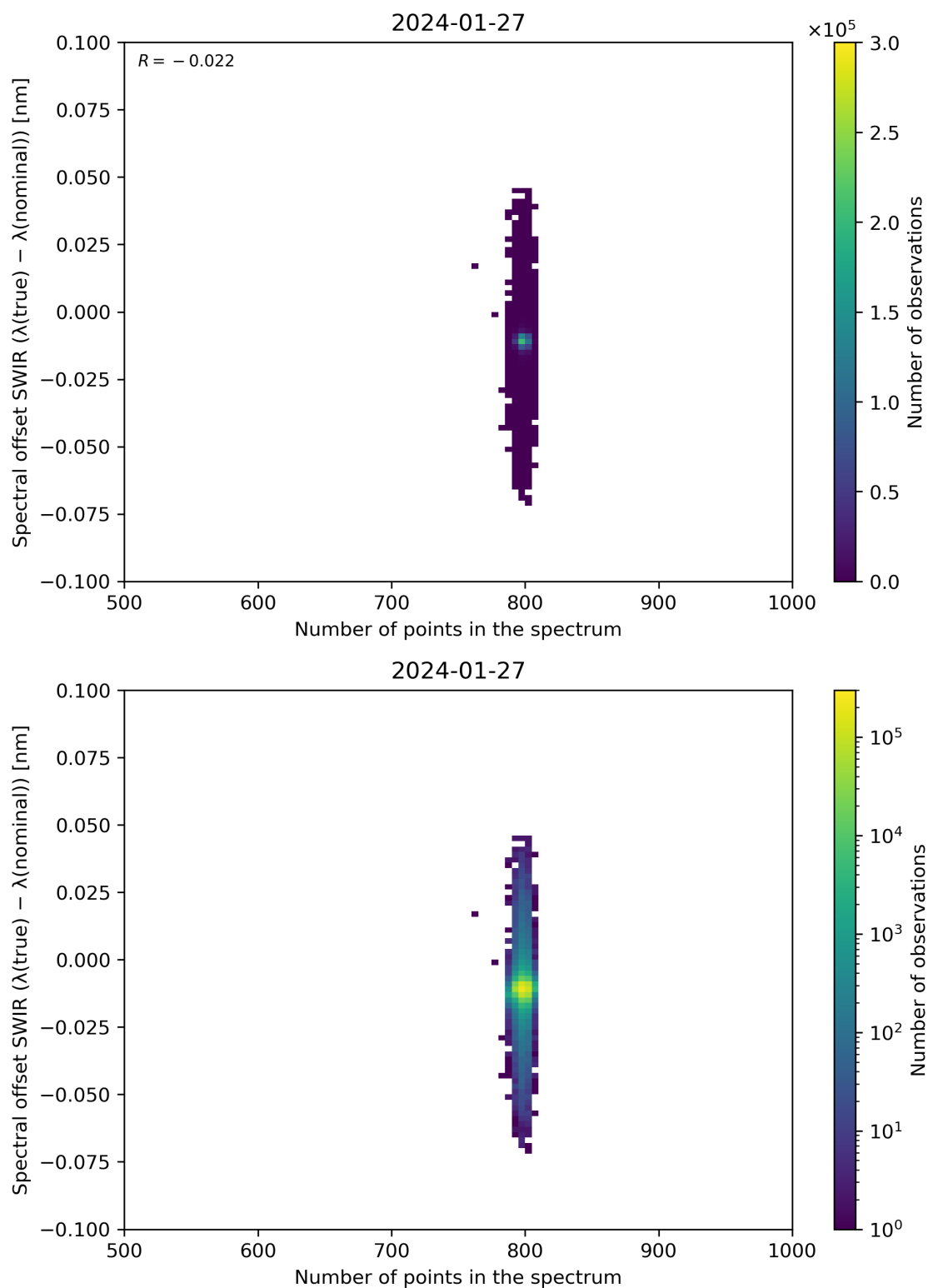
Figure 93: Scatter density plot of “Number of points in the spectrum” against “Spectral offset SWIR ( \lambda(\text{true}) - \lambda(\text{nominal}) )” for 2024-01-26 to 2024-01-28.
