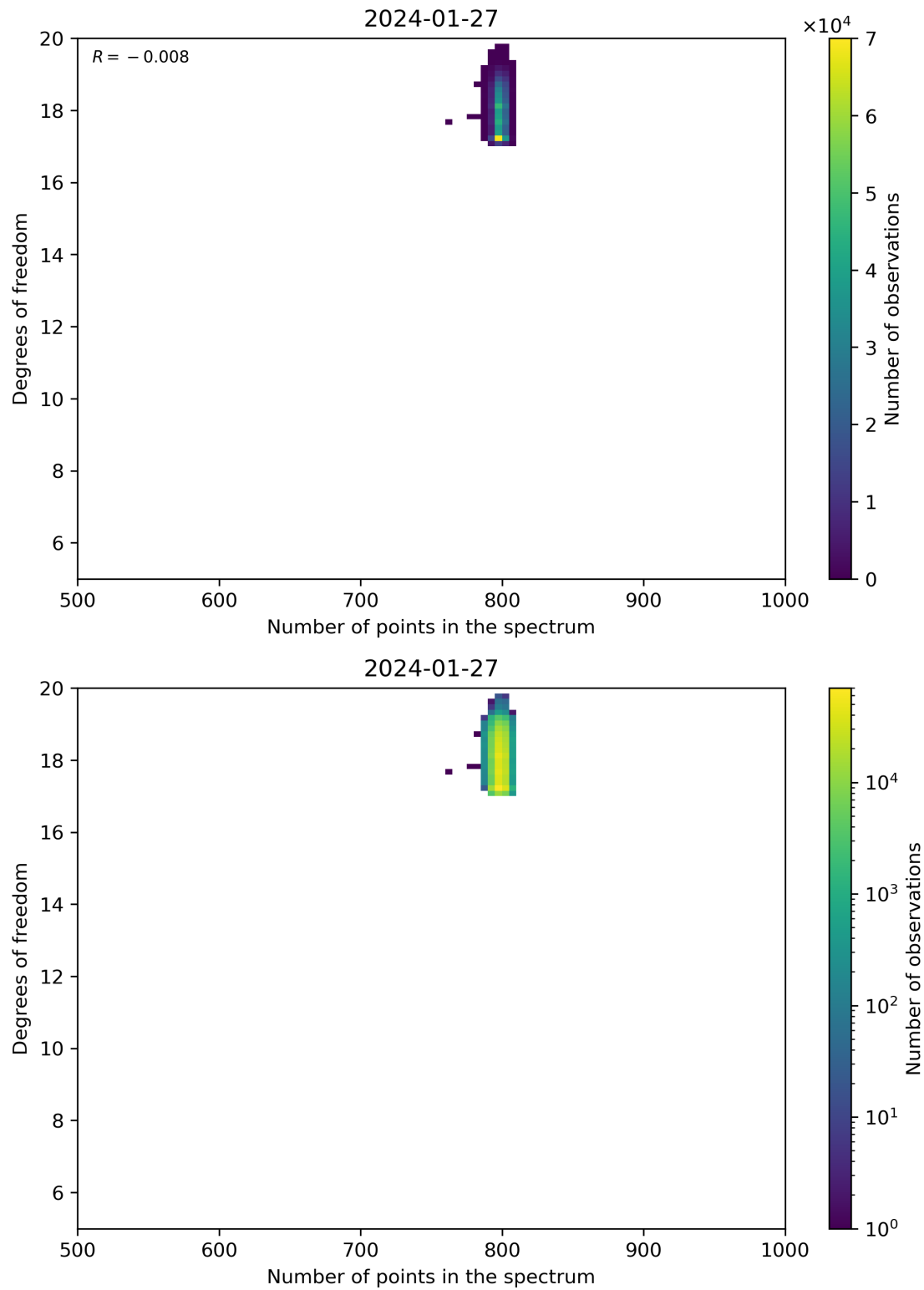
Figure 90: Scatter density plot of “Number of points in the spectrum” against “Degrees of freedom” for 2024-01-26 to 2024-01-28.
