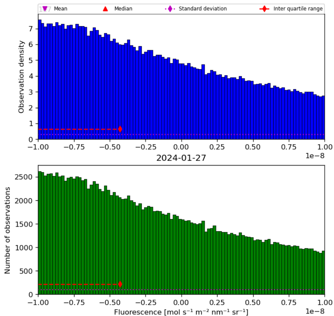
Figure 32: Histogram of “Fluorescence” for 2024-01-26 to 2024-01-28
