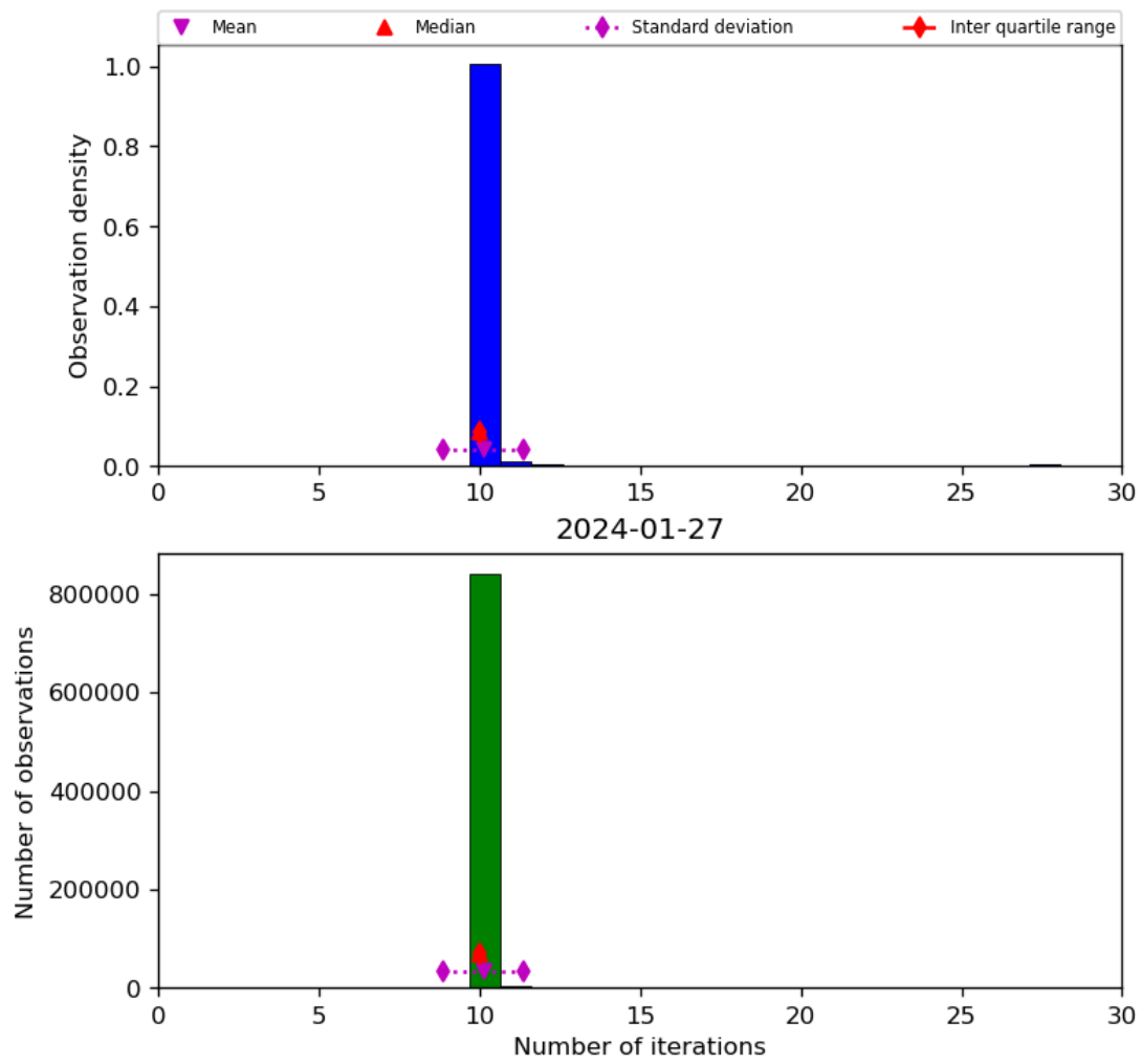
Figure 31: Histogram of “Number of iterations” for 2024-01-26 to 2024-01-28
