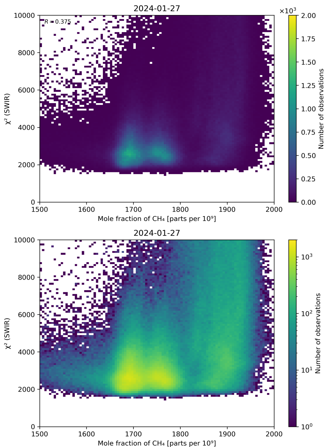
Figure 71: Scatter density plot of “Mole fraction of \text{CH}_4 ” against “ \chi^2 (SWIR)” for 2024-01-26 to 2024-01-28.
