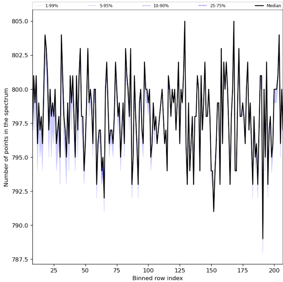
Figure 37: Along track statistics of “Number of points in the spectrum” for 2024-01-26 to 2024-01-28
