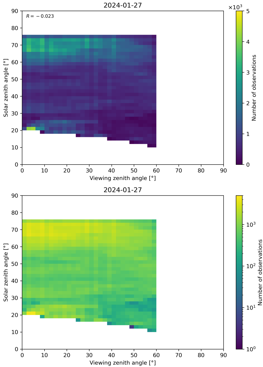
Figure 115: Scatter density plot of “Viewing zenith angle” against “Solar zenith angle” for 2024-01-26 to 2024-01-28.
