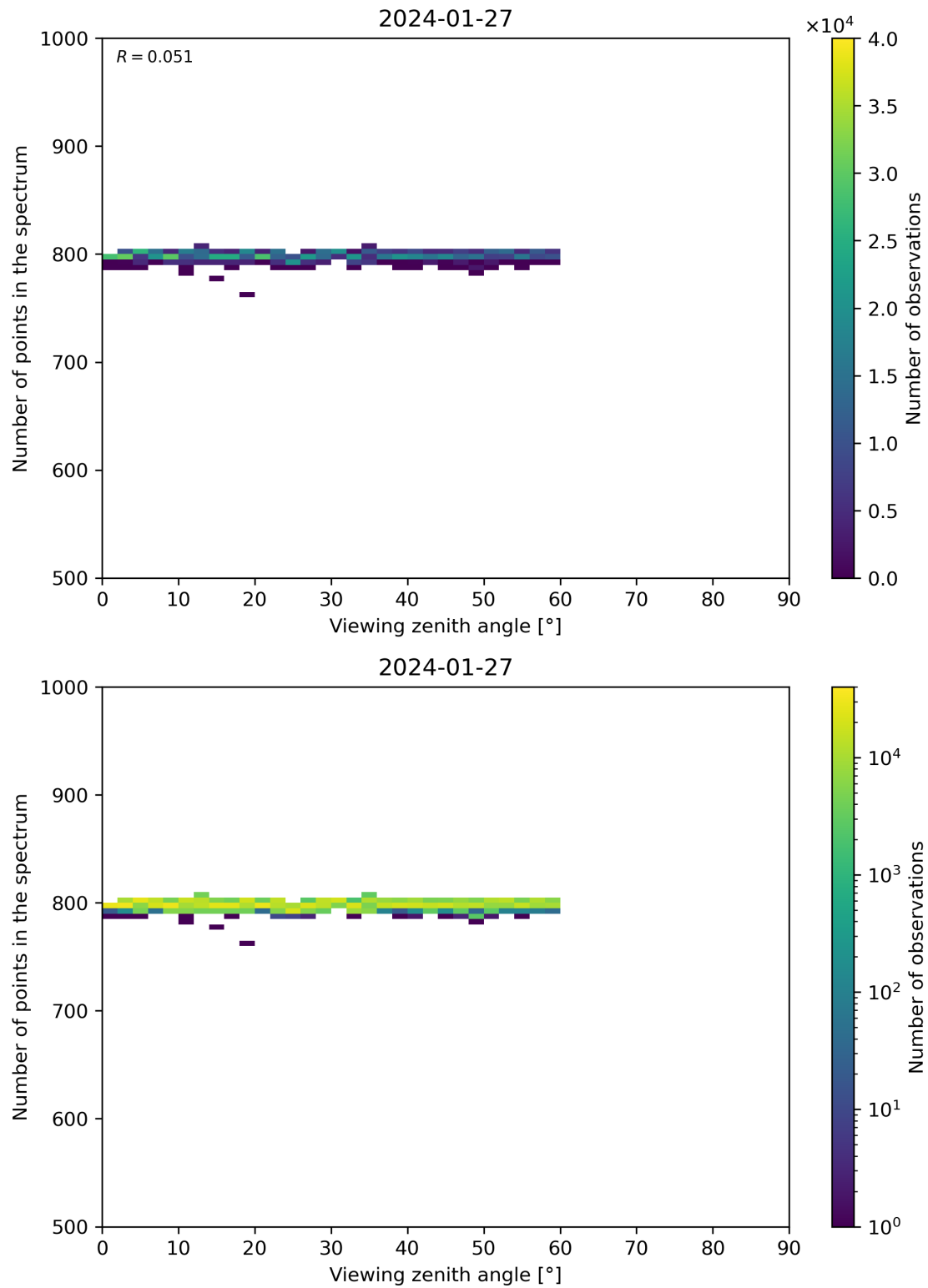
Figure 114: Scatter density plot of “Viewing zenith angle” against “Number of points in the spectrum” for 2024-01-26 to 2024-01-28.
