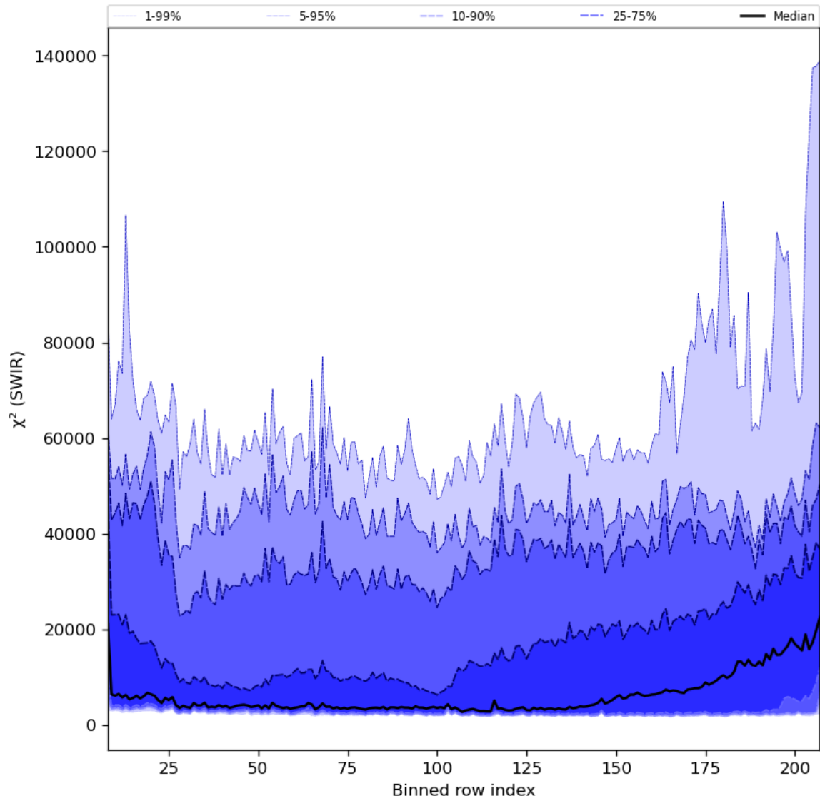
Figure 39: Along track statistics of “ \chi^2 (SWIR)” for 2024-01-26 to 2024-01-28
