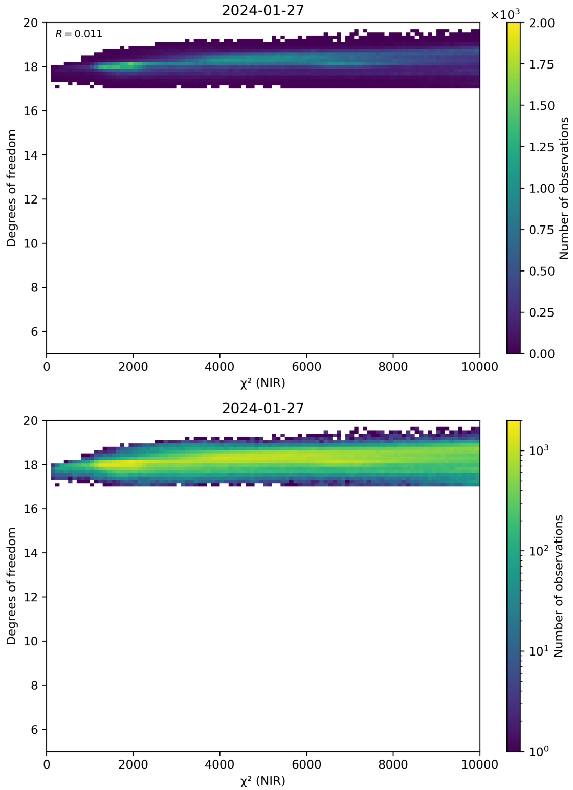
Figure 44: Scatter density plot of “ \chi^2 (NIR)” against “Degrees of freedom” for 2024-01-26 to 2024-01-28.
