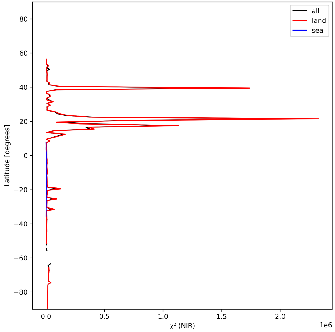
Figure 18: Zonal average of “ \chi^2 (NIR)” for 2024-01-26 to 2024-01-28.
