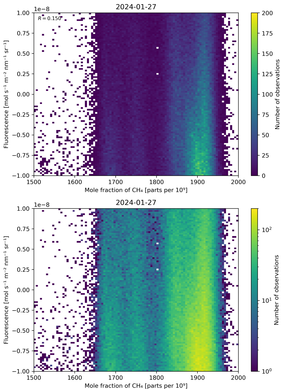
Figure 73: Scatter density plot of “Mole fraction of \text{CH}_4 ” against “Fluorescence” for 2024-01-26 to 2024-01-28.
