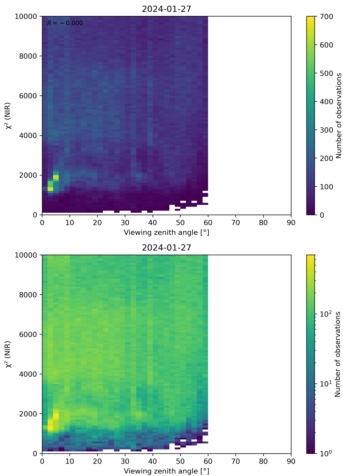
Figure 105: Scatter density plot of “Viewing zenith angle” against “ \chi^2 (NIR)” for 2024-01-26 to 2024-01-28.
