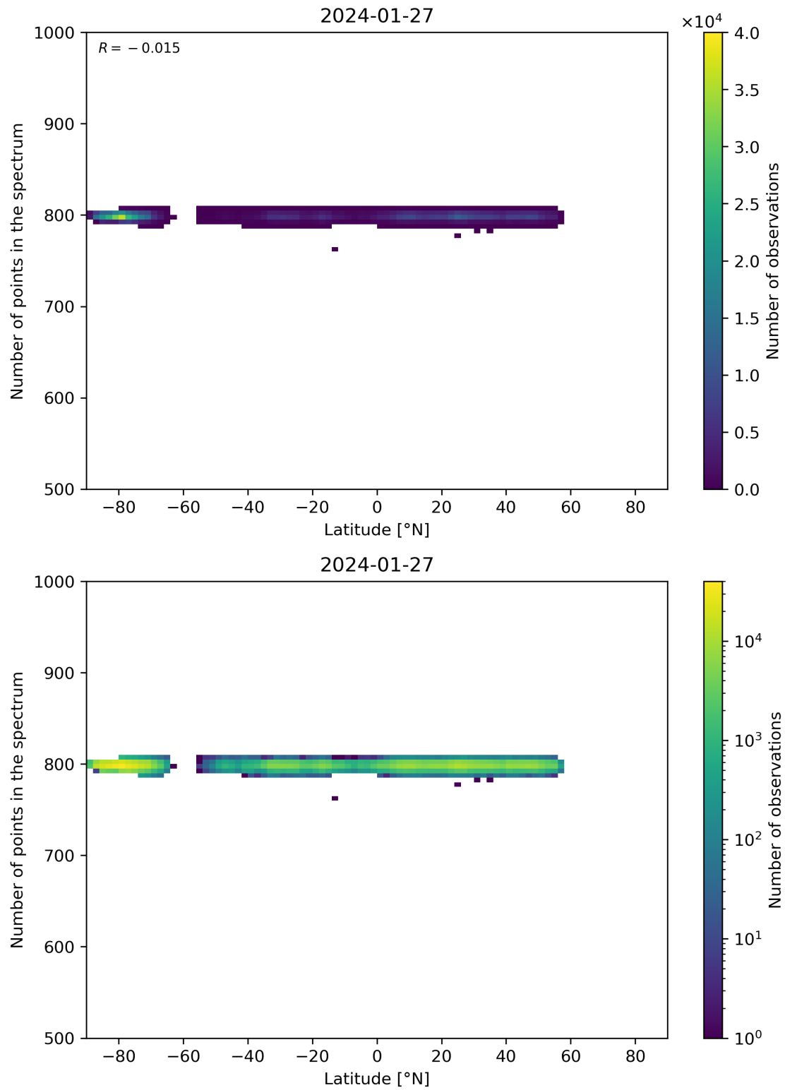
Figure 61: Scatter density plot of “Latitude” against “Number of points in the spectrum” for 2024-01-26 to 2024-01-28.
