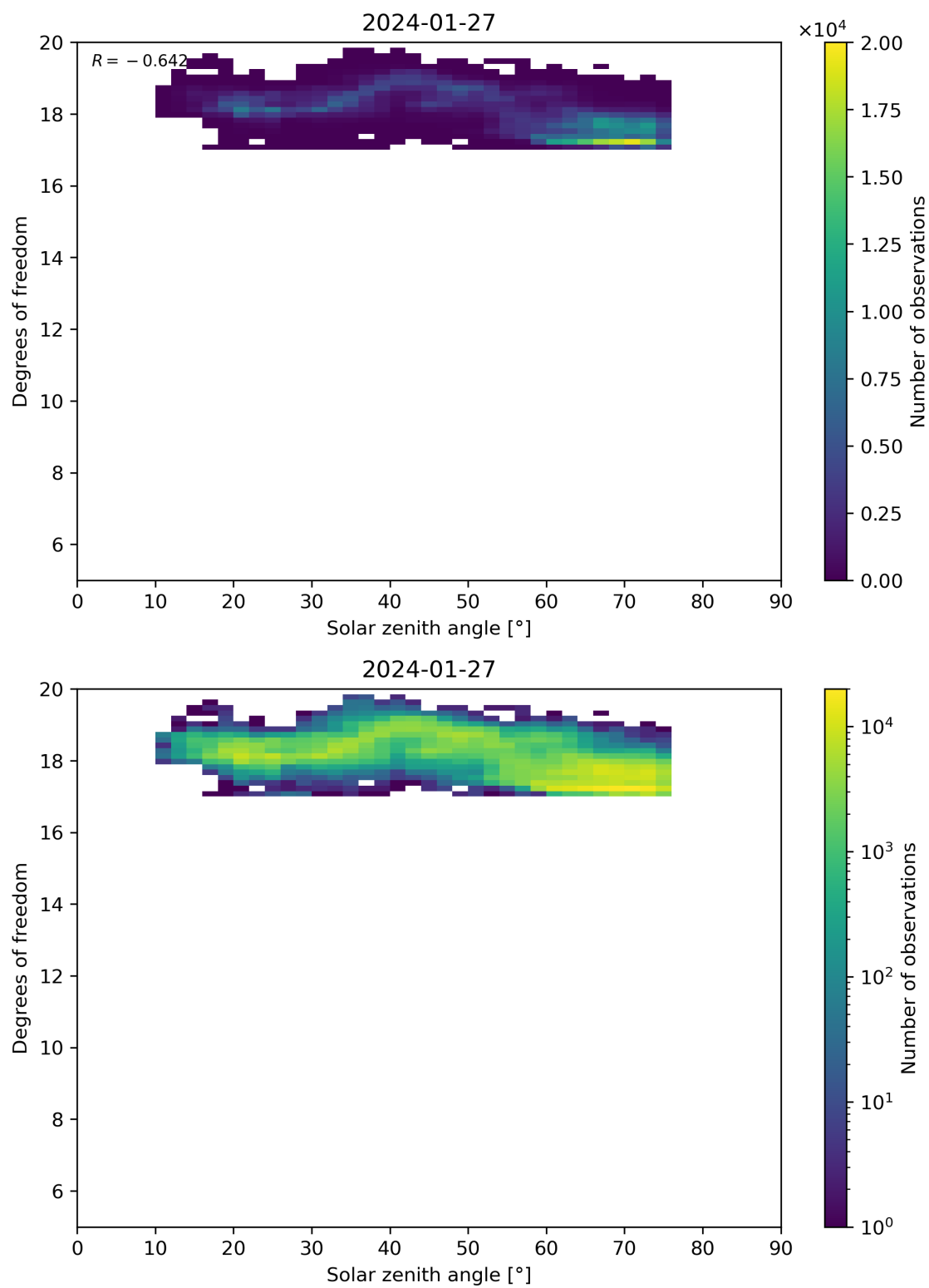
Figure 96: Scatter density plot of “Solar zenith angle” against “Degrees of freedom” for 2024-01-26 to 2024-01-28.
