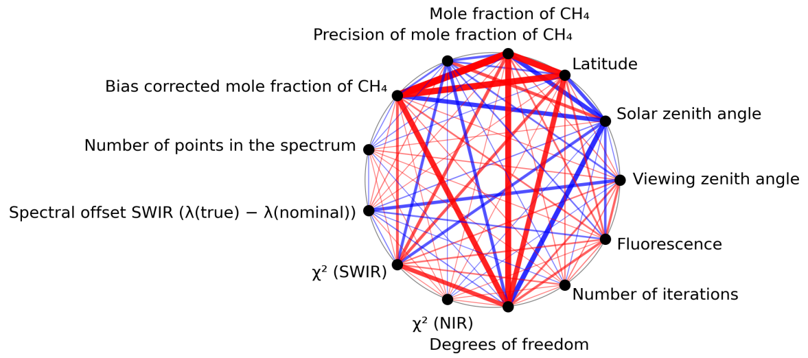
Figure 1: Map of correlation graph for 2024-01-26 to 2024-01-28.
