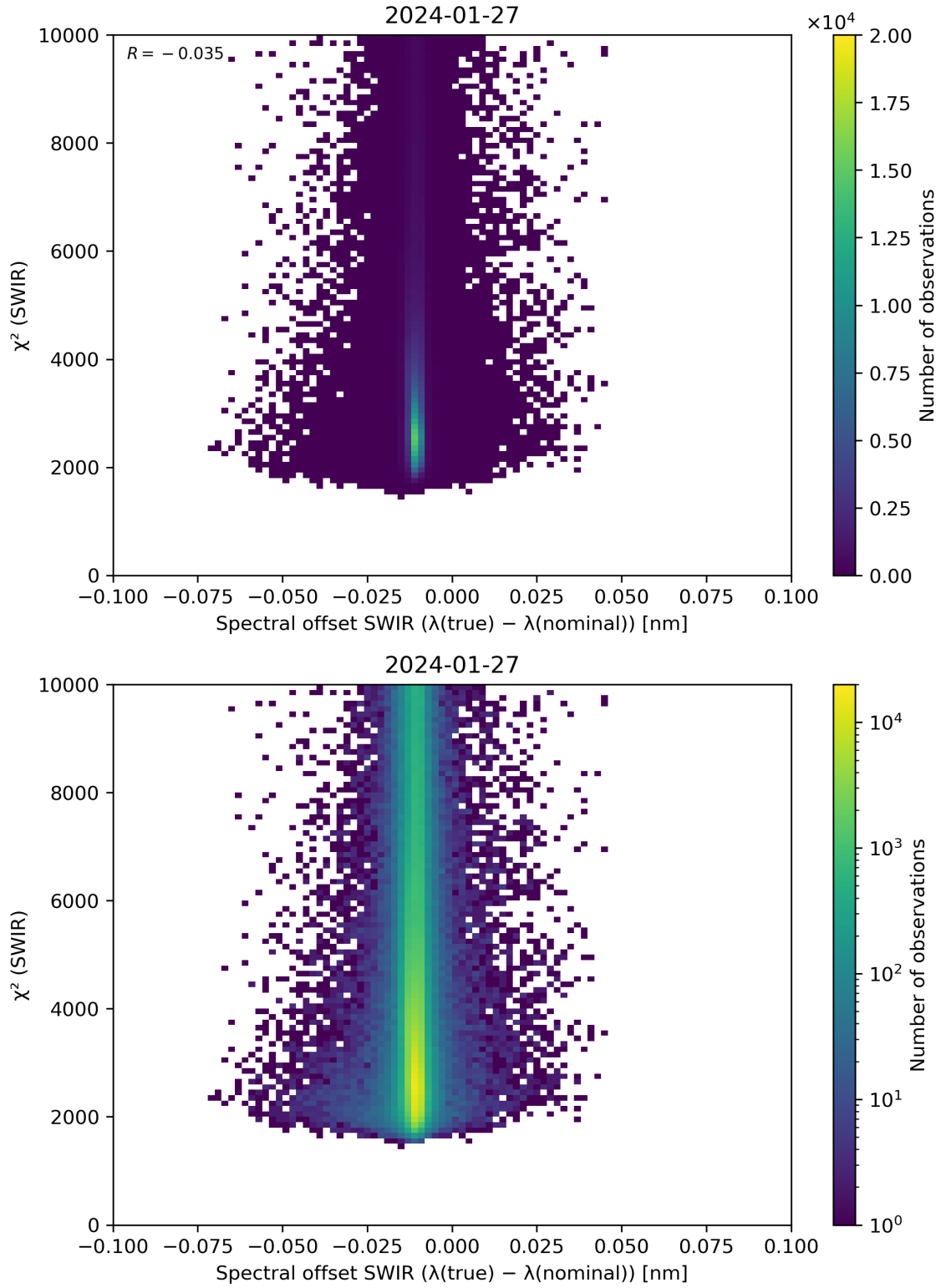
Figure 118: Scatter density plot of “Spectral offset SWIR ( \lambda(\text{true}) - \lambda(\text{nominal}) )” against “ \chi^2 (SWIR)” for 2024-01-26 to 2024-01-28.
