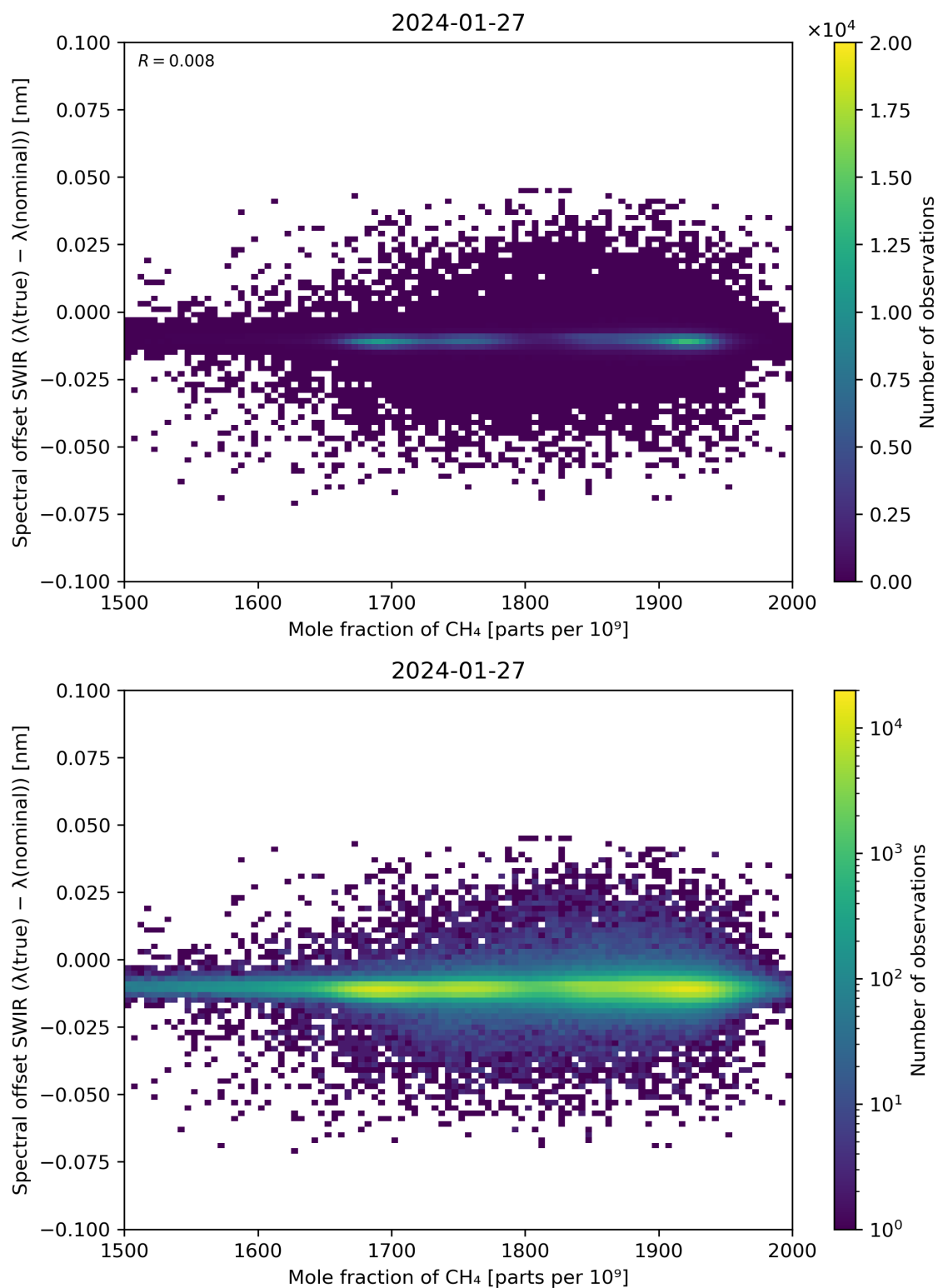
Figure 86: Scatter density plot of “Mole fraction of CH 4 ” against “Spectral offset SWIR ( \lambda(\text{true}) - \lambda(\text{nominal}) )” for 2024-01-26 to 2024-01-28.
