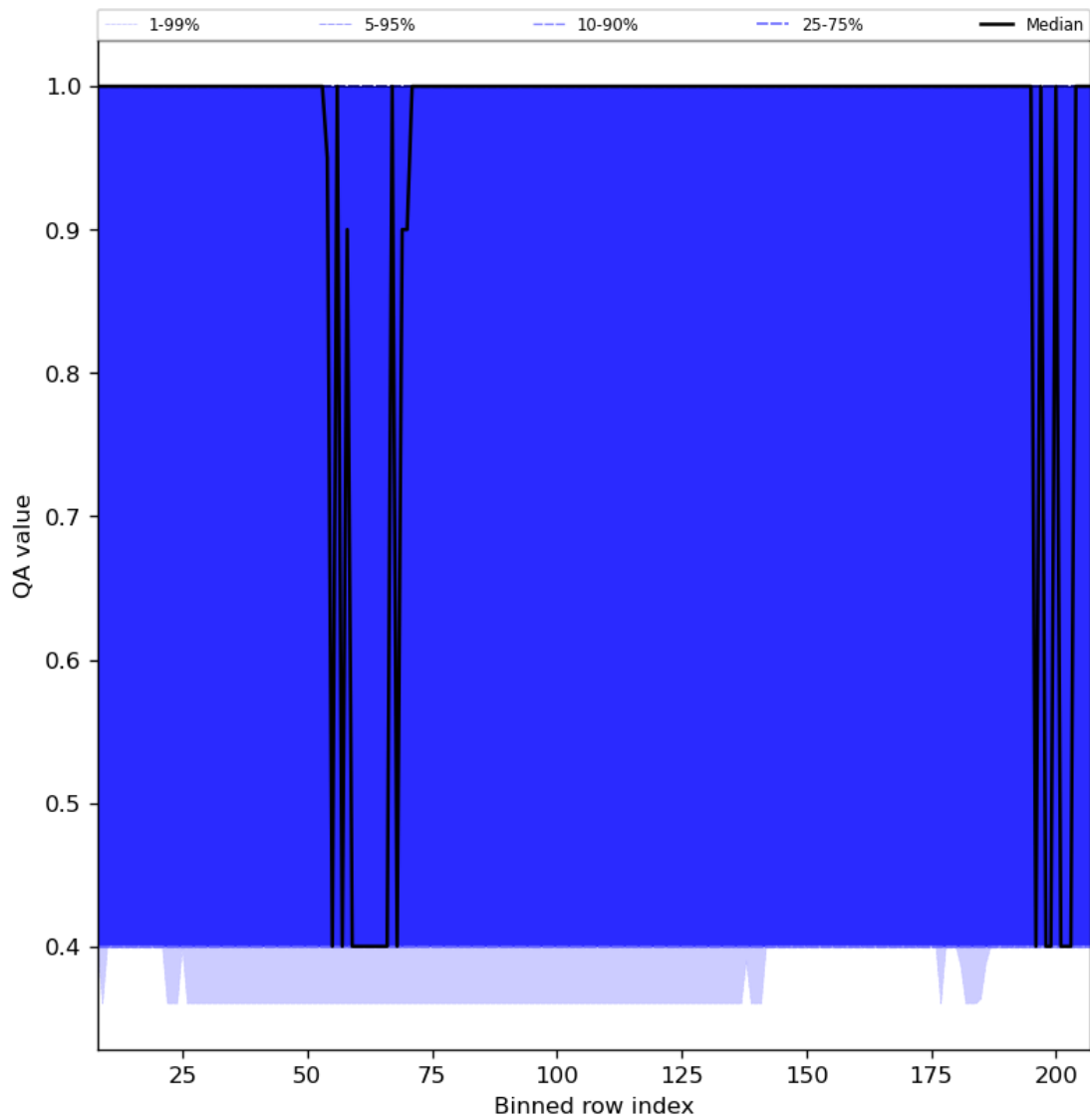
Figure 33: Along track statistics of “QA value” for 2024-01-26 to 2024-01-28
