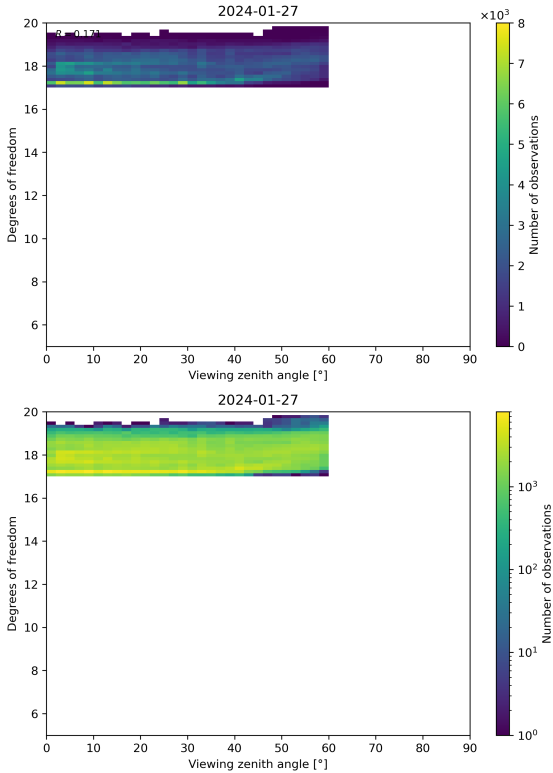
Figure 107: Scatter density plot of “Viewing zenith angle” against “Degrees of freedom” for 2024-01-26 to 2024-01-28.
