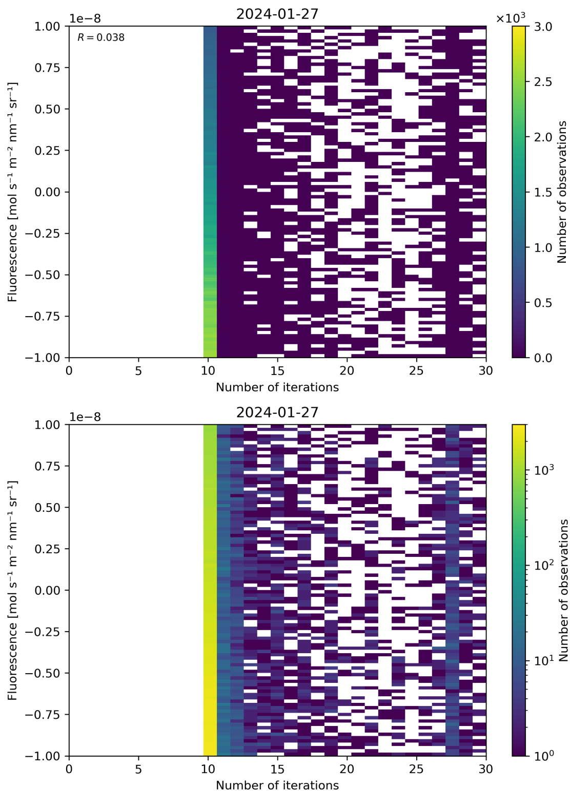
Figure 87: Scatter density plot of “Number of iterations” against “Fluorescence” for 2024-01-26 to 2024-01-28.
