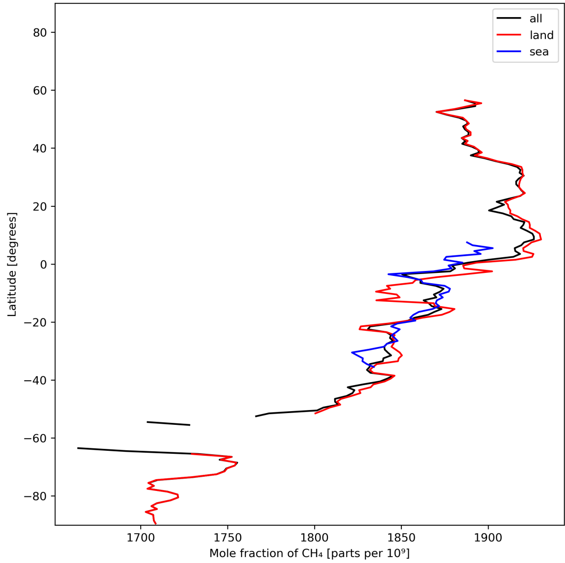
Figure 12: Zonal average of “Mole fraction of \text{CH}_4 ” for 2024-01-26 to 2024-01-28.
