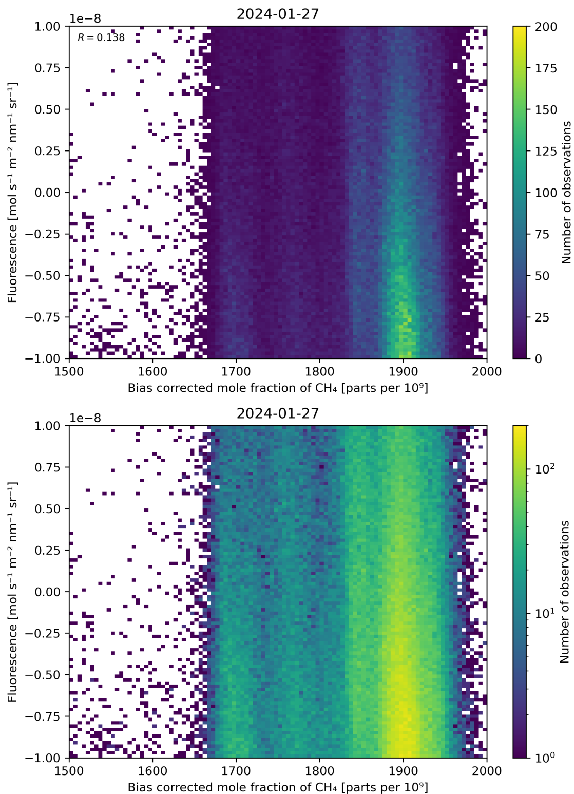
Figure 66: Scatter density plot of “Bias corrected mole fraction of \text{CH}_4 ” against “Fluorescence” for 2024-01-26 to 2024-01-28.
