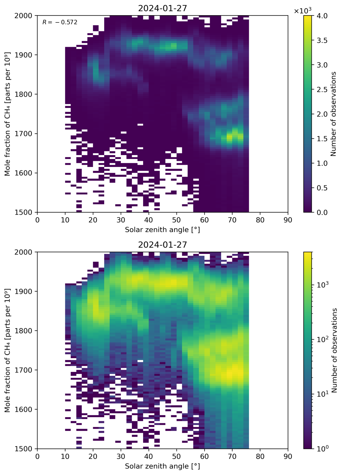
Figure 99: Scatter density plot of “Solar zenith angle” against “Mole fraction of CH 4 ” for 2024-01-26 to 2024-01-28.
