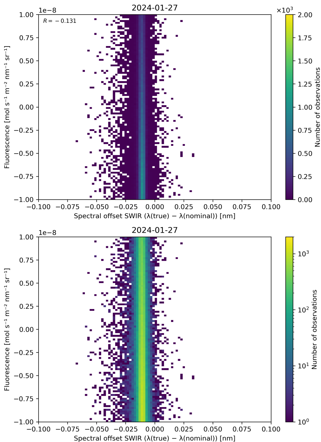
Figure 120: Scatter density plot of “Spectral offset SWIR ( \lambda(\text{true}) - \lambda(\text{nominal}) )” against “Fluorescence” for 2024-01-26 to 2024-01-28.
