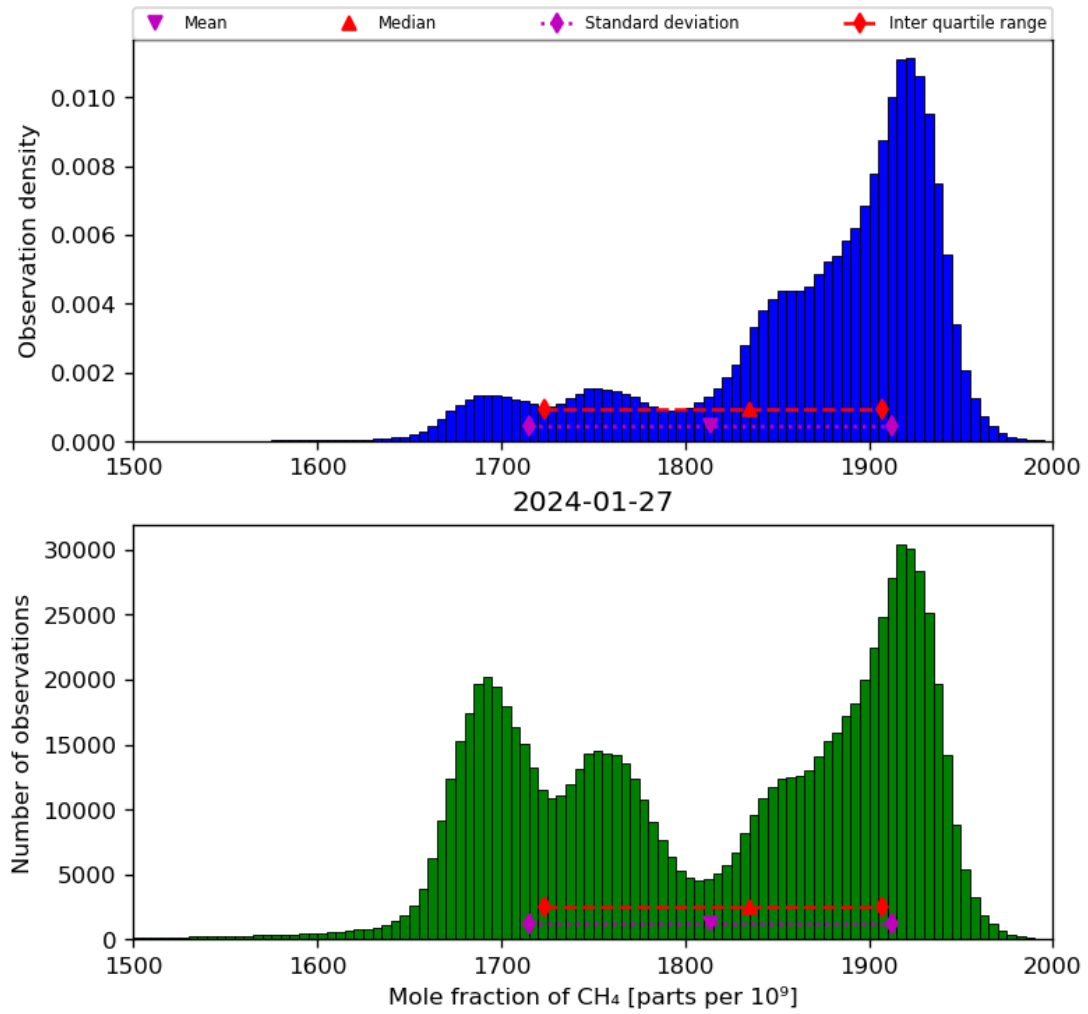
Figure 23: Histogram of “Mole fraction of CH 4 ” for 2024-01-26 to 2024-01-28
