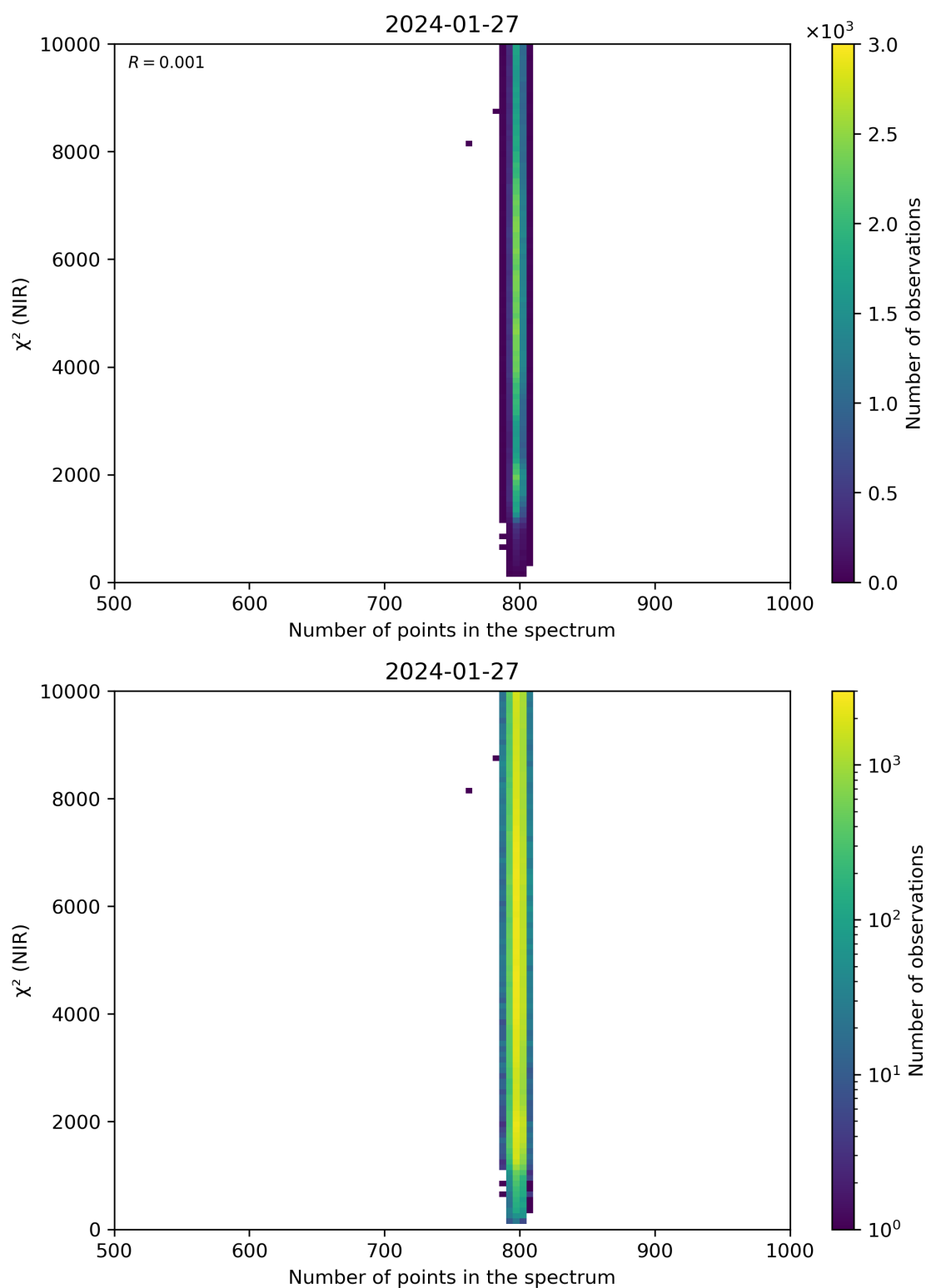
Figure 88: Scatter density plot of “Number of points in the spectrum” against “ \chi^2 (NIR)” for 2024-01-26 to 2024-01-28.
