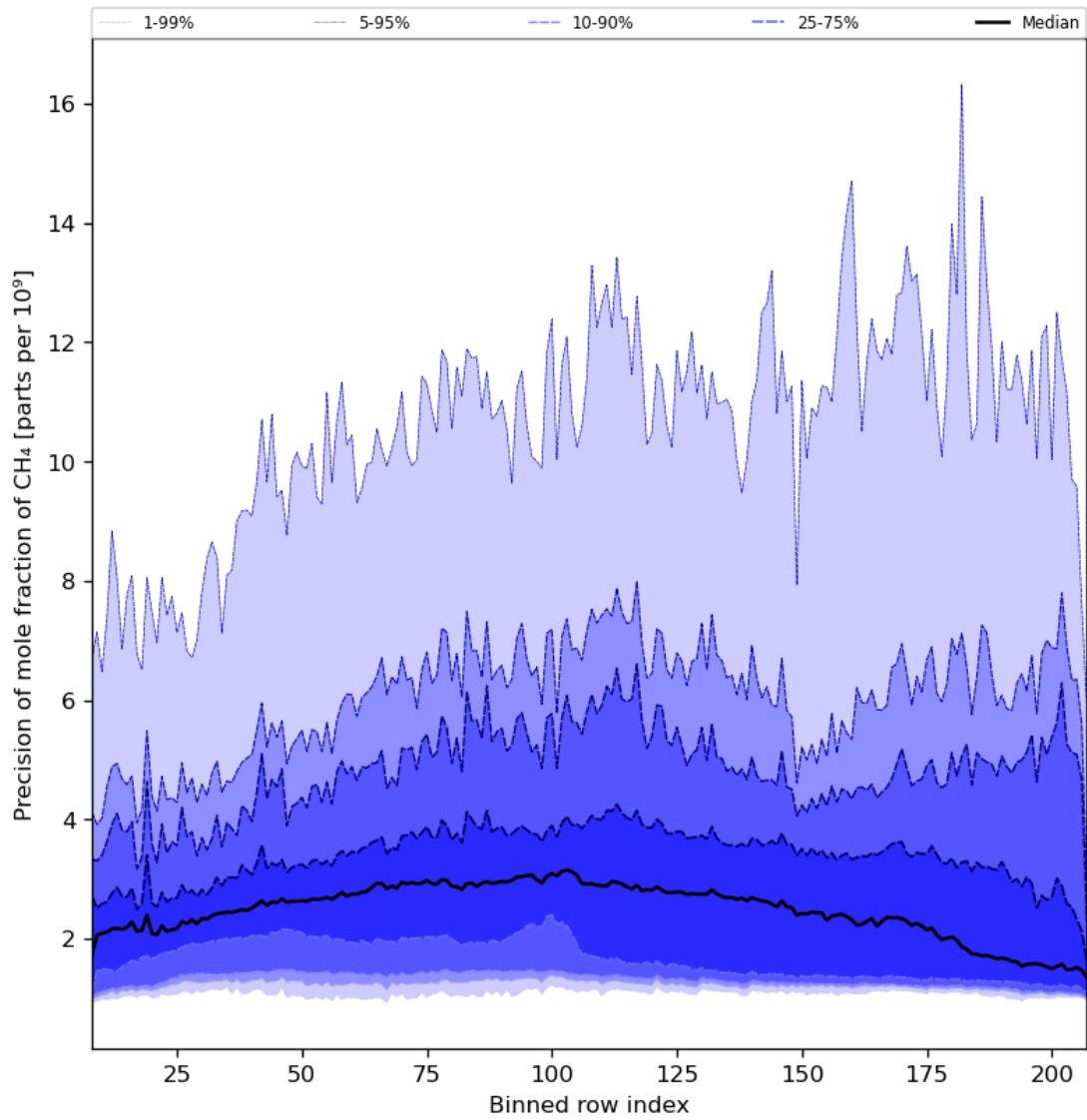
Figure 35: Along track statistics of “Precision of mole fraction of CH 4 ” for 2024-01-26 to 2024-01-28
