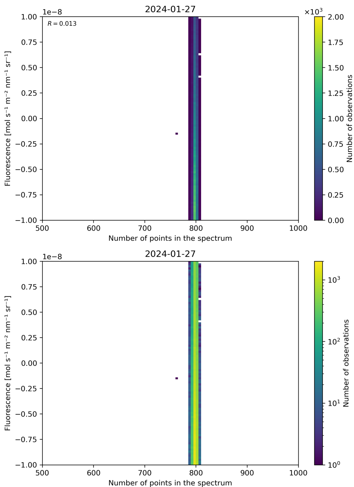
Figure 91: Scatter density plot of “Number of points in the spectrum” against “Fluorescence” for 2024-01-26 to 2024-01-28.
