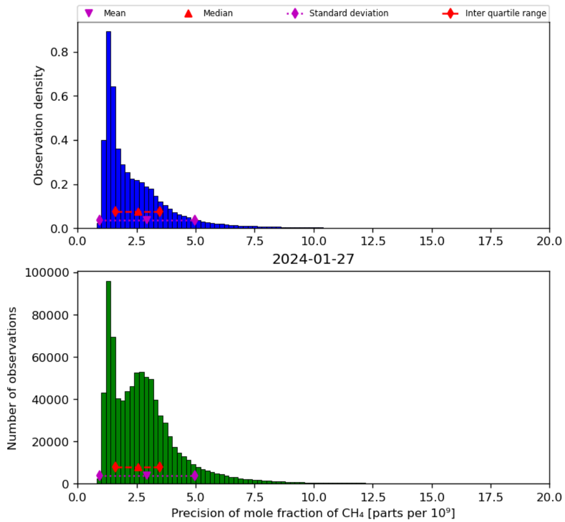
Figure 24: Histogram of “Precision of mole fraction of CH 4 ” for 2024-01-26 to 2024-01-28
