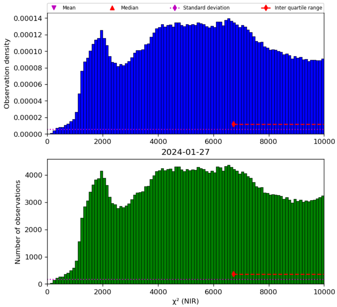
Figure 29: Histogram of “ \chi^2 (NIR)” for 2024-01-26 to 2024-01-28
