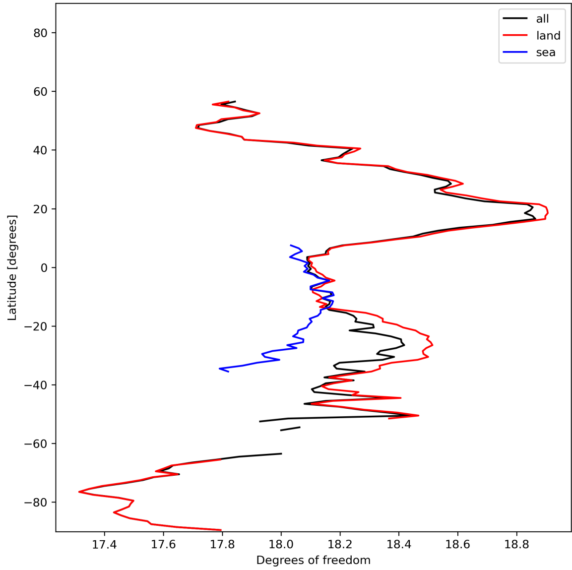
Figure 19: Zonal average of “Degrees of freedom” for 2024-01-26 to 2024-01-28.
