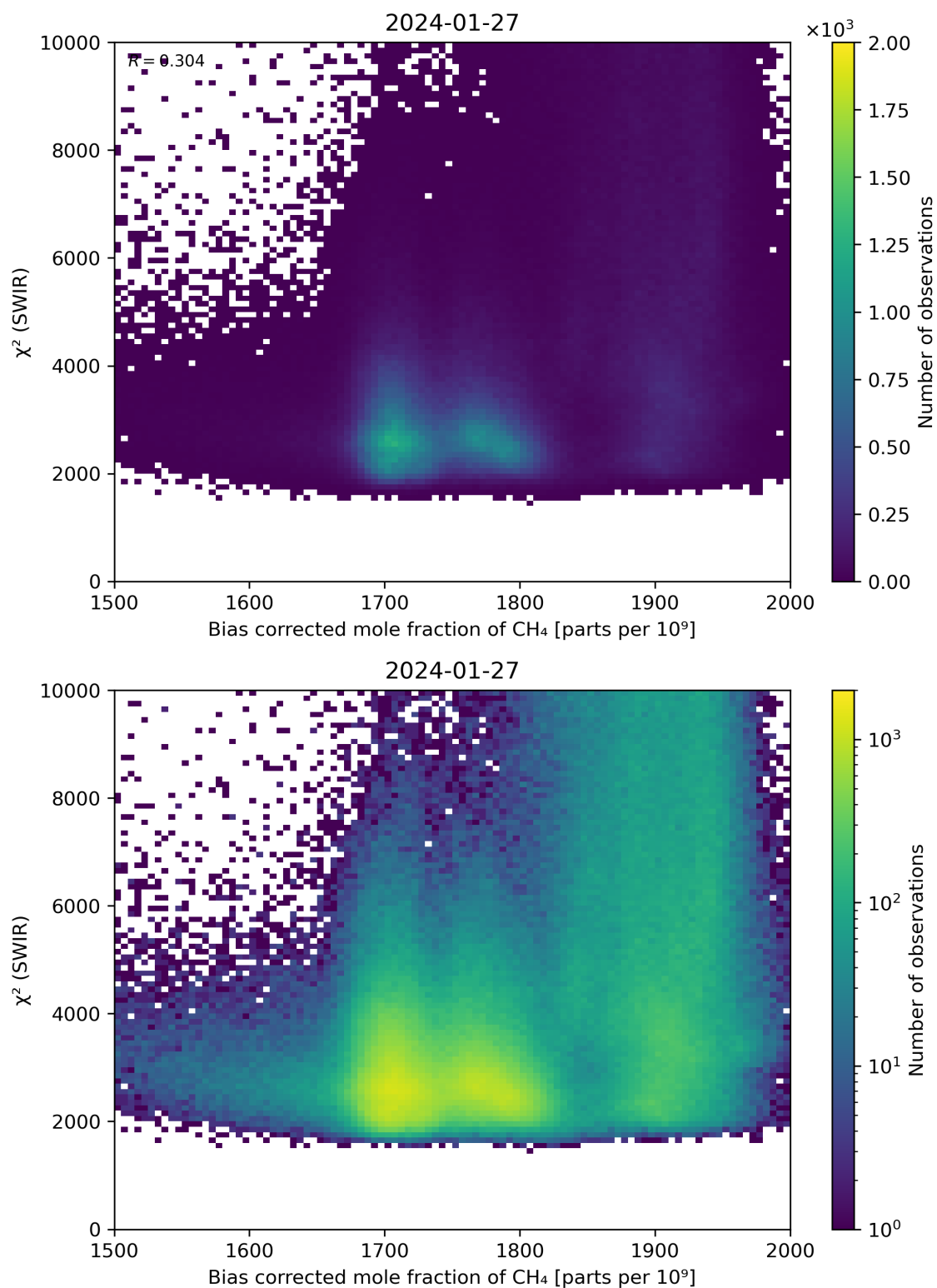
Figure 64: Scatter density plot of “Bias corrected mole fraction of CH 4 ” against “ \chi^2 (SWIR)” for 2024-01-26 to 2024-01-28.
