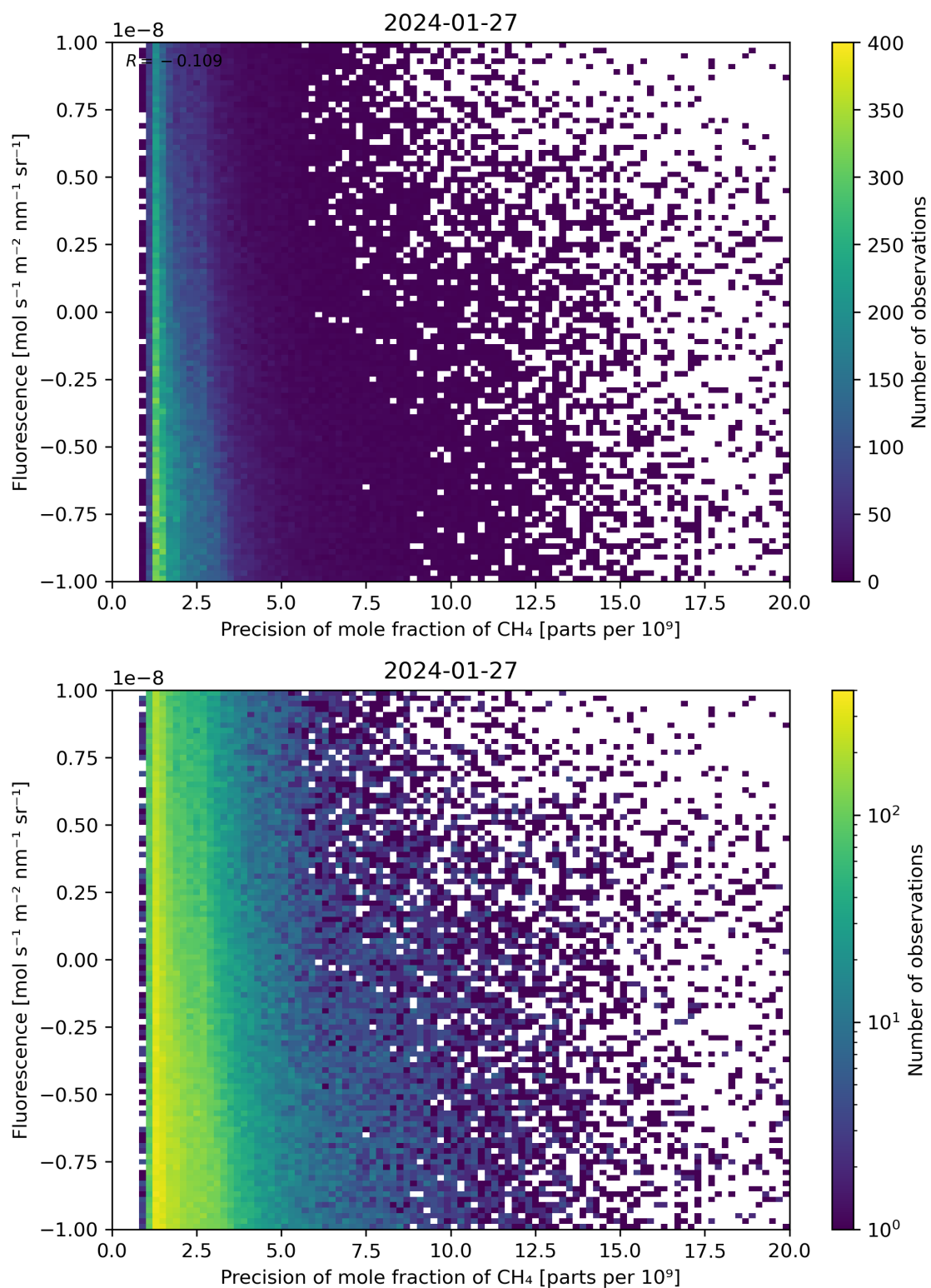
Figure 81: Scatter density plot of “Precision of mole fraction of CH 4 ” against “Fluorescence” for 2024-01-26 to 2024-01-28.
