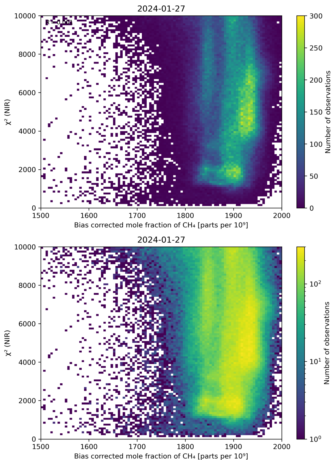
Figure 63: Scatter density plot of “Bias corrected mole fraction of \text{CH}_4 ” against “ \chi^2 (NIR)” for 2024-01-26 to 2024-01-28.
