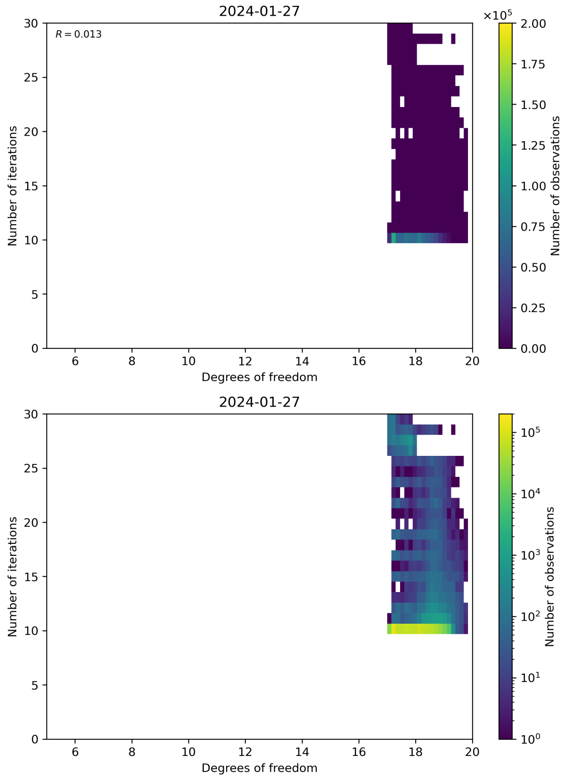
Figure 52: Scatter density plot of “Degrees of freedom” against “Number of iterations” for 2024-01-26 to 2024-01-28.
