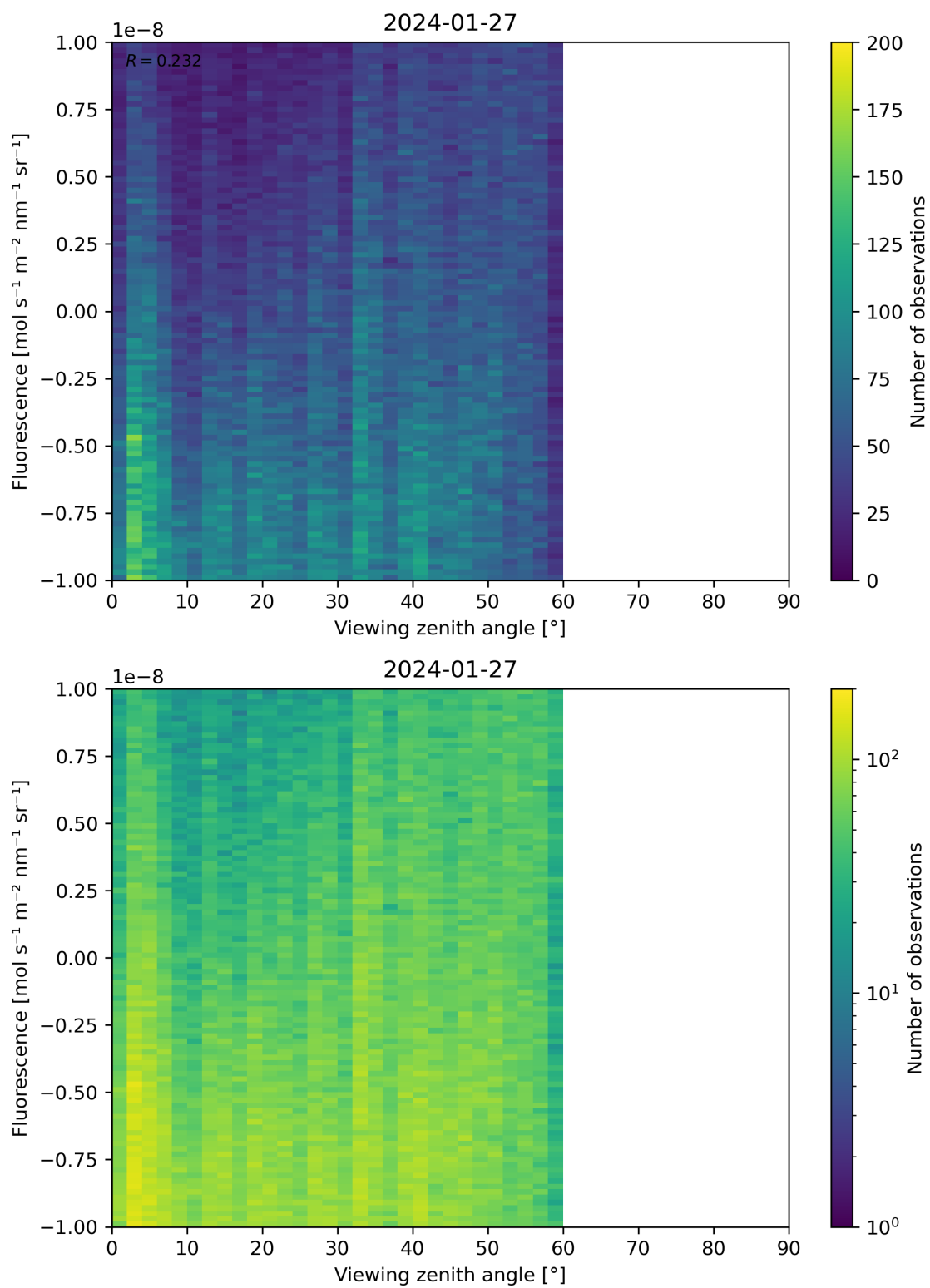
Figure 108: Scatter density plot of “Viewing zenith angle” against “Fluorescence” for 2024-01-26 to 2024-01-28.
