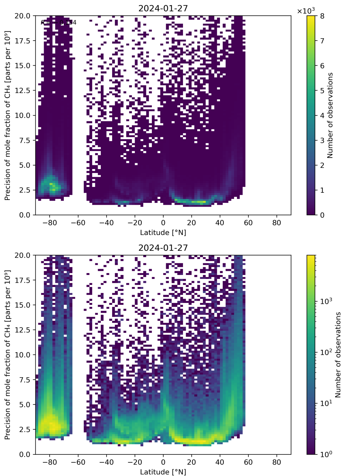
Figure 59: Scatter density plot of “Latitude” against “Precision of mole fraction of CH 4 ” for 2024-01-26 to 2024-01-28.
