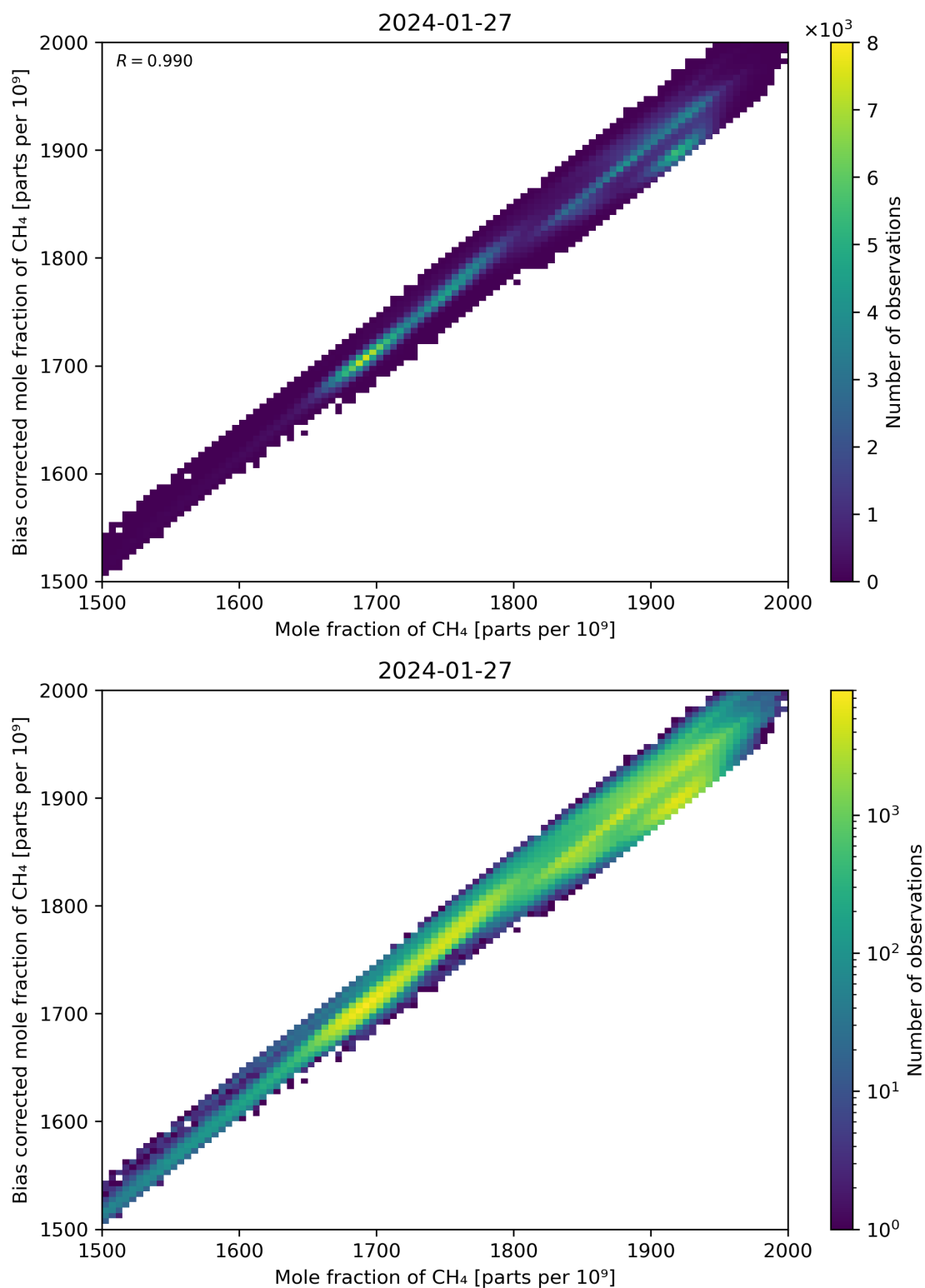
Figure 74: Scatter density plot of “Mole fraction of CH 4 ” against “Bias corrected mole fraction of CH 4 ” for 2024-01-26 to 2024-01-28.
