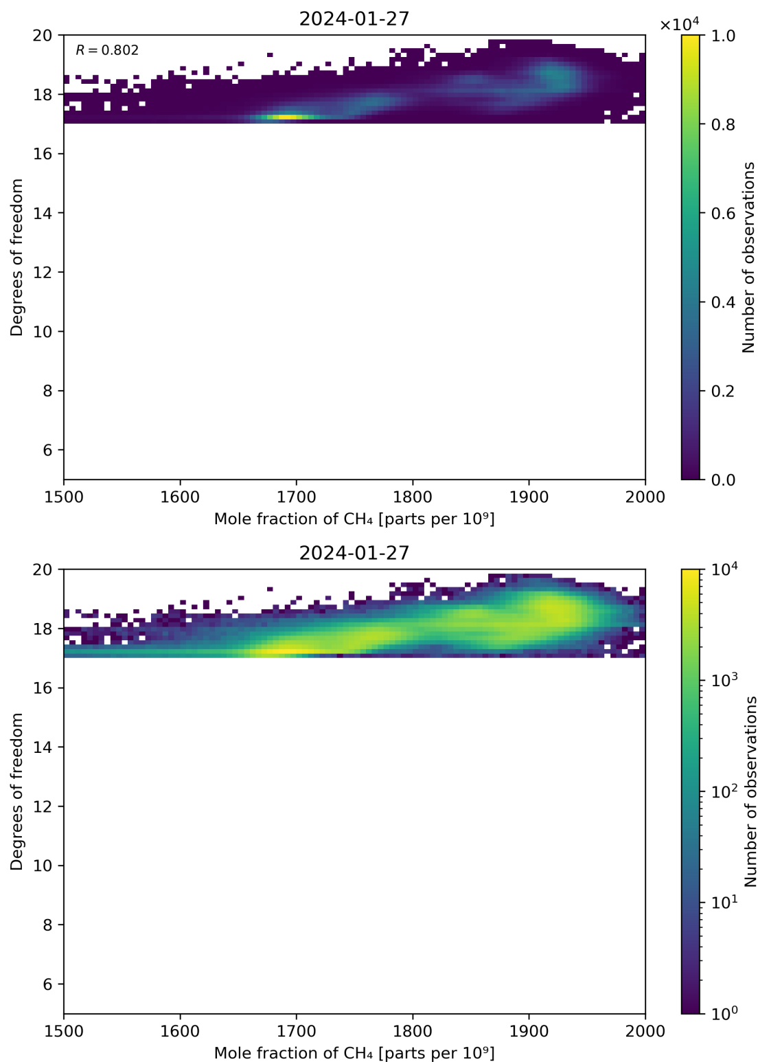
Figure 72: Scatter density plot of “Mole fraction of CH 4 ” against “Degrees of freedom” for 2024-01-26 to 2024-01-28.
