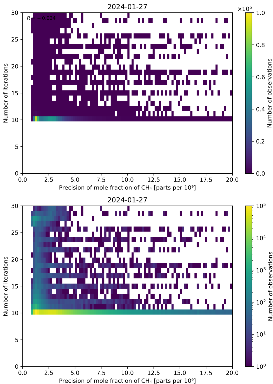
Figure 83: Scatter density plot of “Precision of mole fraction of CH 4 ” against “Number of iterations” for 2024-01-26 to 2024-01-28.
