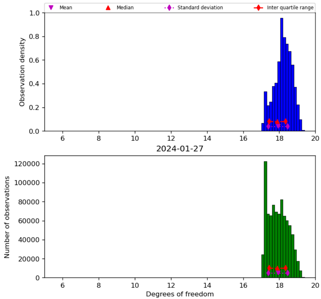
Figure 30: Histogram of “Degrees of freedom” for 2024-01-26 to 2024-01-28
