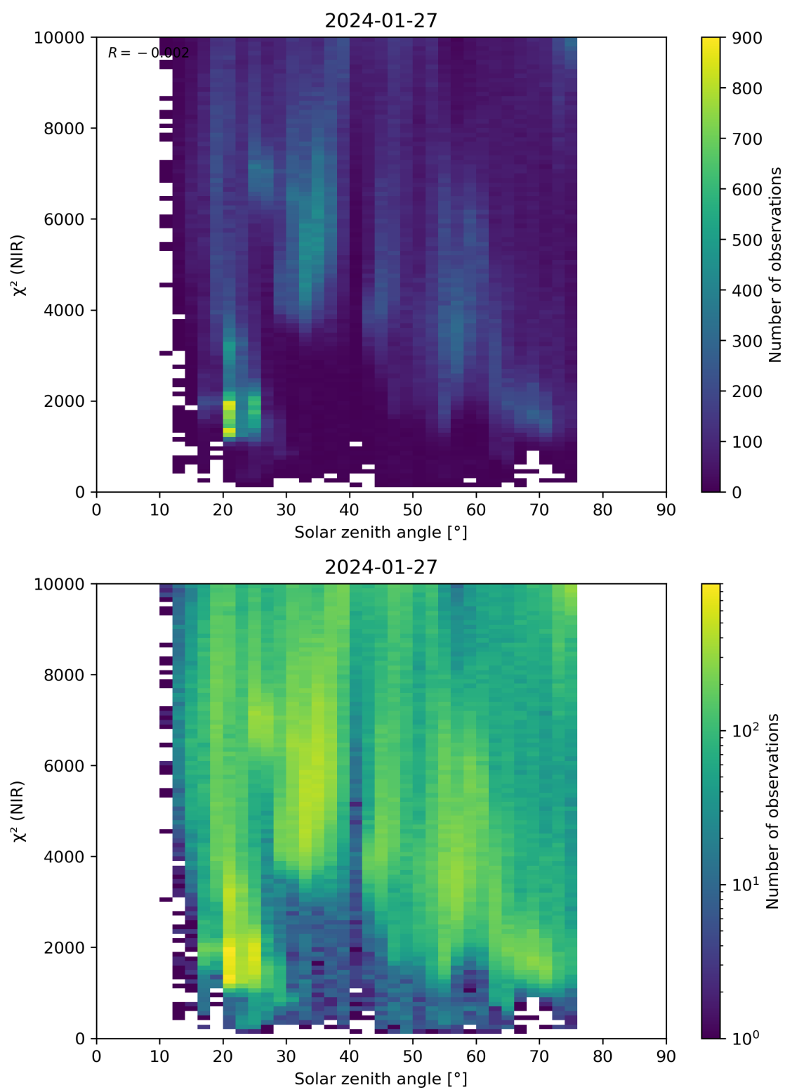
Figure 94: Scatter density plot of “Solar zenith angle” against “ \chi^2 (NIR)” for 2024-01-26 to 2024-01-28.
