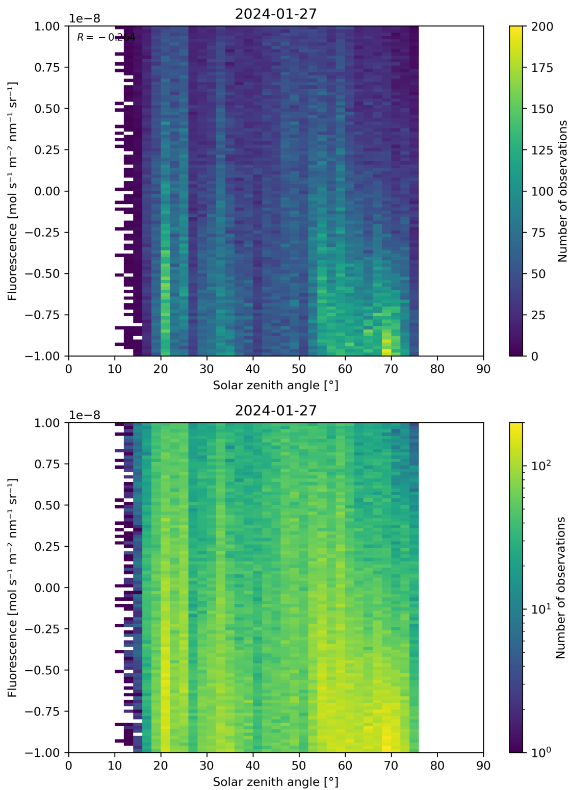
Figure 97: Scatter density plot of “Solar zenith angle” against “Fluorescence” for 2024-01-26 to 2024-01-28.
