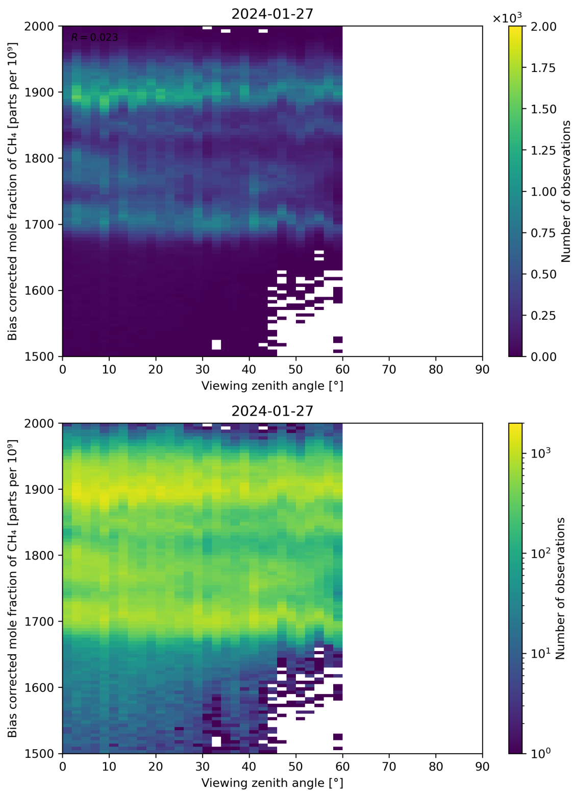
Figure 111: Scatter density plot of “Viewing zenith angle” against “Bias corrected mole fraction of CH 4 ” for 2024-01-26 to 2024-01-28.
