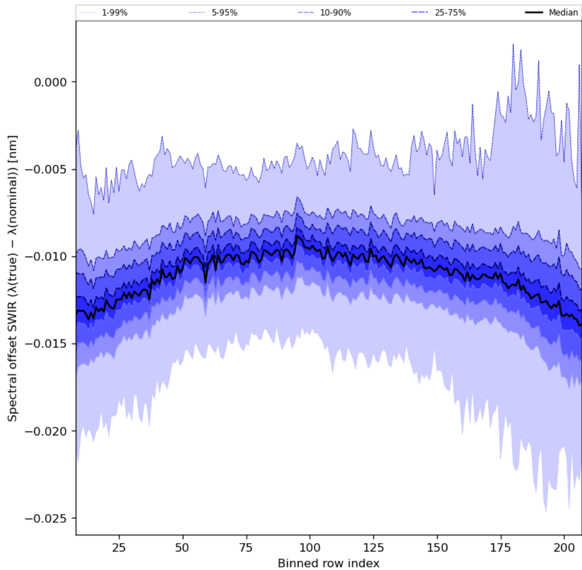
Figure 38: Along track statistics of “Spectral offset SWIR ( \lambda(\text{true}) - \lambda(\text{nominal}) )” for 2024-01-26 to 2024-01-28
