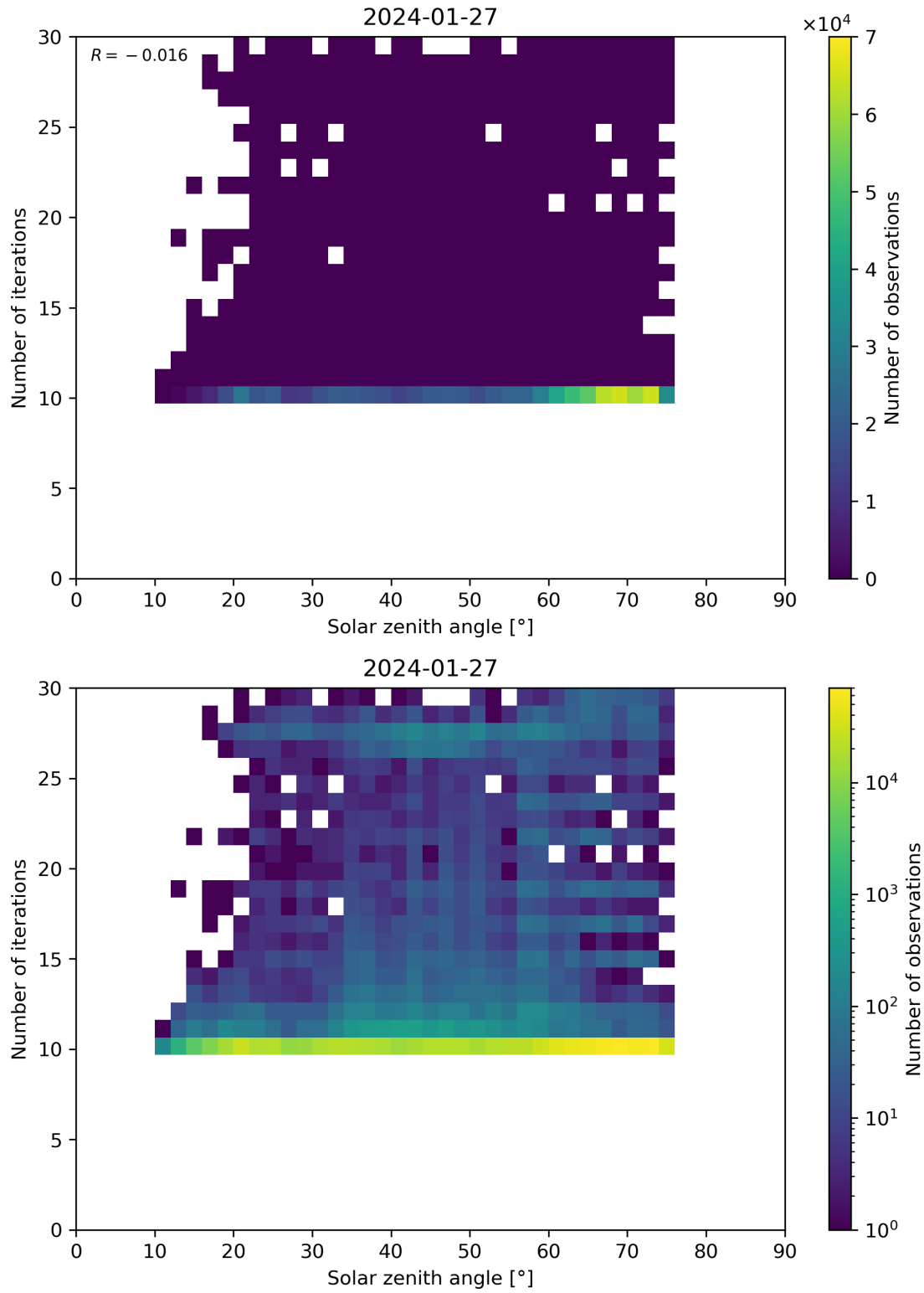
Figure 102: Scatter density plot of “Solar zenith angle” against “Number of iterations” for 2024-01-26 to 2024-01-28.
