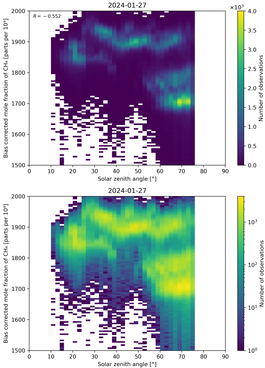
Figure 100: Scatter density plot of “Solar zenith angle” against “Bias corrected mole fraction of \text{CH}_4 ” for 2024-01-26 to 2024-01-28.
