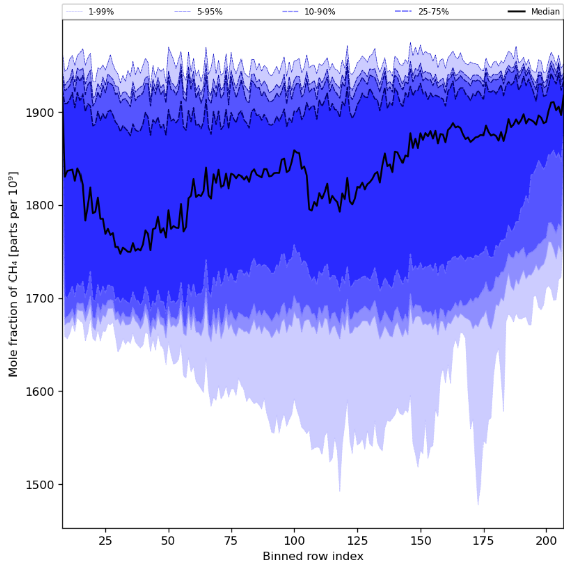
Figure 34: Along track statistics of “Mole fraction of CH 4 ” for 2024-01-26 to 2024-01-28
