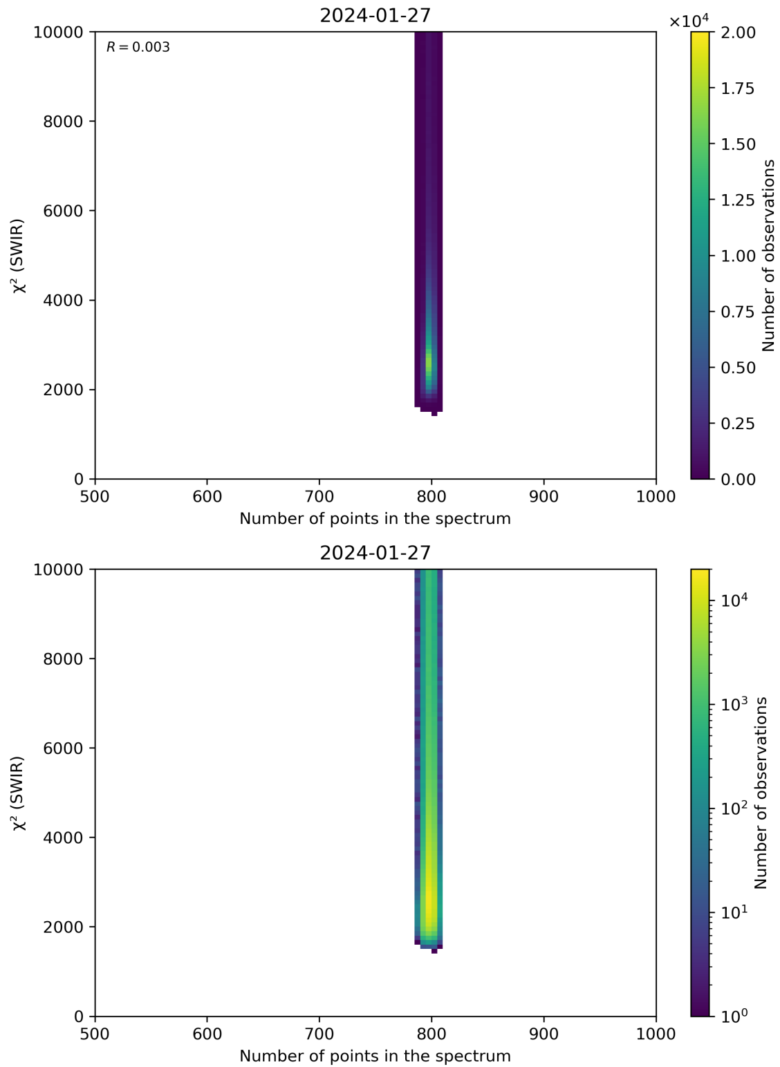
Figure 89: Scatter density plot of “Number of points in the spectrum” against “ \chi^2 (SWIR)” for 2024-01-26 to 2024-01-28.
