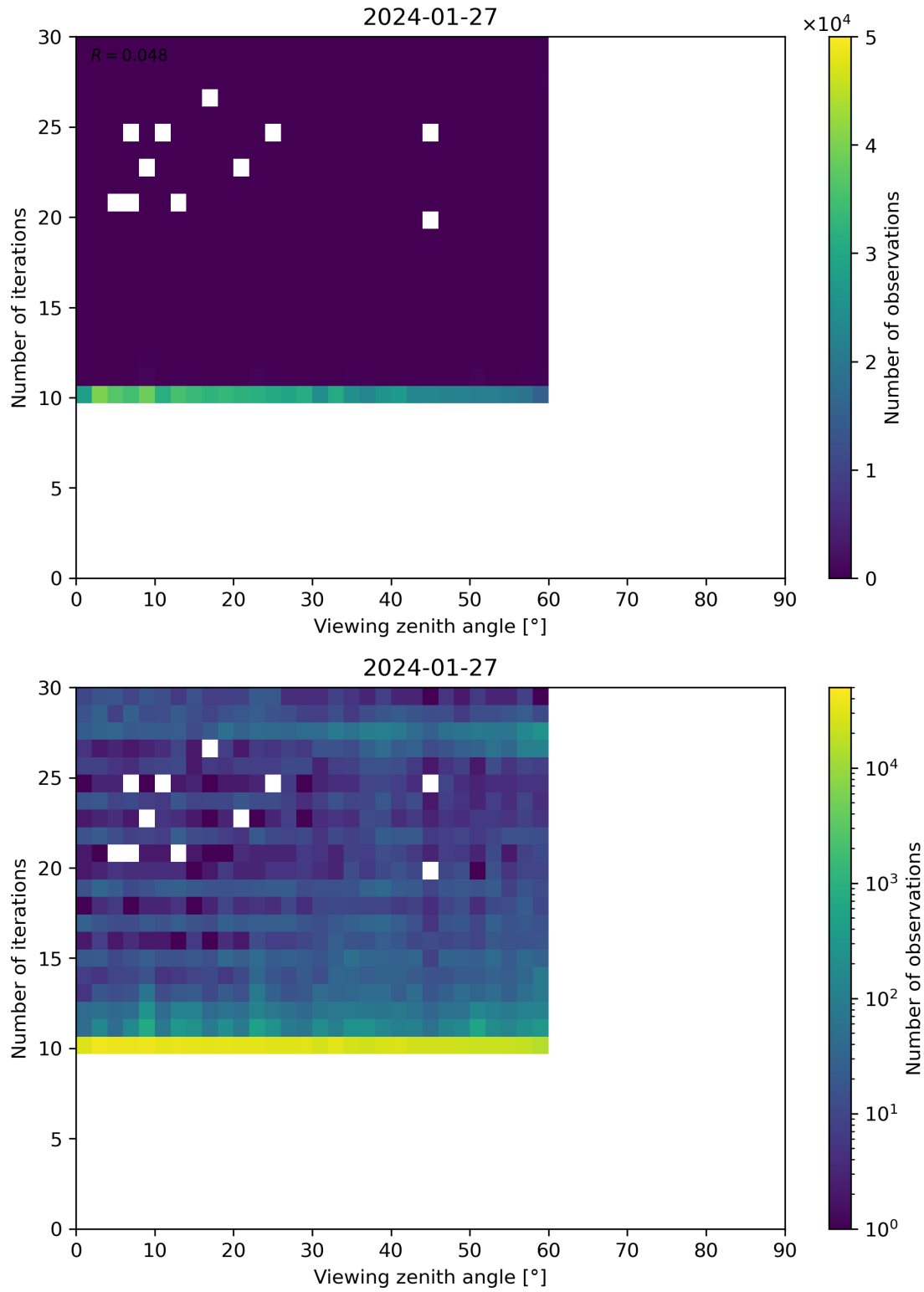
Figure 113: Scatter density plot of “Viewing zenith angle” against “Number of iterations” for 2024-01-26 to 2024-01-28.
