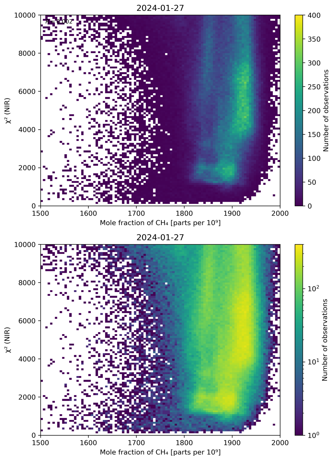
Figure 70: Scatter density plot of “Mole fraction of \text{CH}_4 ” against “ \chi^2 (NIR)” for 2024-01-26 to 2024-01-28.
