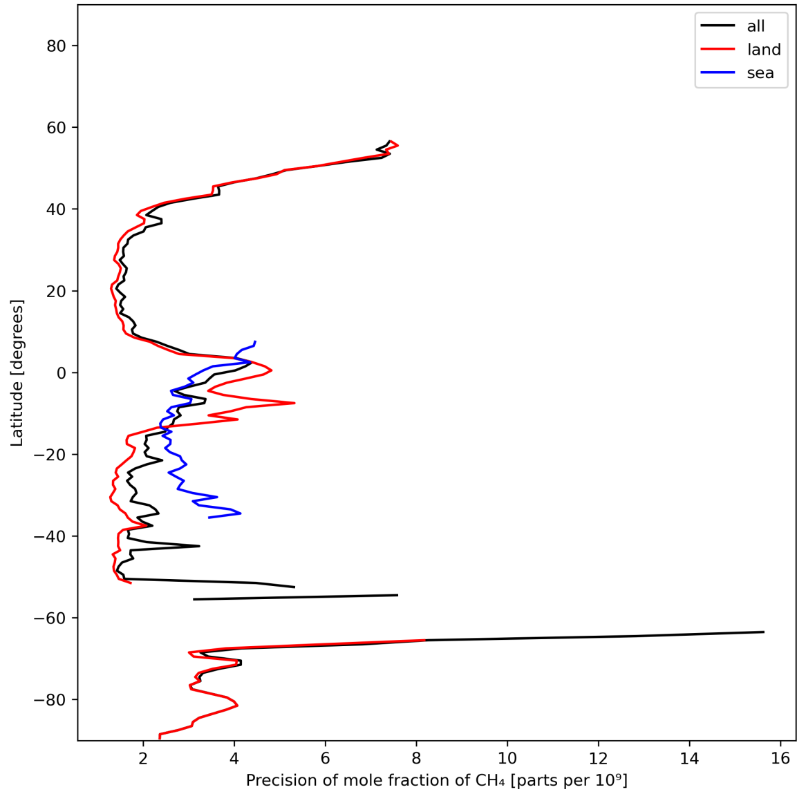
Figure 13: Zonal average of “Precision of mole fraction of \text{CH}_4 ” for 2024-01-26 to 2024-01-28.
