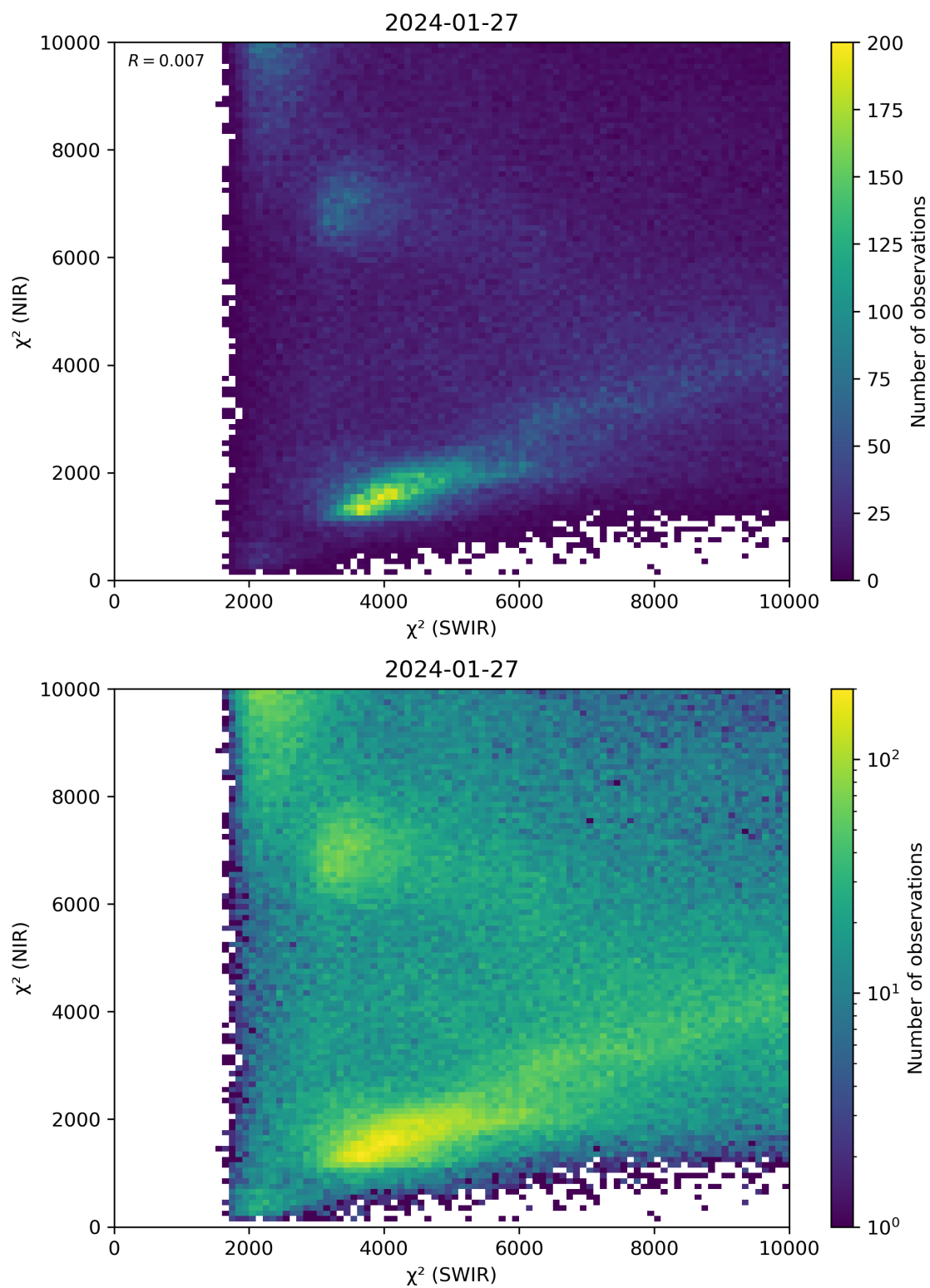
Figure 47: Scatter density plot of “ \chi^2 (SWIR)” against “ \chi^2 (NIR)” for 2024-01-26 to 2024-01-28.
