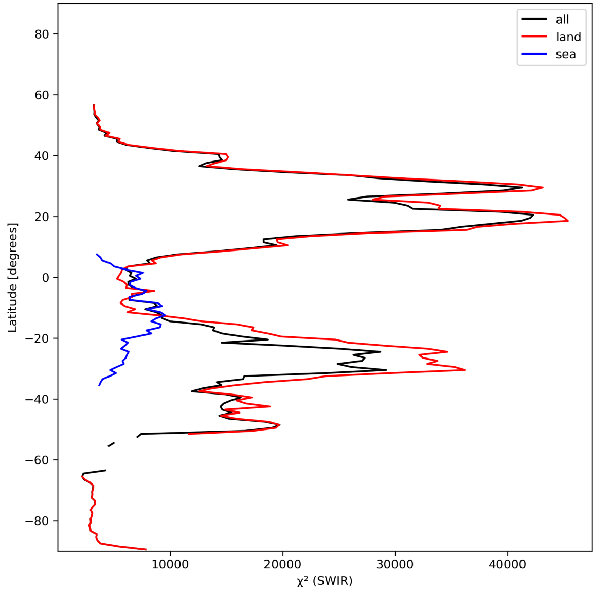
Figure 17: Zonal average of “ \chi^2 (SWIR)” for 2024-01-26 to 2024-01-28.
