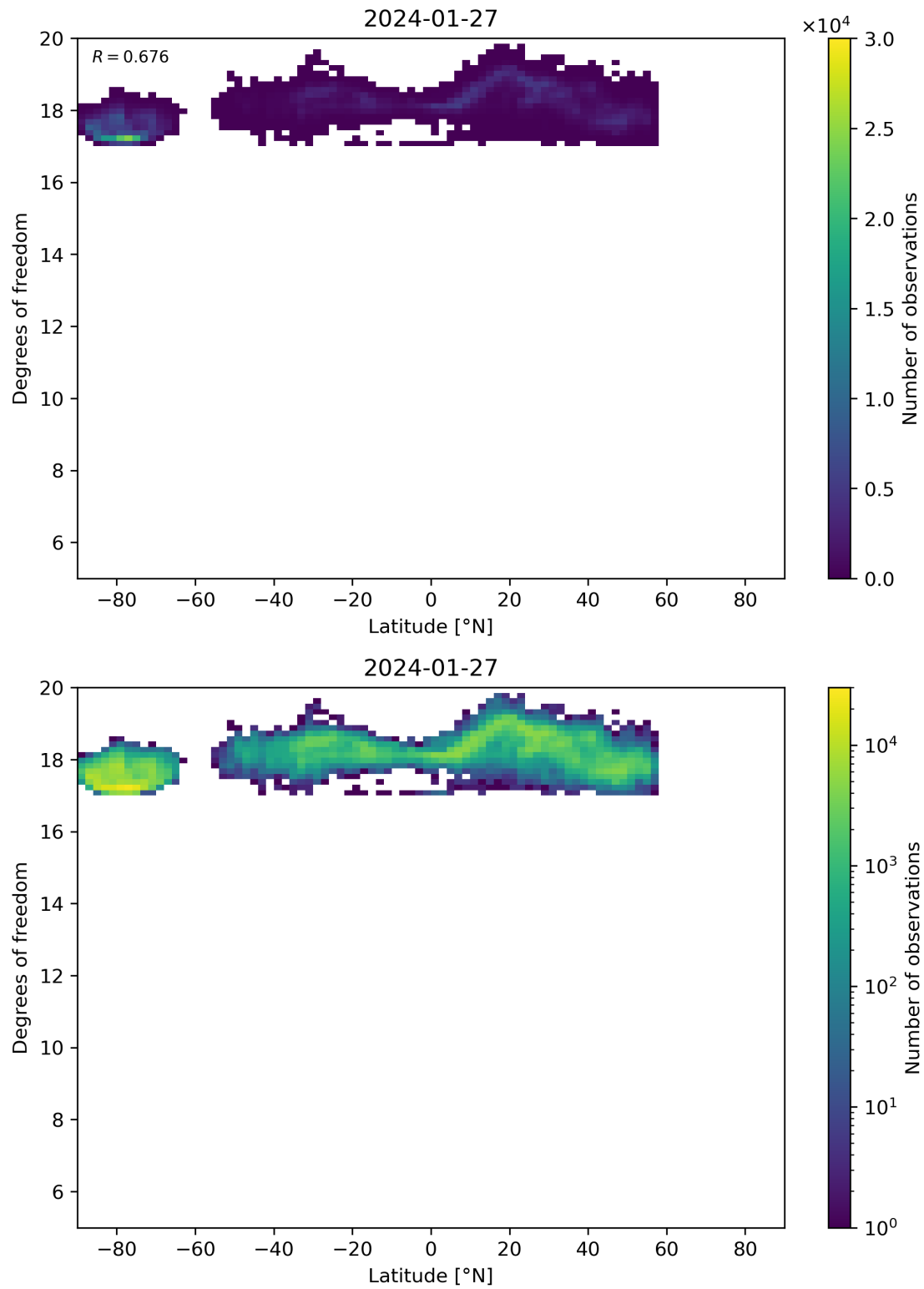
Figure 55: Scatter density plot of “Latitude” against “Degrees of freedom” for 2024-01-26 to 2024-01-28.
