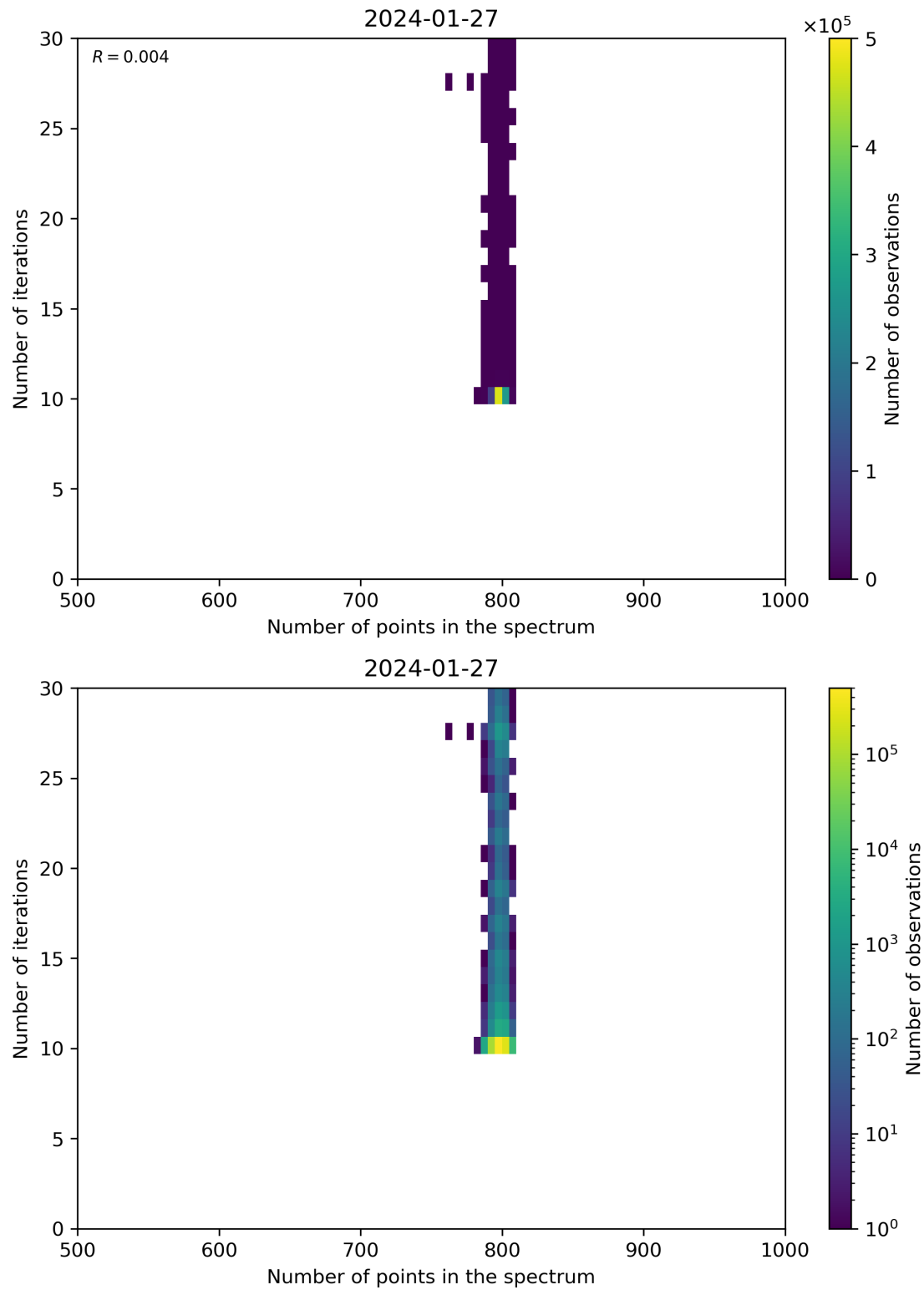
Figure 92: Scatter density plot of “Number of points in the spectrum” against “Number of iterations” for 2024-01-26 to 2024-01-28.
