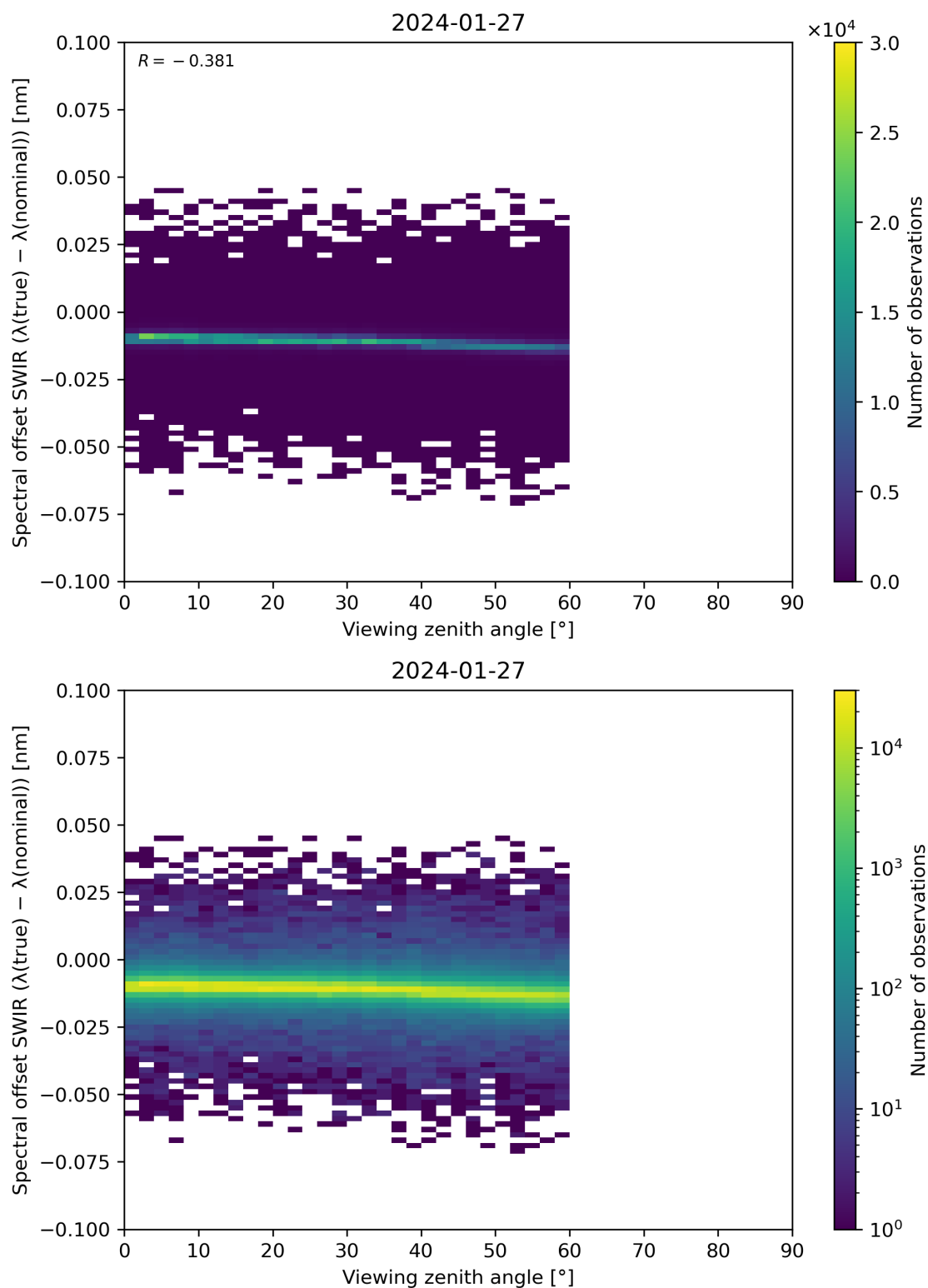
Figure 116: Scatter density plot of “Viewing zenith angle” against “Spectral offset SWIR ( \lambda(\text{true}) - \lambda(\text{nominal}) )” for 2024-01-26 to 2024-01-28.
