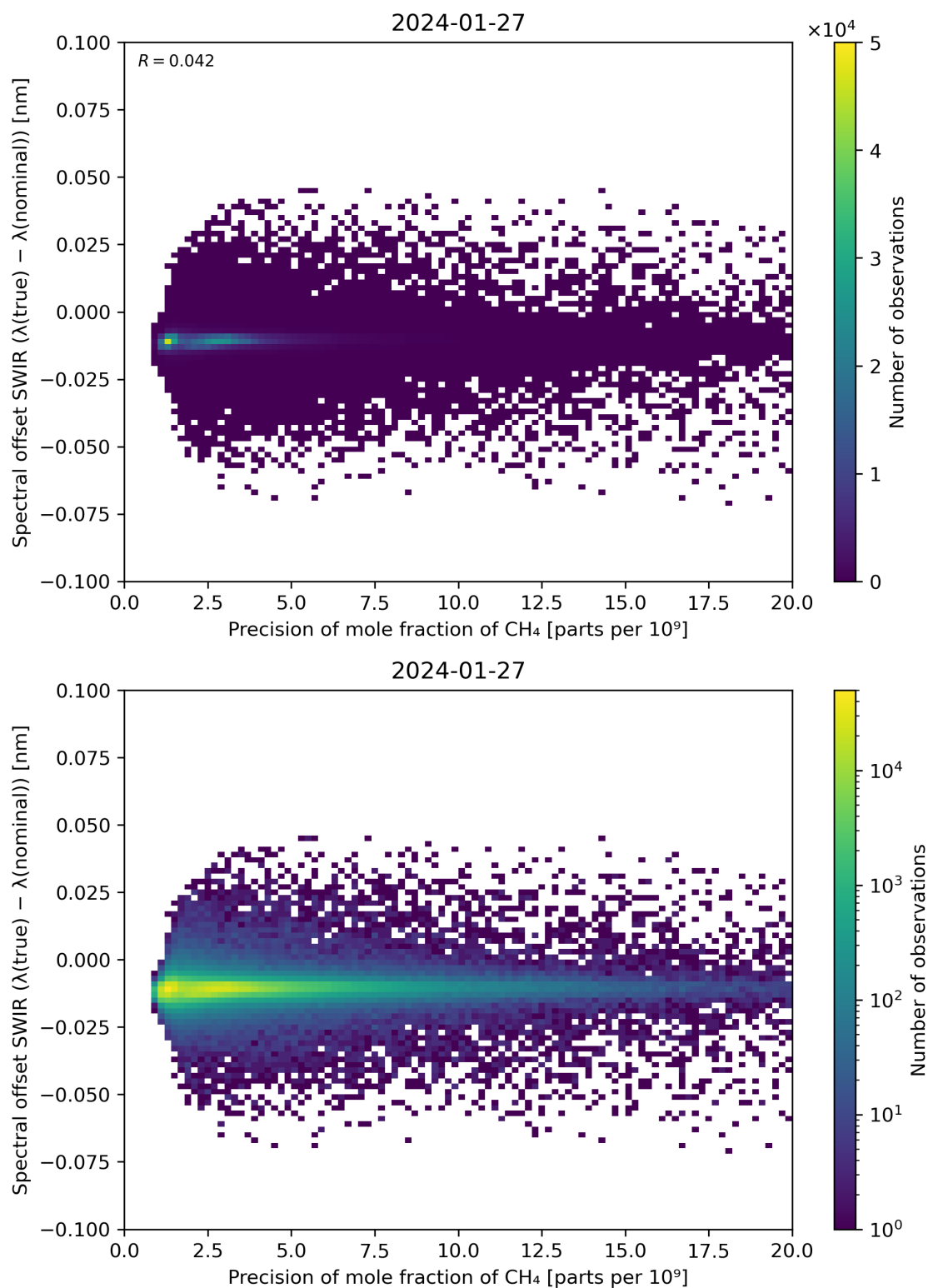
Figure 85: Scatter density plot of “Precision of mole fraction of CH 4 ” against “Spectral offset SWIR ( \lambda(\text{true}) - \lambda(\text{nominal}) )” for 2024-01-26 to 2024-01-28.
