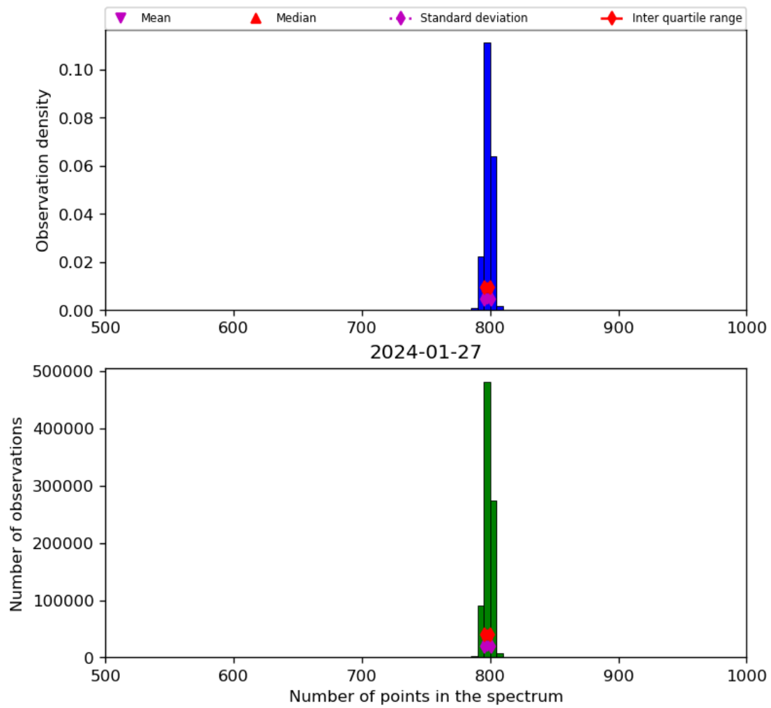
Figure 26: Histogram of “Number of points in the spectrum” for 2024-01-26 to 2024-01-28
