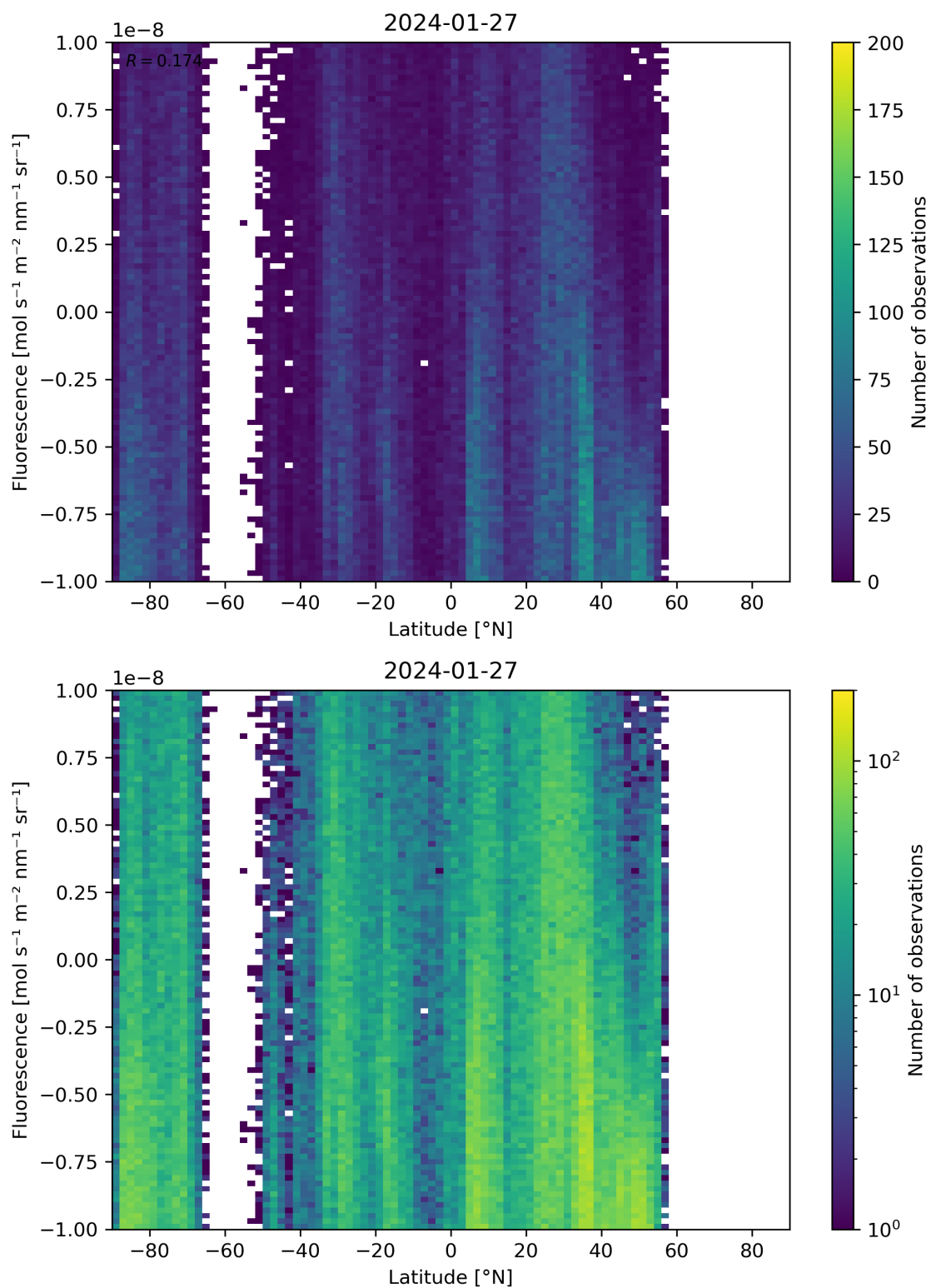
Figure 56: Scatter density plot of “Latitude” against “Fluorescence” for 2024-01-26 to 2024-01-28.
