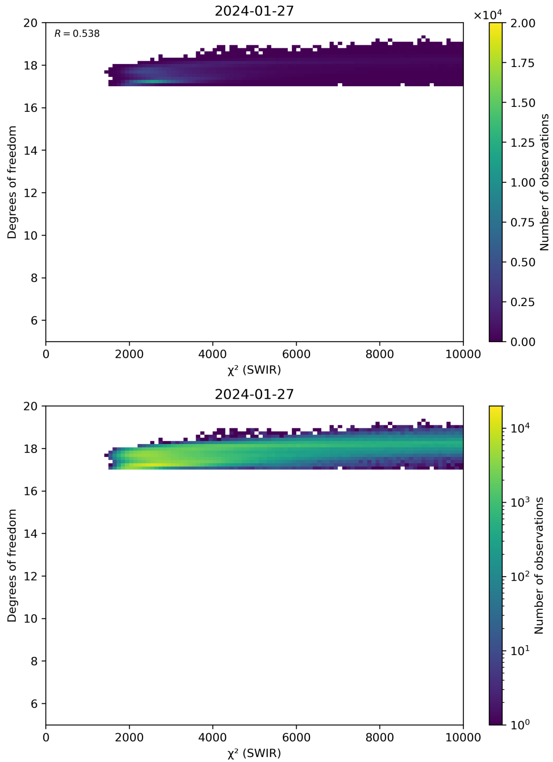
Figure 48: Scatter density plot of “ \chi^2 (SWIR)” against “Degrees of freedom” for 2024-01-26 to 2024-01-28.
