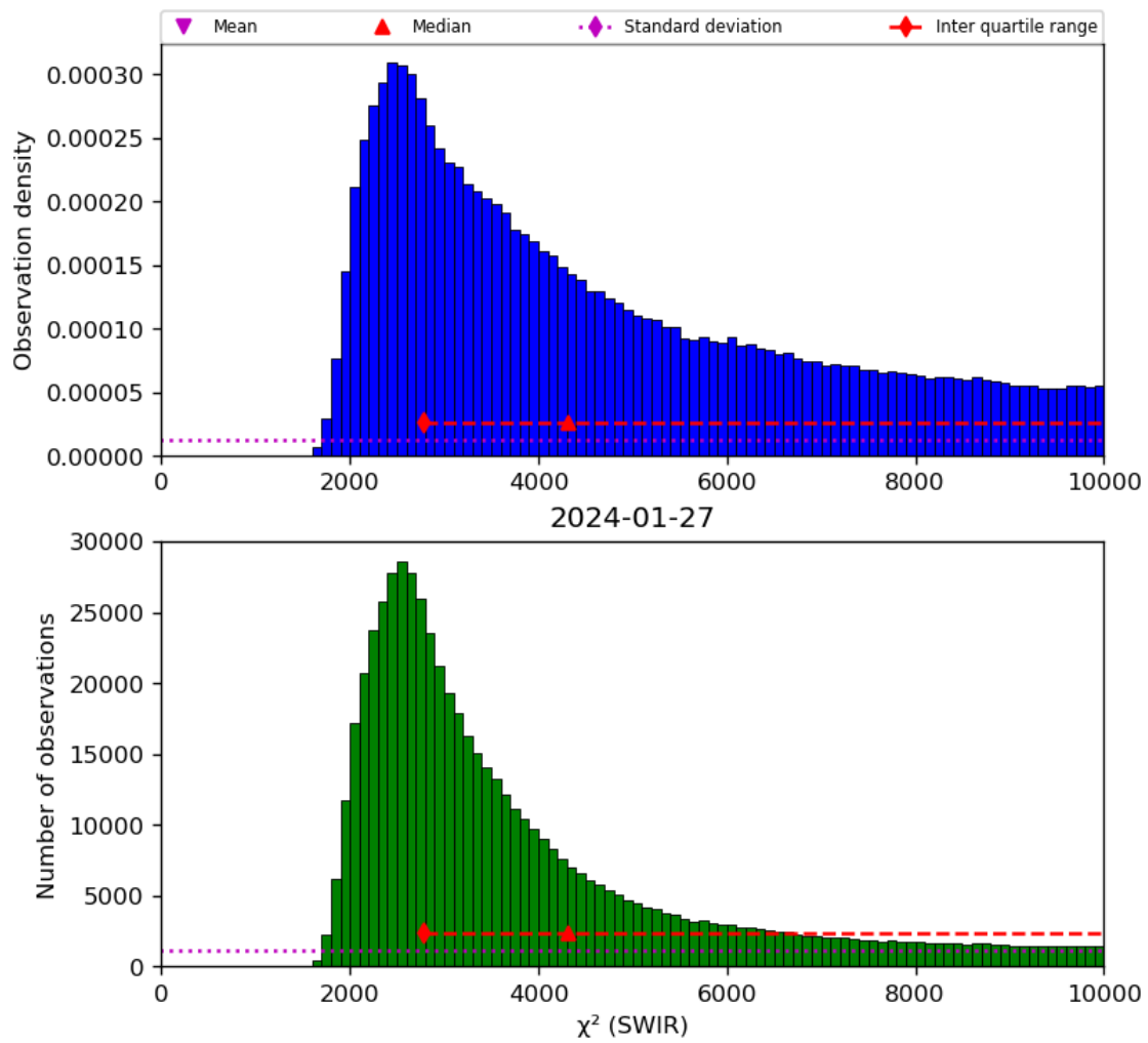
Figure 28: Histogram of “ \chi^2 (SWIR)” for 2024-01-26 to 2024-01-28
