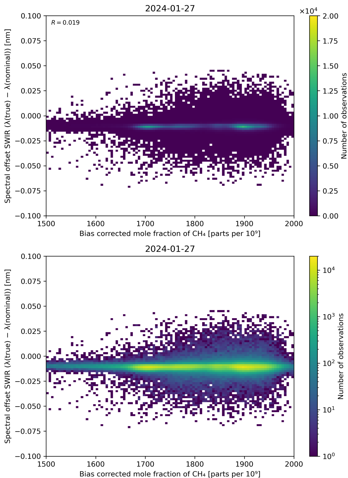
Figure 69: Scatter density plot of “Bias corrected mole fraction of \text{CH}_4 ” against “Spectral offset SWIR ( \lambda(\text{true}) - \lambda(\text{nominal}) )” for 2024-01-26 to 2024-01-28.
