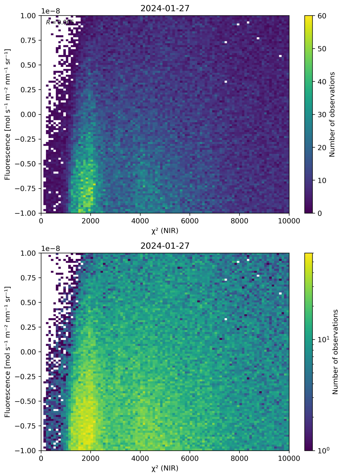
Figure 45: Scatter density plot of “ \chi^2 (NIR)” against “Fluorescence” for 2024-01-26 to 2024-01-28.
