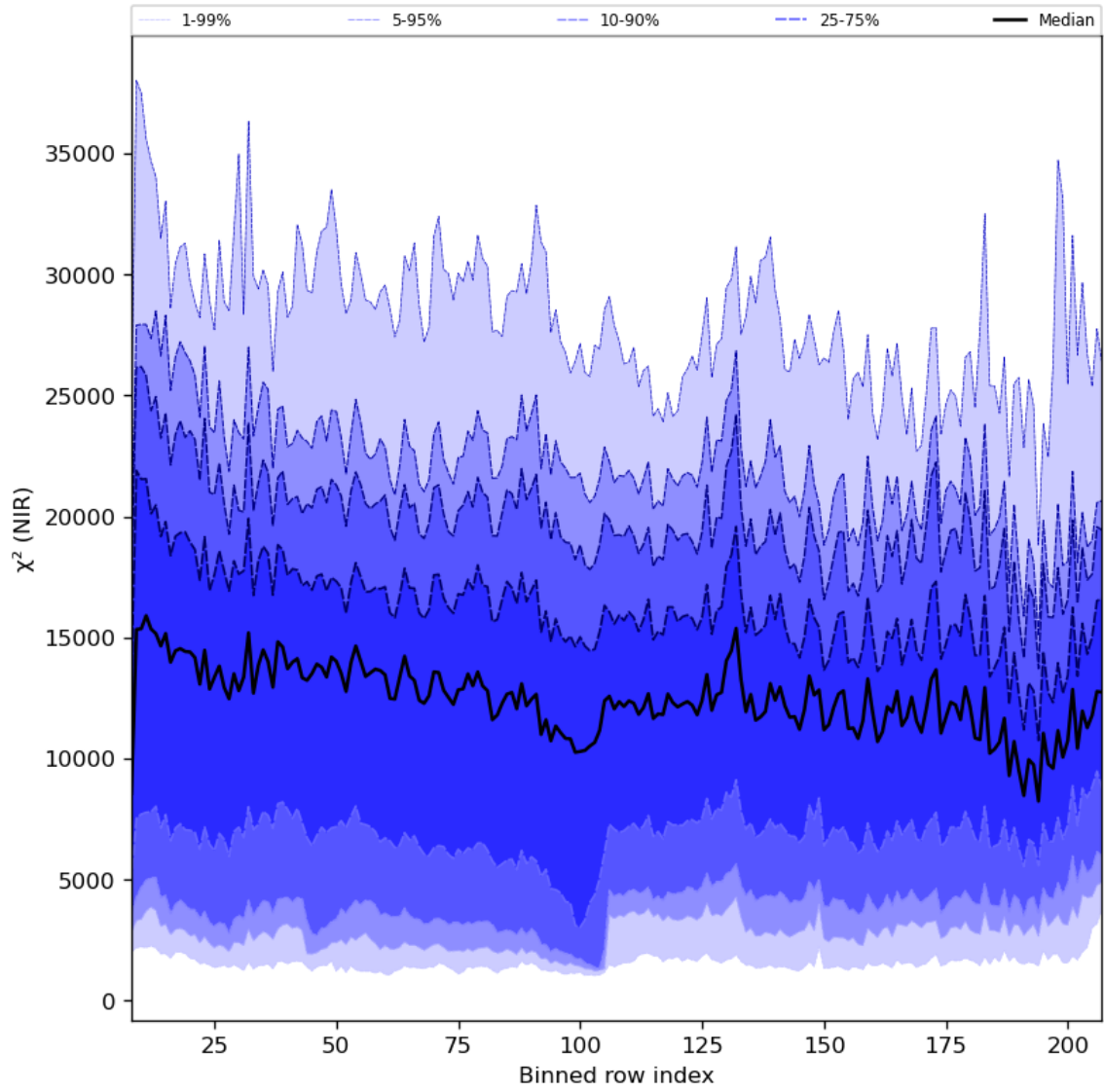
Figure 40: Along track statistics of “ \chi^2 (NIR)” for 2024-01-26 to 2024-01-28
