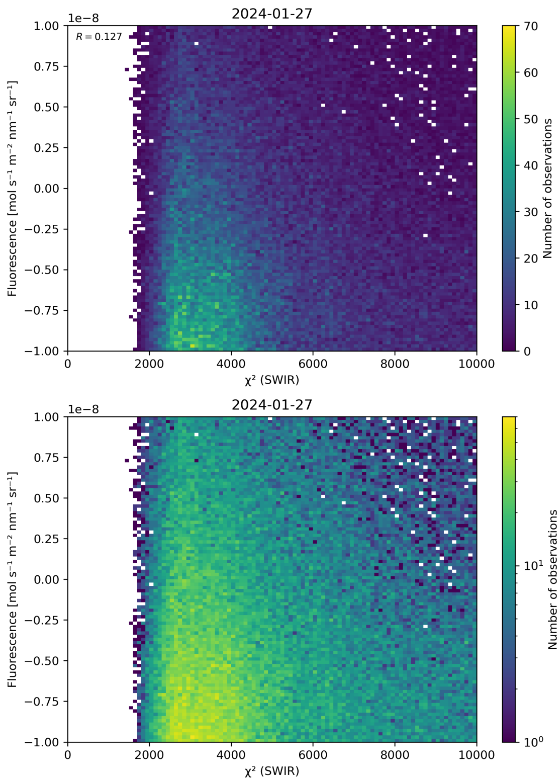
Figure 49: Scatter density plot of “ \chi^2 (SWIR)” against “Fluorescence” for 2024-01-26 to 2024-01-28.
