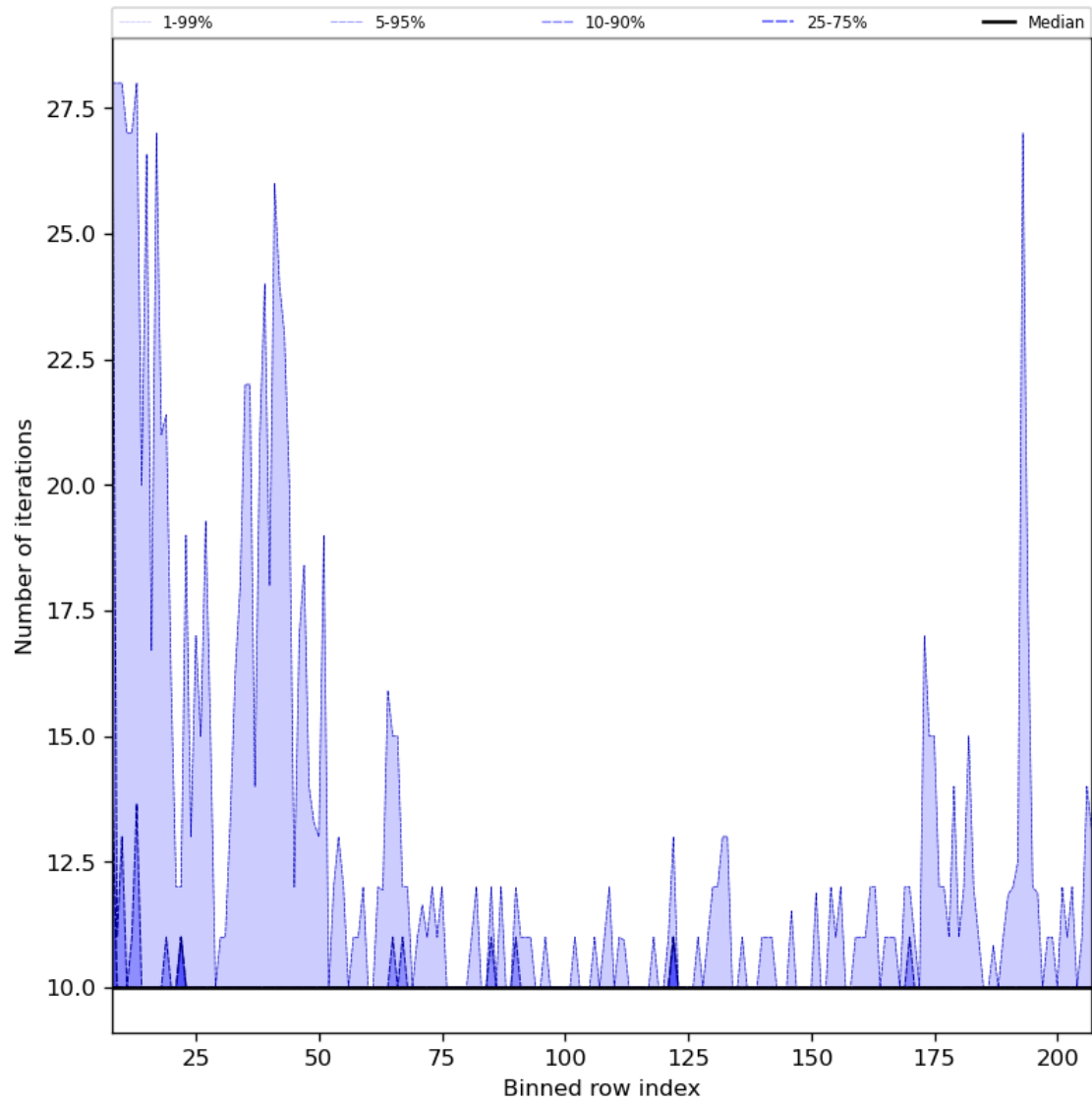
Figure 42: Along track statistics of “Number of iterations” for 2024-01-26 to 2024-01-28
