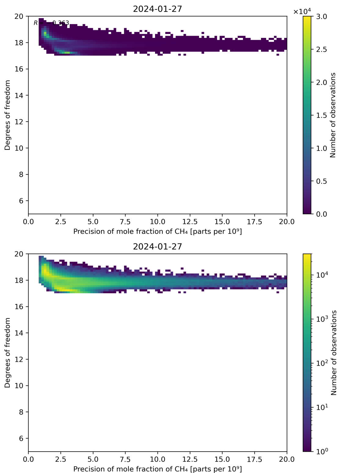
Figure 80: Scatter density plot of “Precision of mole fraction of CH 4 ” against “Degrees of freedom” for 2024-01-26 to 2024-01-28.
