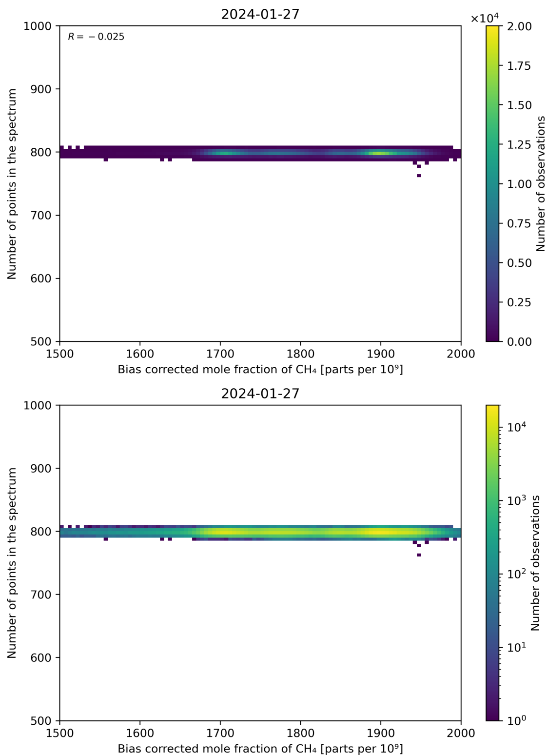
Figure 68: Scatter density plot of “Bias corrected mole fraction of CH 4 ” against “Number of points in the spectrum” for 2024-01-26 to 2024-01-28.
