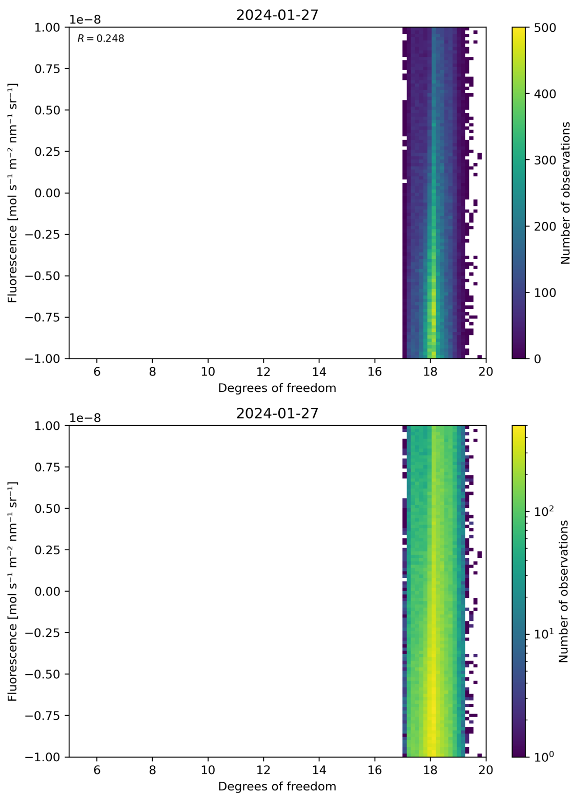
Figure 51: Scatter density plot of “Degrees of freedom” against “Fluorescence” for 2024-01-26 to 2024-01-28.
