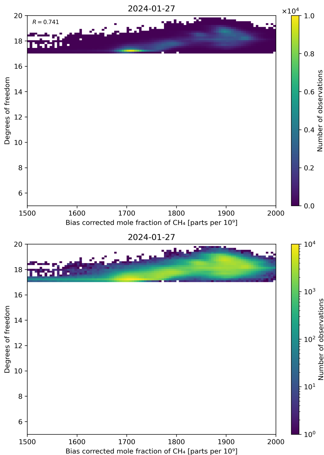
Figure 65: Scatter density plot of “Bias corrected mole fraction of \text{CH}_4 ” against “Degrees of freedom” for 2024-01-26 to 2024-01-28.
