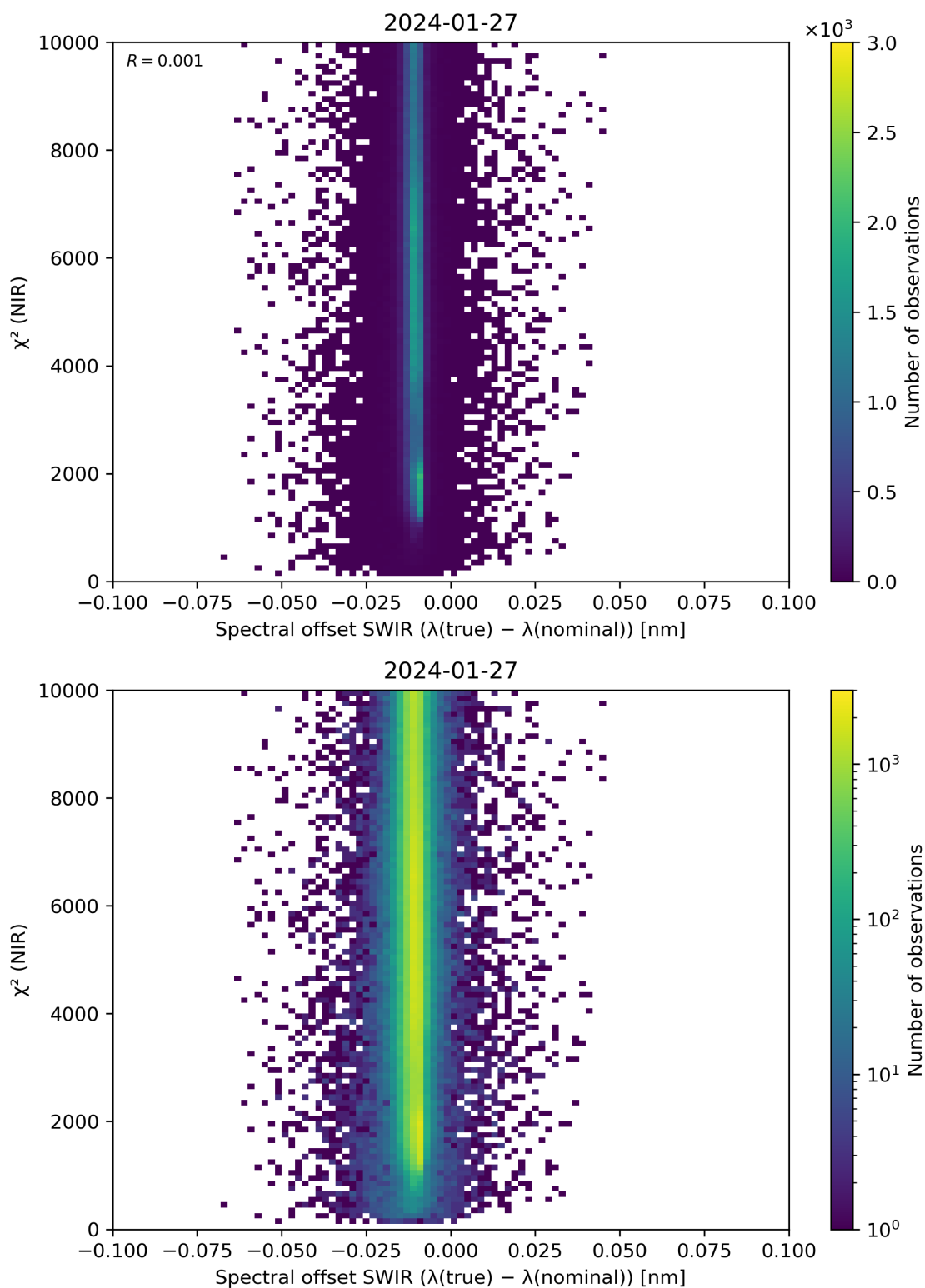
Figure 117: Scatter density plot of “Spectral offset SWIR ( \lambda(\text{true}) - \lambda(\text{nominal}) )” against “ \chi^2 (NIR)” for 2024-01-26 to 2024-01-28.
