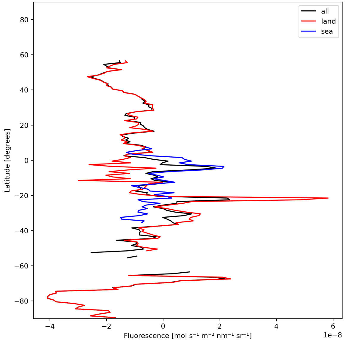
Figure 21: Zonal average of “Fluorescence” for 2024-01-26 to 2024-01-28.
