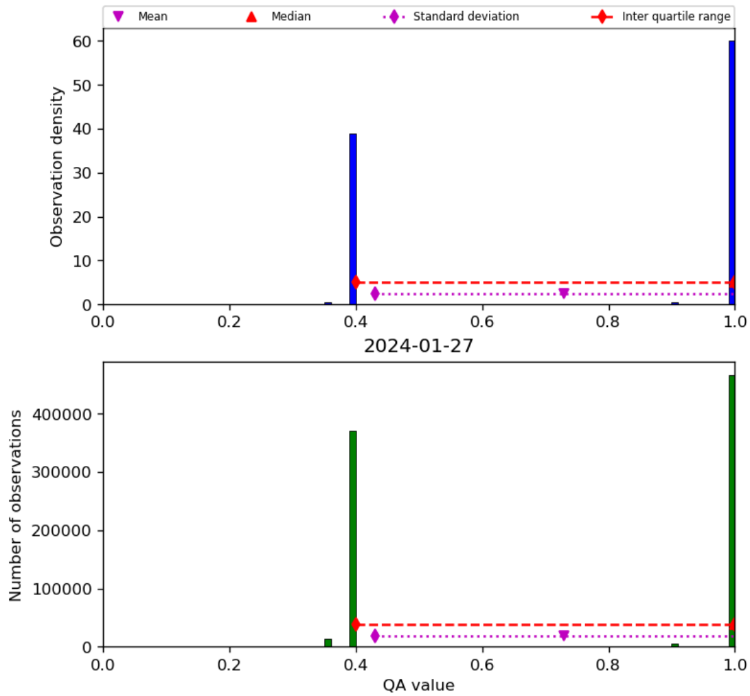
Figure 22: Histogram of “QA value” for 2024-01-26 to 2024-01-28
