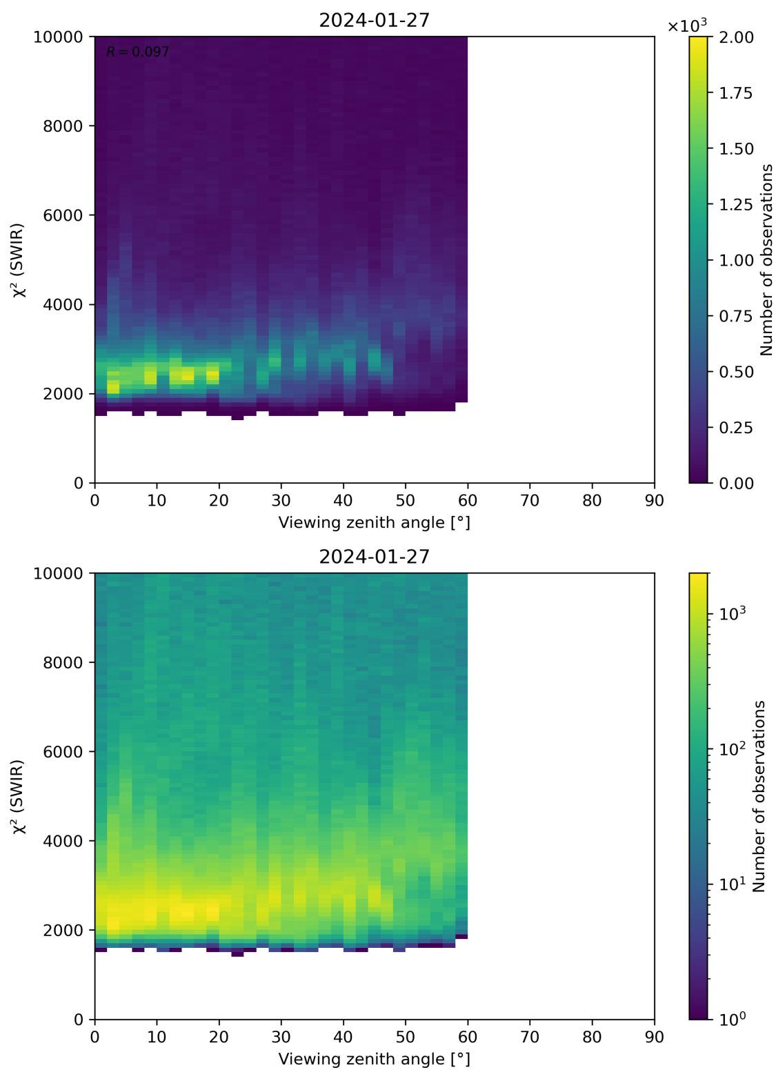
Figure 106: Scatter density plot of “Viewing zenith angle” against “ \chi^2 (SWIR)” for 2024-01-26 to 2024-01-28.
