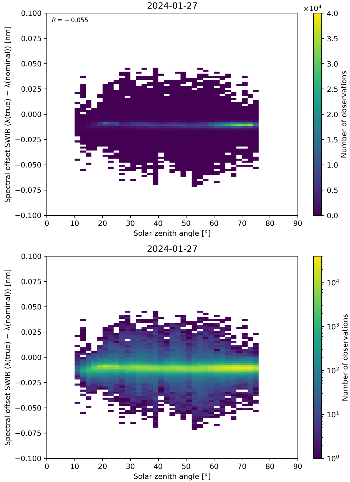
Figure 104: Scatter density plot of “Solar zenith angle” against “Spectral offset SWIR ( \lambda(\text{true}) - \lambda(\text{nominal}) )” for 2024-01-26 to 2024-01-28.
