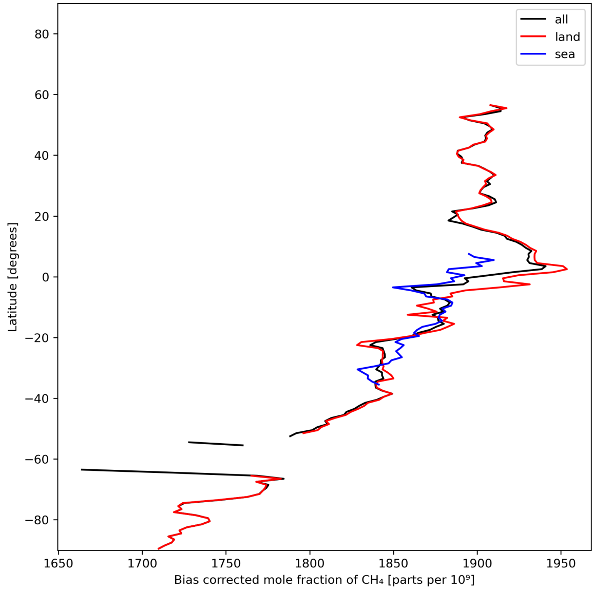
Figure 14: Zonal average of “Bias corrected mole fraction of \text{CH}_4 ” for 2024-01-26 to 2024-01-28.
