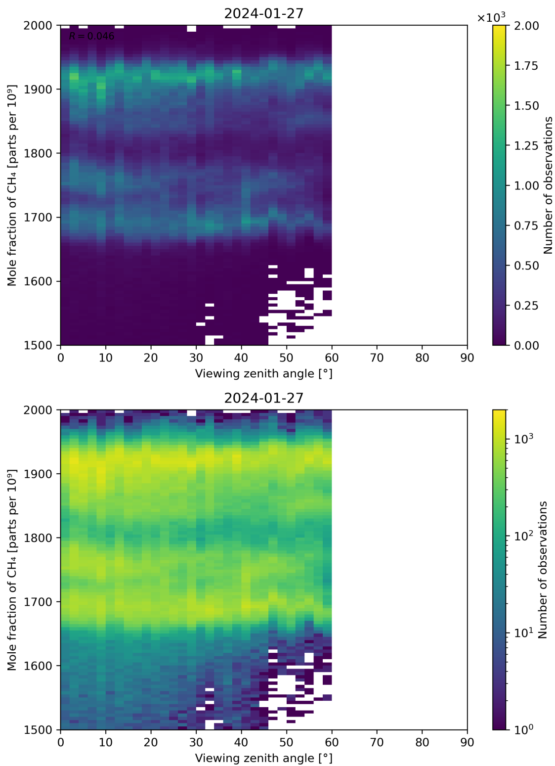
Figure 110: Scatter density plot of “Viewing zenith angle” against “Mole fraction of CH 4 ” for 2024-01-26 to 2024-01-28.
