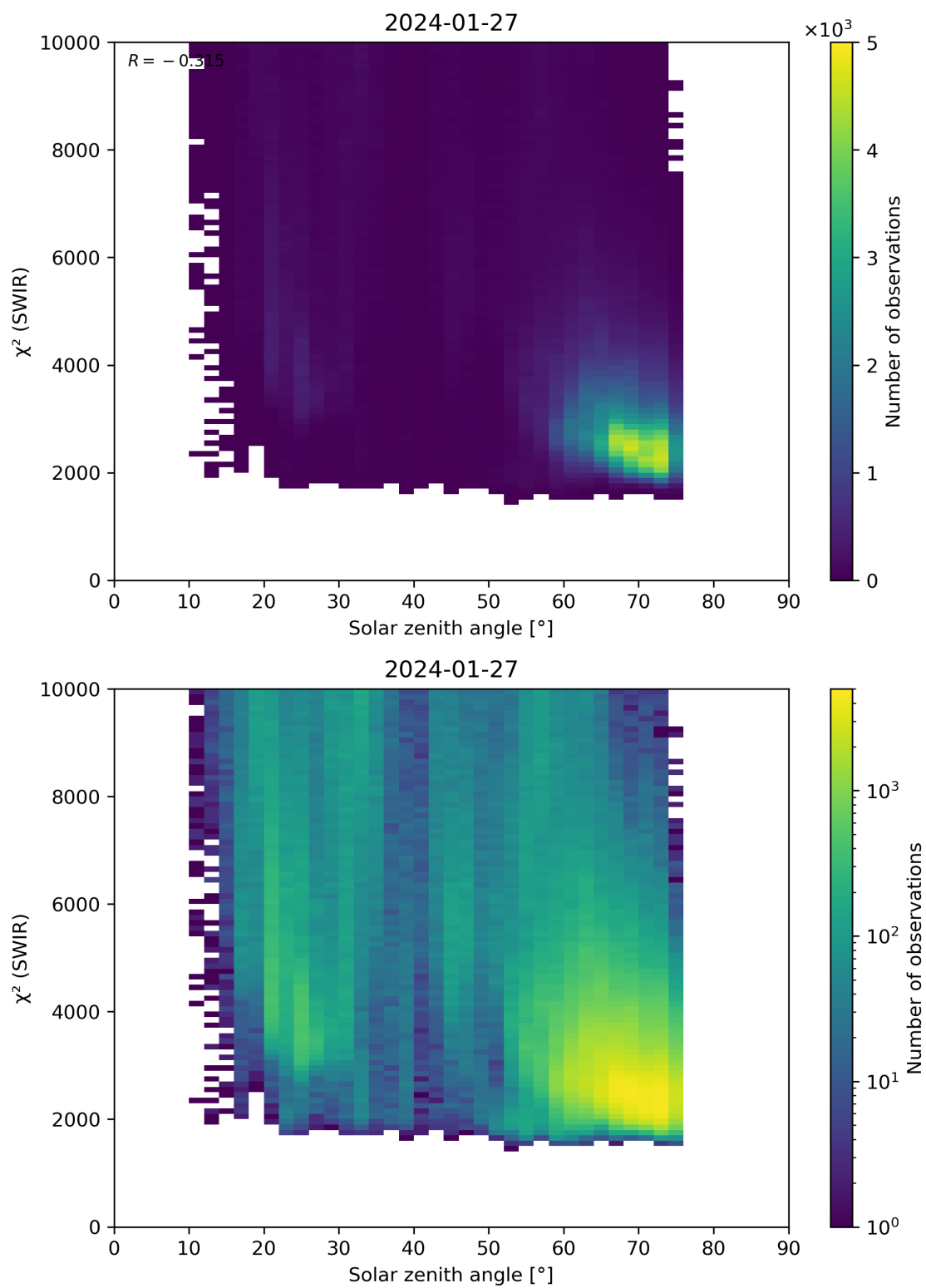
Figure 95: Scatter density plot of “Solar zenith angle” against “ \chi^2 (SWIR)” for 2024-01-26 to 2024-01-28.
