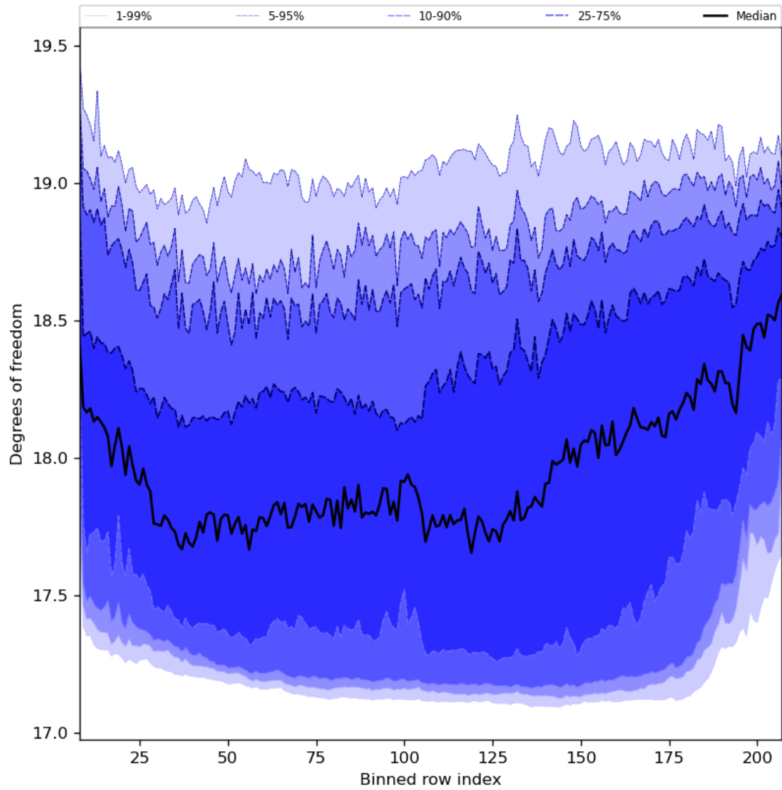
Figure 41: Along track statistics of “Degrees of freedom” for 2024-01-26 to 2024-01-28
