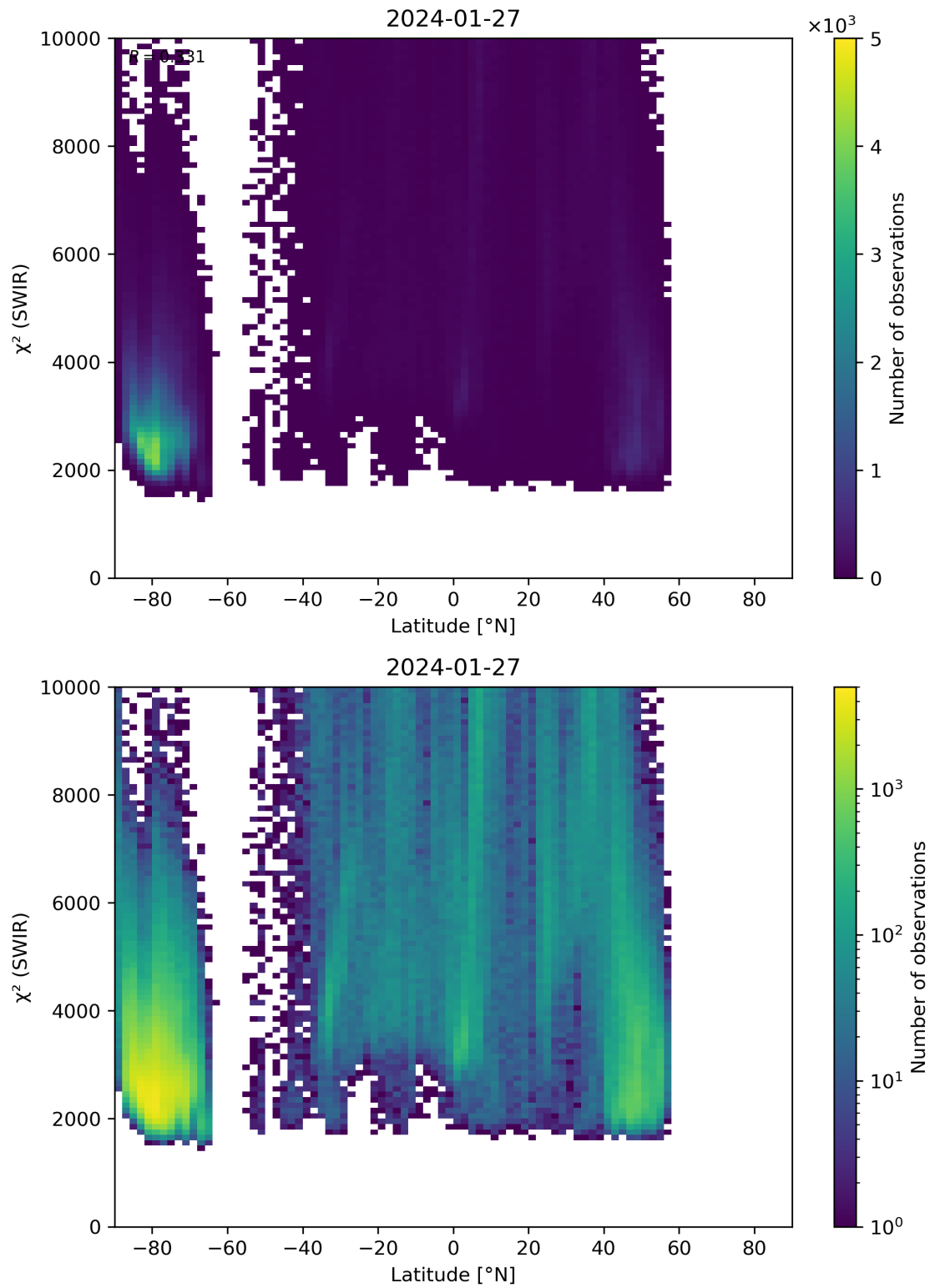
Figure 54: Scatter density plot of “Latitude” against “ \chi^2 (SWIR)” for 2024-01-26 to 2024-01-28.
