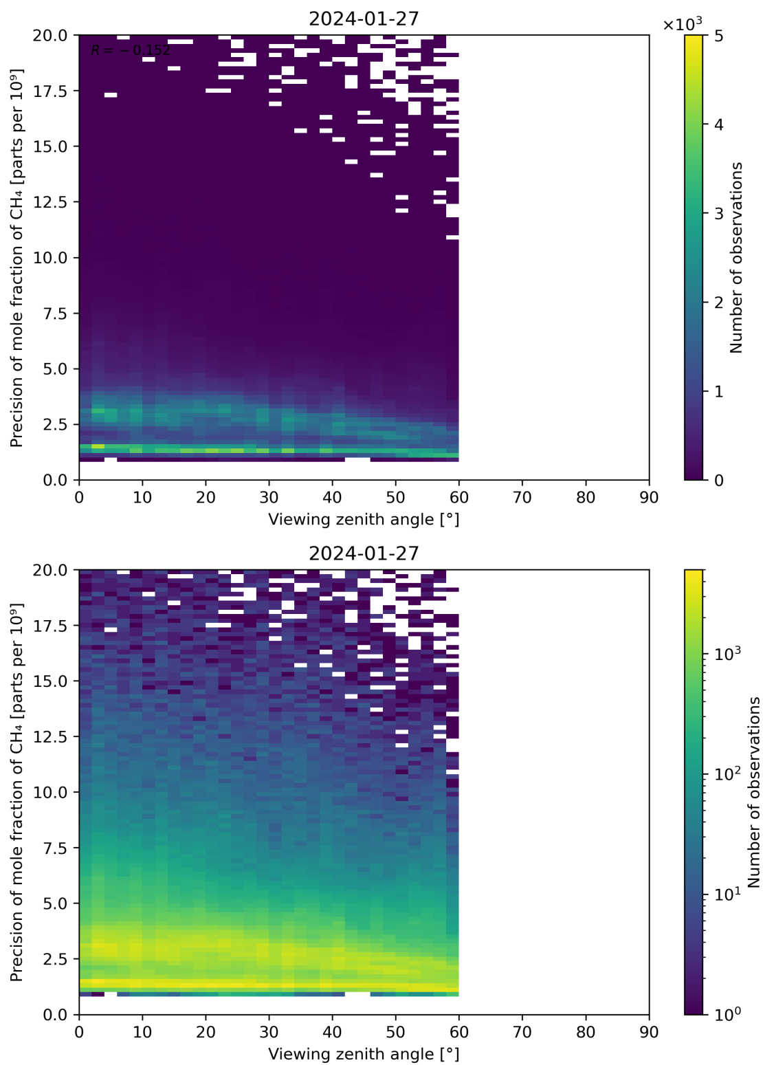
Figure 112: Scatter density plot of “Viewing zenith angle” against “Precision of mole fraction of CH 4 ” for 2024-01-26 to 2024-01-28.
