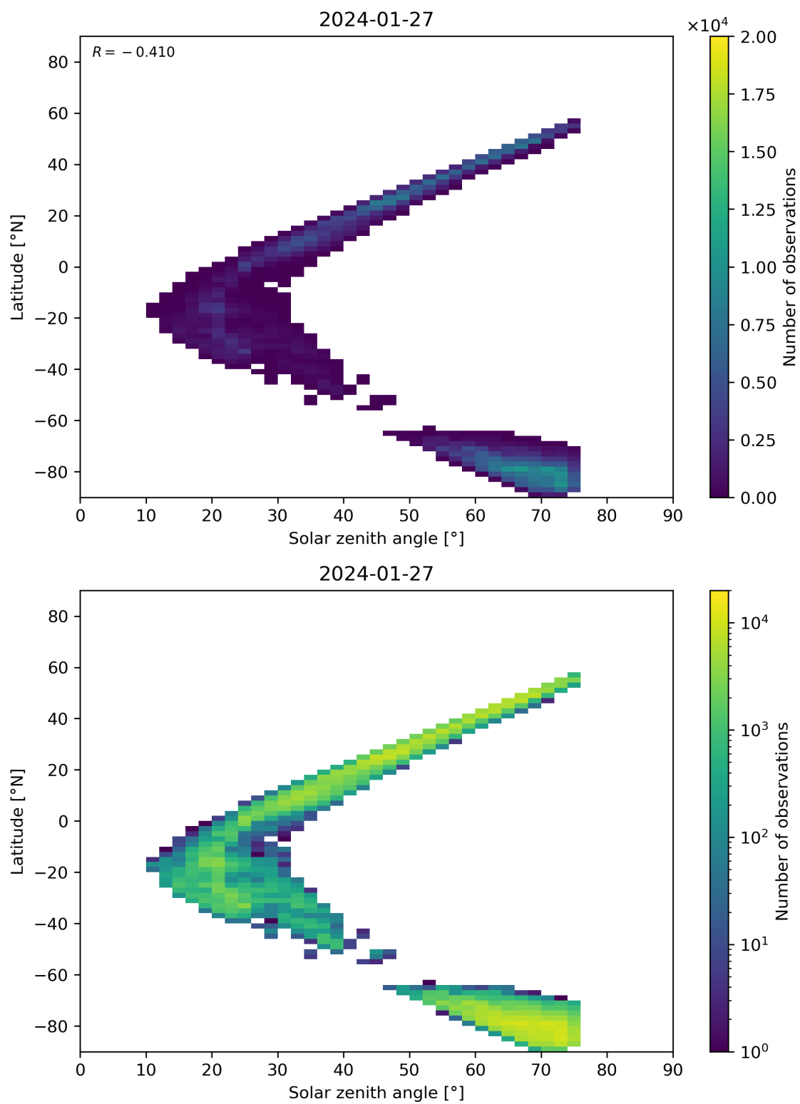
Figure 98: Scatter density plot of “Solar zenith angle” against “Latitude” for 2024-01-26 to 2024-01-28.
