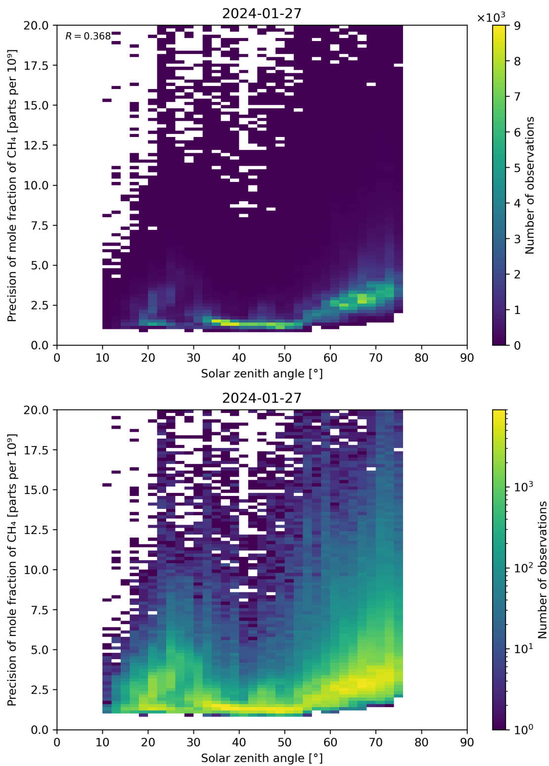
Figure 101: Scatter density plot of “Solar zenith angle” against “Precision of mole fraction of CH 4 ” for 2024-01-26 to 2024-01-28.
