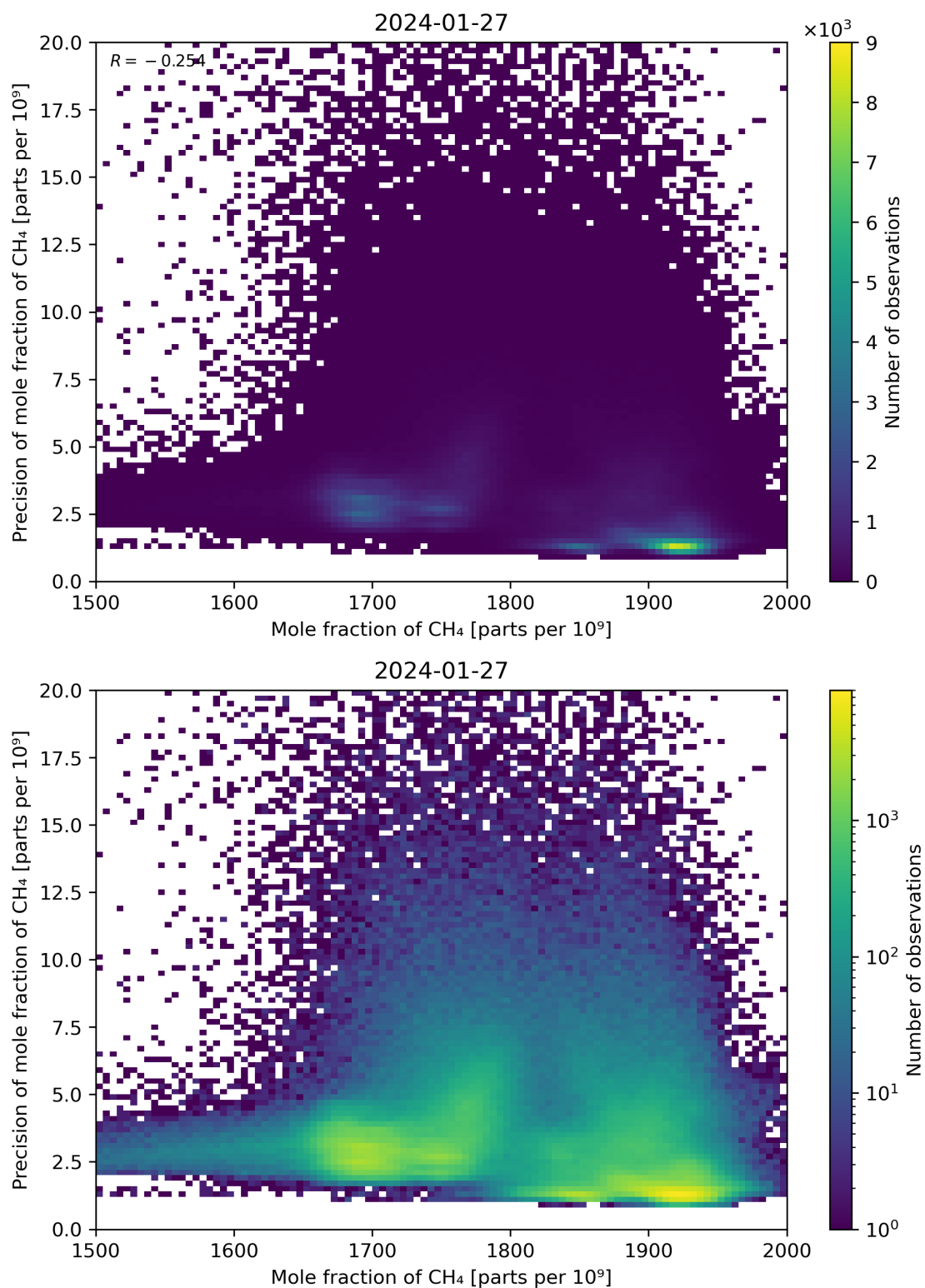
Figure 75: Scatter density plot of “Mole fraction of CH 4 ” against “Precision of mole fraction of CH 4 ” for 2024-01-26 to 2024-01-28.
