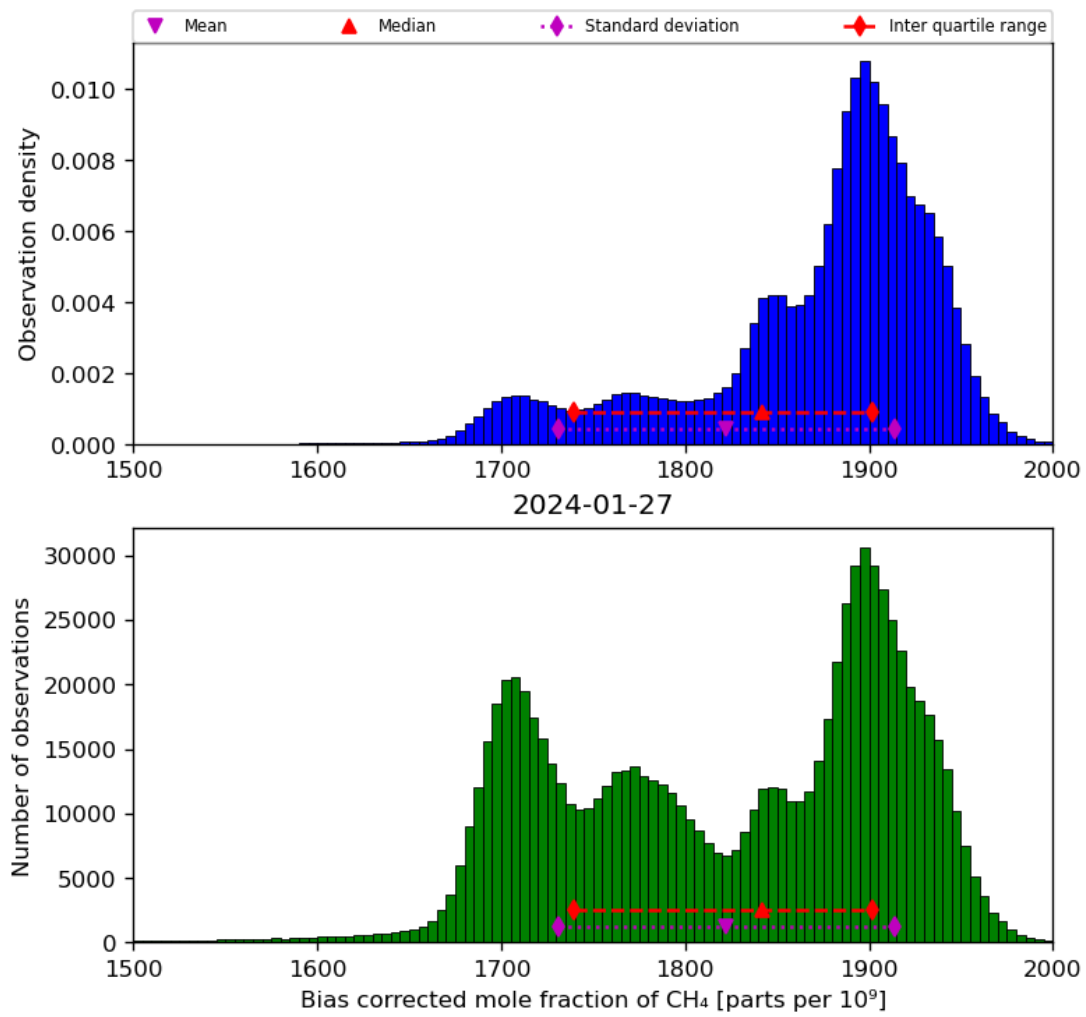
Figure 25: Histogram of “Bias corrected mole fraction of CH 4 ” for 2024-01-26 to 2024-01-28
