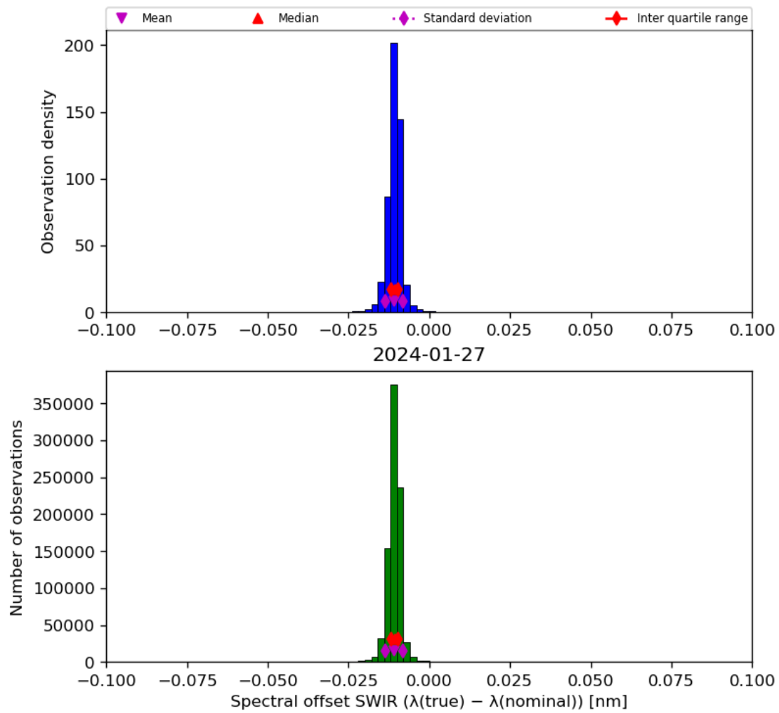
Figure 27: Histogram of “Spectral offset SWIR ( \lambda(\text{true}) - \lambda(\text{nominal}) )” for 2024-01-26 to 2024-01-28
