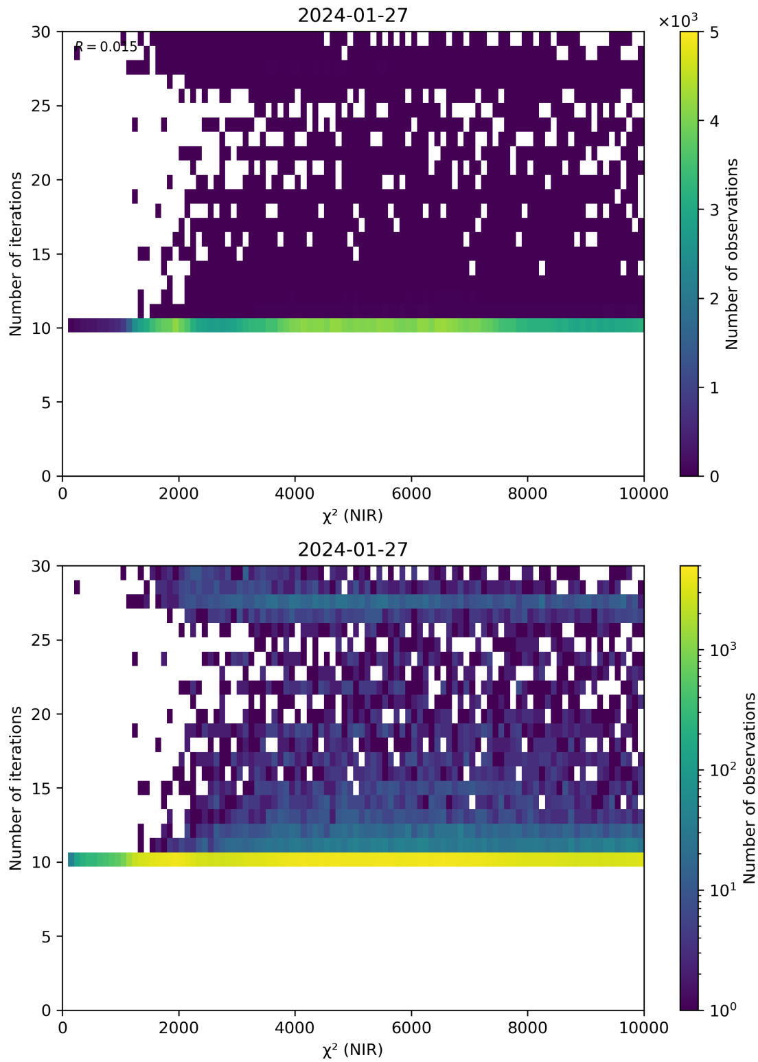
Figure 46: Scatter density plot of “ \chi^2 (NIR)” against “Number of iterations” for 2024-01-26 to 2024-01-28.
