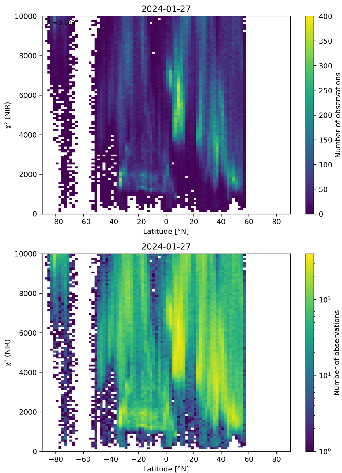
Figure 53: Scatter density plot of “Latitude” against “ \chi^2 (NIR)” for 2024-01-26 to 2024-01-28.
