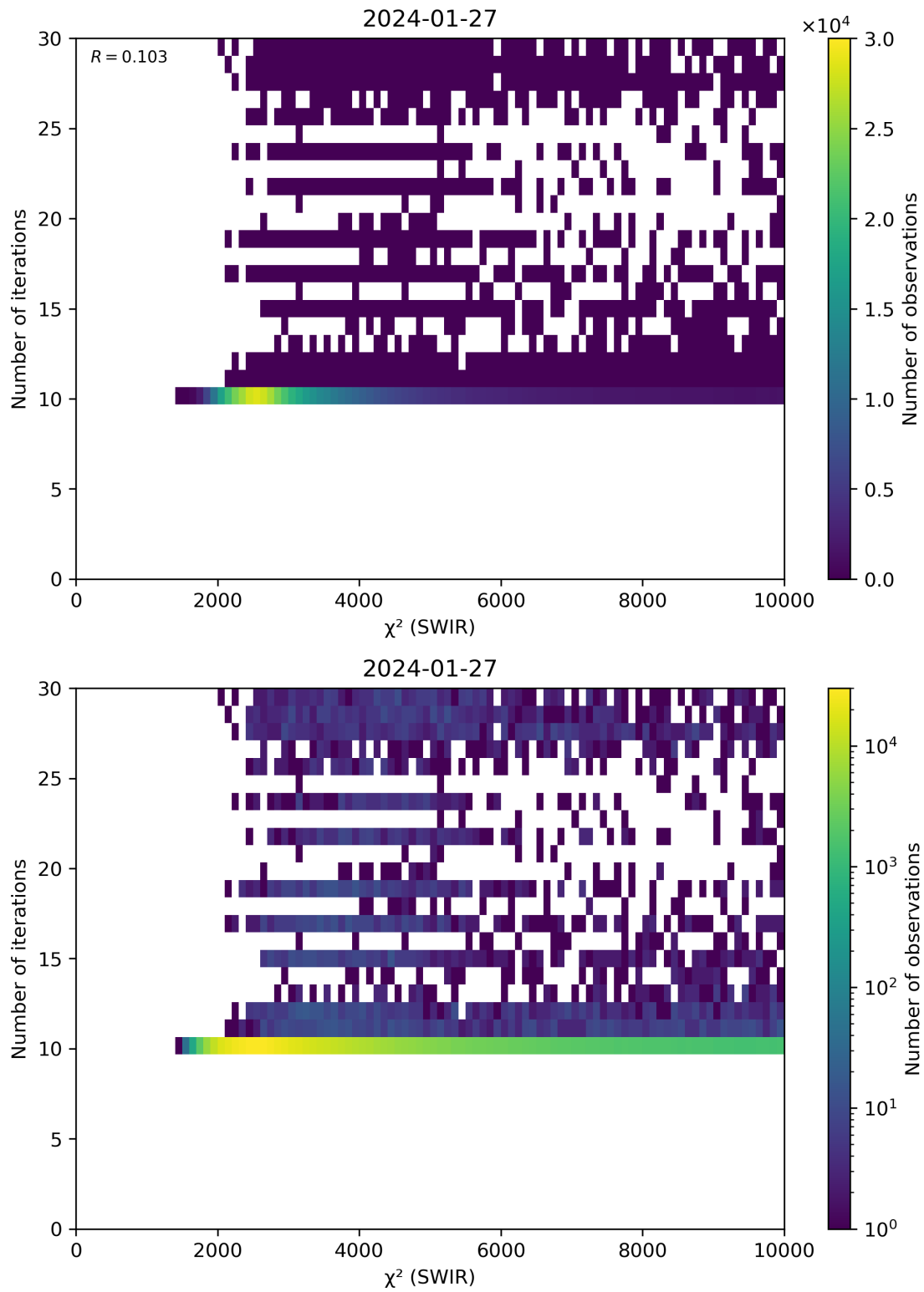
Figure 50: Scatter density plot of “ \chi^2 (SWIR)” against “Number of iterations” for 2024-01-26 to 2024-01-28.
