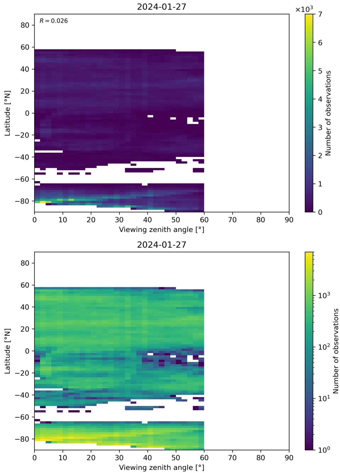
Figure 109: Scatter density plot of “Viewing zenith angle” against “Latitude” for 2024-01-26 to 2024-01-28.
