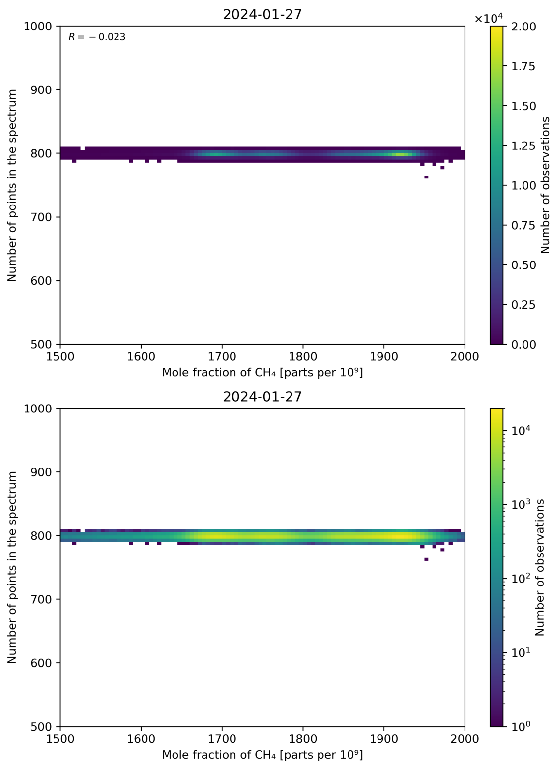
Figure 77: Scatter density plot of “Mole fraction of CH 4 ” against “Number of points in the spectrum” for 2024-01-26 to 2024-01-28.
