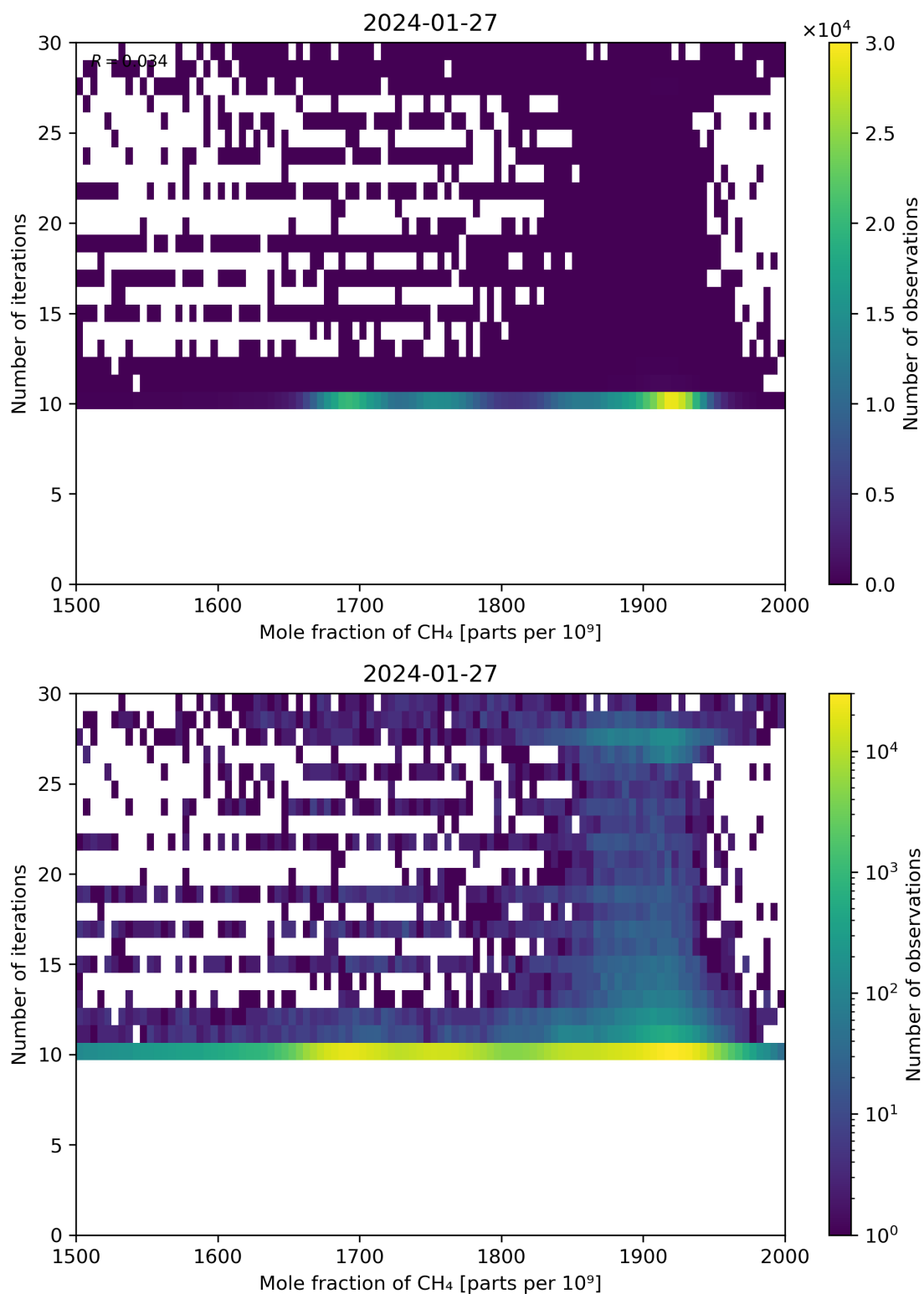
Figure 76: Scatter density plot of “Mole fraction of CH 4 ” against “Number of iterations” for 2024-01-26 to 2024-01-28.
