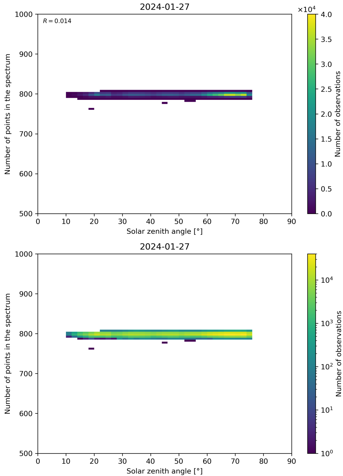
Figure 103: Scatter density plot of “Solar zenith angle” against “Number of points in the spectrum” for 2024-01-26 to 2024-01-28.
