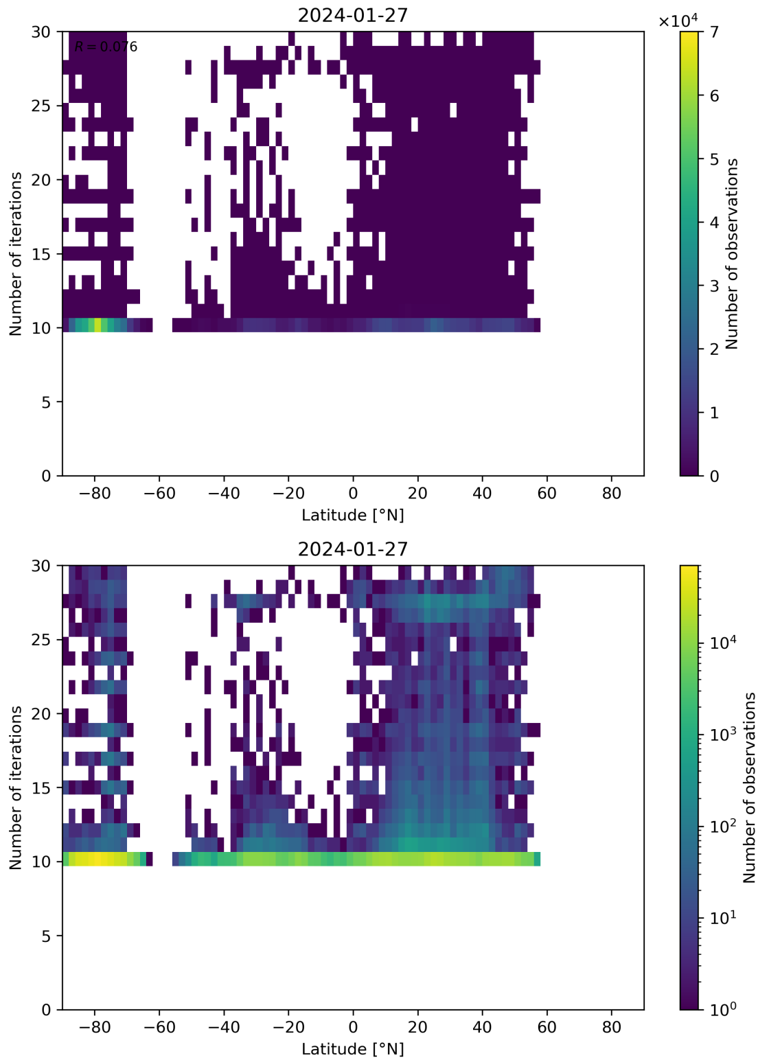
Figure 60: Scatter density plot of “Latitude” against “Number of iterations” for 2024-01-26 to 2024-01-28.
