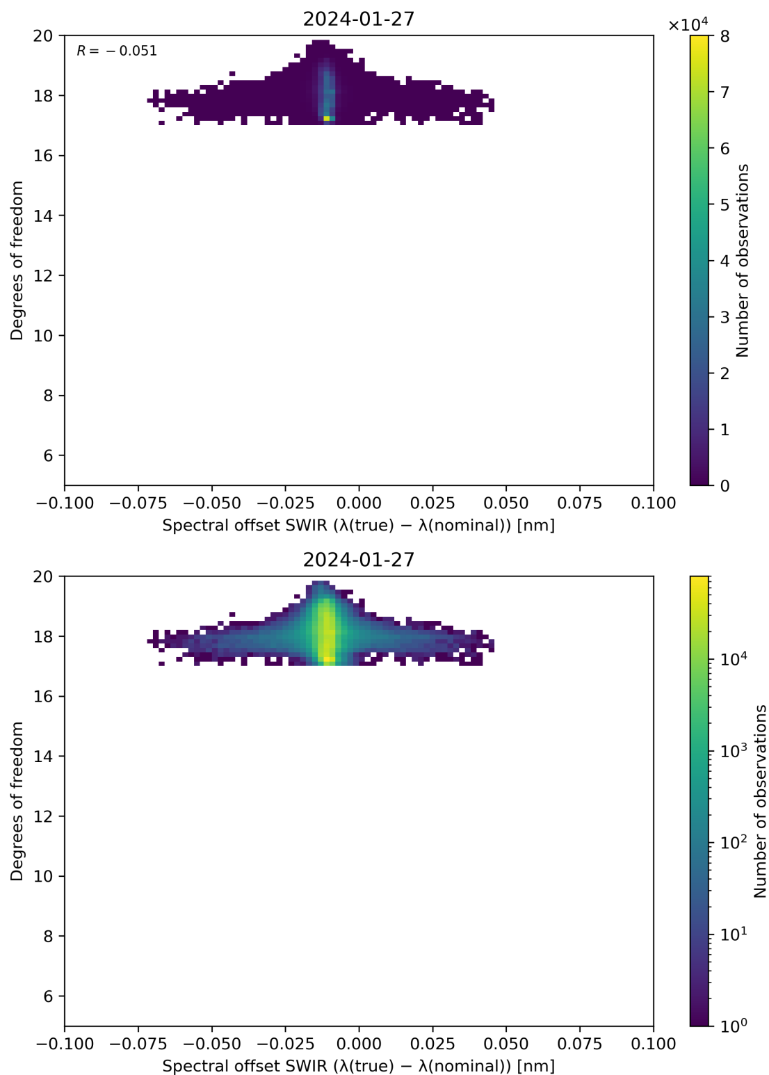
Figure 119: Scatter density plot of “Spectral offset SWIR ( \lambda(\text{true}) - \lambda(\text{nominal}) )” against “Degrees of freedom” for 2024-01-26 to 2024-01-28.
