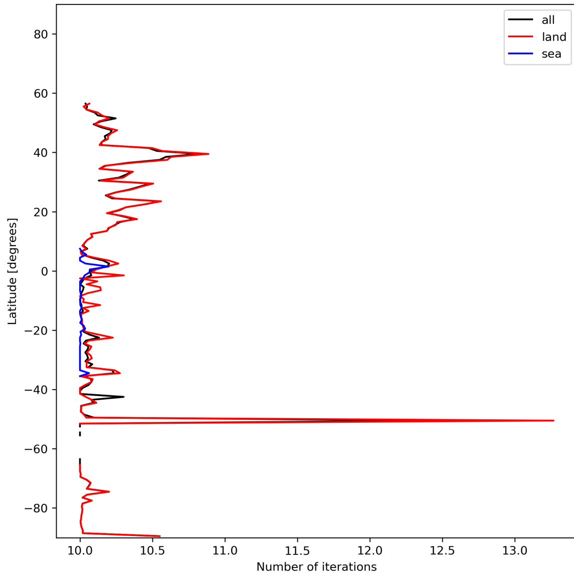
Figure 20: Zonal average of “Number of iterations” for 2024-01-26 to 2024-01-28.
