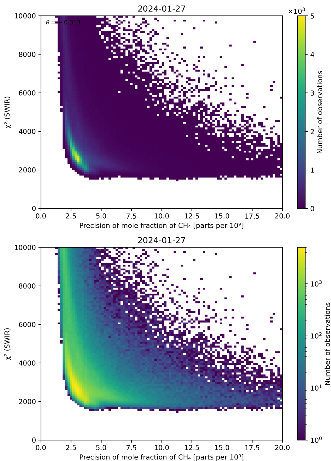
Figure 79: Scatter density plot of “Precision of mole fraction of \text{CH}_4 ” against “ \chi^2 (SWIR)” for 2024-01-26 to 2024-01-28.
