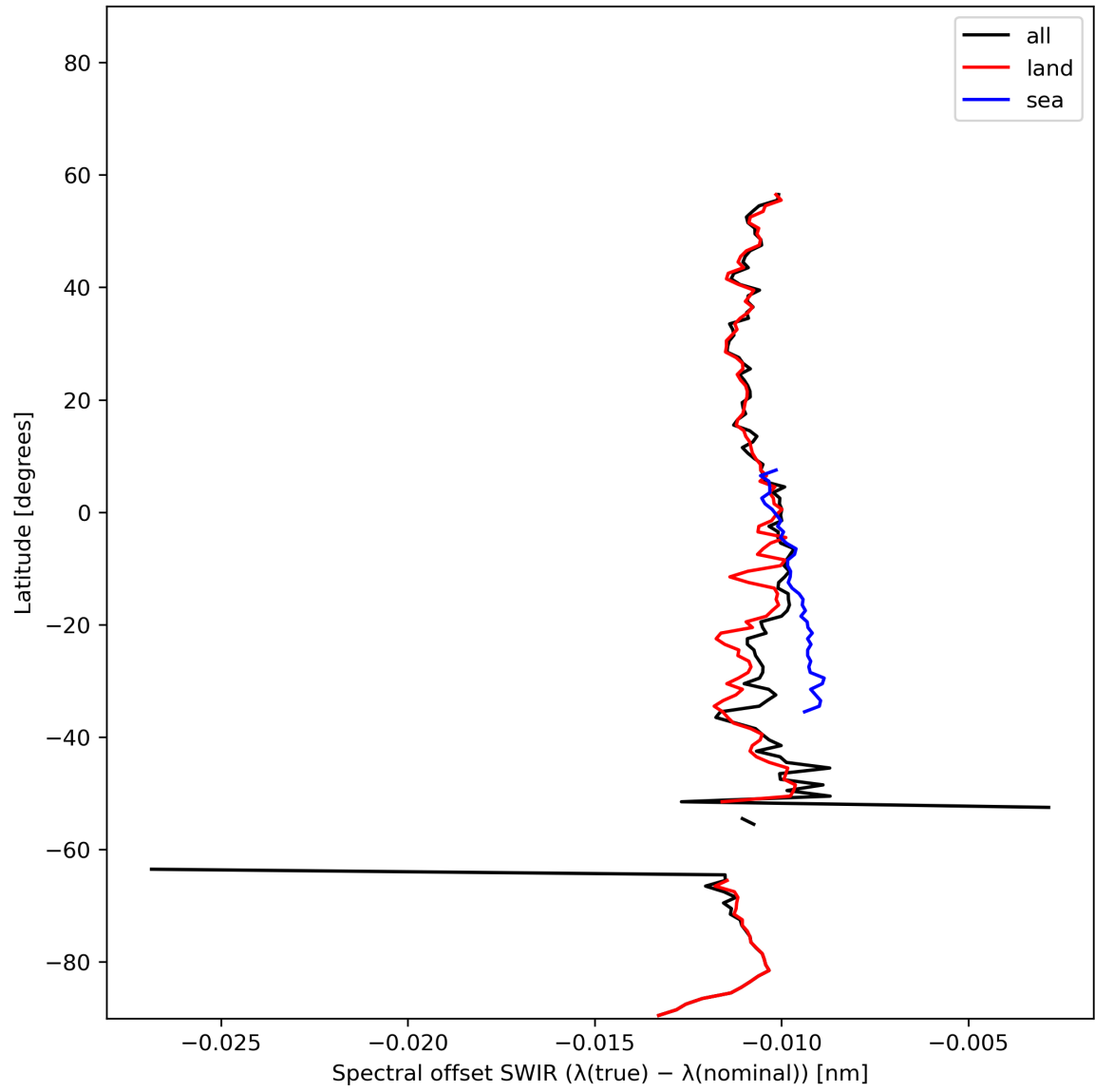
Figure 16: Zonal average of “Spectral offset SWIR ( \lambda(\text{true}) - \lambda(\text{nominal}) )” for 2024-01-26 to 2024-01-28.
