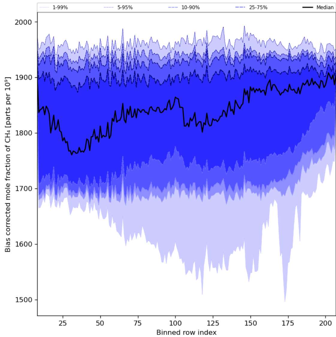
Figure 36: Along track statistics of “Bias corrected mole fraction of CH 4 ” for 2024-01-26 to 2024-01-28
