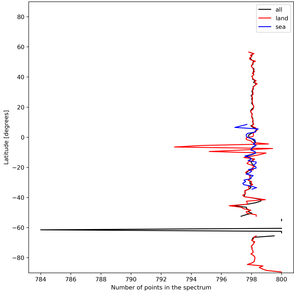
Figure 15: Zonal average of “Number of points in the spectrum” for 2024-01-27 to 2024-01-29.
