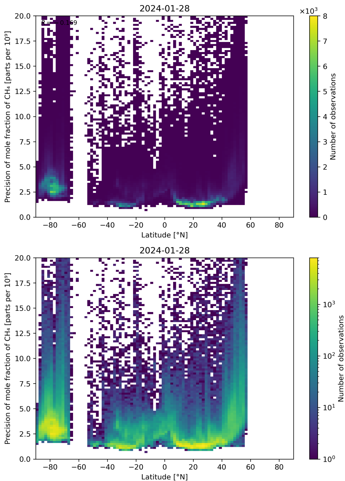
Figure 59: Scatter density plot of “Latitude” against “Precision of mole fraction of CH 4 ” for 2024-01-27 to 2024-01-29.
