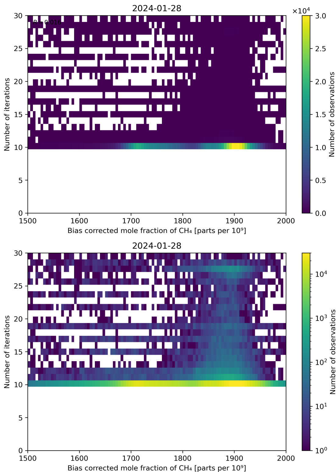
Figure 67: Scatter density plot of “Bias corrected mole fraction of CH 4 ” against “Number of iterations” for 2024-01-27 to 2024-01-29.
