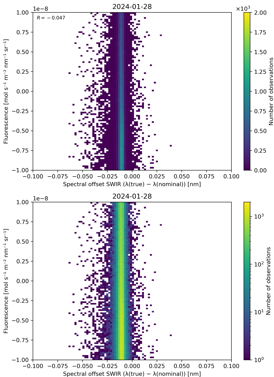
Figure 120: Scatter density plot of “Spectral offset SWIR ( \lambda(\text{true}) - \lambda(\text{nominal}) )” against “Fluorescence” for 2024-01-27 to 2024-01-29.
