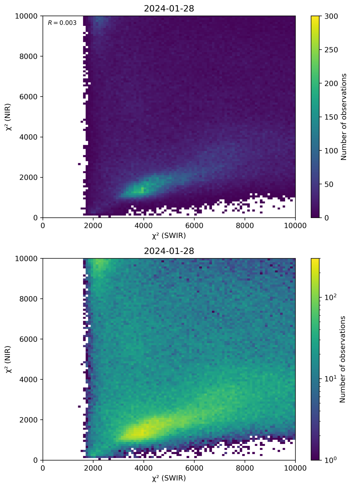
Figure 47: Scatter density plot of “ \chi^2 (SWIR)” against “ \chi^2 (NIR)” for 2024-01-27 to 2024-01-29.
