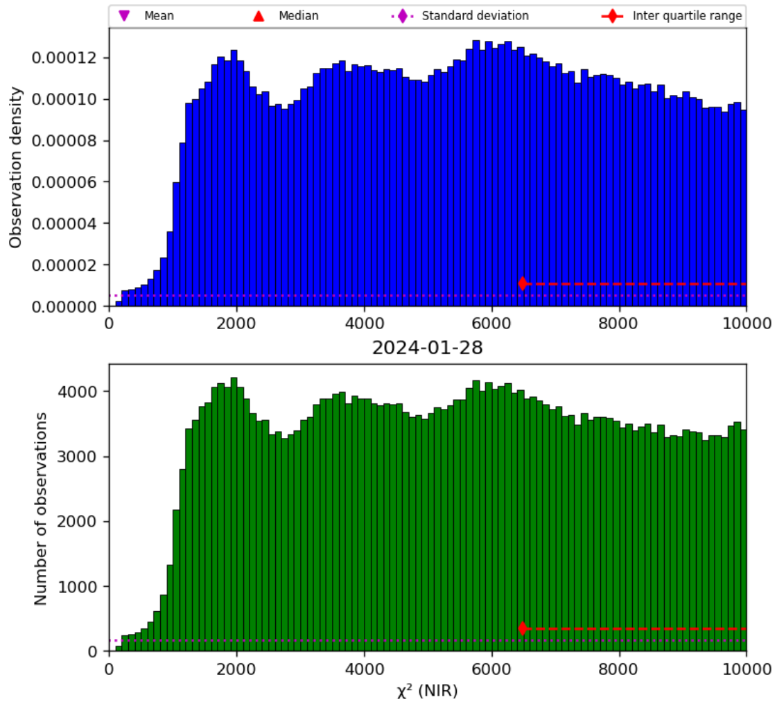
Figure 29: Histogram of “ \chi^2 (NIR)” for 2024-01-27 to 2024-01-29
