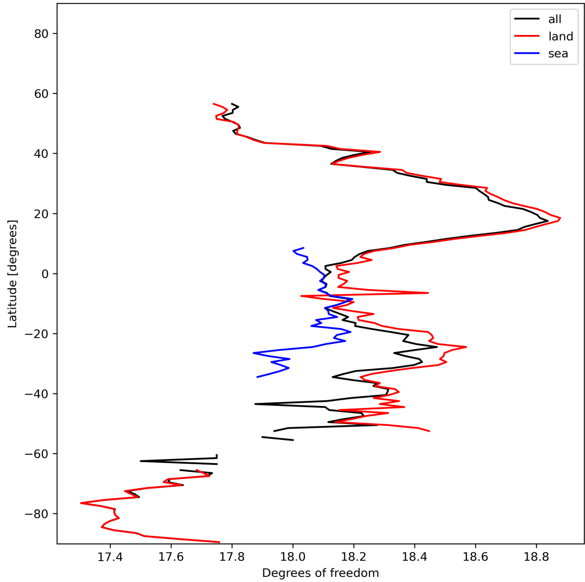
Figure 19: Zonal average of “Degrees of freedom” for 2024-01-27 to 2024-01-29.
