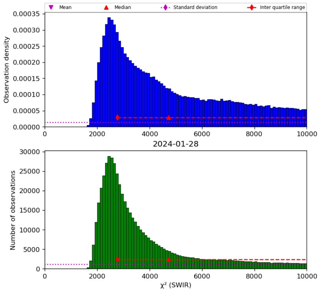
Figure 28: Histogram of “ \chi^2 (SWIR)” for 2024-01-27 to 2024-01-29
