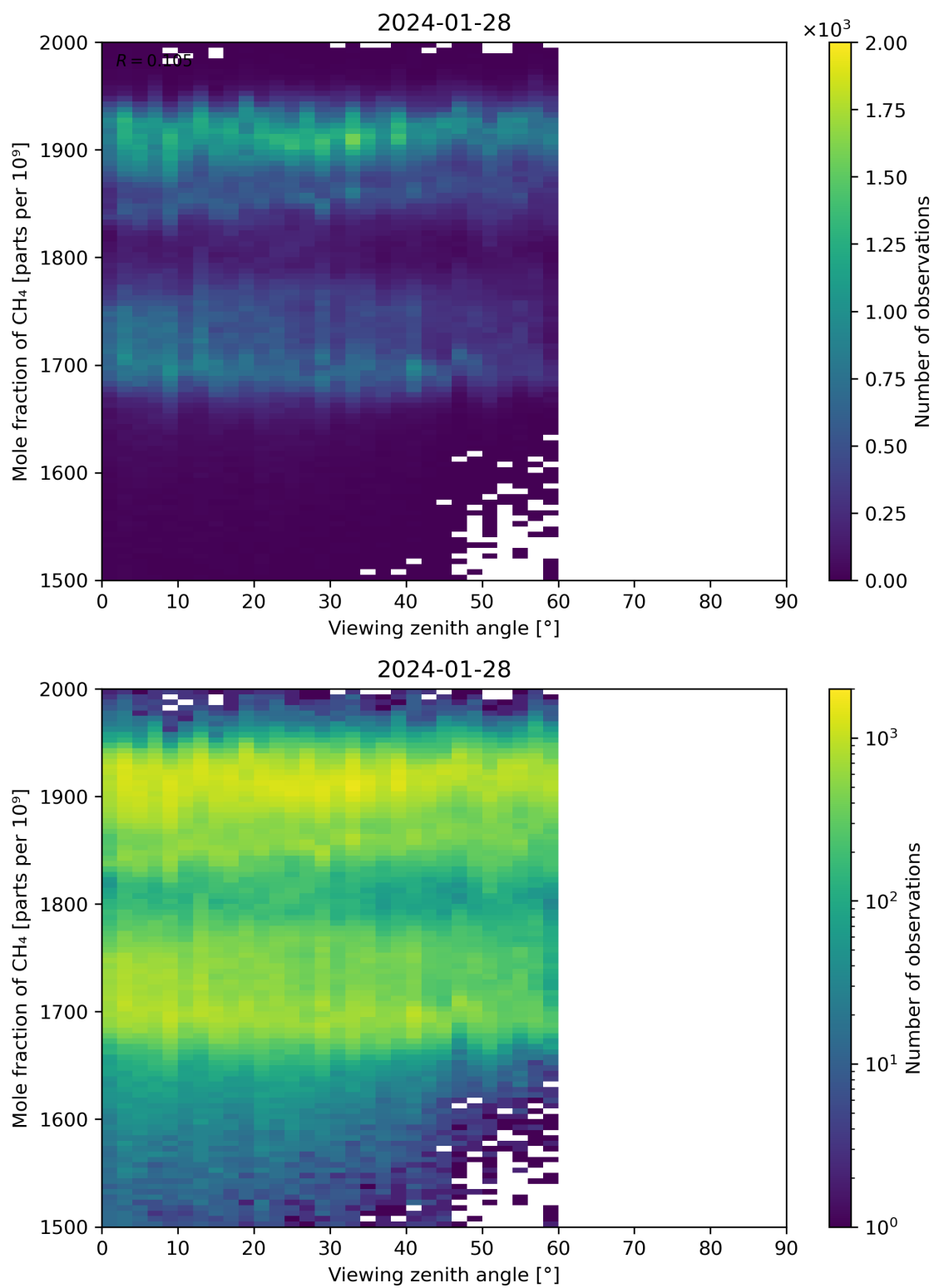
Figure 110: Scatter density plot of “Viewing zenith angle” against “Mole fraction of CH 4 ” for 2024-01-27 to 2024-01-29.
