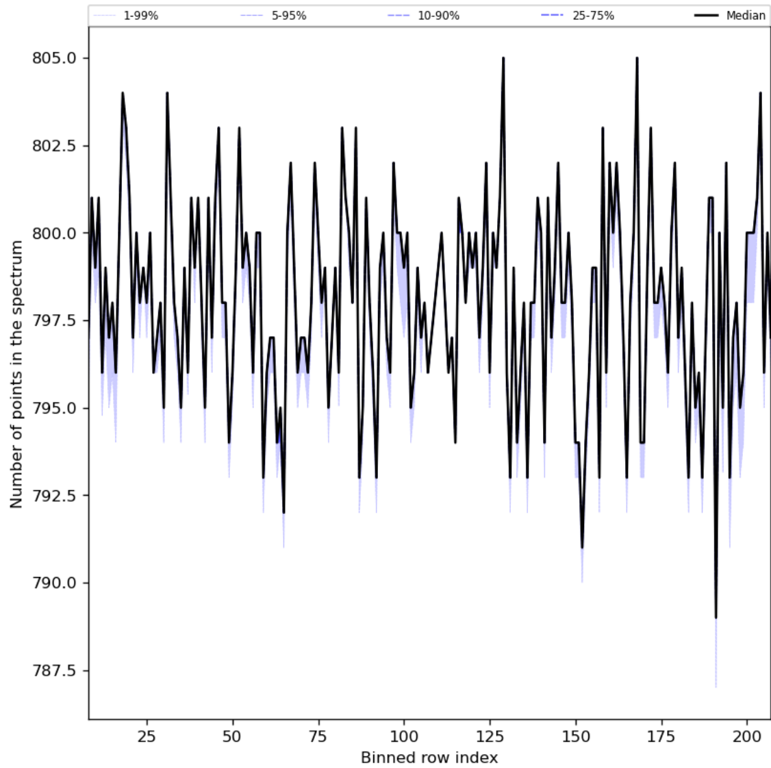
Figure 37: Along track statistics of “Number of points in the spectrum” for 2024-01-27 to 2024-01-29
