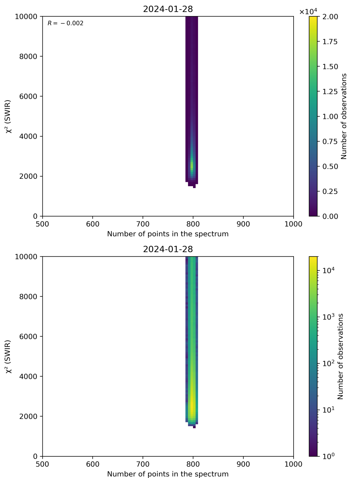
Figure 89: Scatter density plot of “Number of points in the spectrum” against “ \chi^2 (SWIR)” for 2024-01-27 to 2024-01-29.
