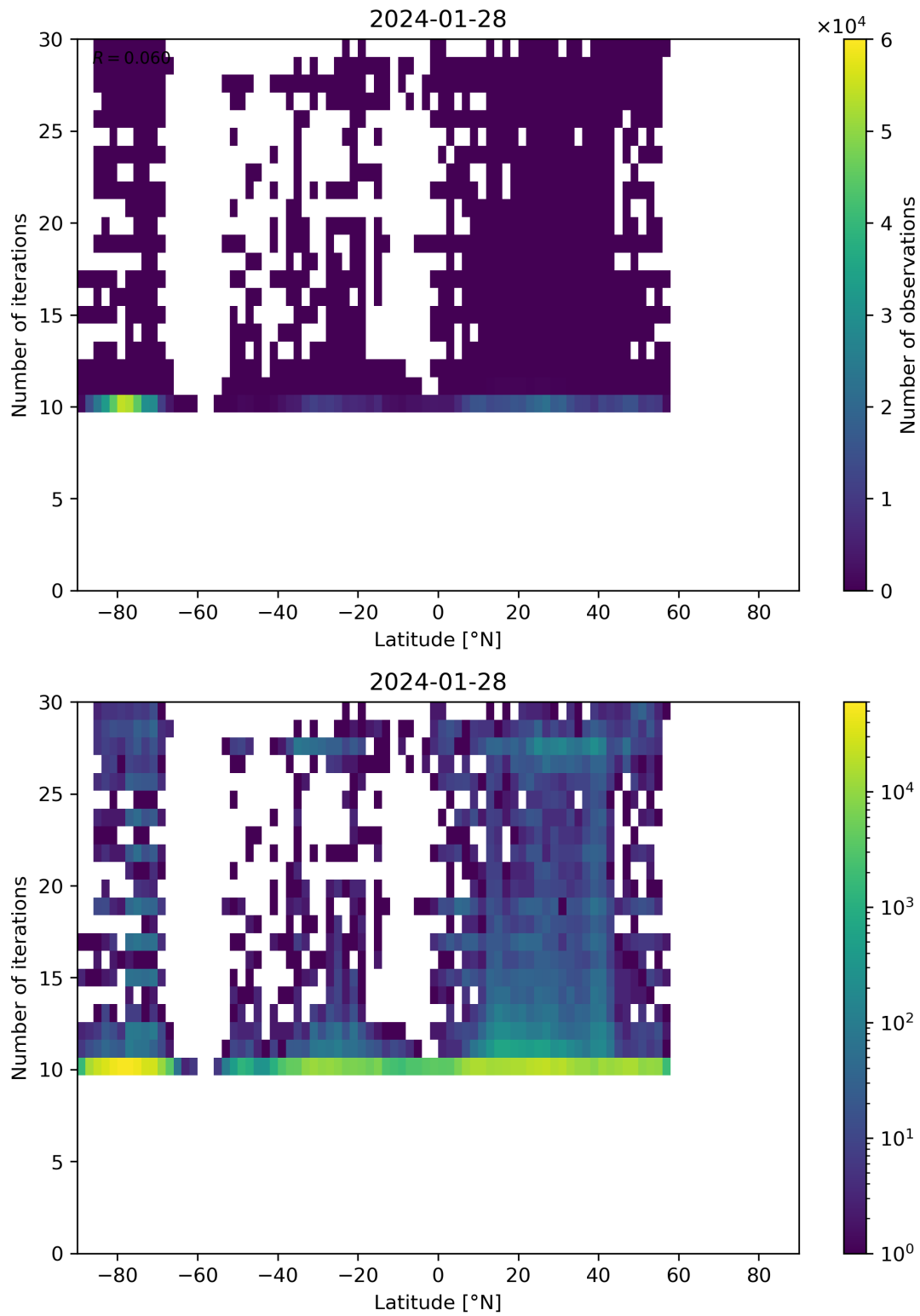
Figure 60: Scatter density plot of “Latitude” against “Number of iterations” for 2024-01-27 to 2024-01-29.
