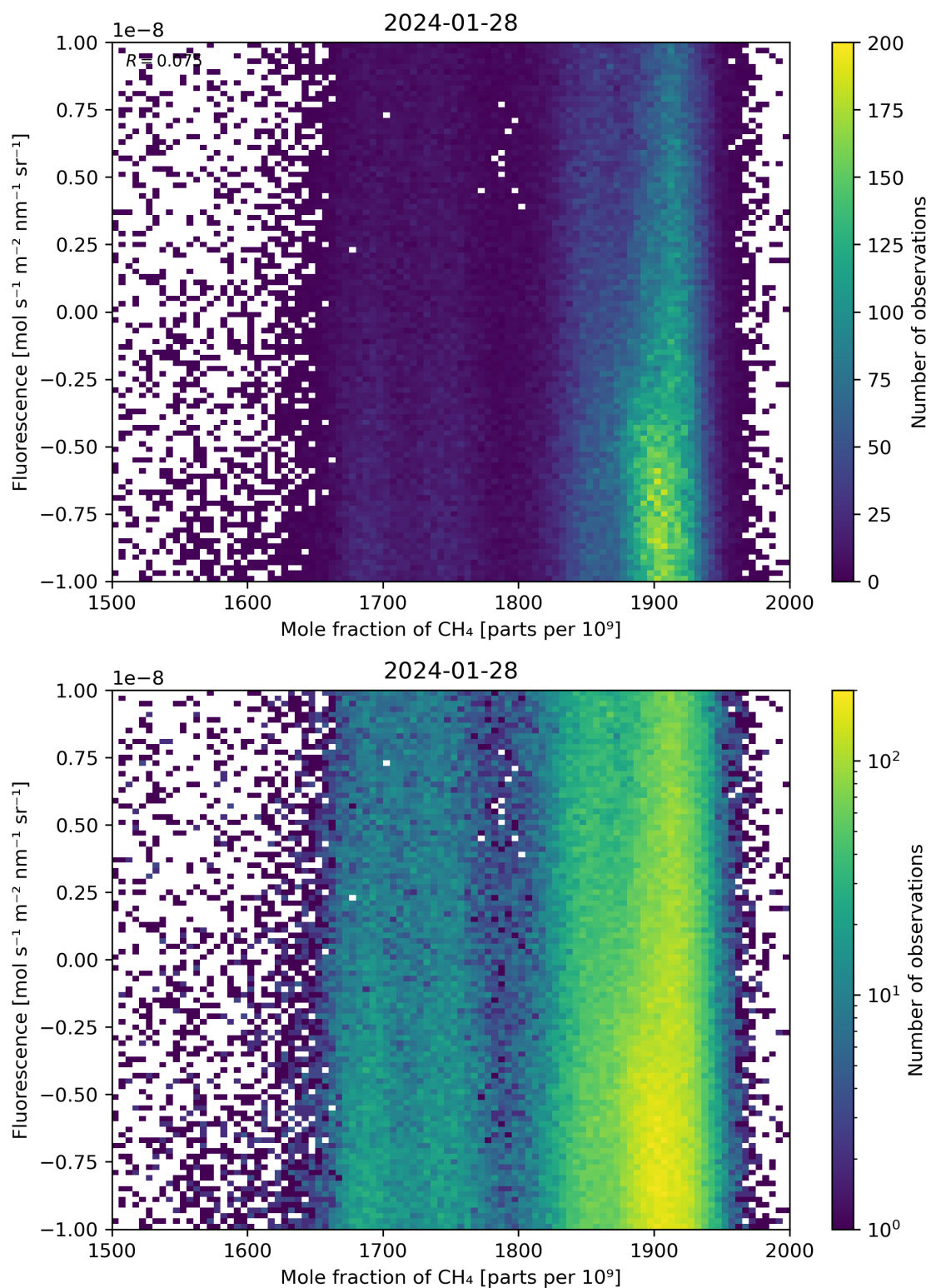
Figure 73: Scatter density plot of “Mole fraction of \text{CH}_4 ” against “Fluorescence” for 2024-01-27 to 2024-01-29.
