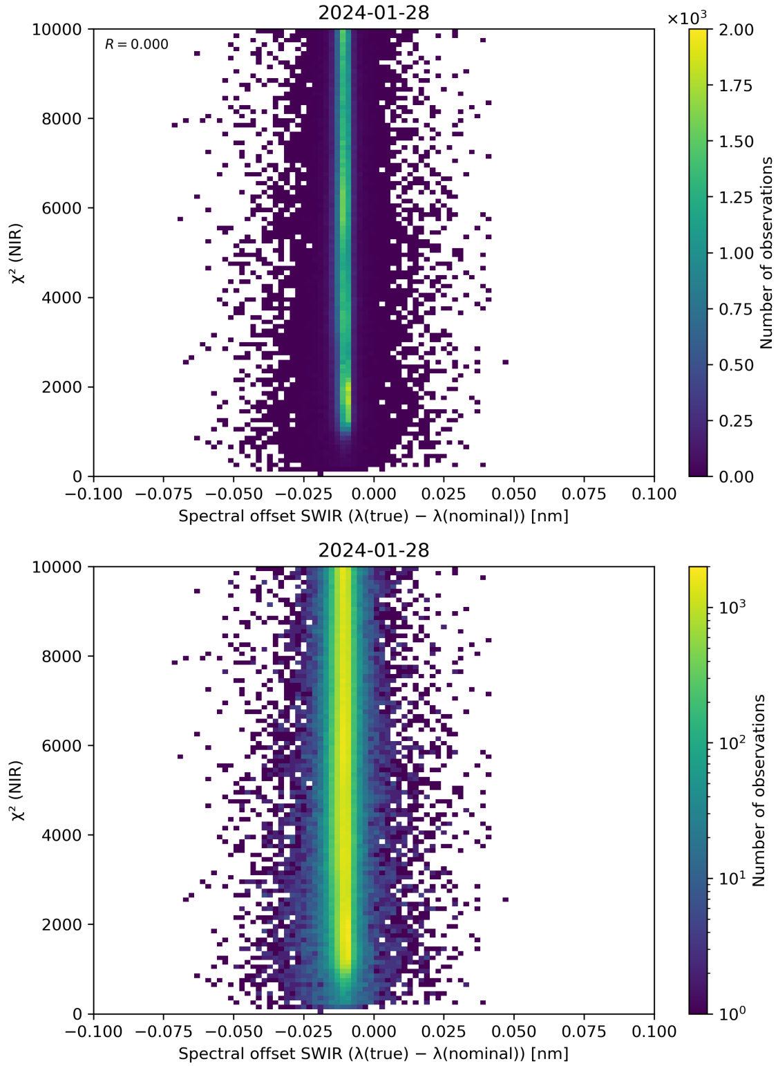
Figure 117: Scatter density plot of “Spectral offset SWIR ( \lambda(\text{true}) - \lambda(\text{nominal}) )” against “ \chi^2 (NIR)” for 2024-01-27 to 2024-01-29.
