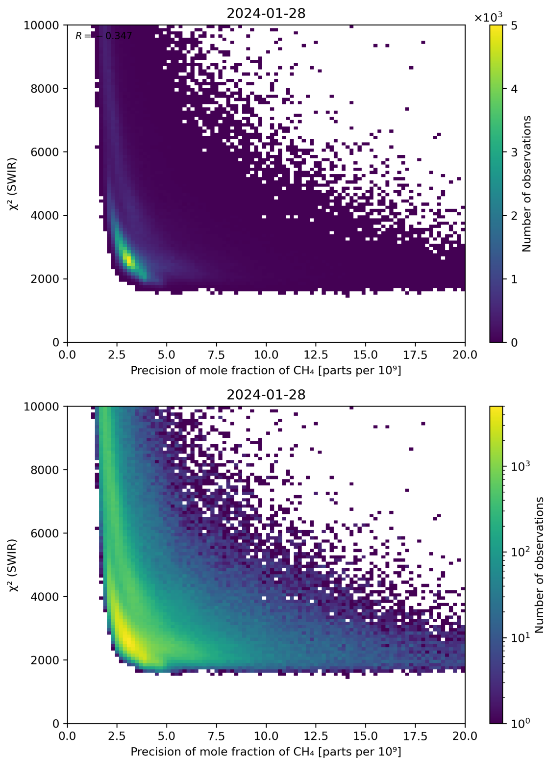
Figure 79: Scatter density plot of “Precision of mole fraction of CH 4 ” against “ \chi^2 (SWIR)” for 2024-01-27 to 2024-01-29.
