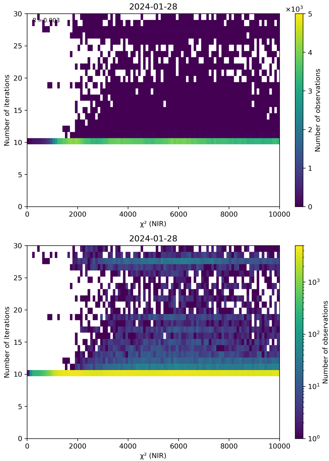
Figure 46: Scatter density plot of “ \chi^2 (NIR)” against “Number of iterations” for 2024-01-27 to 2024-01-29.
