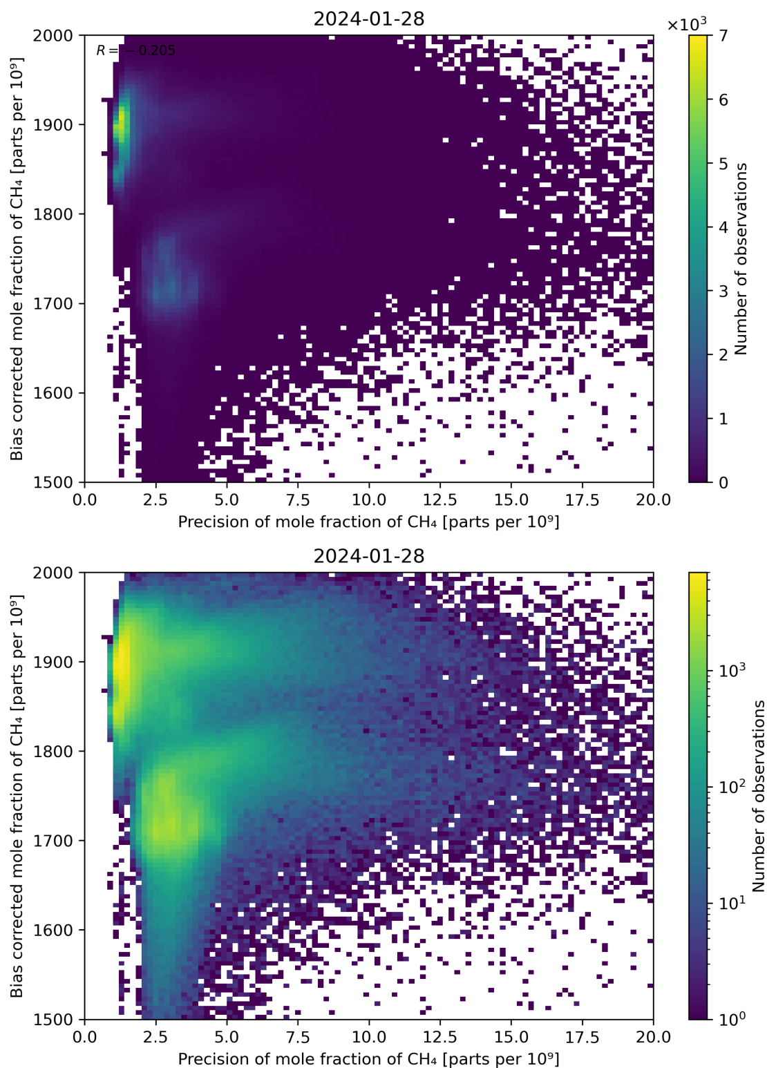
Figure 82: Scatter density plot of “Precision of mole fraction of \text{CH}_4 ” against “Bias corrected mole fraction of \text{CH}_4 ” for 2024-01-27 to 2024-01-29.
