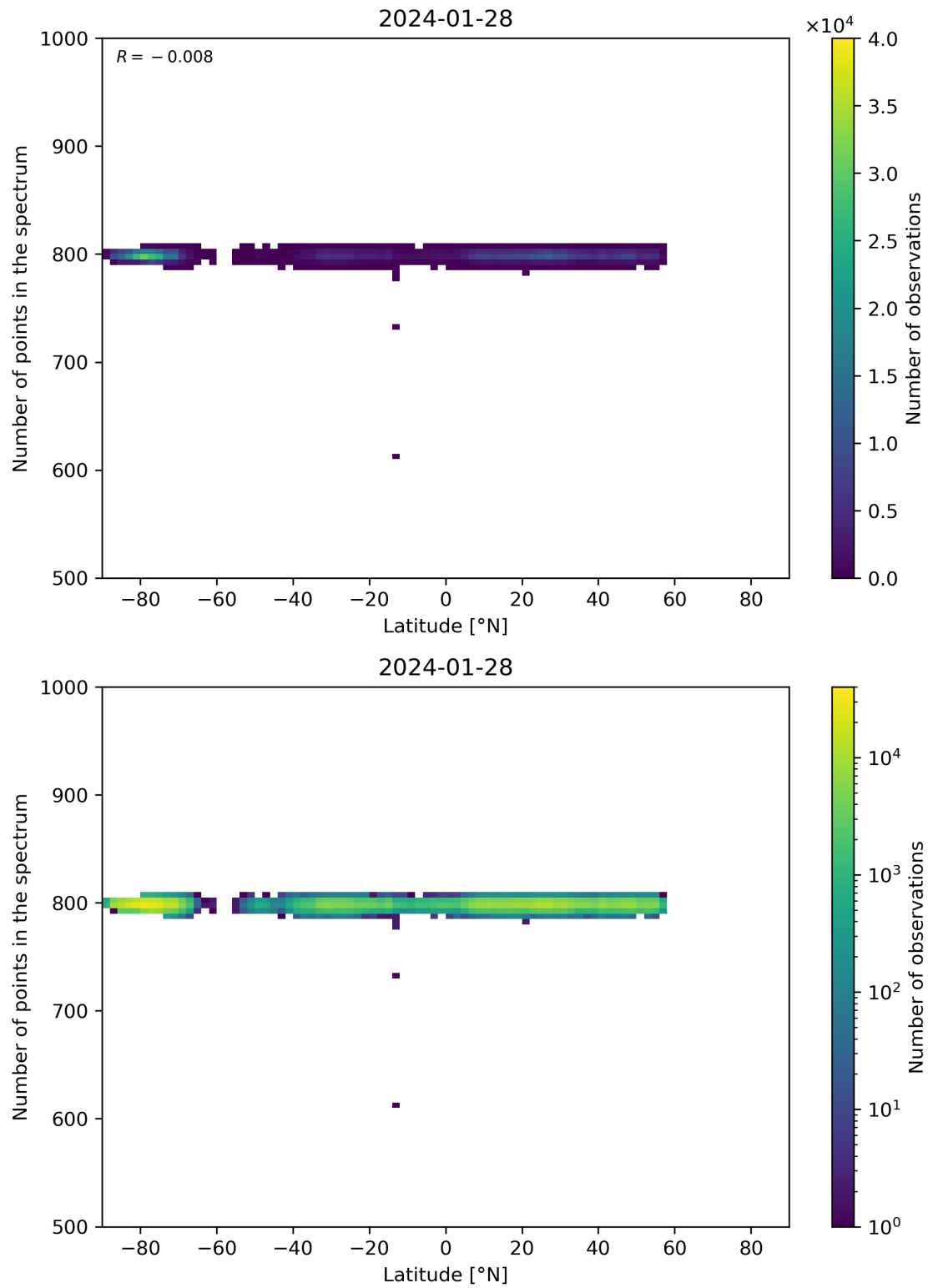
Figure 61: Scatter density plot of “Latitude” against “Number of points in the spectrum” for 2024-01-27 to 2024-01-29.
