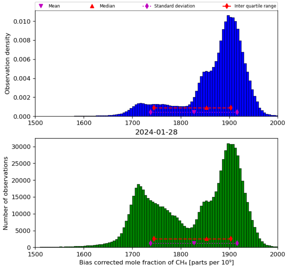
Figure 25: Histogram of “Bias corrected mole fraction of CH 4 ” for 2024-01-27 to 2024-01-29
