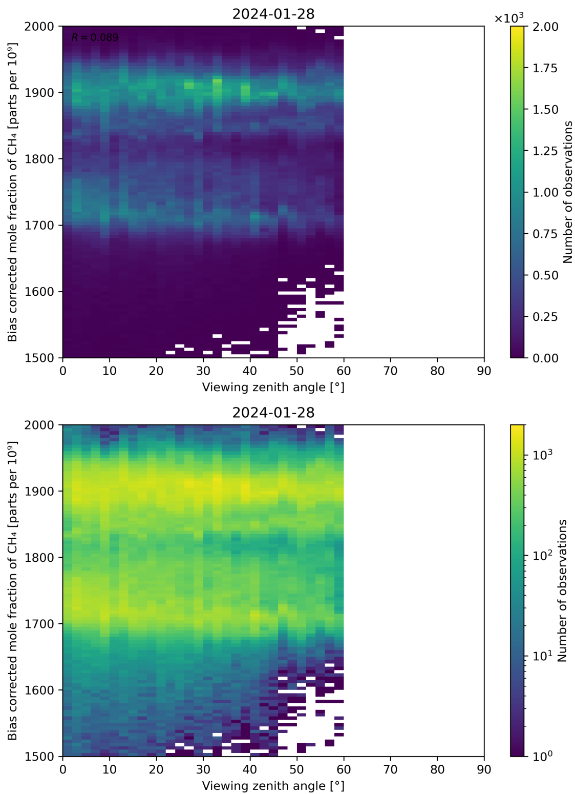
Figure 111: Scatter density plot of “Viewing zenith angle” against “Bias corrected mole fraction of CH 4 ” for 2024-01-27 to 2024-01-29.
