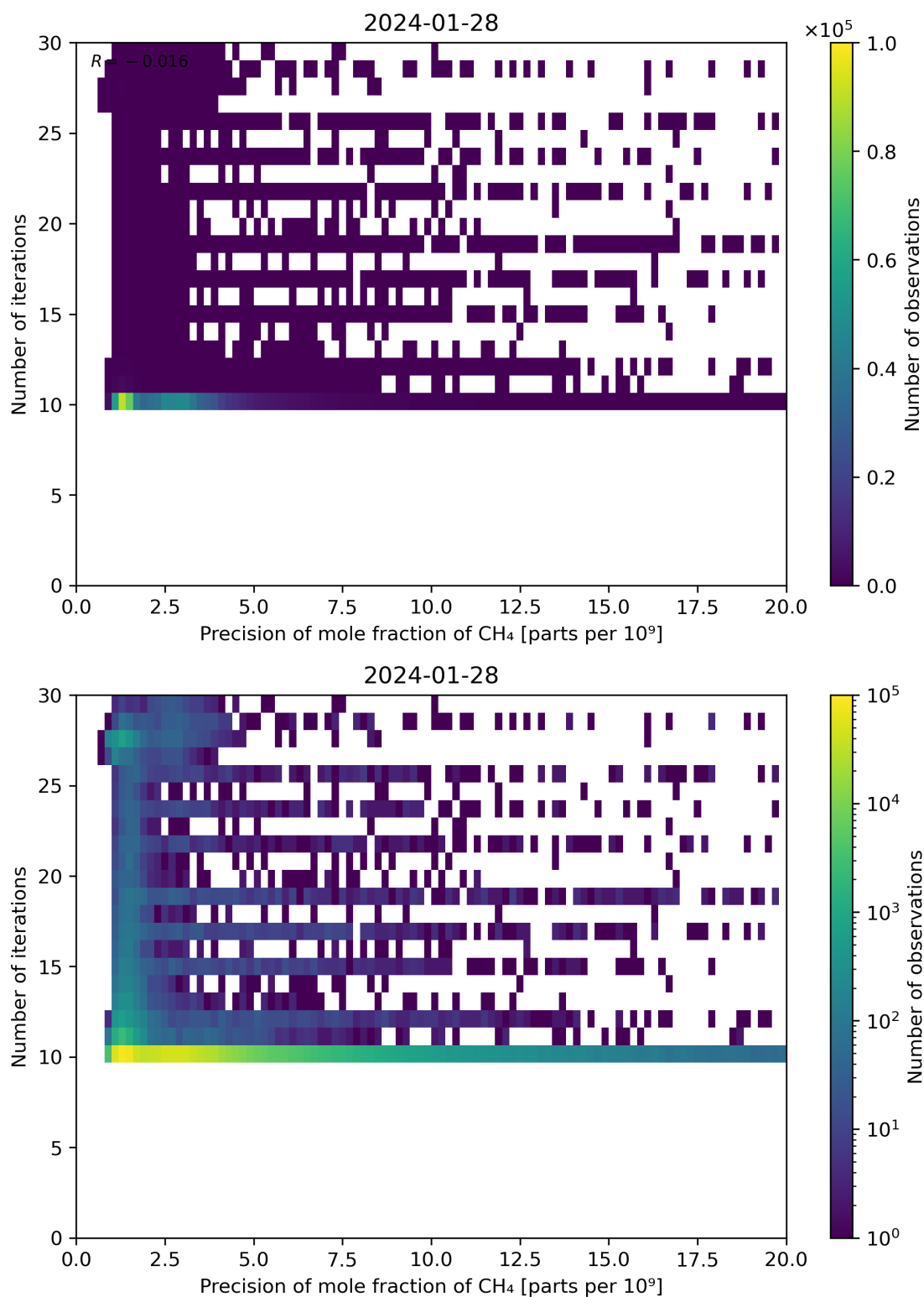
Figure 83: Scatter density plot of “Precision of mole fraction of CH 4 ” against “Number of iterations” for 2024-01-27 to 2024-01-29.
