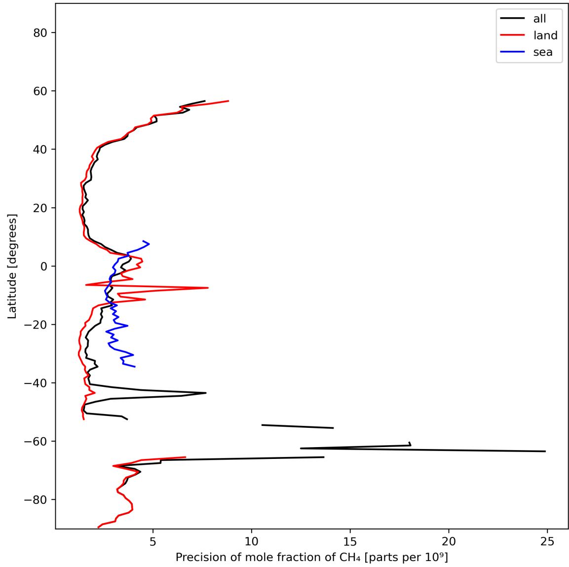
Figure 13: Zonal average of “Precision of mole fraction of CH 4 ” for 2024-01-27 to 2024-01-29.
