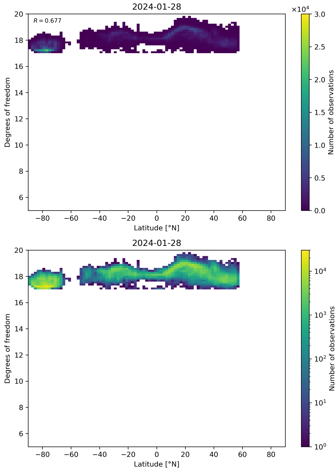
Figure 55: Scatter density plot of “Latitude” against “Degrees of freedom” for 2024-01-27 to 2024-01-29.
