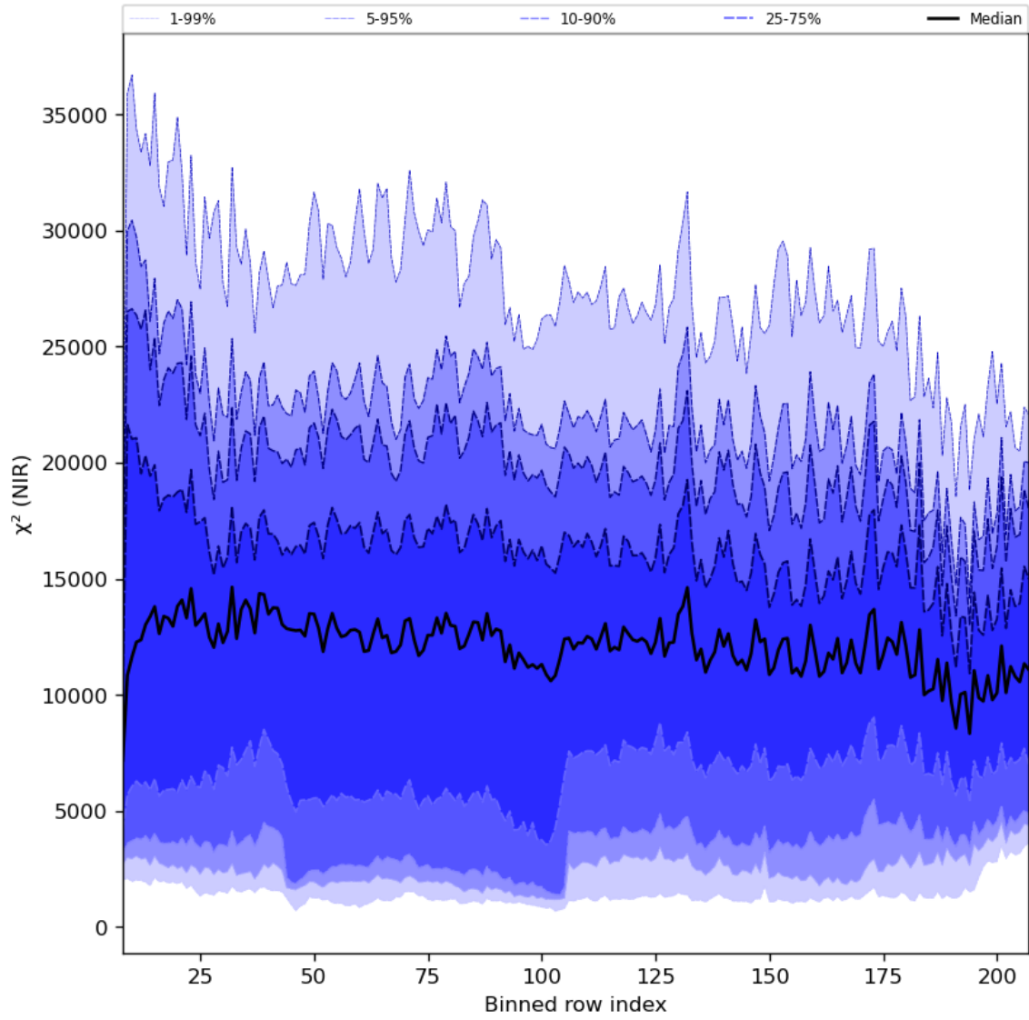
Figure 40: Along track statistics of “ \chi^2 (NIR)” for 2024-01-27 to 2024-01-29
