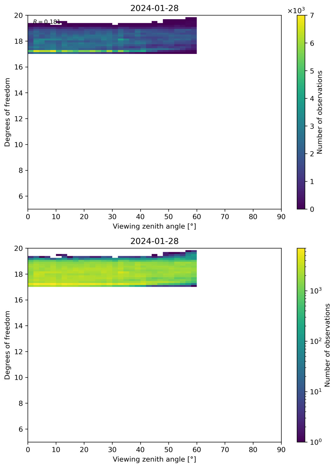
Figure 107: Scatter density plot of “Viewing zenith angle” against “Degrees of freedom” for 2024-01-27 to 2024-01-29.
