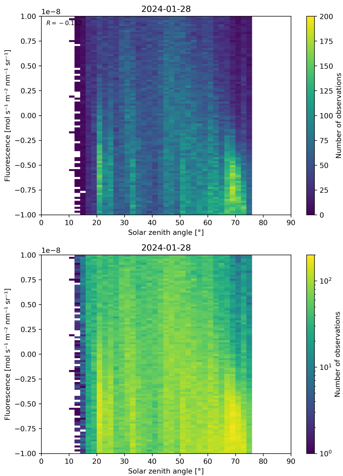
Figure 97: Scatter density plot of “Solar zenith angle” against “Fluorescence” for 2024-01-27 to 2024-01-29.
