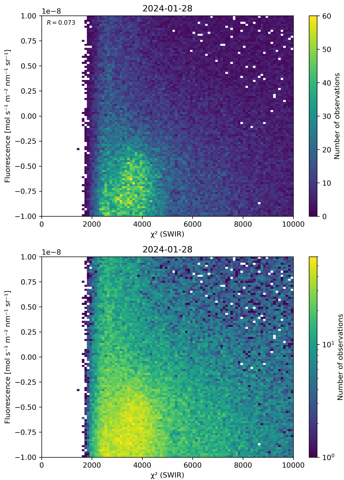
Figure 49: Scatter density plot of “ \chi^2 (SWIR)” against “Fluorescence” for 2024-01-27 to 2024-01-29.
