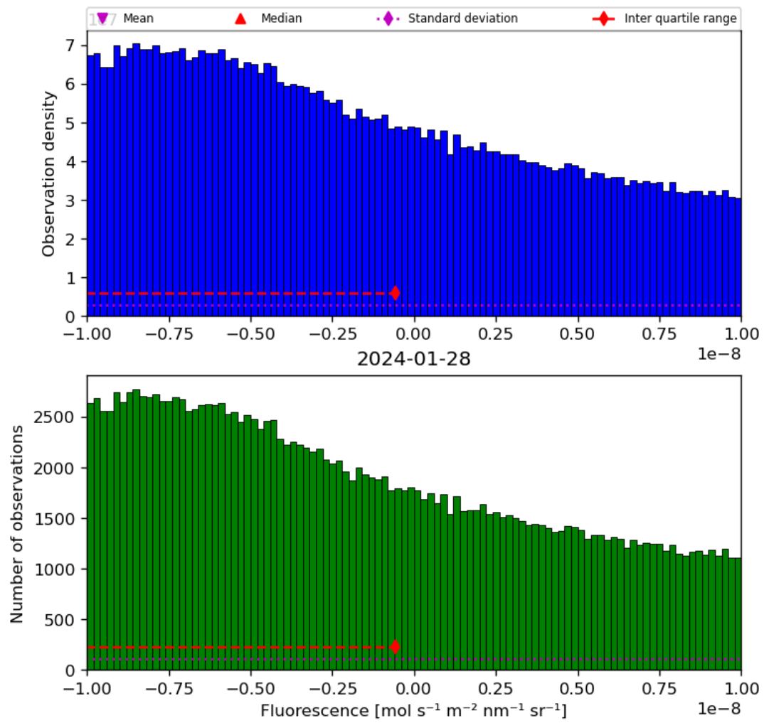
Figure 32: Histogram of “Fluorescence” for 2024-01-27 to 2024-01-29
