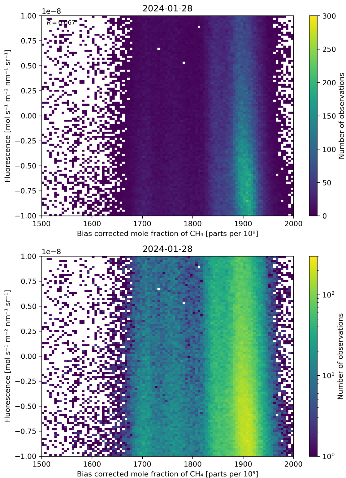
Figure 66: Scatter density plot of “Bias corrected mole fraction of \text{CH}_4 ” against “Fluorescence” for 2024-01-27 to 2024-01-29.
