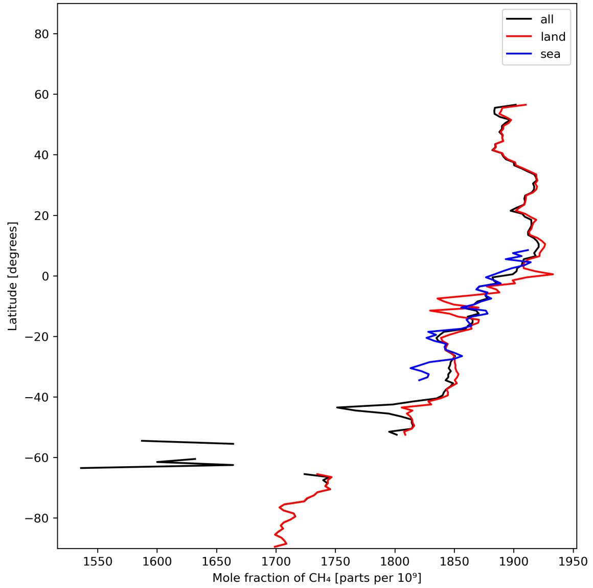
Figure 12: Zonal average of “Mole fraction of \text{CH}_4 ” for 2024-01-27 to 2024-01-29.
