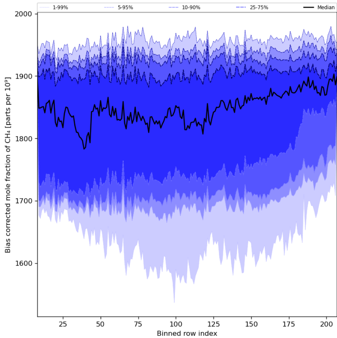
Figure 36: Along track statistics of “Bias corrected mole fraction of CH 4 ” for 2024-01-27 to 2024-01-29
