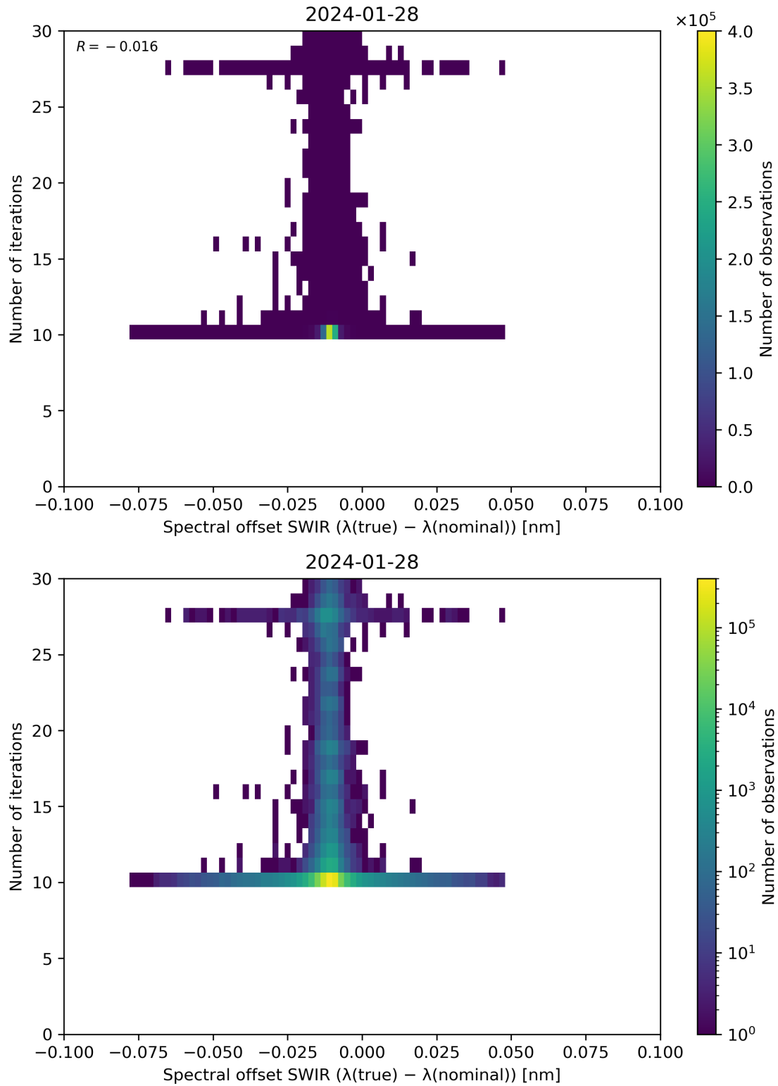
Figure 121: Scatter density plot of “Spectral offset SWIR ( \lambda(\text{true}) - \lambda(\text{nominal}) )” against “Number of iterations” for 2024-01-27 to 2024-01-29.
