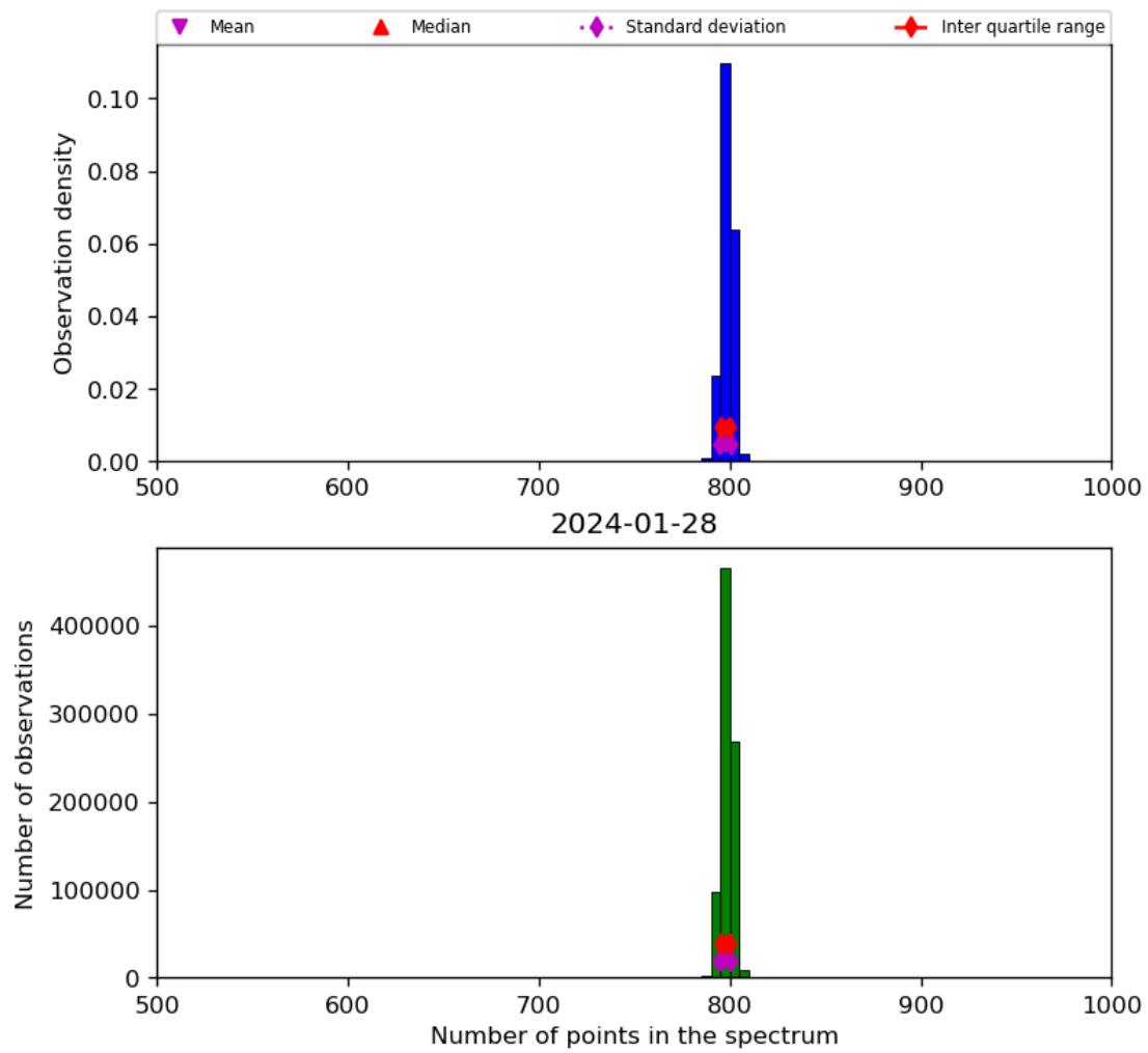
Figure 26: Histogram of “Number of points in the spectrum” for 2024-01-27 to 2024-01-29
