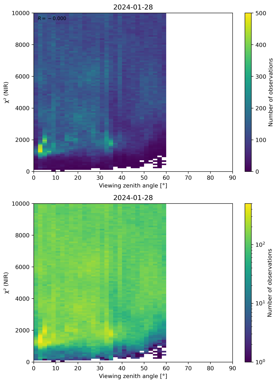
Figure 105: Scatter density plot of “Viewing zenith angle” against “ \chi^2 (NIR)” for 2024-01-27 to 2024-01-29.
