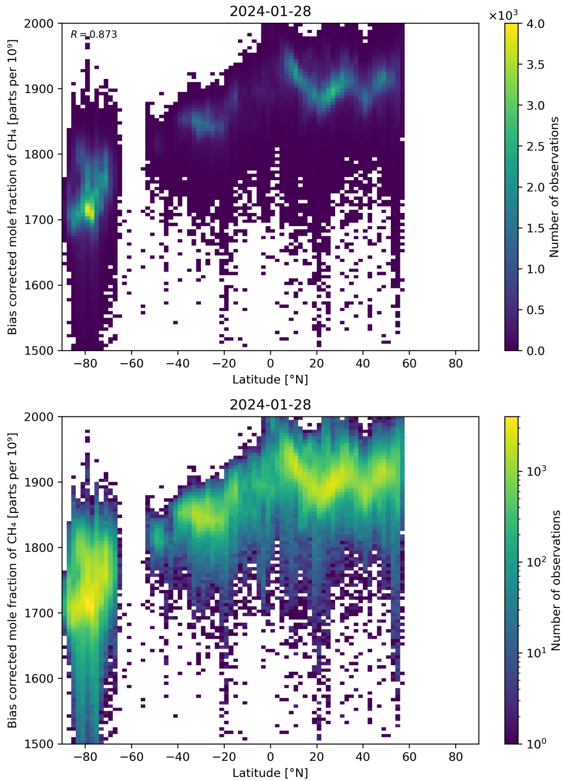
Figure 58: Scatter density plot of “Latitude” against “Bias corrected mole fraction of CH 4 ” for 2024-01-27 to 2024-01-29.
