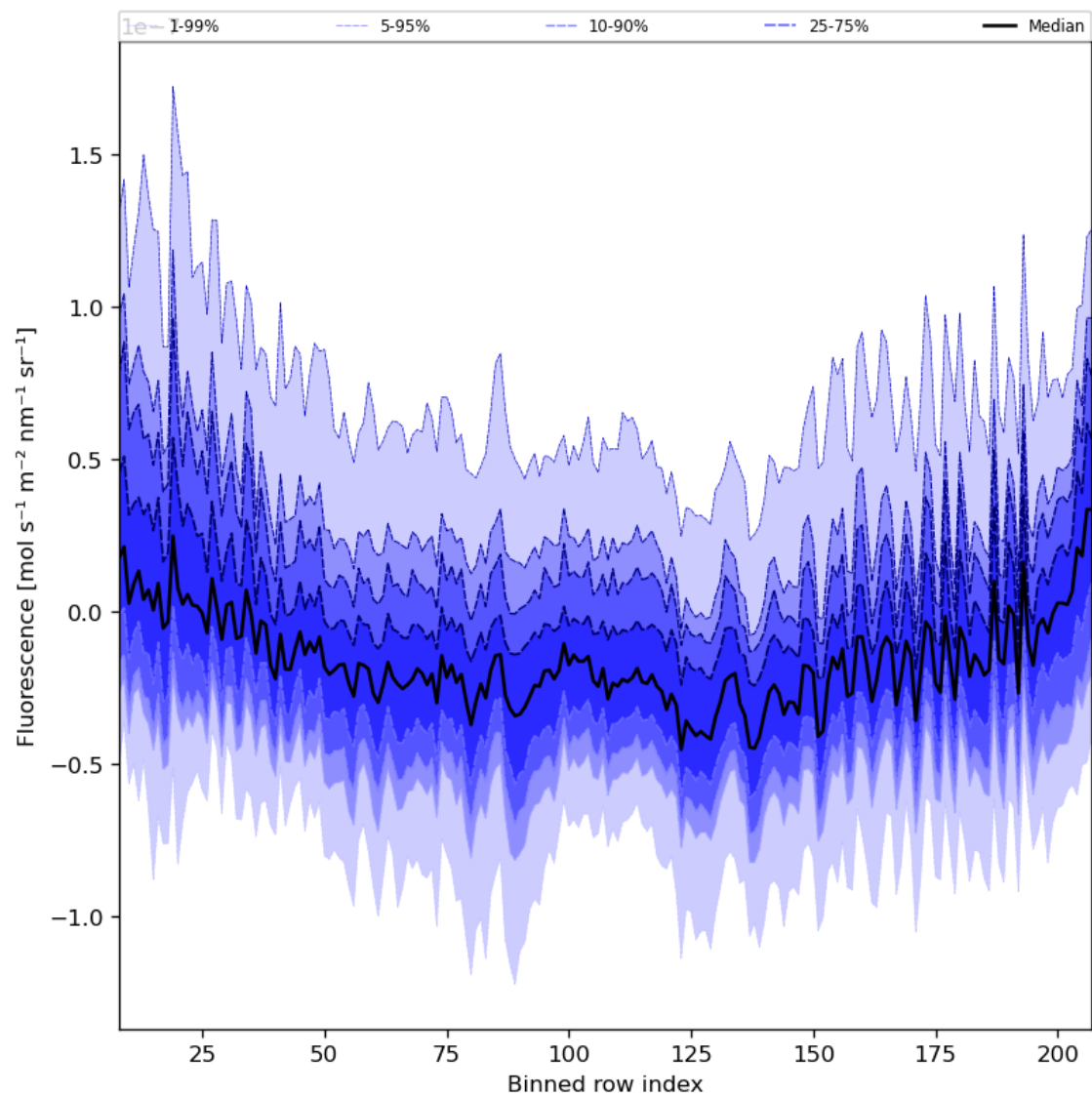
Figure 43: Along track statistics of “Fluorescence” for 2024-01-27 to 2024-01-29
