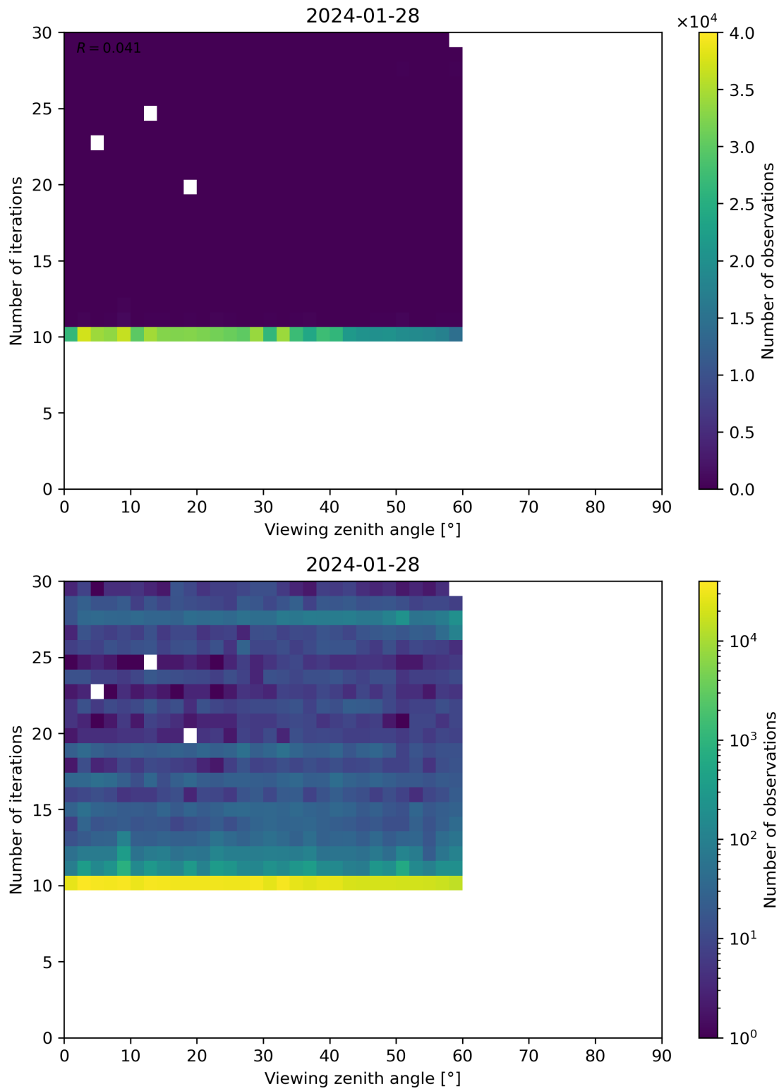
Figure 113: Scatter density plot of “Viewing zenith angle” against “Number of iterations” for 2024-01-27 to 2024-01-29.
