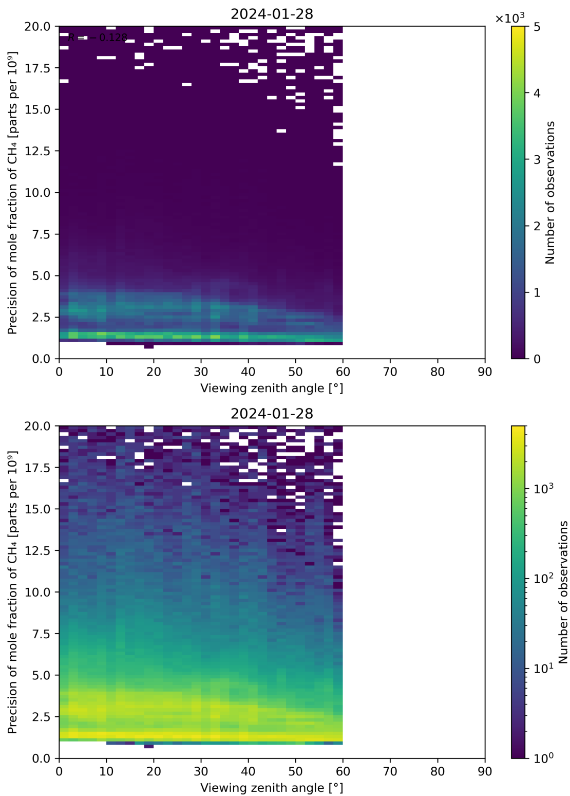
Figure 112: Scatter density plot of “Viewing zenith angle” against “Precision of mole fraction of CH 4 ” for 2024-01-27 to 2024-01-29.
