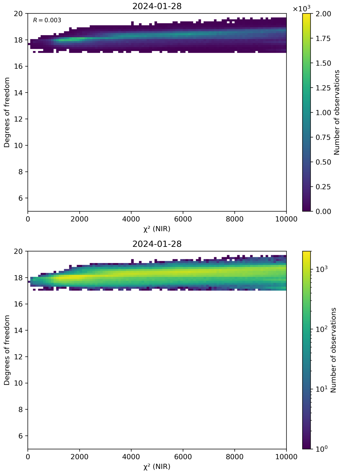
Figure 44: Scatter density plot of “ \chi^2 (NIR)” against “Degrees of freedom” for 2024-01-27 to 2024-01-29.
