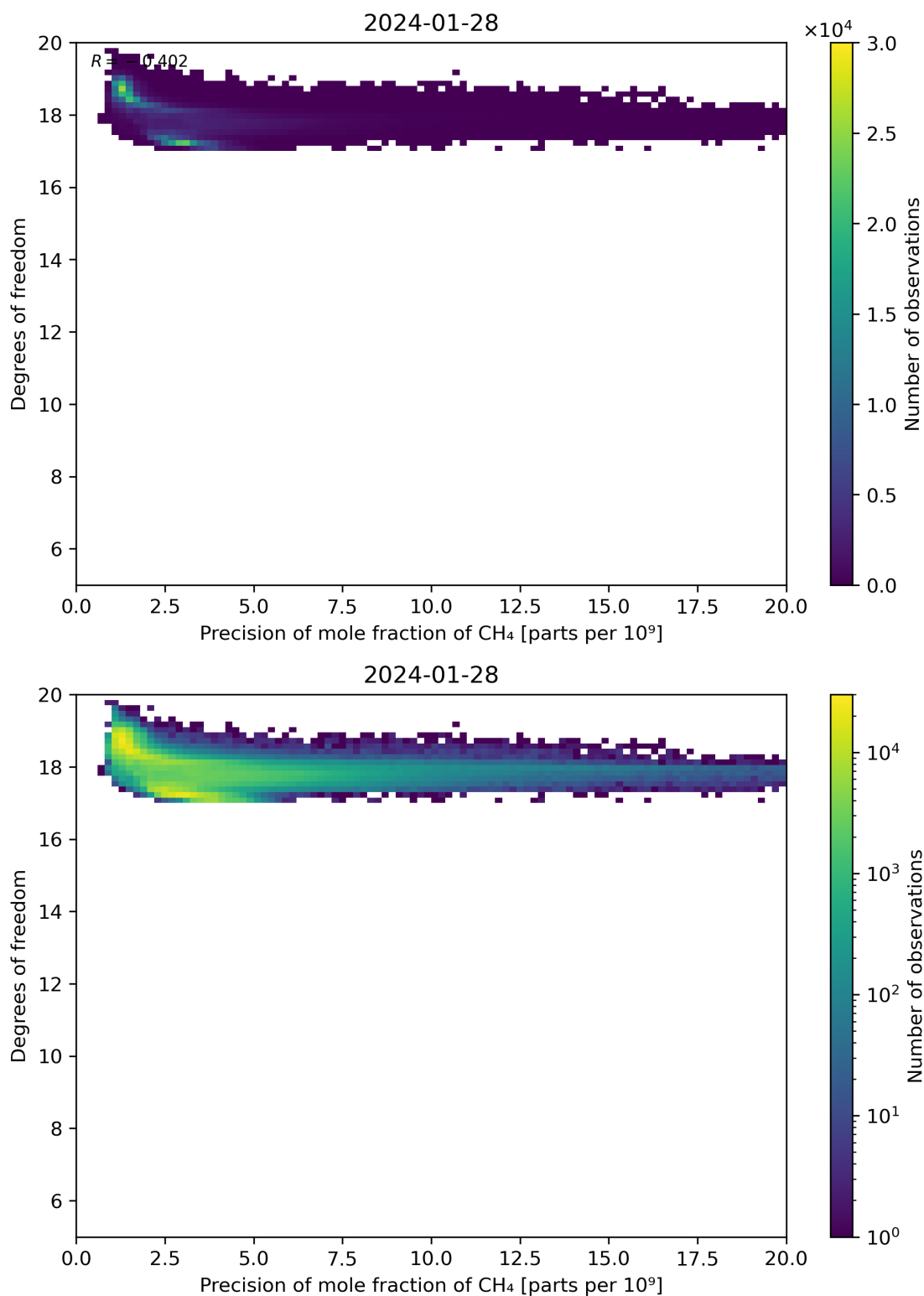
Figure 80: Scatter density plot of “Precision of mole fraction of CH 4 ” against “Degrees of freedom” for 2024-01-27 to 2024-01-29.
