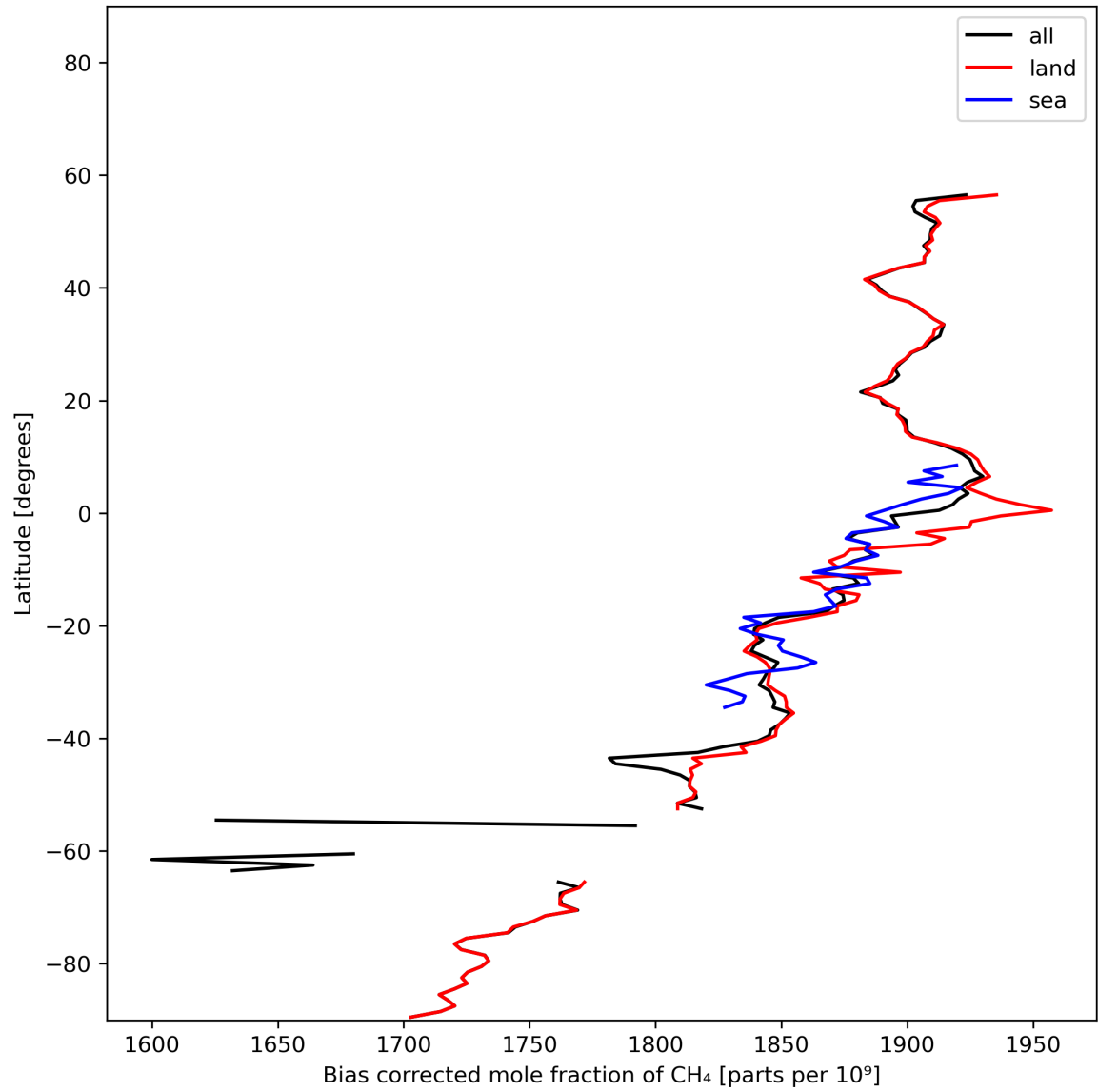
Figure 14: Zonal average of “Bias corrected mole fraction of CH 4 ” for 2024-01-27 to 2024-01-29.
