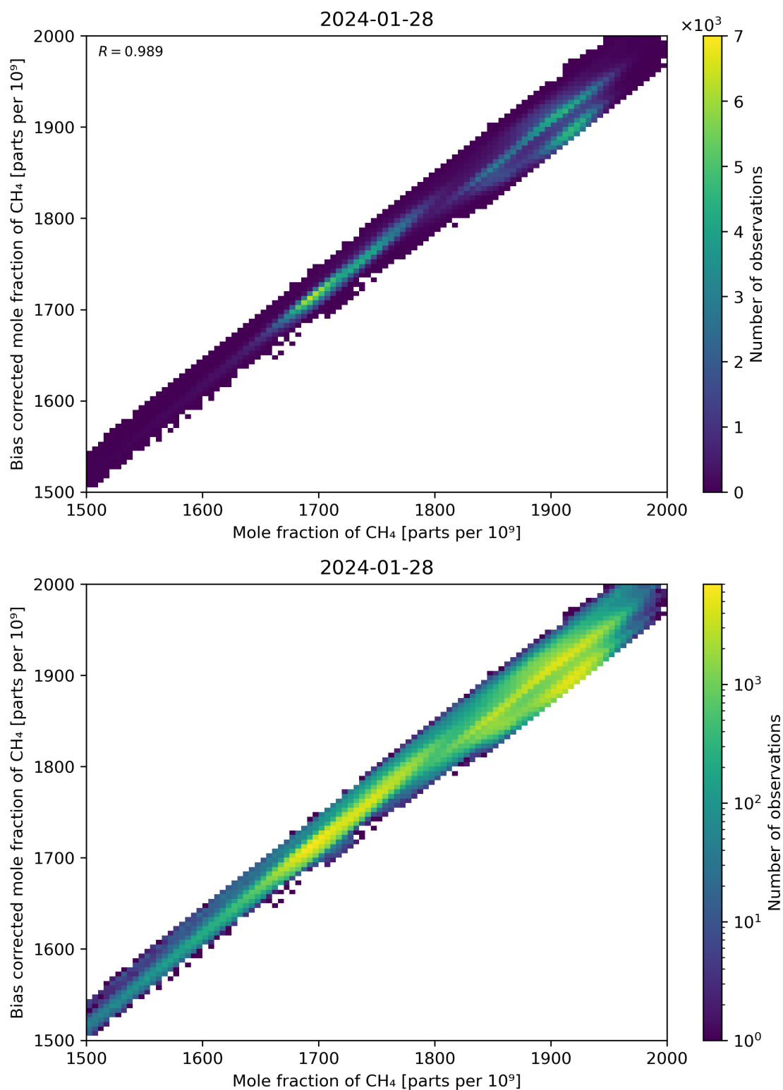
Figure 74: Scatter density plot of “Mole fraction of CH 4 ” against “Bias corrected mole fraction of CH 4 ” for 2024-01-27 to 2024-01-29.
