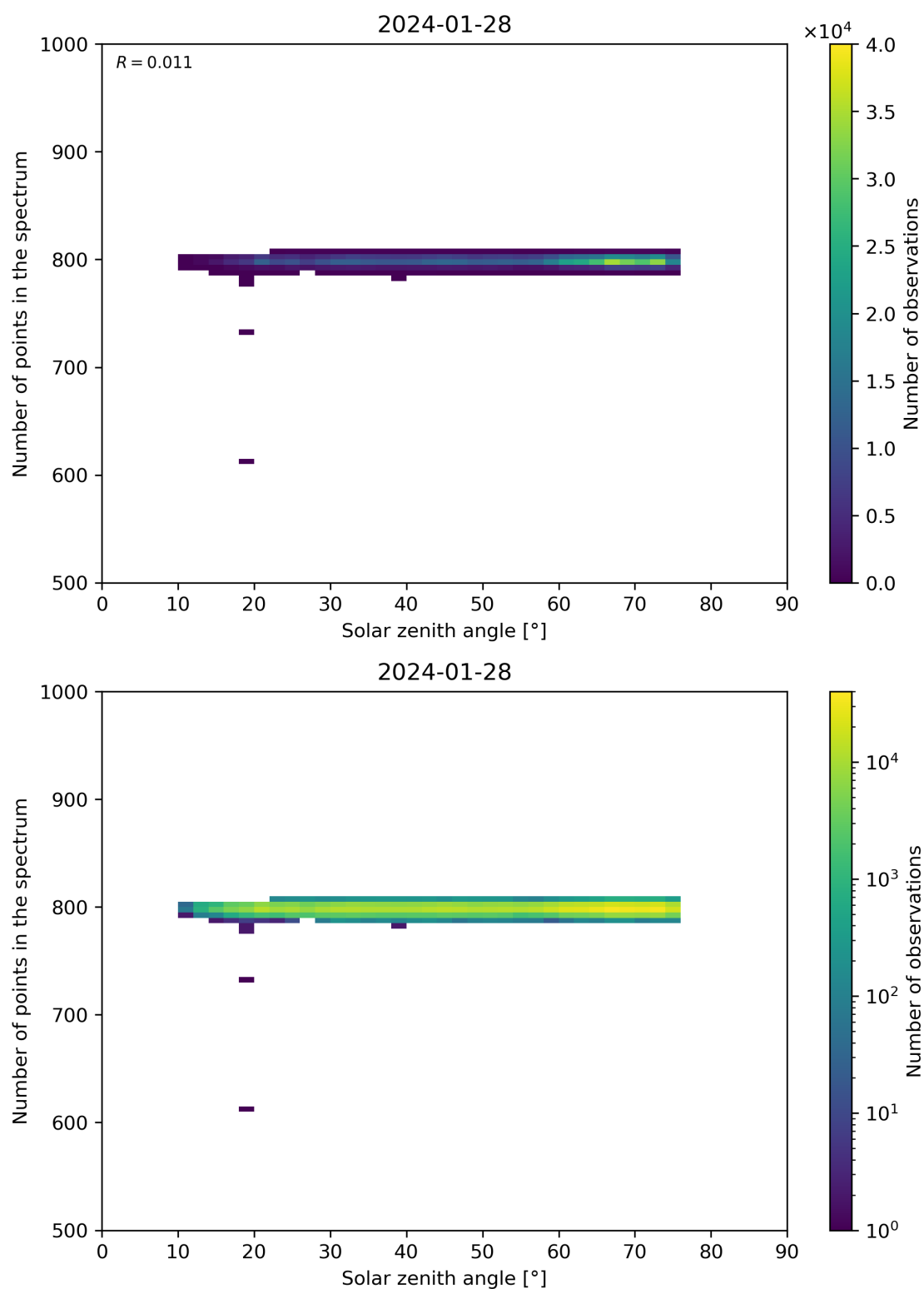
Figure 103: Scatter density plot of “Solar zenith angle” against “Number of points in the spectrum” for 2024-01-27 to 2024-01-29.
