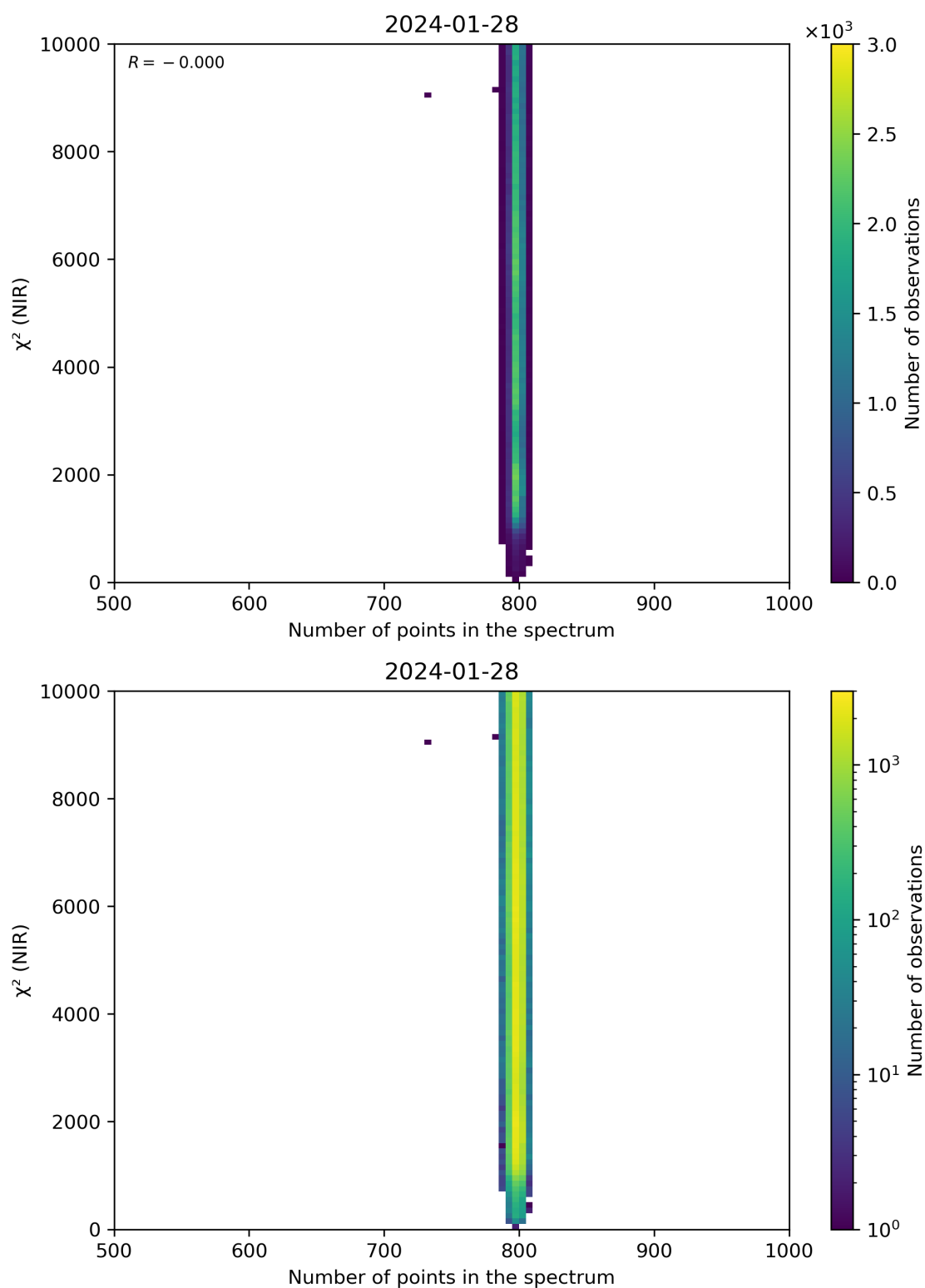
Figure 88: Scatter density plot of “Number of points in the spectrum” against “ \chi^2 (NIR)” for 2024-01-27 to 2024-01-29.
