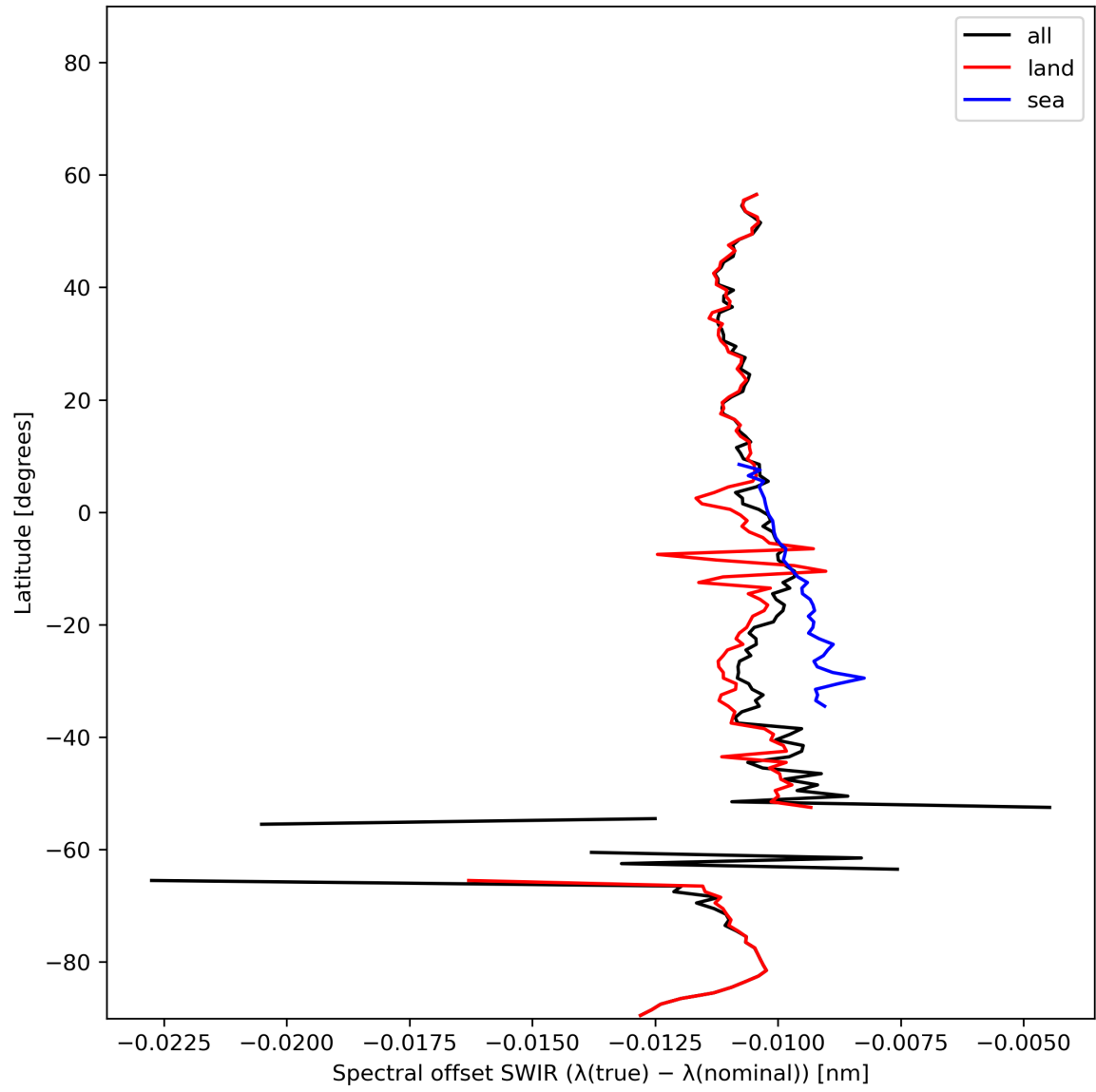
Figure 16: Zonal average of “Spectral offset SWIR ( \lambda(\text{true}) - \lambda(\text{nominal}) )” for 2024-01-27 to 2024-01-29.
