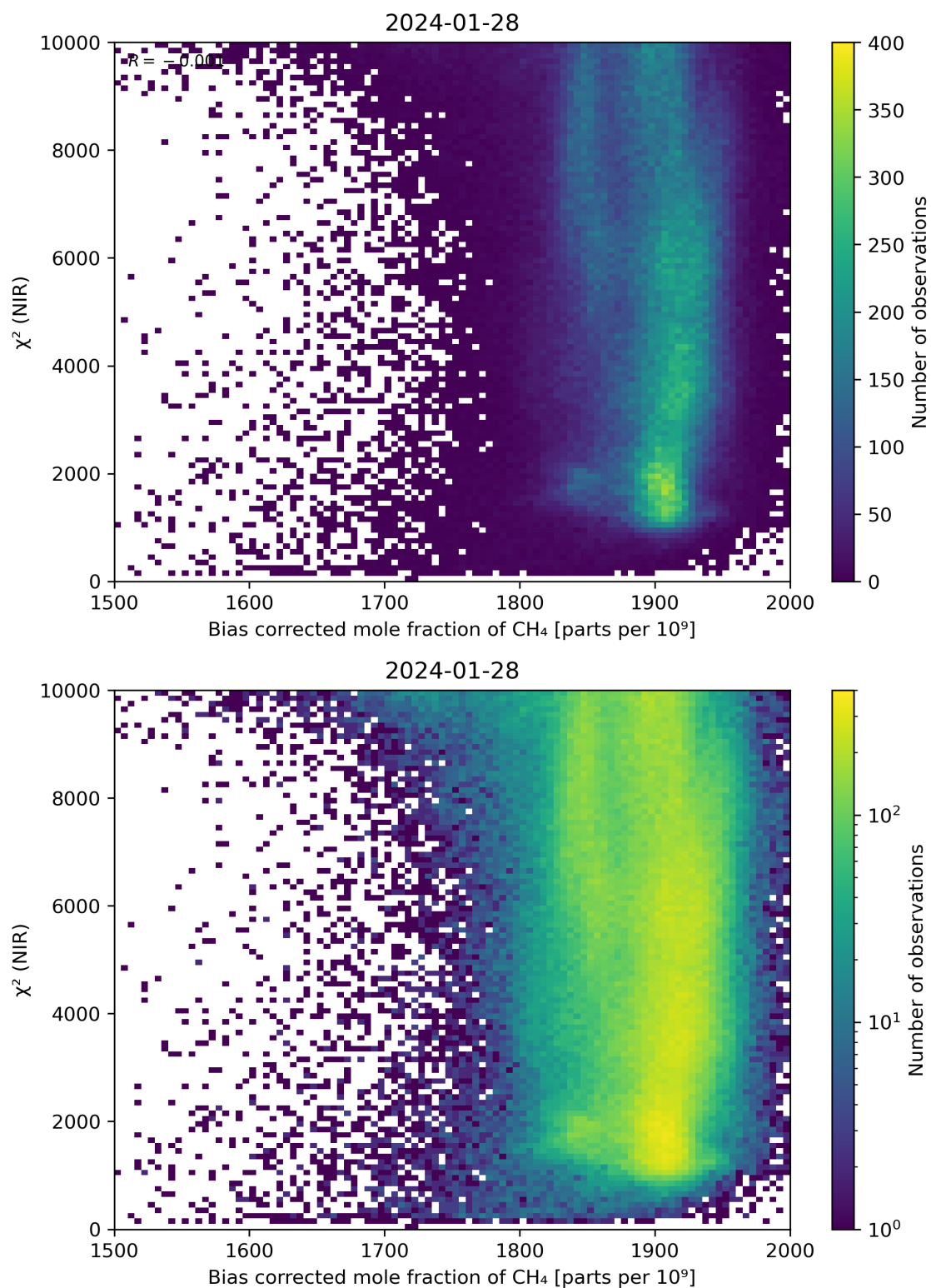
Figure 63: Scatter density plot of “Bias corrected mole fraction of CH 4 ” against “ \chi^2 (NIR)” for 2024-01-27 to 2024-01-29.
