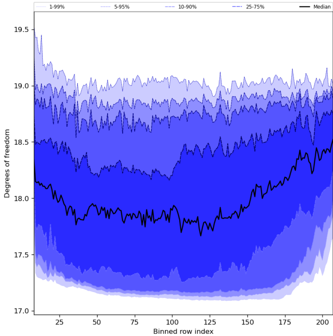
Figure 41: Along track statistics of “Degrees of freedom” for 2024-01-27 to 2024-01-29
