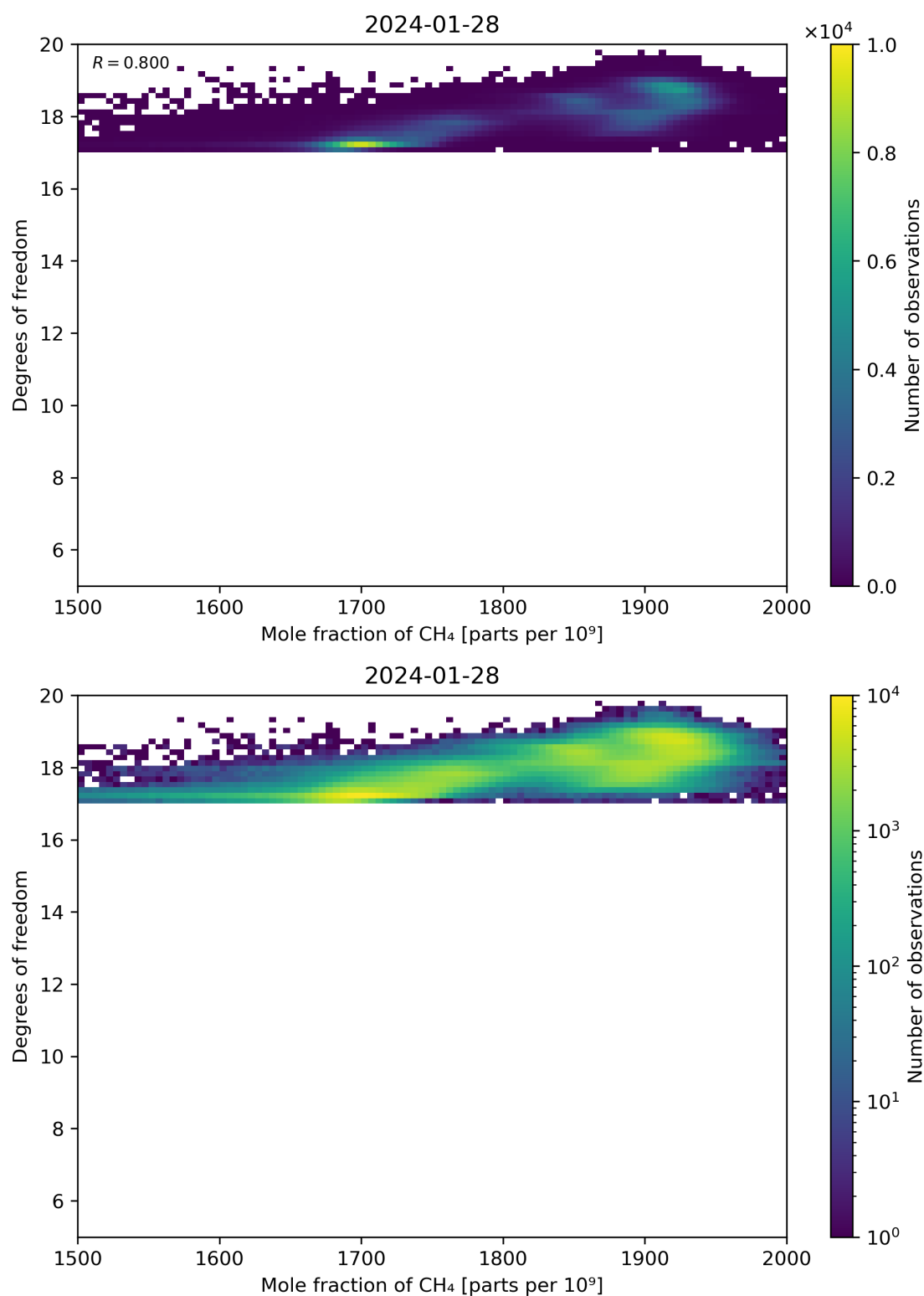
Figure 72: Scatter density plot of “Mole fraction of CH 4 ” against “Degrees of freedom” for 2024-01-27 to 2024-01-29.
