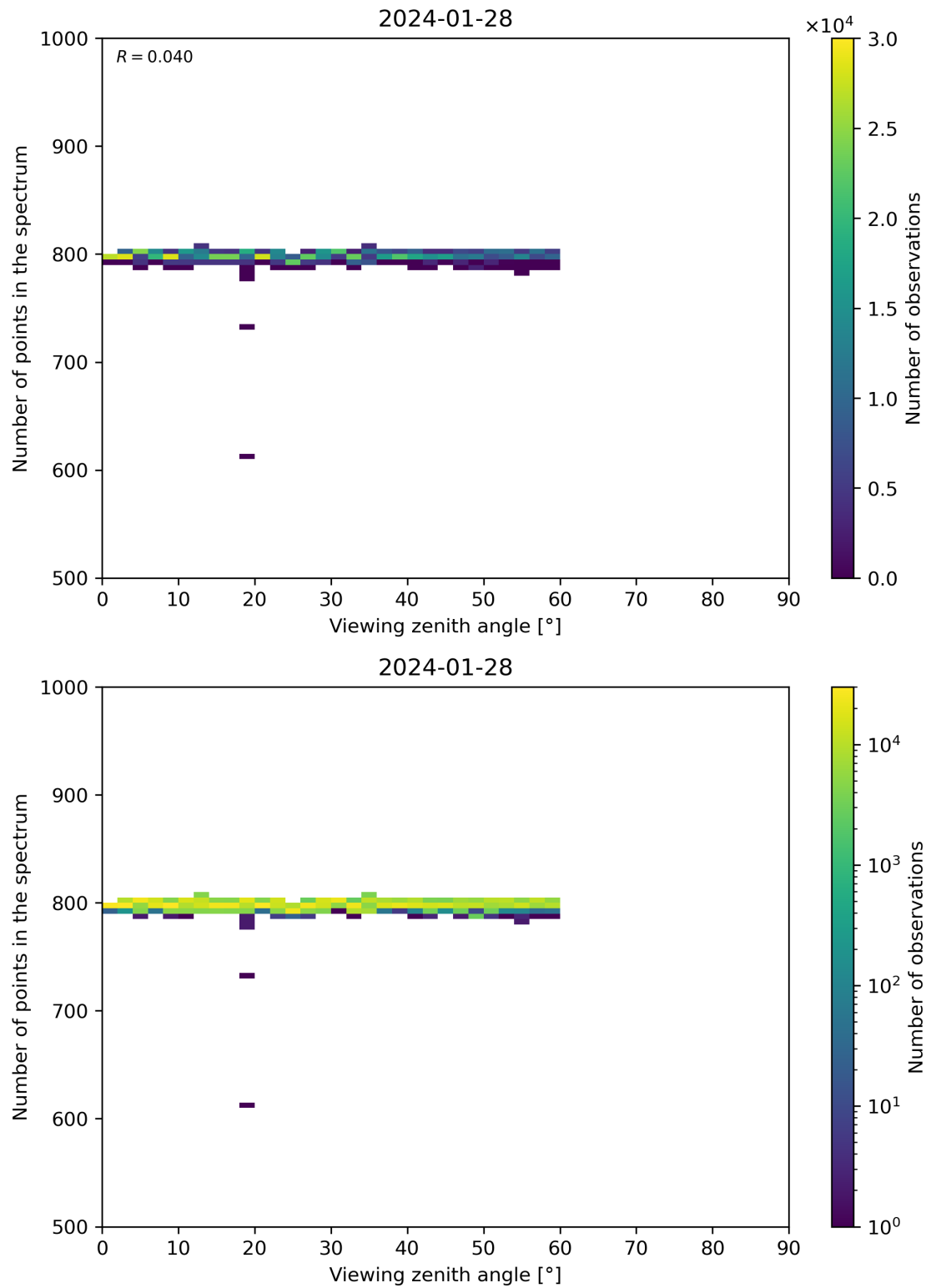
Figure 114: Scatter density plot of “Viewing zenith angle” against “Number of points in the spectrum” for 2024-01-27 to 2024-01-29.
