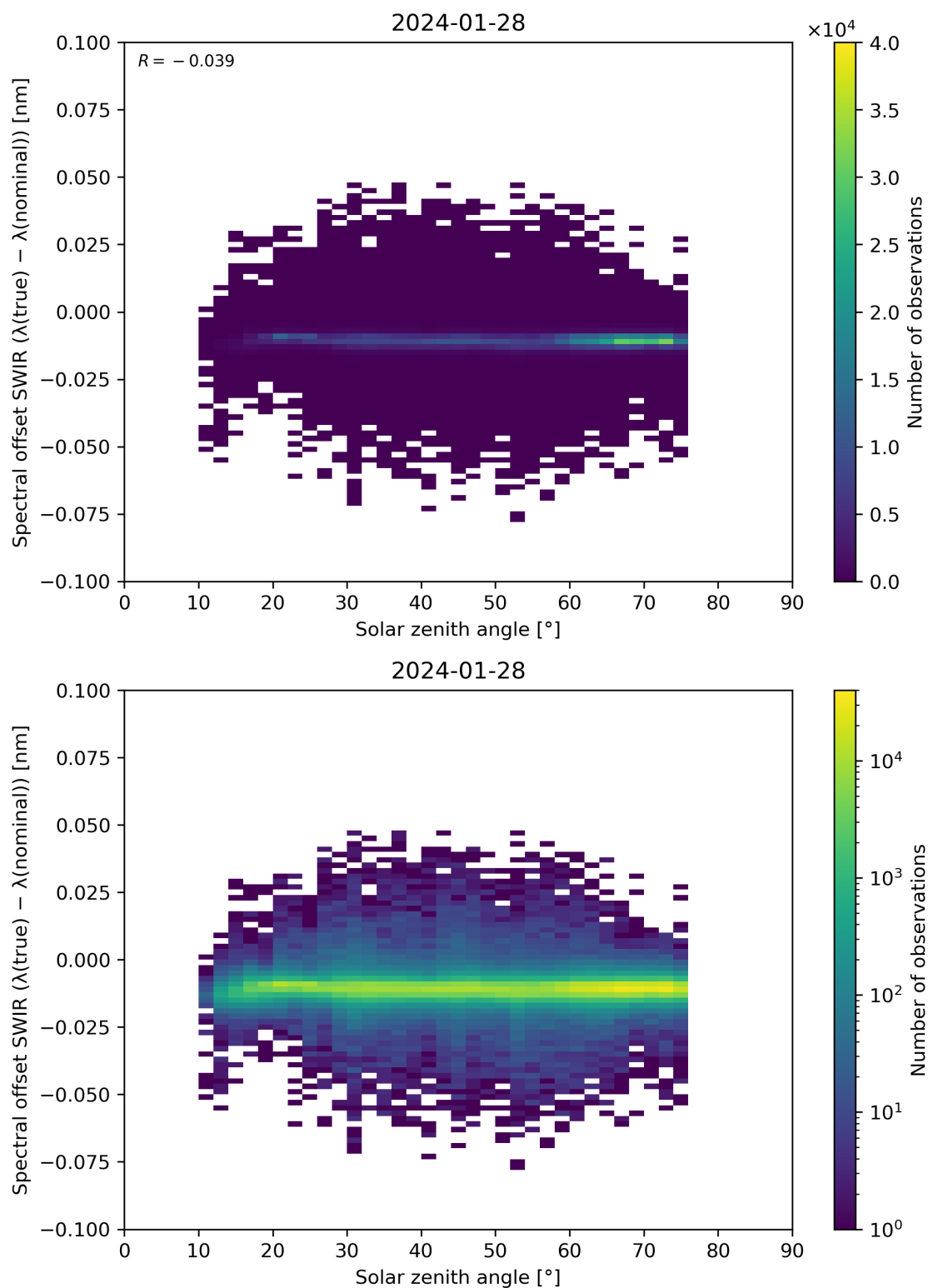
Figure 104: Scatter density plot of “Solar zenith angle” against “Spectral offset SWIR ( \lambda(\text{true}) - \lambda(\text{nominal}) )” for 2024-01-27 to 2024-01-29.
