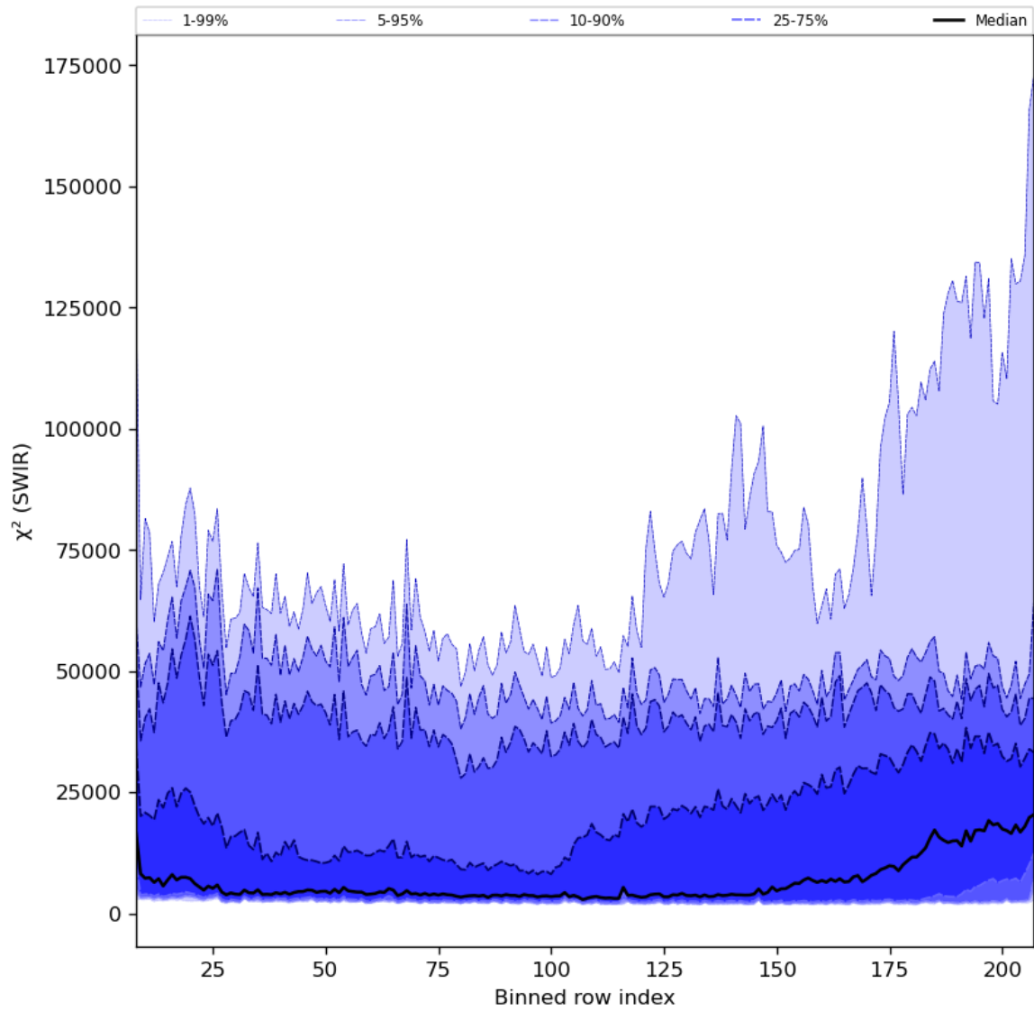
Figure 39: Along track statistics of “ \chi^2 (SWIR)” for 2024-01-27 to 2024-01-29
