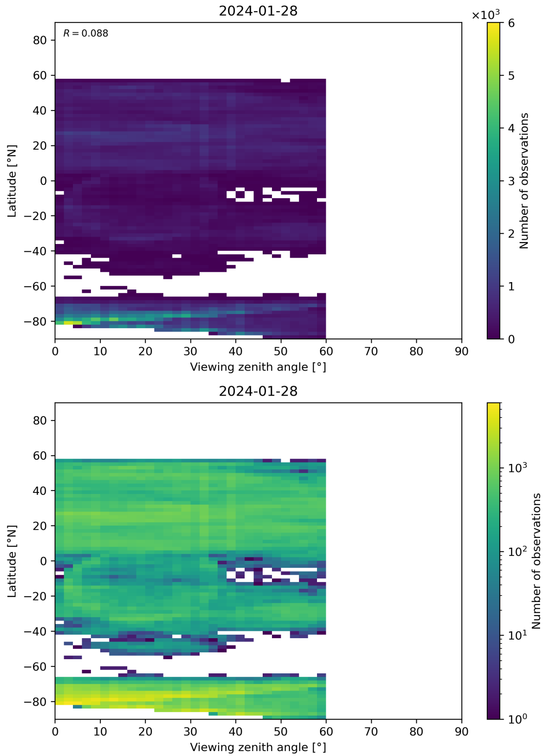
Figure 109: Scatter density plot of “Viewing zenith angle” against “Latitude” for 2024-01-27 to 2024-01-29.
