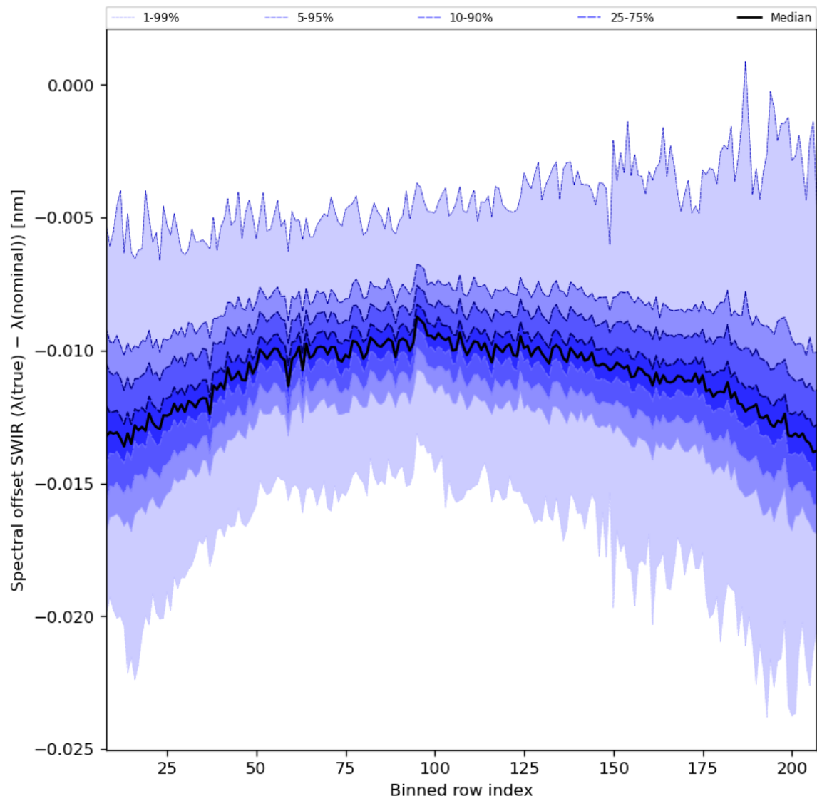
Figure 38: Along track statistics of “Spectral offset SWIR ( \lambda(\text{true}) - \lambda(\text{nominal}) )” for 2024-01-27 to 2024-01-29
