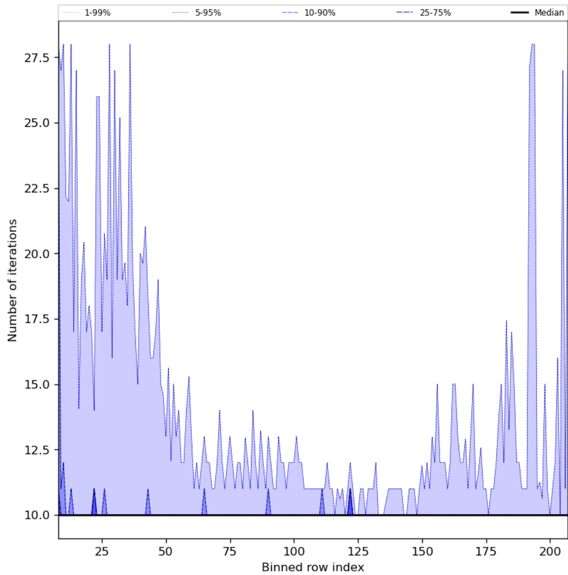
Figure 42: Along track statistics of “Number of iterations” for 2024-01-27 to 2024-01-29
