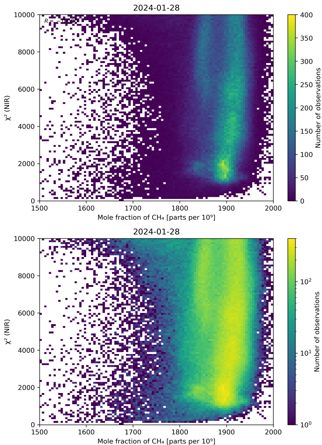
Figure 70: Scatter density plot of “Mole fraction of CH 4 ” against “ \chi^2 (NIR)” for 2024-01-27 to 2024-01-29.
