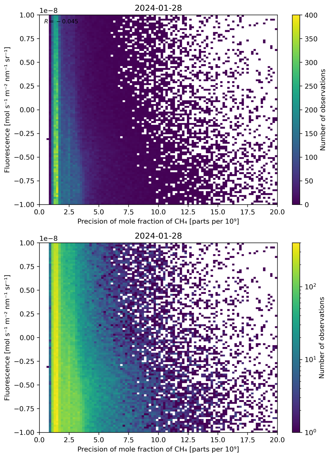
Figure 81: Scatter density plot of “Precision of mole fraction of CH 4 ” against “Fluorescence” for 2024-01-27 to 2024-01-29.
