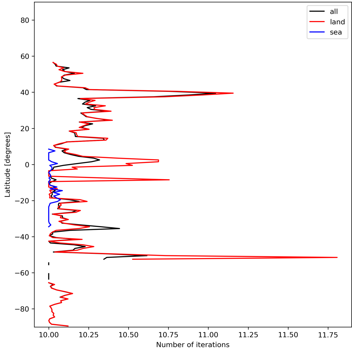
Figure 20: Zonal average of “Number of iterations” for 2024-01-27 to 2024-01-29.
