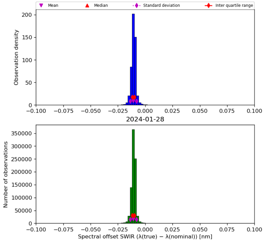
Figure 27: Histogram of “Spectral offset SWIR ( \lambda(\text{true}) - \lambda(\text{nominal}) )” for 2024-01-27 to 2024-01-29
