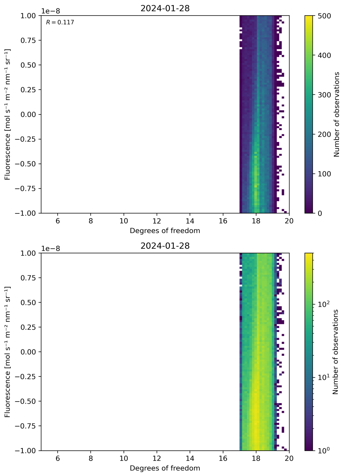
Figure 51: Scatter density plot of “Degrees of freedom” against “Fluorescence” for 2024-01-27 to 2024-01-29.
