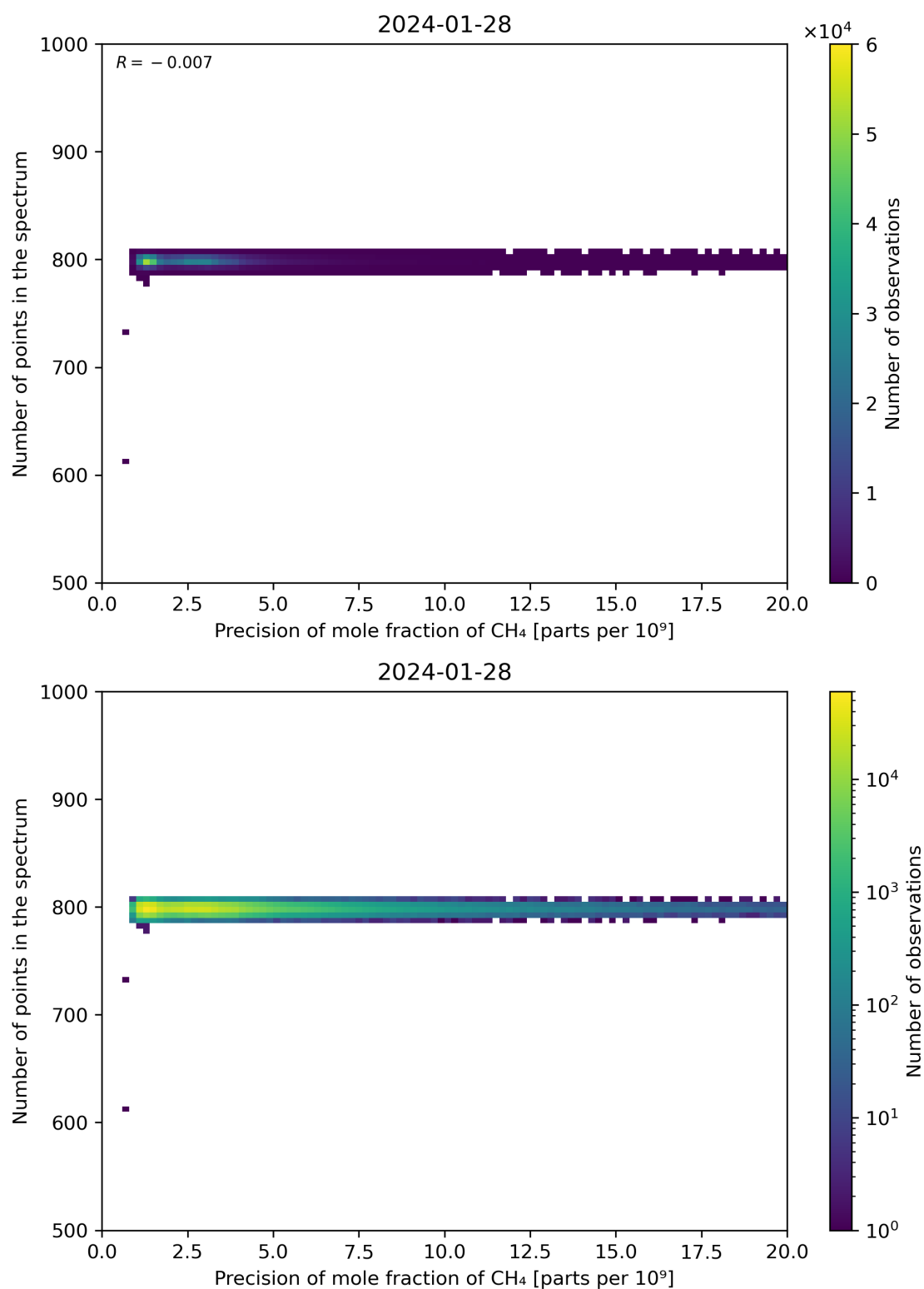
Figure 84: Scatter density plot of “Precision of mole fraction of CH 4 ” against “Number of points in the spectrum” for 2024-01-27 to 2024-01-29.
