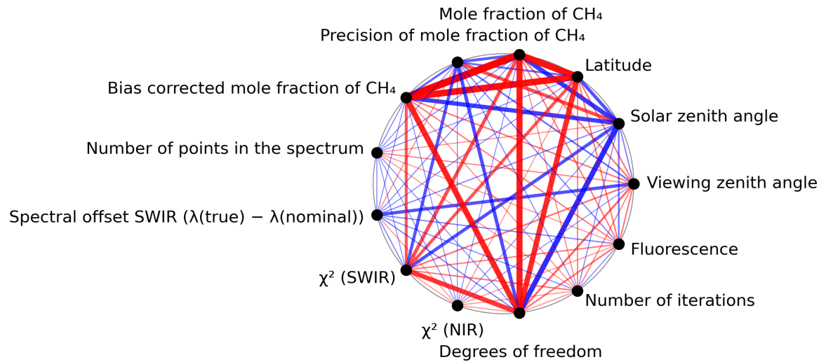
Figure 1: Map of correlation graph for 2024-01-27 to 2024-01-29.
