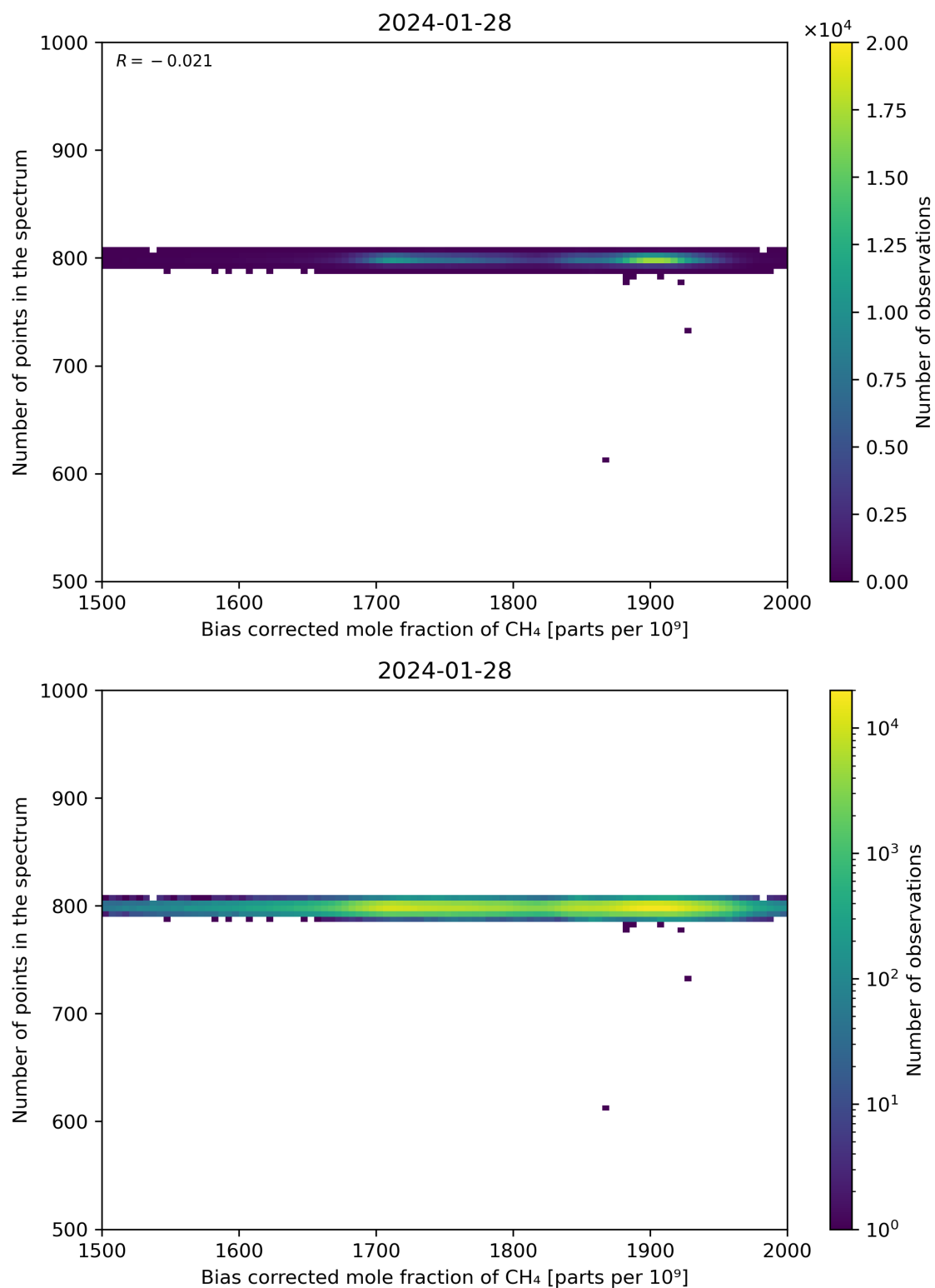
Figure 68: Scatter density plot of “Bias corrected mole fraction of CH 4 ” against “Number of points in the spectrum” for 2024-01-27 to 2024-01-29.
