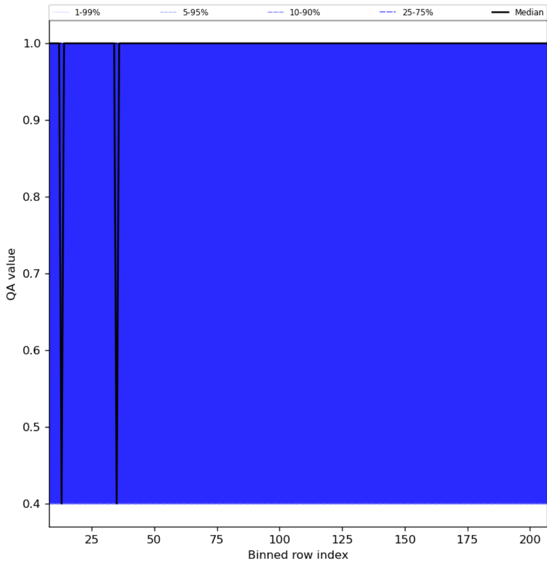
Figure 33: Along track statistics of “QA value” for 2024-01-27 to 2024-01-29
