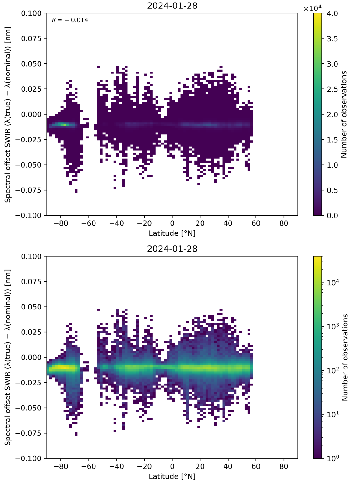
Figure 62: Scatter density plot of “Latitude” against “Spectral offset SWIR ( \lambda(\text{true}) - \lambda(\text{nominal}) )” for 2024-01-27 to 2024-01-29.
