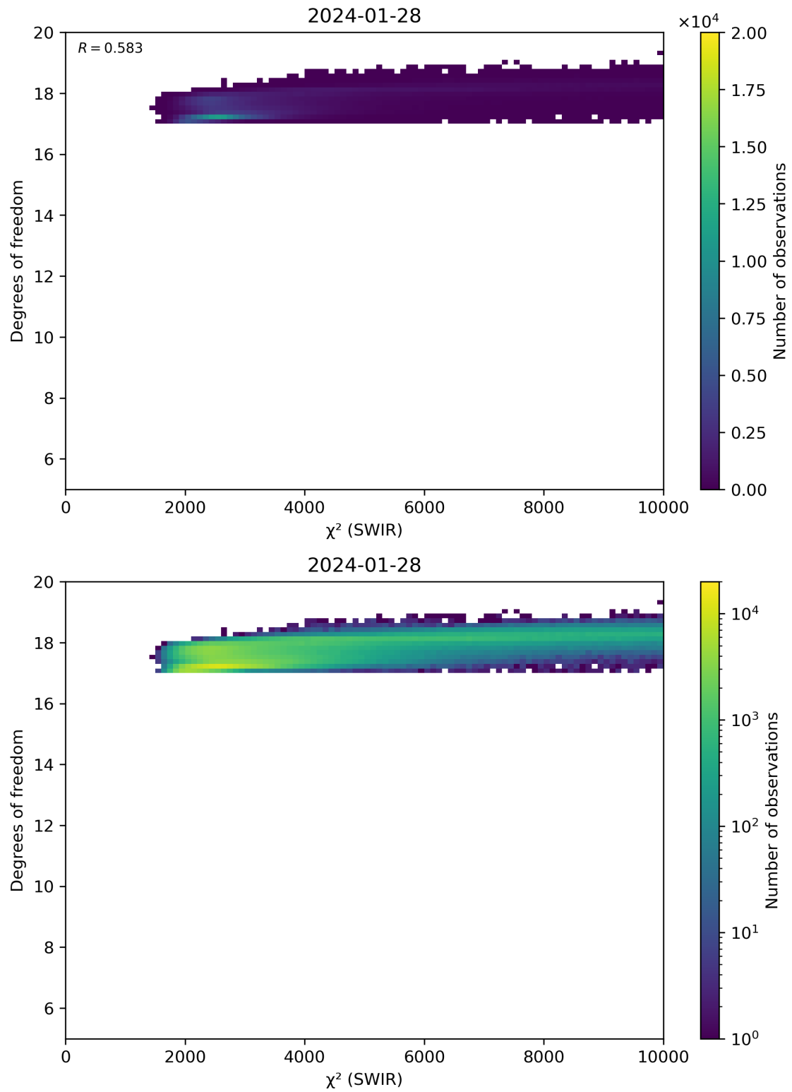
Figure 48: Scatter density plot of “ \chi^2 (SWIR)” against “Degrees of freedom” for 2024-01-27 to 2024-01-29.
