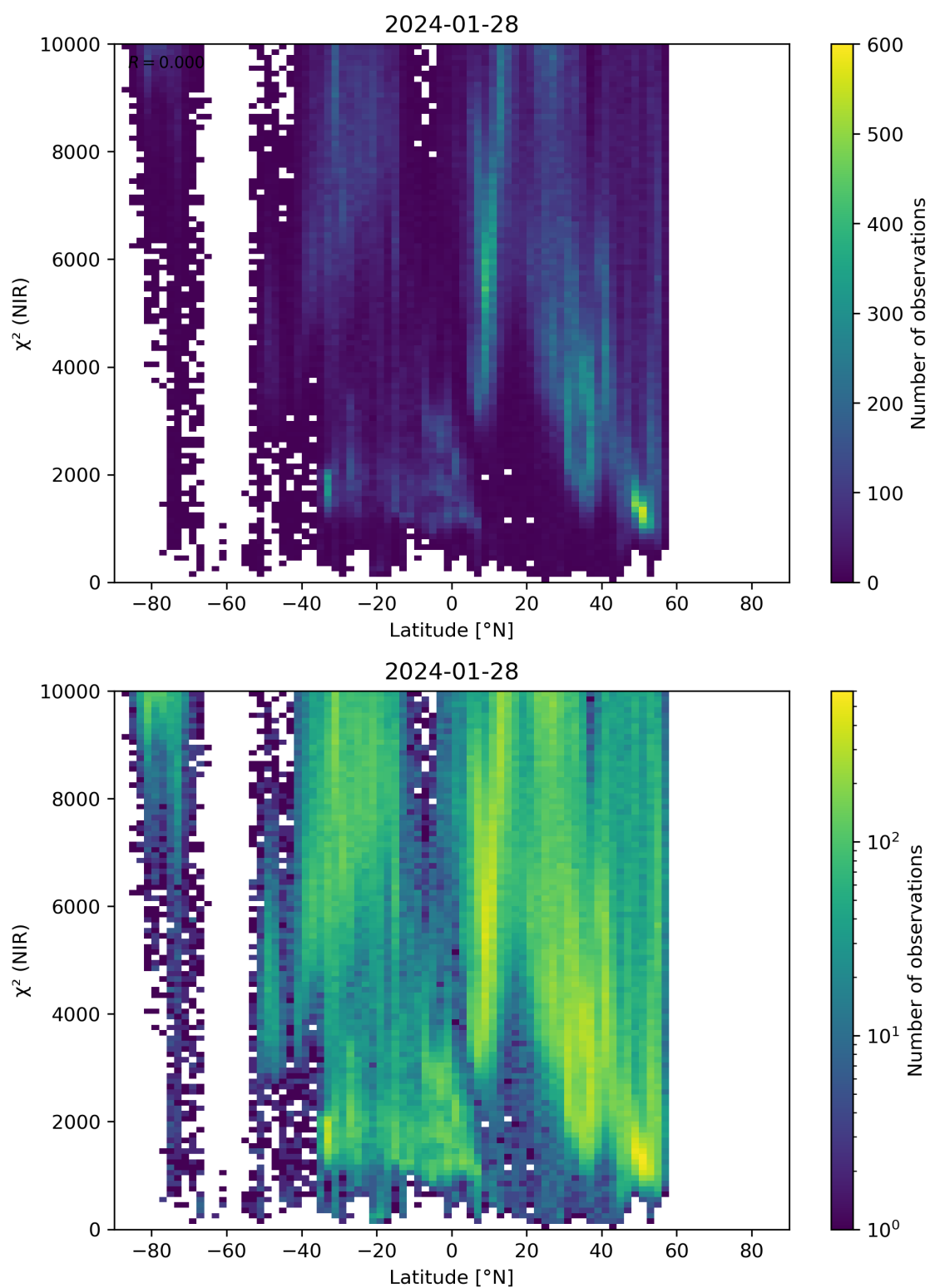
Figure 53: Scatter density plot of “Latitude” against “ \chi^2 (NIR)” for 2024-01-27 to 2024-01-29.
