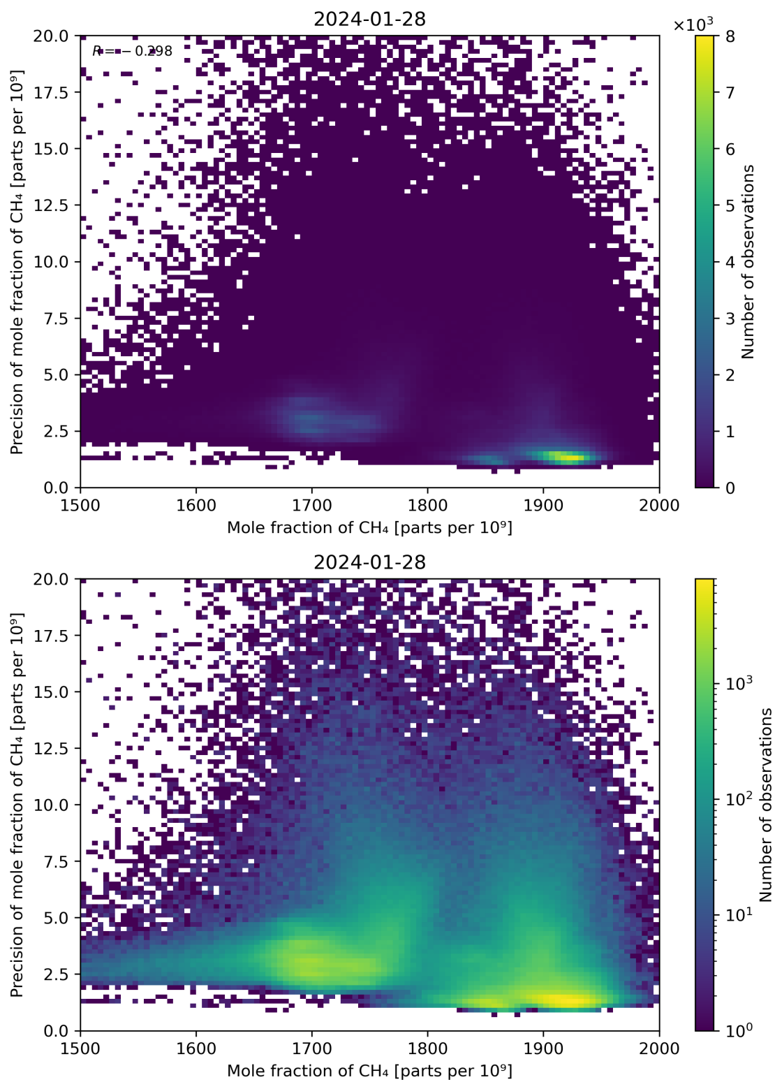
Figure 75: Scatter density plot of “Mole fraction of CH 4 ” against “Precision of mole fraction of CH 4 ” for 2024-01-27 to 2024-01-29.
