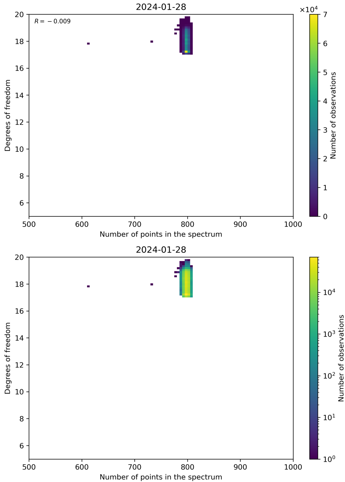
Figure 90: Scatter density plot of “Number of points in the spectrum” against “Degrees of freedom” for 2024-01-27 to 2024-01-29.
