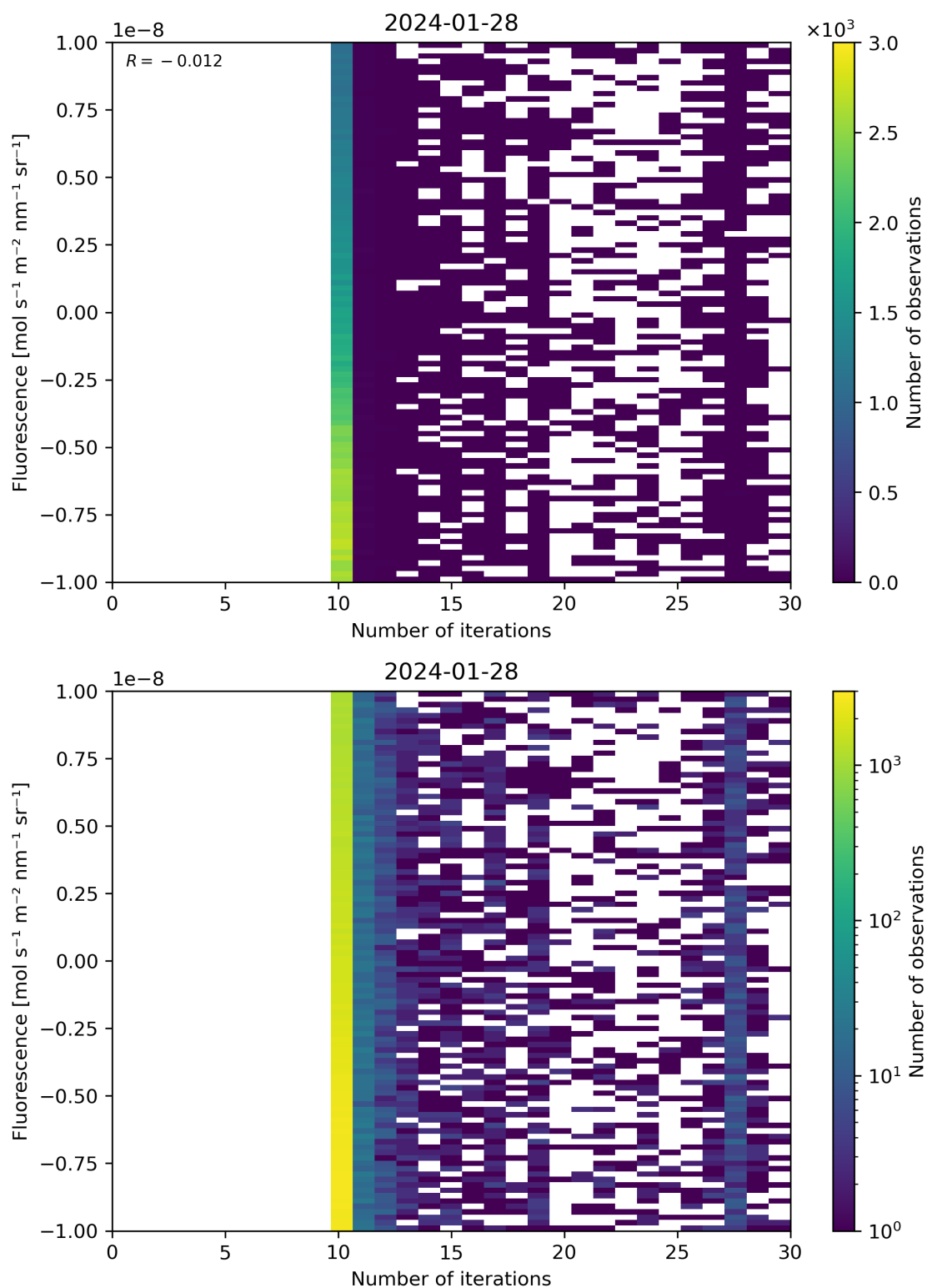
Figure 87: Scatter density plot of “Number of iterations” against “Fluorescence” for 2024-01-27 to 2024-01-29.
