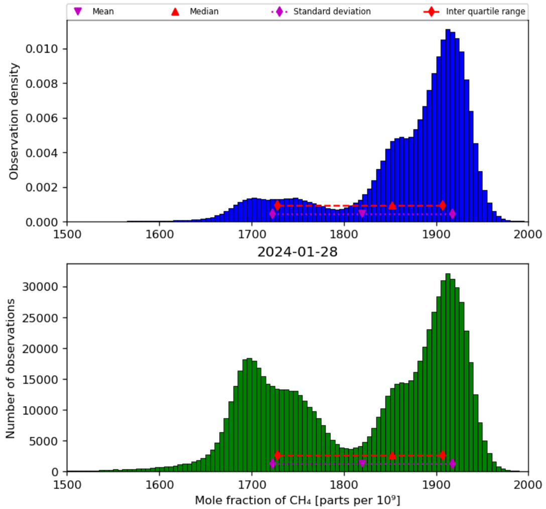
Figure 23: Histogram of “Mole fraction of CH 4 ” for 2024-01-27 to 2024-01-29
