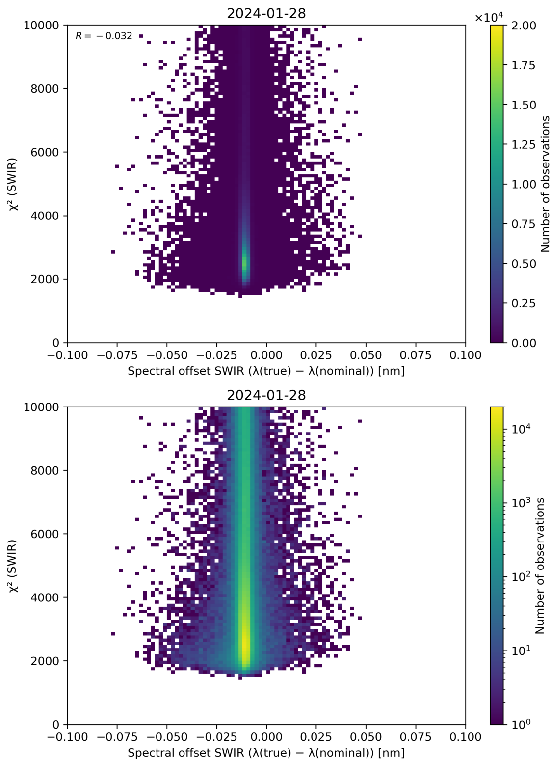
Figure 118: Scatter density plot of “Spectral offset SWIR ( \lambda(\text{true}) - \lambda(\text{nominal}) )” against “ \chi^2 (SWIR)” for 2024-01-27 to 2024-01-29.
