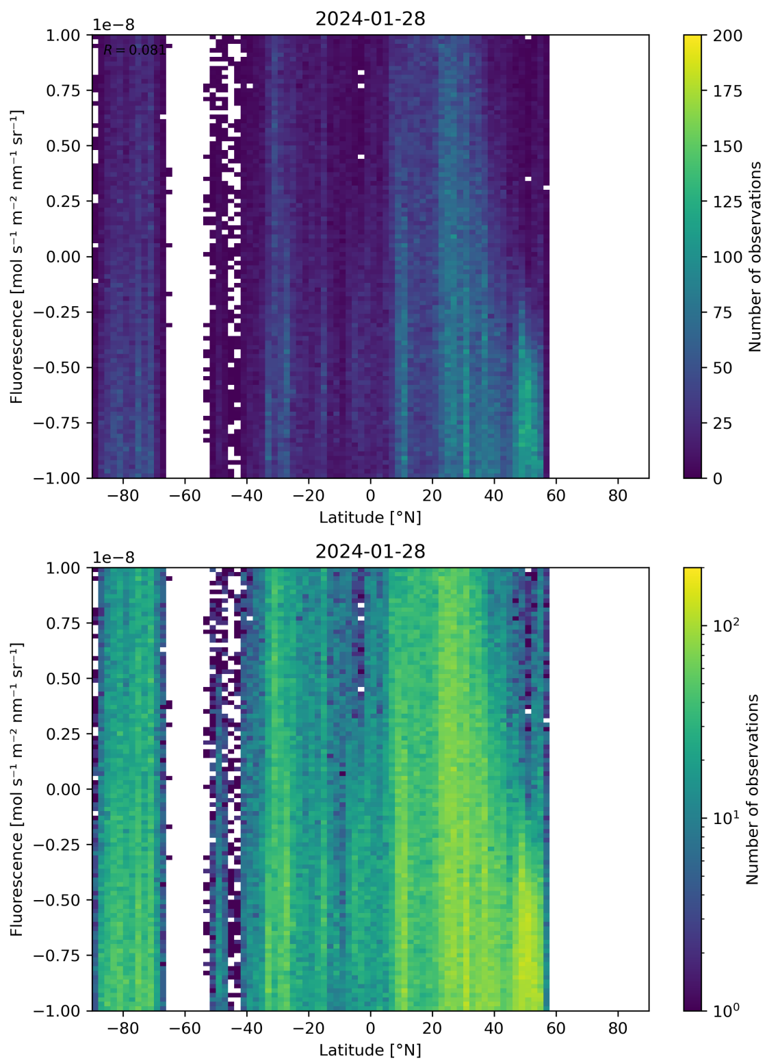
Figure 56: Scatter density plot of “Latitude” against “Fluorescence” for 2024-01-27 to 2024-01-29.
