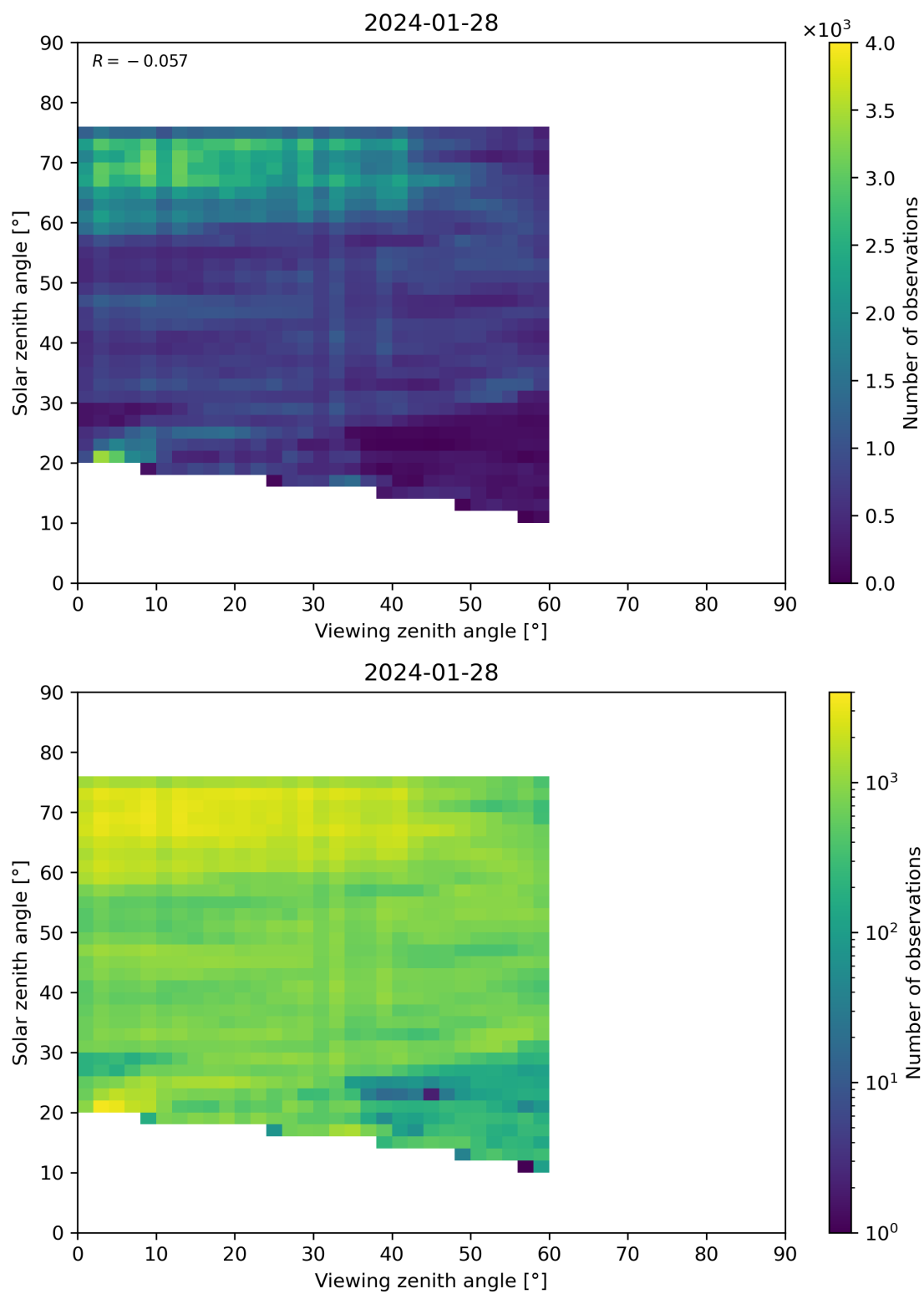
Figure 115: Scatter density plot of “Viewing zenith angle” against “Solar zenith angle” for 2024-01-27 to 2024-01-29.
