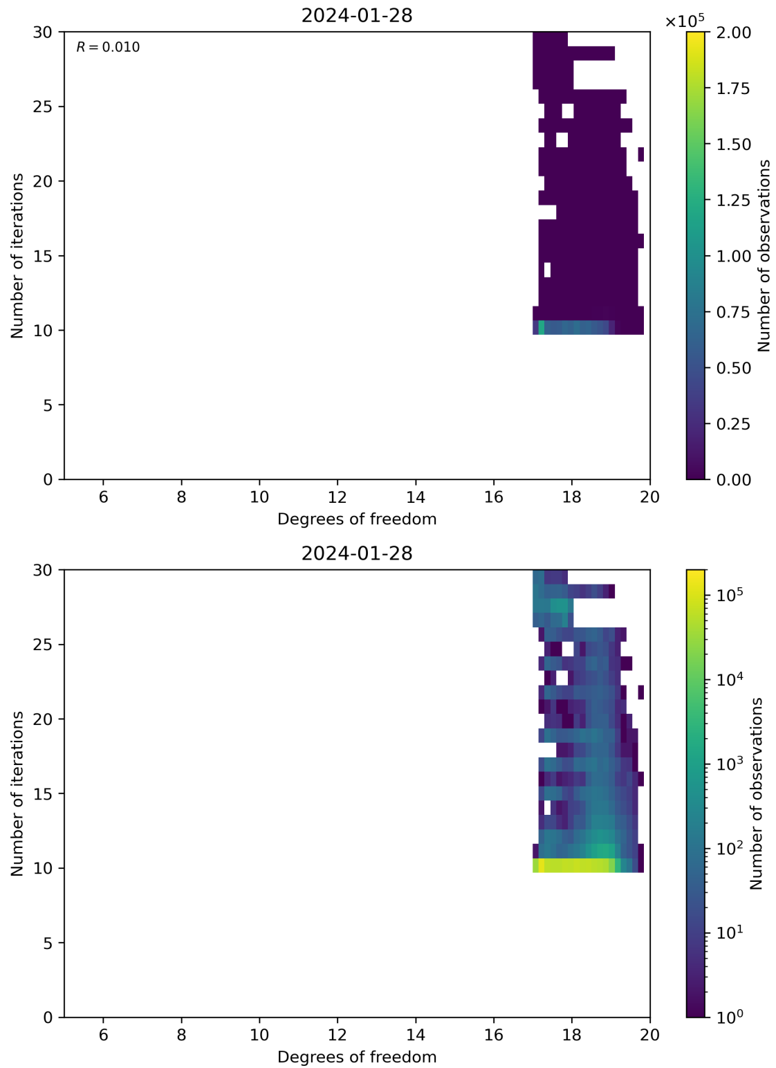
Figure 52: Scatter density plot of “Degrees of freedom” against “Number of iterations” for 2024-01-27 to 2024-01-29.
