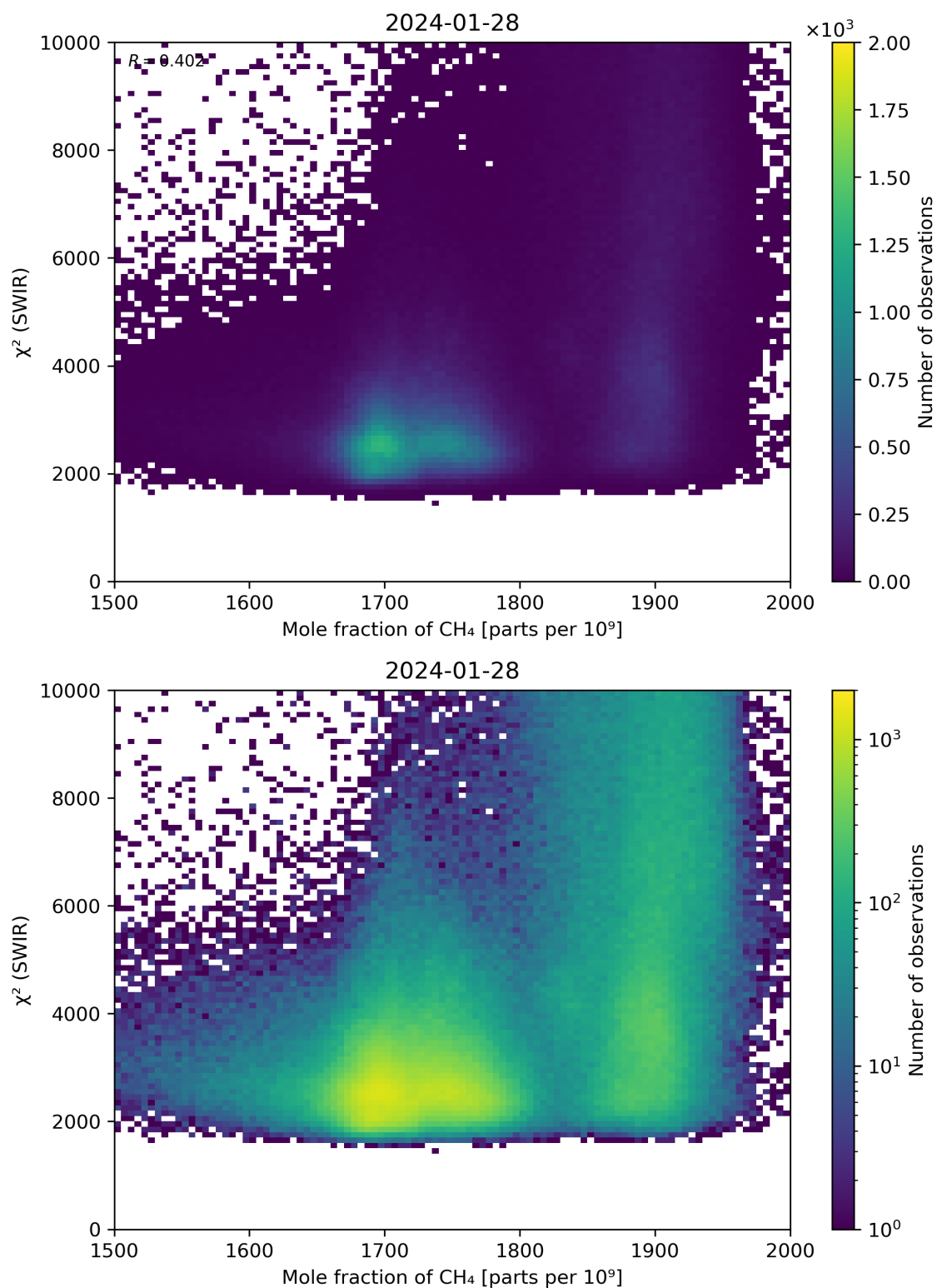
Figure 71: Scatter density plot of “Mole fraction of \text{CH}_4 ” against “ \chi^2 (SWIR)” for 2024-01-27 to 2024-01-29.
