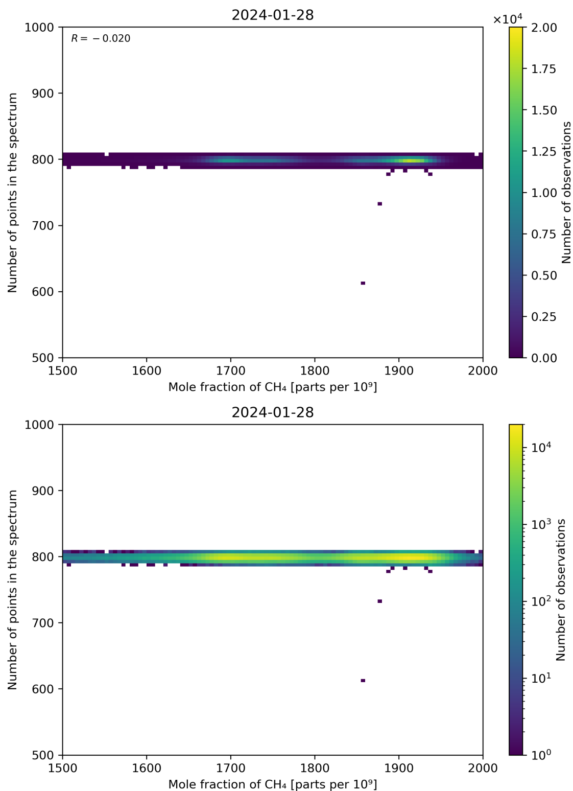
Figure 77: Scatter density plot of “Mole fraction of CH 4 ” against “Number of points in the spectrum” for 2024-01-27 to 2024-01-29.
