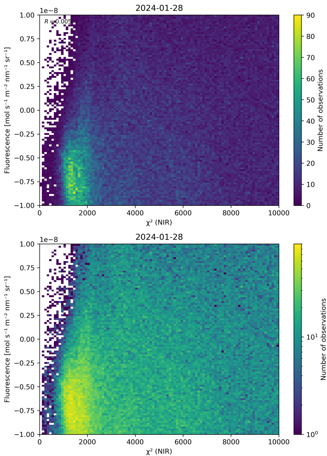
Figure 45: Scatter density plot of “ \chi^2 (NIR)” against “Fluorescence” for 2024-01-27 to 2024-01-29.
