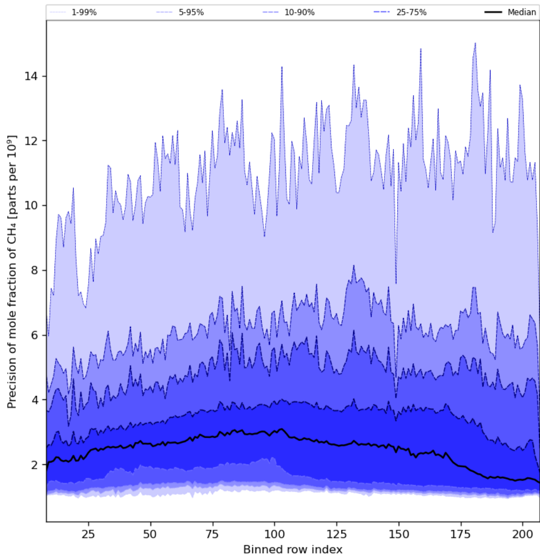
Figure 35: Along track statistics of “Precision of mole fraction of CH 4 ” for 2024-01-27 to 2024-01-29
