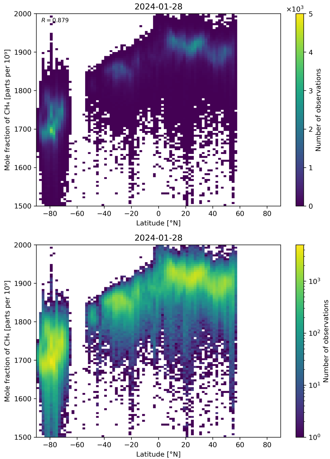
Figure 57: Scatter density plot of “Latitude” against “Mole fraction of CH 4 ” for 2024-01-27 to 2024-01-29.
