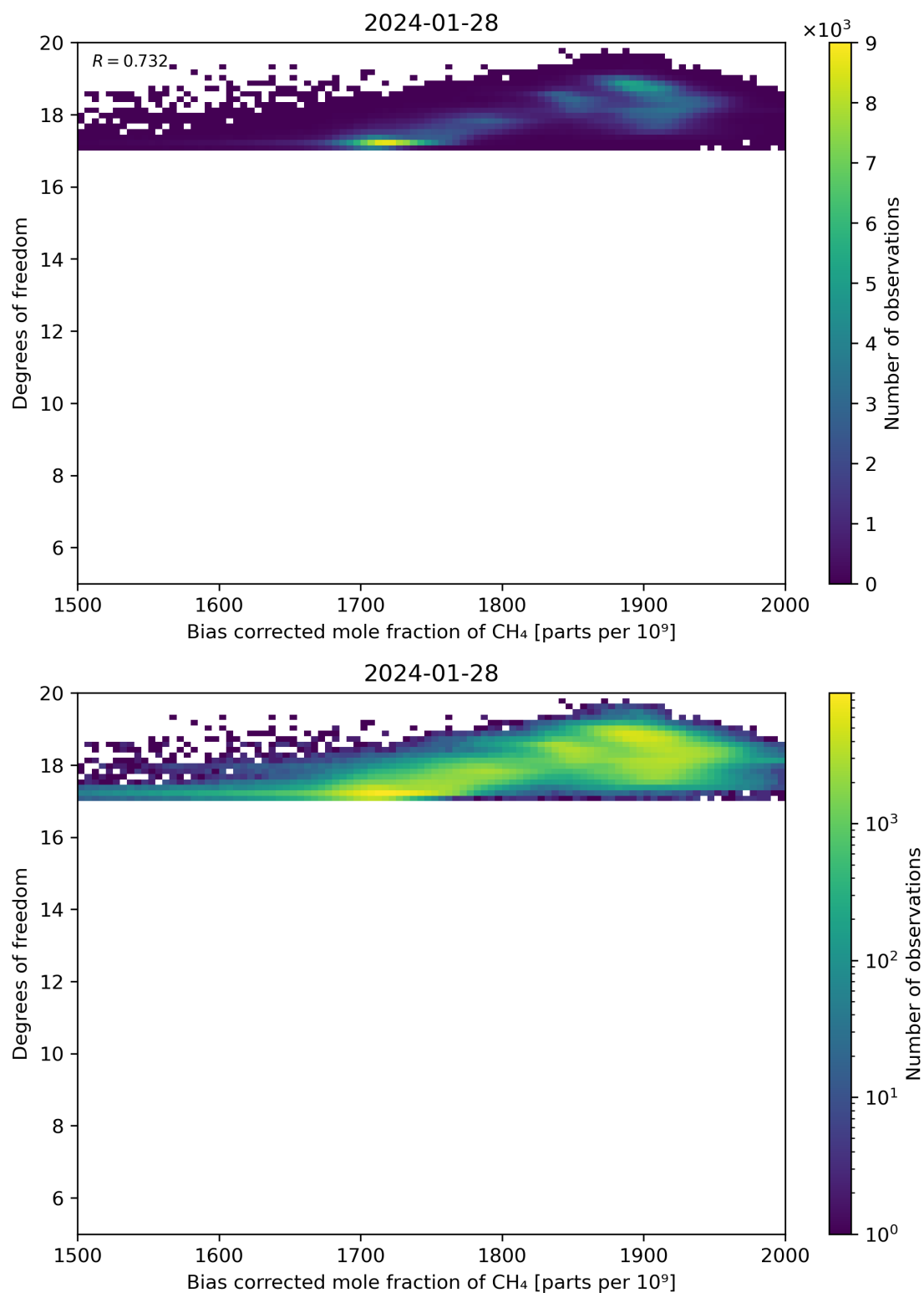
Figure 65: Scatter density plot of “Bias corrected mole fraction of CH 4 ” against “Degrees of freedom” for 2024-01-27 to 2024-01-29.
