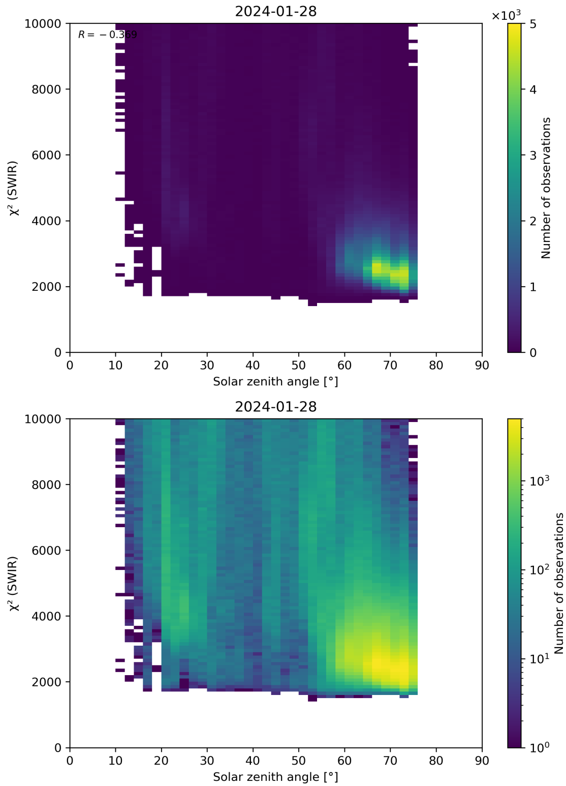
Figure 95: Scatter density plot of “Solar zenith angle” against “ \chi^2 (SWIR)” for 2024-01-27 to 2024-01-29.
