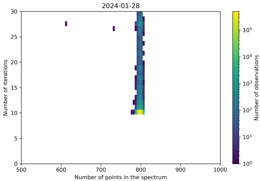
Figure 92: Scatter density plot of “Number of points in the spectrum” against “Number of iterations” for 2024-01-27 to 2024-01-29.
