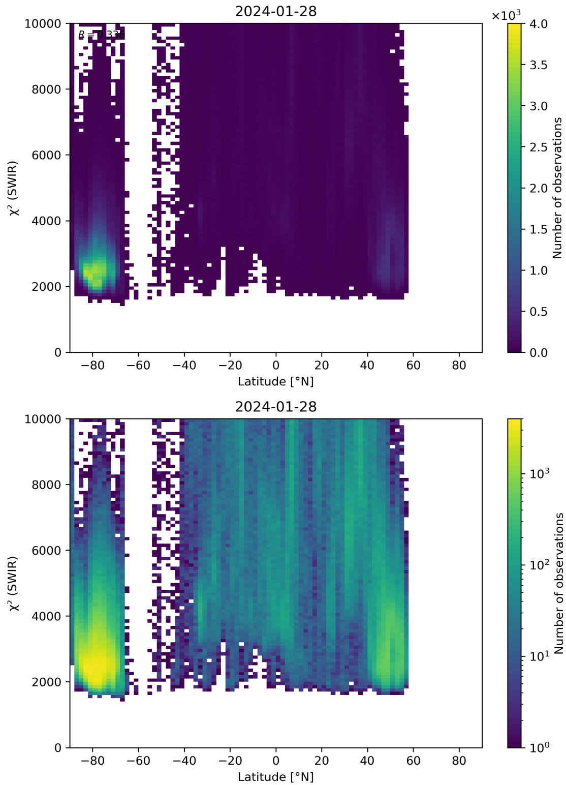
Figure 54: Scatter density plot of “Latitude” against “ \chi^2 (SWIR)” for 2024-01-27 to 2024-01-29.
