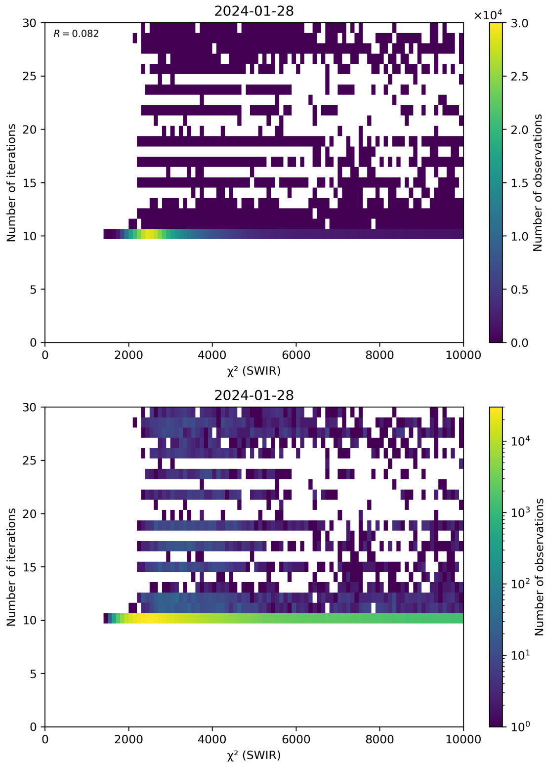
Figure 50: Scatter density plot of “ \chi^2 (SWIR)” against “Number of iterations” for 2024-01-27 to 2024-01-29.
