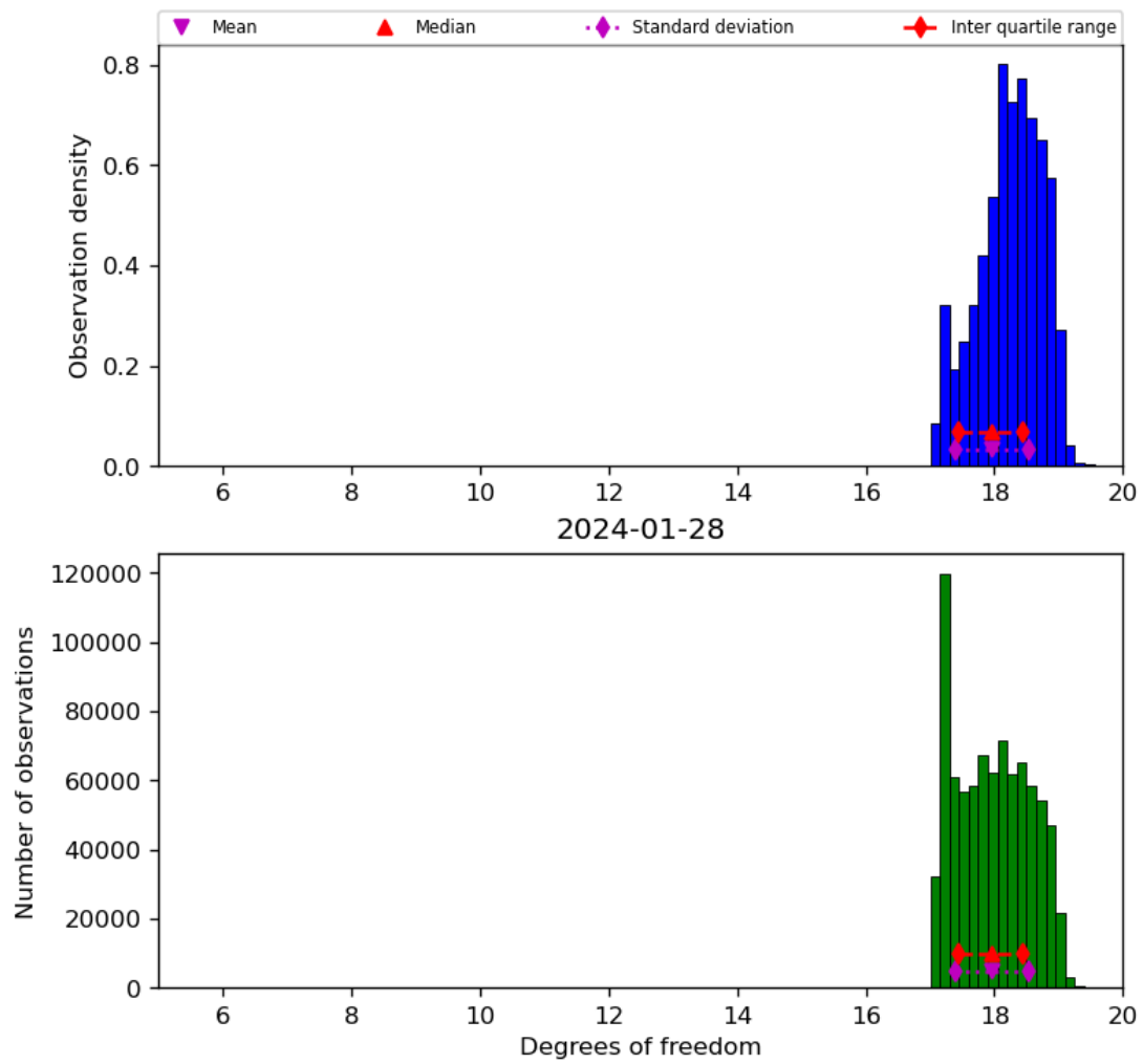
Figure 30: Histogram of “Degrees of freedom” for 2024-01-27 to 2024-01-29
