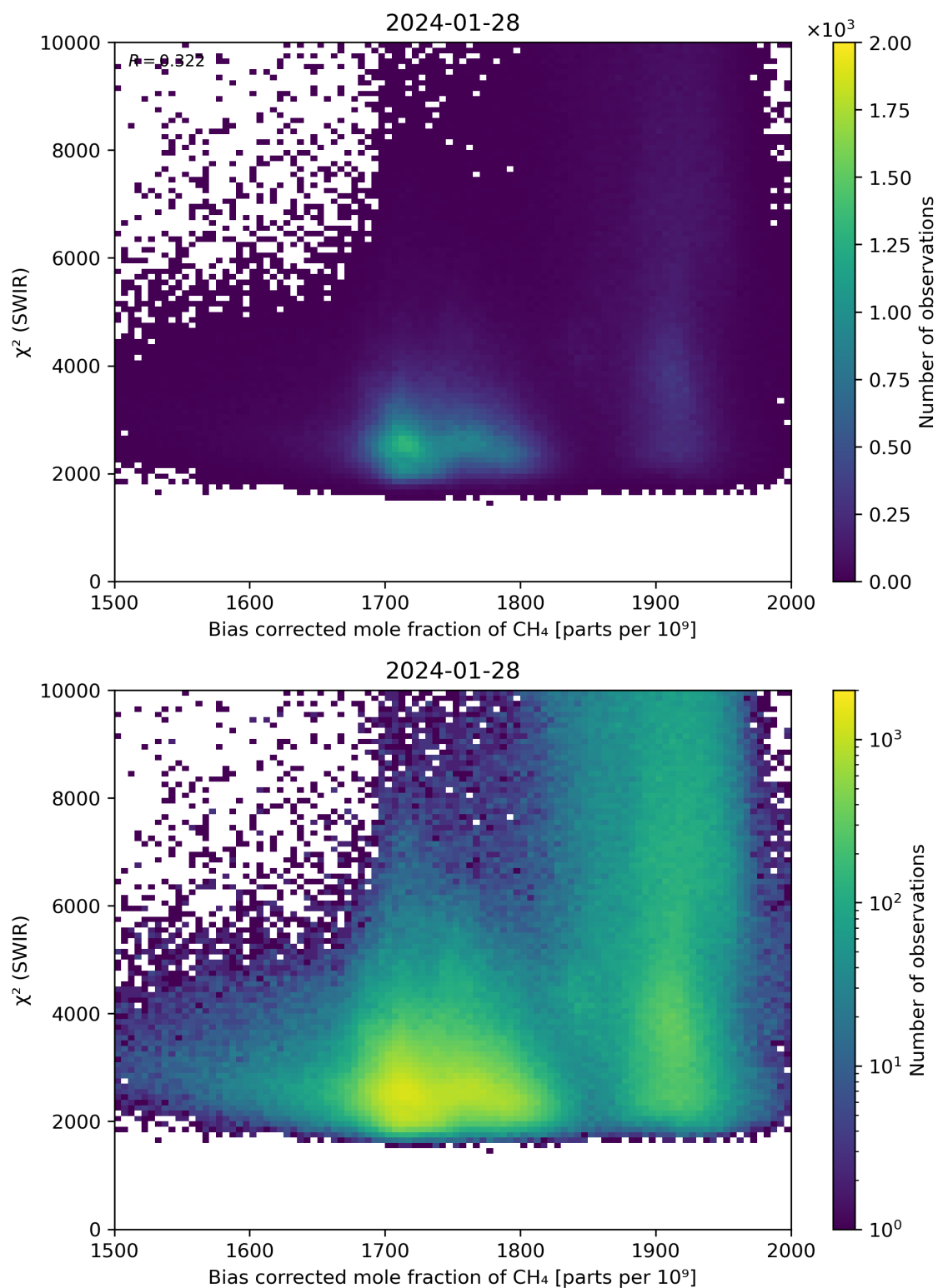
Figure 64: Scatter density plot of “Bias corrected mole fraction of CH 4 ” against “ \chi^2 (SWIR)” for 2024-01-27 to 2024-01-29.
