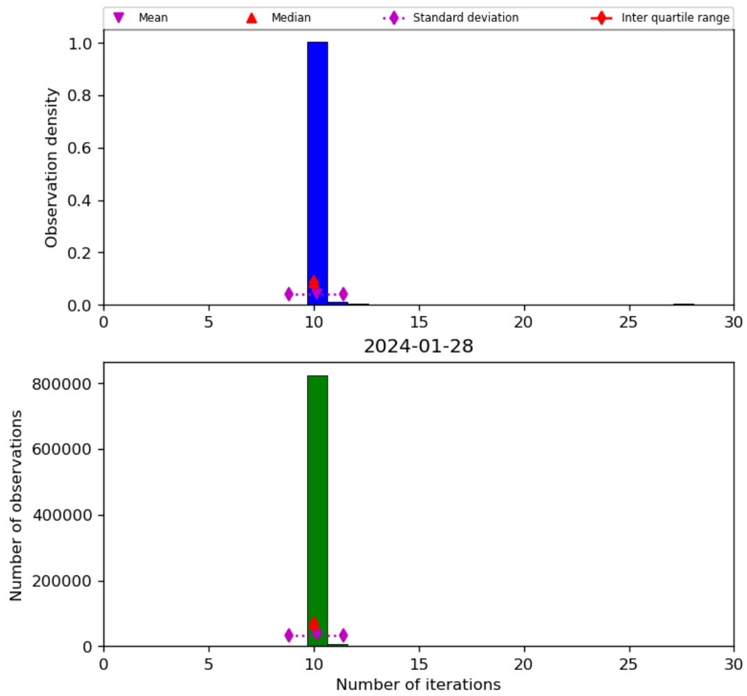
Figure 31: Histogram of "Number of iterations" for 2024-01-27 to 2024-01-29
