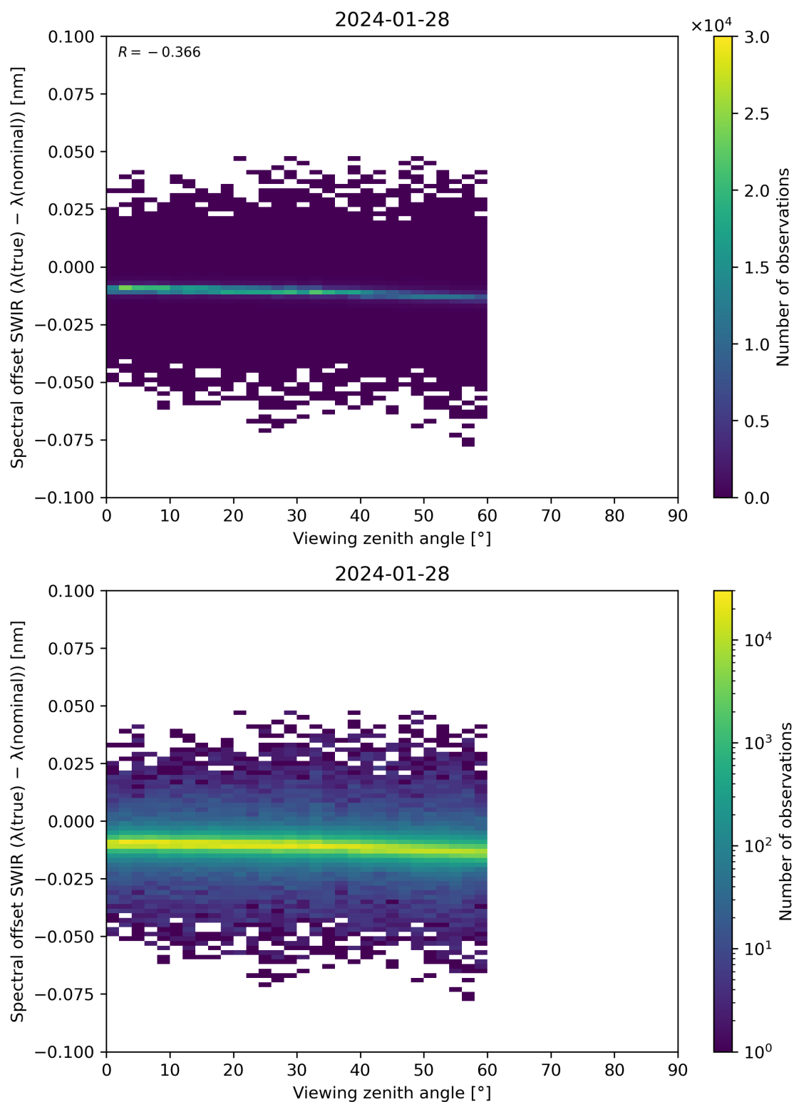
Figure 116: Scatter density plot of “Viewing zenith angle” against “Spectral offset SWIR ( \lambda(\text{true}) - \lambda(\text{nominal}) )” for 2024-01-27 to 2024-01-29.
