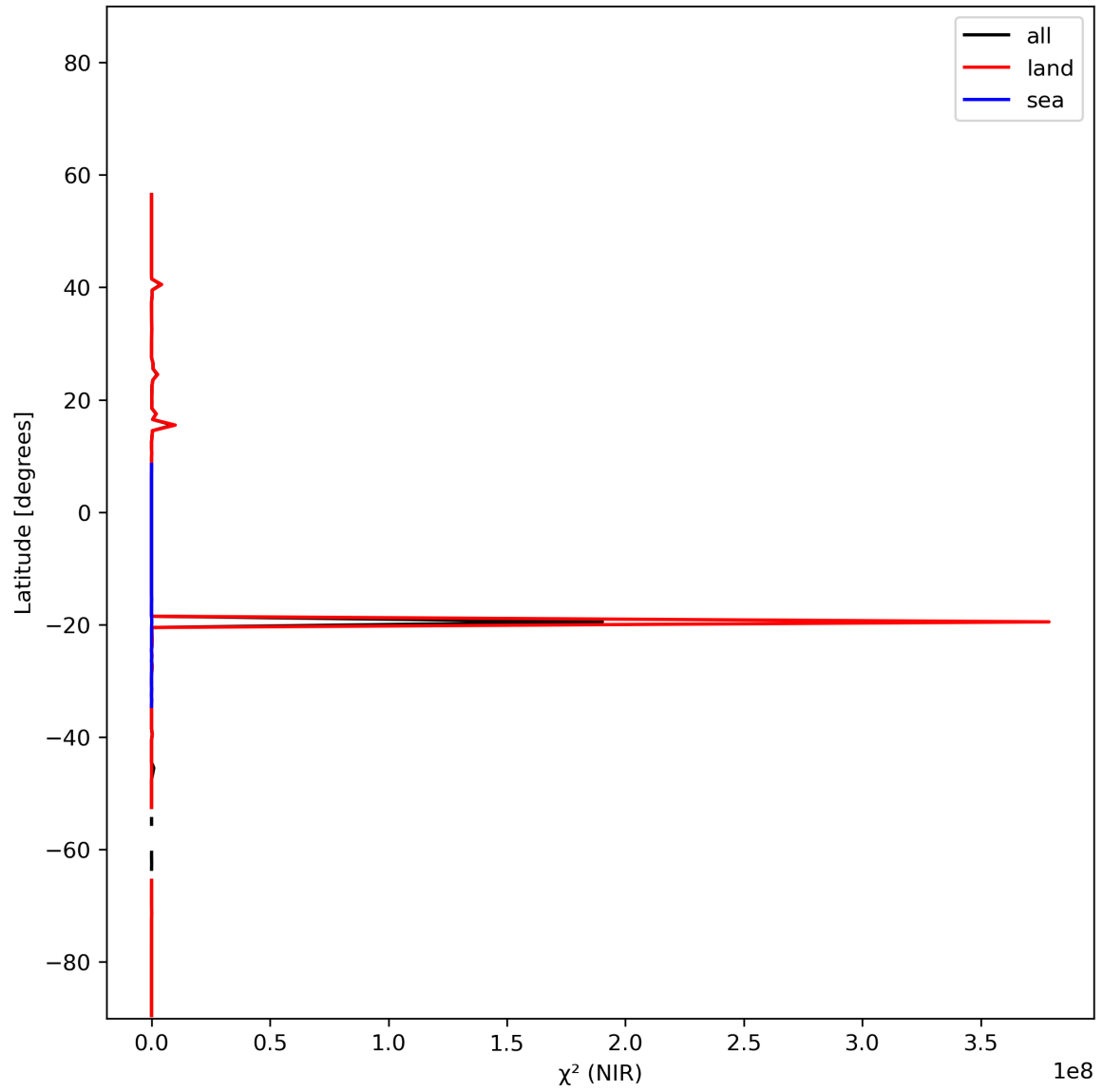
Figure 18: Zonal average of “ \chi^2 (NIR)” for 2024-01-27 to 2024-01-29.
