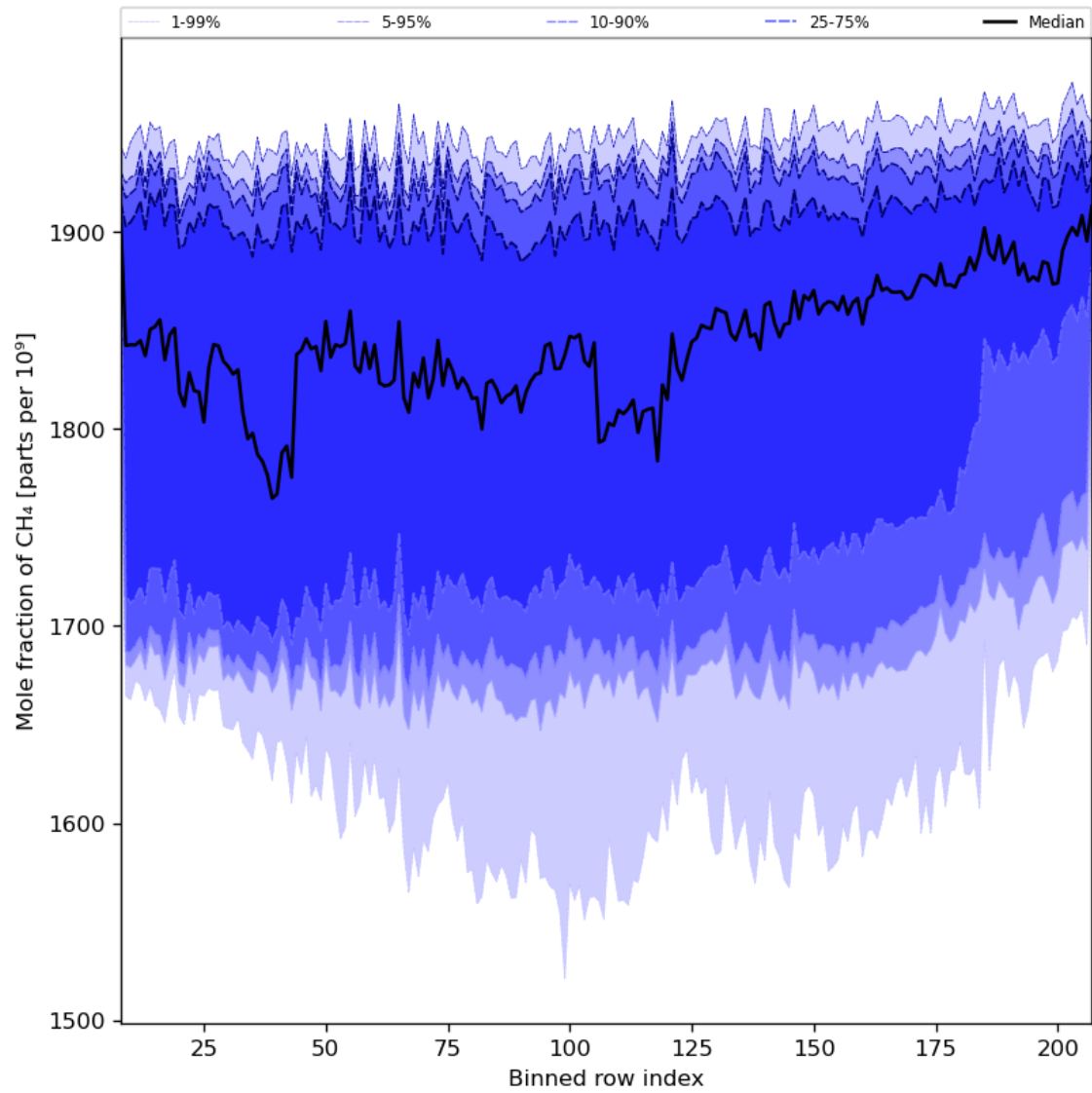
Figure 34: Along track statistics of “Mole fraction of CH 4 ” for 2024-01-27 to 2024-01-29
