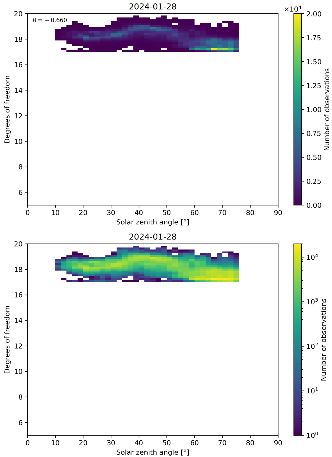
Figure 96: Scatter density plot of “Solar zenith angle” against “Degrees of freedom” for 2024-01-27 to 2024-01-29.
