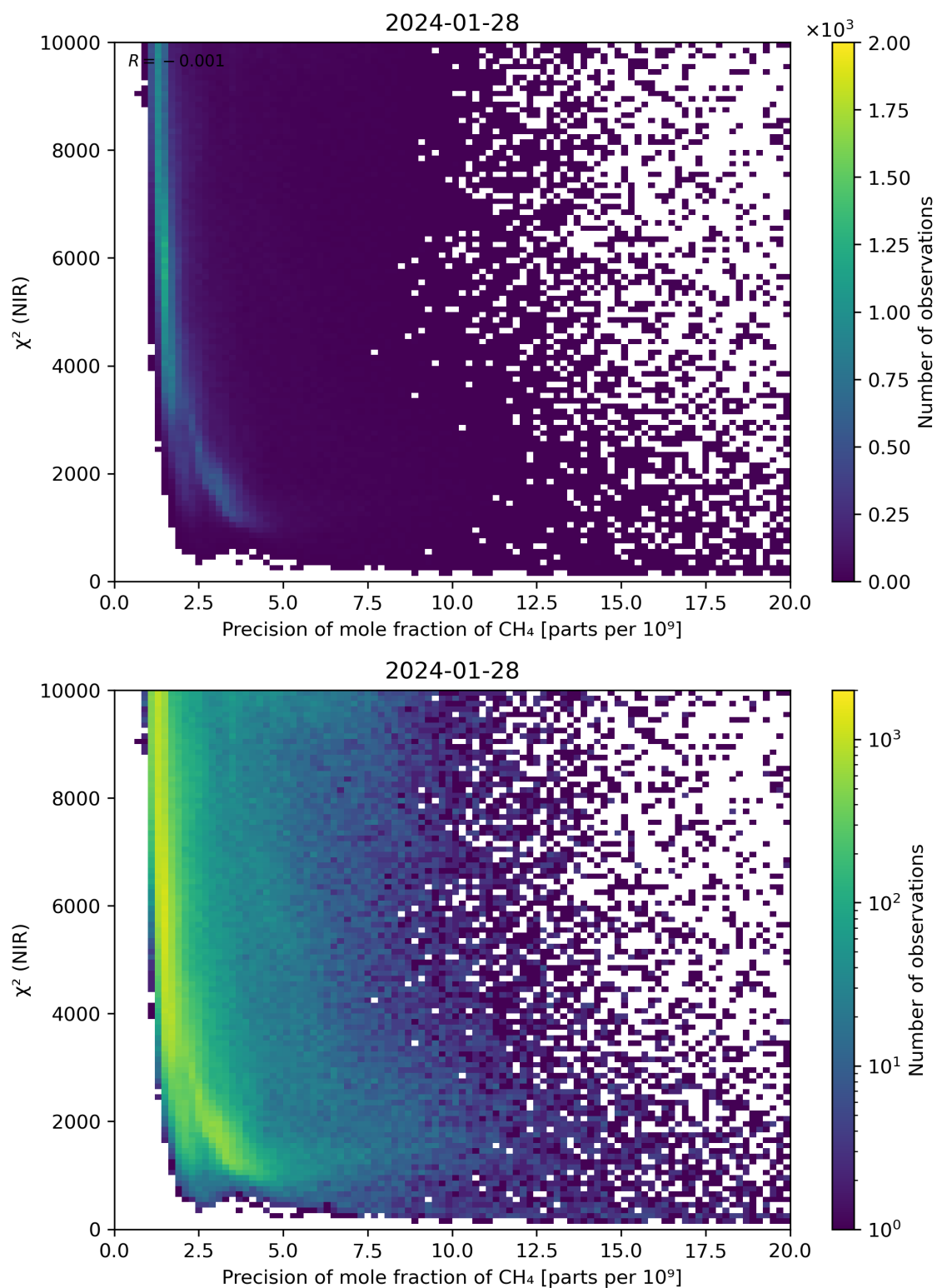
Figure 78: Scatter density plot of “Precision of mole fraction of CH 4 ” against “ \chi^2 (NIR)” for 2024-01-27 to 2024-01-29.
