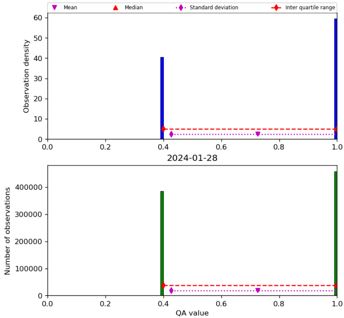
Figure 22: Histogram of “QA value” for 2024-01-27 to 2024-01-29
