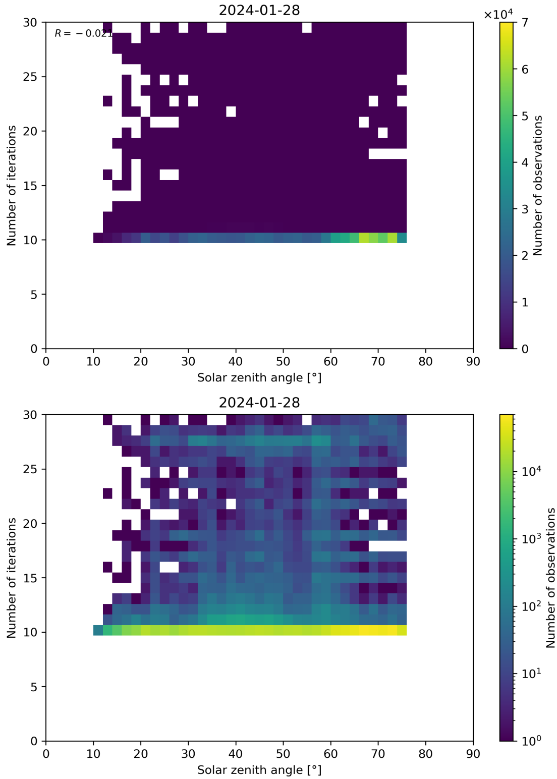
Figure 102: Scatter density plot of “Solar zenith angle” against “Number of iterations” for 2024-01-27 to 2024-01-29.
