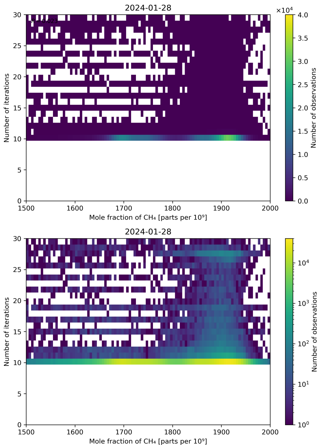
Figure 76: Scatter density plot of “Mole fraction of CH 4 ” against “Number of iterations” for 2024-01-27 to 2024-01-29.
