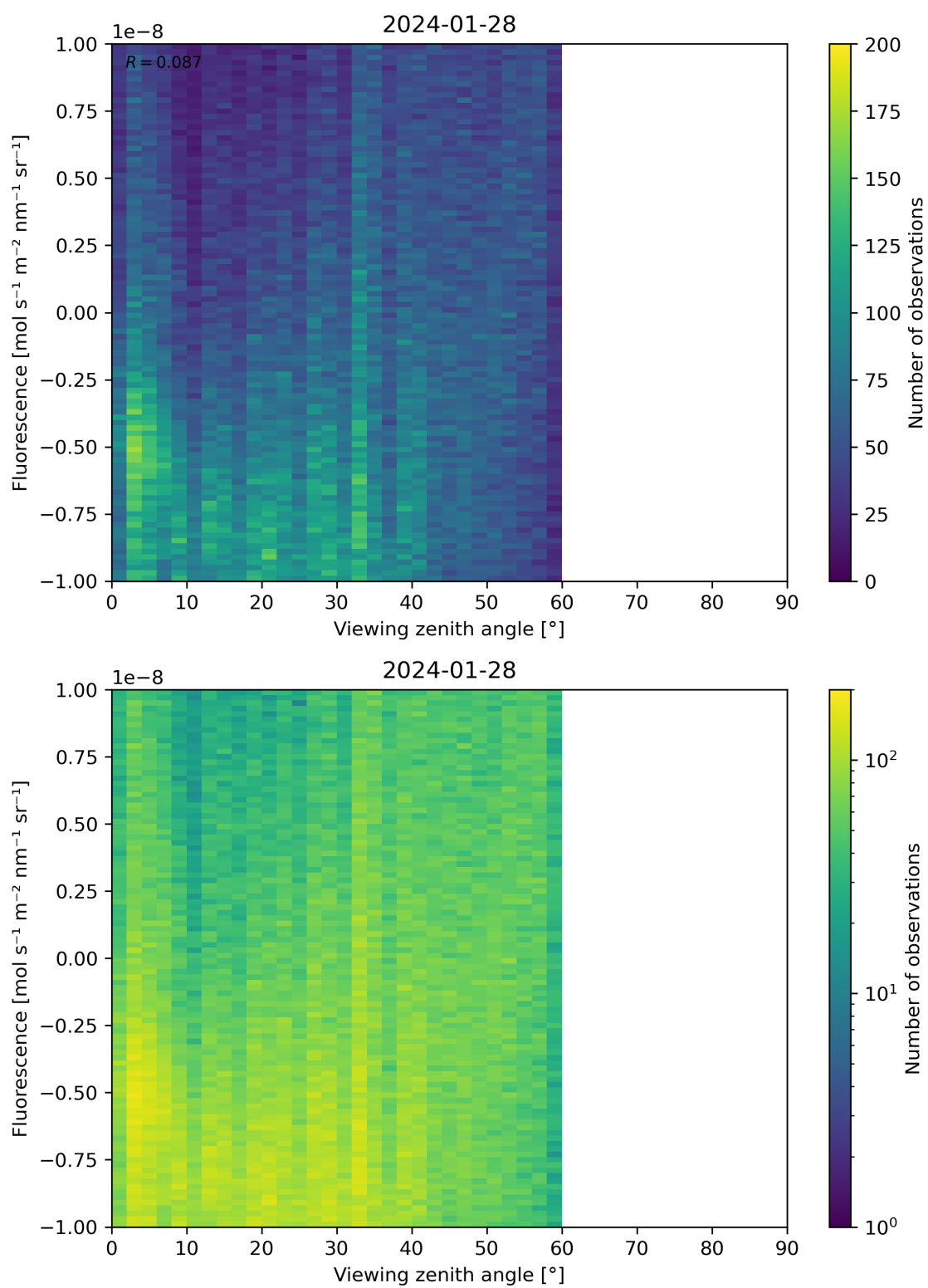
Figure 108: Scatter density plot of “Viewing zenith angle” against “Fluorescence” for 2024-01-27 to 2024-01-29.
