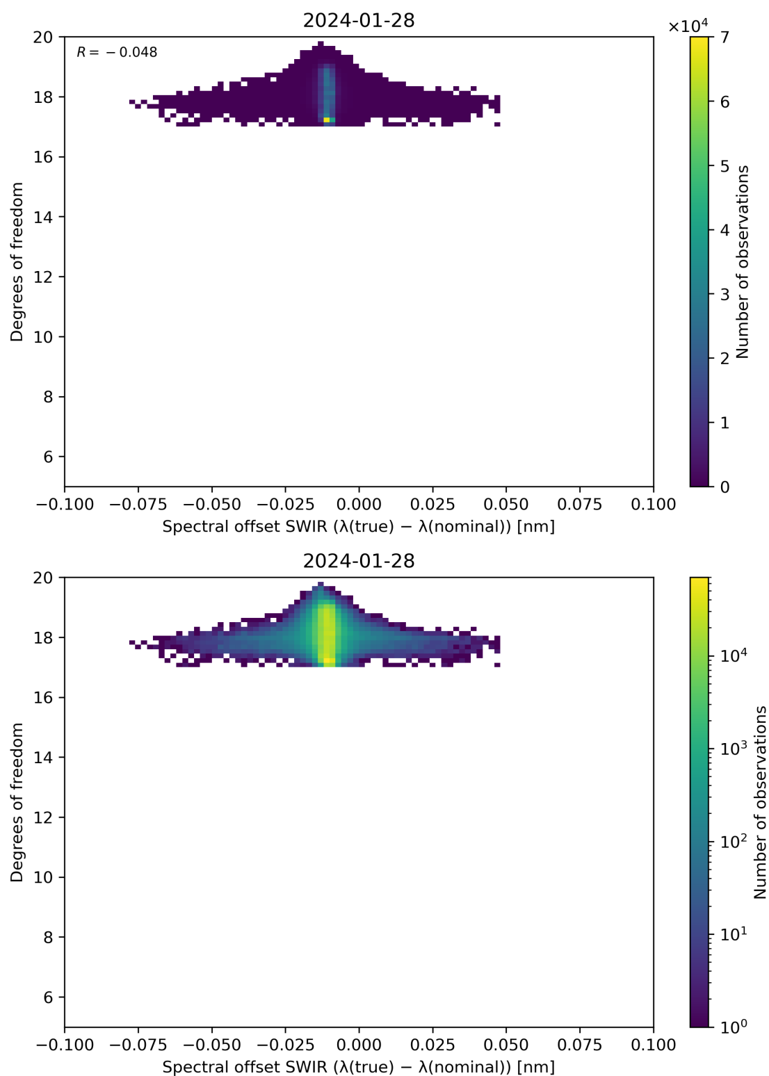
Figure 119: Scatter density plot of “Spectral offset SWIR ( \lambda(\text{true}) - \lambda(\text{nominal}) )” against “Degrees of freedom” for 2024-01-27 to 2024-01-29.
