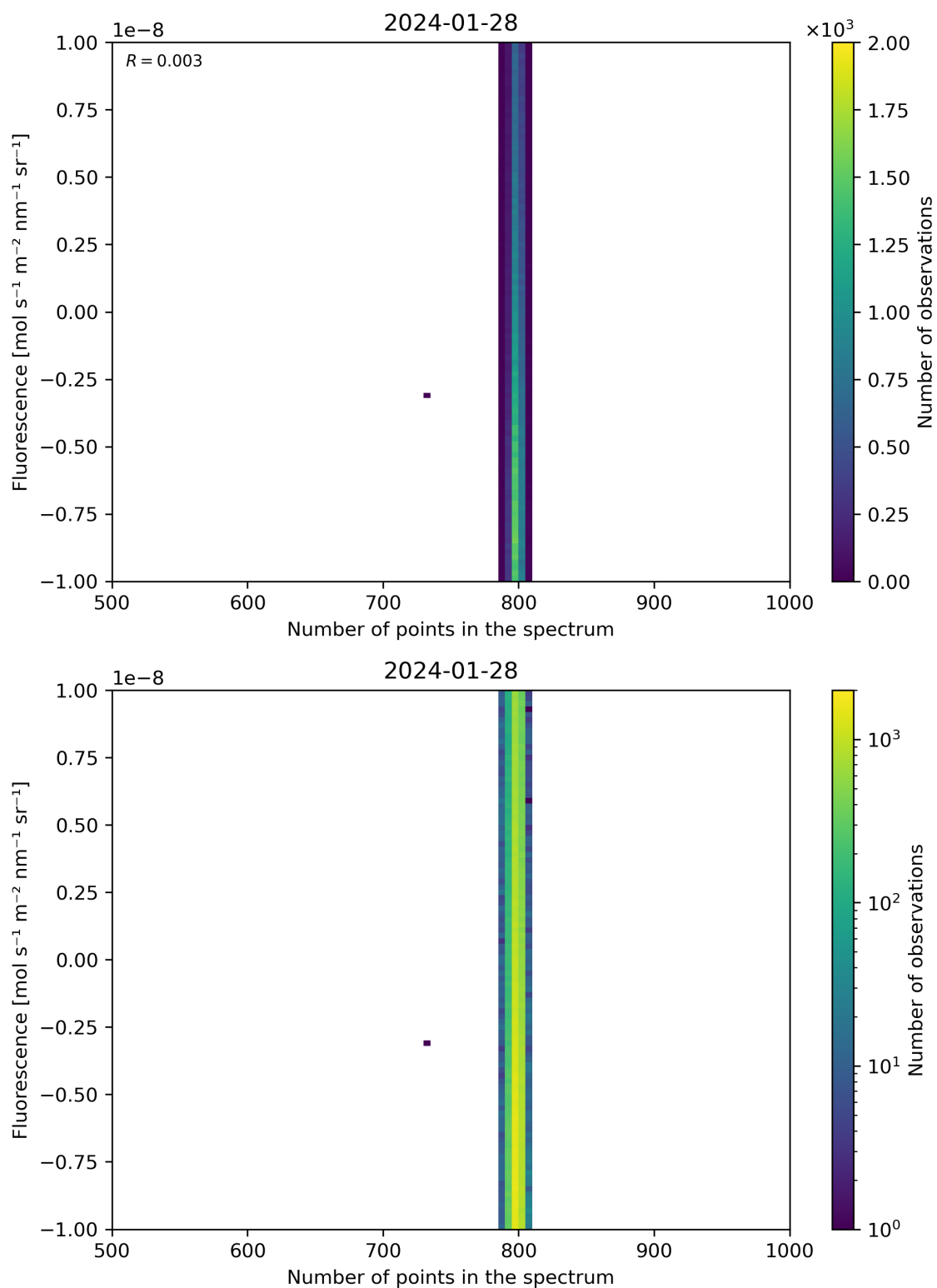
Figure 91: Scatter density plot of “Number of points in the spectrum” against “Fluorescence” for 2024-01-27 to 2024-01-29.
