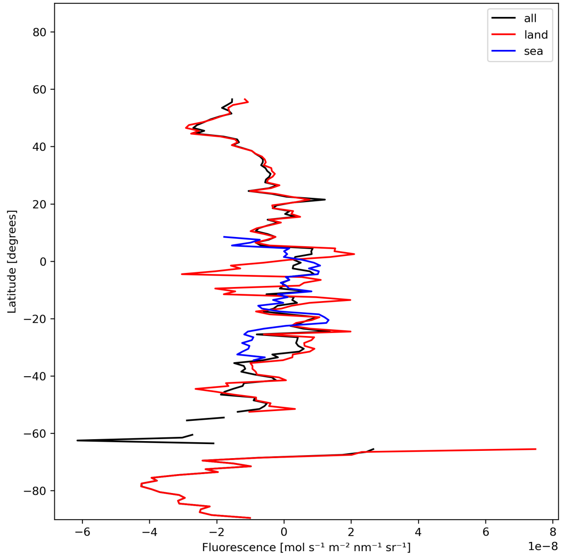
Figure 21: Zonal average of “Fluorescence” for 2024-01-27 to 2024-01-29.
