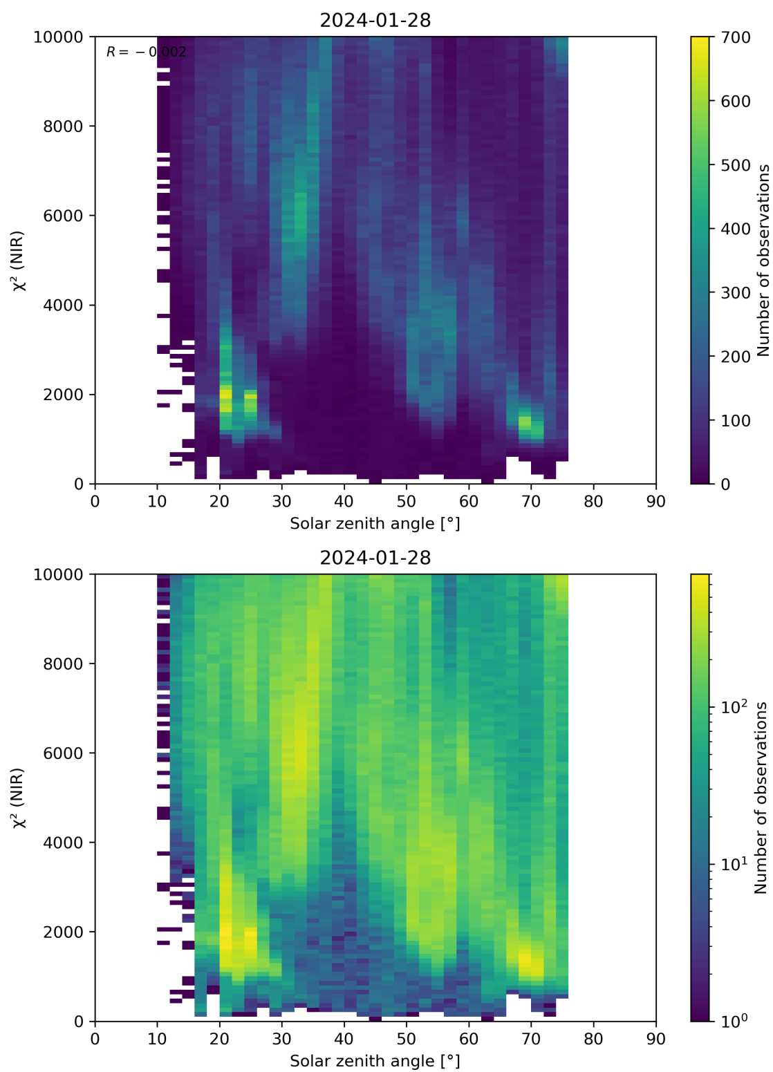
Figure 94: Scatter density plot of “Solar zenith angle” against “ \chi^2 (NIR)” for 2024-01-27 to 2024-01-29.
