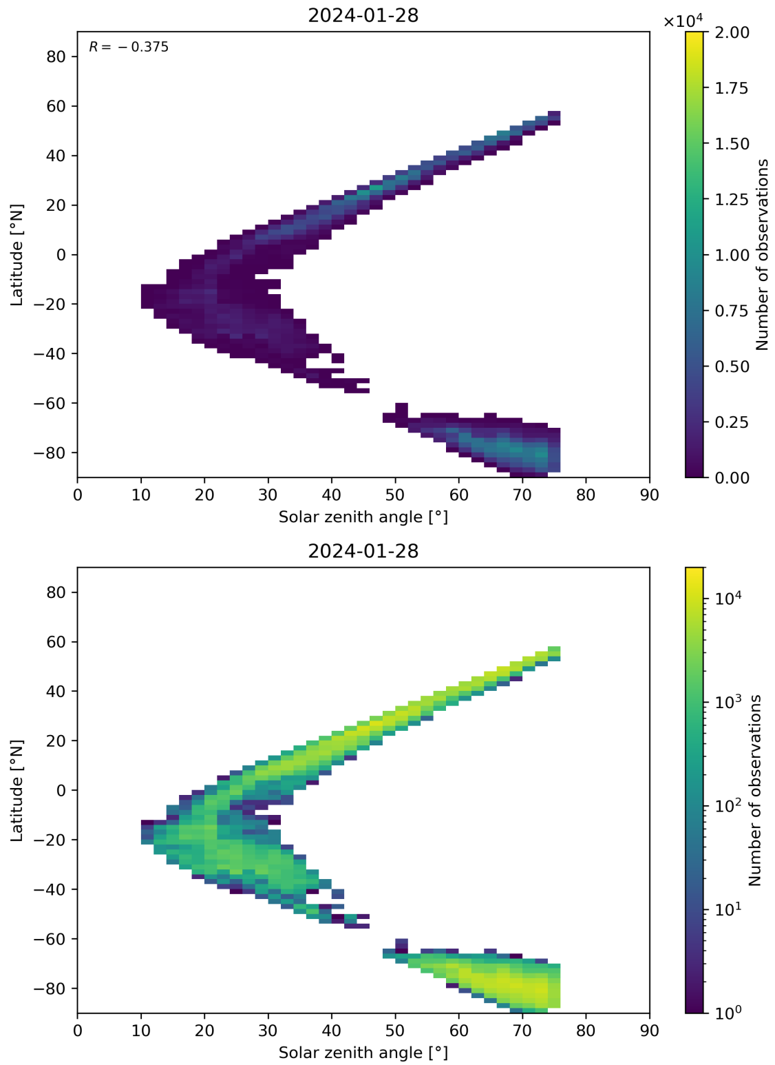
Figure 98: Scatter density plot of “Solar zenith angle” against “Latitude” for 2024-01-27 to 2024-01-29.
