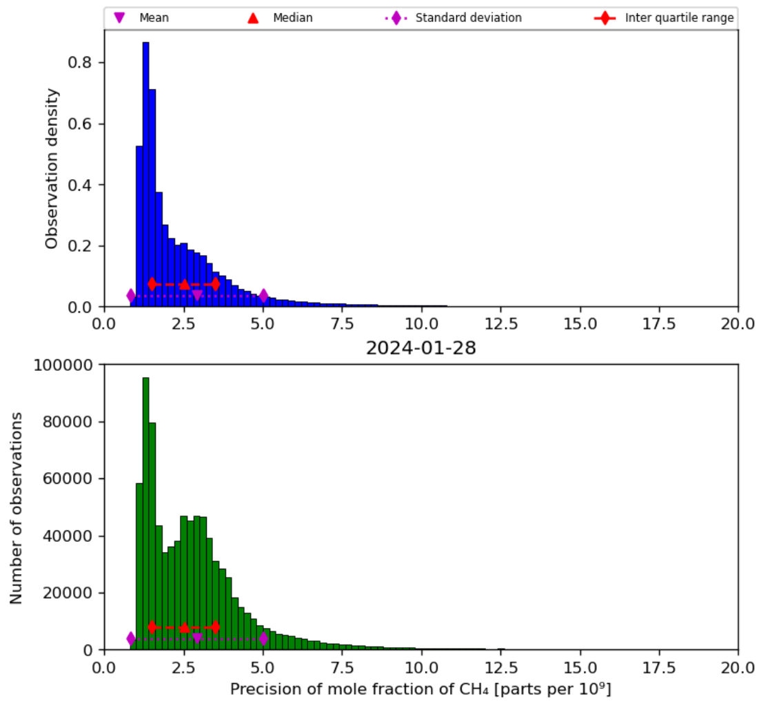
Figure 24: Histogram of “Precision of mole fraction of CH 4 ” for 2024-01-27 to 2024-01-29
