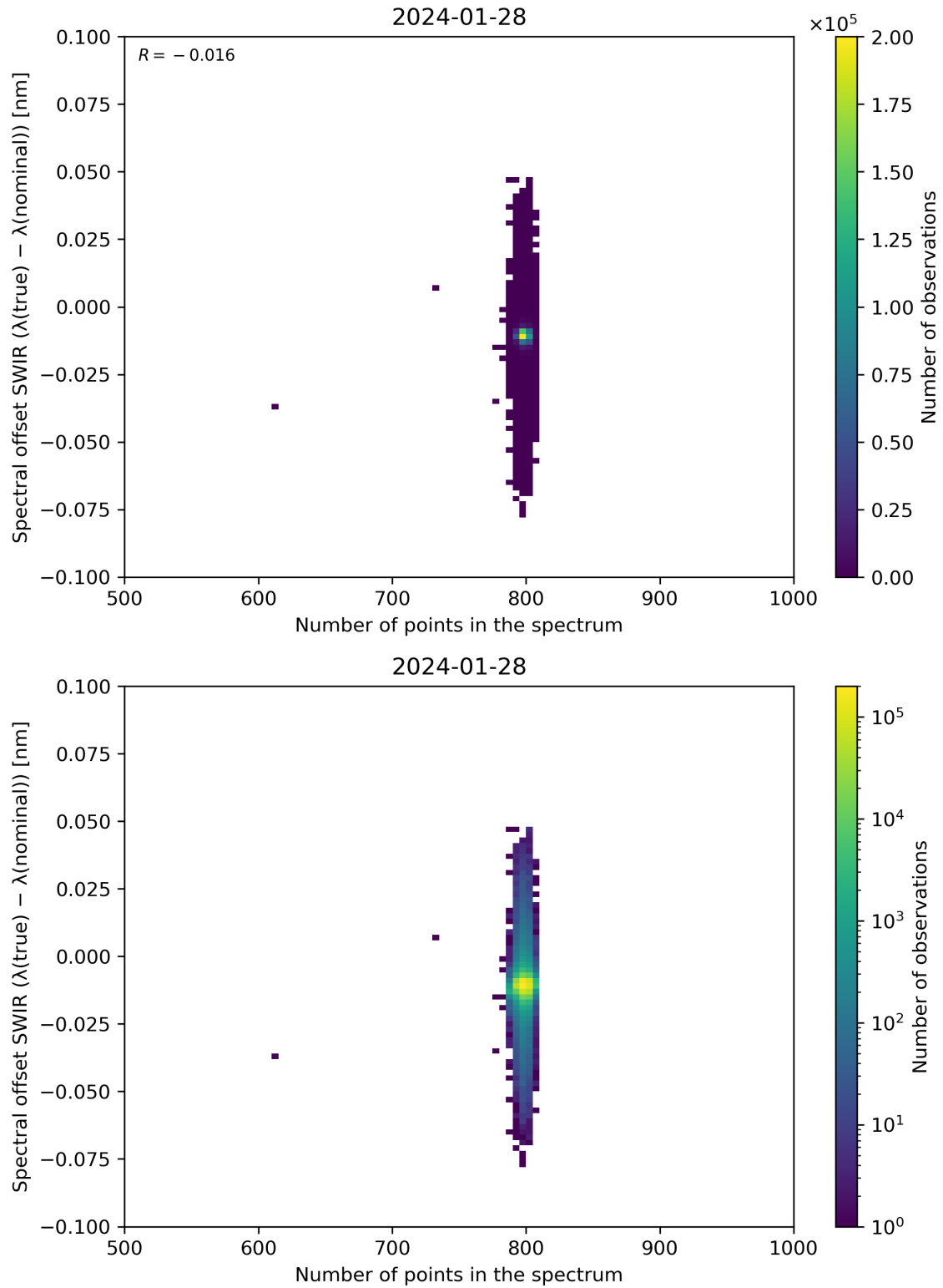
Figure 93: Scatter density plot of “Number of points in the spectrum” against “Spectral offset SWIR ( \lambda(\text{true}) - \lambda(\text{nominal}) )” for 2024-01-27 to 2024-01-29.
