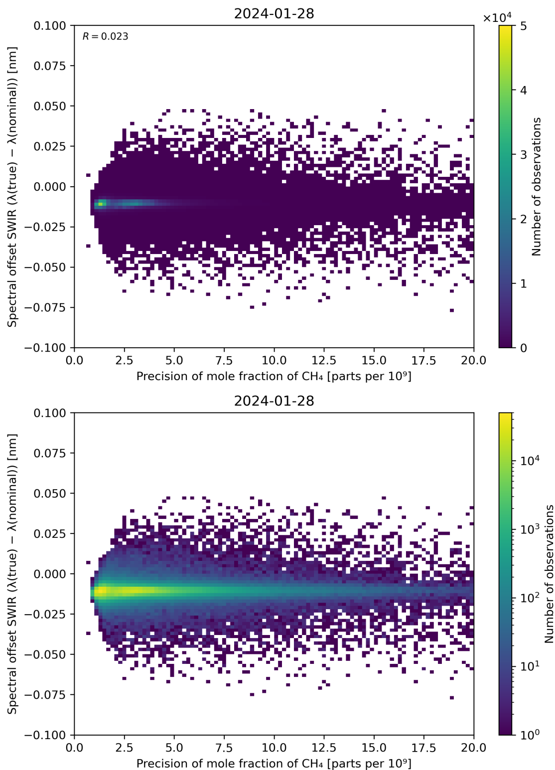
Figure 85: Scatter density plot of “Precision of mole fraction of \text{CH}_4 ” against “Spectral offset SWIR ( \lambda(\text{true}) - \lambda(\text{nominal}) )” for 2024-01-27 to 2024-01-29.
