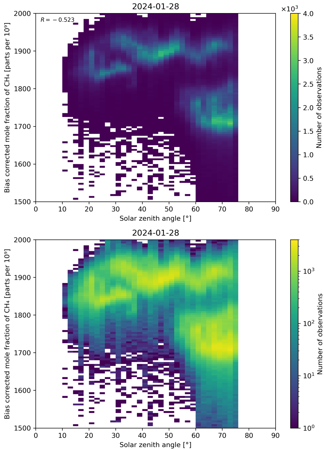
Figure 100: Scatter density plot of “Solar zenith angle” against “Bias corrected mole fraction of \text{CH}_4 ” for 2024-01-27 to 2024-01-29.
