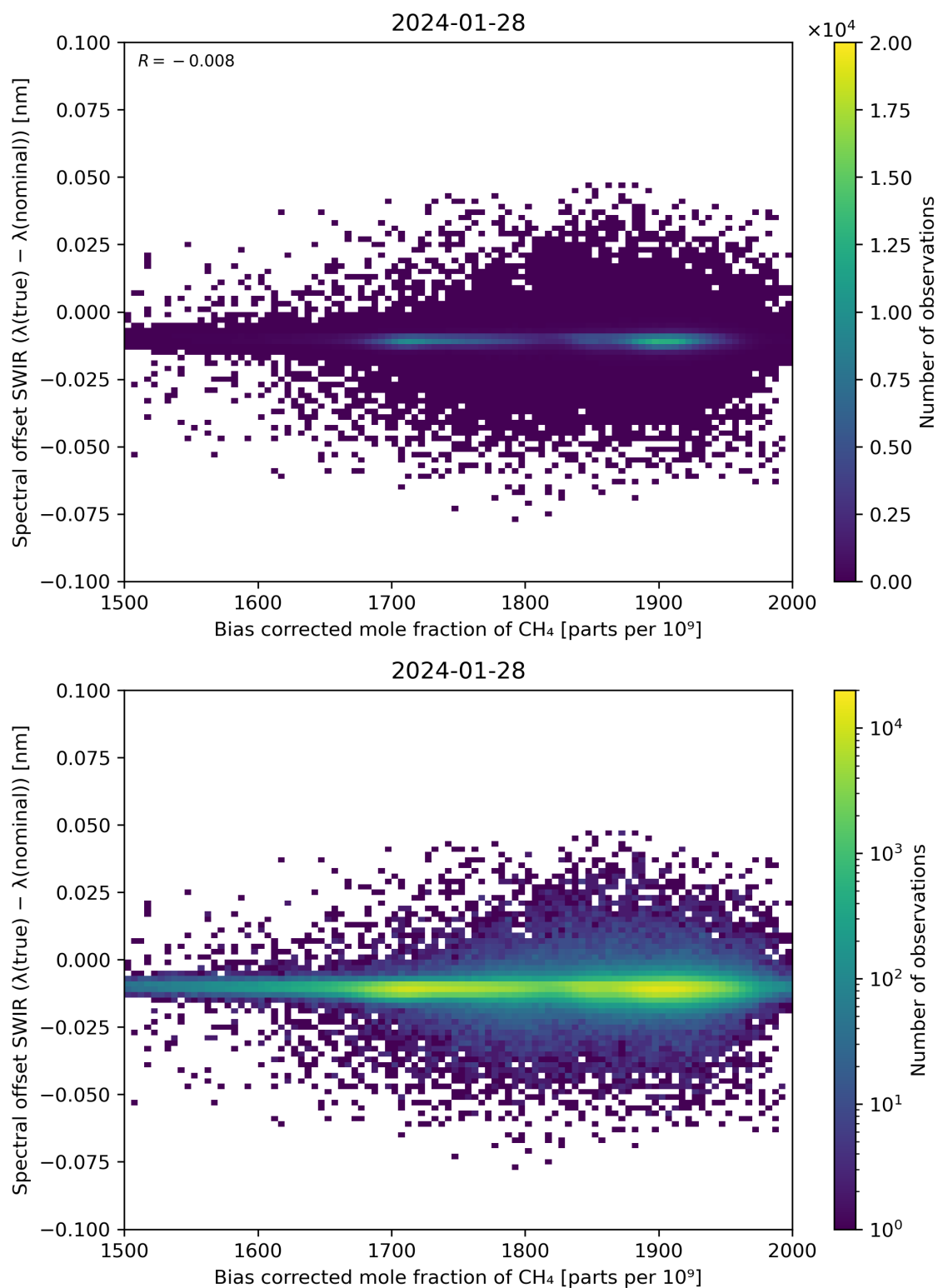
Figure 69: Scatter density plot of “Bias corrected mole fraction of \text{CH}_4 ” against “Spectral offset SWIR ( \lambda(\text{true}) - \lambda(\text{nominal}) )” for 2024-01-27 to 2024-01-29.
