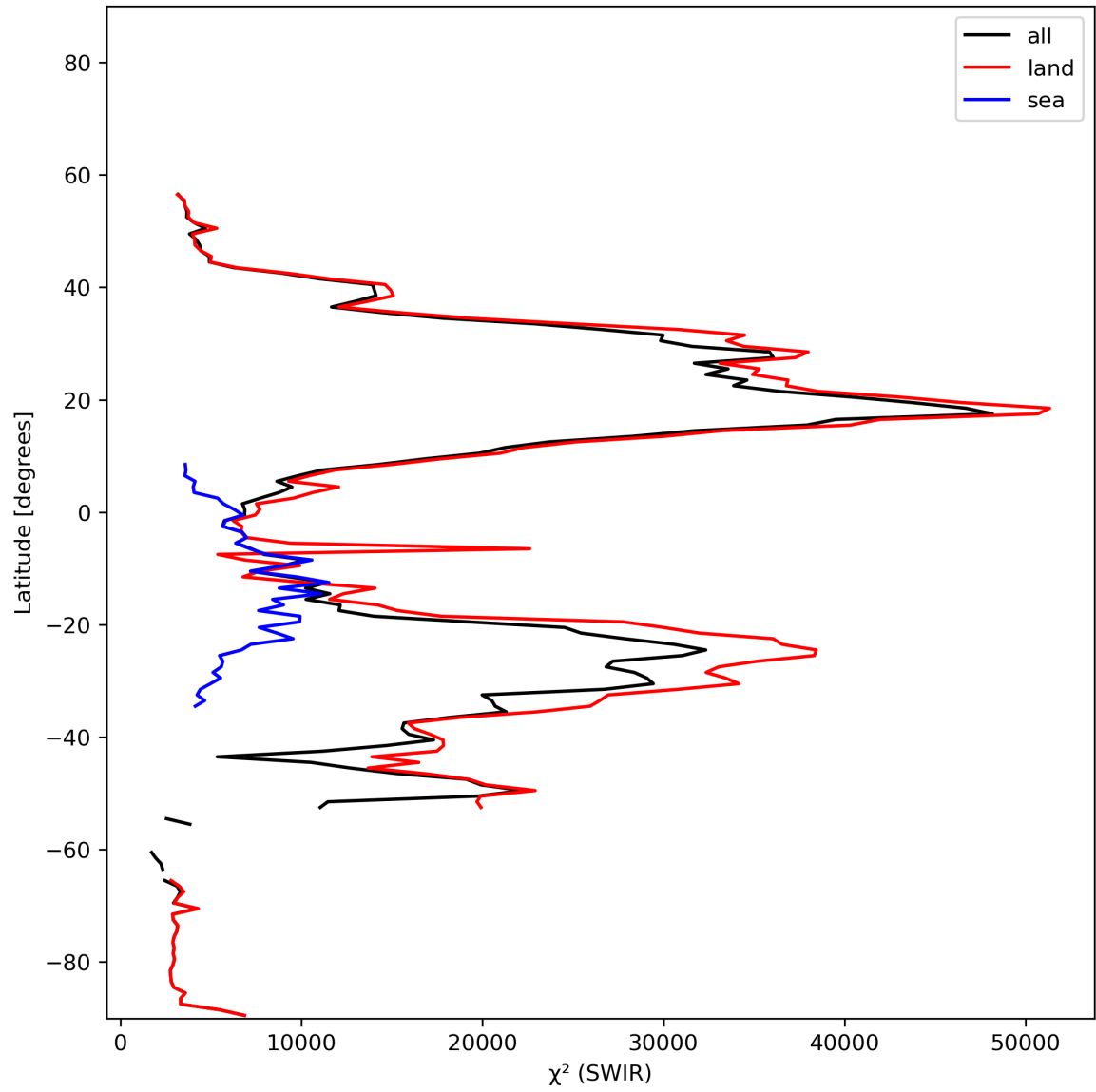
Figure 17: Zonal average of “ \chi^2 (SWIR)” for 2024-01-27 to 2024-01-29.
