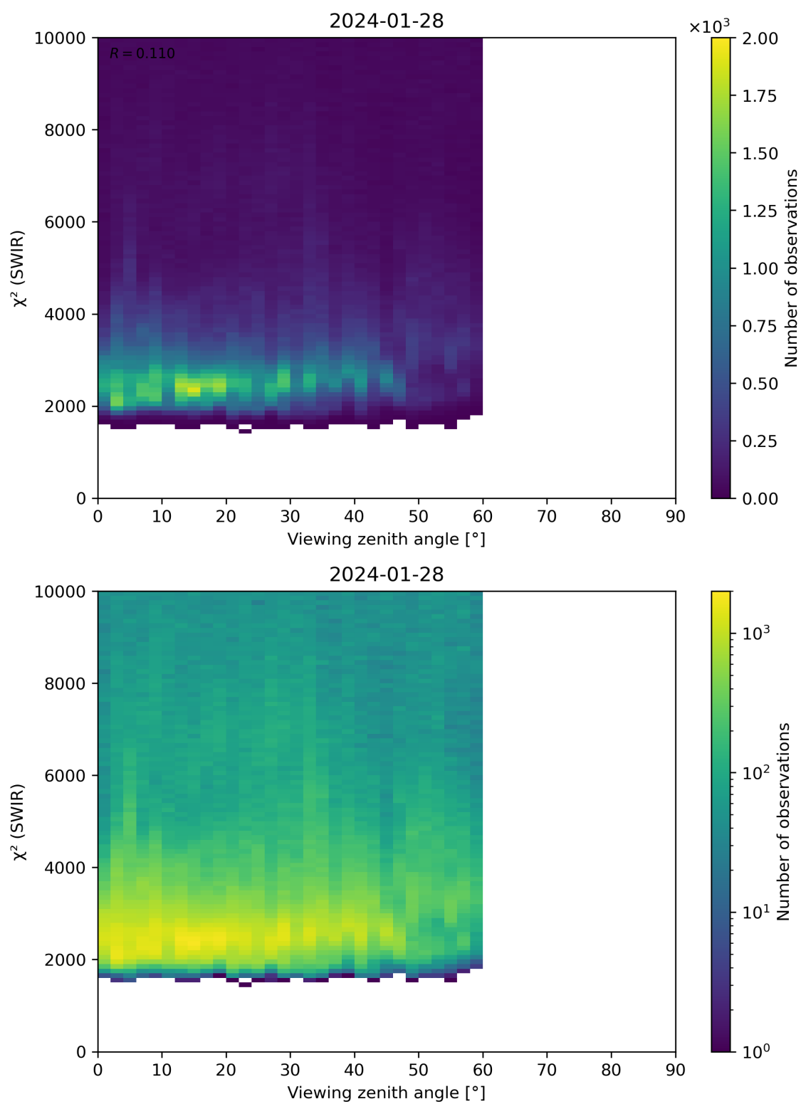
Figure 106: Scatter density plot of “Viewing zenith angle” against “ \chi^2 (SWIR)” for 2024-01-27 to 2024-01-29.
