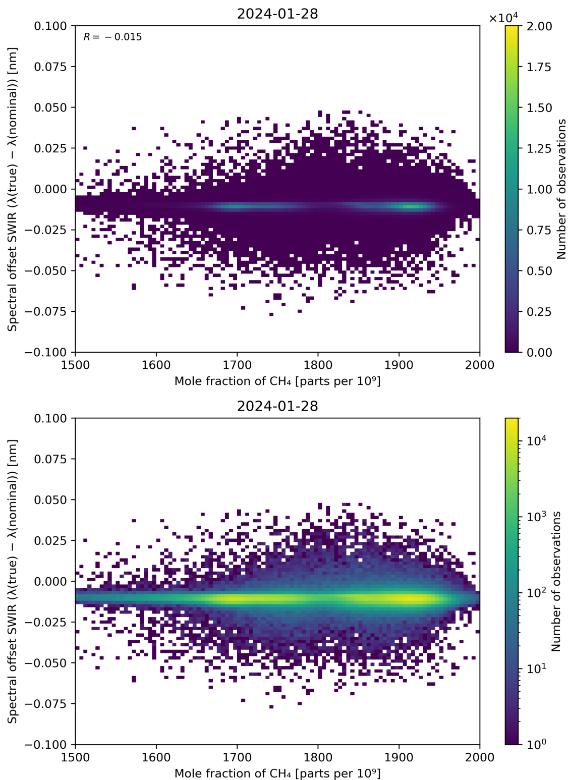
Figure 86: Scatter density plot of “Mole fraction of CH 4 ” against “Spectral offset SWIR ( \lambda(\text{true}) - \lambda(\text{nominal}) )” for 2024-01-27 to 2024-01-29.
