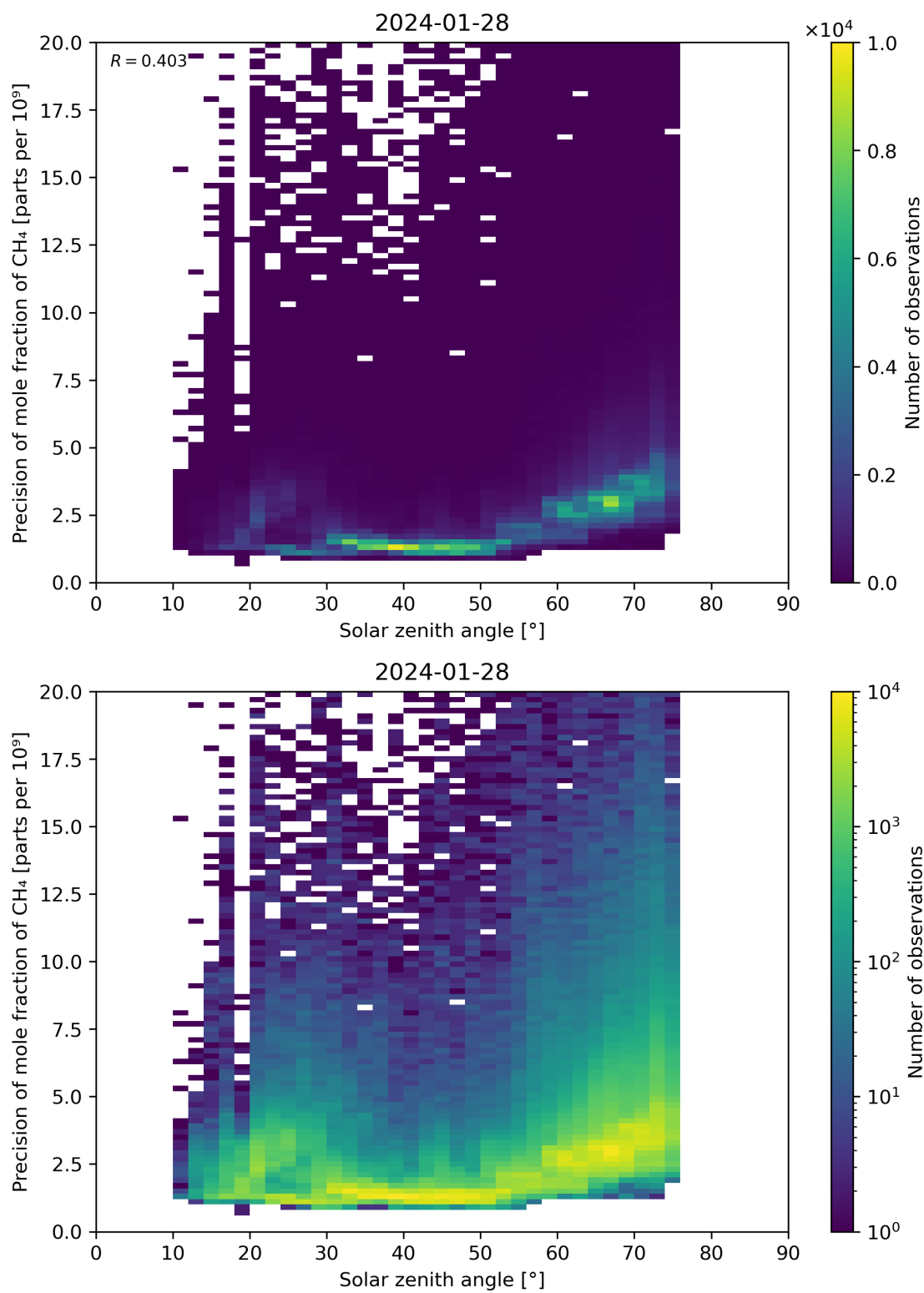
Figure 101: Scatter density plot of “Solar zenith angle” against “Precision of mole fraction of CH 4 ” for 2024-01-27 to 2024-01-29.
