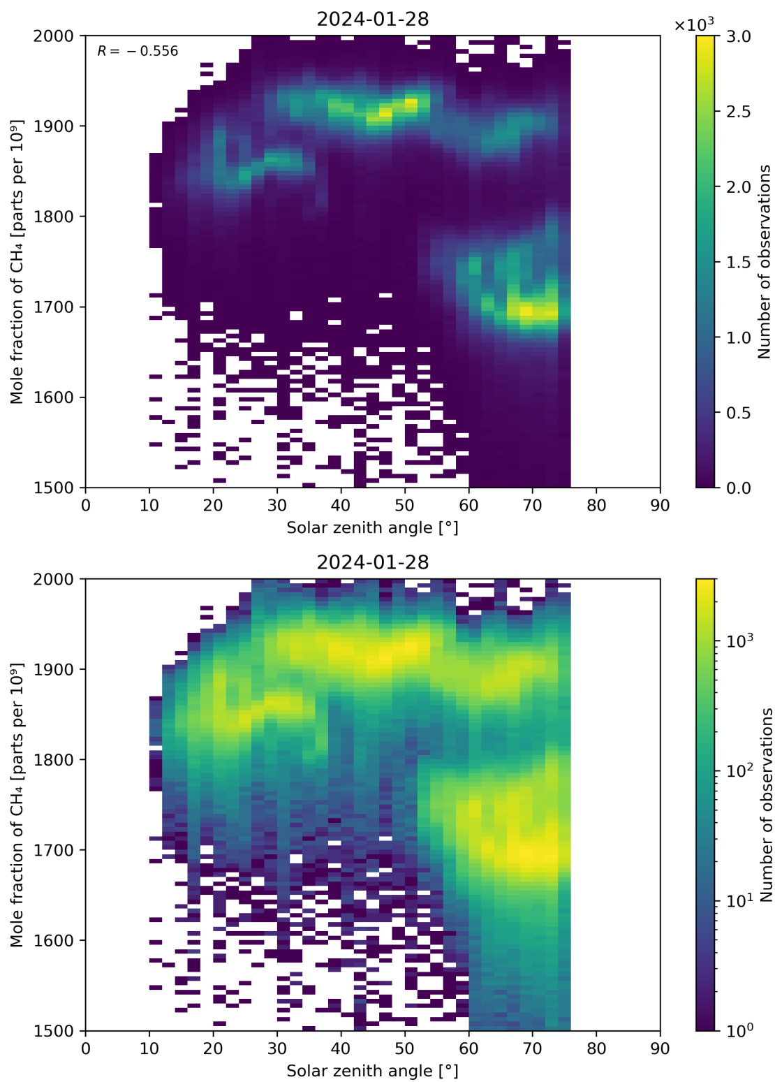
Figure 99: Scatter density plot of “Solar zenith angle” against “Mole fraction of \text{CH}_4 ” for 2024-01-27 to 2024-01-29.
