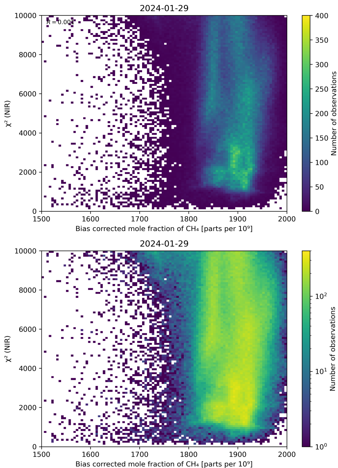
Figure 63: Scatter density plot of “Bias corrected mole fraction of CH 4 ” against “ \chi^2 (NIR)” for 2024-01-28 to 2024-01-30.
