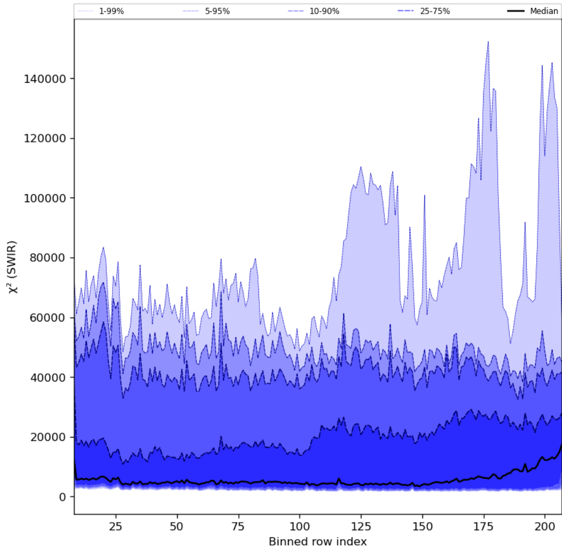
Figure 39: Along track statistics of “ \chi^2 (SWIR)” for 2024-01-28 to 2024-01-30
