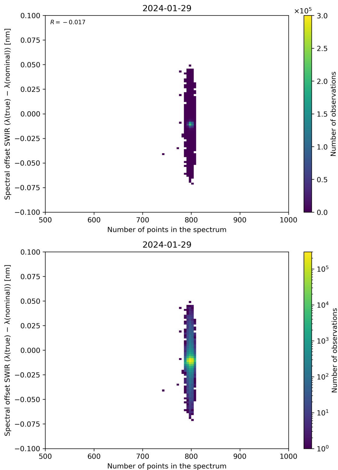
Figure 93: Scatter density plot of “Number of points in the spectrum” against “Spectral offset SWIR ( \lambda(\text{true}) - \lambda(\text{nominal}) )” for 2024-01-28 to 2024-01-30.
