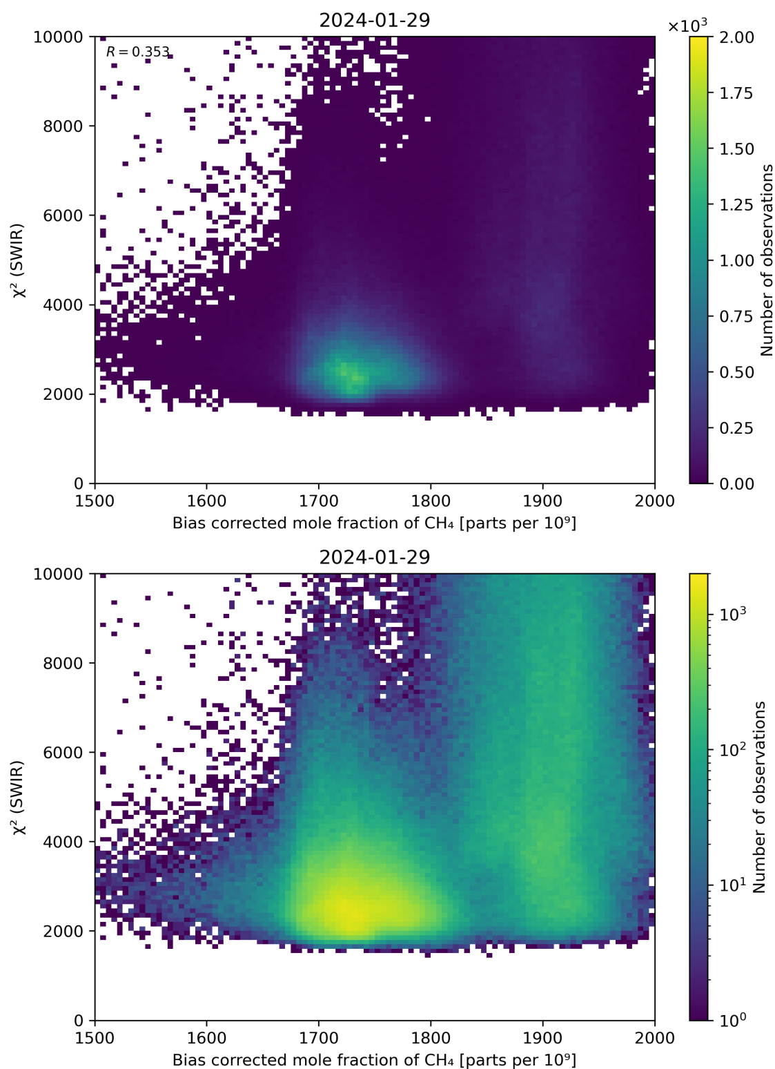
Figure 64: Scatter density plot of “Bias corrected mole fraction of \text{CH}_4 ” against “ \chi^2 (SWIR)” for 2024-01-28 to 2024-01-30.
