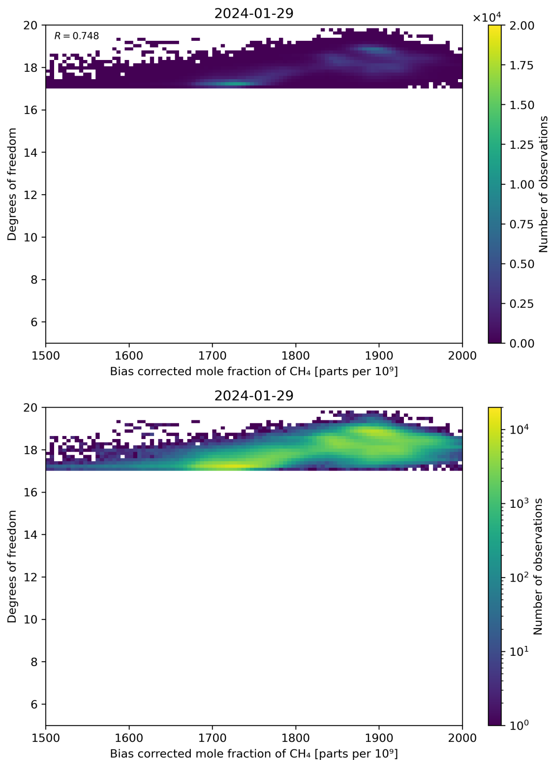
Figure 65: Scatter density plot of “Bias corrected mole fraction of CH 4 ” against “Degrees of freedom” for 2024-01-28 to 2024-01-30.
