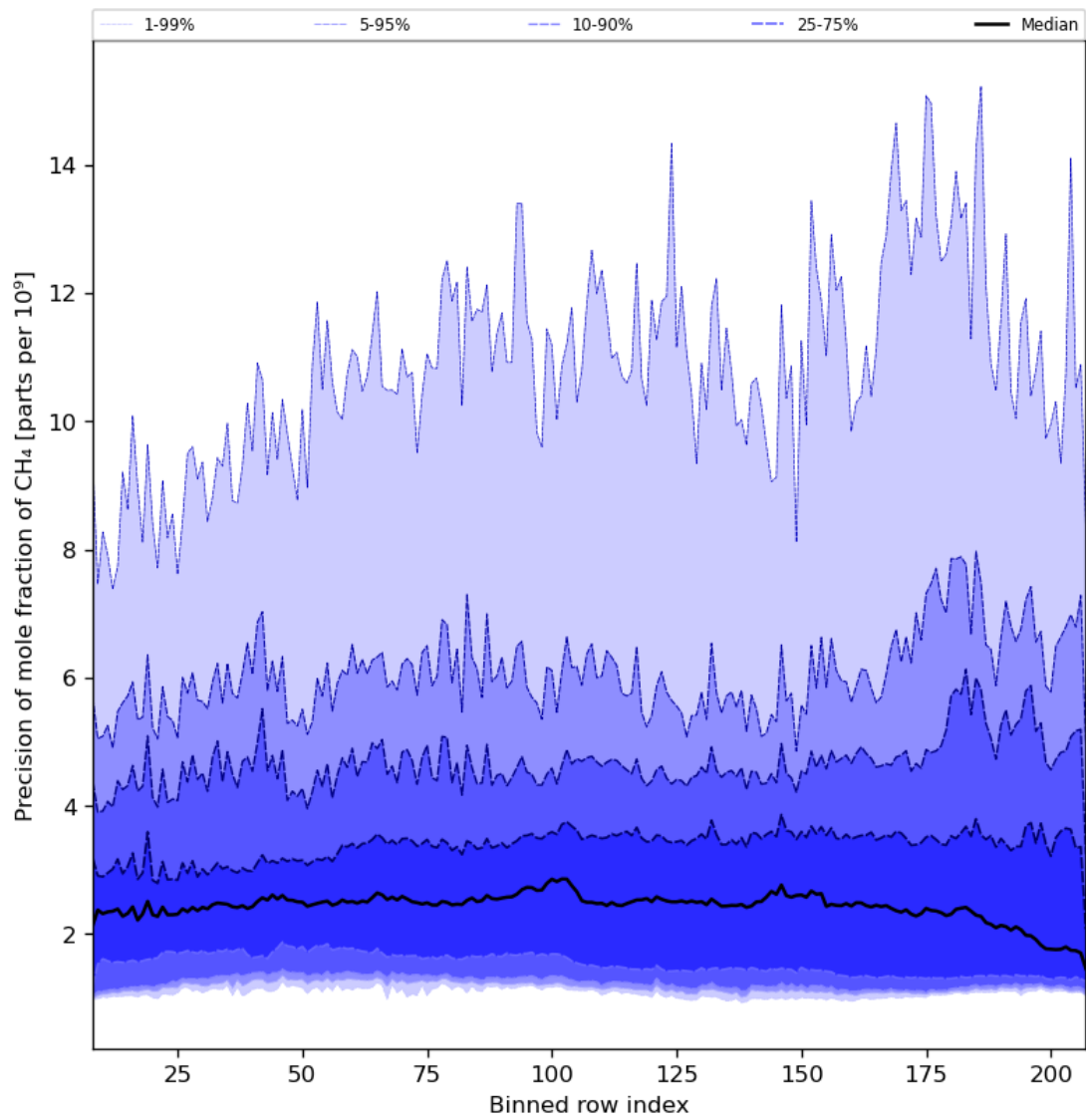
Figure 35: Along track statistics of “Precision of mole fraction of CH 4 ” for 2024-01-28 to 2024-01-30
