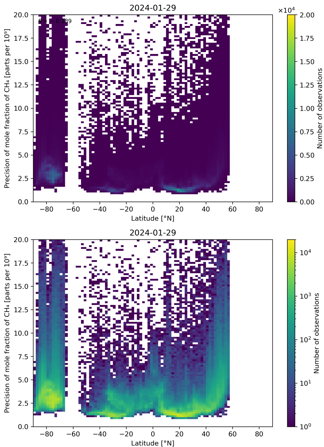
Figure 59: Scatter density plot of “Latitude” against “Precision of mole fraction of CH 4 ” for 2024-01-28 to 2024-01-30.
