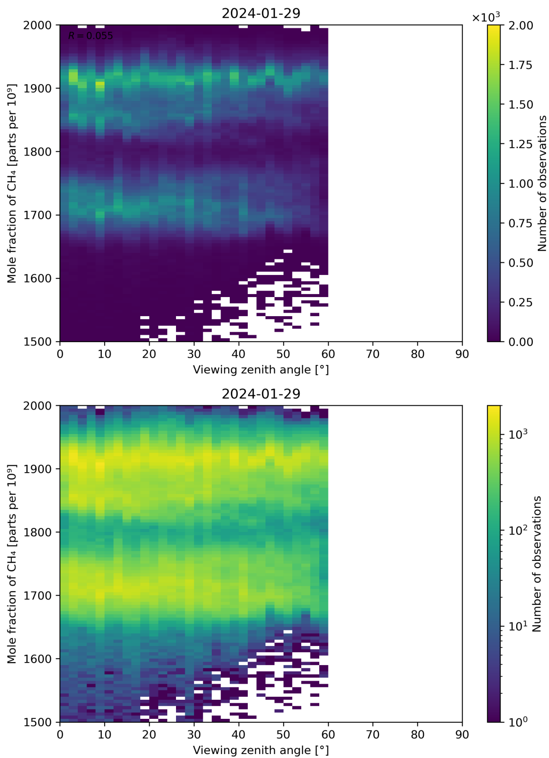
Figure 110: Scatter density plot of “Viewing zenith angle” against “Mole fraction of \text{CH}_4 ” for 2024-01-28 to 2024-01-30.
