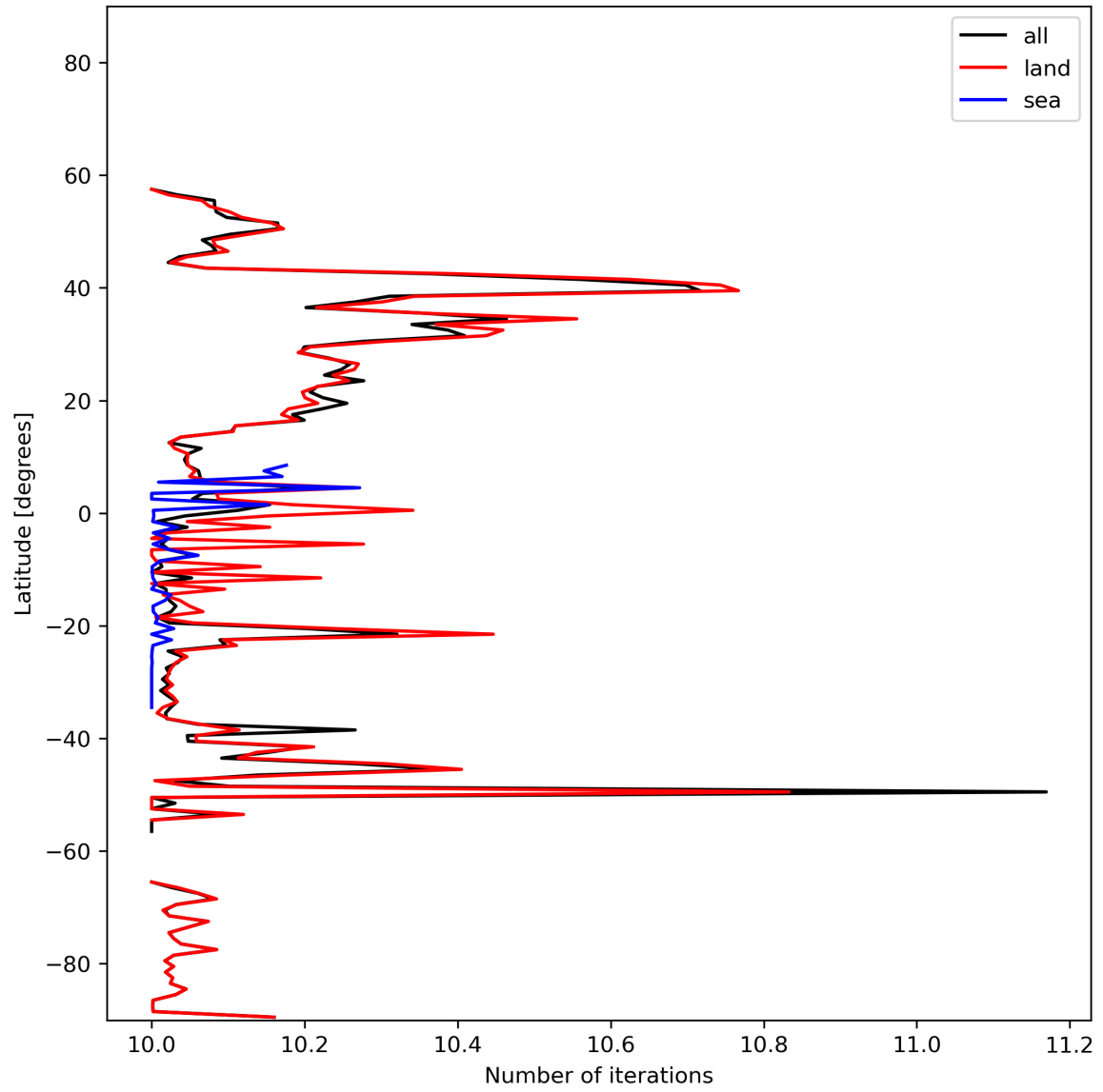
Figure 20: Zonal average of “Number of iterations” for 2024-01-28 to 2024-01-30.
