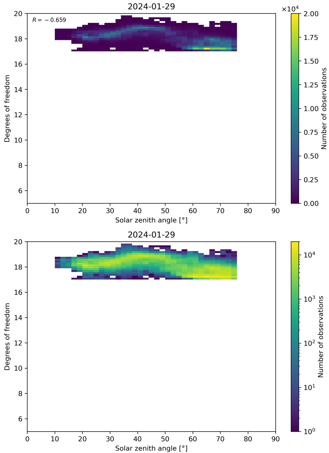
Figure 96: Scatter density plot of “Solar zenith angle” against “Degrees of freedom” for 2024-01-28 to 2024-01-30.
