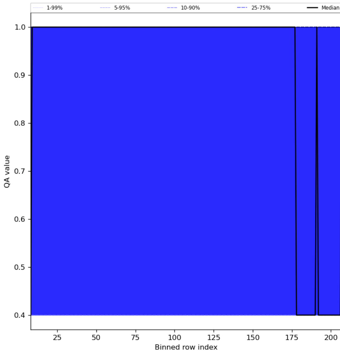
Figure 33: Along track statistics of “QA value” for 2024-01-28 to 2024-01-30
