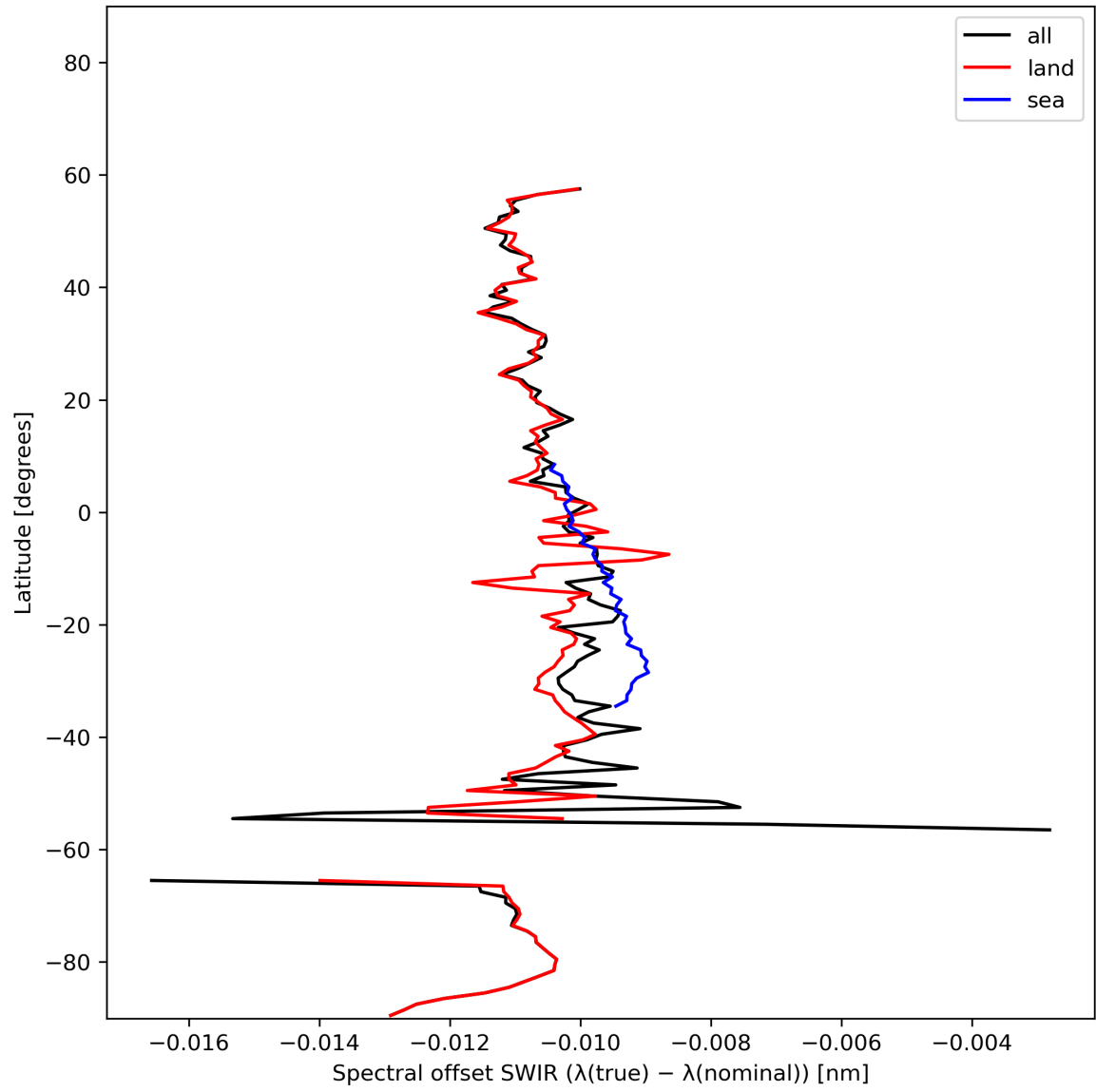
Figure 16: Zonal average of “Spectral offset SWIR ( \lambda(\text{true}) - \lambda(\text{nominal}) )” for 2024-01-28 to 2024-01-30.
