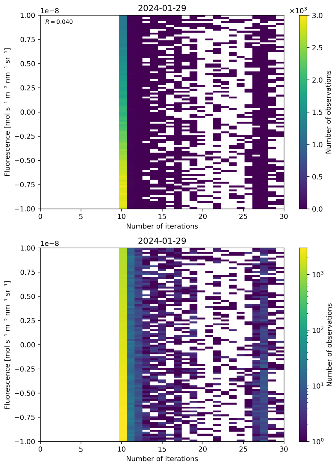
Figure 87: Scatter density plot of “Number of iterations” against “Fluorescence” for 2024-01-28 to 2024-01-30.
