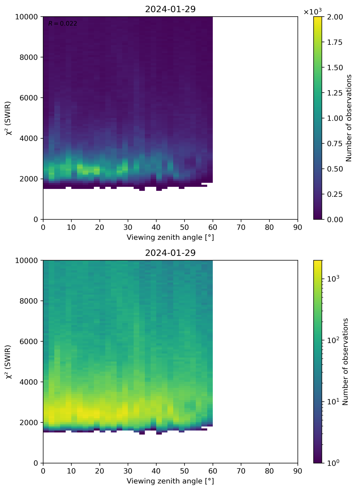
Figure 106: Scatter density plot of “Viewing zenith angle” against “ \chi^2 (SWIR)” for 2024-01-28 to 2024-01-30.
