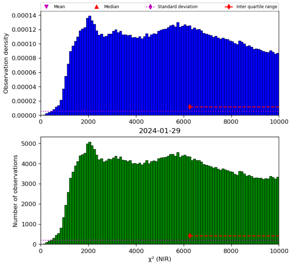
Figure 29: Histogram of “ \chi^2 (NIR)” for 2024-01-28 to 2024-01-30
