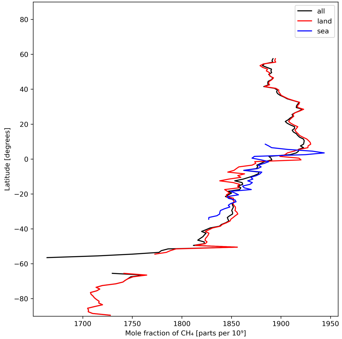
Figure 12: Zonal average of “Mole fraction of CH 4 ” for 2024-01-28 to 2024-01-30.
