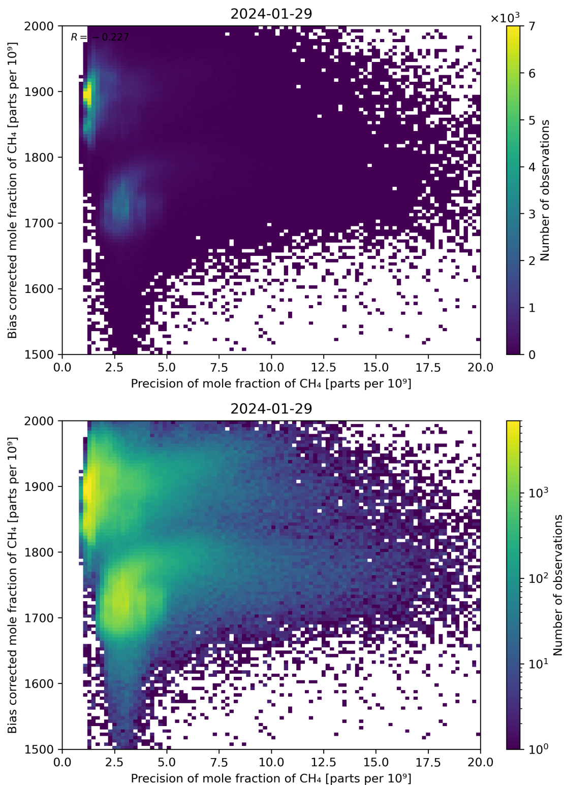
Figure 82: Scatter density plot of “Precision of mole fraction of CH 4 ” against “Bias corrected mole fraction of CH 4 ” for 2024-01-28 to 2024-01-30.
