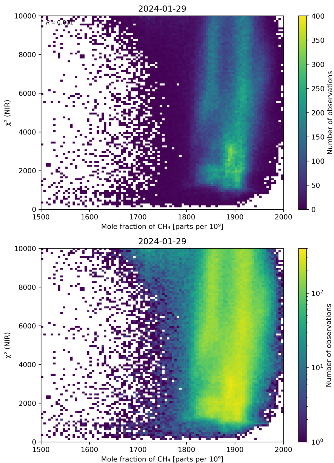
Figure 70: Scatter density plot of “Mole fraction of CH 4 ” against “ \chi^2 (NIR)” for 2024-01-28 to 2024-01-30.
