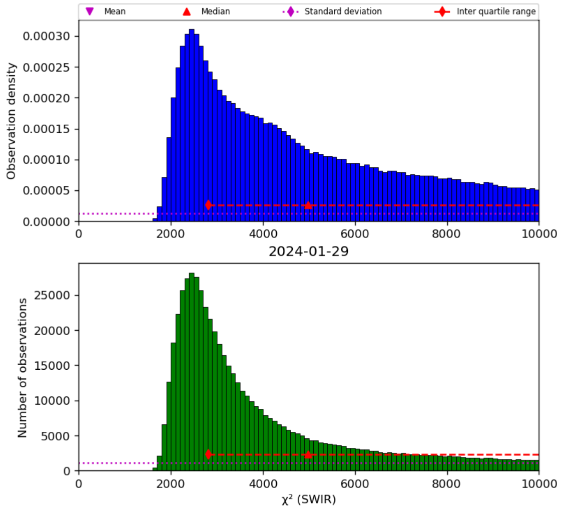
Figure 28: Histogram of “ \chi^2 (SWIR)” for 2024-01-28 to 2024-01-30
