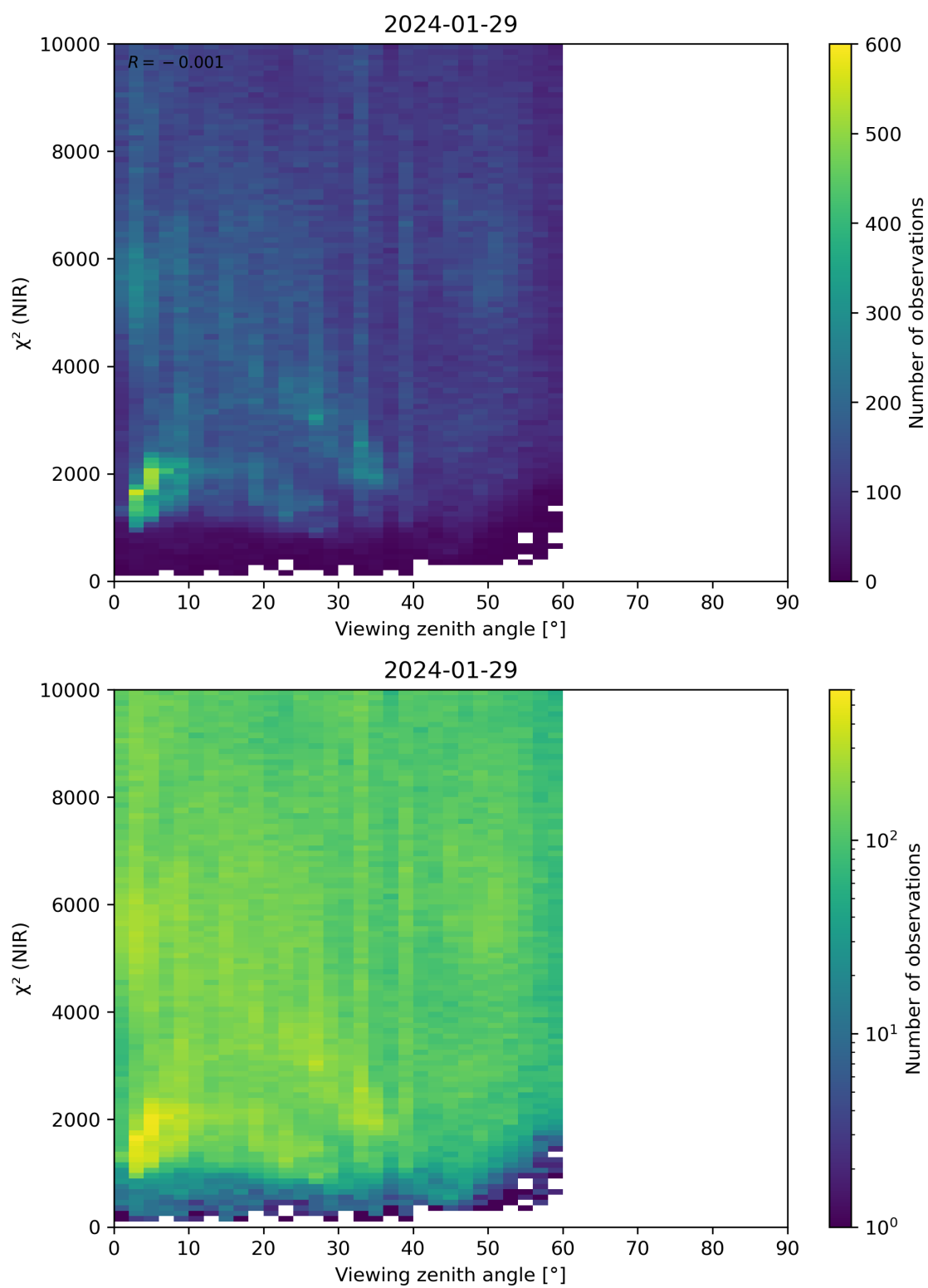
Figure 105: Scatter density plot of “Viewing zenith angle” against “ \chi^2 (NIR)” for 2024-01-28 to 2024-01-30.
