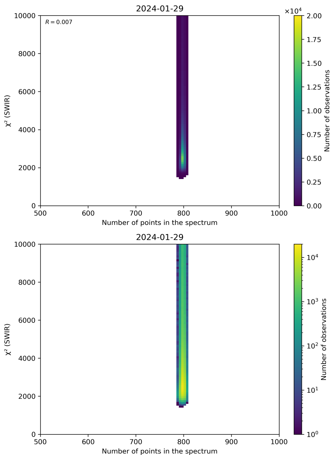
Figure 89: Scatter density plot of “Number of points in the spectrum” against “ \chi^2 (SWIR)” for 2024-01-28 to 2024-01-30.
