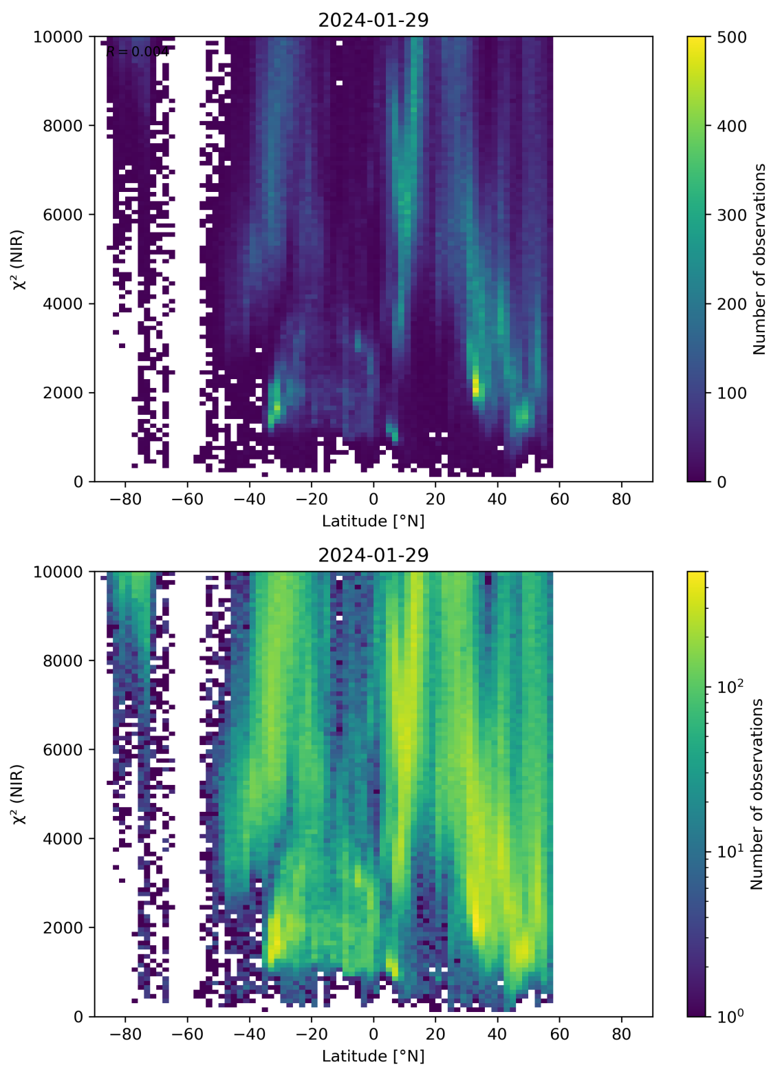
Figure 53: Scatter density plot of “Latitude” against “ \chi^2 (NIR)” for 2024-01-28 to 2024-01-30.
