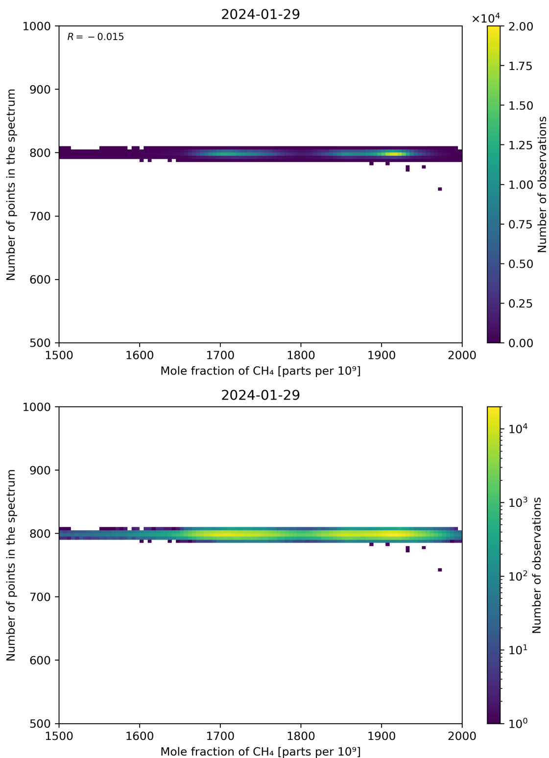
Figure 77: Scatter density plot of “Mole fraction of CH 4 ” against “Number of points in the spectrum” for 2024-01-28 to 2024-01-30.
