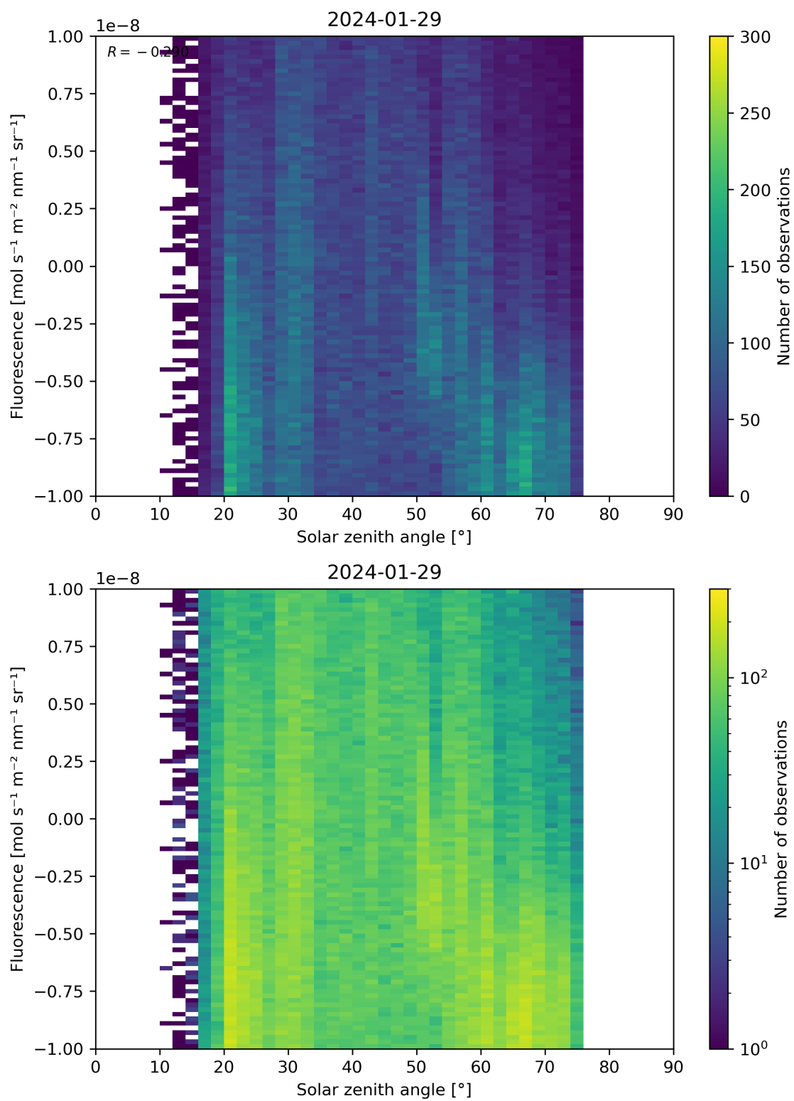
Figure 97: Scatter density plot of “Solar zenith angle” against “Fluorescence” for 2024-01-28 to 2024-01-30.
