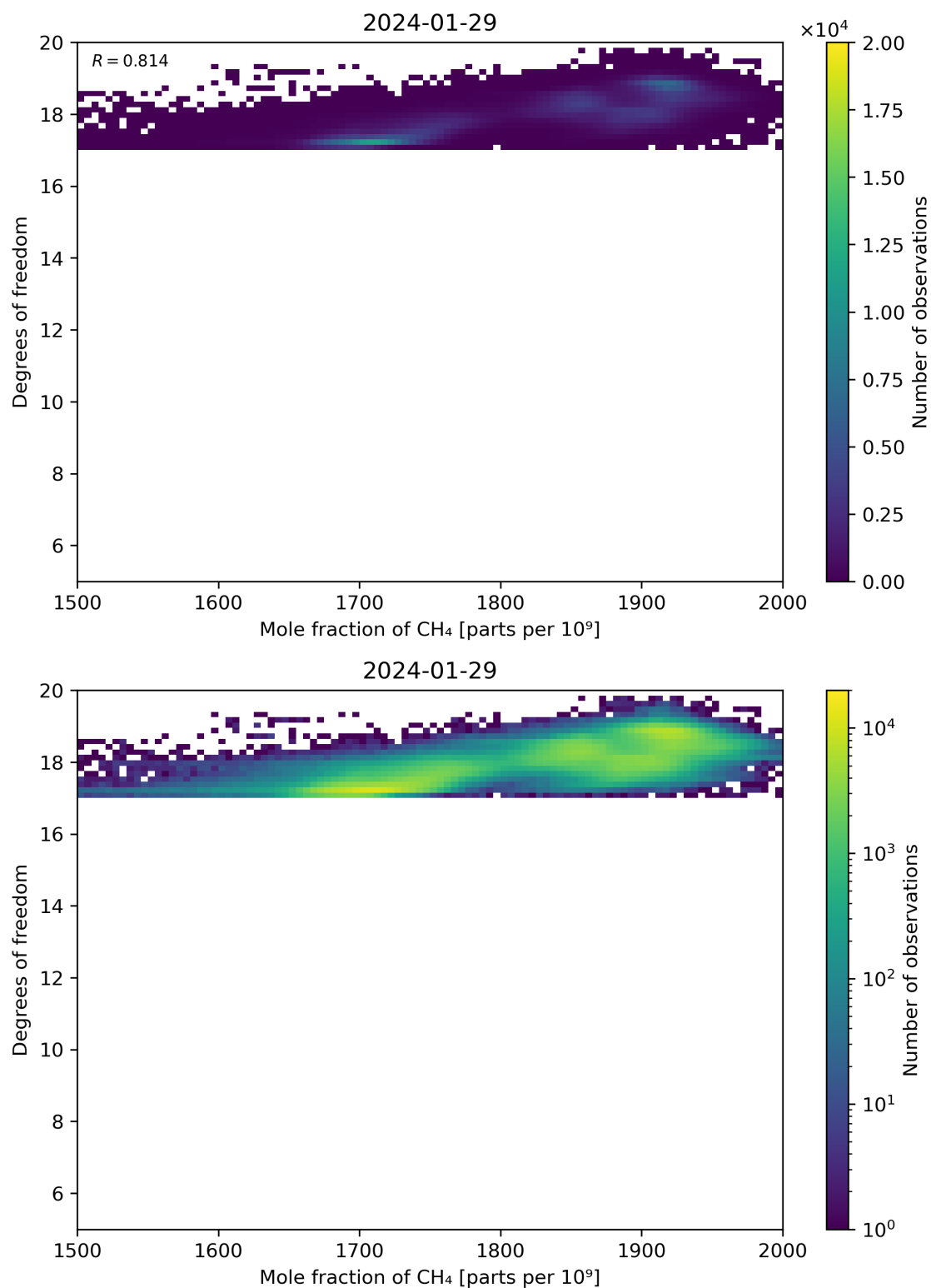
Figure 72: Scatter density plot of “Mole fraction of CH 4 ” against “Degrees of freedom” for 2024-01-28 to 2024-01-30.
