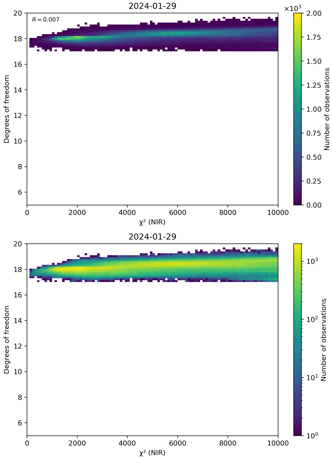
Figure 44: Scatter density plot of “ \chi^2 (NIR)” against “Degrees of freedom” for 2024-01-28 to 2024-01-30.
