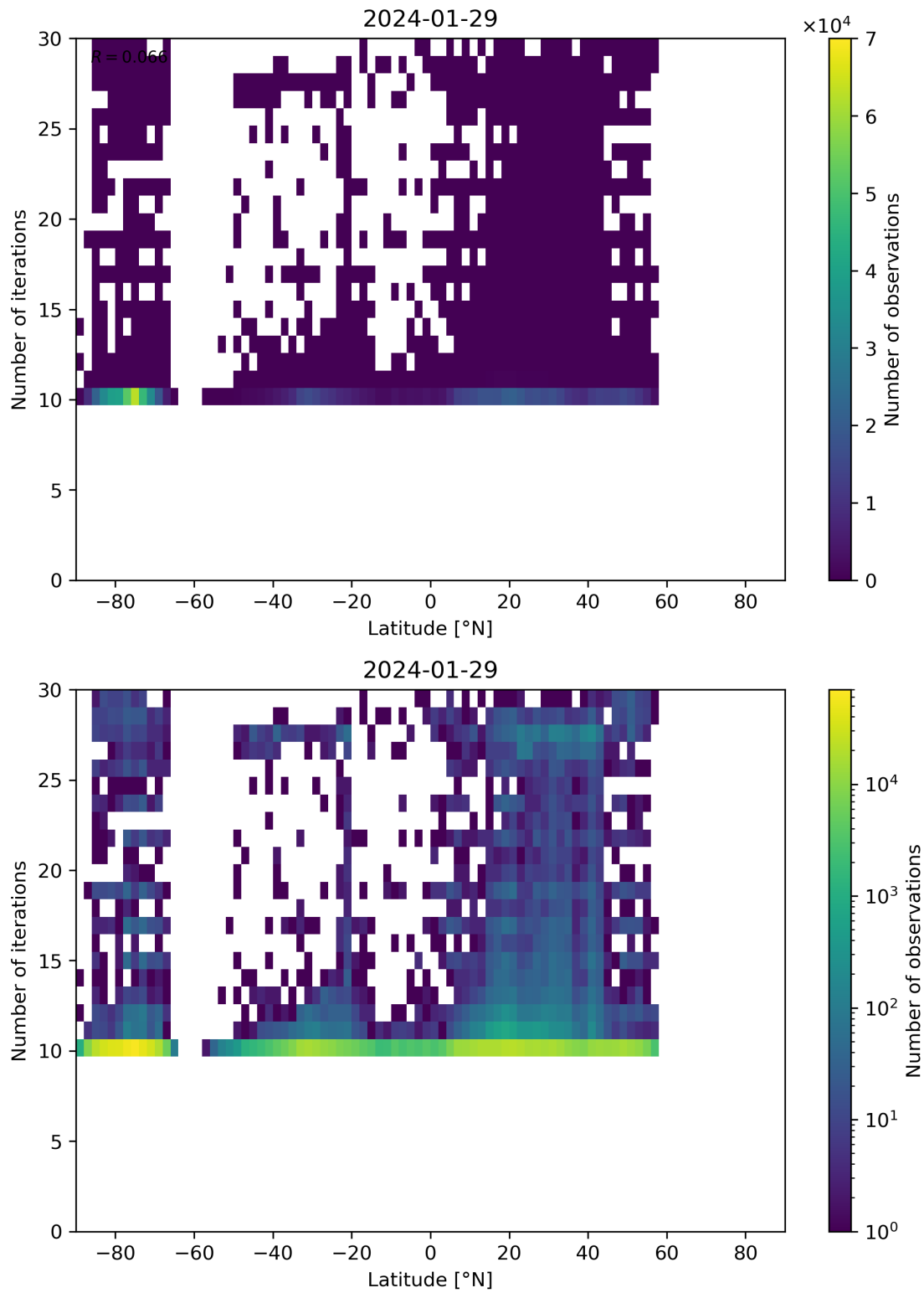
Figure 60: Scatter density plot of “Latitude” against “Number of iterations” for 2024-01-28 to 2024-01-30.
