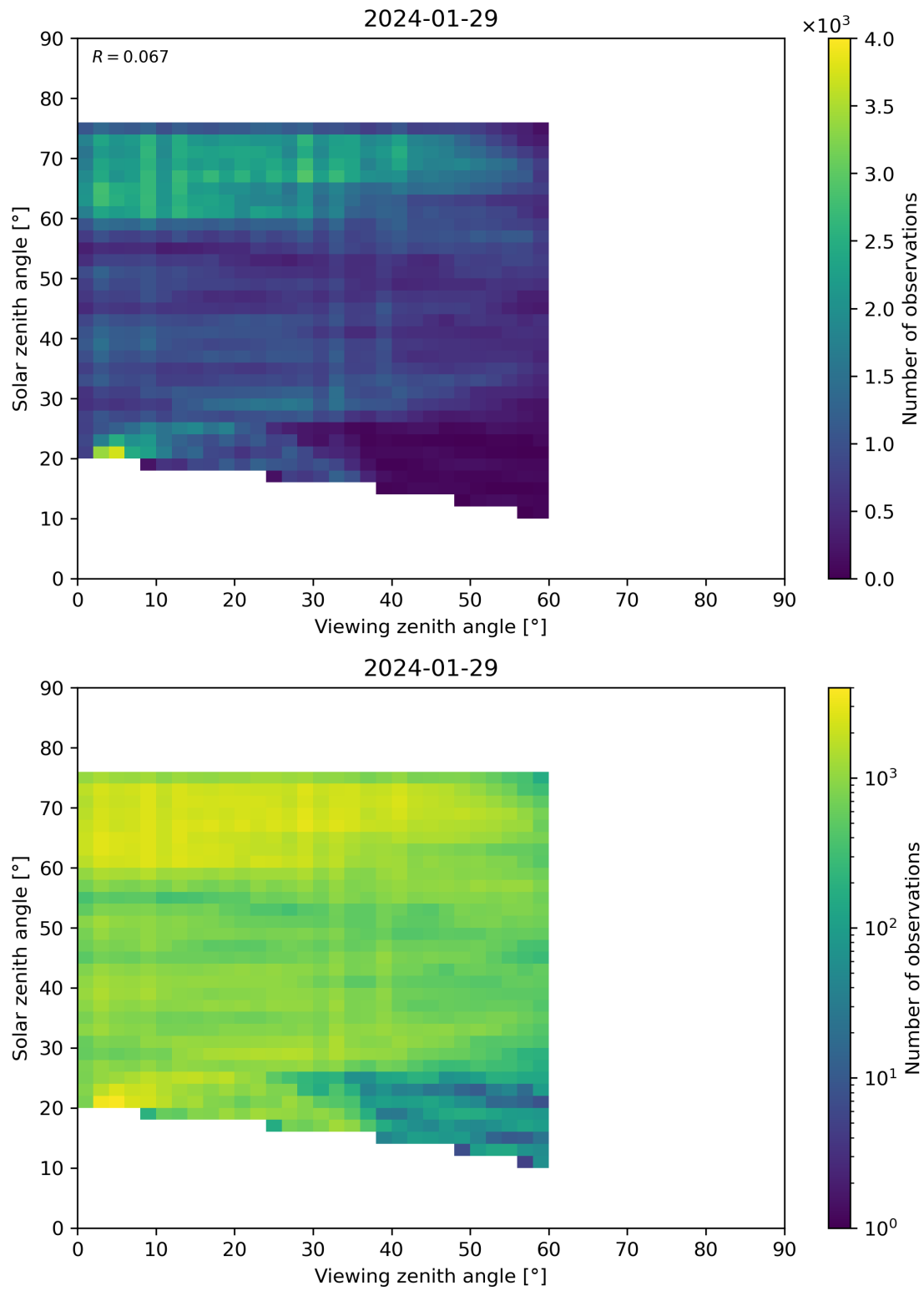
Figure 115: Scatter density plot of “Viewing zenith angle” against “Solar zenith angle” for 2024-01-28 to 2024-01-30.
