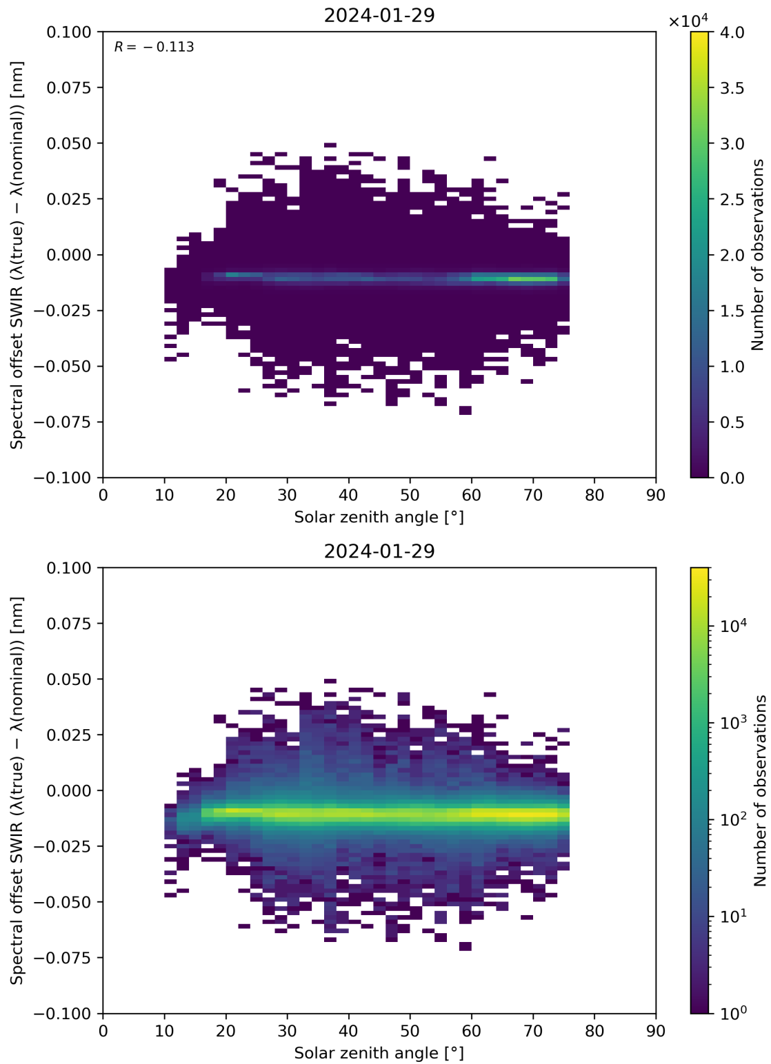
Figure 104: Scatter density plot of “Solar zenith angle” against “Spectral offset SWIR ( \lambda(\text{true}) - \lambda(\text{nominal}) )” for 2024-01-28 to 2024-01-30.
