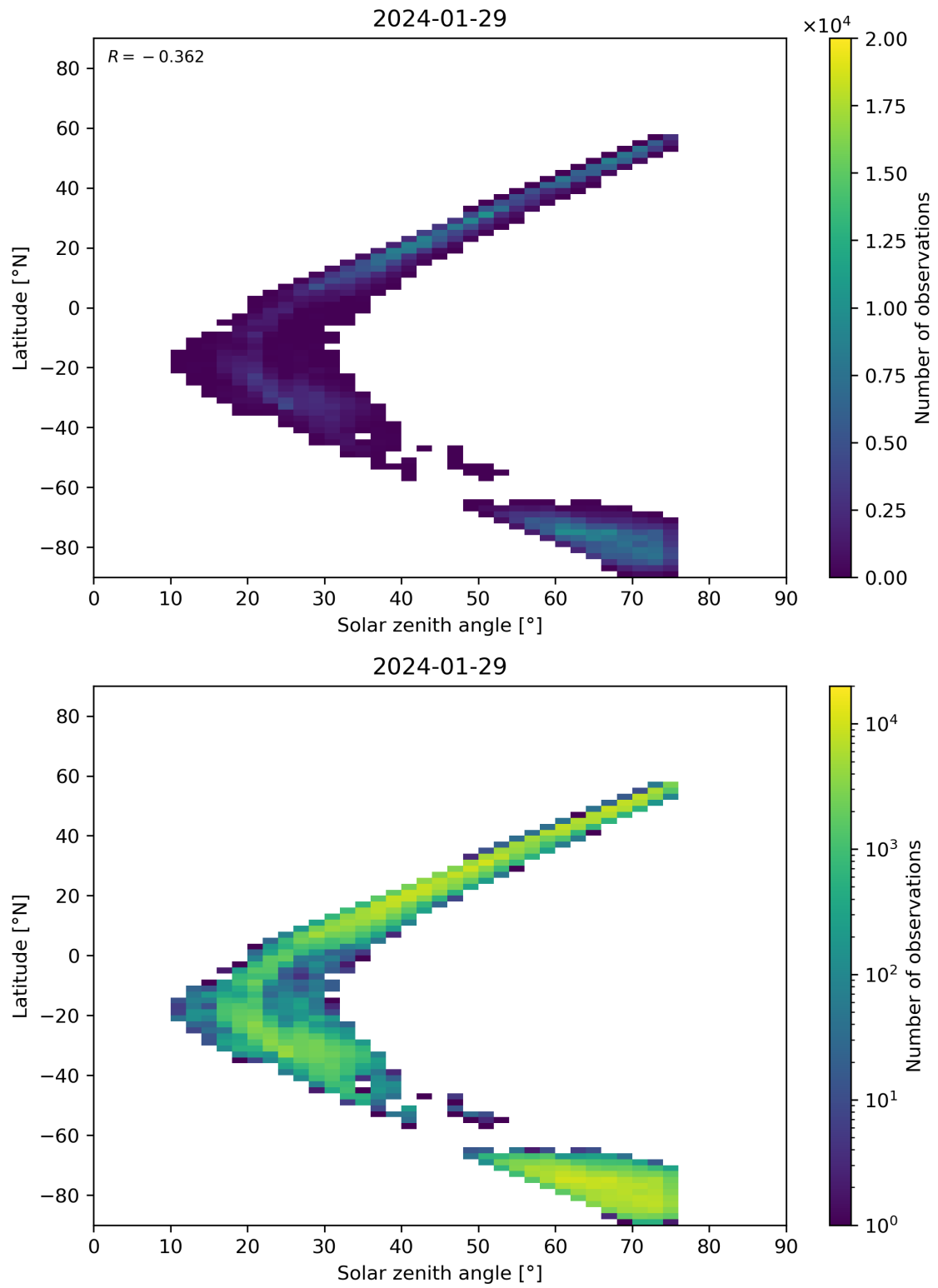
Figure 98: Scatter density plot of “Solar zenith angle” against “Latitude” for 2024-01-28 to 2024-01-30.
