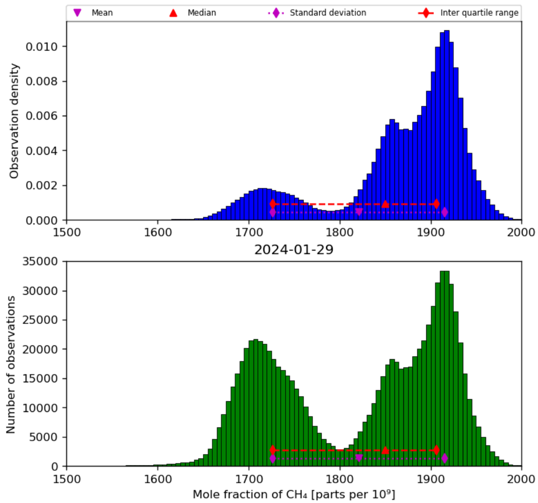
Figure 23: Histogram of “Mole fraction of CH 4 ” for 2024-01-28 to 2024-01-30
