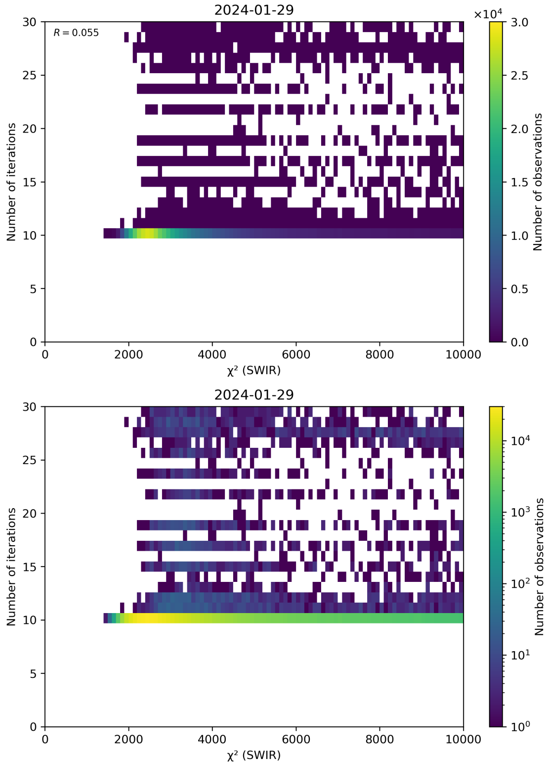
Figure 50: Scatter density plot of “ \chi^2 (SWIR)” against “Number of iterations” for 2024-01-28 to 2024-01-30.
