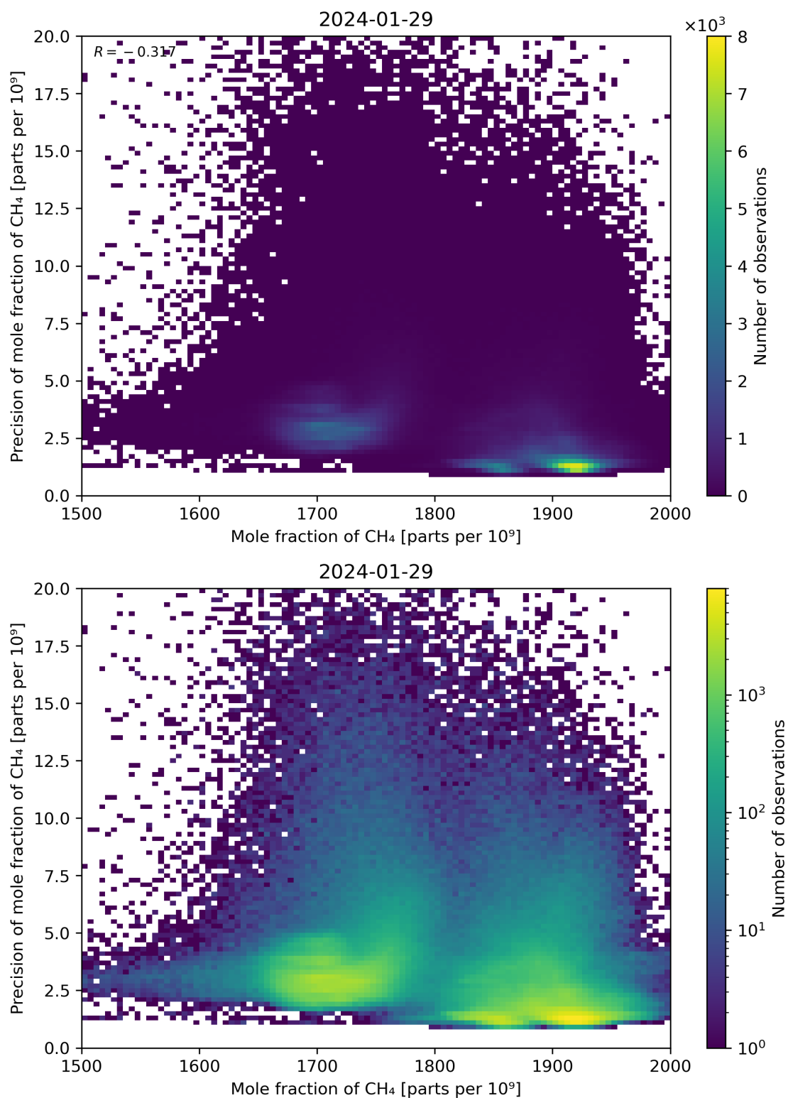
Figure 75: Scatter density plot of “Mole fraction of CH 4 ” against “Precision of mole fraction of CH 4 ” for 2024-01-28 to 2024-01-30.
