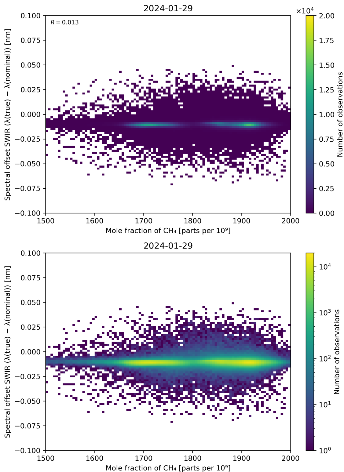
Figure 86: Scatter density plot of “Mole fraction of CH 4 ” against “Spectral offset SWIR ( \lambda(\text{true}) - \lambda(\text{nominal}) )” for 2024-01-28 to 2024-01-30.
