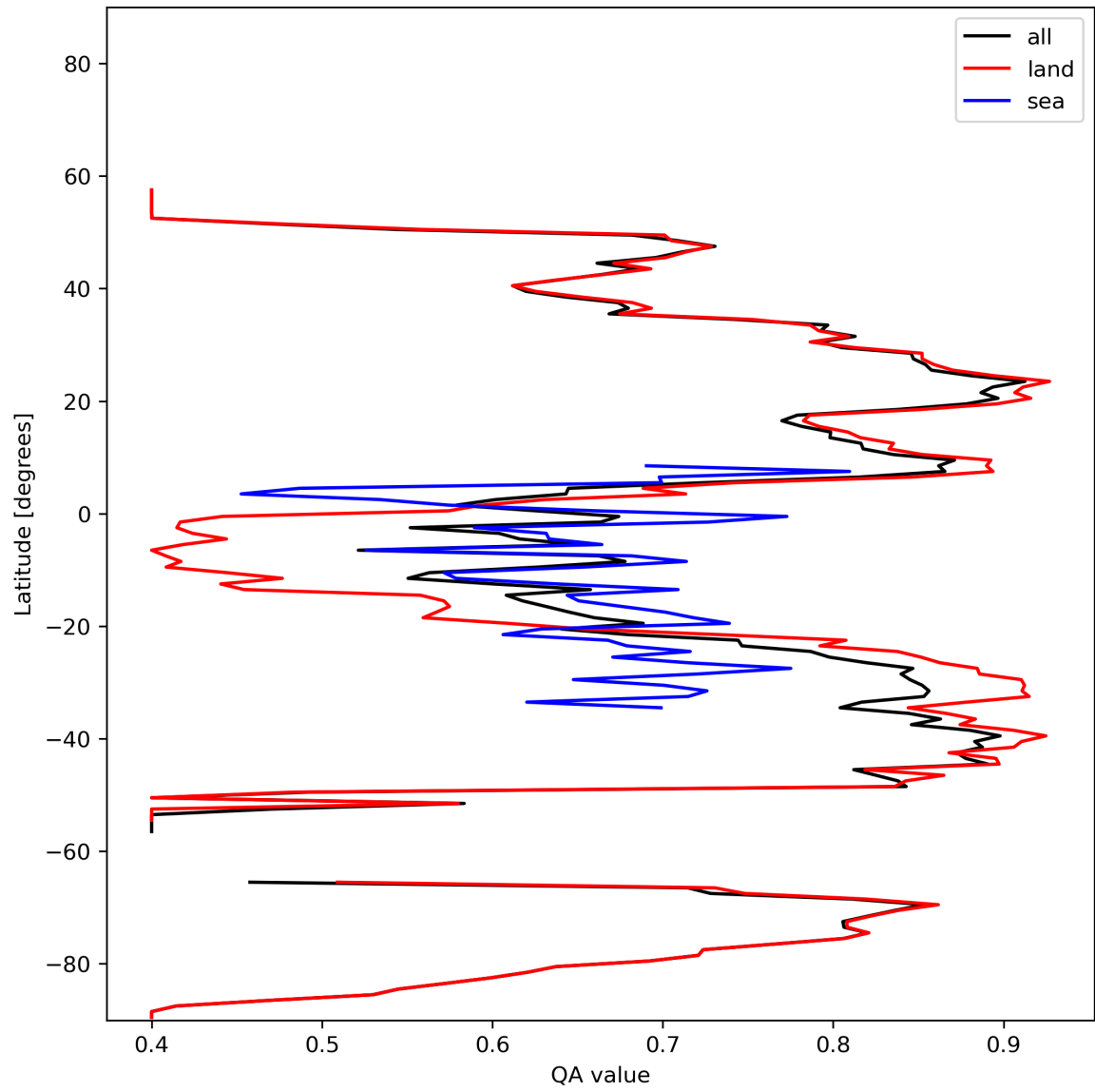
Figure 11: Zonal average of “QA value” for 2024-01-28 to 2024-01-30.
