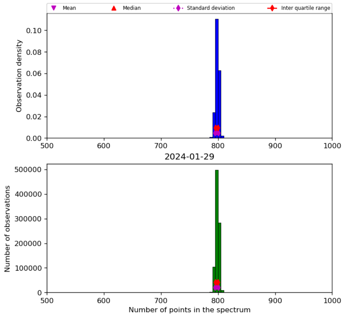
Figure 26: Histogram of “Number of points in the spectrum” for 2024-01-28 to 2024-01-30
