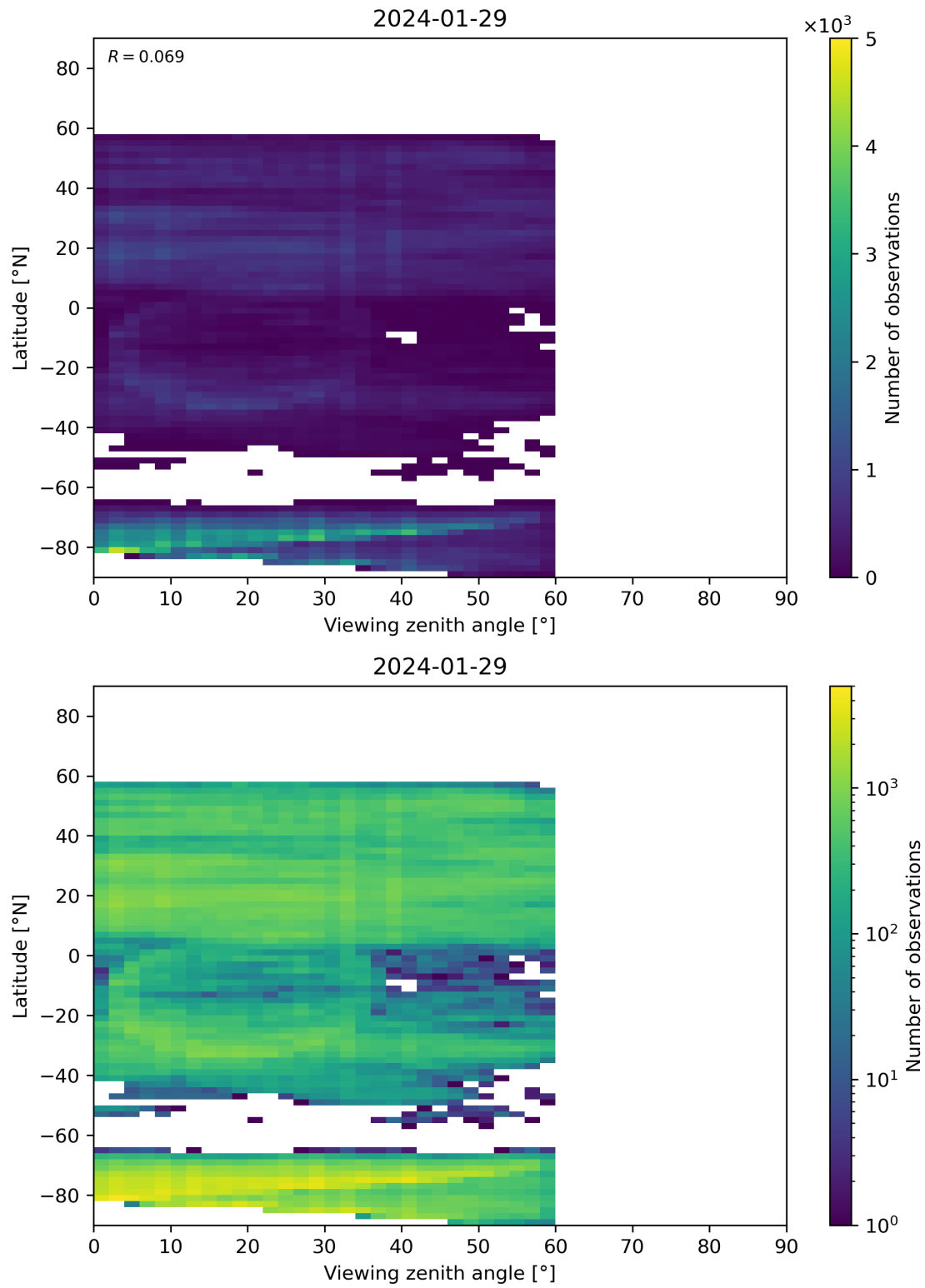
Figure 109: Scatter density plot of “Viewing zenith angle” against “Latitude” for 2024-01-28 to 2024-01-30.
