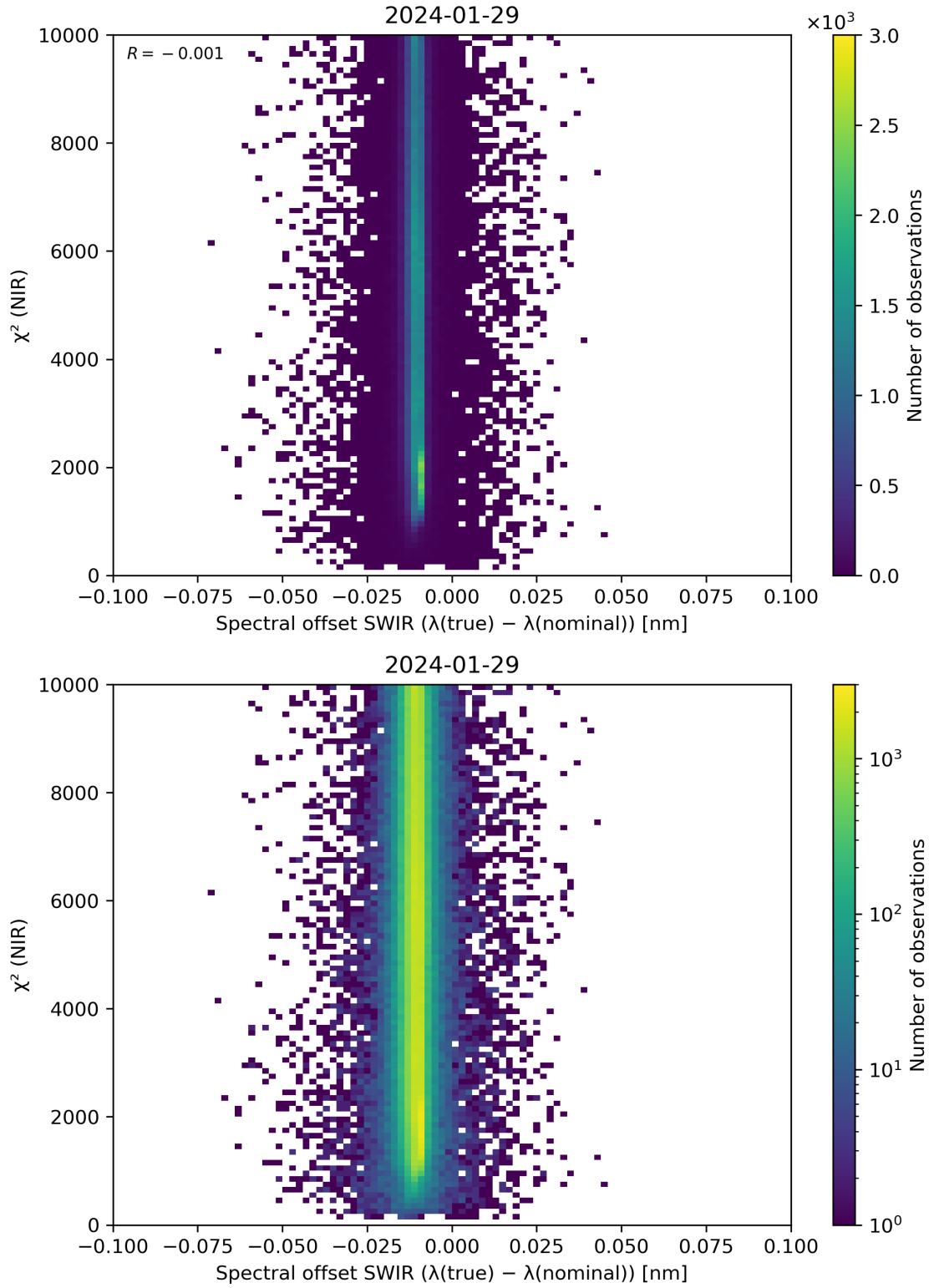
Figure 117: Scatter density plot of “Spectral offset SWIR ( \lambda(\text{true}) - \lambda(\text{nominal}) )” against “ \chi^2 (NIR)” for 2024-01-28 to 2024-01-30.
