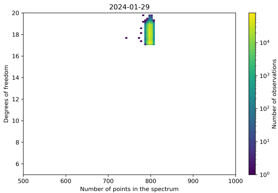
Figure 90: Scatter density plot of “Number of points in the spectrum” against “Degrees of freedom” for 2024-01-28 to 2024-01-30.
