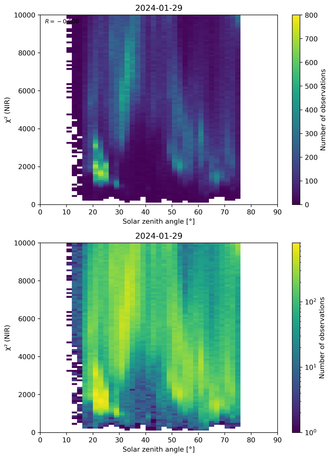
Figure 94: Scatter density plot of “Solar zenith angle” against “ \chi^2 (NIR)” for 2024-01-28 to 2024-01-30.
