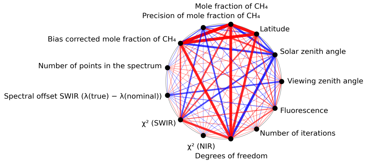
Figure 1: Map of correlation graph for 2024-01-28 to 2024-01-30.
