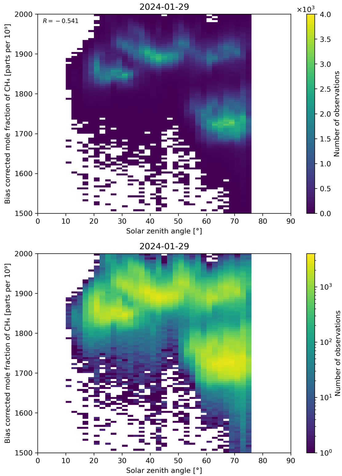
Figure 100: Scatter density plot of “Solar zenith angle” against “Bias corrected mole fraction of \text{CH}_4 ” for 2024-01-28 to 2024-01-30.
