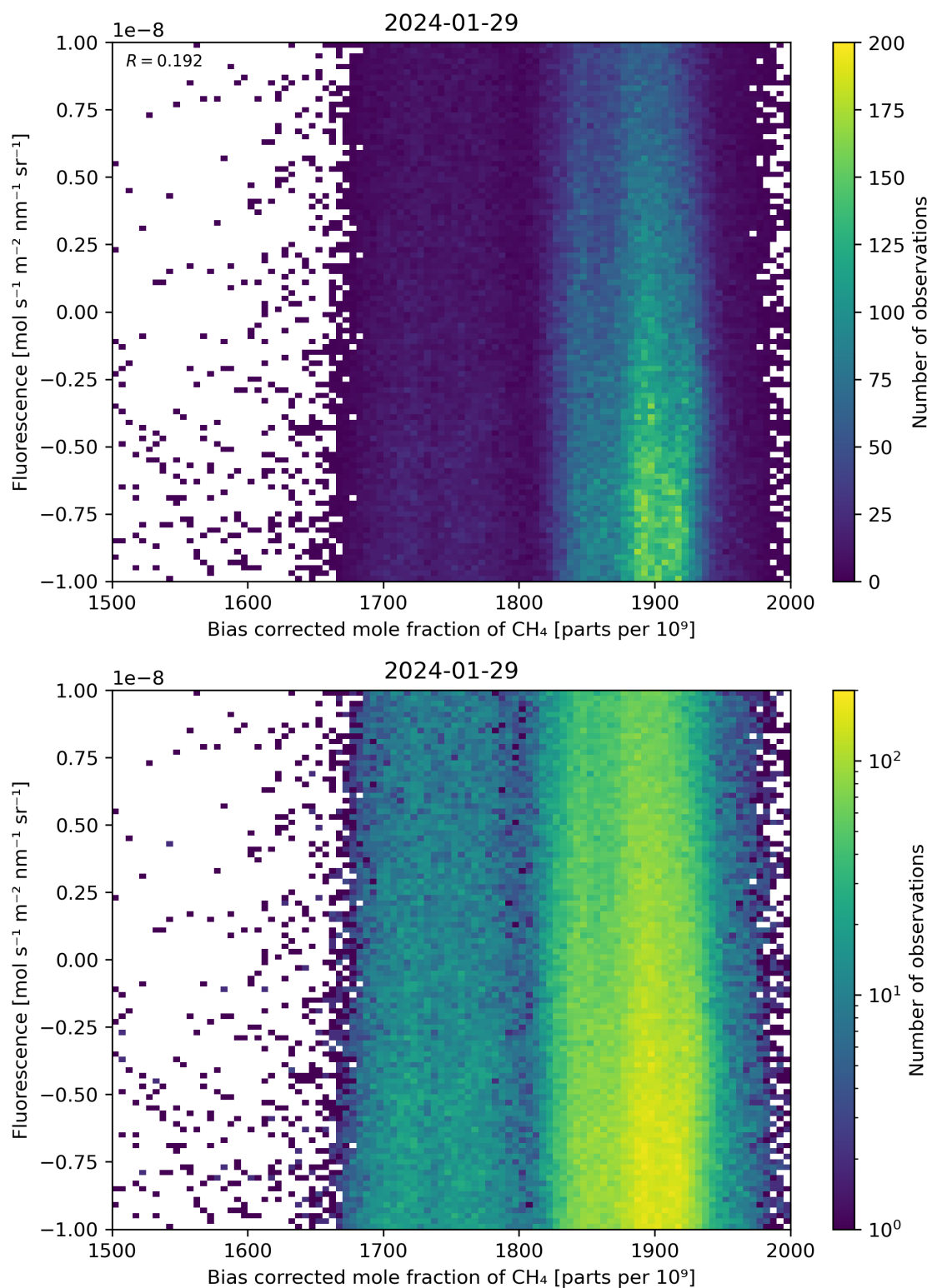
Figure 66: Scatter density plot of “Bias corrected mole fraction of \text{CH}_4 ” against “Fluorescence” for 2024-01-28 to 2024-01-30.
