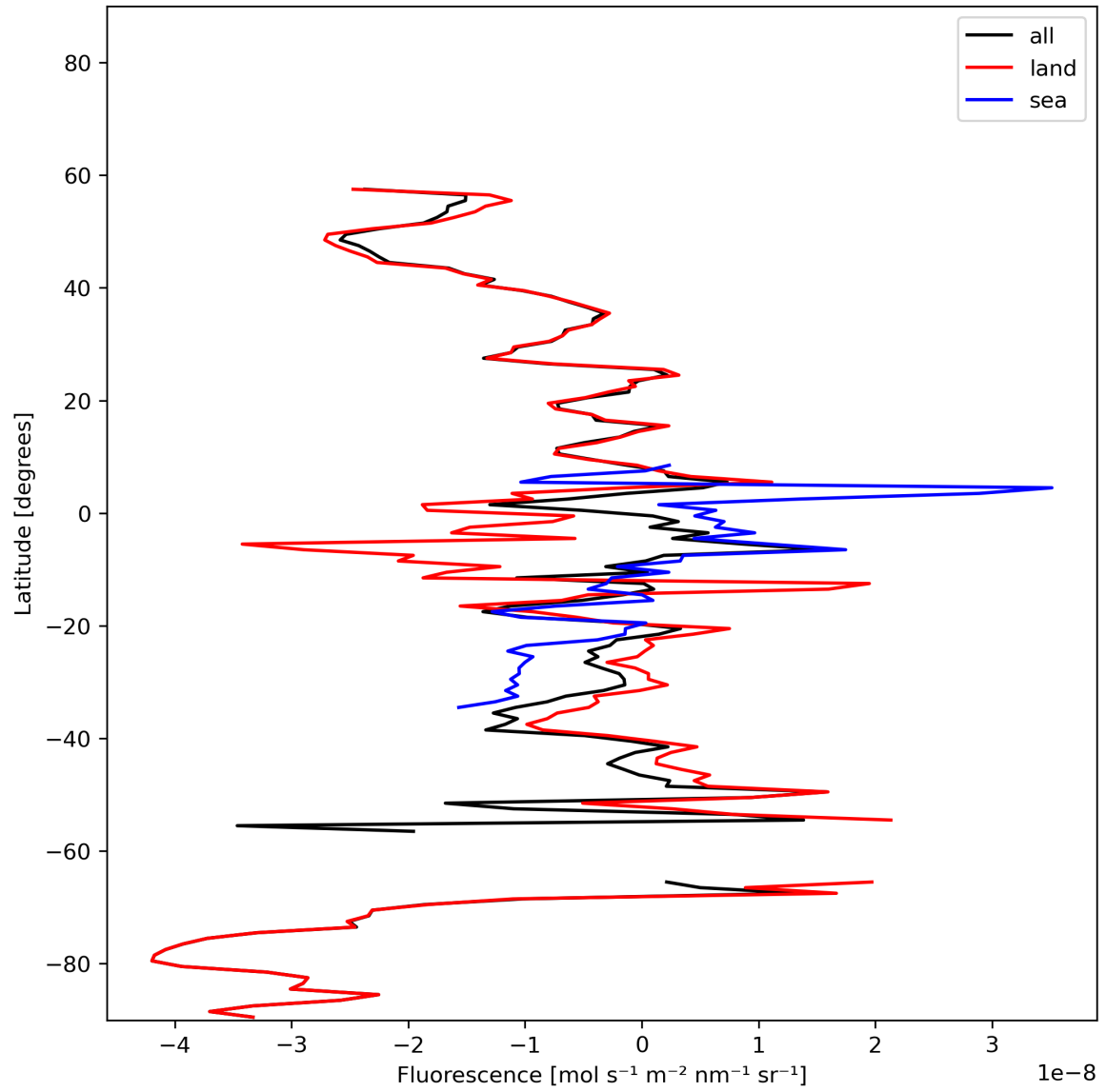
Figure 21: Zonal average of “Fluorescence” for 2024-01-28 to 2024-01-30.
