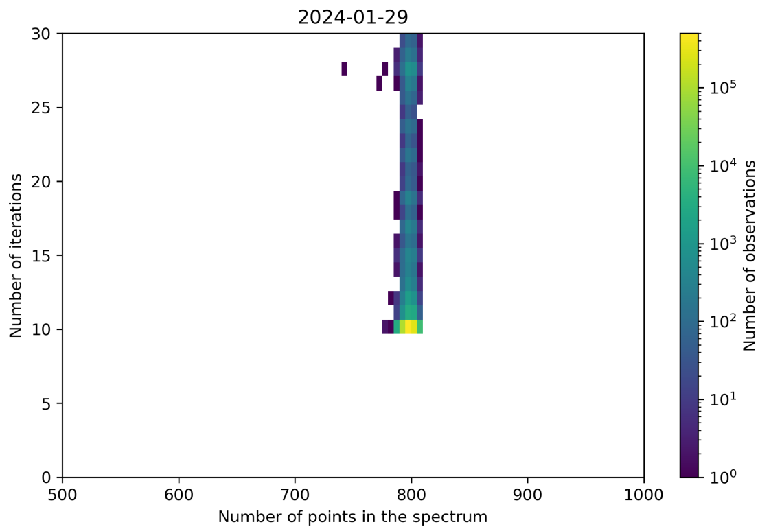
Figure 92: Scatter density plot of “Number of points in the spectrum” against “Number of iterations” for 2024-01-28 to 2024-01-30.
