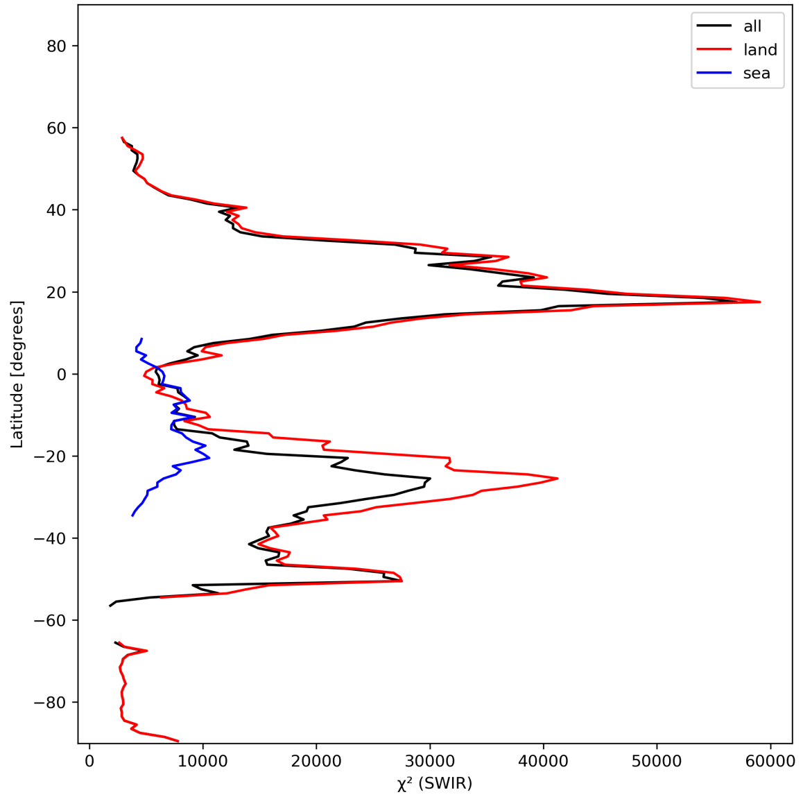
Figure 17: Zonal average of “ \chi^2 (SWIR)” for 2024-01-28 to 2024-01-30.
