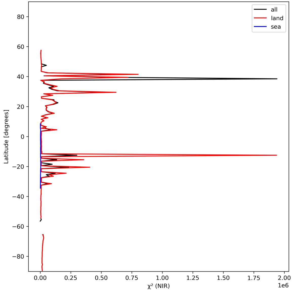
Figure 18: Zonal average of “ \chi^2 (NIR)” for 2024-01-28 to 2024-01-30.
