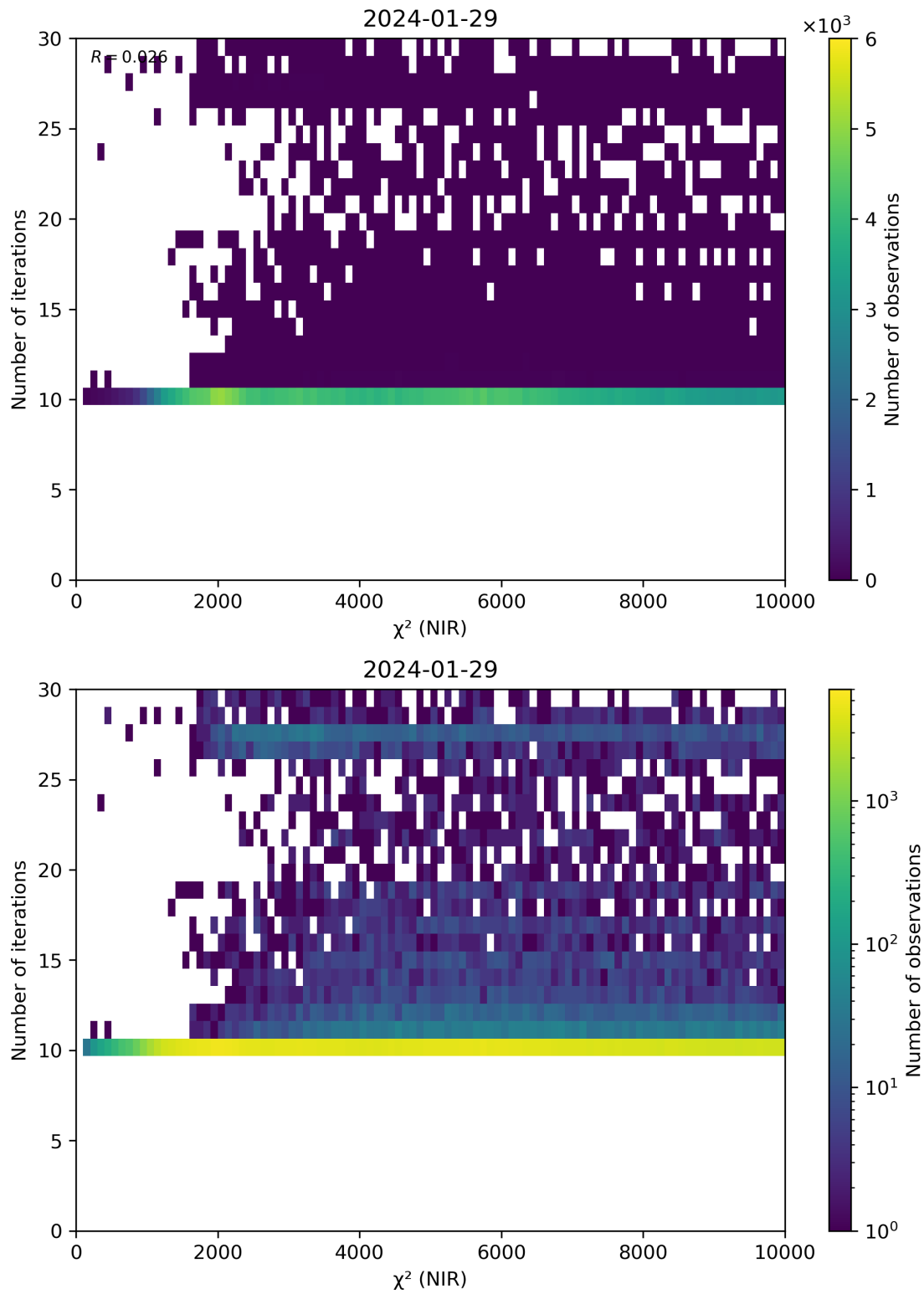
Figure 46: Scatter density plot of “ \chi^2 (NIR)” against “Number of iterations” for 2024-01-28 to 2024-01-30.
