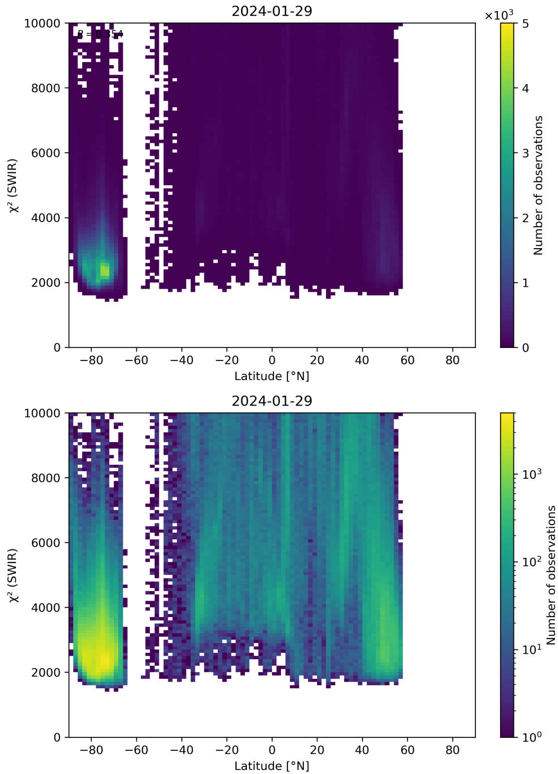
Figure 54: Scatter density plot of “Latitude” against “ \chi^2 (SWIR)” for 2024-01-28 to 2024-01-30.
