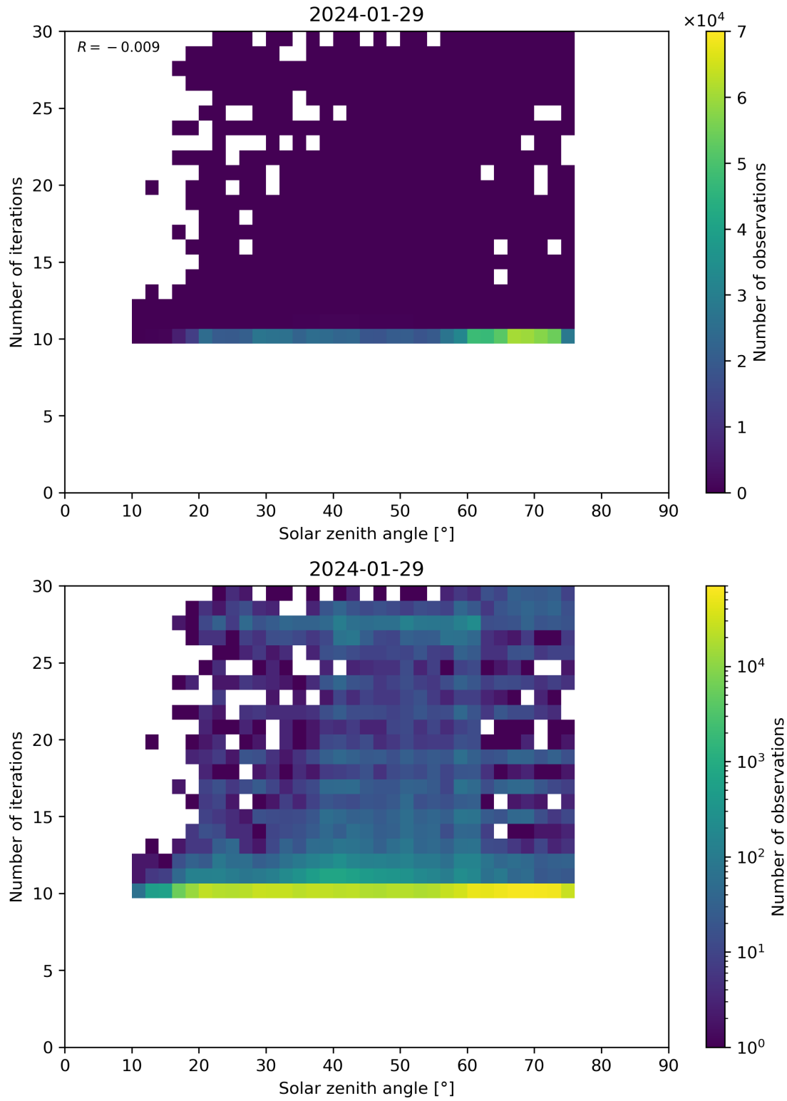
Figure 102: Scatter density plot of “Solar zenith angle” against “Number of iterations” for 2024-01-28 to 2024-01-30.
