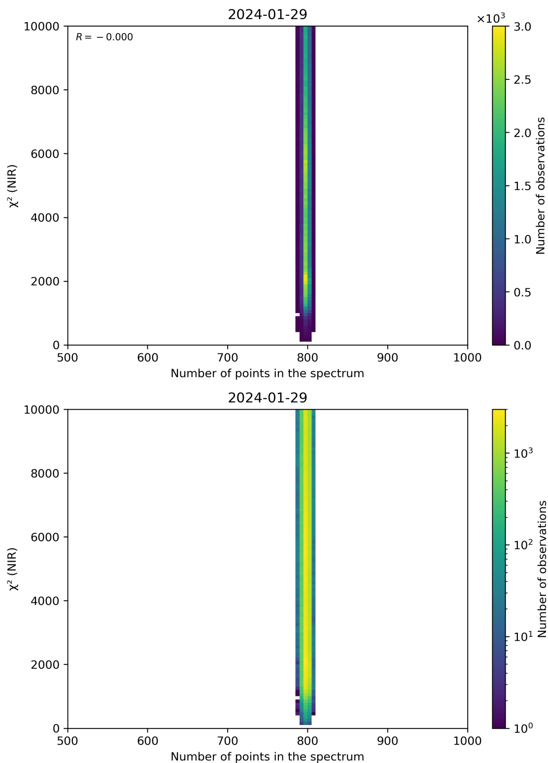
Figure 88: Scatter density plot of “Number of points in the spectrum” against “ \chi^2 (NIR)” for 2024-01-28 to 2024-01-30.
