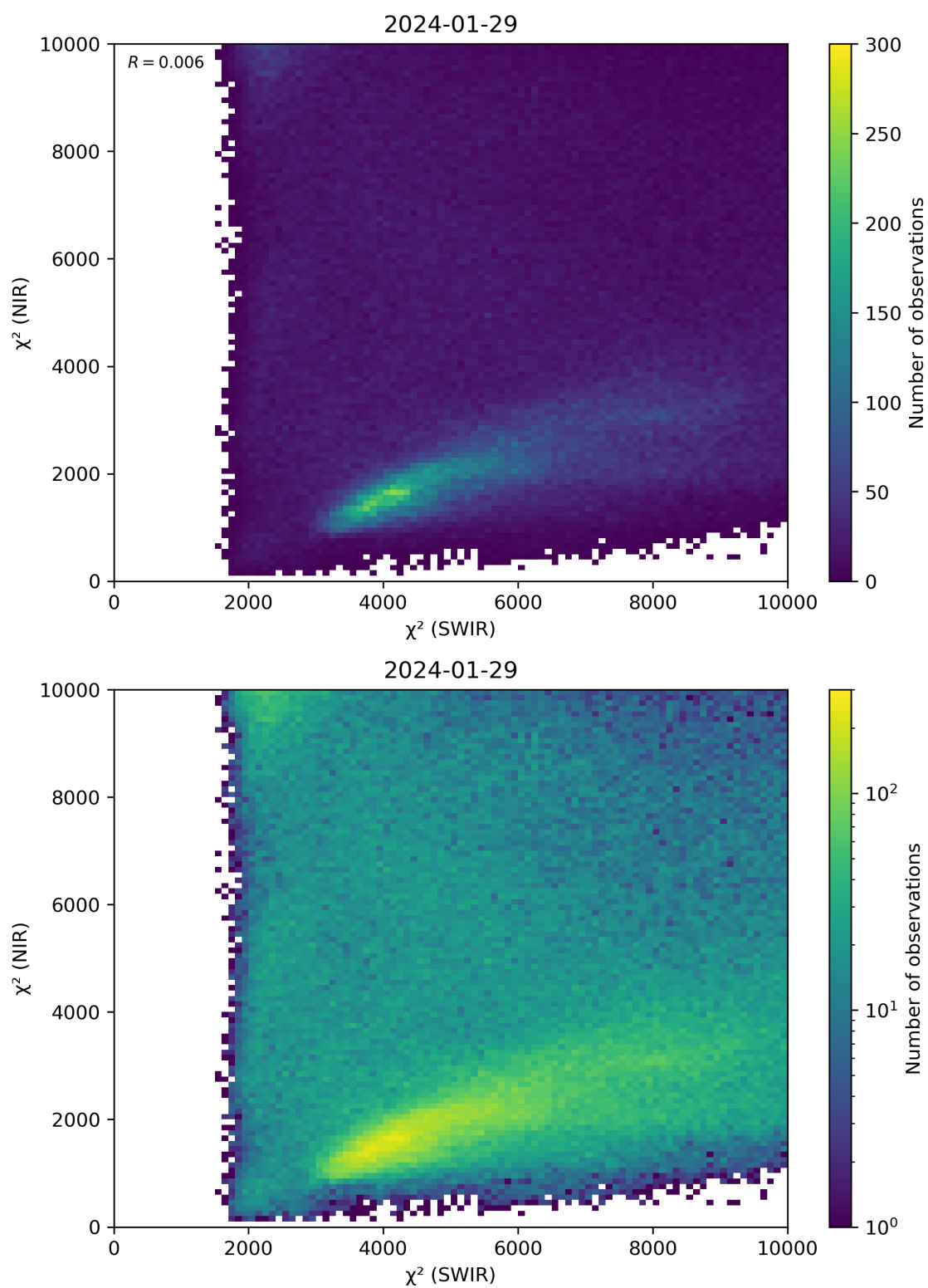
Figure 47: Scatter density plot of “ \chi^2 (SWIR)” against “ \chi^2 (NIR)” for 2024-01-28 to 2024-01-30.
