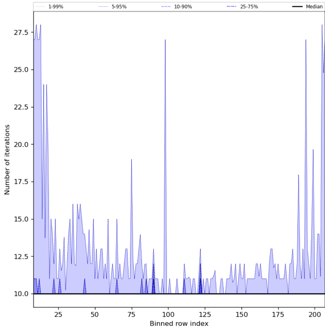
Figure 42: Along track statistics of “Number of iterations” for 2024-01-28 to 2024-01-30
