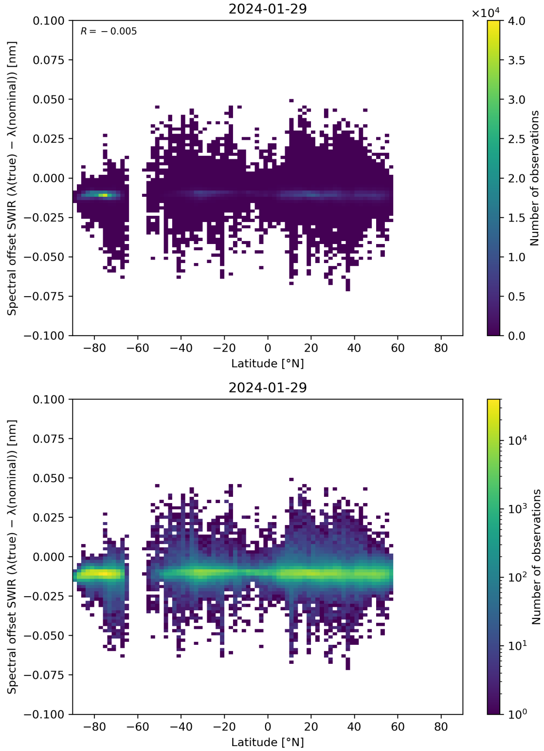
Figure 62: Scatter density plot of “Latitude” against “Spectral offset SWIR ( \lambda(\text{true}) - \lambda(\text{nominal}) )” for 2024-01-28 to 2024-01-30.
