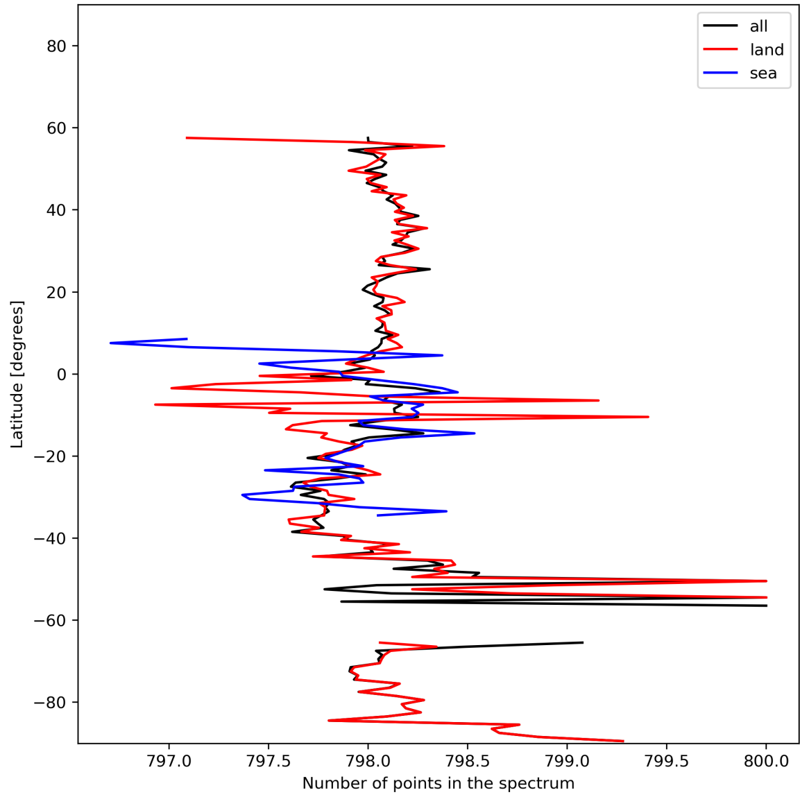
Figure 15: Zonal average of “Number of points in the spectrum” for 2024-01-28 to 2024-01-30.
