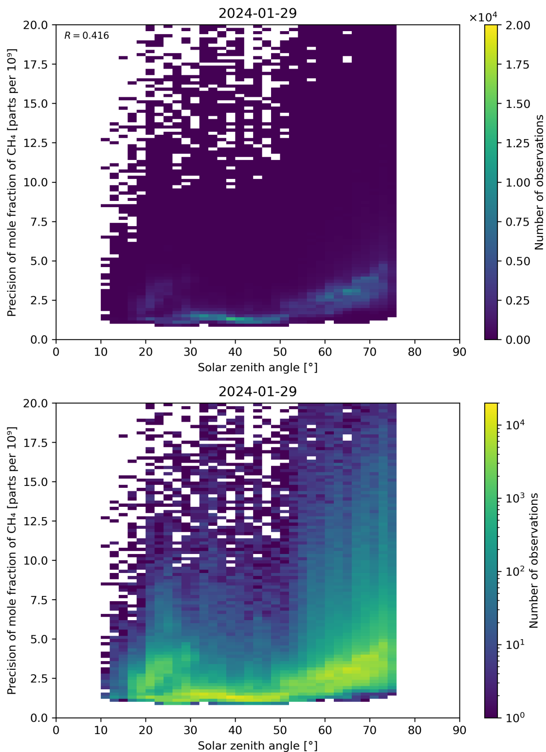
Figure 101: Scatter density plot of “Solar zenith angle” against “Precision of mole fraction of CH 4 ” for 2024-01-28 to 2024-01-30.
