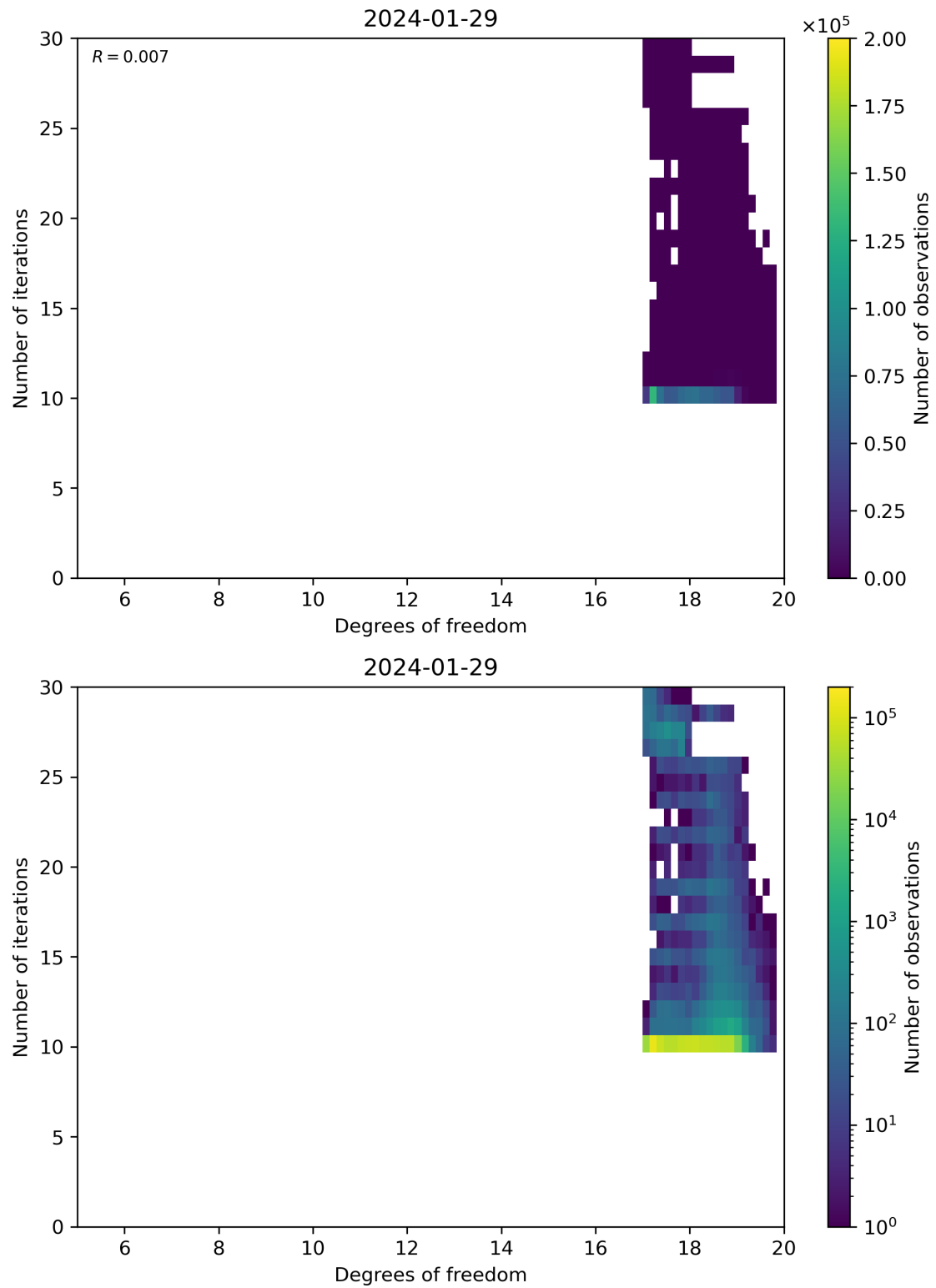
Figure 52: Scatter density plot of “Degrees of freedom” against “Number of iterations” for 2024-01-28 to 2024-01-30.
