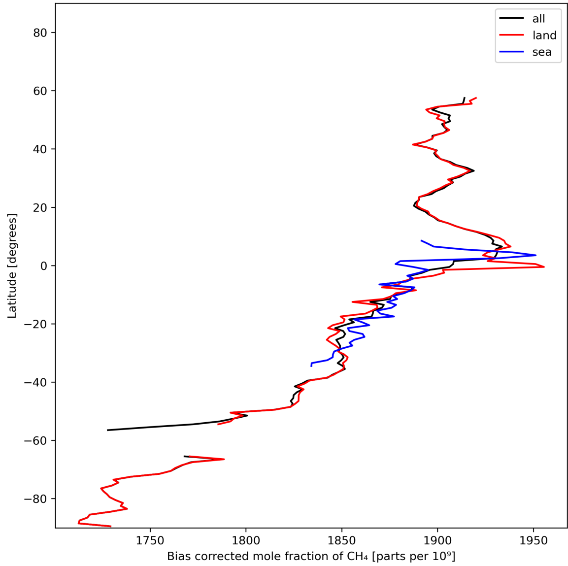
Figure 14: Zonal average of “Bias corrected mole fraction of CH 4 ” for 2024-01-28 to 2024-01-30.
