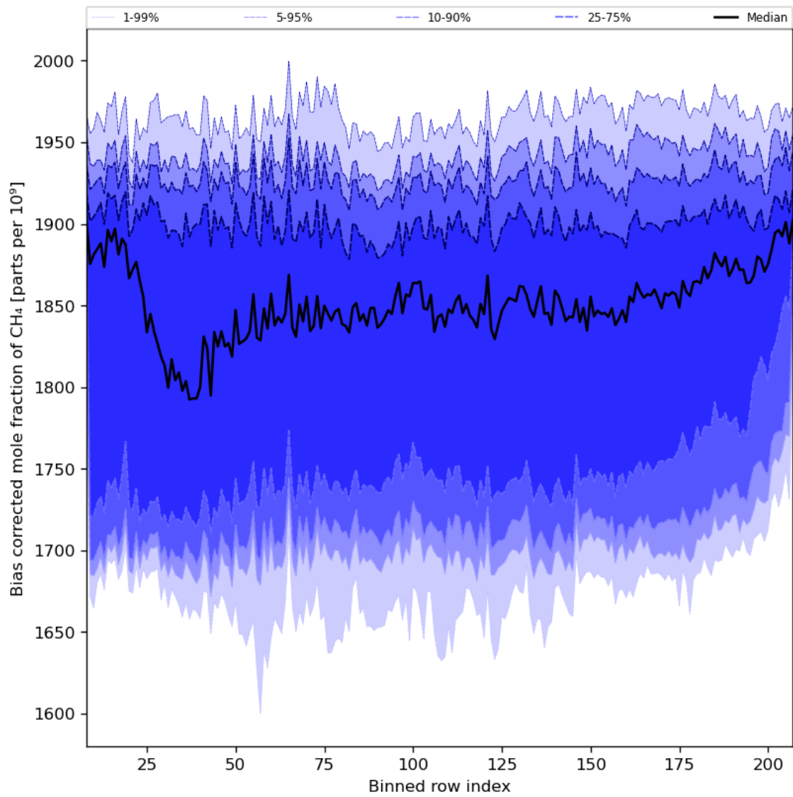
Figure 36: Along track statistics of “Bias corrected mole fraction of CH 4 ” for 2024-01-28 to 2024-01-30
