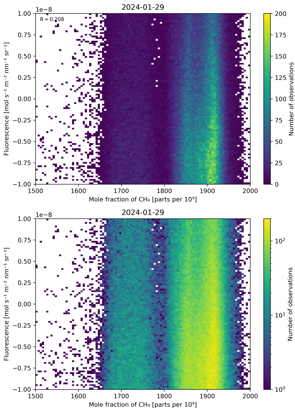
Figure 73: Scatter density plot of “Mole fraction of \text{CH}_4 ” against “Fluorescence” for 2024-01-28 to 2024-01-30.
