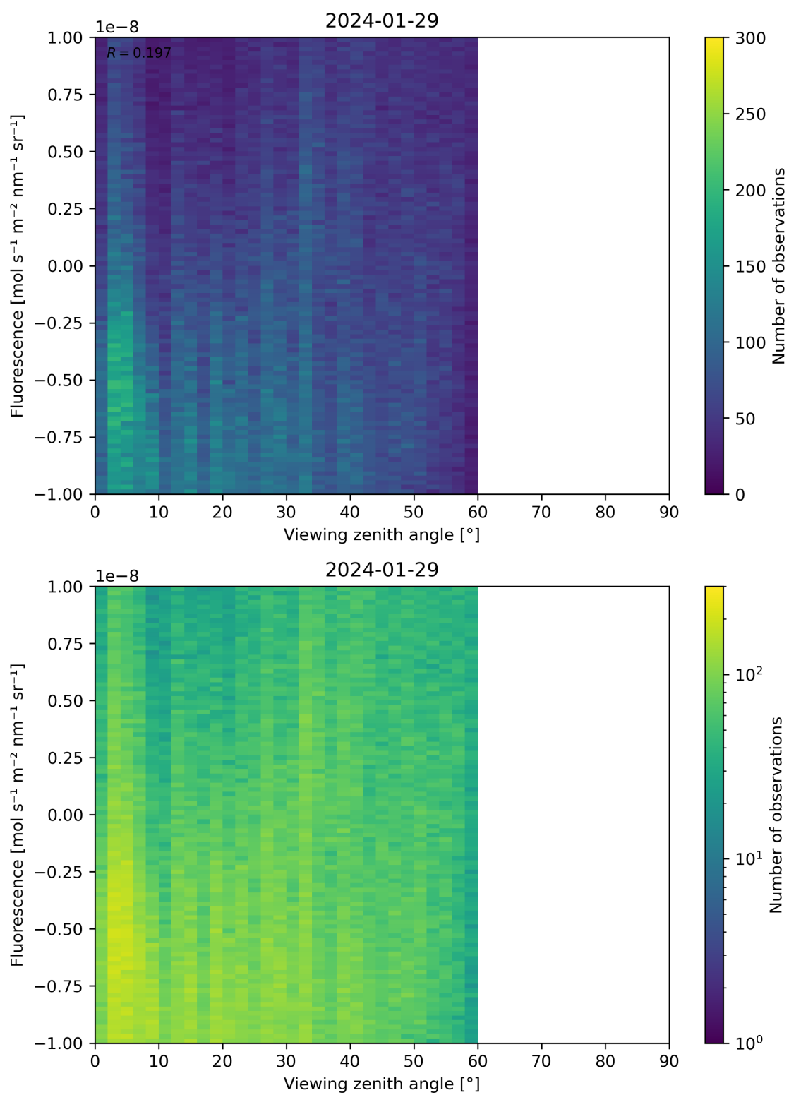
Figure 108: Scatter density plot of “Viewing zenith angle” against “Fluorescence” for 2024-01-28 to 2024-01-30.
