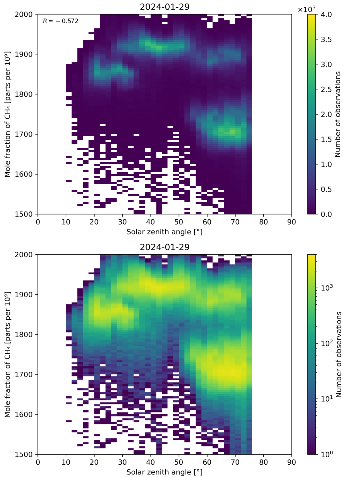
Figure 99: Scatter density plot of “Solar zenith angle” against “Mole fraction of CH 4 ” for 2024-01-28 to 2024-01-30.
