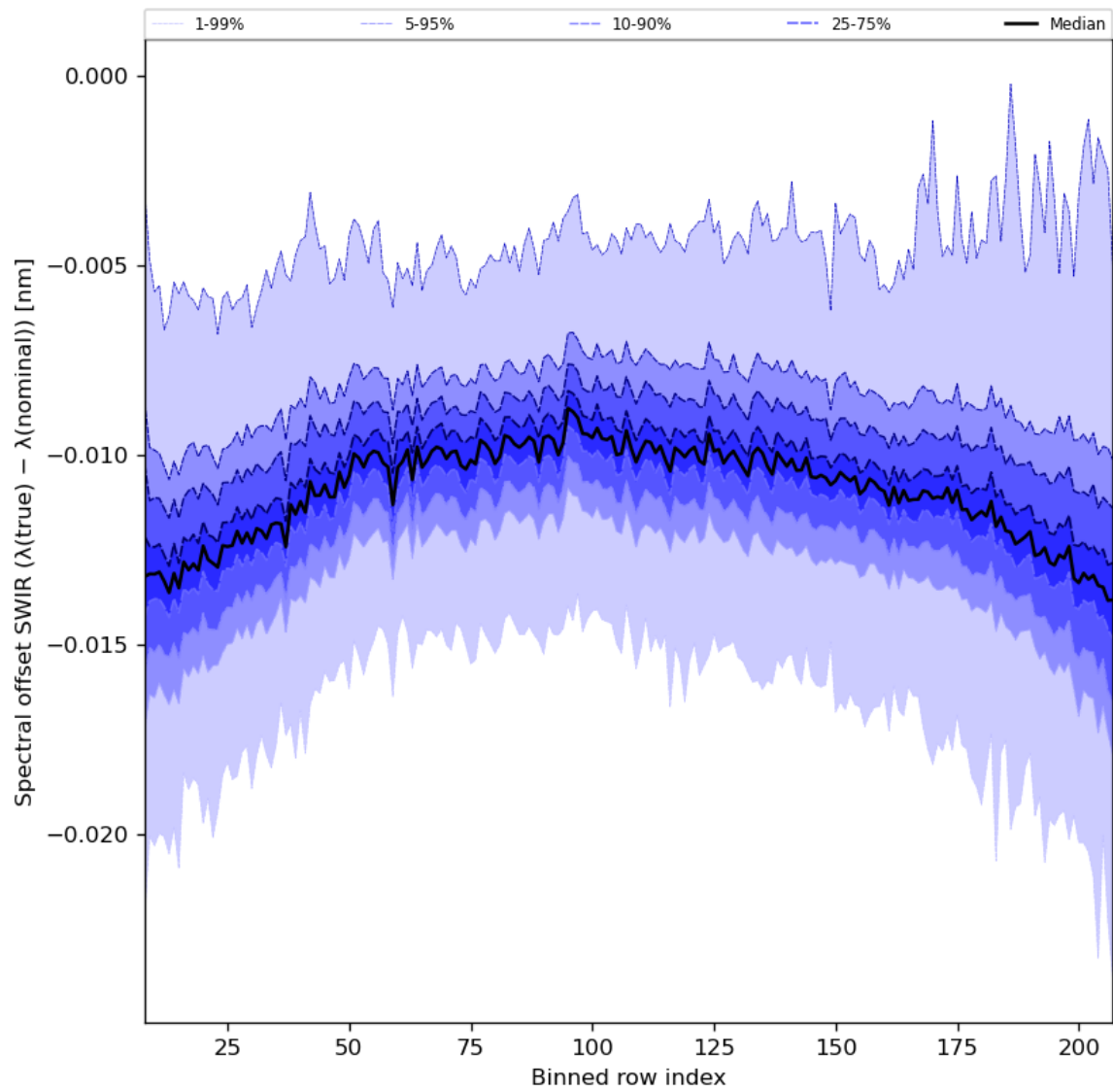
Figure 38: Along track statistics of “Spectral offset SWIR ( \lambda(\text{true}) - \lambda(\text{nominal}) )” for 2024-01-28 to 2024-01-30
