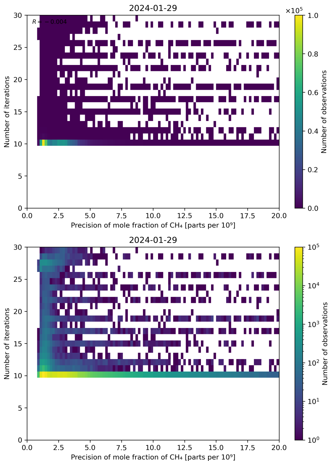
Figure 83: Scatter density plot of “Precision of mole fraction of CH 4 ” against “Number of iterations” for 2024-01-28 to 2024-01-30.
