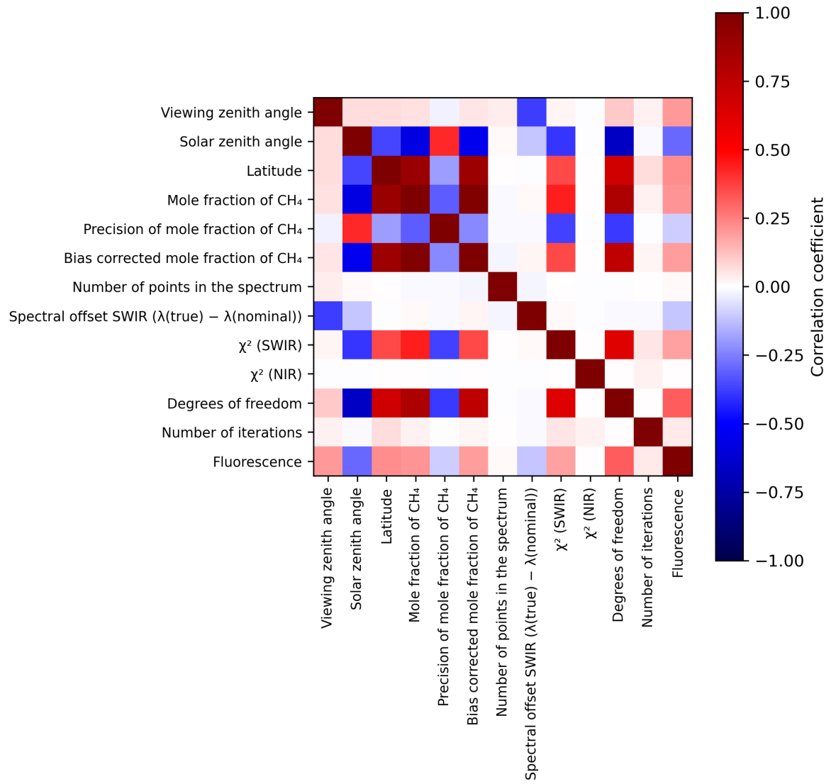
Figure 2: Map of correlation matrix for 2024-01-28 to 2024-01-30.
