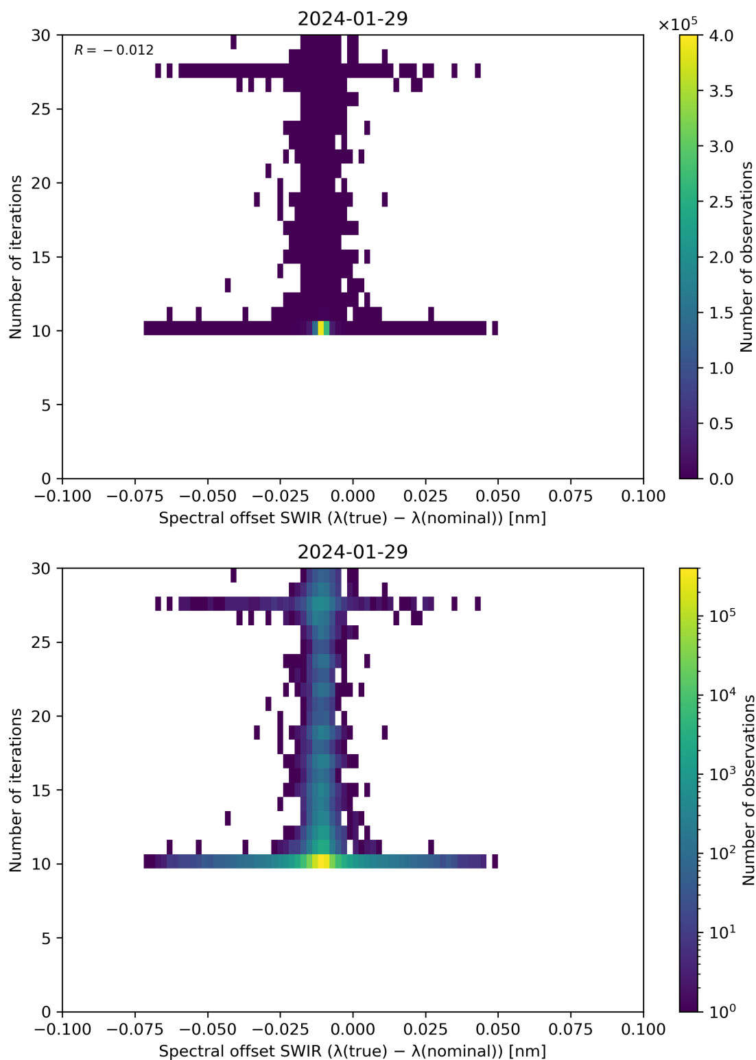
Figure 121: Scatter density plot of “Spectral offset SWIR ( \lambda(\text{true}) - \lambda(\text{nominal}) )” against “Number of iterations” for 2024-01-28 to 2024-01-30.
