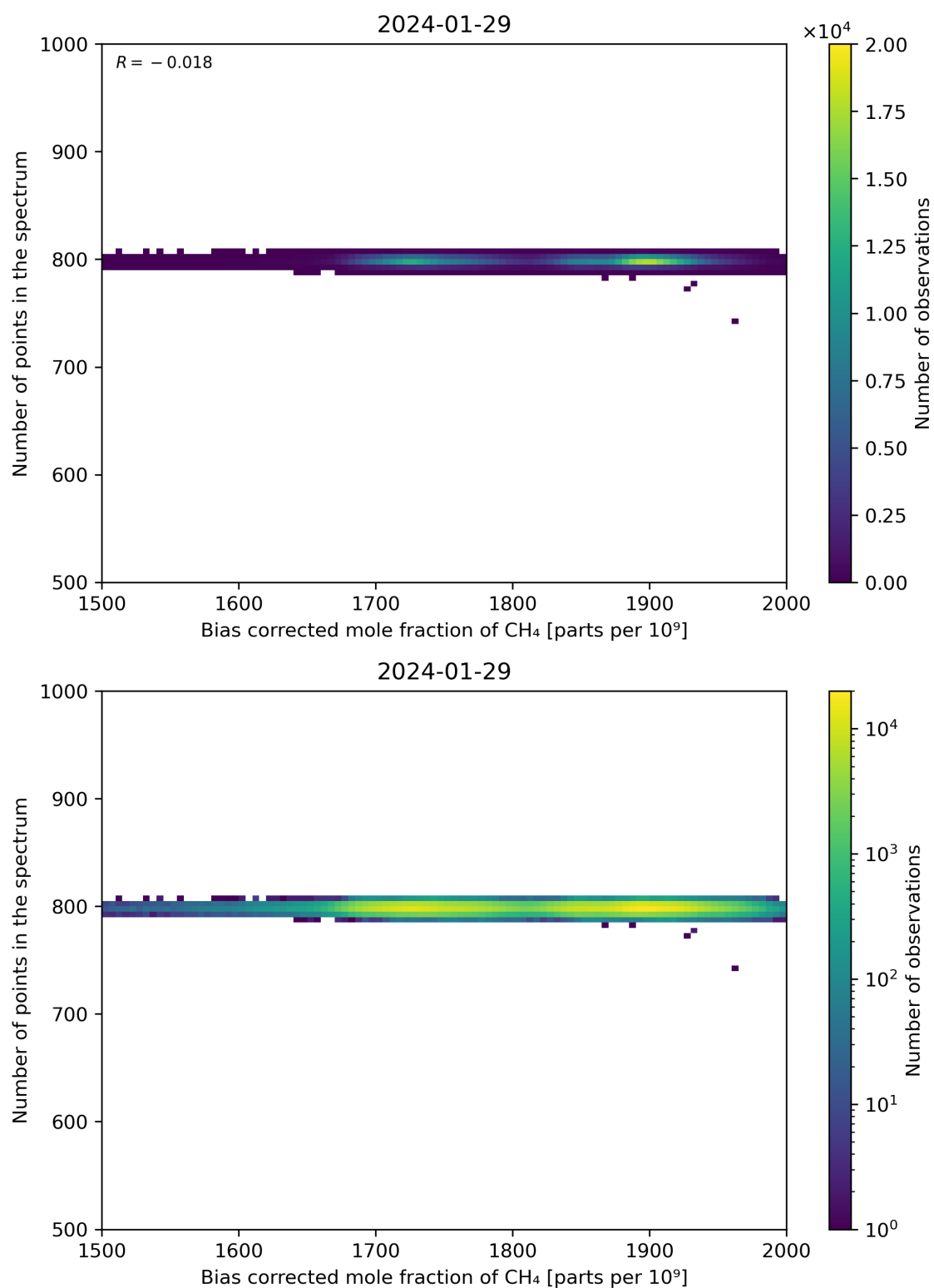
Figure 68: Scatter density plot of “Bias corrected mole fraction of CH 4 ” against “Number of points in the spectrum” for 2024-01-28 to 2024-01-30.
