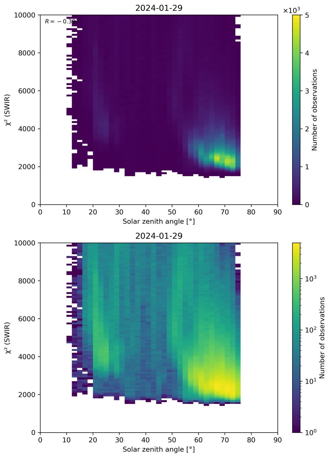
Figure 95: Scatter density plot of “Solar zenith angle” against “ \chi^2 (SWIR)” for 2024-01-28 to 2024-01-30.
