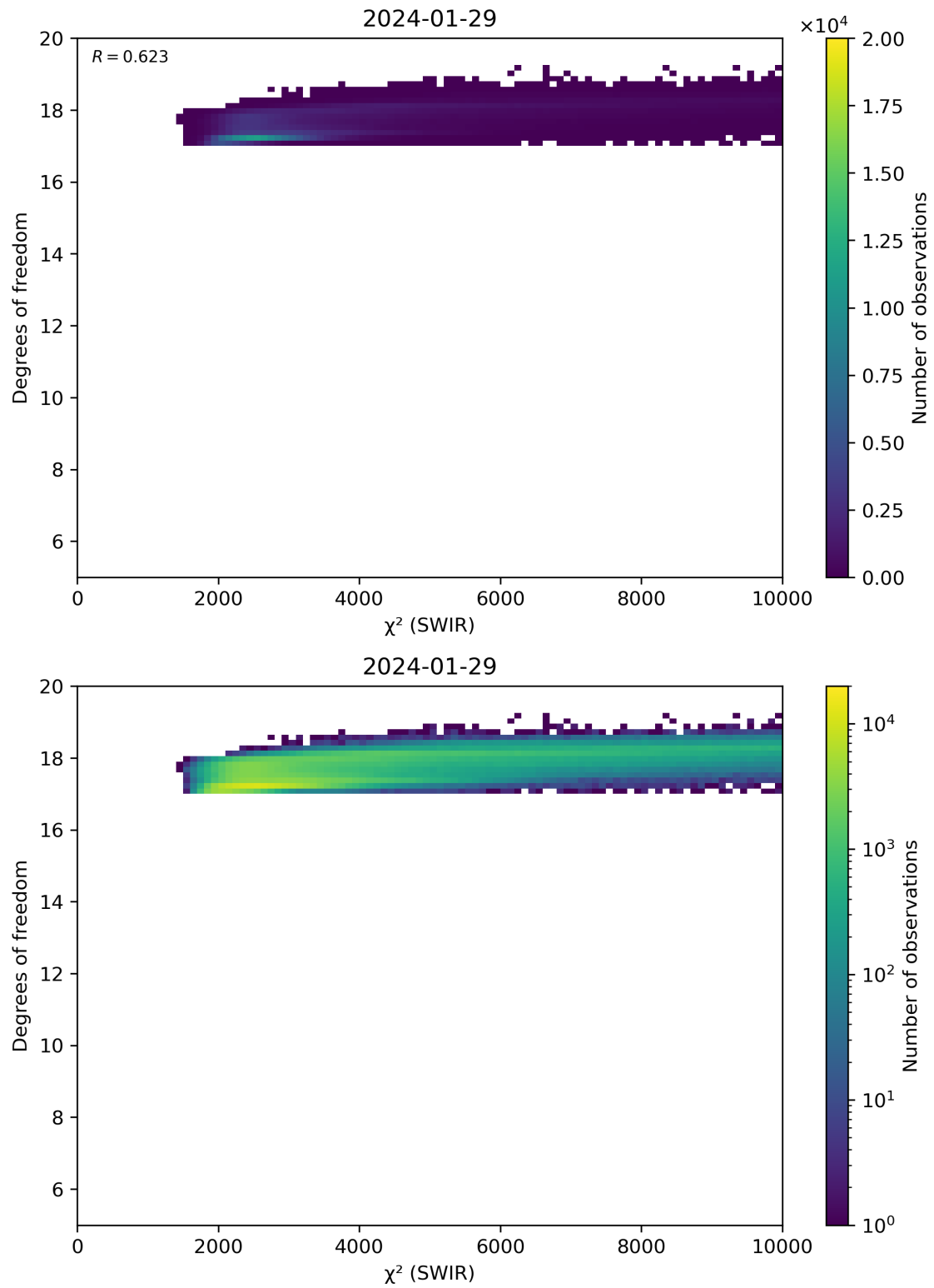
Figure 48: Scatter density plot of “ \chi^2 (SWIR)” against “Degrees of freedom” for 2024-01-28 to 2024-01-30.
