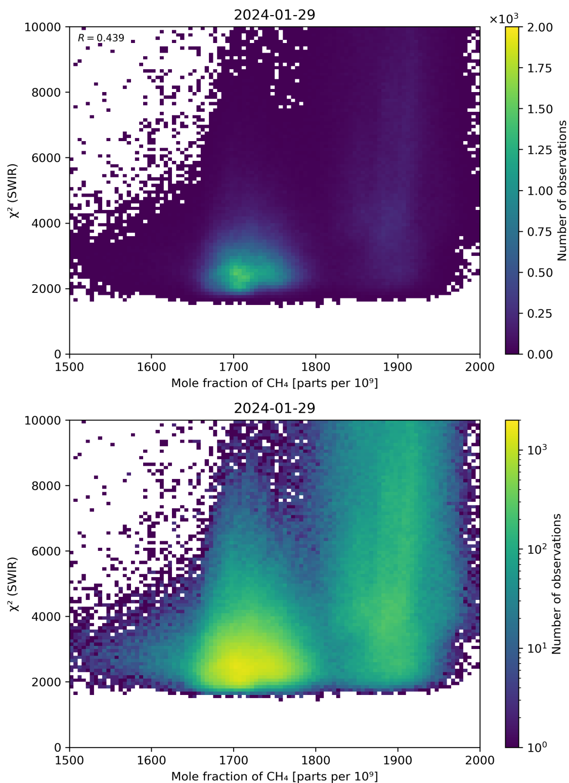
Figure 71: Scatter density plot of “Mole fraction of \text{CH}_4 ” against “ \chi^2 (SWIR)” for 2024-01-28 to 2024-01-30.
