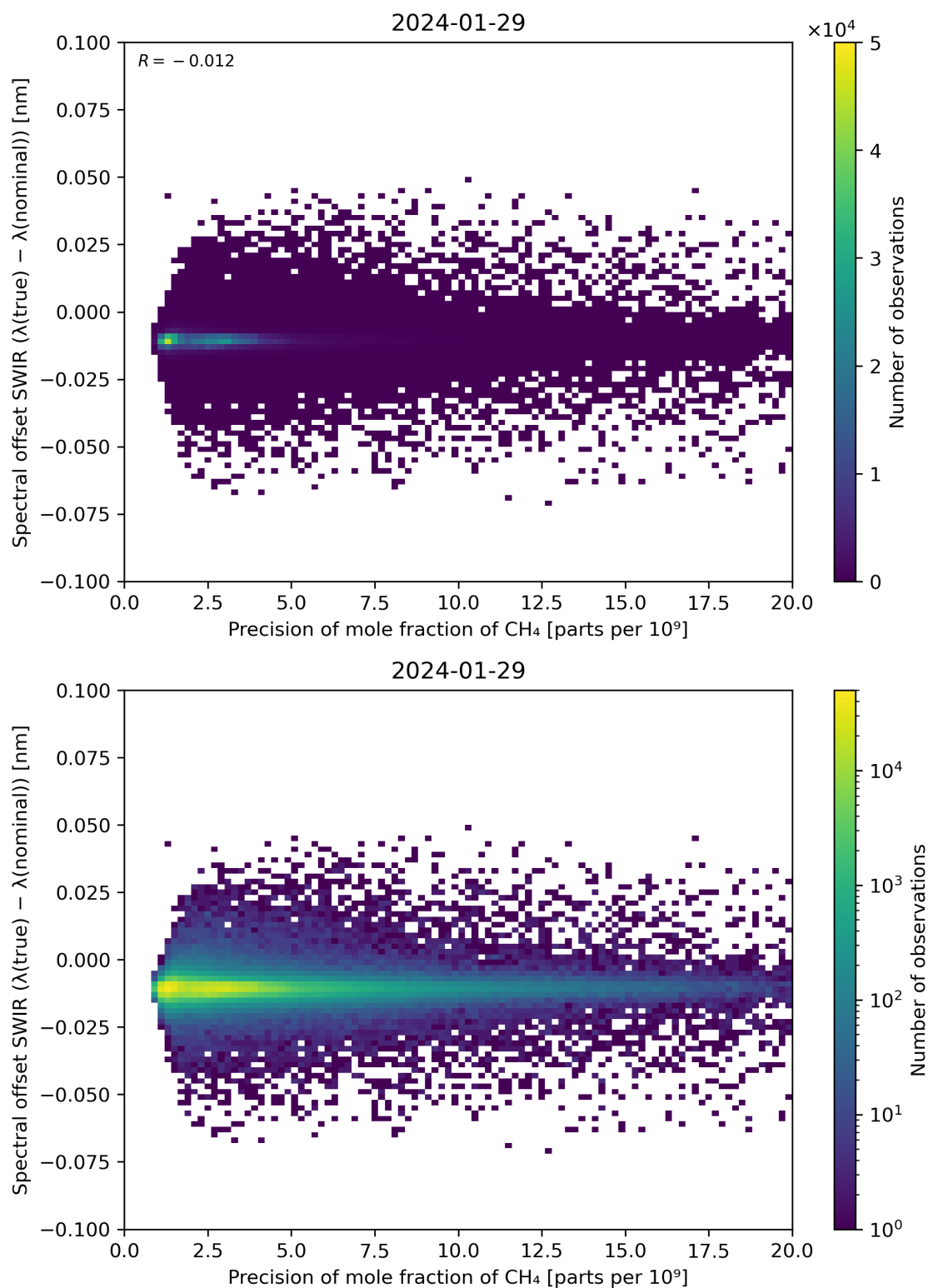
Figure 85: Scatter density plot of “Precision of mole fraction of \text{CH}_4 ” against “Spectral offset SWIR ( \lambda(\text{true}) - \lambda(\text{nominal}) )” for 2024-01-28 to 2024-01-30.
