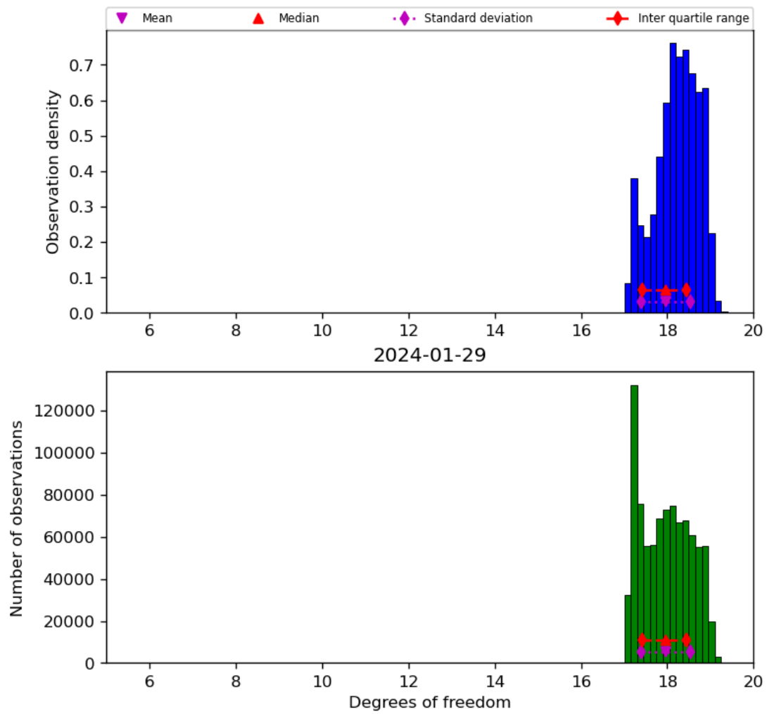
Figure 30: Histogram of “Degrees of freedom” for 2024-01-28 to 2024-01-30
