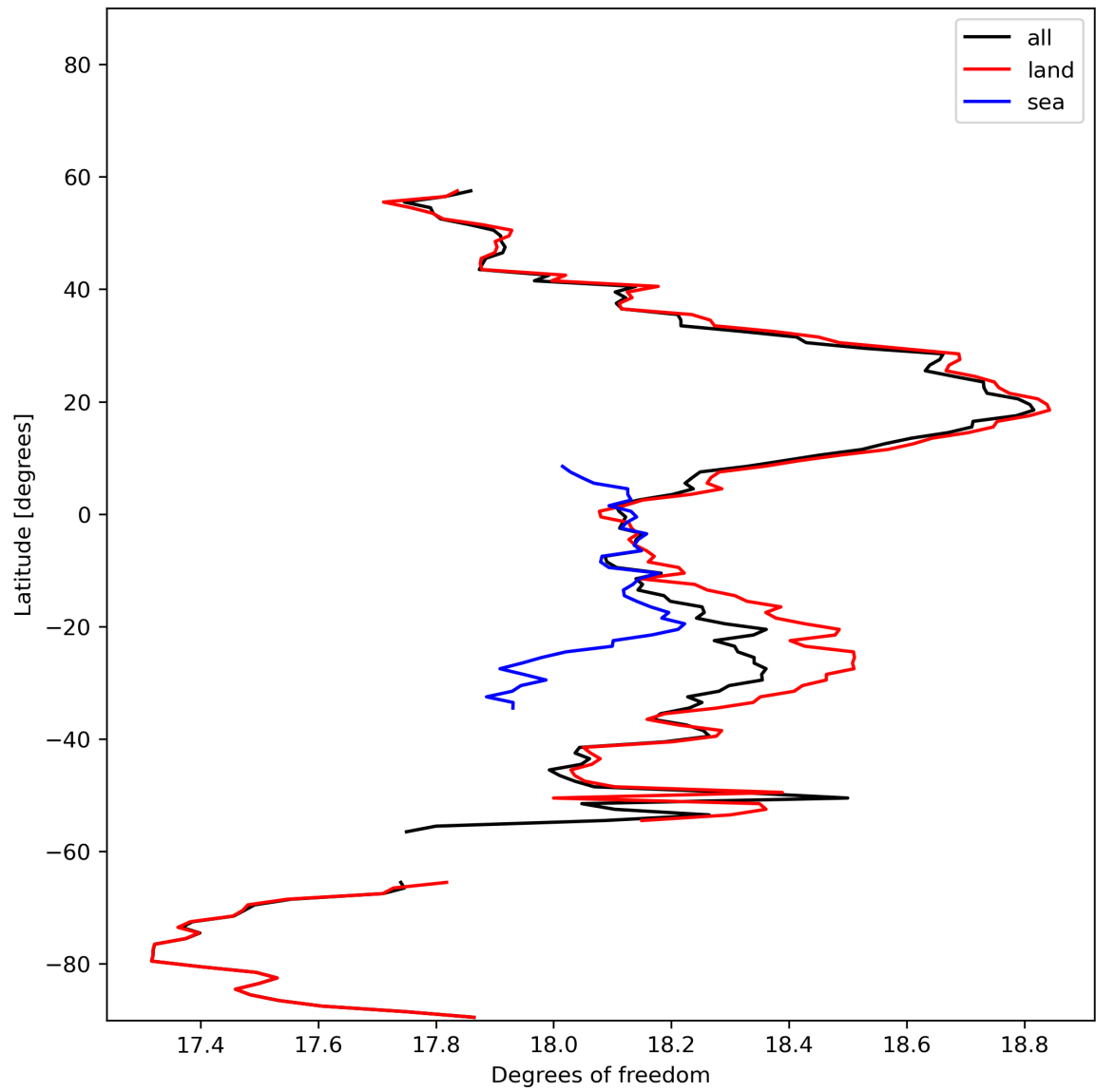
Figure 19: Zonal average of “Degrees of freedom” for 2024-01-28 to 2024-01-30.
