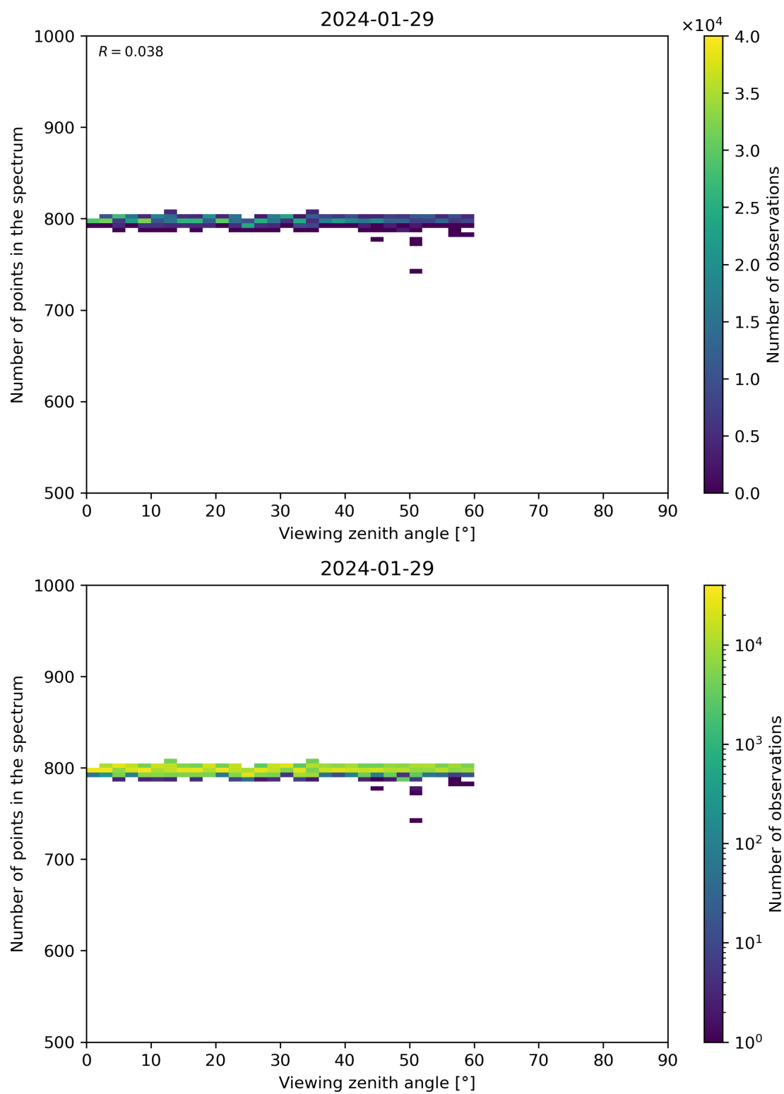
Figure 114: Scatter density plot of “Viewing zenith angle” against “Number of points in the spectrum” for 2024-01-28 to 2024-01-30.
