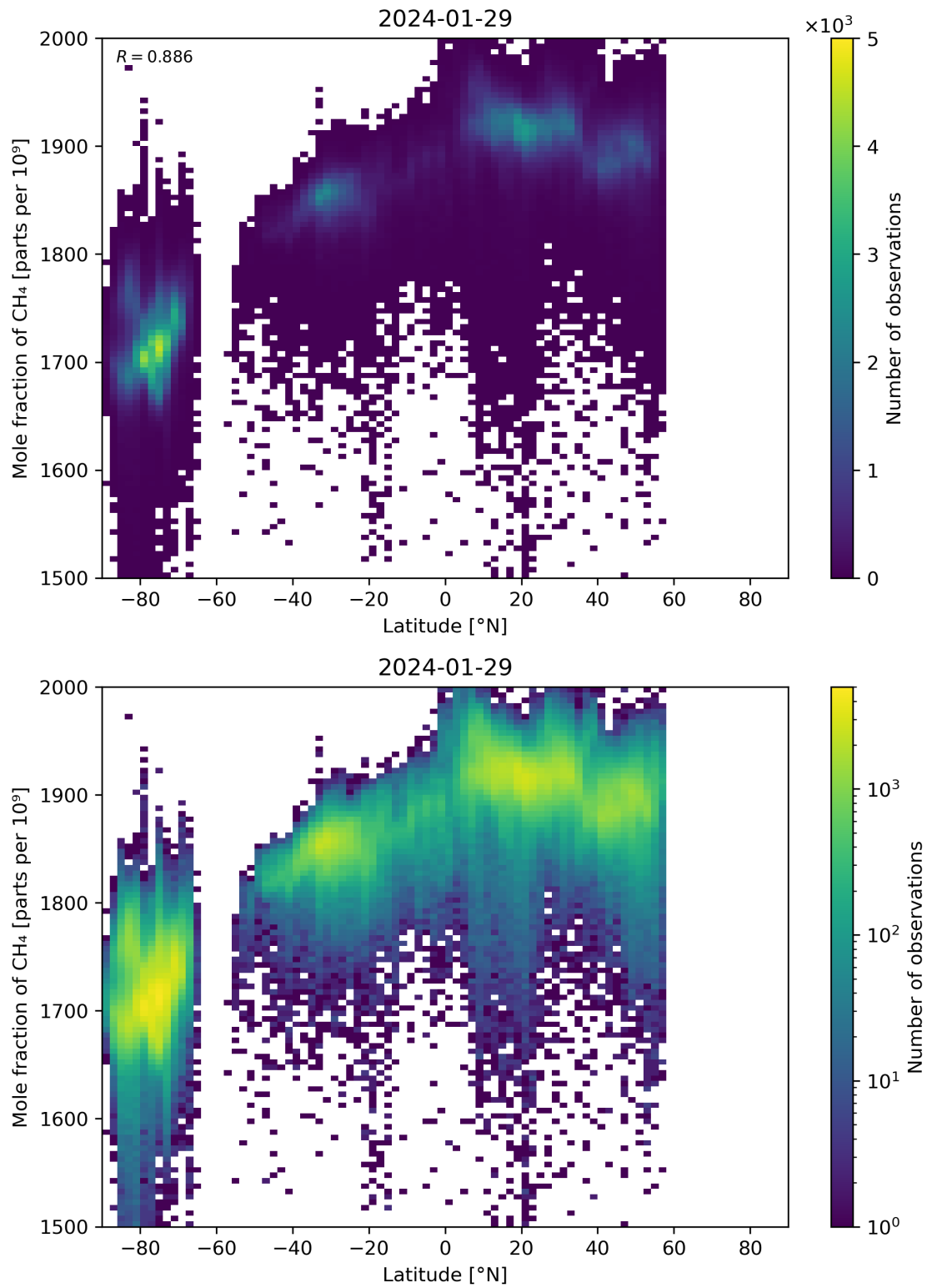
Figure 57: Scatter density plot of “Latitude” against “Mole fraction of CH 4 ” for 2024-01-28 to 2024-01-30.
