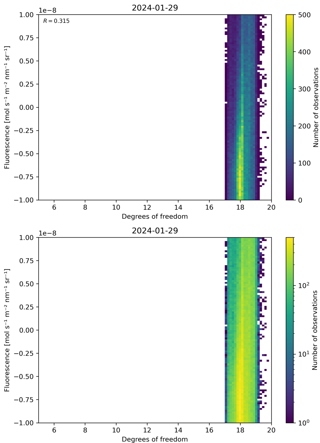
Figure 51: Scatter density plot of “Degrees of freedom” against “Fluorescence” for 2024-01-28 to 2024-01-30.
