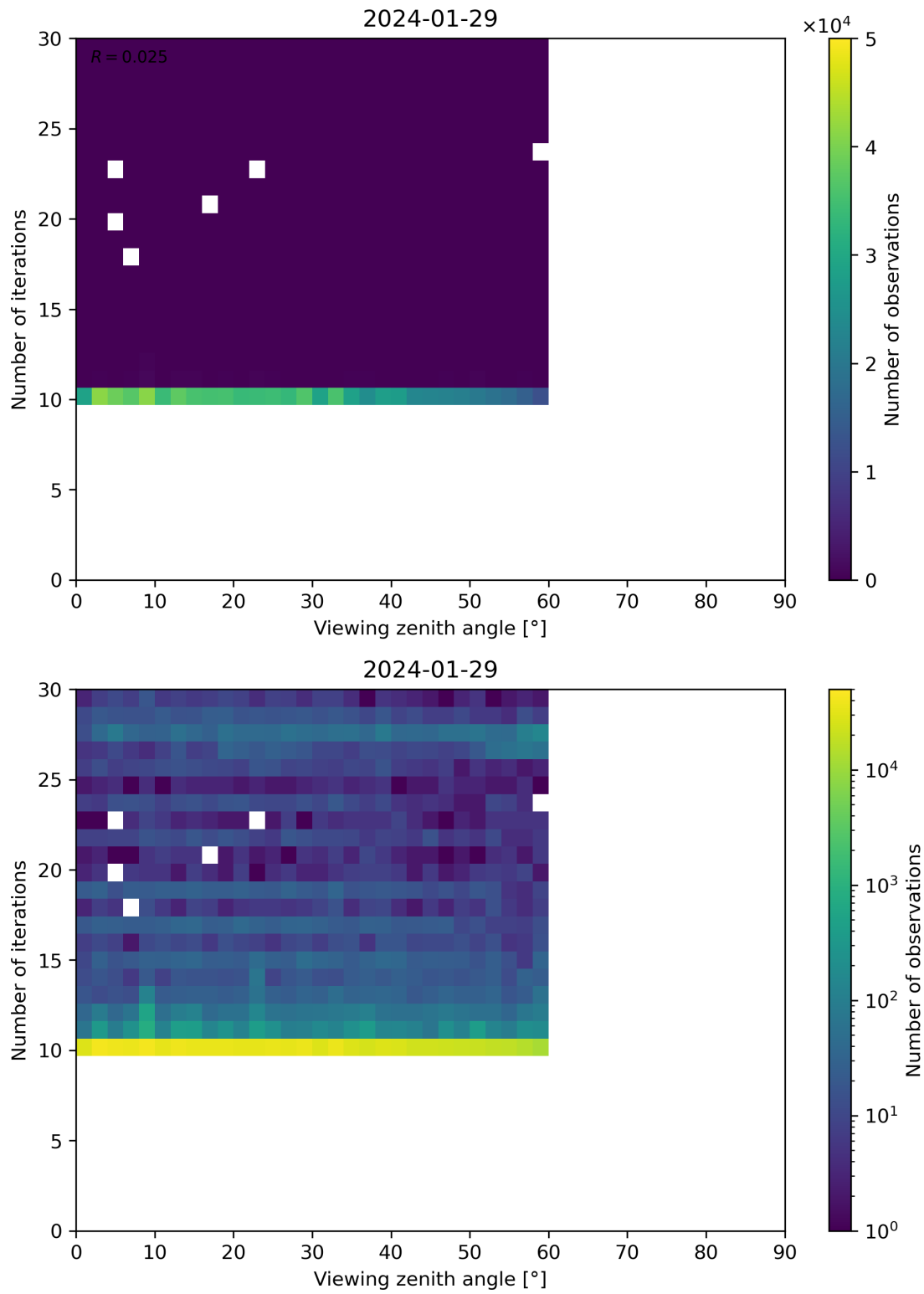
Figure 113: Scatter density plot of “Viewing zenith angle” against “Number of iterations” for 2024-01-28 to 2024-01-30.
