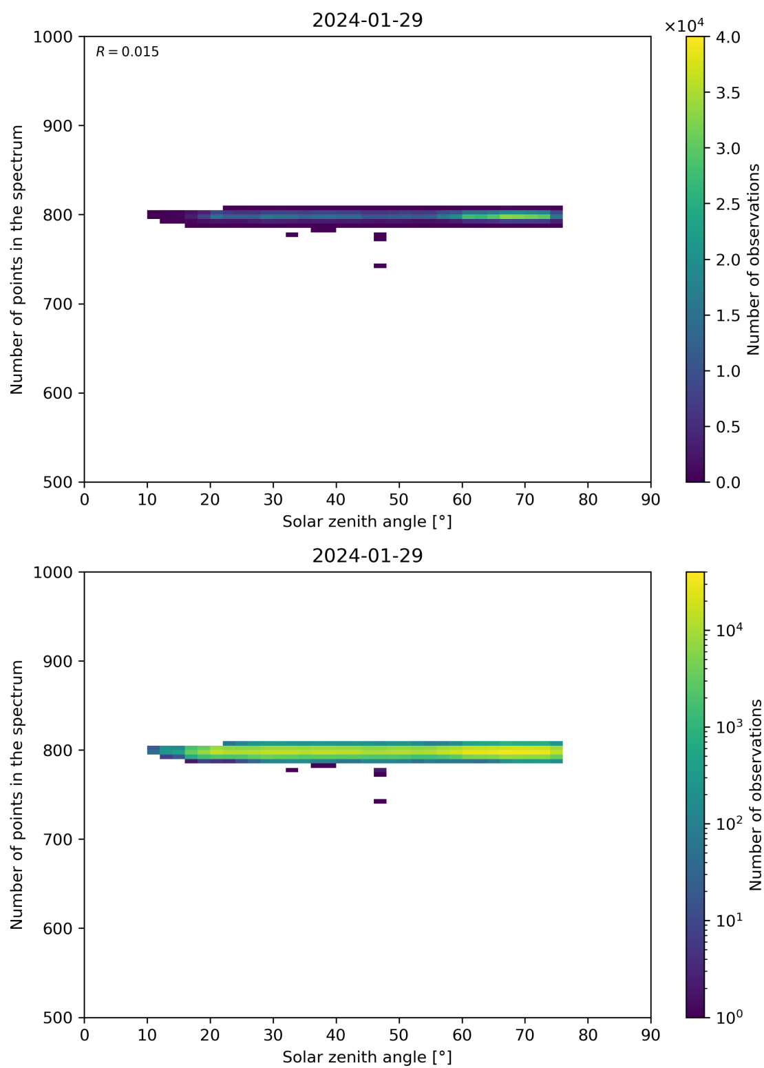
Figure 103: Scatter density plot of “Solar zenith angle” against “Number of points in the spectrum” for 2024-01-28 to 2024-01-30.
