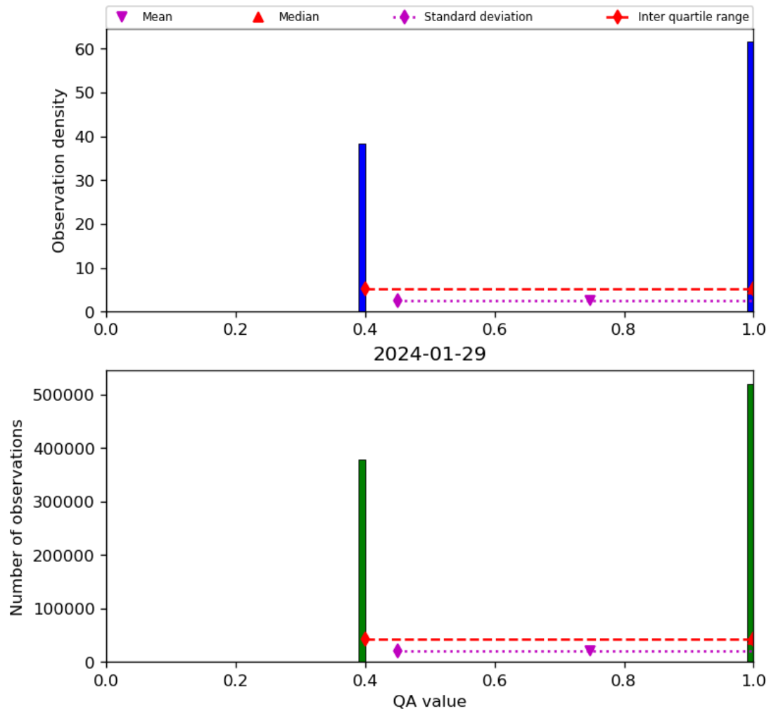
Figure 22: Histogram of “QA value” for 2024-01-28 to 2024-01-30
