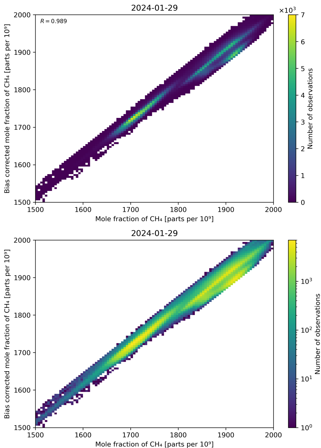
Figure 74: Scatter density plot of “Mole fraction of CH 4 ” against “Bias corrected mole fraction of CH 4 ” for 2024-01-28 to 2024-01-30.
