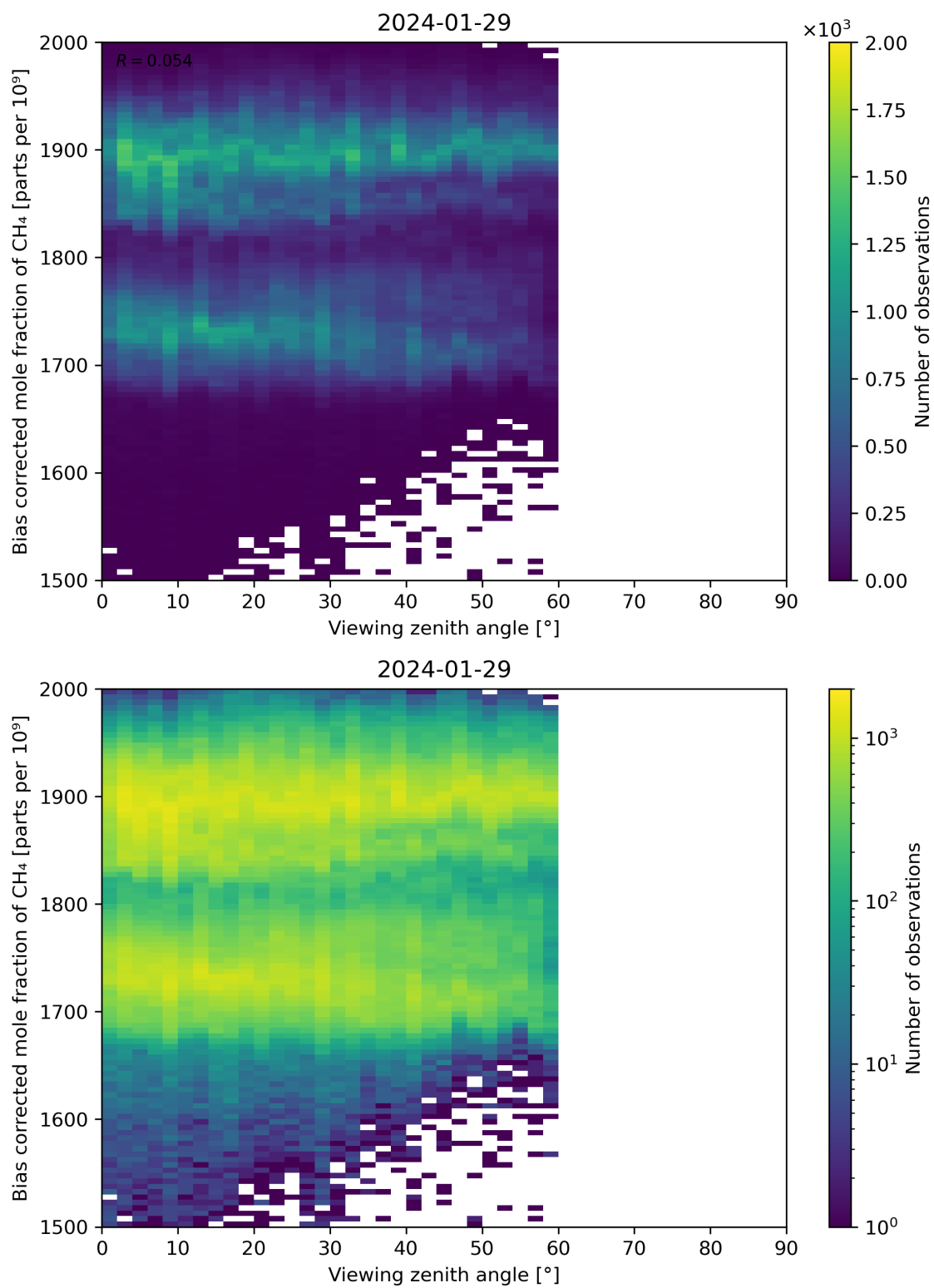
Figure 111: Scatter density plot of “Viewing zenith angle” against “Bias corrected mole fraction of CH 4 ” for 2024-01-28 to 2024-01-30.
