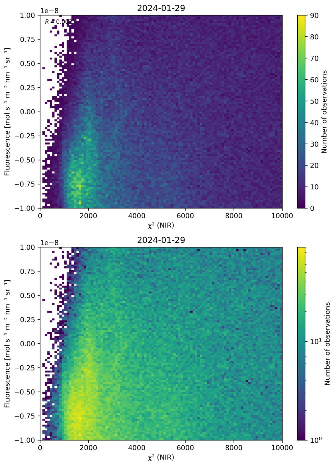
Figure 45: Scatter density plot of “ \chi^2 (NIR)” against “Fluorescence” for 2024-01-28 to 2024-01-30.
