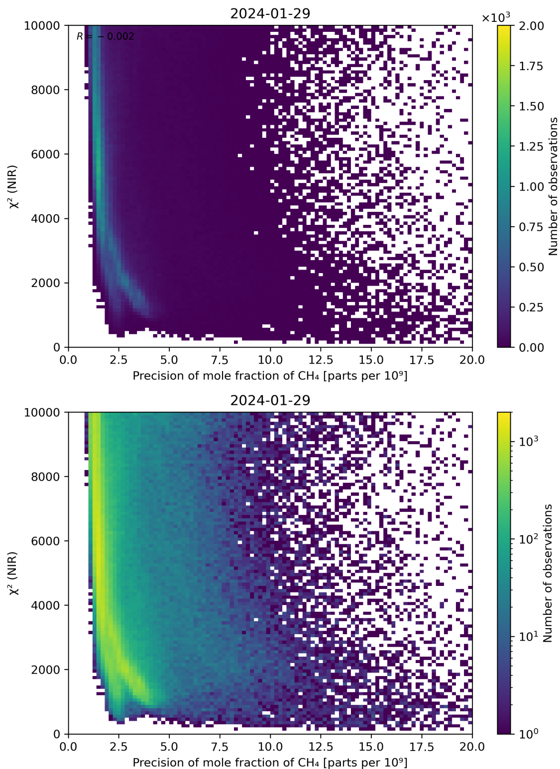
Figure 78: Scatter density plot of “Precision of mole fraction of CH 4 ” against “ \chi^2 (NIR)” for 2024-01-28 to 2024-01-30.
