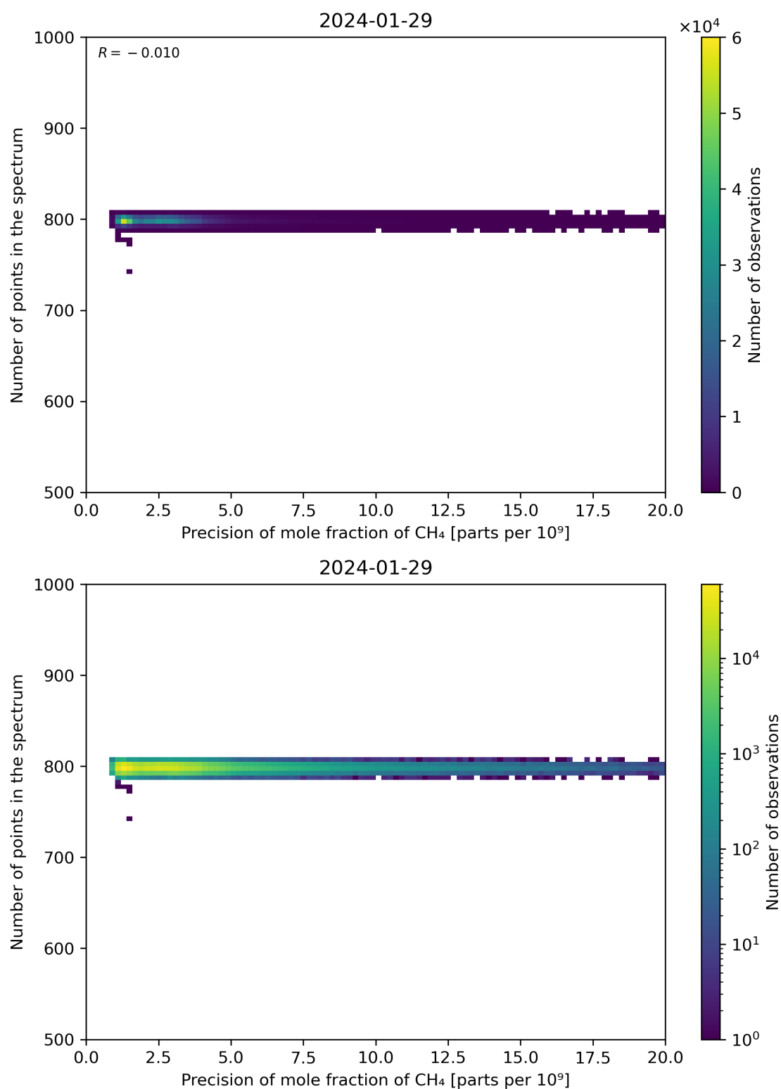
Figure 84: Scatter density plot of “Precision of mole fraction of CH 4 ” against “Number of points in the spectrum” for 2024-01-28 to 2024-01-30.
