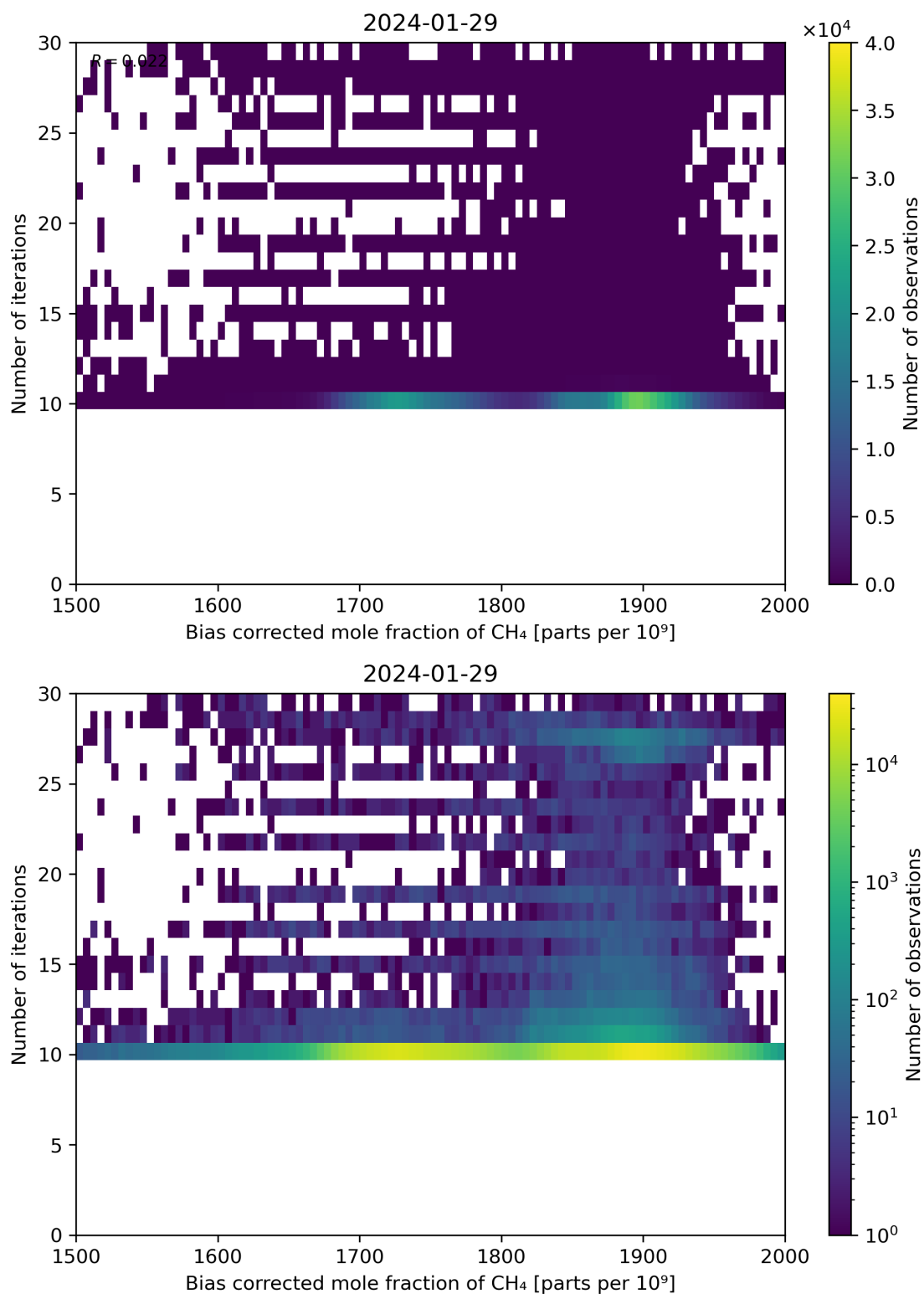
Figure 67: Scatter density plot of “Bias corrected mole fraction of \text{CH}_4 ” against “Number of iterations” for 2024-01-28 to 2024-01-30.
