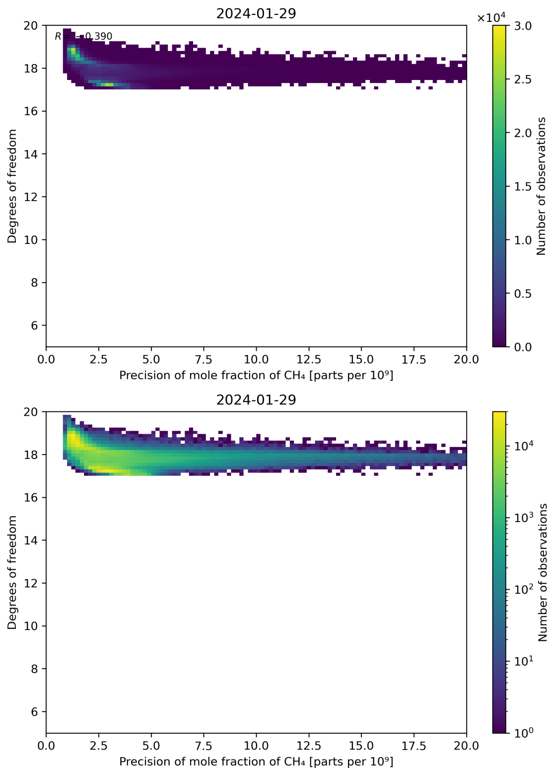
Figure 80: Scatter density plot of “Precision of mole fraction of CH 4 ” against “Degrees of freedom” for 2024-01-28 to 2024-01-30.
