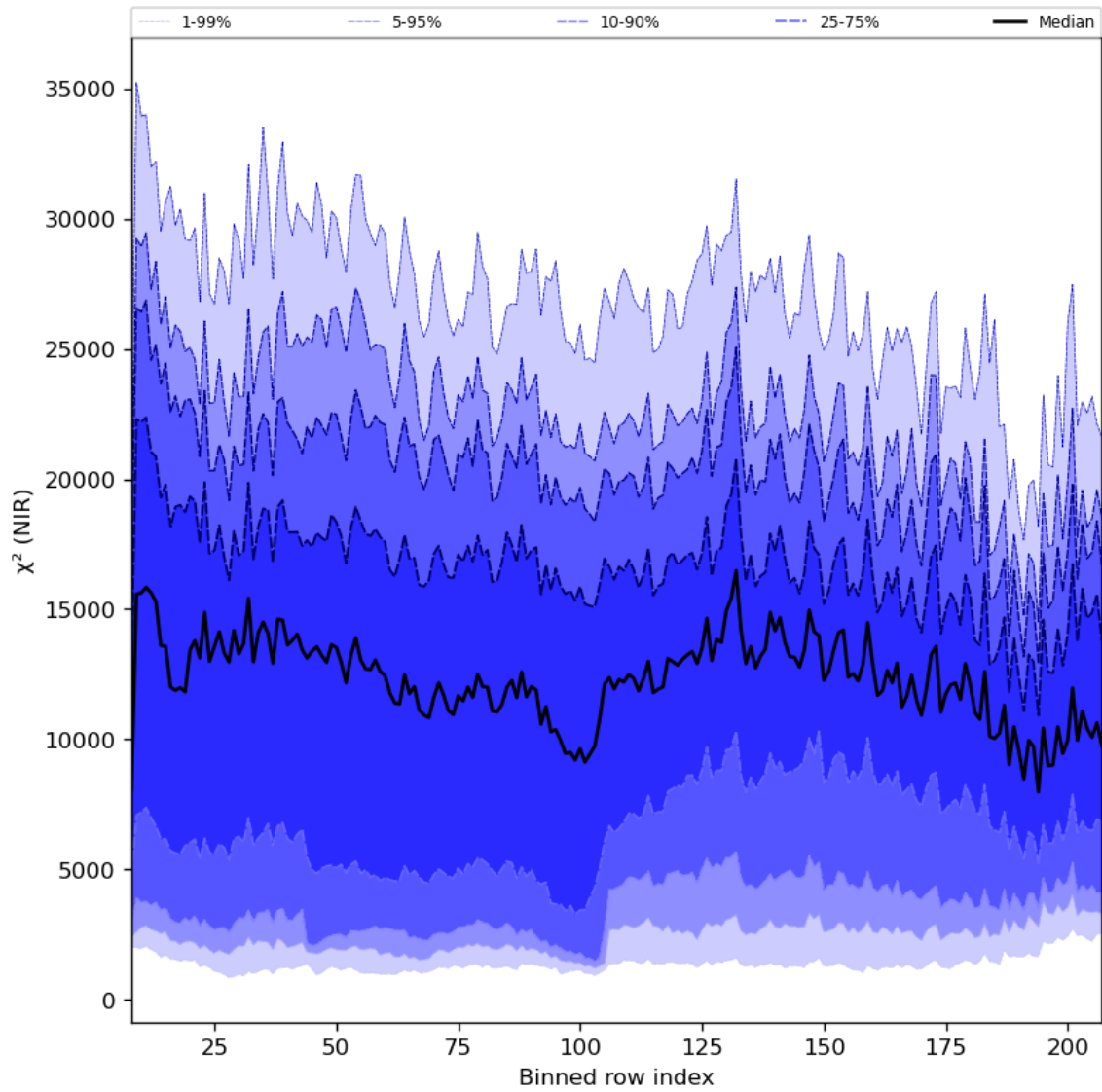
Figure 40: Along track statistics of “ \chi^2 (NIR)” for 2024-01-28 to 2024-01-30
