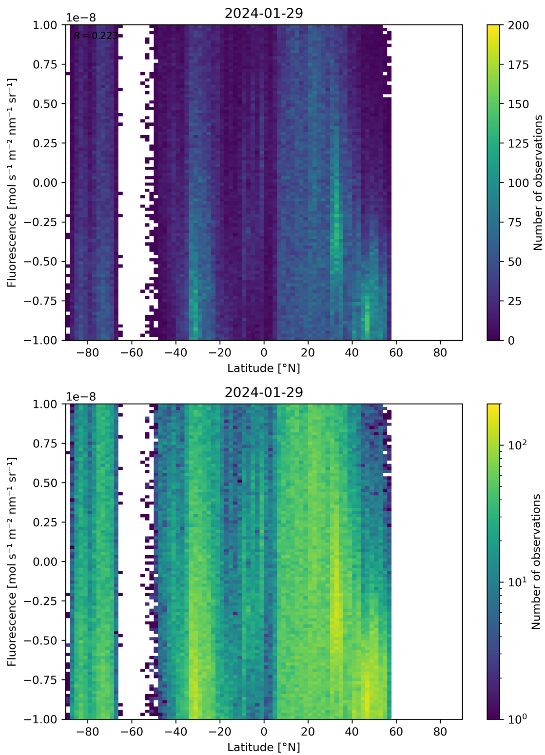
Figure 56: Scatter density plot of “Latitude” against “Fluorescence” for 2024-01-28 to 2024-01-30.
