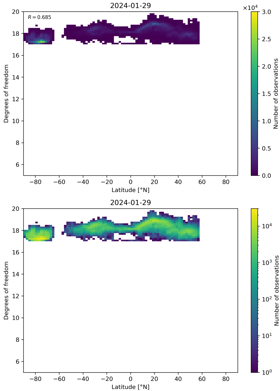
Figure 55: Scatter density plot of “Latitude” against “Degrees of freedom” for 2024-01-28 to 2024-01-30.
