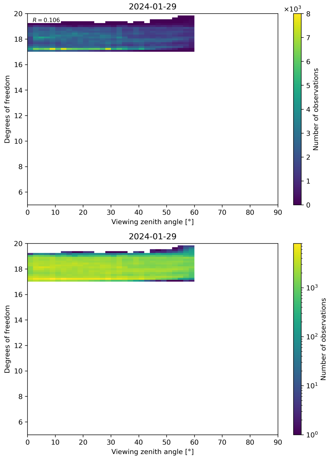
Figure 107: Scatter density plot of “Viewing zenith angle” against “Degrees of freedom” for 2024-01-28 to 2024-01-30.
