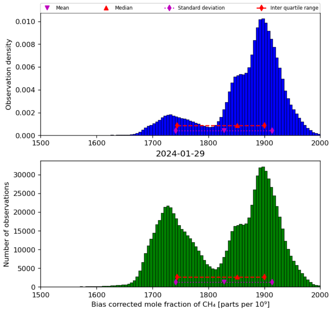
Figure 25: Histogram of “Bias corrected mole fraction of CH 4 ” for 2024-01-28 to 2024-01-30
