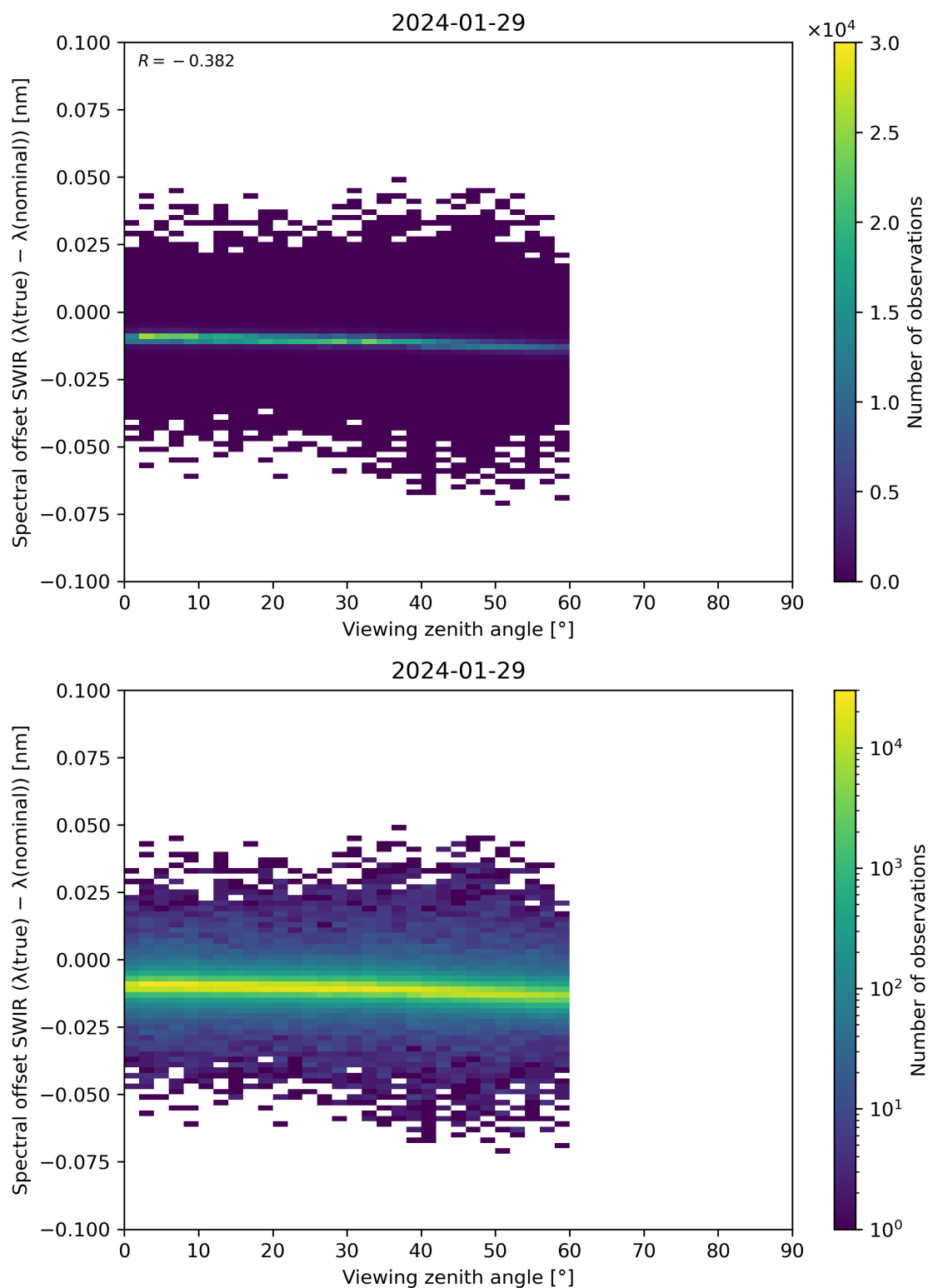
Figure 116: Scatter density plot of “Viewing zenith angle” against “Spectral offset SWIR ( \lambda(\text{true}) - \lambda(\text{nominal}) )” for 2024-01-28 to 2024-01-30.
