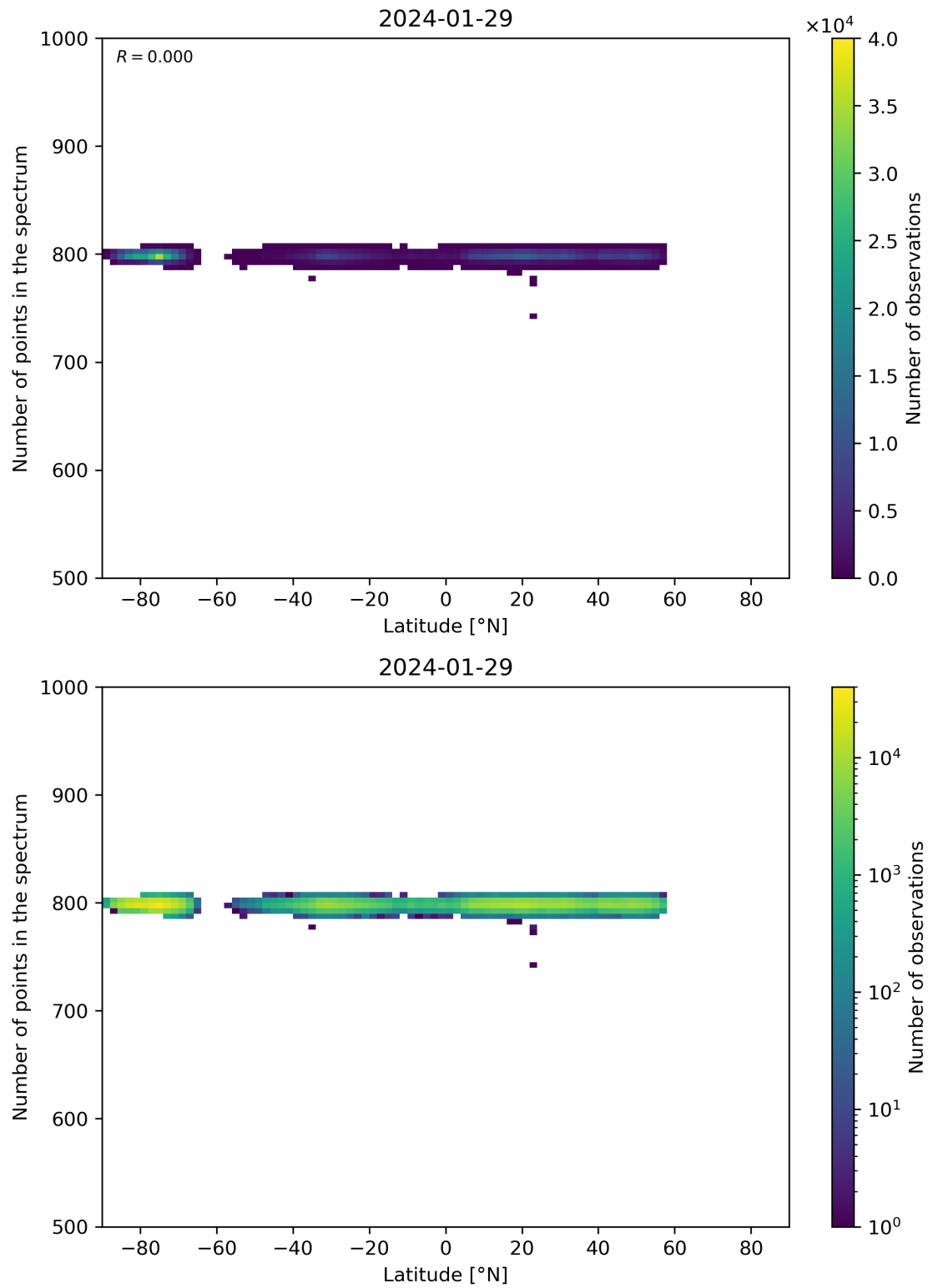
Figure 61: Scatter density plot of “Latitude” against “Number of points in the spectrum” for 2024-01-28 to 2024-01-30.
