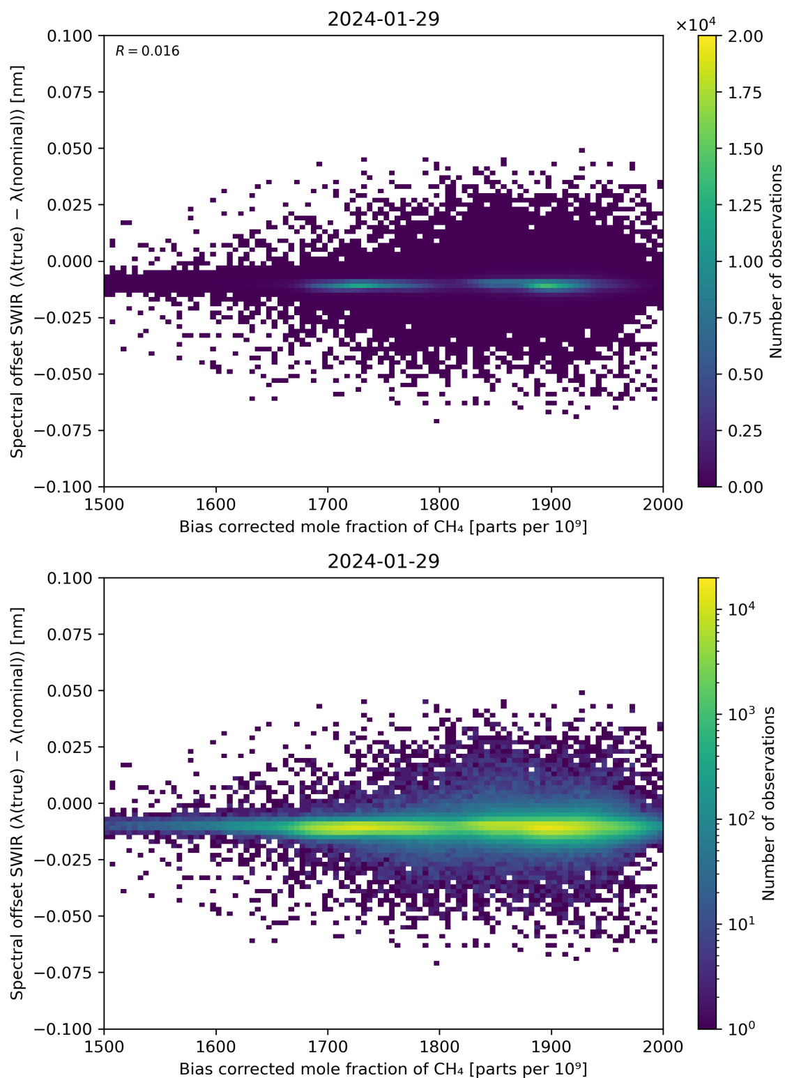
Figure 69: Scatter density plot of “Bias corrected mole fraction of \text{CH}_4 ” against “Spectral offset SWIR ( \lambda(\text{true}) - \lambda(\text{nominal}) )” for 2024-01-28 to 2024-01-30.
