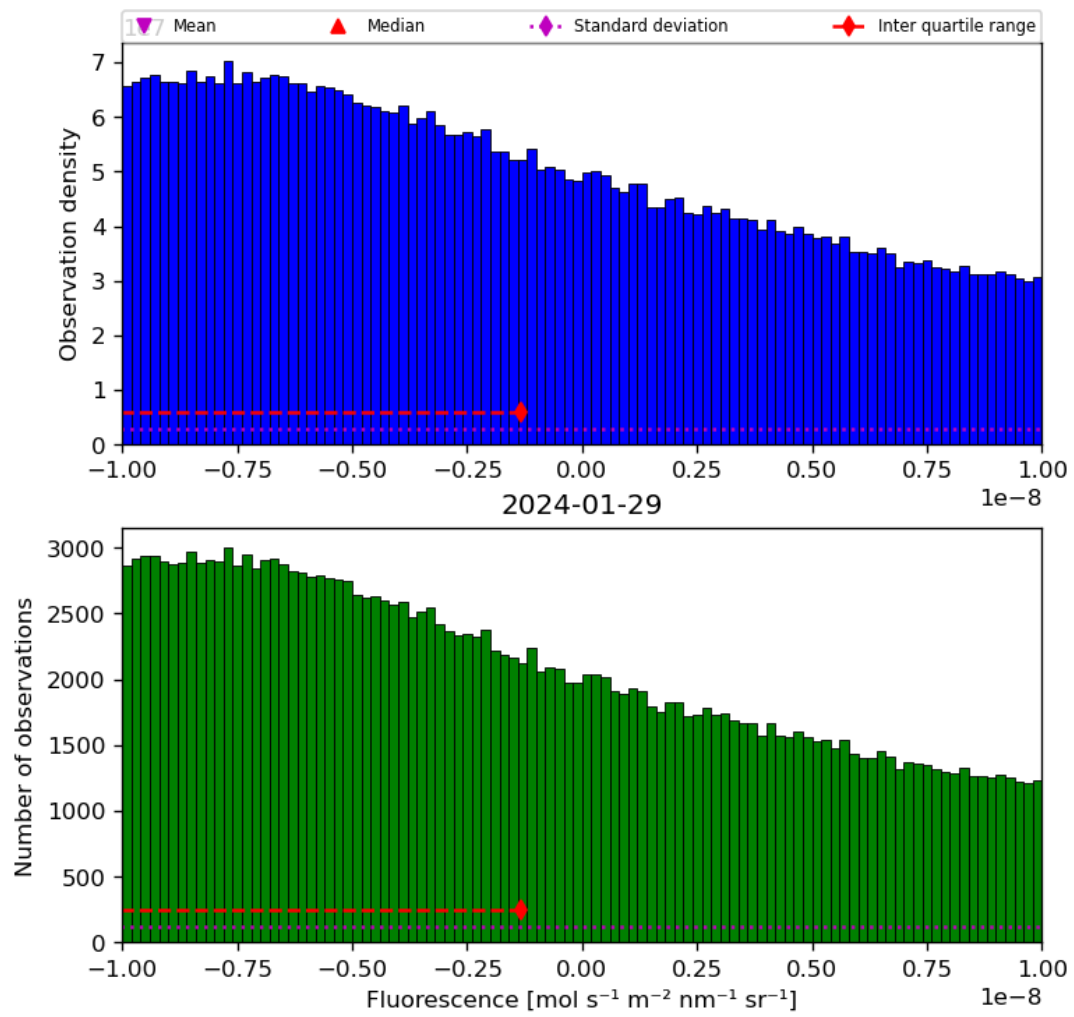
Figure 32: Histogram of “Fluorescence” for 2024-01-28 to 2024-01-30
