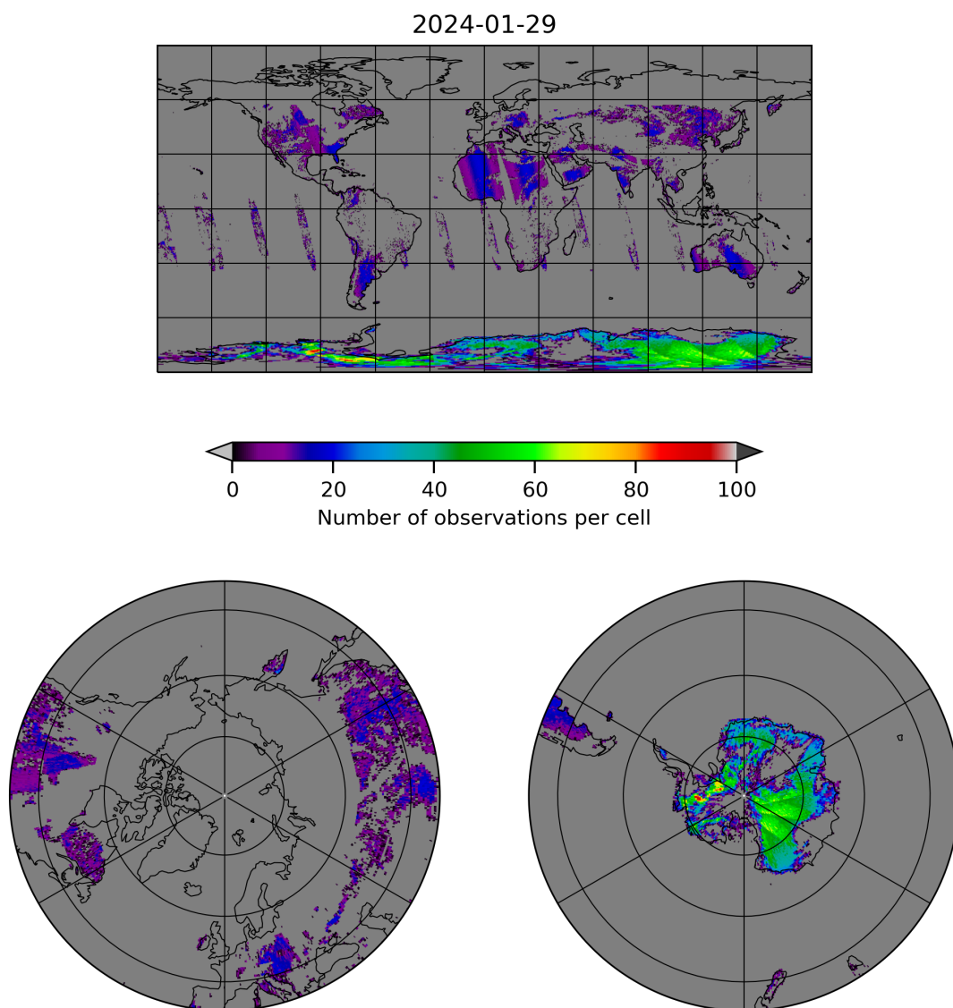
Figure 10: Map of the number of observations for 2024-01-28 to 2024-01-30
