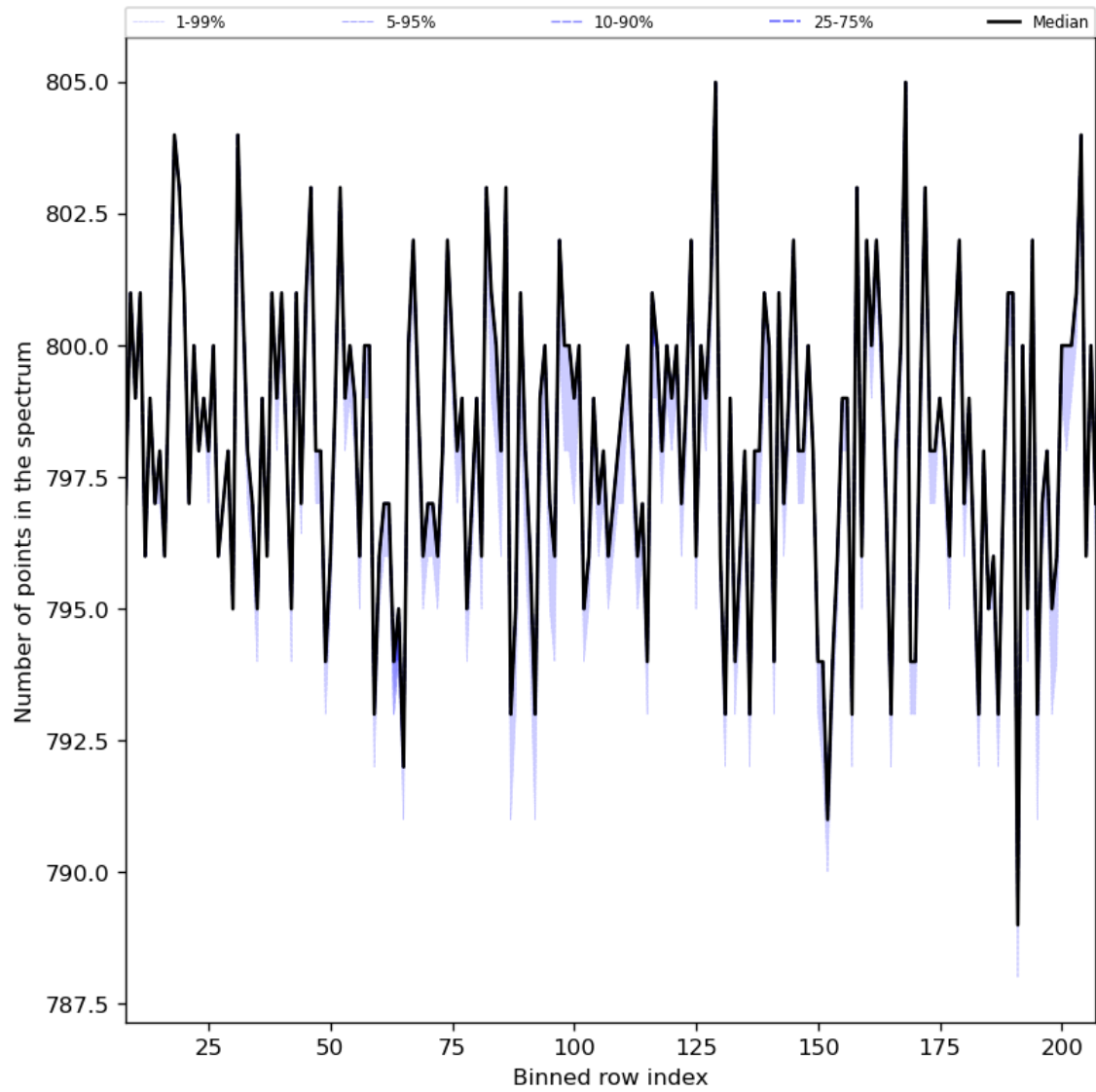
Figure 37: Along track statistics of “Number of points in the spectrum” for 2024-01-28 to 2024-01-30
