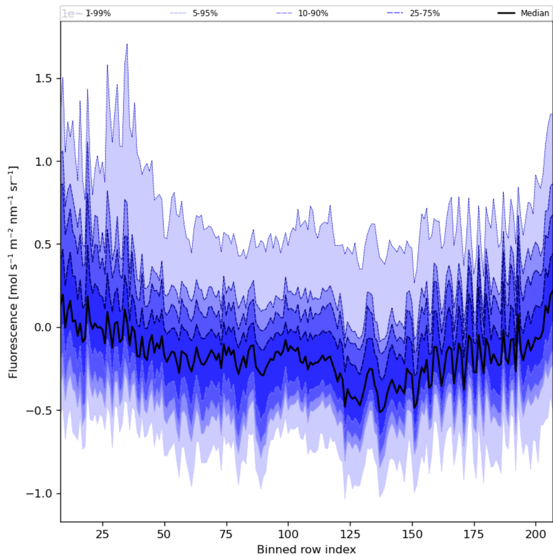
Figure 43: Along track statistics of “Fluorescence” for 2024-01-28 to 2024-01-30
