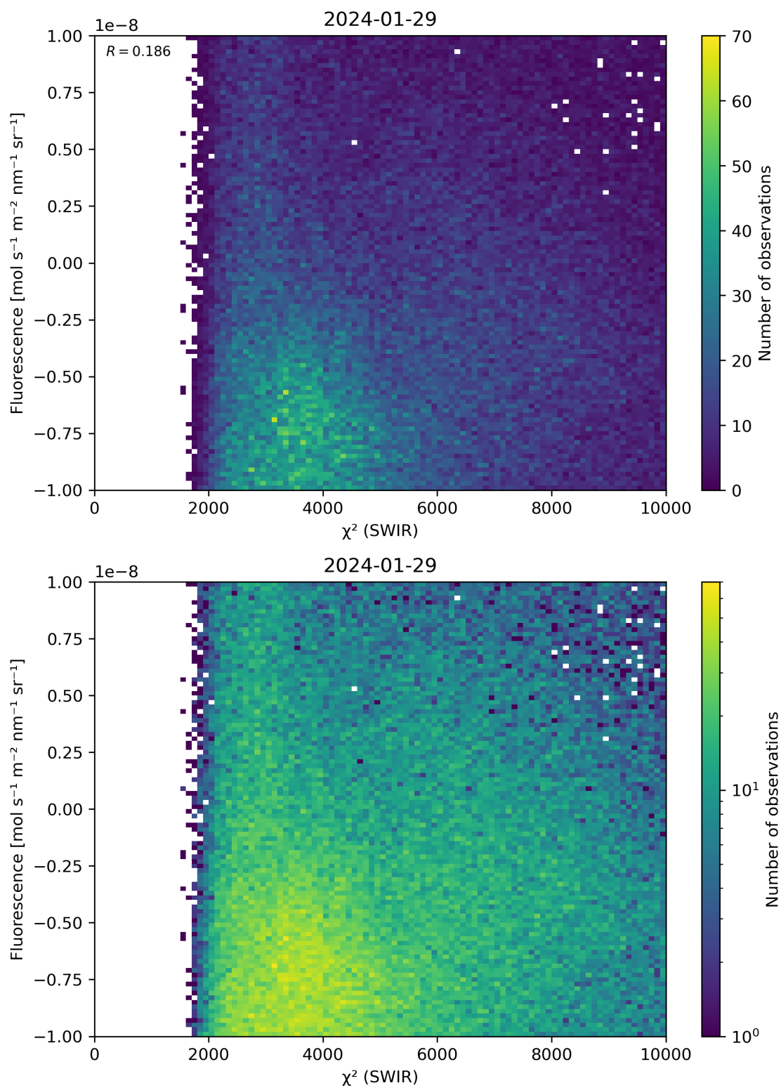
Figure 49: Scatter density plot of “ \chi^2 (SWIR)” against “Fluorescence” for 2024-01-28 to 2024-01-30.
