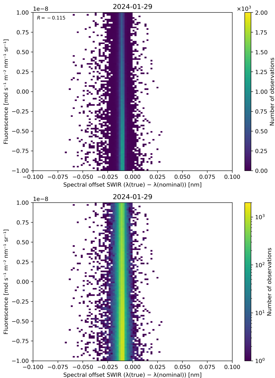
Figure 120: Scatter density plot of “Spectral offset SWIR ( \lambda(\text{true}) - \lambda(\text{nominal}) )” against “Fluorescence” for 2024-01-28 to 2024-01-30.
