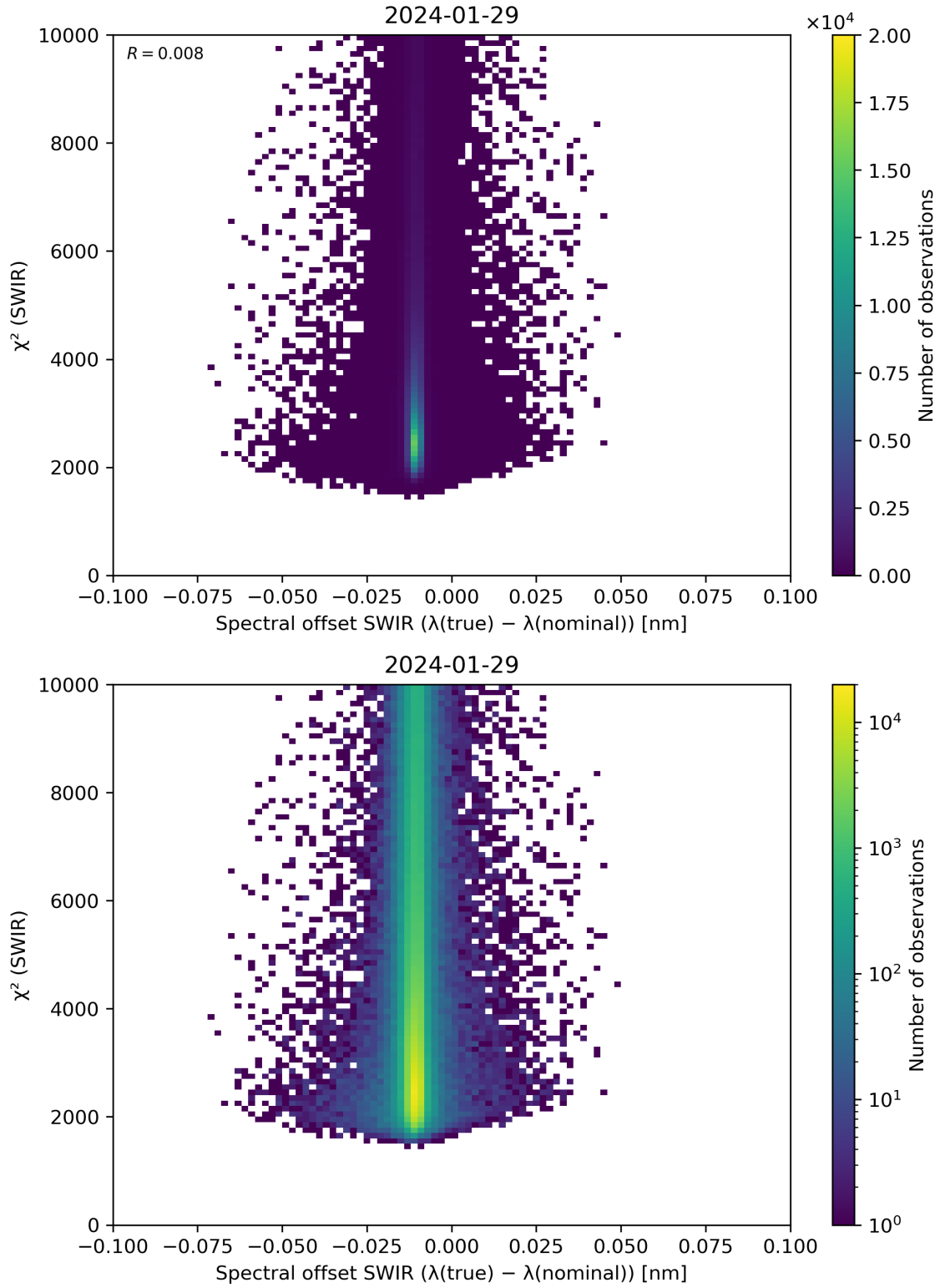
Figure 118: Scatter density plot of “Spectral offset SWIR ( \lambda(\text{true}) - \lambda(\text{nominal}) )” against “ \chi^2 (SWIR)” for 2024-01-28 to 2024-01-30.
