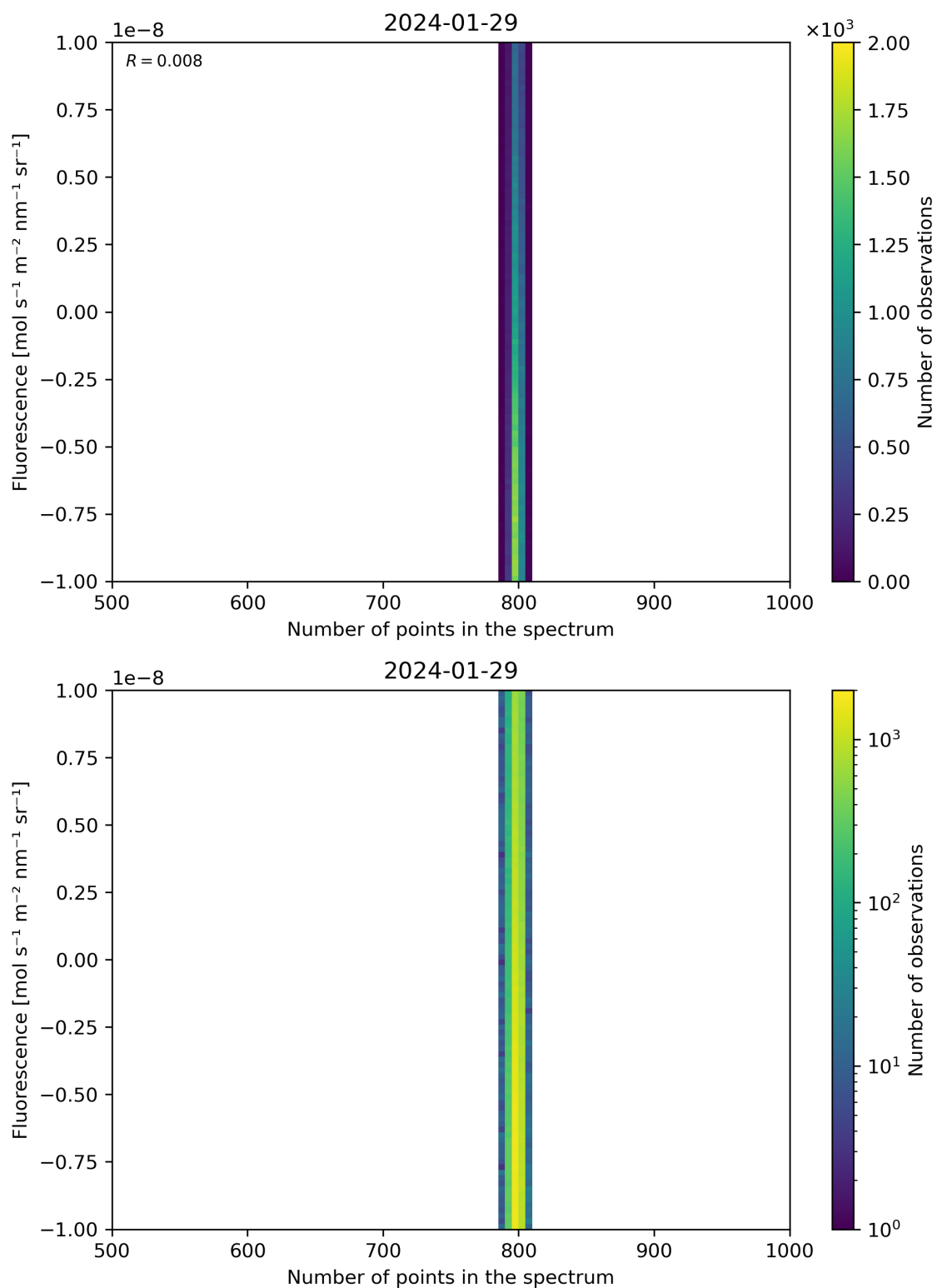
Figure 91: Scatter density plot of “Number of points in the spectrum” against “Fluorescence” for 2024-01-28 to 2024-01-30.
