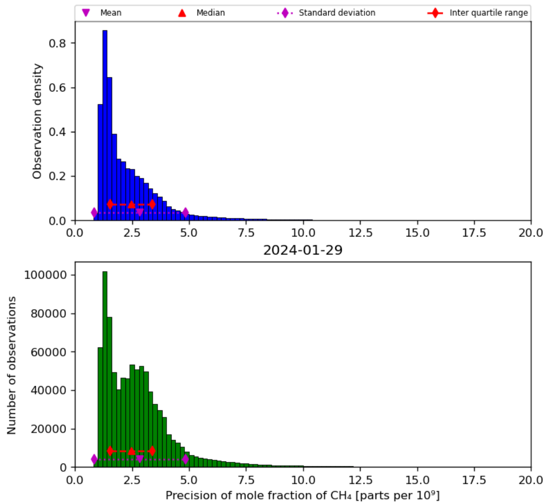
Figure 24: Histogram of “Precision of mole fraction of CH 4 ” for 2024-01-28 to 2024-01-30
