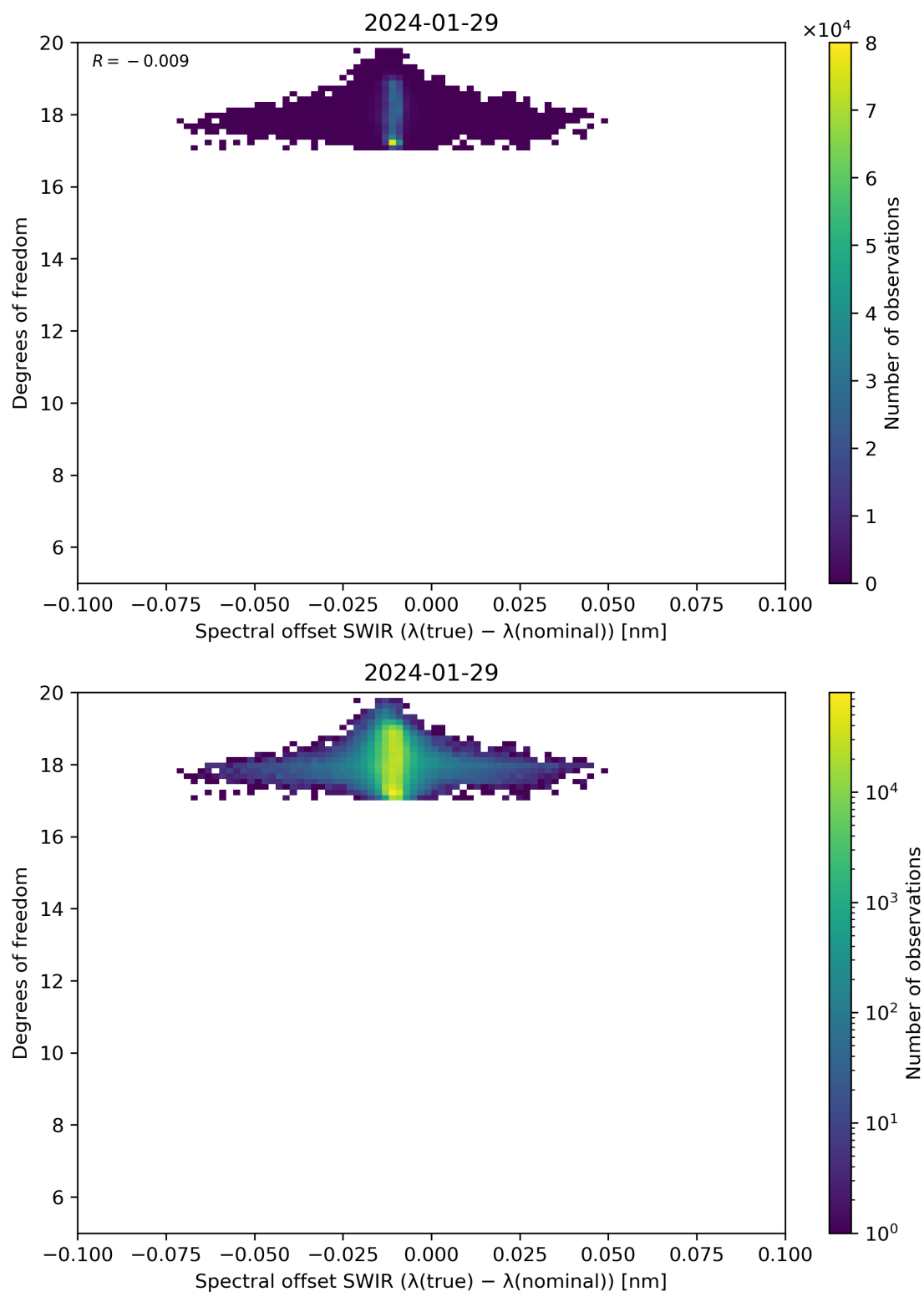
Figure 119: Scatter density plot of “Spectral offset SWIR ( \lambda(\text{true}) - \lambda(\text{nominal}) )” against “Degrees of freedom” for 2024-01-28 to 2024-01-30.
