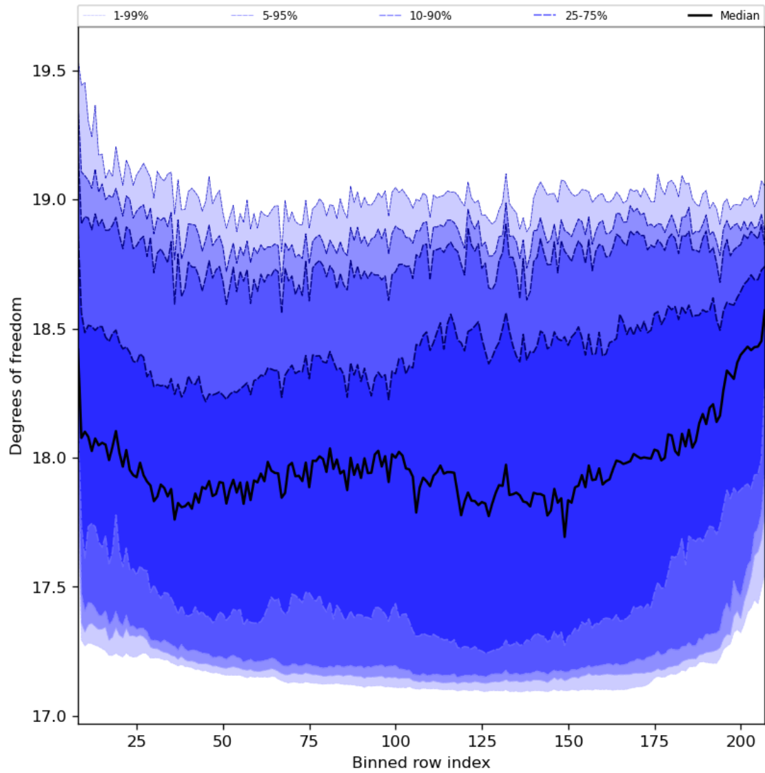
Figure 41: Along track statistics of “Degrees of freedom” for 2024-01-28 to 2024-01-30
