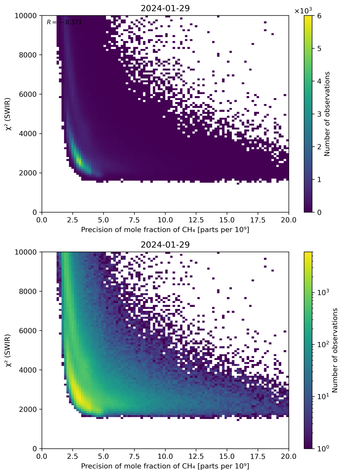
Figure 79: Scatter density plot of “Precision of mole fraction of CH 4 ” against “ \chi^2 (SWIR)” for 2024-01-28 to 2024-01-30.
