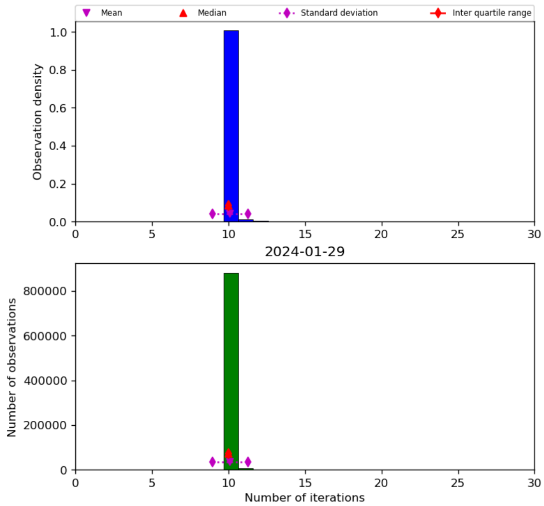
Figure 31: Histogram of “Number of iterations” for 2024-01-28 to 2024-01-30
