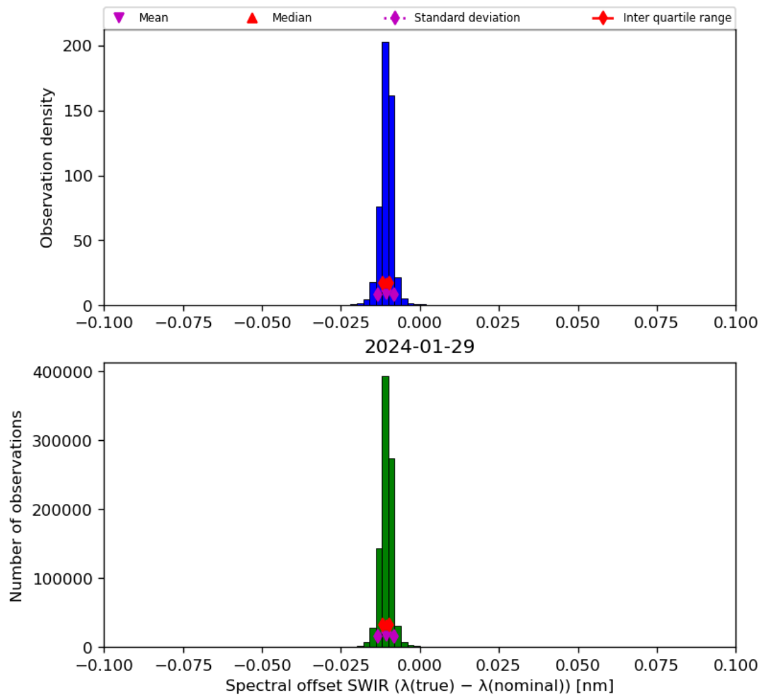
Figure 27: Histogram of “Spectral offset SWIR ( \lambda(\text{true}) - \lambda(\text{nominal}) )” for 2024-01-28 to 2024-01-30
