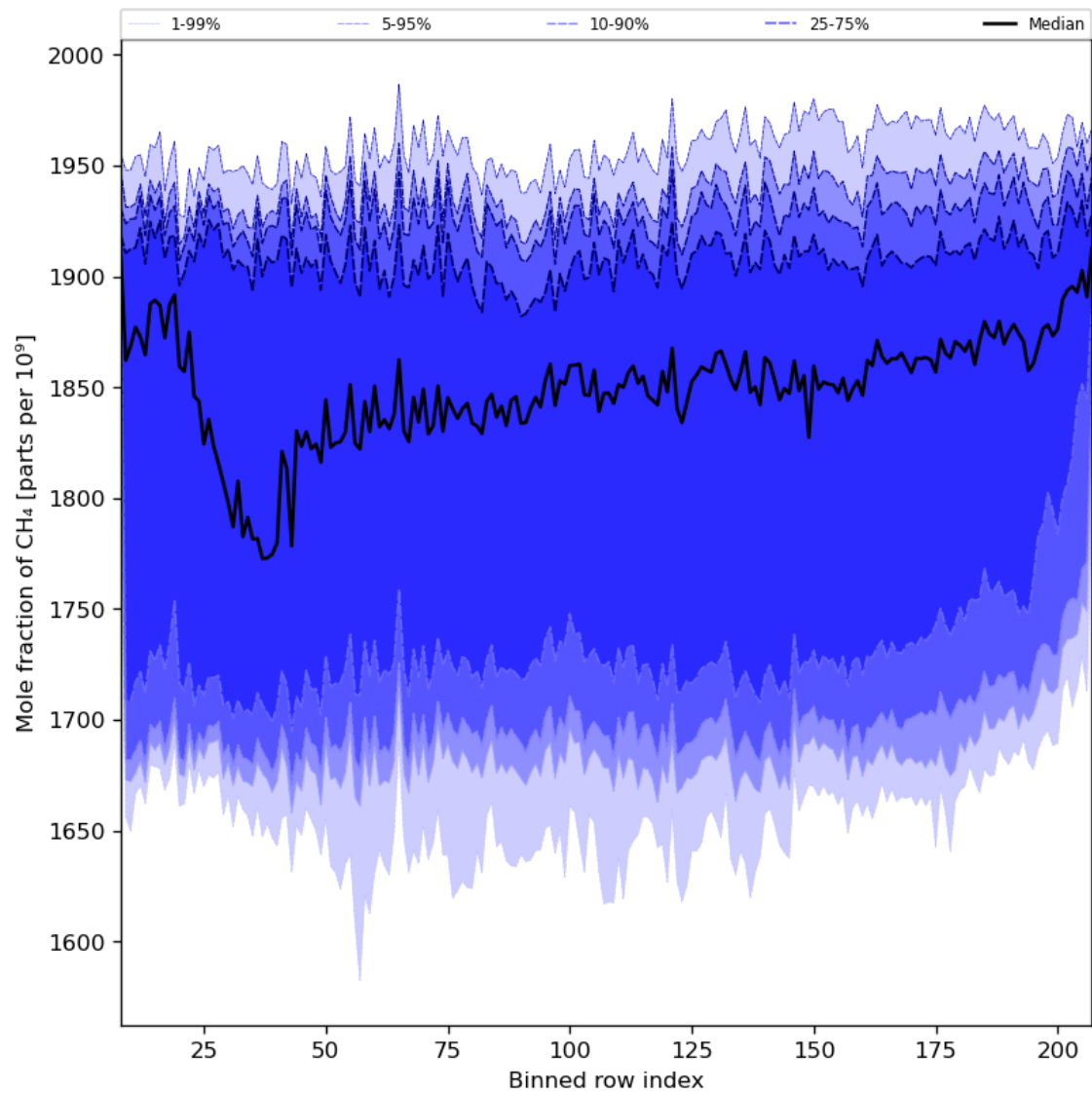
Figure 34: Along track statistics of “Mole fraction of CH 4 ” for 2024-01-28 to 2024-01-30
