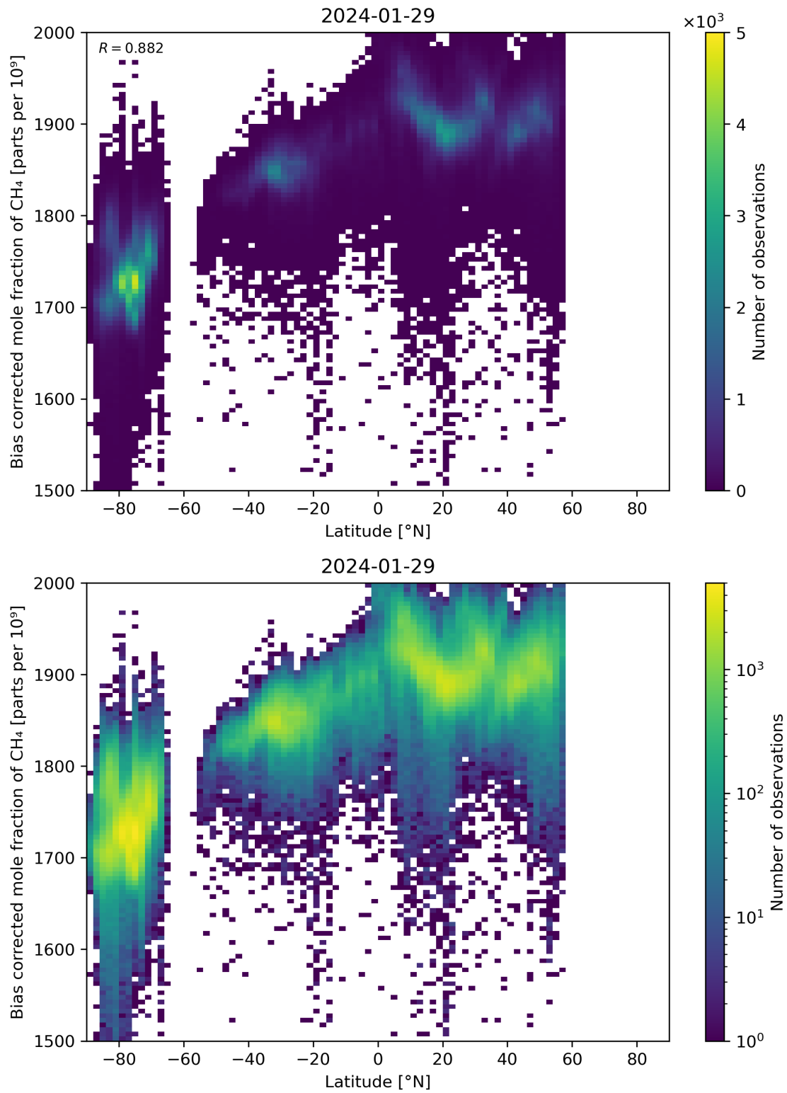
Figure 58: Scatter density plot of “Latitude” against “Bias corrected mole fraction of \text{CH}_4 ” for 2024-01-28 to 2024-01-30.
