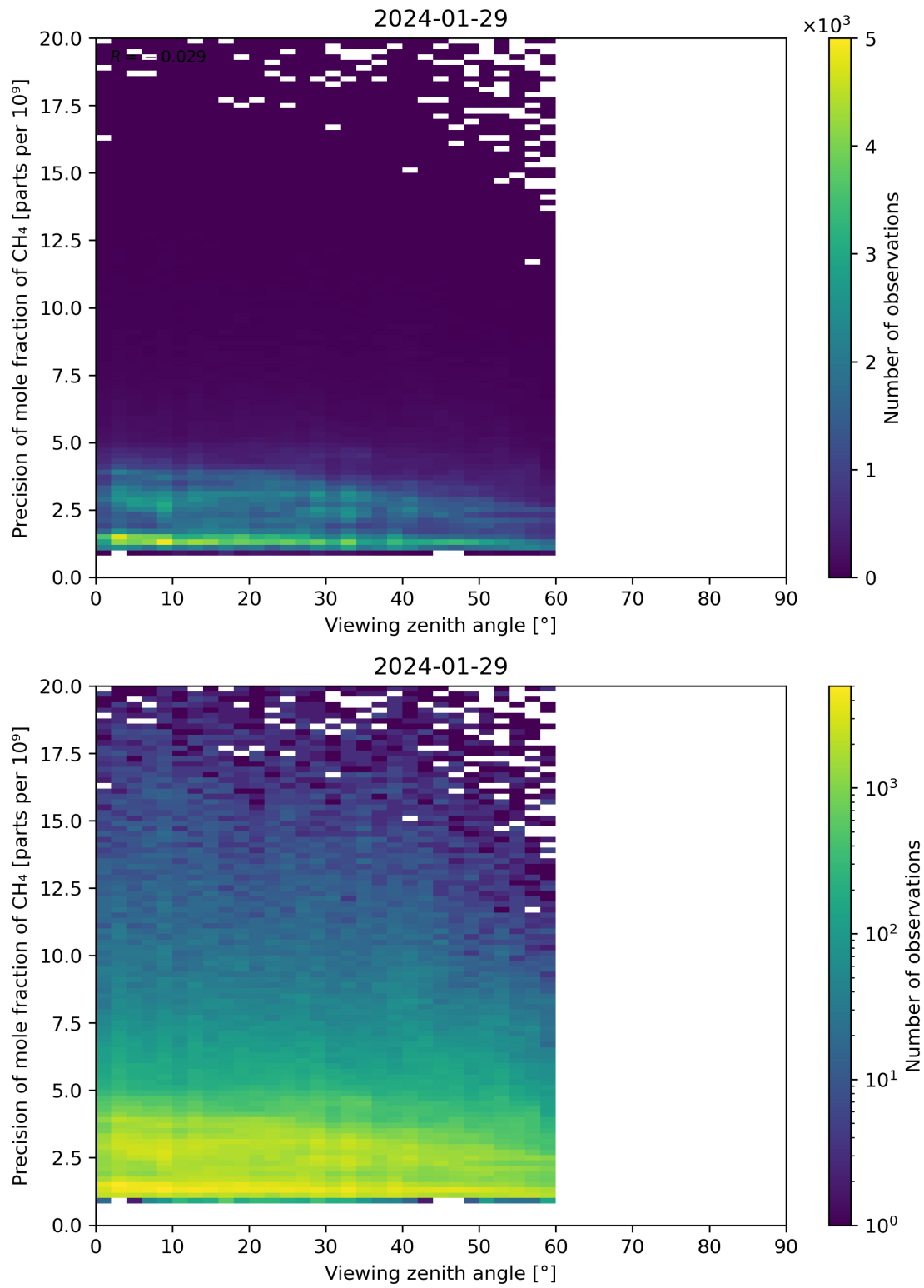
Figure 112: Scatter density plot of “Viewing zenith angle” against “Precision of mole fraction of CH 4 ” for 2024-01-28 to 2024-01-30.
