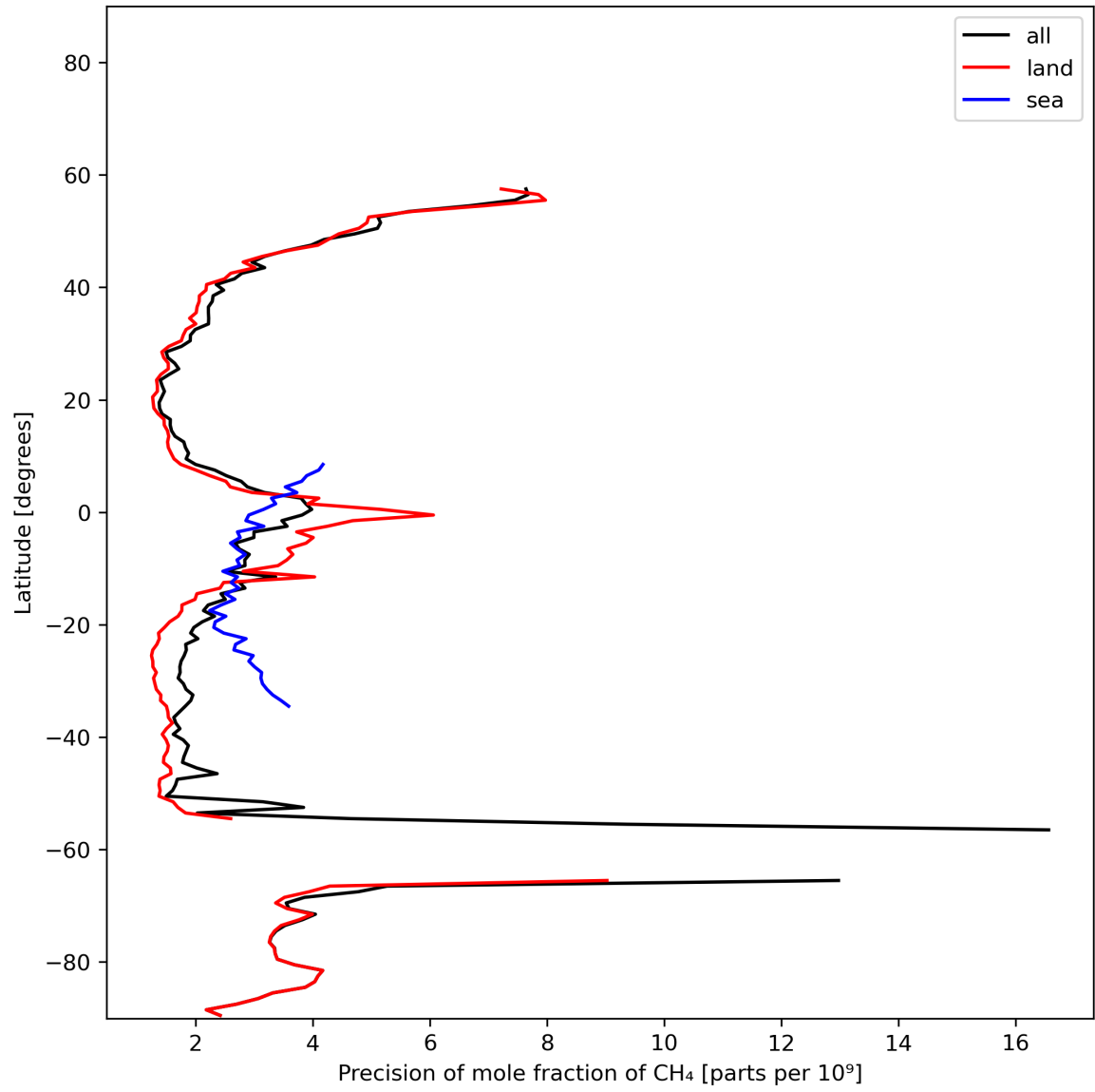
Figure 13: Zonal average of “Precision of mole fraction of CH 4 ” for 2024-01-28 to 2024-01-30.
