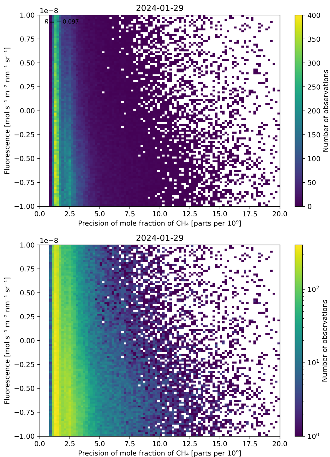
Figure 81: Scatter density plot of “Precision of mole fraction of \text{CH}_4 ” against “Fluorescence” for 2024-01-28 to 2024-01-30.
