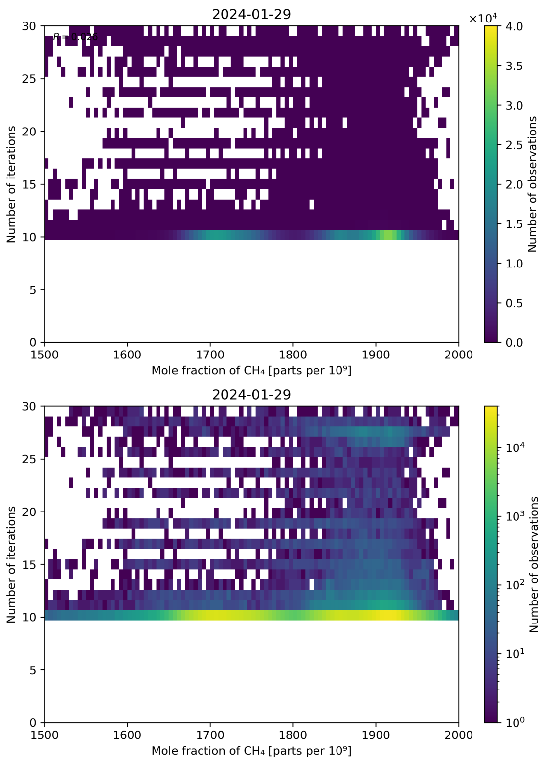
Figure 76: Scatter density plot of “Mole fraction of CH 4 ” against “Number of iterations” for 2024-01-28 to 2024-01-30.
