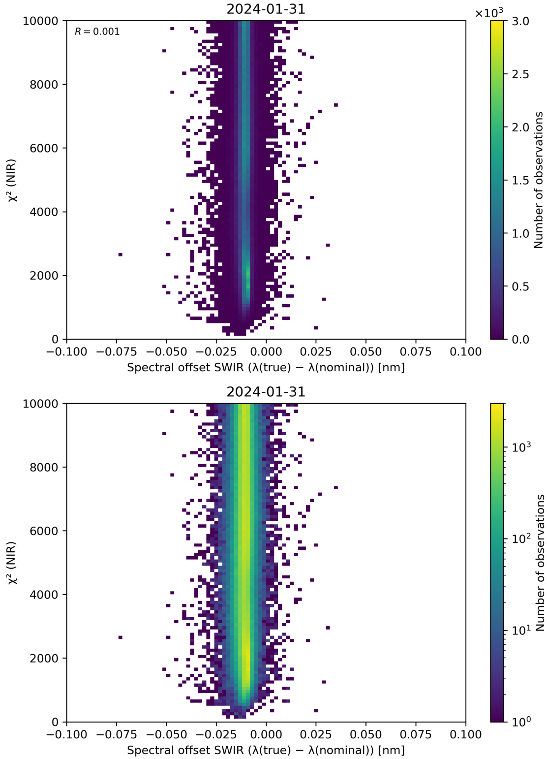
Figure 117: Scatter density plot of “Spectral offset SWIR ( \lambda(\text{true}) - \lambda(\text{nominal}) )” against “ \chi^2 (NIR)” for 2024-01-31 to 2024-02-01.
