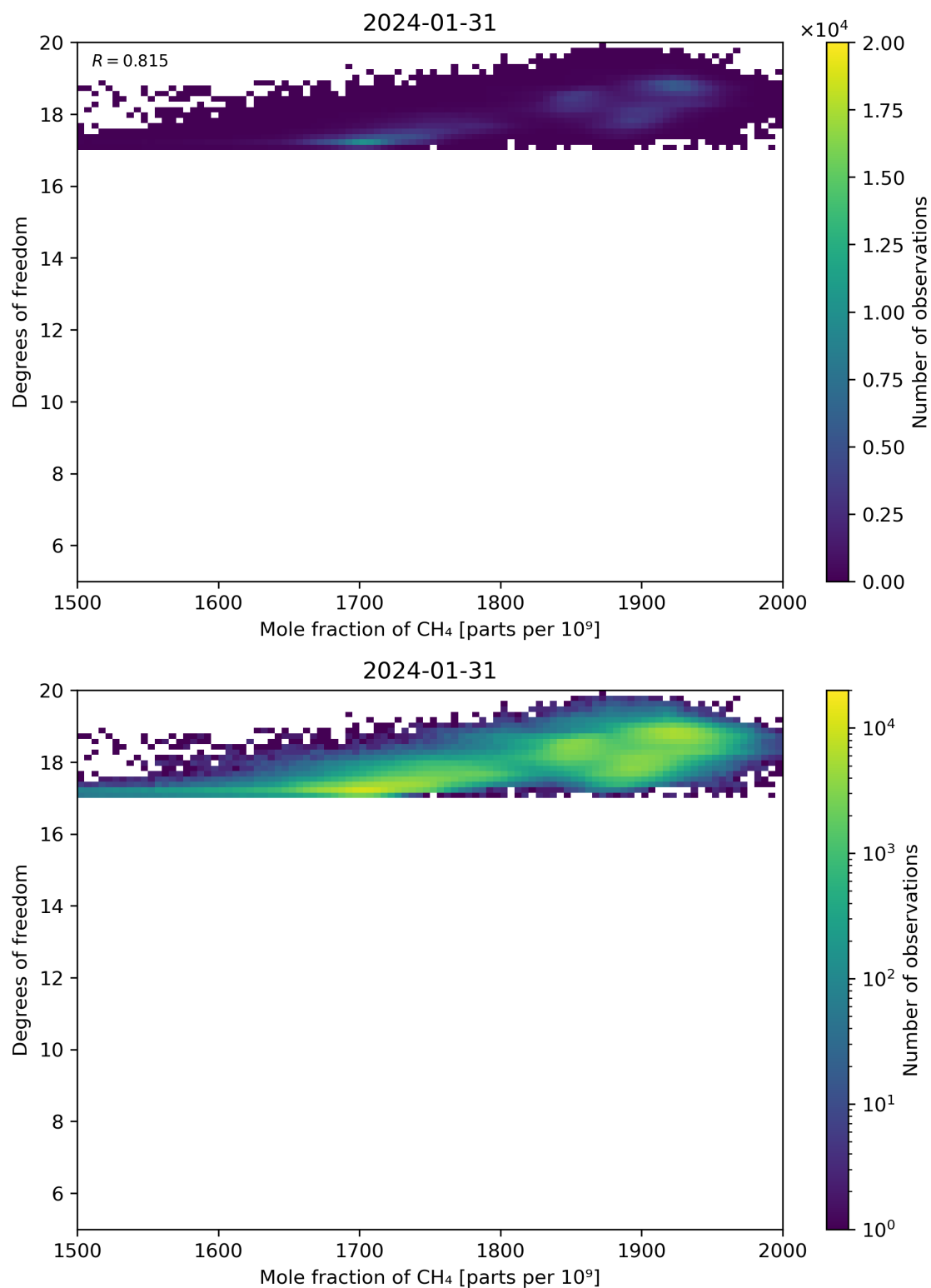
Figure 72: Scatter density plot of “Mole fraction of CH 4 ” against “Degrees of freedom” for 2024-01-31 to 2024-02-01.
