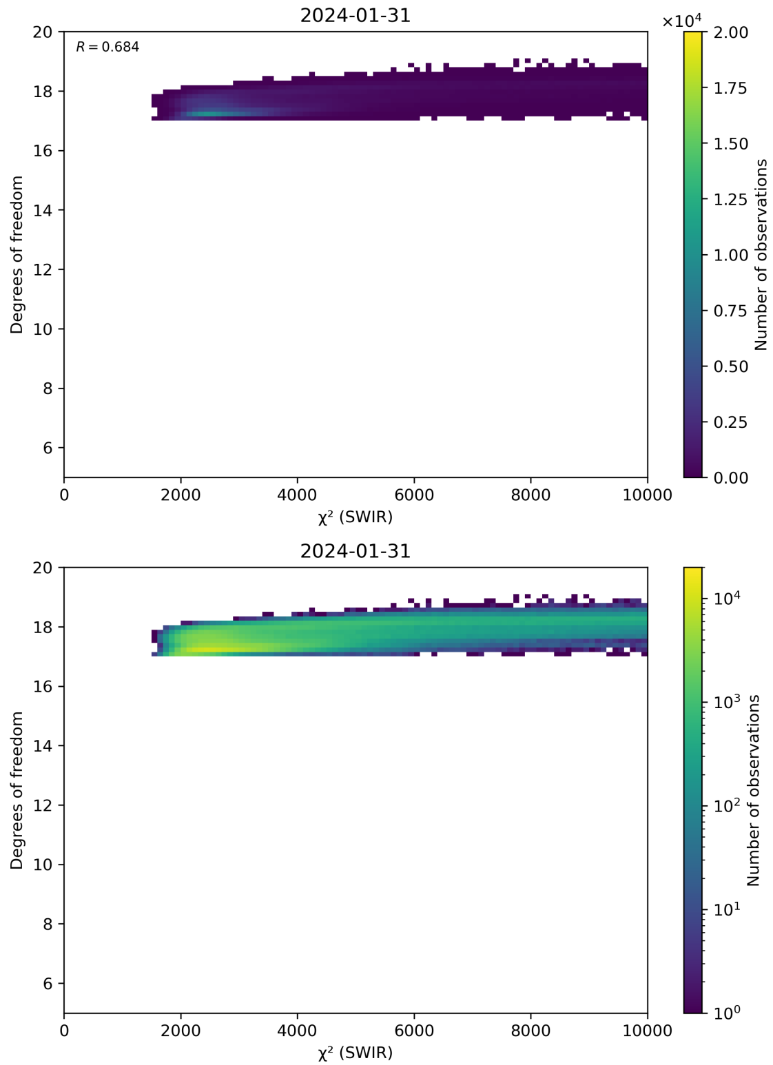
Figure 48: Scatter density plot of " \chi^2 (SWIR)" against "Degrees of freedom" for 2024-01-31 to 2024-02-01.
