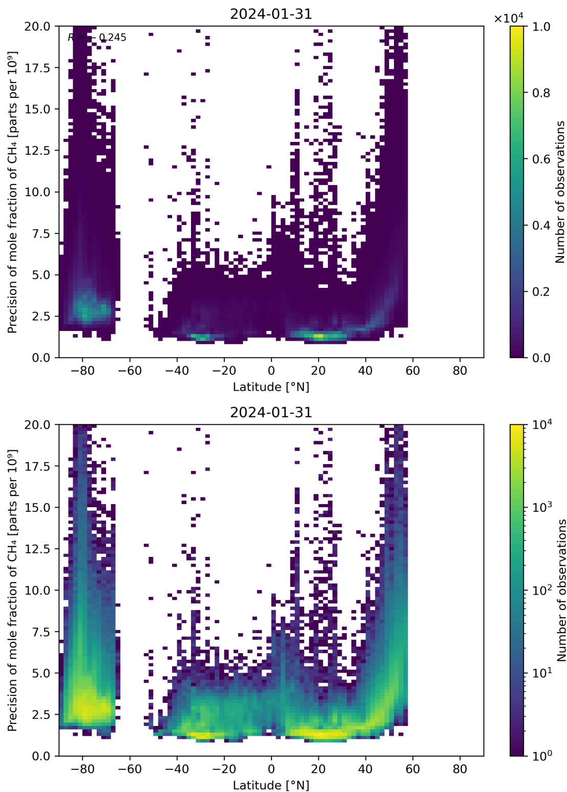
Figure 59: Scatter density plot of “Latitude” against “Precision of mole fraction of CH 4 ” for 2024-01-31 to 2024-02-01.
