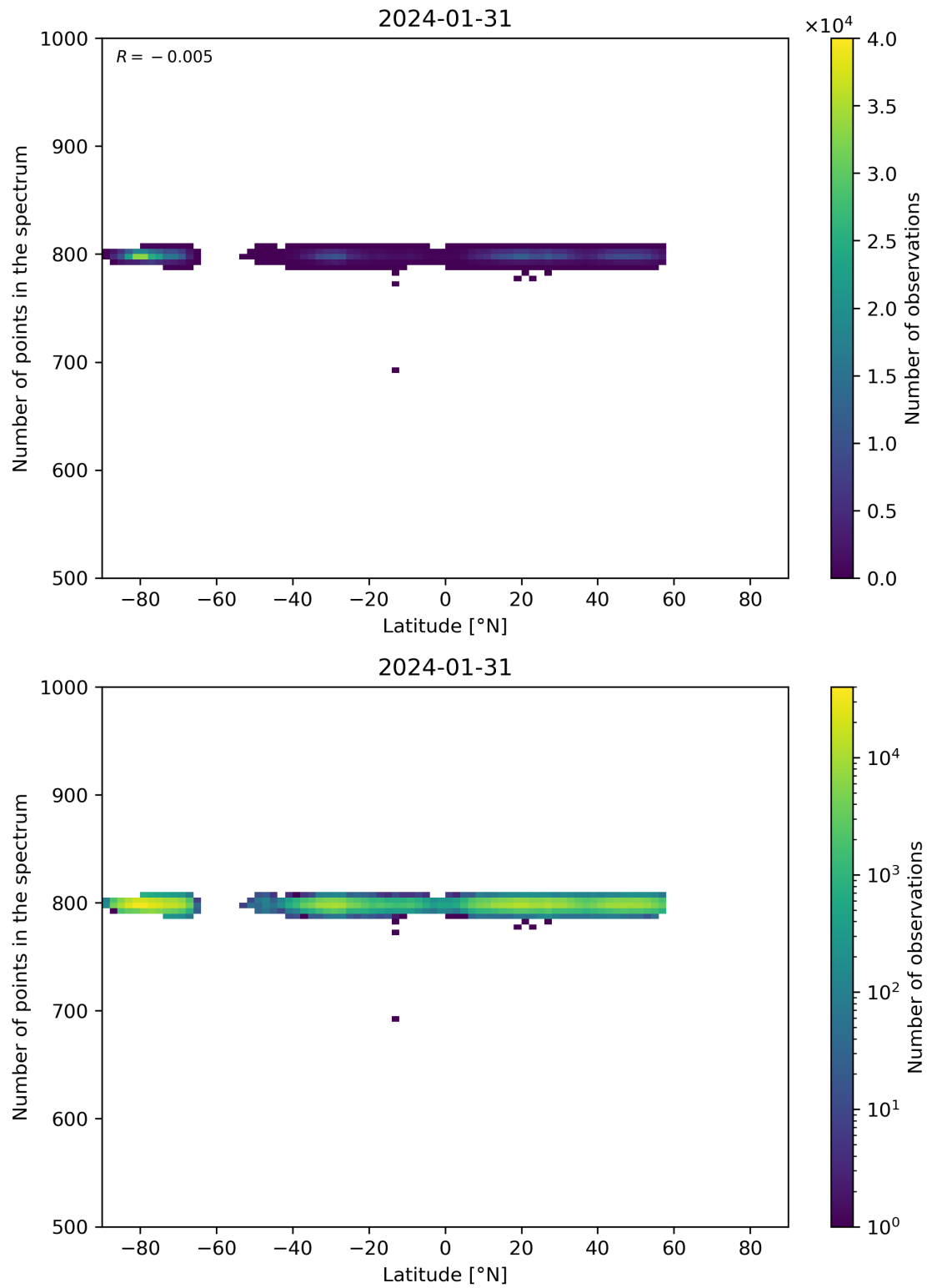
Figure 61: Scatter density plot of “Latitude” against “Number of points in the spectrum” for 2024-01-31 to 2024-02-01.
