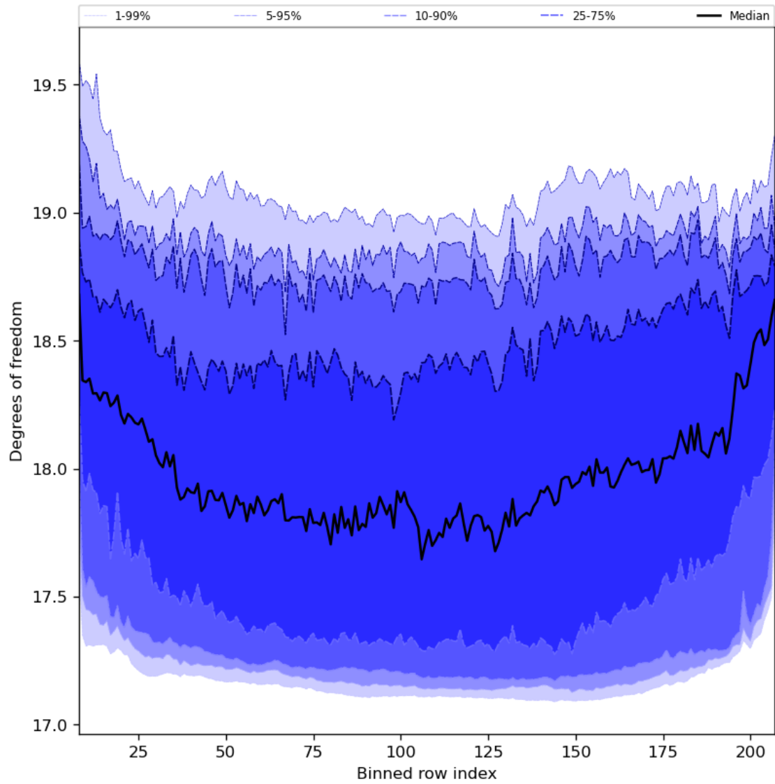
Figure 41: Along track statistics of “Degrees of freedom” for 2024-01-31 to 2024-02-01
