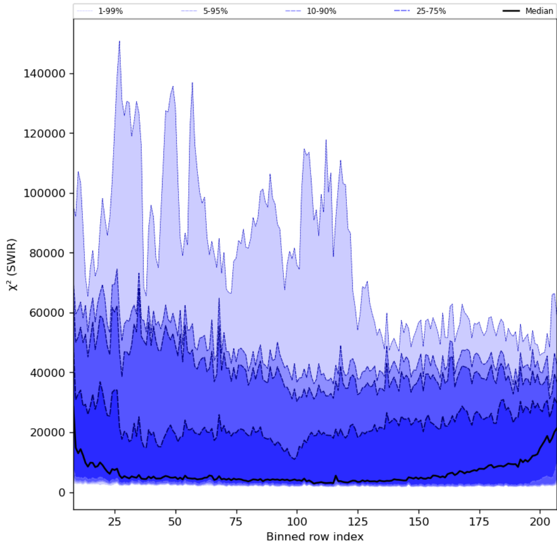
Figure 39: Along track statistics of “ \chi^2 (SWIR)” for 2024-01-31 to 2024-02-01
