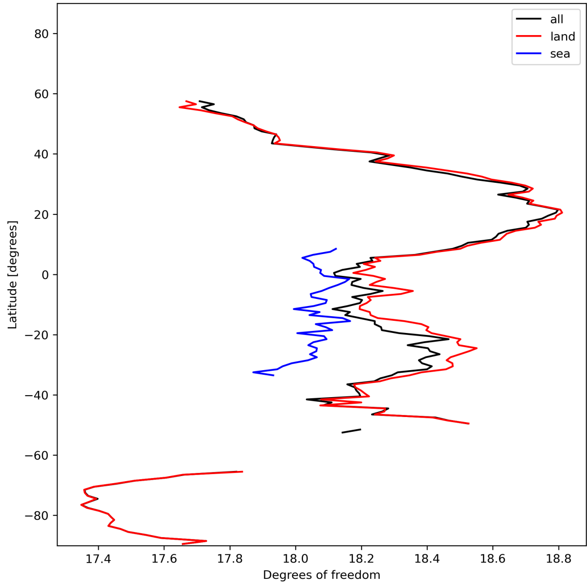
Figure 19: Zonal average of “Degrees of freedom” for 2024-01-31 to 2024-02-01.
