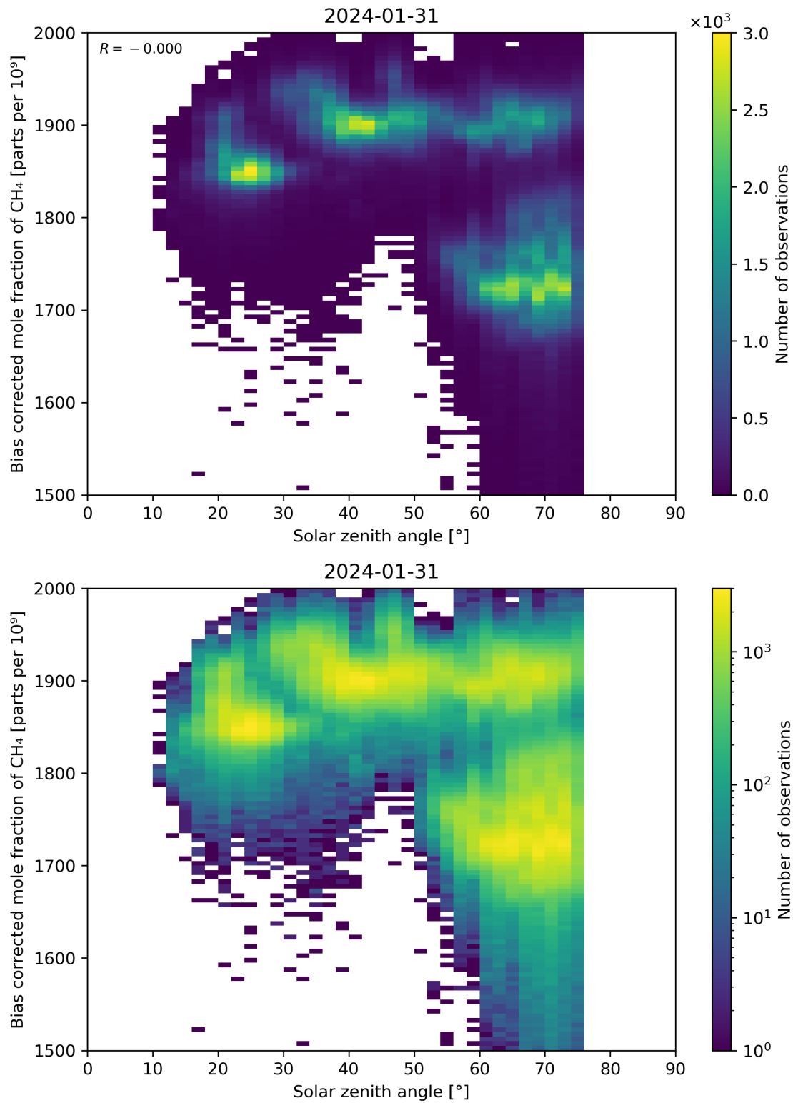
Figure 100: Scatter density plot of “Solar zenith angle” against “Bias corrected mole fraction of CH 4 ” for 2024-01-31 to 2024-02-01.
