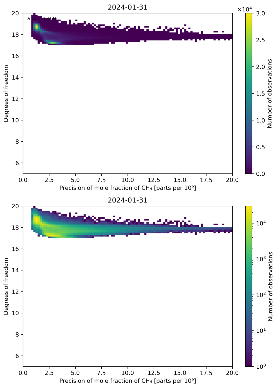
Figure 80: Scatter density plot of “Precision of mole fraction of CH 4 ” against “Degrees of freedom” for 2024-01-31 to 2024-02-01.
