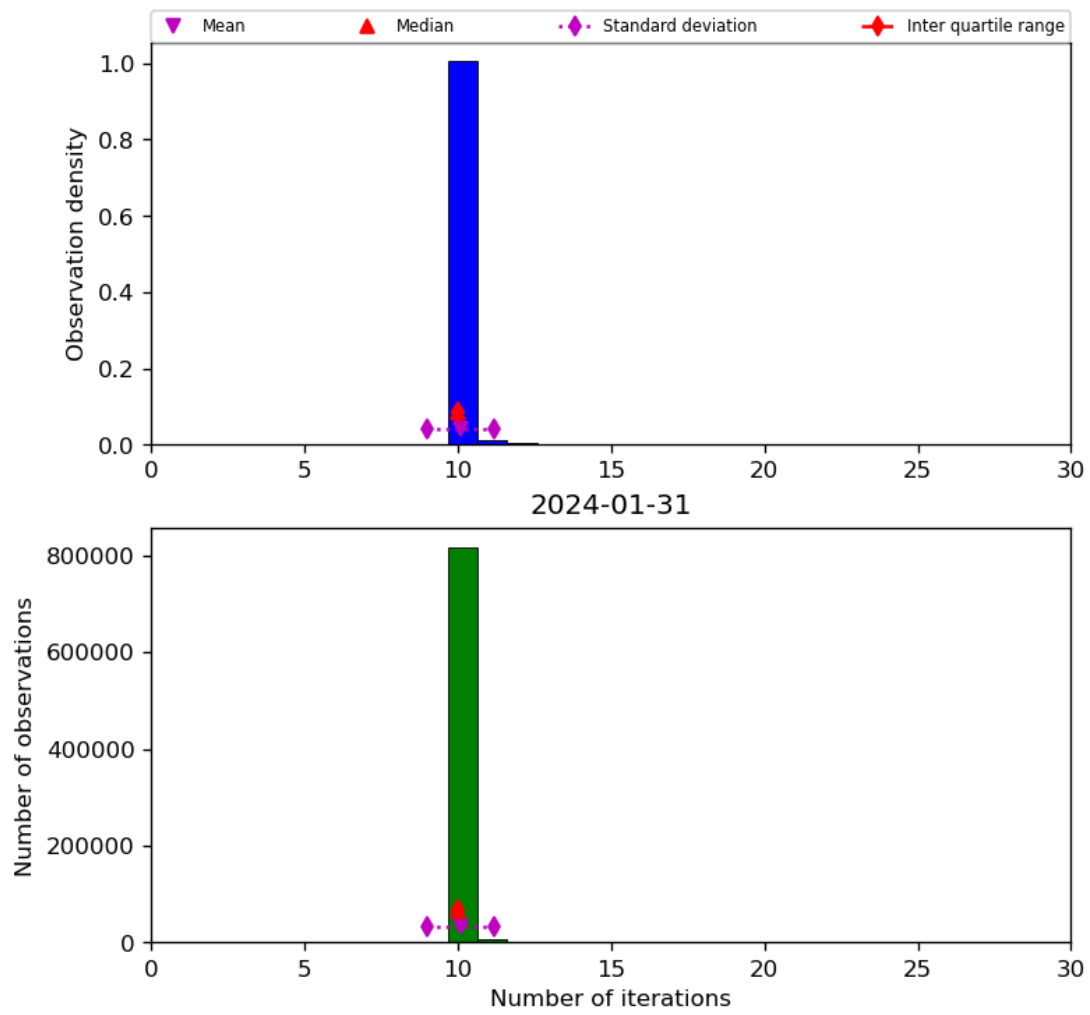
Figure 31: Histogram of “Number of iterations” for 2024-01-31 to 2024-02-01
