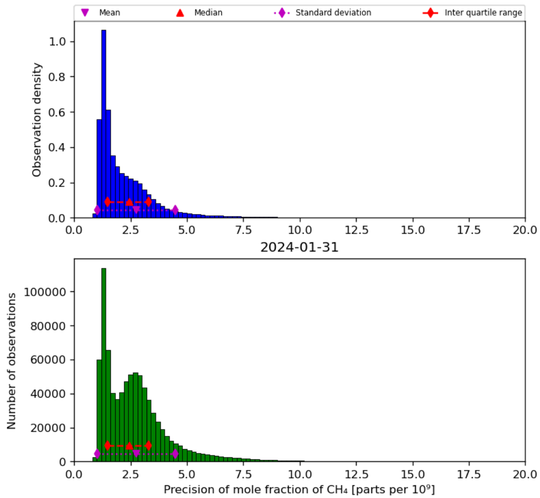
Figure 24: Histogram of “Precision of mole fraction of CH 4 ” for 2024-01-31 to 2024-02-01
