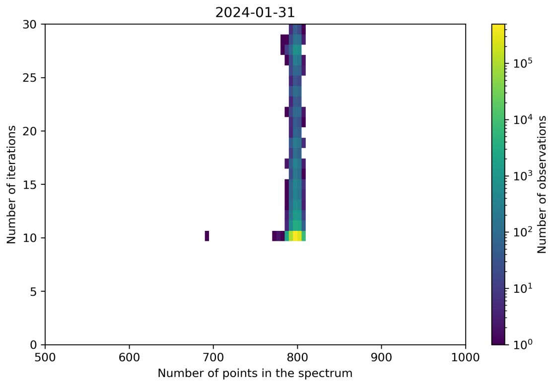
Figure 92: Scatter density plot of “Number of points in the spectrum” against “Number of iterations” for 2024-01-31 to 2024-02-01.
