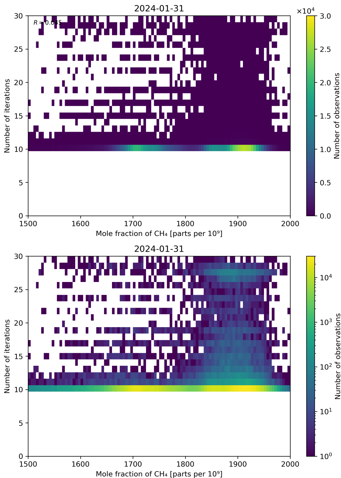
Figure 76: Scatter density plot of “Mole fraction of CH 4 ” against “Number of iterations” for 2024-01-31 to 2024-02-01.
