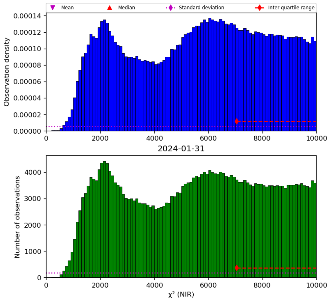
Figure 29: Histogram of “ \chi^2 (NIR)” for 2024-01-31 to 2024-02-01
