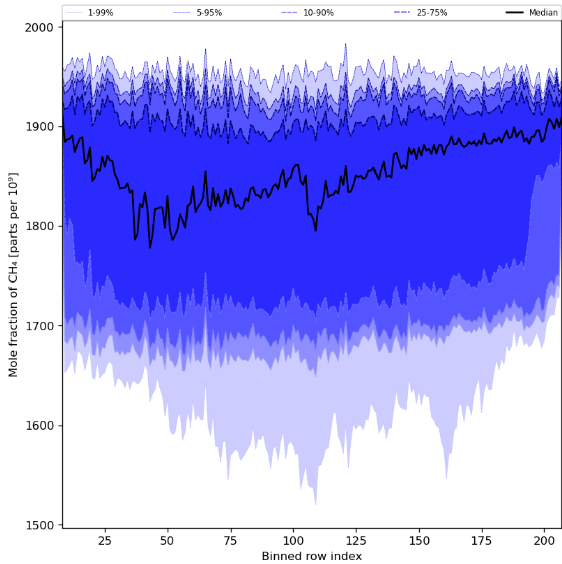
Figure 34: Along track statistics of “Mole fraction of CH 4 ” for 2024-01-31 to 2024-02-01
