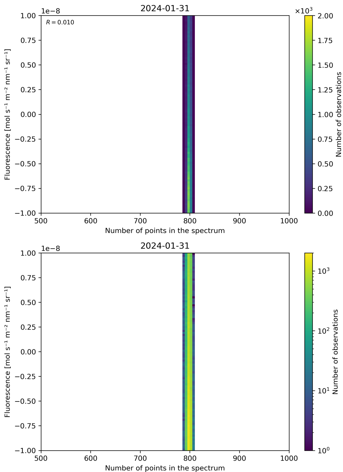
Figure 91: Scatter density plot of “Number of points in the spectrum” against “Fluorescence” for 2024-01-31 to 2024-02-01.
