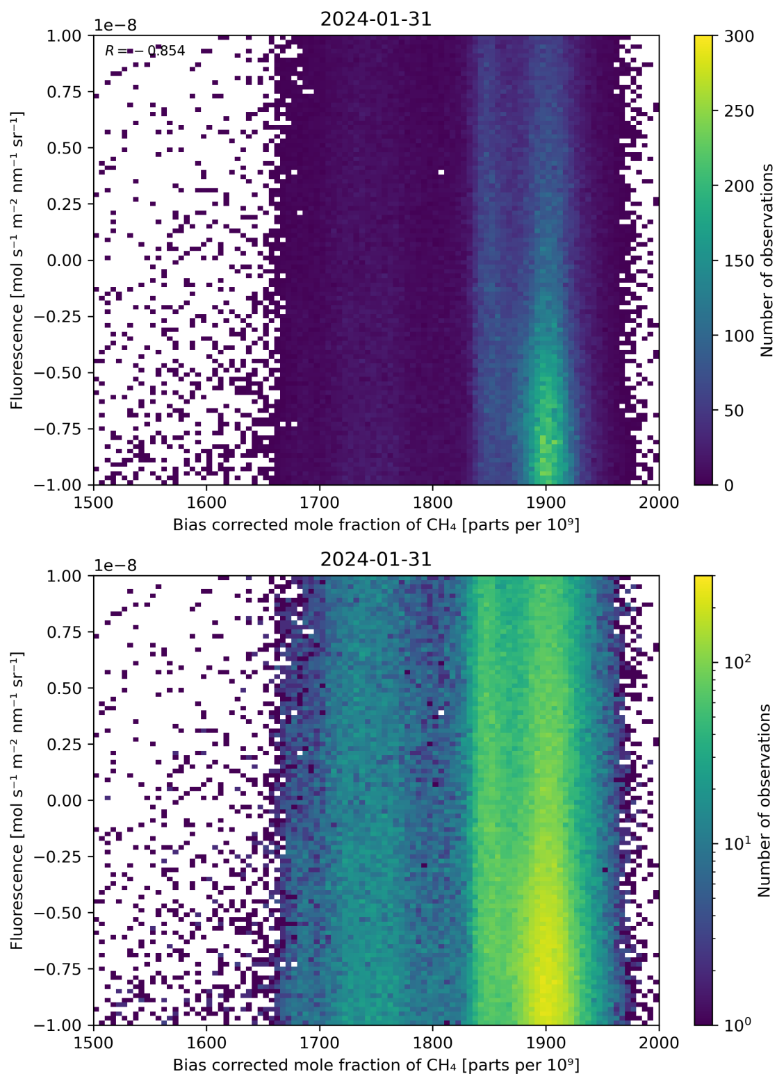
Figure 66: Scatter density plot of “Bias corrected mole fraction of CH 4 ” against “Fluorescence” for 2024-01-31 to 2024-02-01.
