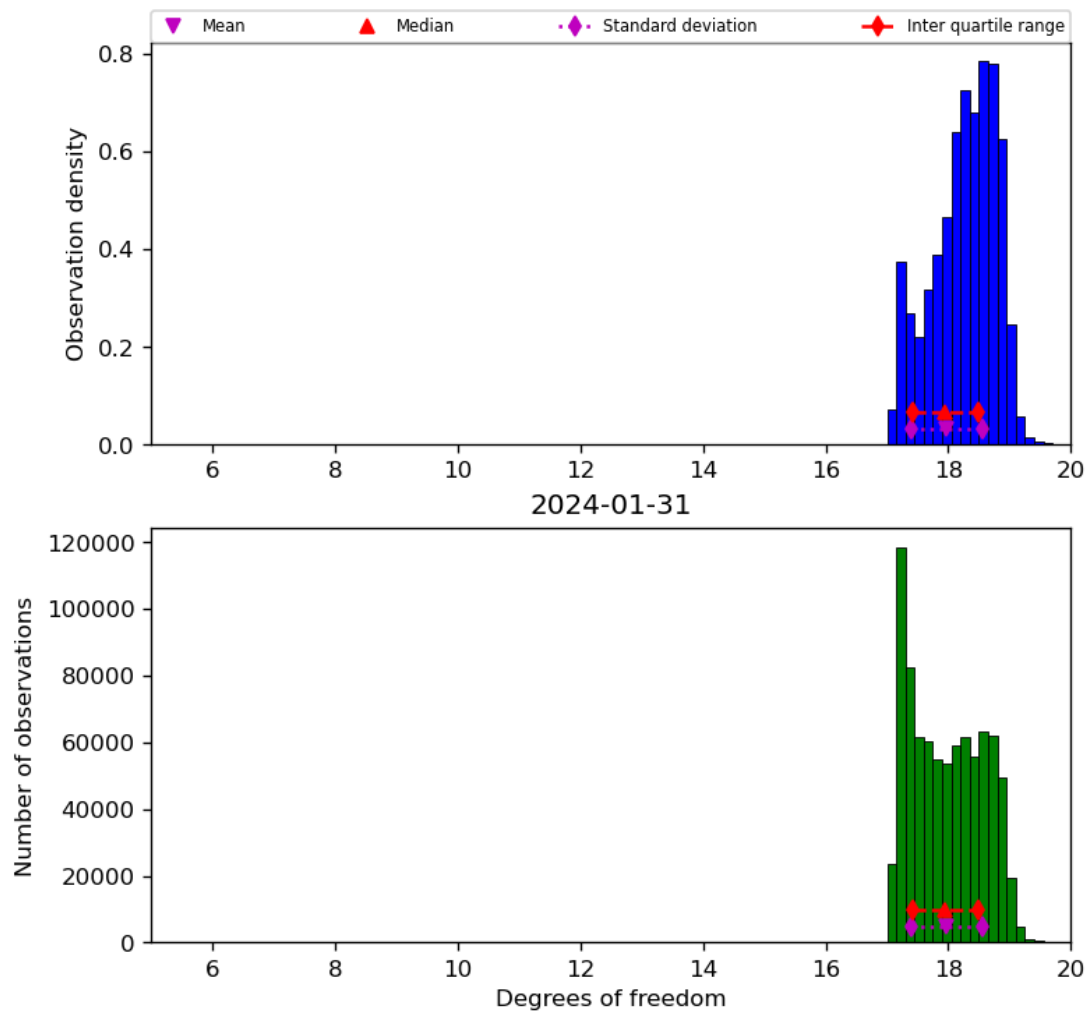
Figure 30: Histogram of “Degrees of freedom” for 2024-01-31 to 2024-02-01
