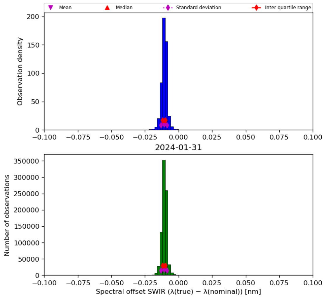
Figure 27: Histogram of “Spectral offset SWIR ( \lambda(\text{true}) - \lambda(\text{nominal}) )” for 2024-01-31 to 2024-02-01
