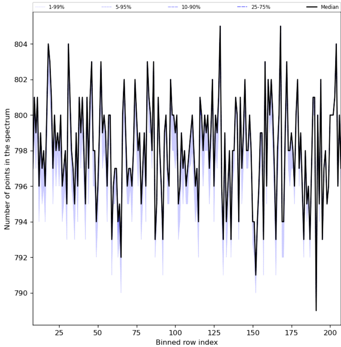
Figure 37: Along track statistics of “Number of points in the spectrum” for 2024-01-31 to 2024-02-01
