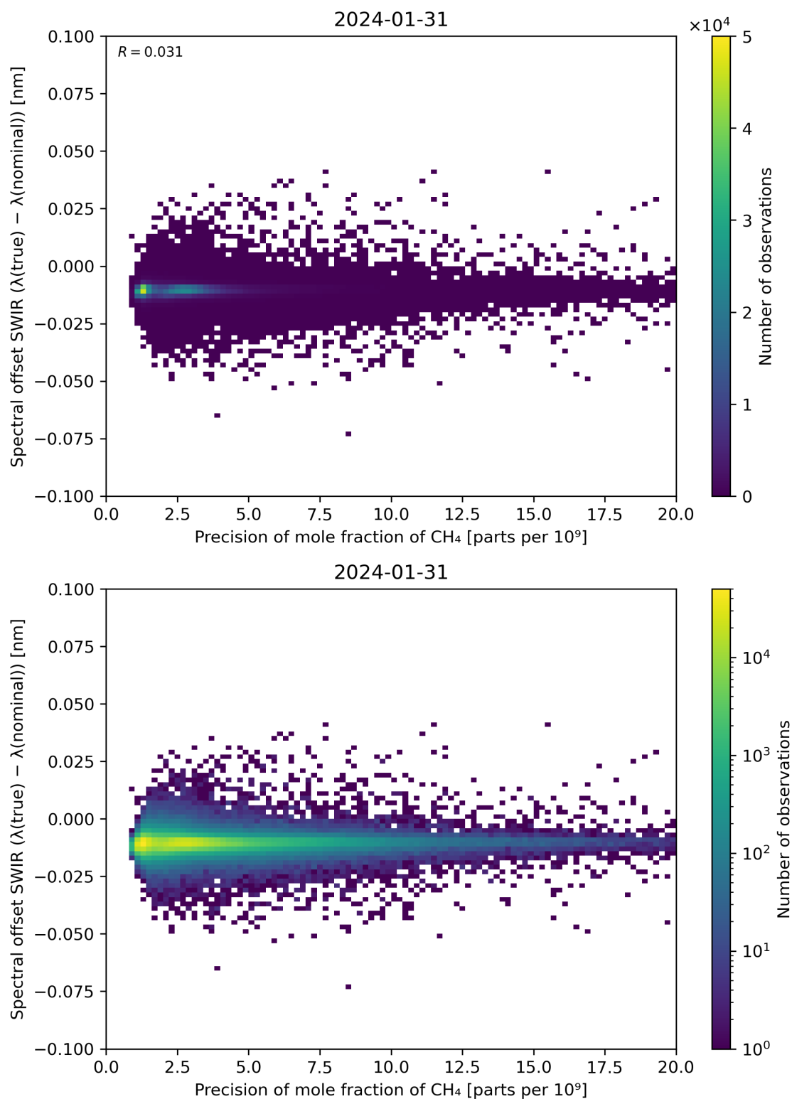
Figure 85: Scatter density plot of “Precision of mole fraction of \text{CH}_4 ” against “Spectral offset SWIR ( \lambda(\text{true}) - \lambda(\text{nominal}) )” for 2024-01-31 to 2024-02-01.
