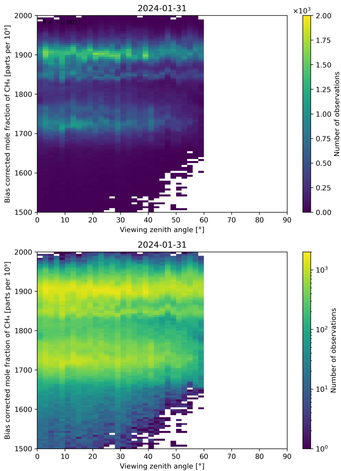
Figure 111: Scatter density plot of “Viewing zenith angle” against “Bias corrected mole fraction of CH 4 ” for 2024-01-31 to 2024-02-01.
