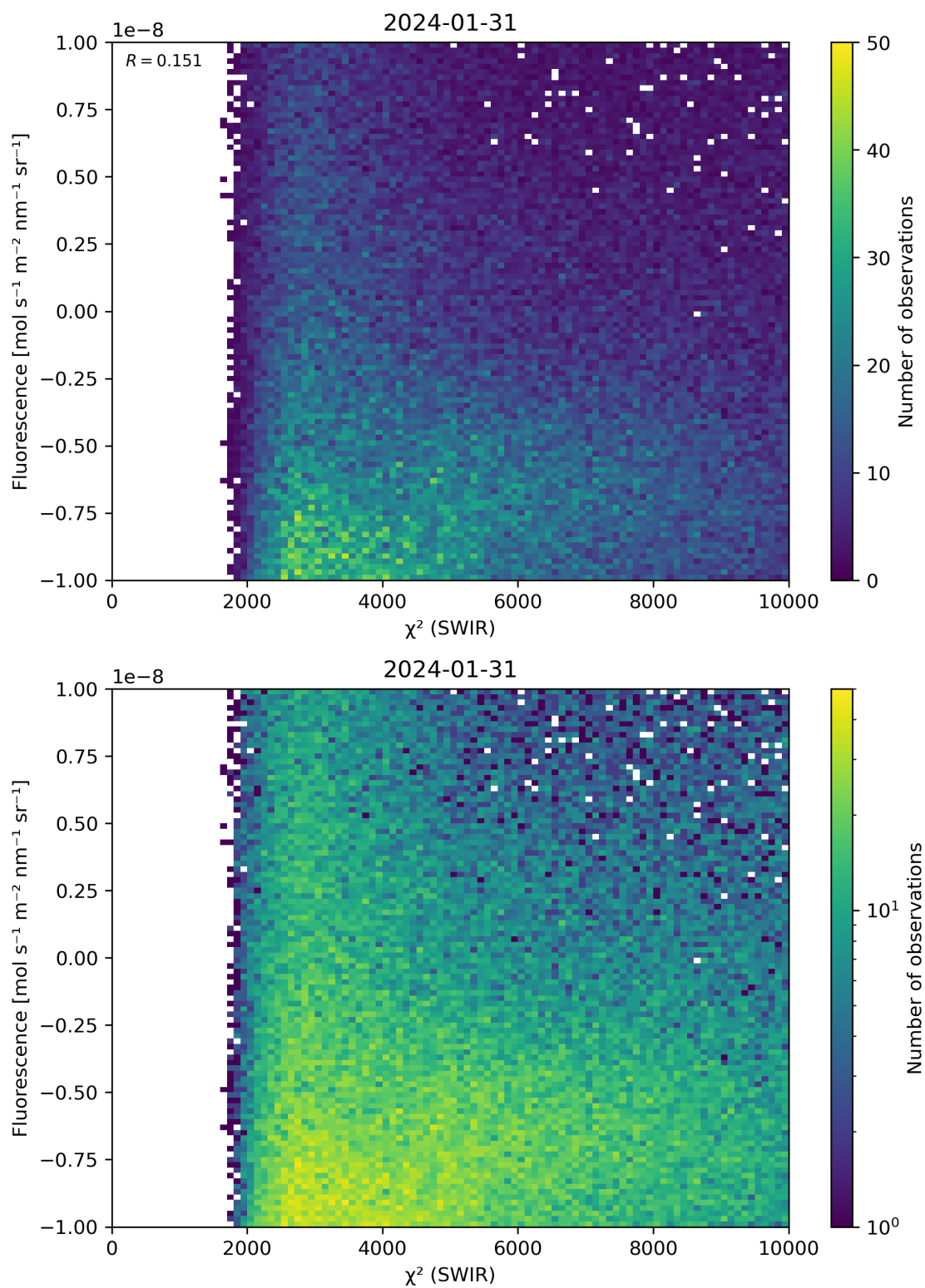
Figure 49: Scatter density plot of “ \chi^2 (SWIR)” against “Fluorescence” for 2024-01-31 to 2024-02-01.
