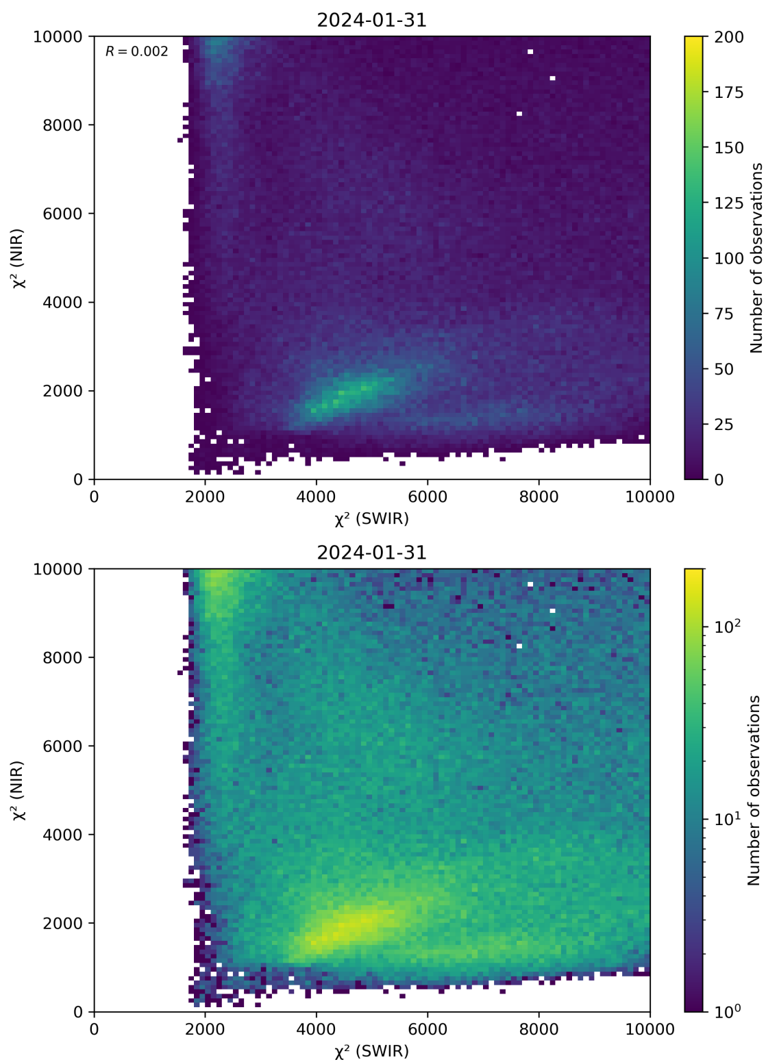
Figure 47: Scatter density plot of “ \chi^2 (SWIR)” against “ \chi^2 (NIR)” for 2024-01-31 to 2024-02-01.
