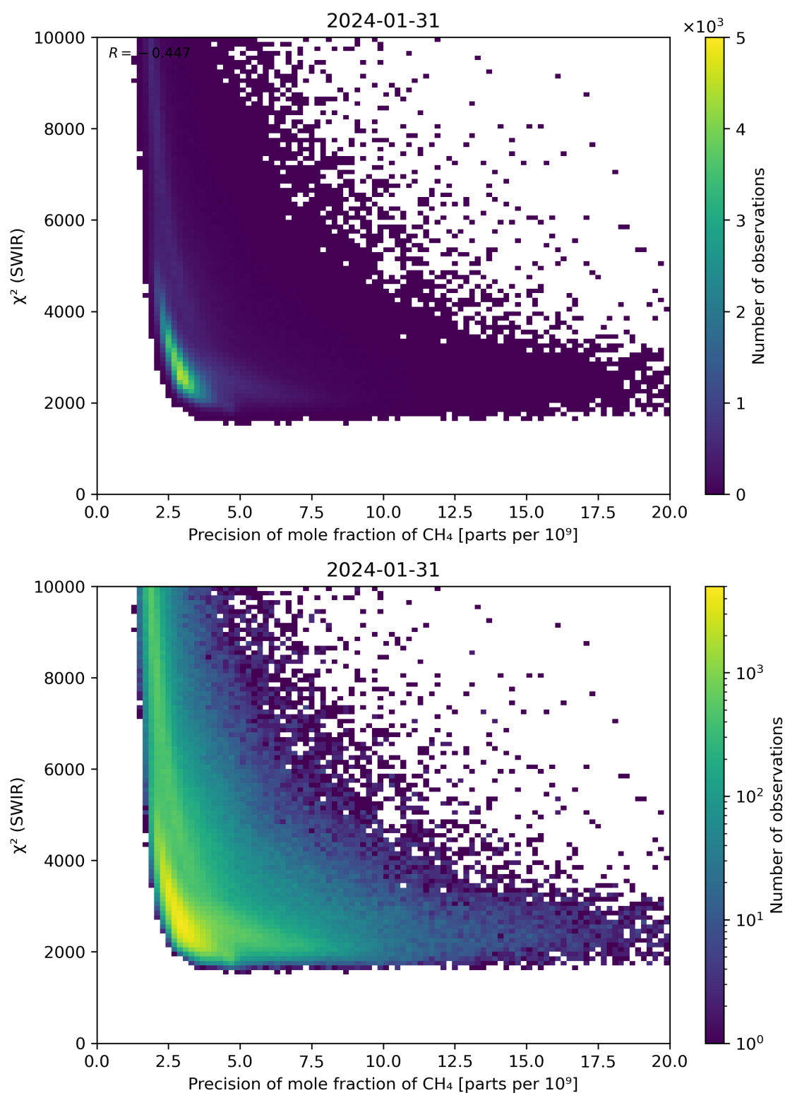
Figure 79: Scatter density plot of “Precision of mole fraction of CH 4 ” against “ \chi^2 (SWIR)” for 2024-01-31 to 2024-02-01.
