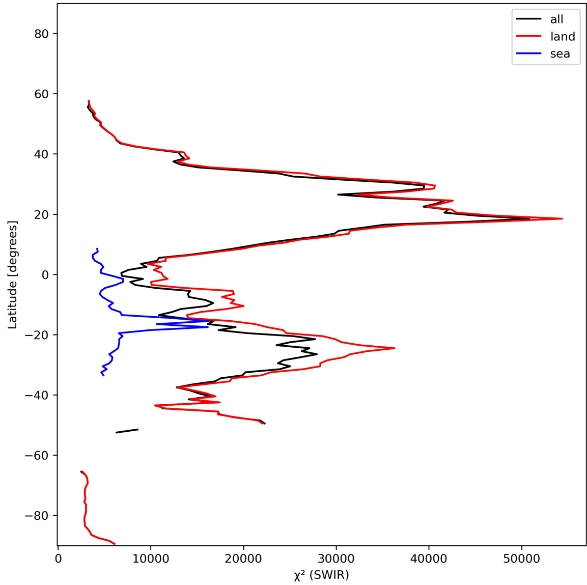
Figure 17: Zonal average of “ \chi^2 (SWIR)” for 2024-01-31 to 2024-02-01.
