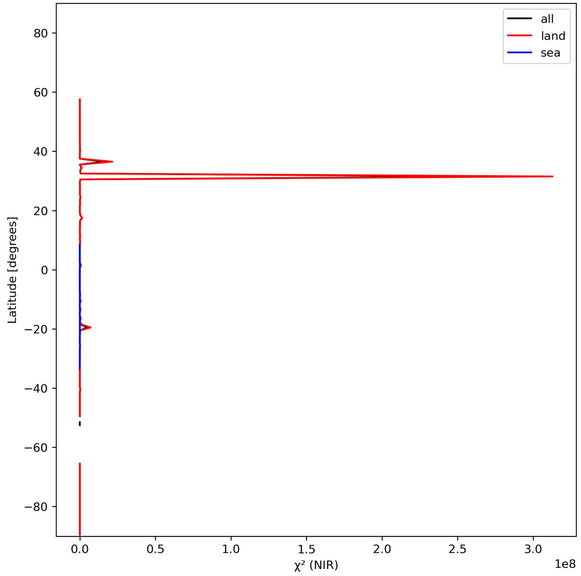
Figure 18: Zonal average of “ \chi^2 (NIR)” for 2024-01-31 to 2024-02-01.
