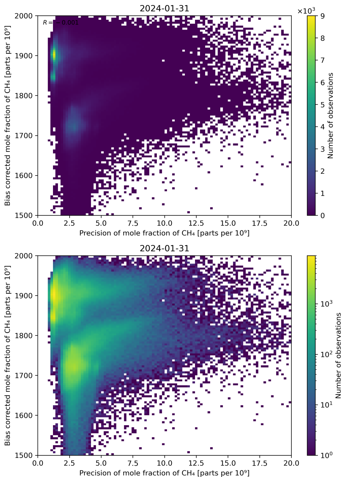
Figure 82: Scatter density plot of “Precision of mole fraction of CH 4 ” against “Bias corrected mole fraction of CH 4 ” for 2024-01-31 to 2024-02-01.
