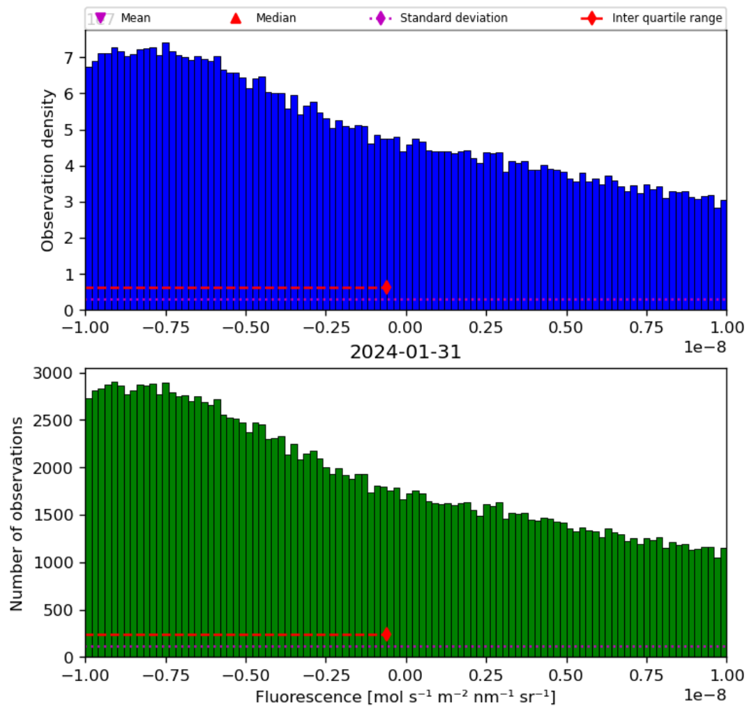
Figure 32: Histogram of “Fluorescence” for 2024-01-31 to 2024-02-01
