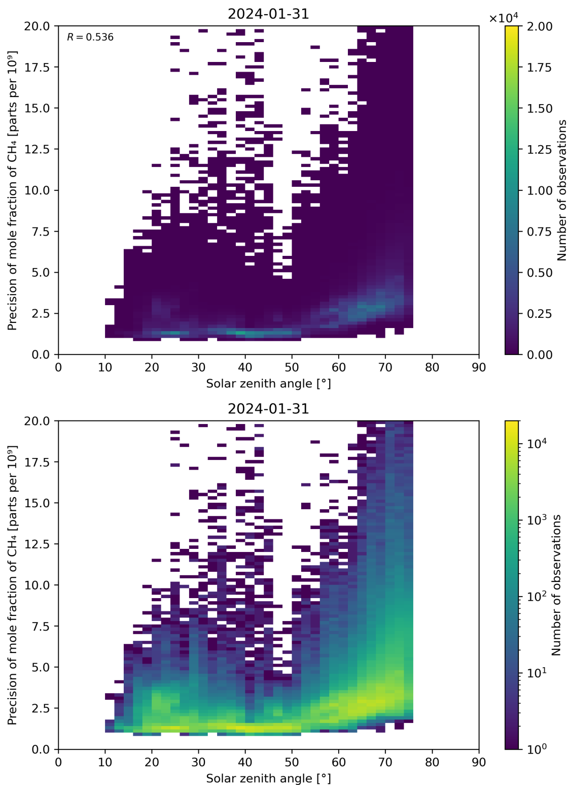
Figure 101: Scatter density plot of “Solar zenith angle” against “Precision of mole fraction of \text{CH}_4 ” for 2024-01-31 to 2024-02-01.
