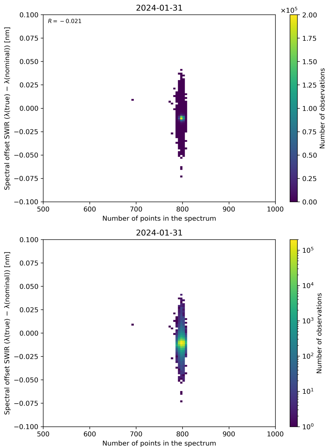
Figure 93: Scatter density plot of “Number of points in the spectrum” against “Spectral offset SWIR ( \lambda(\text{true}) - \lambda(\text{nominal}) )” for 2024-01-31 to 2024-02-01.
