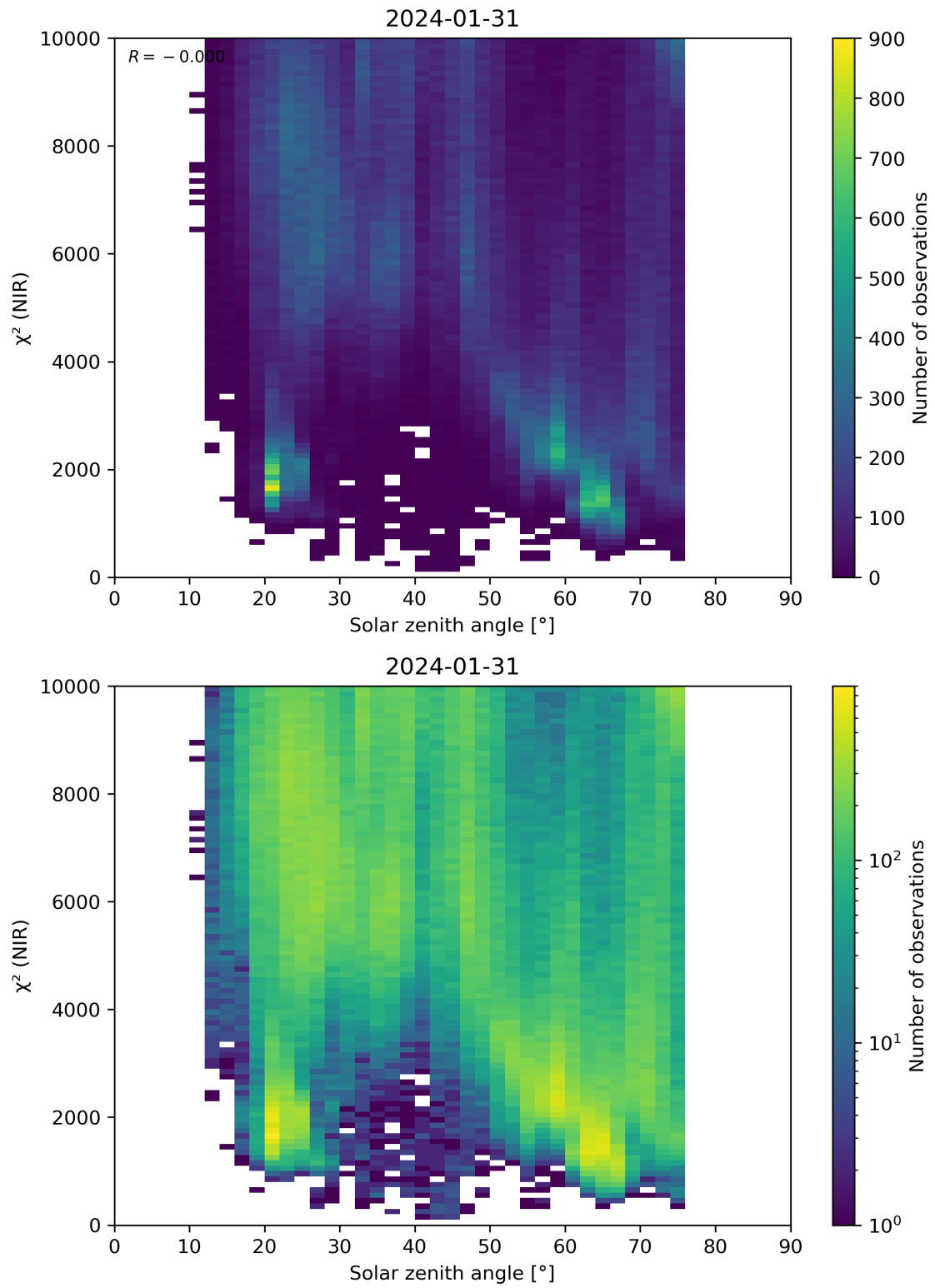
Figure 94: Scatter density plot of “Solar zenith angle” against “ \chi^2 (NIR)” for 2024-01-31 to 2024-02-01.
