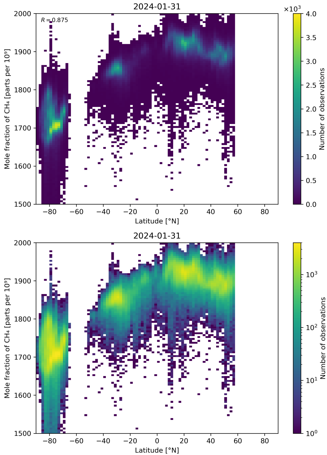
Figure 57: Scatter density plot of “Latitude” against “Mole fraction of CH 4 ” for 2024-01-31 to 2024-02-01.
