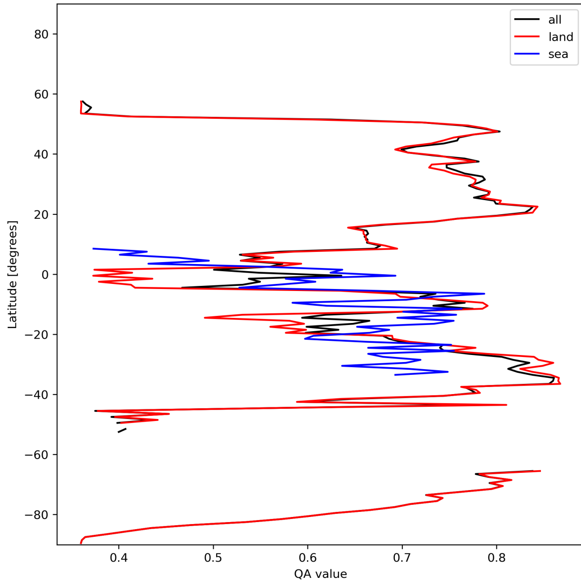
Figure 11: Zonal average of “QA value” for 2024-01-31 to 2024-02-01.
