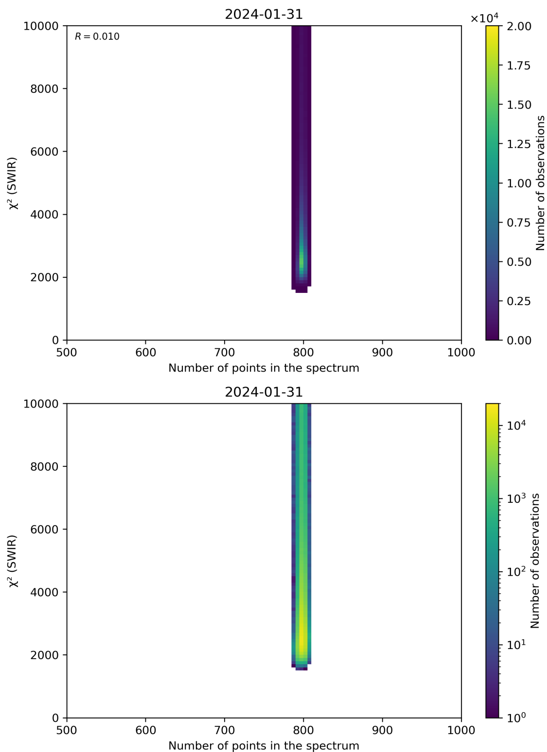
Figure 89: Scatter density plot of “Number of points in the spectrum” against “ \chi^2 (SWIR)” for 2024-01-31 to 2024-02-01.
