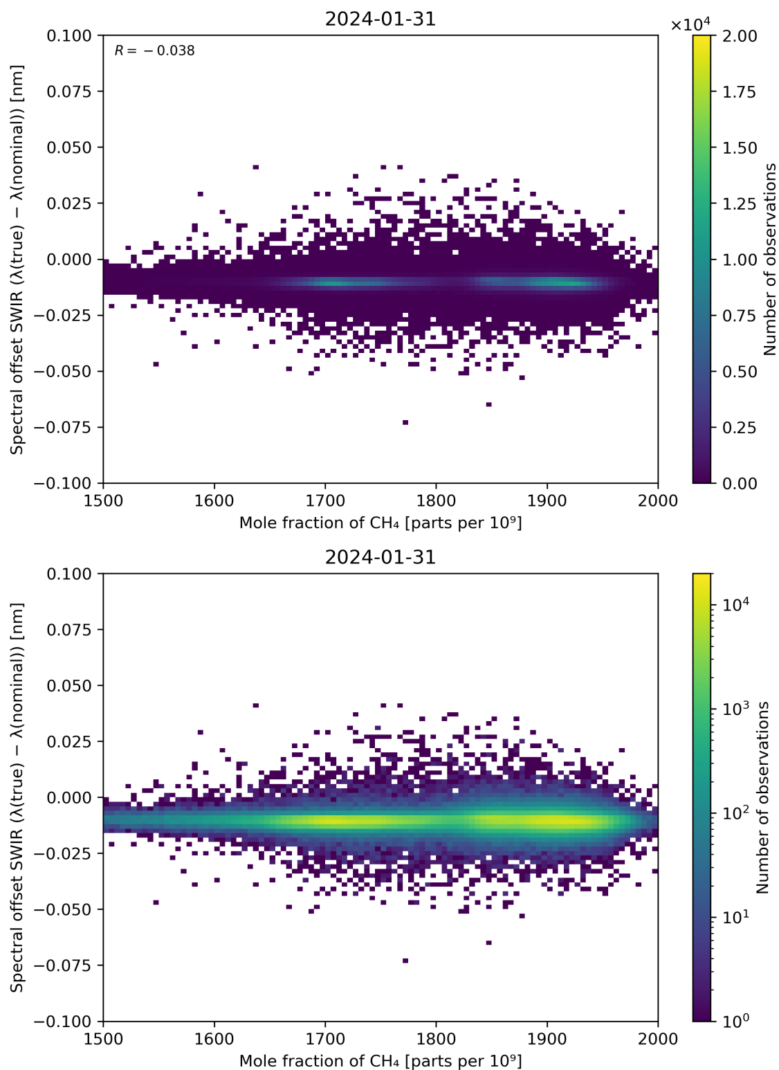
Figure 86: Scatter density plot of “Mole fraction of CH 4 ” against “Spectral offset SWIR ( \lambda(\text{true}) - \lambda(\text{nominal}) )” for 2024-01-31 to 2024-02-01.
