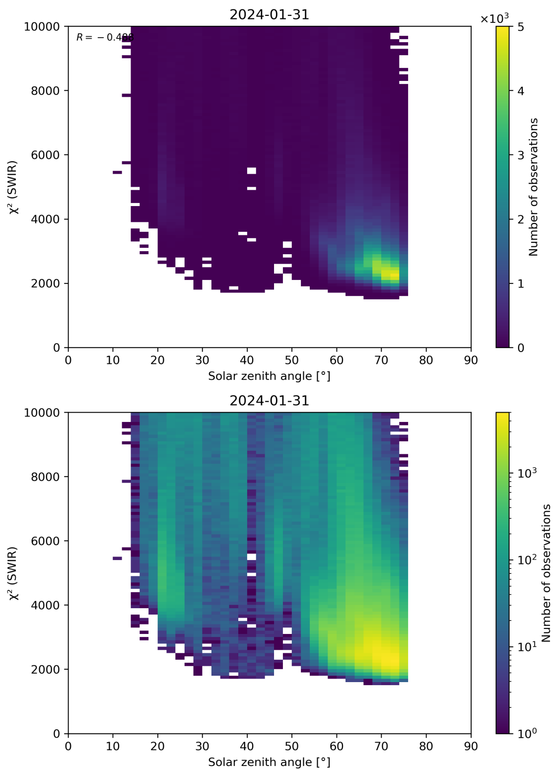
Figure 95: Scatter density plot of “Solar zenith angle” against “ \chi^2 (SWIR)” for 2024-01-31 to 2024-02-01.
