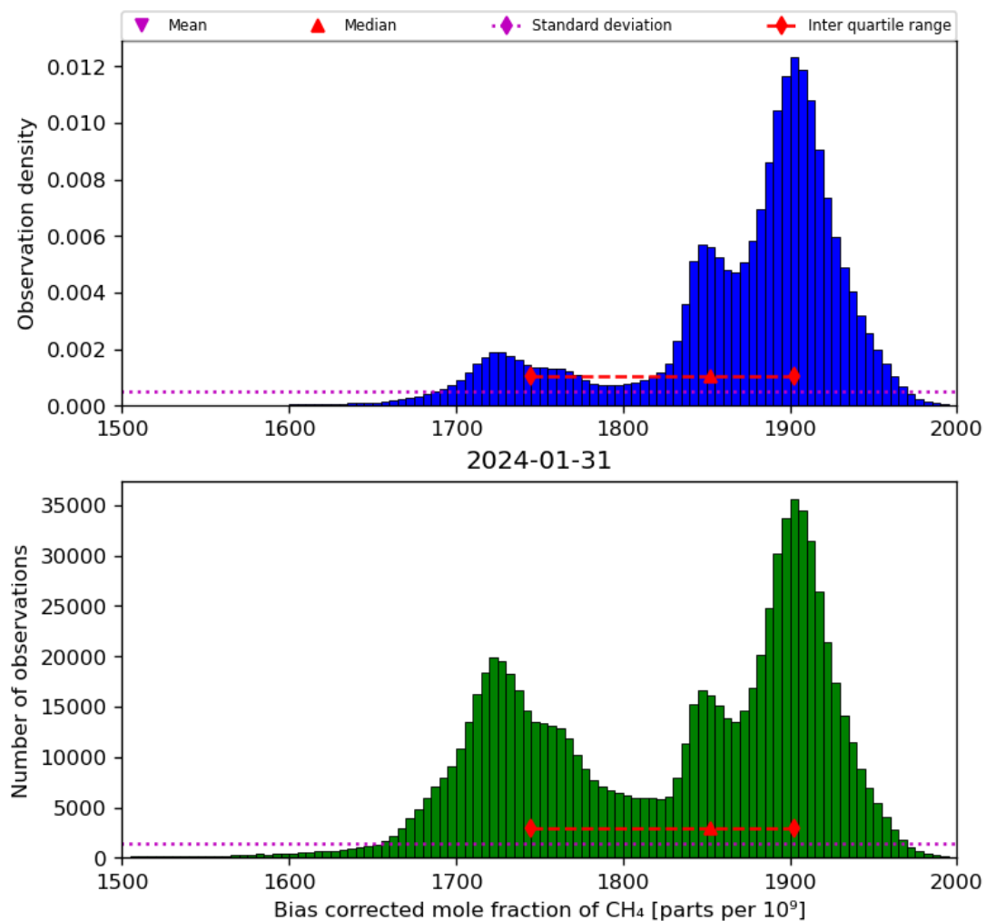
Figure 25: Histogram of “Bias corrected mole fraction of CH 4 ” for 2024-01-31 to 2024-02-01
