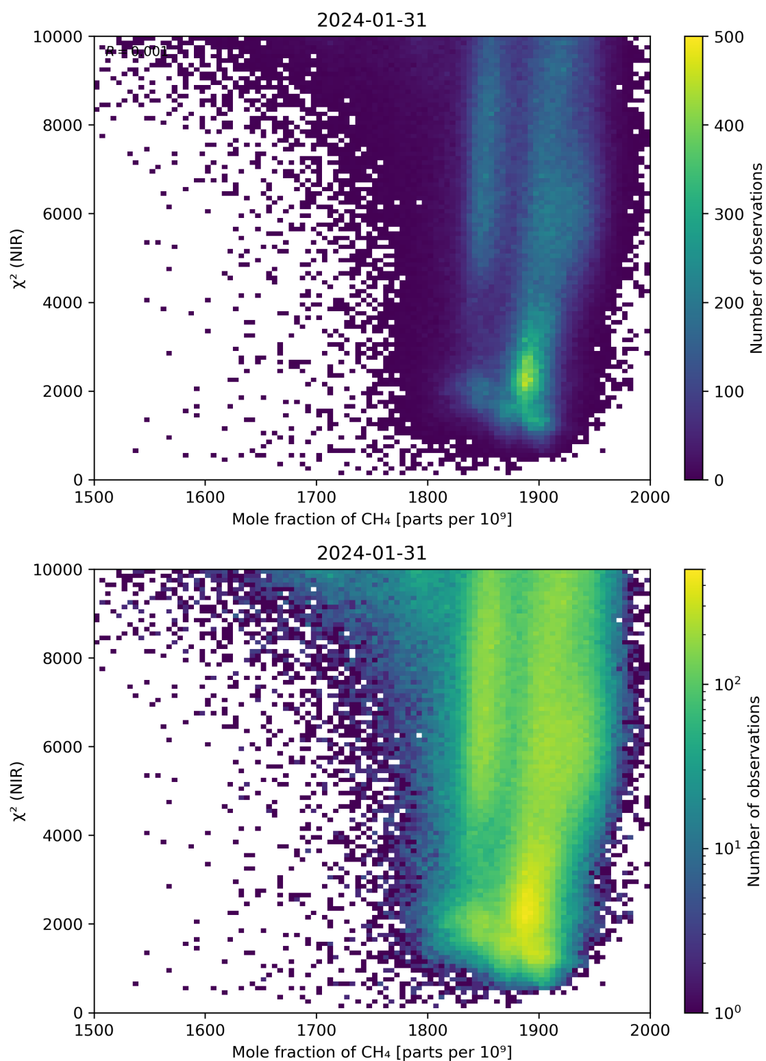
Figure 70: Scatter density plot of “Mole fraction of \text{CH}_4 ” against “ \chi^2 (NIR)” for 2024-01-31 to 2024-02-01.
