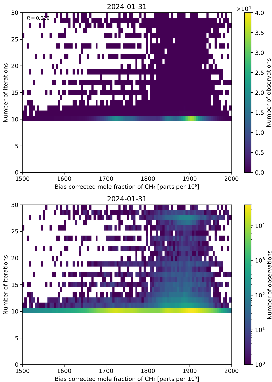
Figure 67: Scatter density plot of “Bias corrected mole fraction of \text{CH}_4 ” against “Number of iterations” for 2024-01-31 to 2024-02-01.
