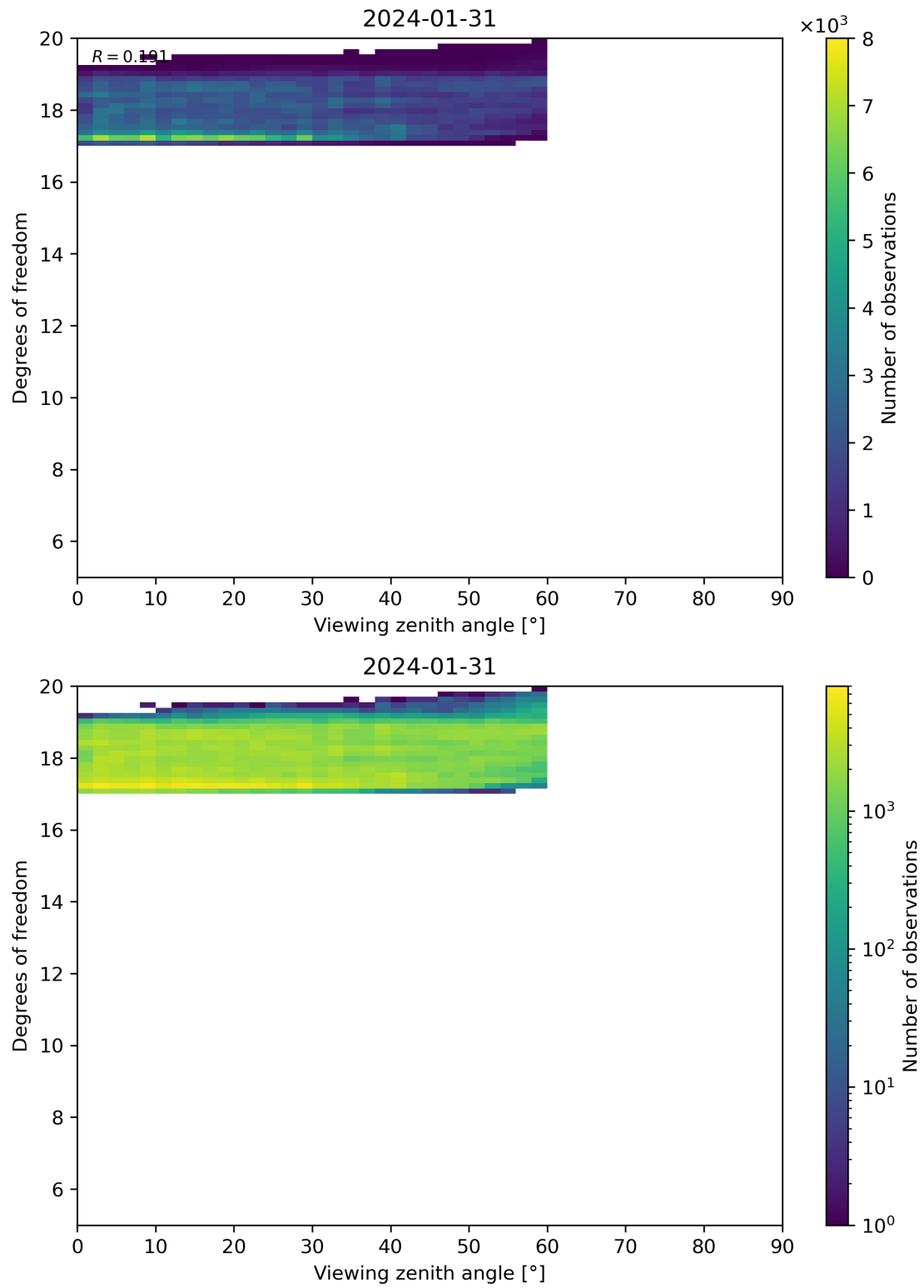
Figure 107: Scatter density plot of “Viewing zenith angle” against “Degrees of freedom” for 2024-01-31 to 2024-02-01.
