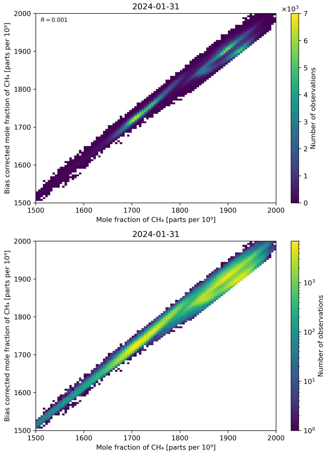
Figure 74: Scatter density plot of “Mole fraction of CH 4 ” against “Bias corrected mole fraction of CH 4 ” for 2024-01-31 to 2024-02-01.
