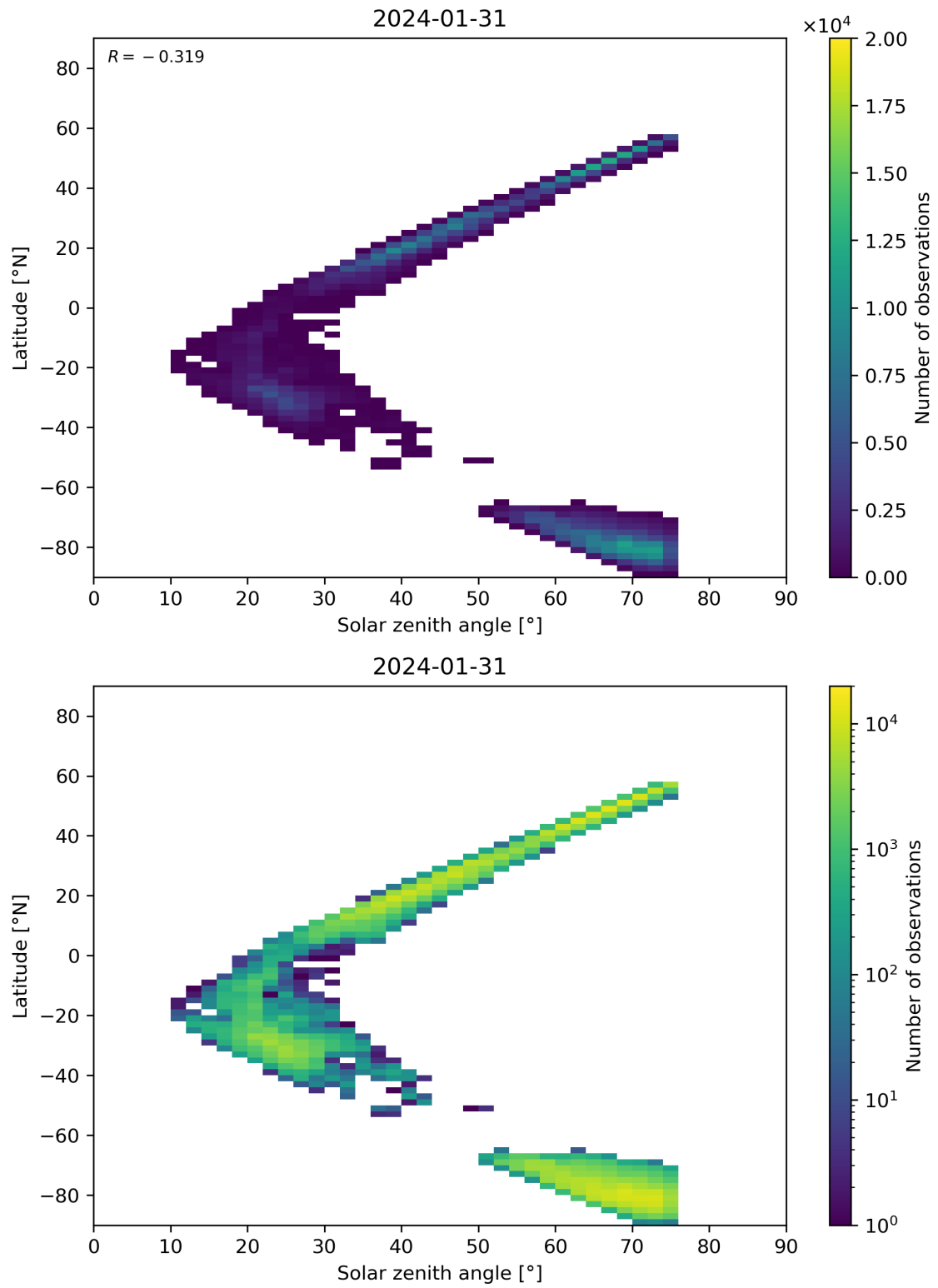
Figure 98: Scatter density plot of “Solar zenith angle” against “Latitude” for 2024-01-31 to 2024-02-01.
