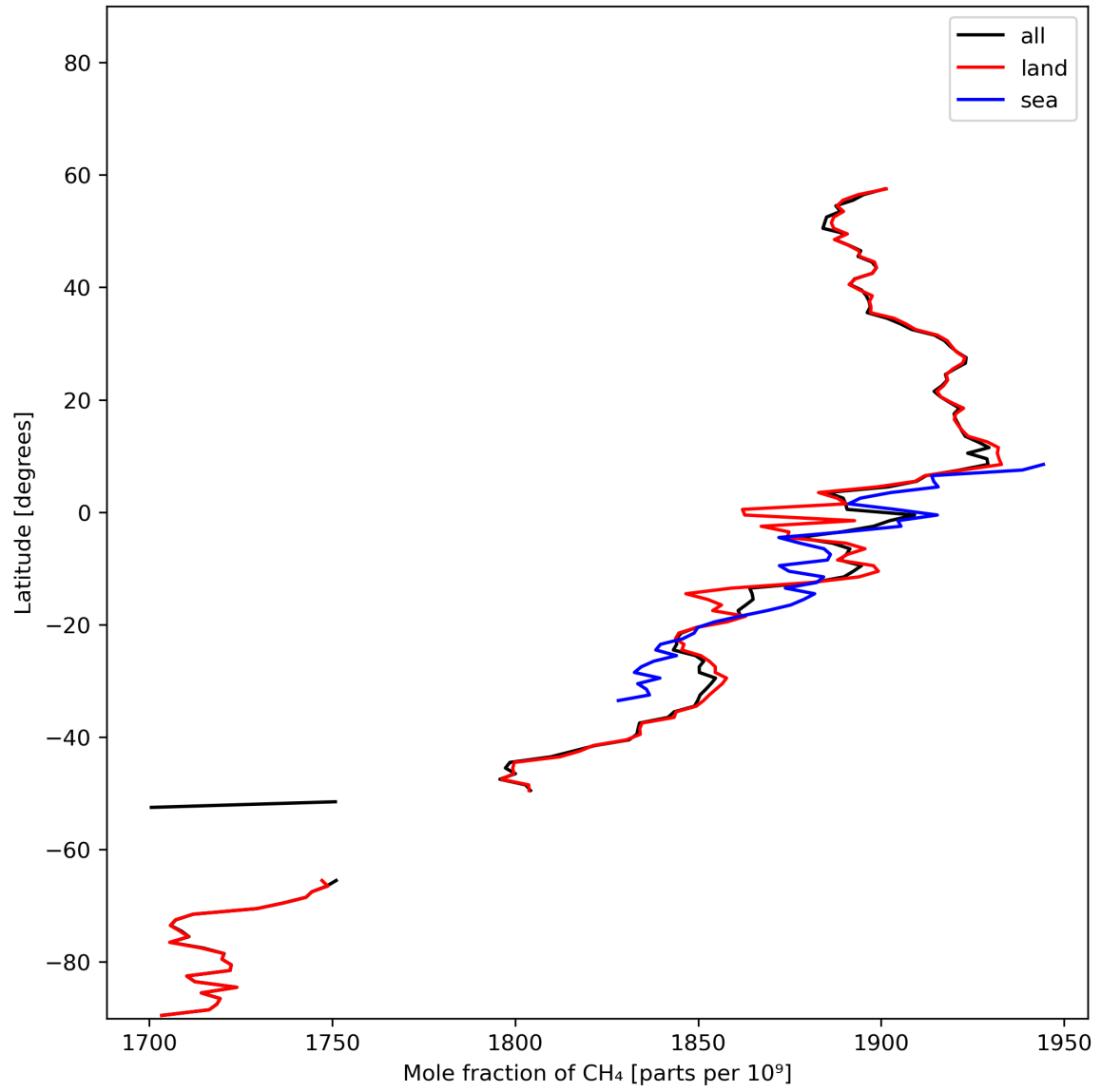
Figure 12: Zonal average of “Mole fraction of CH 4 ” for 2024-01-31 to 2024-02-01.
