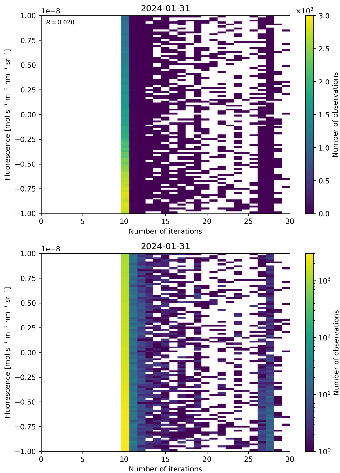
Figure 87: Scatter density plot of “Number of iterations” against “Fluorescence” for 2024-01-31 to 2024-02-01.
