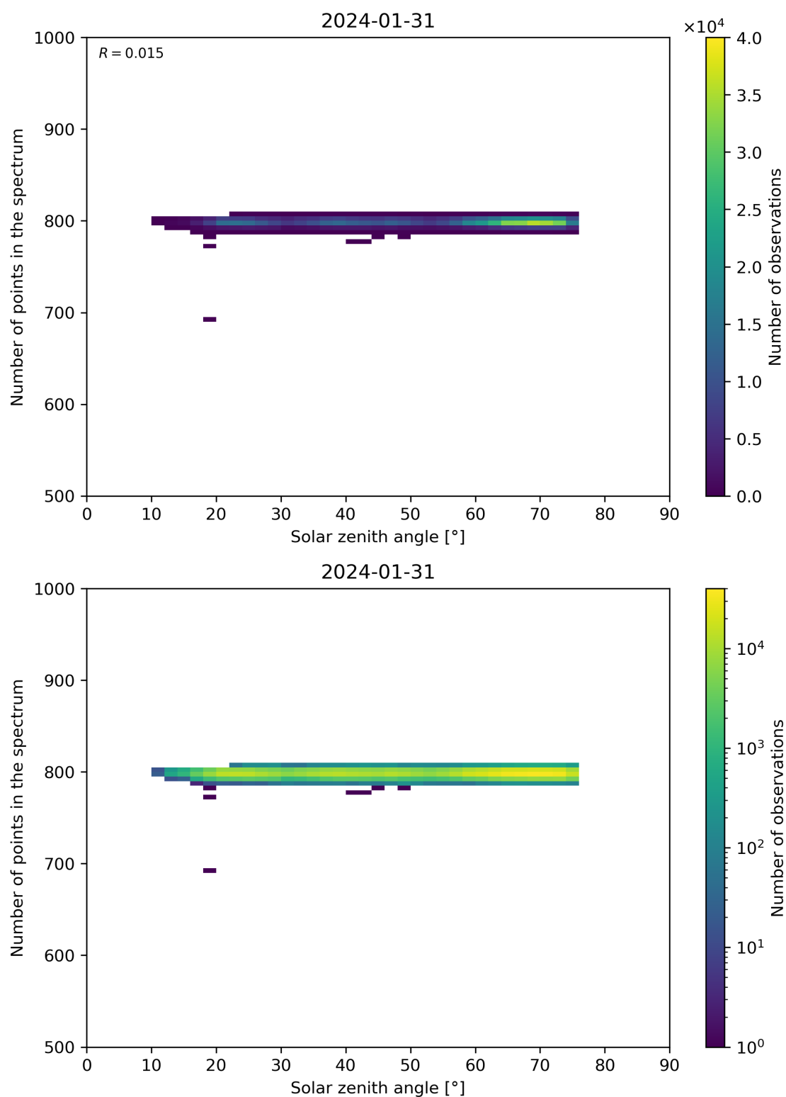
Figure 103: Scatter density plot of “Solar zenith angle” against “Number of points in the spectrum” for 2024-01-31 to 2024-02-01.
