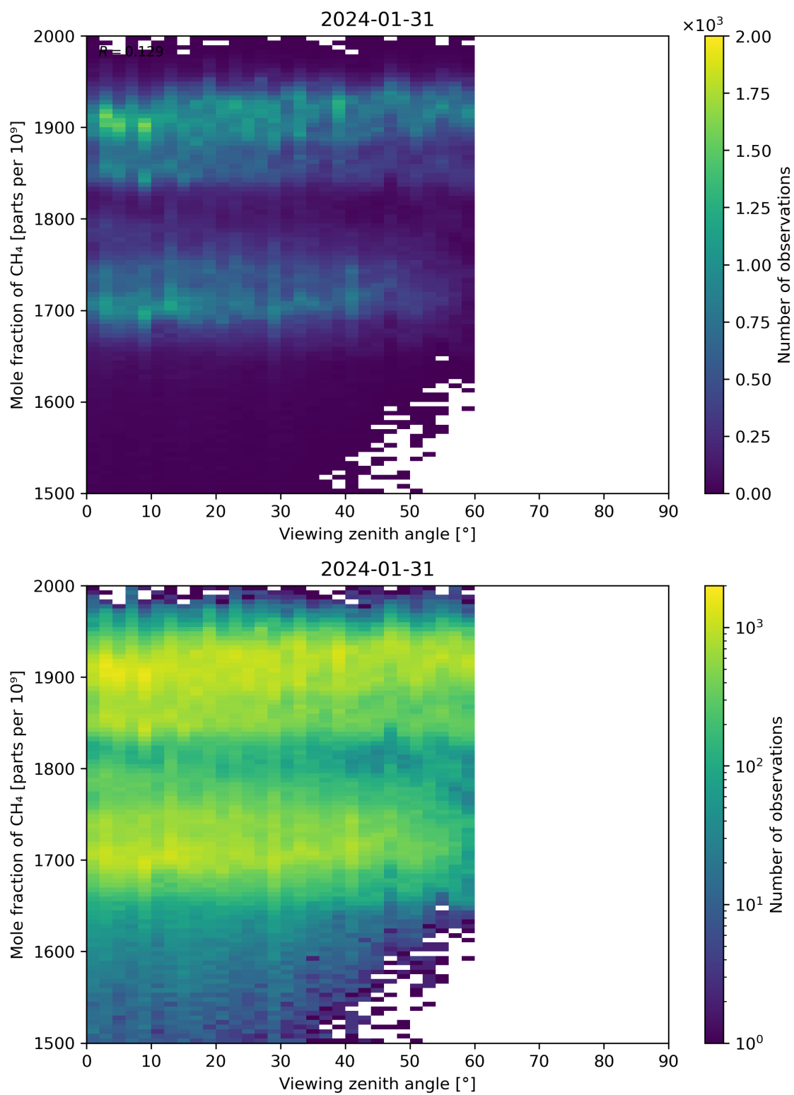
Figure 110: Scatter density plot of “Viewing zenith angle” against “Mole fraction of CH 4 ” for 2024-01-31 to 2024-02-01.
