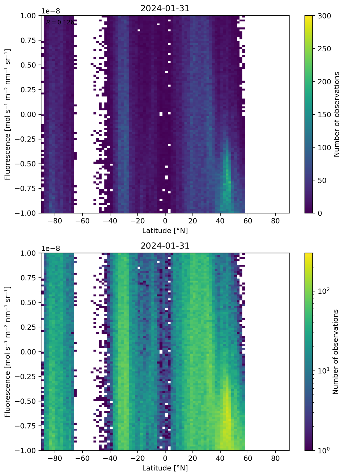
Figure 56: Scatter density plot of “Latitude” against “Fluorescence” for 2024-01-31 to 2024-02-01.
