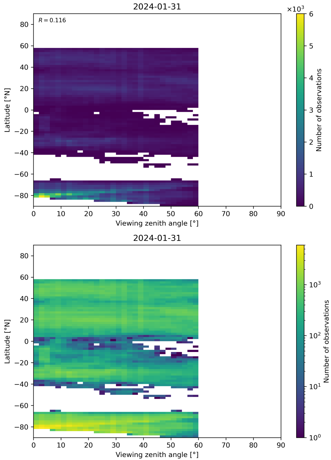
Figure 109: Scatter density plot of “Viewing zenith angle” against “Latitude” for 2024-01-31 to 2024-02-01.
