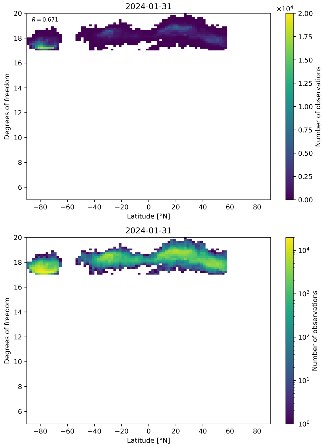
Figure 55: Scatter density plot of “Latitude” against “Degrees of freedom” for 2024-01-31 to 2024-02-01.
