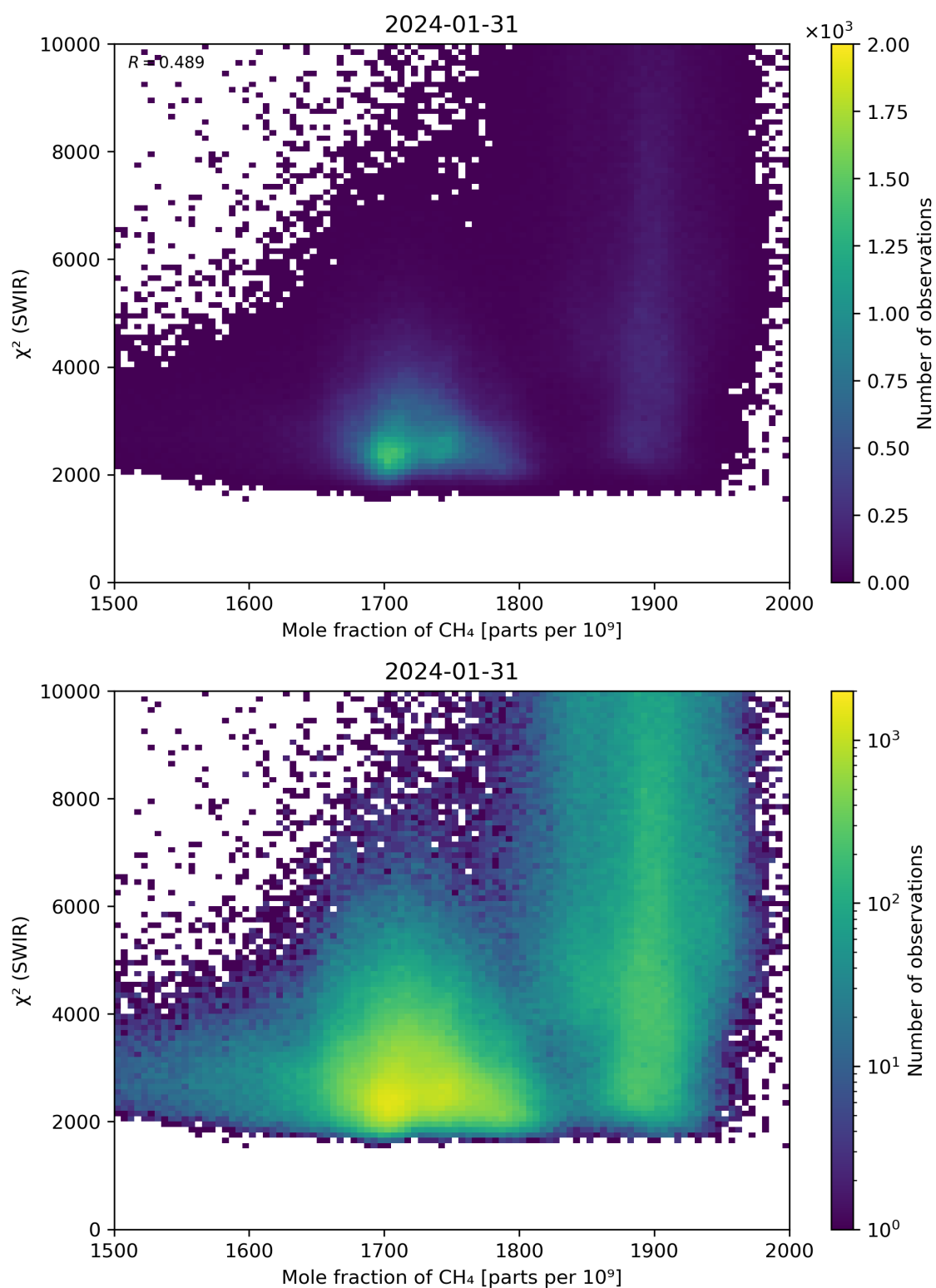
Figure 71: Scatter density plot of “Mole fraction of \text{CH}_4 ” against “ \chi^2 (SWIR)” for 2024-01-31 to 2024-02-01.
