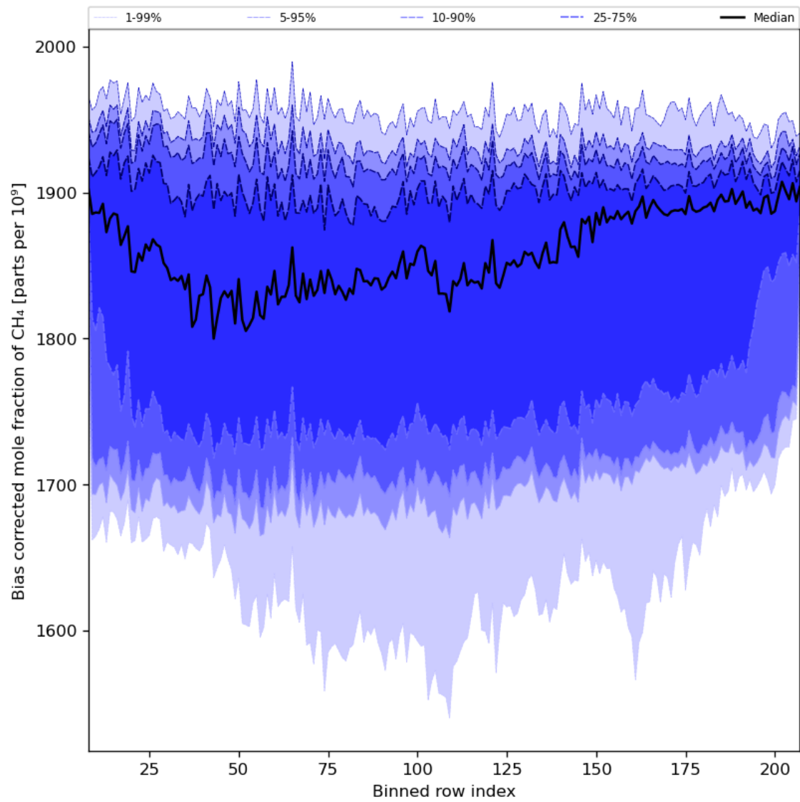
Figure 36: Along track statistics of “Bias corrected mole fraction of CH 4 ” for 2024-01-31 to 2024-02-01
