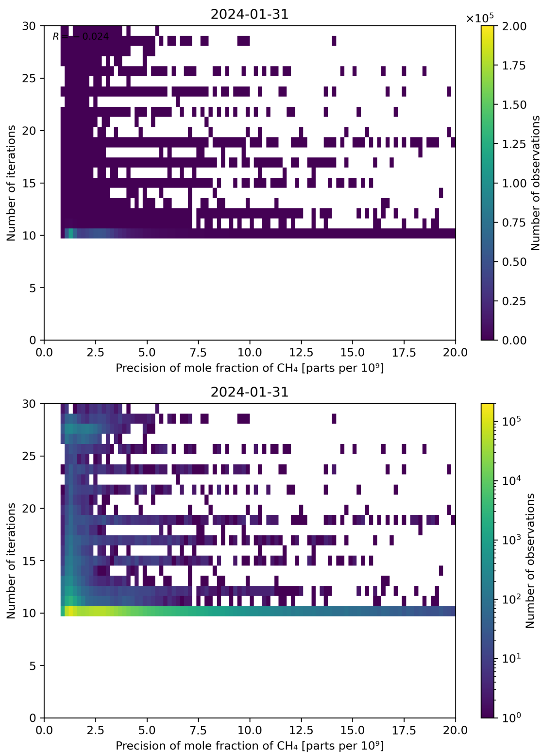
Figure 83: Scatter density plot of “Precision of mole fraction of CH 4 ” against “Number of iterations” for 2024-01-31 to 2024-02-01.
