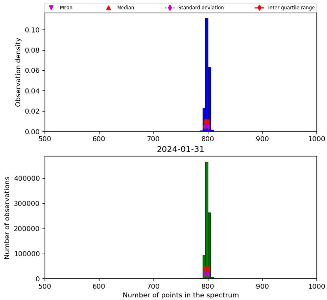
Figure 26: Histogram of “Number of points in the spectrum” for 2024-01-31 to 2024-02-01
