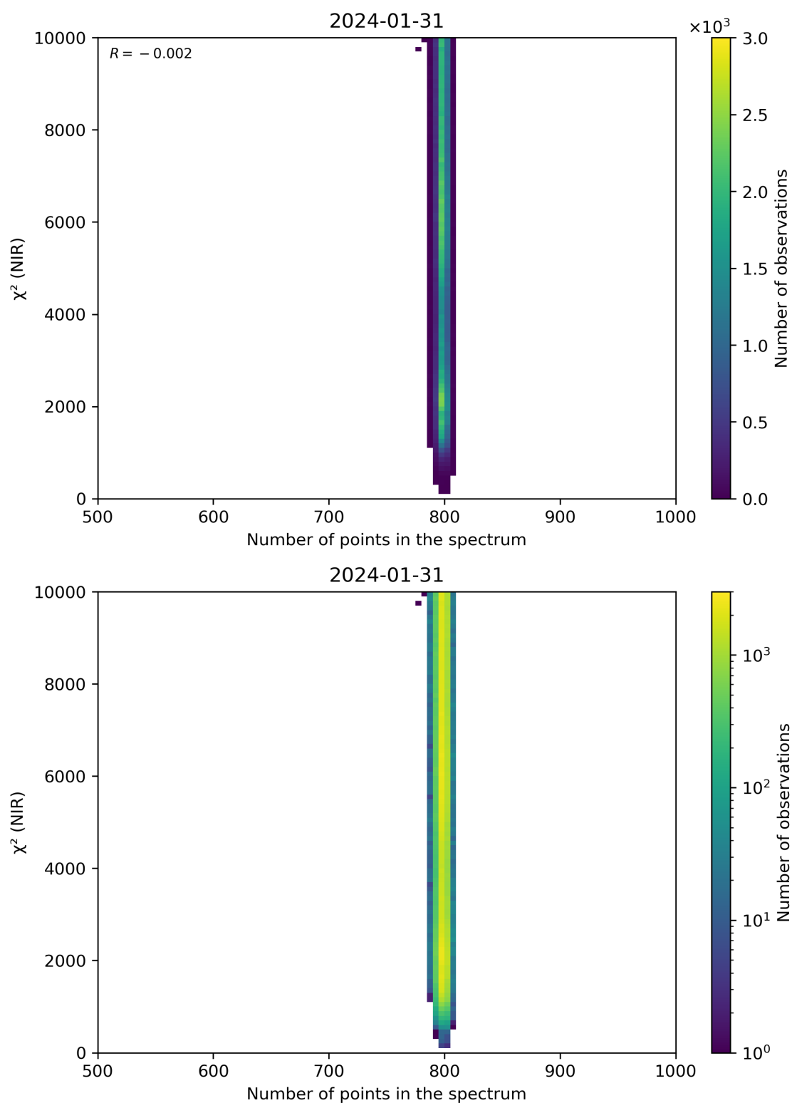
Figure 88: Scatter density plot of “Number of points in the spectrum” against “ \chi^2 (NIR)” for 2024-01-31 to 2024-02-01.
