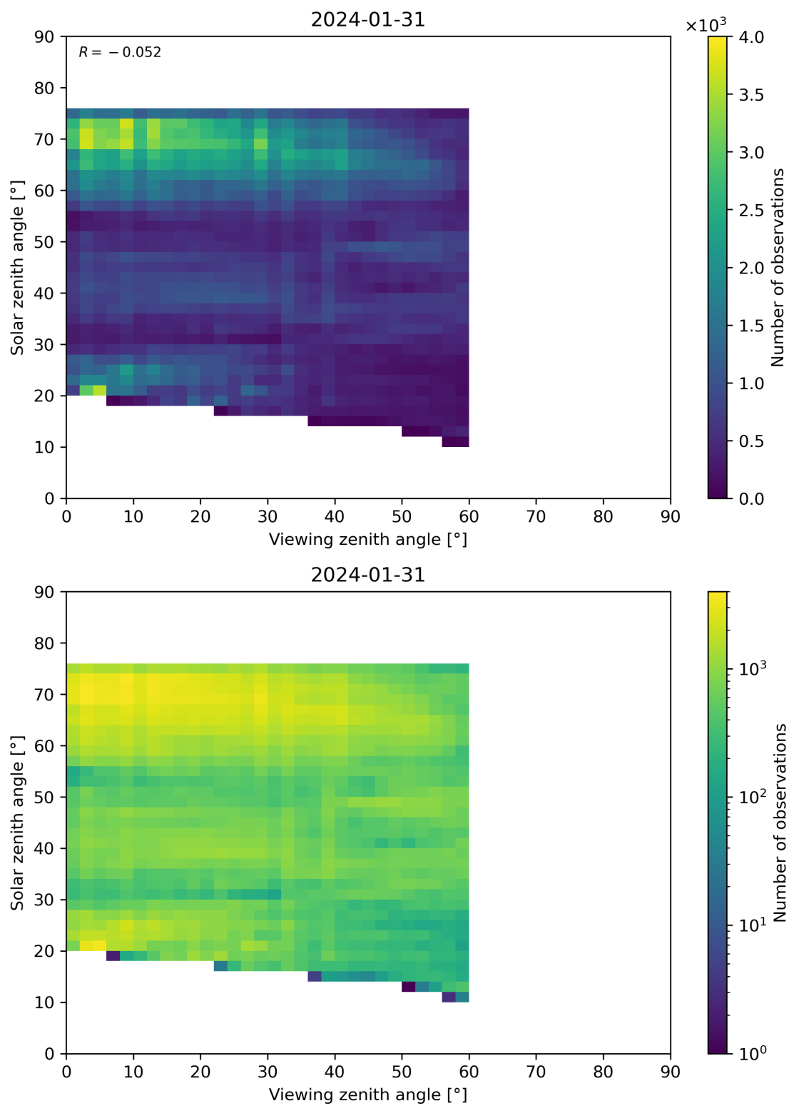
Figure 115: Scatter density plot of “Viewing zenith angle” against “Solar zenith angle” for 2024-01-31 to 2024-02-01.
