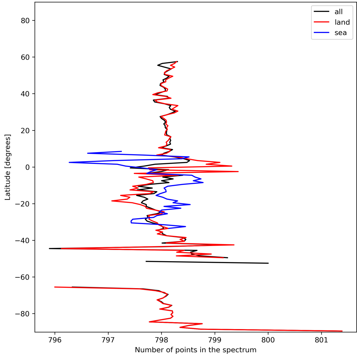
Figure 15: Zonal average of “Number of points in the spectrum” for 2024-01-31 to 2024-02-01.
