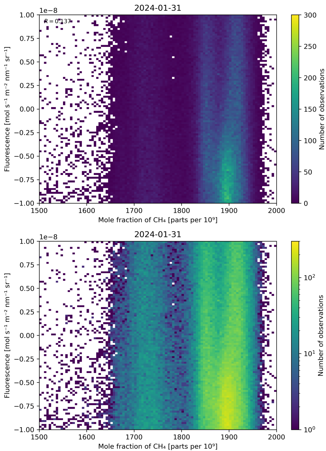
Figure 73: Scatter density plot of “Mole fraction of \text{CH}_4 ” against “Fluorescence” for 2024-01-31 to 2024-02-01.
