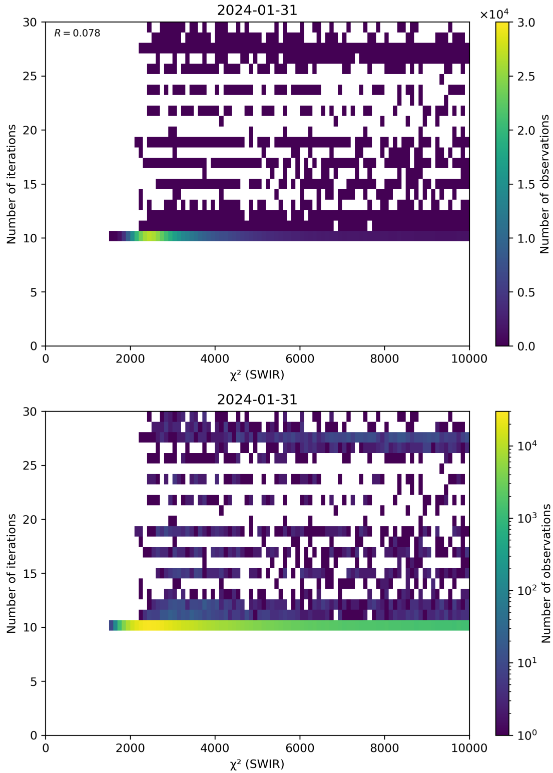
Figure 50: Scatter density plot of " \chi^2 (SWIR)" against "Number of iterations" for 2024-01-31 to 2024-02-01.
