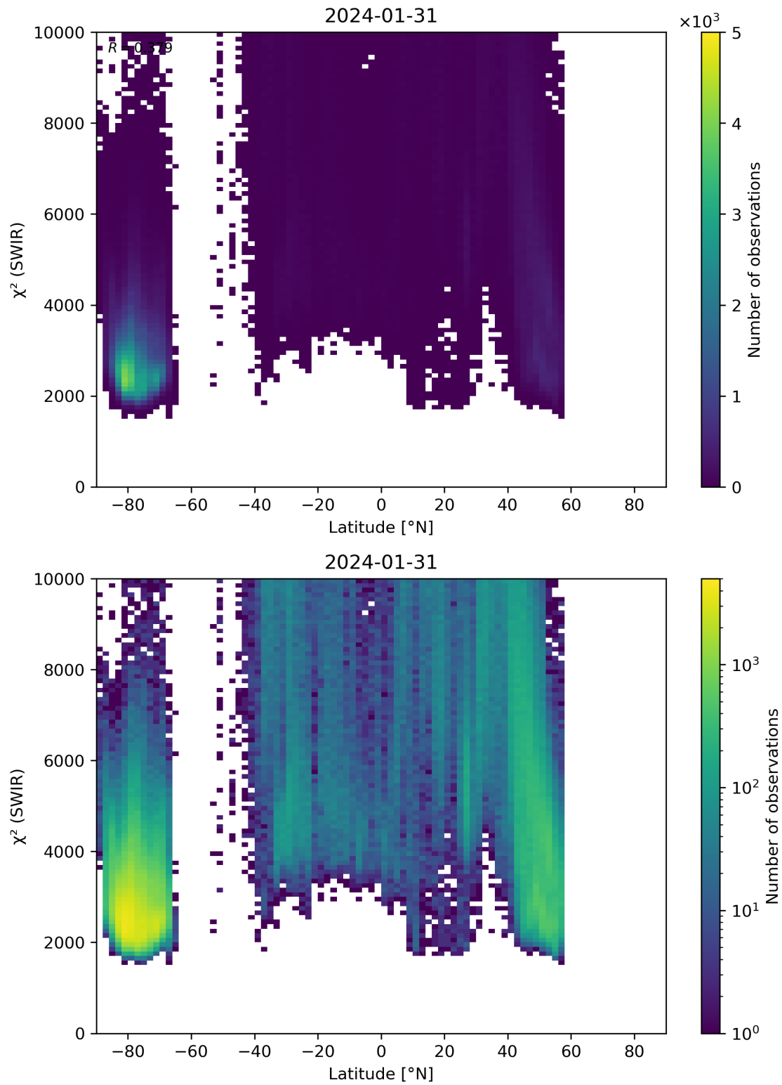
Figure 54: Scatter density plot of “Latitude” against “ \chi^2 (SWIR)” for 2024-01-31 to 2024-02-01.
