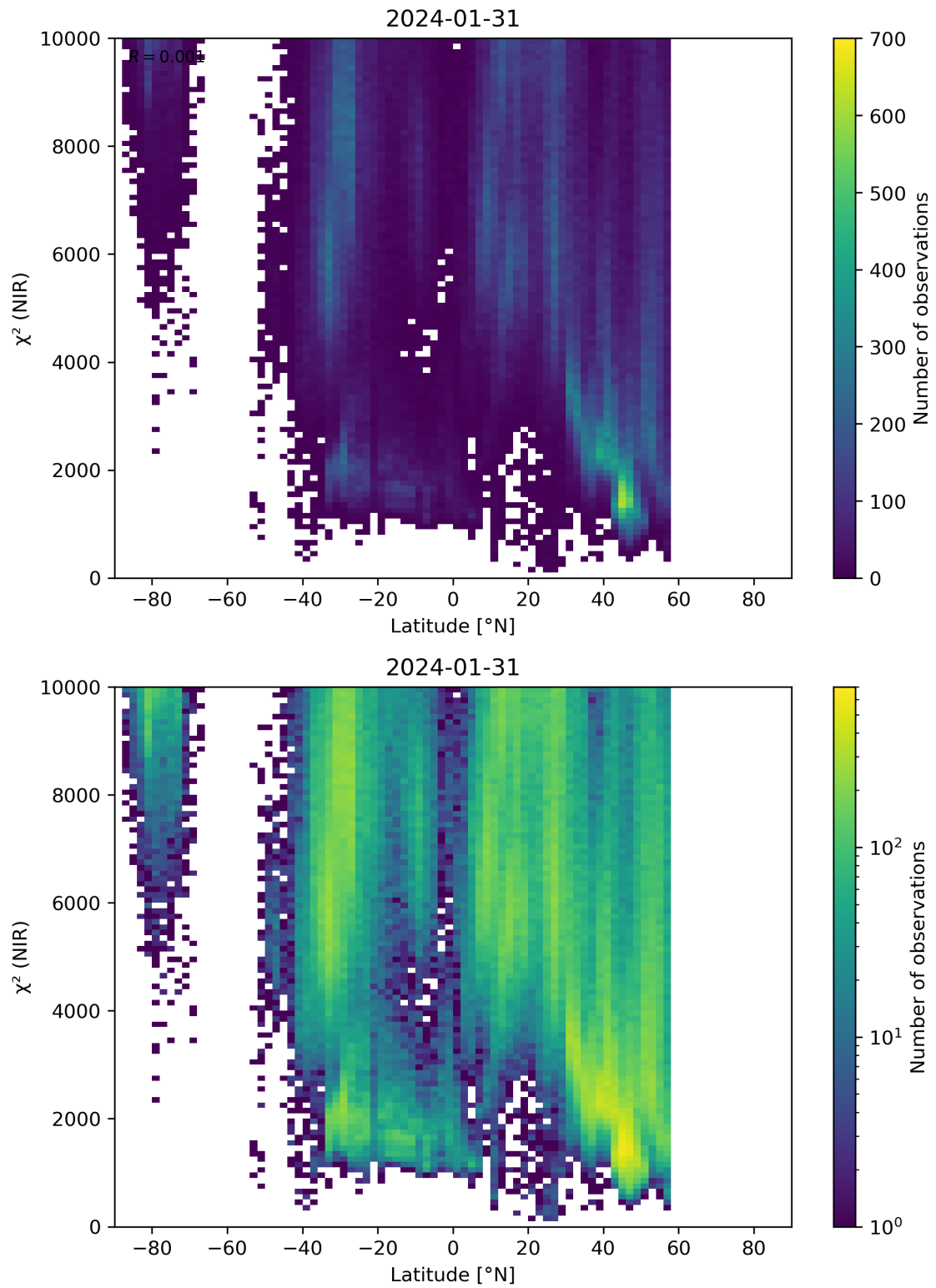
Figure 53: Scatter density plot of “Latitude” against “ \chi^2 (NIR)” for 2024-01-31 to 2024-02-01.
