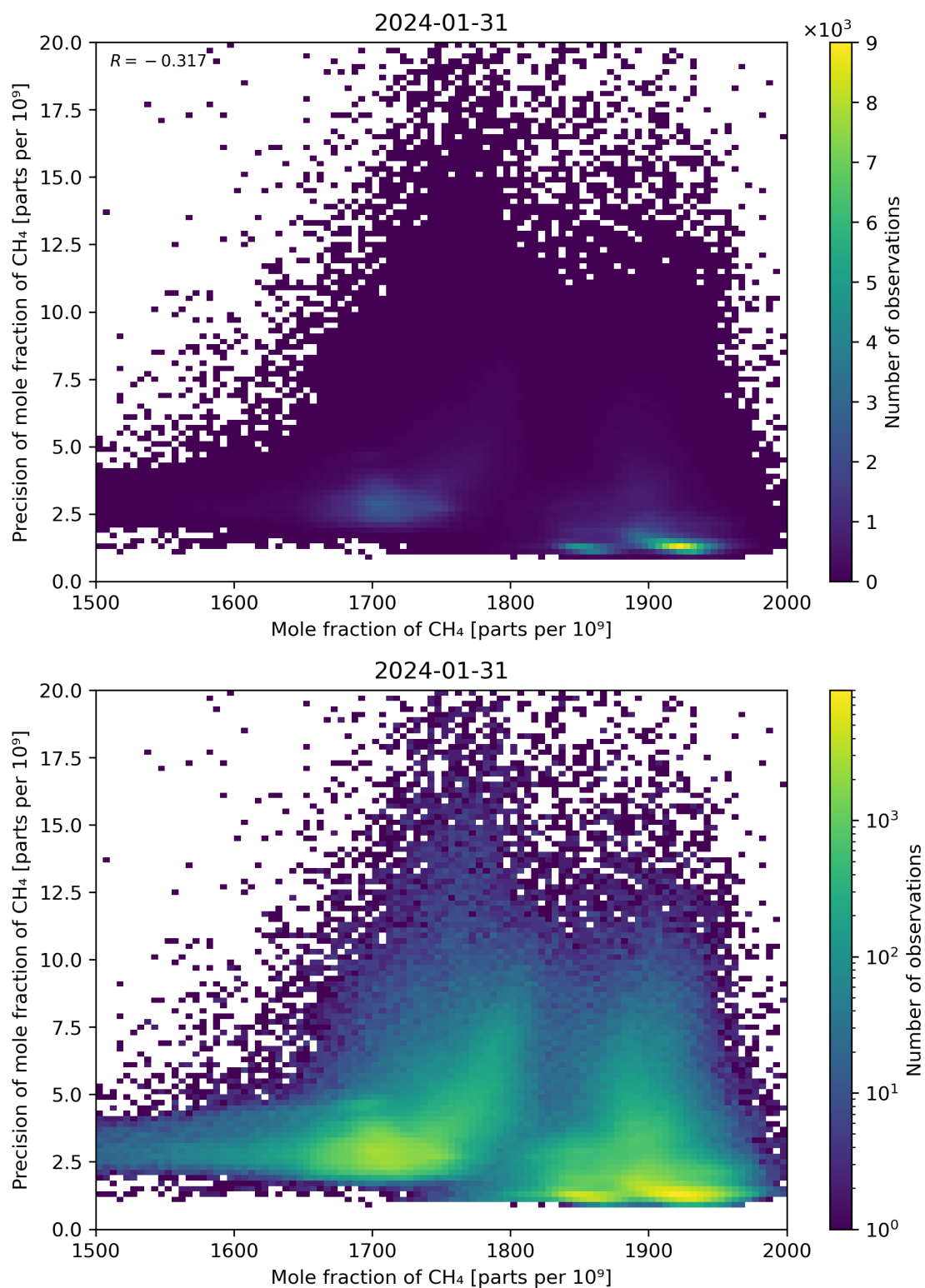
Figure 75: Scatter density plot of “Mole fraction of CH 4 ” against “Precision of mole fraction of CH 4 ” for 2024-01-31 to 2024-02-01.
