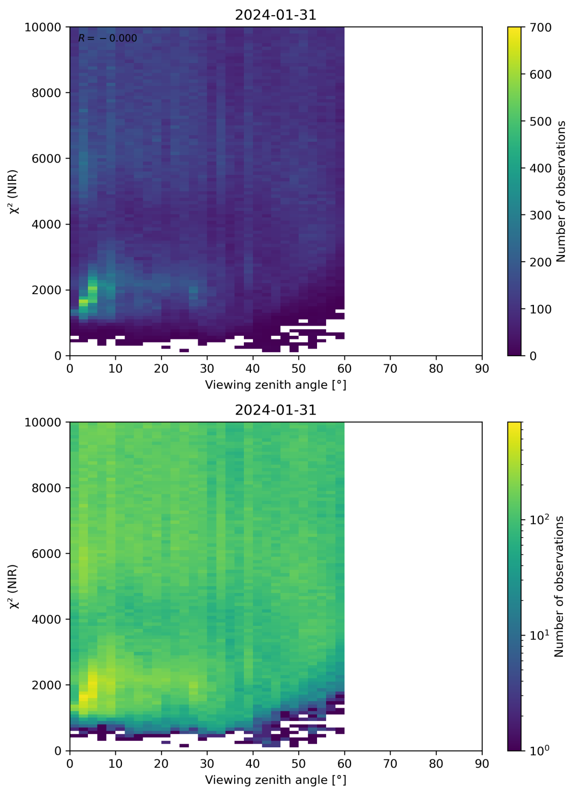
Figure 105: Scatter density plot of “Viewing zenith angle” against “ \chi^2 (NIR)” for 2024-01-31 to 2024-02-01.
