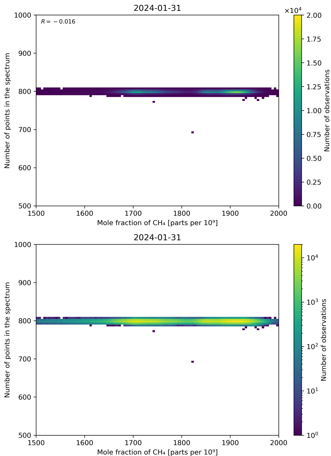
Figure 77: Scatter density plot of “Mole fraction of CH 4 ” against “Number of points in the spectrum” for 2024-01-31 to 2024-02-01.
