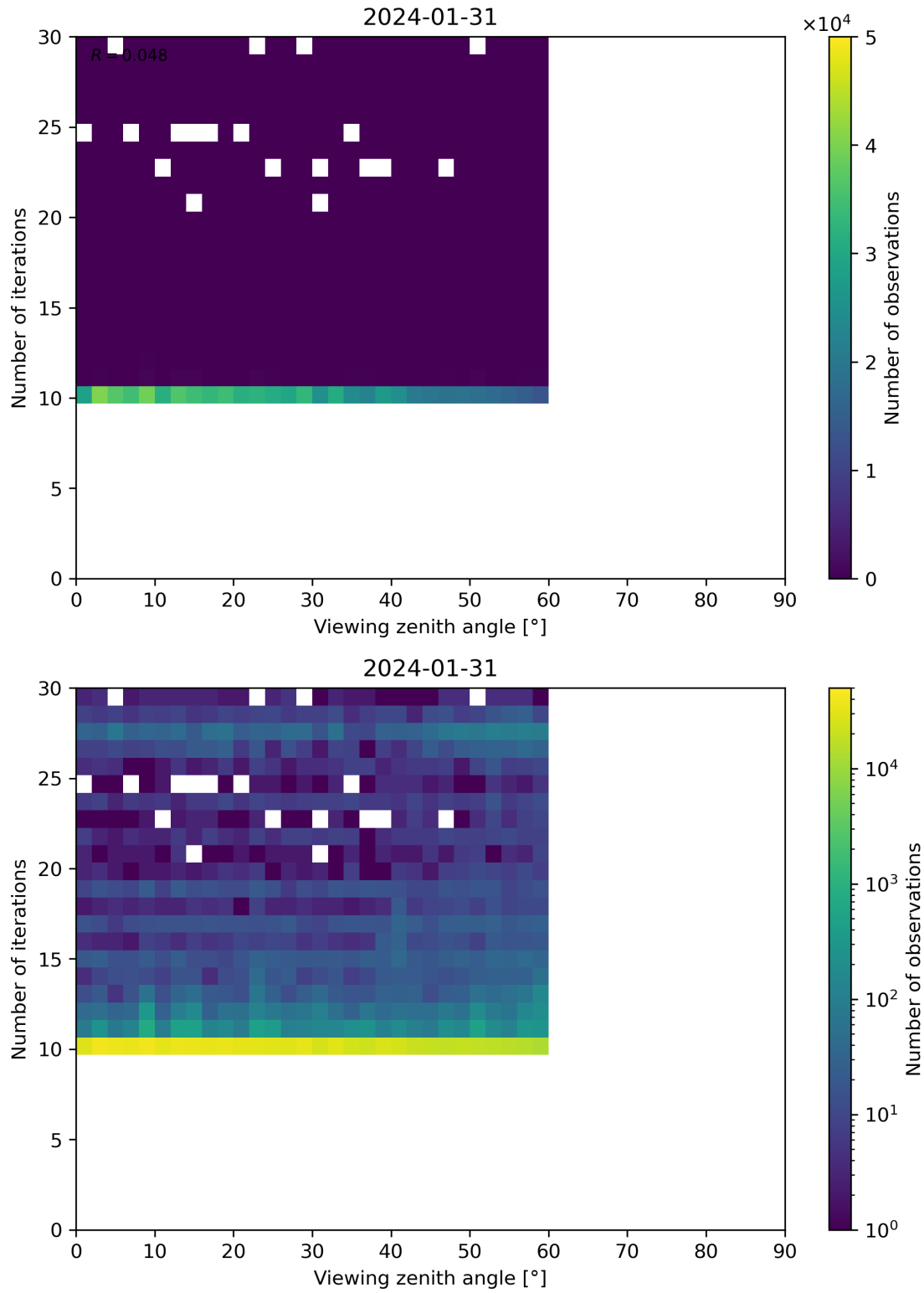
Figure 113: Scatter density plot of “Viewing zenith angle” against “Number of iterations” for 2024-01-31 to 2024-02-01.
