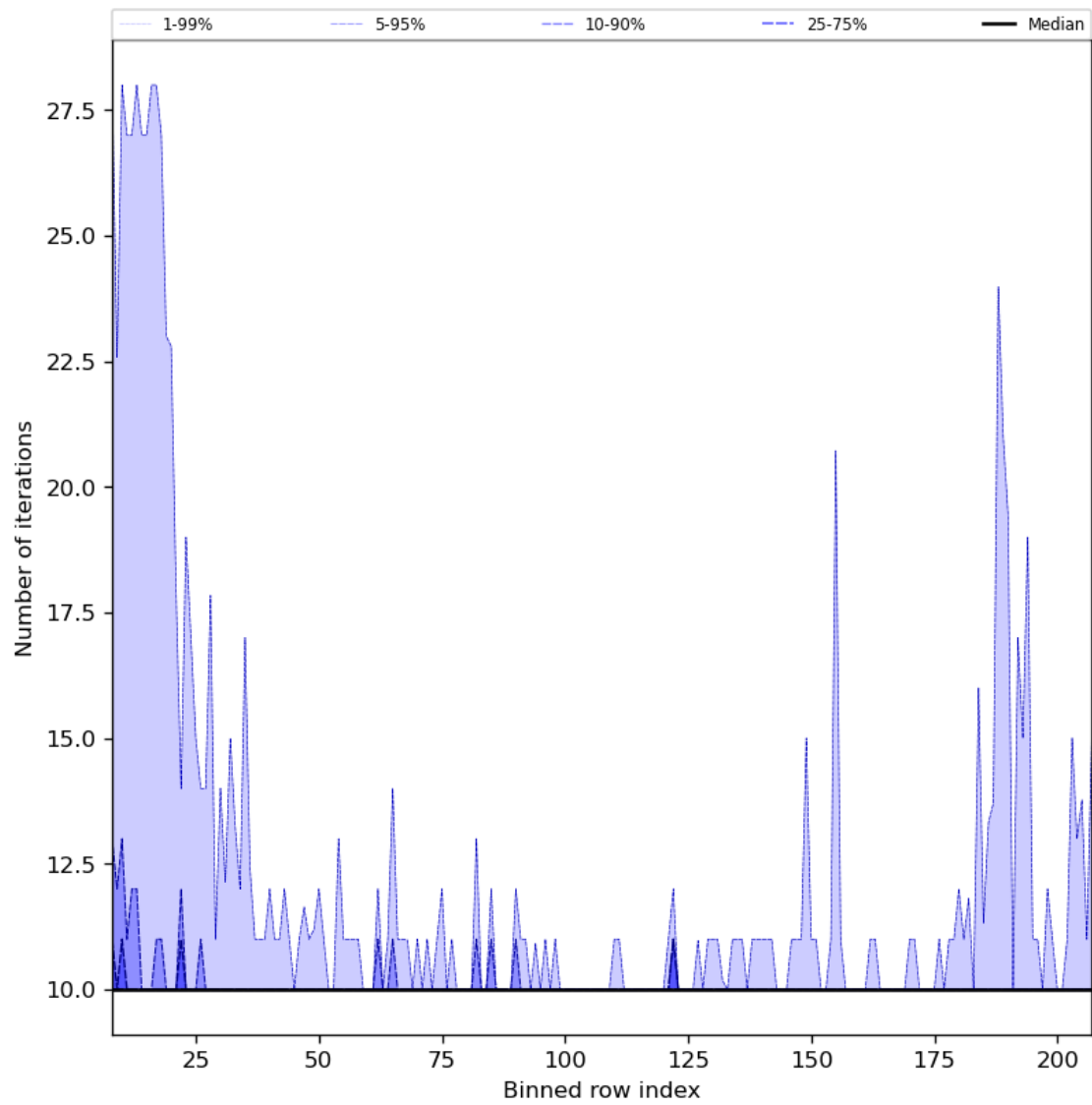
Figure 42: Along track statistics of “Number of iterations” for 2024-01-31 to 2024-02-01
