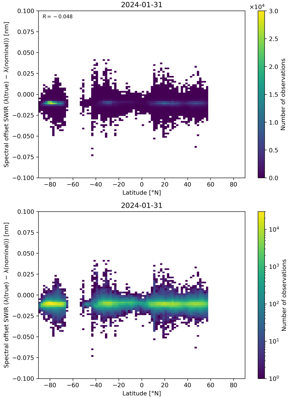
Figure 62: Scatter density plot of “Latitude” against “Spectral offset SWIR ( \lambda(\text{true}) - \lambda(\text{nominal}) )” for 2024-01-31 to 2024-02-01.
