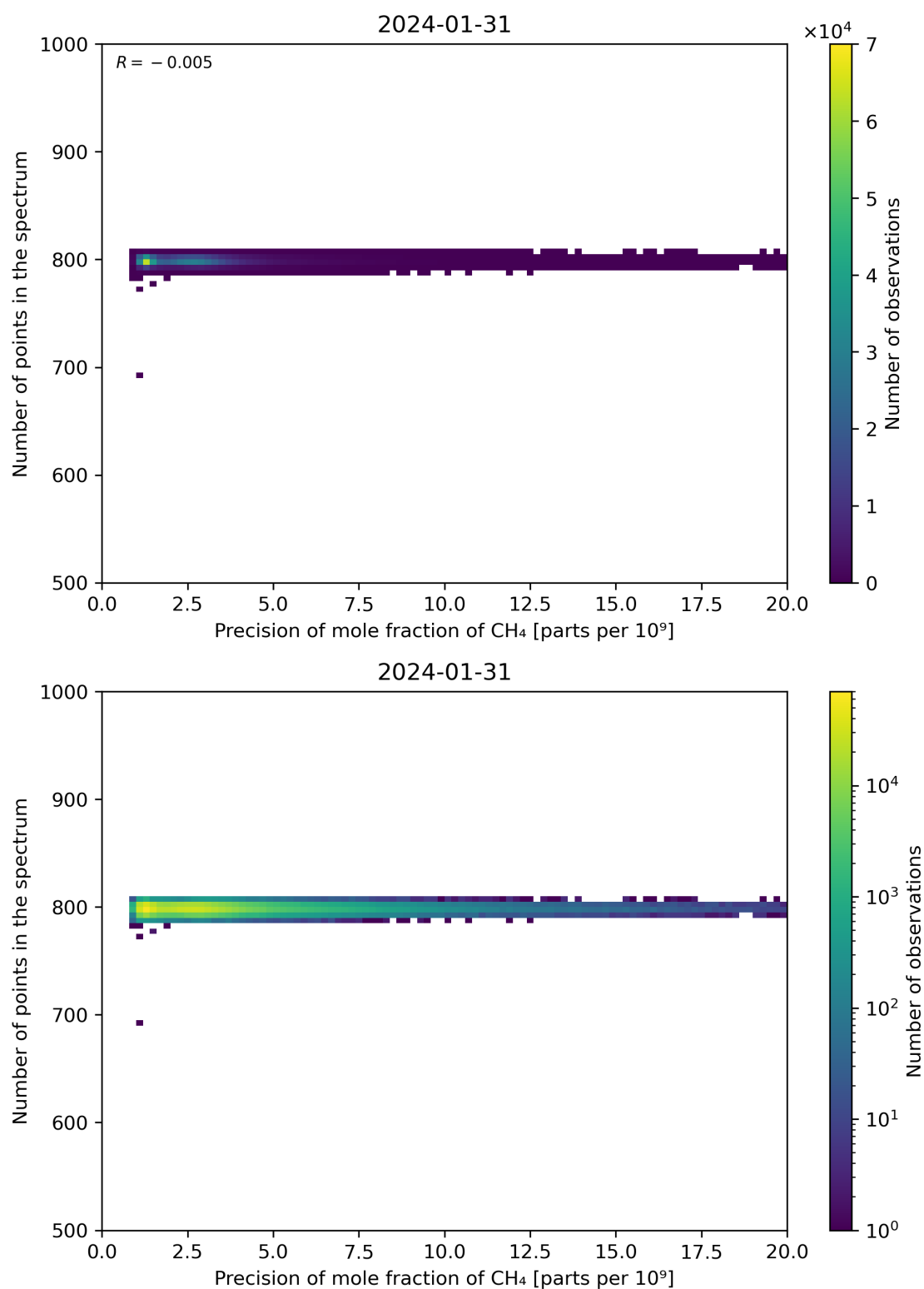
Figure 84: Scatter density plot of “Precision of mole fraction of CH 4 ” against “Number of points in the spectrum” for 2024-01-31 to 2024-02-01.
