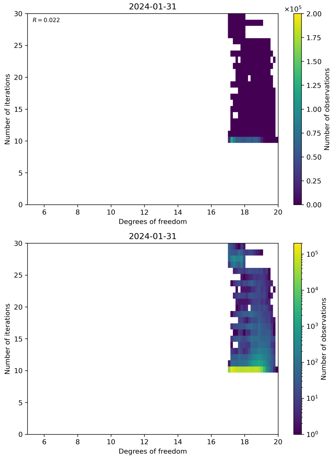
Figure 52: Scatter density plot of “Degrees of freedom” against “Number of iterations” for 2024-01-31 to 2024-02-01.
