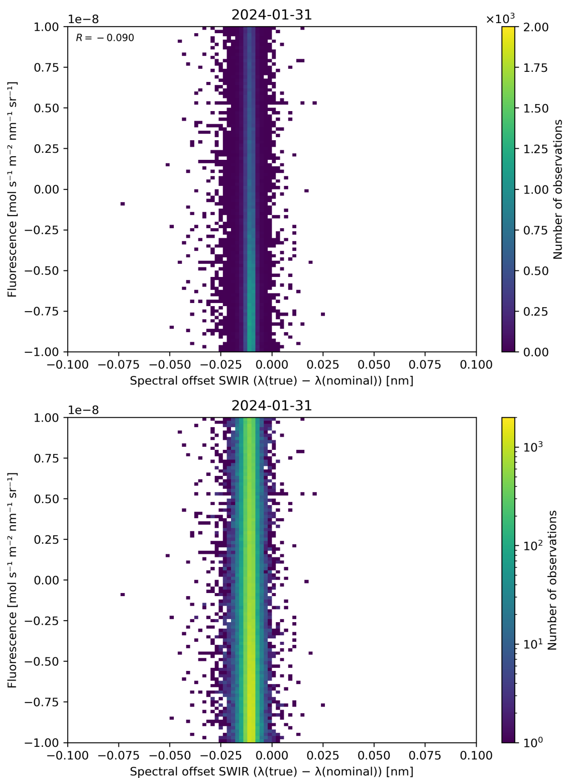
Figure 120: Scatter density plot of “Spectral offset SWIR ( \lambda(\text{true}) - \lambda(\text{nominal}) )” against “Fluorescence” for 2024-01-31 to 2024-02-01.
