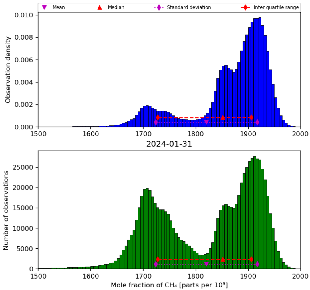
Figure 23: Histogram of “Mole fraction of CH 4 ” for 2024-01-31 to 2024-02-01
