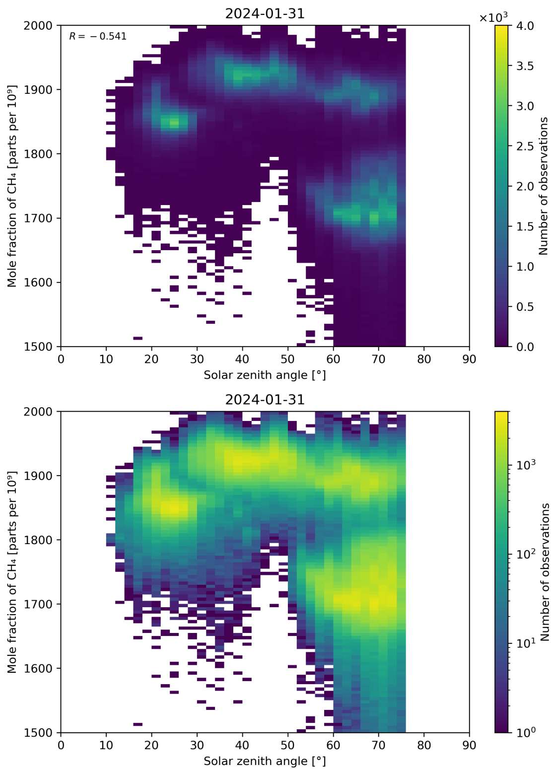
Figure 99: Scatter density plot of “Solar zenith angle” against “Mole fraction of CH 4 ” for 2024-01-31 to 2024-02-01.
