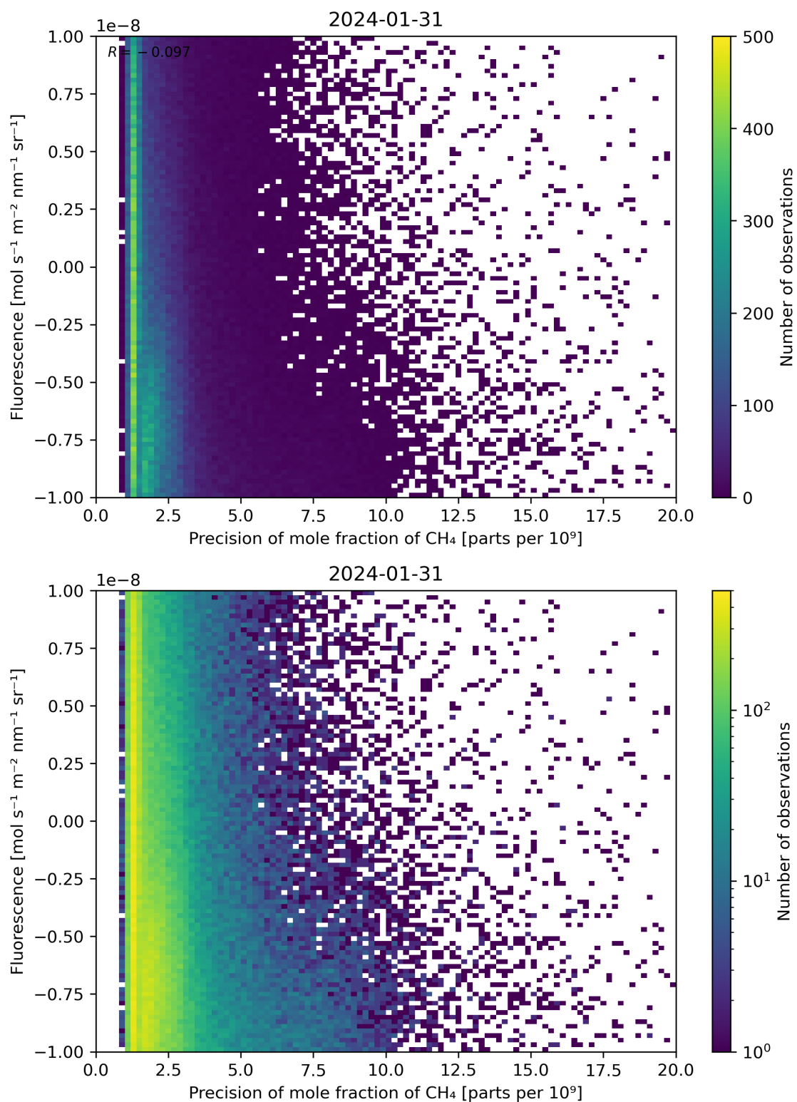
Figure 81: Scatter density plot of “Precision of mole fraction of CH 4 ” against “Fluorescence” for 2024-01-31 to 2024-02-01.
