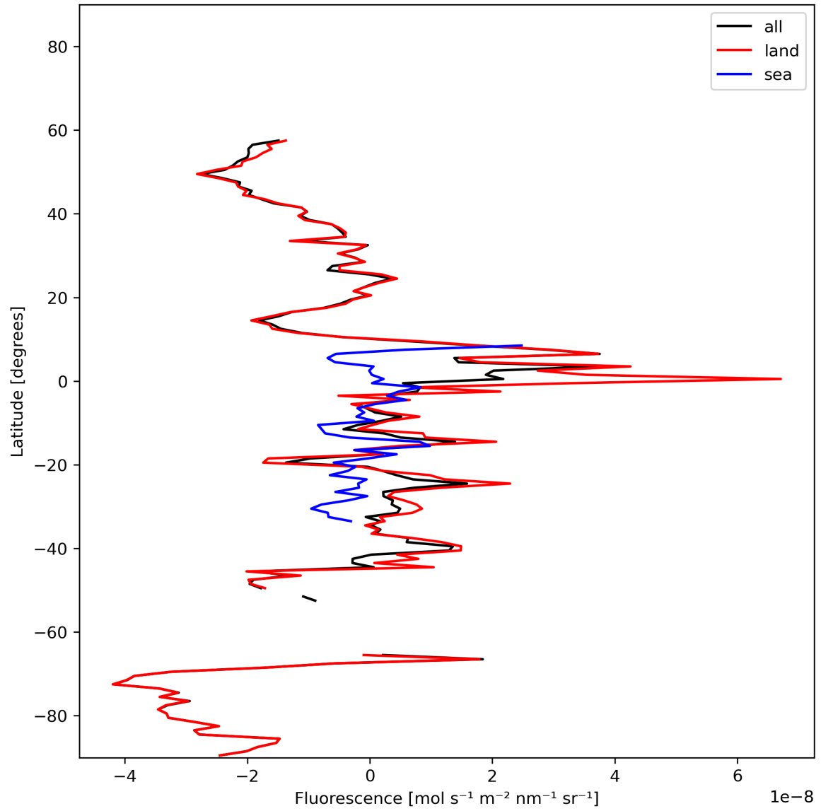
Figure 21: Zonal average of “Fluorescence” for 2024-01-31 to 2024-02-01.
