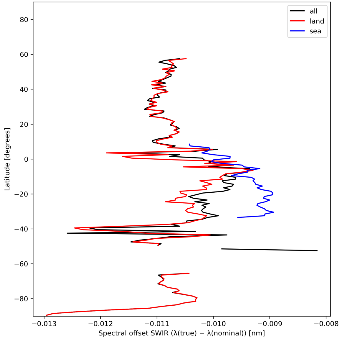
Figure 16: Zonal average of “Spectral offset SWIR ( \lambda(\text{true}) - \lambda(\text{nominal}) )” for 2024-01-31 to 2024-02-01.
