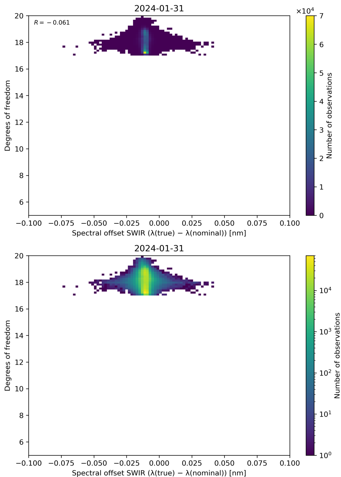
Figure 119: Scatter density plot of “Spectral offset SWIR ( \lambda(\text{true}) - \lambda(\text{nominal}) )” against “Degrees of freedom” for 2024-01-31 to 2024-02-01.
