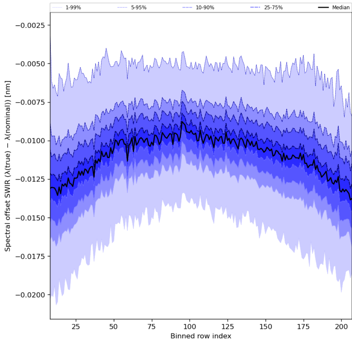
Figure 38: Along track statistics of “Spectral offset SWIR ( \lambda(\text{true}) - \lambda(\text{nominal}) )” for 2024-01-31 to 2024-02-01
