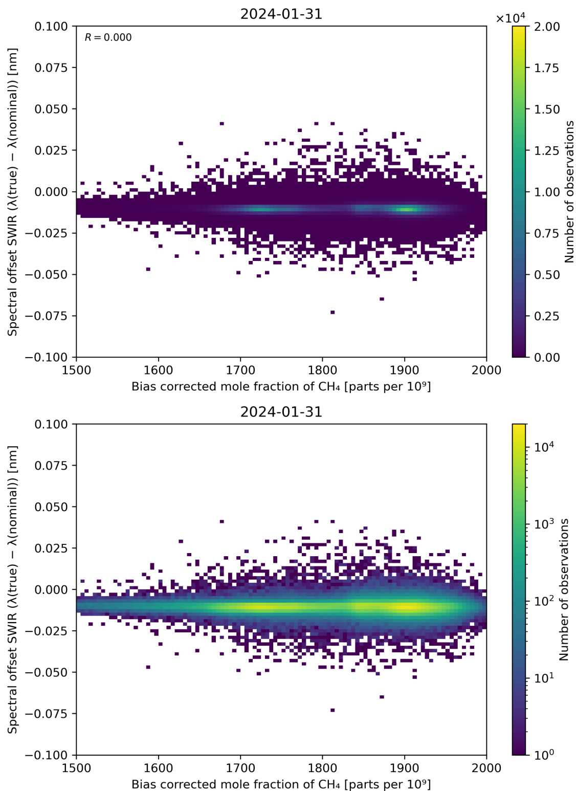
Figure 69: Scatter density plot of “Bias corrected mole fraction of \text{CH}_4 ” against “Spectral offset SWIR ( \lambda(\text{true}) - \lambda(\text{nominal}) )” for 2024-01-31 to 2024-02-01.
