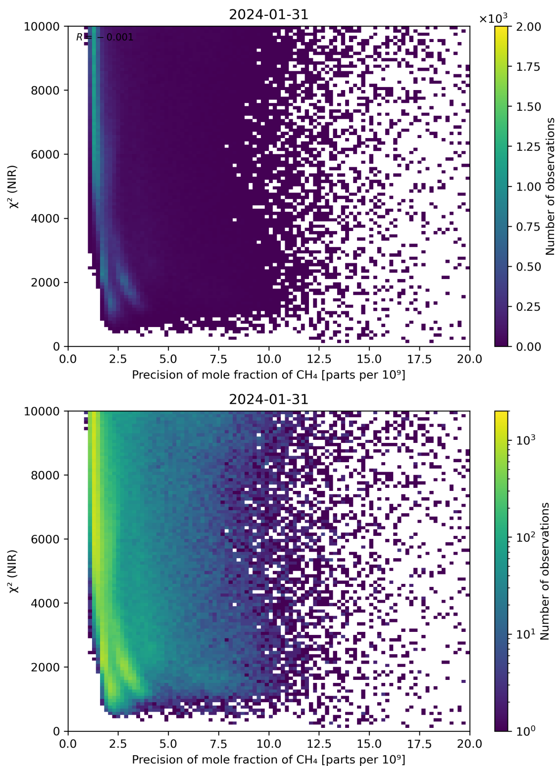
Figure 78: Scatter density plot of “Precision of mole fraction of \text{CH}_4 ” against “ \chi^2 (NIR)” for 2024-01-31 to 2024-02-01.
