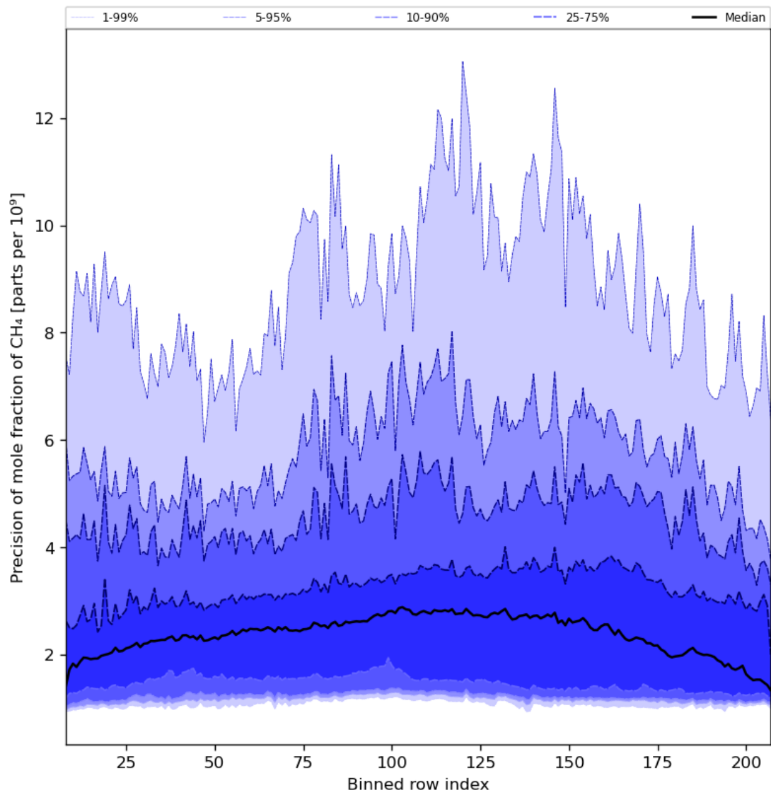
Figure 35: Along track statistics of “Precision of mole fraction of CH 4 ” for 2024-01-31 to 2024-02-01
