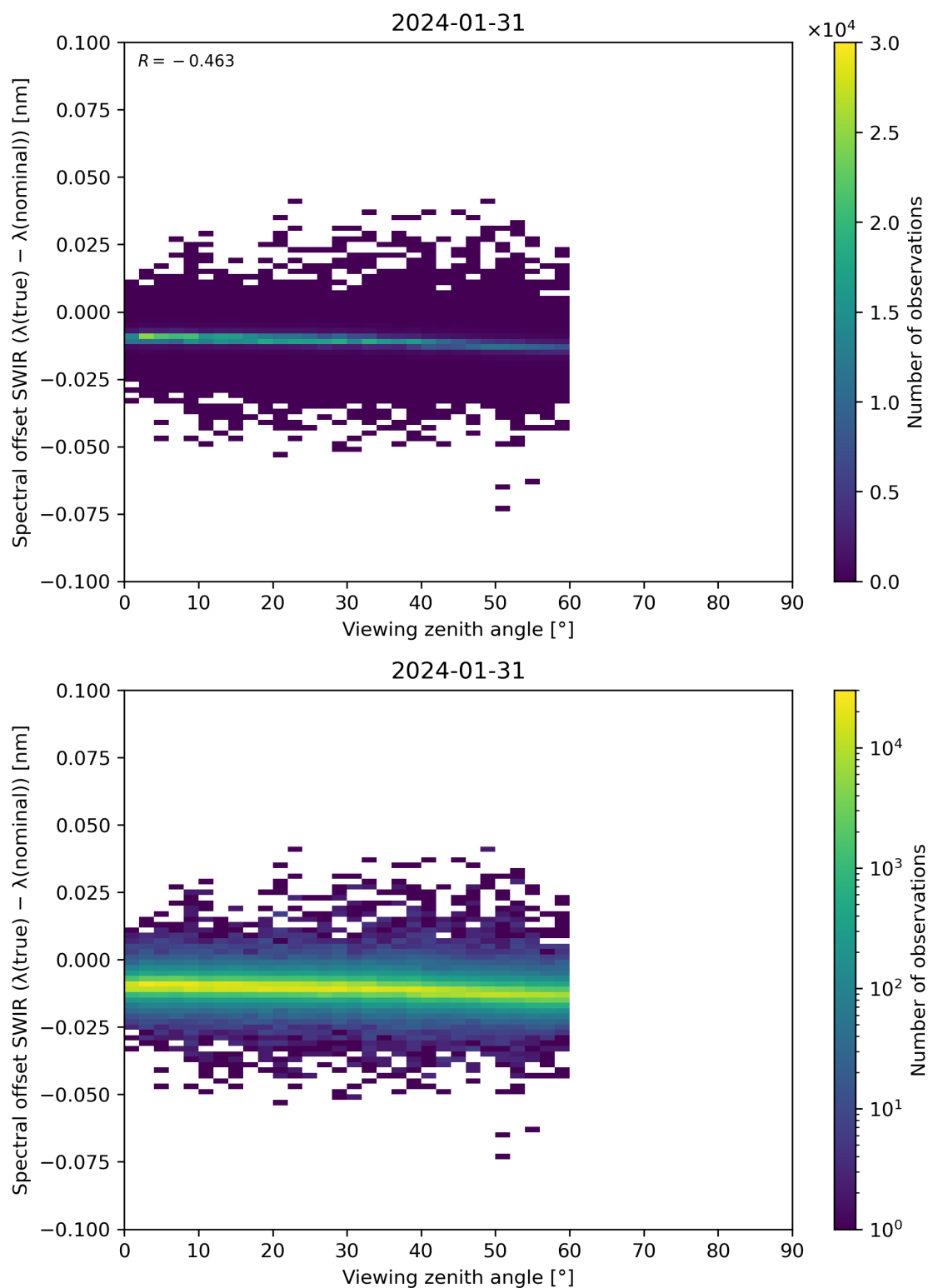
Figure 116: Scatter density plot of “Viewing zenith angle” against “Spectral offset SWIR ( \lambda(\text{true}) - \lambda(\text{nominal}) )” for 2024-01-31 to 2024-02-01.
