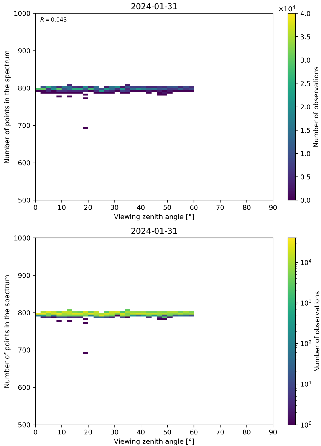
Figure 114: Scatter density plot of “Viewing zenith angle” against “Number of points in the spectrum” for 2024-01-31 to 2024-02-01.
