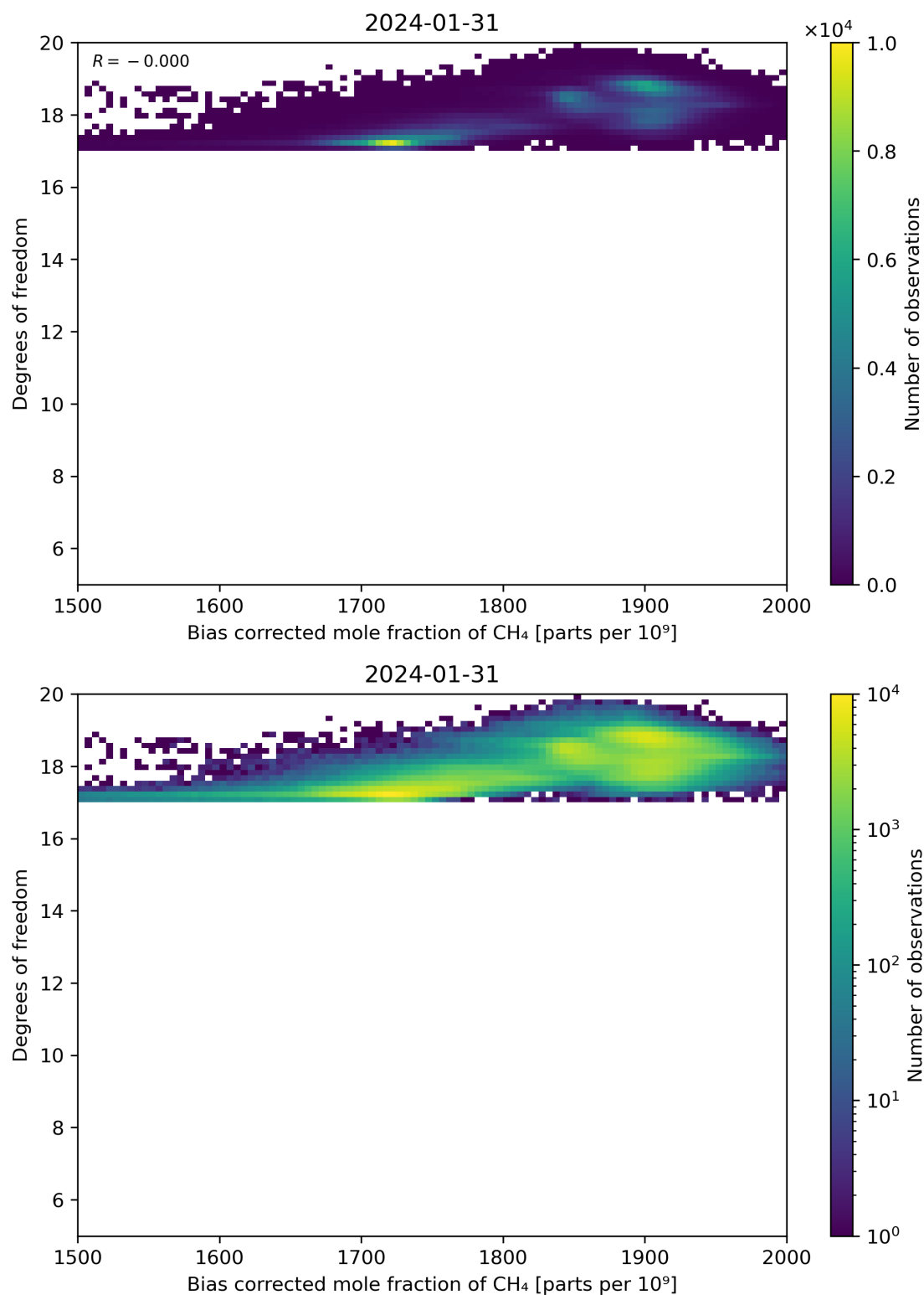
Figure 65: Scatter density plot of “Bias corrected mole fraction of CH 4 ” against “Degrees of freedom” for 2024-01-31 to 2024-02-01.
