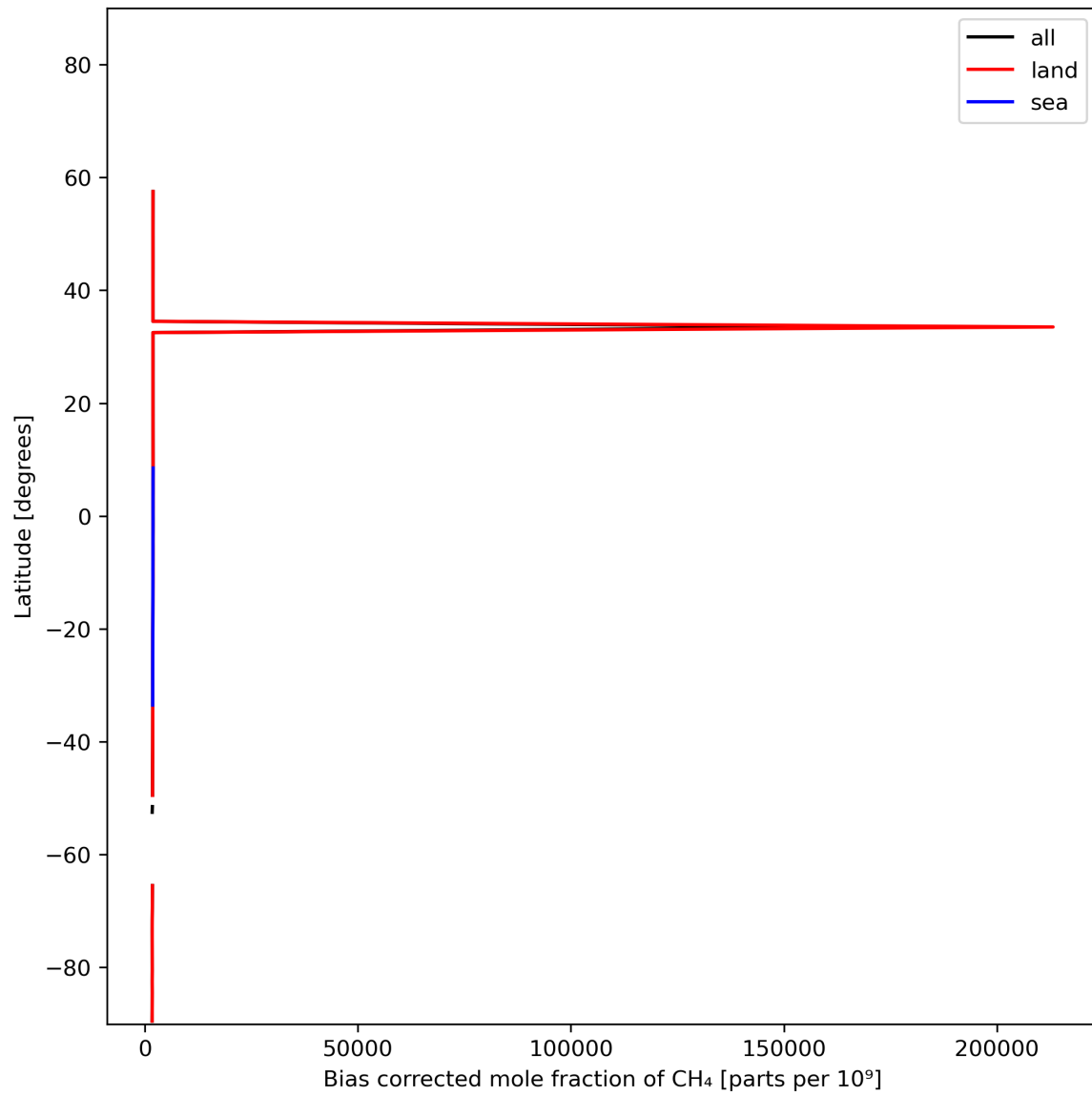
Figure 14: Zonal average of “Bias corrected mole fraction of CH 4 ” for 2024-01-31 to 2024-02-01.
