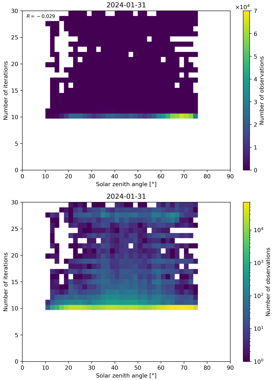
Figure 102: Scatter density plot of “Solar zenith angle” against “Number of iterations” for 2024-01-31 to 2024-02-01.
