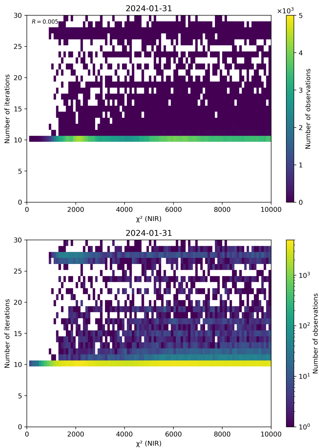
Figure 46: Scatter density plot of “ \chi^2 (NIR)” against “Number of iterations” for 2024-01-31 to 2024-02-01.
