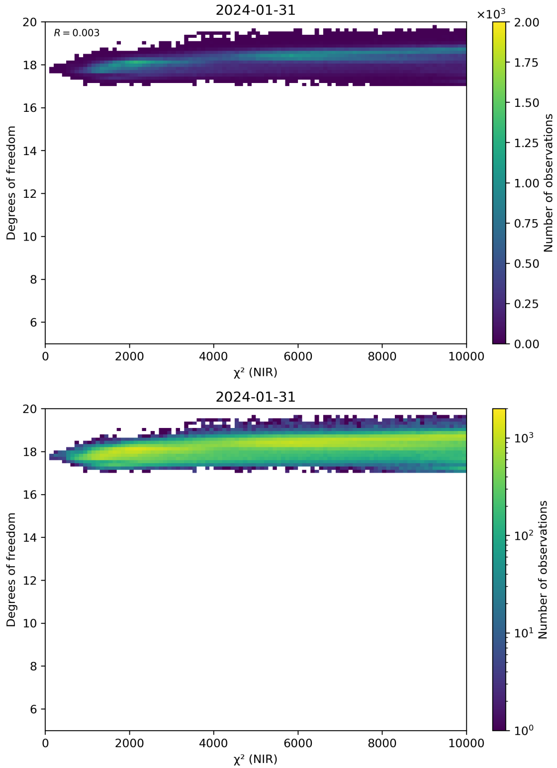
Figure 44: Scatter density plot of “ \chi^2 (NIR)” against “Degrees of freedom” for 2024-01-31 to 2024-02-01.
