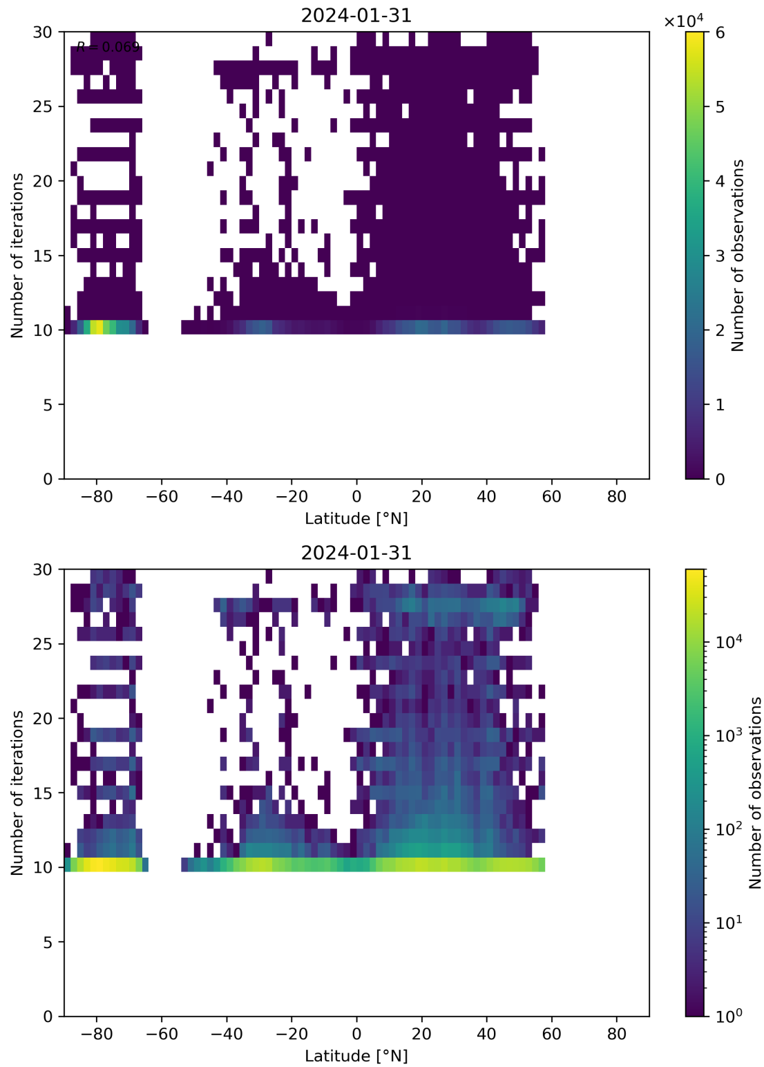
Figure 60: Scatter density plot of “Latitude” against “Number of iterations” for 2024-01-31 to 2024-02-01.
