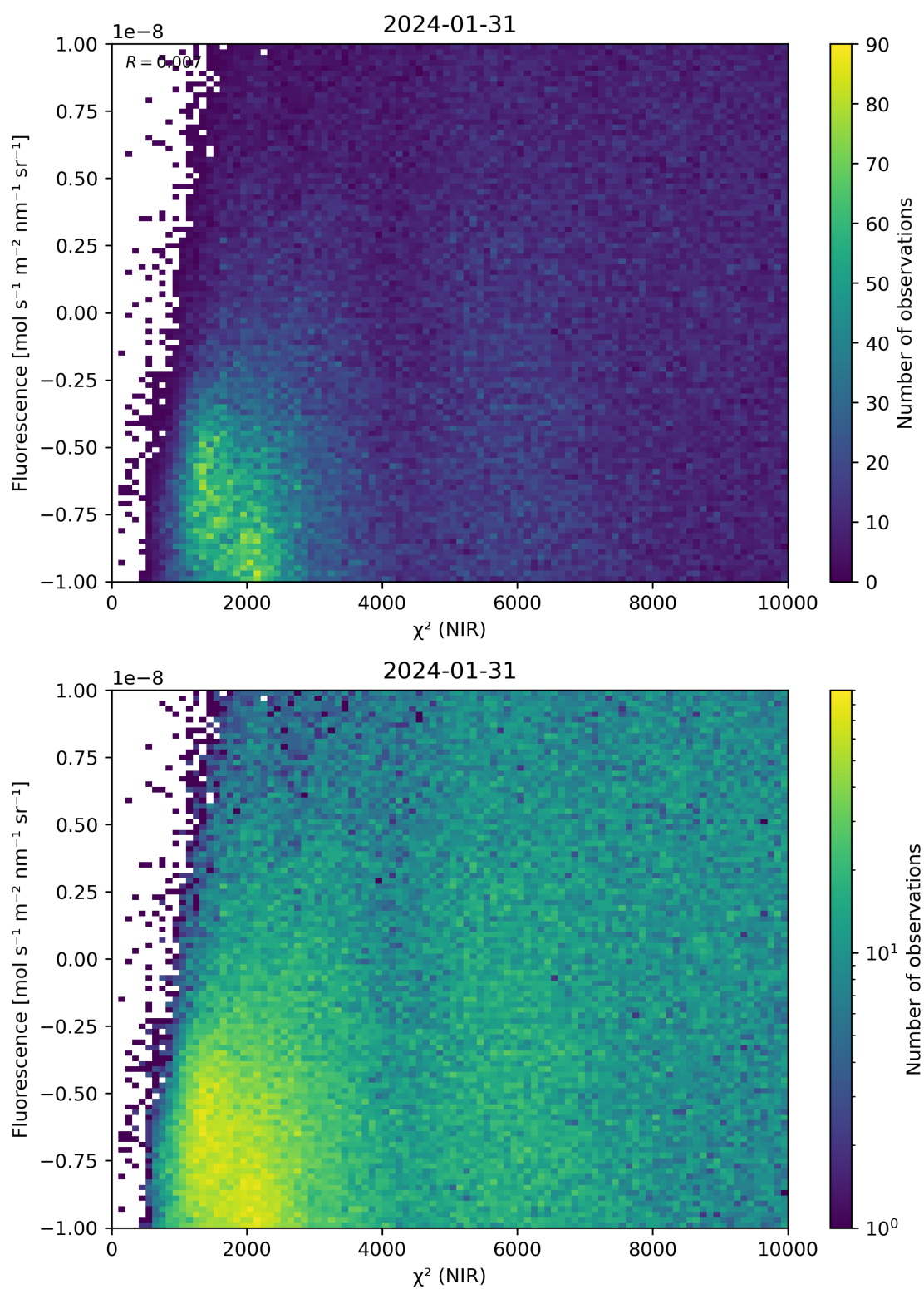
Figure 45: Scatter density plot of “ \chi^2 (NIR)” against “Fluorescence” for 2024-01-31 to 2024-02-01.
