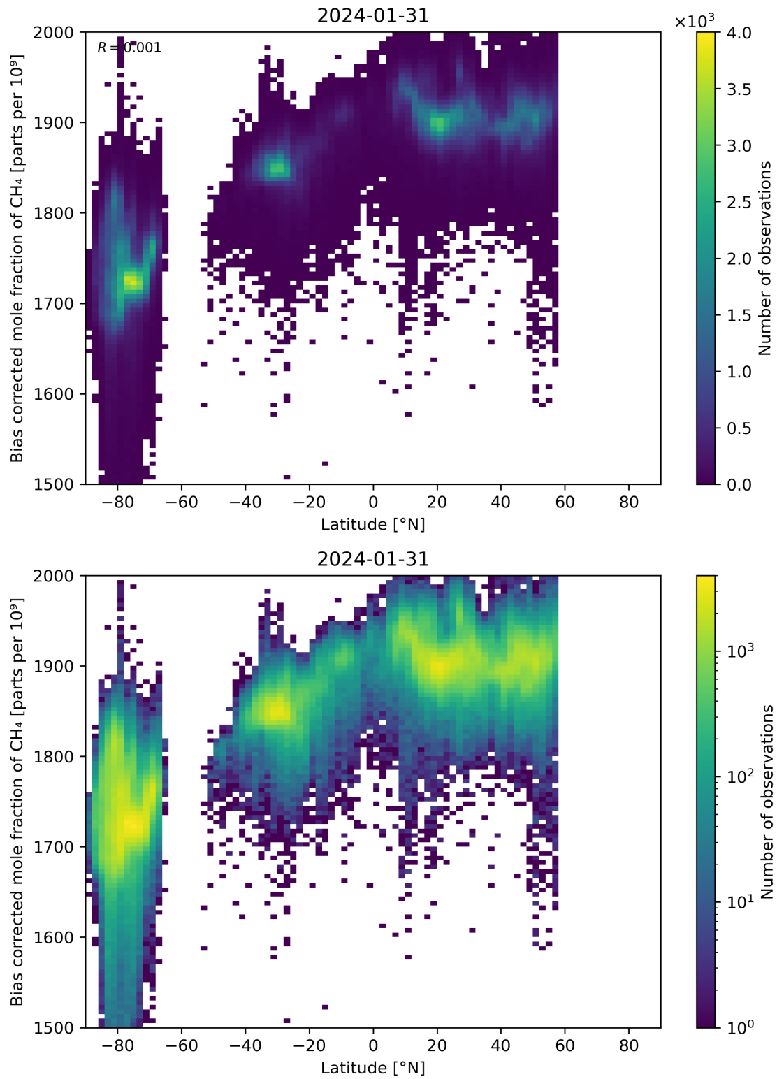
Figure 58: Scatter density plot of “Latitude” against “Bias corrected mole fraction of CH 4 ” for 2024-01-31 to 2024-02-01.
