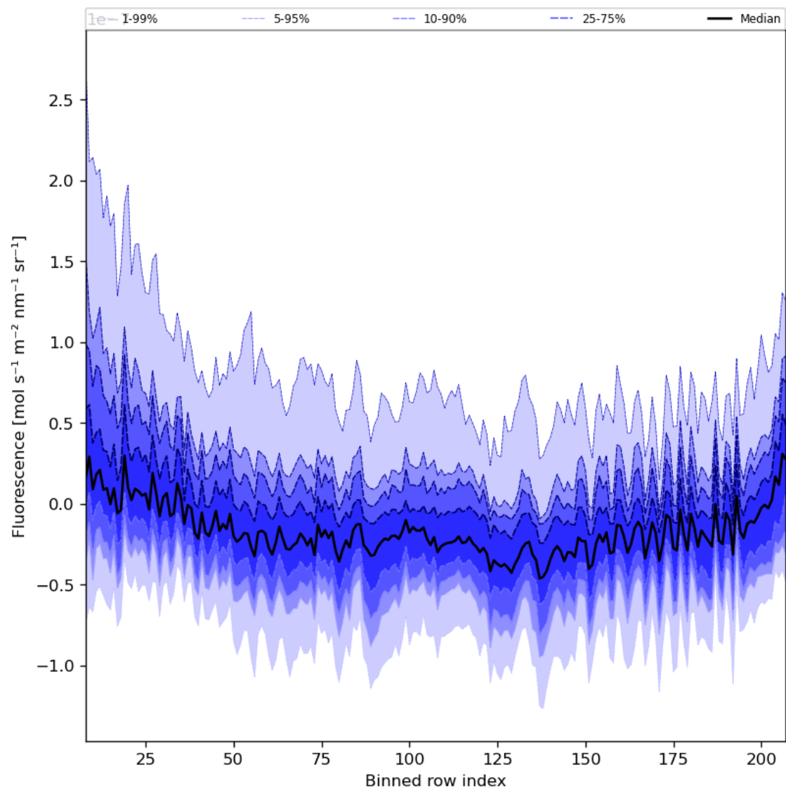
Figure 43: Along track statistics of “Fluorescence” for 2024-01-31 to 2024-02-01
