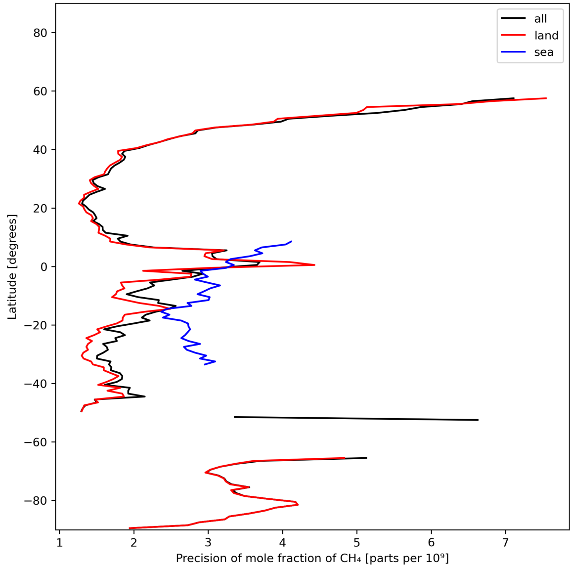
Figure 13: Zonal average of “Precision of mole fraction of CH 4 ” for 2024-01-31 to 2024-02-01.
