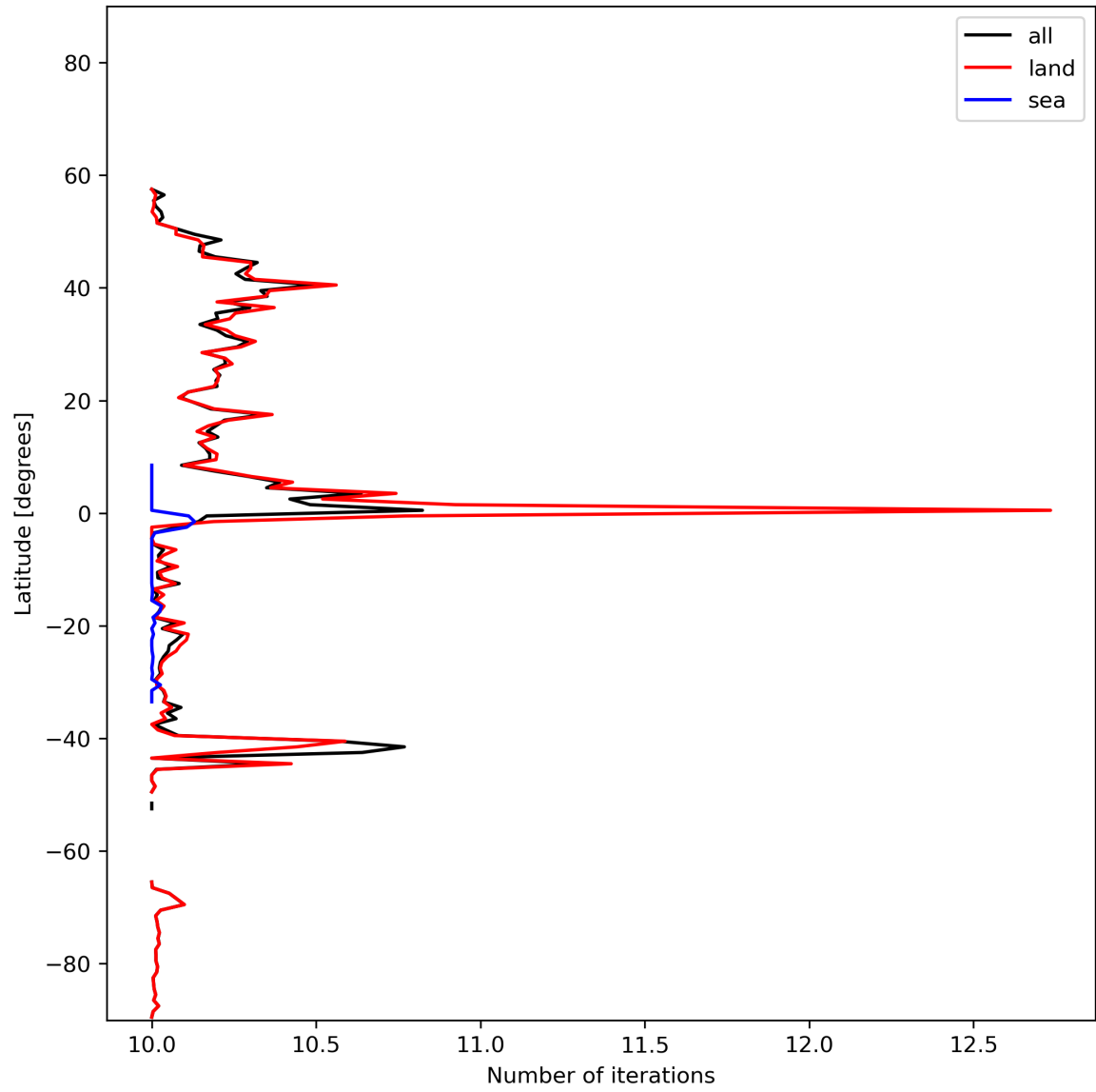
Figure 20: Zonal average of “Number of iterations” for 2024-01-31 to 2024-02-01.
