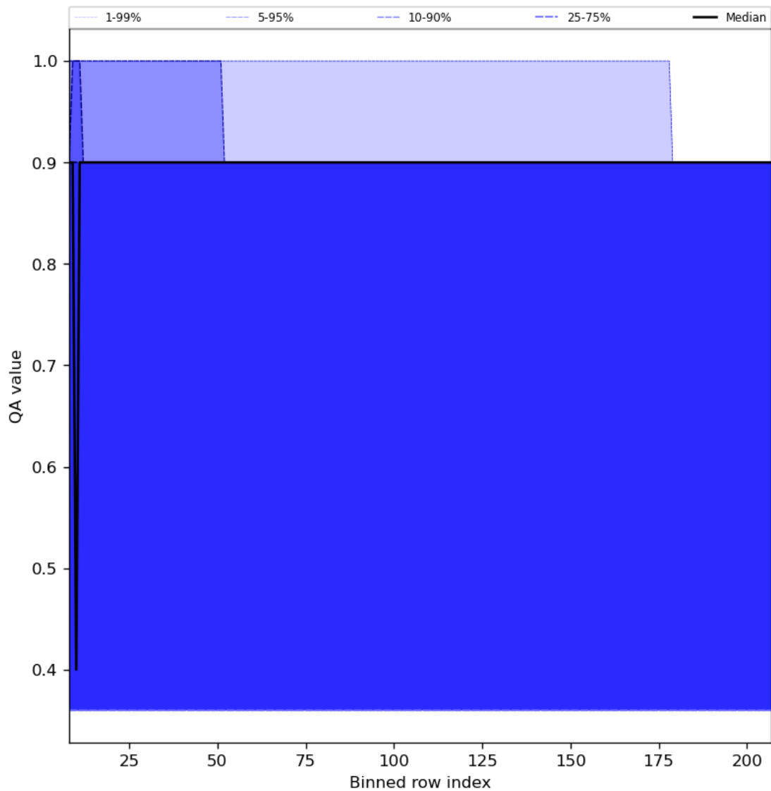
Figure 33: Along track statistics of “QA value” for 2024-01-31 to 2024-02-01
