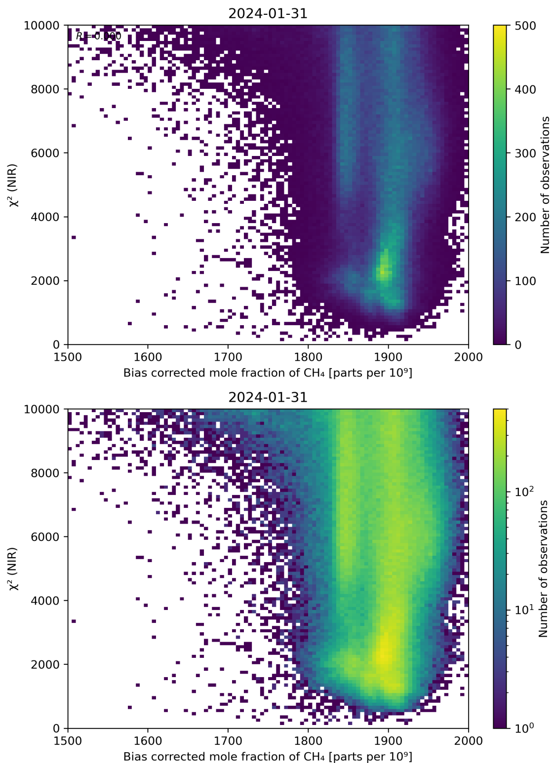
Figure 63: Scatter density plot of “Bias corrected mole fraction of \text{CH}_4 ” against “ \chi^2 (NIR)” for 2024-01-31 to 2024-02-01.
