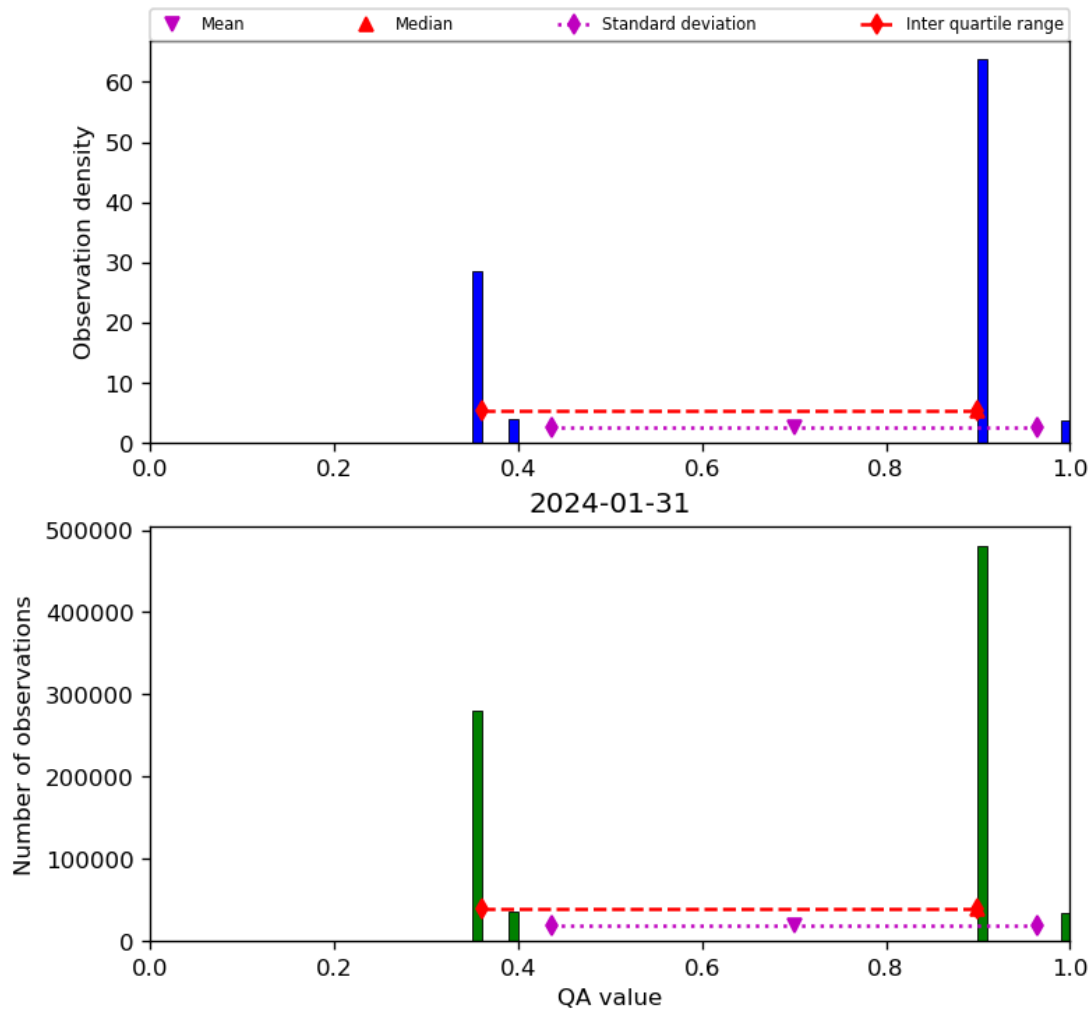
Figure 22: Histogram of “QA value” for 2024-01-31 to 2024-02-01
