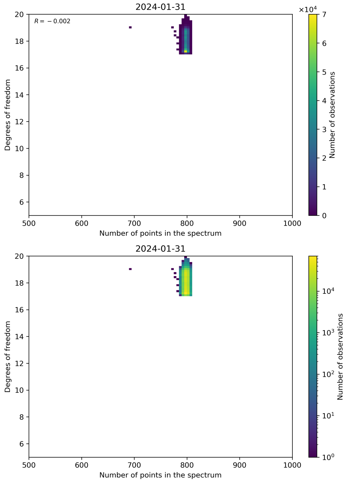
Figure 90: Scatter density plot of “Number of points in the spectrum” against “Degrees of freedom” for 2024-01-31 to 2024-02-01.
