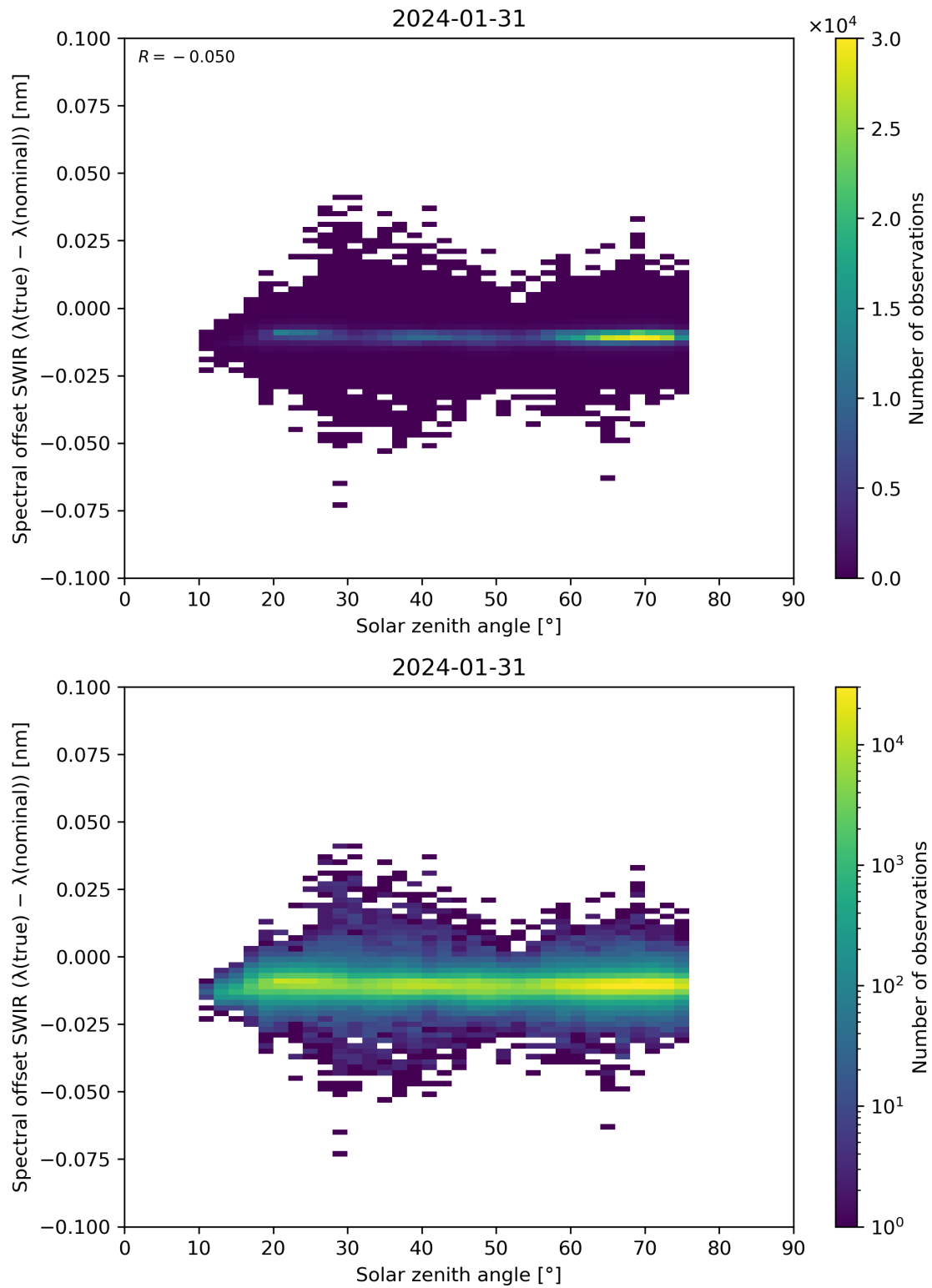
Figure 104: Scatter density plot of “Solar zenith angle” against “Spectral offset SWIR ( \lambda(\text{true}) - \lambda(\text{nominal}) )” for 2024-01-31 to 2024-02-01.
