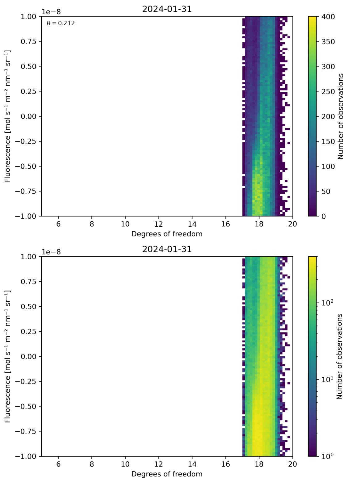
Figure 51: Scatter density plot of “Degrees of freedom” against “Fluorescence” for 2024-01-31 to 2024-02-01.
