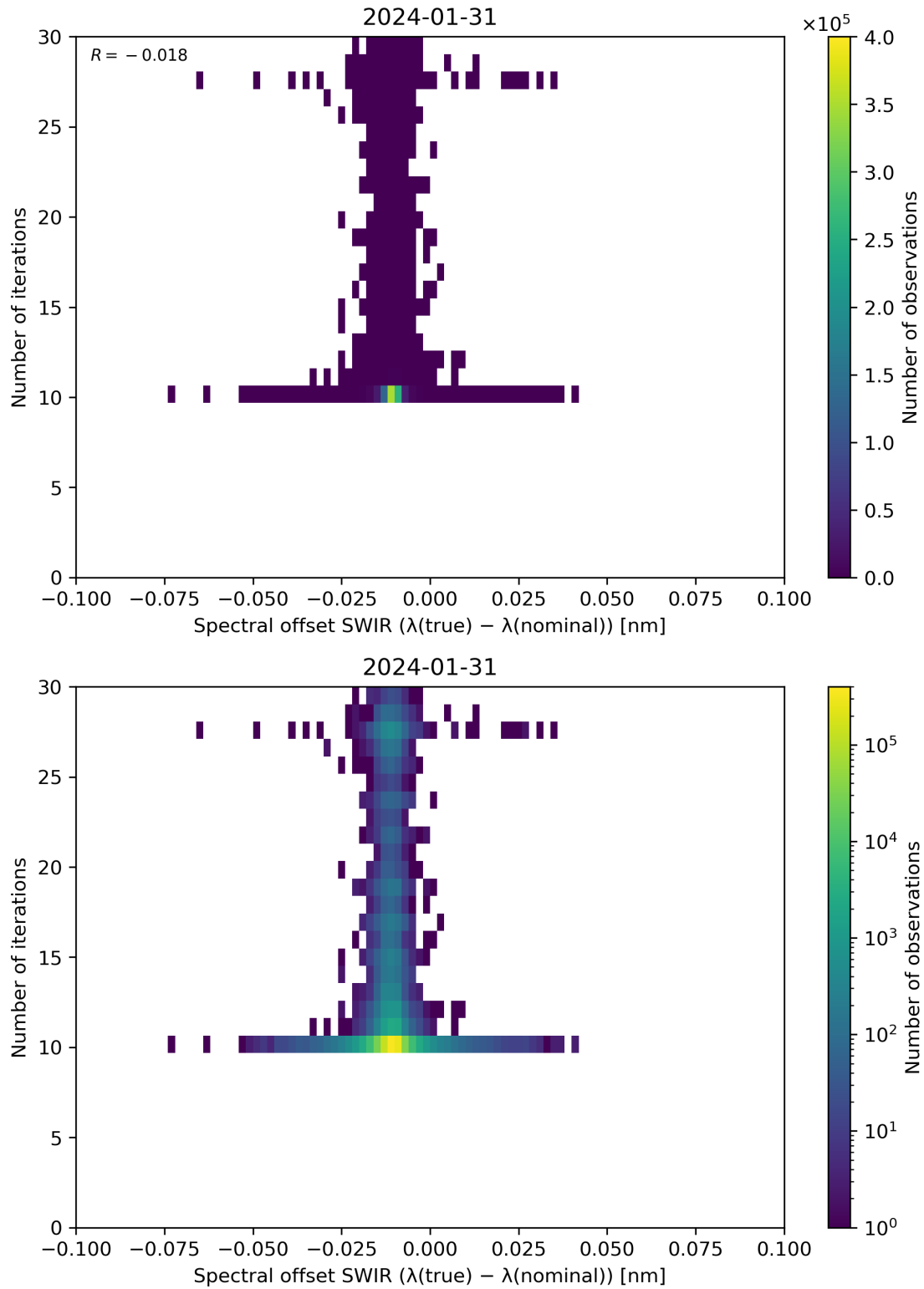
Figure 121: Scatter density plot of “Spectral offset SWIR ( \lambda(\text{true}) - \lambda(\text{nominal}) )” against “Number of iterations” for 2024-01-31 to 2024-02-01.
