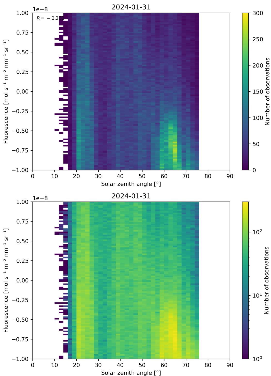
Figure 97: Scatter density plot of “Solar zenith angle” against “Fluorescence” for 2024-01-31 to 2024-02-01.
