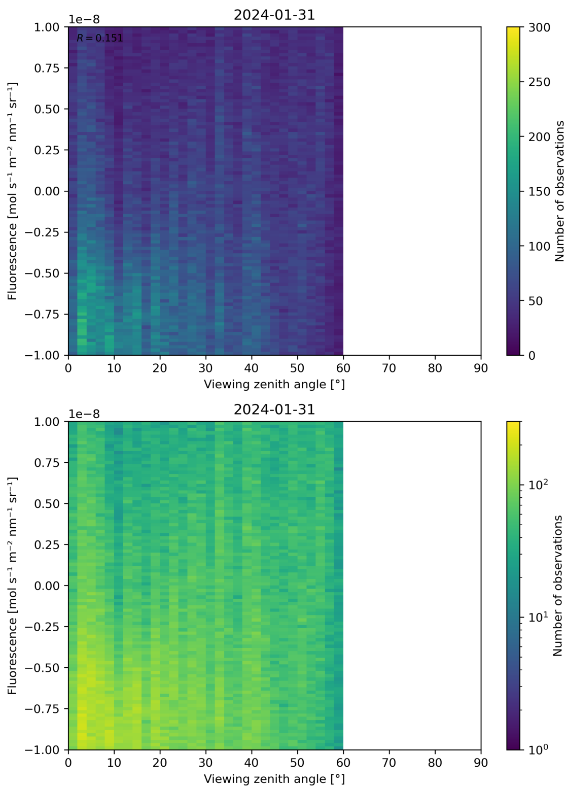
Figure 108: Scatter density plot of “Viewing zenith angle” against “Fluorescence” for 2024-01-31 to 2024-02-01.
