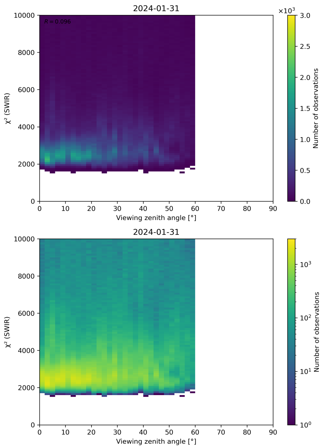
Figure 106: Scatter density plot of “Viewing zenith angle” against “ \chi^2 (SWIR)” for 2024-01-31 to 2024-02-01.
