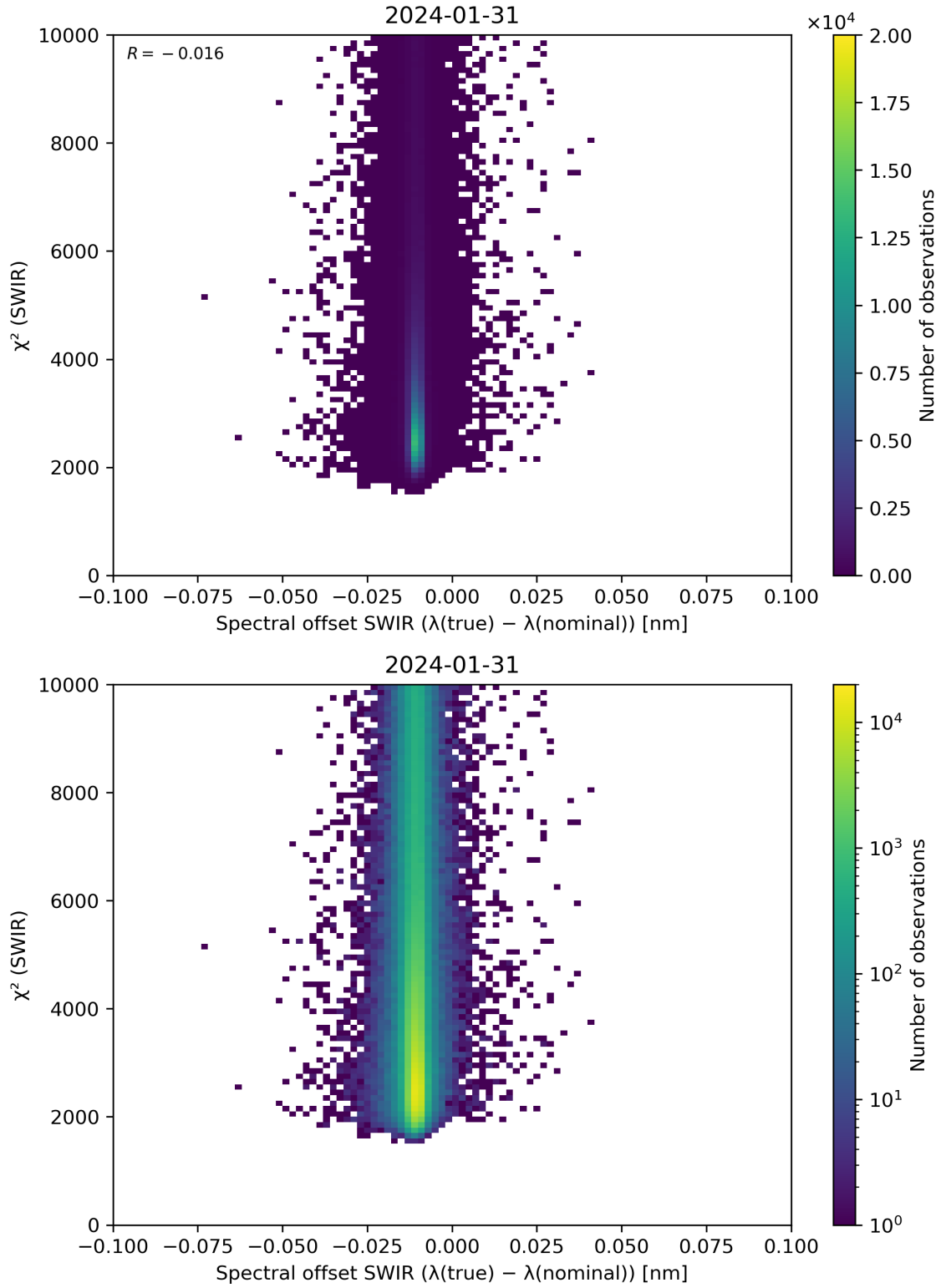
Figure 118: Scatter density plot of “Spectral offset SWIR ( \lambda(\text{true}) - \lambda(\text{nominal}) )” against “ \chi^2 (SWIR)” for 2024-01-31 to 2024-02-01.
