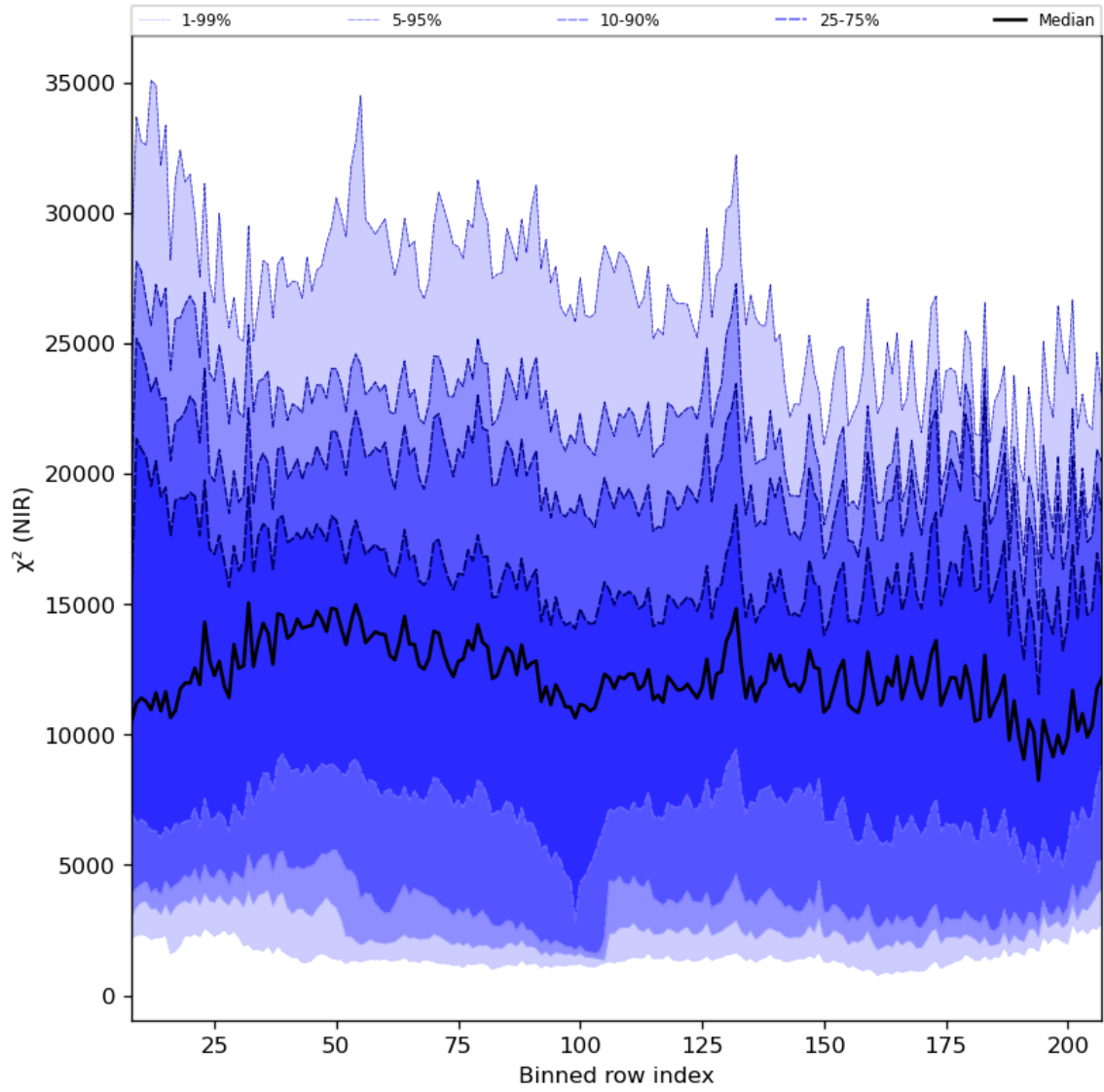
Figure 40: Along track statistics of “ \chi^2 (NIR)” for 2024-01-31 to 2024-02-01
