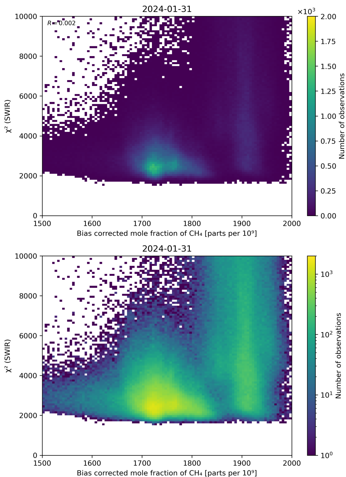
Figure 64: Scatter density plot of “Bias corrected mole fraction of CH 4 ” against “ \chi^2 (SWIR)” for 2024-01-31 to 2024-02-01.
