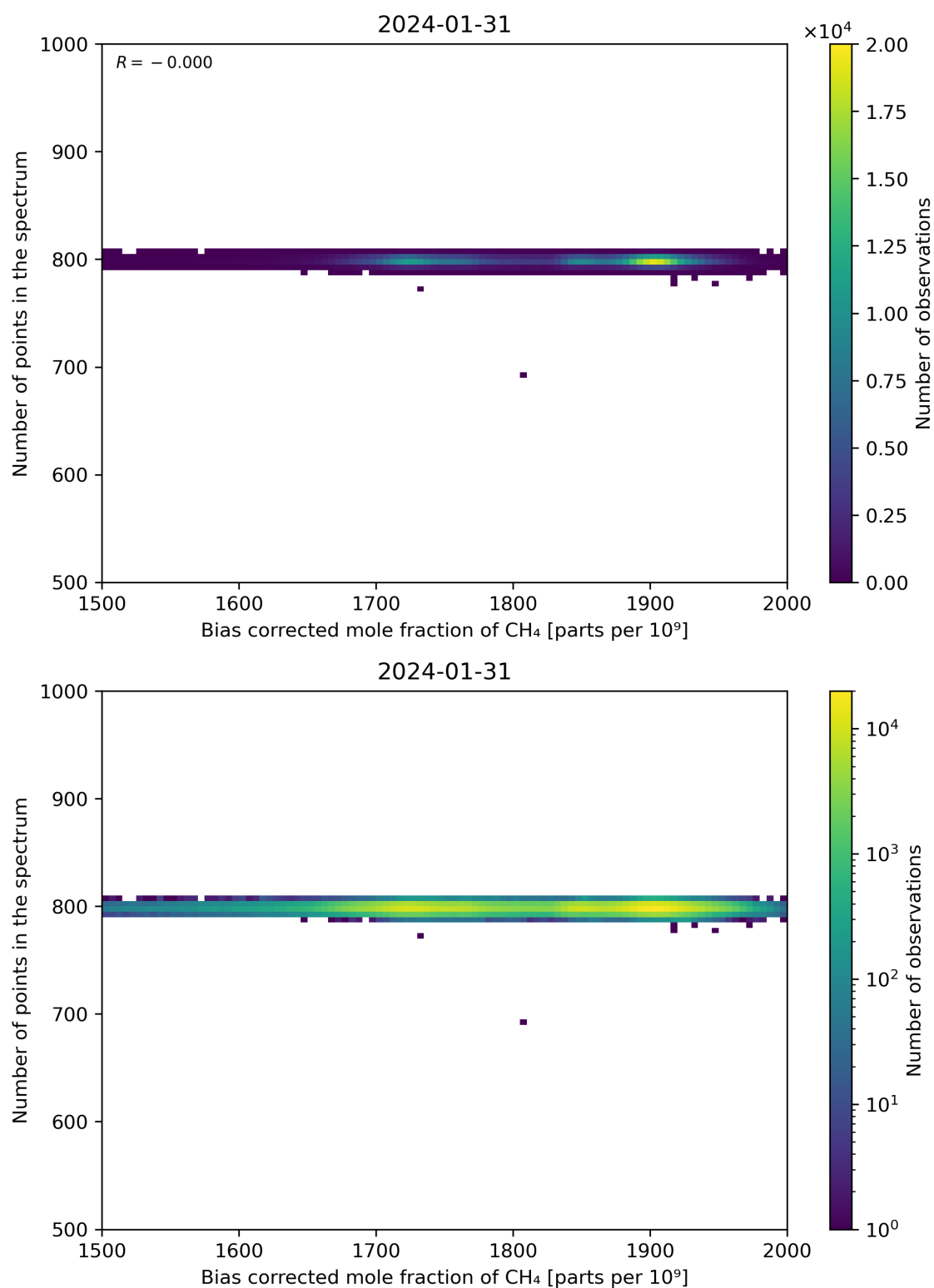
Figure 68: Scatter density plot of “Bias corrected mole fraction of CH 4 ” against “Number of points in the spectrum” for 2024-01-31 to 2024-02-01.
