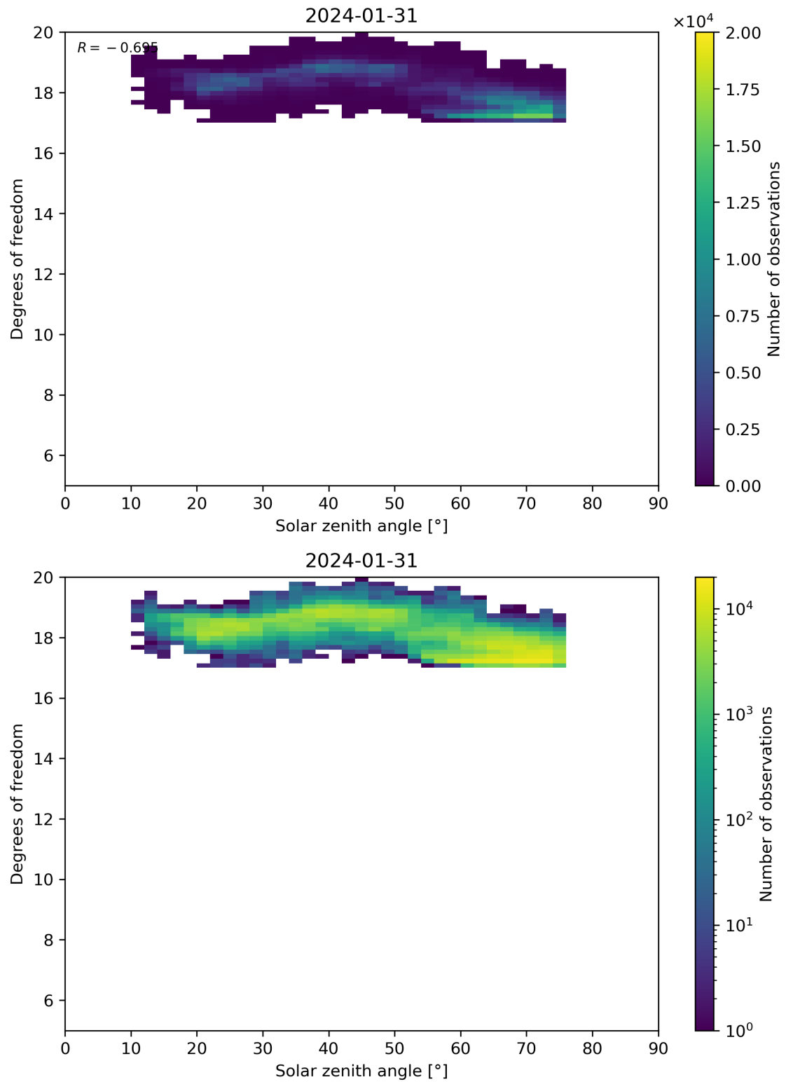
Figure 96: Scatter density plot of “Solar zenith angle” against “Degrees of freedom” for 2024-01-31 to 2024-02-01.
