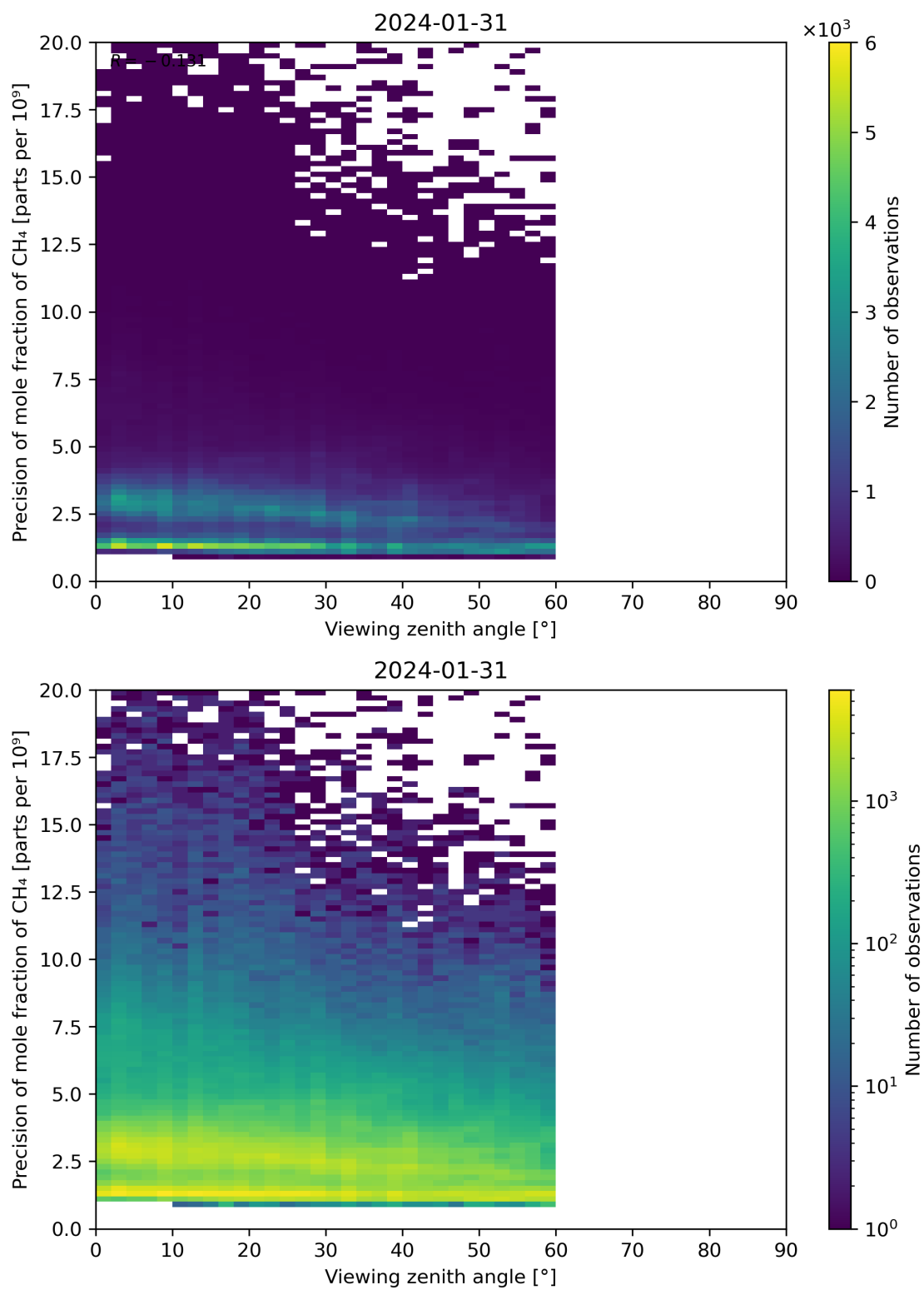
Figure 112: Scatter density plot of “Viewing zenith angle” against “Precision of mole fraction of CH 4 ” for 2024-01-31 to 2024-02-01.
