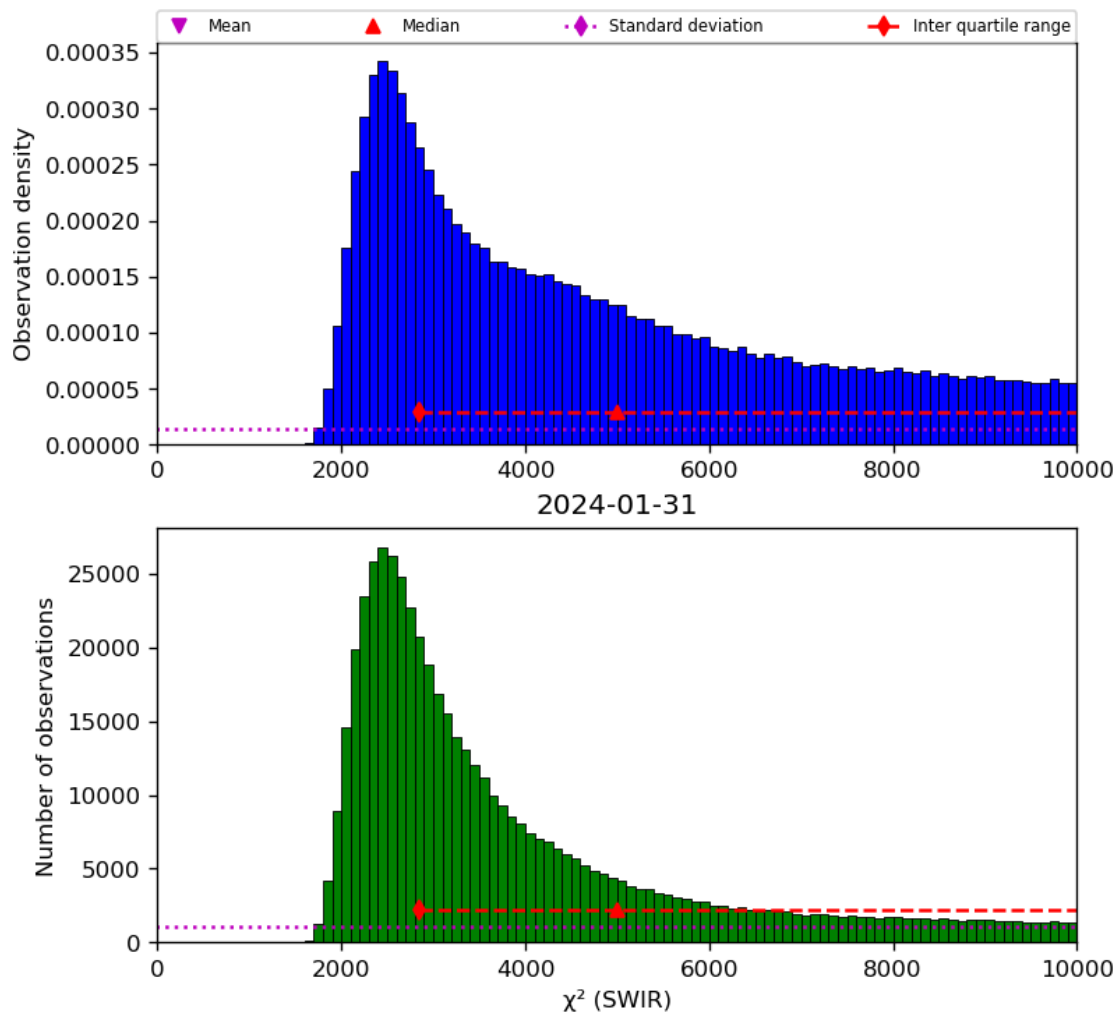
Figure 28: Histogram of “ \chi^2 (SWIR)” for 2024-01-31 to 2024-02-01
