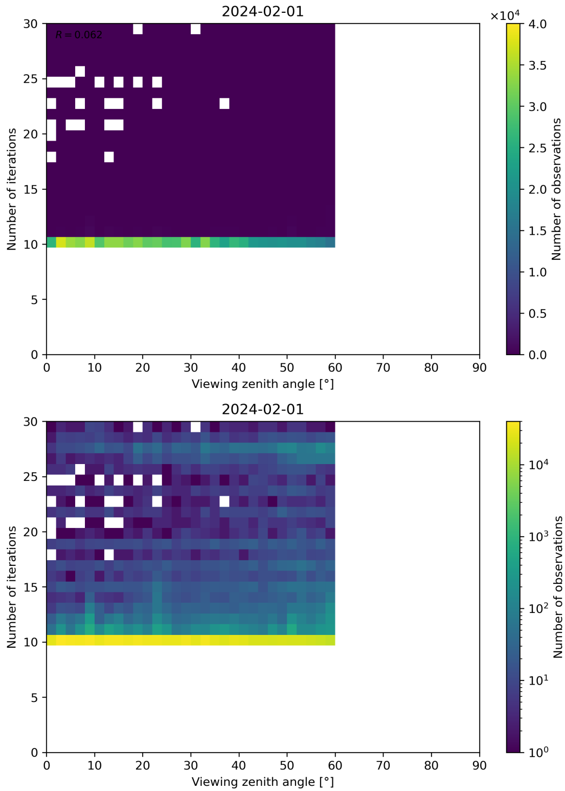
Figure 113: Scatter density plot of “Viewing zenith angle” against “Number of iterations” for 2024-01-31 to 2024-02-02.
