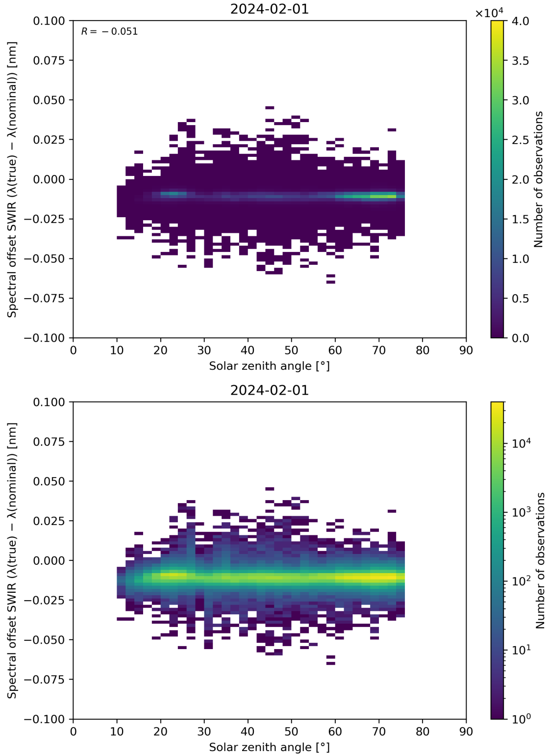
Figure 104: Scatter density plot of “Solar zenith angle” against “Spectral offset SWIR ( \lambda(\text{true}) - \lambda(\text{nominal}) )” for 2024-01-31 to 2024-02-02.
