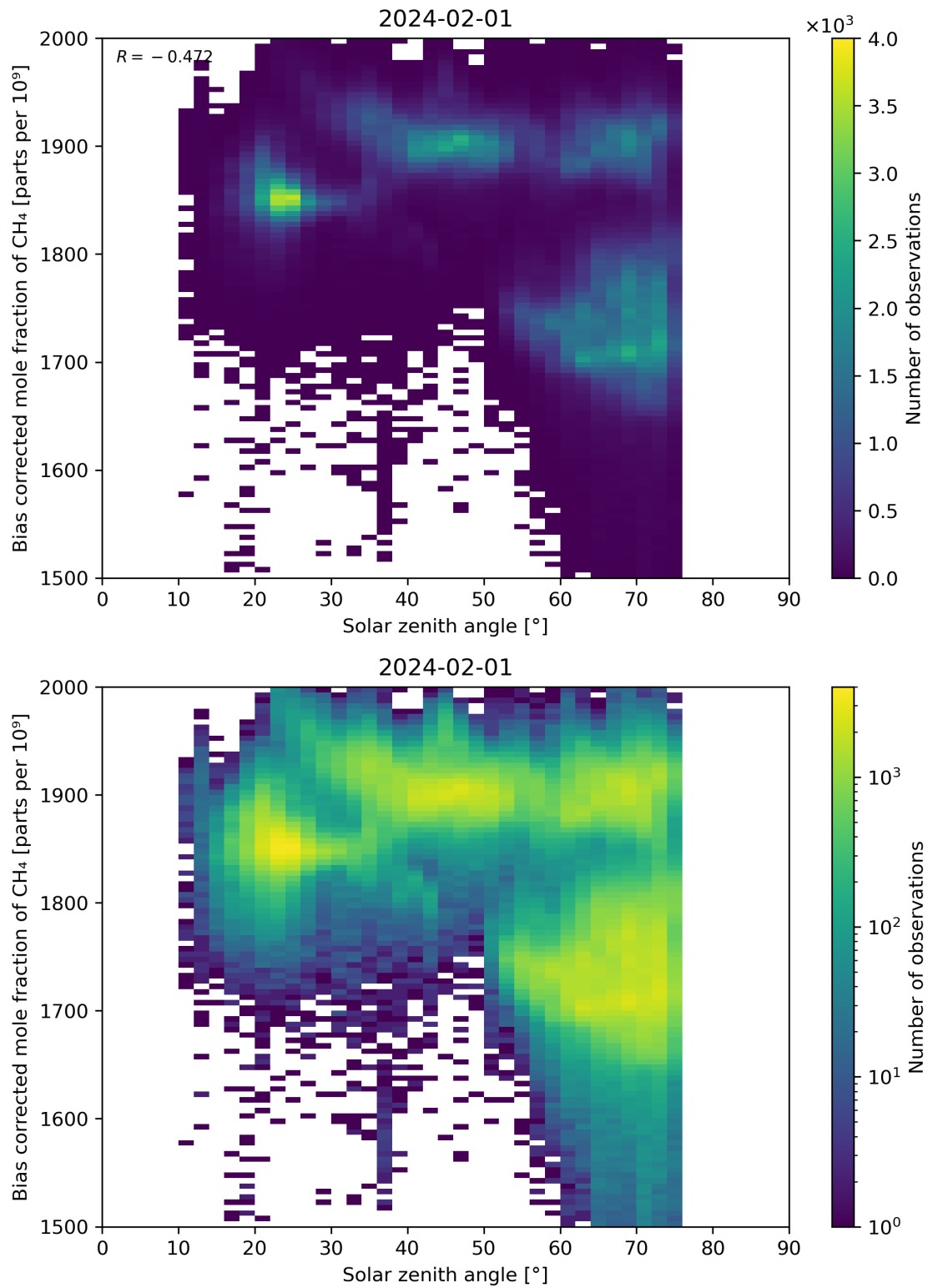
Figure 100: Scatter density plot of “Solar zenith angle” against “Bias corrected mole fraction of CH 4 ” for 2024-01-31 to 2024-02-02.
