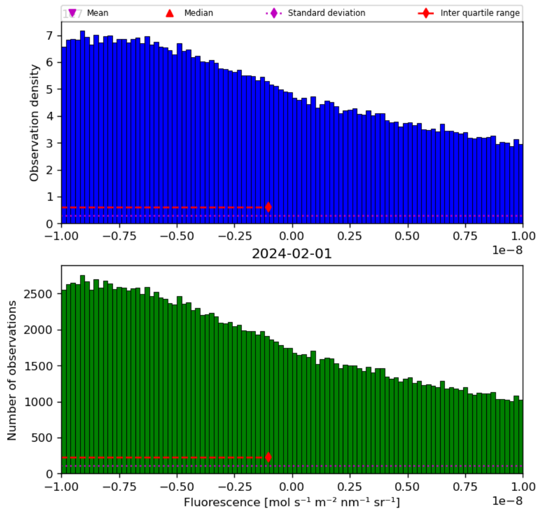
Figure 32: Histogram of “Fluorescence” for 2024-01-31 to 2024-02-02
