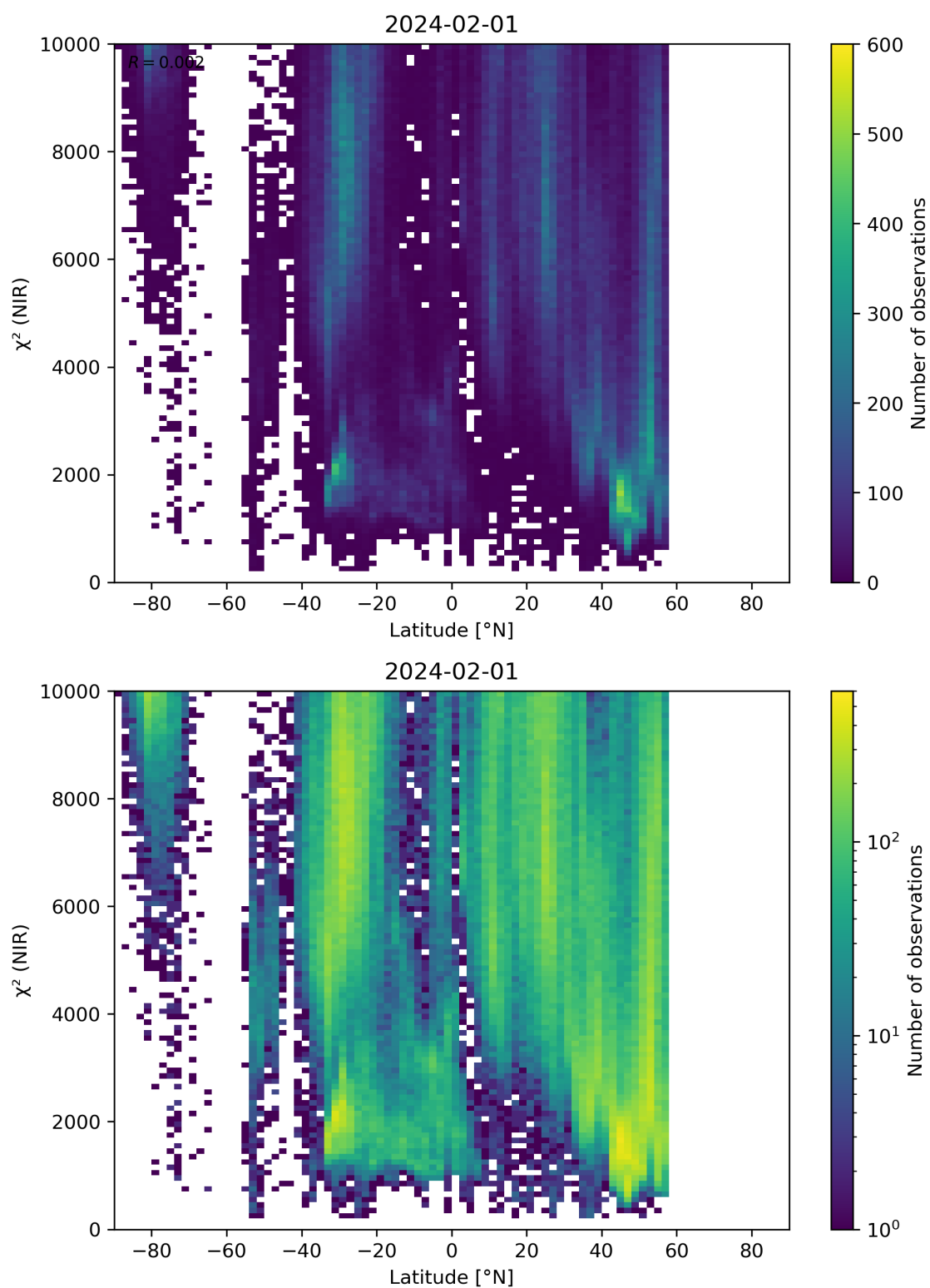
Figure 53: Scatter density plot of “Latitude” against “ \chi^2 (NIR)” for 2024-01-31 to 2024-02-02.
