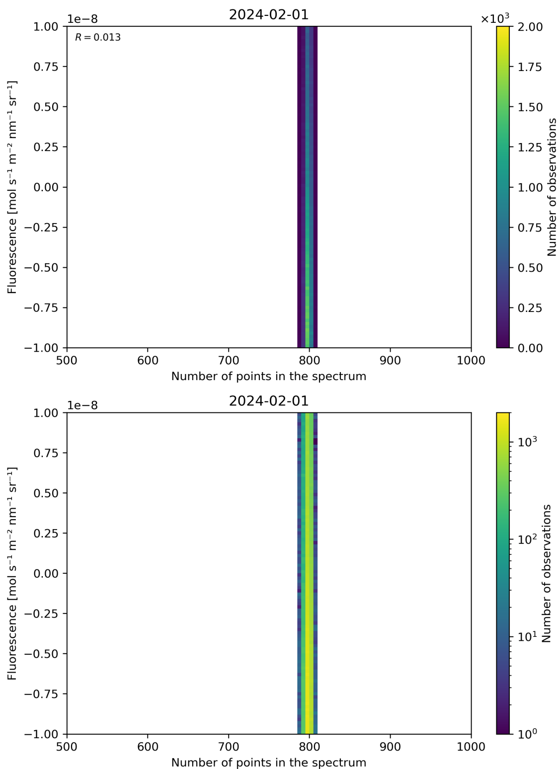
Figure 91: Scatter density plot of “Number of points in the spectrum” against “Fluorescence” for 2024-01-31 to 2024-02-02.
