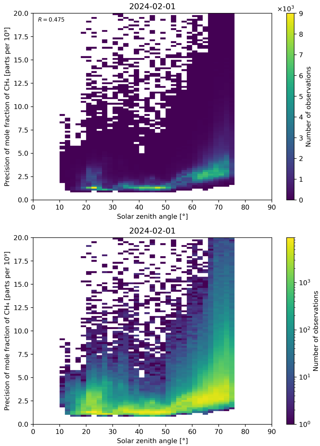
Figure 101: Scatter density plot of “Solar zenith angle” against “Precision of mole fraction of \text{CH}_4 ” for 2024-01-31 to 2024-02-02.
