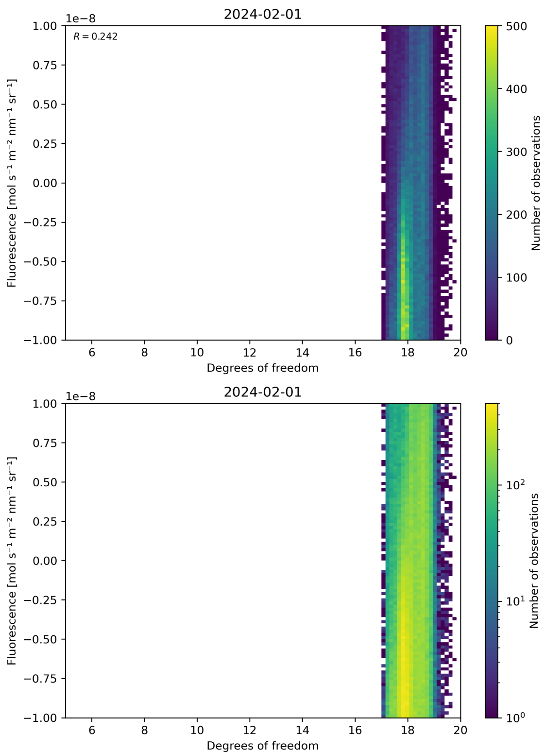
Figure 51: Scatter density plot of “Degrees of freedom” against “Fluorescence” for 2024-01-31 to 2024-02-02.
