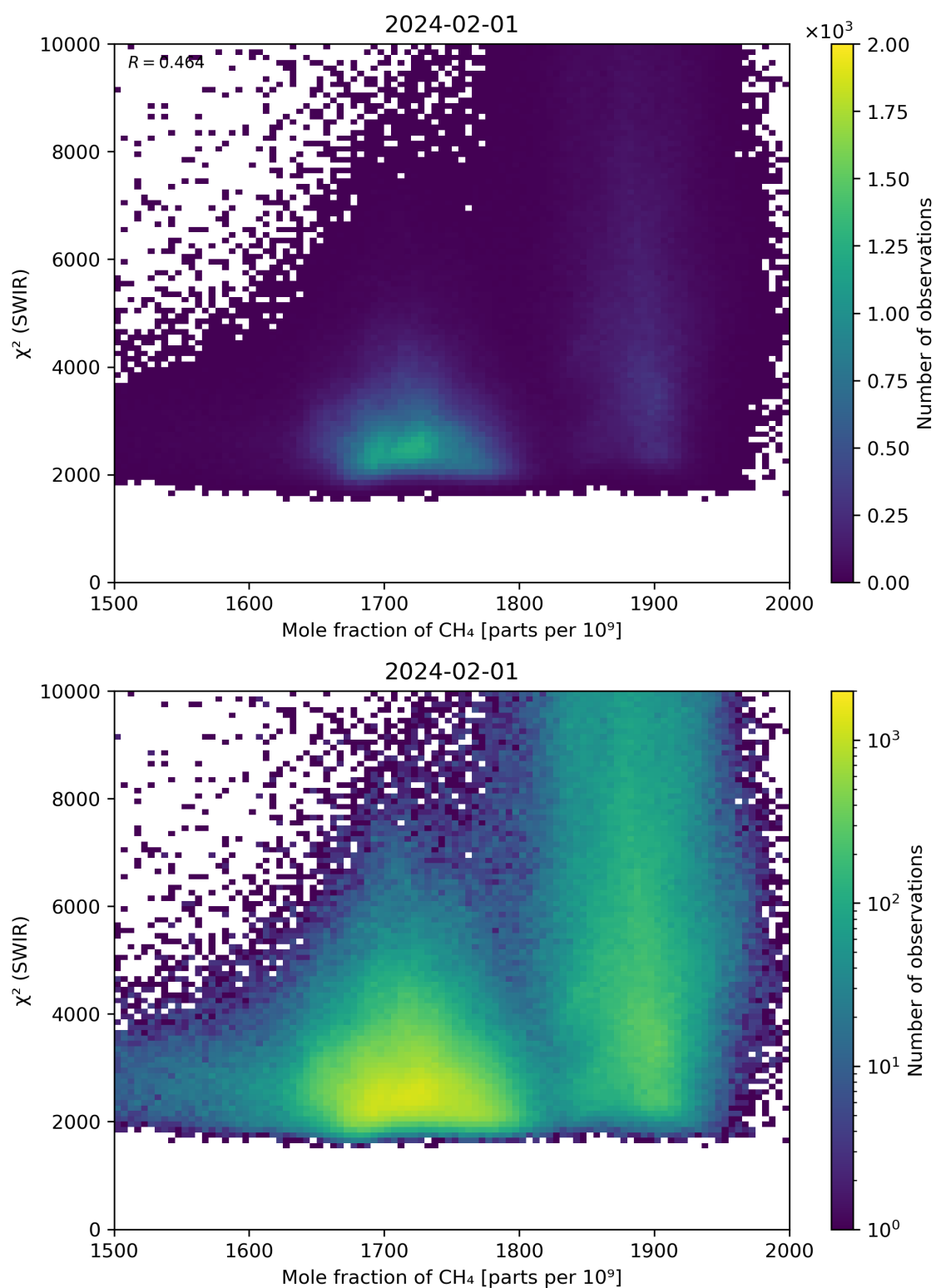
Figure 71: Scatter density plot of “Mole fraction of \text{CH}_4 ” against “ \chi^2 (SWIR)” for 2024-01-31 to 2024-02-02.
