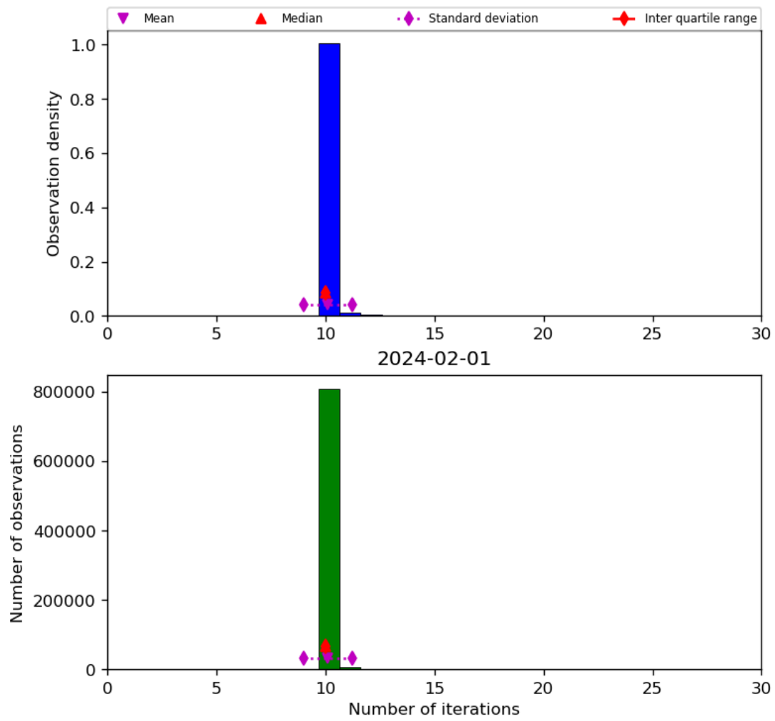
Figure 31: Histogram of “Number of iterations” for 2024-01-31 to 2024-02-02
