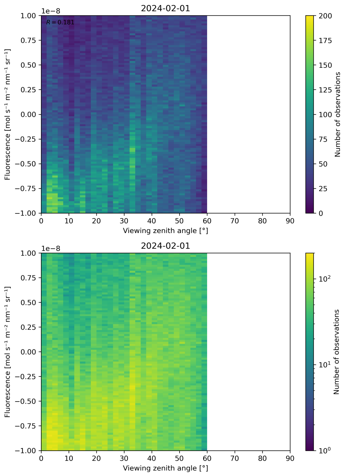
Figure 108: Scatter density plot of “Viewing zenith angle” against “Fluorescence” for 2024-01-31 to 2024-02-02.
