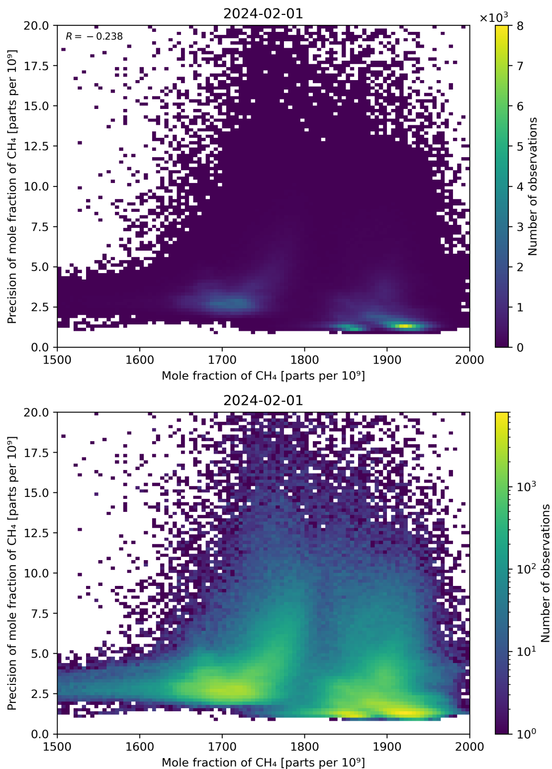
Figure 75: Scatter density plot of “Mole fraction of CH 4 ” against “Precision of mole fraction of CH 4 ” for 2024-01-31 to 2024-02-02.
