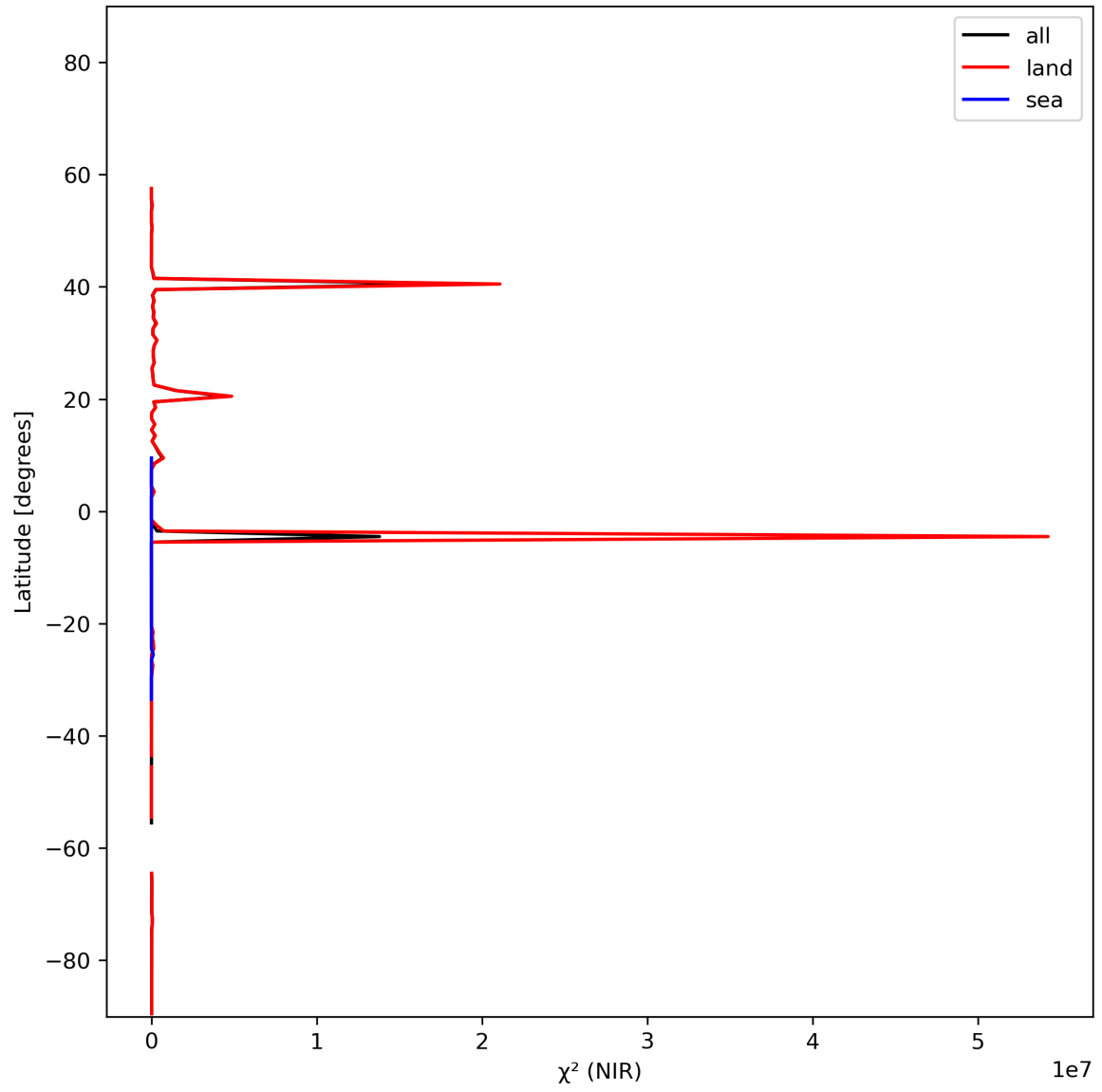
Figure 18: Zonal average of “ \chi^2 (NIR)” for 2024-01-31 to 2024-02-02.
