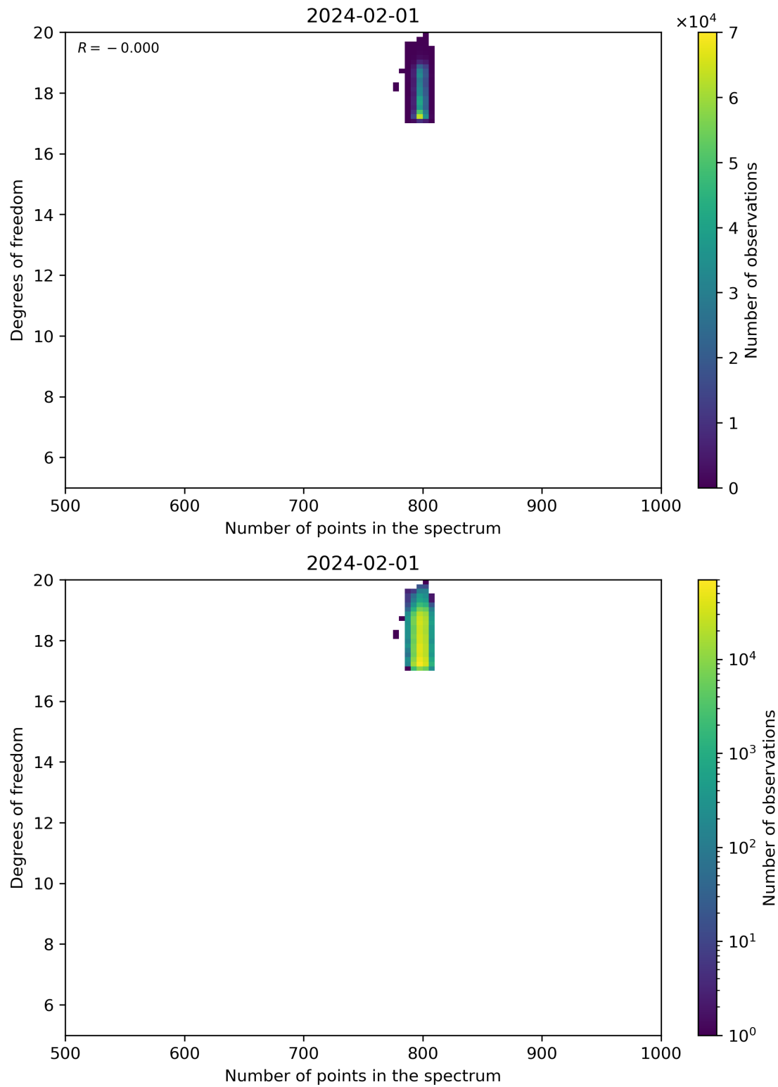
Figure 90: Scatter density plot of “Number of points in the spectrum” against “Degrees of freedom” for 2024-01-31 to 2024-02-02.
