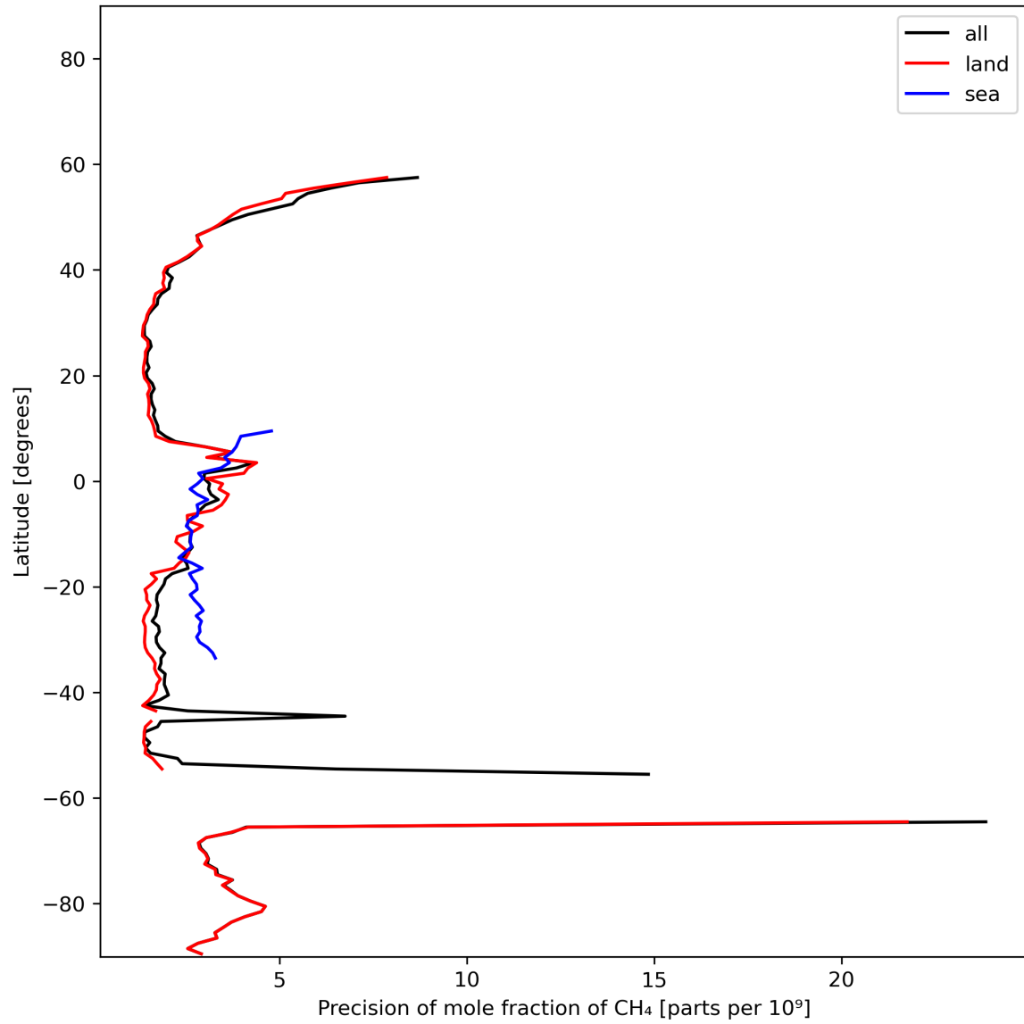
Figure 13: Zonal average of “Precision of mole fraction of CH 4 ” for 2024-01-31 to 2024-02-02.
