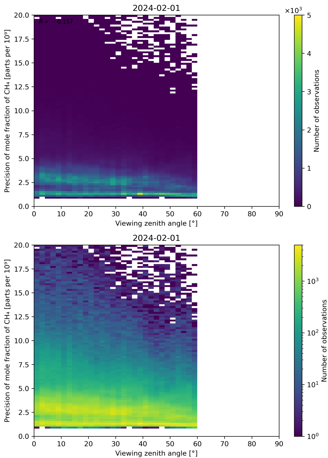
Figure 112: Scatter density plot of “Viewing zenith angle” against “Precision of mole fraction of CH 4 ” for 2024-01-31 to 2024-02-02.
