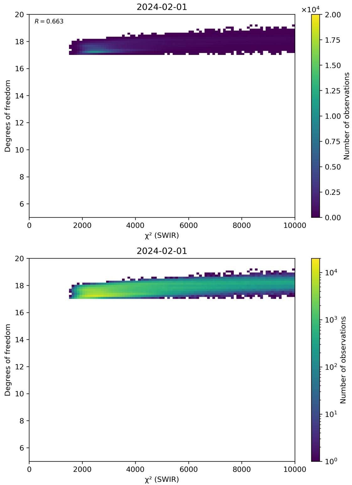
Figure 48: Scatter density plot of “ \chi^2 (SWIR)” against “Degrees of freedom” for 2024-01-31 to 2024-02-02.
