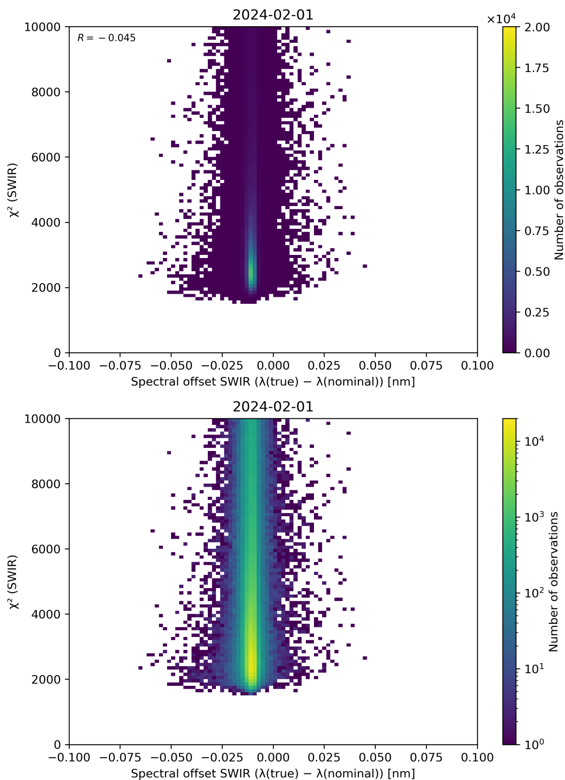
Figure 118: Scatter density plot of “Spectral offset SWIR ( \lambda(\text{true}) - \lambda(\text{nominal}) )” against “ \chi^2 (SWIR)” for 2024-01-31 to 2024-02-02.
