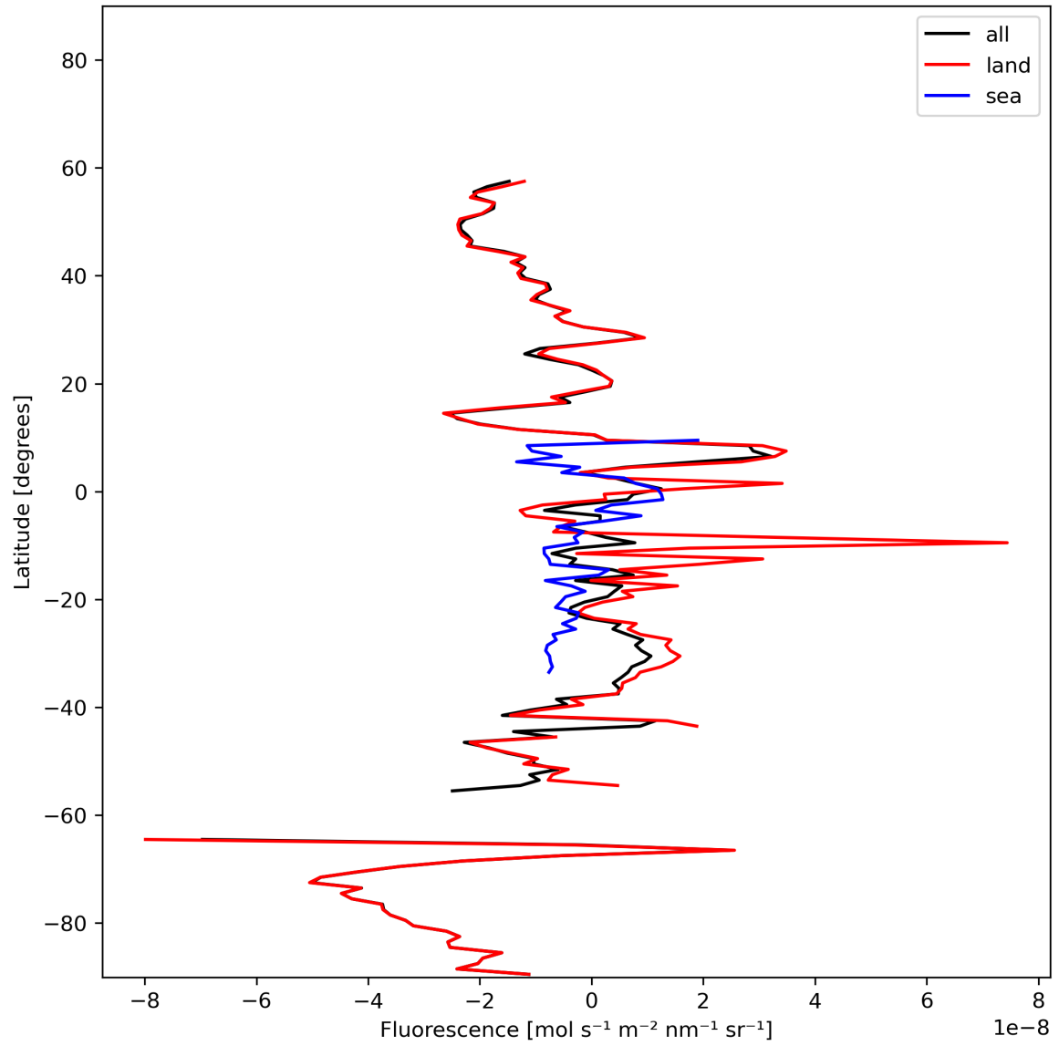
Figure 21: Zonal average of “Fluorescence” for 2024-01-31 to 2024-02-02.
