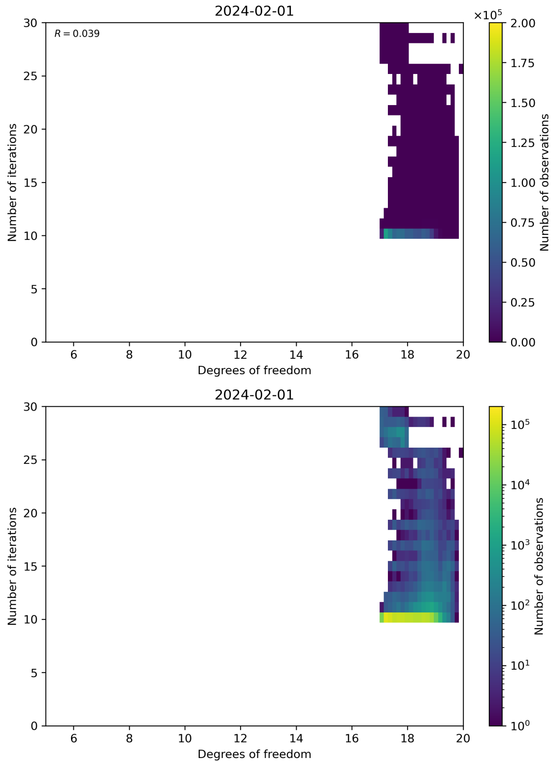
Figure 52: Scatter density plot of “Degrees of freedom” against “Number of iterations” for 2024-01-31 to 2024-02-02.
