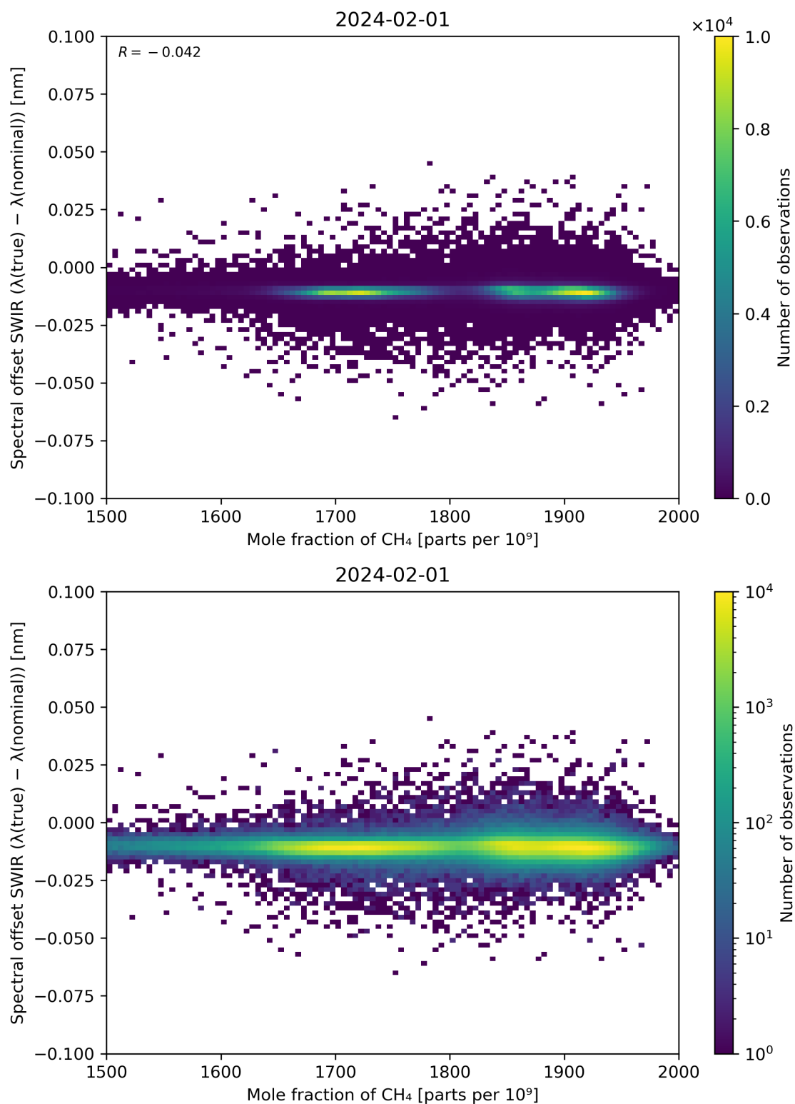
Figure 86: Scatter density plot of “Mole fraction of CH 4 ” against “Spectral offset SWIR ( \lambda(\text{true}) - \lambda(\text{nominal}) )” for 2024-01-31 to 2024-02-02.
