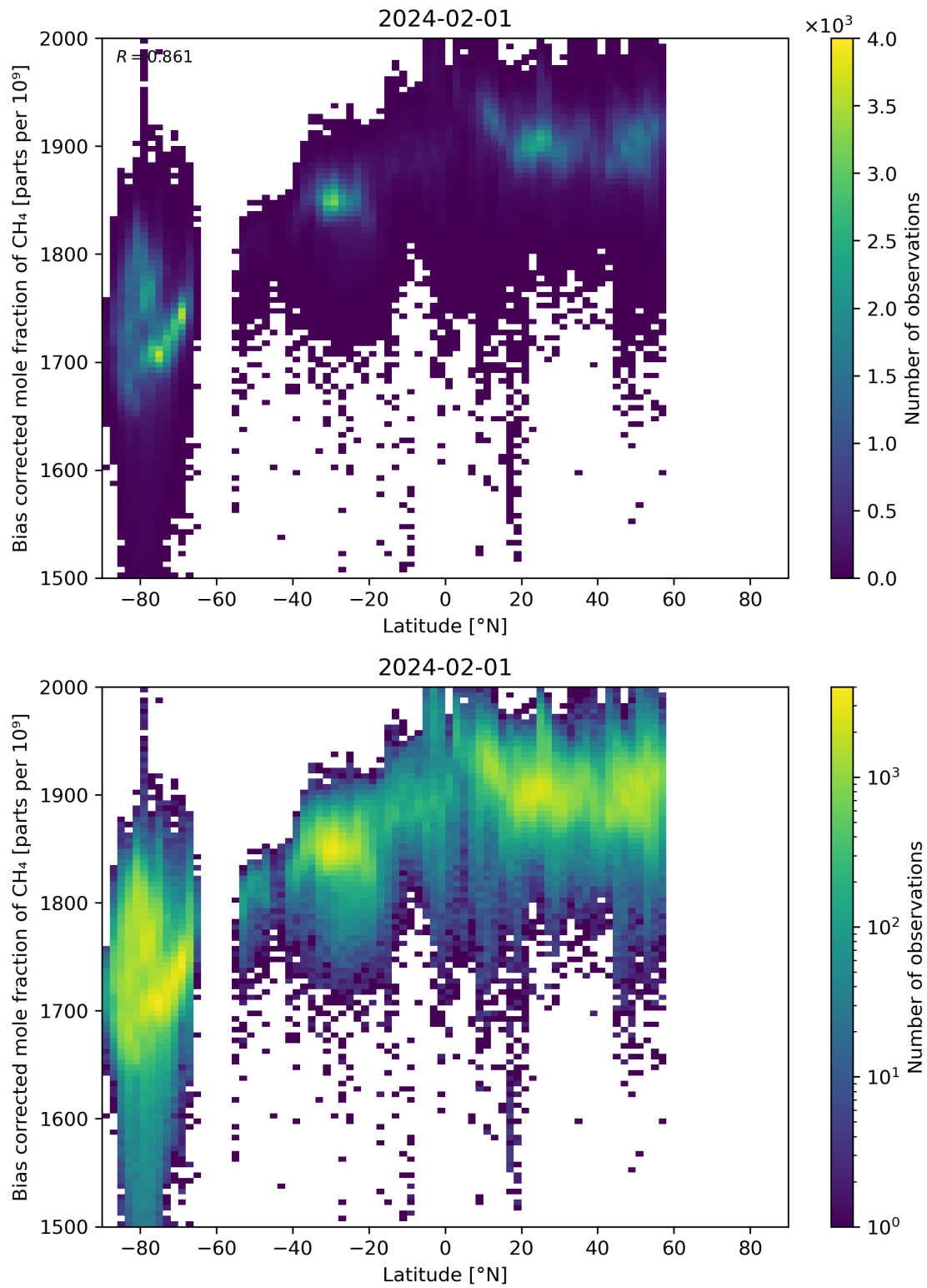
Figure 58: Scatter density plot of “Latitude” against “Bias corrected mole fraction of CH 4 ” for 2024-01-31 to 2024-02-02.
