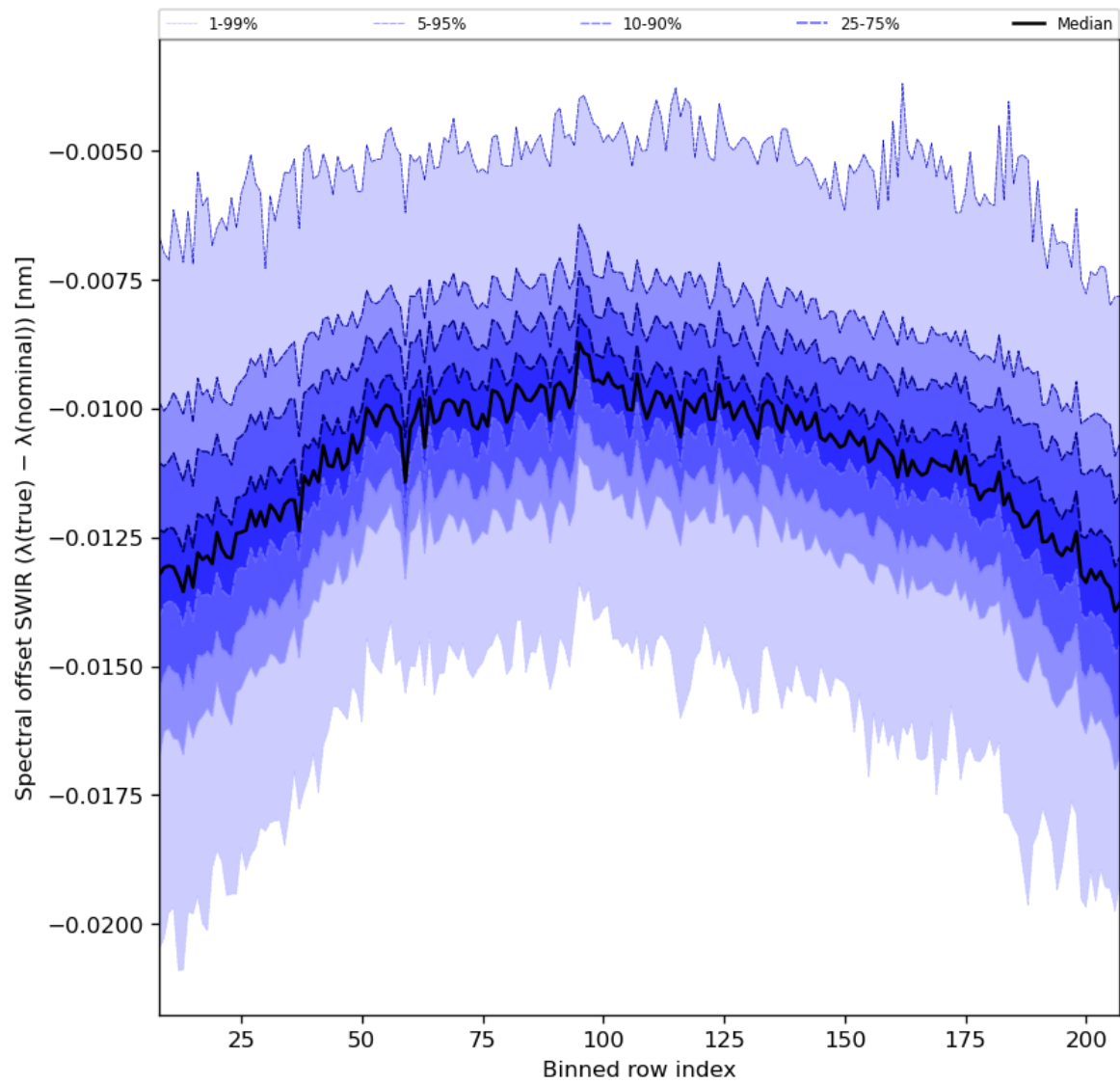
Figure 38: Along track statistics of “Spectral offset SWIR ( \lambda(\text{true}) - \lambda(\text{nominal}) )” for 2024-01-31 to 2024-02-02
