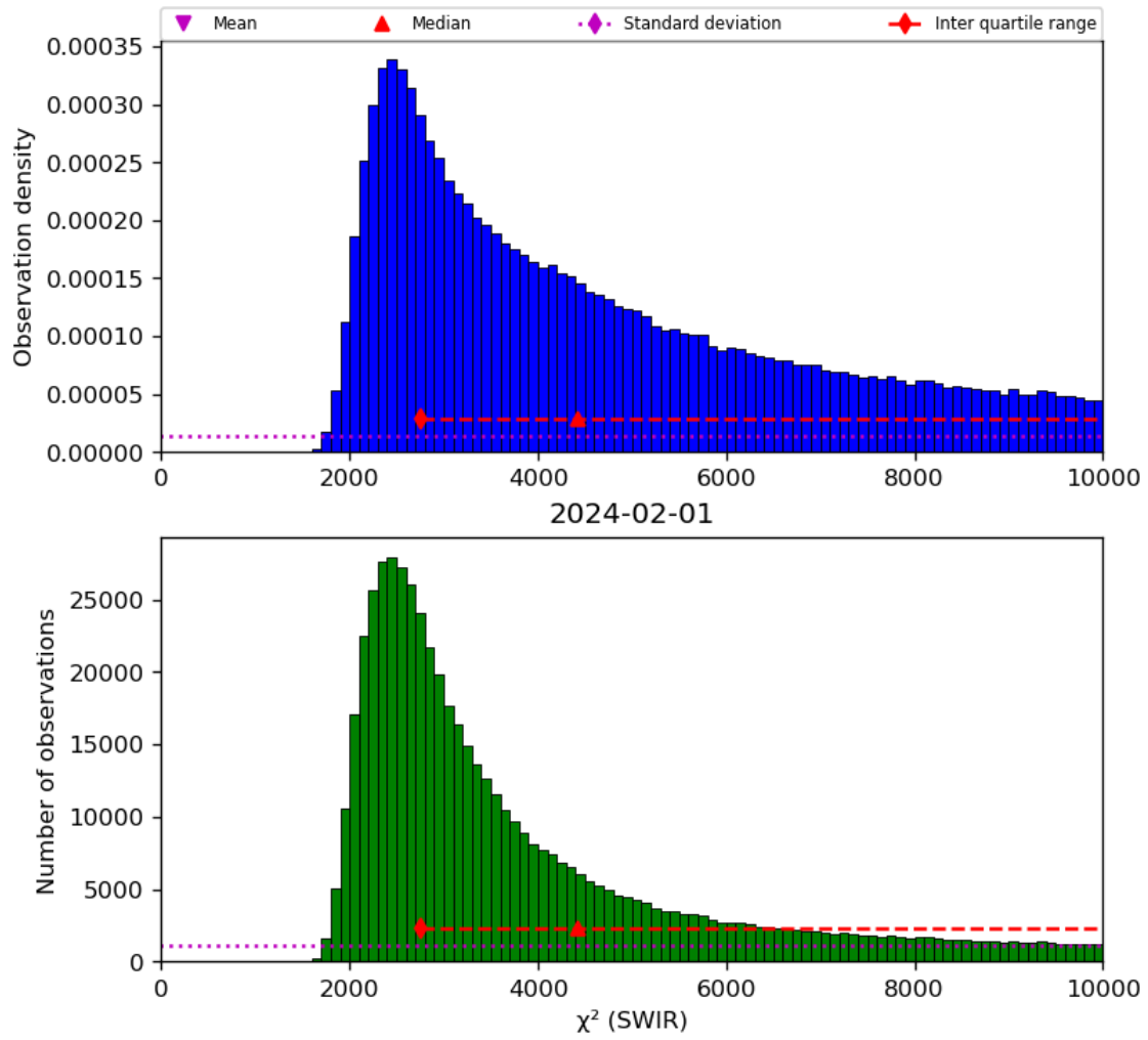
Figure 28: Histogram of “ \chi^2 (SWIR)” for 2024-01-31 to 2024-02-02
