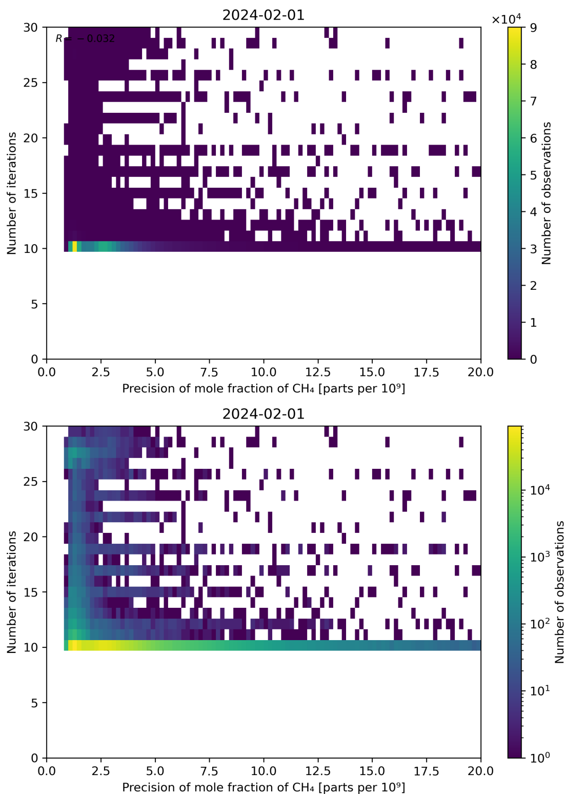
Figure 83: Scatter density plot of “Precision of mole fraction of CH 4 ” against “Number of iterations” for 2024-01-31 to 2024-02-02.
