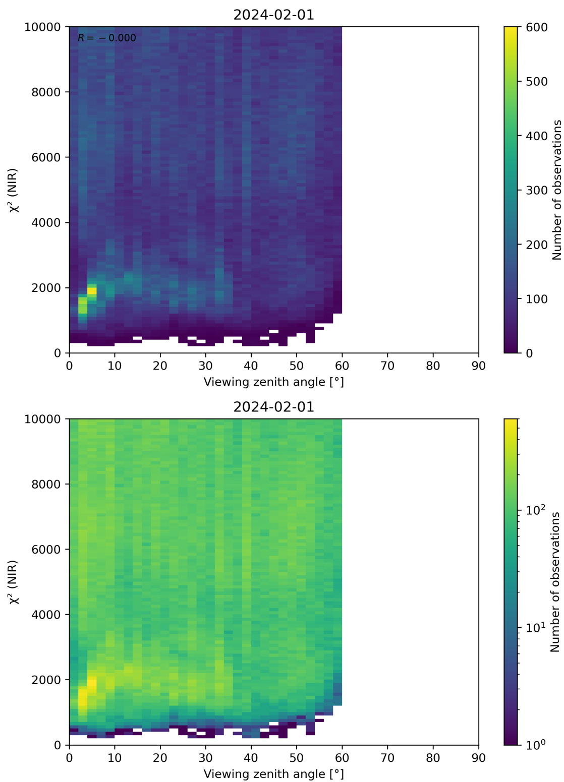
Figure 105: Scatter density plot of “Viewing zenith angle” against “ \chi^2 (NIR)” for 2024-01-31 to 2024-02-02.
