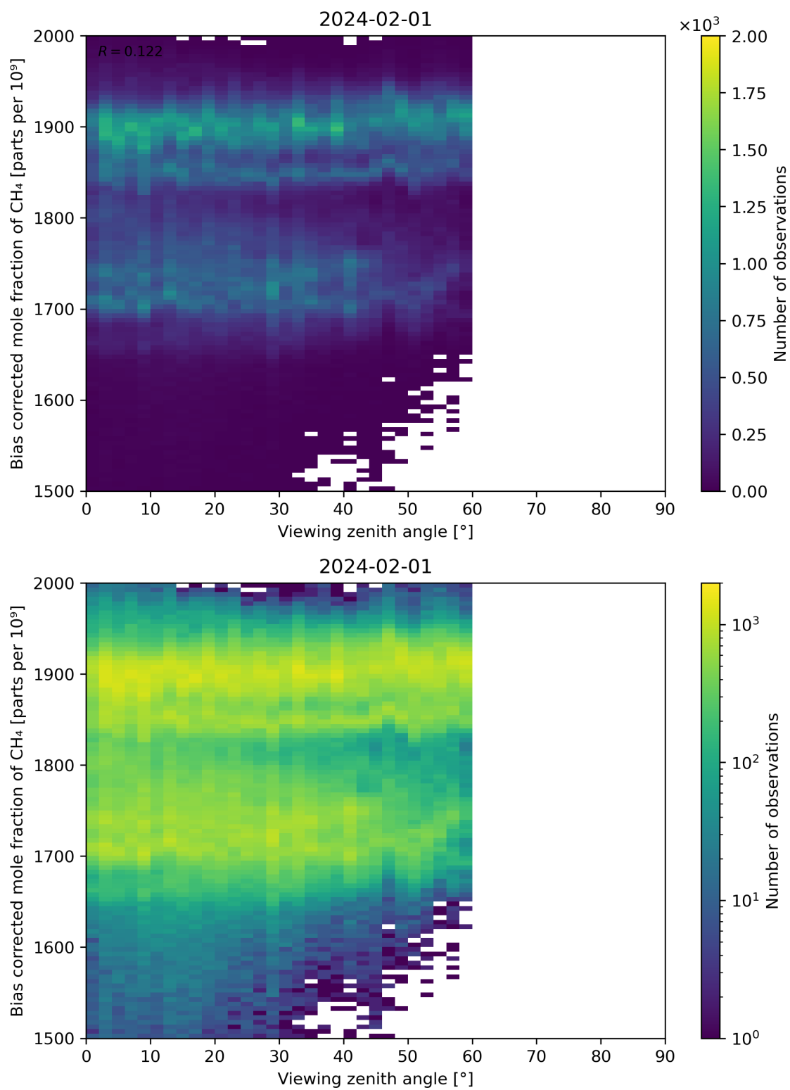
Figure 111: Scatter density plot of “Viewing zenith angle” against “Bias corrected mole fraction of CH 4 ” for 2024-01-31 to 2024-02-02.
