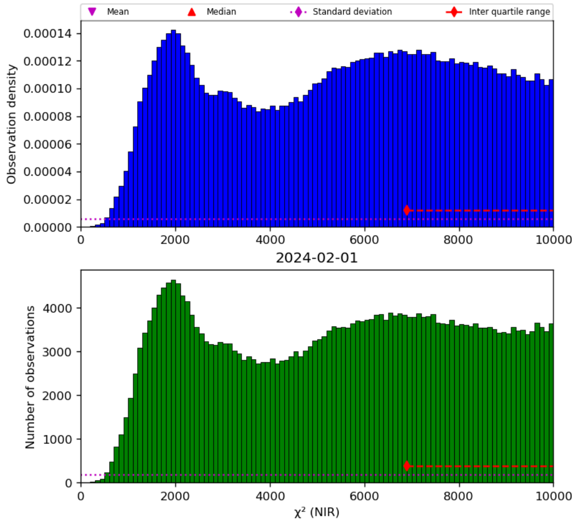
Figure 29: Histogram of " \chi^2 (NIR)" for 2024-01-31 to 2024-02-02
