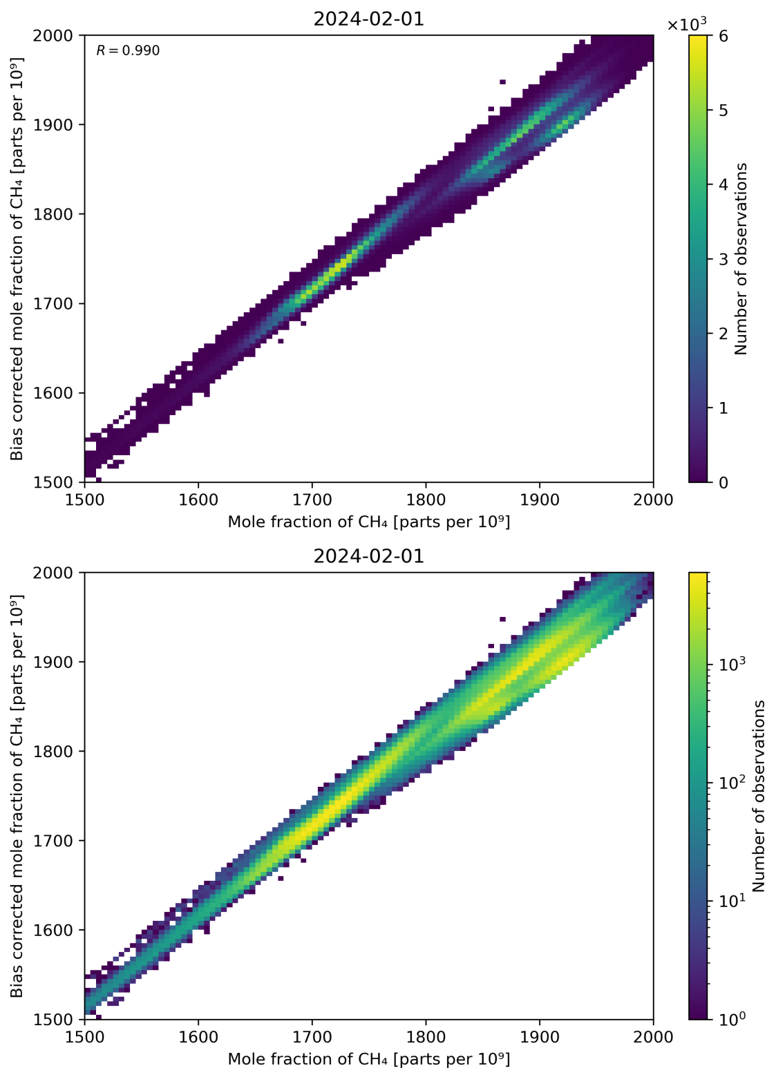
Figure 74: Scatter density plot of “Mole fraction of CH 4 ” against “Bias corrected mole fraction of CH 4 ” for 2024-01-31 to 2024-02-02.
