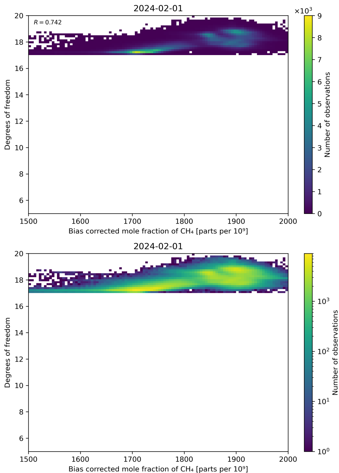
Figure 65: Scatter density plot of “Bias corrected mole fraction of CH 4 ” against “Degrees of freedom” for 2024-01-31 to 2024-02-02.
