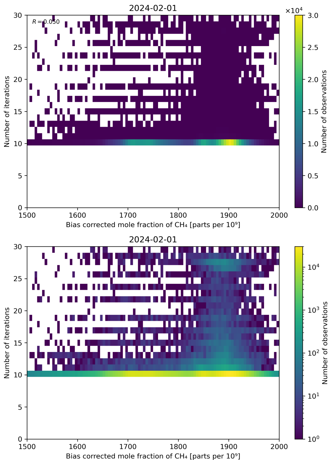
Figure 67: Scatter density plot of “Bias corrected mole fraction of CH 4 ” against “Number of iterations” for 2024-01-31 to 2024-02-02.
