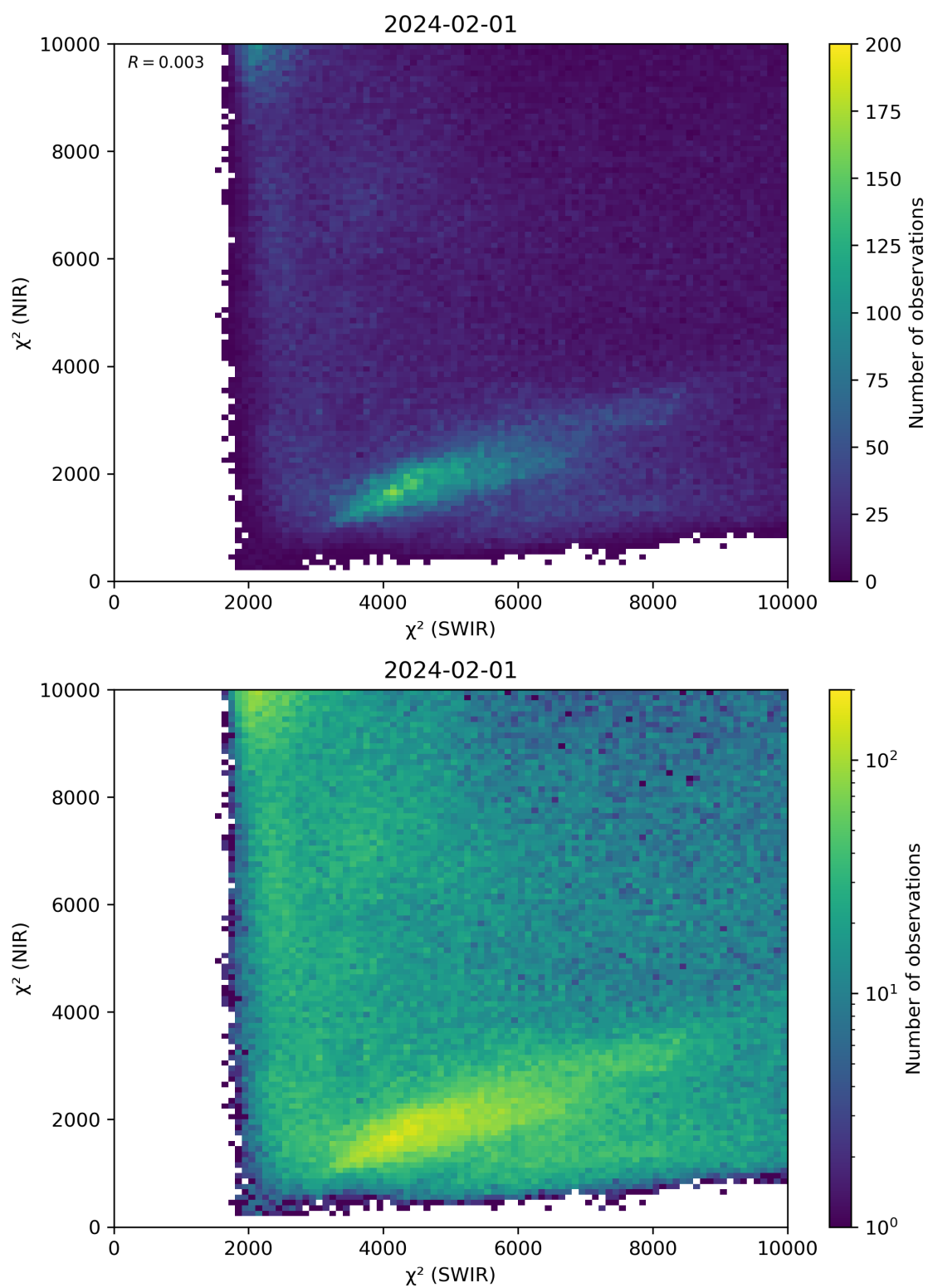
Figure 47: Scatter density plot of “ \chi^2 (SWIR)” against “ \chi^2 (NIR)” for 2024-01-31 to 2024-02-02.
