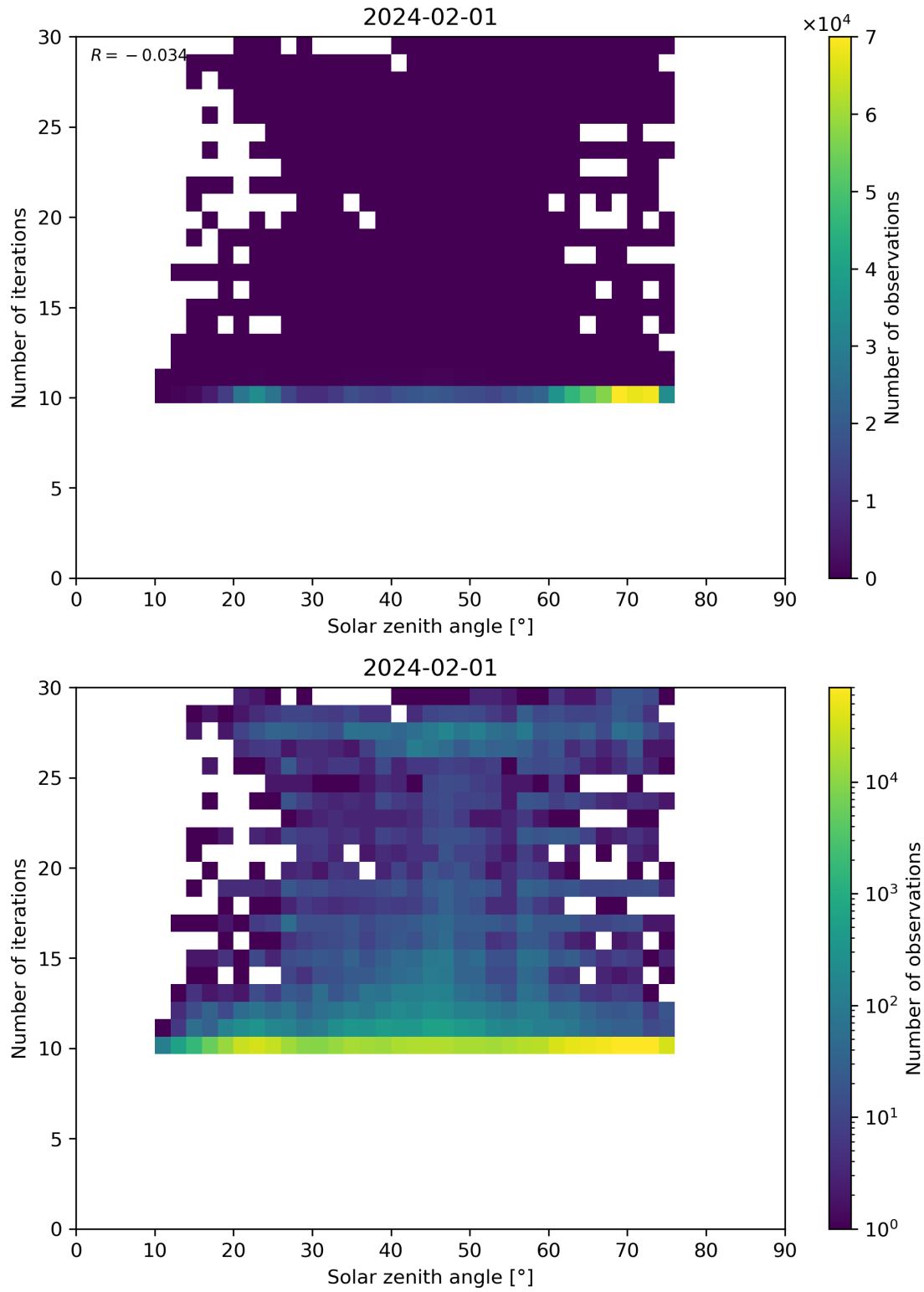
Figure 102: Scatter density plot of “Solar zenith angle” against “Number of iterations” for 2024-01-31 to 2024-02-02.
