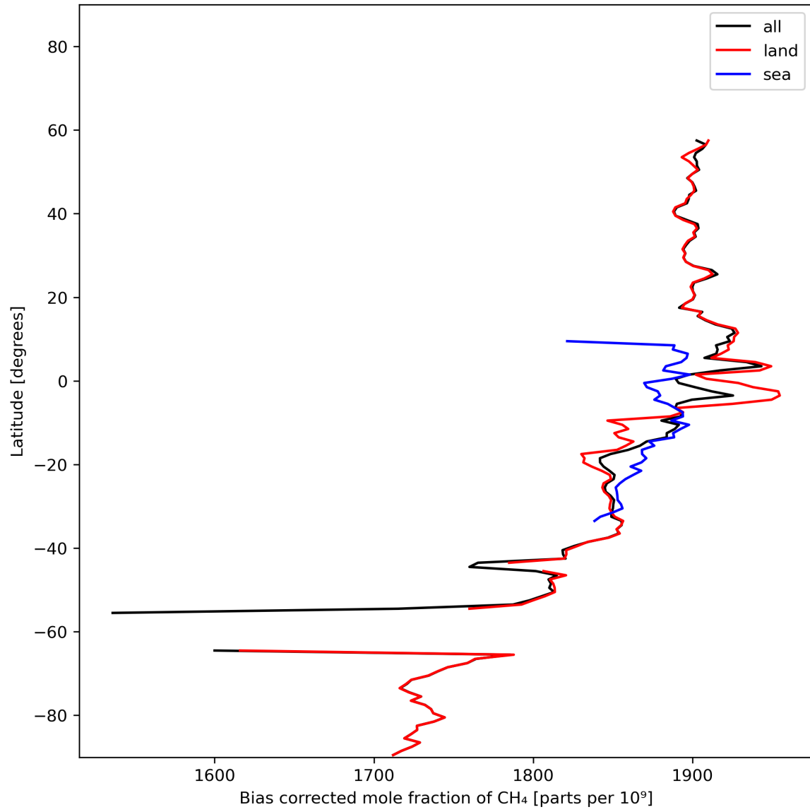
Figure 14: Zonal average of “Bias corrected mole fraction of CH 4 ” for 2024-01-31 to 2024-02-02.
