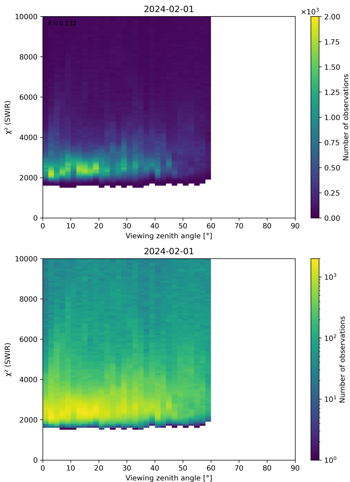
Figure 106: Scatter density plot of “Viewing zenith angle” against “ \chi^2 (SWIR)” for 2024-01-31 to 2024-02-02.
