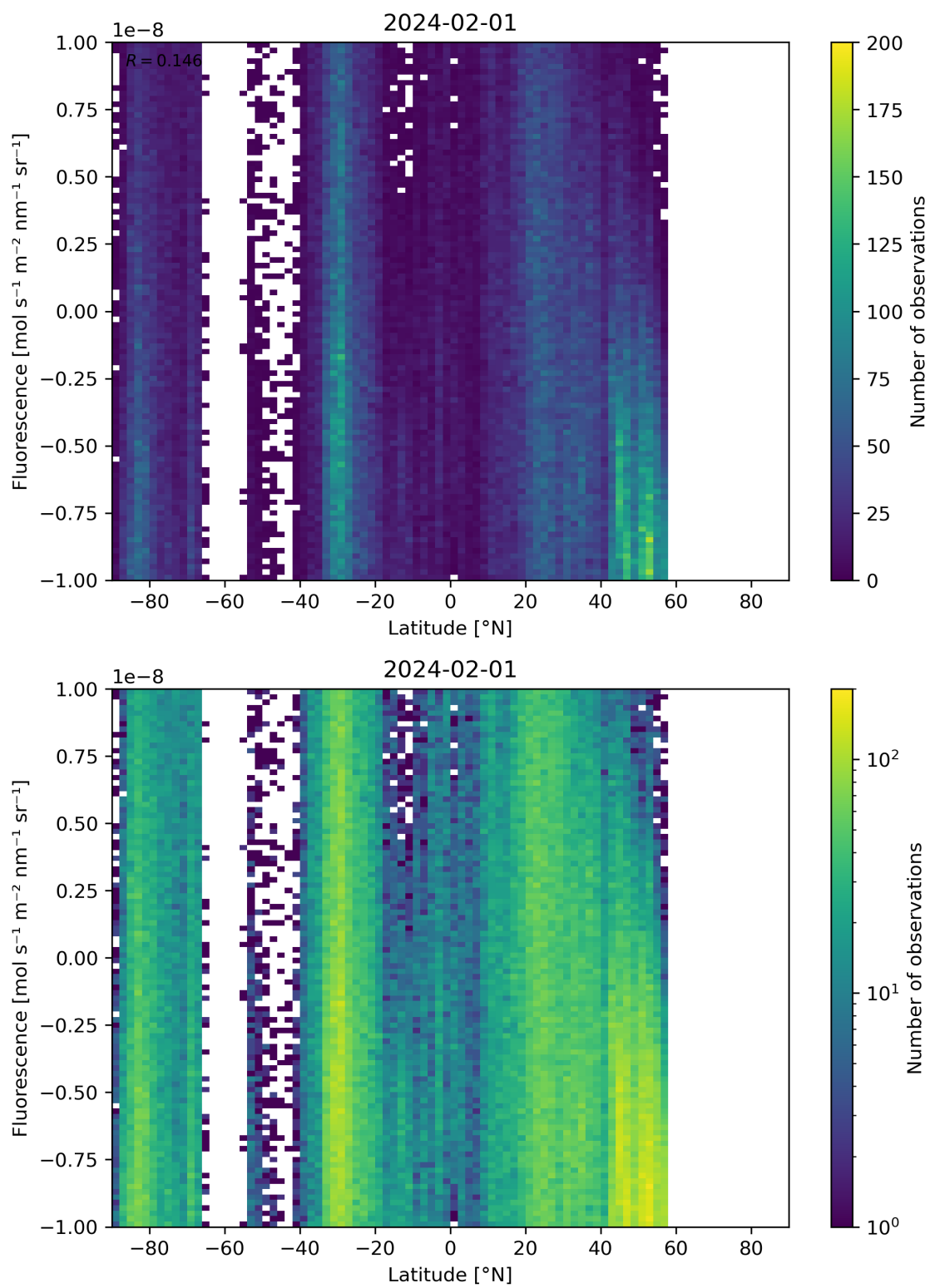
Figure 56: Scatter density plot of “Latitude” against “Fluorescence” for 2024-01-31 to 2024-02-02.
