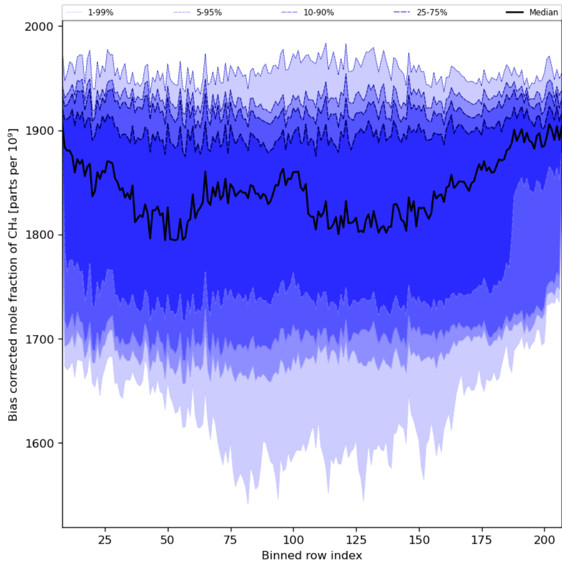
Figure 36: Along track statistics of “Bias corrected mole fraction of CH 4 ” for 2024-01-31 to 2024-02-02
