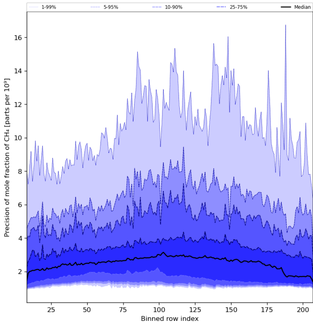
Figure 35: Along track statistics of “Precision of mole fraction of CH 4 ” for 2024-01-31 to 2024-02-02
