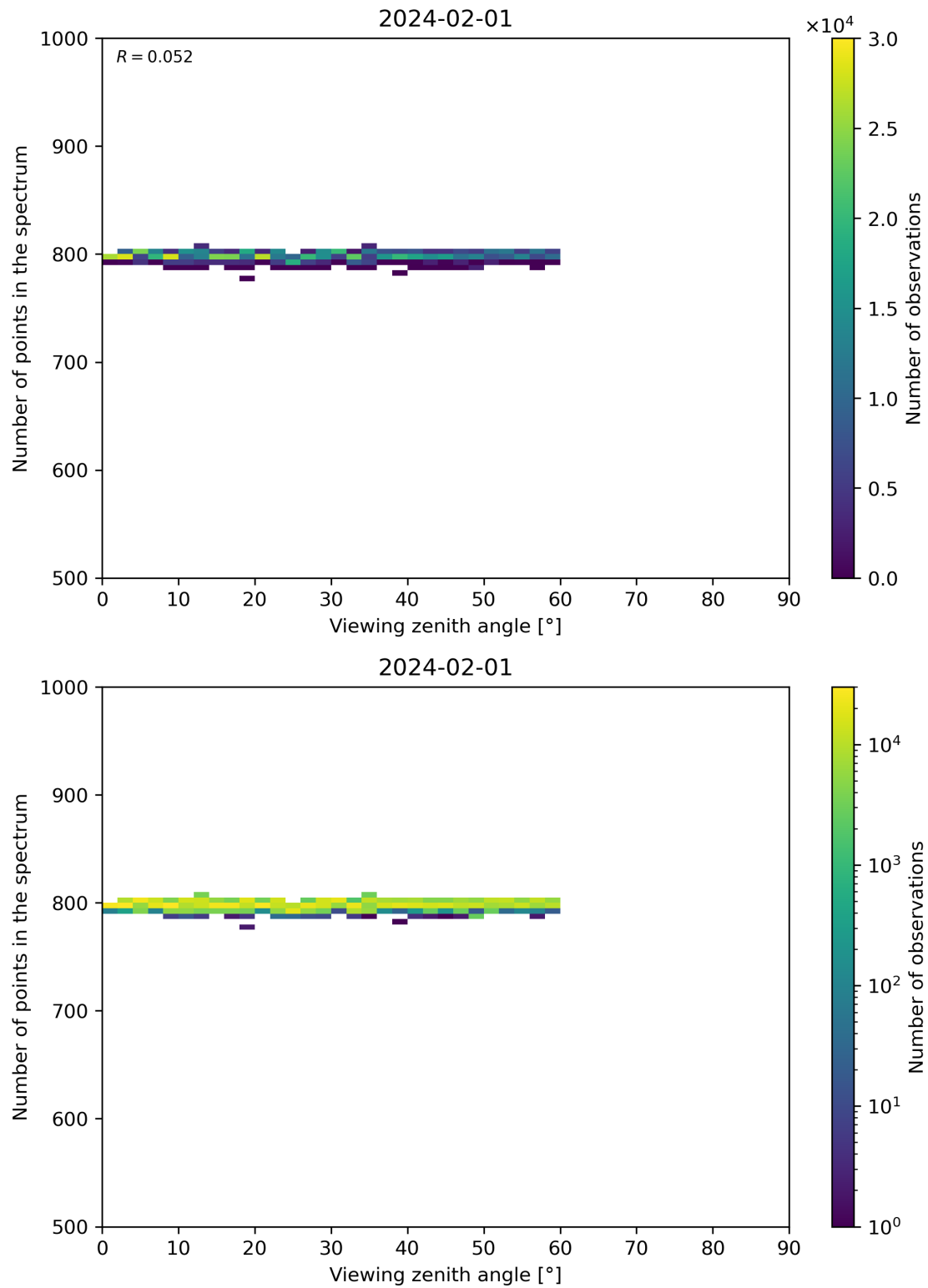
Figure 114: Scatter density plot of “Viewing zenith angle” against “Number of points in the spectrum” for 2024-01-31 to 2024-02-02.
