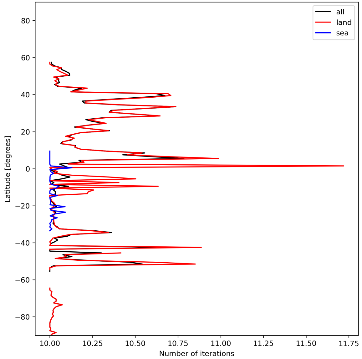
Figure 20: Zonal average of “Number of iterations” for 2024-01-31 to 2024-02-02.
