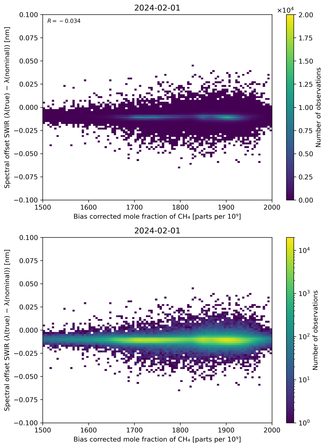
Figure 69: Scatter density plot of “Bias corrected mole fraction of \text{CH}_4 ” against “Spectral offset SWIR ( \lambda(\text{true}) - \lambda(\text{nominal}) )” for 2024-01-31 to 2024-02-02.
