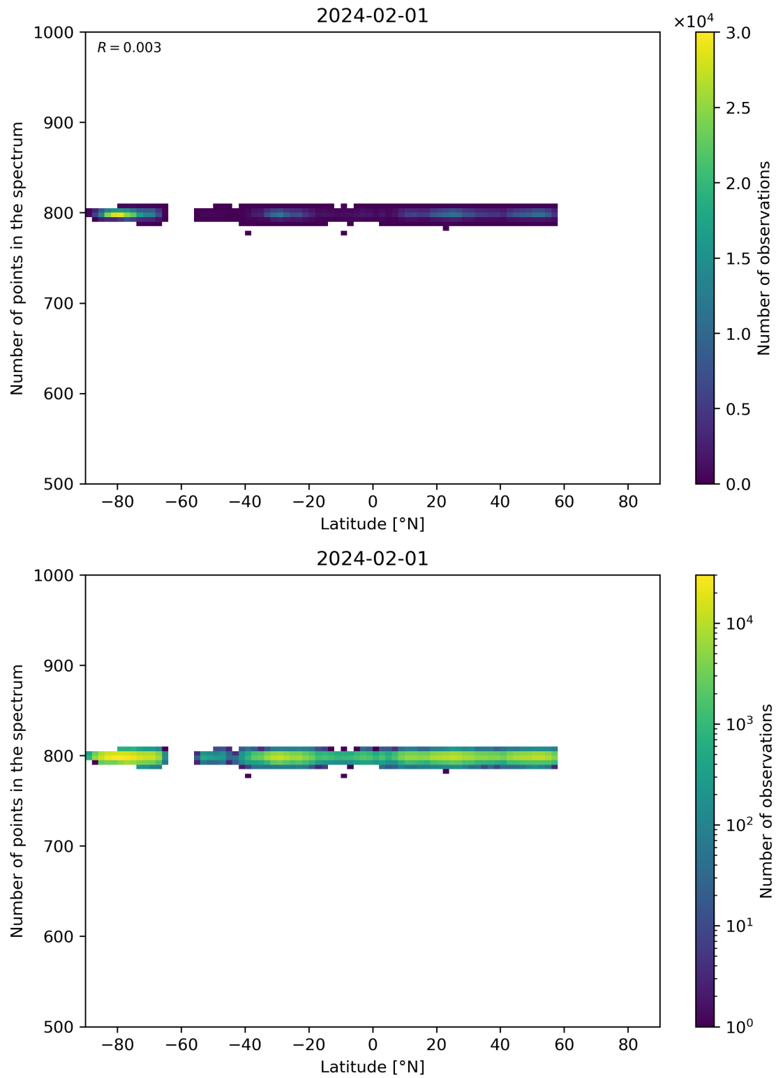
Figure 61: Scatter density plot of “Latitude” against “Number of points in the spectrum” for 2024-01-31 to 2024-02-02.
