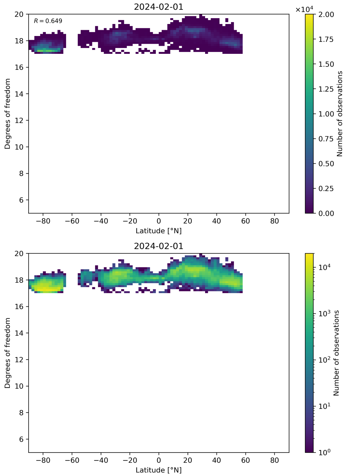
Figure 55: Scatter density plot of “Latitude” against “Degrees of freedom” for 2024-01-31 to 2024-02-02.
