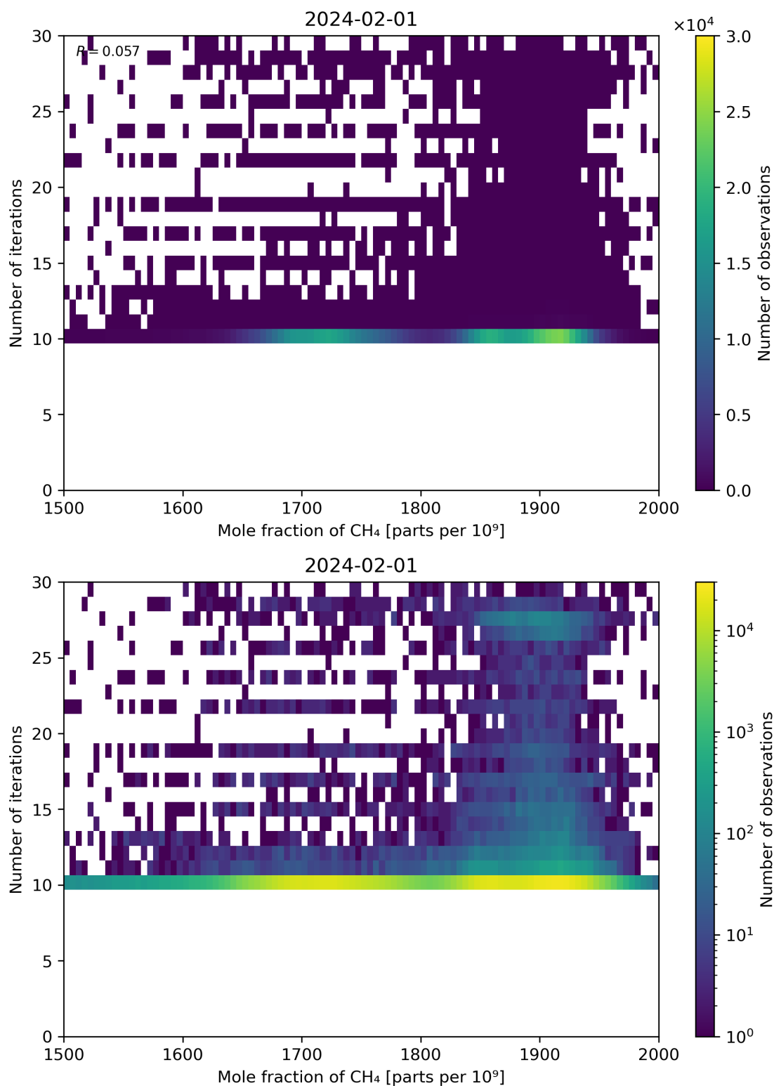
Figure 76: Scatter density plot of “Mole fraction of CH 4 ” against “Number of iterations” for 2024-01-31 to 2024-02-02.
