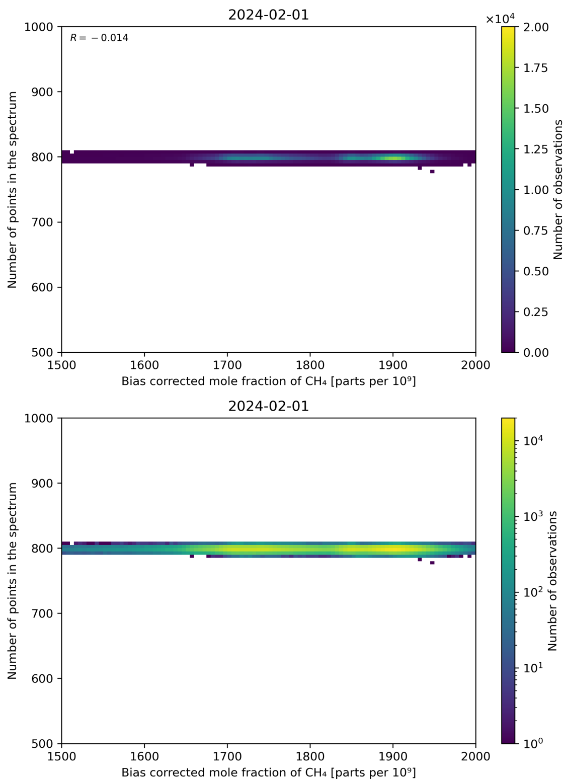
Figure 68: Scatter density plot of “Bias corrected mole fraction of CH 4 ” against “Number of points in the spectrum” for 2024-01-31 to 2024-02-02.
