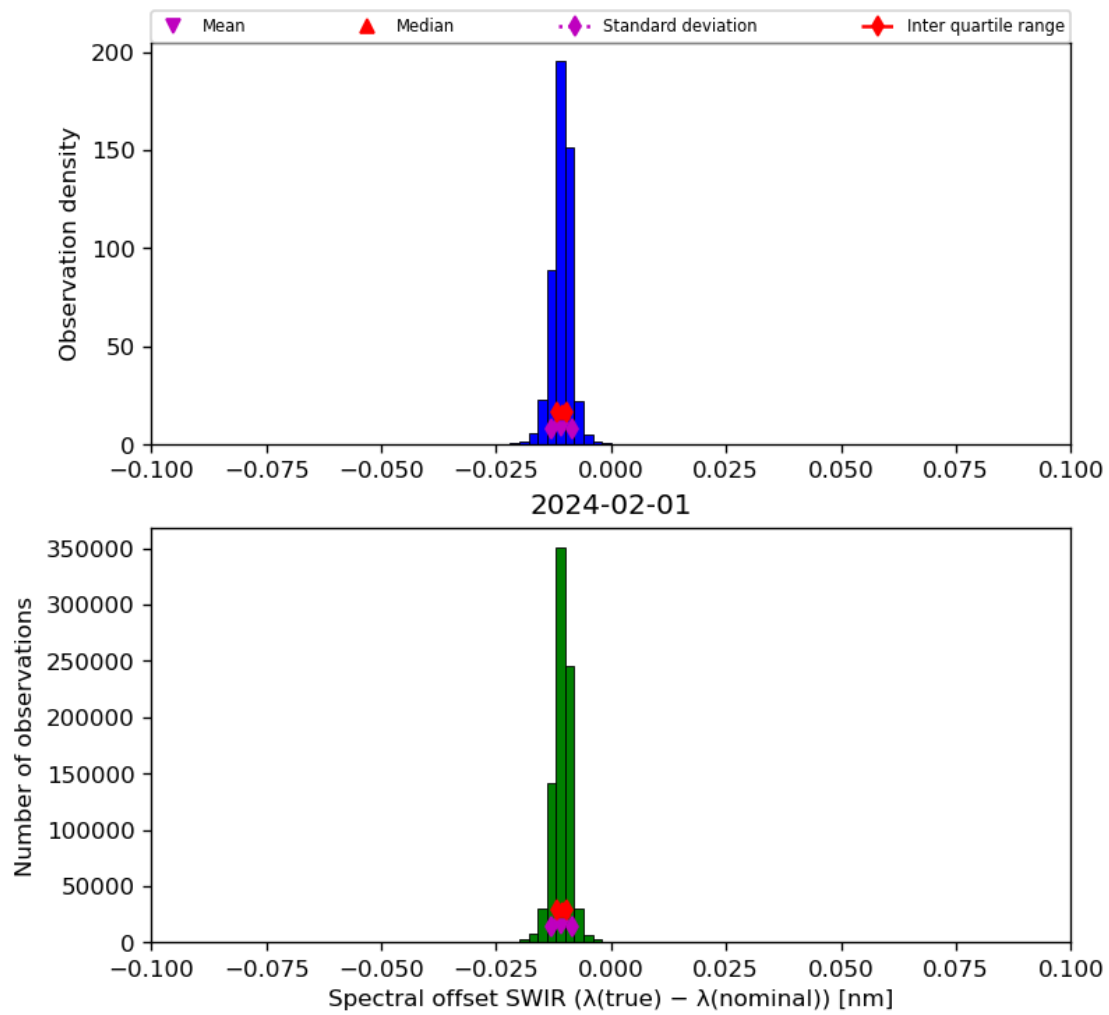
Figure 27: Histogram of “Spectral offset SWIR ( \lambda(\text{true}) - \lambda(\text{nominal}) )” for 2024-01-31 to 2024-02-02
