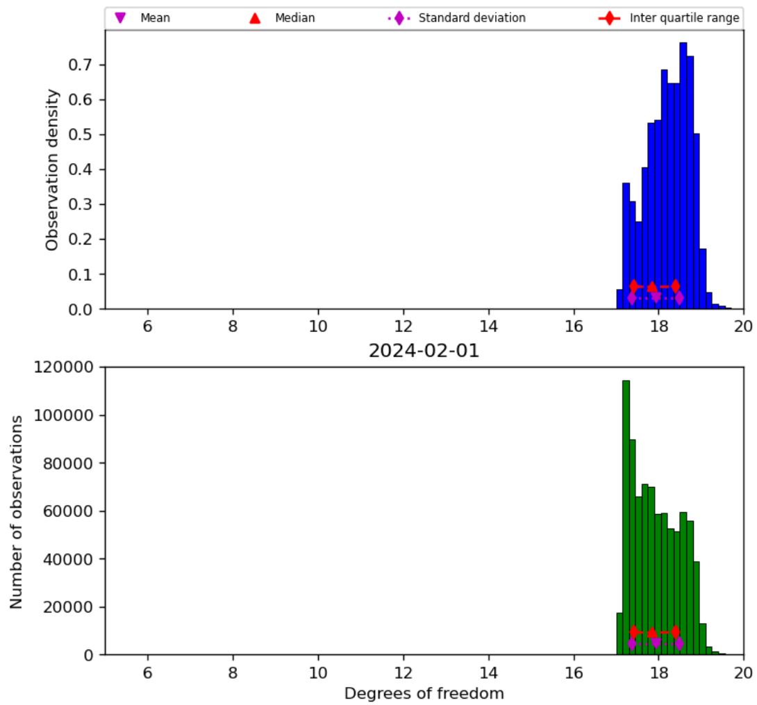
Figure 30: Histogram of “Degrees of freedom” for 2024-01-31 to 2024-02-02
