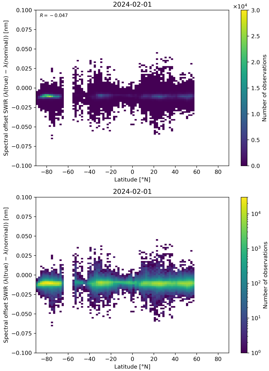
Figure 62: Scatter density plot of “Latitude” against “Spectral offset SWIR ( \lambda(\text{true}) - \lambda(\text{nominal}) )” for 2024-01-31 to 2024-02-02.
