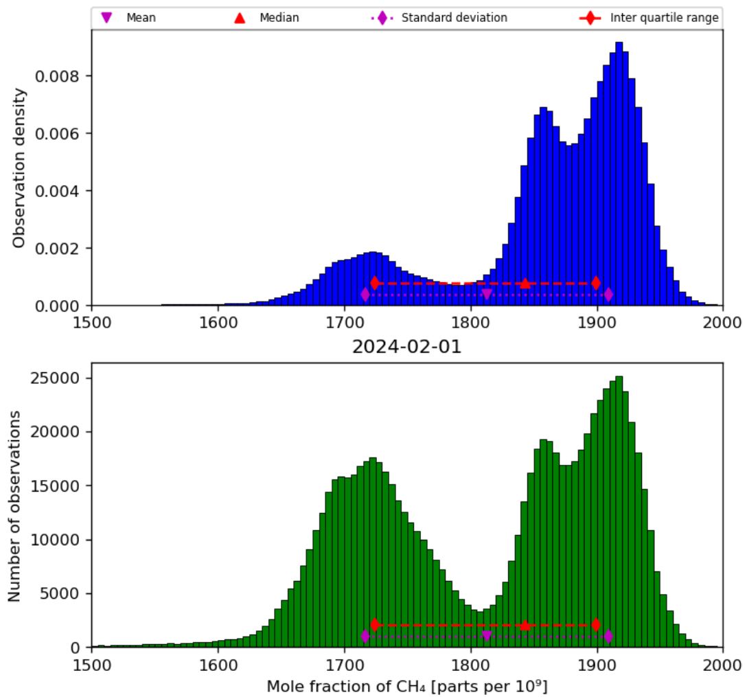
Figure 23: Histogram of “Mole fraction of CH 4 ” for 2024-01-31 to 2024-02-02
