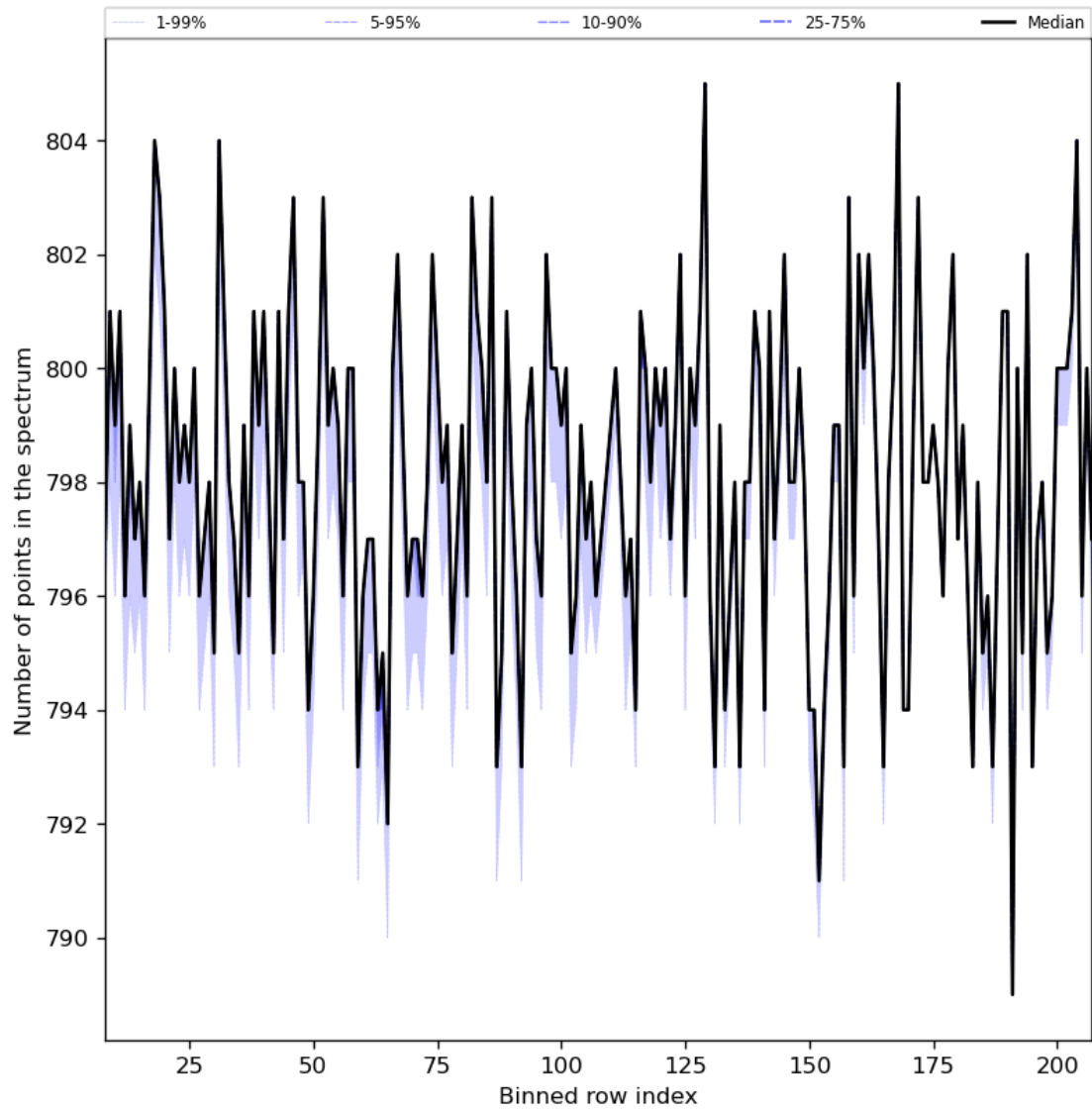
Figure 37: Along track statistics of “Number of points in the spectrum” for 2024-01-31 to 2024-02-02
