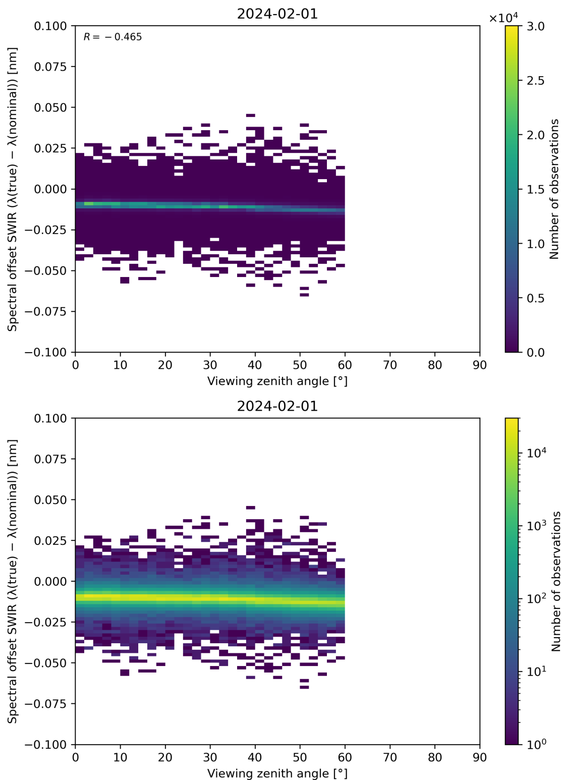
Figure 116: Scatter density plot of “Viewing zenith angle” against “Spectral offset SWIR ( \lambda(\text{true}) - \lambda(\text{nominal}) )” for 2024-01-31 to 2024-02-02.
