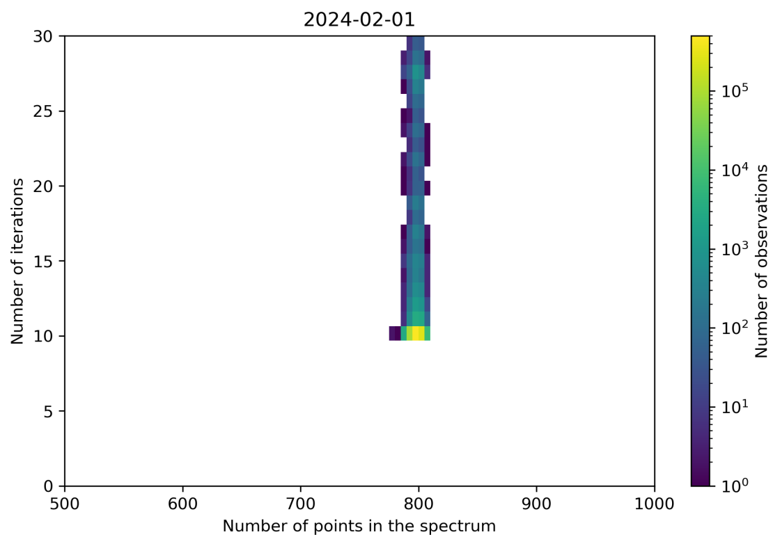
Figure 92: Scatter density plot of “Number of points in the spectrum” against “Number of iterations” for 2024-01-31 to 2024-02-02.
