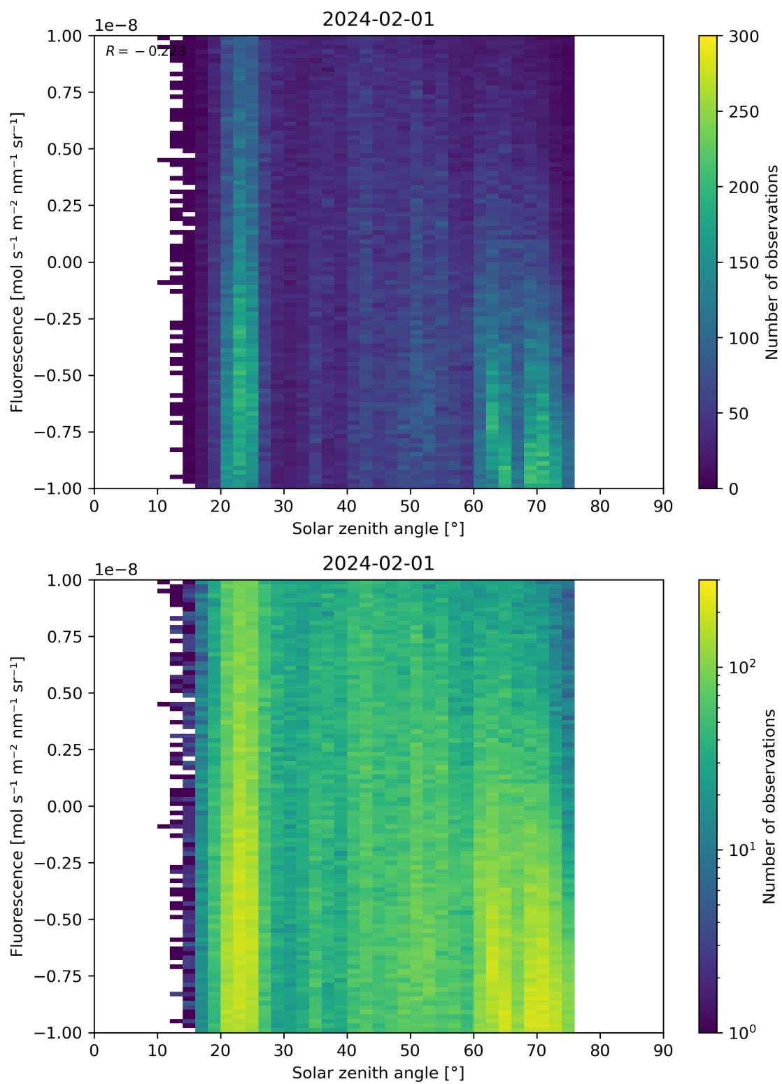
Figure 97: Scatter density plot of “Solar zenith angle” against “Fluorescence” for 2024-01-31 to 2024-02-02.
