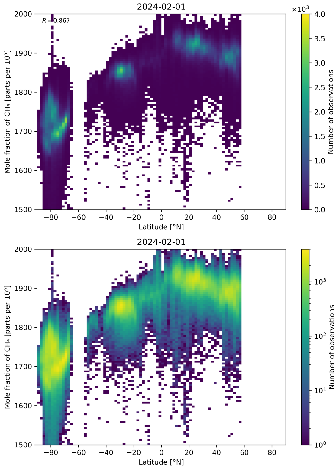
Figure 57: Scatter density plot of “Latitude” against “Mole fraction of CH 4 ” for 2024-01-31 to 2024-02-02.
