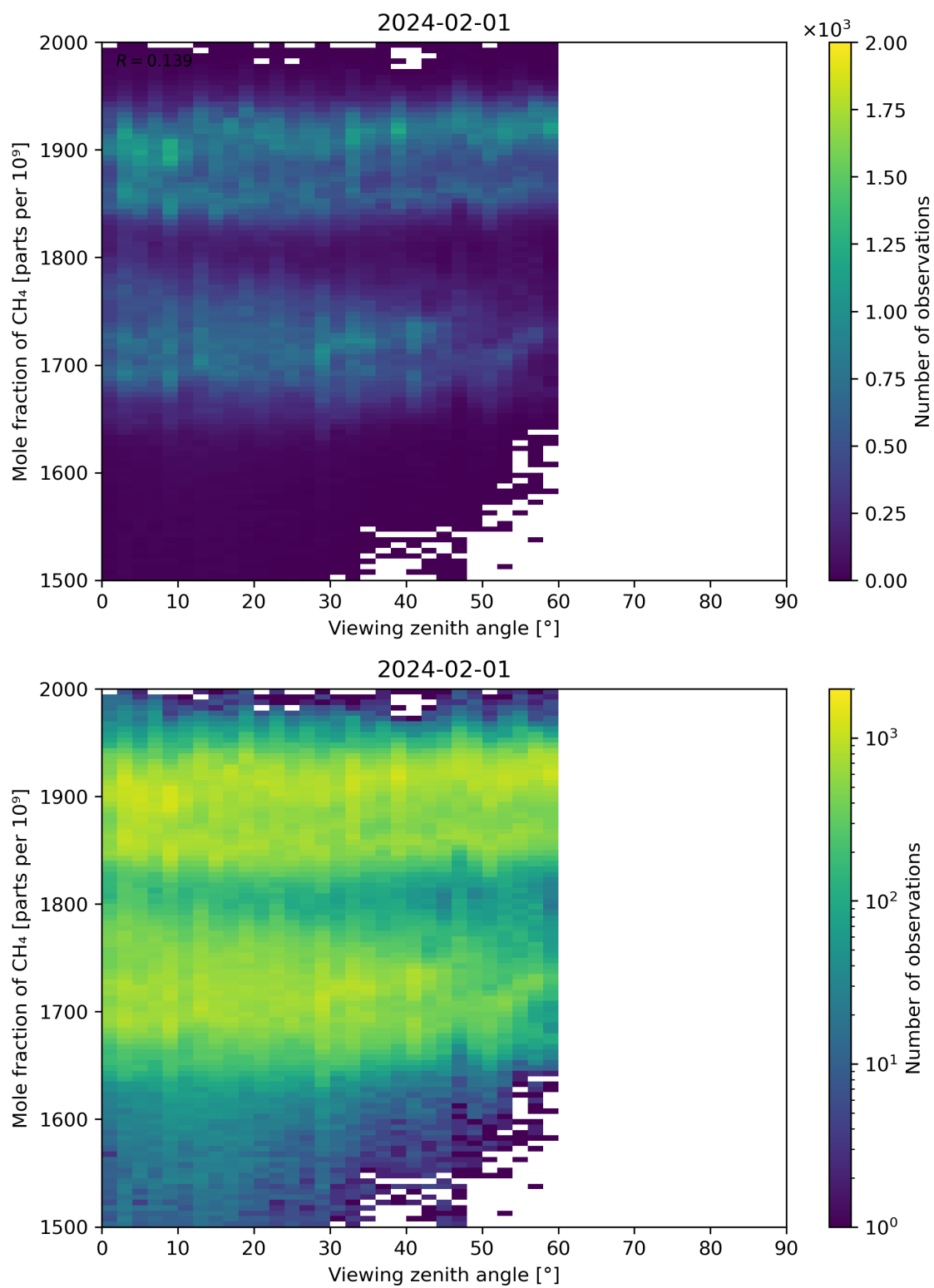
Figure 110: Scatter density plot of “Viewing zenith angle” against “Mole fraction of CH 4 ” for 2024-01-31 to 2024-02-02.
