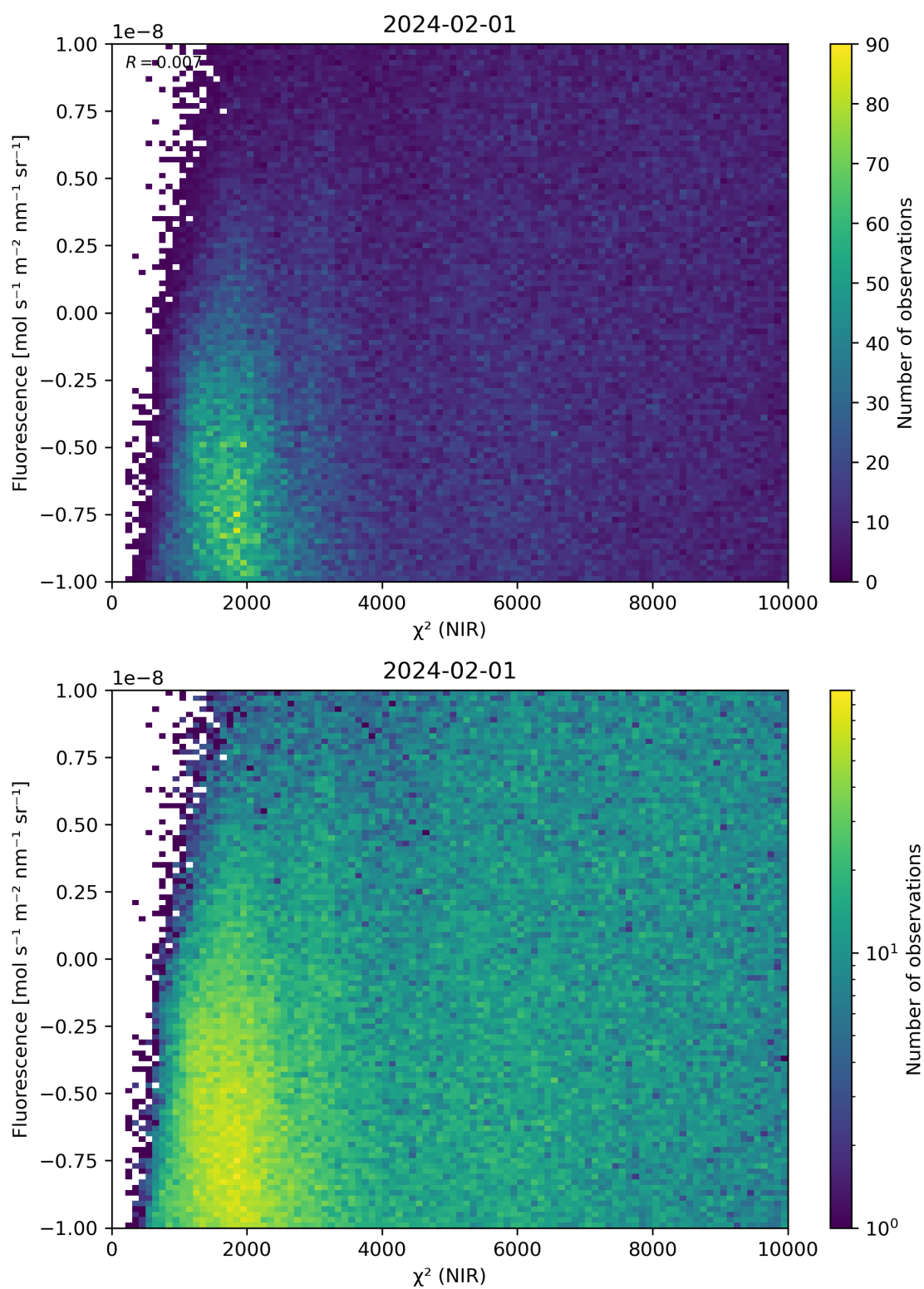
Figure 45: Scatter density plot of “ \chi^2 (NIR)” against “Fluorescence” for 2024-01-31 to 2024-02-02.
