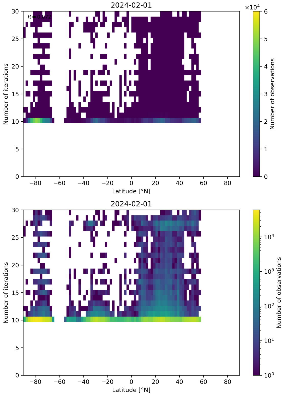
Figure 60: Scatter density plot of “Latitude” against “Number of iterations” for 2024-01-31 to 2024-02-02.
