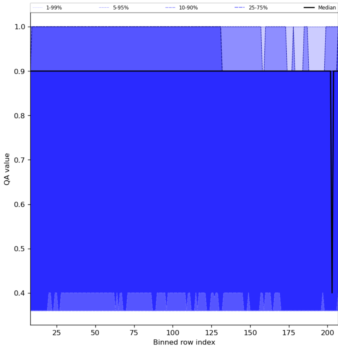
Figure 33: Along track statistics of “QA value” for 2024-01-31 to 2024-02-02
