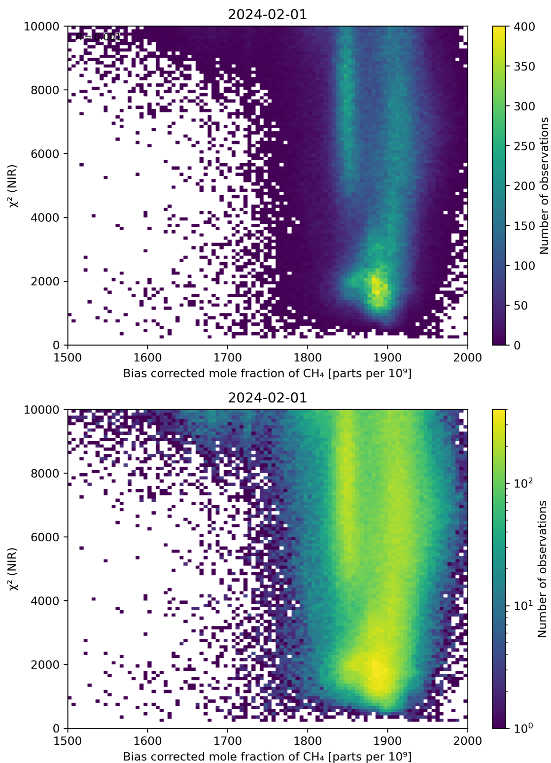
Figure 63: Scatter density plot of “Bias corrected mole fraction of CH 4 ” against “ \chi^2 (NIR)” for 2024-01-31 to 2024-02-02.
