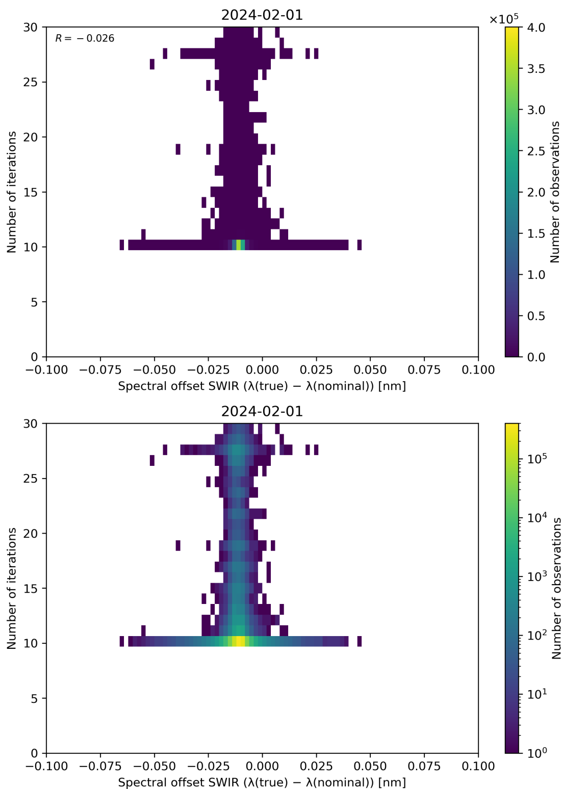
Figure 121: Scatter density plot of “Spectral offset SWIR ( \lambda(\text{true}) - \lambda(\text{nominal}) )” against “Number of iterations” for 2024-01-31 to 2024-02-02.
