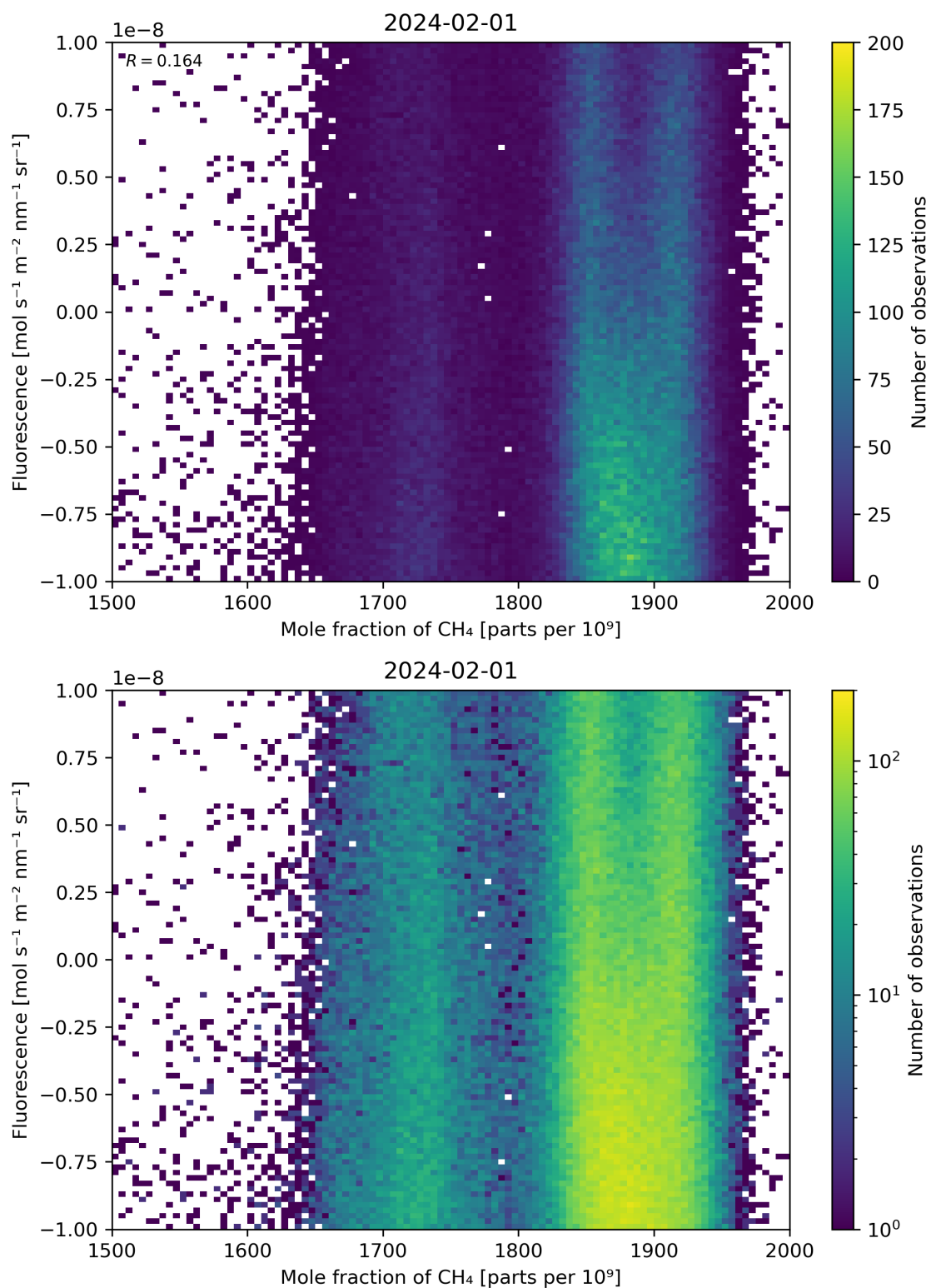
Figure 73: Scatter density plot of “Mole fraction of \text{CH}_4 ” against “Fluorescence” for 2024-01-31 to 2024-02-02.
