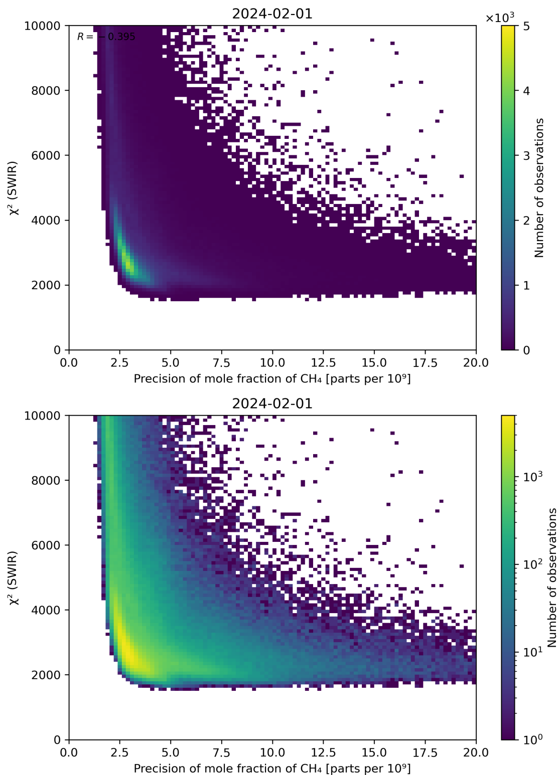
Figure 79: Scatter density plot of “Precision of mole fraction of \text{CH}_4 ” against “ \chi^2 (SWIR)” for 2024-01-31 to 2024-02-02.
