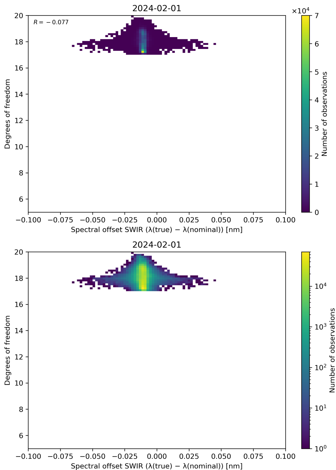
Figure 119: Scatter density plot of “Spectral offset SWIR ( \lambda(\text{true}) - \lambda(\text{nominal}) )” against “Degrees of freedom” for 2024-01-31 to 2024-02-02.
