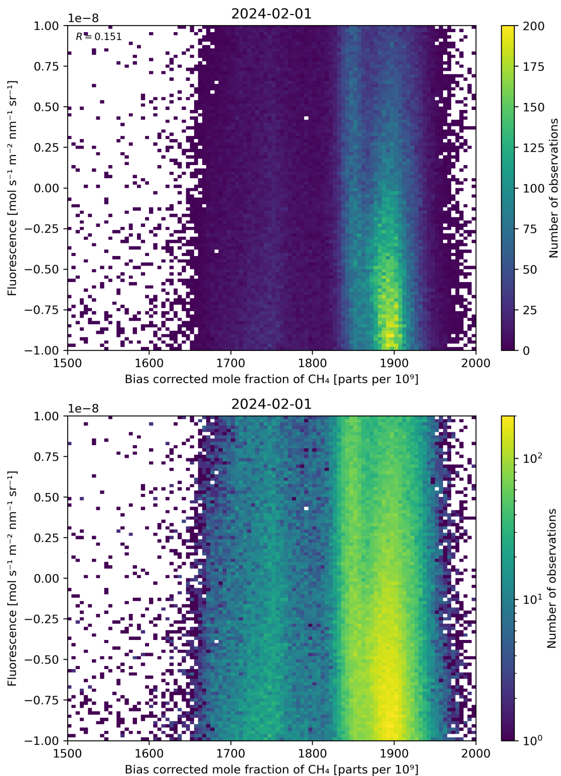
Figure 66: Scatter density plot of “Bias corrected mole fraction of CH 4 ” against “Fluorescence” for 2024-01-31 to 2024-02-02.
