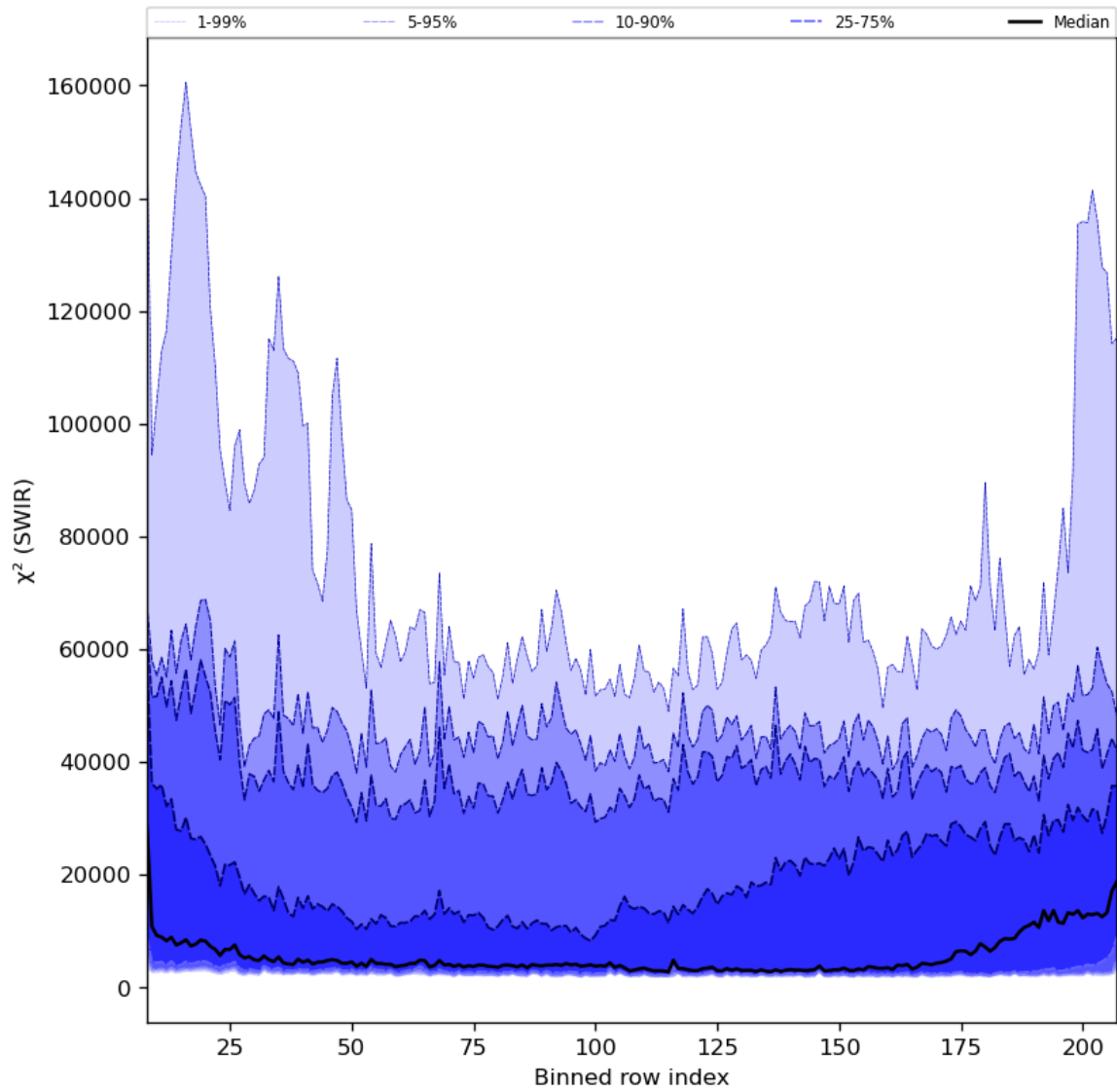
Figure 39: Along track statistics of “ \chi^2 (SWIR)” for 2024-01-31 to 2024-02-02
