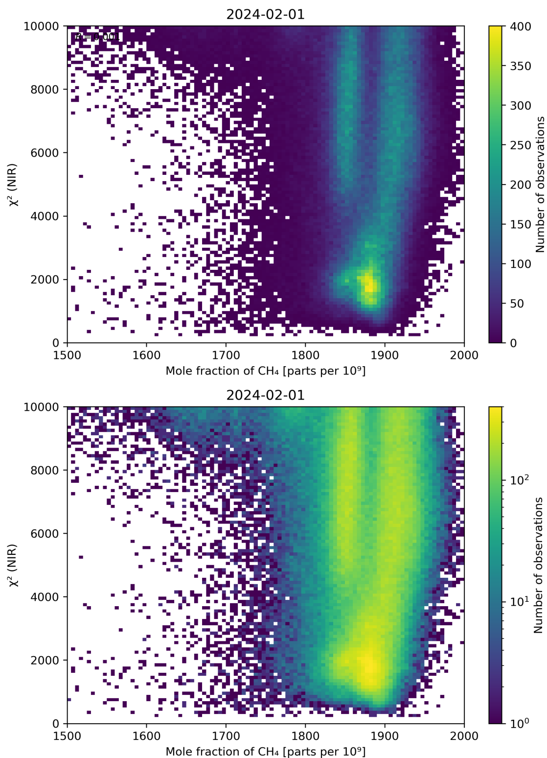
Figure 70: Scatter density plot of “Mole fraction of CH 4 ” against “ \chi^2 (NIR)” for 2024-01-31 to 2024-02-02.
