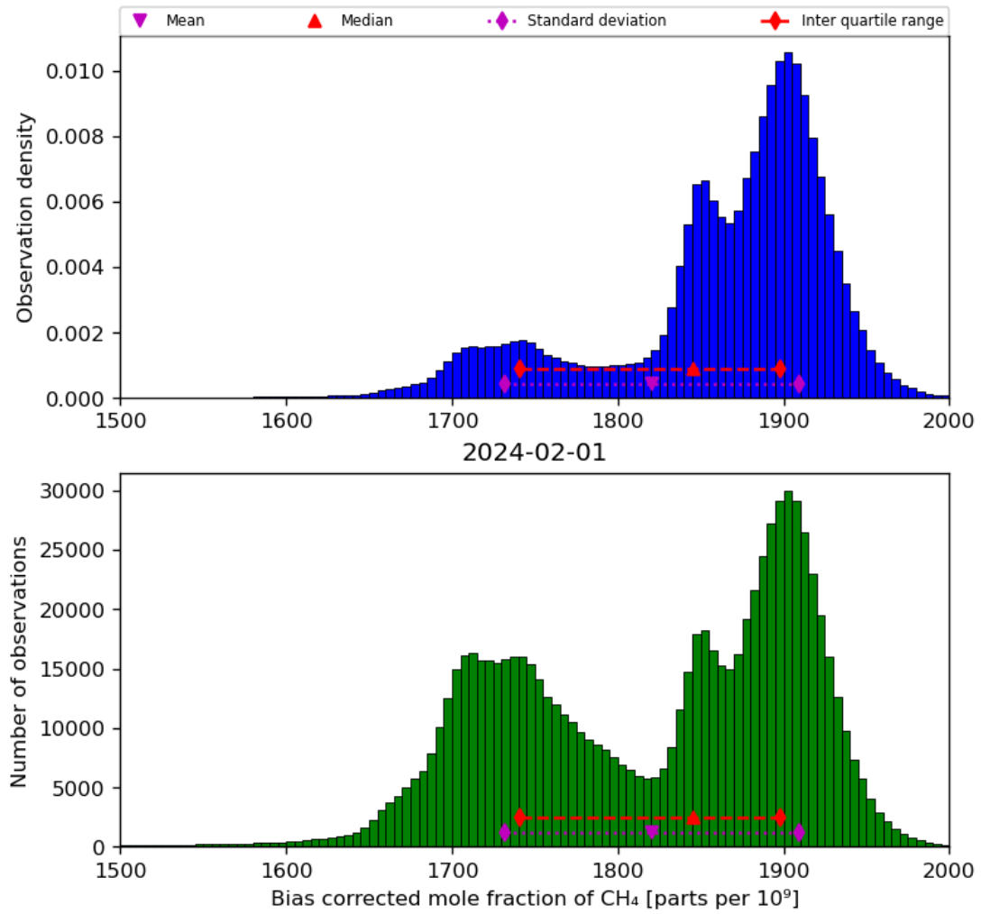
Figure 25: Histogram of “Bias corrected mole fraction of CH 4 ” for 2024-01-31 to 2024-02-02
