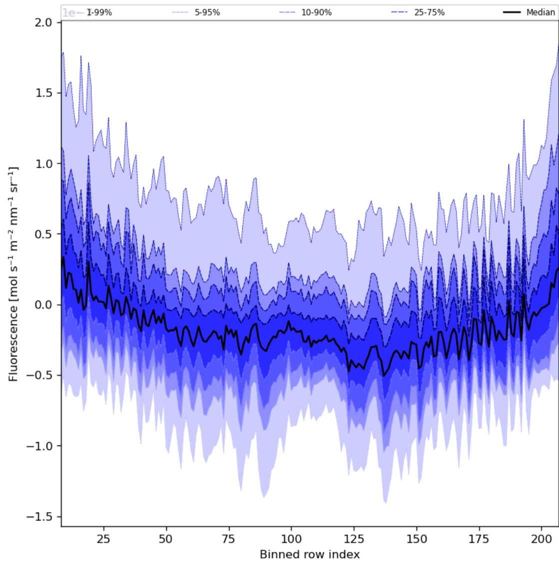
Figure 43: Along track statistics of “Fluorescence” for 2024-01-31 to 2024-02-02
