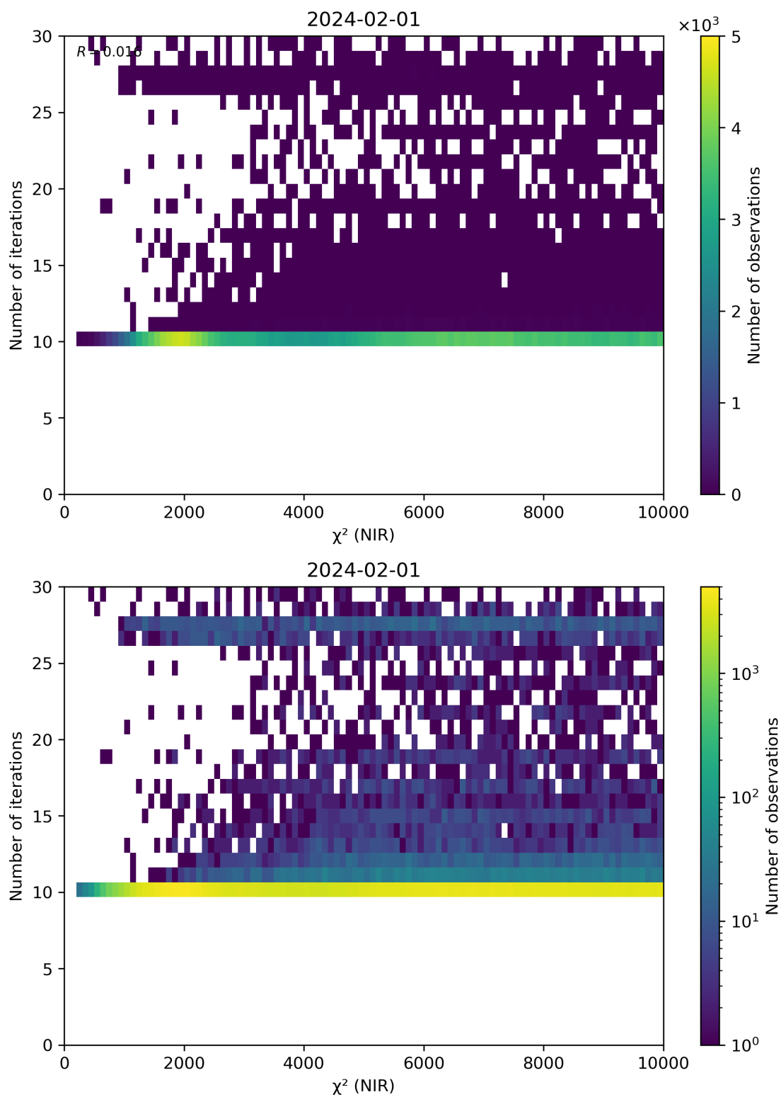
Figure 46: Scatter density plot of “ \chi^2 (NIR)” against “Number of iterations” for 2024-01-31 to 2024-02-02.
