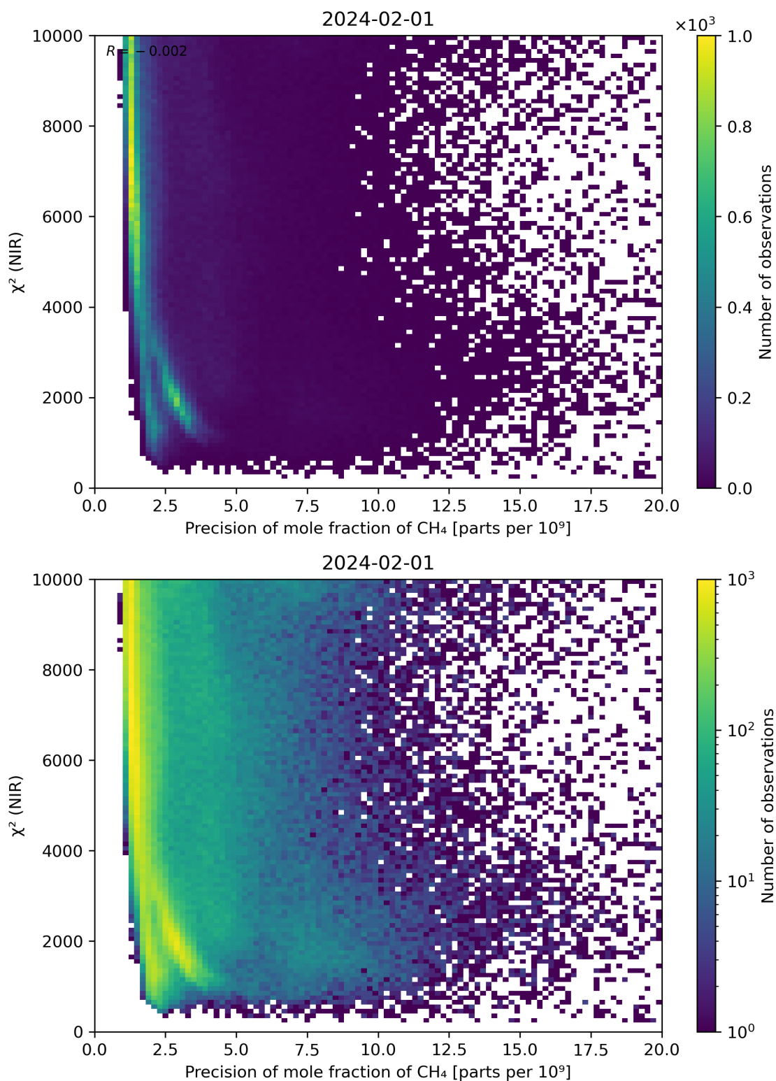
Figure 78: Scatter density plot of “Precision of mole fraction of \text{CH}_4 ” against “ \chi^2 (NIR)” for 2024-01-31 to 2024-02-02.
