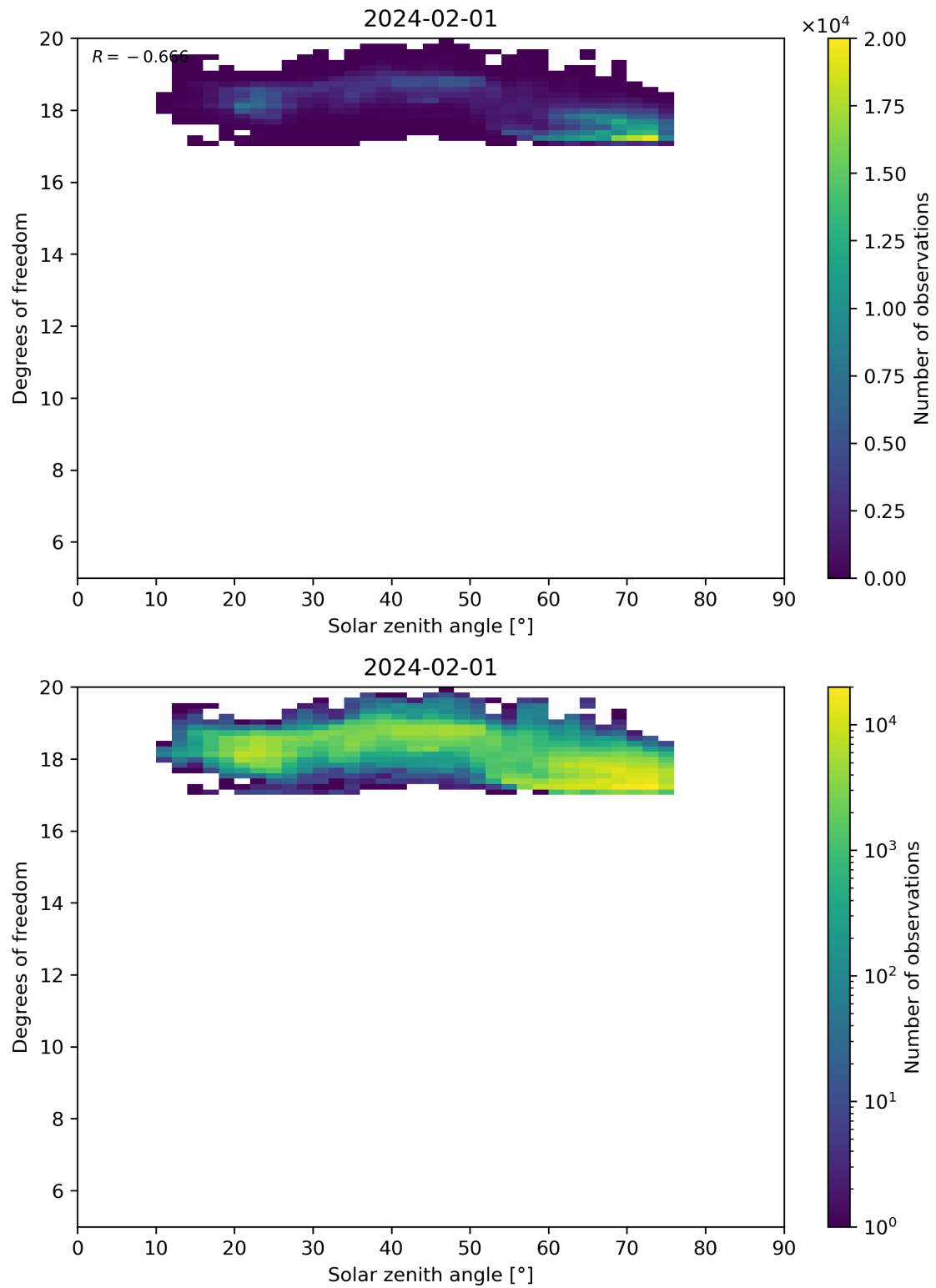
Figure 96: Scatter density plot of “Solar zenith angle” against “Degrees of freedom” for 2024-01-31 to 2024-02-02.
