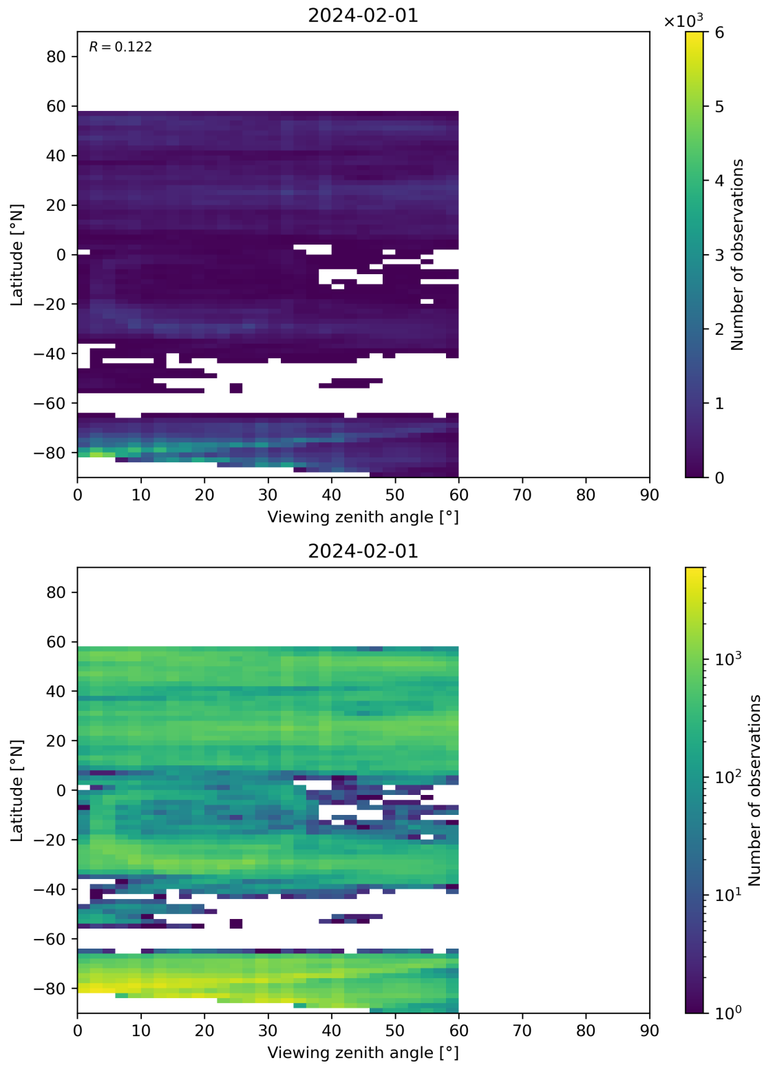
Figure 109: Scatter density plot of “Viewing zenith angle” against “Latitude” for 2024-01-31 to 2024-02-02.
