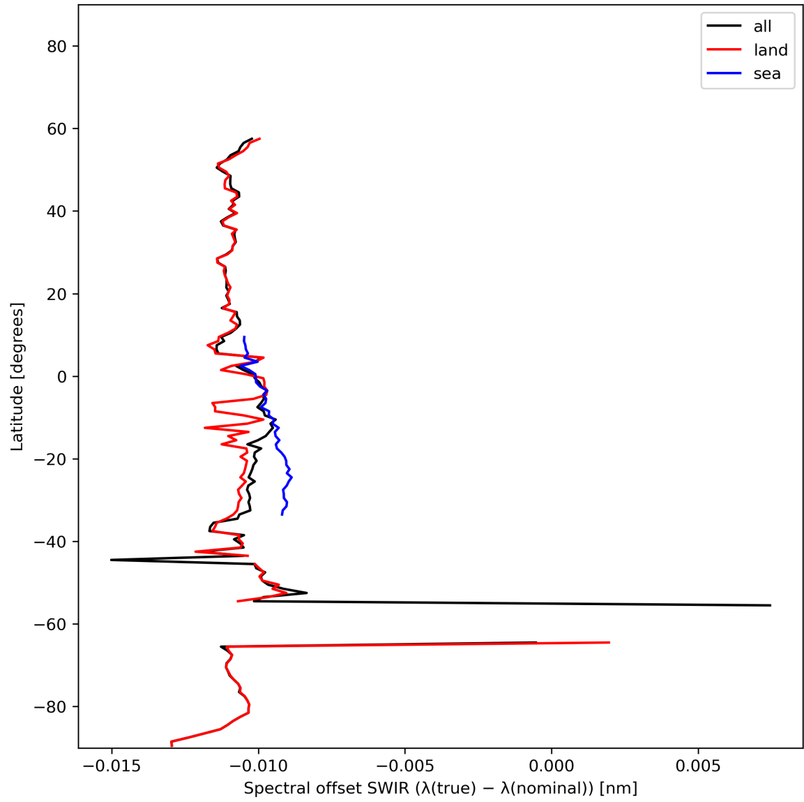
Figure 16: Zonal average of “Spectral offset SWIR ( \lambda(\text{true}) - \lambda(\text{nominal}) )” for 2024-01-31 to 2024-02-02.
