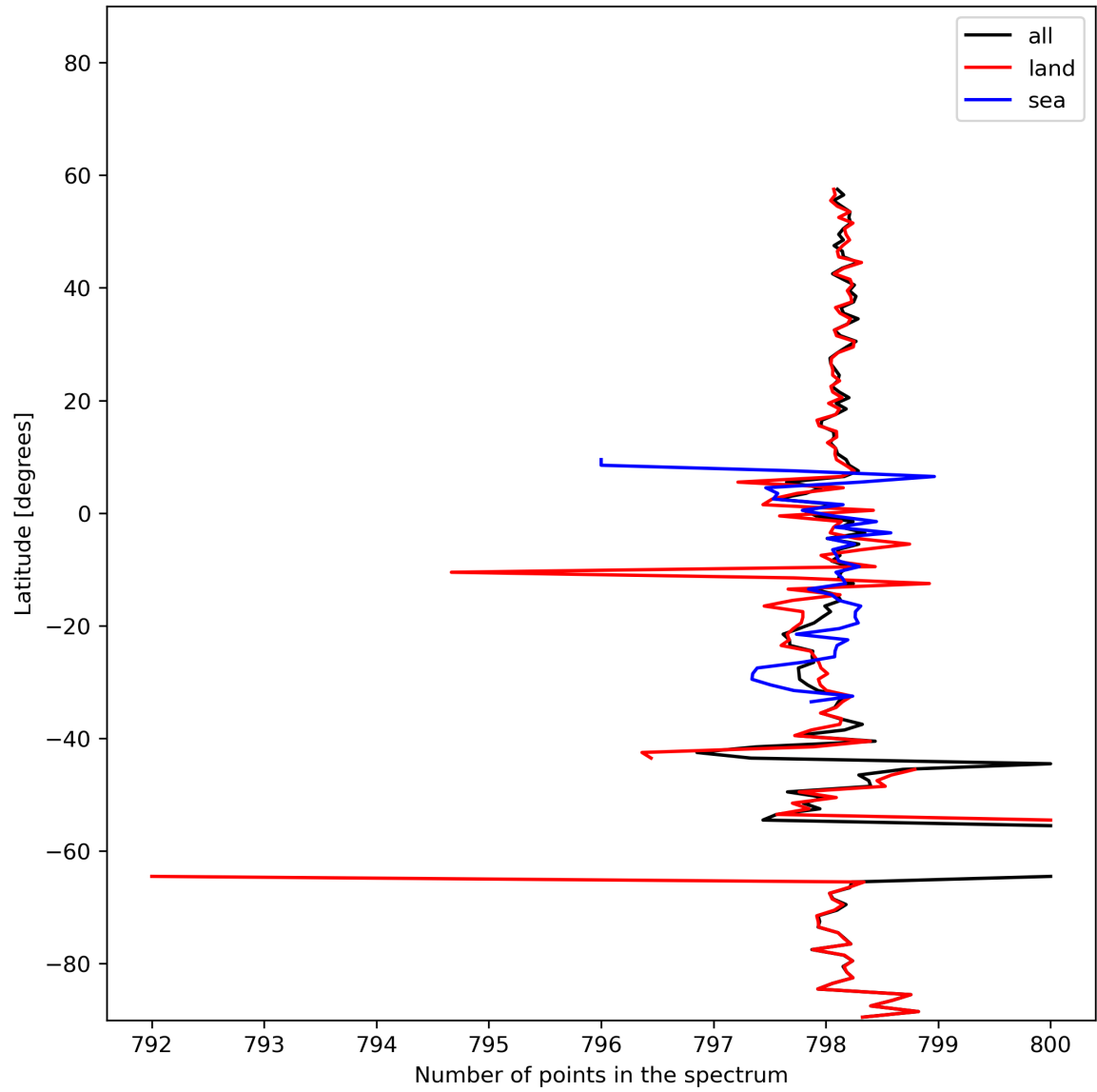
Figure 15: Zonal average of “Number of points in the spectrum” for 2024-01-31 to 2024-02-02.
