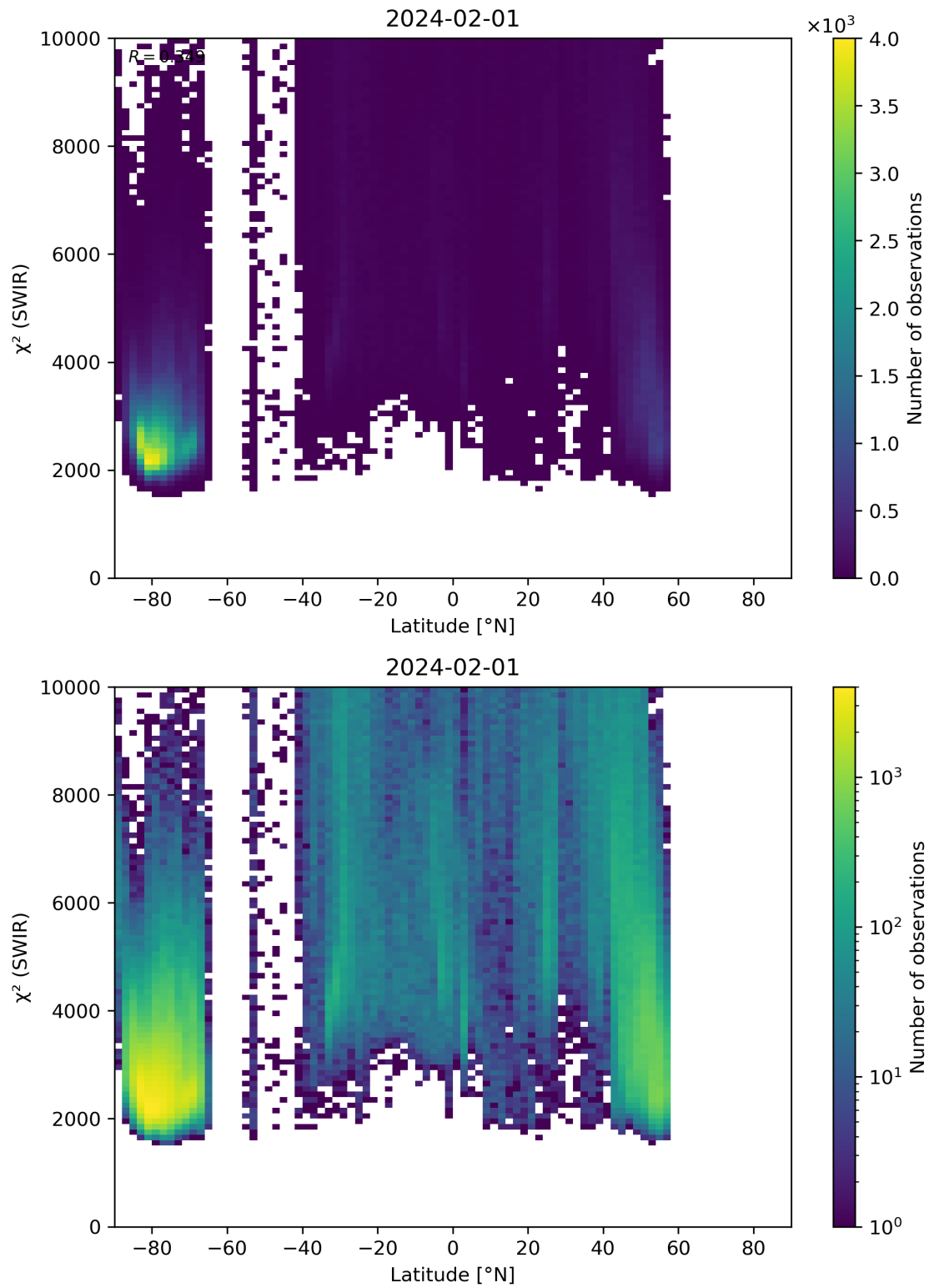
Figure 54: Scatter density plot of “Latitude” against “ \chi^2 (SWIR)” for 2024-01-31 to 2024-02-02.
