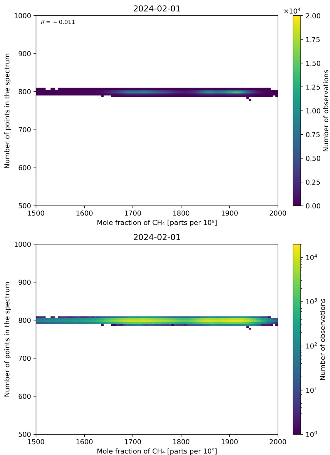
Figure 77: Scatter density plot of “Mole fraction of CH 4 ” against “Number of points in the spectrum” for 2024-01-31 to 2024-02-02.
