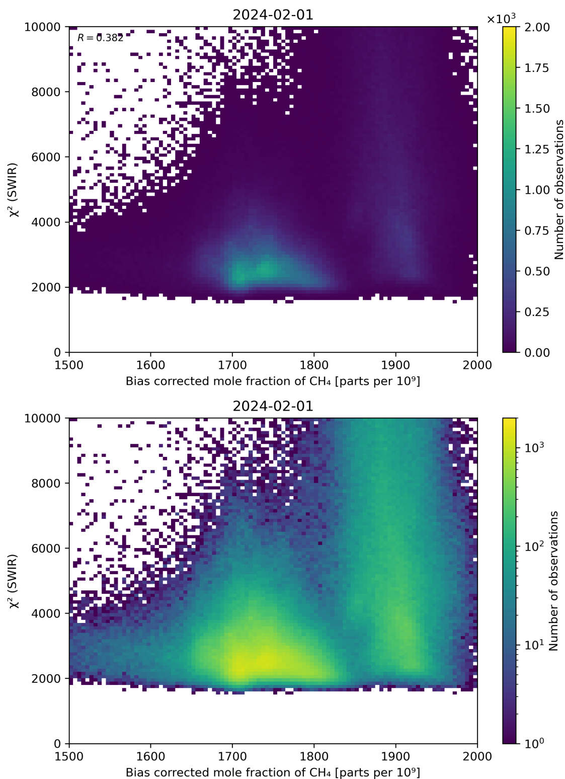
Figure 64: Scatter density plot of “Bias corrected mole fraction of CH 4 ” against “ \chi^2 (SWIR)” for 2024-01-31 to 2024-02-02.
