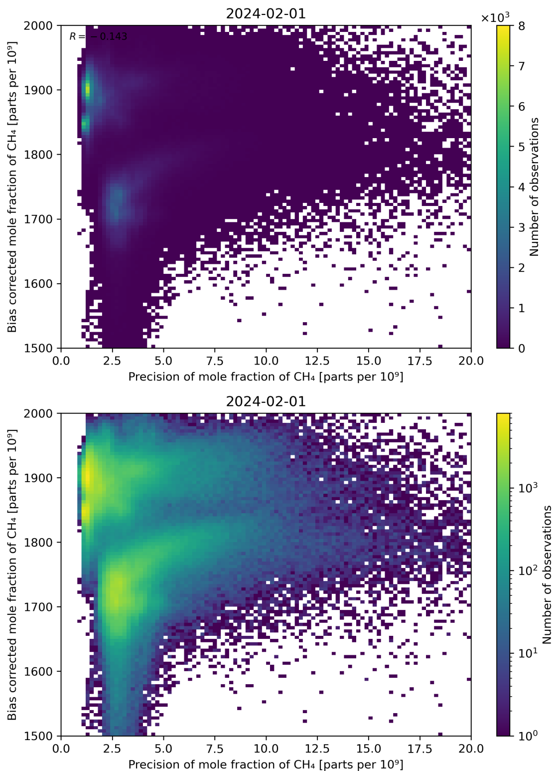
Figure 82: Scatter density plot of “Precision of mole fraction of CH 4 ” against “Bias corrected mole fraction of CH 4 ” for 2024-01-31 to 2024-02-02.
