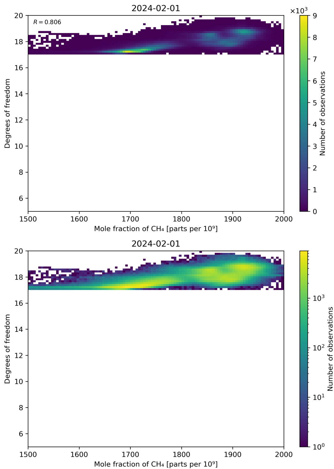
Figure 72: Scatter density plot of “Mole fraction of CH 4 ” against “Degrees of freedom” for 2024-01-31 to 2024-02-02.
