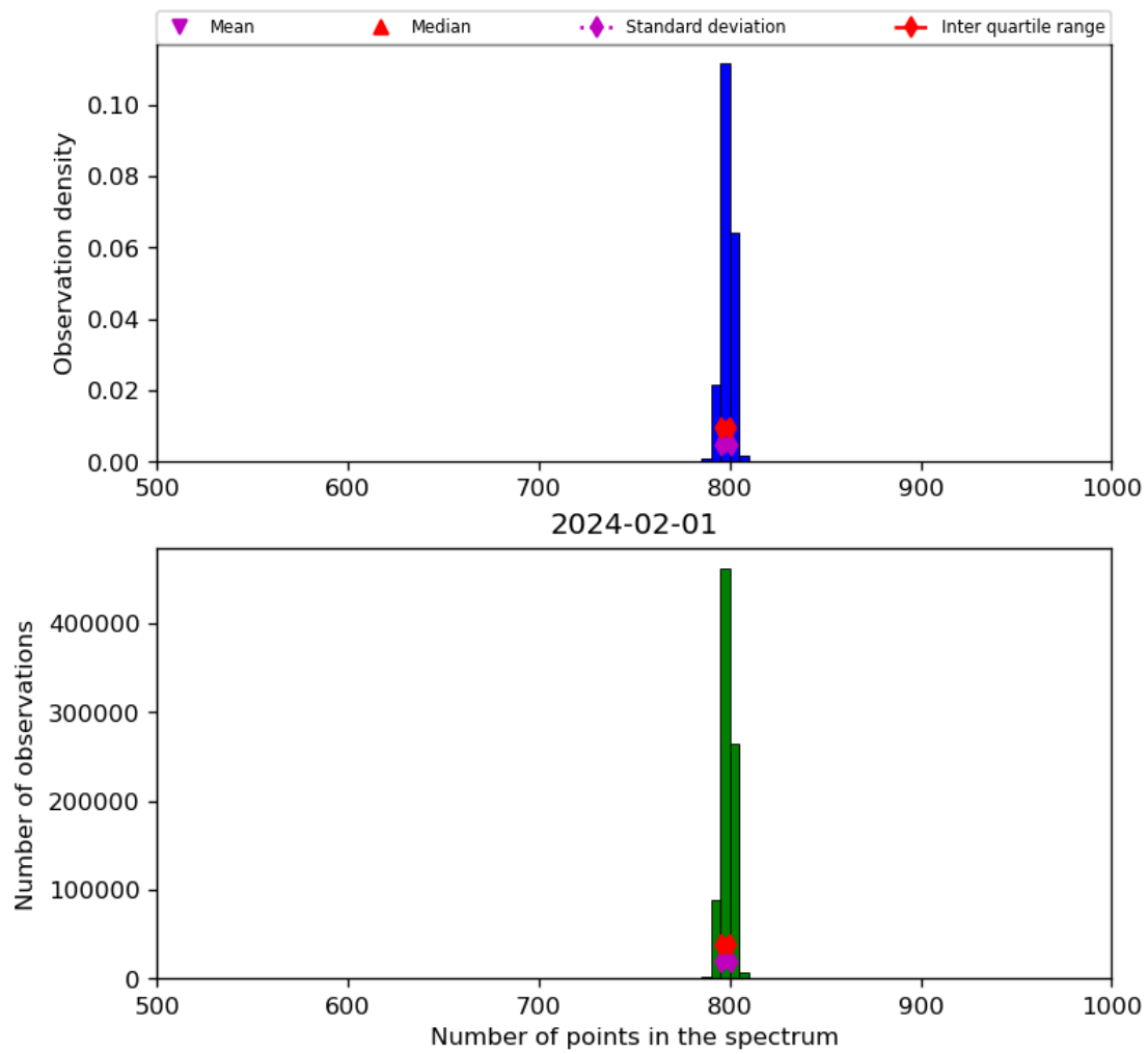
Figure 26: Histogram of “Number of points in the spectrum” for 2024-01-31 to 2024-02-02
