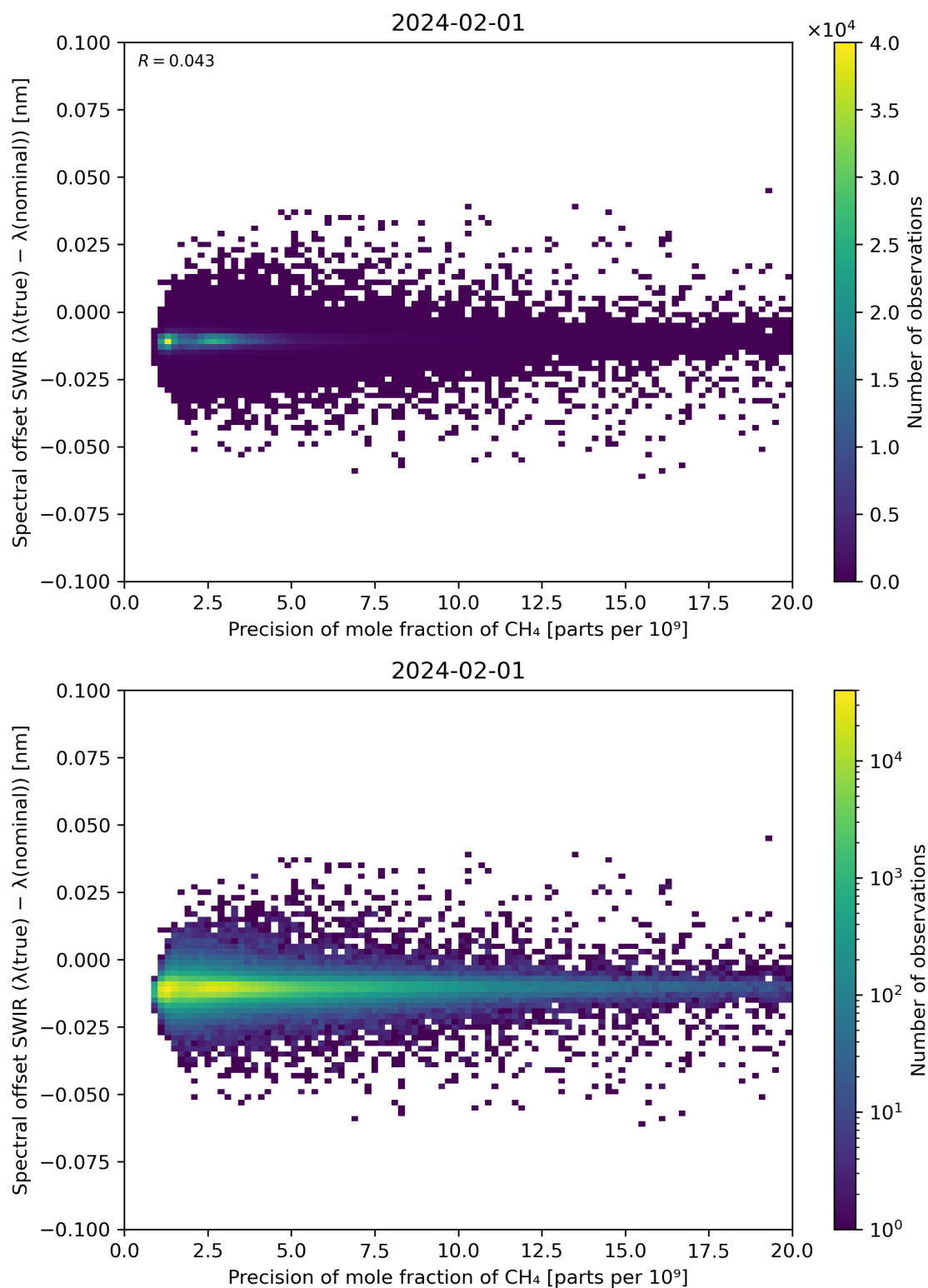
Figure 85: Scatter density plot of “Precision of mole fraction of \text{CH}_4 ” against “Spectral offset SWIR ( \lambda(\text{true}) - \lambda(\text{nominal}) )” for 2024-01-31 to 2024-02-02.
