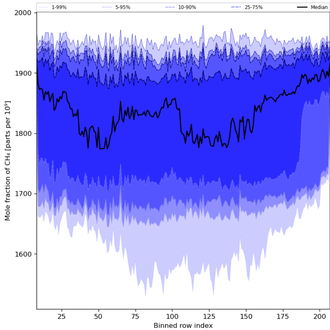
Figure 34: Along track statistics of “Mole fraction of CH 4 ” for 2024-01-31 to 2024-02-02
