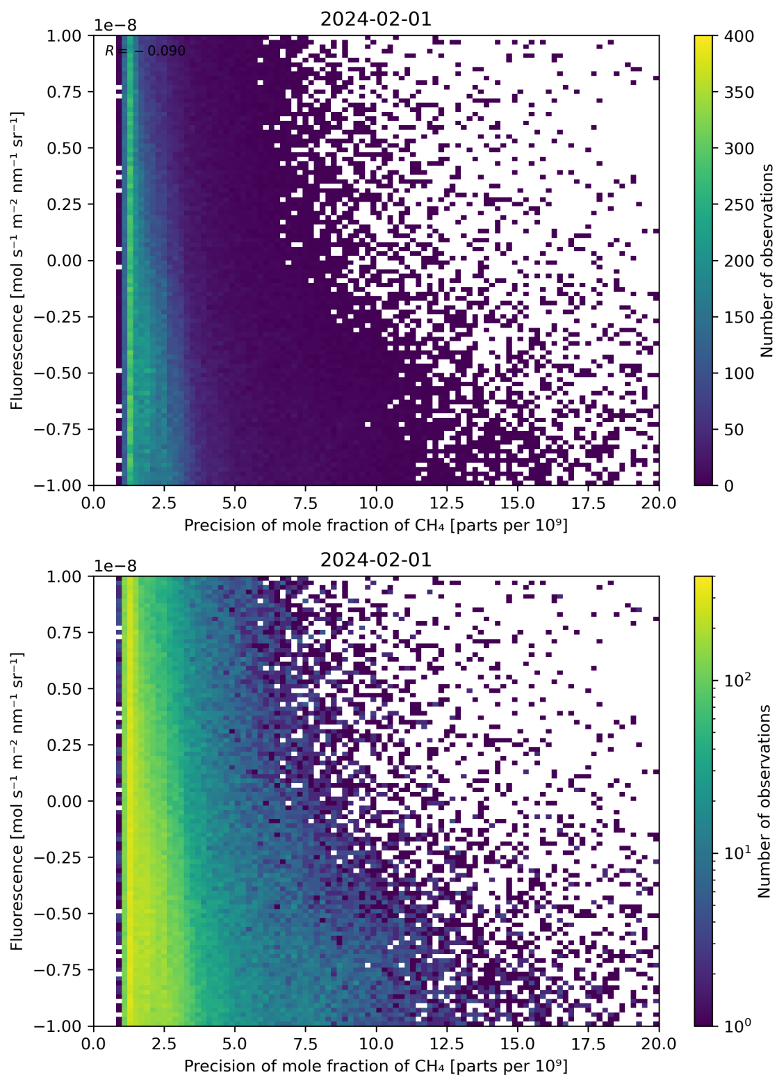
Figure 81: Scatter density plot of “Precision of mole fraction of \text{CH}_4 ” against “Fluorescence” for 2024-01-31 to 2024-02-02.
