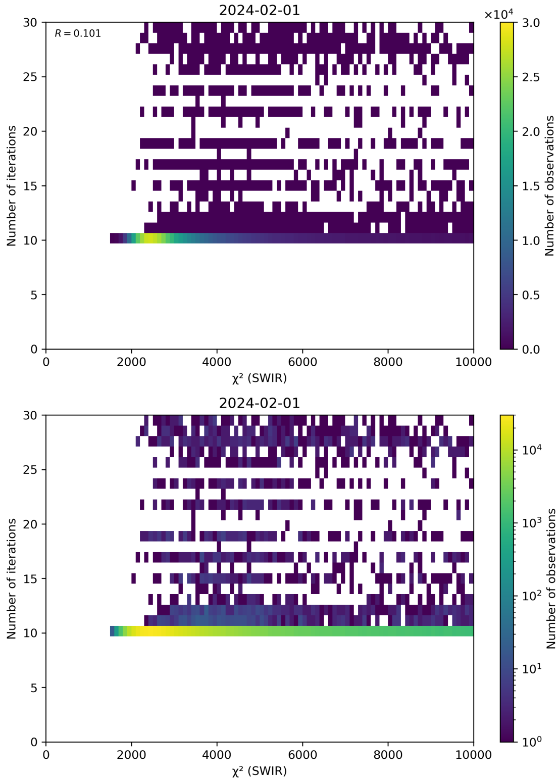
Figure 50: Scatter density plot of “ \chi^2 (SWIR)” against “Number of iterations” for 2024-01-31 to 2024-02-02.
