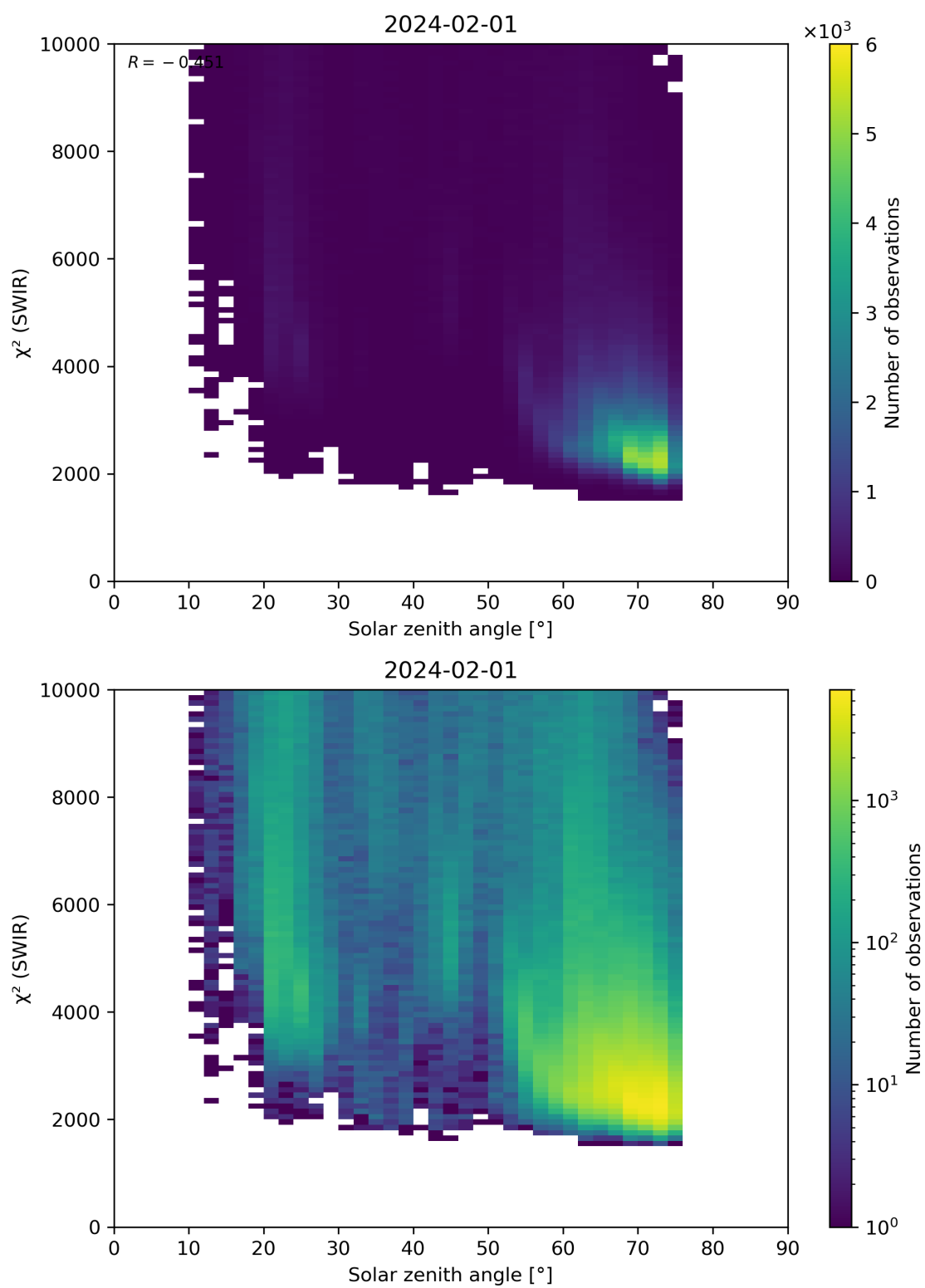
Figure 95: Scatter density plot of “Solar zenith angle” against “ \chi^2 (SWIR)” for 2024-01-31 to 2024-02-02.
