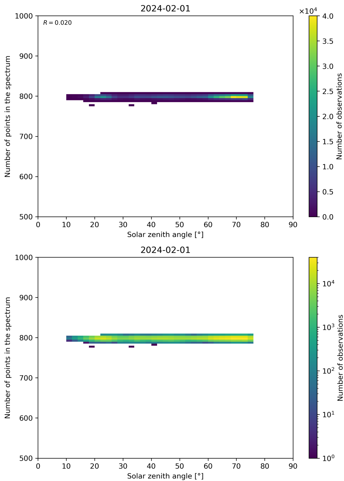
Figure 103: Scatter density plot of “Solar zenith angle” against “Number of points in the spectrum” for 2024-01-31 to 2024-02-02.
