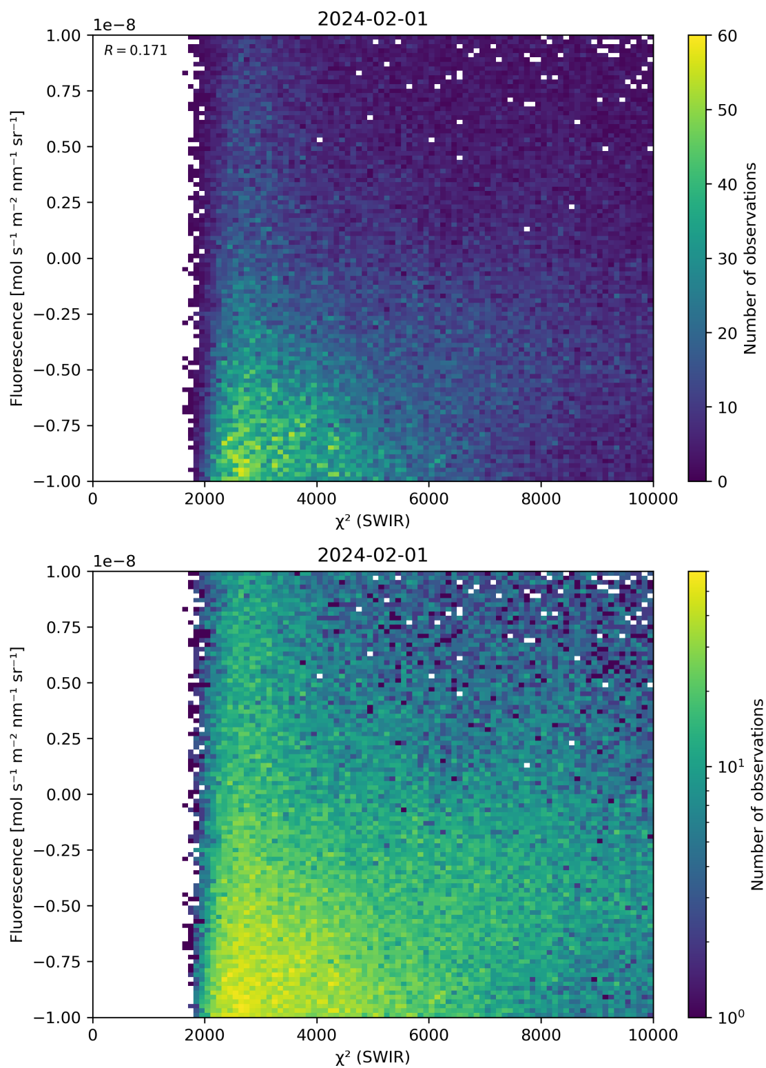
Figure 49: Scatter density plot of “ \chi^2 (SWIR)” against “Fluorescence” for 2024-01-31 to 2024-02-02.
