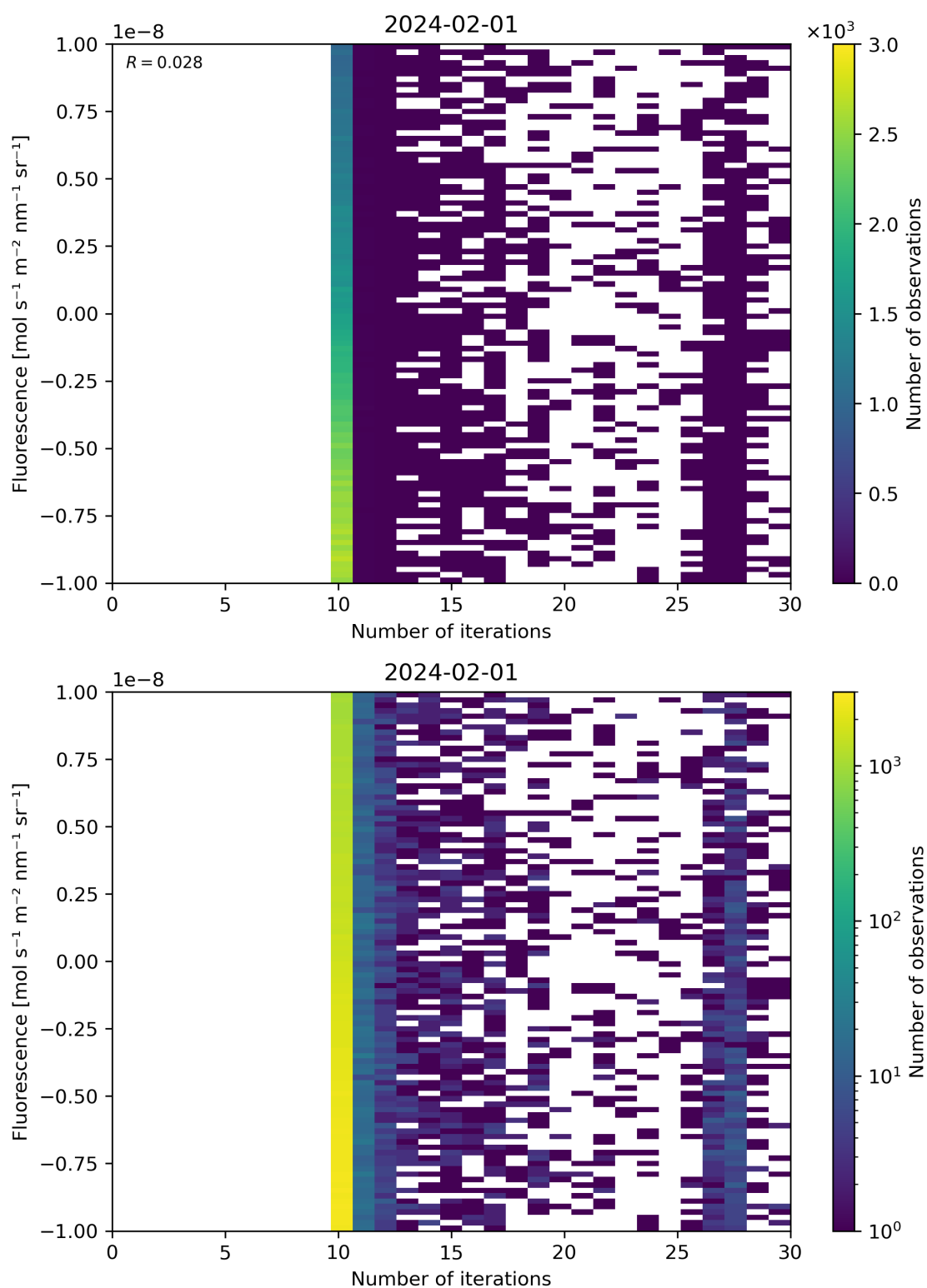
Figure 87: Scatter density plot of “Number of iterations” against “Fluorescence” for 2024-01-31 to 2024-02-02.
