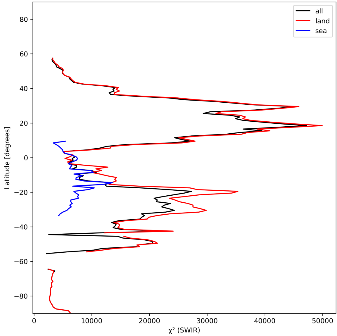
Figure 17: Zonal average of “ \chi^2 (SWIR)” for 2024-01-31 to 2024-02-02.
