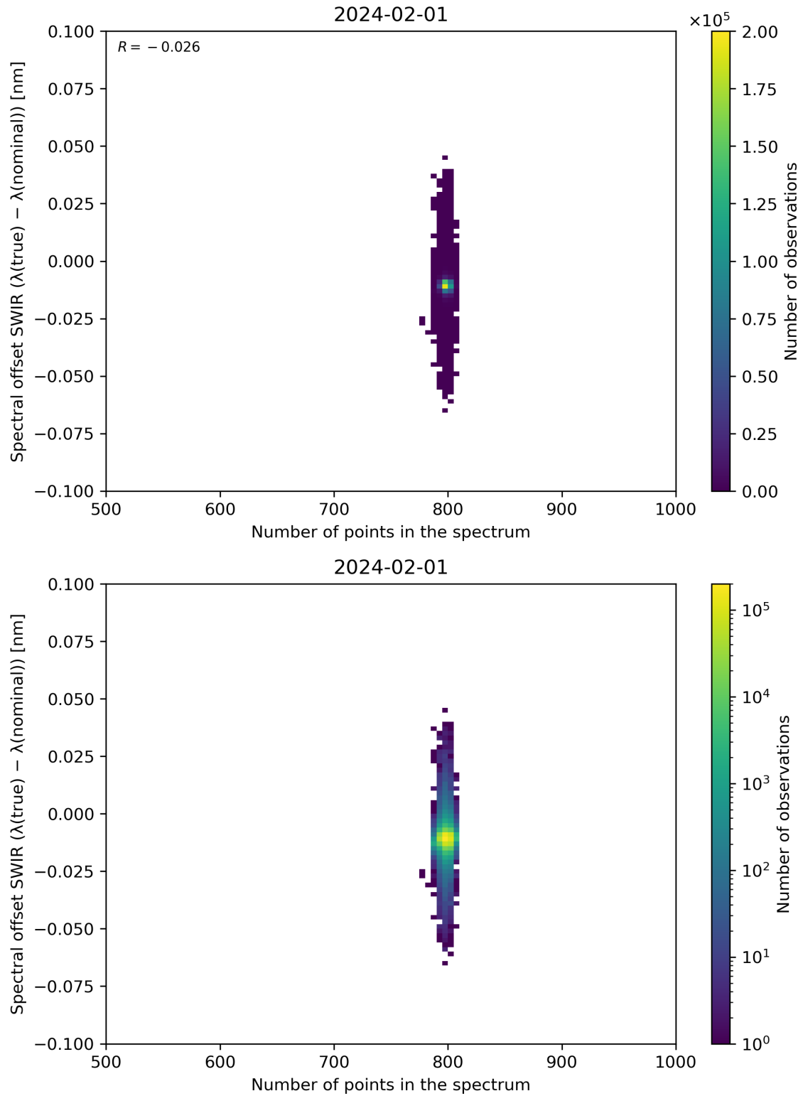
Figure 93: Scatter density plot of “Number of points in the spectrum” against “Spectral offset SWIR ( \lambda(\text{true}) - \lambda(\text{nominal}) )” for 2024-01-31 to 2024-02-02.
