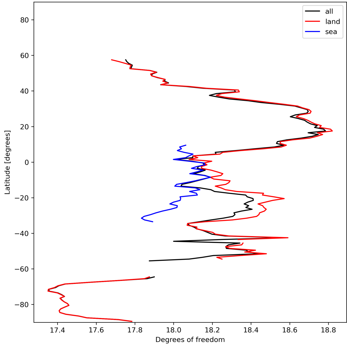
Figure 19: Zonal average of “Degrees of freedom” for 2024-01-31 to 2024-02-02.
