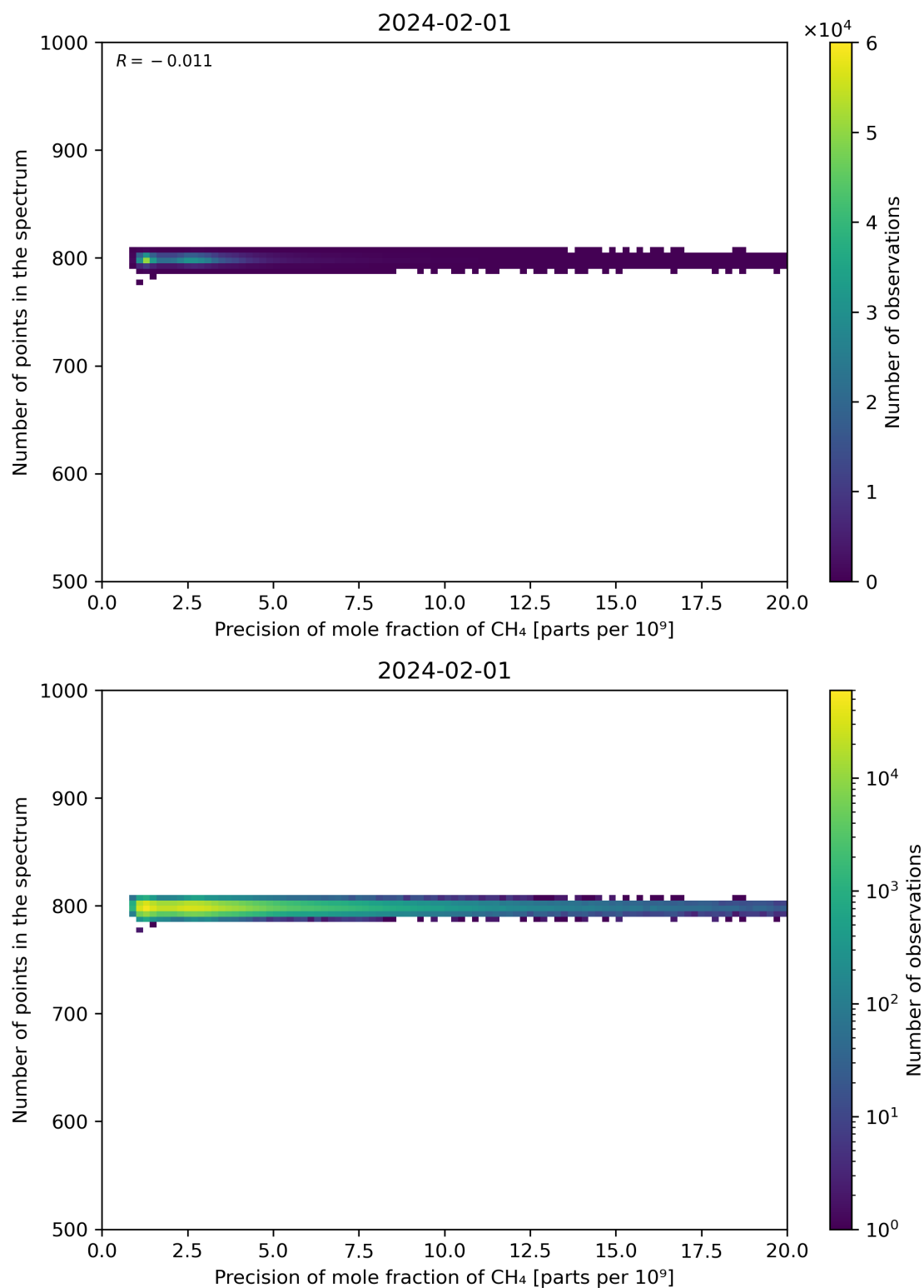
Figure 84: Scatter density plot of “Precision of mole fraction of CH 4 ” against “Number of points in the spectrum” for 2024-01-31 to 2024-02-02.
