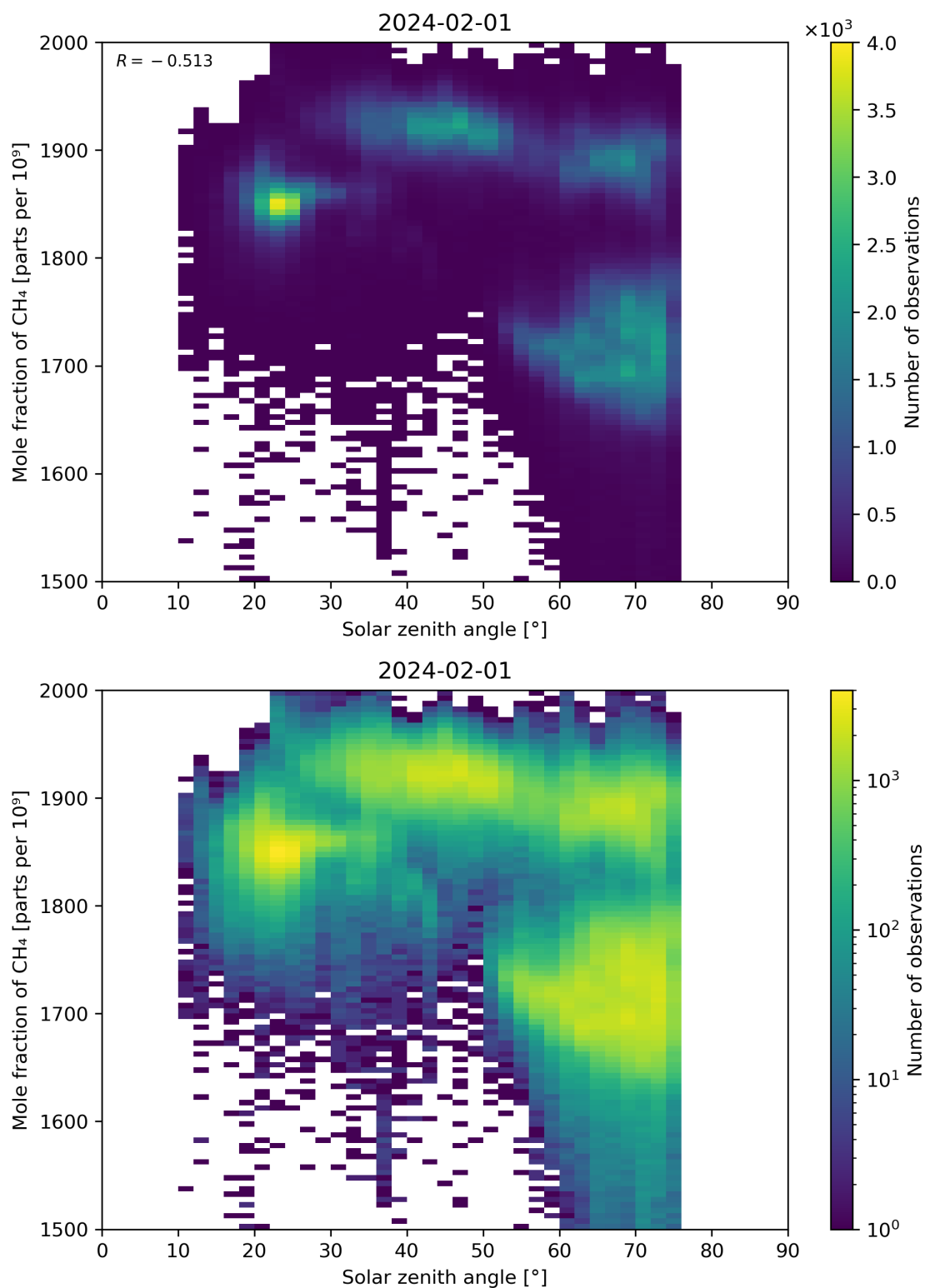
Figure 99: Scatter density plot of “Solar zenith angle” against “Mole fraction of CH 4 ” for 2024-01-31 to 2024-02-02.
