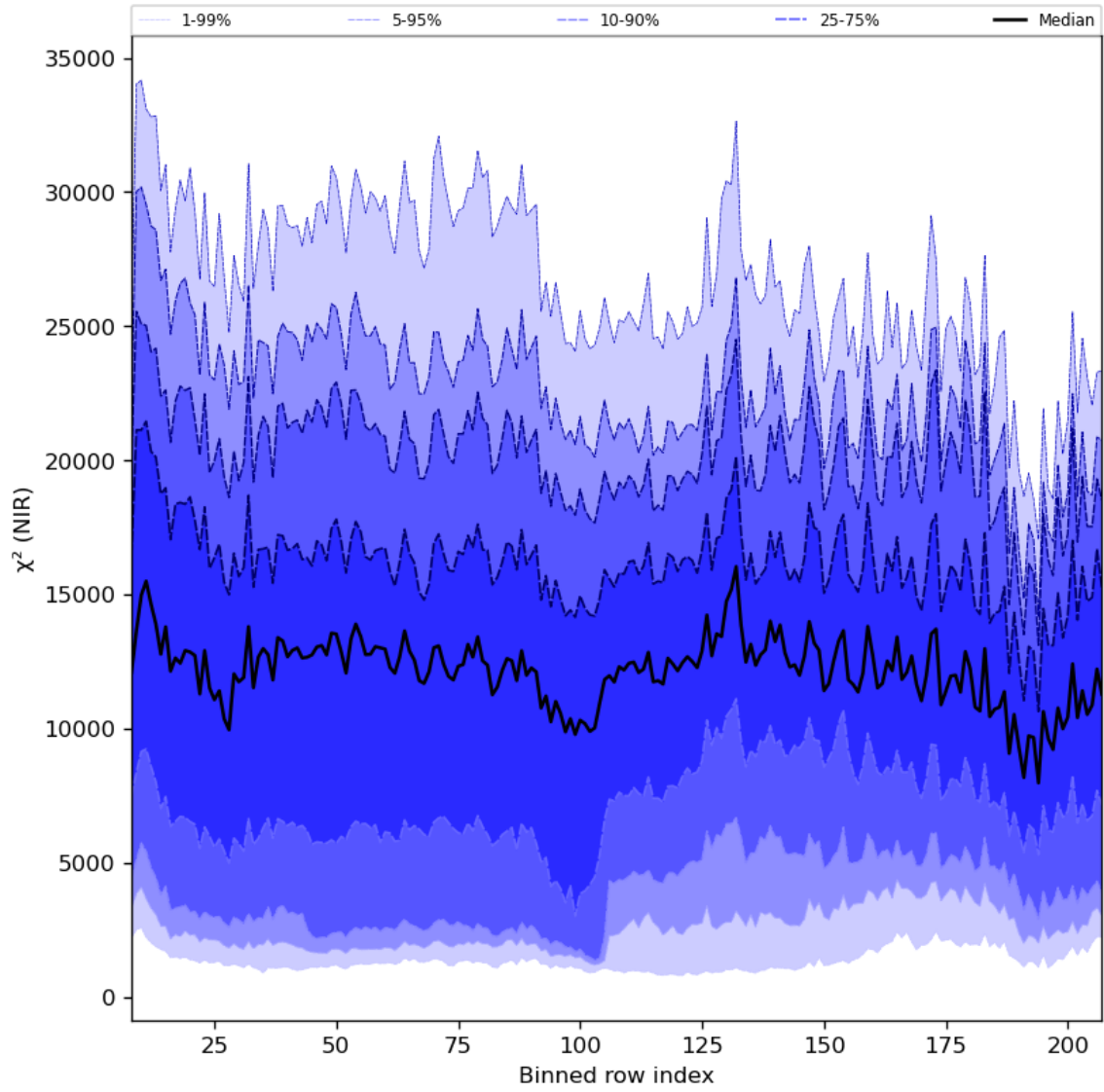
Figure 40: Along track statistics of “ \chi^2 (NIR)” for 2024-01-31 to 2024-02-02
