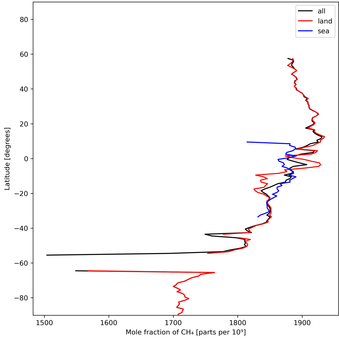
Figure 12: Zonal average of “Mole fraction of \text{CH}_4 ” for 2024-01-31 to 2024-02-02.
