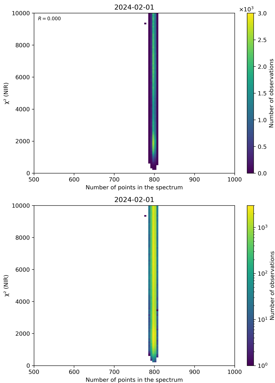
Figure 88: Scatter density plot of “Number of points in the spectrum” against “ \chi^2 (NIR)” for 2024-01-31 to 2024-02-02.
