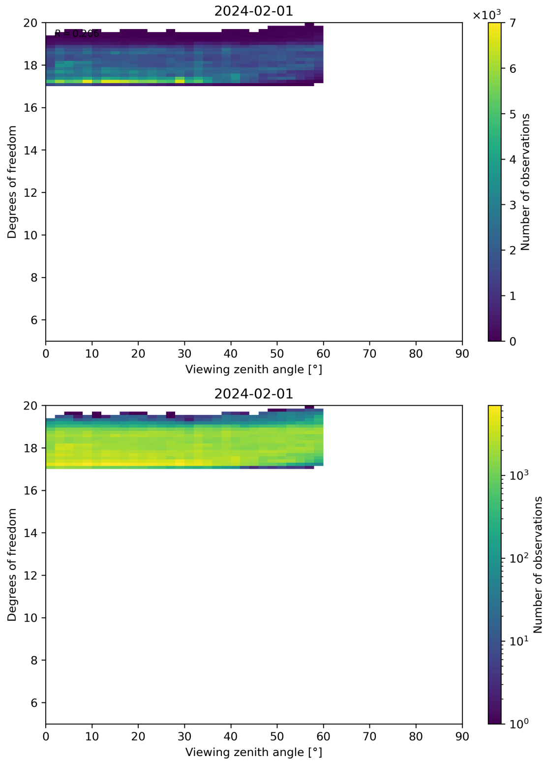
Figure 107: Scatter density plot of “Viewing zenith angle” against “Degrees of freedom” for 2024-01-31 to 2024-02-02.
