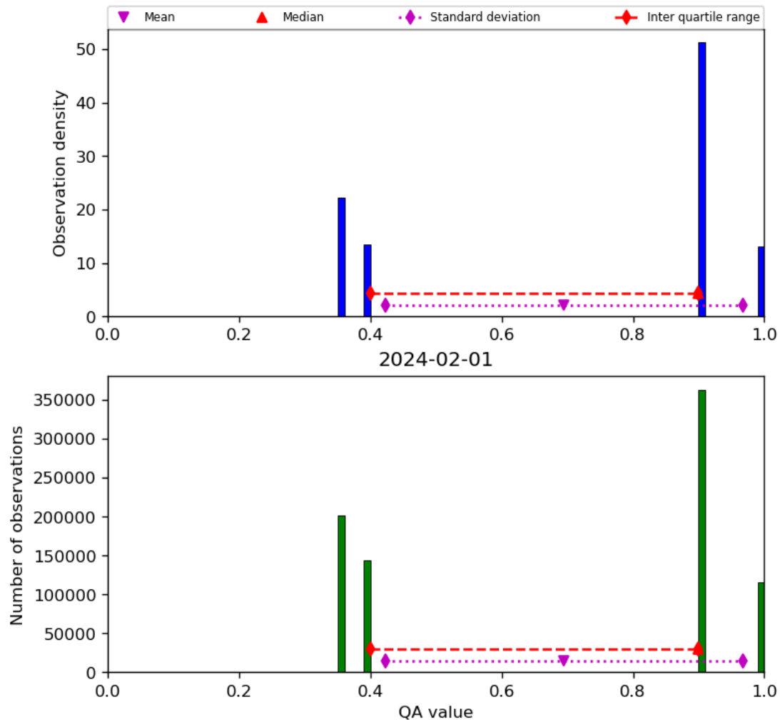
Figure 22: Histogram of “QA value” for 2024-01-31 to 2024-02-02
