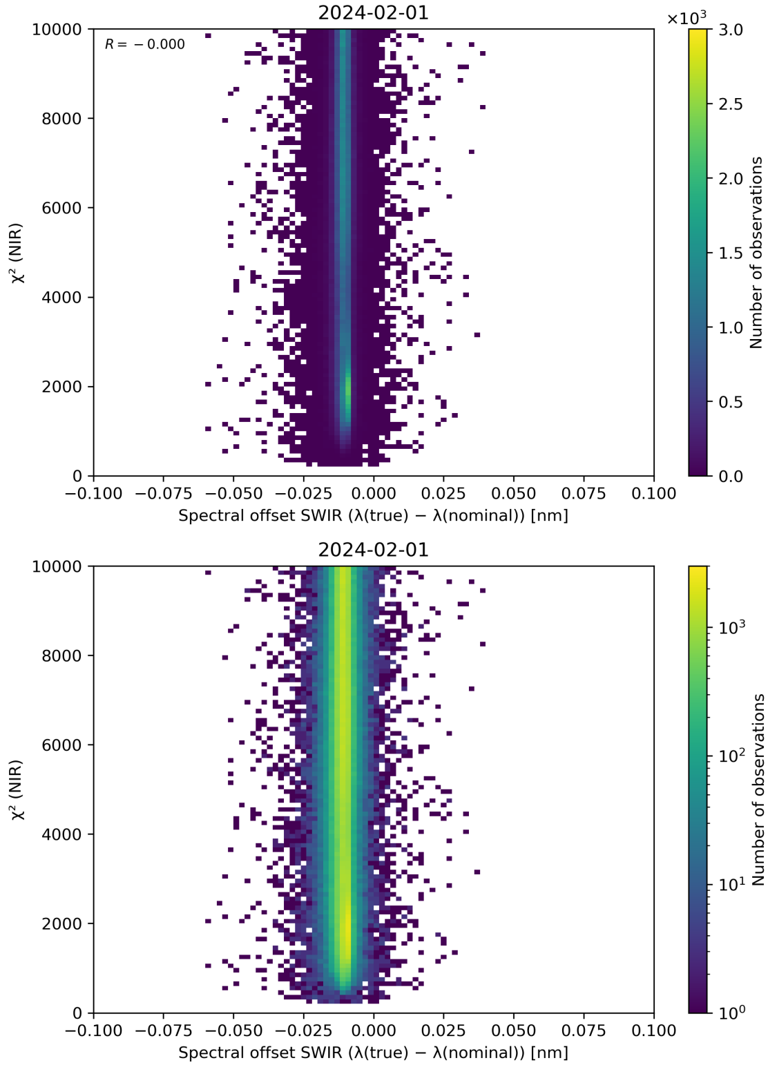
Figure 117: Scatter density plot of “Spectral offset SWIR ( \lambda(\text{true}) - \lambda(\text{nominal}) )” against “ \chi^2 (NIR)” for 2024-01-31 to 2024-02-02.
