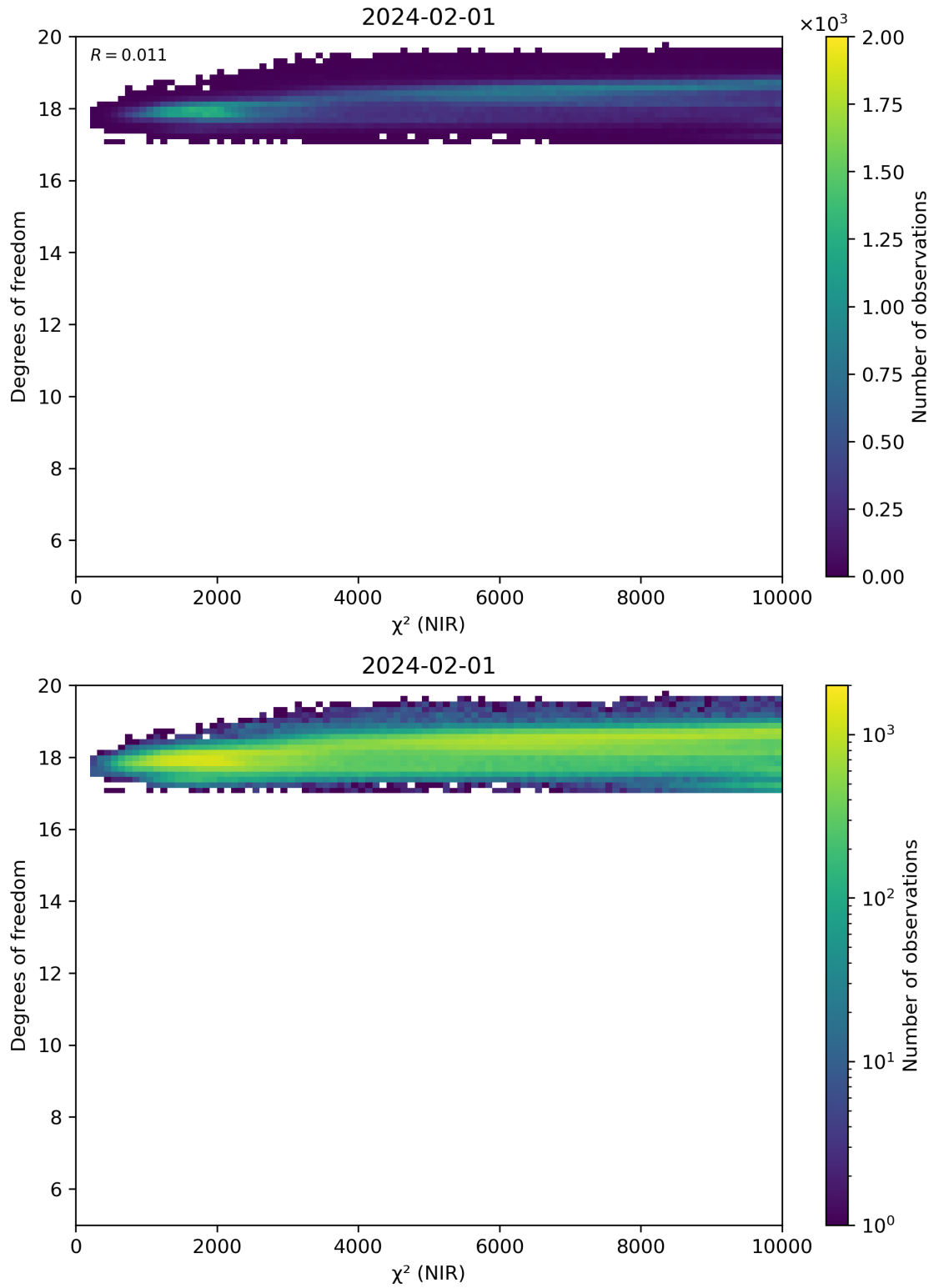
Figure 44: Scatter density plot of “ \chi^2 (NIR)” against “Degrees of freedom” for 2024-01-31 to 2024-02-02.
