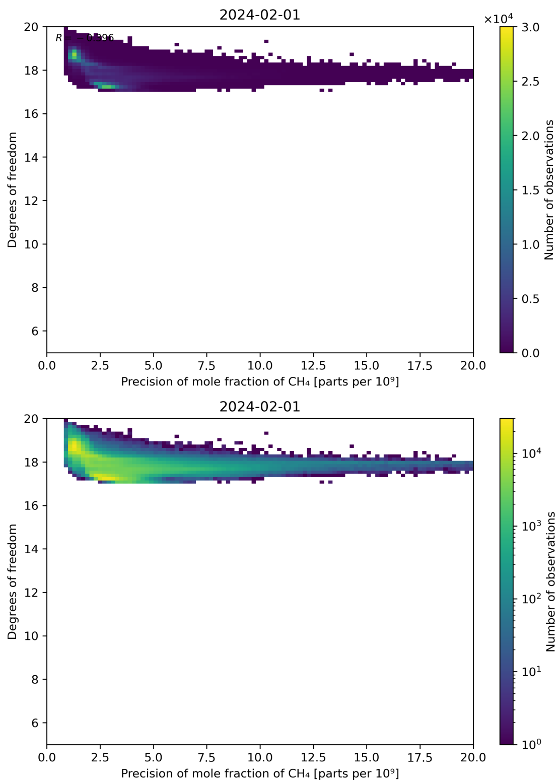
Figure 80: Scatter density plot of “Precision of mole fraction of CH 4 ” against “Degrees of freedom” for 2024-01-31 to 2024-02-02.
