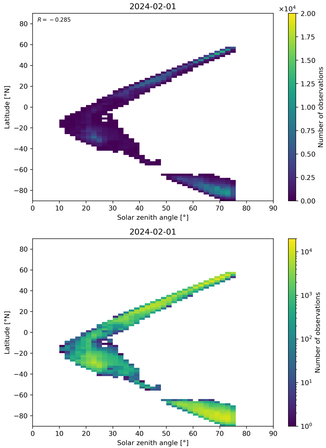
Figure 98: Scatter density plot of “Solar zenith angle” against “Latitude” for 2024-01-31 to 2024-02-02.
