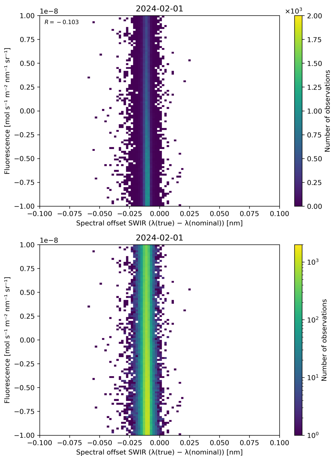
Figure 120: Scatter density plot of “Spectral offset SWIR ( \lambda(\text{true}) - \lambda(\text{nominal}) )” against “Fluorescence” for 2024-01-31 to 2024-02-02.
