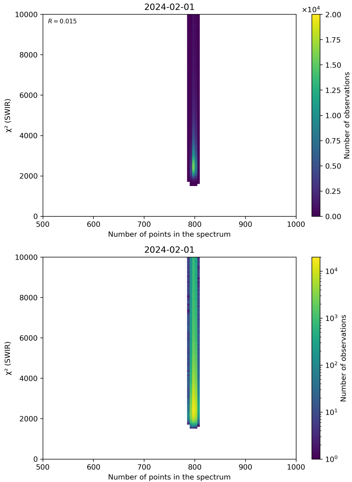
Figure 89: Scatter density plot of “Number of points in the spectrum” against “ \chi^2 (SWIR)” for 2024-01-31 to 2024-02-02.
