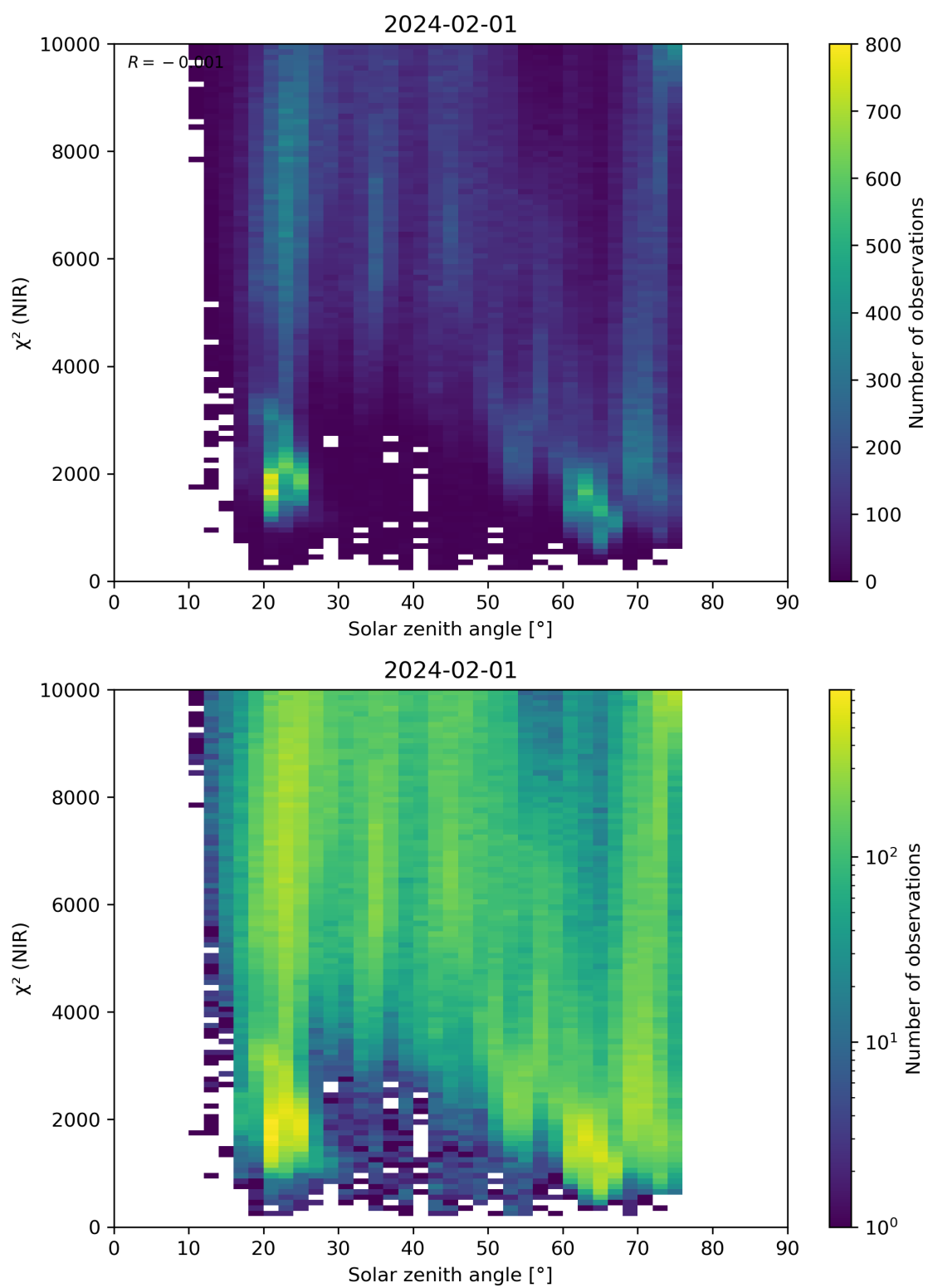
Figure 94: Scatter density plot of “Solar zenith angle” against “ \chi^2 (NIR)” for 2024-01-31 to 2024-02-02.
