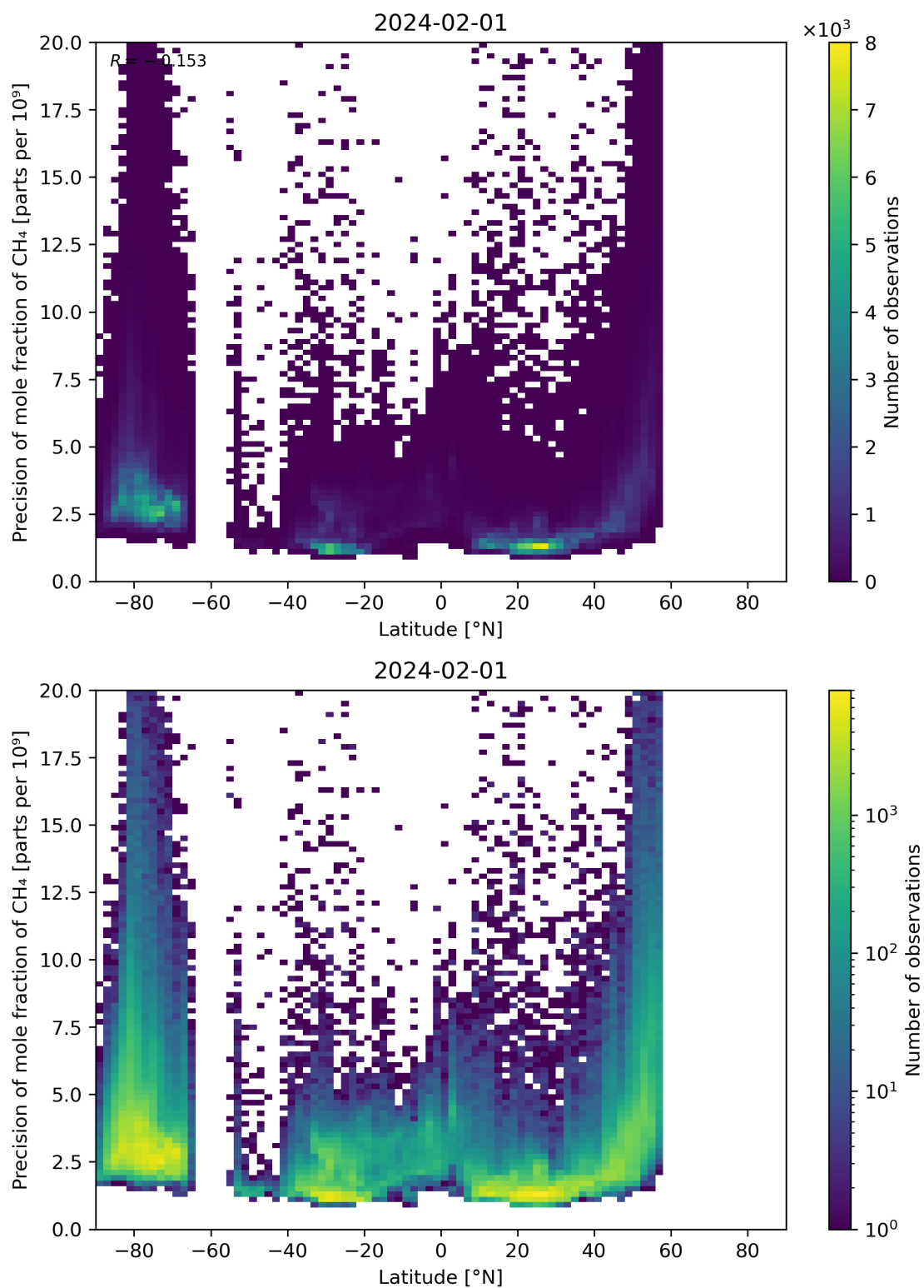
Figure 59: Scatter density plot of “Latitude” against “Precision of mole fraction of CH 4 ” for 2024-01-31 to 2024-02-02.
