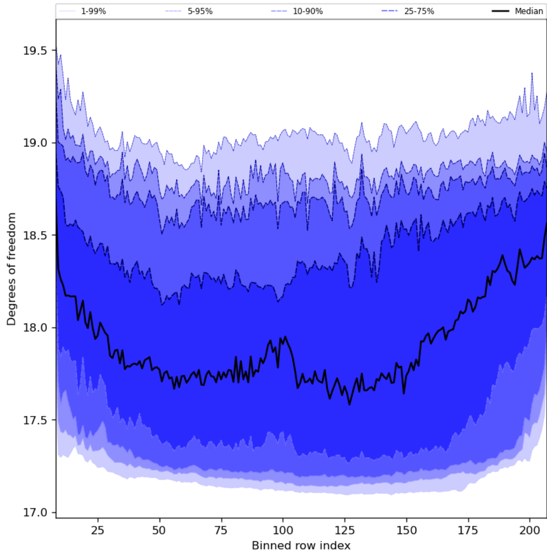
Figure 41: Along track statistics of “Degrees of freedom” for 2024-01-31 to 2024-02-02
