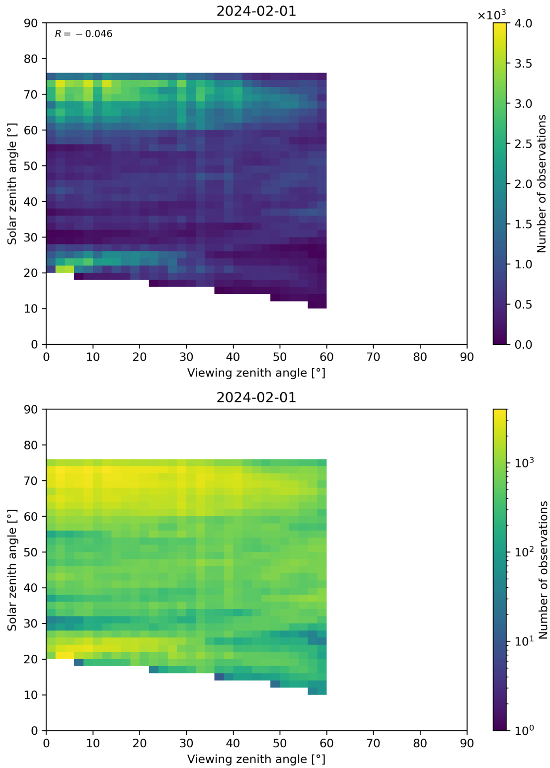
Figure 115: Scatter density plot of “Viewing zenith angle” against “Solar zenith angle” for 2024-01-31 to 2024-02-02.
