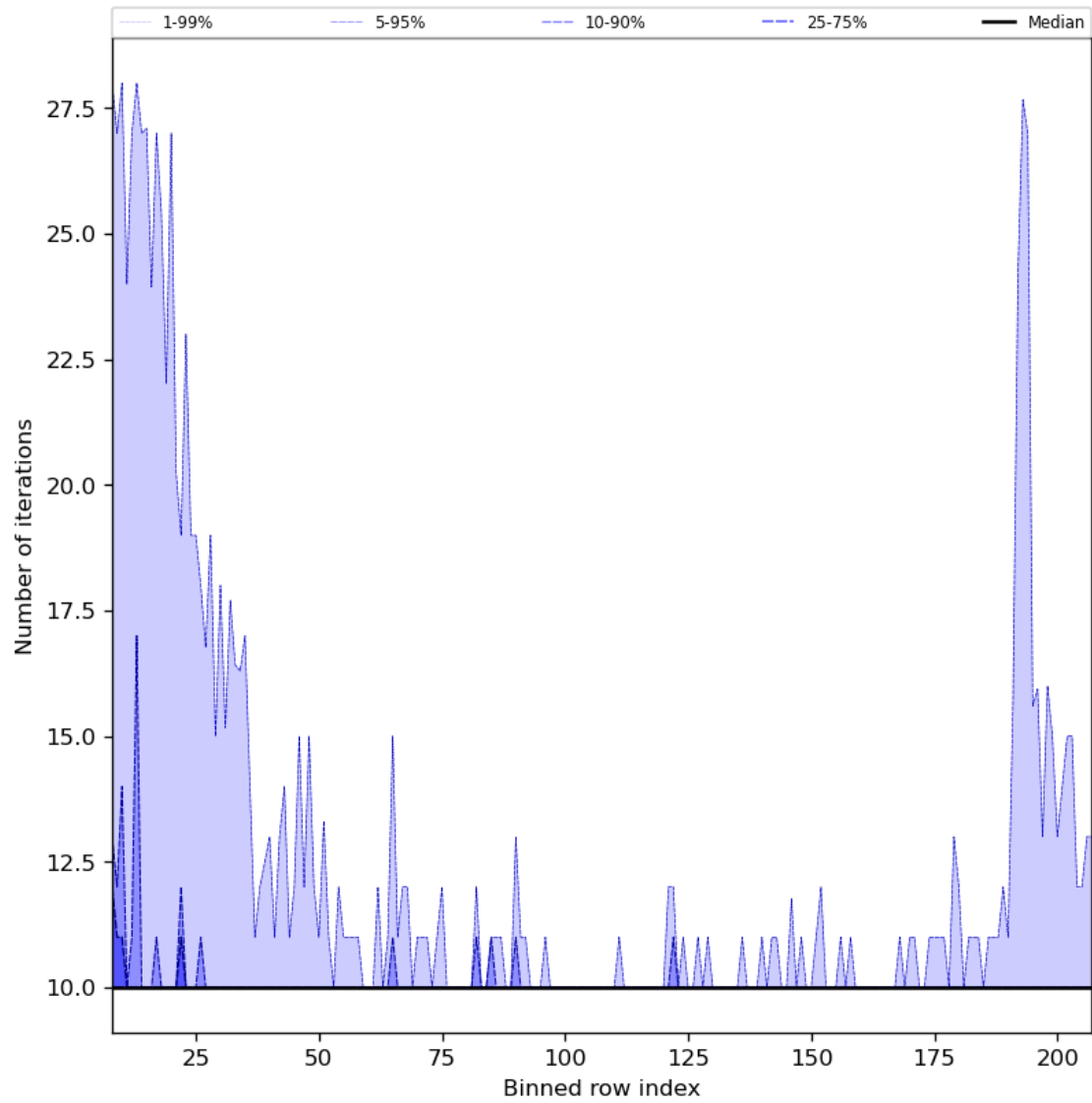
Figure 42: Along track statistics of “Number of iterations” for 2024-01-31 to 2024-02-02
