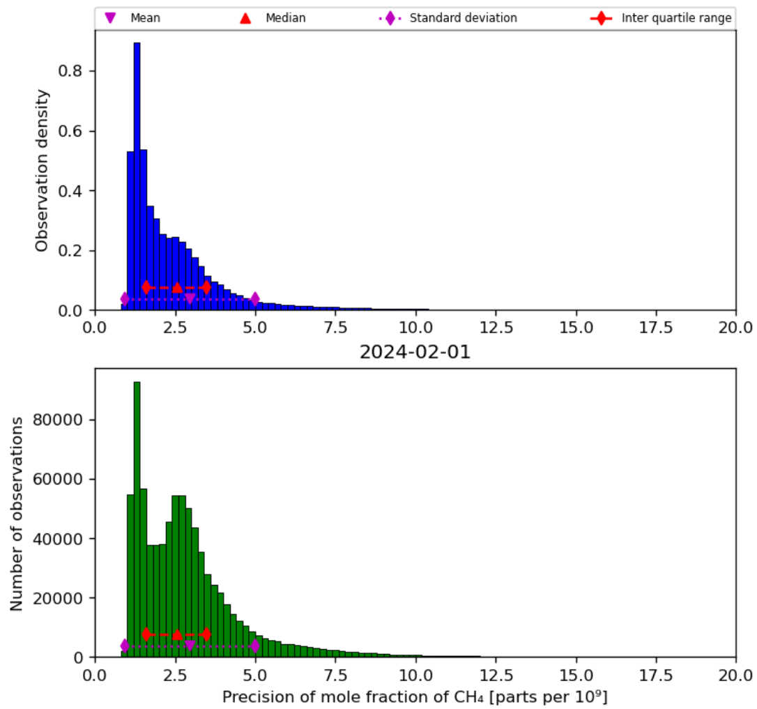
Figure 24: Histogram of “Precision of mole fraction of CH 4 ” for 2024-01-31 to 2024-02-02
