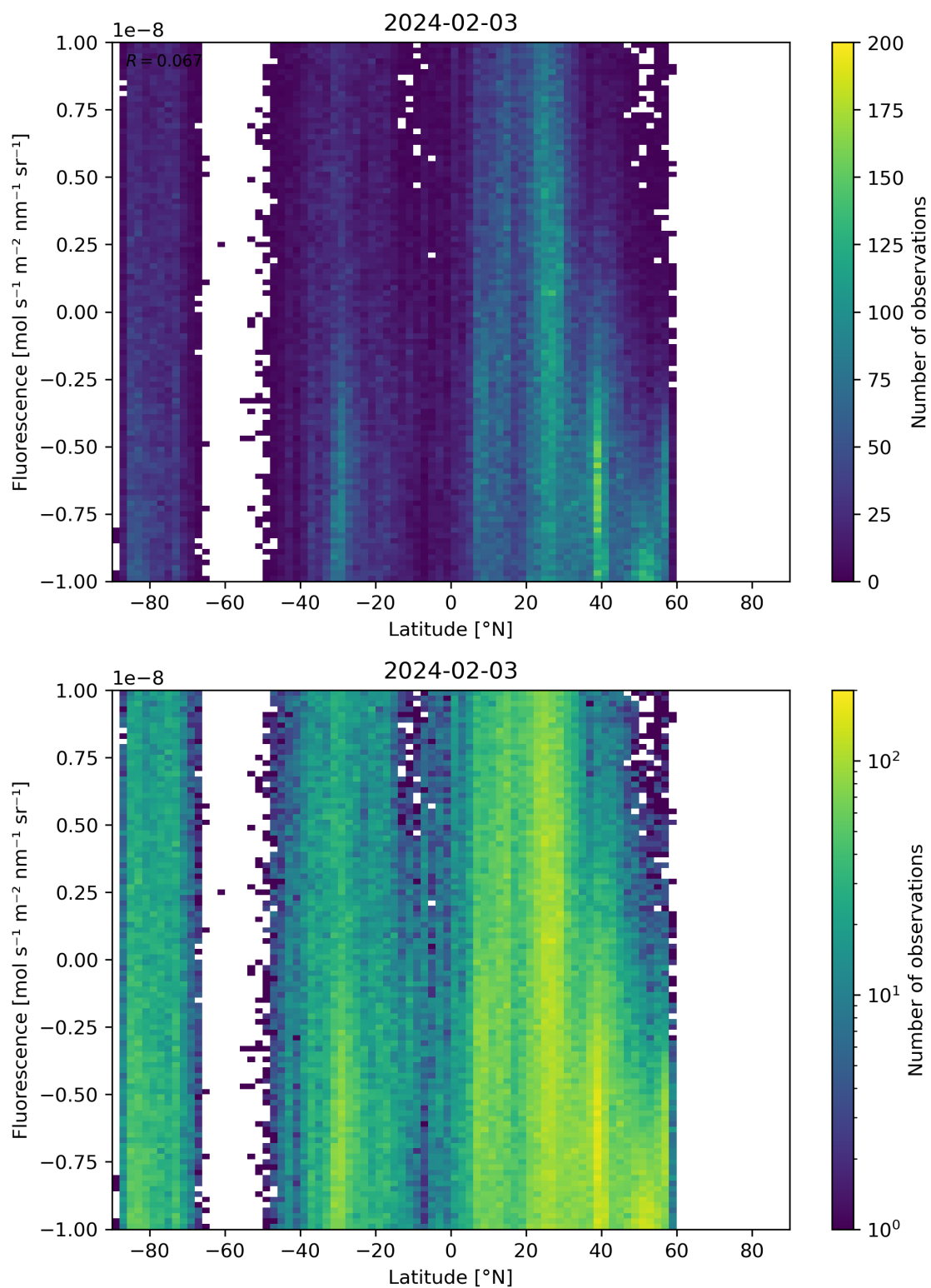
Figure 56: Scatter density plot of “Latitude” against “Fluorescence” for 2024-02-02 to 2024-02-04.
