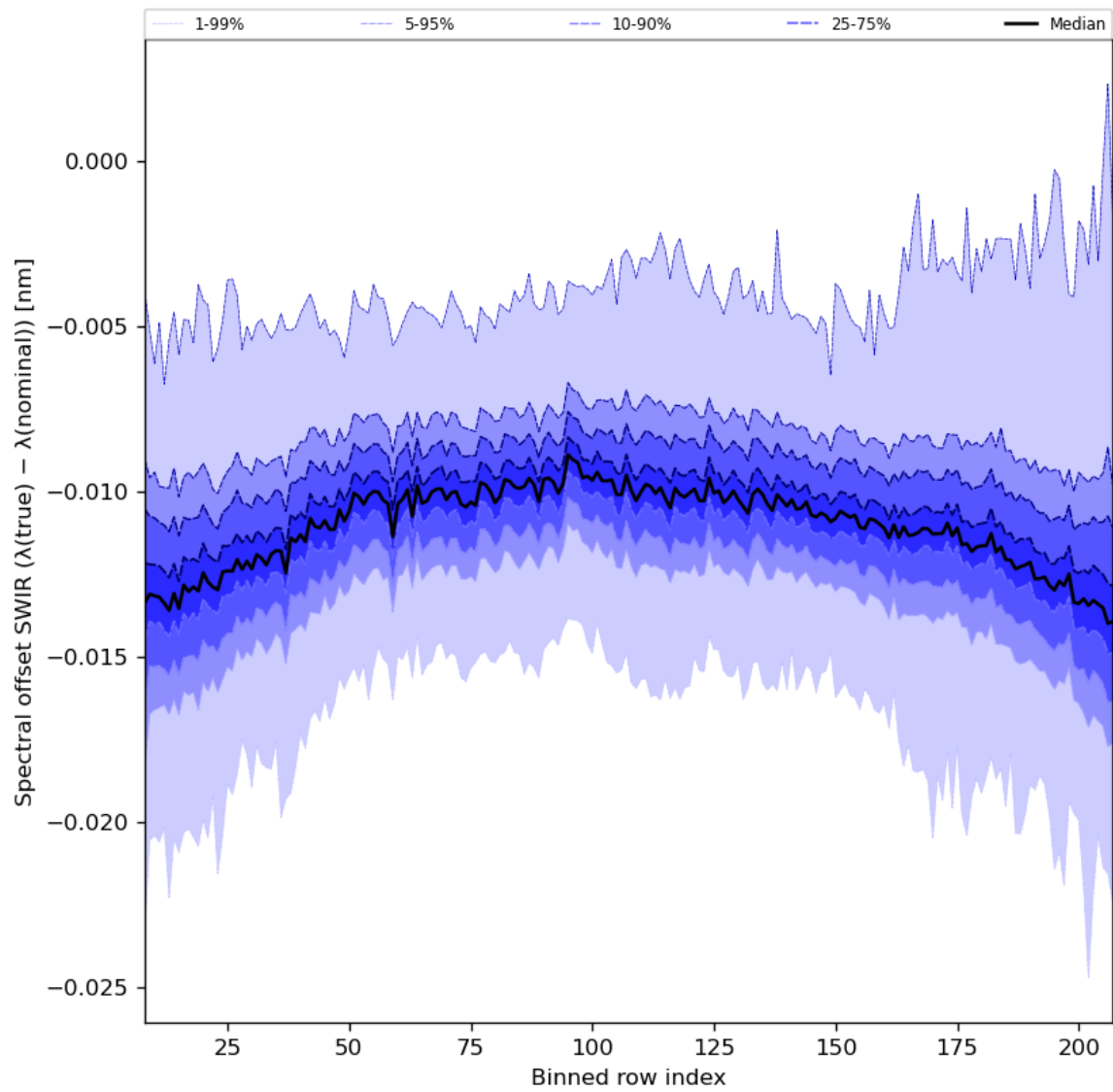
Figure 38: Along track statistics of “Spectral offset SWIR ( \lambda(\text{true}) - \lambda(\text{nominal}) )” for 2024-02-02 to 2024-02-04
