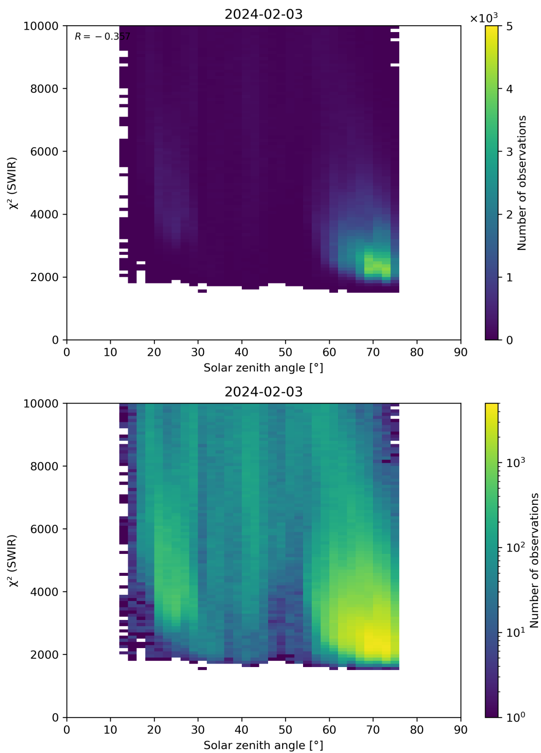
Figure 95: Scatter density plot of “Solar zenith angle” against “ \chi^2 (SWIR)” for 2024-02-02 to 2024-02-04.
