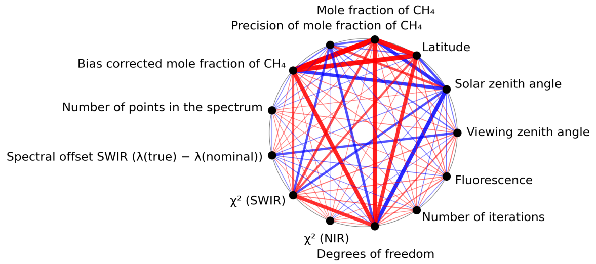
Figure 1: Map of correlation graph for 2024-02-02 to 2024-02-04.
