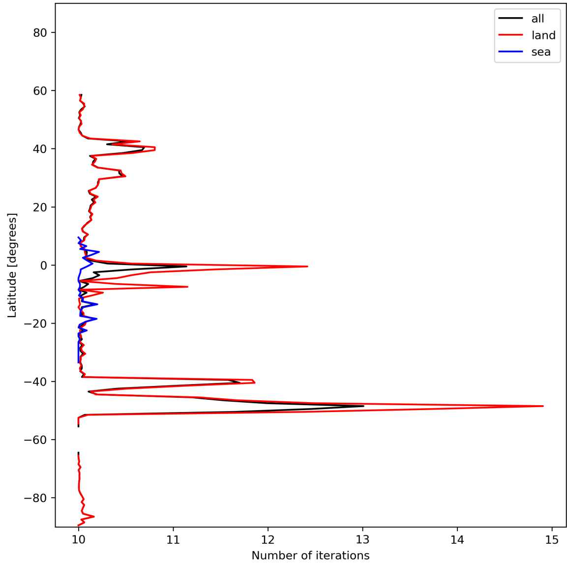
Figure 20: Zonal average of “Number of iterations” for 2024-02-02 to 2024-02-04.
