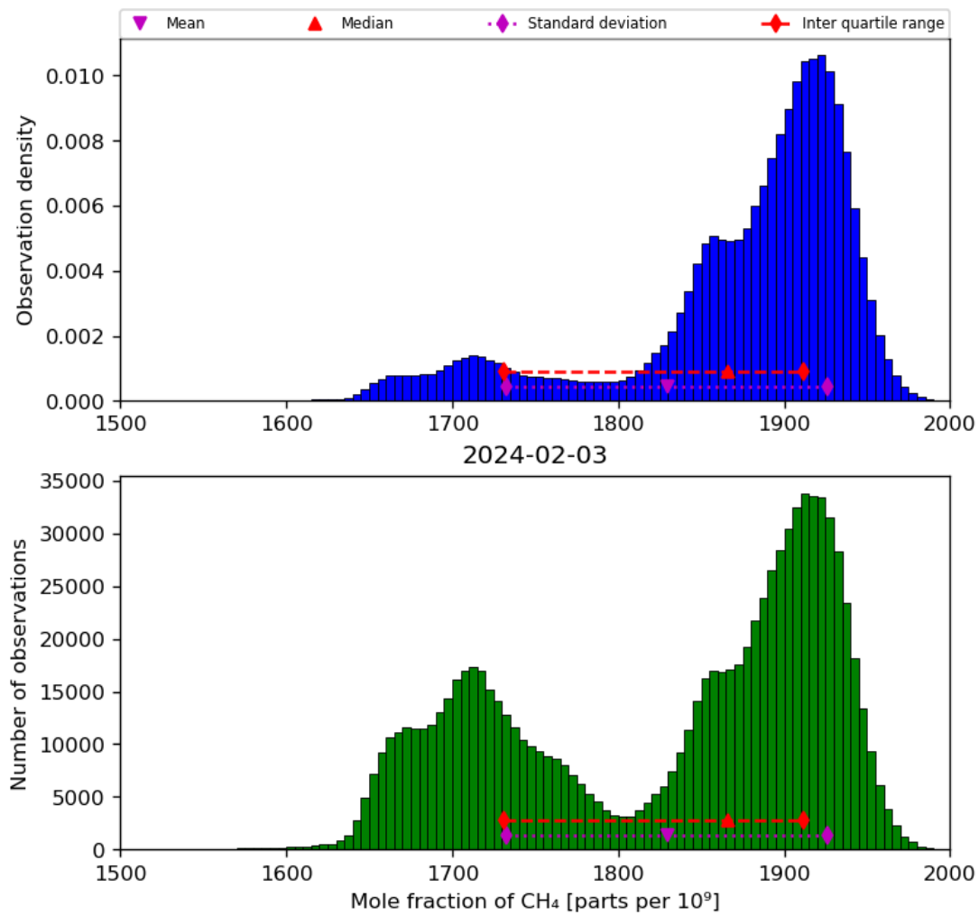
Figure 23: Histogram of “Mole fraction of CH 4 ” for 2024-02-02 to 2024-02-04
