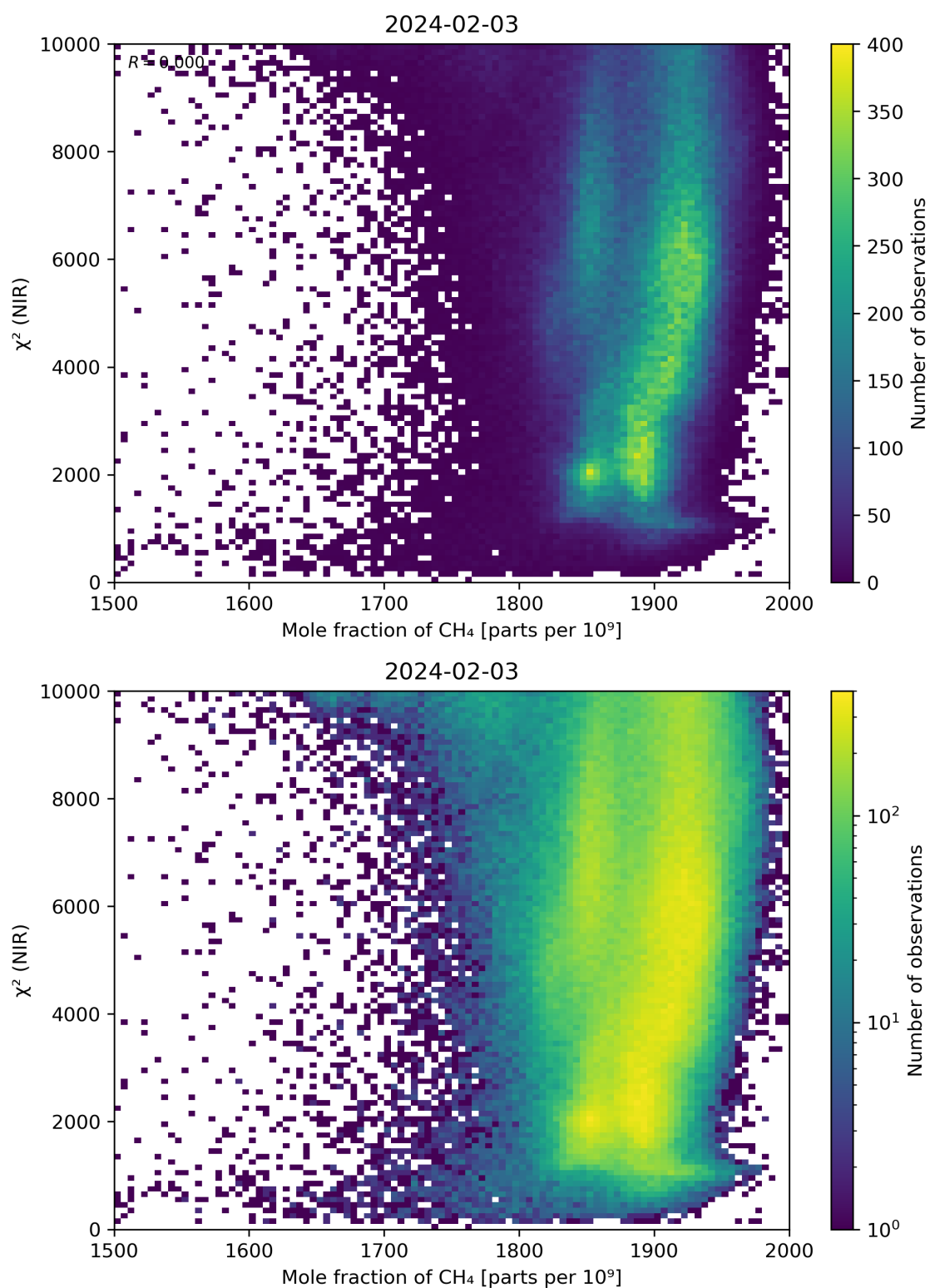
Figure 70: Scatter density plot of “Mole fraction of CH 4 ” against “ \chi^2 (NIR)” for 2024-02-02 to 2024-02-04.
