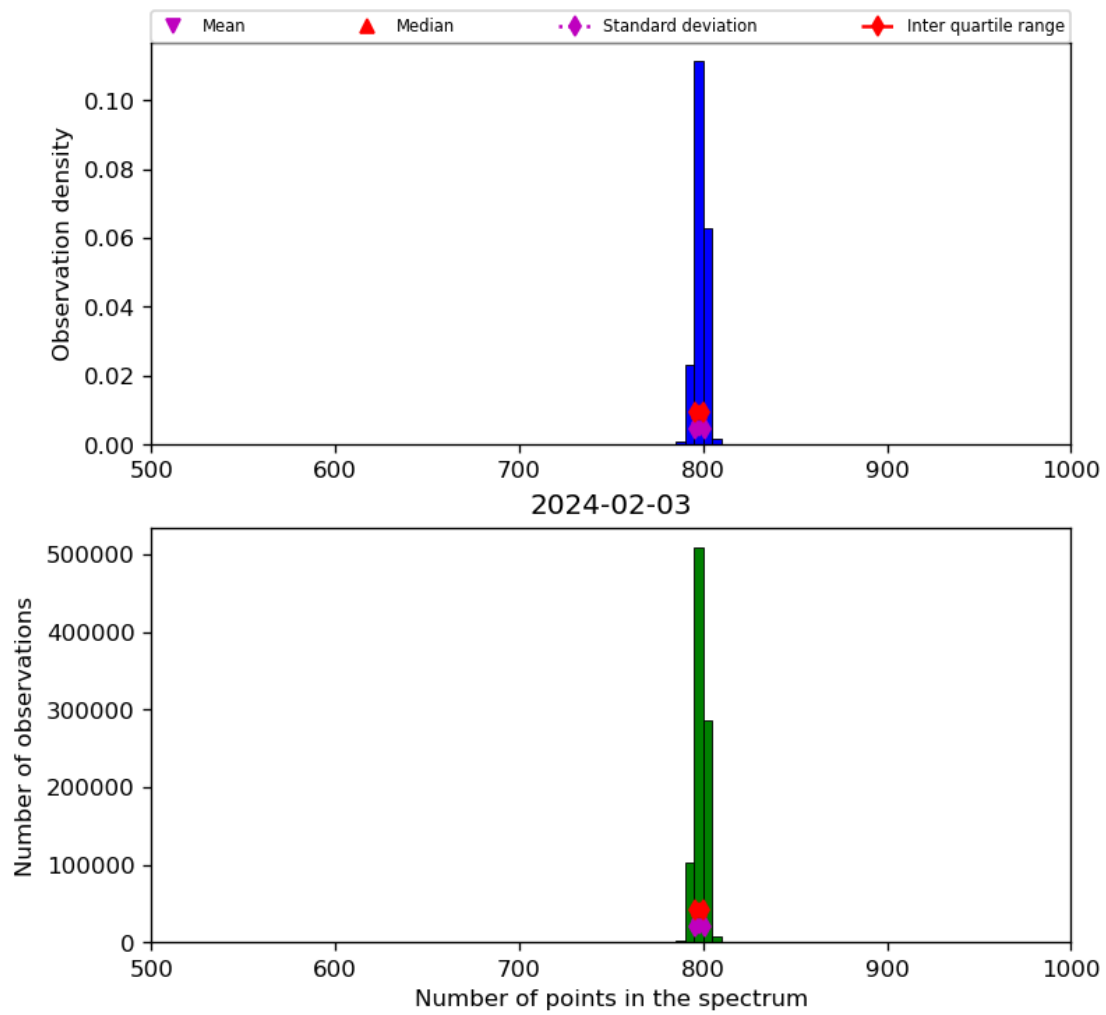
Figure 26: Histogram of “Number of points in the spectrum” for 2024-02-02 to 2024-02-04
