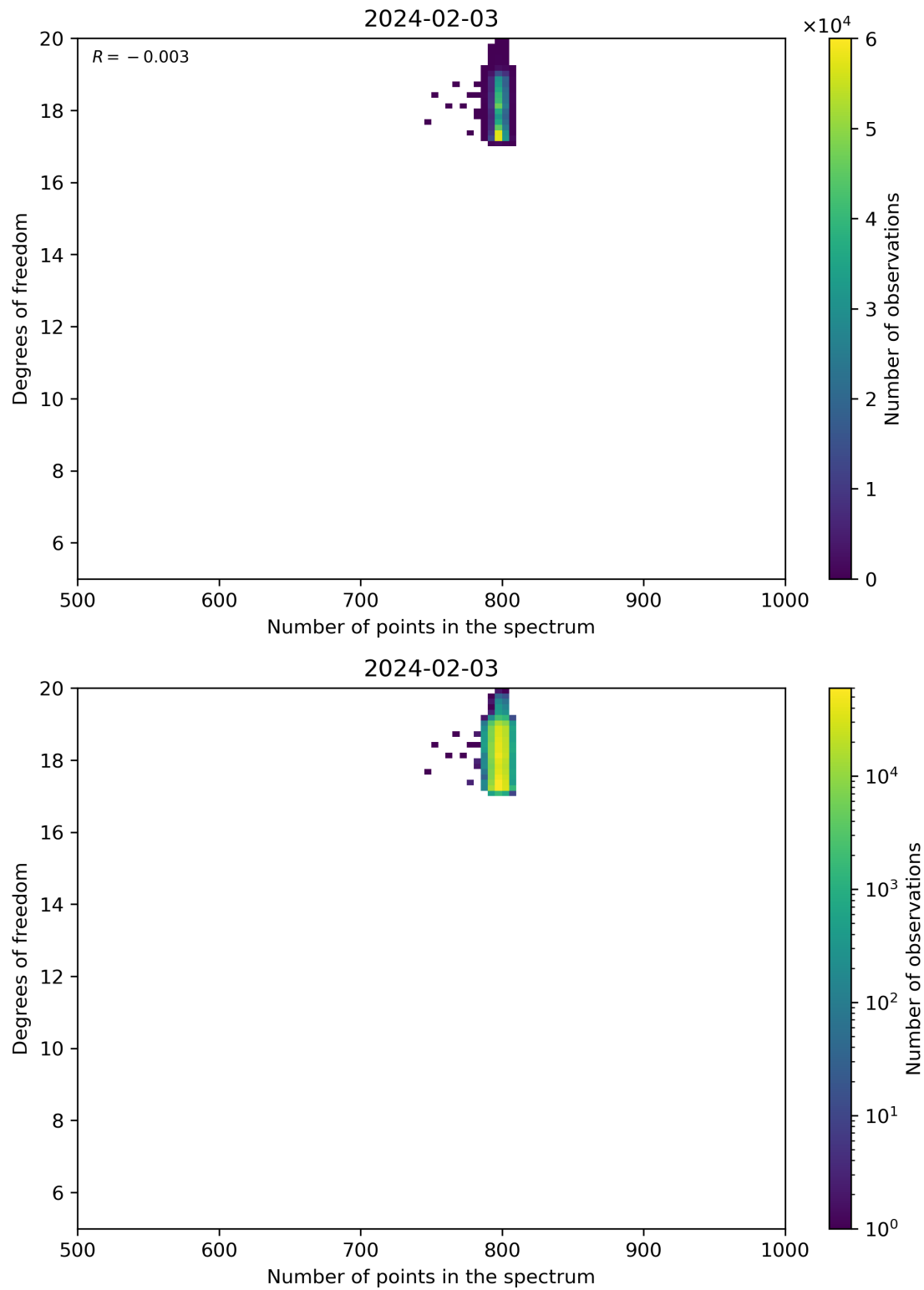
Figure 90: Scatter density plot of “Number of points in the spectrum” against “Degrees of freedom” for 2024-02-02 to 2024-02-04.
