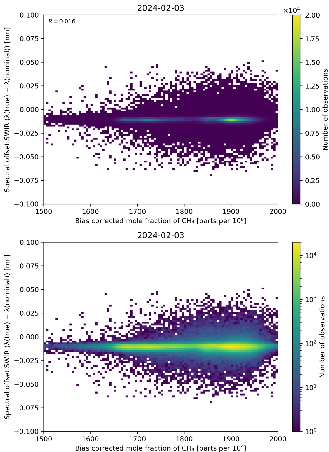
Figure 69: Scatter density plot of “Bias corrected mole fraction of \text{CH}_4 ” against “Spectral offset SWIR ( \lambda(\text{true}) - \lambda(\text{nominal}) )” for 2024-02-02 to 2024-02-04.
