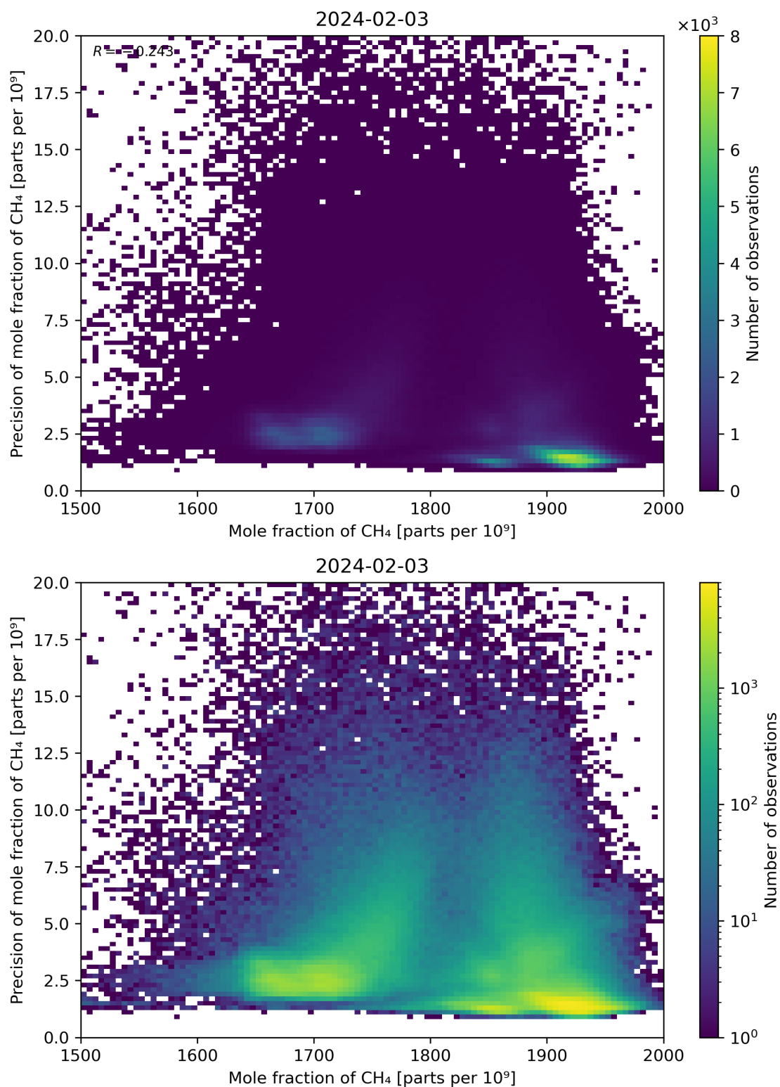
Figure 75: Scatter density plot of “Mole fraction of CH 4 ” against “Precision of mole fraction of CH 4 ” for 2024-02-02 to 2024-02-04.
