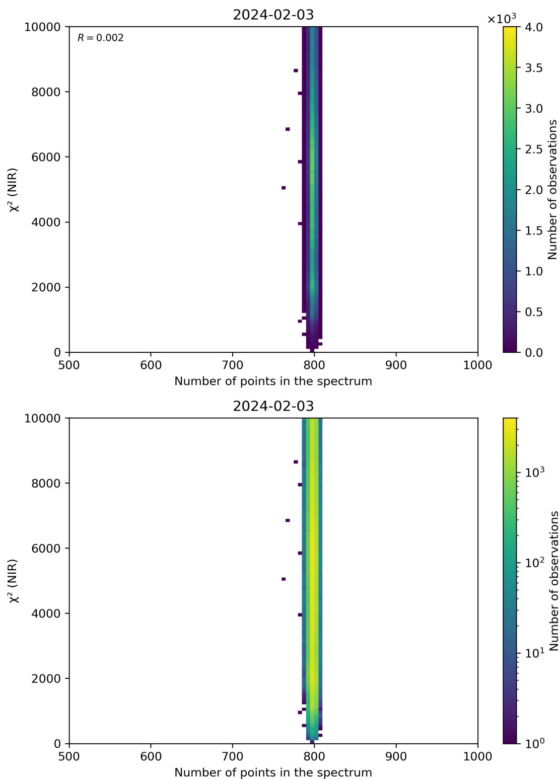
Figure 88: Scatter density plot of “Number of points in the spectrum” against “ \chi^2 (NIR)” for 2024-02-02 to 2024-02-04.
