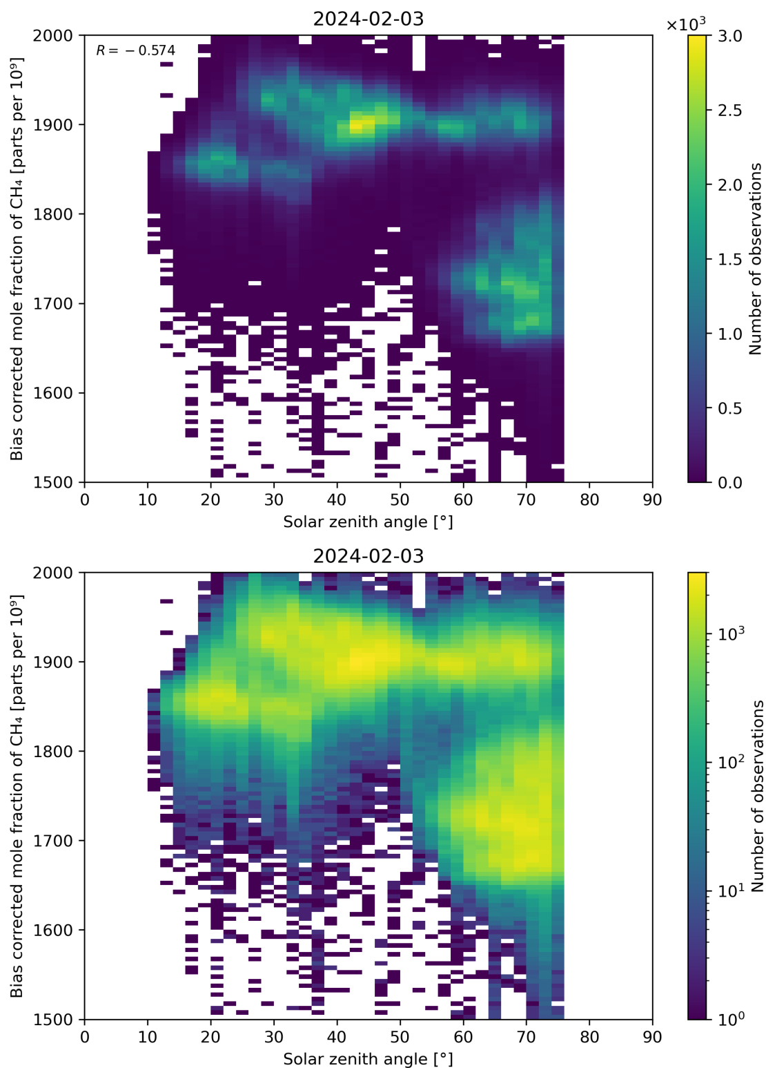
Figure 100: Scatter density plot of “Solar zenith angle” against “Bias corrected mole fraction of \text{CH}_4 ” for 2024-02-02 to 2024-02-04.
