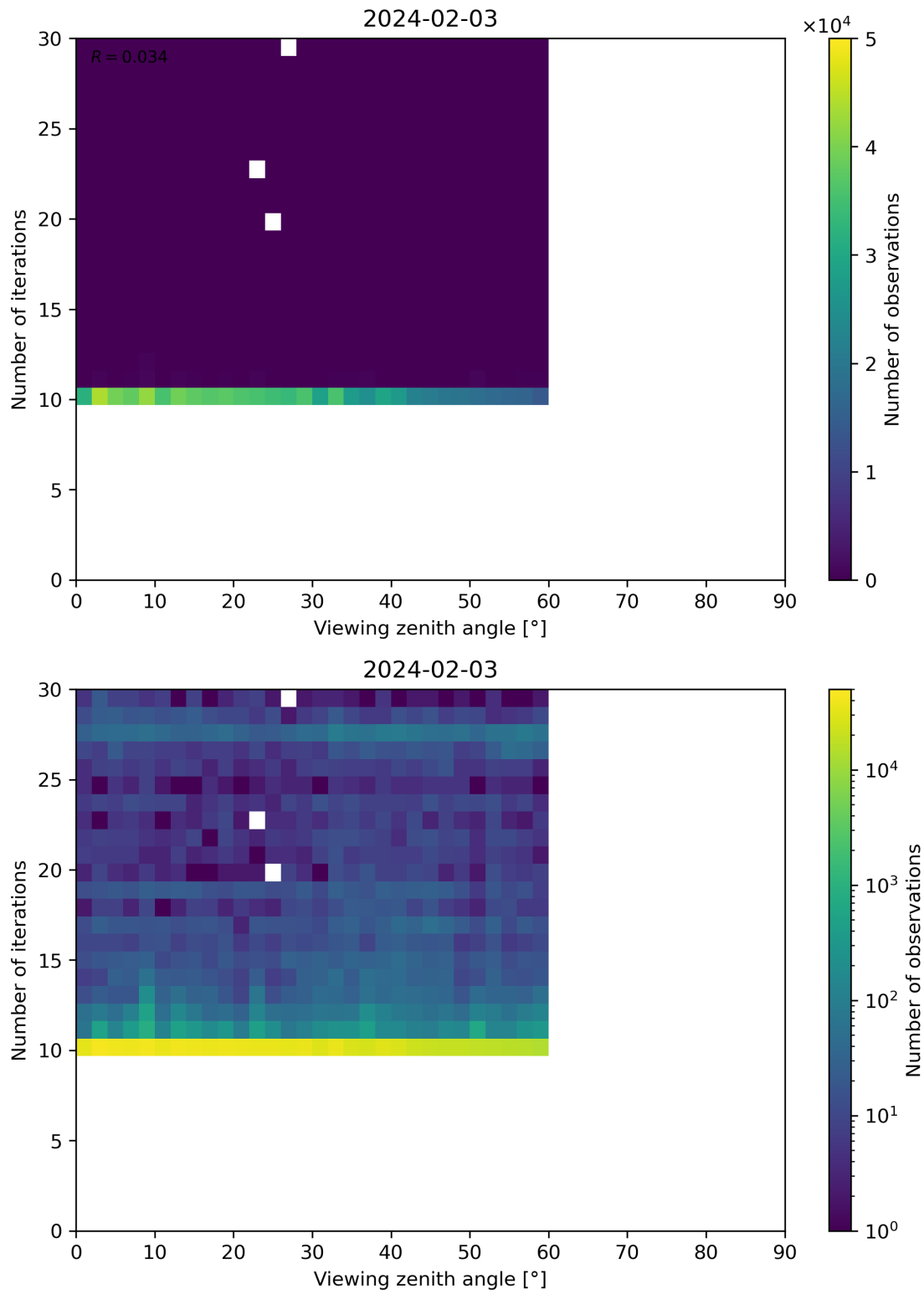
Figure 113: Scatter density plot of “Viewing zenith angle” against “Number of iterations” for 2024-02-02 to 2024-02-04.
