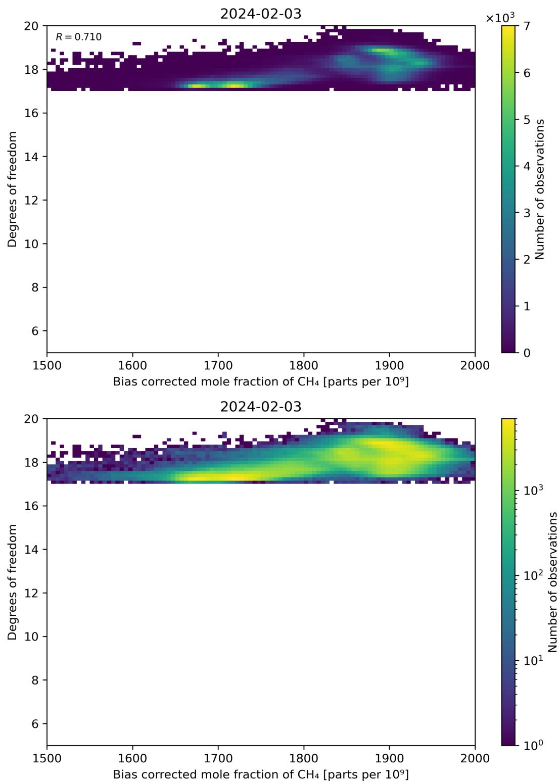
Figure 65: Scatter density plot of “Bias corrected mole fraction of CH 4 ” against “Degrees of freedom” for 2024-02-02 to 2024-02-04.
