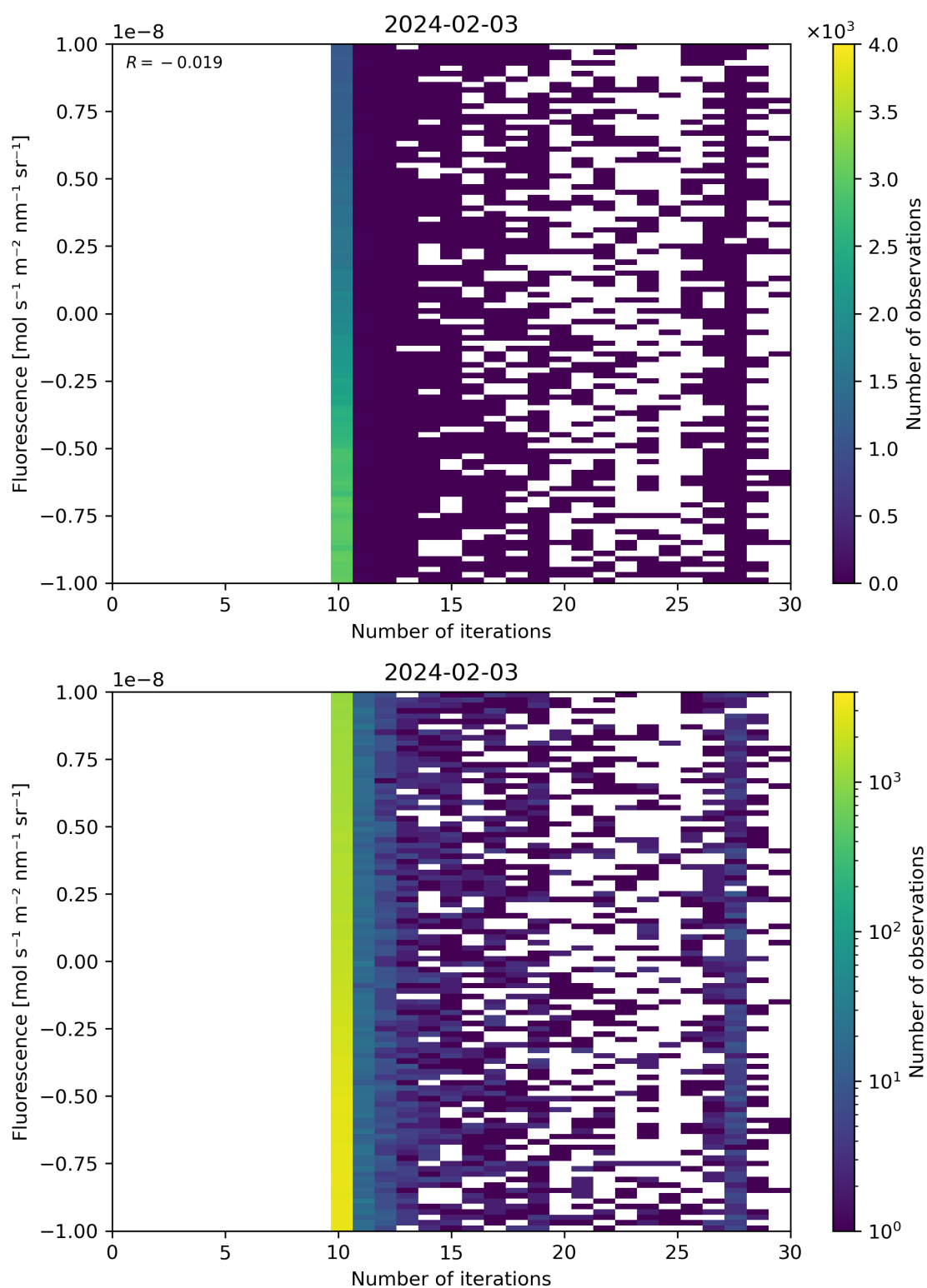
Figure 87: Scatter density plot of “Number of iterations” against “Fluorescence” for 2024-02-02 to 2024-02-04.
