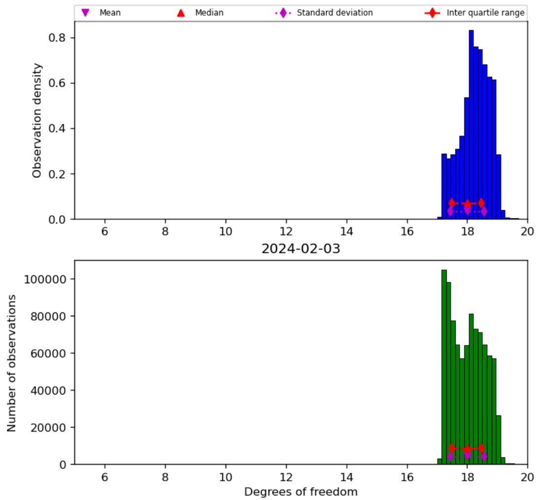
Figure 30: Histogram of “Degrees of freedom” for 2024-02-02 to 2024-02-04
