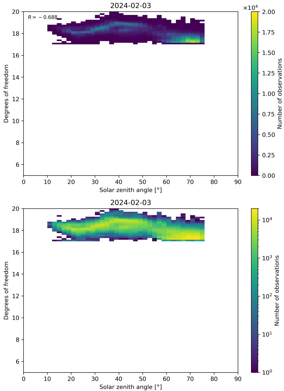
Figure 96: Scatter density plot of “Solar zenith angle” against “Degrees of freedom” for 2024-02-02 to 2024-02-04.
