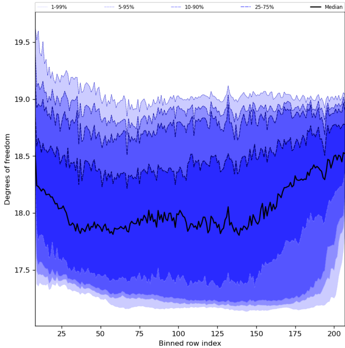
Figure 41: Along track statistics of “Degrees of freedom” for 2024-02-02 to 2024-02-04
