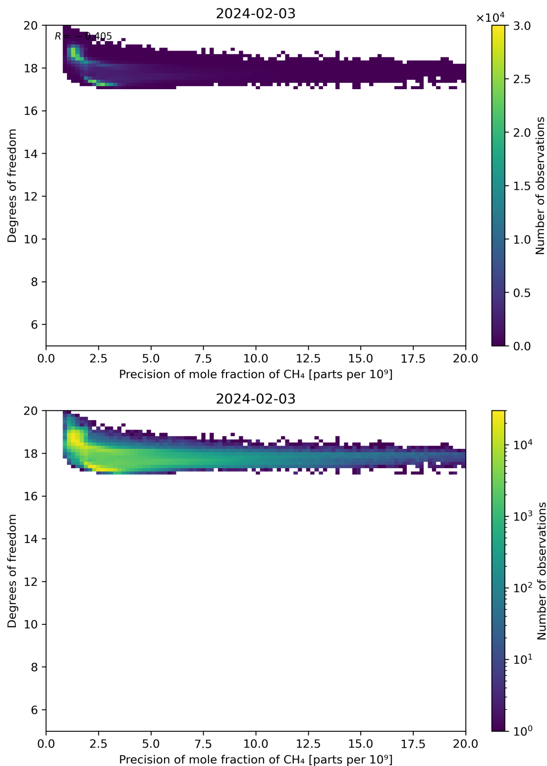
Figure 80: Scatter density plot of “Precision of mole fraction of CH 4 ” against “Degrees of freedom” for 2024-02-02 to 2024-02-04.
