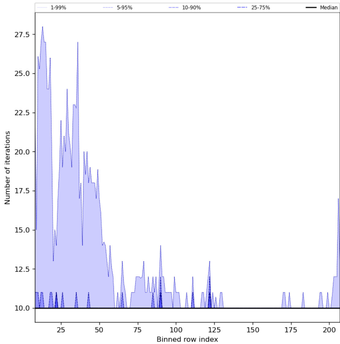
Figure 42: Along track statistics of “Number of iterations” for 2024-02-02 to 2024-02-04
