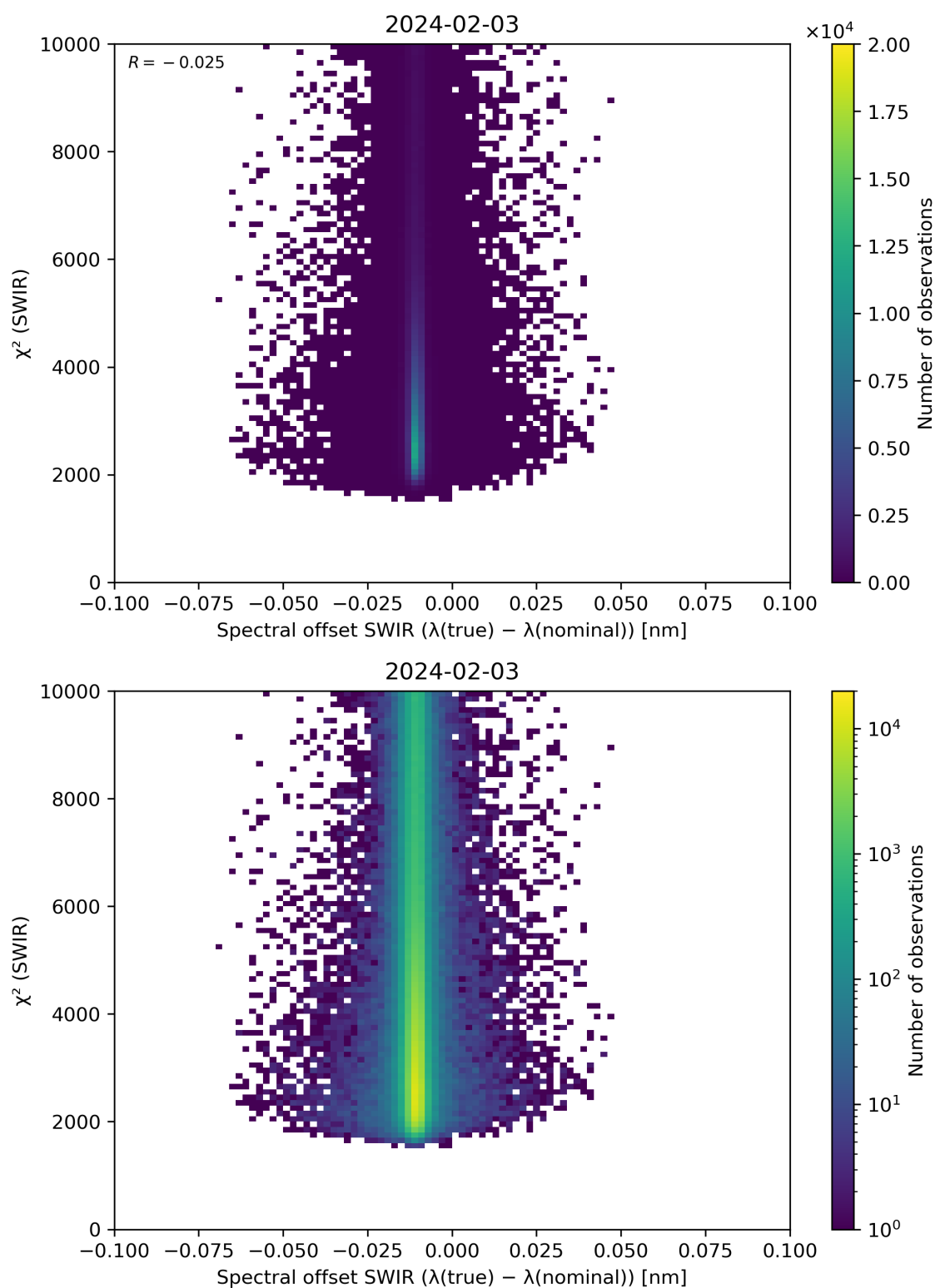
Figure 118: Scatter density plot of “Spectral offset SWIR ( \lambda(\text{true}) - \lambda(\text{nominal}) )” against “ \chi^2 (SWIR)” for 2024-02-02 to 2024-02-04.
