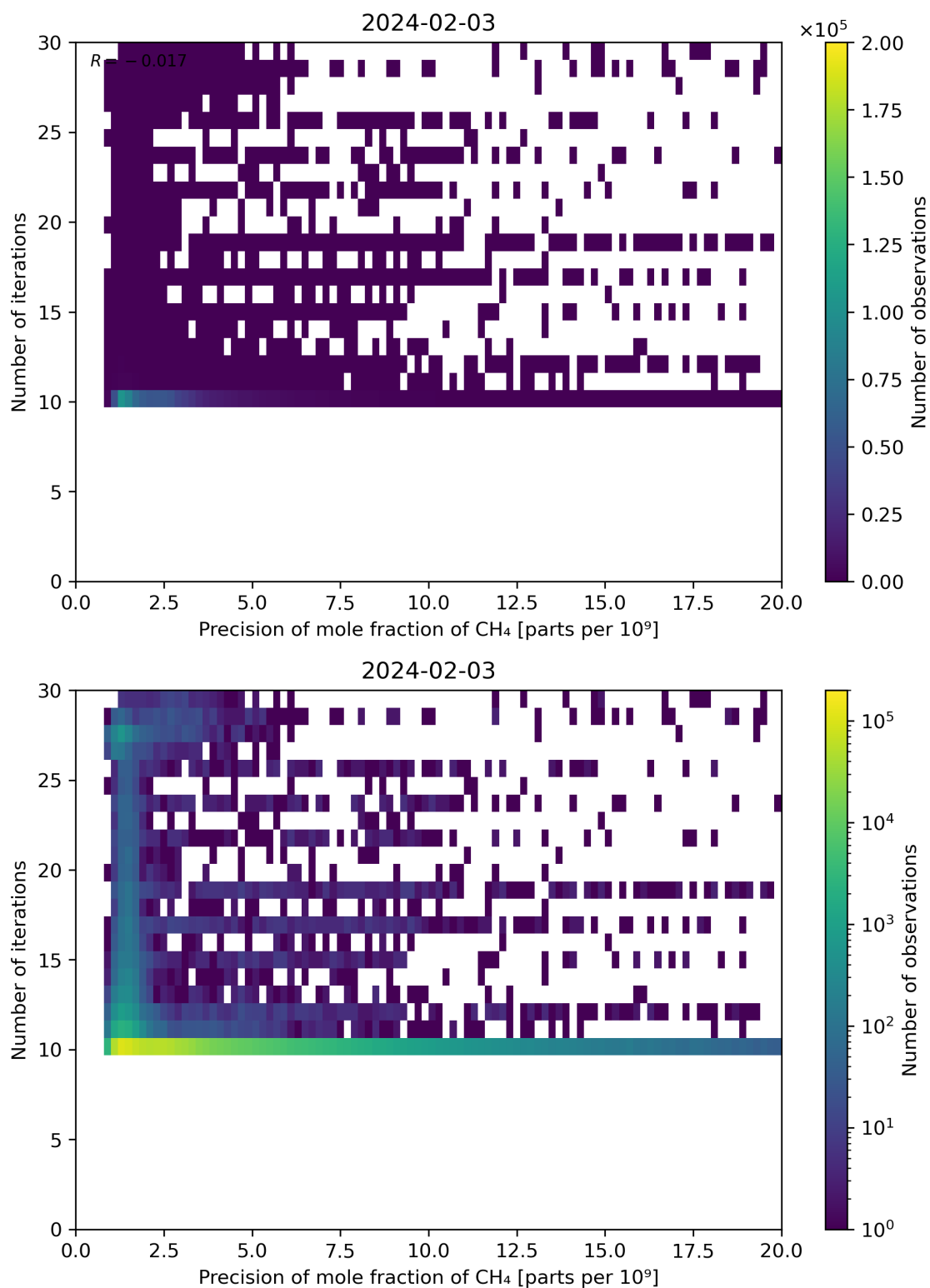
Figure 83: Scatter density plot of “Precision of mole fraction of CH 4 ” against “Number of iterations” for 2024-02-02 to 2024-02-04.
