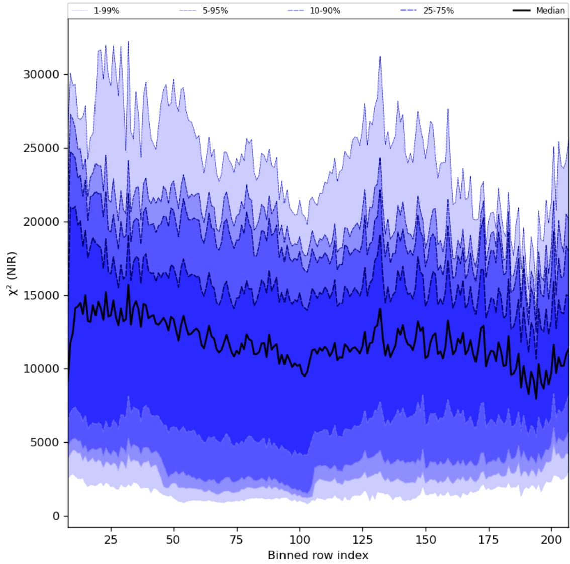
Figure 40: Along track statistics of “ \chi^2 (NIR)” for 2024-02-02 to 2024-02-04
