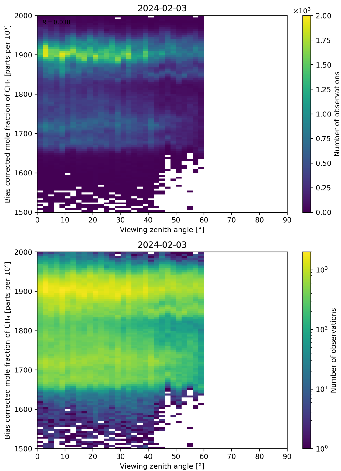
Figure 111: Scatter density plot of “Viewing zenith angle” against “Bias corrected mole fraction of CH 4 ” for 2024-02-02 to 2024-02-04.
