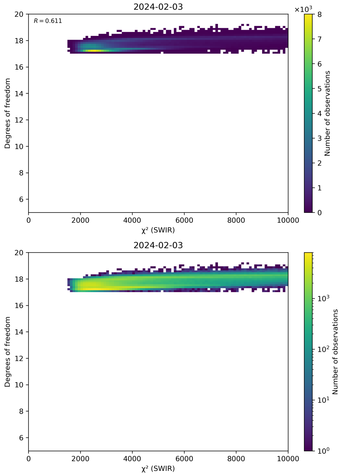
Figure 48: Scatter density plot of “ \chi^2 (SWIR)” against “Degrees of freedom” for 2024-02-02 to 2024-02-04.
