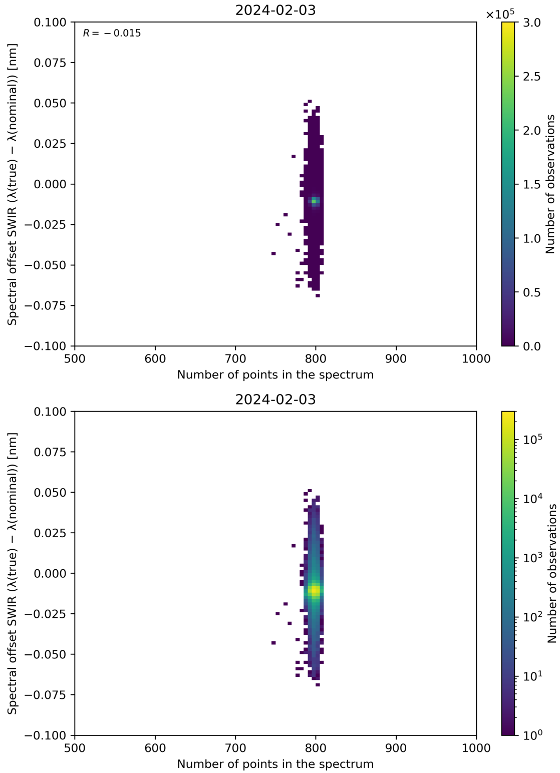
Figure 93: Scatter density plot of “Number of points in the spectrum” against “Spectral offset SWIR ( \lambda(\text{true}) - \lambda(\text{nominal}) )” for 2024-02-02 to 2024-02-04.
