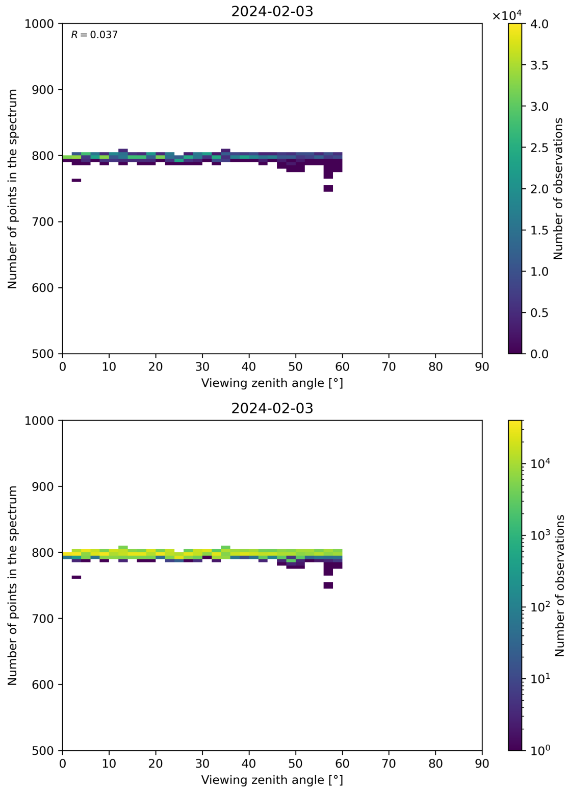
Figure 114: Scatter density plot of “Viewing zenith angle” against “Number of points in the spectrum” for 2024-02-02 to 2024-02-04.
