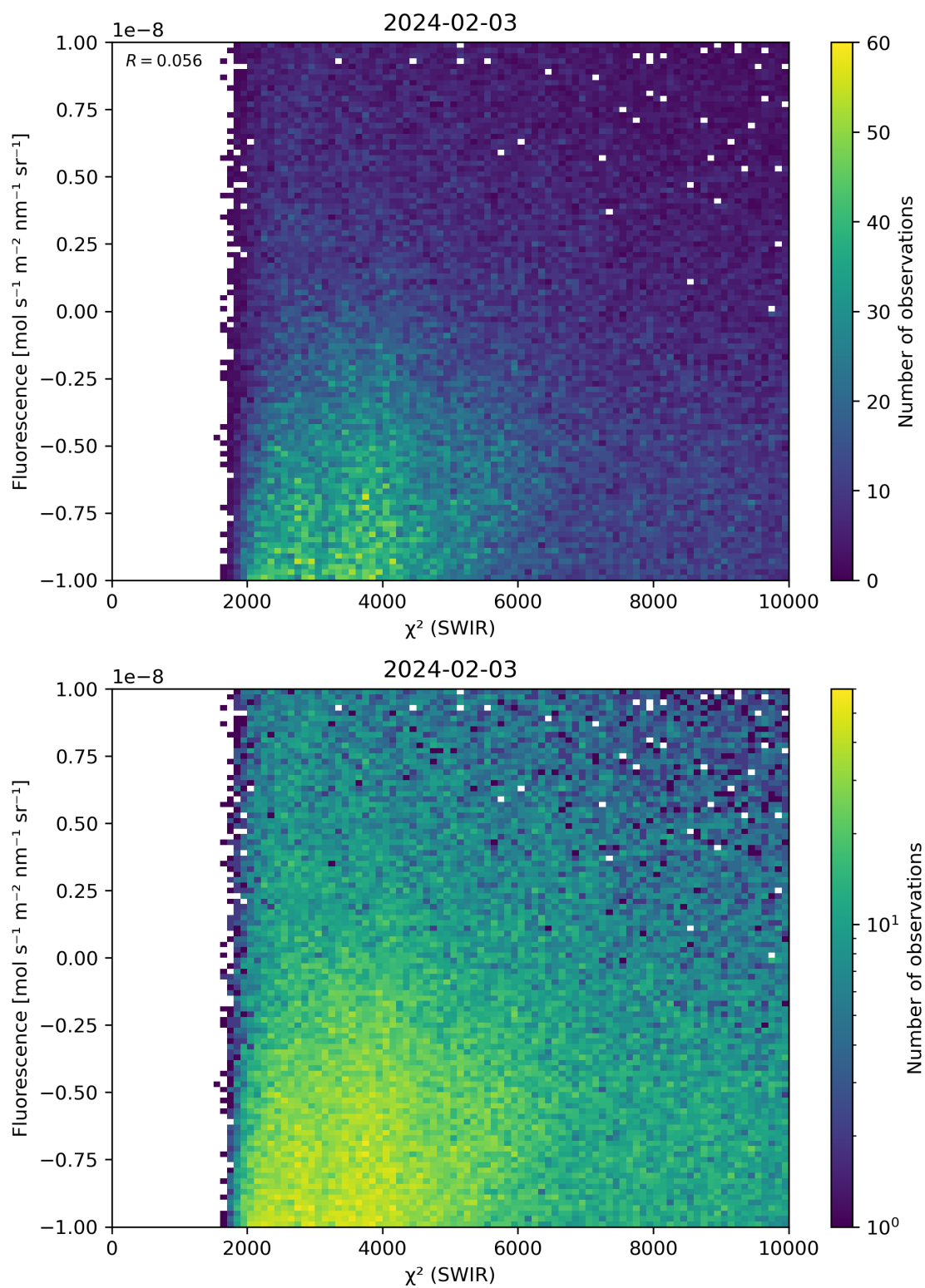
Figure 49: Scatter density plot of “ \chi^2 (SWIR)” against “Fluorescence” for 2024-02-02 to 2024-02-04.
