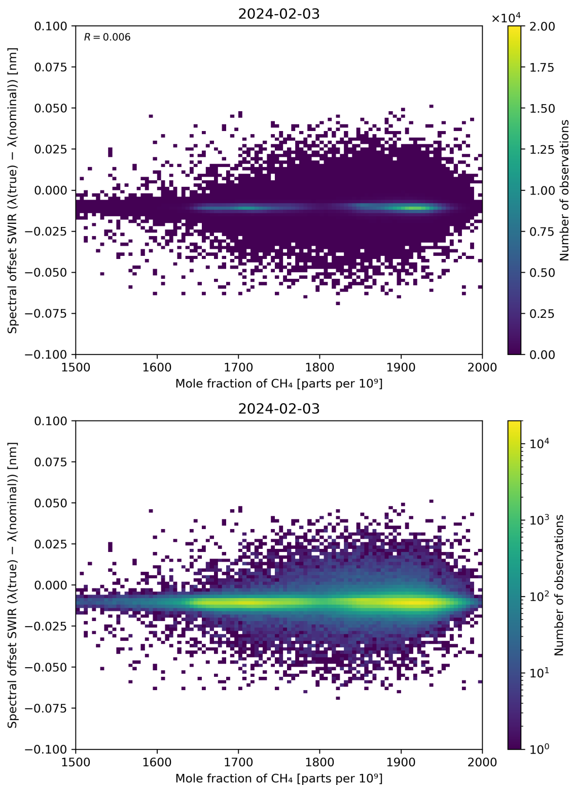
Figure 86: Scatter density plot of “Mole fraction of CH 4 ” against “Spectral offset SWIR ( \lambda(\text{true}) - \lambda(\text{nominal}) )” for 2024-02-02 to 2024-02-04.
