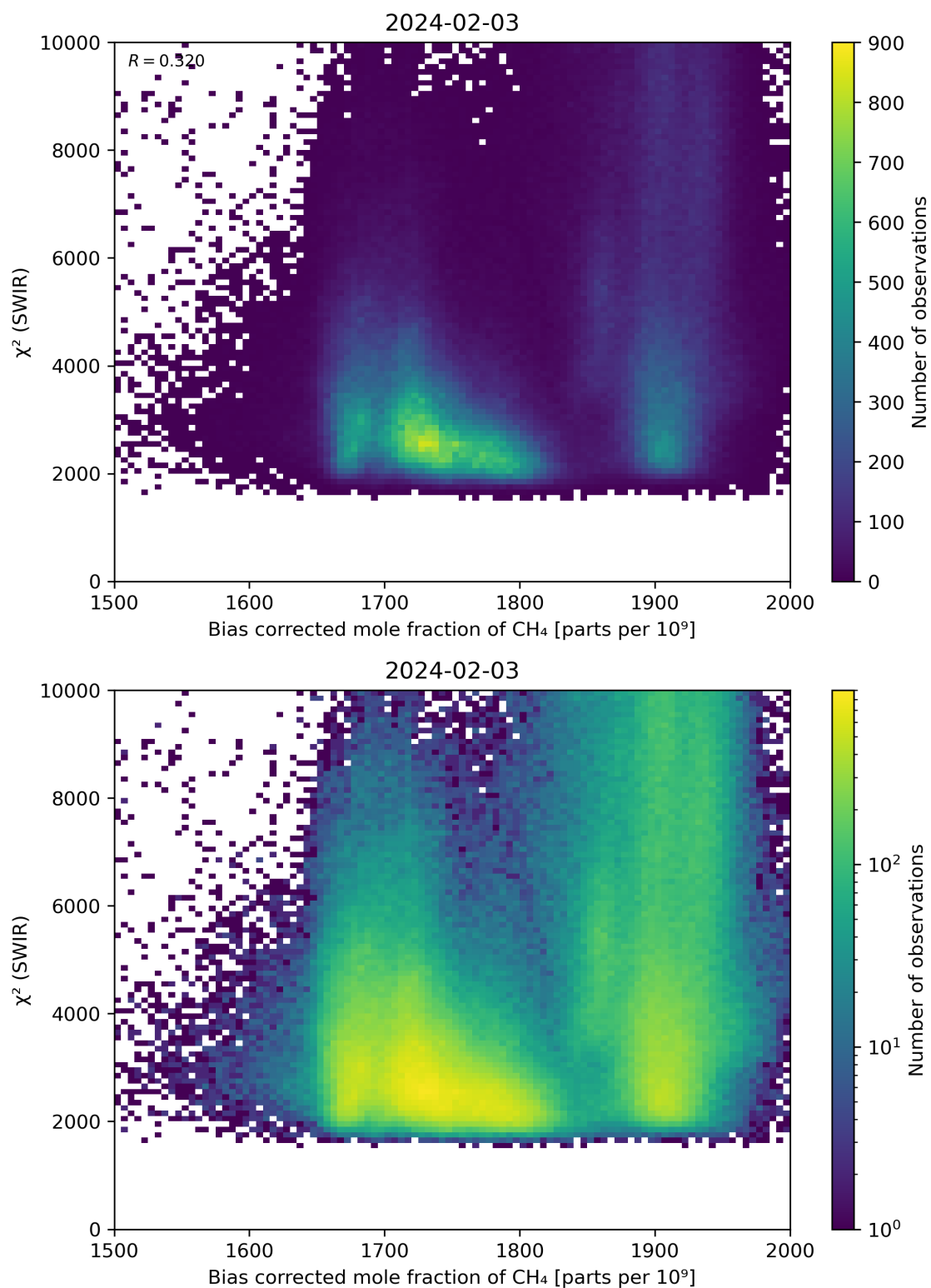
Figure 64: Scatter density plot of “Bias corrected mole fraction of CH 4 ” against “ \chi^2 (SWIR)” for 2024-02-02 to 2024-02-04.
