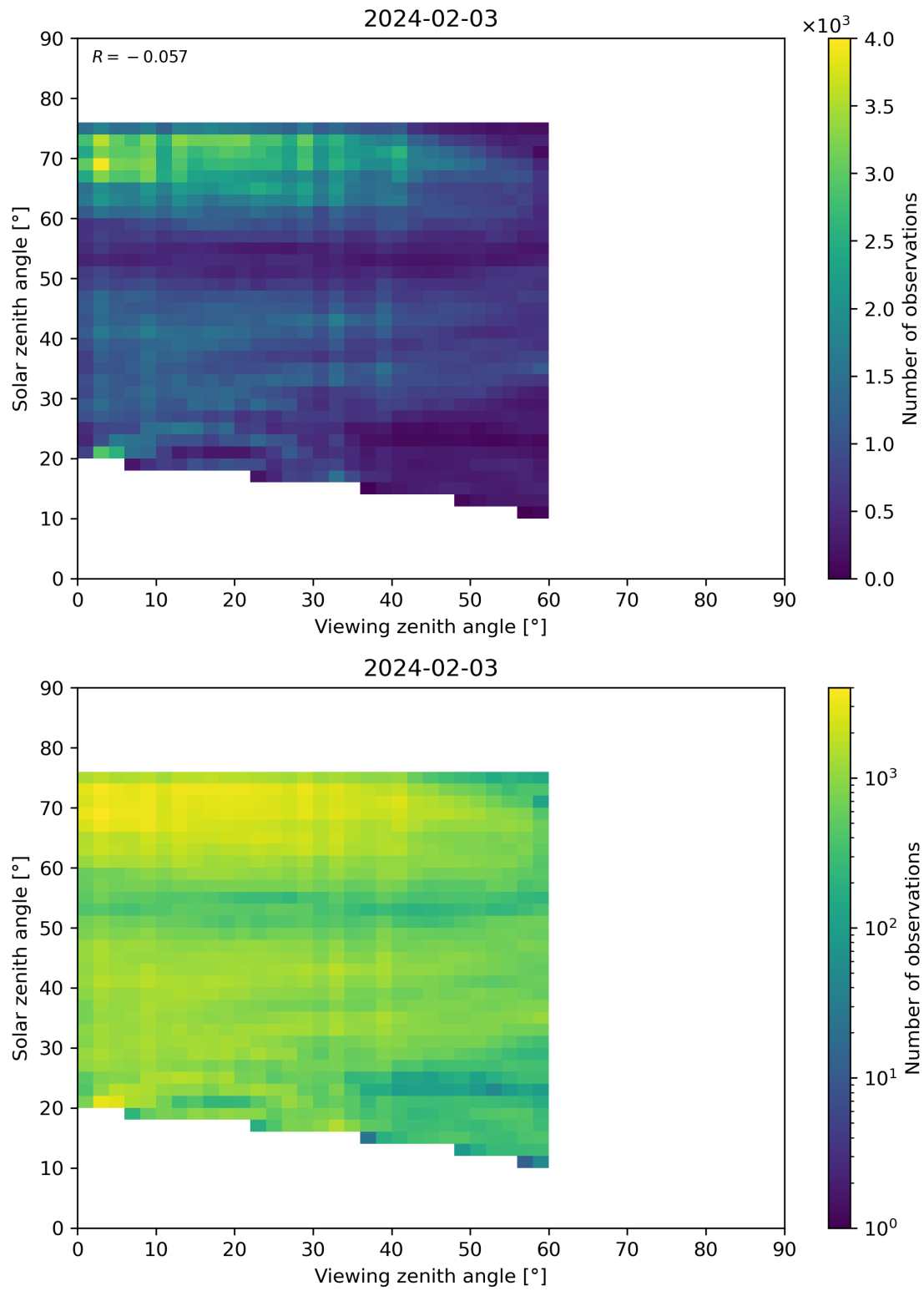
Figure 115: Scatter density plot of “Viewing zenith angle” against “Solar zenith angle” for 2024-02-02 to 2024-02-04.
