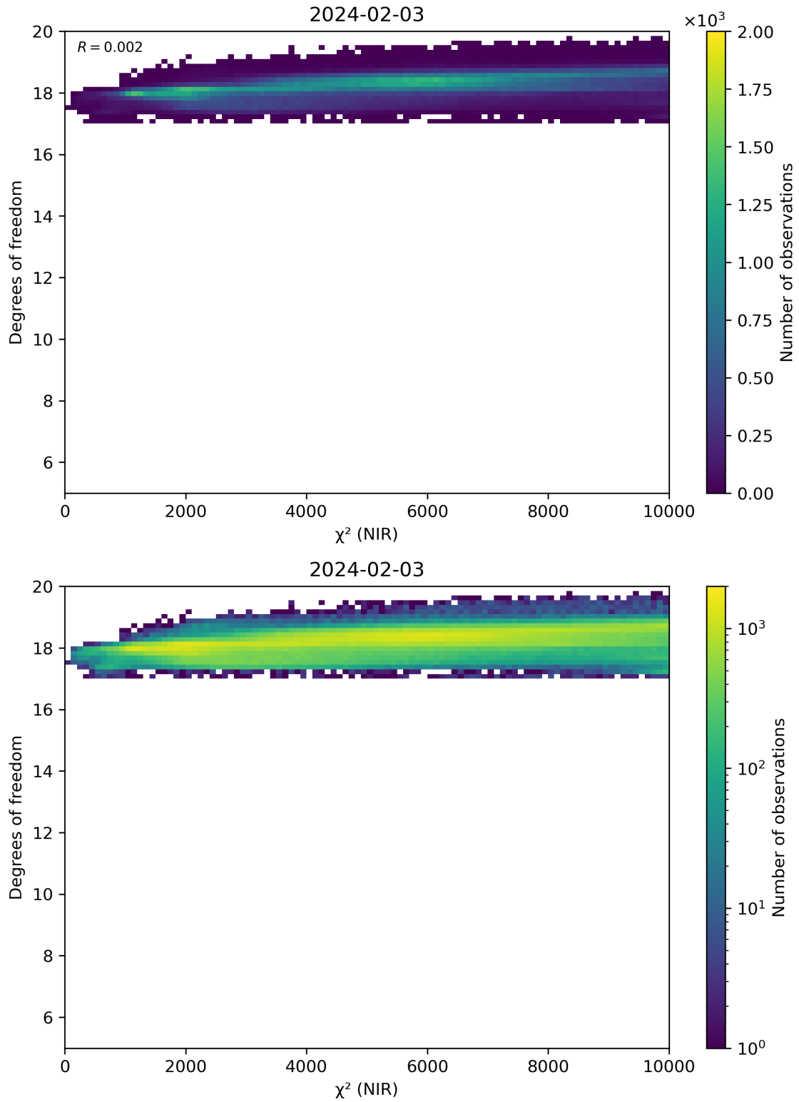
Figure 44: Scatter density plot of “ \chi^2 (NIR)” against “Degrees of freedom” for 2024-02-02 to 2024-02-04.
