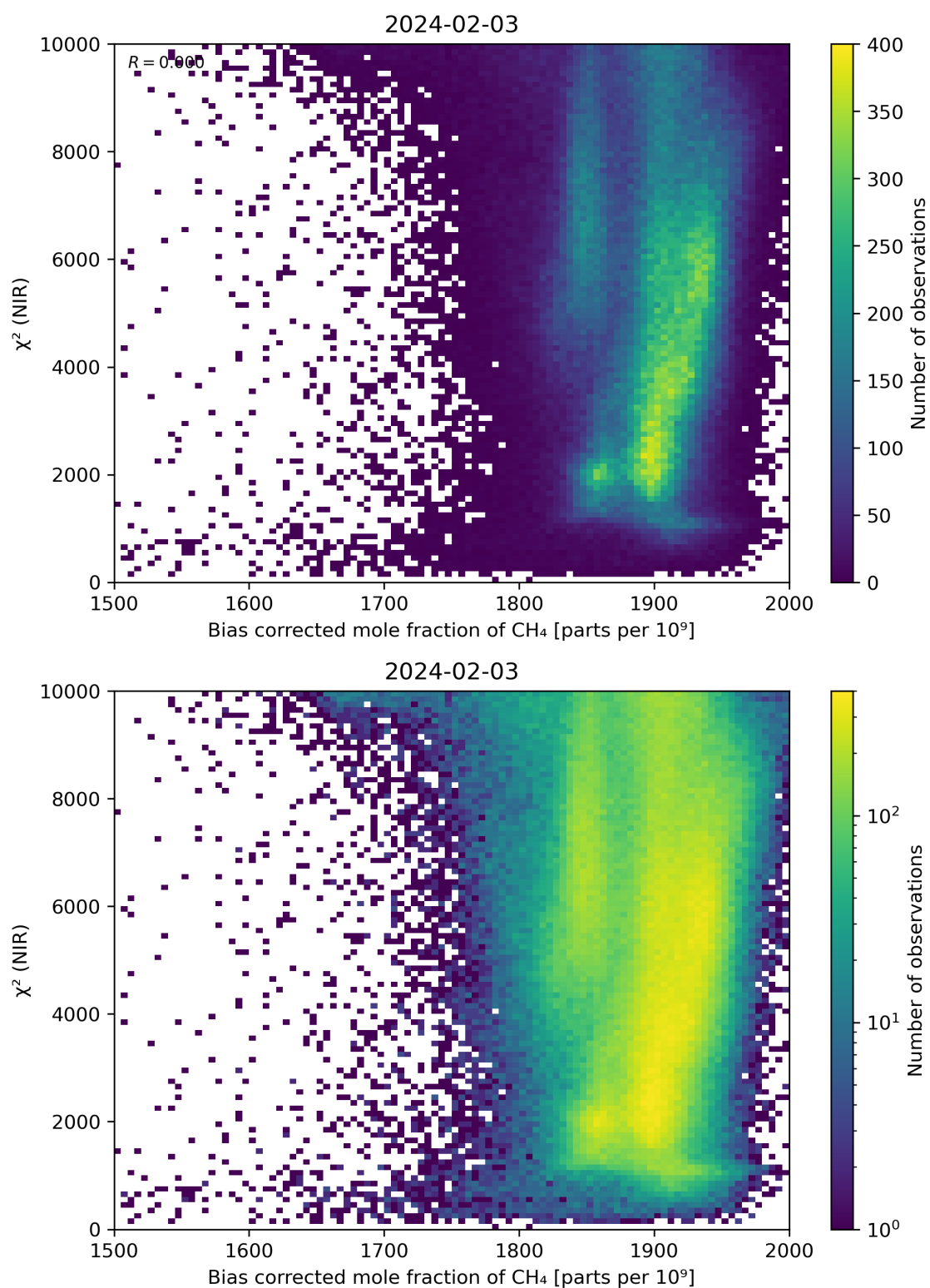
Figure 63: Scatter density plot of “Bias corrected mole fraction of CH 4 ” against “ \chi^2 (NIR)” for 2024-02-02 to 2024-02-04.
