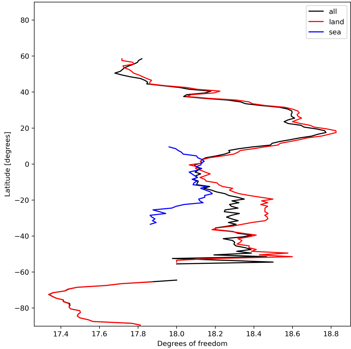
Figure 19: Zonal average of “Degrees of freedom” for 2024-02-02 to 2024-02-04.
