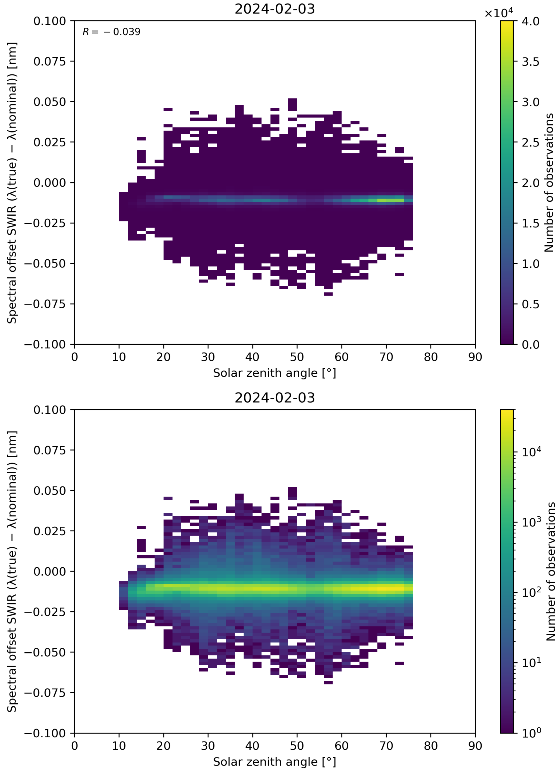
Figure 104: Scatter density plot of “Solar zenith angle” against “Spectral offset SWIR ( \lambda(\text{true}) - \lambda(\text{nominal}) )” for 2024-02-02 to 2024-02-04.
