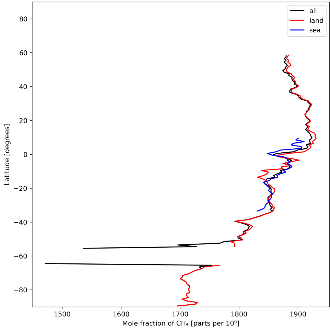
Figure 12: Zonal average of “Mole fraction of \text{CH}_4 ” for 2024-02-02 to 2024-02-04.
