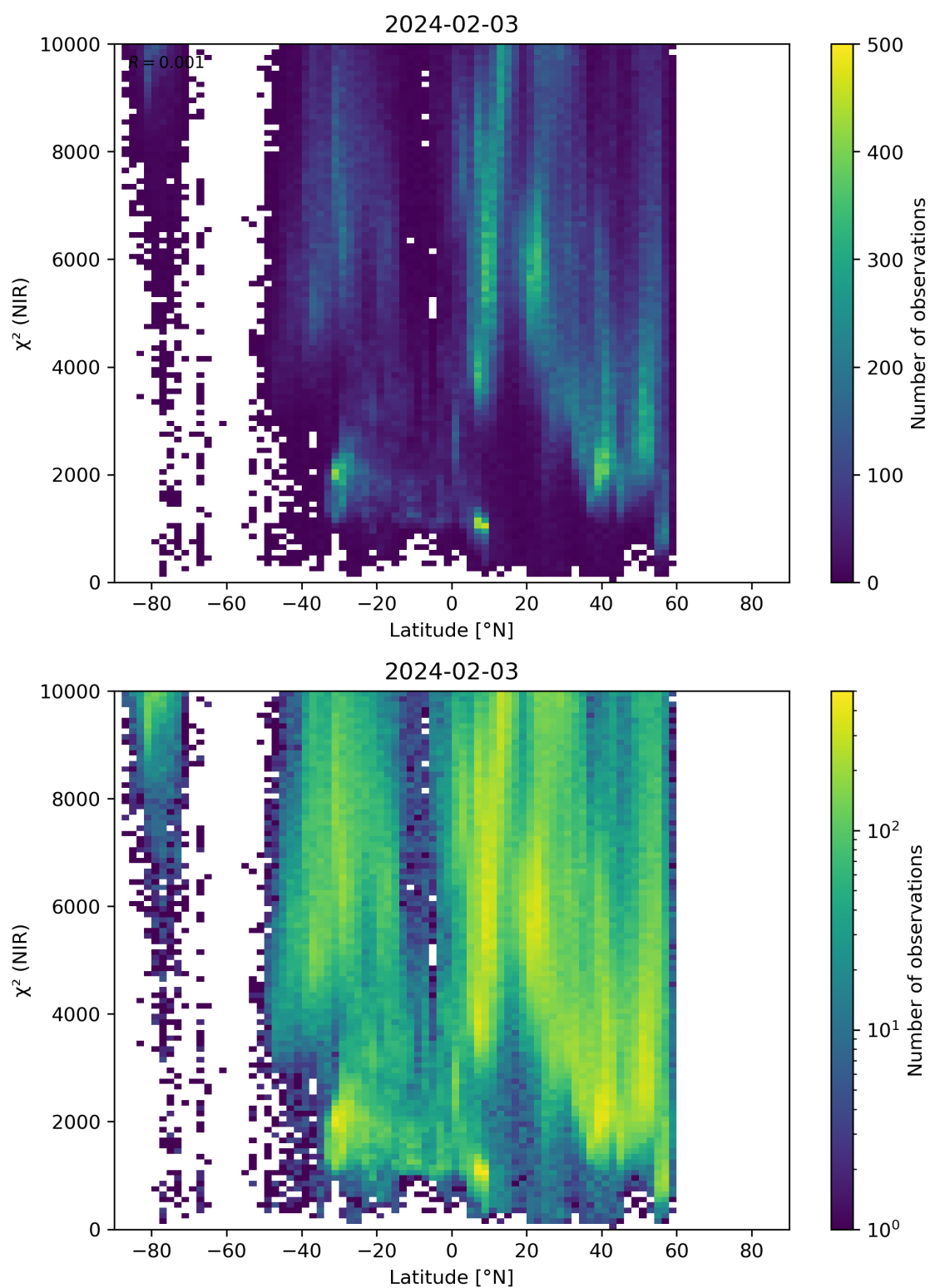
Figure 53: Scatter density plot of “Latitude” against “ \chi^2 (NIR)” for 2024-02-02 to 2024-02-04.
