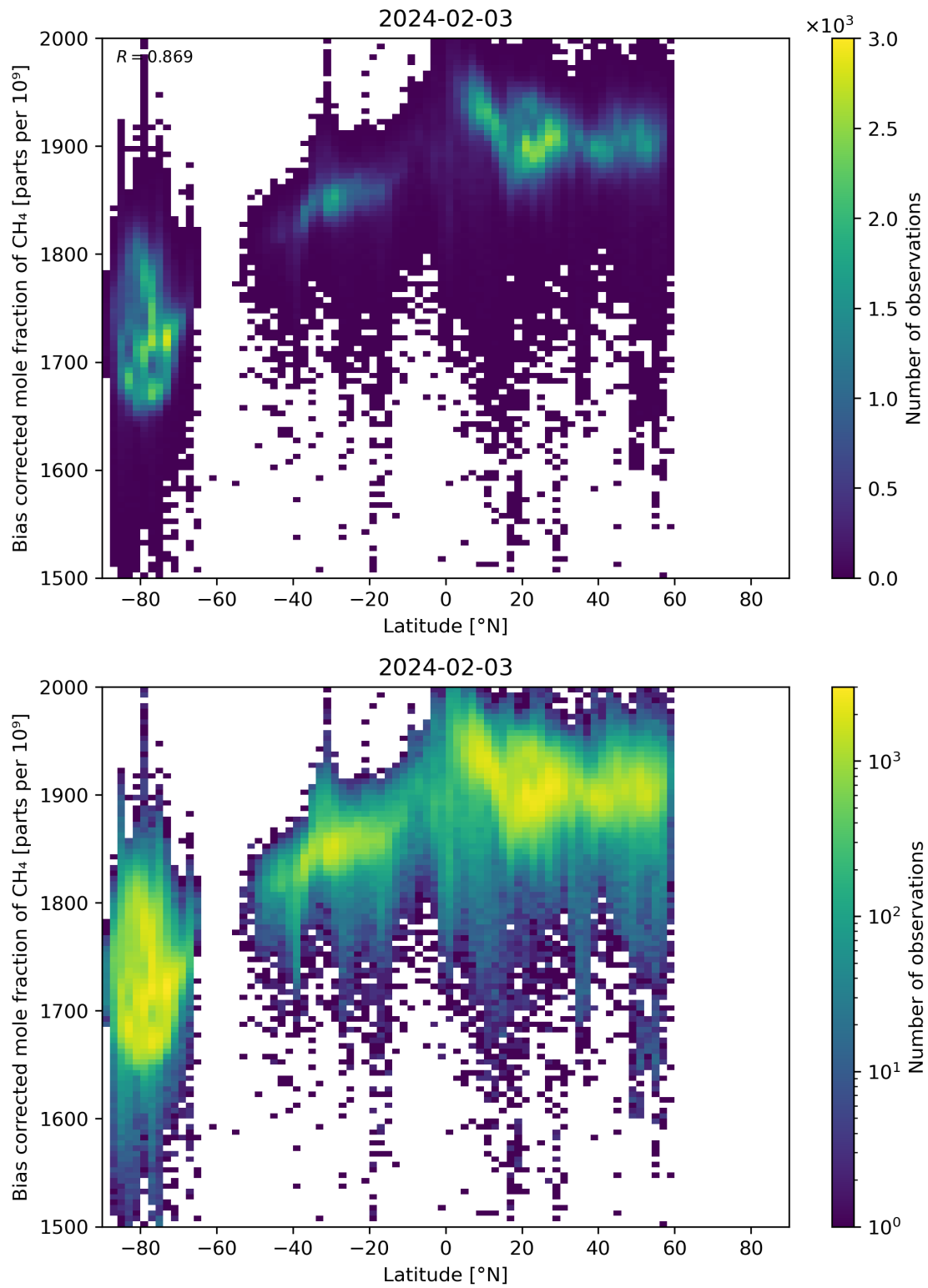
Figure 58: Scatter density plot of “Latitude” against “Bias corrected mole fraction of CH 4 ” for 2024-02-02 to 2024-02-04.
