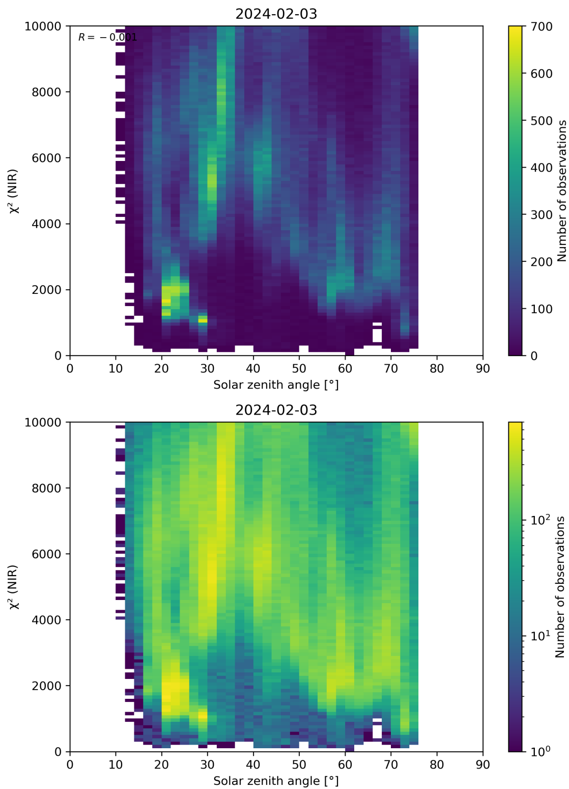
Figure 94: Scatter density plot of “Solar zenith angle” against “ \chi^2 (NIR)” for 2024-02-02 to 2024-02-04.
