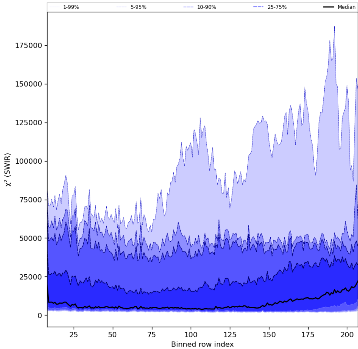
Figure 39: Along track statistics of " \chi^2 (SWIR)" for 2024-02-02 to 2024-02-04
