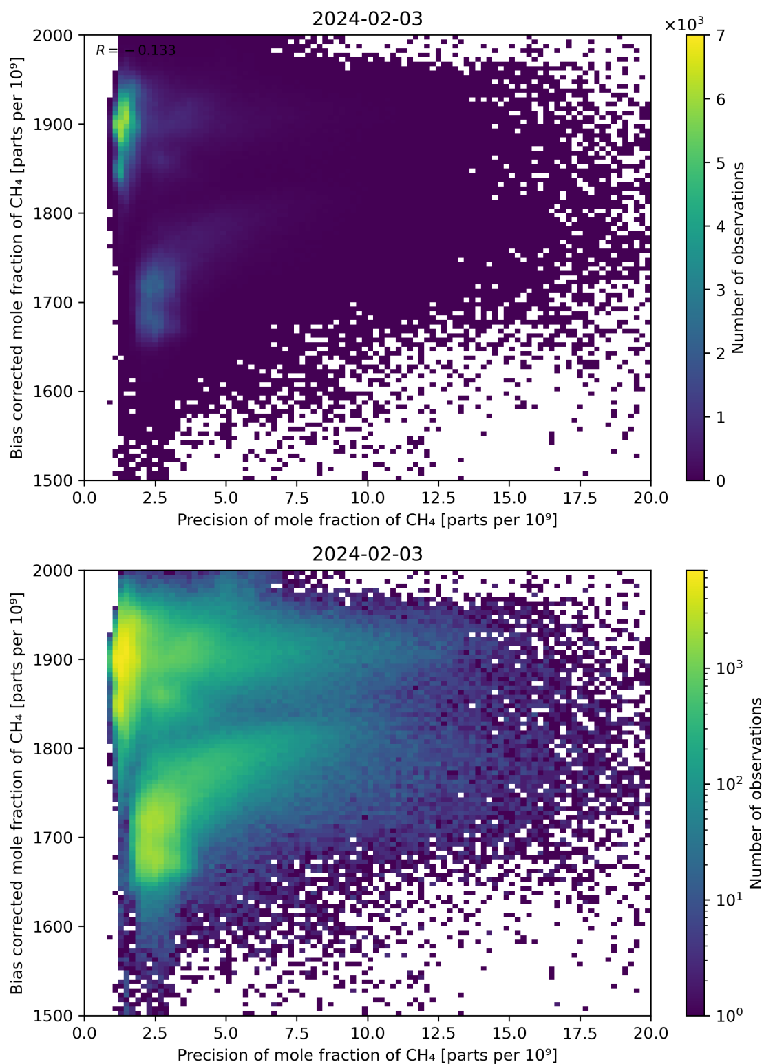
Figure 82: Scatter density plot of “Precision of mole fraction of CH 4 ” against “Bias corrected mole fraction of CH 4 ” for 2024-02-02 to 2024-02-04.
