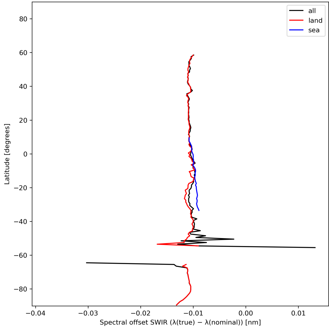
Figure 16: Zonal average of “Spectral offset SWIR ( \lambda(\text{true}) - \lambda(\text{nominal}) )” for 2024-02-02 to 2024-02-04.
