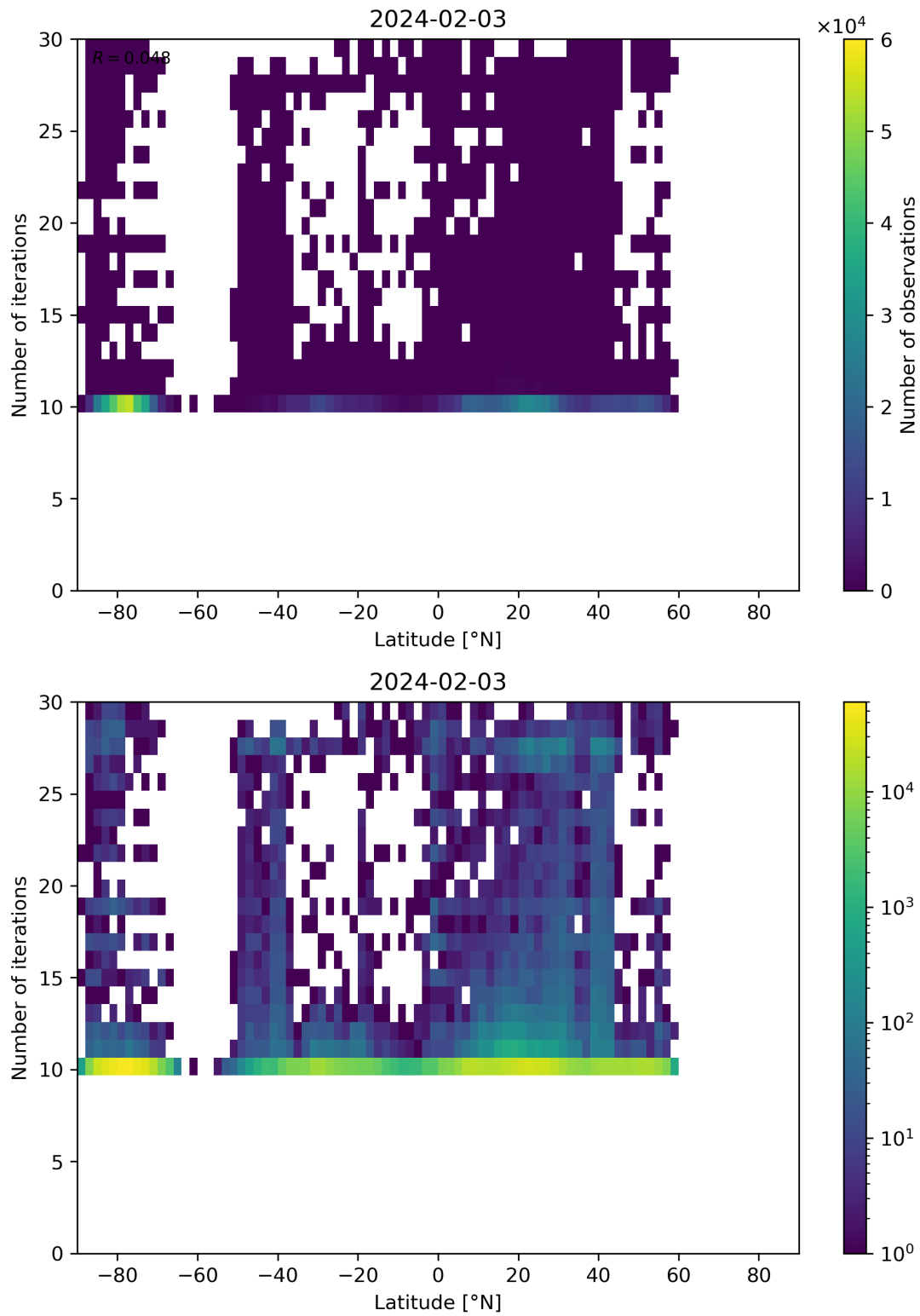
Figure 60: Scatter density plot of “Latitude” against “Number of iterations” for 2024-02-02 to 2024-02-04.
