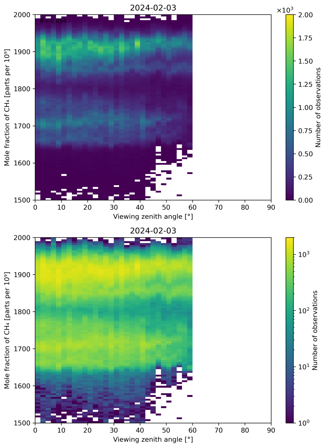
Figure 110: Scatter density plot of “Viewing zenith angle” against “Mole fraction of CH 4 ” for 2024-02-02 to 2024-02-04.
