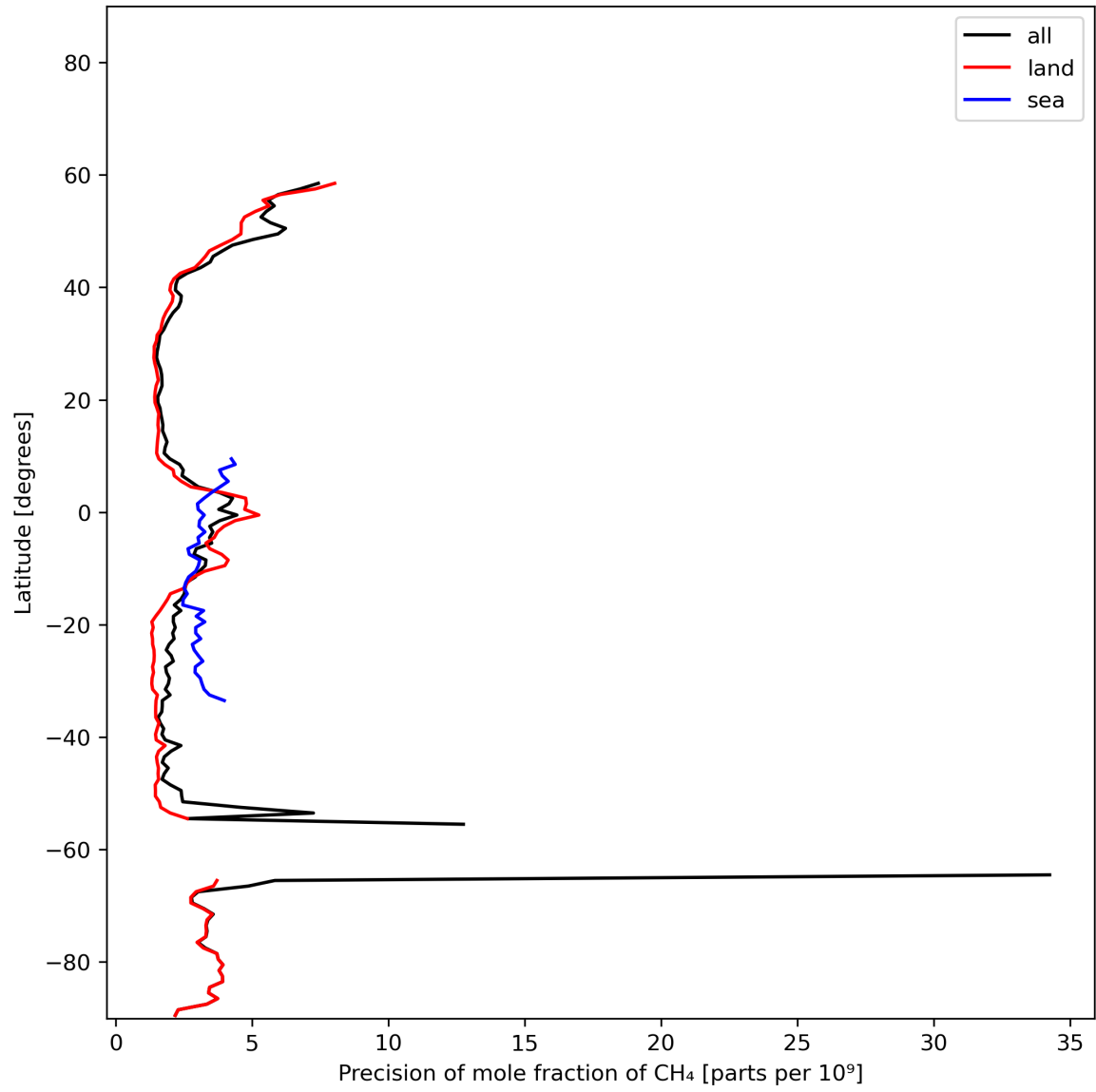
Figure 13: Zonal average of “Precision of mole fraction of CH 4 ” for 2024-02-02 to 2024-02-04.
