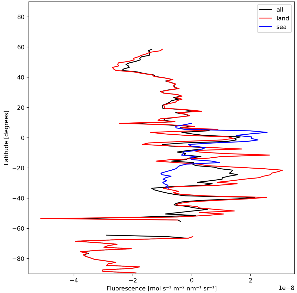
Figure 21: Zonal average of “Fluorescence” for 2024-02-02 to 2024-02-04.
