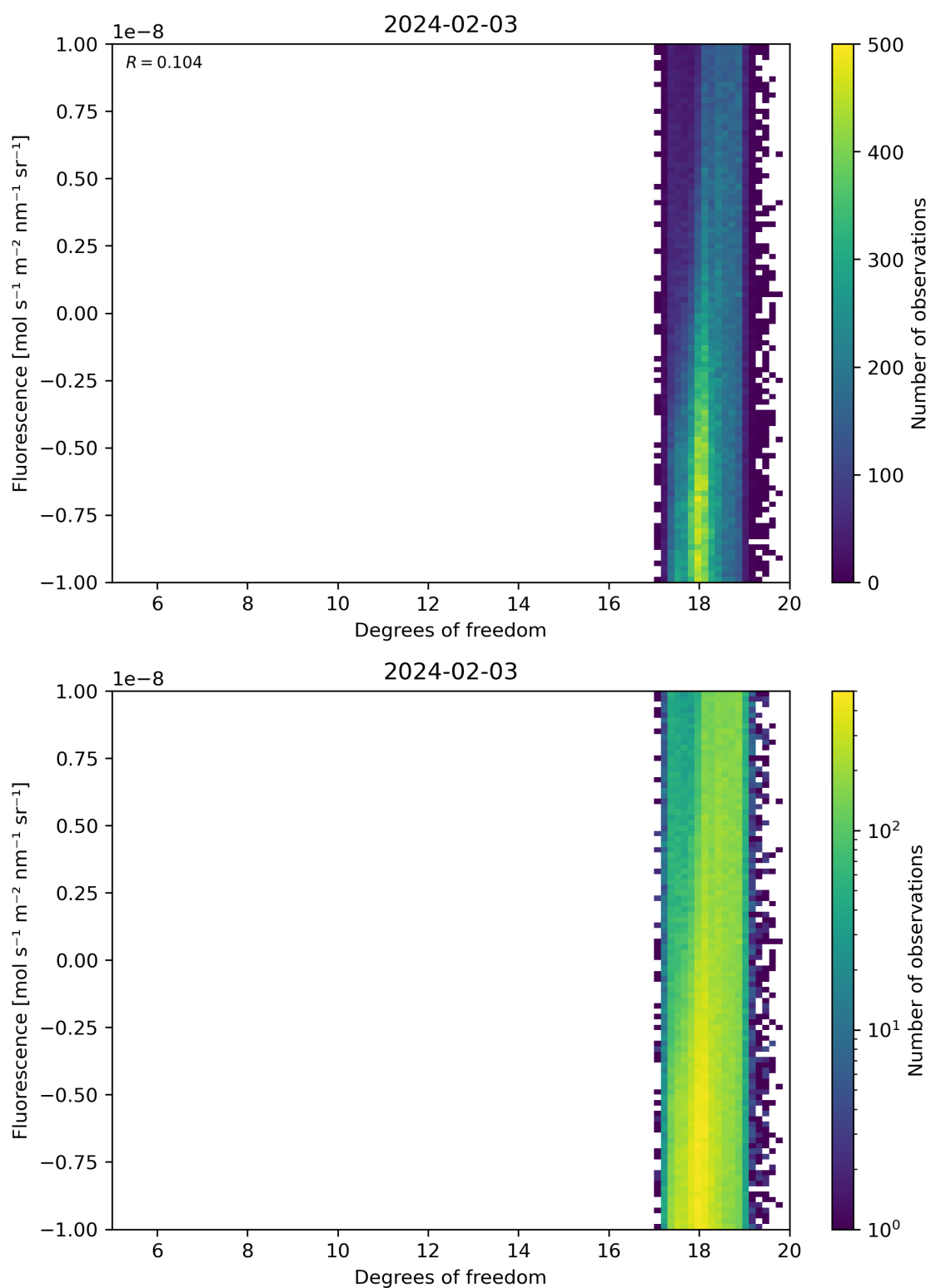
Figure 51: Scatter density plot of “Degrees of freedom” against “Fluorescence” for 2024-02-02 to 2024-02-04.
