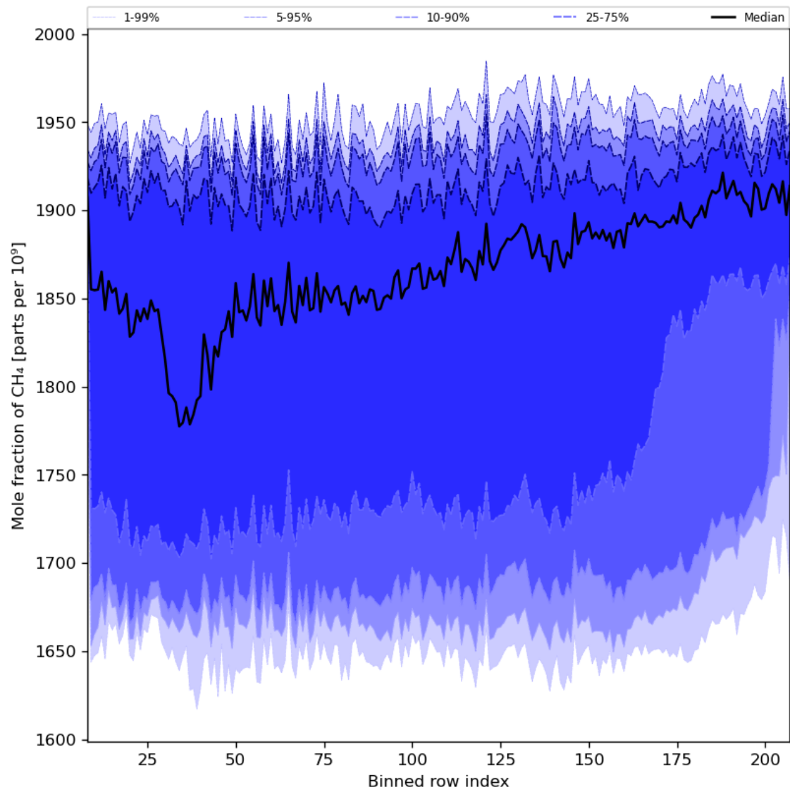
Figure 34: Along track statistics of “Mole fraction of CH 4 ” for 2024-02-02 to 2024-02-04
