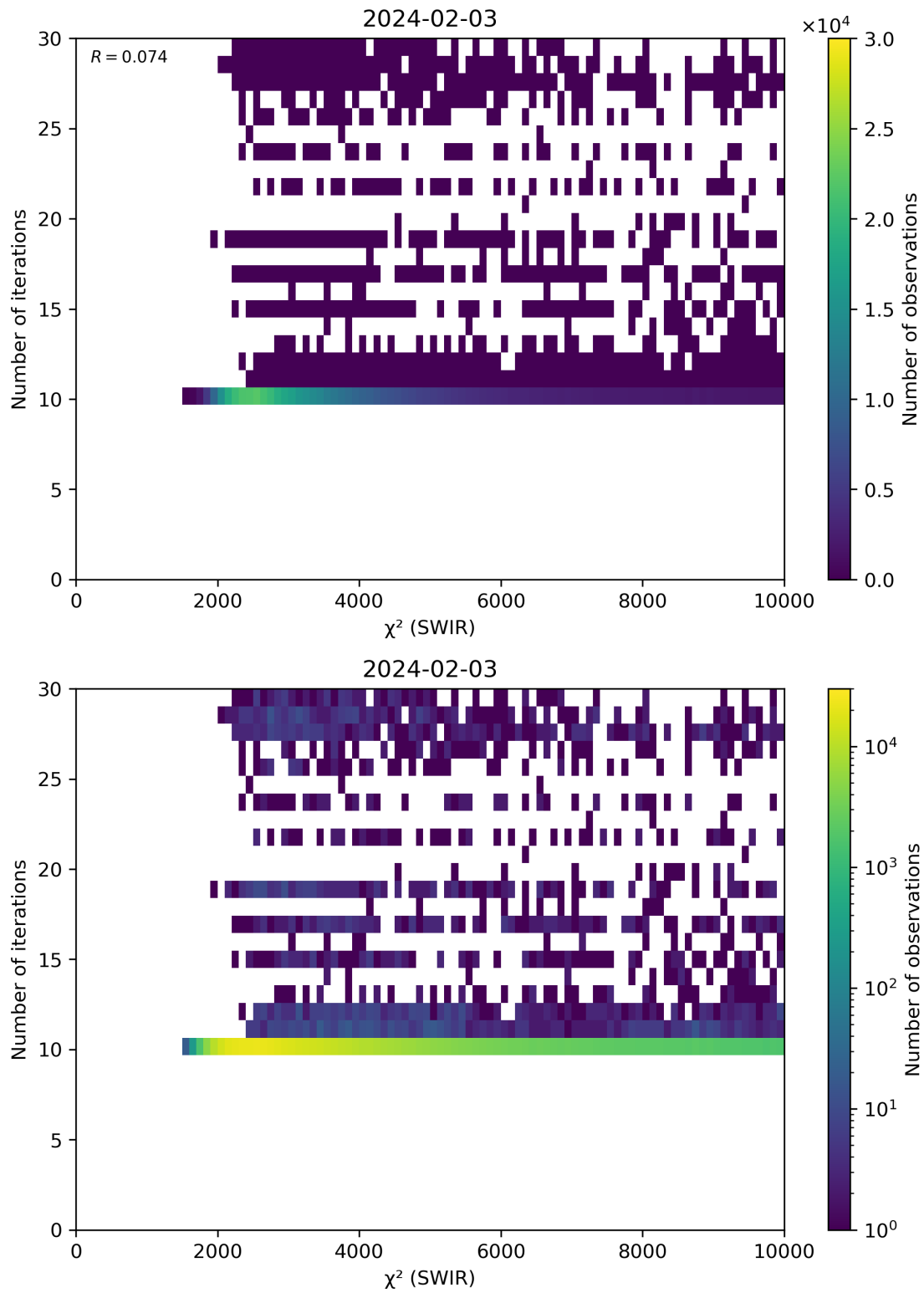
Figure 50: Scatter density plot of “ \chi^2 (SWIR)” against “Number of iterations” for 2024-02-02 to 2024-02-04.
