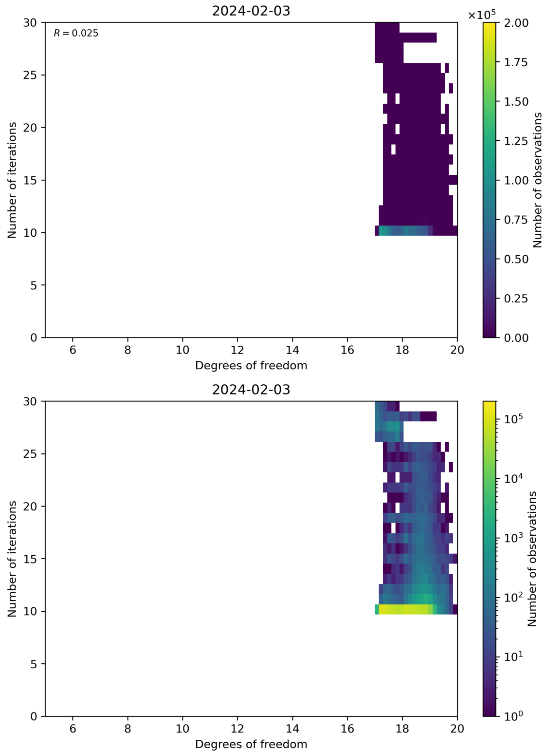
Figure 52: Scatter density plot of “Degrees of freedom” against “Number of iterations” for 2024-02-02 to 2024-02-04.
