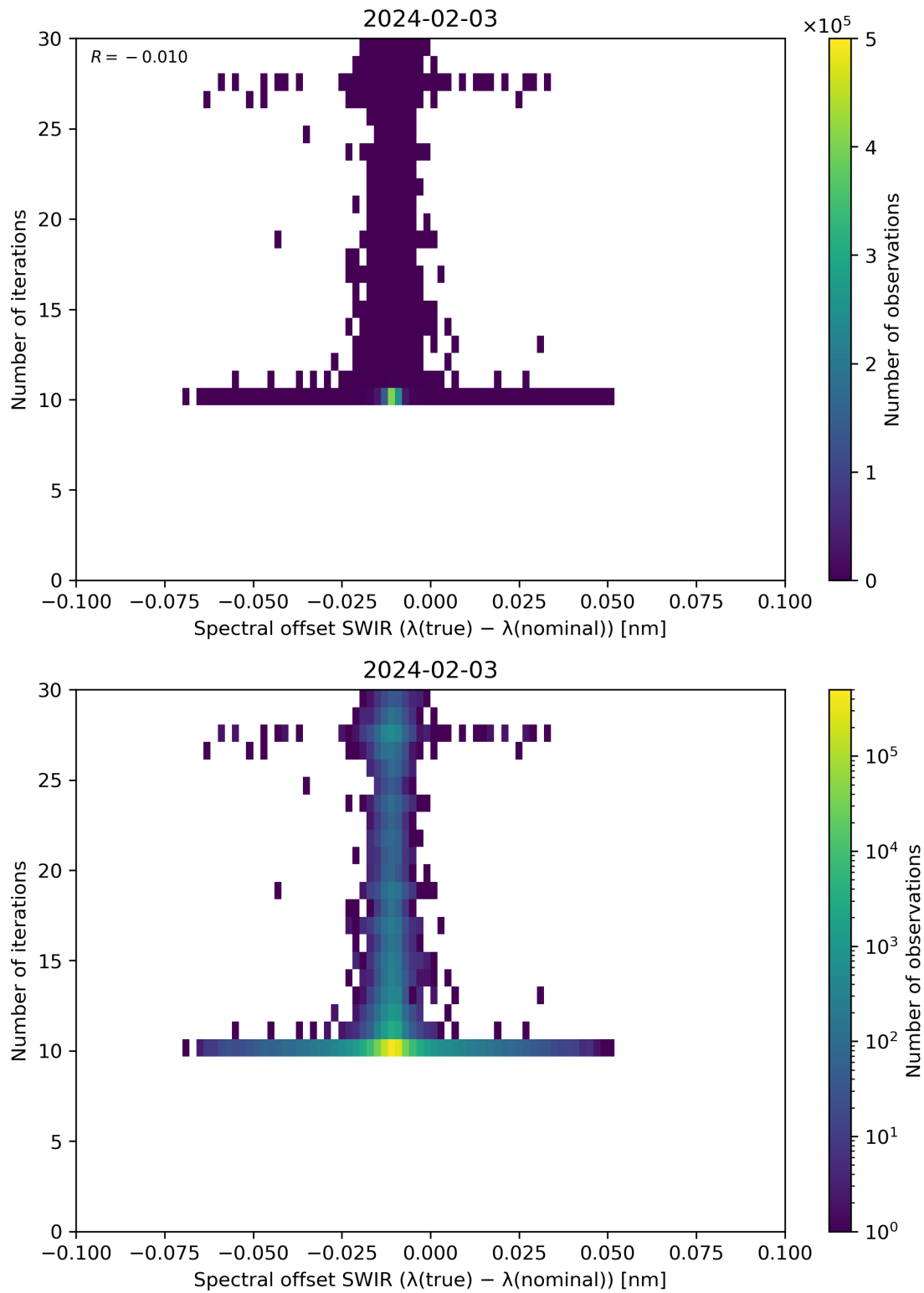
Figure 121: Scatter density plot of “Spectral offset SWIR ( \lambda(\text{true}) - \lambda(\text{nominal}) )” against “Number of iterations” for 2024-02-02 to 2024-02-04.
