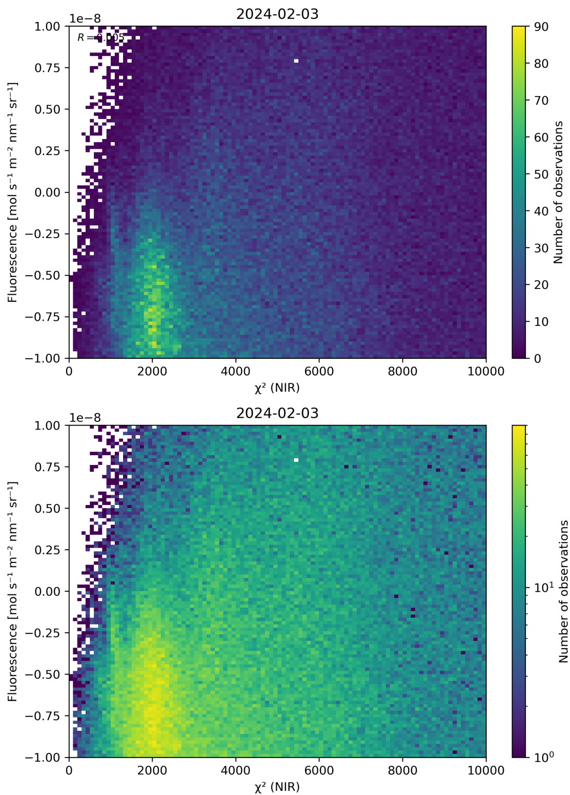
Figure 45: Scatter density plot of “ \chi^2 (NIR)” against “Fluorescence” for 2024-02-02 to 2024-02-04.
