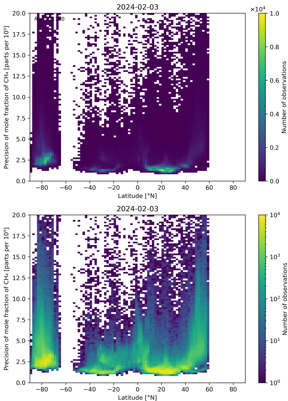
Figure 59: Scatter density plot of “Latitude” against “Precision of mole fraction of CH 4 ” for 2024-02-02 to 2024-02-04.
