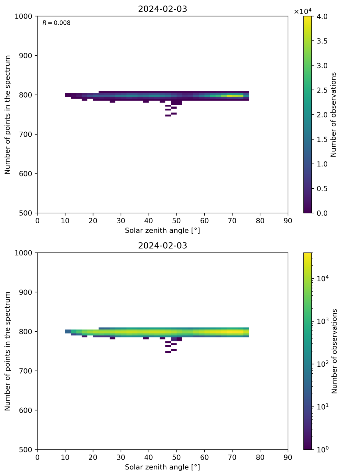
Figure 103: Scatter density plot of “Solar zenith angle” against “Number of points in the spectrum” for 2024-02-02 to 2024-02-04.
