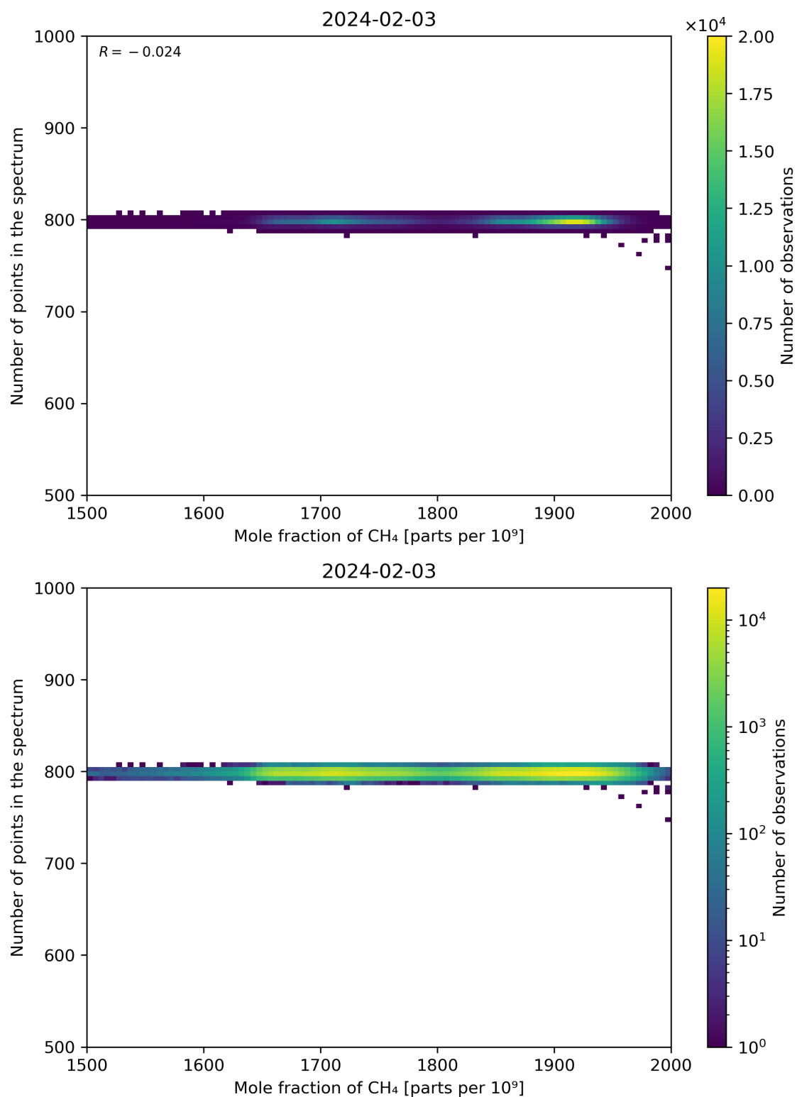
Figure 77: Scatter density plot of “Mole fraction of CH 4 ” against “Number of points in the spectrum” for 2024-02-02 to 2024-02-04.
