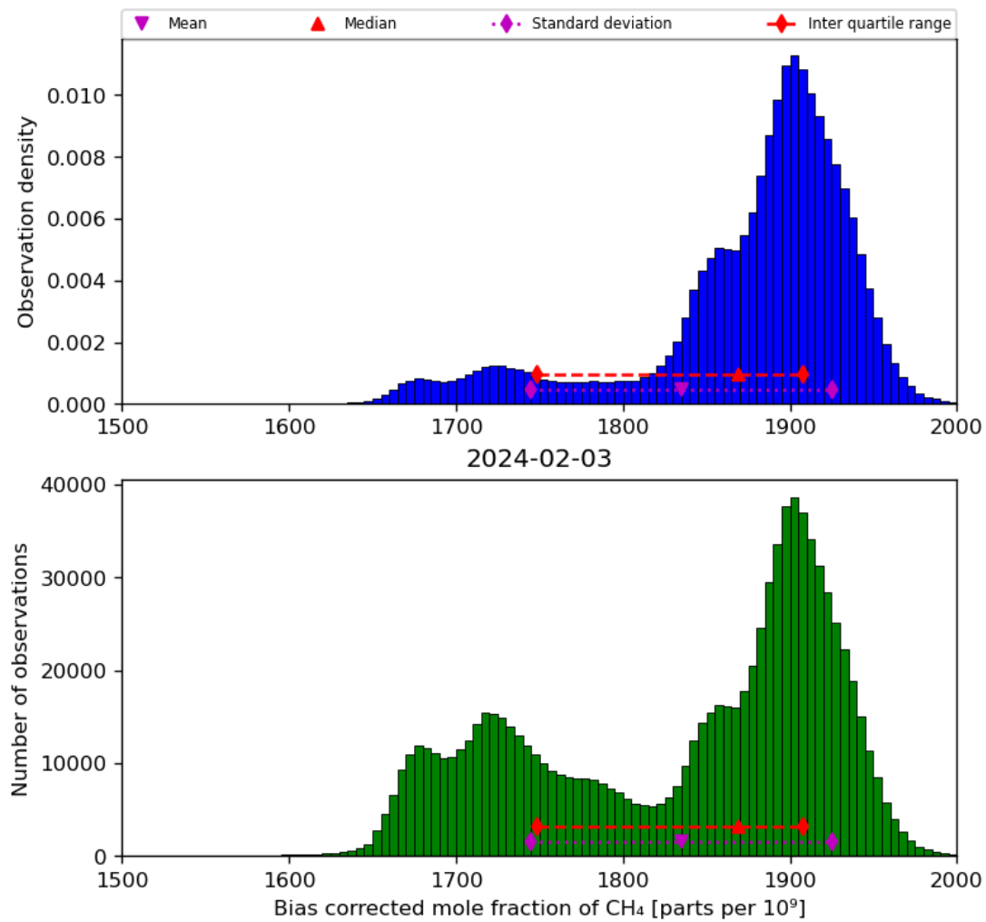
Figure 25: Histogram of “Bias corrected mole fraction of CH 4 ” for 2024-02-02 to 2024-02-04
