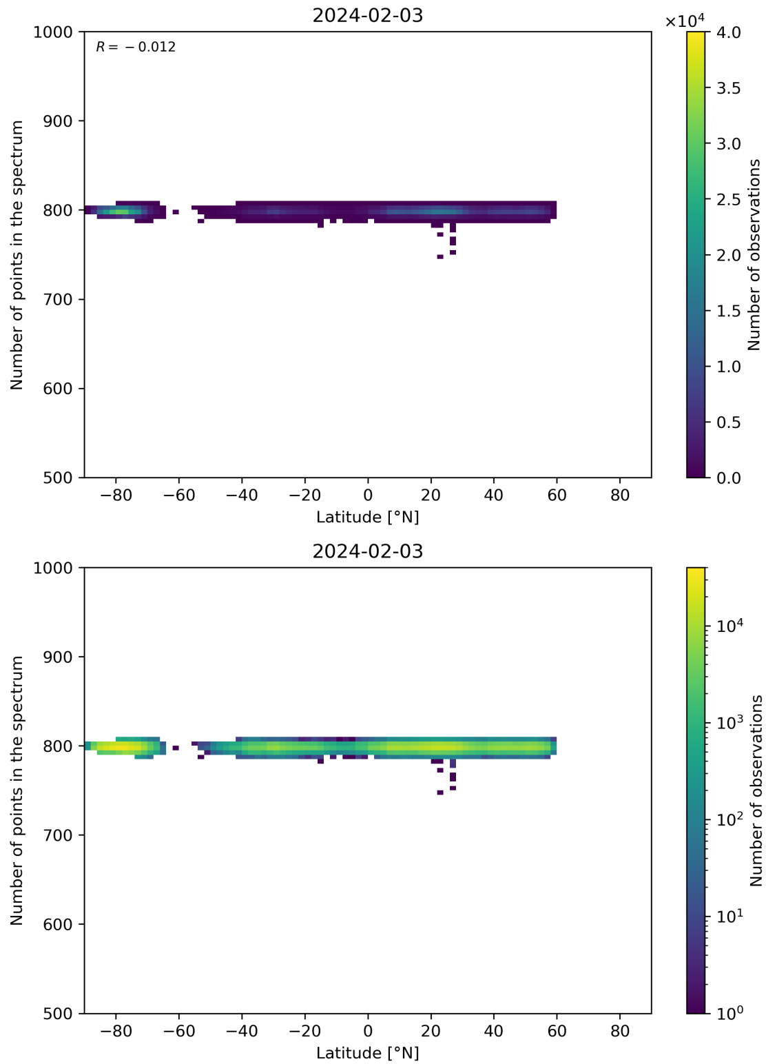
Figure 61: Scatter density plot of “Latitude” against “Number of points in the spectrum” for 2024-02-02 to 2024-02-04.
