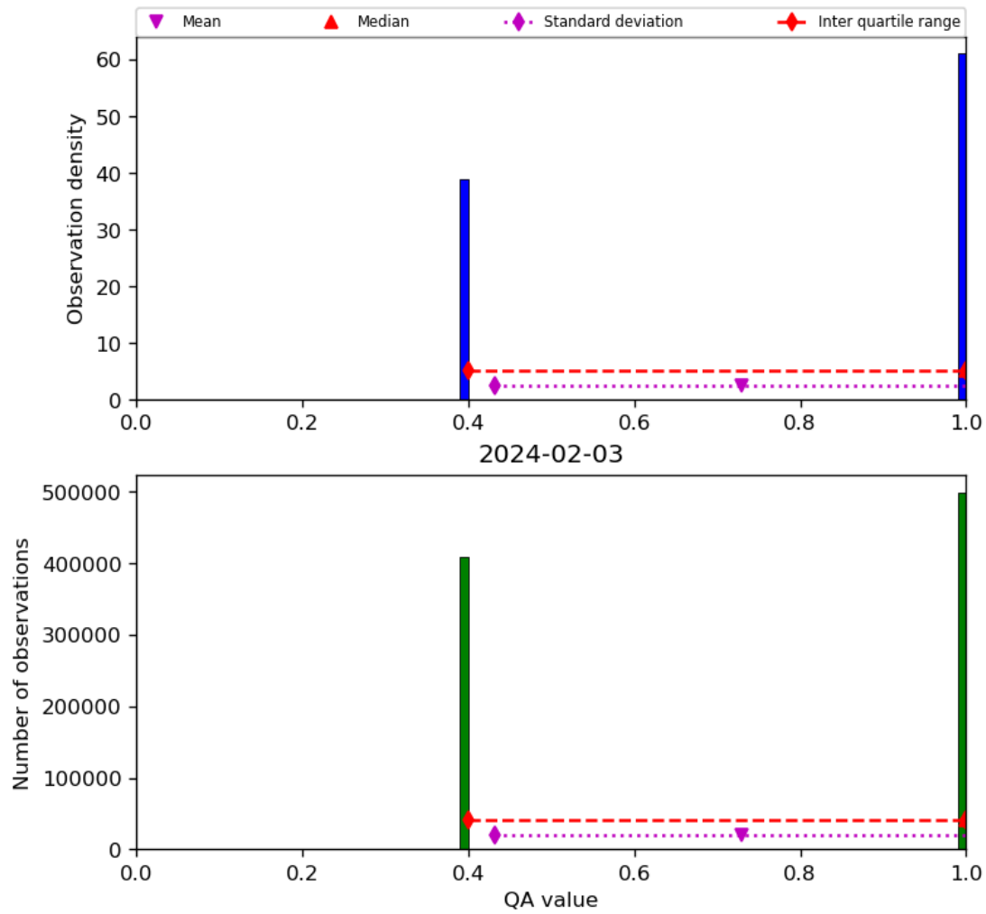
Figure 22: Histogram of “QA value” for 2024-02-02 to 2024-02-04
