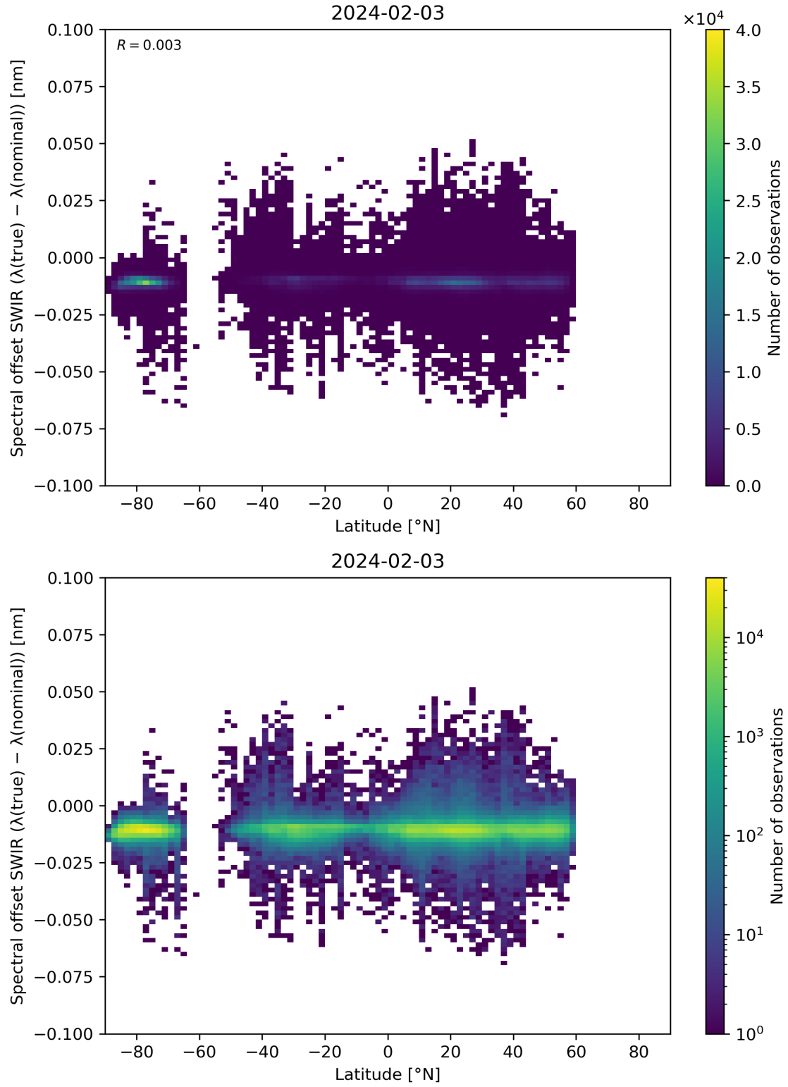
Figure 62: Scatter density plot of “Latitude” against “Spectral offset SWIR ( \lambda(\text{true}) - \lambda(\text{nominal}) )” for 2024-02-02 to 2024-02-04.
