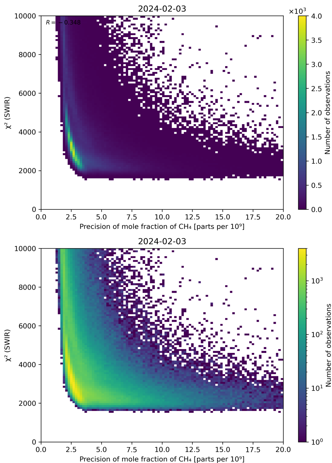
Figure 79: Scatter density plot of “Precision of mole fraction of \text{CH}_4 ” against “ \chi^2 (SWIR)” for 2024-02-02 to 2024-02-04.
