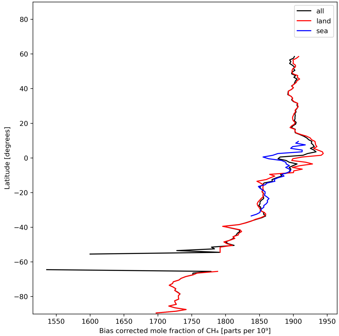
Figure 14: Zonal average of “Bias corrected mole fraction of CH 4 ” for 2024-02-02 to 2024-02-04.
