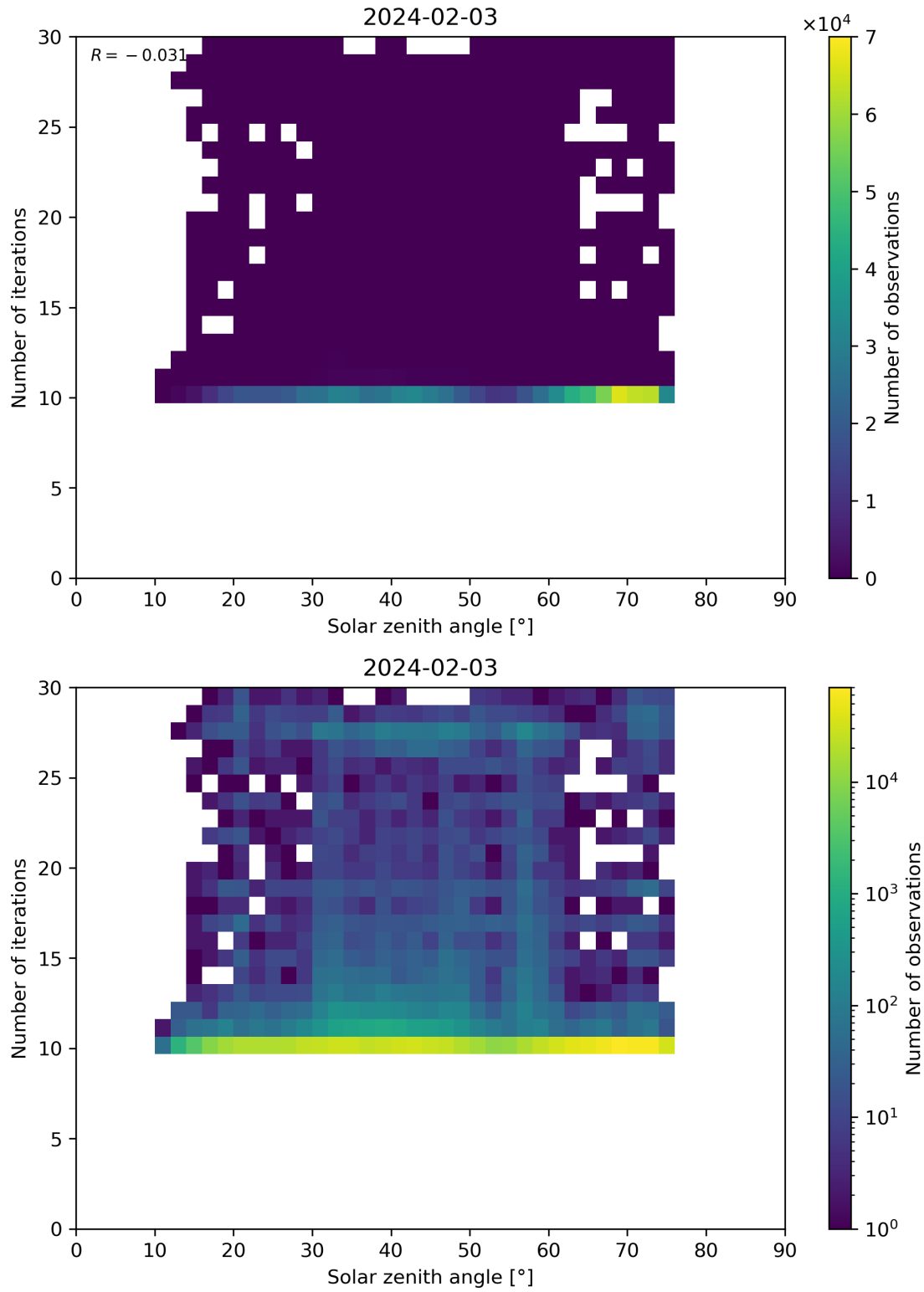
Figure 102: Scatter density plot of “Solar zenith angle” against “Number of iterations” for 2024-02-02 to 2024-02-04.
