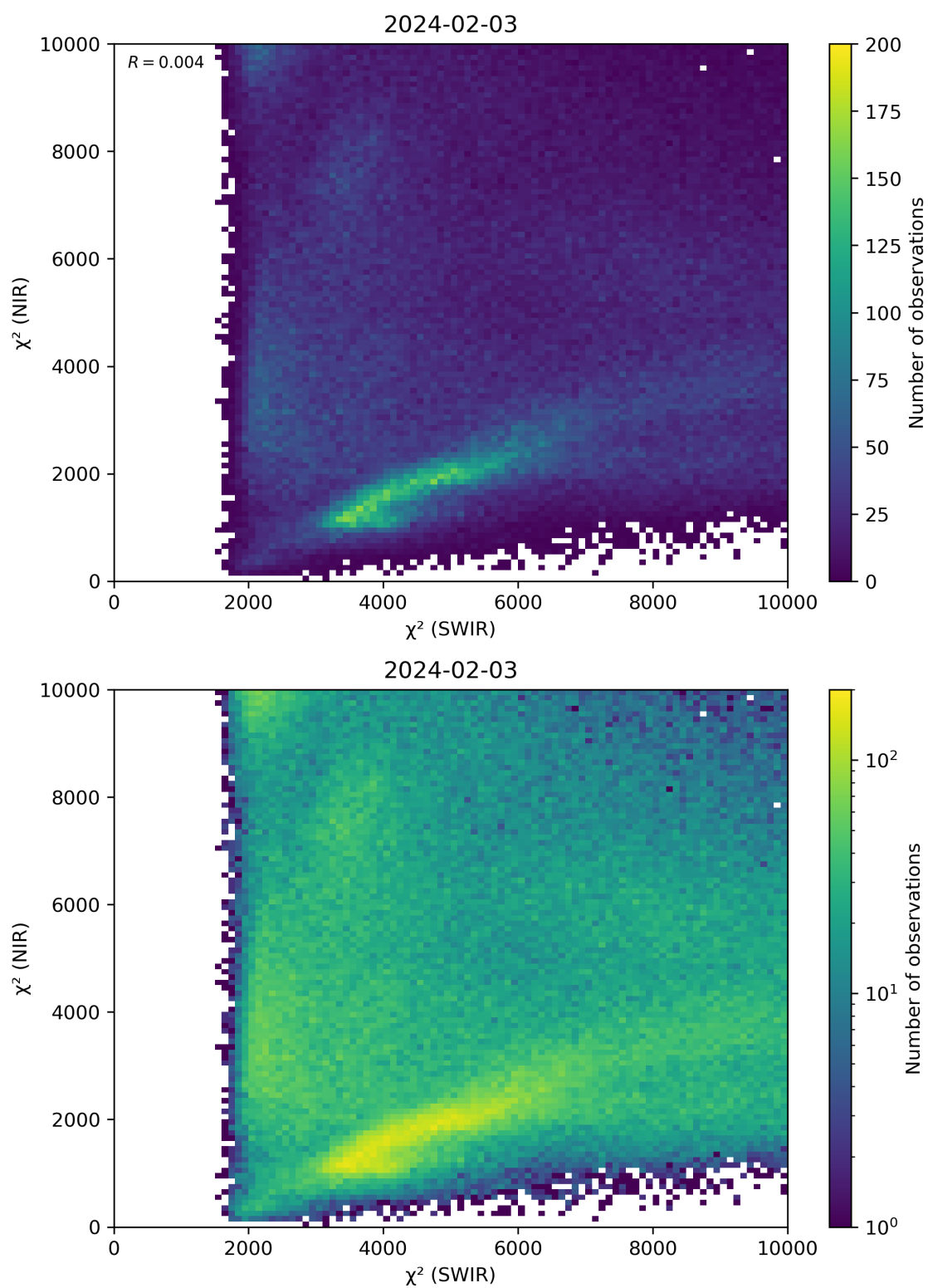
Figure 47: Scatter density plot of “ \chi^2 (SWIR)” against “ \chi^2 (NIR)” for 2024-02-02 to 2024-02-04.
