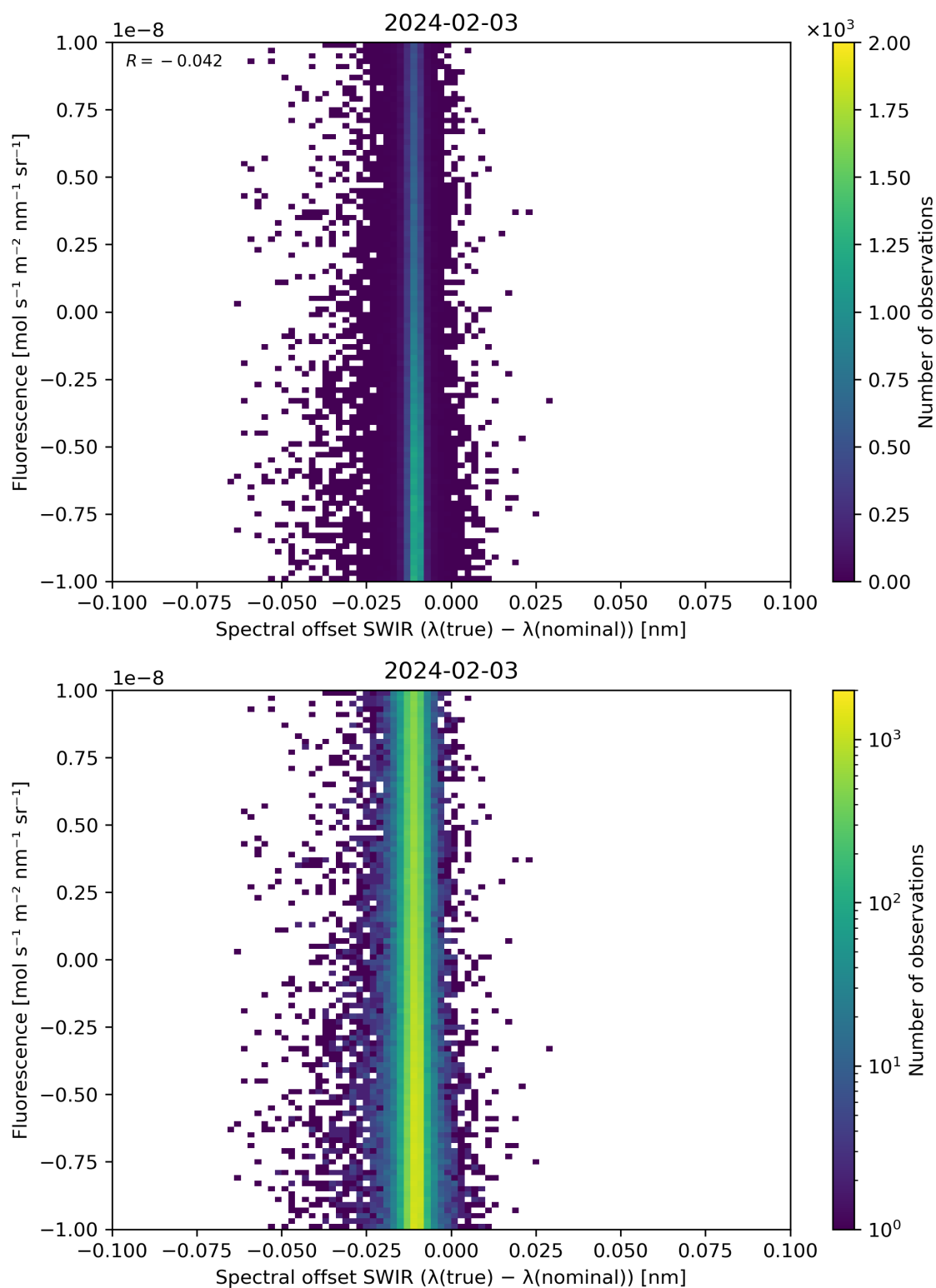
Figure 120: Scatter density plot of “Spectral offset SWIR ( \lambda(\text{true}) - \lambda(\text{nominal}) )” against “Fluorescence” for 2024-02-02 to 2024-02-04.
