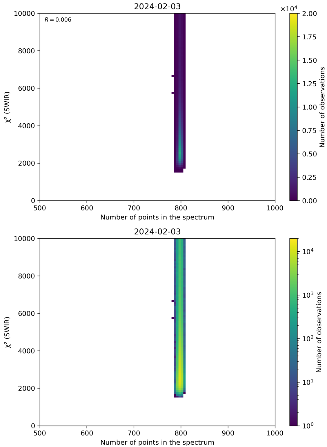
Figure 89: Scatter density plot of “Number of points in the spectrum” against “ \chi^2 (SWIR)” for 2024-02-02 to 2024-02-04.
