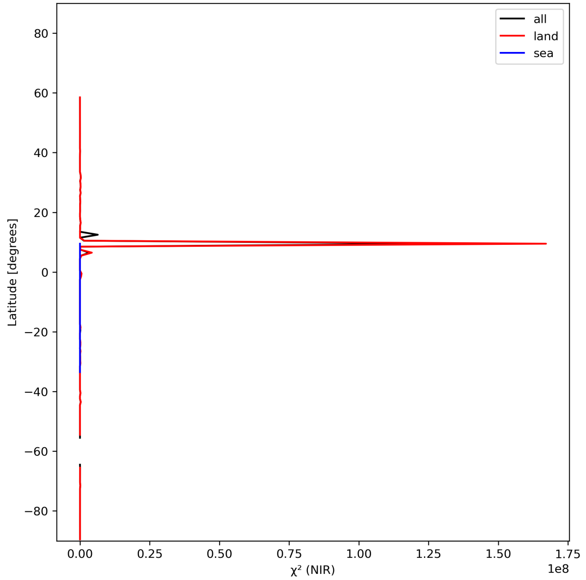
Figure 18: Zonal average of “ \chi^2 (NIR)” for 2024-02-02 to 2024-02-04.
