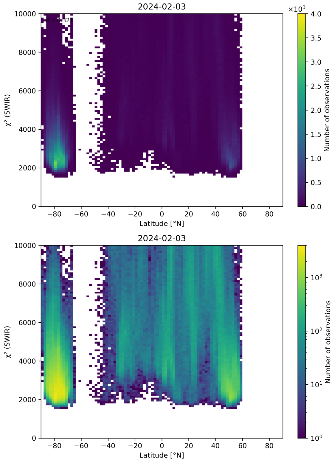
Figure 54: Scatter density plot of “Latitude” against “ \chi^2 (SWIR)” for 2024-02-02 to 2024-02-04.
