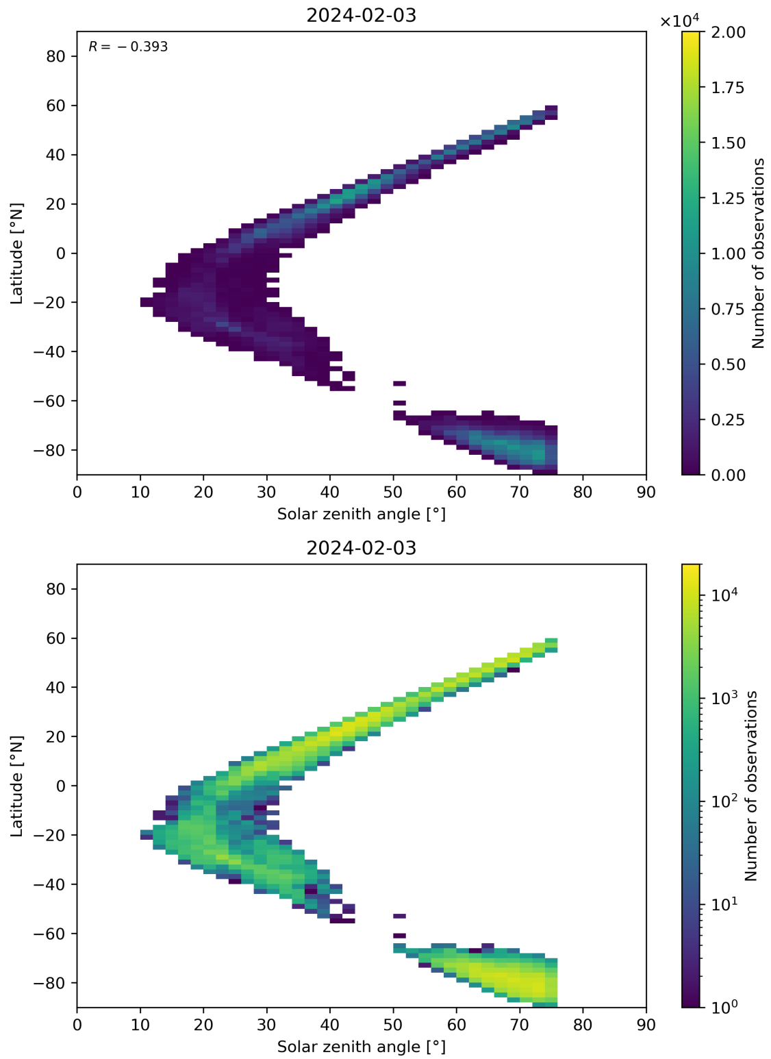
Figure 98: Scatter density plot of “Solar zenith angle” against “Latitude” for 2024-02-02 to 2024-02-04.
