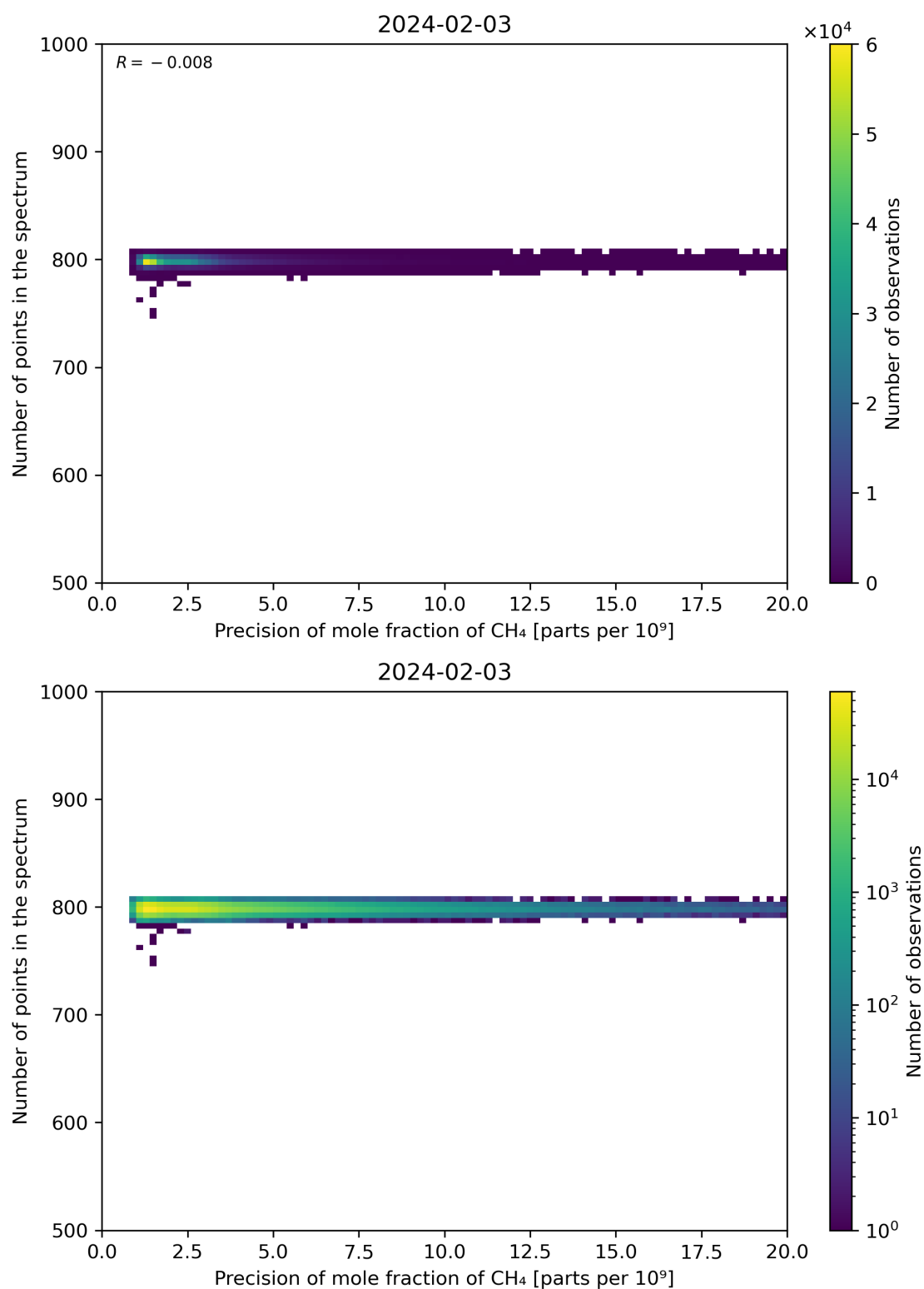
Figure 84: Scatter density plot of “Precision of mole fraction of CH 4 ” against “Number of points in the spectrum” for 2024-02-02 to 2024-02-04.
