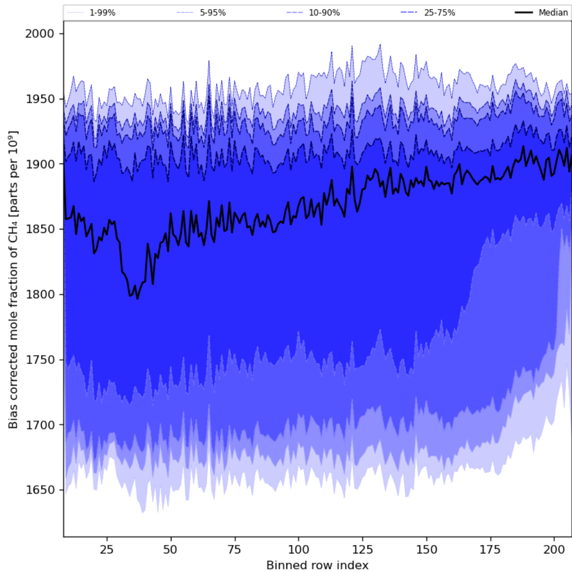
Figure 36: Along track statistics of “Bias corrected mole fraction of CH 4 ” for 2024-02-02 to 2024-02-04
