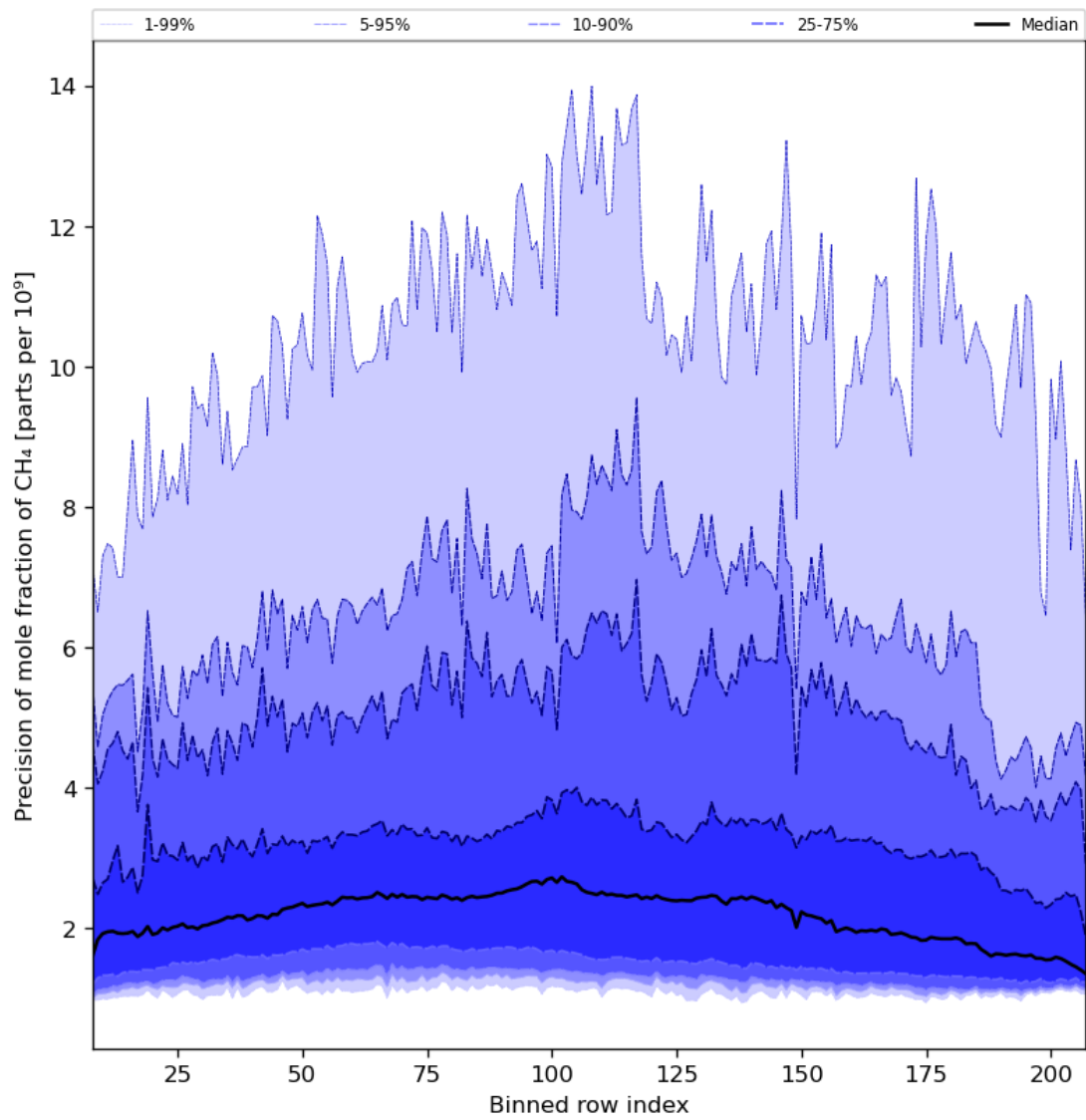
Figure 35: Along track statistics of “Precision of mole fraction of CH 4 ” for 2024-02-02 to 2024-02-04
