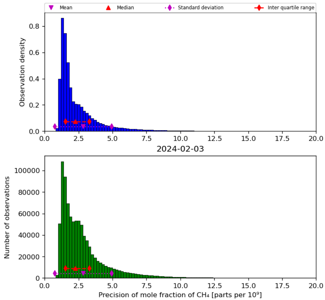
Figure 24: Histogram of “Precision of mole fraction of CH 4 ” for 2024-02-02 to 2024-02-04
