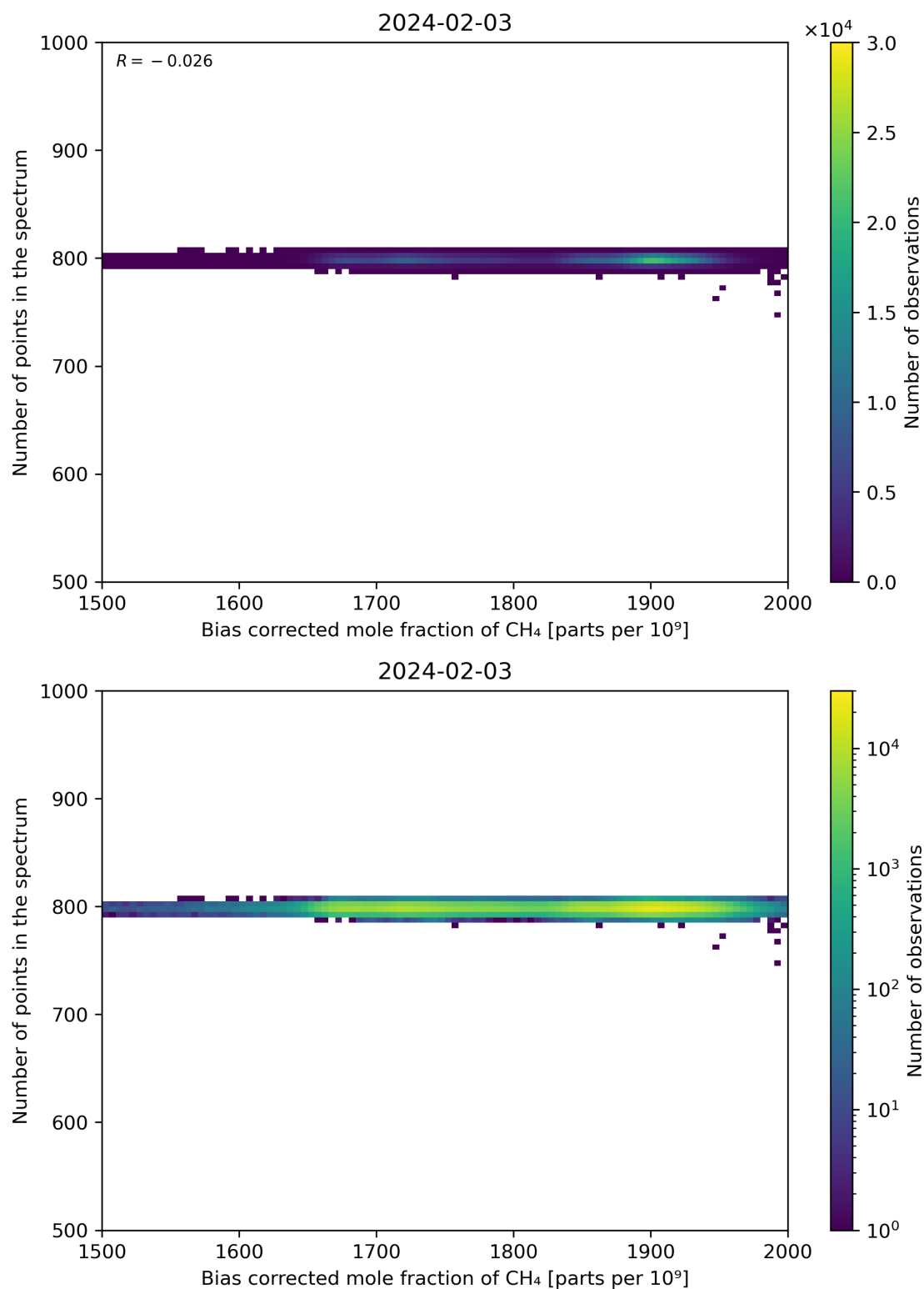
Figure 68: Scatter density plot of “Bias corrected mole fraction of CH 4 ” against “Number of points in the spectrum” for 2024-02-02 to 2024-02-04.
