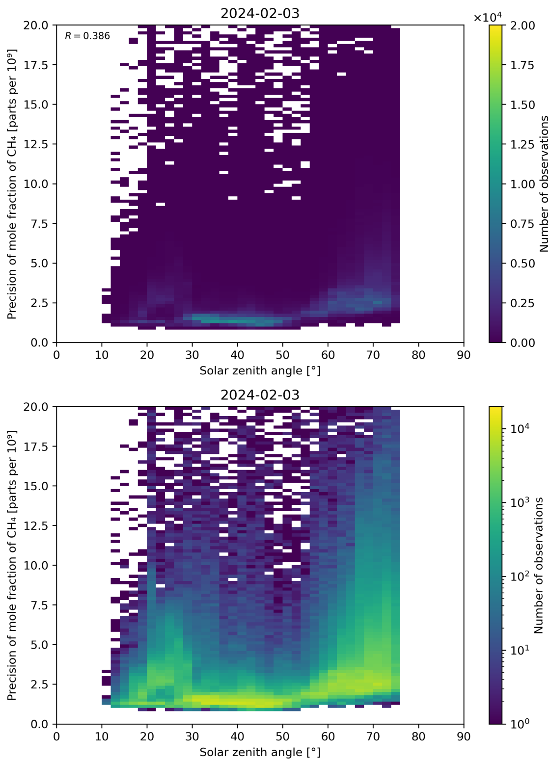
Figure 101: Scatter density plot of “Solar zenith angle” against “Precision of mole fraction of CH 4 ” for 2024-02-02 to 2024-02-04.
