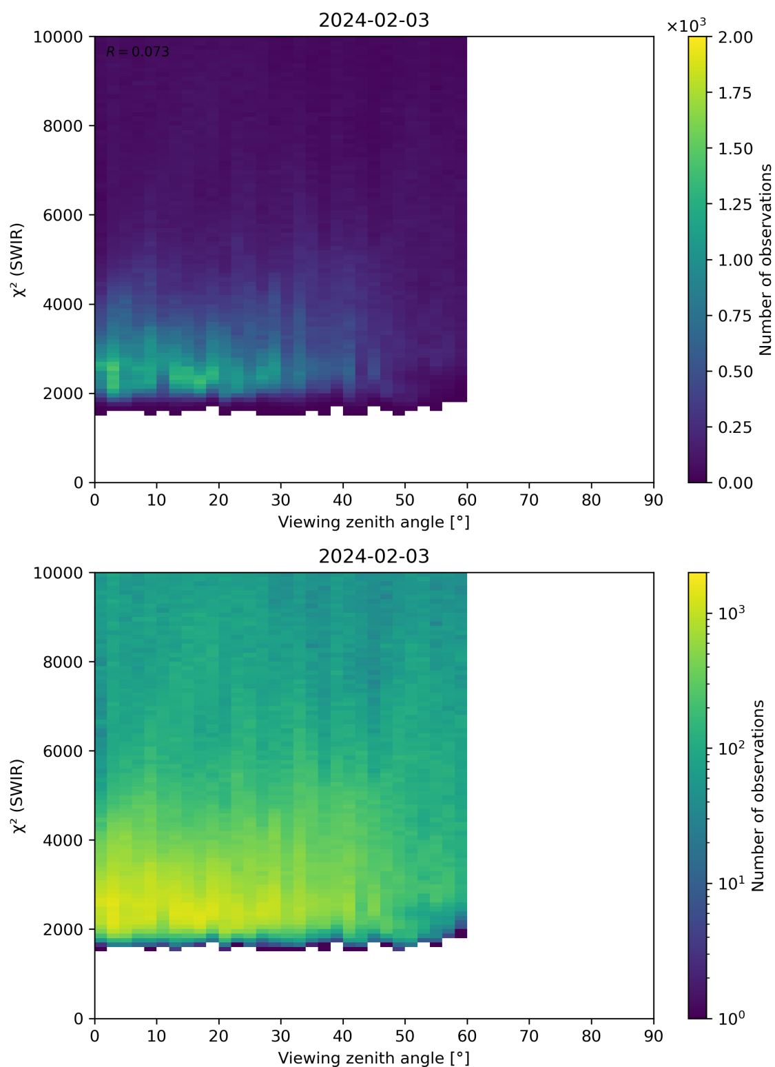
Figure 106: Scatter density plot of “Viewing zenith angle” against “ \chi^2 (SWIR)” for 2024-02-02 to 2024-02-04.
