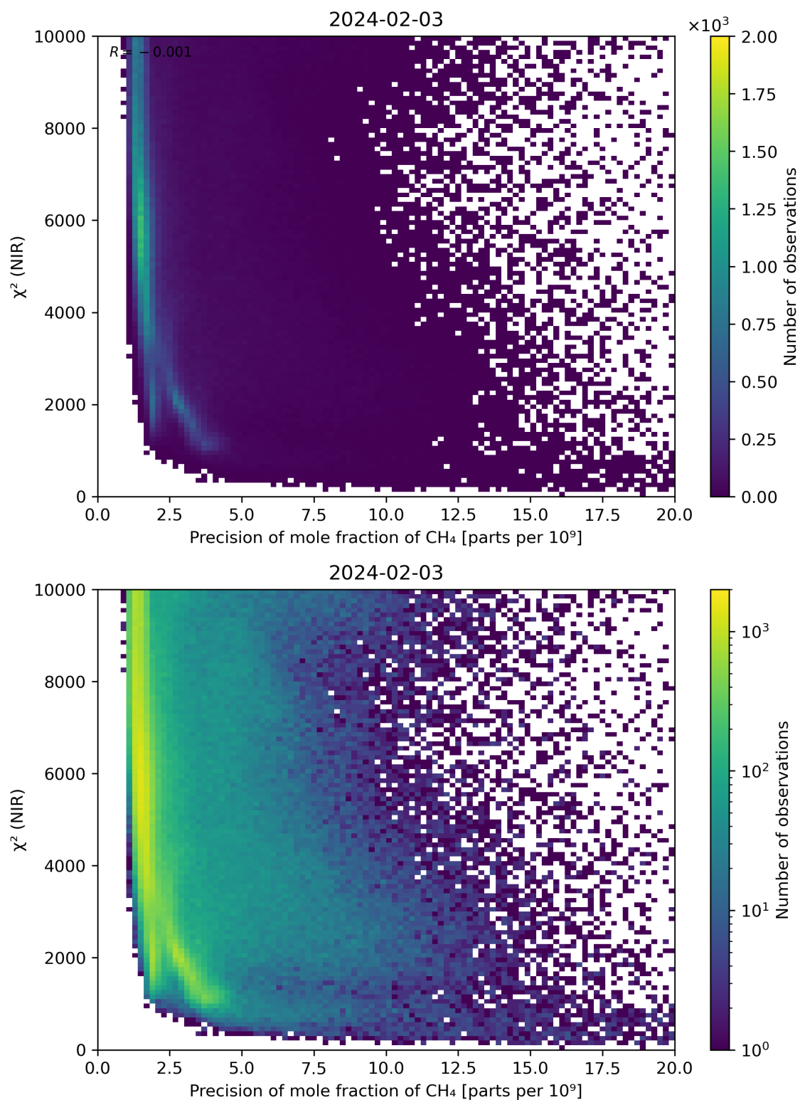
Figure 78: Scatter density plot of “Precision of mole fraction of CH 4 ” against “ \chi^2 (NIR)” for 2024-02-02 to 2024-02-04.
