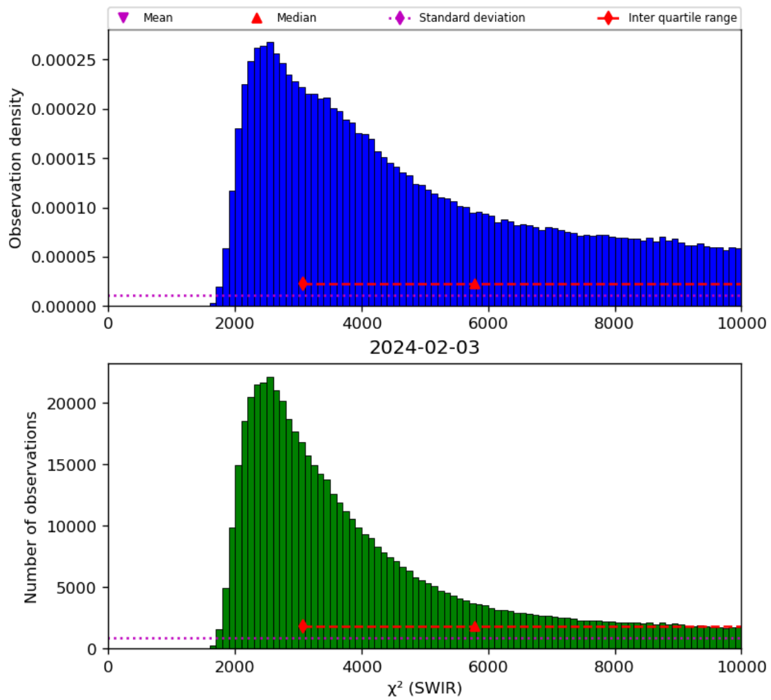
Figure 28: Histogram of “ \chi^2 (SWIR)” for 2024-02-02 to 2024-02-04
