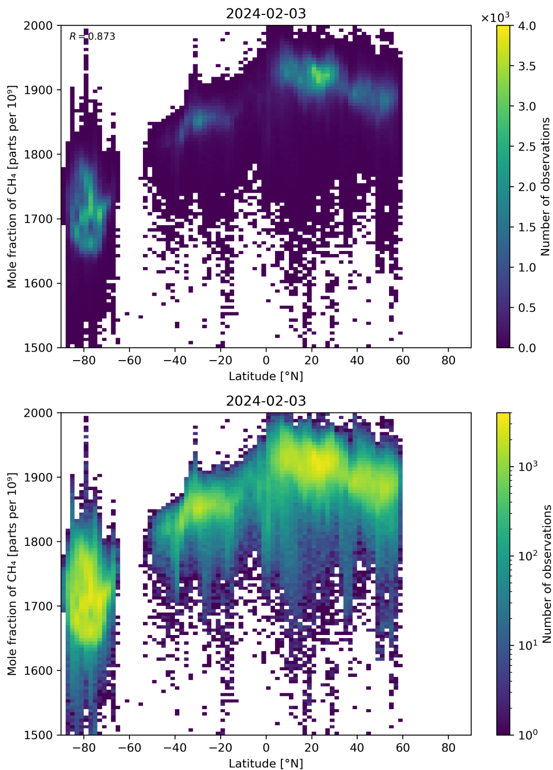
Figure 57: Scatter density plot of “Latitude” against “Mole fraction of CH 4 ” for 2024-02-02 to 2024-02-04.
