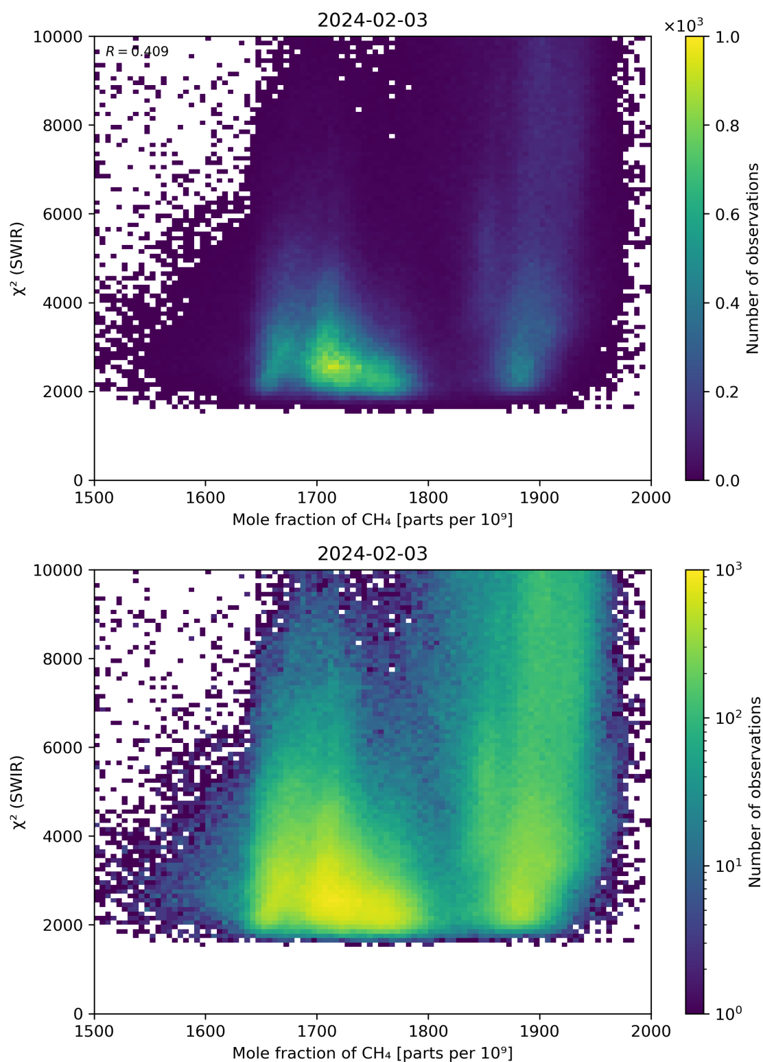
Figure 71: Scatter density plot of “Mole fraction of \text{CH}_4 ” against “ \chi^2 (SWIR)” for 2024-02-02 to 2024-02-04.
