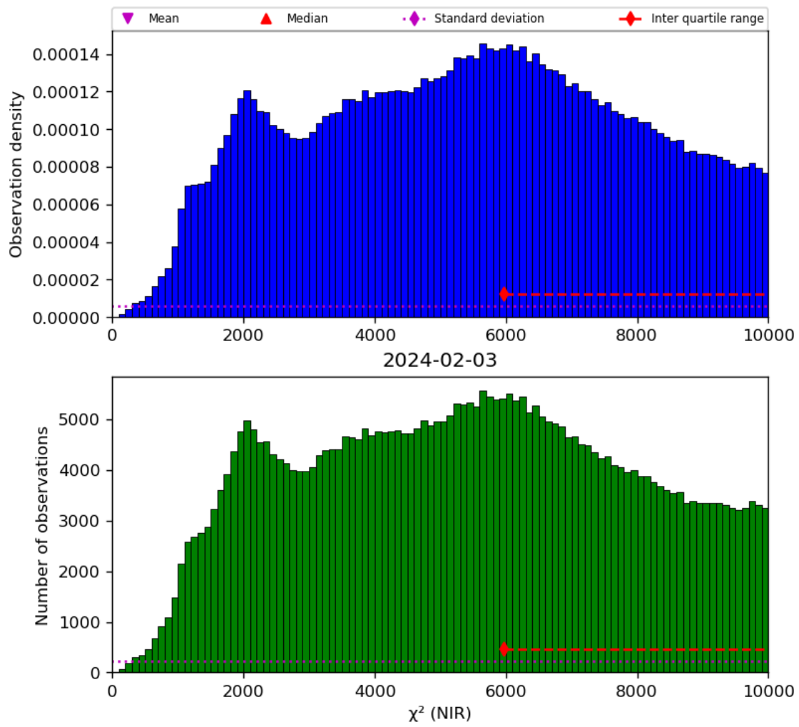
Figure 29: Histogram of “ \chi^2 (NIR)” for 2024-02-02 to 2024-02-04
