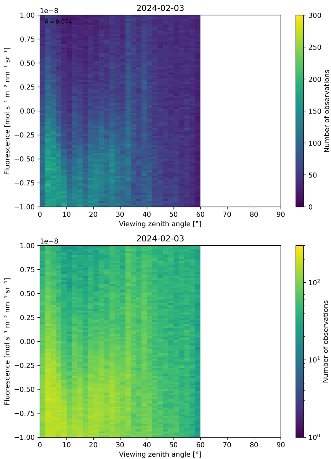
Figure 108: Scatter density plot of “Viewing zenith angle” against “Fluorescence” for 2024-02-02 to 2024-02-04.
