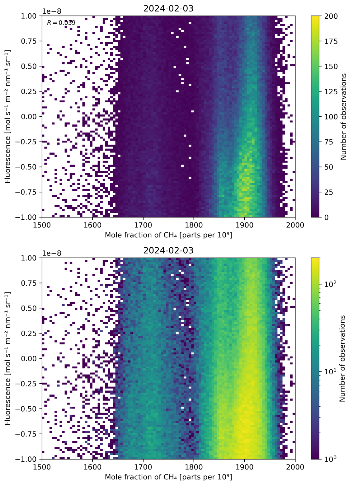
Figure 73: Scatter density plot of “Mole fraction of \text{CH}_4 ” against “Fluorescence” for 2024-02-02 to 2024-02-04.
