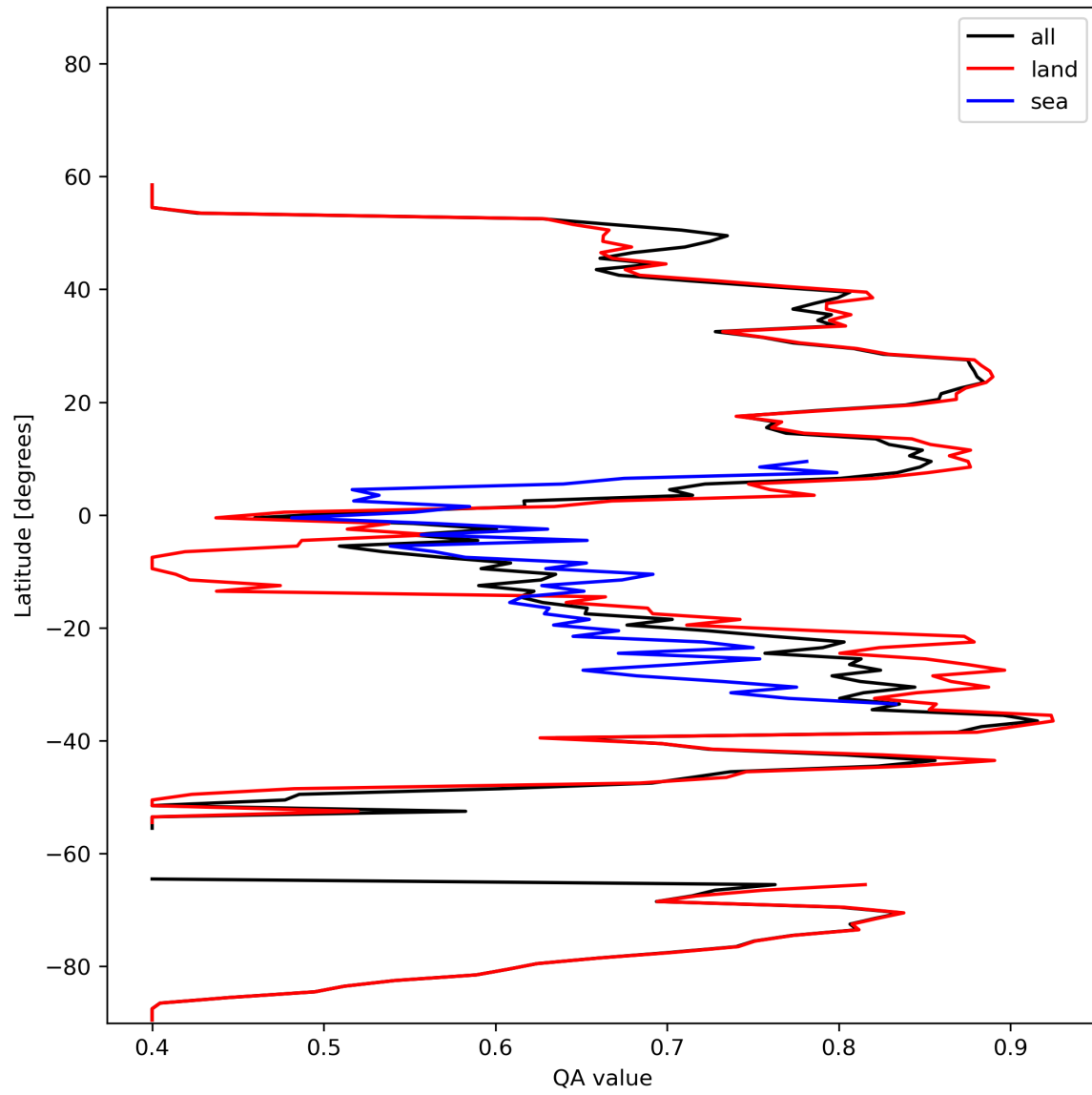
Figure 11: Zonal average of “QA value” for 2024-02-02 to 2024-02-04.
