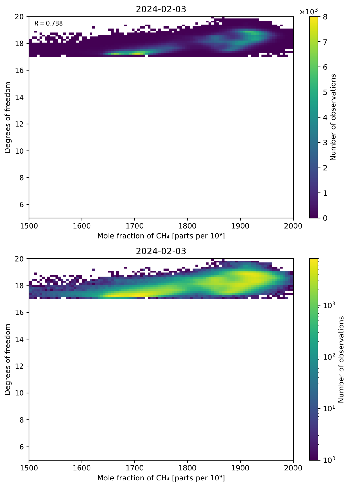
Figure 72: Scatter density plot of “Mole fraction of CH 4 ” against “Degrees of freedom” for 2024-02-02 to 2024-02-04.
