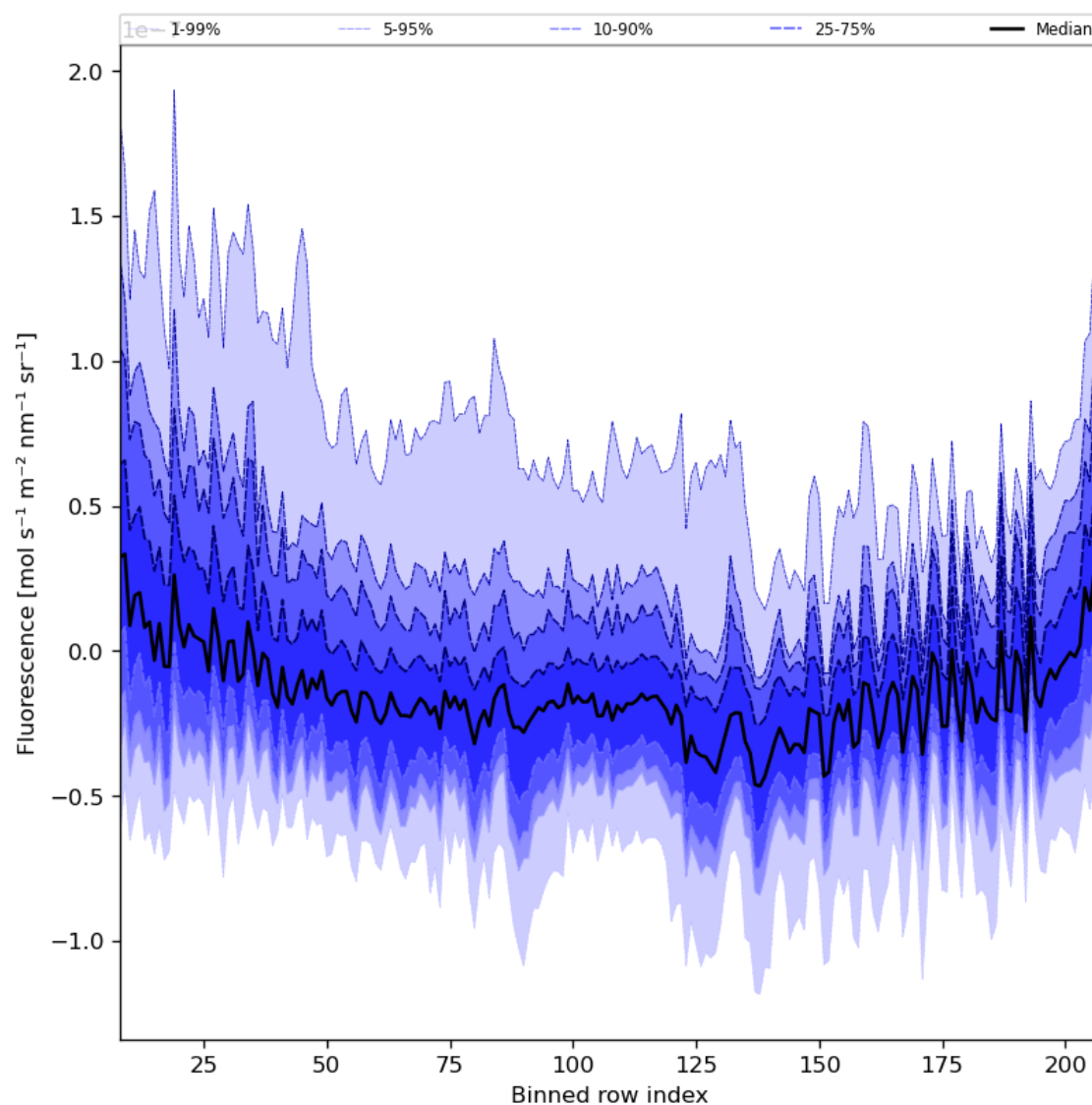
Figure 43: Along track statistics of “Fluorescence” for 2024-02-02 to 2024-02-04
