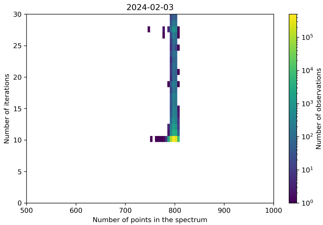
Figure 92: Scatter density plot of “Number of points in the spectrum” against “Number of iterations” for 2024-02-02 to 2024-02-04.
