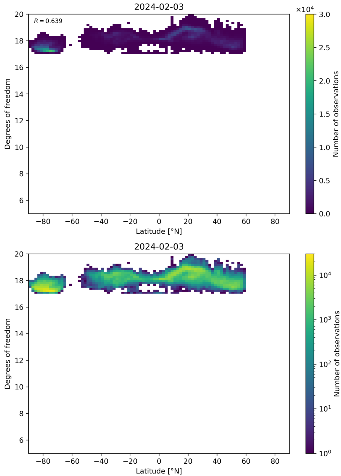
Figure 55: Scatter density plot of “Latitude” against “Degrees of freedom” for 2024-02-02 to 2024-02-04.
