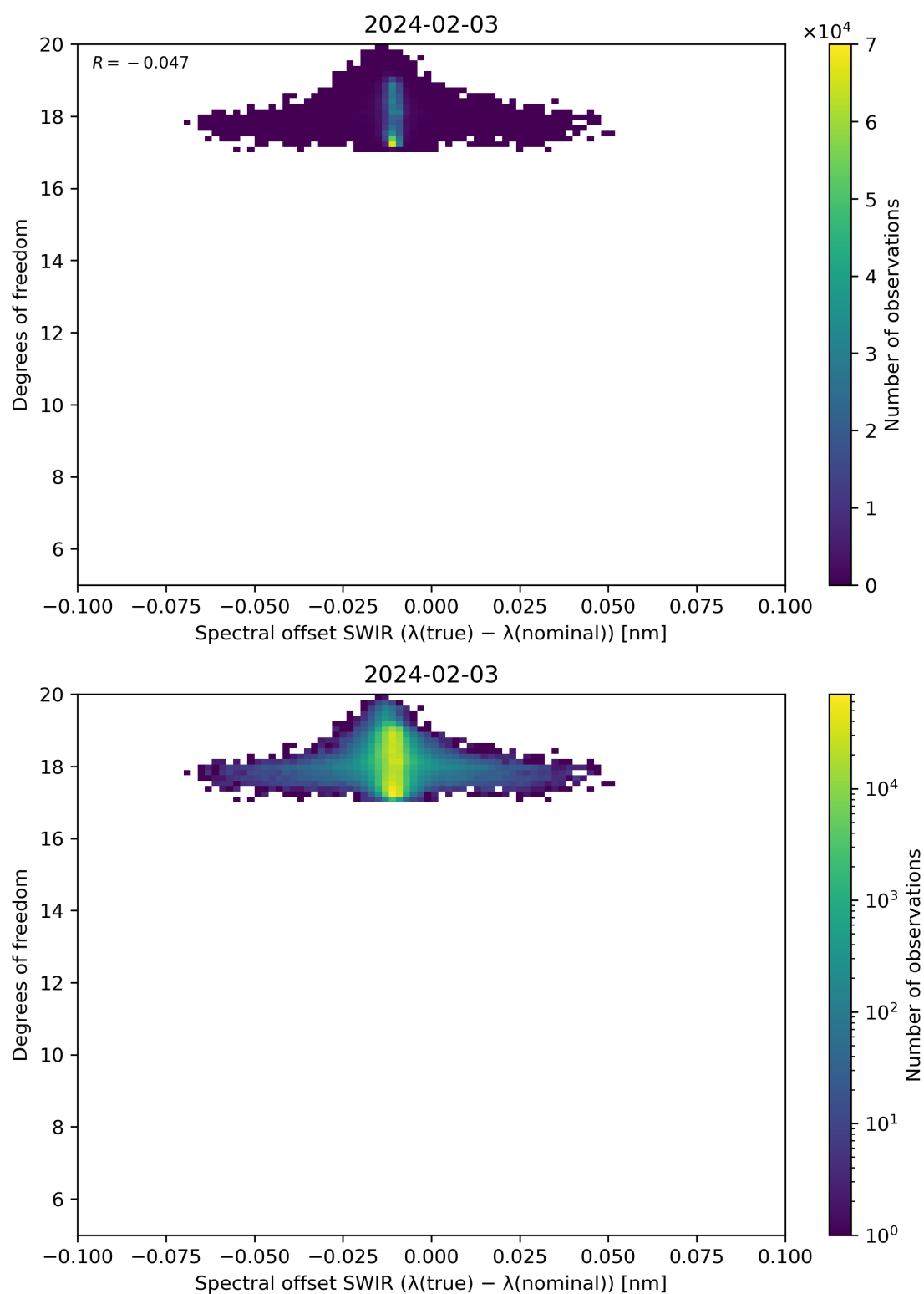
Figure 119: Scatter density plot of “Spectral offset SWIR ( \lambda(\text{true}) - \lambda(\text{nominal}) )” against “Degrees of freedom” for 2024-02-02 to 2024-02-04.
