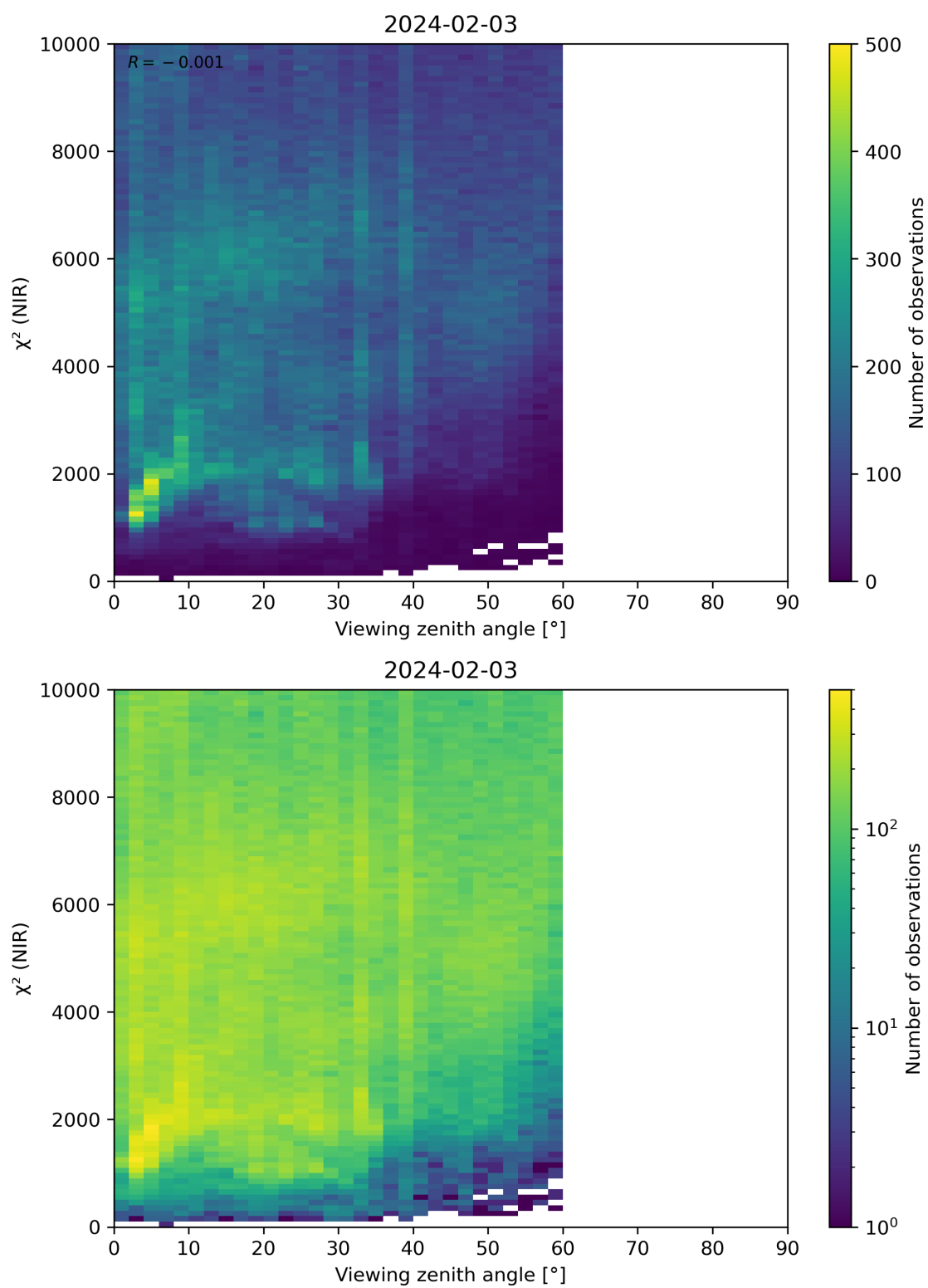
Figure 105: Scatter density plot of “Viewing zenith angle” against “ \chi^2 (NIR)” for 2024-02-02 to 2024-02-04.
