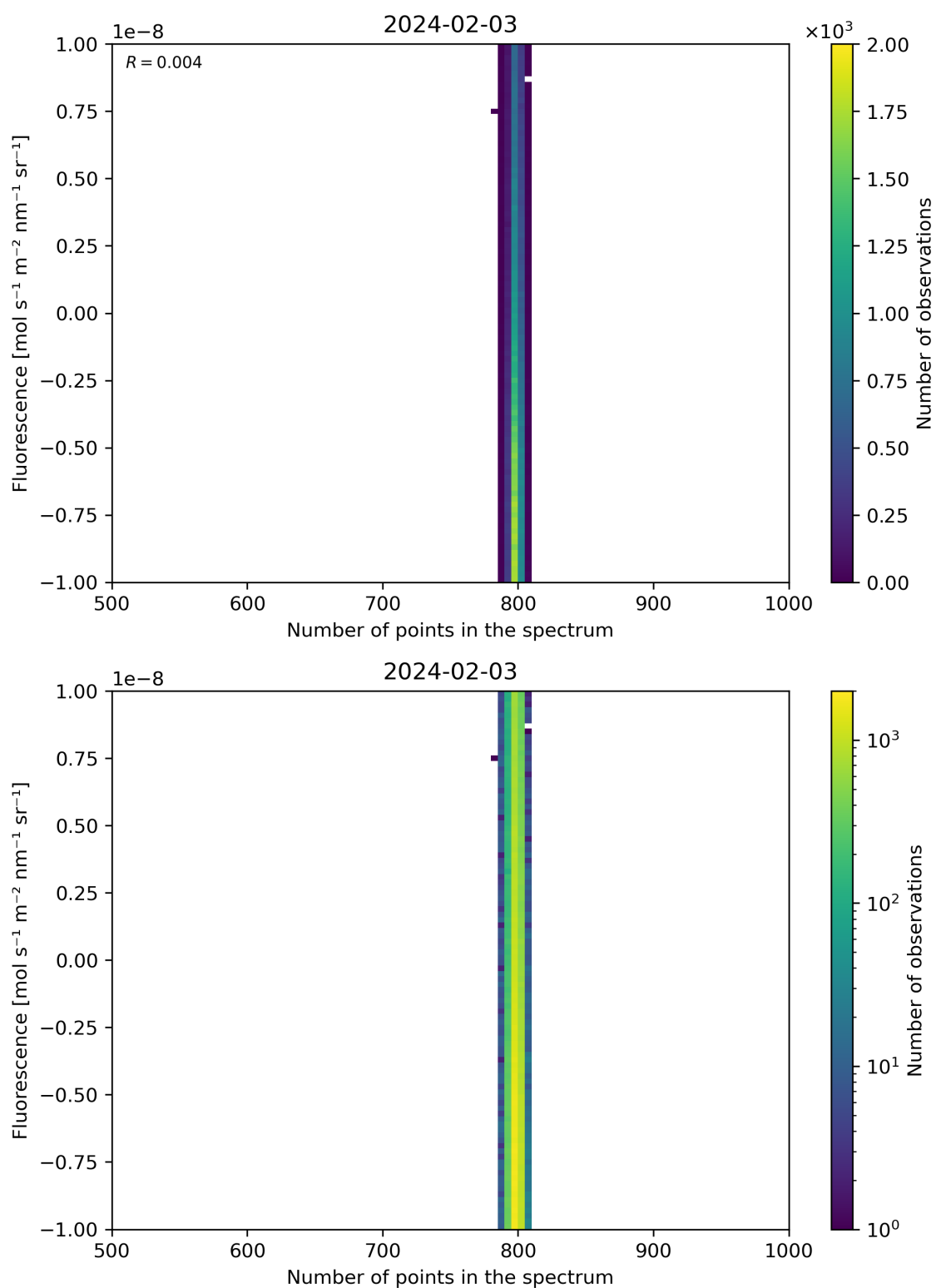
Figure 91: Scatter density plot of “Number of points in the spectrum” against “Fluorescence” for 2024-02-02 to 2024-02-04.
