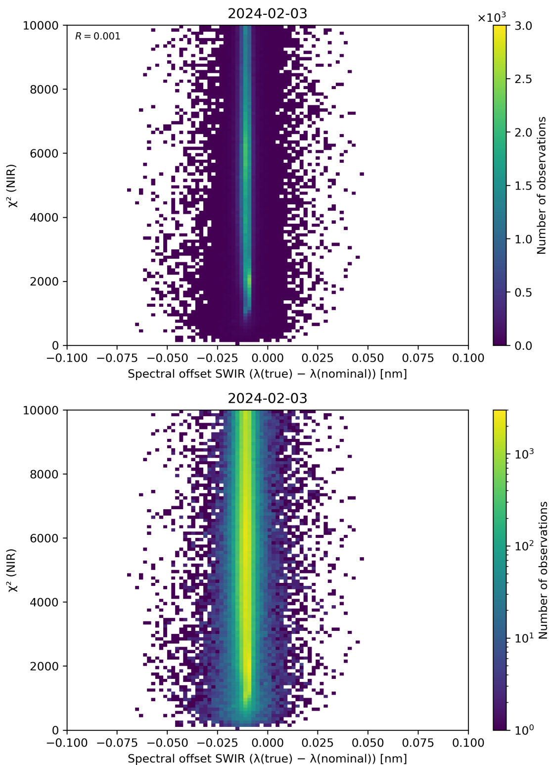
Figure 117: Scatter density plot of “Spectral offset SWIR ( \lambda(\text{true}) - \lambda(\text{nominal}) )” against “ \chi^2 (NIR)” for 2024-02-02 to 2024-02-04.
