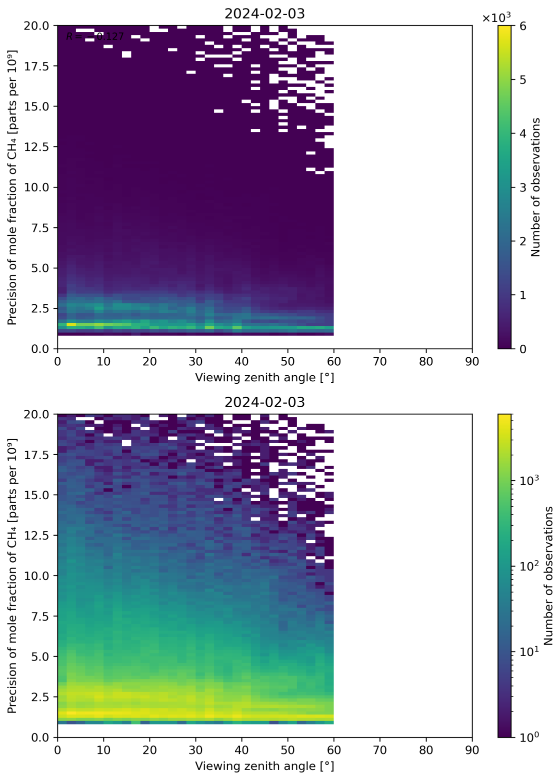
Figure 112: Scatter density plot of “Viewing zenith angle” against “Precision of mole fraction of CH 4 ” for 2024-02-02 to 2024-02-04.
