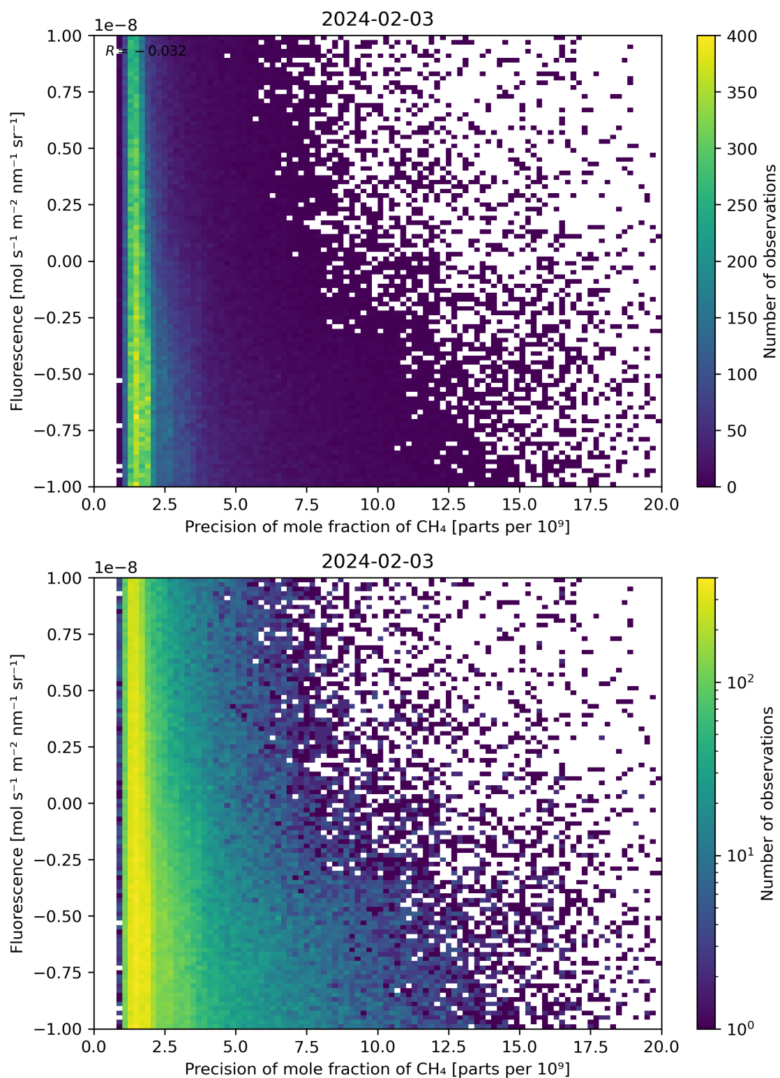
Figure 81: Scatter density plot of “Precision of mole fraction of \text{CH}_4 ” against “Fluorescence” for 2024-02-02 to 2024-02-04.
