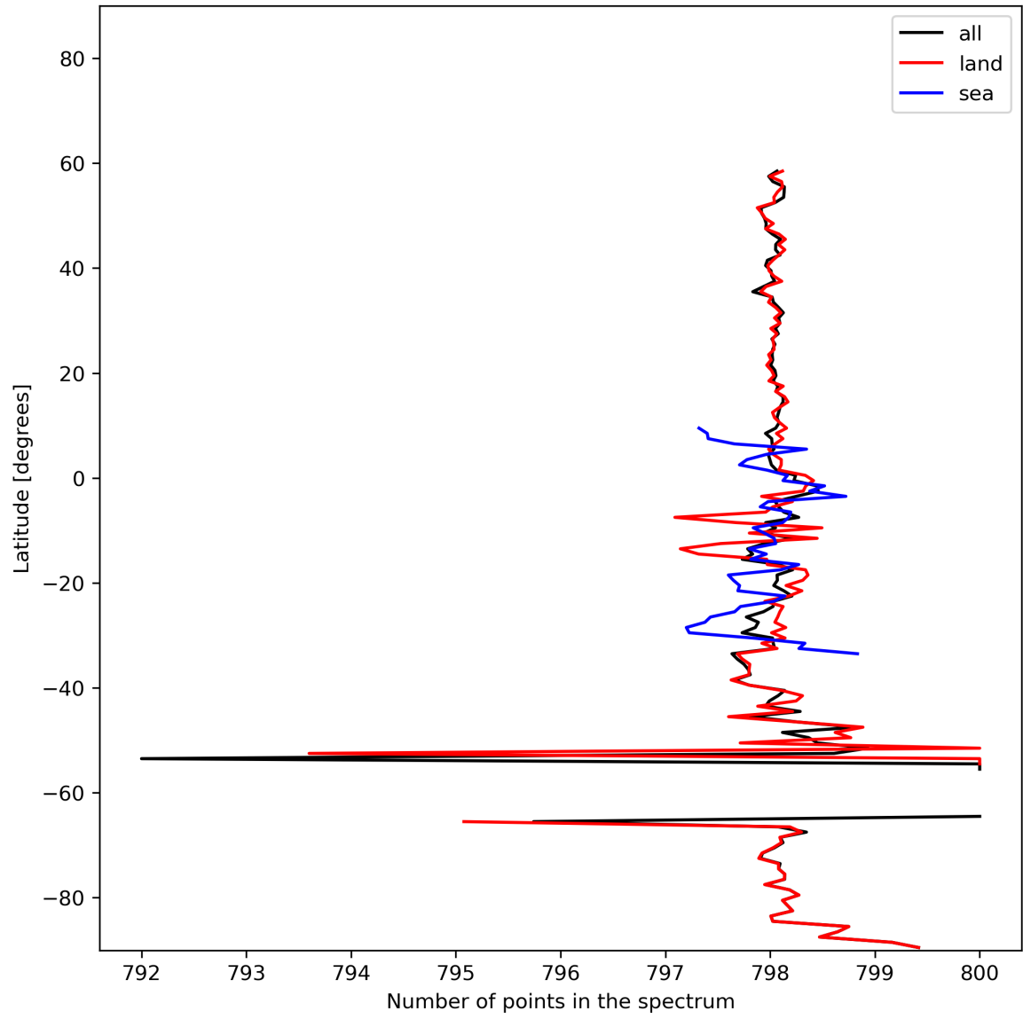
Figure 15: Zonal average of “Number of points in the spectrum” for 2024-02-02 to 2024-02-04.
