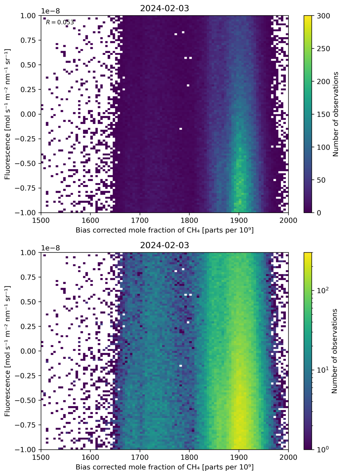
Figure 66: Scatter density plot of “Bias corrected mole fraction of \text{CH}_4 ” against “Fluorescence” for 2024-02-02 to 2024-02-04.
