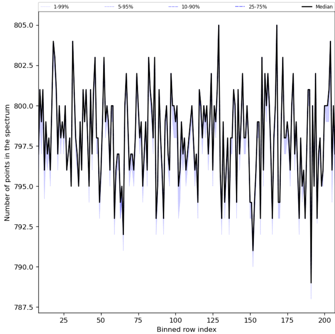
Figure 37: Along track statistics of “Number of points in the spectrum” for 2024-02-02 to 2024-02-04
