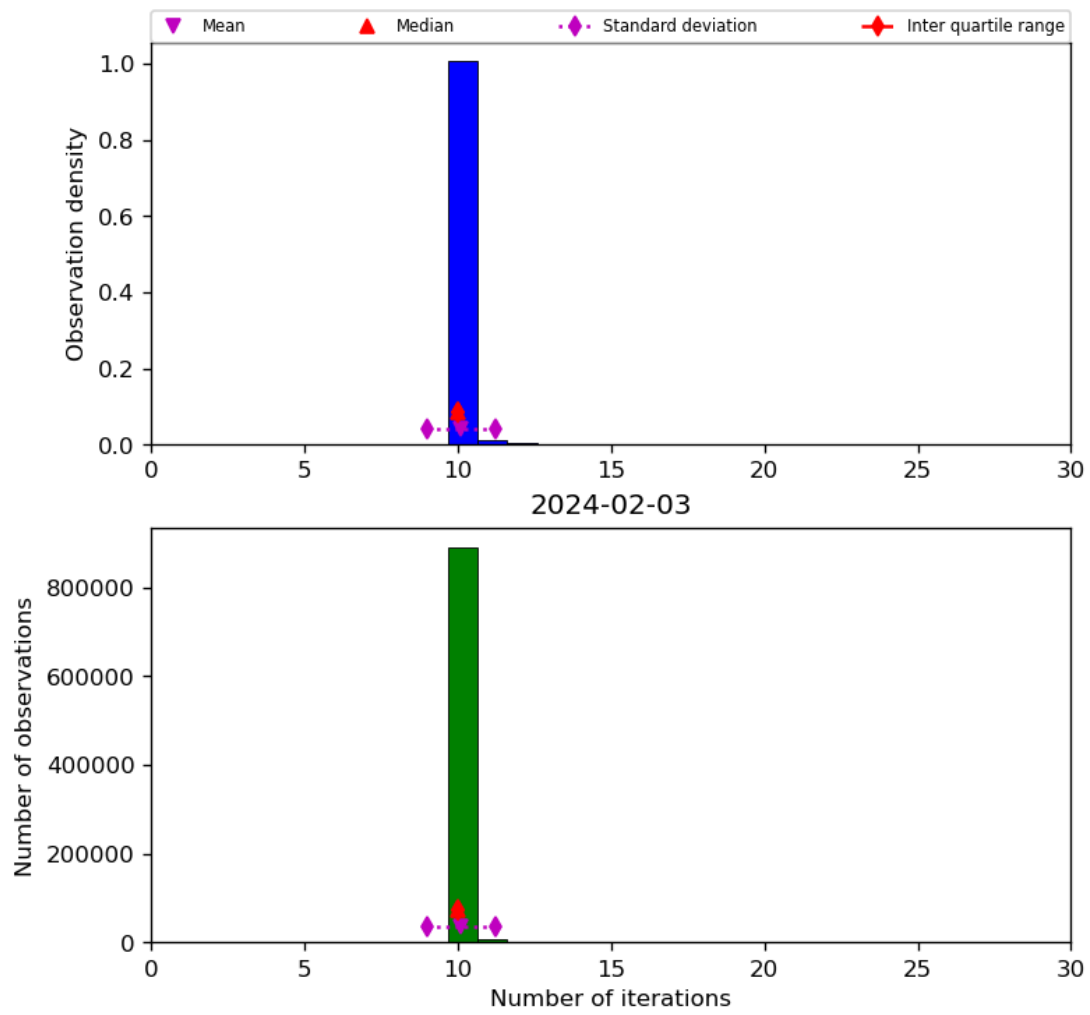
Figure 31: Histogram of “Number of iterations” for 2024-02-02 to 2024-02-04
