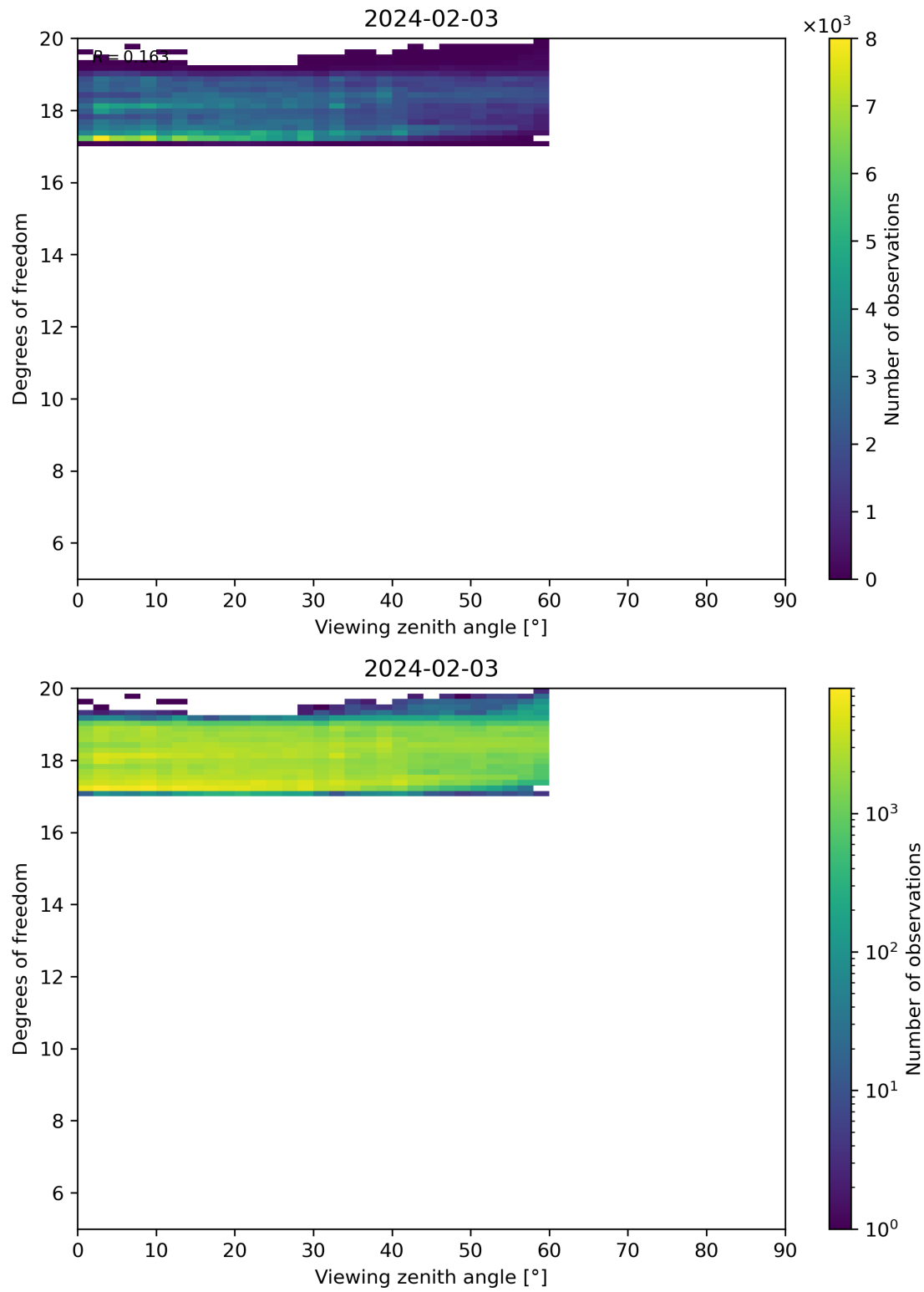
Figure 107: Scatter density plot of “Viewing zenith angle” against “Degrees of freedom” for 2024-02-02 to 2024-02-04.
