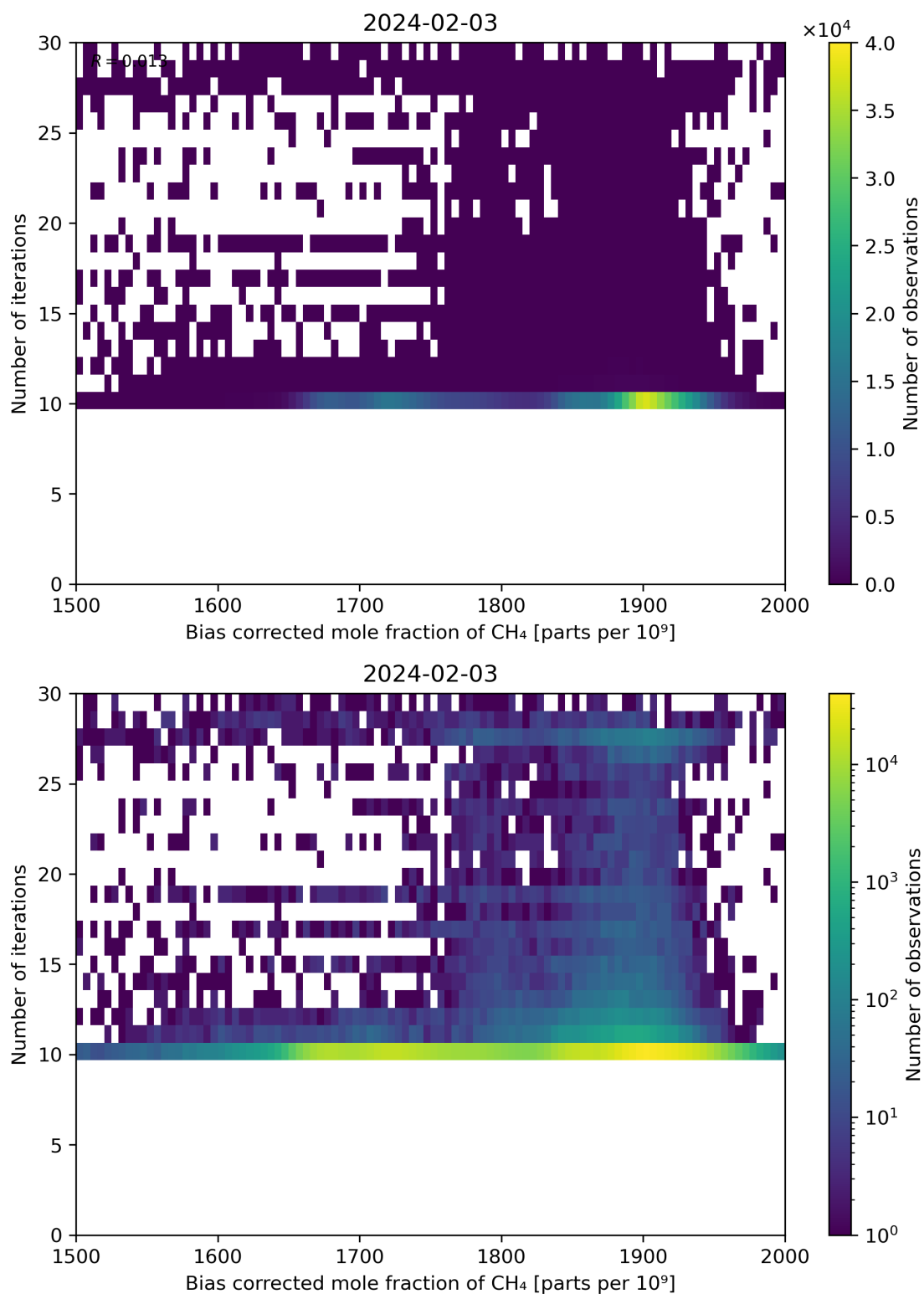
Figure 67: Scatter density plot of “Bias corrected mole fraction of \text{CH}_4 ” against “Number of iterations” for 2024-02-02 to 2024-02-04.
