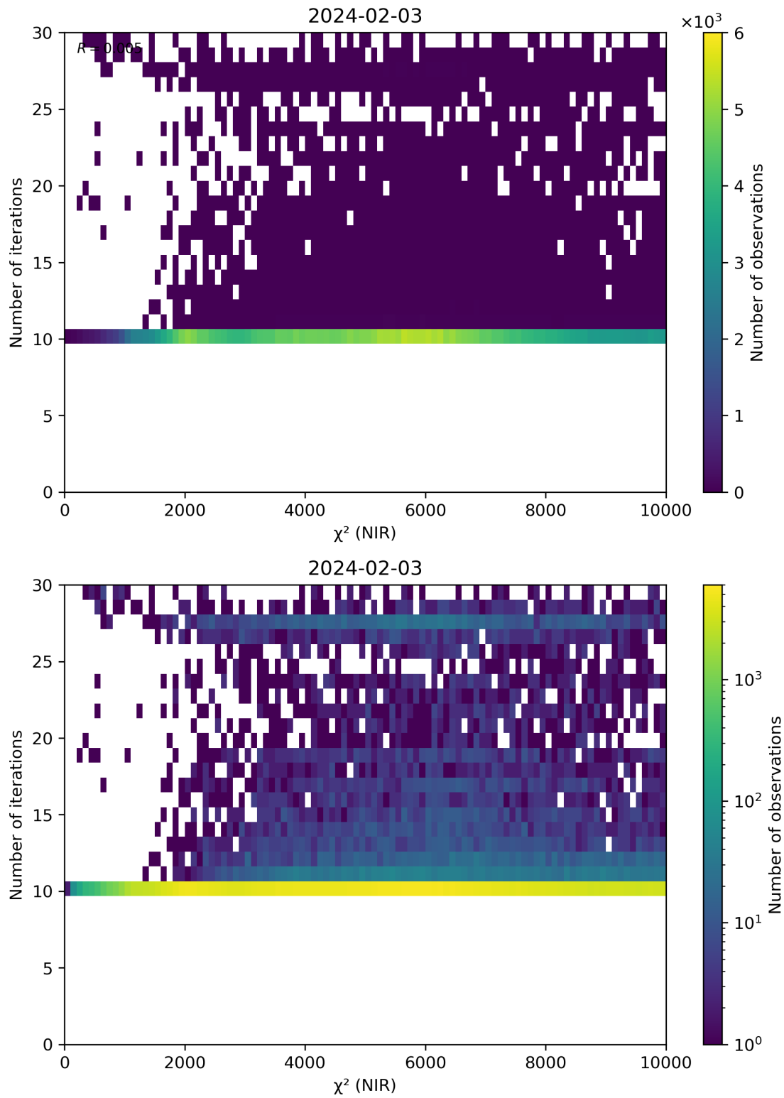
Figure 46: Scatter density plot of “ \chi^2 (NIR)” against “Number of iterations” for 2024-02-02 to 2024-02-04.
