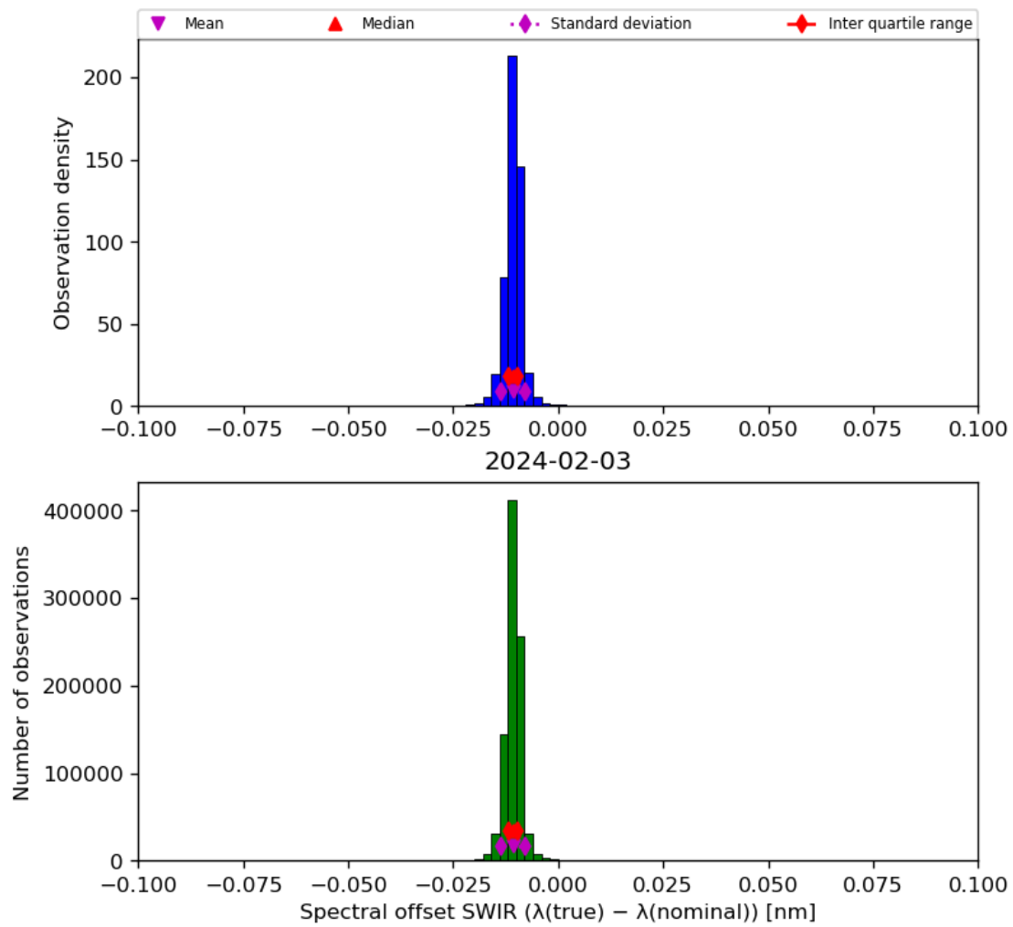
Figure 27: Histogram of “Spectral offset SWIR ( \lambda(\text{true}) - \lambda(\text{nominal}) )” for 2024-02-02 to 2024-02-04
