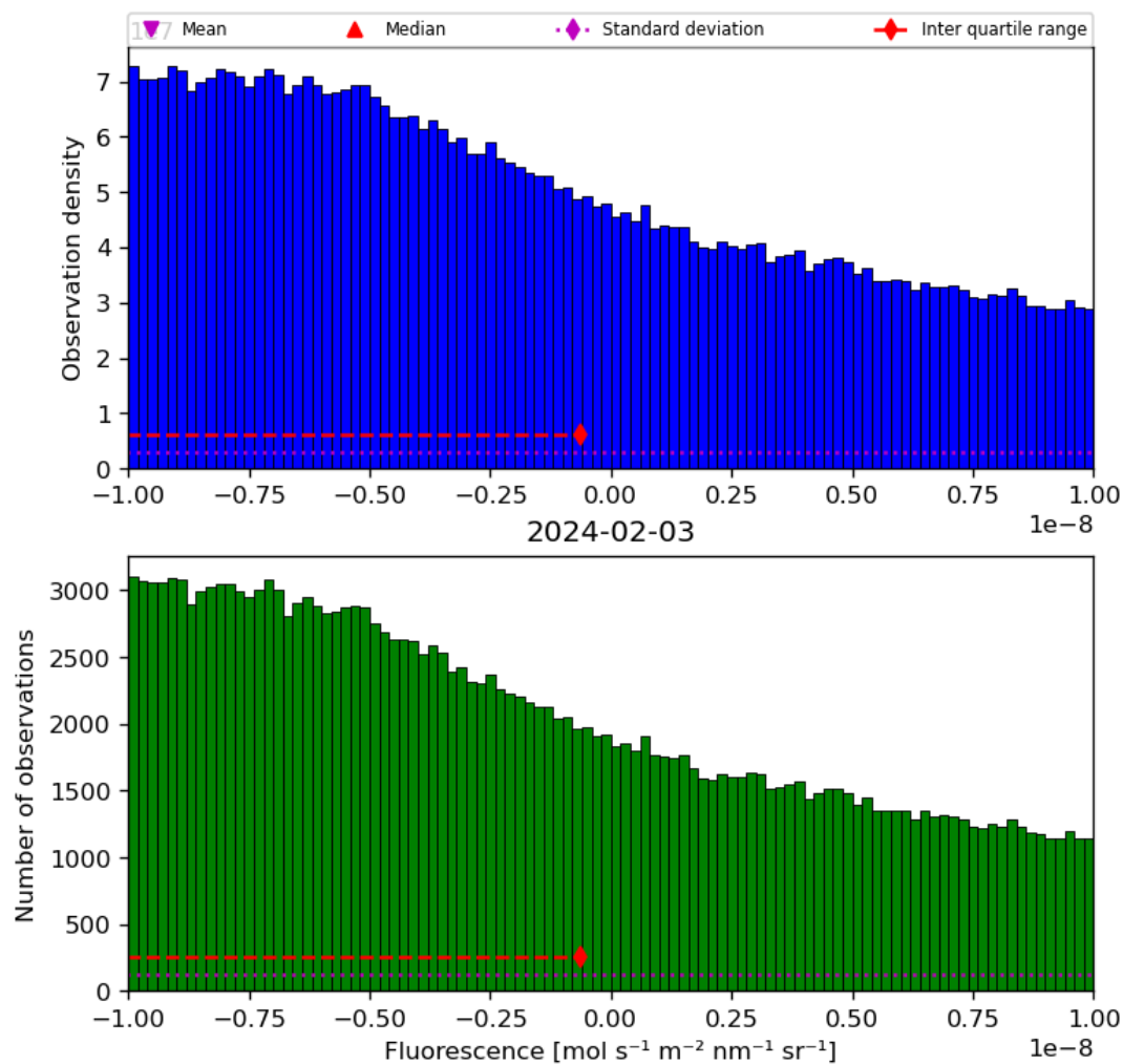
Figure 32: Histogram of “Fluorescence” for 2024-02-02 to 2024-02-04
