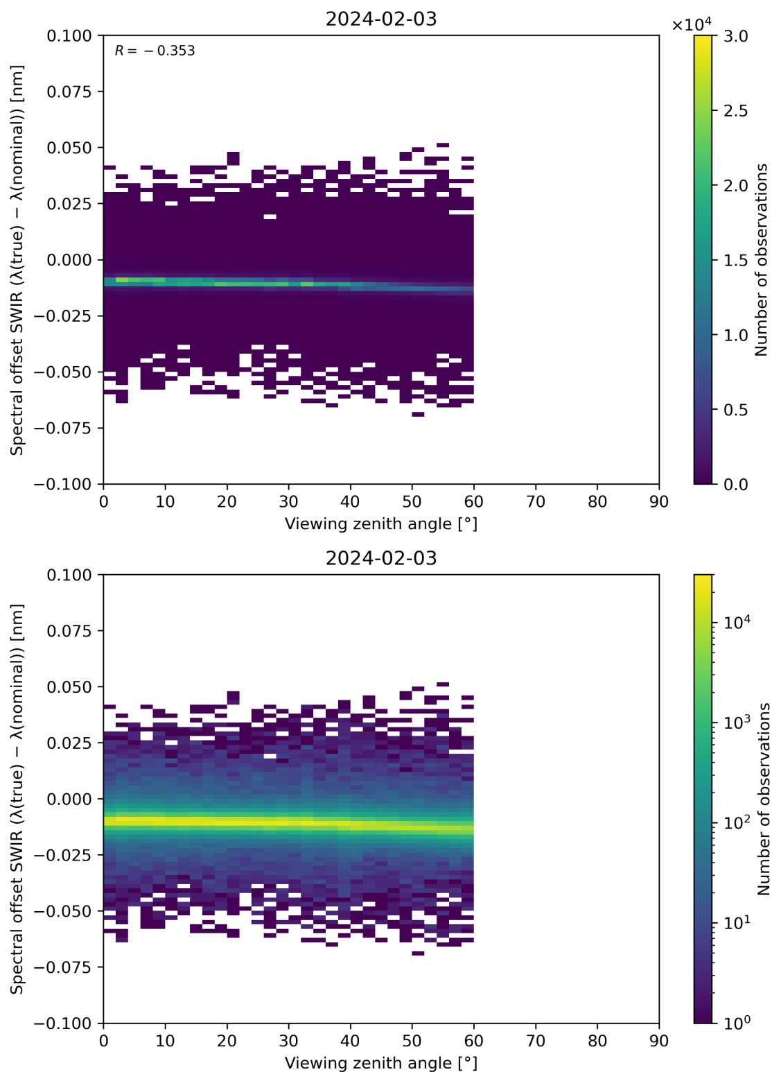
Figure 116: Scatter density plot of “Viewing zenith angle” against “Spectral offset SWIR ( \lambda(\text{true}) - \lambda(\text{nominal}) )” for 2024-02-02 to 2024-02-04.
