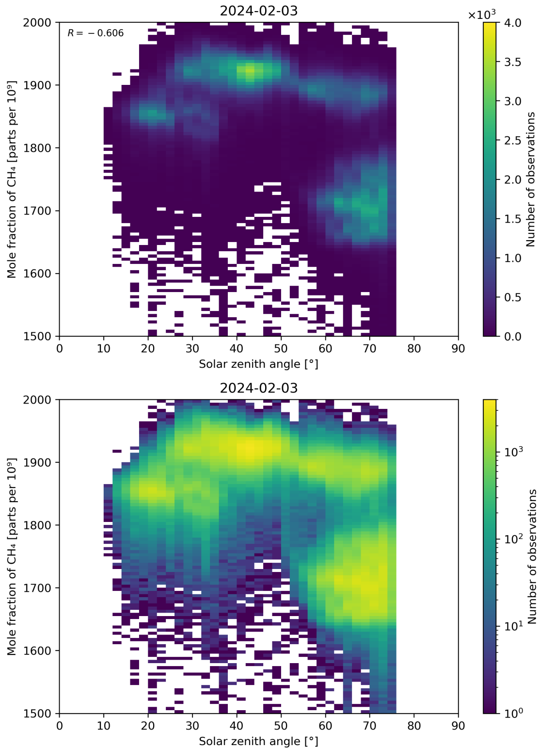
Figure 99: Scatter density plot of “Solar zenith angle” against “Mole fraction of CH 4 ” for 2024-02-02 to 2024-02-04.
