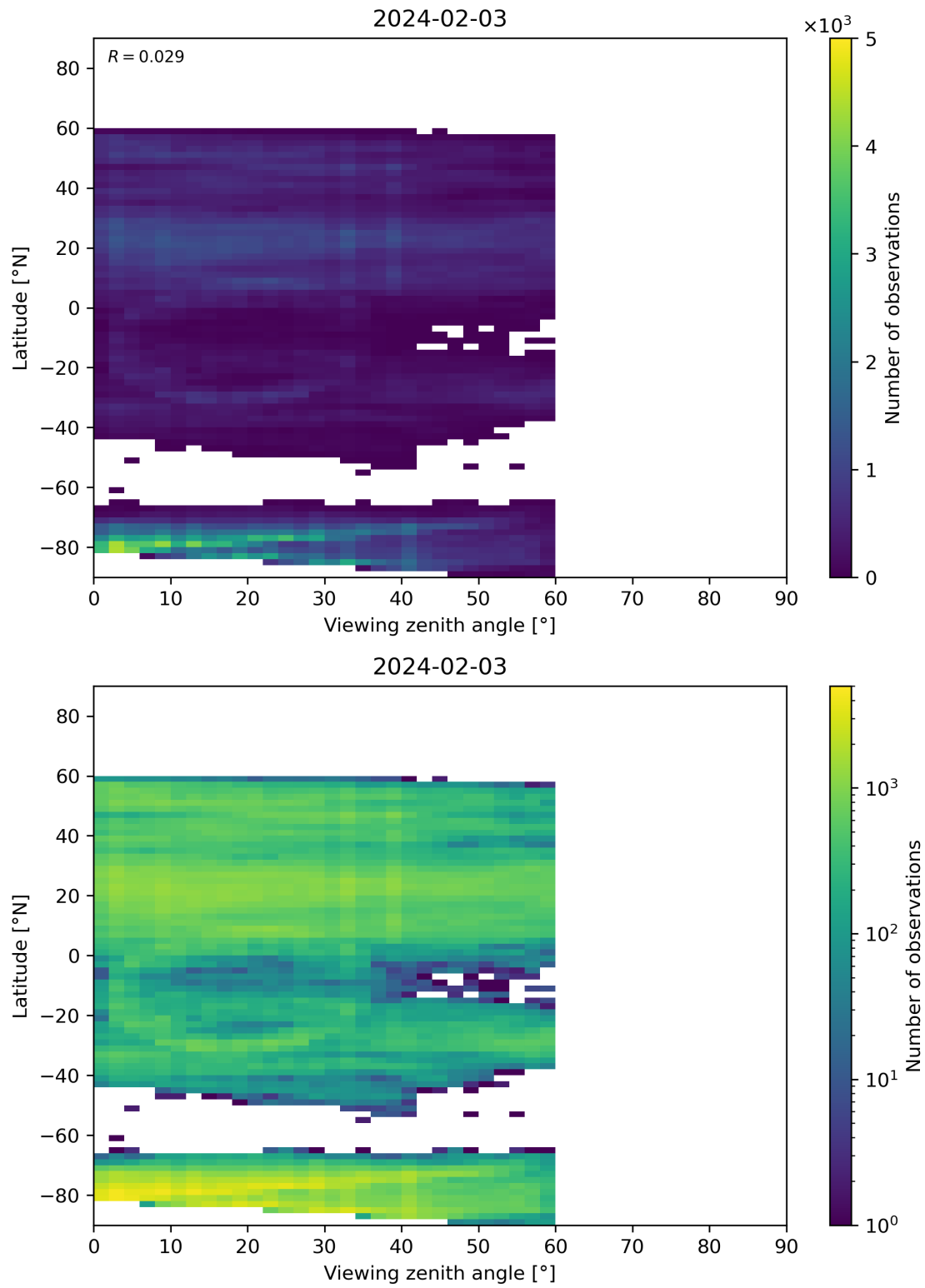
Figure 109: Scatter density plot of “Viewing zenith angle” against “Latitude” for 2024-02-02 to 2024-02-04.
