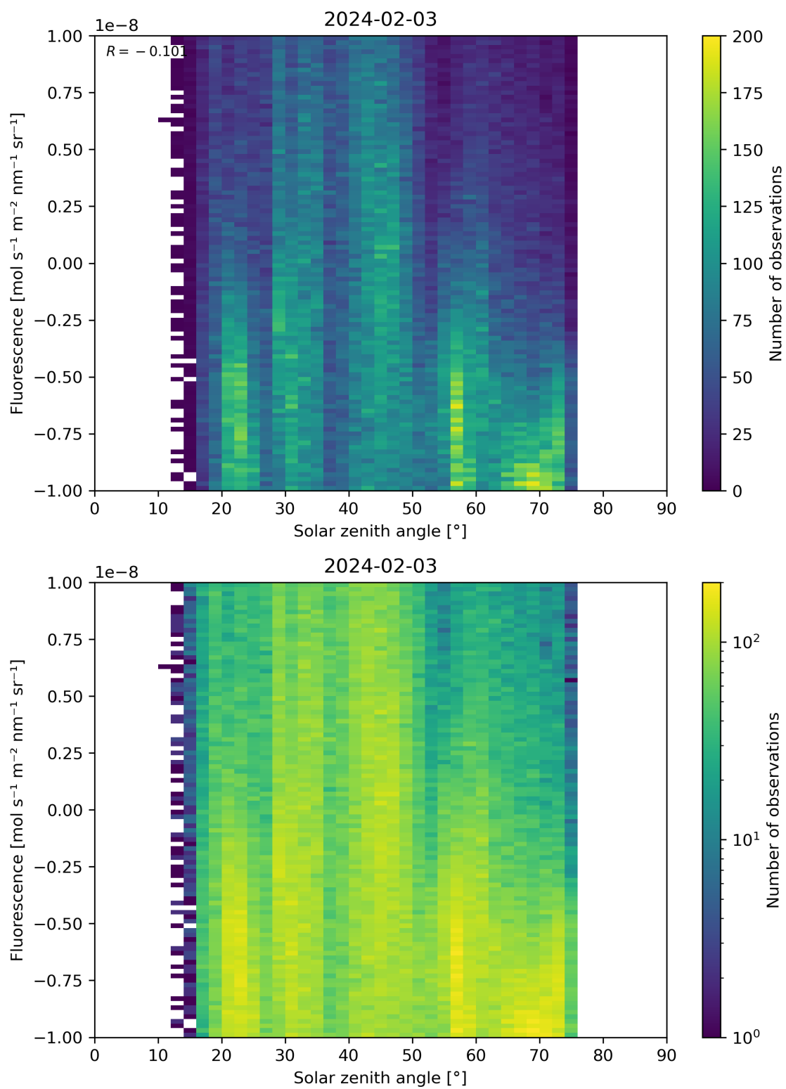
Figure 97: Scatter density plot of “Solar zenith angle” against “Fluorescence” for 2024-02-02 to 2024-02-04.
