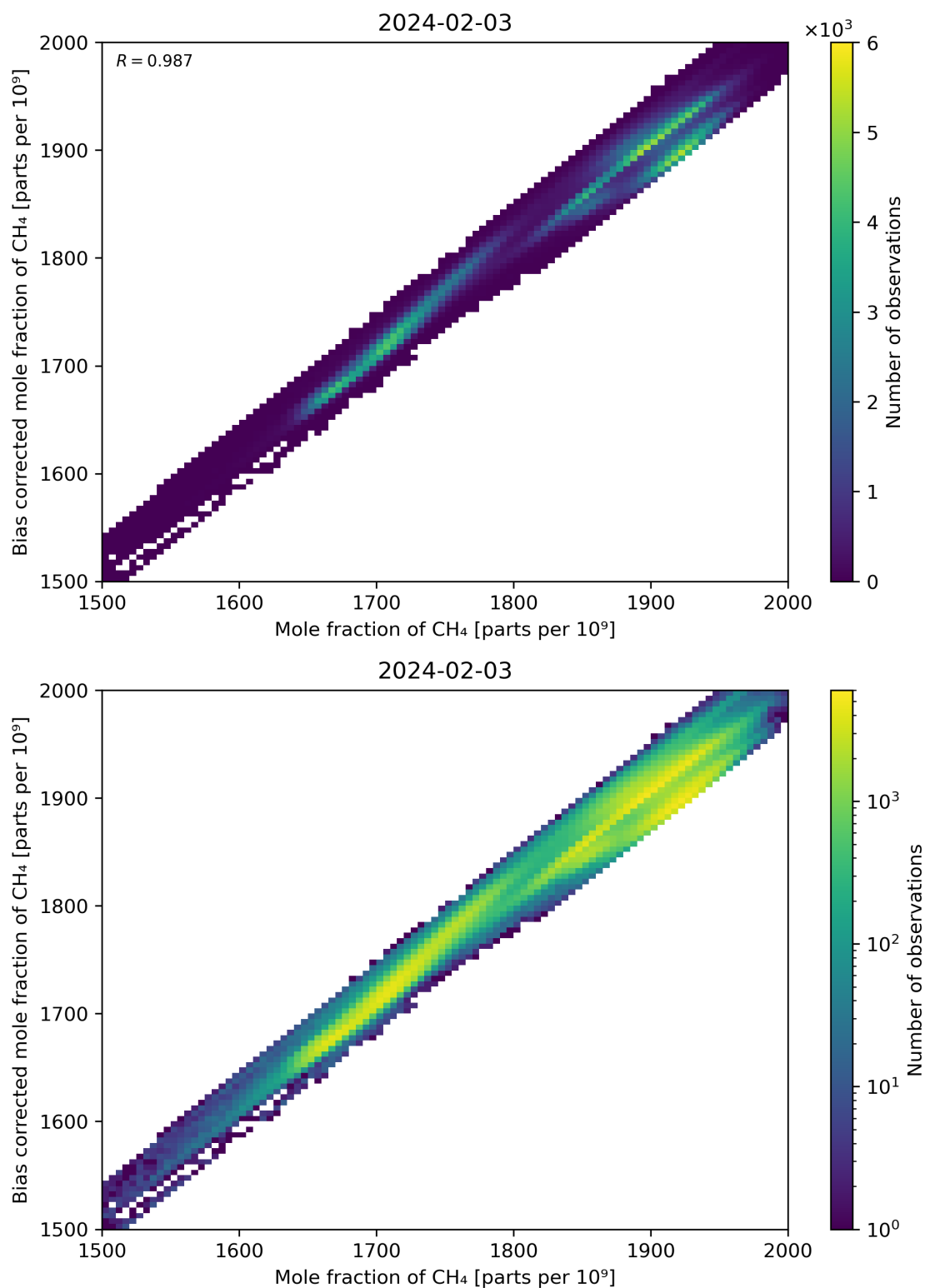
Figure 74: Scatter density plot of “Mole fraction of CH 4 ” against “Bias corrected mole fraction of CH 4 ” for 2024-02-02 to 2024-02-04.
