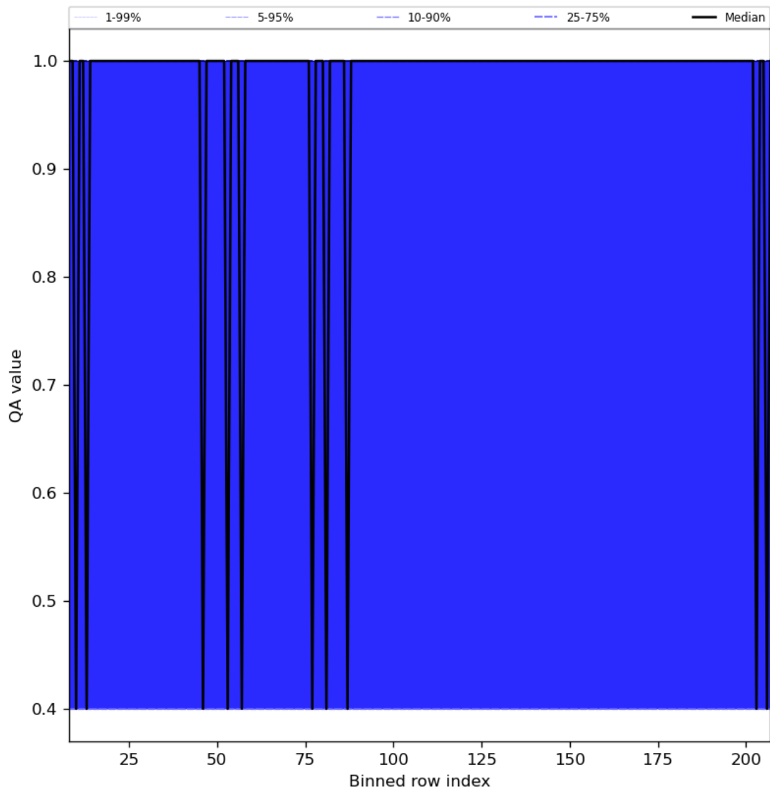
Figure 33: Along track statistics of “QA value” for 2024-02-02 to 2024-02-04
