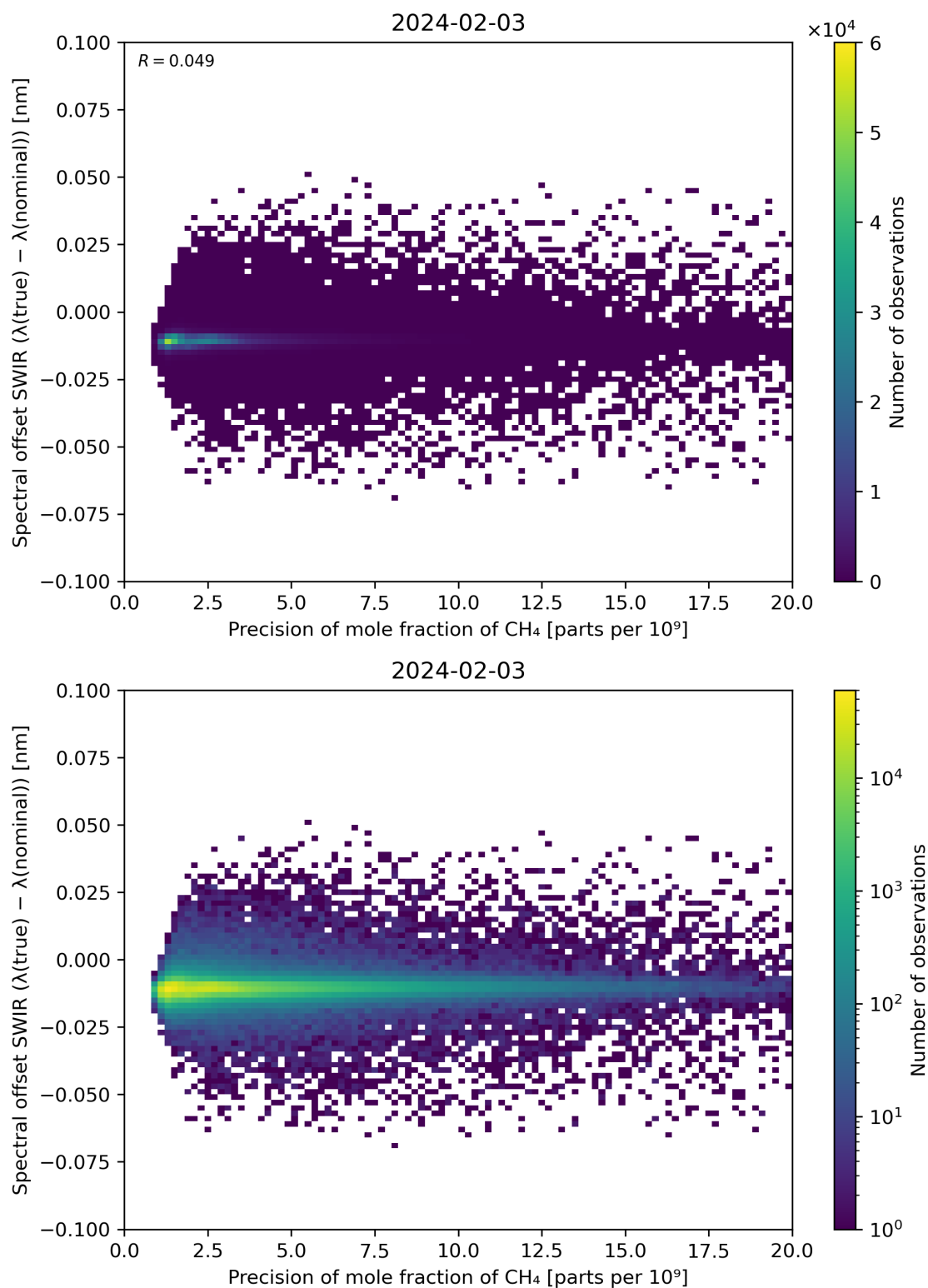
Figure 85: Scatter density plot of “Precision of mole fraction of CH 4 ” against “Spectral offset SWIR ( \lambda(\text{true}) - \lambda(\text{nominal}) )” for 2024-02-02 to 2024-02-04.
