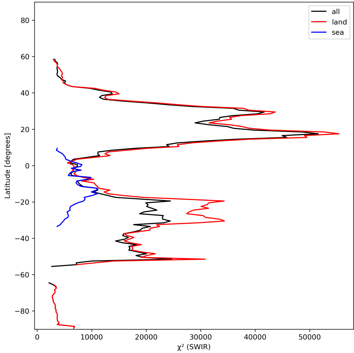
Figure 17: Zonal average of “ \chi^2 (SWIR)” for 2024-02-02 to 2024-02-04.
