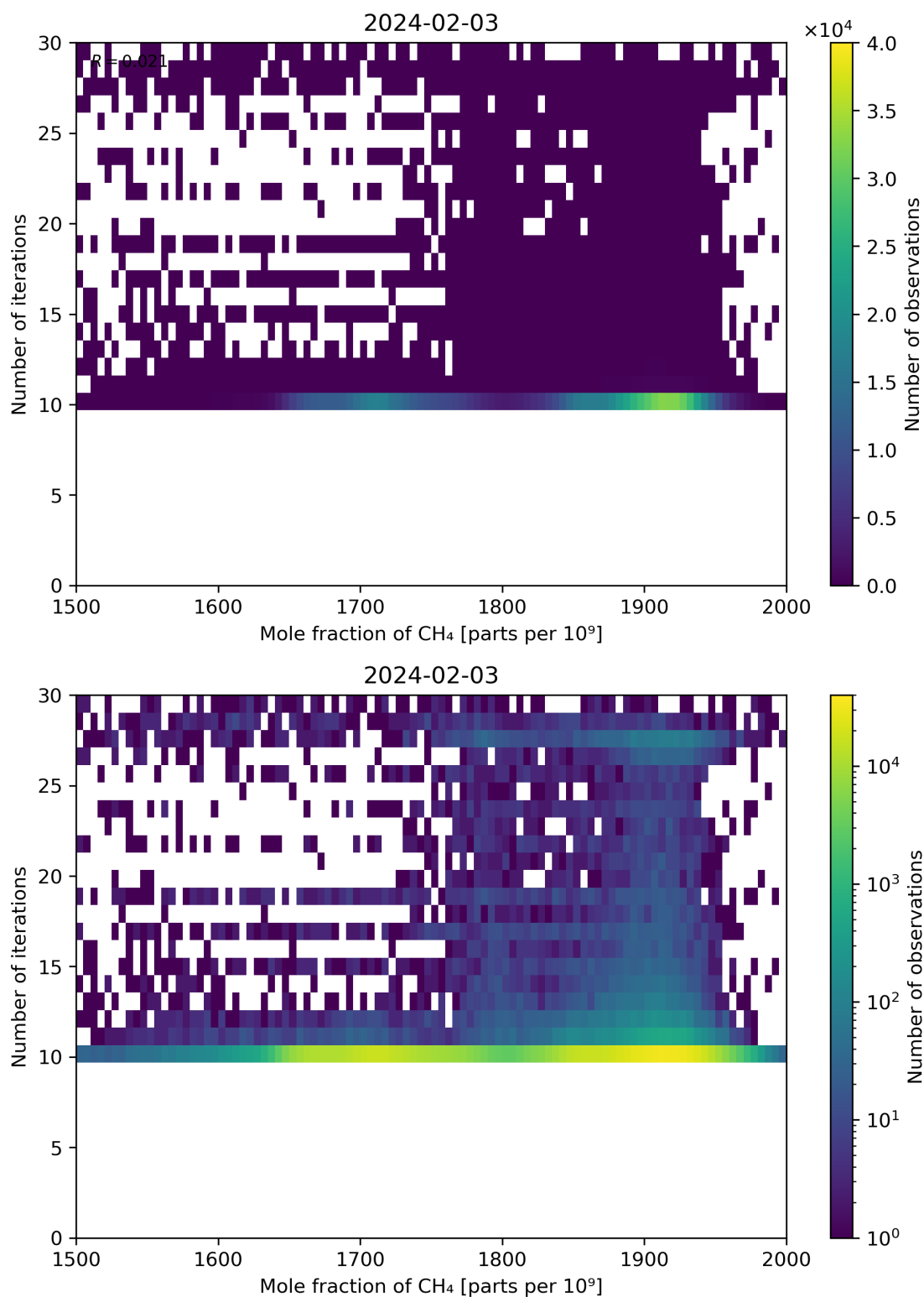
Figure 76: Scatter density plot of “Mole fraction of CH 4 ” against “Number of iterations” for 2024-02-02 to 2024-02-04.
