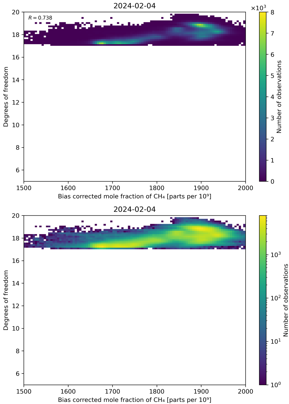
Figure 65: Scatter density plot of “Bias corrected mole fraction of CH 4 ” against “Degrees of freedom” for 2024-02-03 to 2024-02-05.
