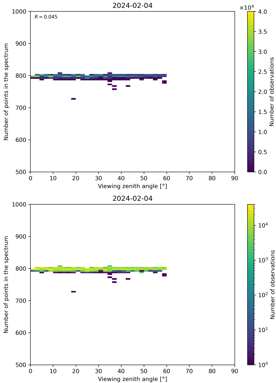
Figure 114: Scatter density plot of “Viewing zenith angle” against “Number of points in the spectrum” for 2024-02-03 to 2024-02-05.
