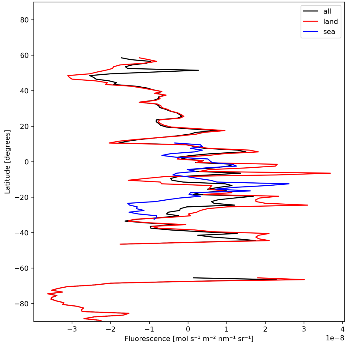
Figure 21: Zonal average of “Fluorescence” for 2024-02-03 to 2024-02-05.
