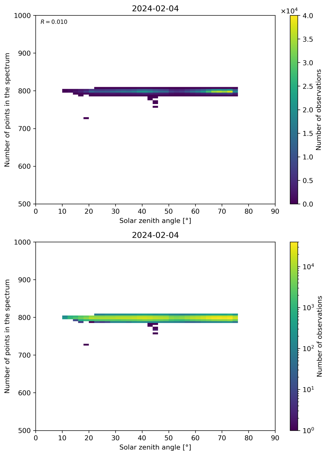
Figure 103: Scatter density plot of “Solar zenith angle” against “Number of points in the spectrum” for 2024-02-03 to 2024-02-05.
