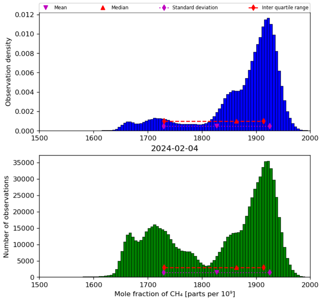
Figure 23: Histogram of “Mole fraction of CH 4 ” for 2024-02-03 to 2024-02-05
