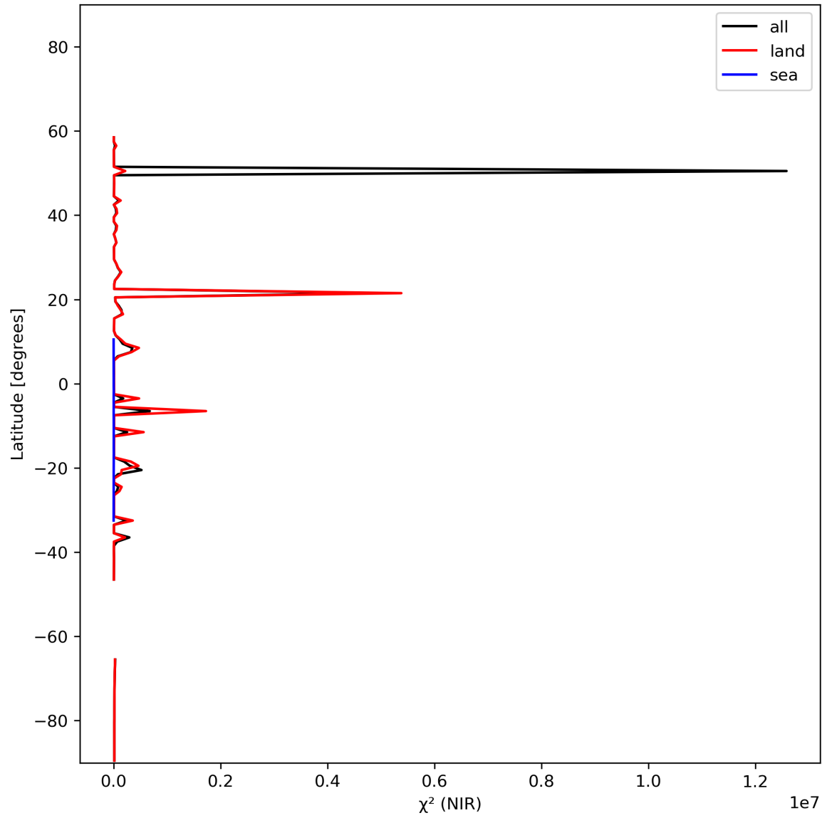
Figure 18: Zonal average of “ \chi^2 (NIR)” for 2024-02-03 to 2024-02-05.
