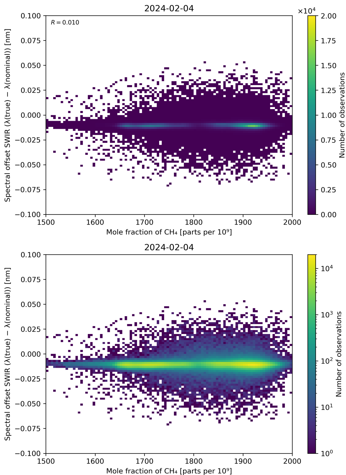
Figure 86: Scatter density plot of “Mole fraction of \text{CH}_4 ” against “Spectral offset SWIR ( \lambda(\text{true}) - \lambda(\text{nominal}) )” for 2024-02-03 to 2024-02-05.
