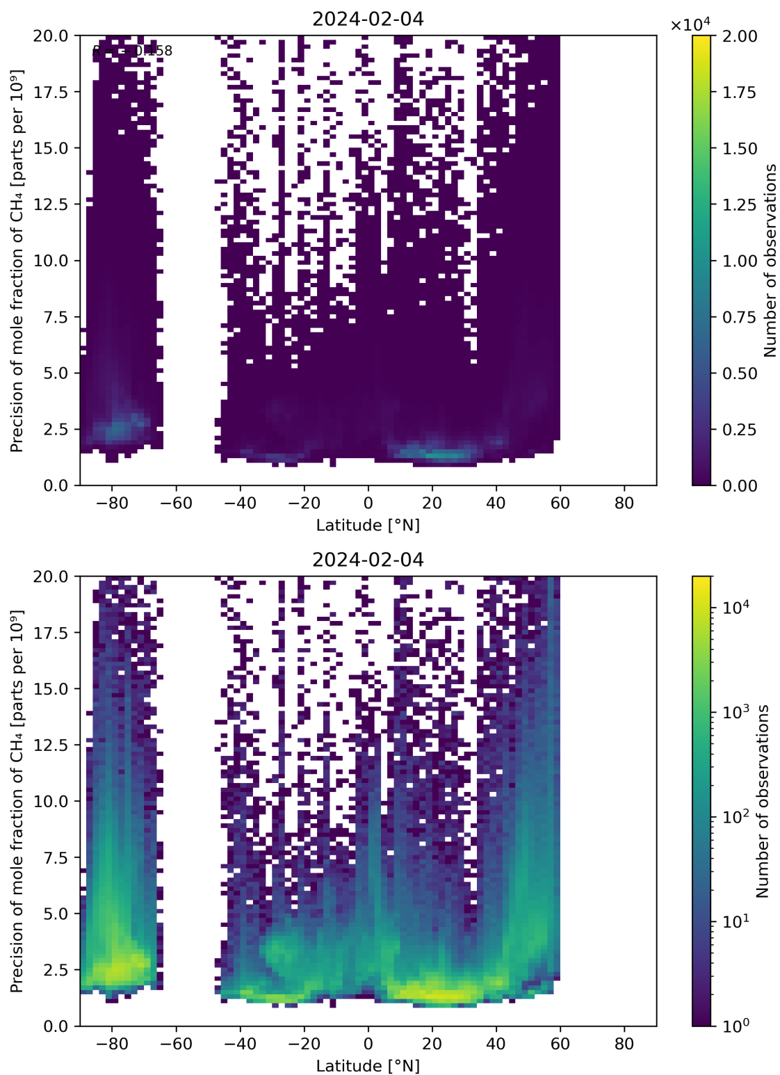
Figure 59: Scatter density plot of “Latitude” against “Precision of mole fraction of CH 4 ” for 2024-02-03 to 2024-02-05.
