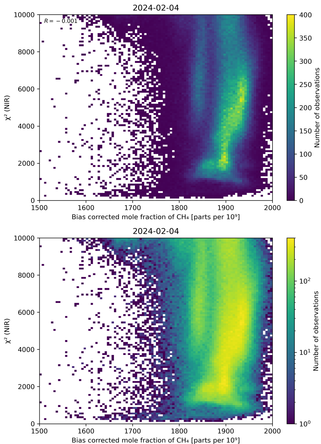
Figure 63: Scatter density plot of “Bias corrected mole fraction of CH 4 ” against “ \chi^2 (NIR)” for 2024-02-03 to 2024-02-05.
