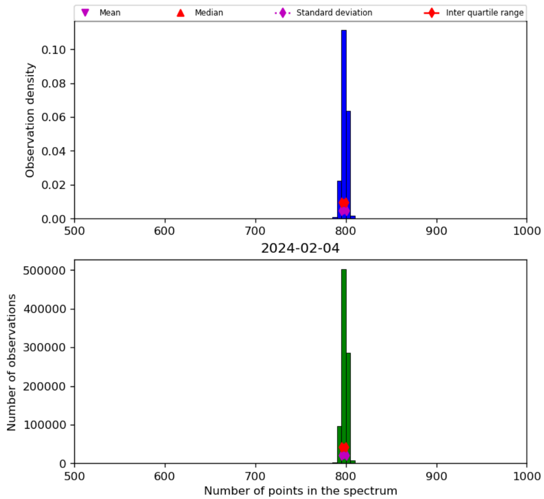
Figure 26: Histogram of “Number of points in the spectrum” for 2024-02-03 to 2024-02-05
