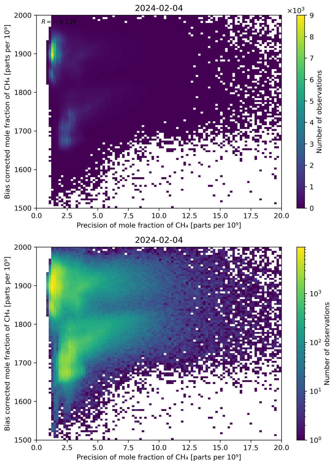
Figure 82: Scatter density plot of “Precision of mole fraction of CH 4 ” against “Bias corrected mole fraction of CH 4 ” for 2024-02-03 to 2024-02-05.
