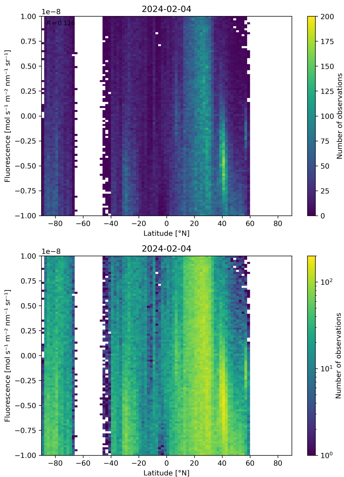
Figure 56: Scatter density plot of “Latitude” against “Fluorescence” for 2024-02-03 to 2024-02-05.
