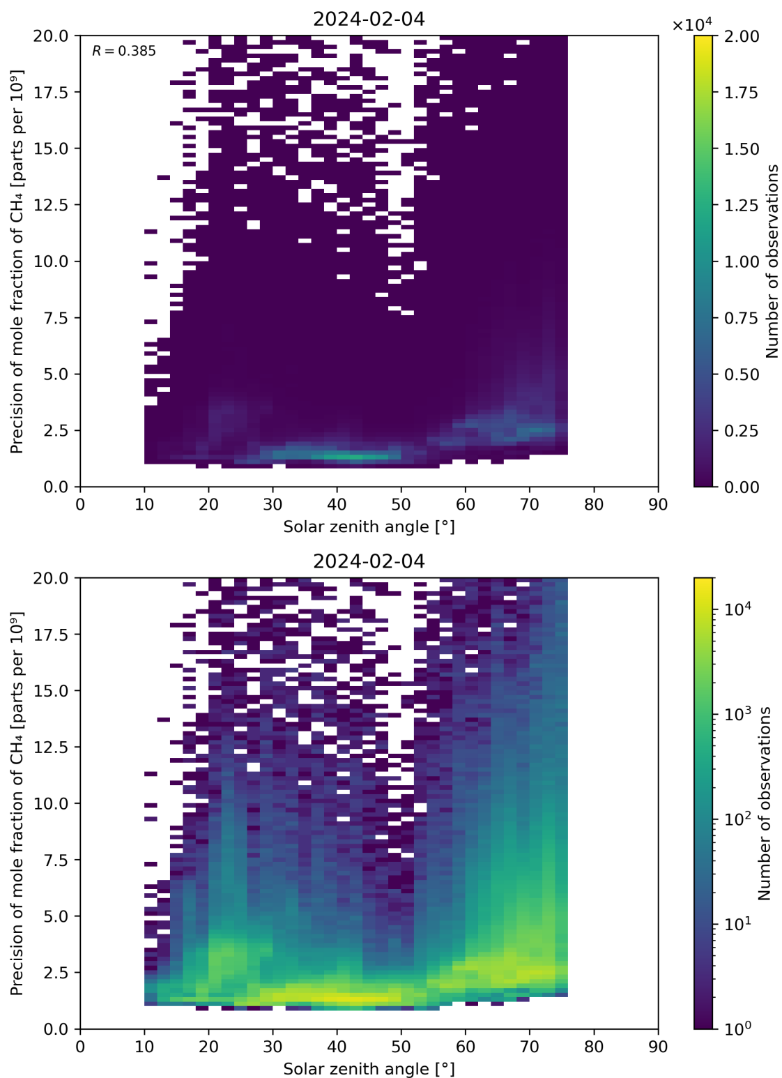
Figure 101: Scatter density plot of “Solar zenith angle” against “Precision of mole fraction of CH 4 ” for 2024-02-03 to 2024-02-05.
