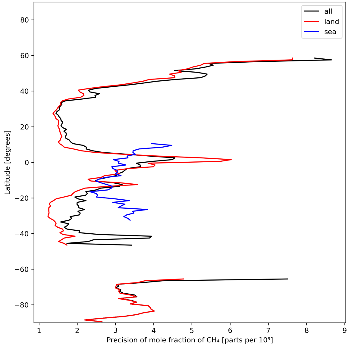
Figure 13: Zonal average of “Precision of mole fraction of CH 4 ” for 2024-02-03 to 2024-02-05.
