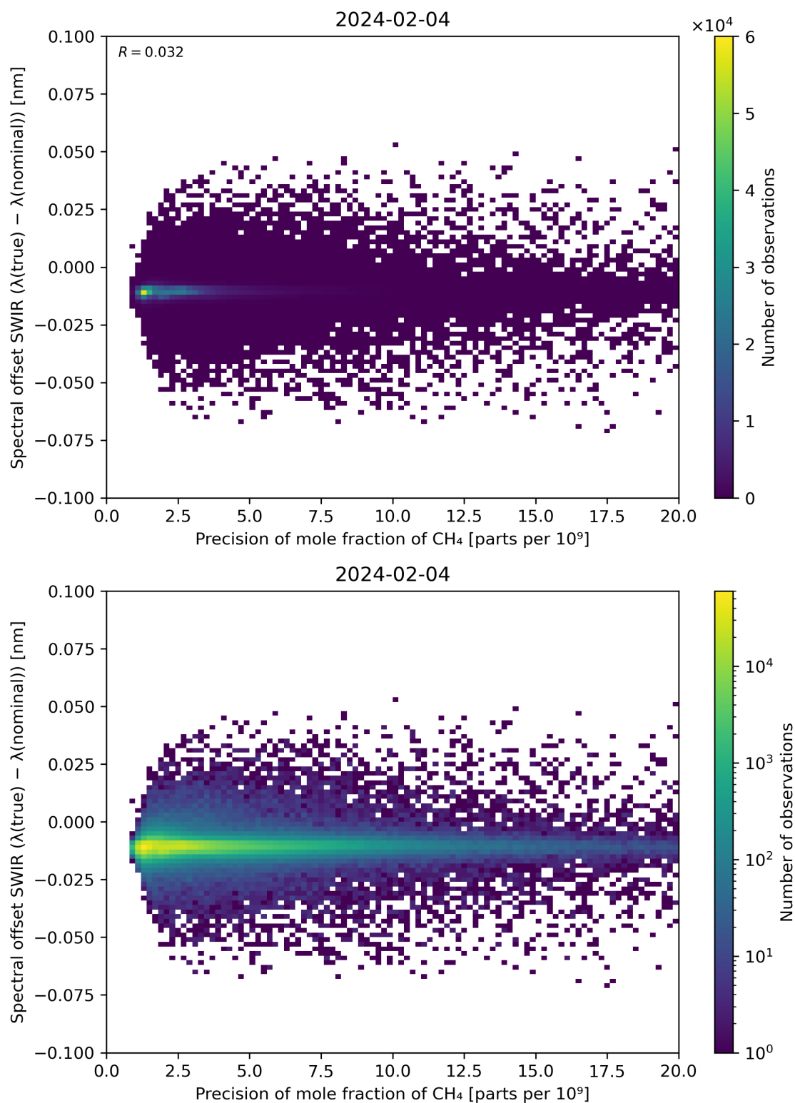
Figure 85: Scatter density plot of “Precision of mole fraction of \text{CH}_4 ” against “Spectral offset SWIR ( \lambda(\text{true}) - \lambda(\text{nominal}) )” for 2024-02-03 to 2024-02-05.
