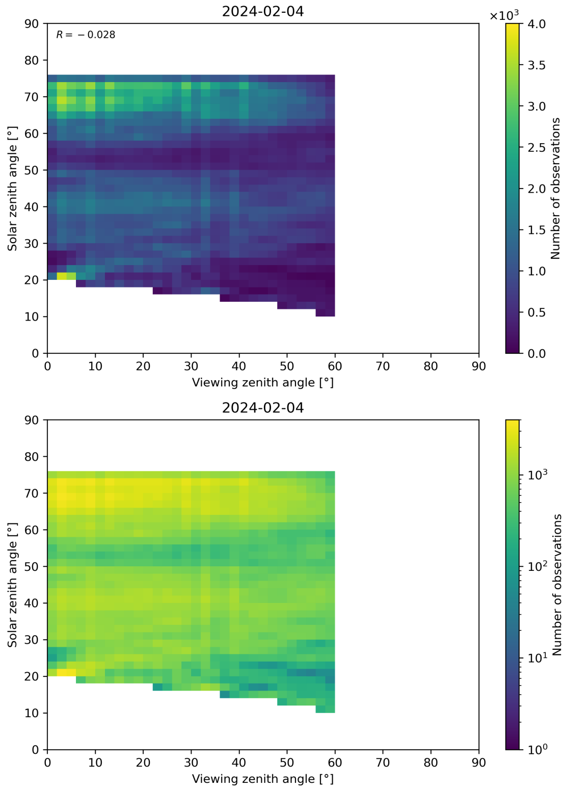
Figure 115: Scatter density plot of “Viewing zenith angle” against “Solar zenith angle” for 2024-02-03 to 2024-02-05.
