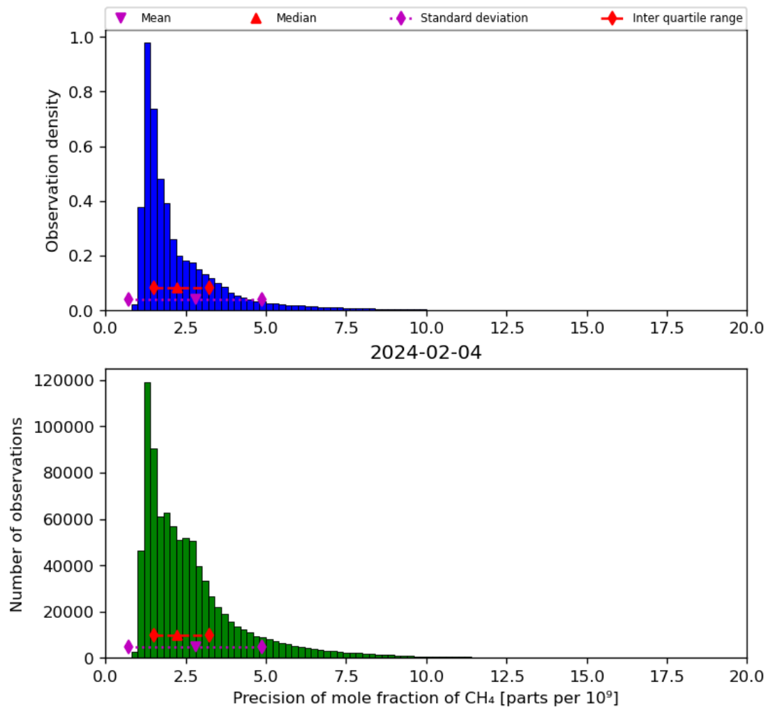
Figure 24: Histogram of “Precision of mole fraction of CH 4 ” for 2024-02-03 to 2024-02-05
