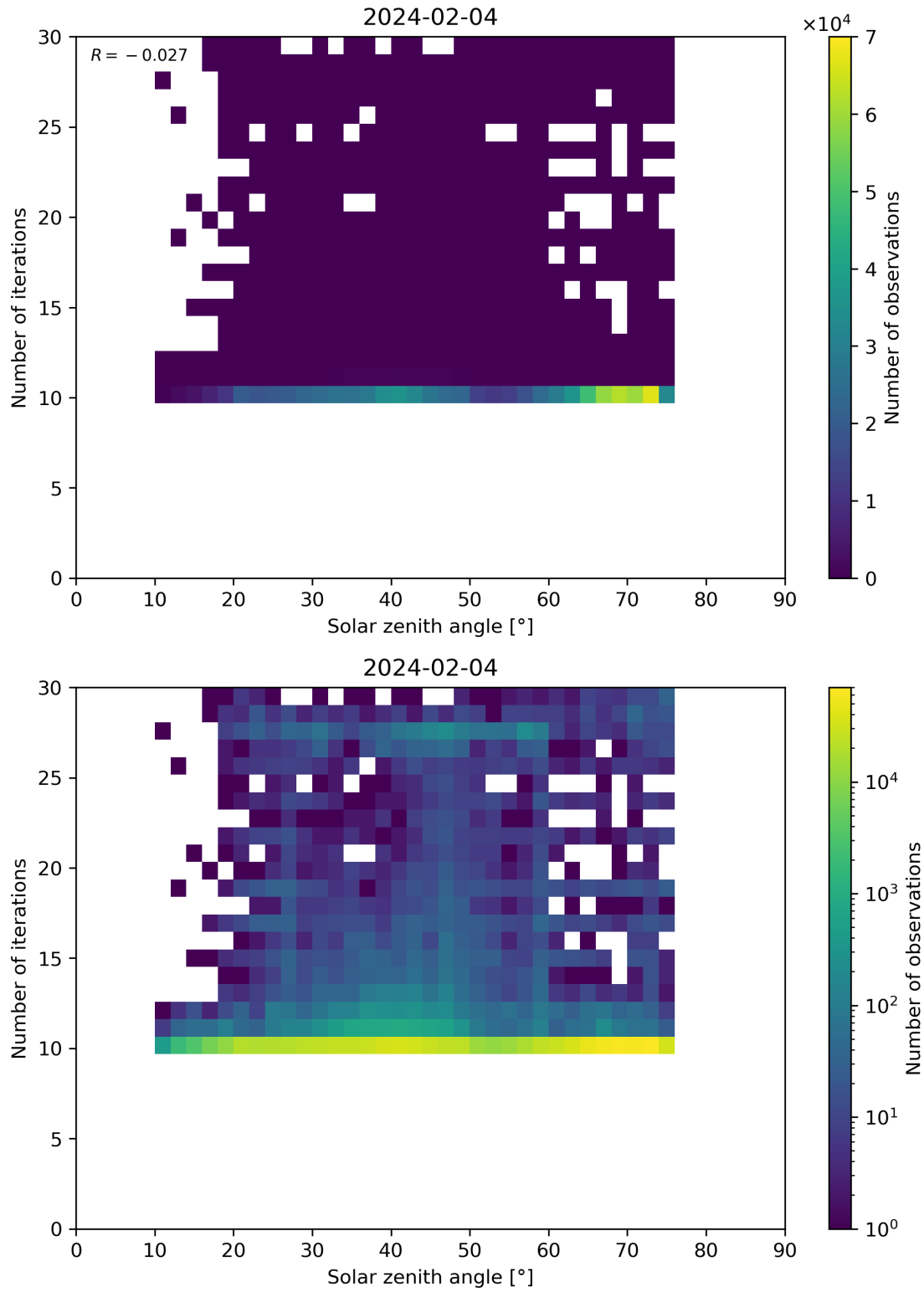
Figure 102: Scatter density plot of “Solar zenith angle” against “Number of iterations” for 2024-02-03 to 2024-02-05.
