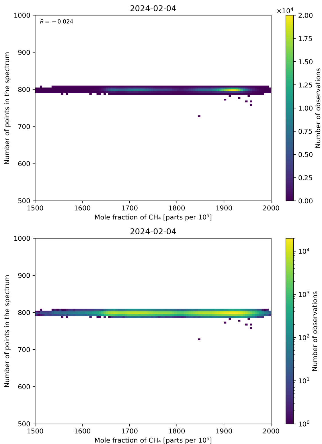
Figure 77: Scatter density plot of “Mole fraction of CH 4 ” against “Number of points in the spectrum” for 2024-02-03 to 2024-02-05.
