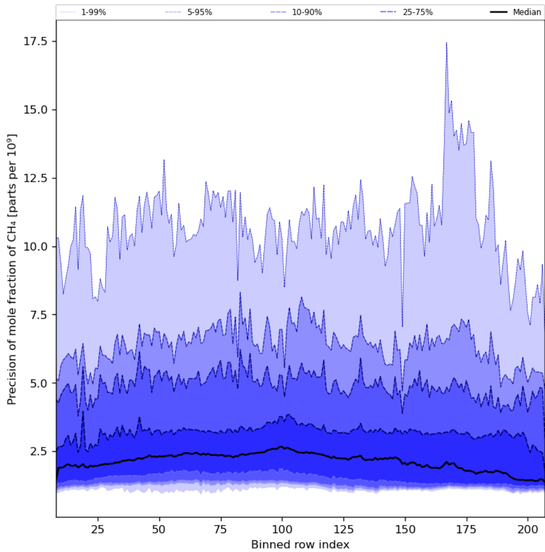
Figure 35: Along track statistics of “Precision of mole fraction of CH 4 ” for 2024-02-03 to 2024-02-05
