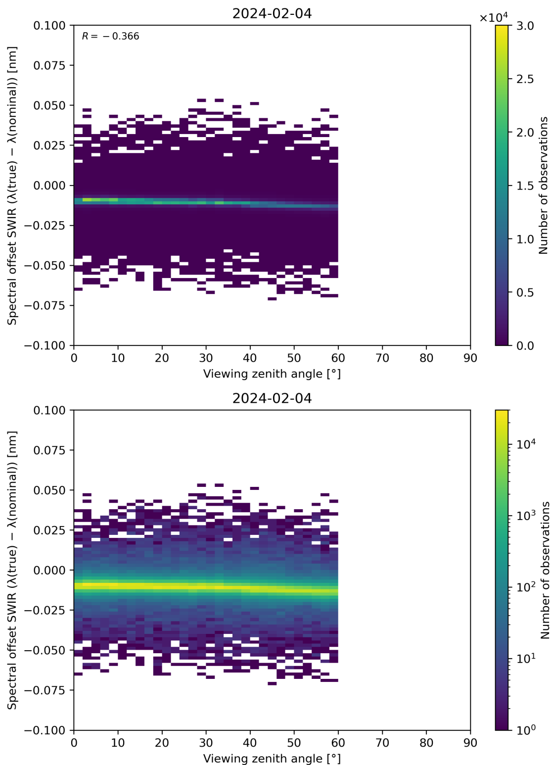
Figure 116: Scatter density plot of “Viewing zenith angle” against “Spectral offset SWIR ( \lambda(\text{true}) - \lambda(\text{nominal}) )” for 2024-02-03 to 2024-02-05.
