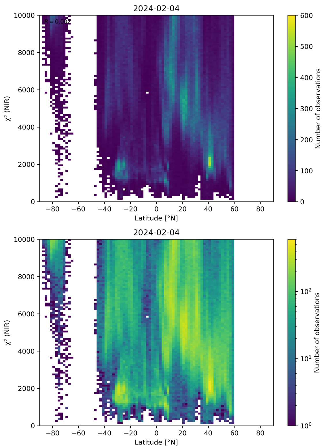
Figure 53: Scatter density plot of “Latitude” against “ \chi^2 (NIR)” for 2024-02-03 to 2024-02-05.
