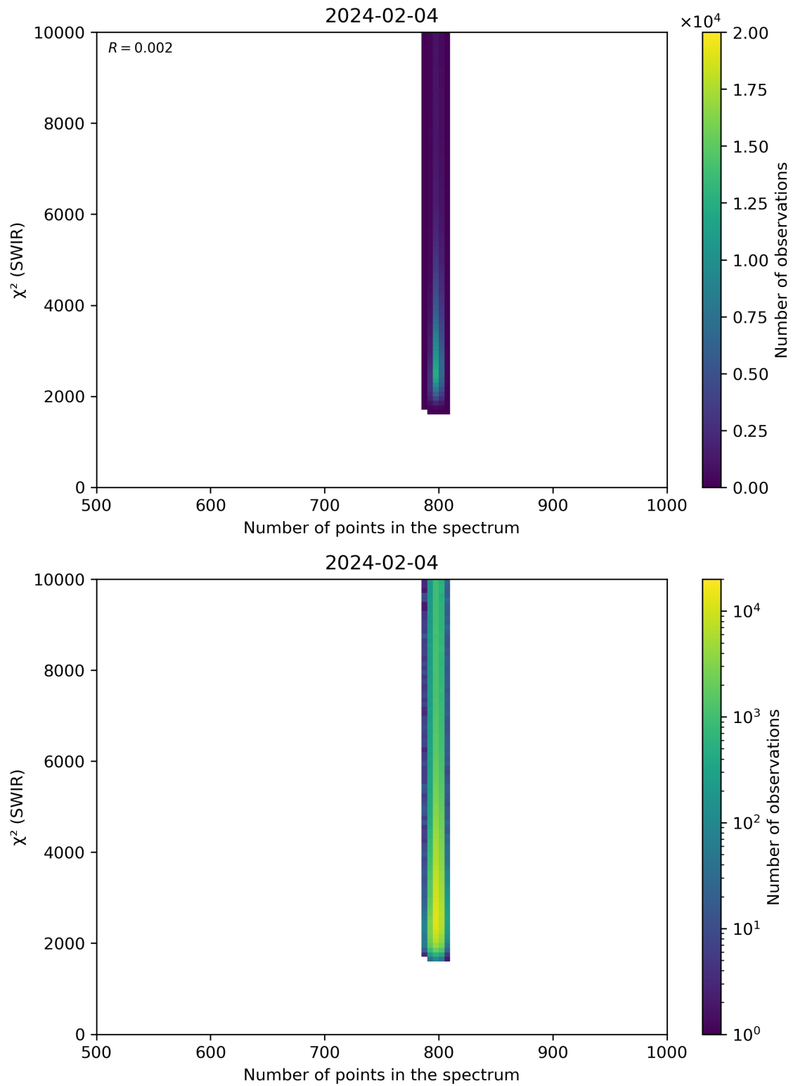
Figure 89: Scatter density plot of “Number of points in the spectrum” against “ \chi^2 (SWIR)” for 2024-02-03 to 2024-02-05.
