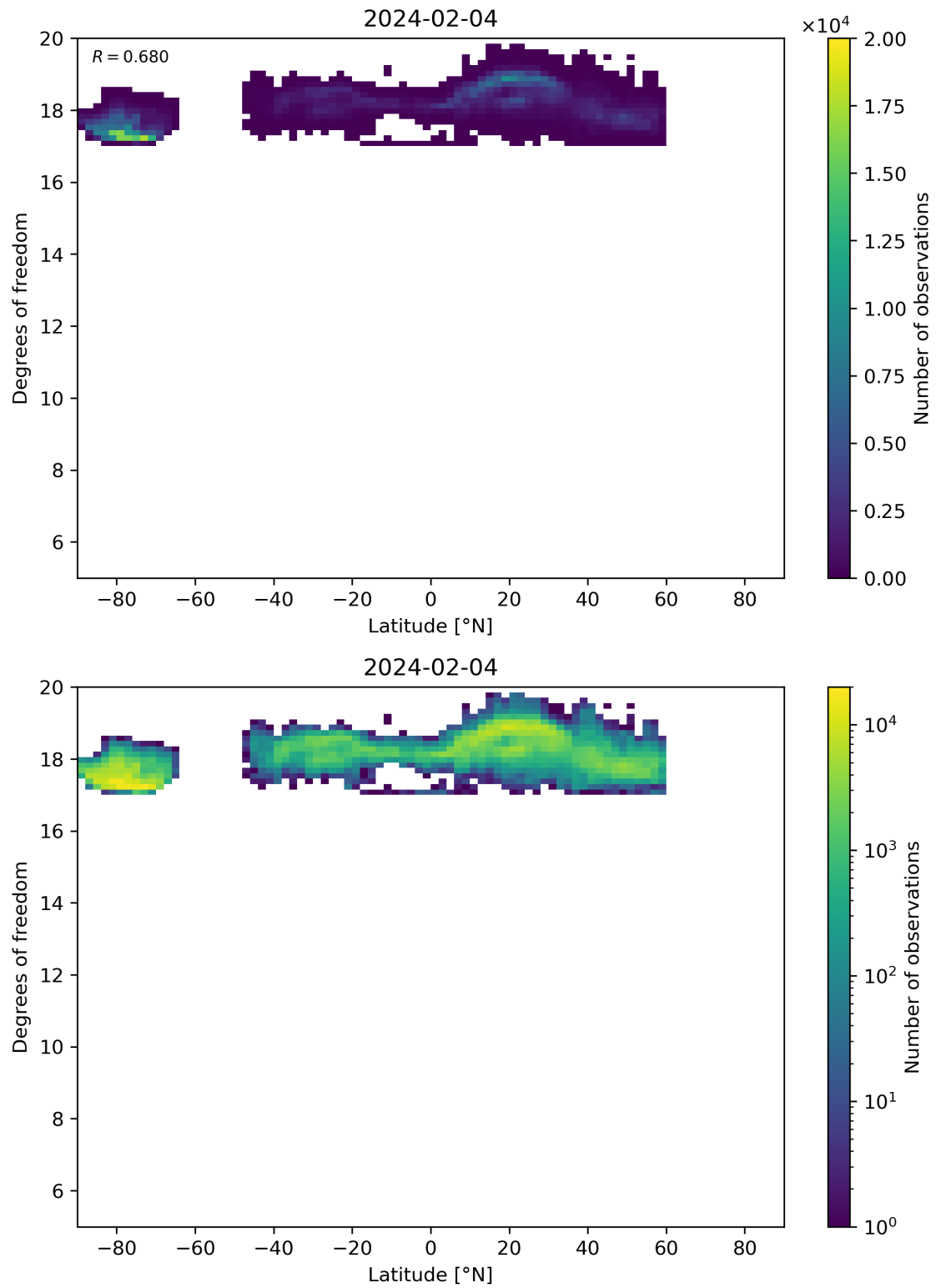
Figure 55: Scatter density plot of “Latitude” against “Degrees of freedom” for 2024-02-03 to 2024-02-05.
