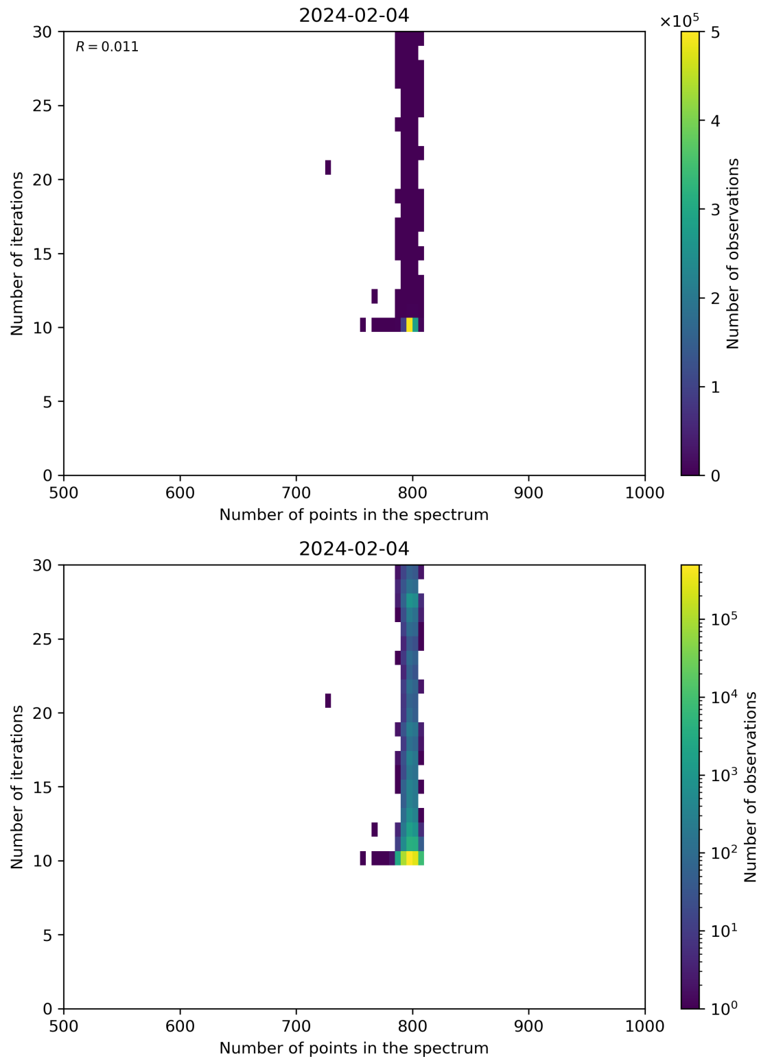
Figure 92: Scatter density plot of “Number of points in the spectrum” against “Number of iterations” for 2024-02-03 to 2024-02-05.
