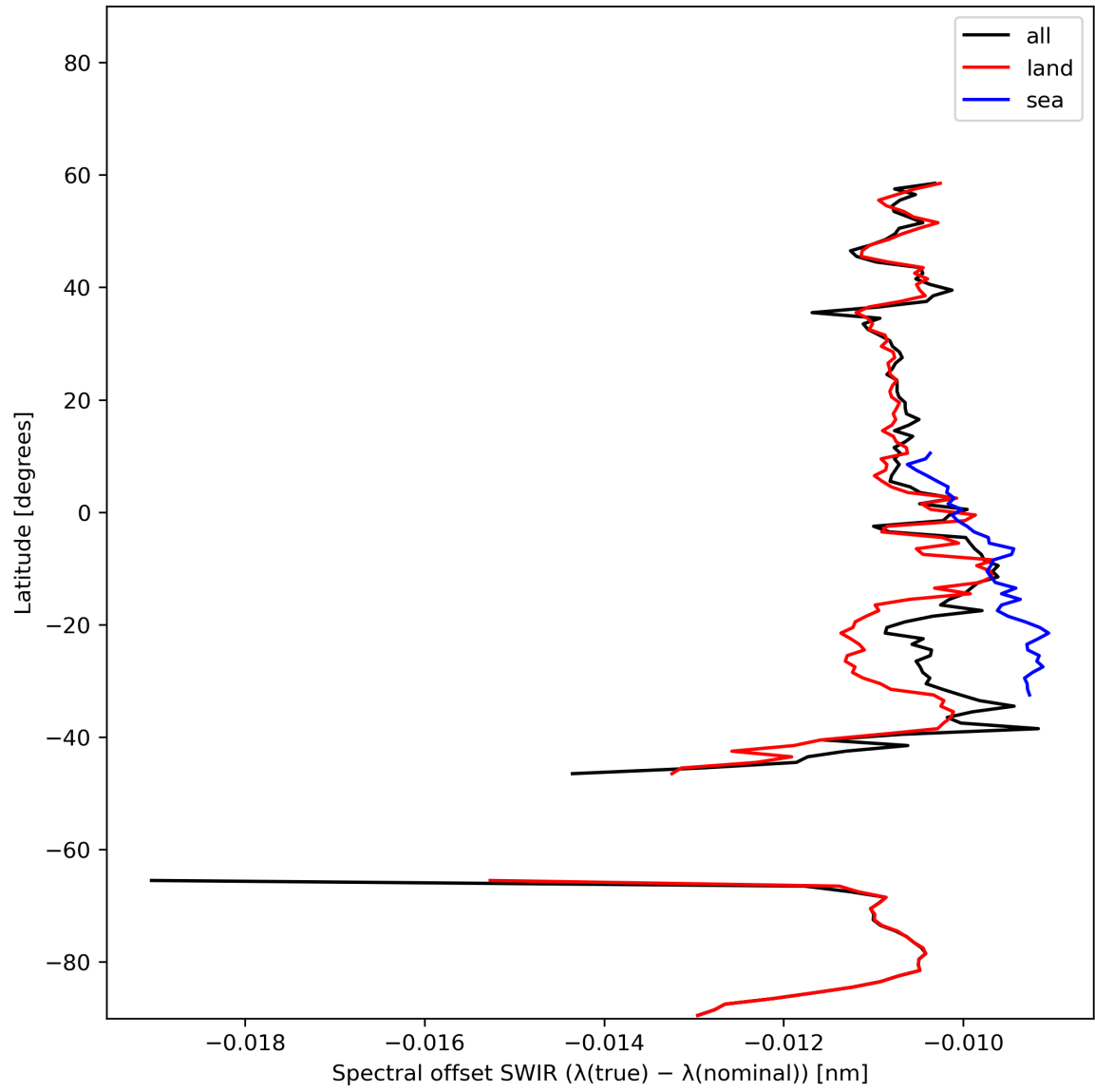
Figure 16: Zonal average of “Spectral offset SWIR ( \lambda(\text{true}) - \lambda(\text{nominal}) )” for 2024-02-03 to 2024-02-05.
