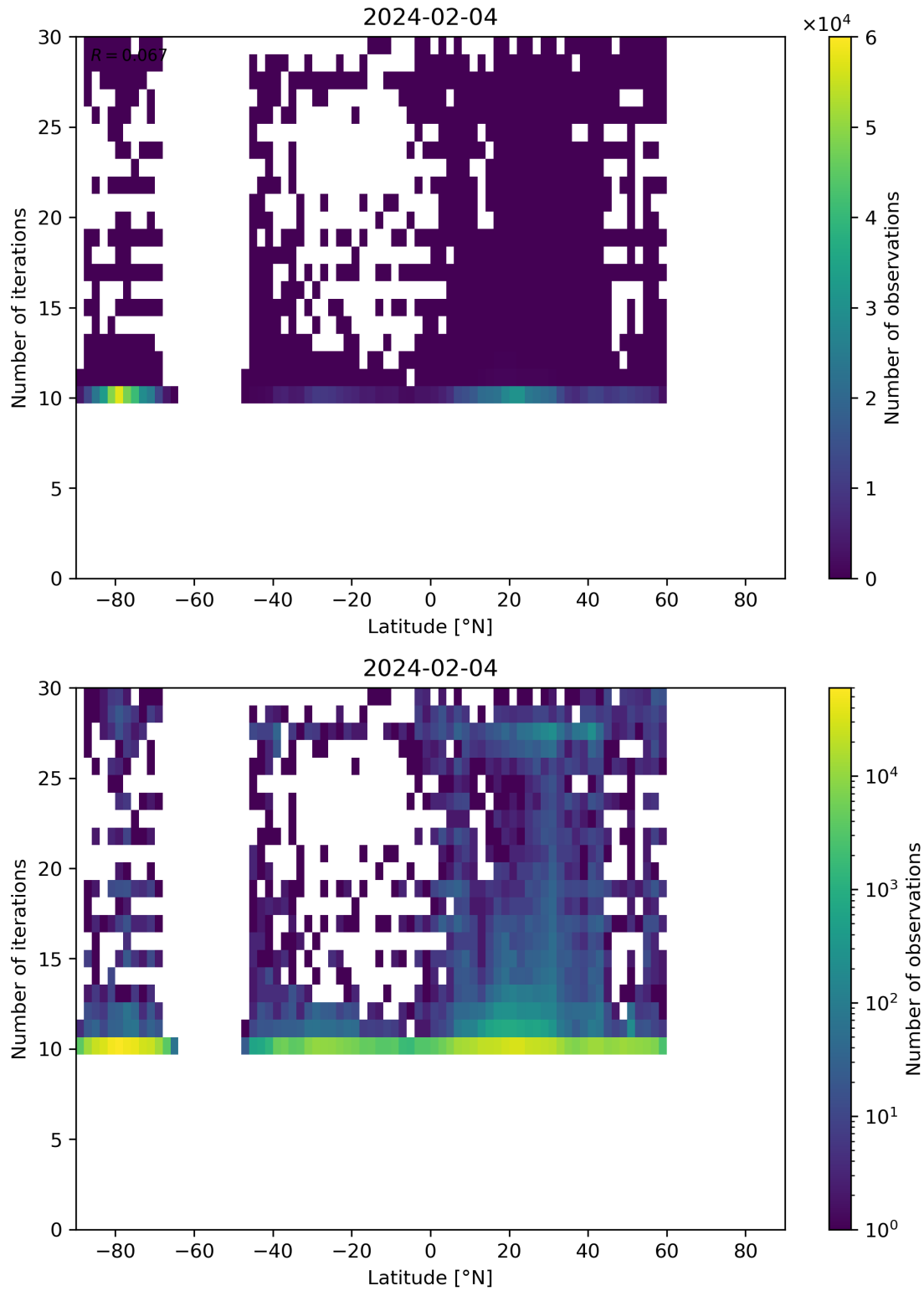
Figure 60: Scatter density plot of “Latitude” against “Number of iterations” for 2024-02-03 to 2024-02-05.
