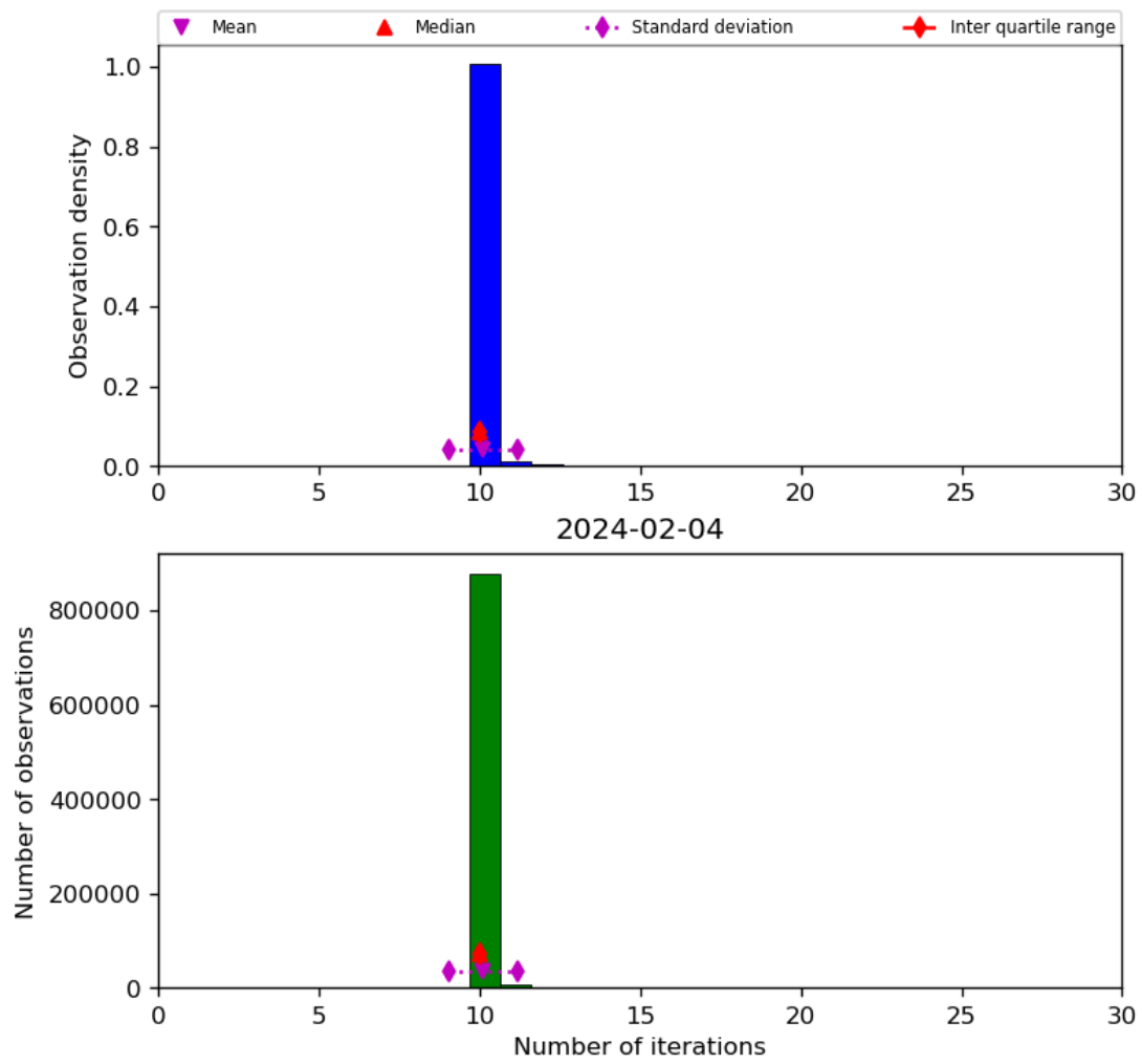
Figure 31: Histogram of “Number of iterations” for 2024-02-03 to 2024-02-05
