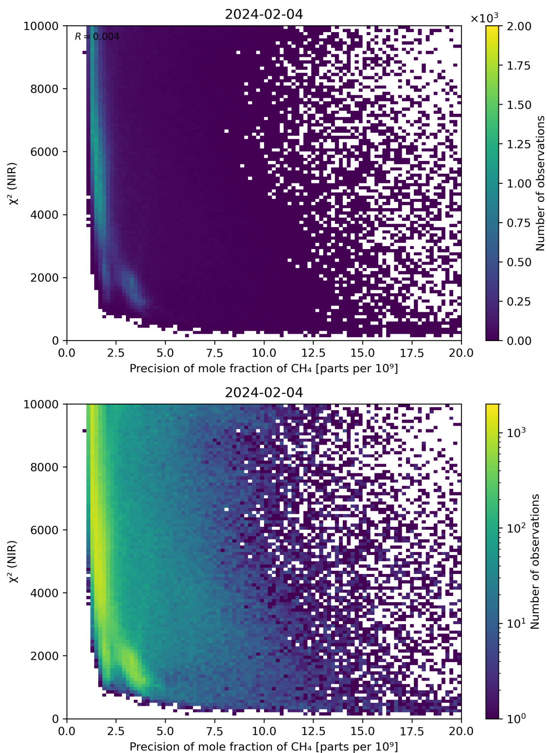
Figure 78: Scatter density plot of “Precision of mole fraction of \text{CH}_4 ” against “ \chi^2 (NIR)” for 2024-02-03 to 2024-02-05.
