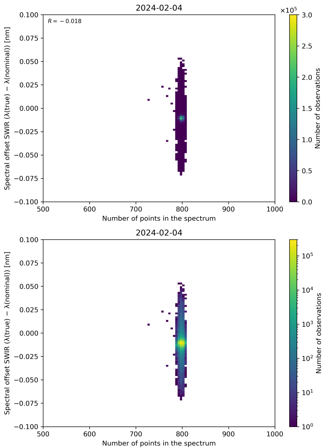
Figure 93: Scatter density plot of “Number of points in the spectrum” against “Spectral offset SWIR ( \lambda(\text{true}) - \lambda(\text{nominal}) )” for 2024-02-03 to 2024-02-05.
