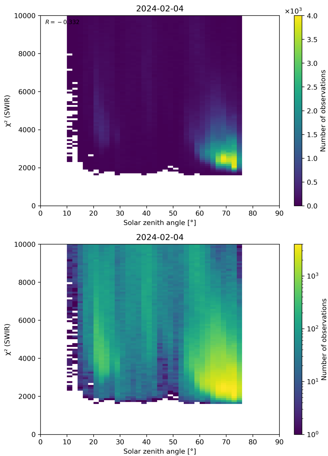
Figure 95: Scatter density plot of “Solar zenith angle” against “ \chi^2 (SWIR)” for 2024-02-03 to 2024-02-05.
