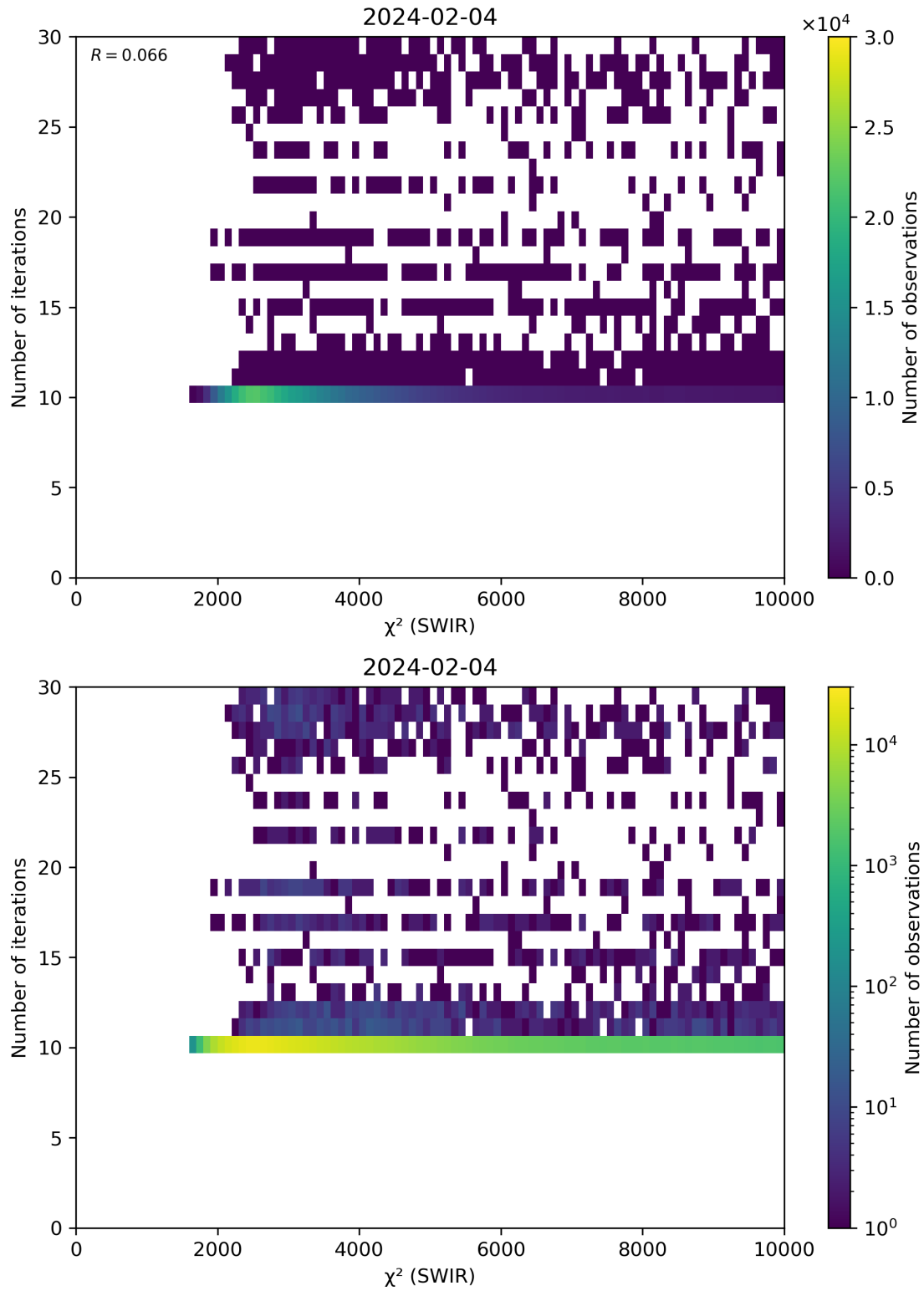
Figure 50: Scatter density plot of “ \chi^2 (SWIR)” against “Number of iterations” for 2024-02-03 to 2024-02-05.
