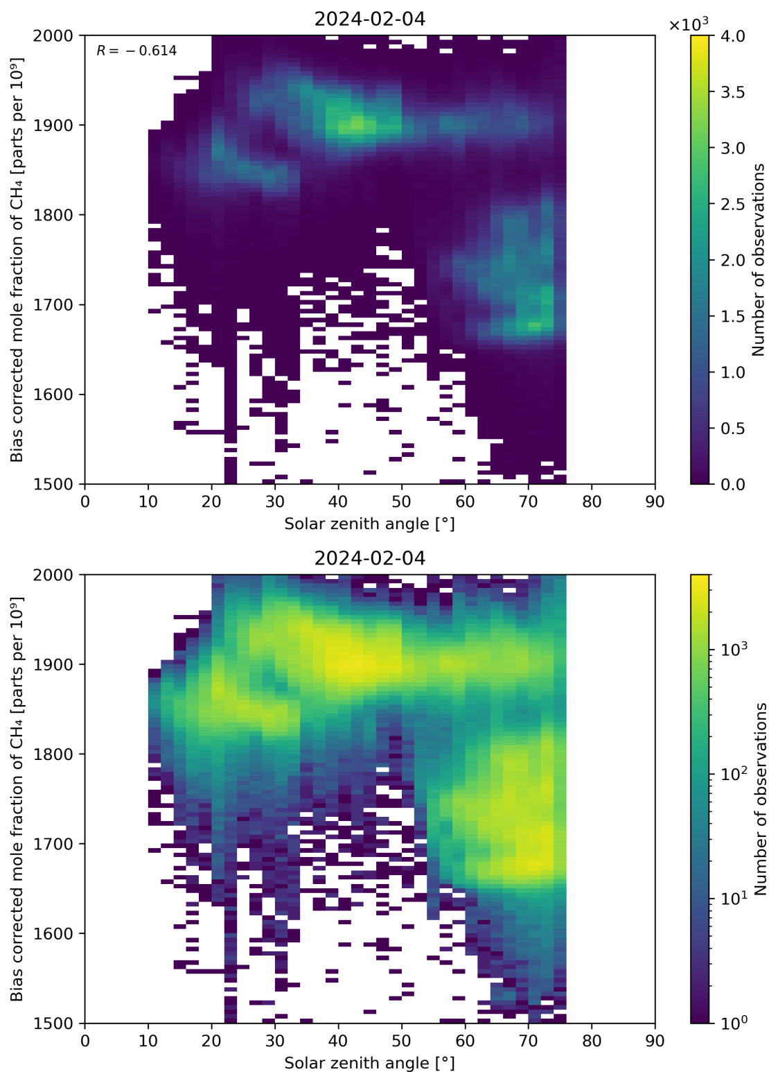
Figure 100: Scatter density plot of “Solar zenith angle” against “Bias corrected mole fraction of \text{CH}_4 ” for 2024-02-03 to 2024-02-05.
