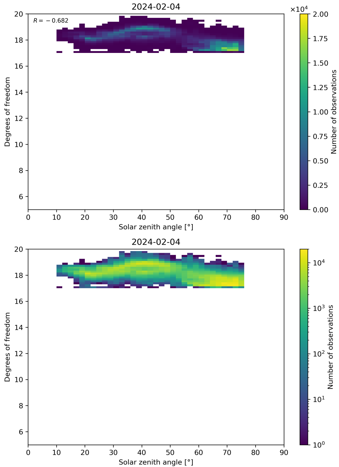
Figure 96: Scatter density plot of “Solar zenith angle” against “Degrees of freedom” for 2024-02-03 to 2024-02-05.
