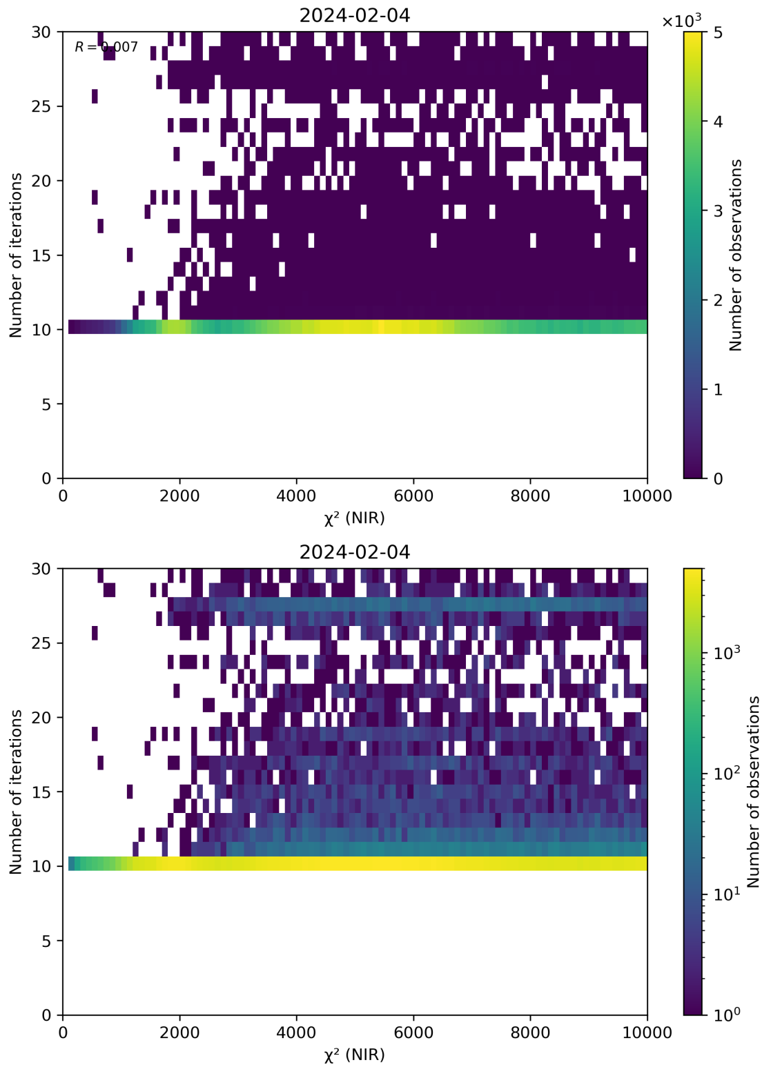
Figure 46: Scatter density plot of “ \chi^2 (NIR)” against “Number of iterations” for 2024-02-03 to 2024-02-05.
