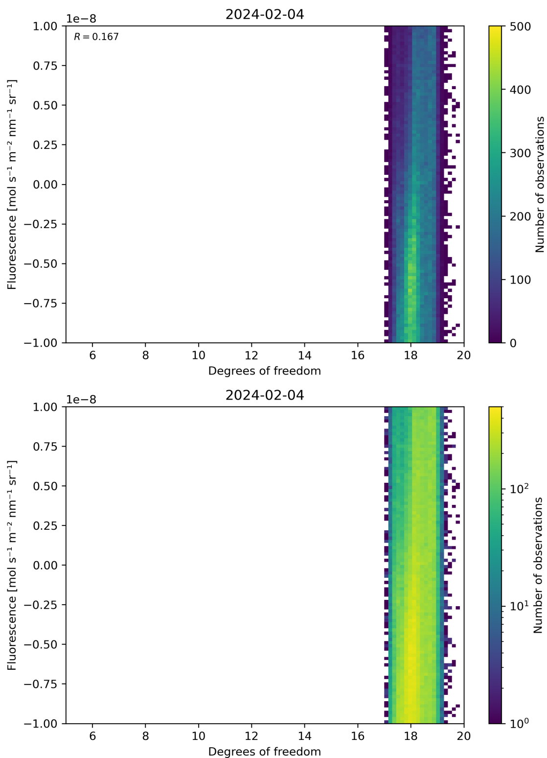
Figure 51: Scatter density plot of “Degrees of freedom” against “Fluorescence” for 2024-02-03 to 2024-02-05.
