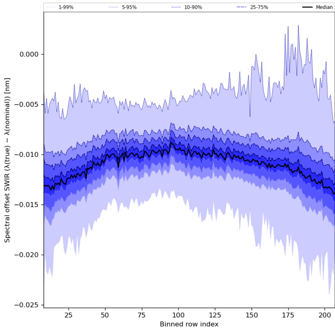
Figure 38: Along track statistics of “Spectral offset SWIR ( \lambda(\text{true}) - \lambda(\text{nominal}) )” for 2024-02-03 to 2024-02-05
