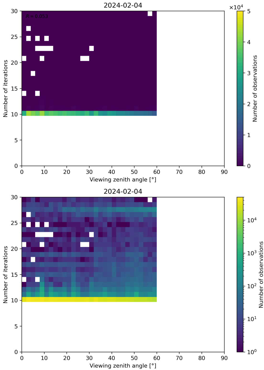
Figure 113: Scatter density plot of “Viewing zenith angle” against “Number of iterations” for 2024-02-03 to 2024-02-05.
