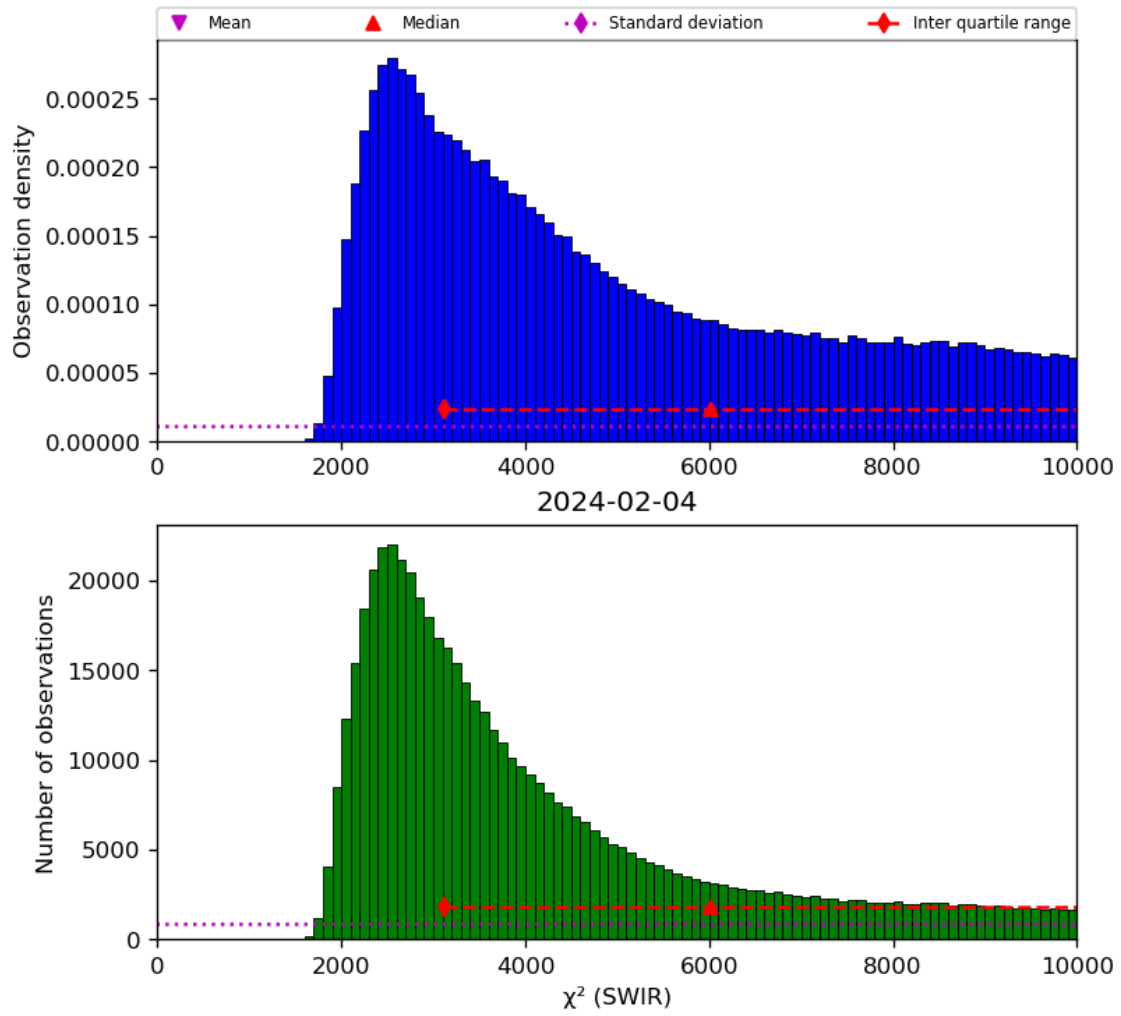
Figure 28: Histogram of “ \chi^2 (SWIR)” for 2024-02-03 to 2024-02-05
