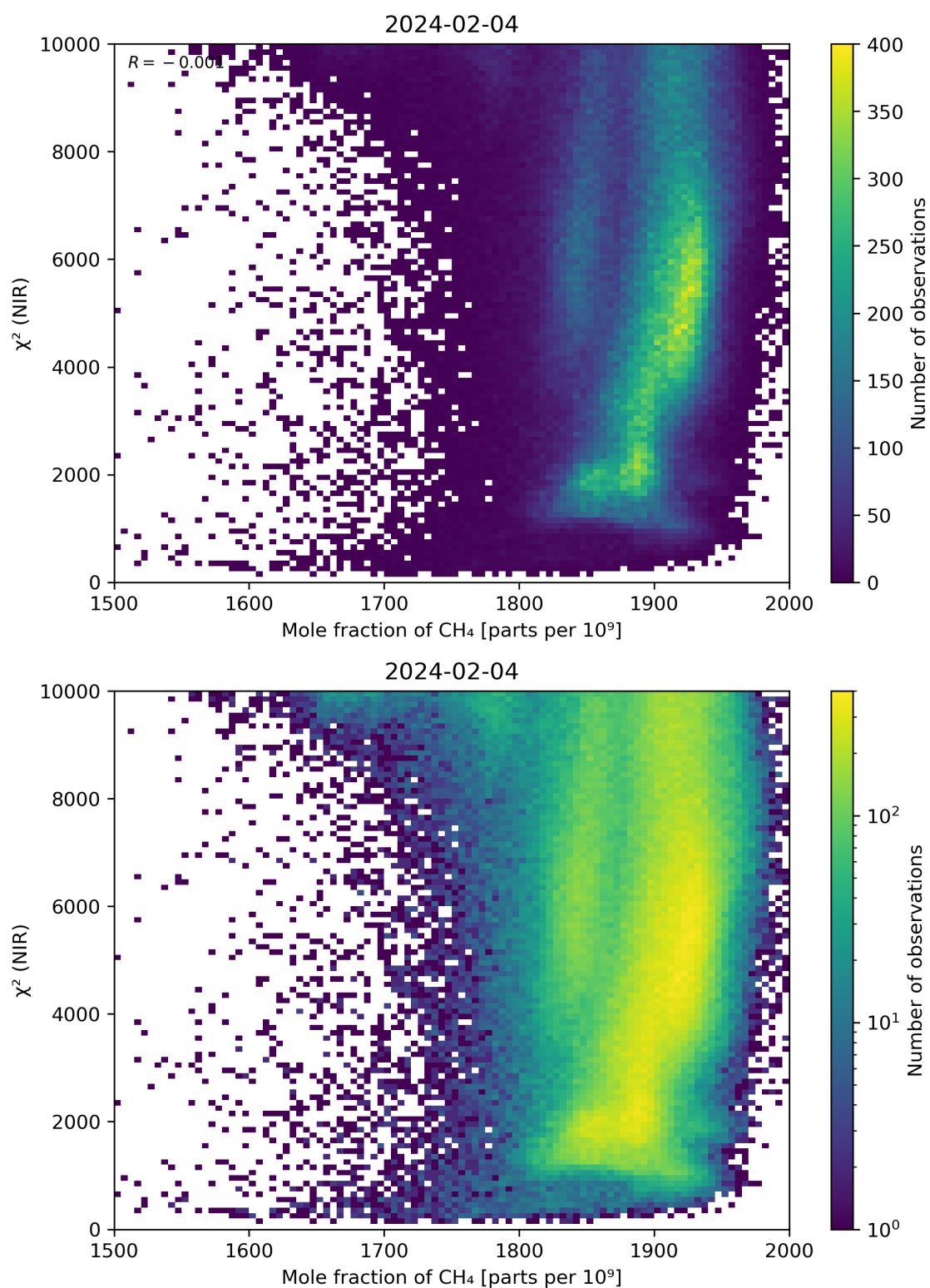
Figure 70: Scatter density plot of “Mole fraction of CH 4 ” against “ \chi^2 (NIR)” for 2024-02-03 to 2024-02-05.
