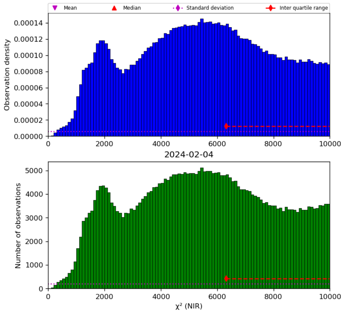
Figure 29: Histogram of “ \chi^2 (NIR)” for 2024-02-03 to 2024-02-05
