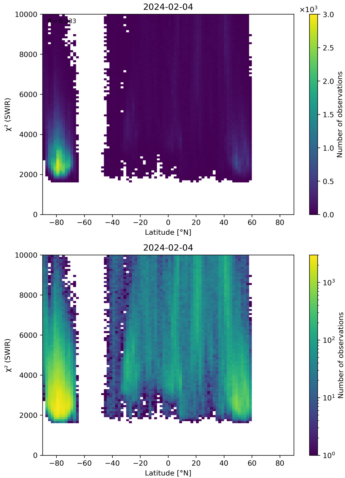
Figure 54: Scatter density plot of “Latitude” against “ \chi^2 (SWIR)” for 2024-02-03 to 2024-02-05.
