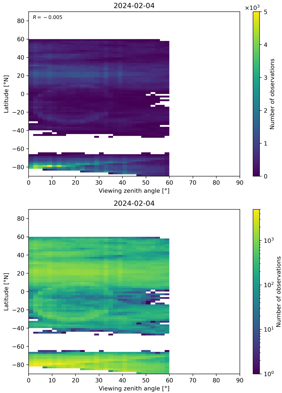
Figure 109: Scatter density plot of “Viewing zenith angle” against “Latitude” for 2024-02-03 to 2024-02-05.
