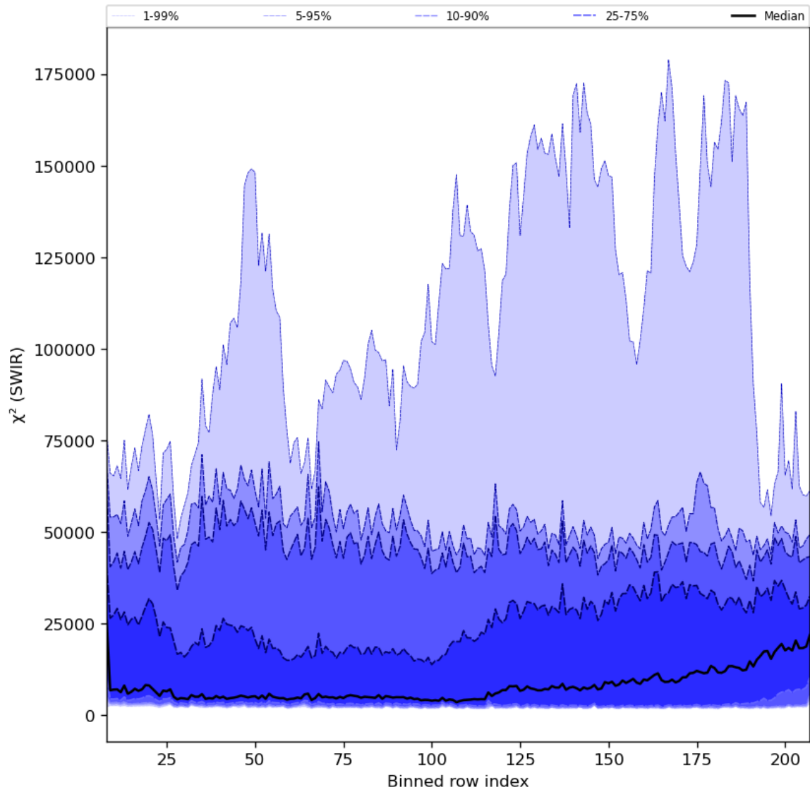
Figure 39: Along track statistics of “ \chi^2 (SWIR)” for 2024-02-03 to 2024-02-05
