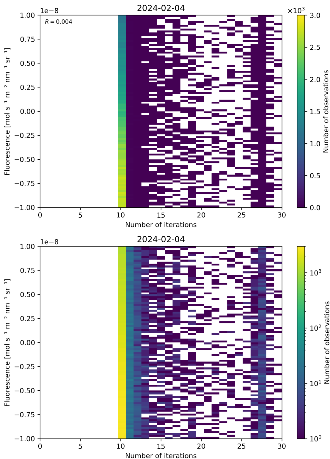
Figure 87: Scatter density plot of “Number of iterations” against “Fluorescence” for 2024-02-03 to 2024-02-05.
