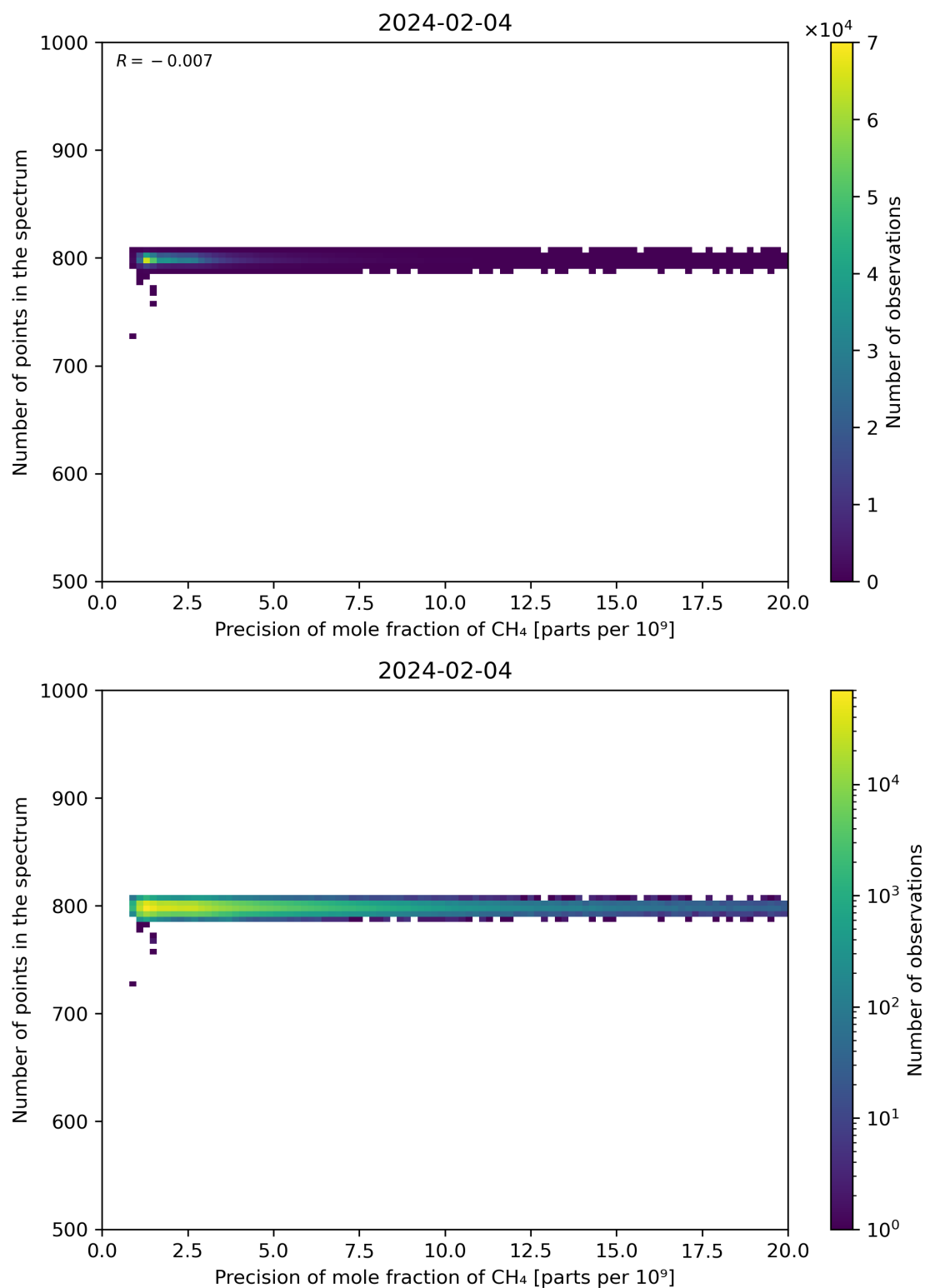
Figure 84: Scatter density plot of “Precision of mole fraction of CH 4 ” against “Number of points in the spectrum” for 2024-02-03 to 2024-02-05.
