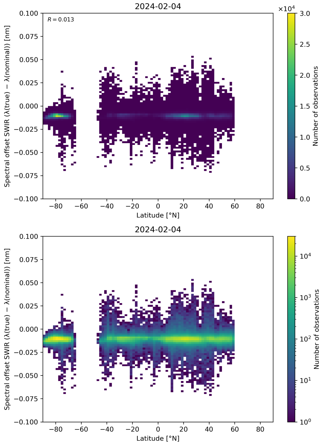
Figure 62: Scatter density plot of “Latitude” against “Spectral offset SWIR ( \lambda(\text{true}) - \lambda(\text{nominal}) )” for 2024-02-03 to 2024-02-05.
