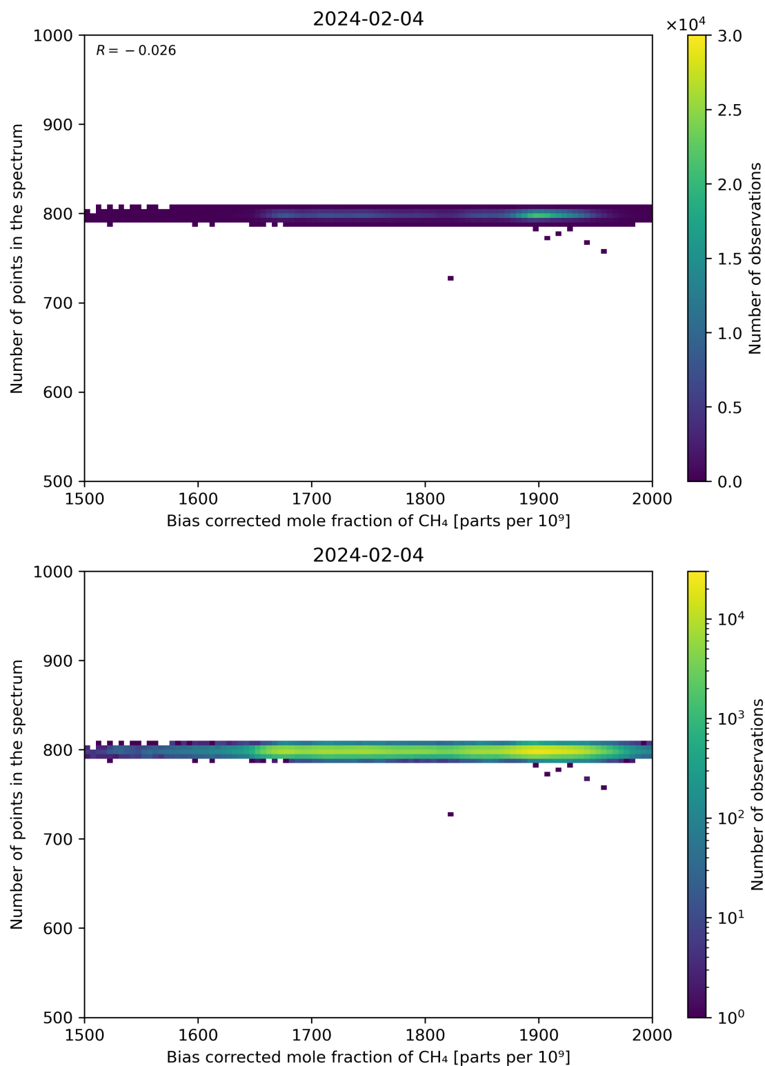
Figure 68: Scatter density plot of “Bias corrected mole fraction of CH 4 ” against “Number of points in the spectrum” for 2024-02-03 to 2024-02-05.
