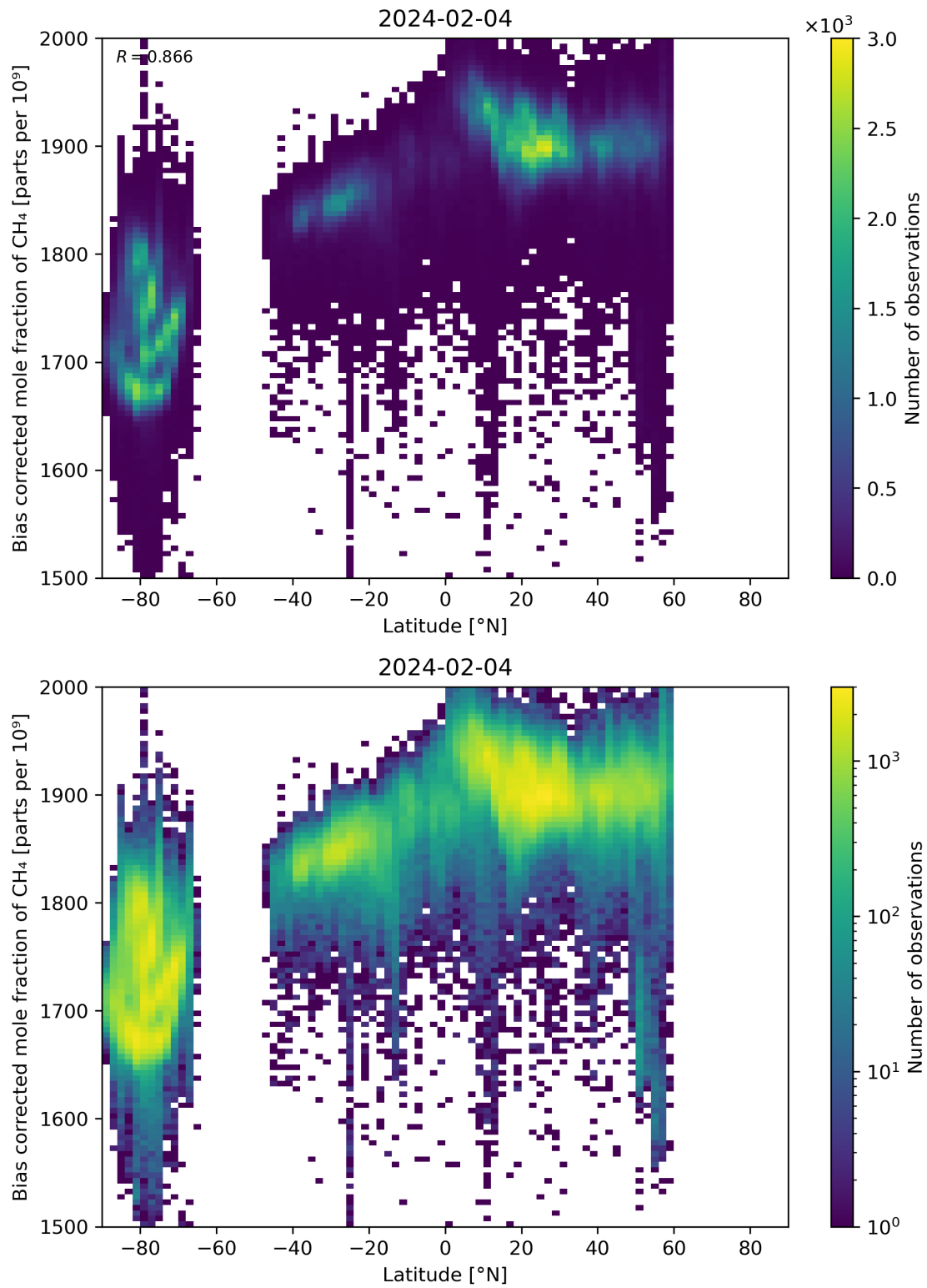
Figure 58: Scatter density plot of “Latitude” against “Bias corrected mole fraction of CH 4 ” for 2024-02-03 to 2024-02-05.
