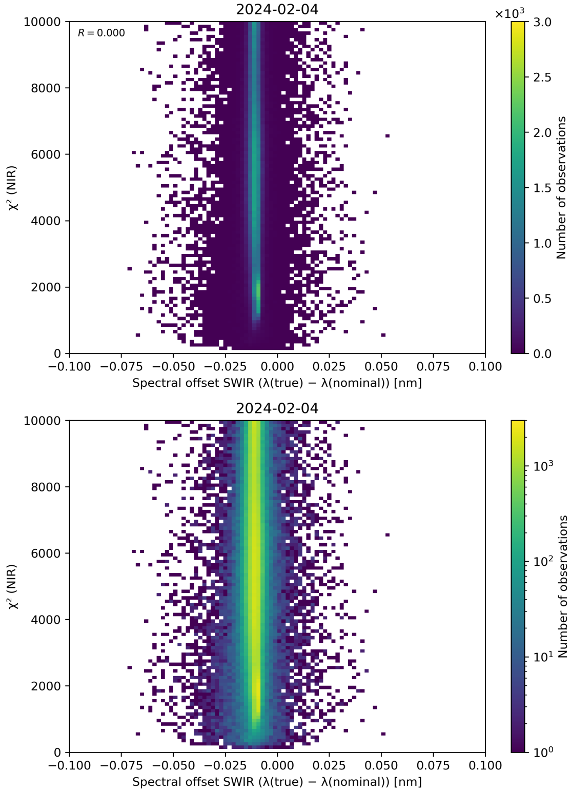
Figure 117: Scatter density plot of “Spectral offset SWIR ( \lambda(\text{true}) - \lambda(\text{nominal}) )” against “ \chi^2 (NIR)” for 2024-02-03 to 2024-02-05.
