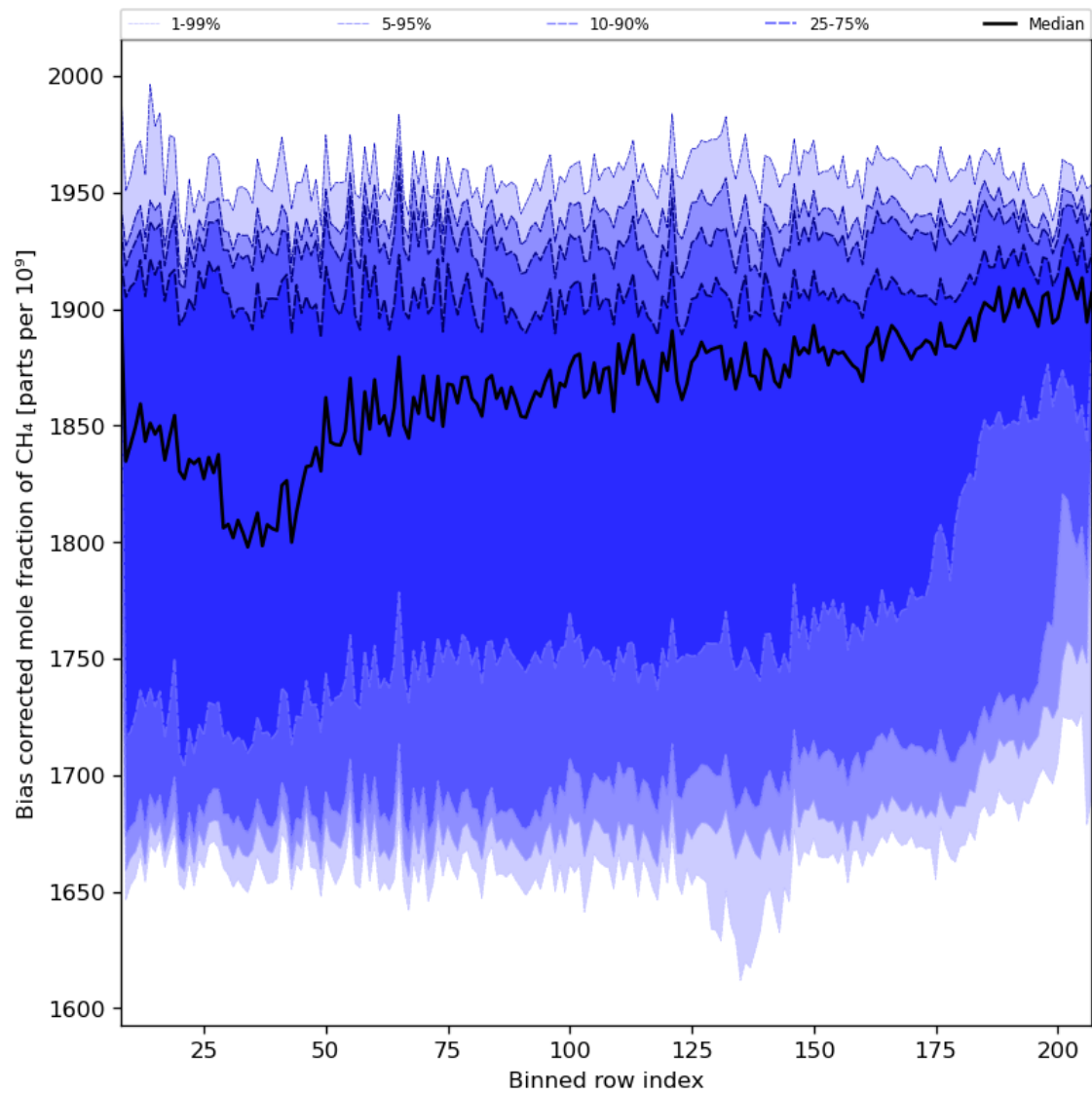
Figure 36: Along track statistics of “Bias corrected mole fraction of CH 4 ” for 2024-02-03 to 2024-02-05
