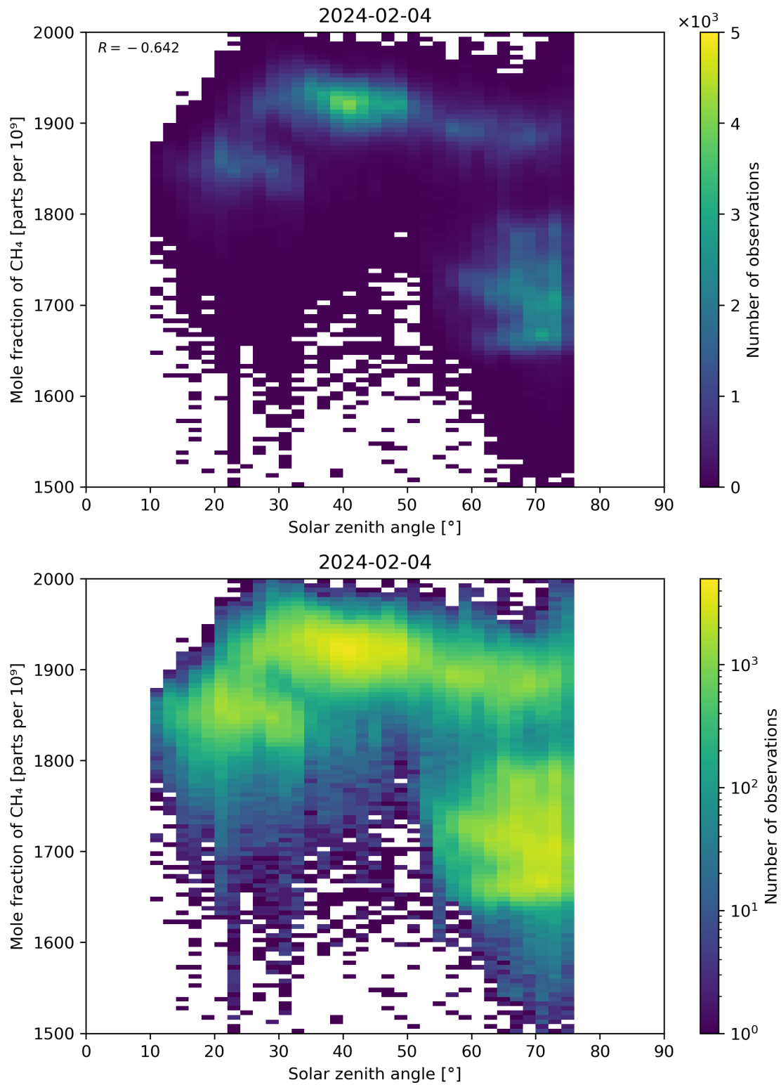
Figure 99: Scatter density plot of “Solar zenith angle” against “Mole fraction of CH 4 ” for 2024-02-03 to 2024-02-05.
