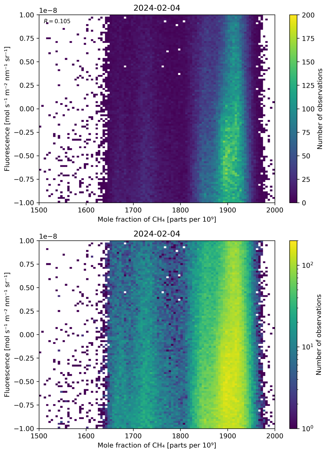
Figure 73: Scatter density plot of “Mole fraction of \text{CH}_4 ” against “Fluorescence” for 2024-02-03 to 2024-02-05.
