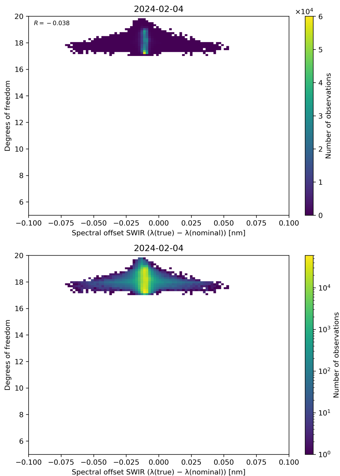
Figure 119: Scatter density plot of “Spectral offset SWIR ( \lambda(\text{true}) - \lambda(\text{nominal}) )” against “Degrees of freedom” for 2024-02-03 to 2024-02-05.
