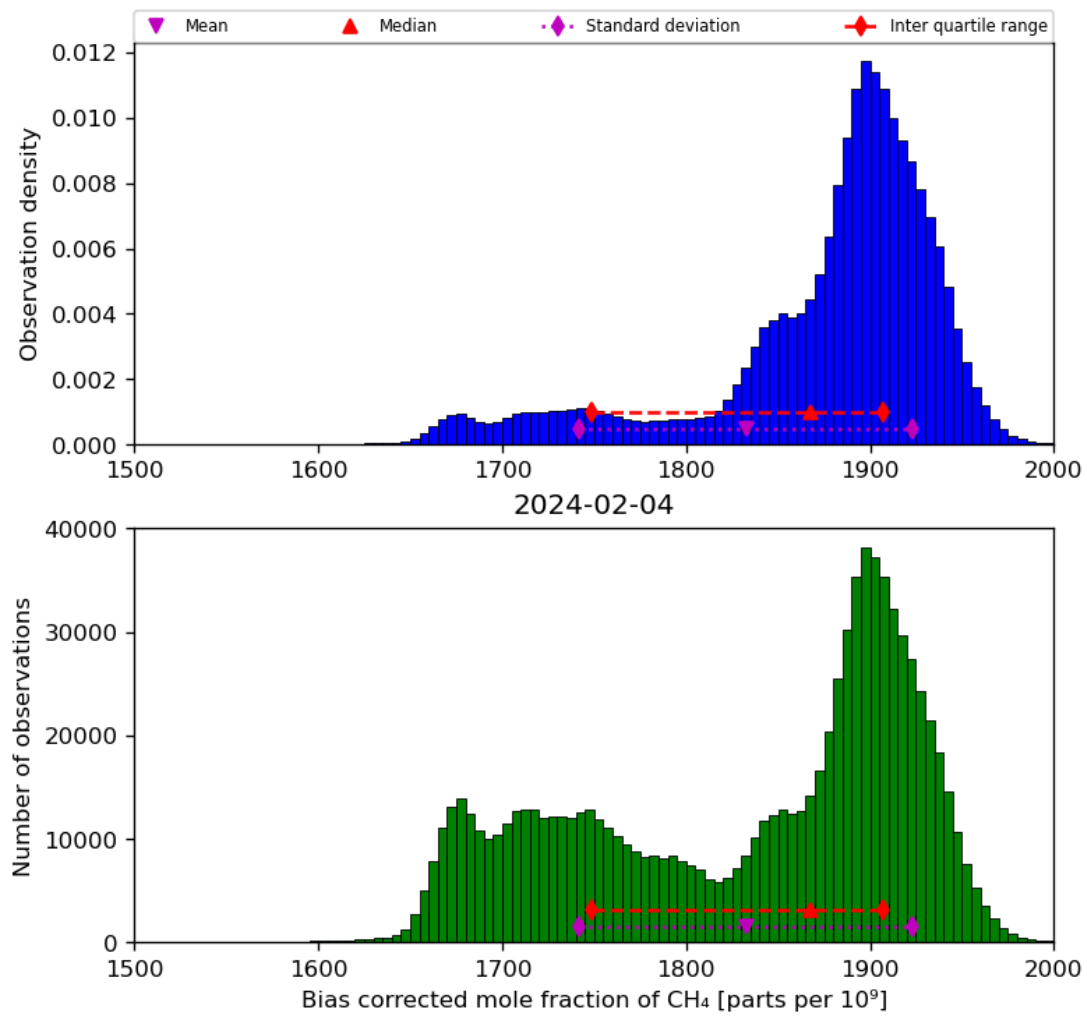
Figure 25: Histogram of “Bias corrected mole fraction of CH 4 ” for 2024-02-03 to 2024-02-05
