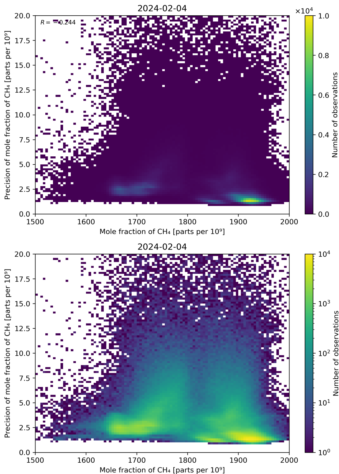
Figure 75: Scatter density plot of “Mole fraction of CH 4 ” against “Precision of mole fraction of CH 4 ” for 2024-02-03 to 2024-02-05.
