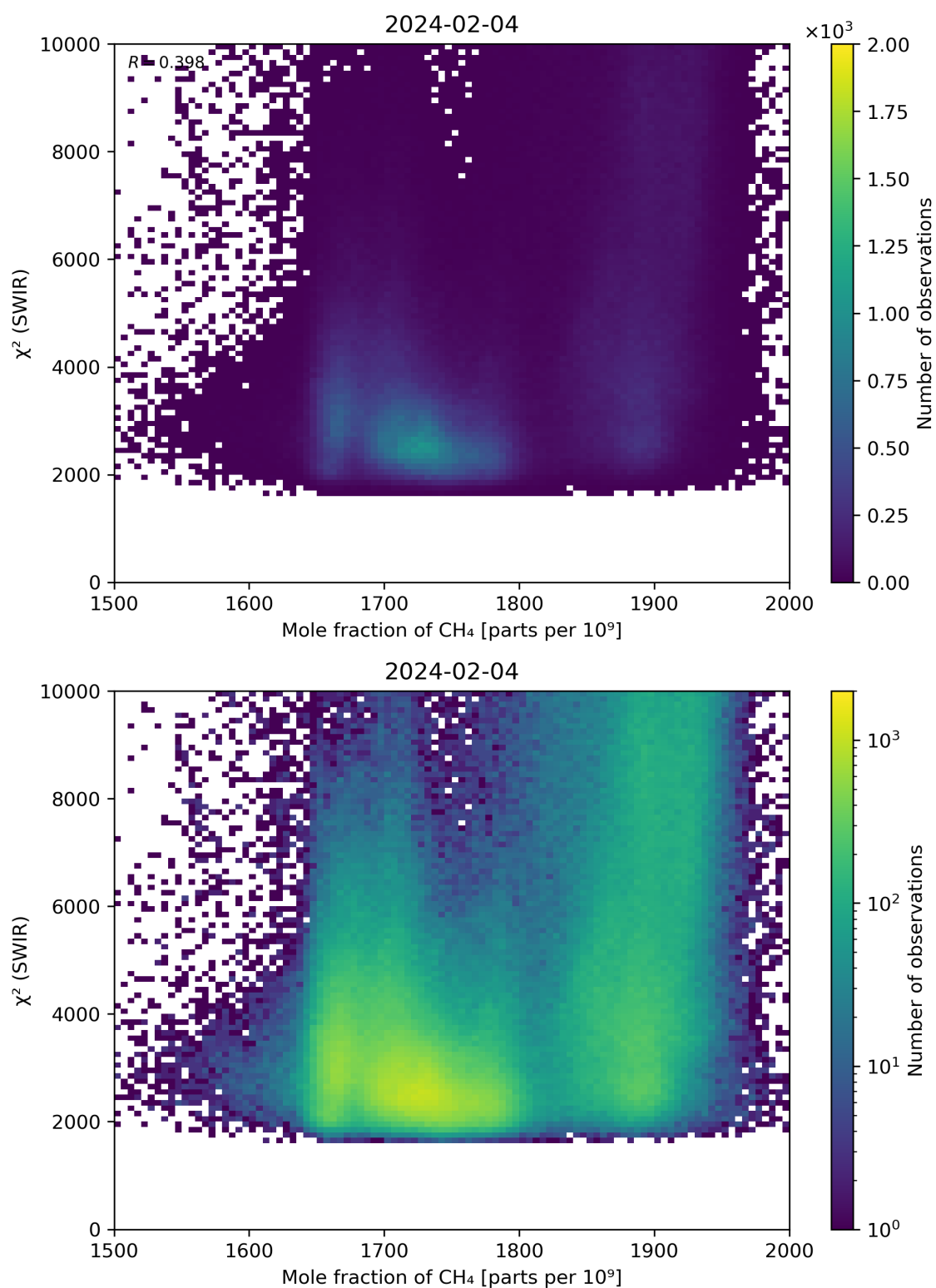
Figure 71: Scatter density plot of “Mole fraction of \text{CH}_4 ” against “ \chi^2 (SWIR)” for 2024-02-03 to 2024-02-05.
