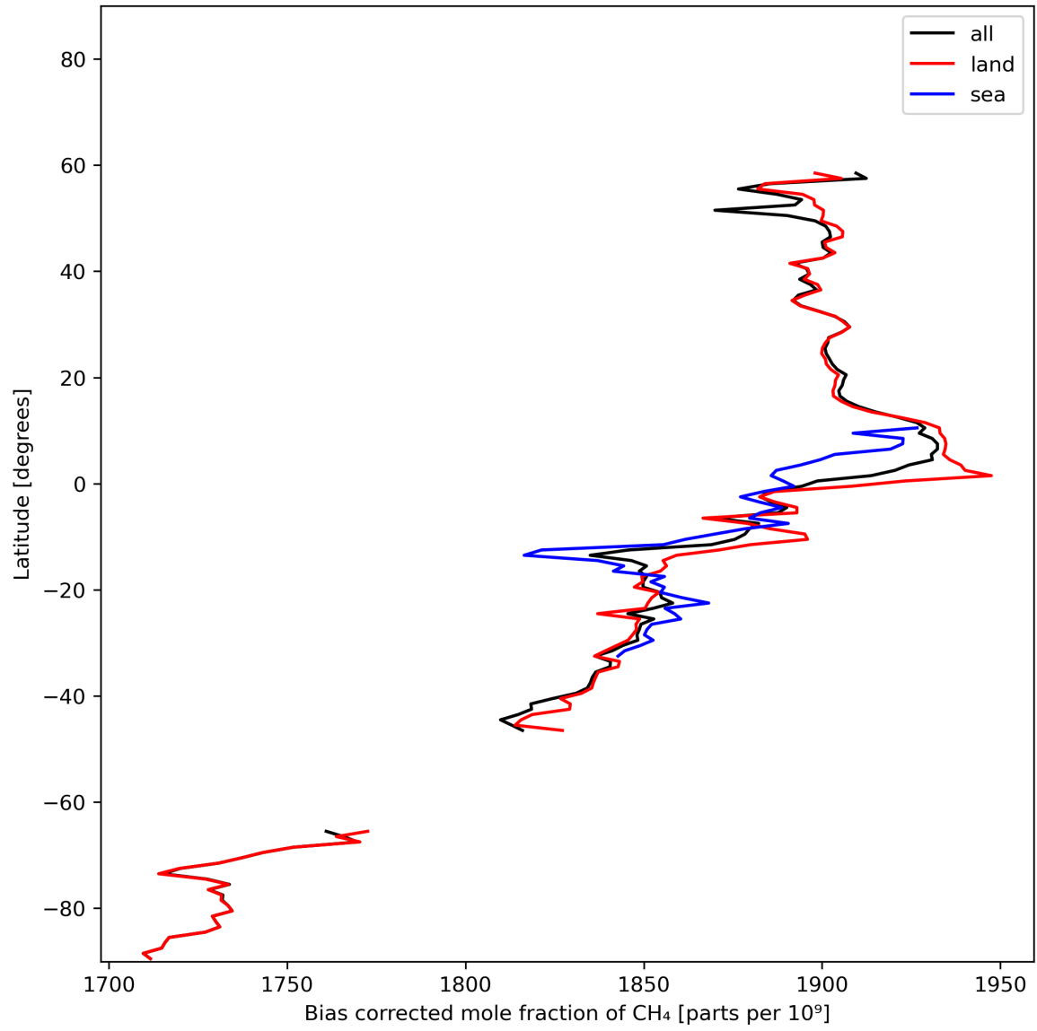
Figure 14: Zonal average of “Bias corrected mole fraction of CH 4 ” for 2024-02-03 to 2024-02-05.
