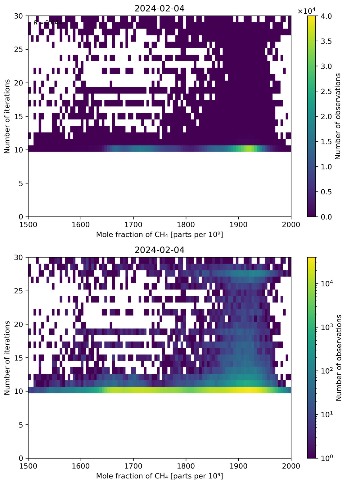
Figure 76: Scatter density plot of “Mole fraction of CH 4 ” against “Number of iterations” for 2024-02-03 to 2024-02-05.
