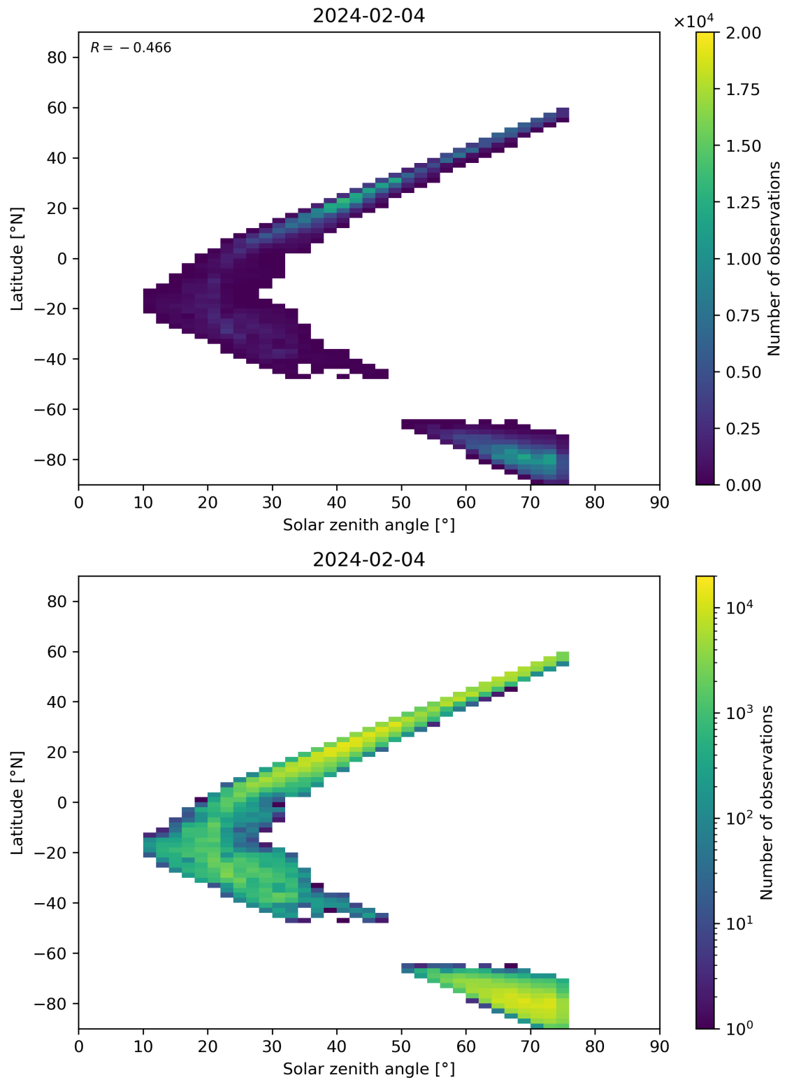
Figure 98: Scatter density plot of “Solar zenith angle” against “Latitude” for 2024-02-03 to 2024-02-05.
