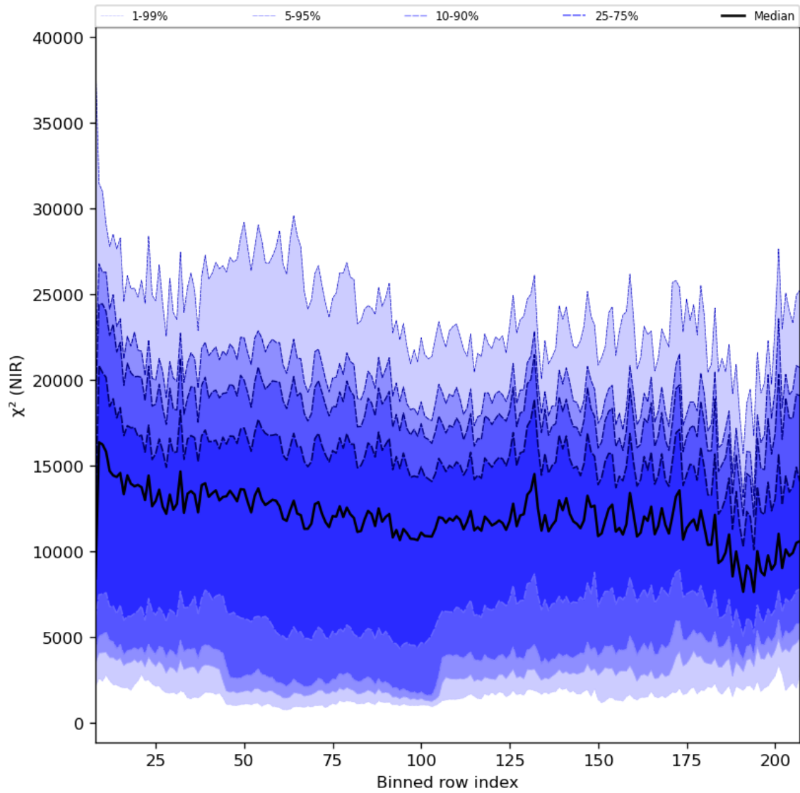
Figure 40: Along track statistics of “ \chi^2 (NIR)” for 2024-02-03 to 2024-02-05
