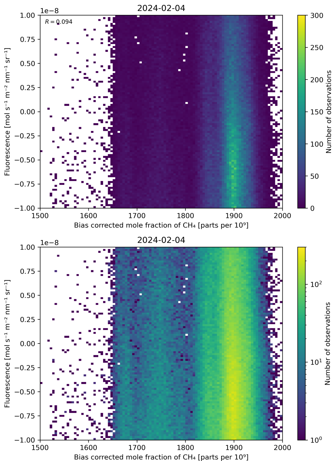
Figure 66: Scatter density plot of “Bias corrected mole fraction of \text{CH}_4 ” against “Fluorescence” for 2024-02-03 to 2024-02-05.
