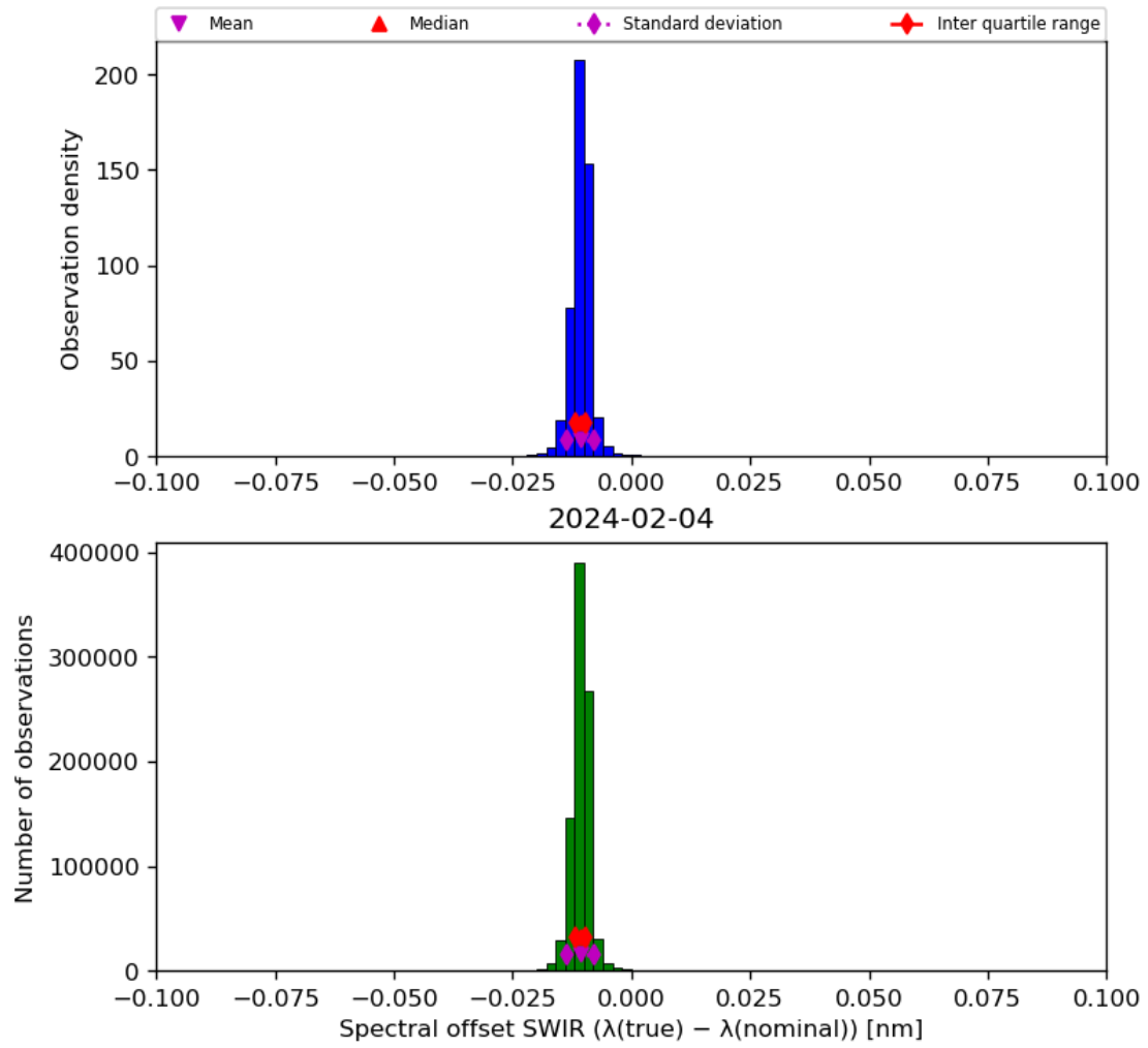
Figure 27: Histogram of “Spectral offset SWIR ( \lambda(\text{true}) - \lambda(\text{nominal}) )” for 2024-02-03 to 2024-02-05
