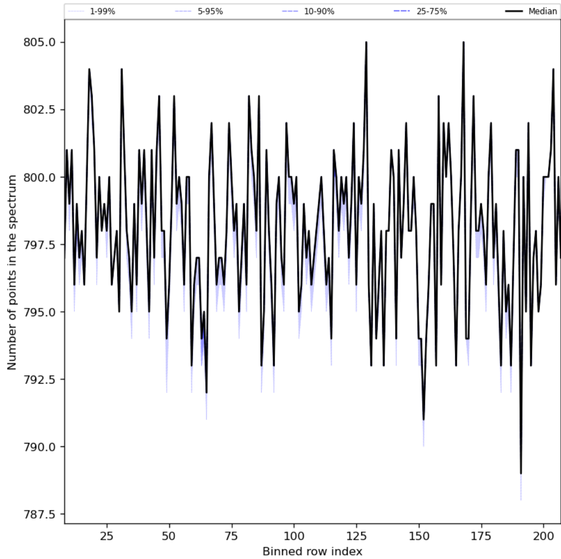
Figure 37: Along track statistics of “Number of points in the spectrum” for 2024-02-03 to 2024-02-05
