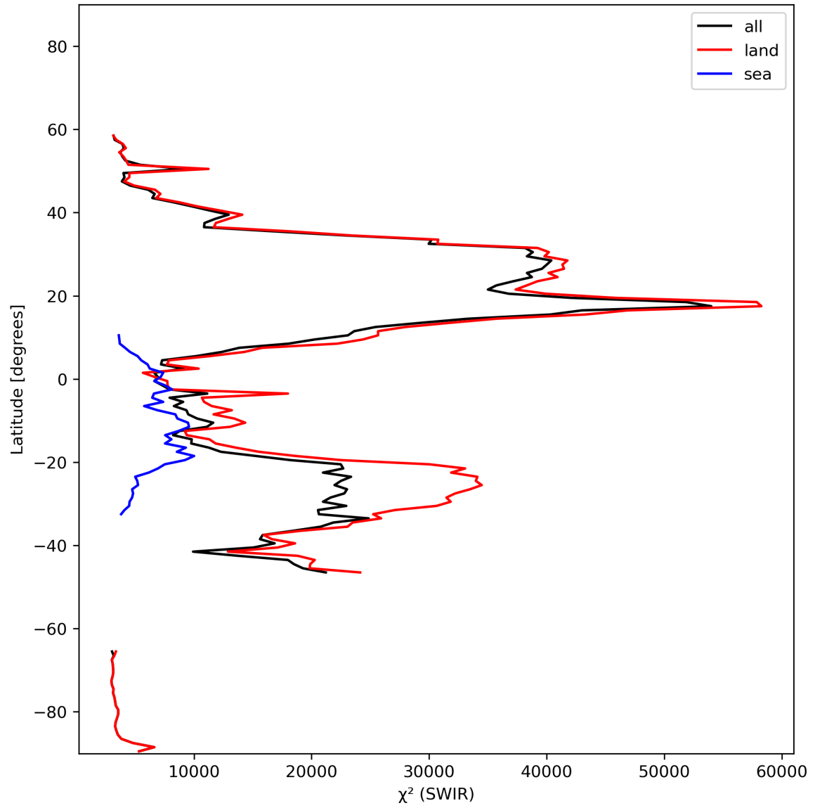
Figure 17: Zonal average of “ \chi^2 (SWIR)” for 2024-02-03 to 2024-02-05.
