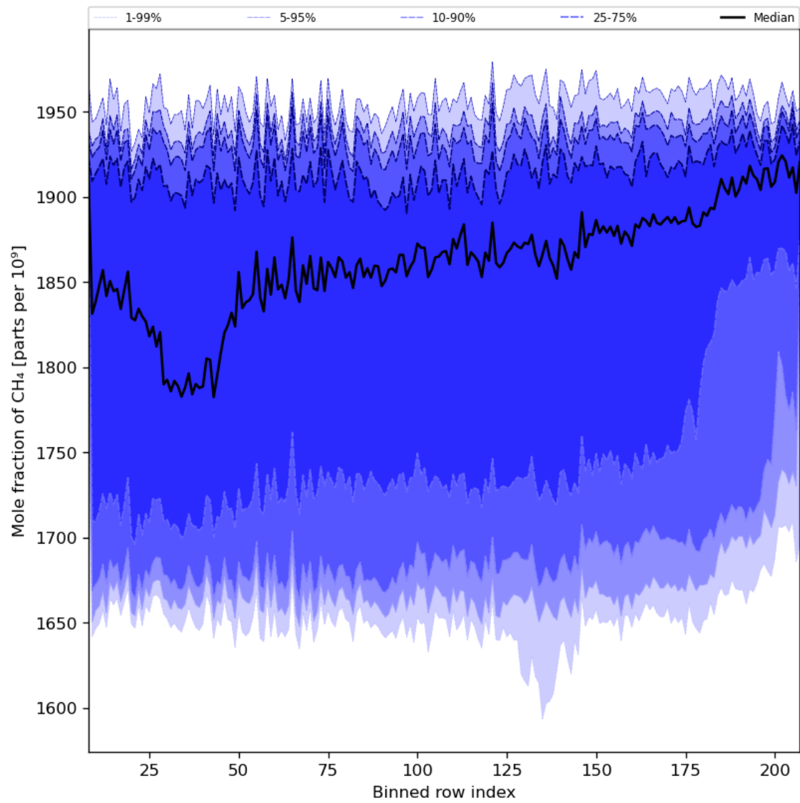
Figure 34: Along track statistics of “Mole fraction of CH 4 ” for 2024-02-03 to 2024-02-05
