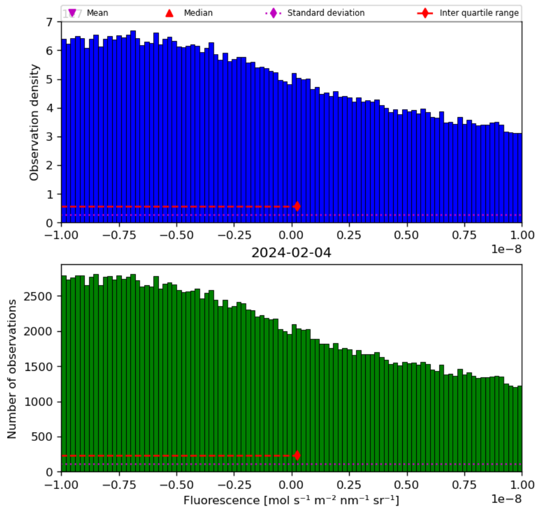
Figure 32: Histogram of “Fluorescence” for 2024-02-03 to 2024-02-05
