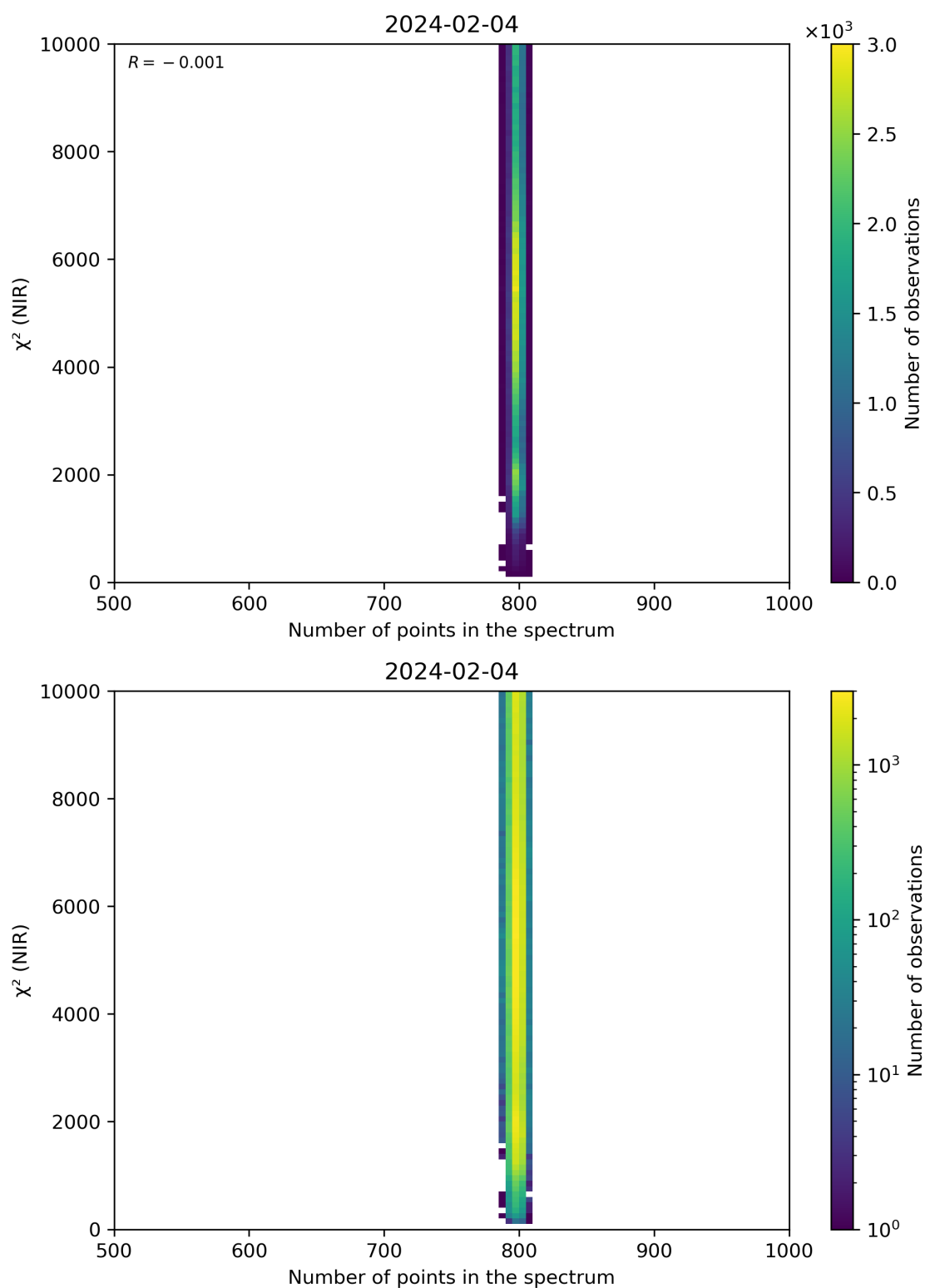
Figure 88: Scatter density plot of “Number of points in the spectrum” against “ \chi^2 (NIR)” for 2024-02-03 to 2024-02-05.
