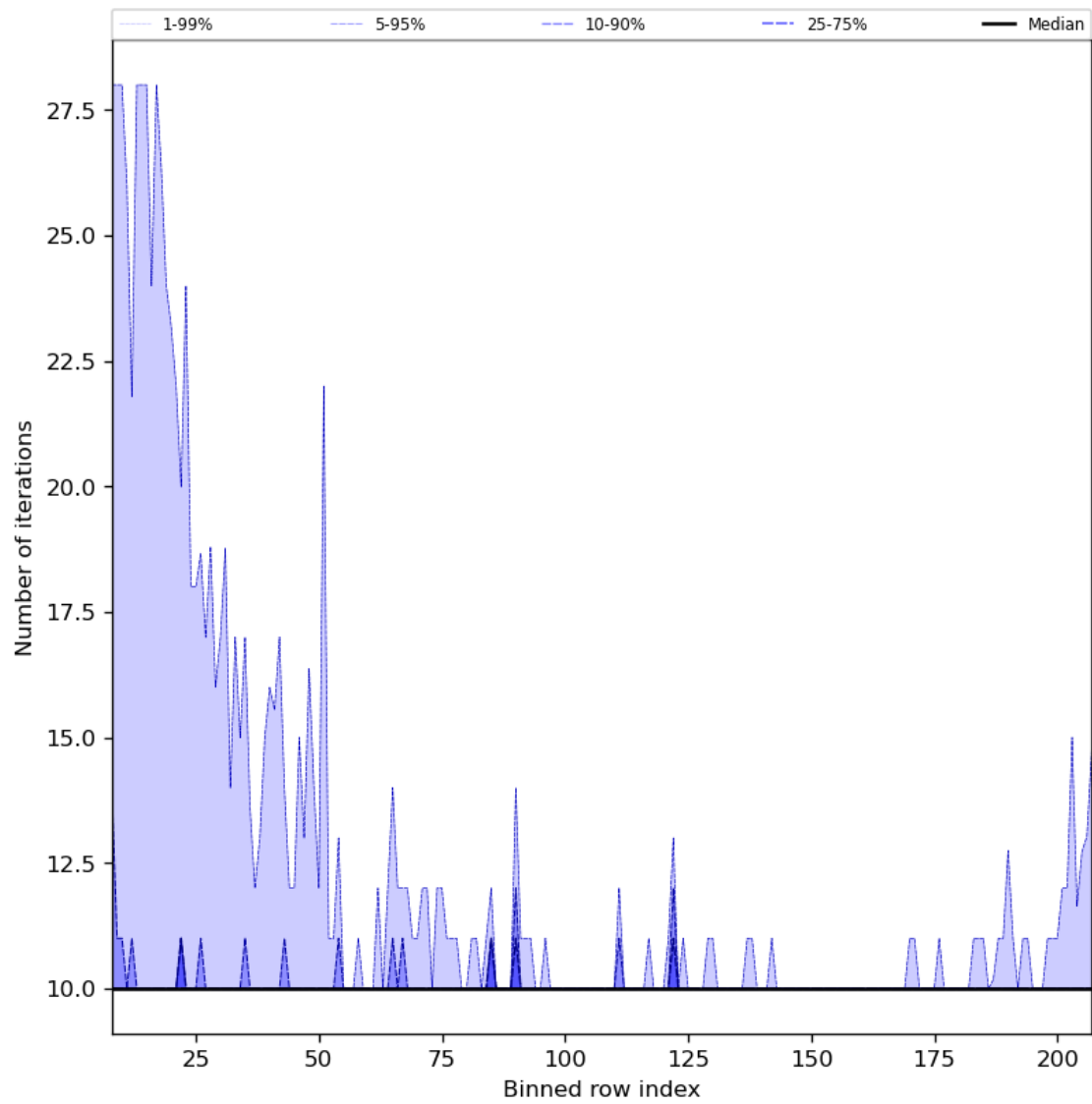
Figure 42: Along track statistics of “Number of iterations” for 2024-02-03 to 2024-02-05
