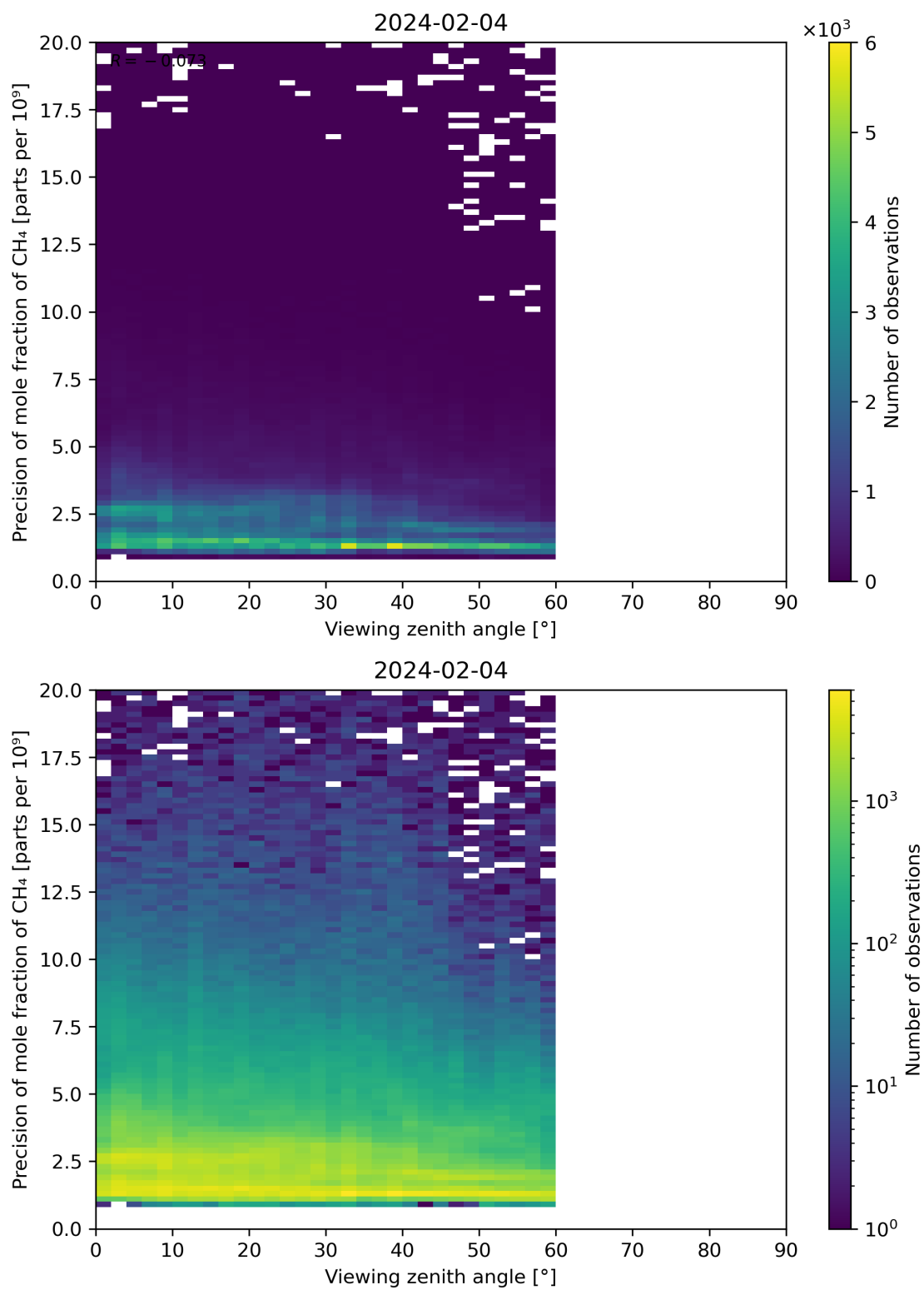
Figure 112: Scatter density plot of “Viewing zenith angle” against “Precision of mole fraction of CH 4 ” for 2024-02-03 to 2024-02-05.
