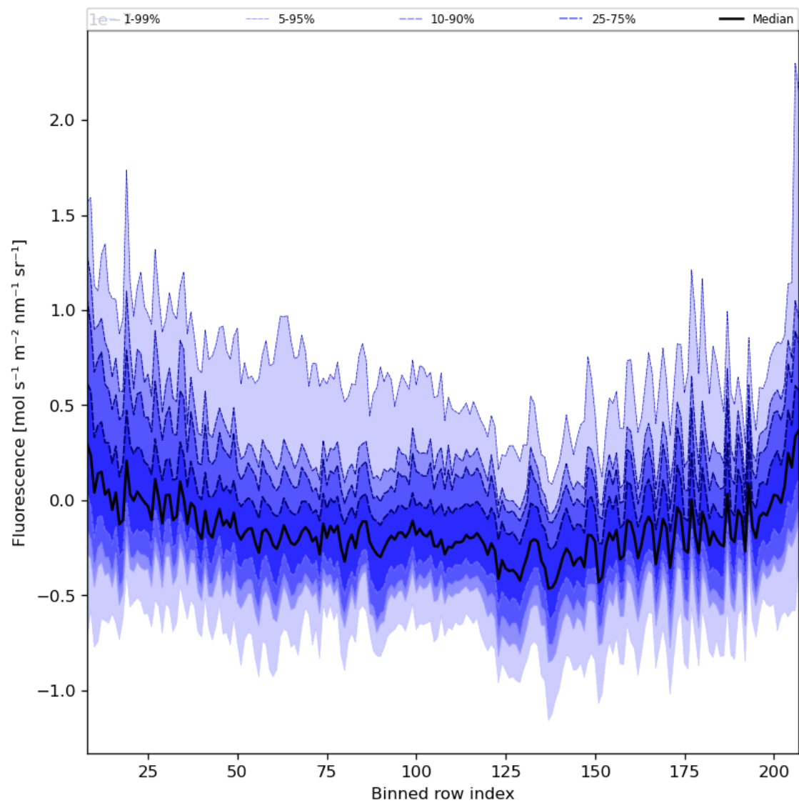
Figure 43: Along track statistics of “Fluorescence” for 2024-02-03 to 2024-02-05
