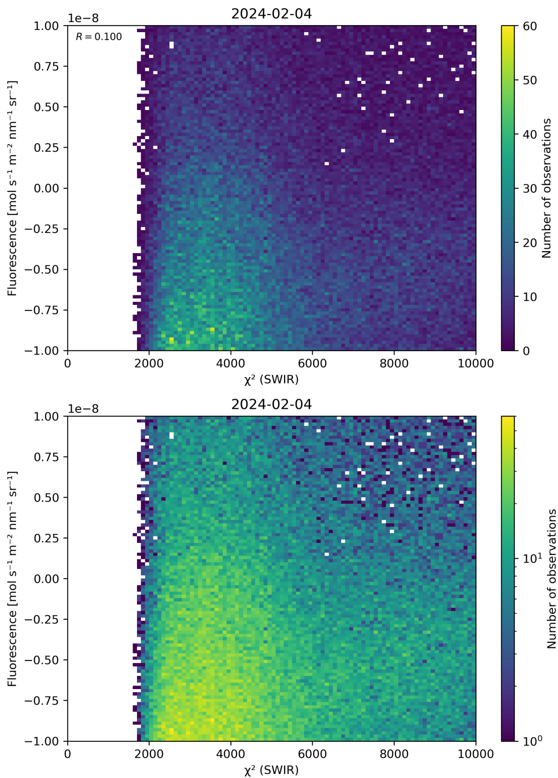
Figure 49: Scatter density plot of “ \chi^2 (SWIR)” against “Fluorescence” for 2024-02-03 to 2024-02-05.
