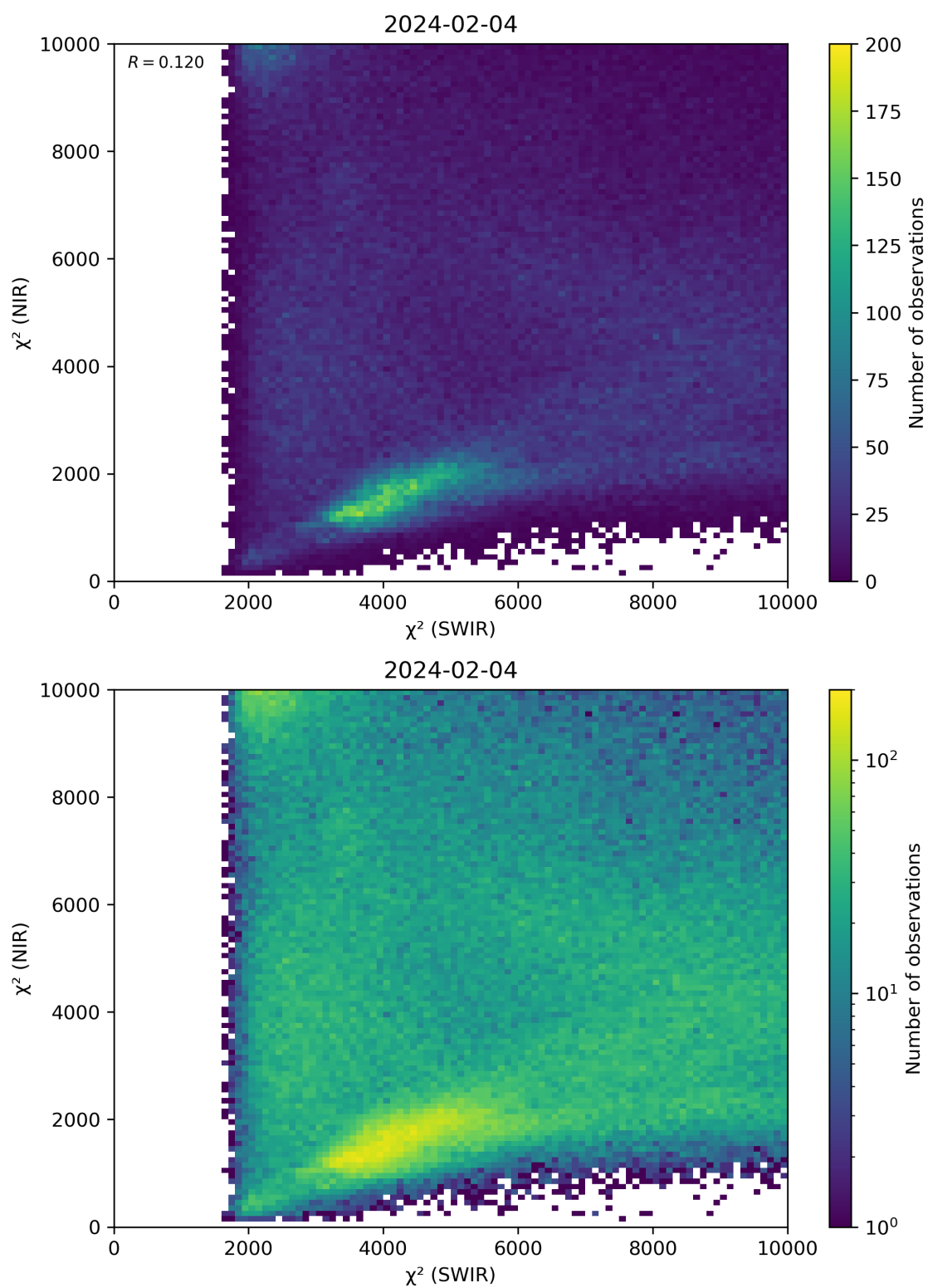
Figure 47: Scatter density plot of “ \chi^2 (SWIR)” against “ \chi^2 (NIR)” for 2024-02-03 to 2024-02-05.
