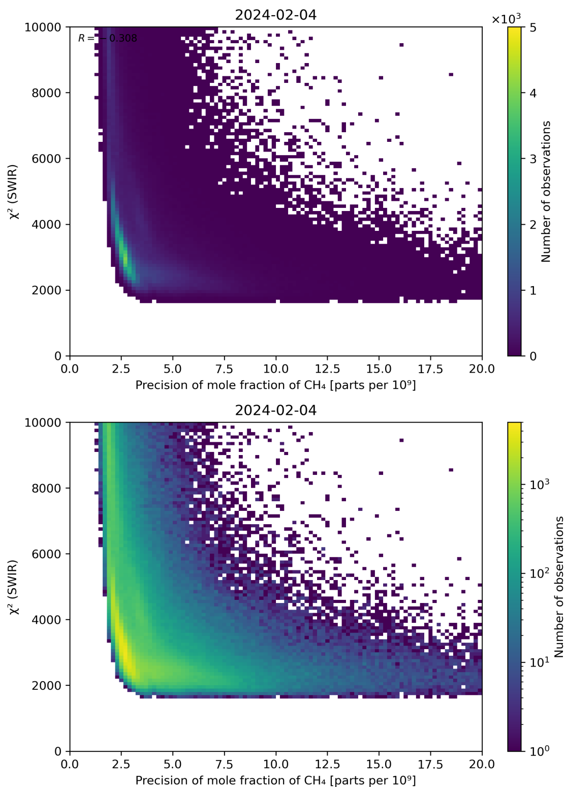
Figure 79: Scatter density plot of “Precision of mole fraction of CH 4 ” against “ \chi^2 (SWIR)” for 2024-02-03 to 2024-02-05.
