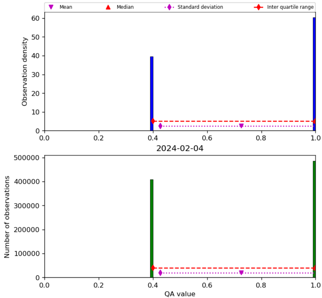
Figure 22: Histogram of “QA value” for 2024-02-03 to 2024-02-05
