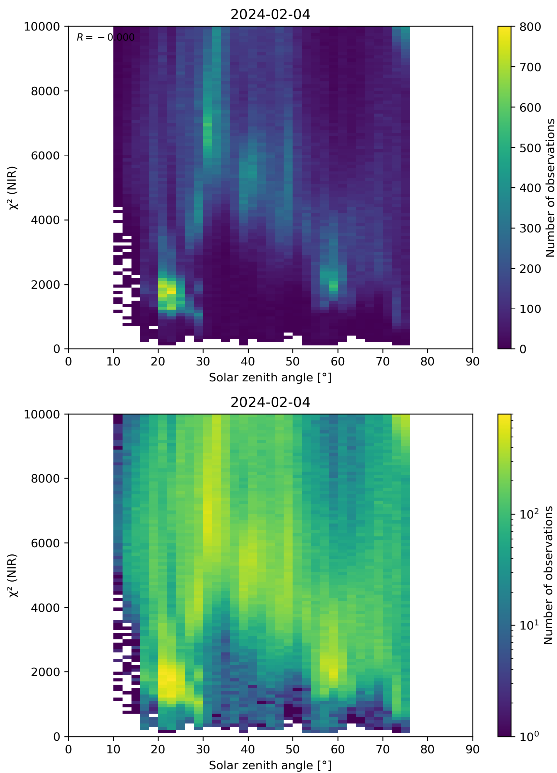
Figure 94: Scatter density plot of “Solar zenith angle” against “ \chi^2 (NIR)” for 2024-02-03 to 2024-02-05.
