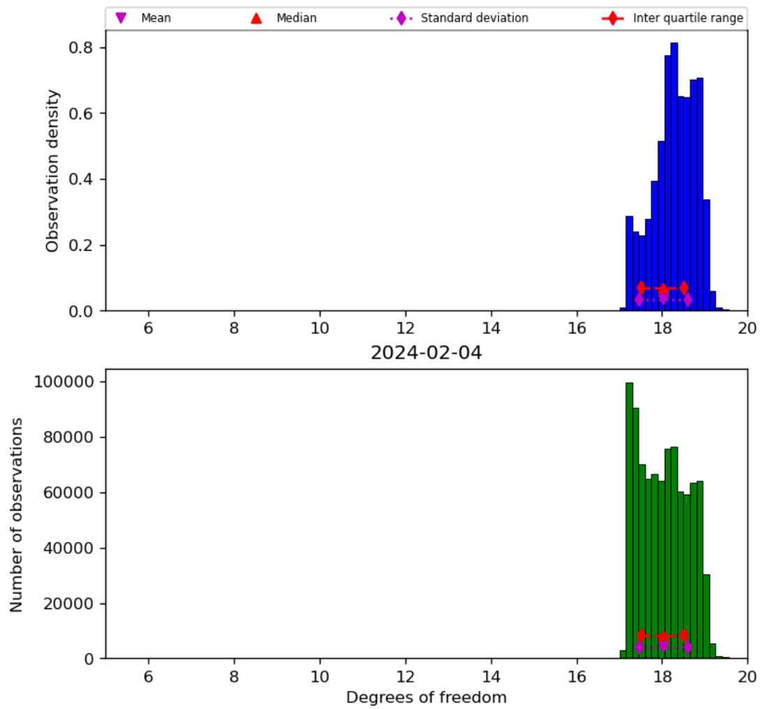
Figure 30: Histogram of “Degrees of freedom” for 2024-02-03 to 2024-02-05
