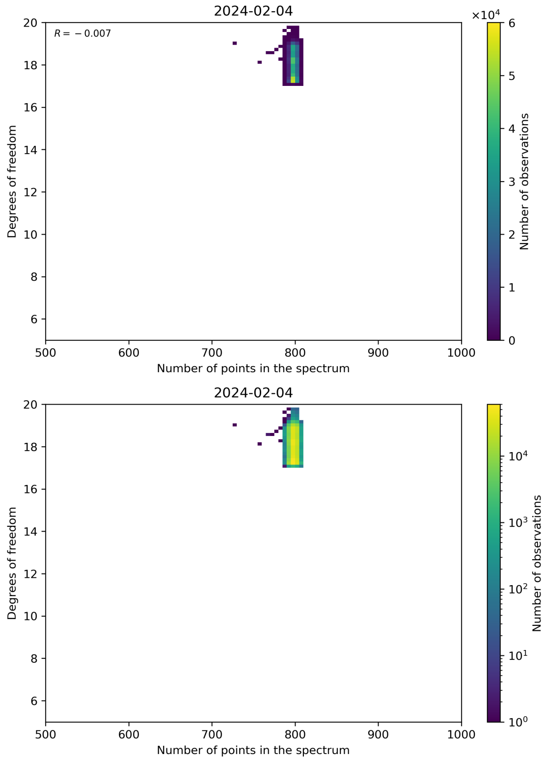
Figure 90: Scatter density plot of “Number of points in the spectrum” against “Degrees of freedom” for 2024-02-03 to 2024-02-05.
