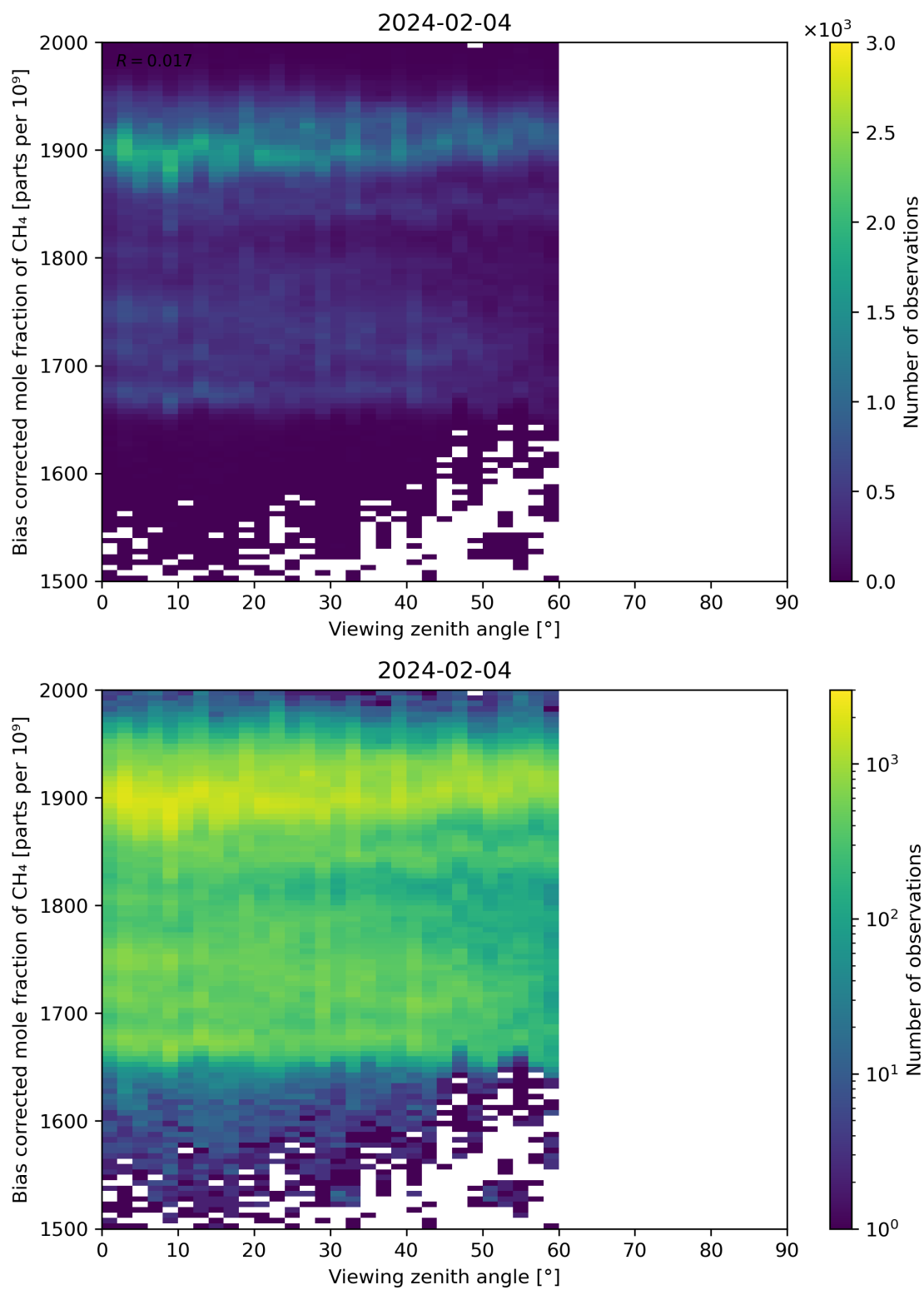
Figure 111: Scatter density plot of “Viewing zenith angle” against “Bias corrected mole fraction of CH 4 ” for 2024-02-03 to 2024-02-05.
