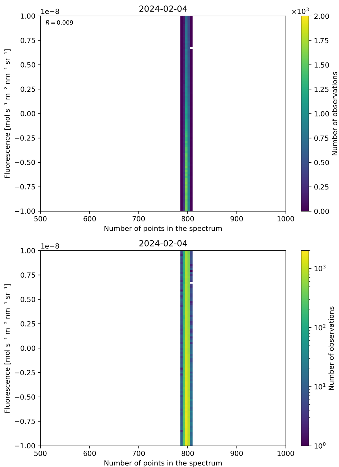
Figure 91: Scatter density plot of “Number of points in the spectrum” against “Fluorescence” for 2024-02-03 to 2024-02-05.
