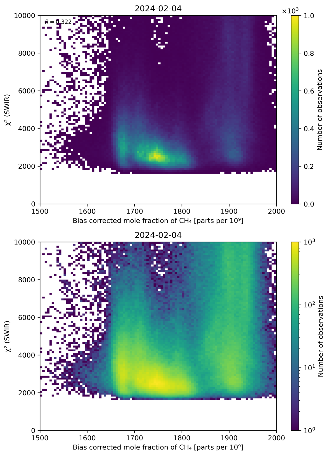
Figure 64: Scatter density plot of “Bias corrected mole fraction of CH 4 ” against “ \chi^2 (SWIR)” for 2024-02-03 to 2024-02-05.
