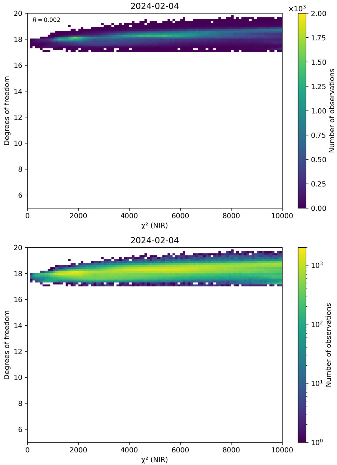
Figure 44: Scatter density plot of “ \chi^2 (NIR)” against “Degrees of freedom” for 2024-02-03 to 2024-02-05.
