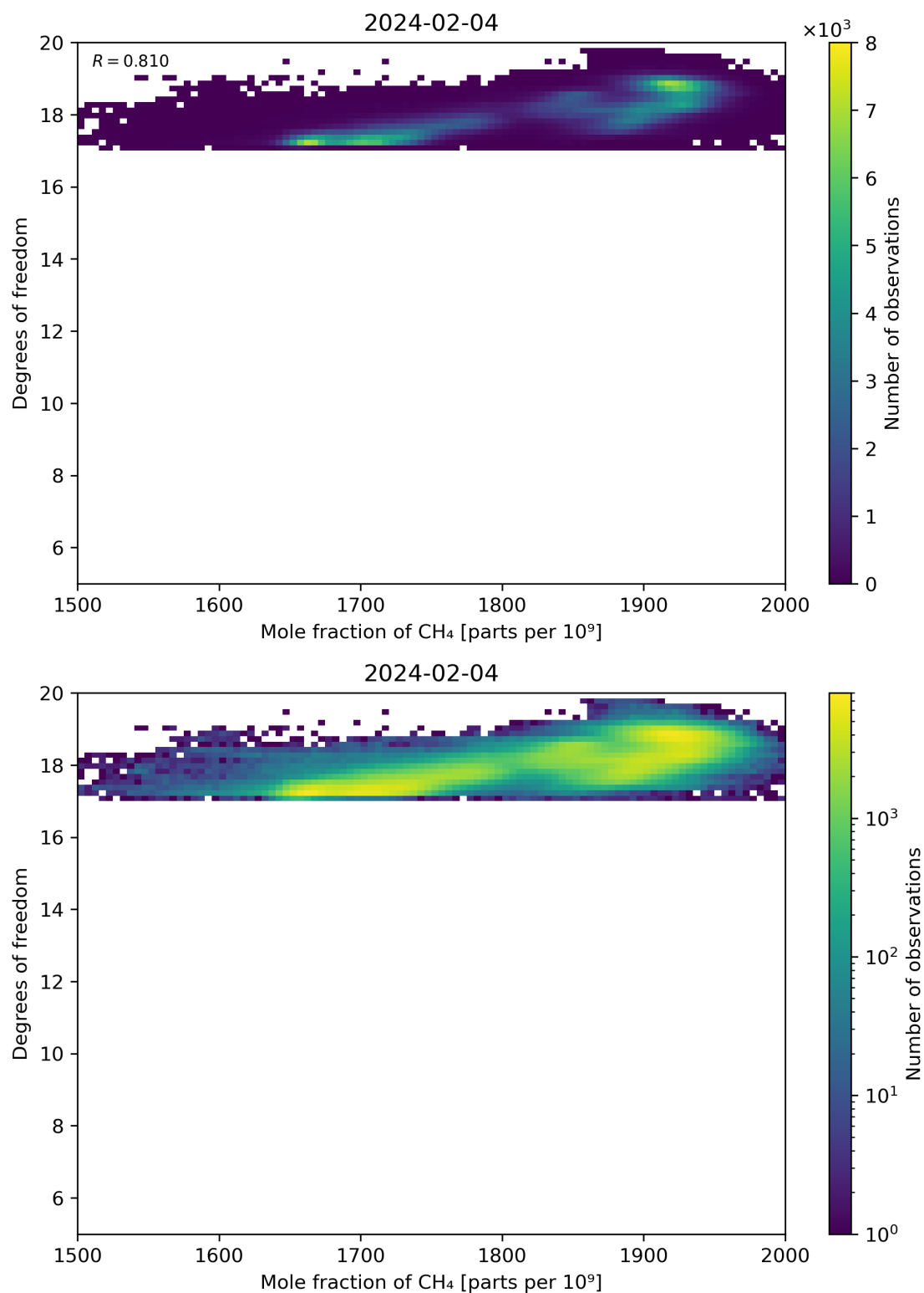
Figure 72: Scatter density plot of “Mole fraction of CH 4 ” against “Degrees of freedom” for 2024-02-03 to 2024-02-05.
