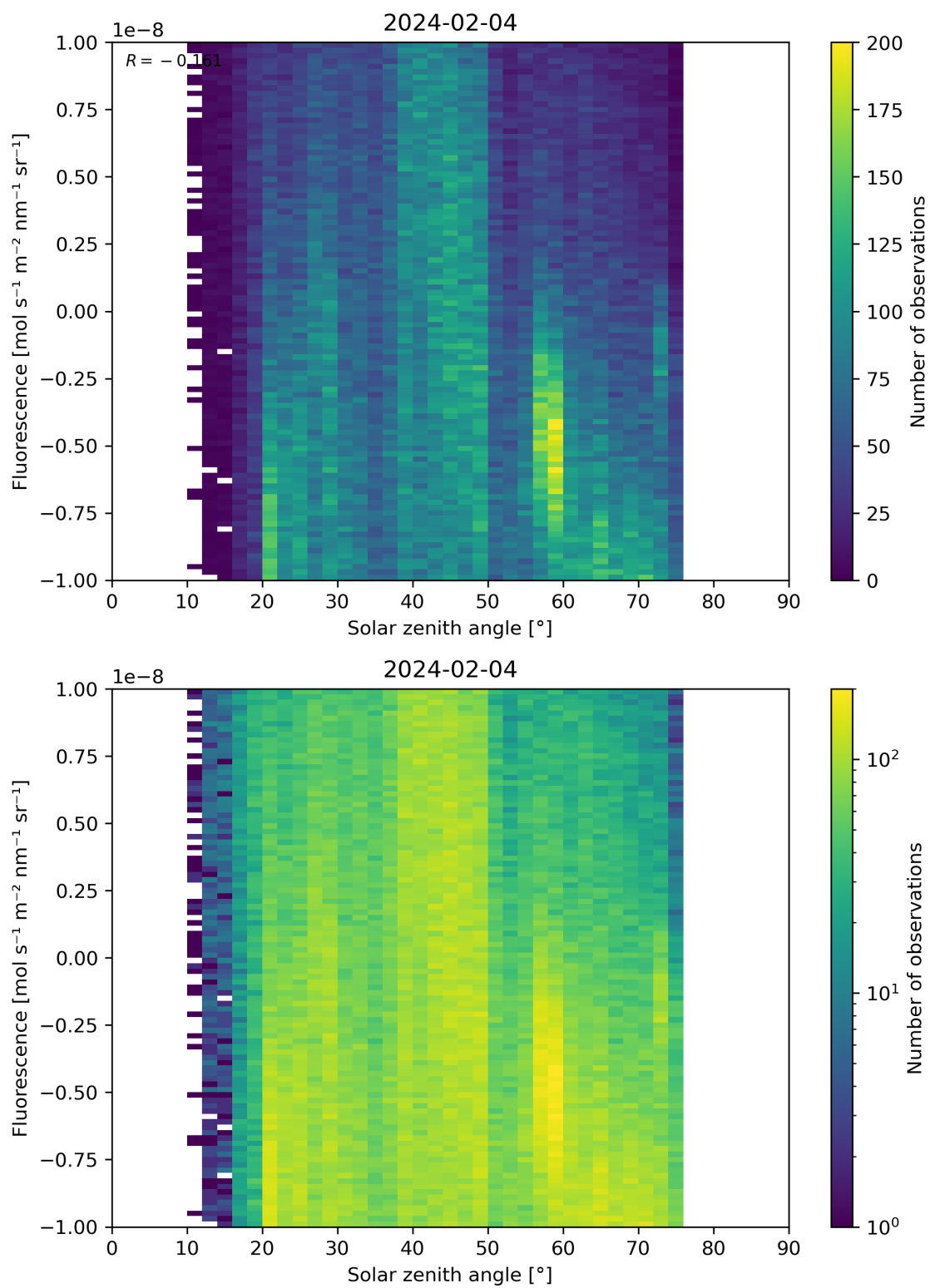
Figure 97: Scatter density plot of “Solar zenith angle” against “Fluorescence” for 2024-02-03 to 2024-02-05.
