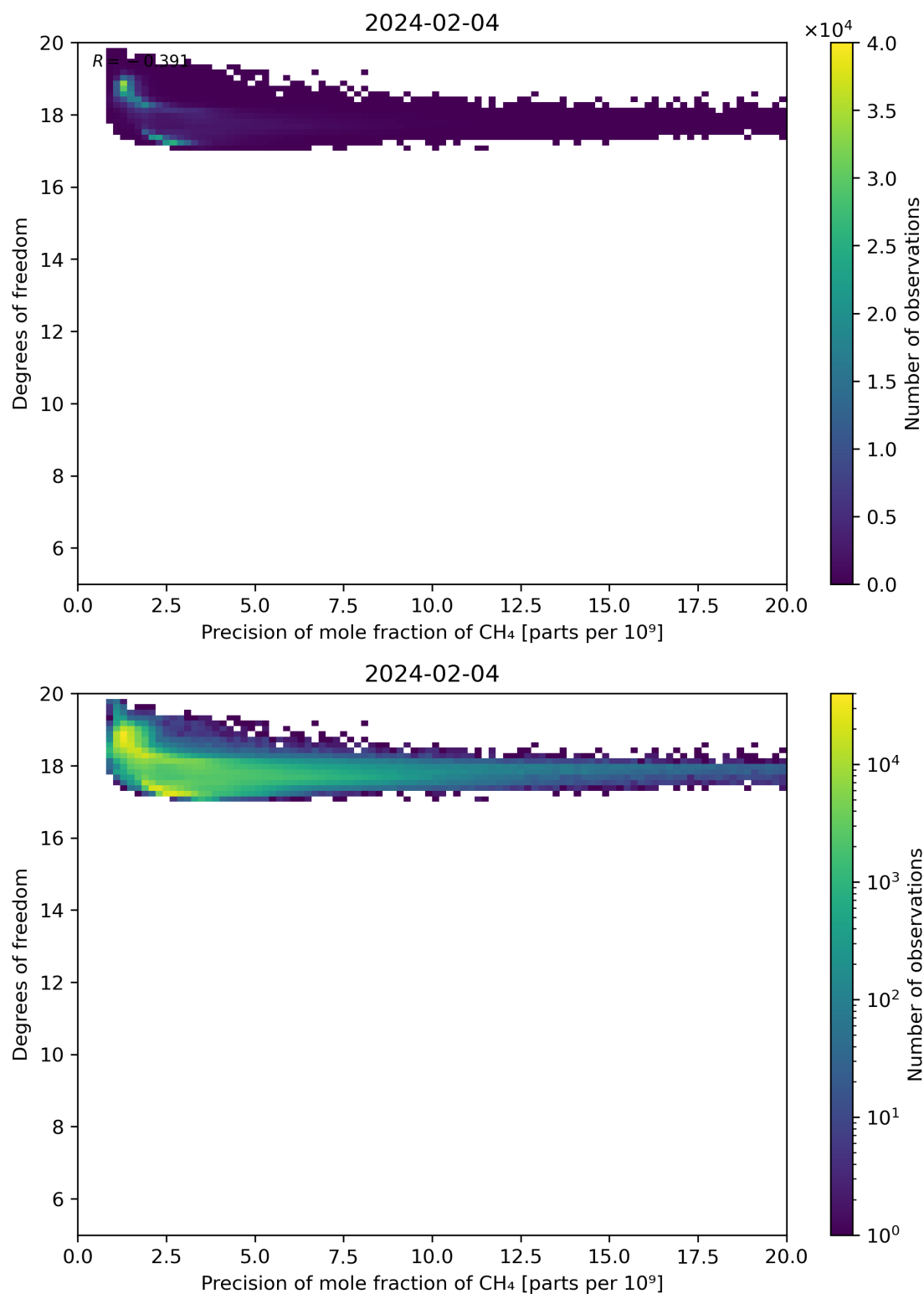
Figure 80: Scatter density plot of “Precision of mole fraction of CH 4 ” against “Degrees of freedom” for 2024-02-03 to 2024-02-05.
