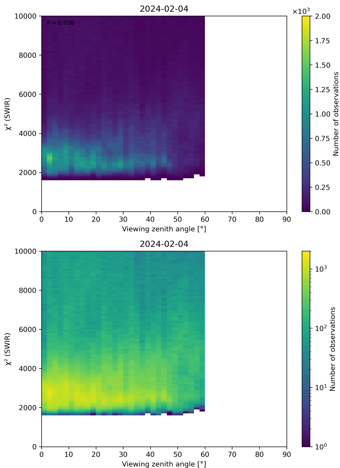
Figure 106: Scatter density plot of “Viewing zenith angle” against “ \chi^2 (SWIR)” for 2024-02-03 to 2024-02-05.
