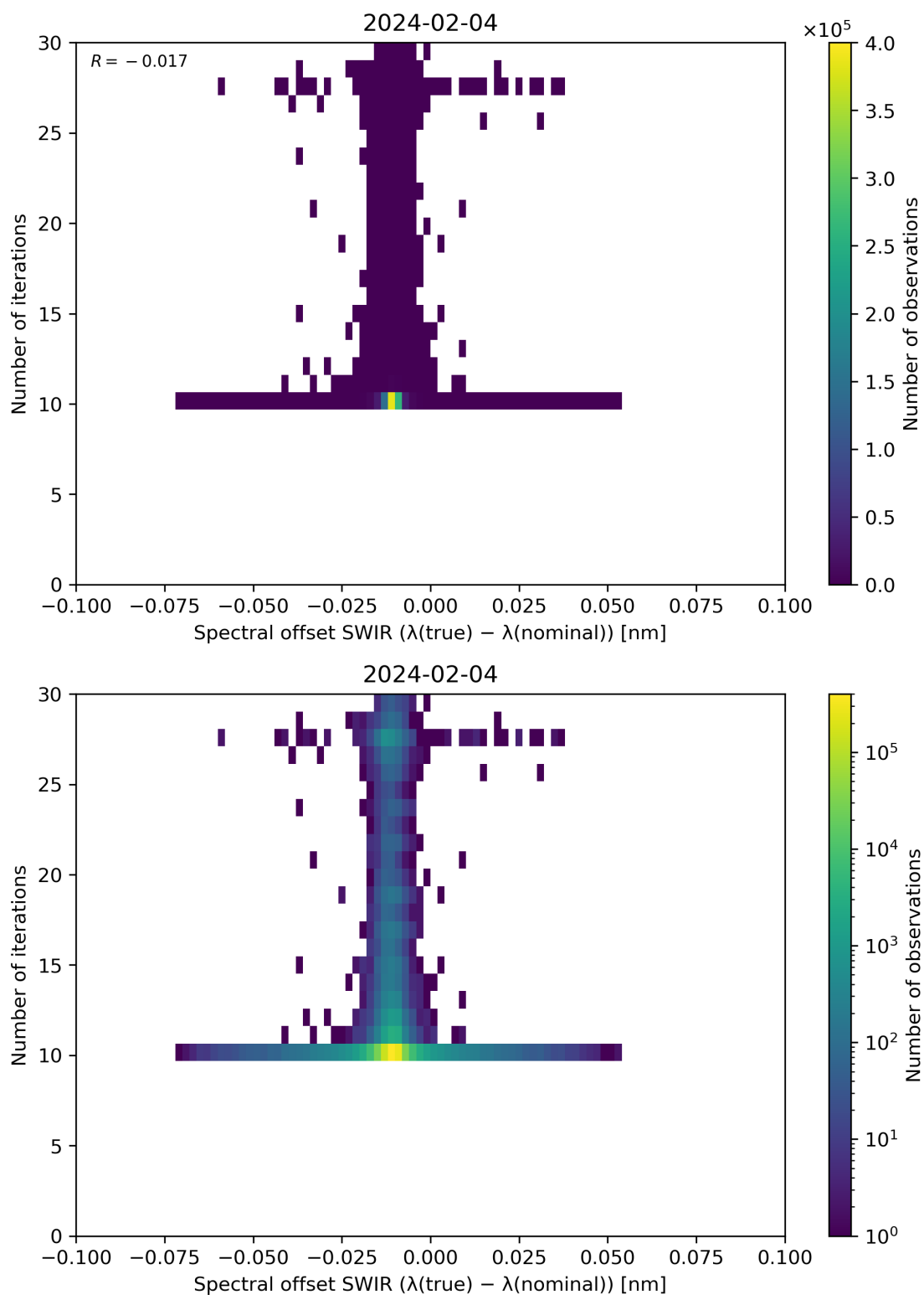
Figure 121: Scatter density plot of “Spectral offset SWIR ( \lambda(\text{true}) - \lambda(\text{nominal}) )” against “Number of iterations” for 2024-02-03 to 2024-02-05.
