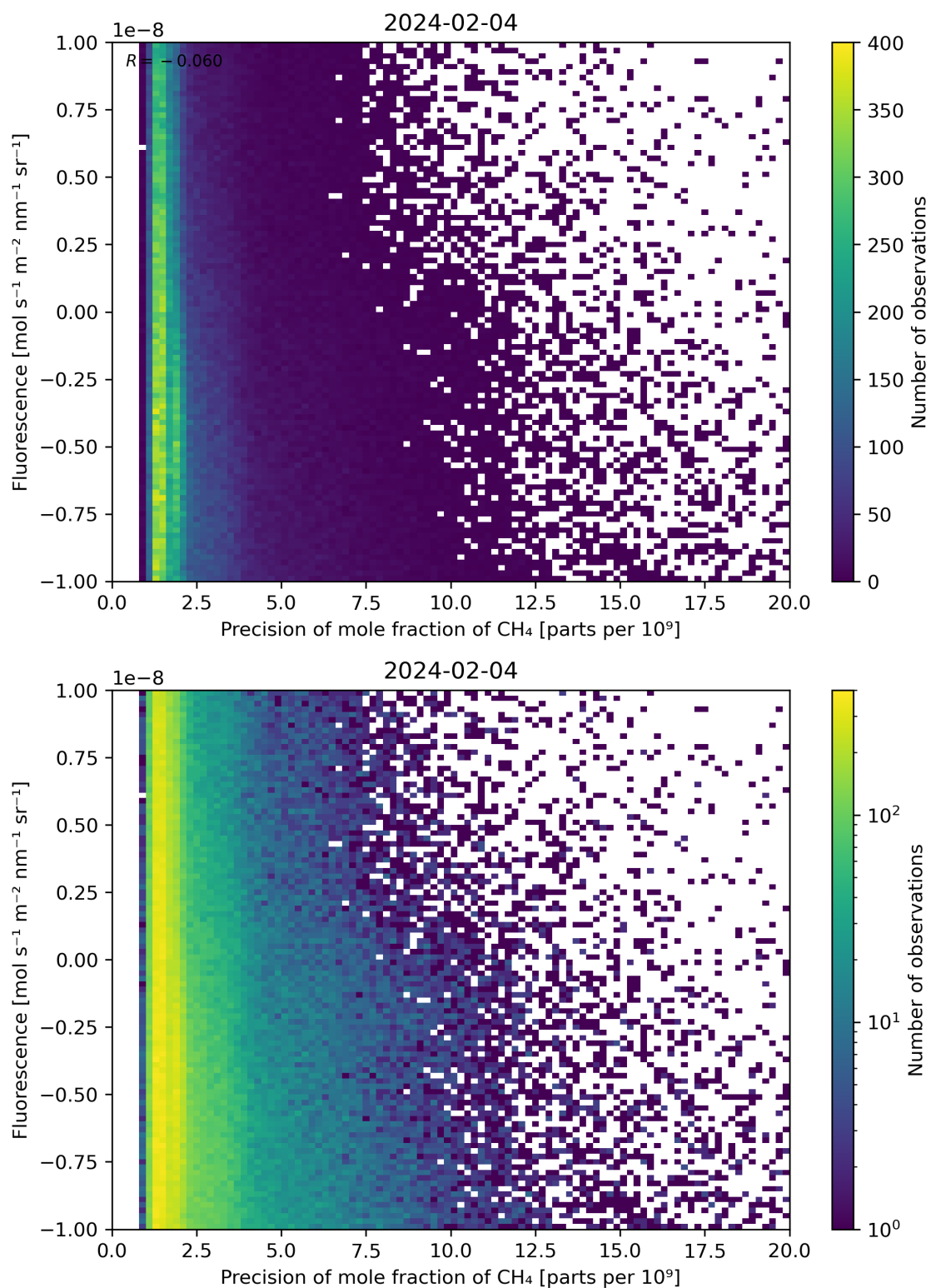
Figure 81: Scatter density plot of “Precision of mole fraction of \text{CH}_4 ” against “Fluorescence” for 2024-02-03 to 2024-02-05.
