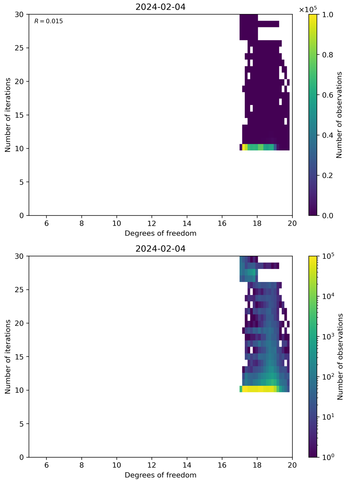
Figure 52: Scatter density plot of “Degrees of freedom” against “Number of iterations” for 2024-02-03 to 2024-02-05.
