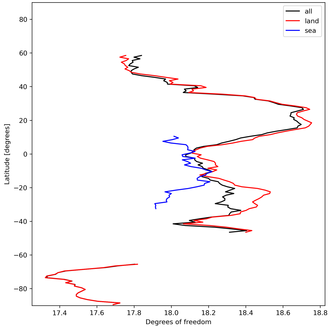
Figure 19: Zonal average of “Degrees of freedom” for 2024-02-03 to 2024-02-05.
