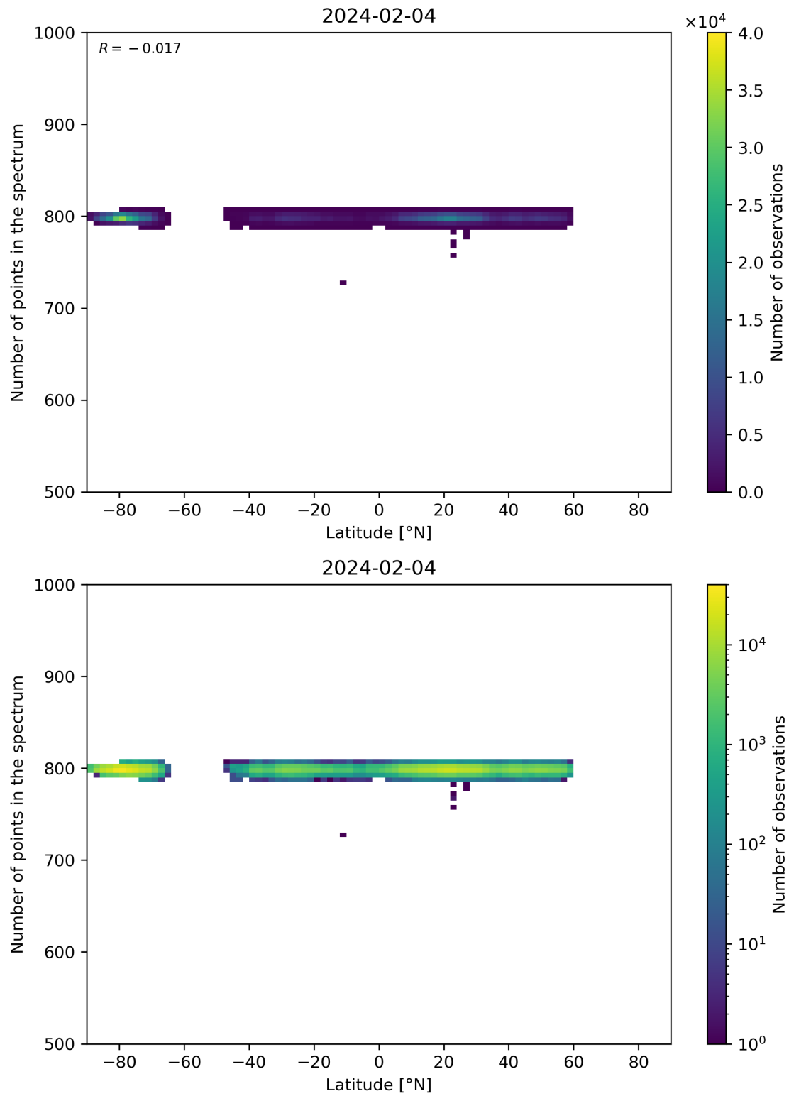
Figure 61: Scatter density plot of “Latitude” against “Number of points in the spectrum” for 2024-02-03 to 2024-02-05.
