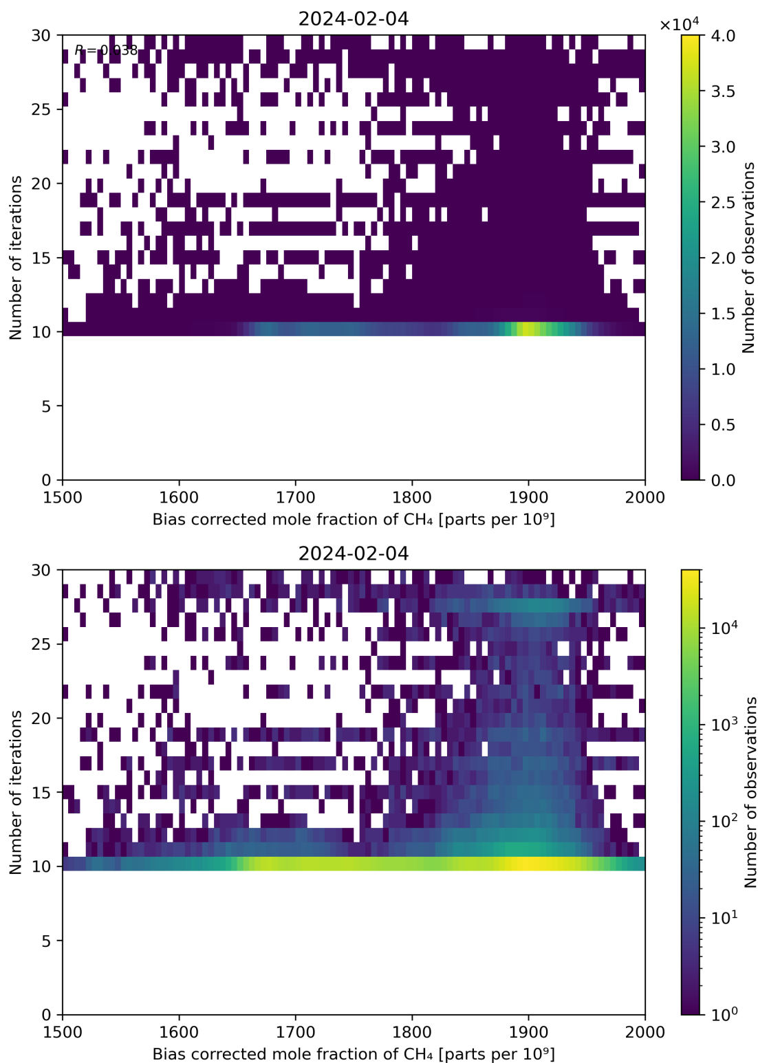
Figure 67: Scatter density plot of “Bias corrected mole fraction of \text{CH}_4 ” against “Number of iterations” for 2024-02-03 to 2024-02-05.
