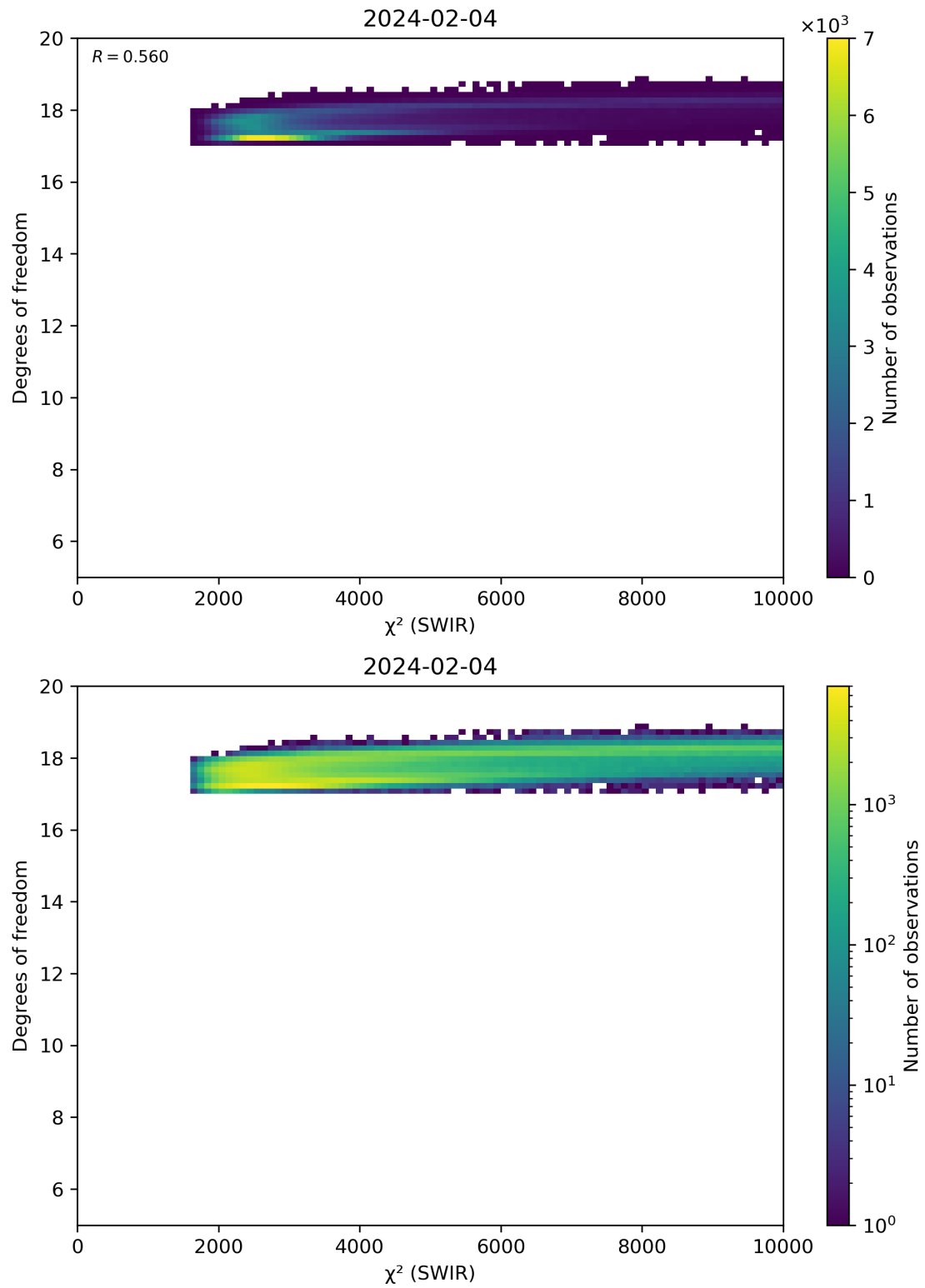
Figure 48: Scatter density plot of “ \chi^2 (SWIR)” against “Degrees of freedom” for 2024-02-03 to 2024-02-05.
