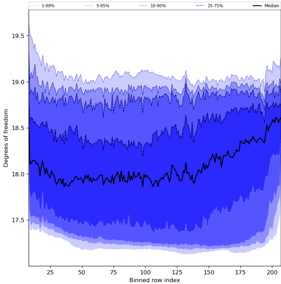
Figure 41: Along track statistics of “Degrees of freedom” for 2024-02-03 to 2024-02-05
