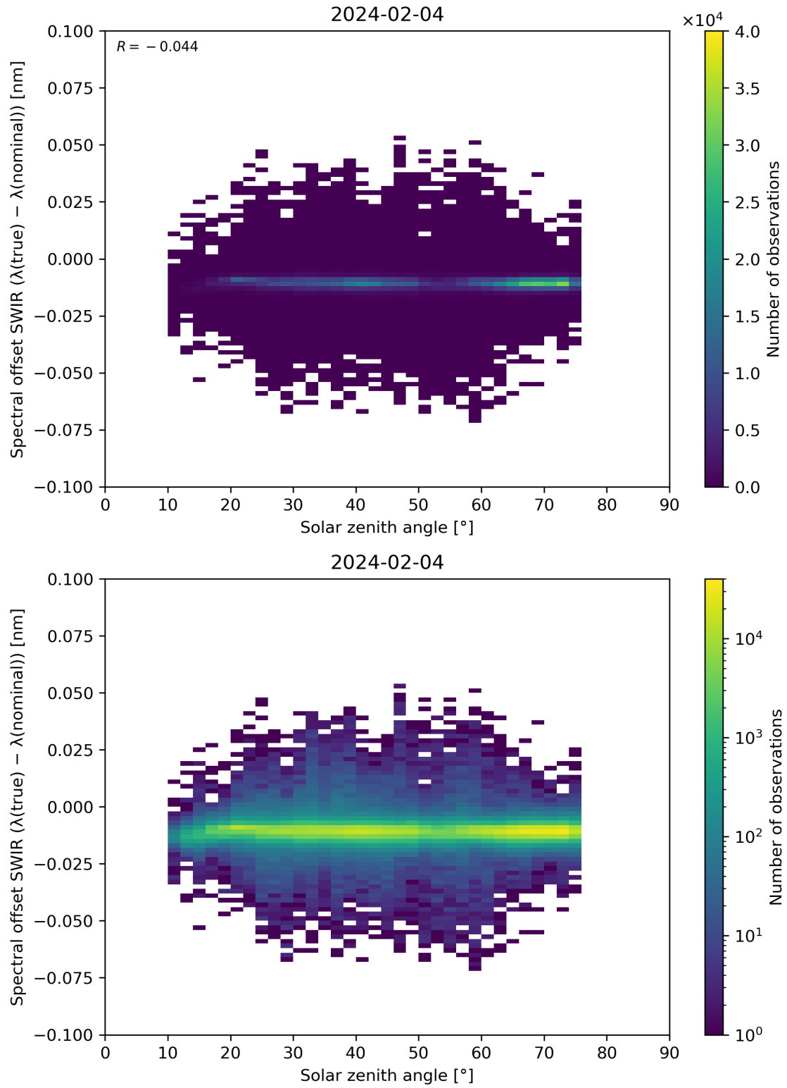
Figure 104: Scatter density plot of “Solar zenith angle” against “Spectral offset SWIR ( \lambda(\text{true}) - \lambda(\text{nominal}) )” for 2024-02-03 to 2024-02-05.
