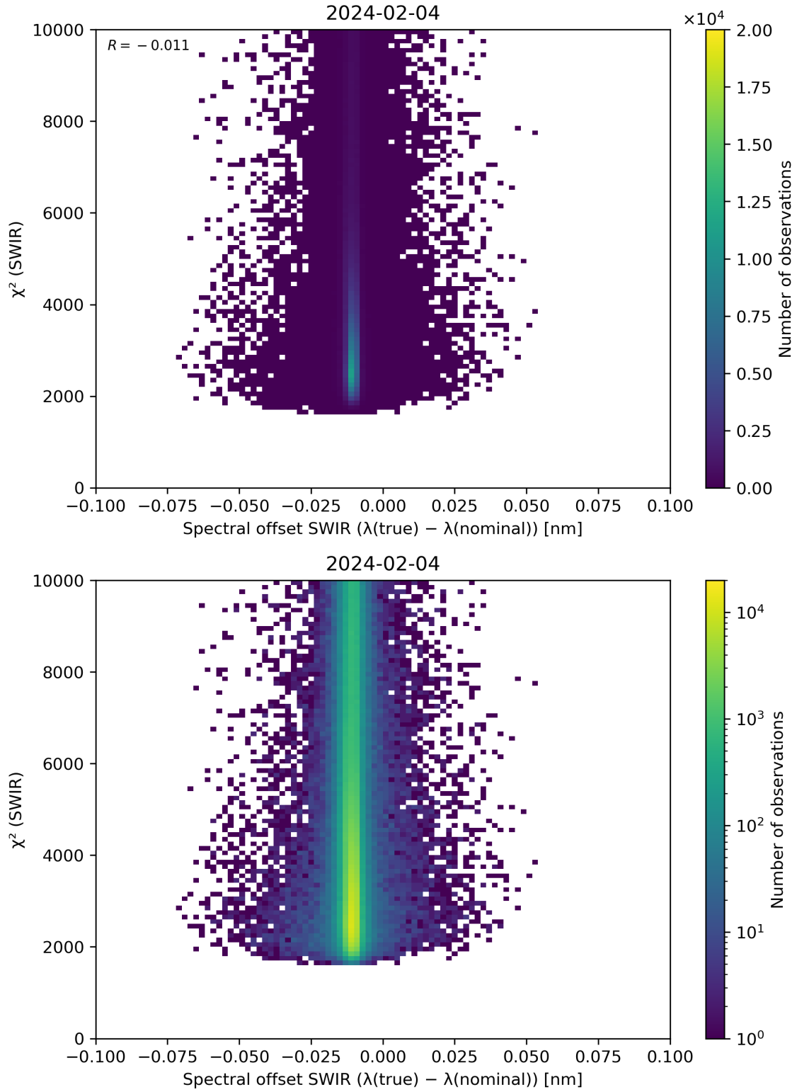
Figure 118: Scatter density plot of “Spectral offset SWIR ( \lambda(\text{true}) - \lambda(\text{nominal}) )” against “ \chi^2 (SWIR)” for 2024-02-03 to 2024-02-05.
