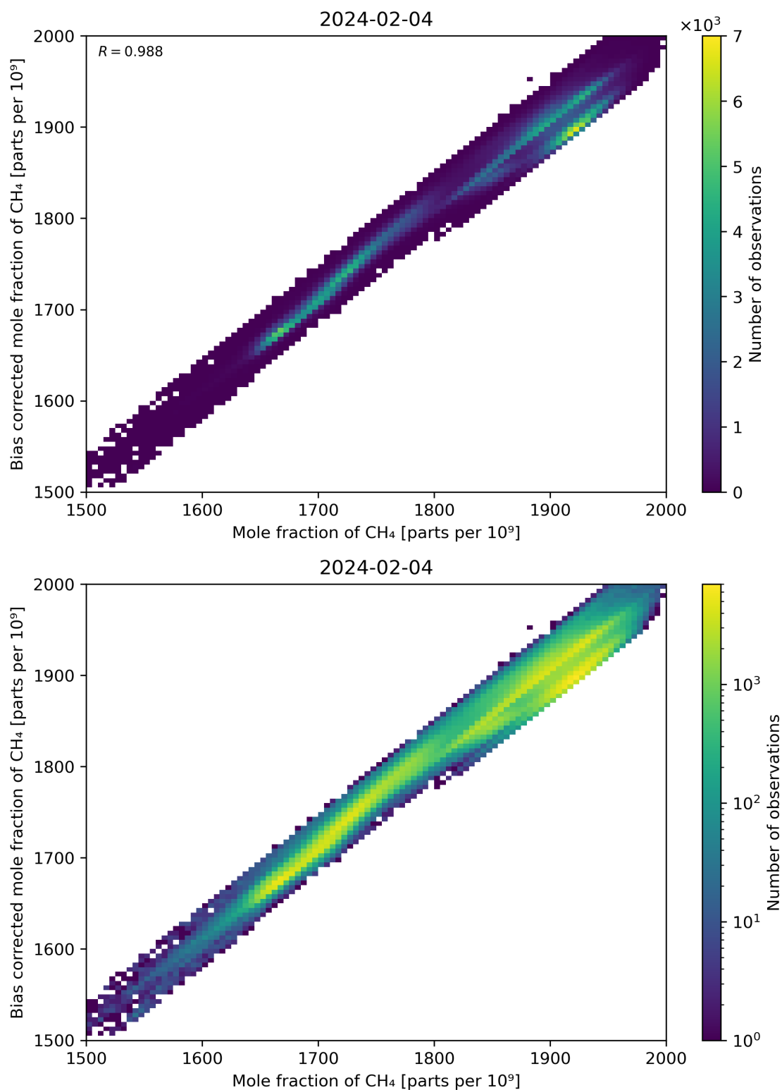
Figure 74: Scatter density plot of “Mole fraction of CH 4 ” against “Bias corrected mole fraction of CH 4 ” for 2024-02-03 to 2024-02-05.
