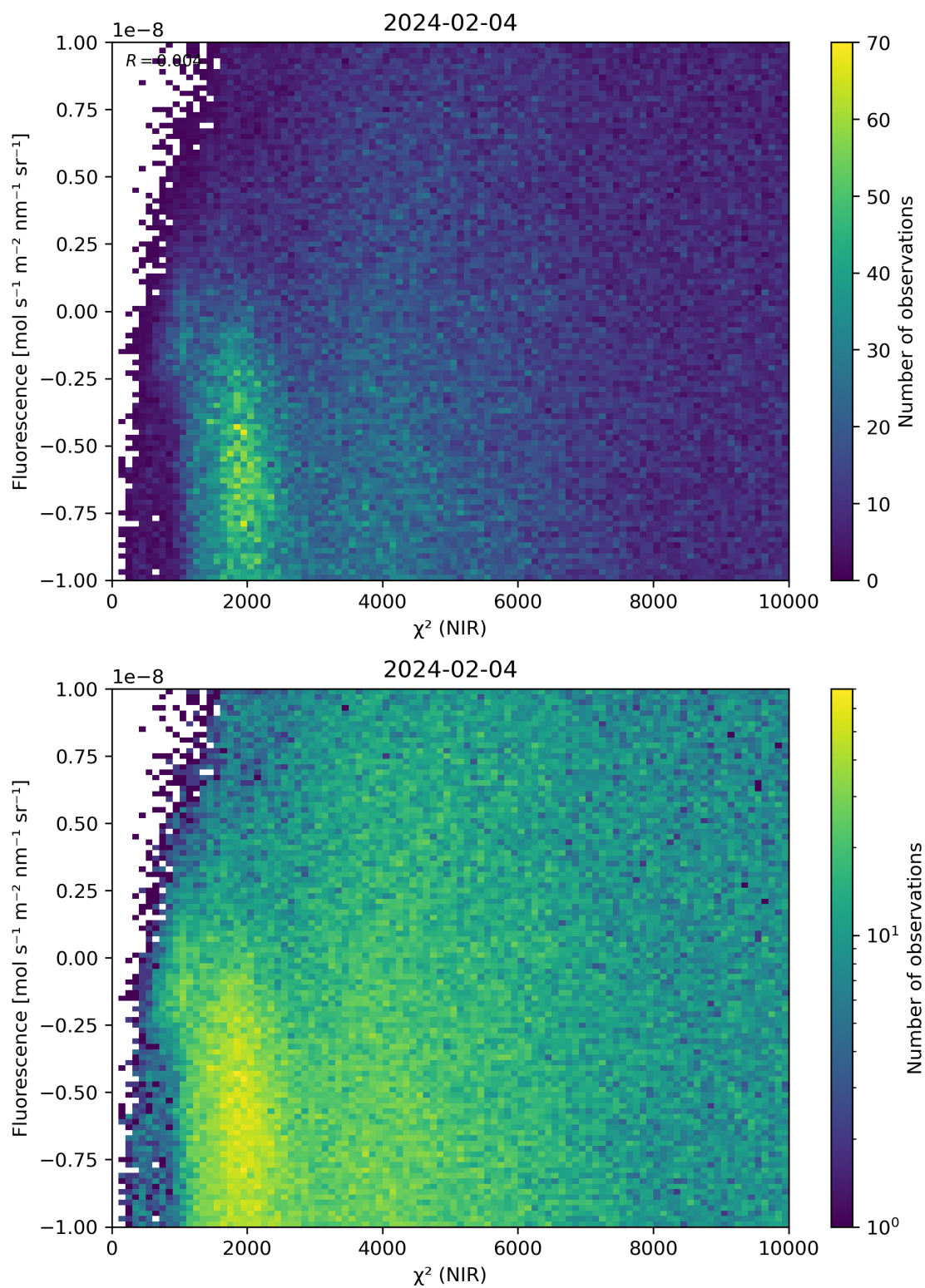
Figure 45: Scatter density plot of “ \chi^2 (NIR)” against “Fluorescence” for 2024-02-03 to 2024-02-05.
