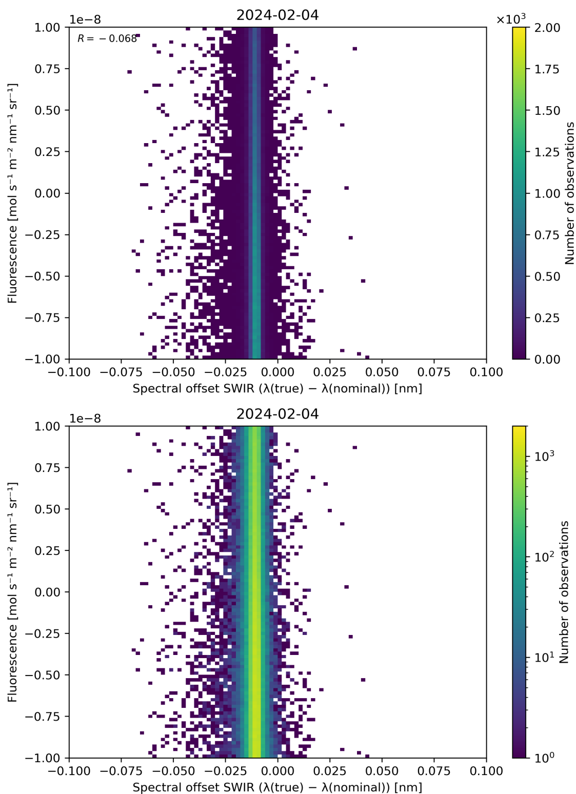
Figure 120: Scatter density plot of “Spectral offset SWIR ( \lambda(\text{true}) - \lambda(\text{nominal}) )” against “Fluorescence” for 2024-02-03 to 2024-02-05.
