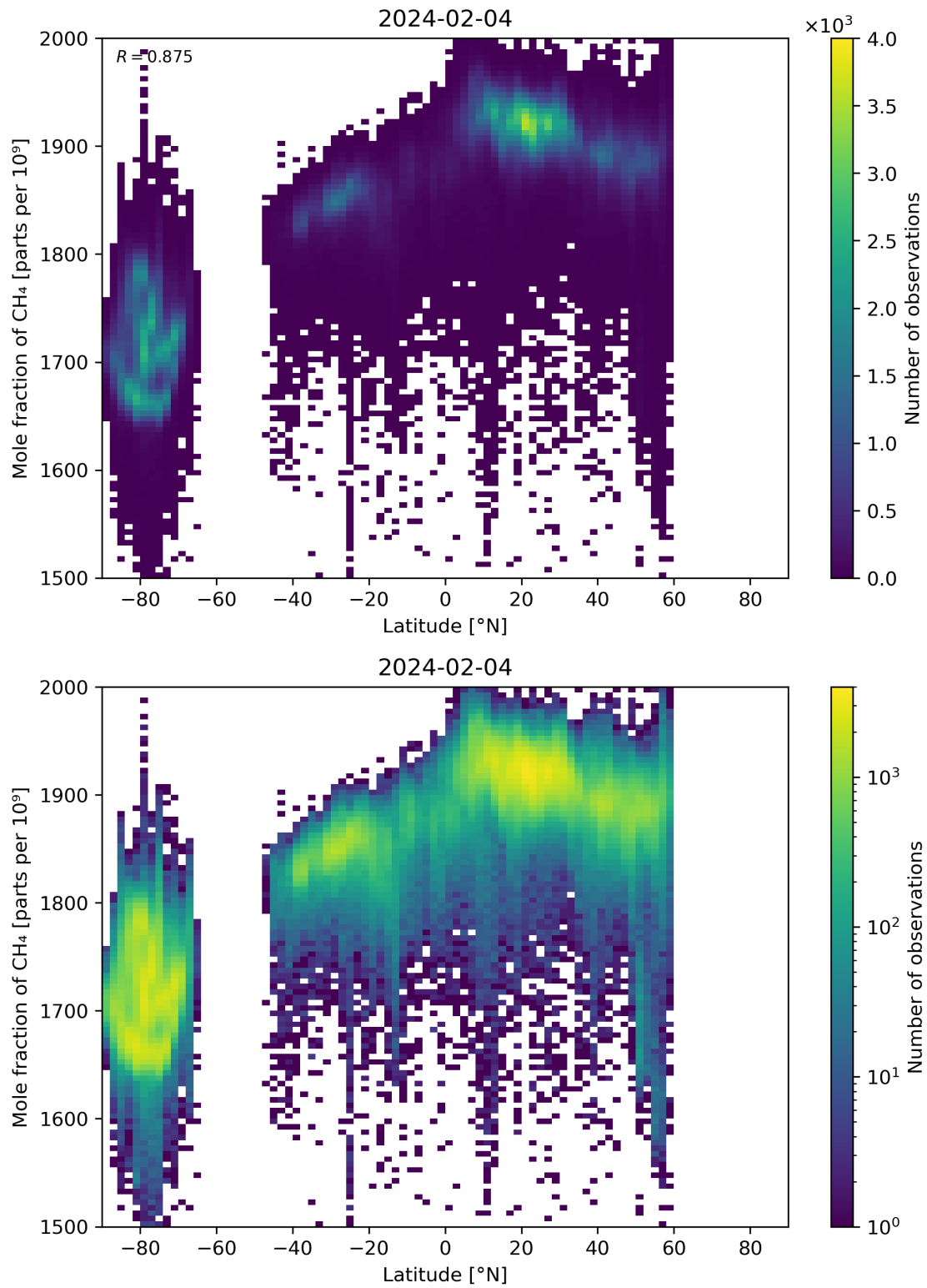
Figure 57: Scatter density plot of “Latitude” against “Mole fraction of CH 4 ” for 2024-02-03 to 2024-02-05.
