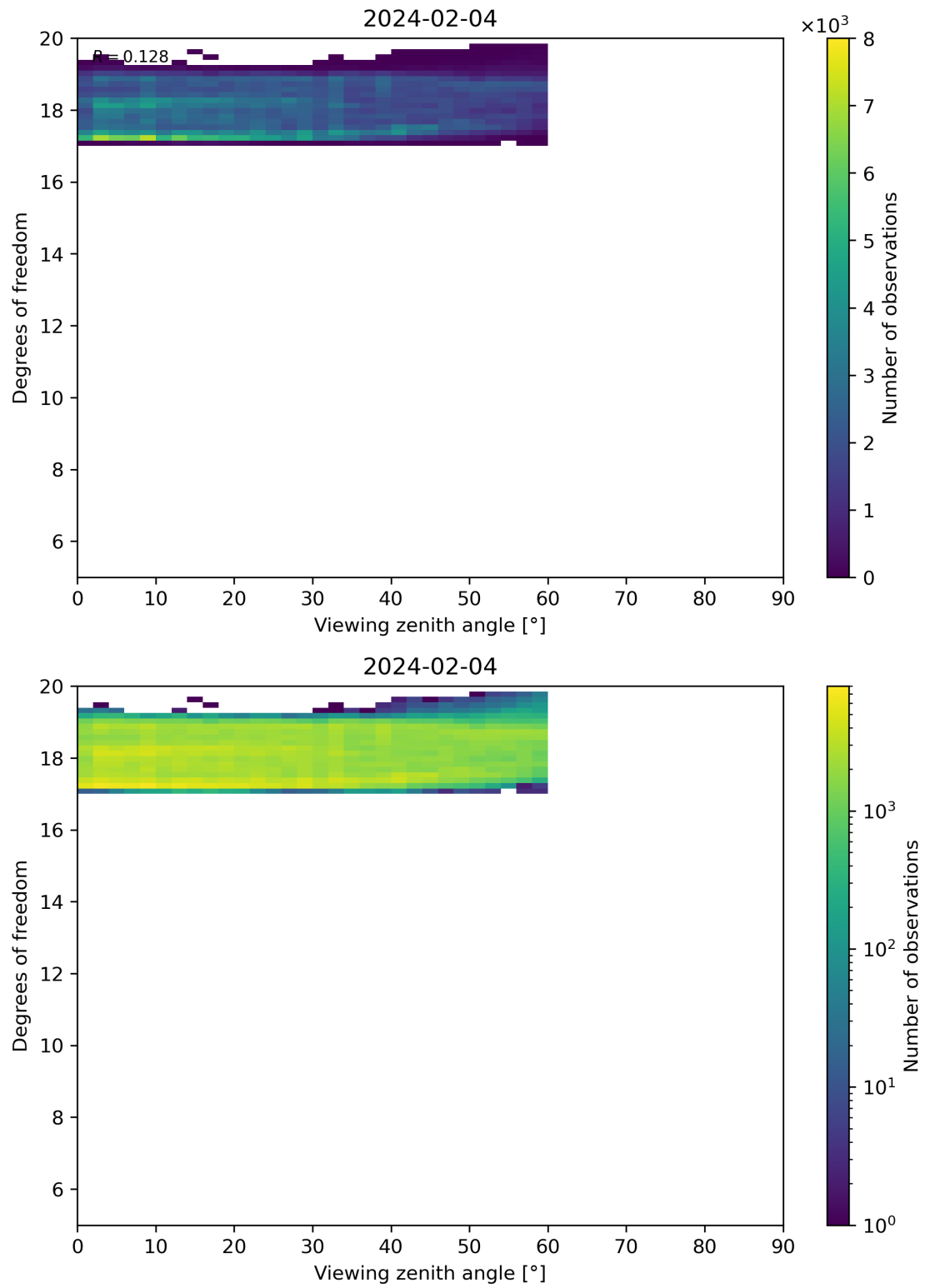
Figure 107: Scatter density plot of “Viewing zenith angle” against “Degrees of freedom” for 2024-02-03 to 2024-02-05.
