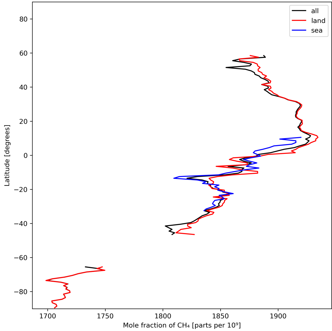
Figure 12: Zonal average of “Mole fraction of \text{CH}_4 ” for 2024-02-03 to 2024-02-05.
