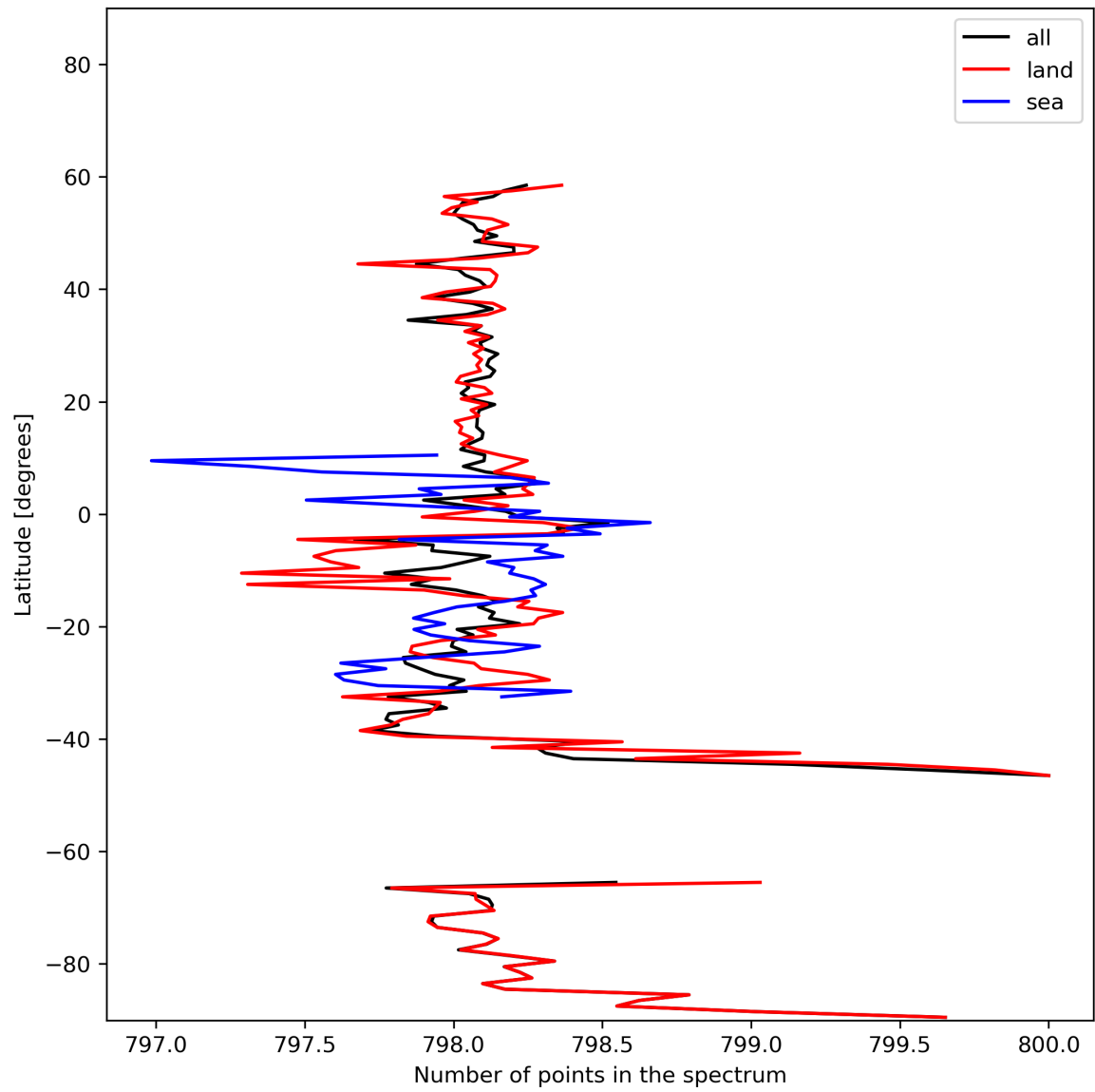
Figure 15: Zonal average of “Number of points in the spectrum” for 2024-02-03 to 2024-02-05.
