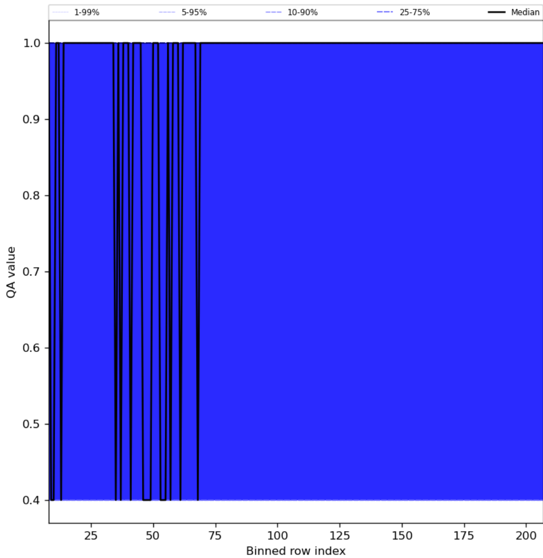
Figure 33: Along track statistics of “QA value” for 2024-02-03 to 2024-02-05
