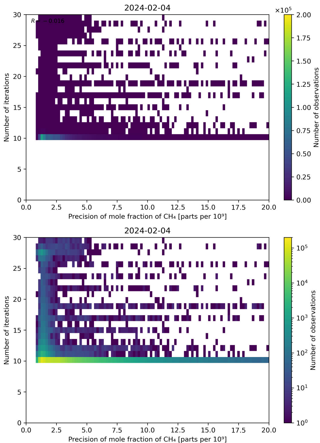
Figure 83: Scatter density plot of “Precision of mole fraction of CH 4 ” against “Number of iterations” for 2024-02-03 to 2024-02-05.
