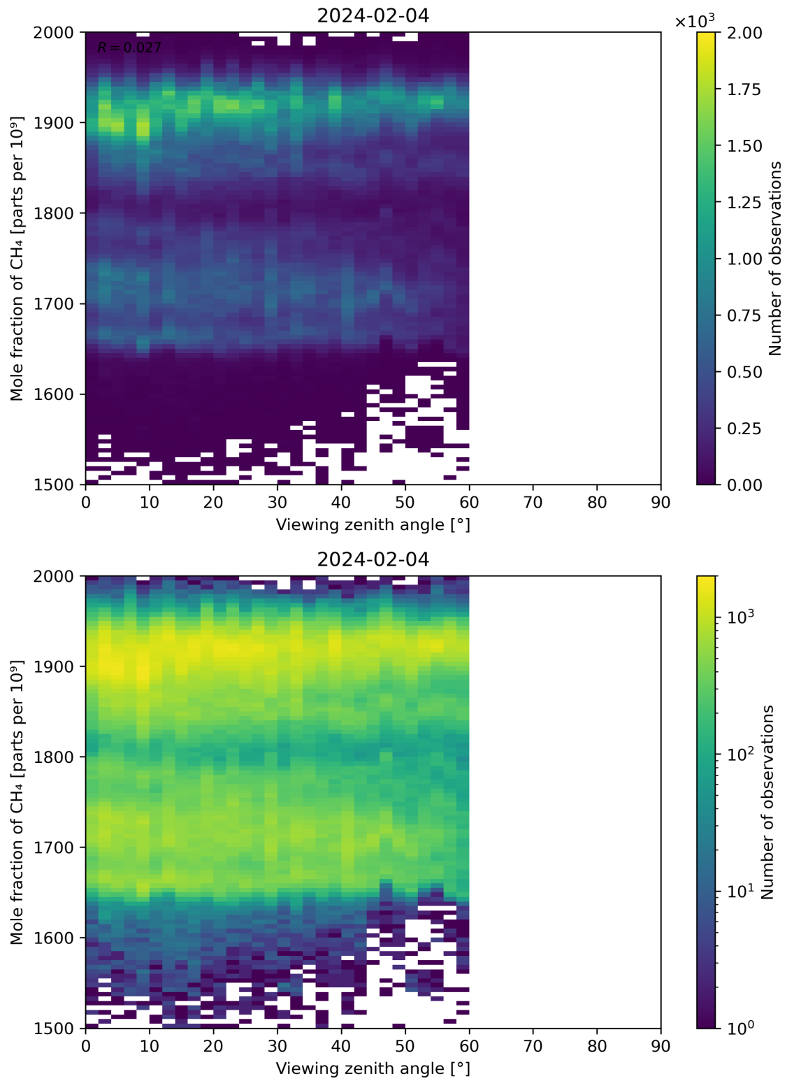
Figure 110: Scatter density plot of “Viewing zenith angle” against “Mole fraction of CH 4 ” for 2024-02-03 to 2024-02-05.
