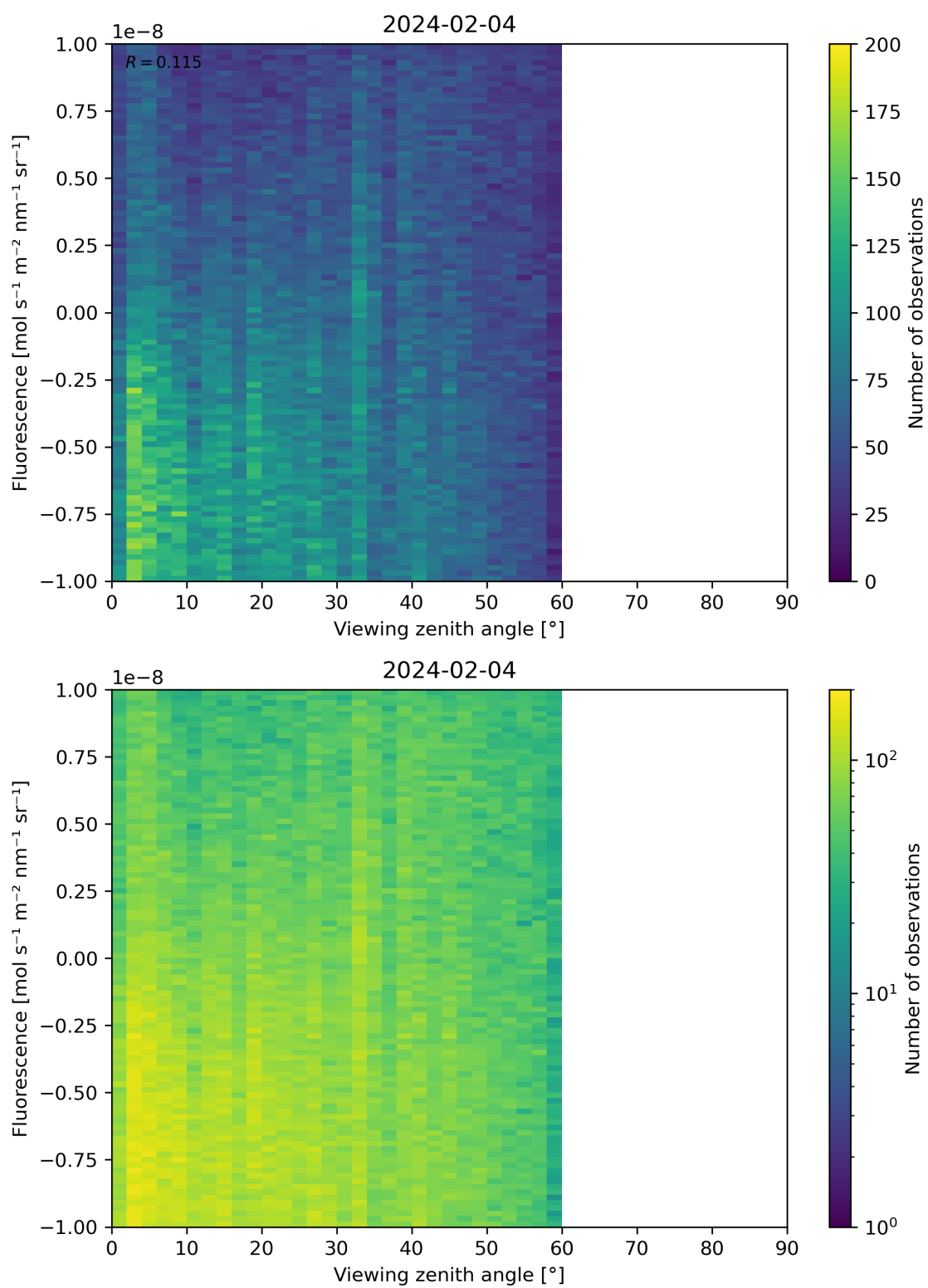
Figure 108: Scatter density plot of “Viewing zenith angle” against “Fluorescence” for 2024-02-03 to 2024-02-05.
