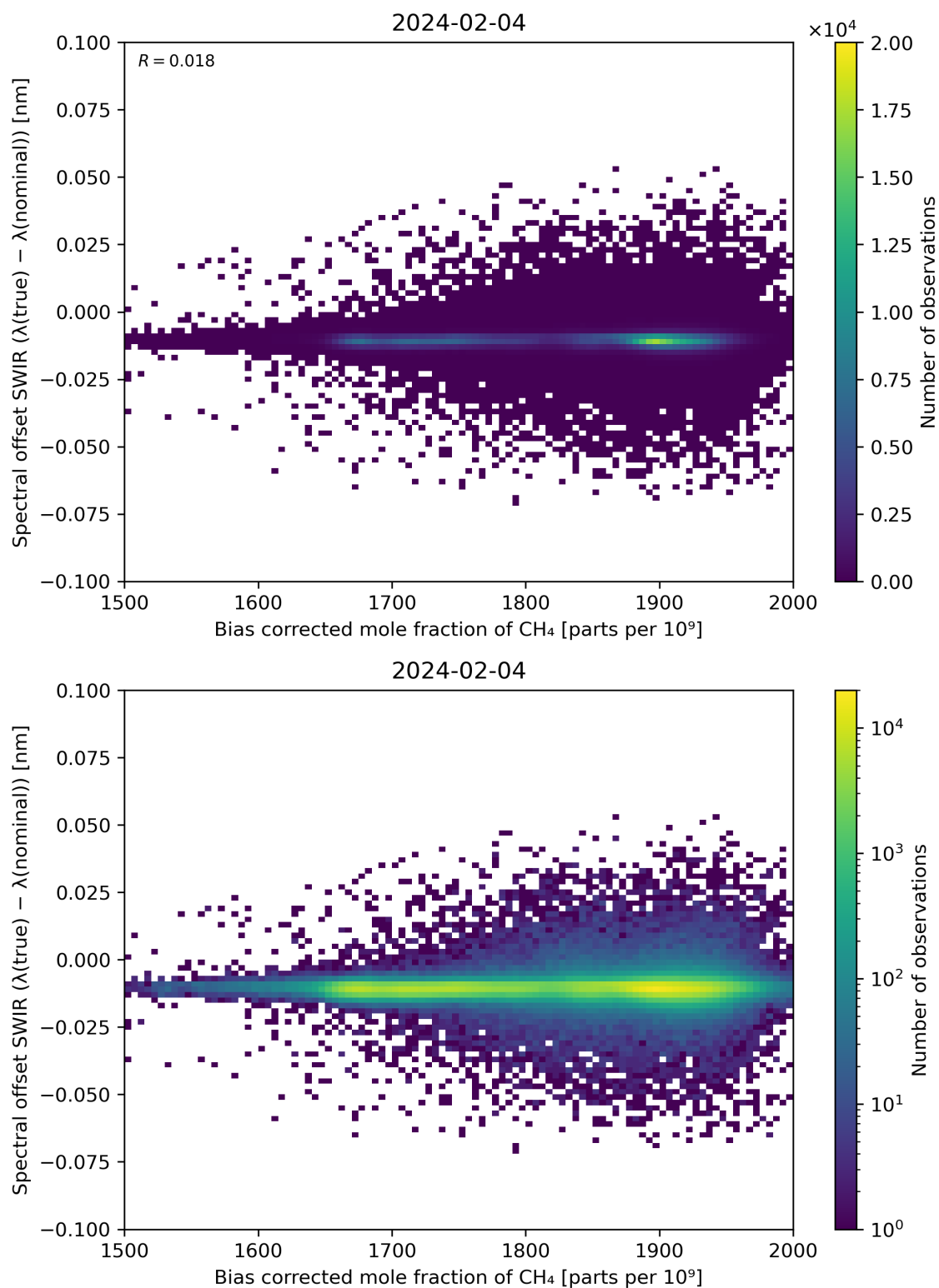
Figure 69: Scatter density plot of “Bias corrected mole fraction of \text{CH}_4 ” against “Spectral offset SWIR ( \lambda(\text{true}) - \lambda(\text{nominal}) )” for 2024-02-03 to 2024-02-05.
