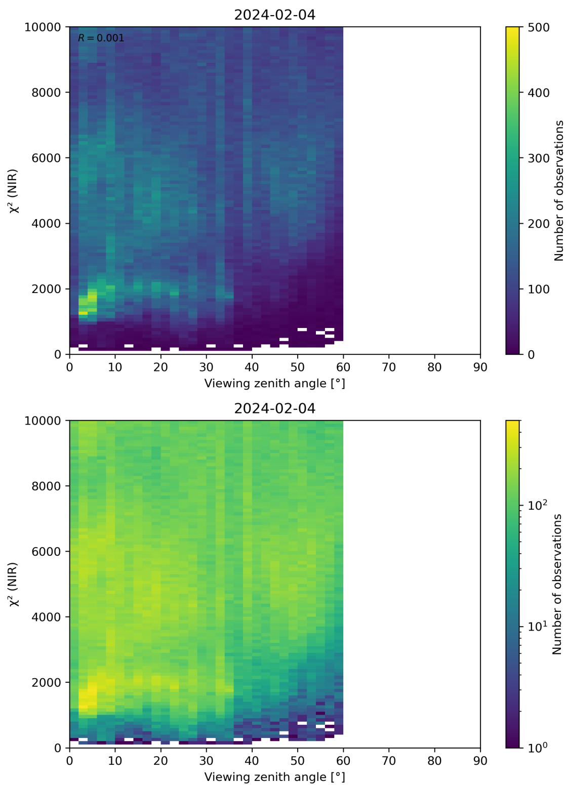
Figure 105: Scatter density plot of “Viewing zenith angle” against “ \chi^2 (NIR)” for 2024-02-03 to 2024-02-05.
