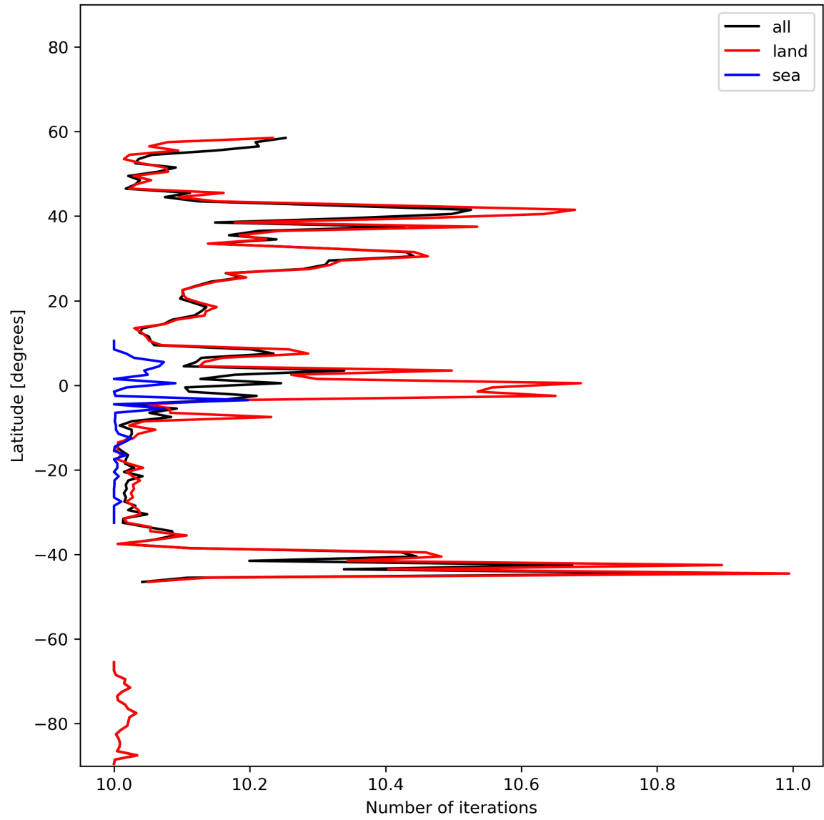
Figure 20: Zonal average of “Number of iterations” for 2024-02-03 to 2024-02-05.
