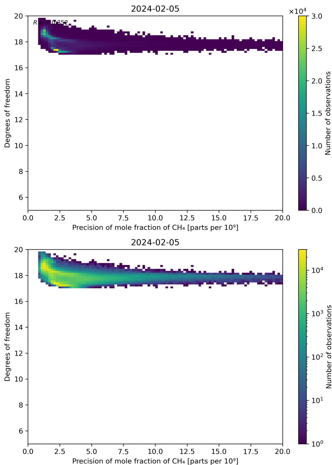
Figure 80: Scatter density plot of “Precision of mole fraction of CH 4 ” against “Degrees of freedom” for 2024-02-04 to 2024-02-06.
