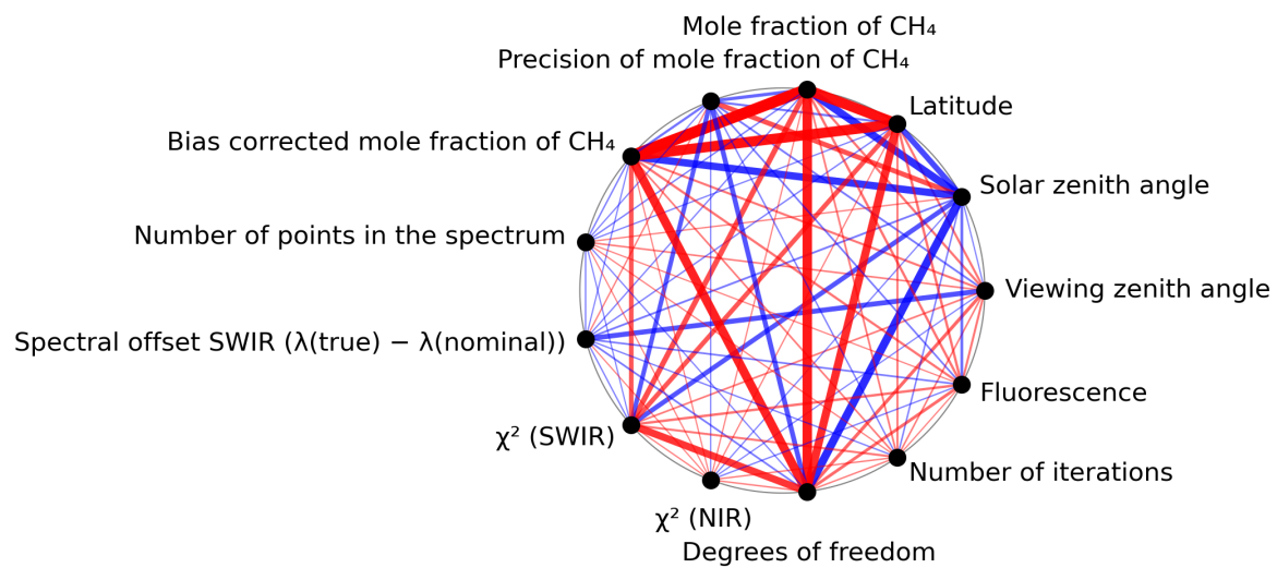
Figure 1: Map of correlation graph for 2024-02-04 to 2024-02-06.
