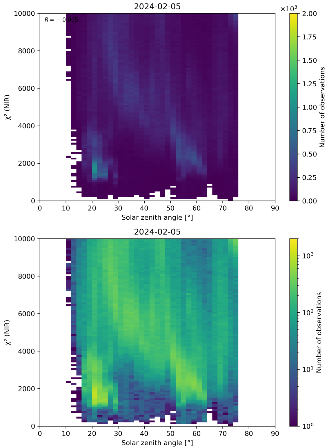
Figure 94: Scatter density plot of “Solar zenith angle” against “ \chi^2 (NIR)” for 2024-02-04 to 2024-02-06.
