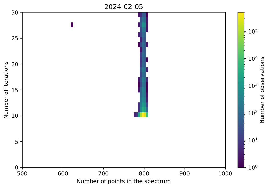
Figure 92: Scatter density plot of “Number of points in the spectrum” against “Number of iterations” for 2024-02-04 to 2024-02-06.
