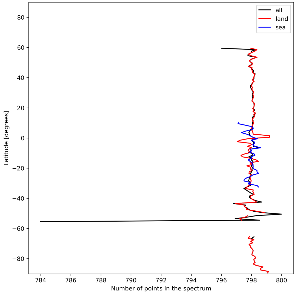
Figure 15: Zonal average of “Number of points in the spectrum” for 2024-02-04 to 2024-02-06.
