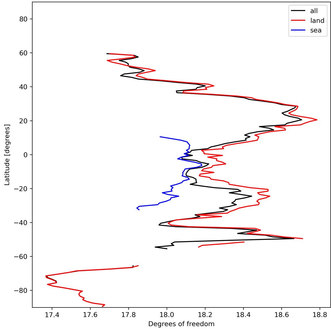
Figure 19: Zonal average of “Degrees of freedom” for 2024-02-04 to 2024-02-06.
