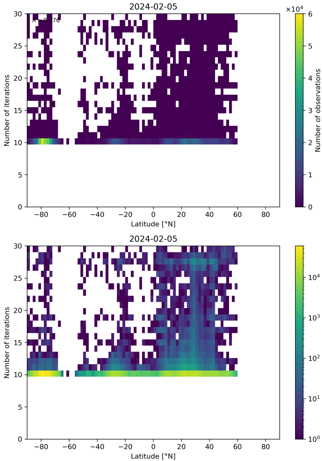
Figure 60: Scatter density plot of “Latitude” against “Number of iterations” for 2024-02-04 to 2024-02-06.
