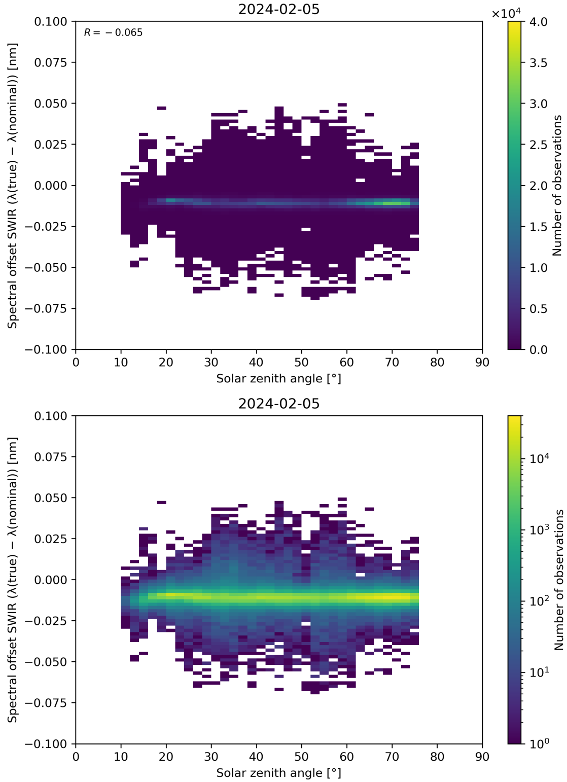
Figure 104: Scatter density plot of “Solar zenith angle” against “Spectral offset SWIR ( \lambda(\text{true}) - \lambda(\text{nominal}) )” for 2024-02-04 to 2024-02-06.
