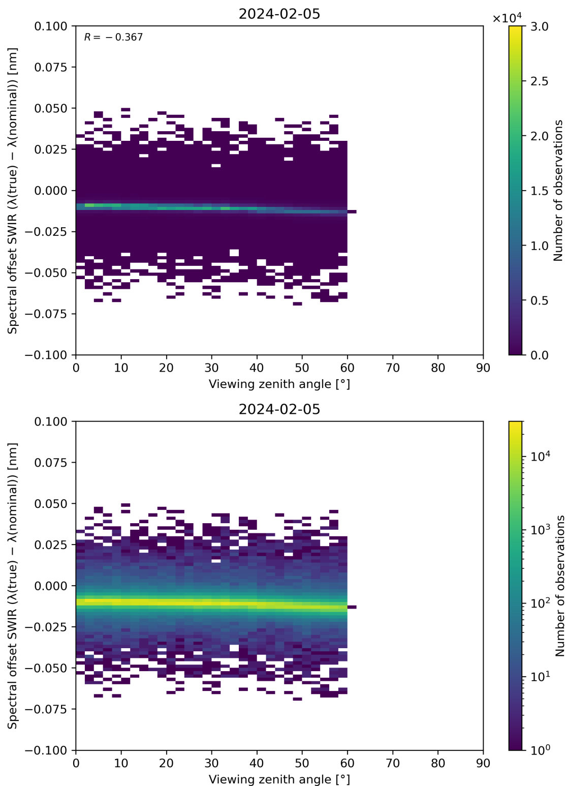
Figure 116: Scatter density plot of “Viewing zenith angle” against “Spectral offset SWIR ( \lambda(\text{true}) - \lambda(\text{nominal}) )” for 2024-02-04 to 2024-02-06.
