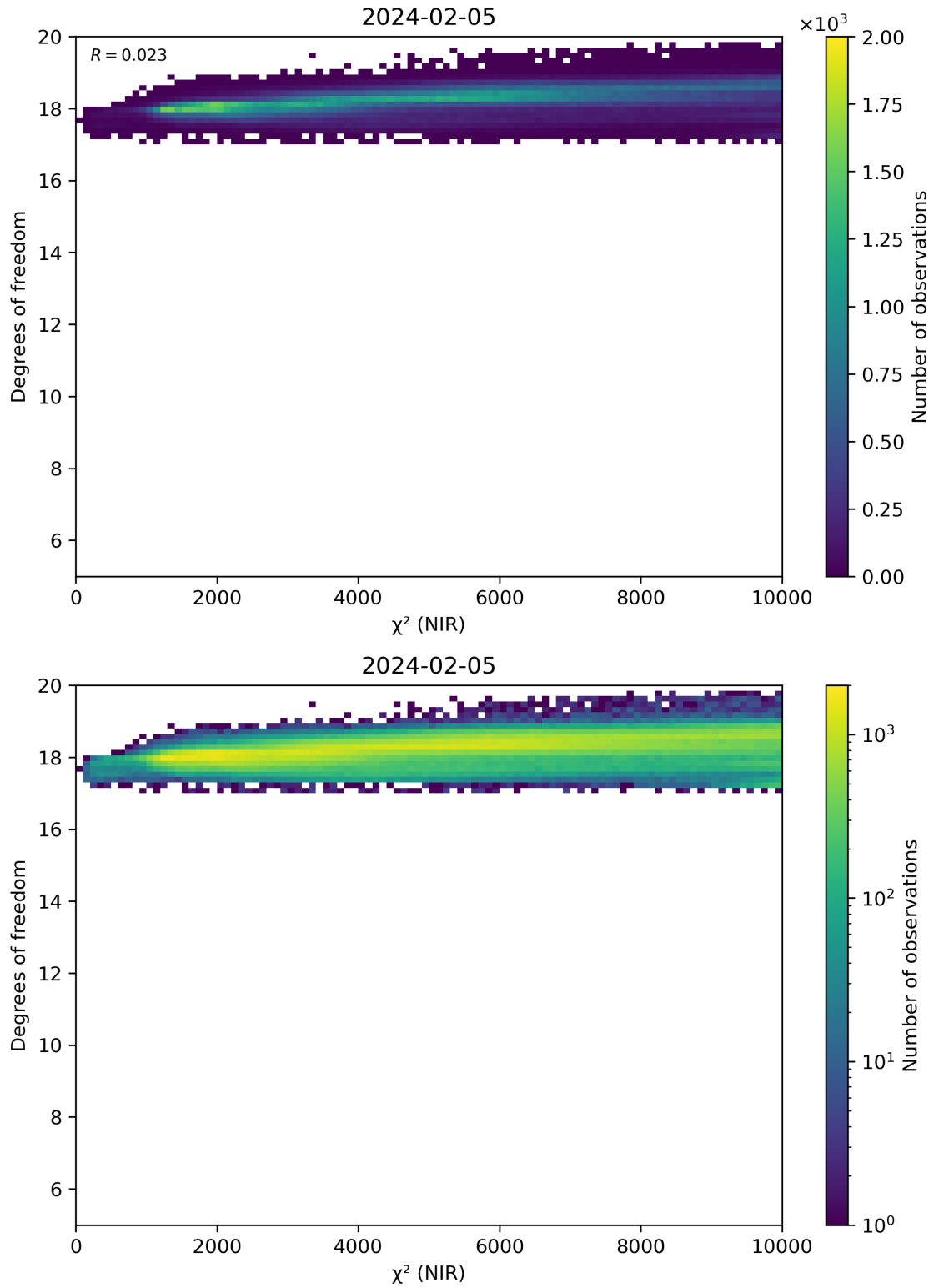
Figure 44: Scatter density plot of “ \chi^2 (NIR)” against “Degrees of freedom” for 2024-02-04 to 2024-02-06.
