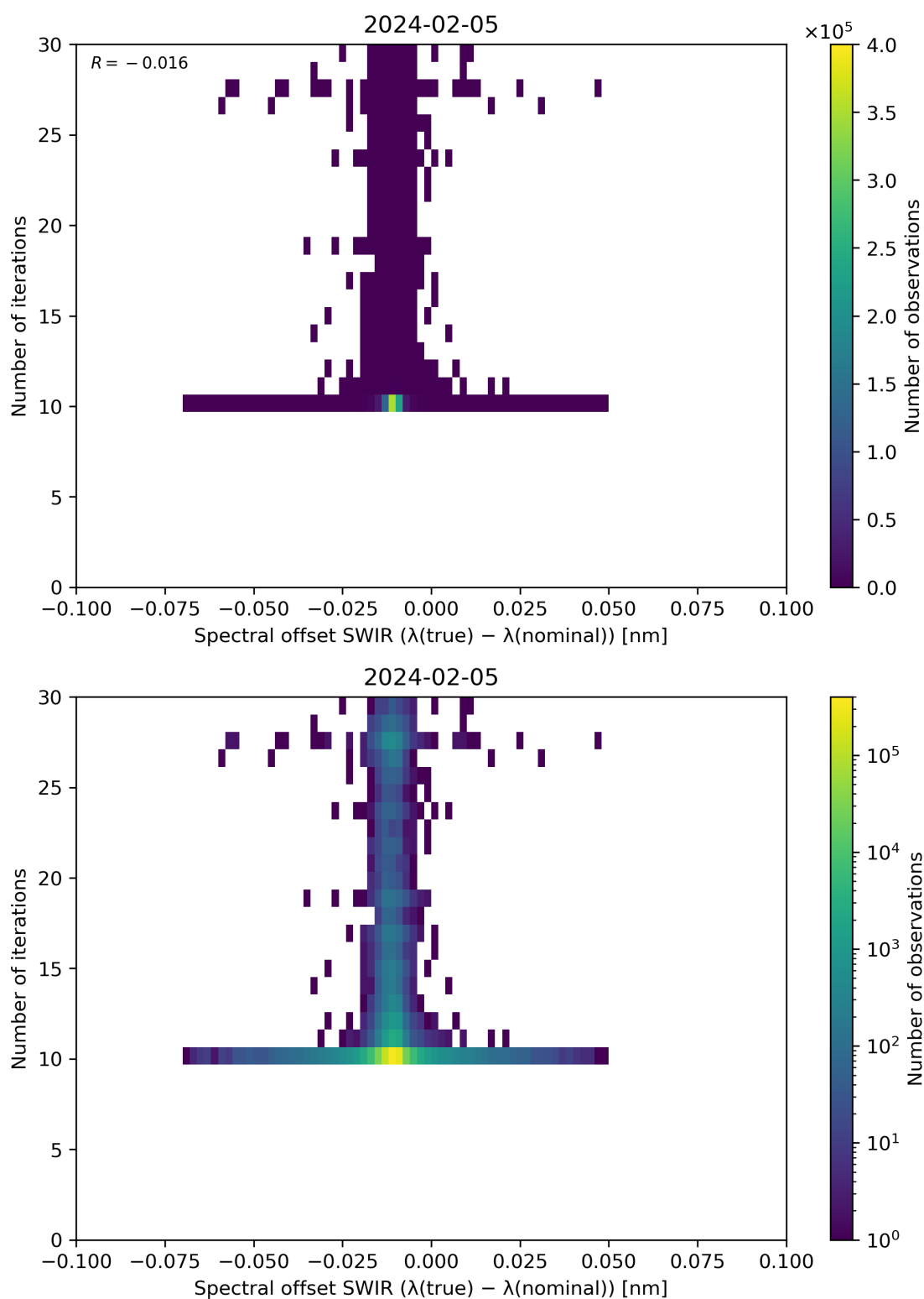
Figure 121: Scatter density plot of “Spectral offset SWIR ( \lambda(\text{true}) - \lambda(\text{nominal}) )” against “Number of iterations” for 2024-02-04 to 2024-02-06.
