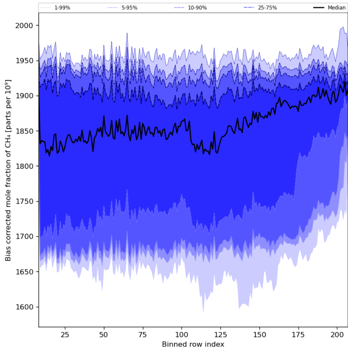
Figure 36: Along track statistics of “Bias corrected mole fraction of CH 4 ” for 2024-02-04 to 2024-02-06
