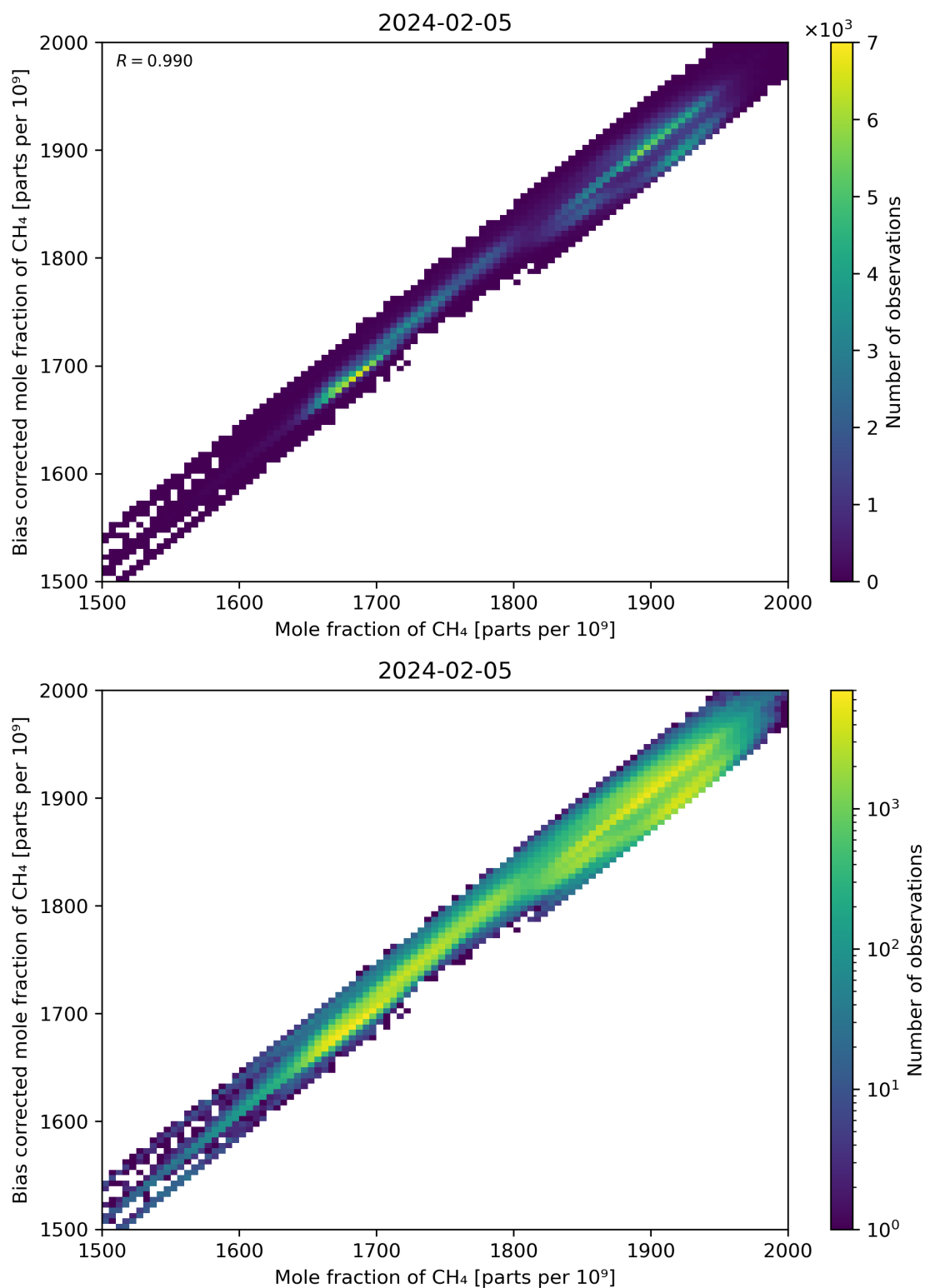
Figure 74: Scatter density plot of “Mole fraction of CH 4 ” against “Bias corrected mole fraction of CH 4 ” for 2024-02-04 to 2024-02-06.
