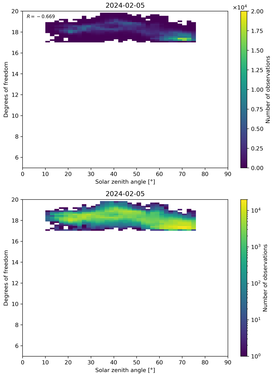
Figure 96: Scatter density plot of “Solar zenith angle” against “Degrees of freedom” for 2024-02-04 to 2024-02-06.
