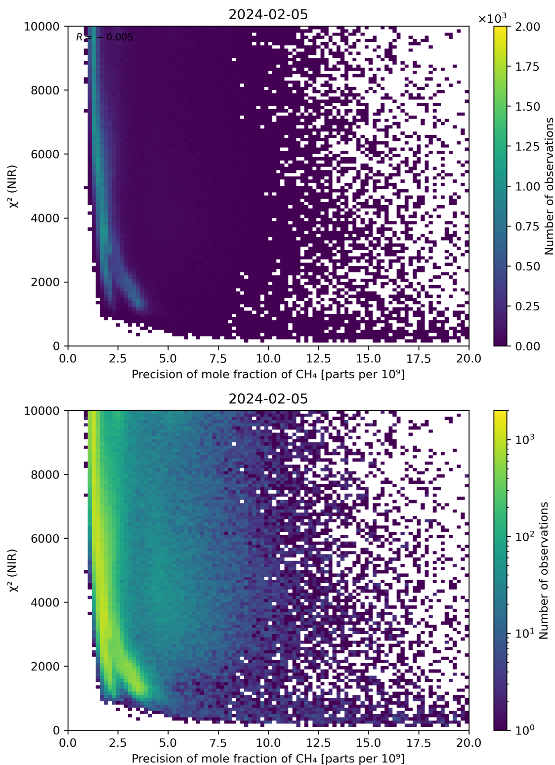
Figure 78: Scatter density plot of “Precision of mole fraction of CH 4 ” against “ \chi^2 (NIR)” for 2024-02-04 to 2024-02-06.
