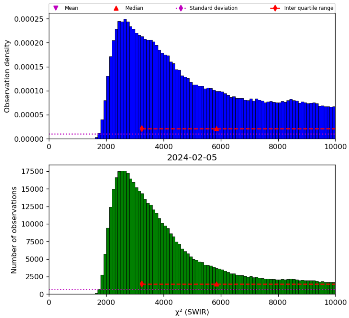
Figure 28: Histogram of “ \chi^2 (SWIR)” for 2024-02-04 to 2024-02-06
