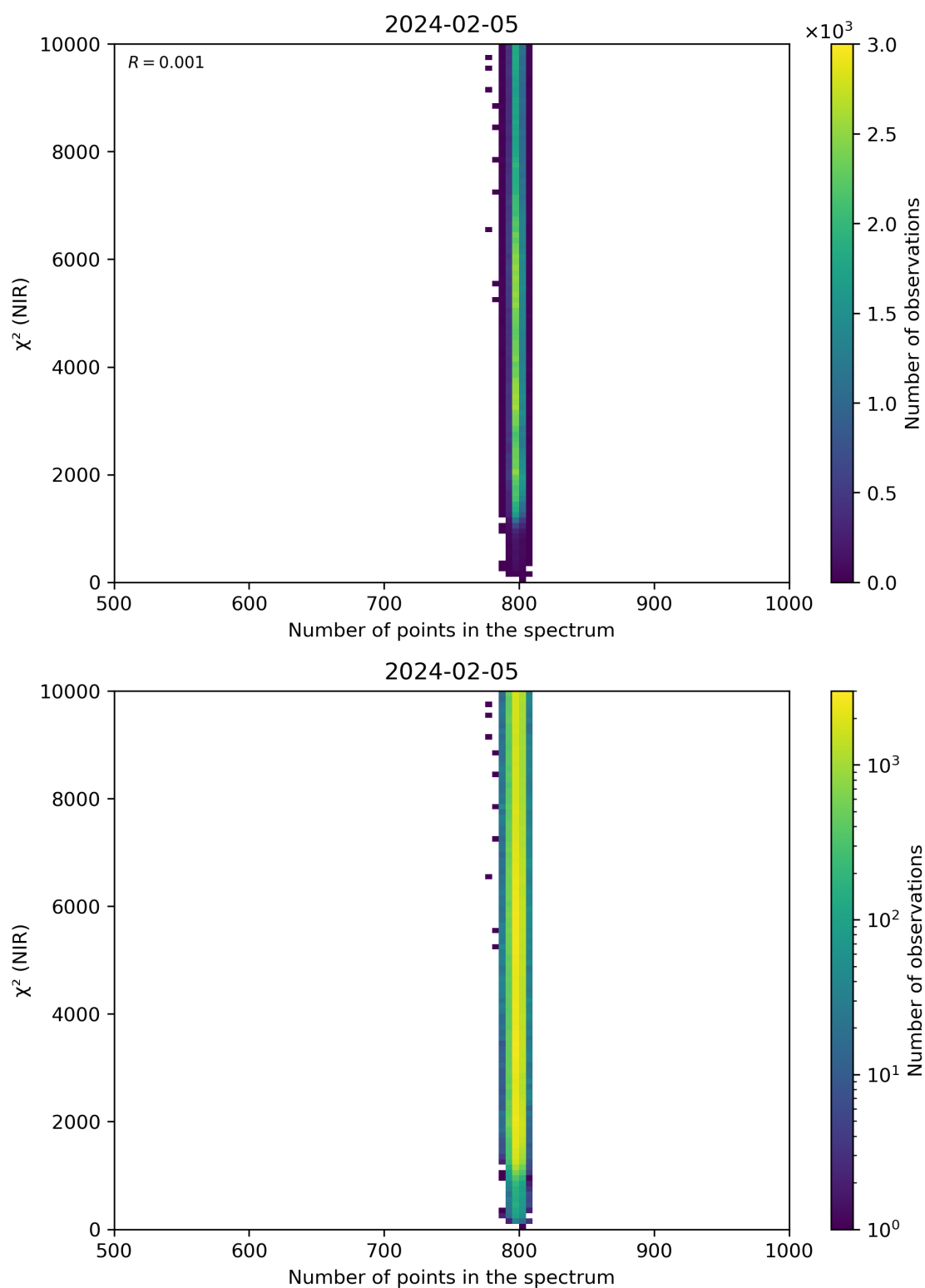
Figure 88: Scatter density plot of “Number of points in the spectrum” against “ \chi^2 (NIR)” for 2024-02-04 to 2024-02-06.
