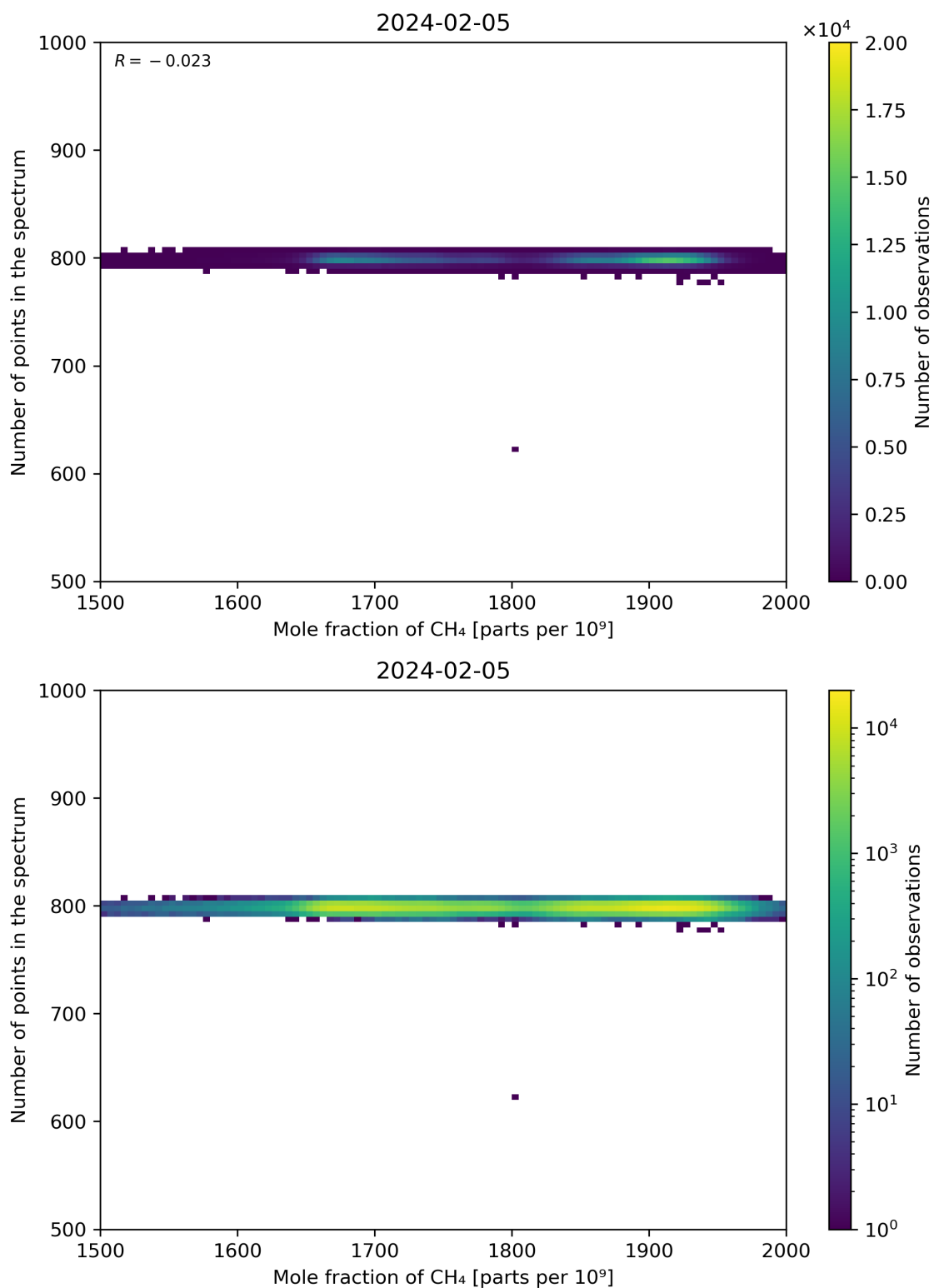
Figure 77: Scatter density plot of “Mole fraction of CH 4 ” against “Number of points in the spectrum” for 2024-02-04 to 2024-02-06.
