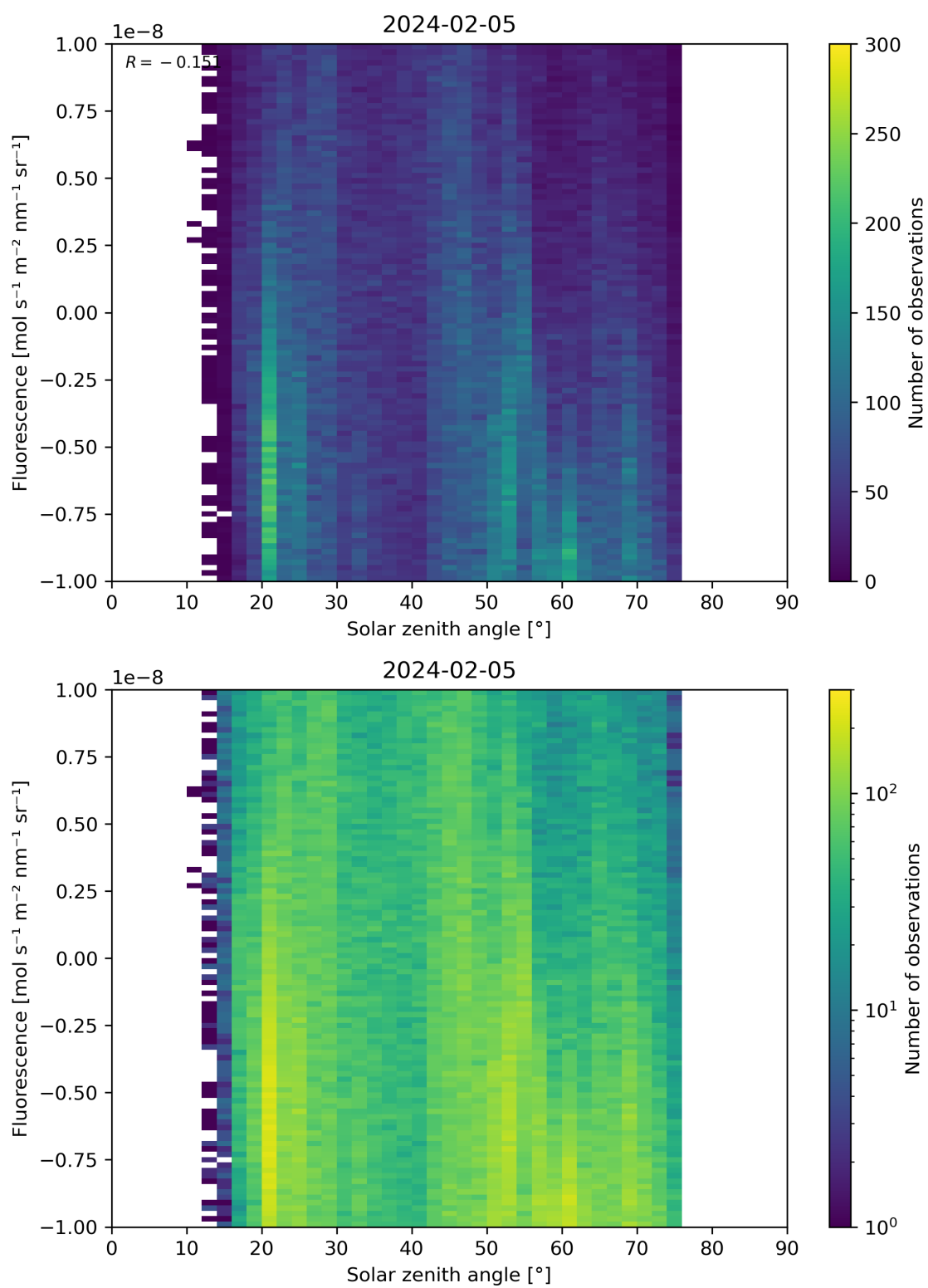
Figure 97: Scatter density plot of “Solar zenith angle” against “Fluorescence” for 2024-02-04 to 2024-02-06.
