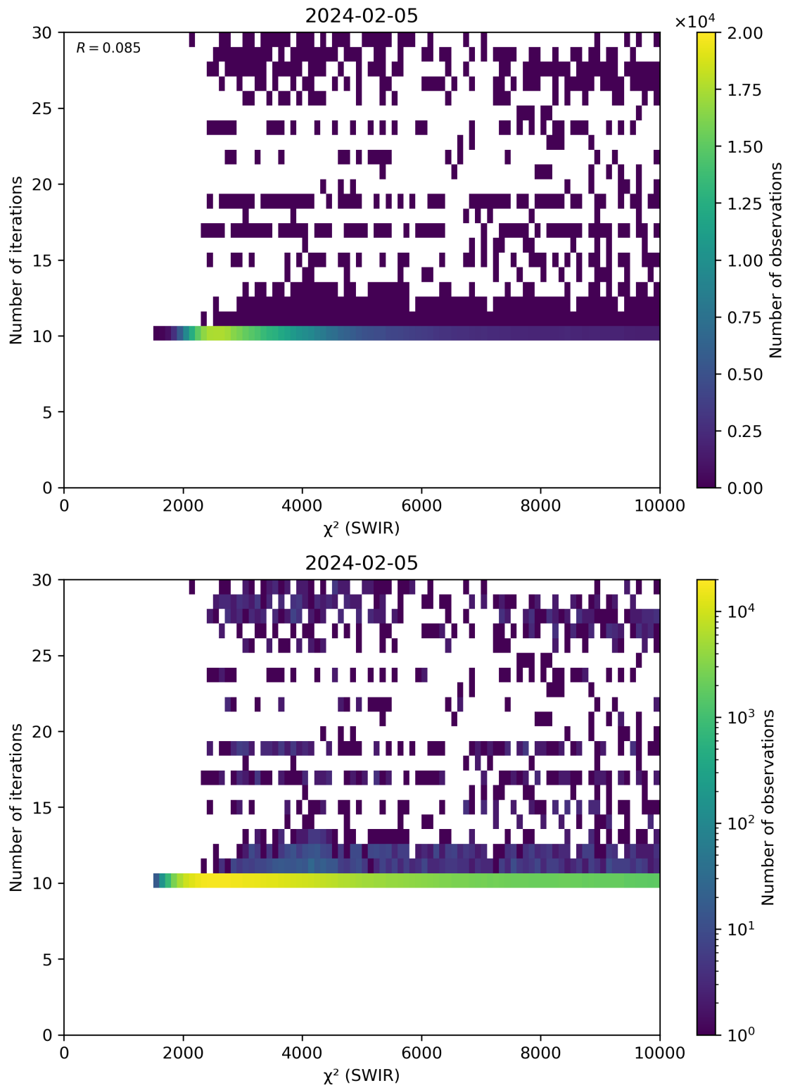
Figure 50: Scatter density plot of “ \chi^2 (SWIR)” against “Number of iterations” for 2024-02-04 to 2024-02-06.
