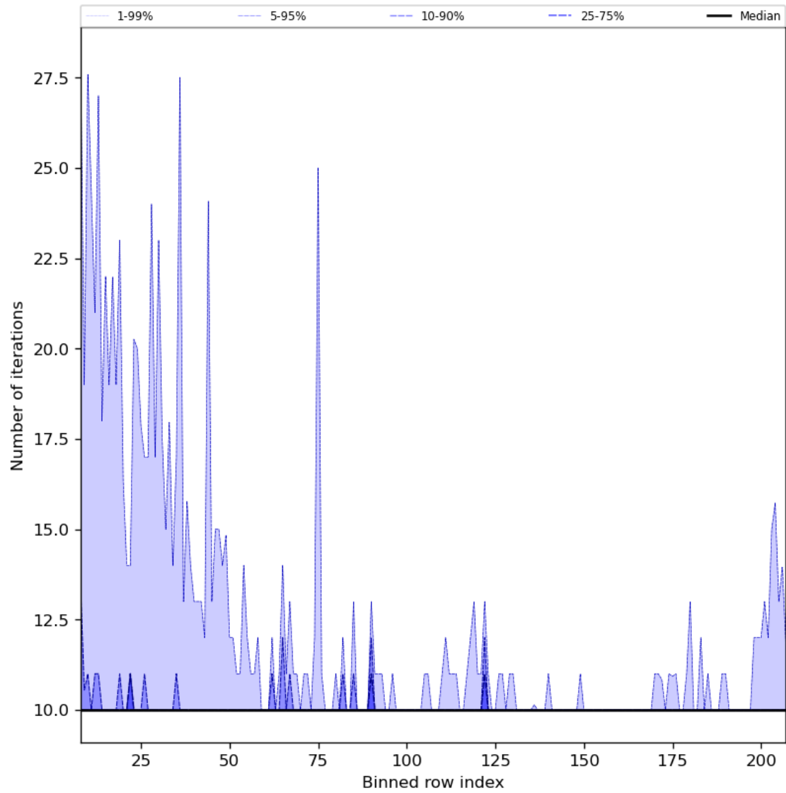
Figure 42: Along track statistics of “Number of iterations” for 2024-02-04 to 2024-02-06
