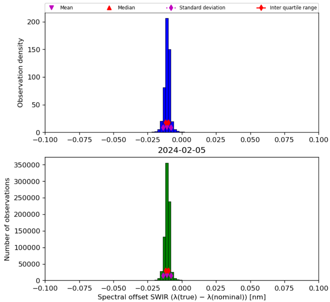
Figure 27: Histogram of “Spectral offset SWIR ( \lambda(\text{true}) - \lambda(\text{nominal}) )” for 2024-02-04 to 2024-02-06
