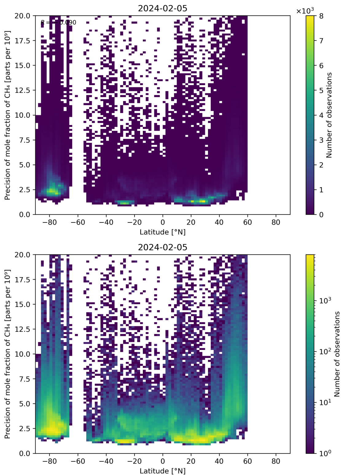
Figure 59: Scatter density plot of “Latitude” against “Precision of mole fraction of CH 4 ” for 2024-02-04 to 2024-02-06.
