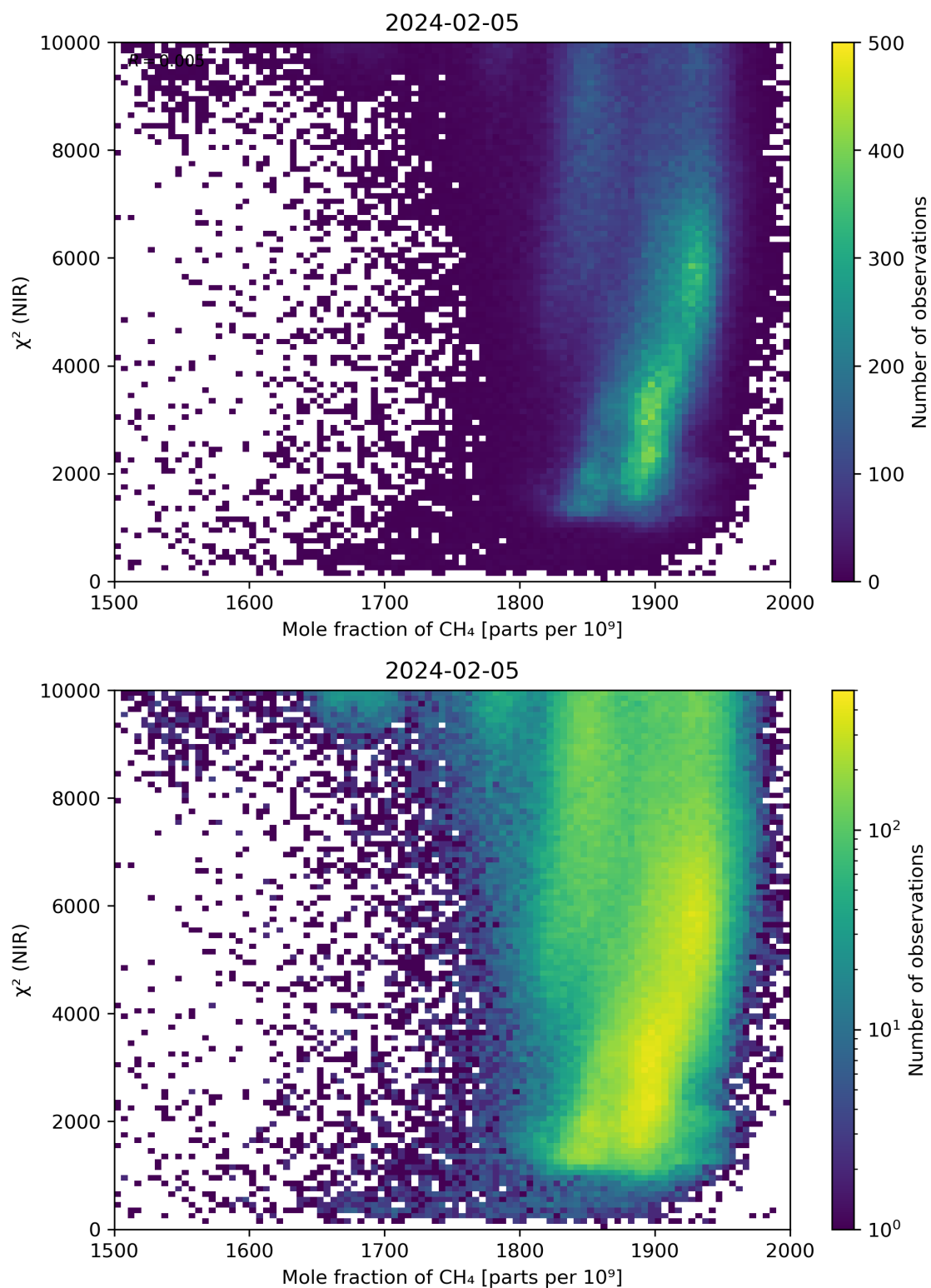
Figure 70: Scatter density plot of “Mole fraction of \text{CH}_4 ” against “ \chi^2 (NIR)” for 2024-02-04 to 2024-02-06.
