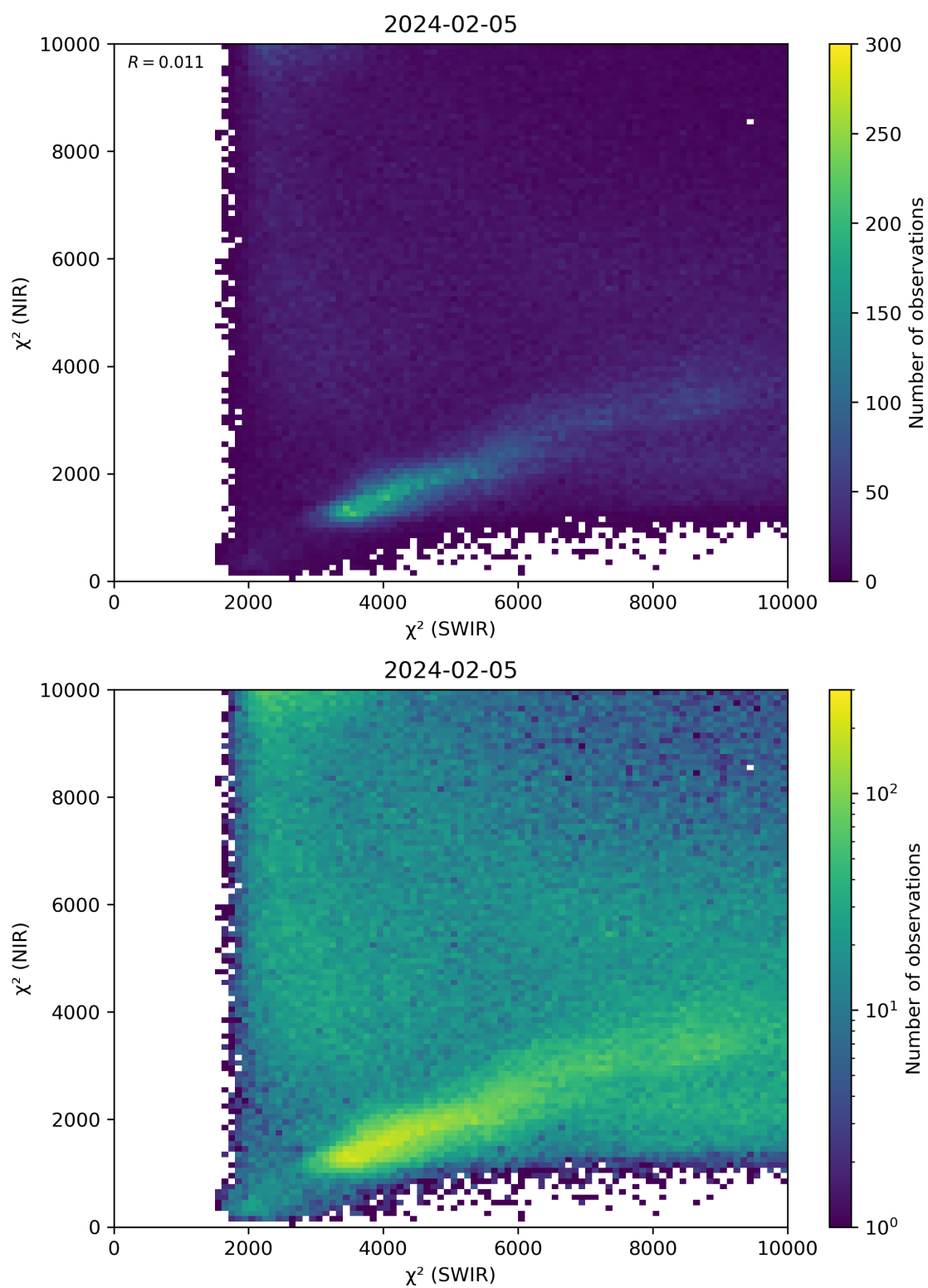
Figure 47: Scatter density plot of “ \chi^2 (SWIR)” against “ \chi^2 (NIR)” for 2024-02-04 to 2024-02-06.
