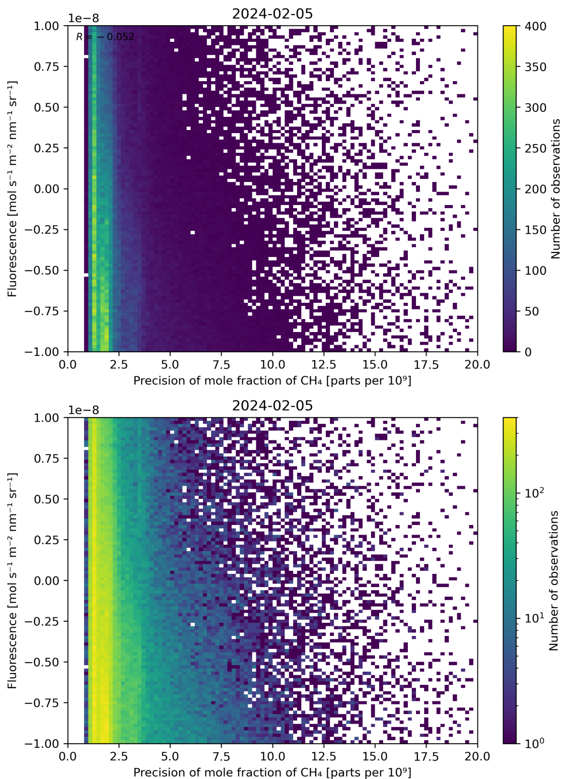
Figure 81: Scatter density plot of “Precision of mole fraction of \text{CH}_4 ” against “Fluorescence” for 2024-02-04 to 2024-02-06.
