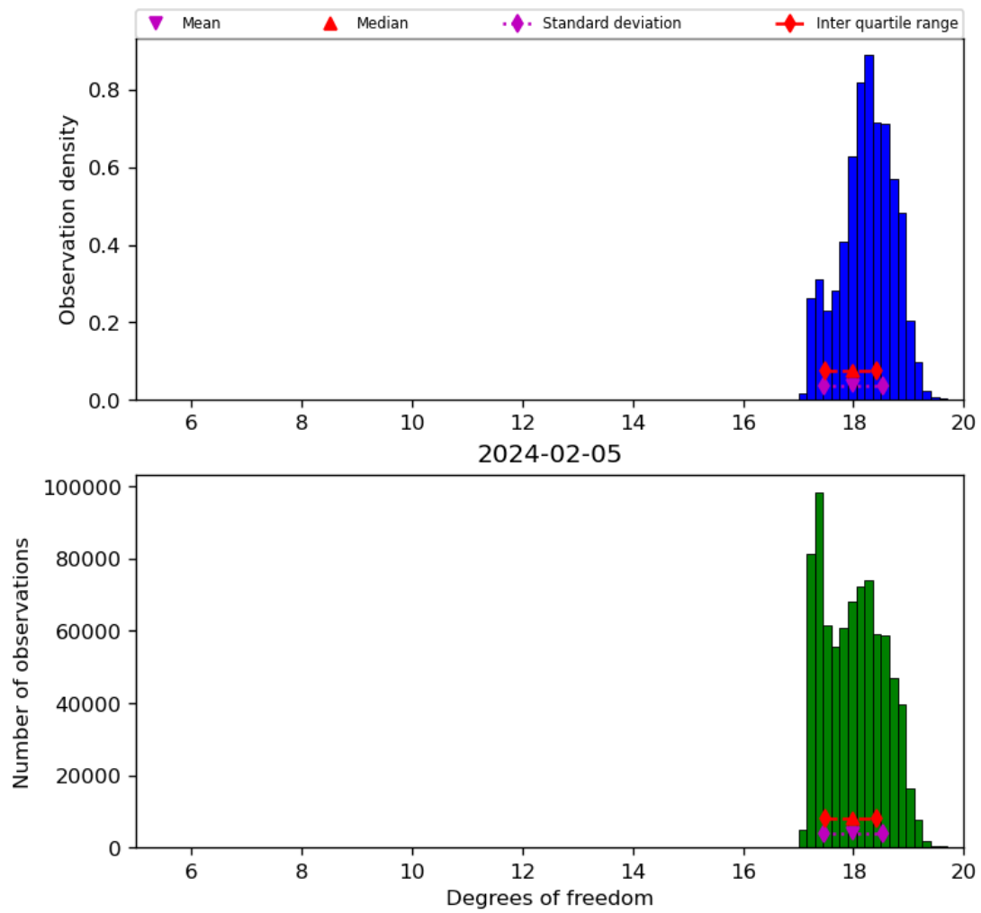
Figure 30: Histogram of “Degrees of freedom” for 2024-02-04 to 2024-02-06
