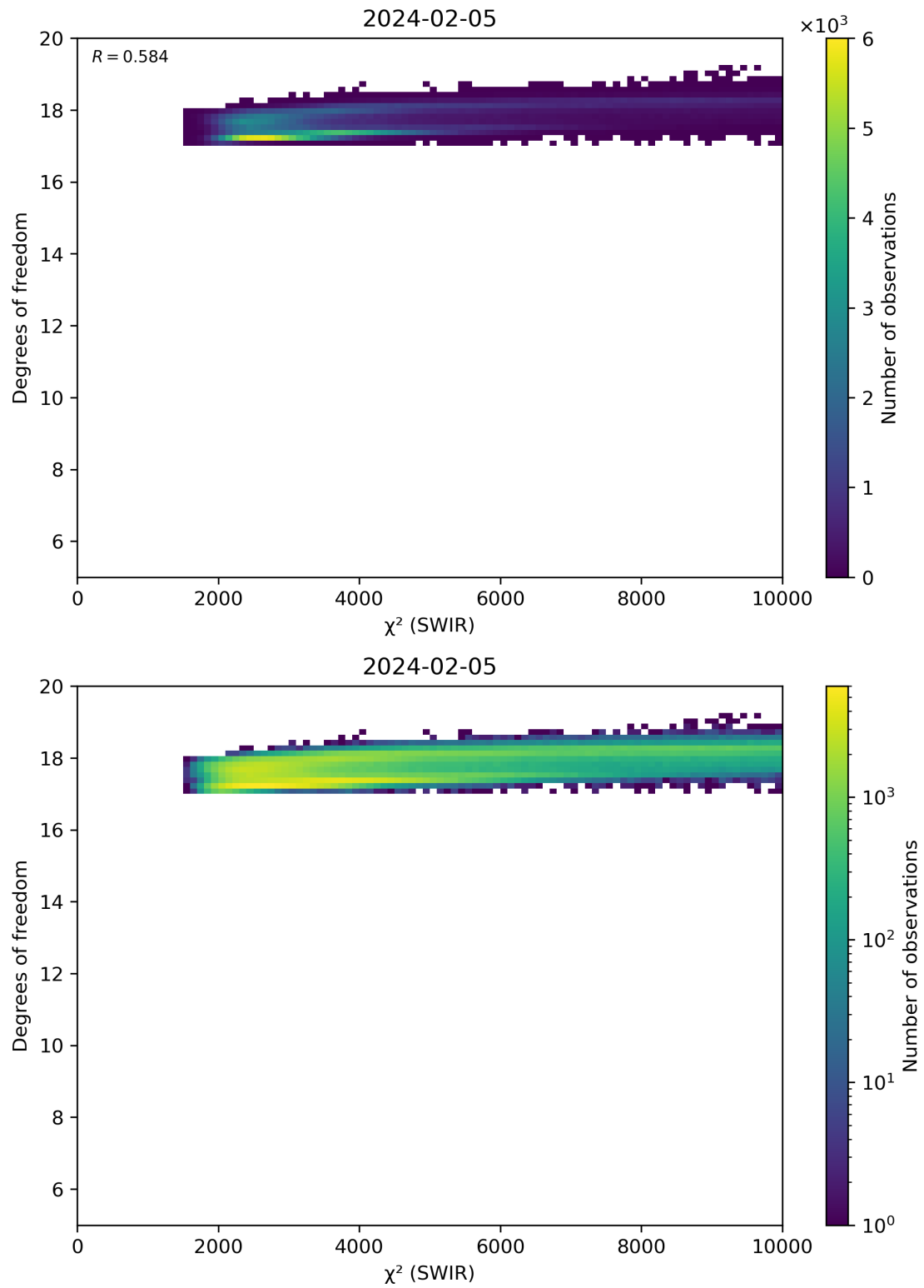
Figure 48: Scatter density plot of “ \chi^2 (SWIR)” against “Degrees of freedom” for 2024-02-04 to 2024-02-06.
