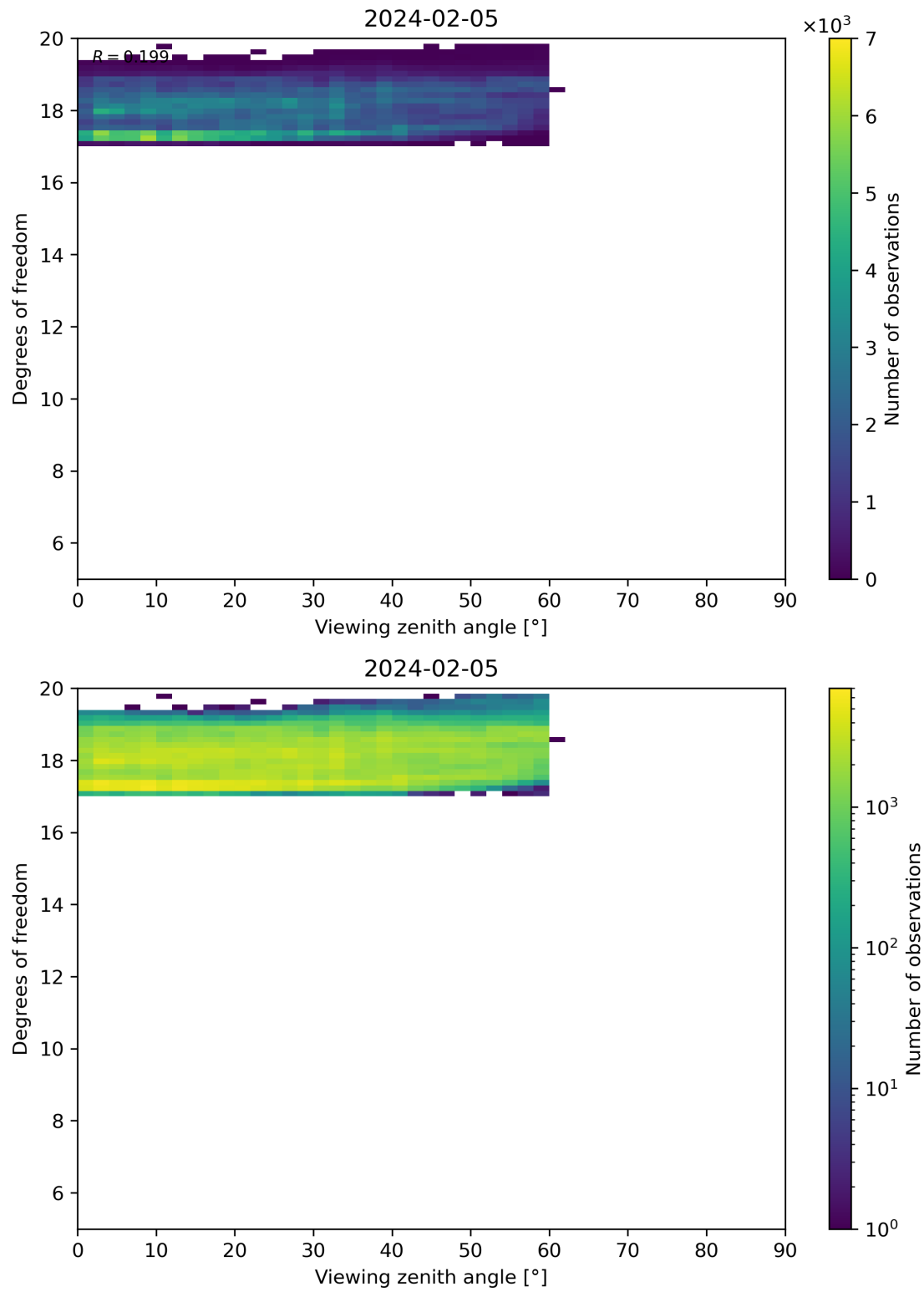
Figure 107: Scatter density plot of “Viewing zenith angle” against “Degrees of freedom” for 2024-02-04 to 2024-02-06.
