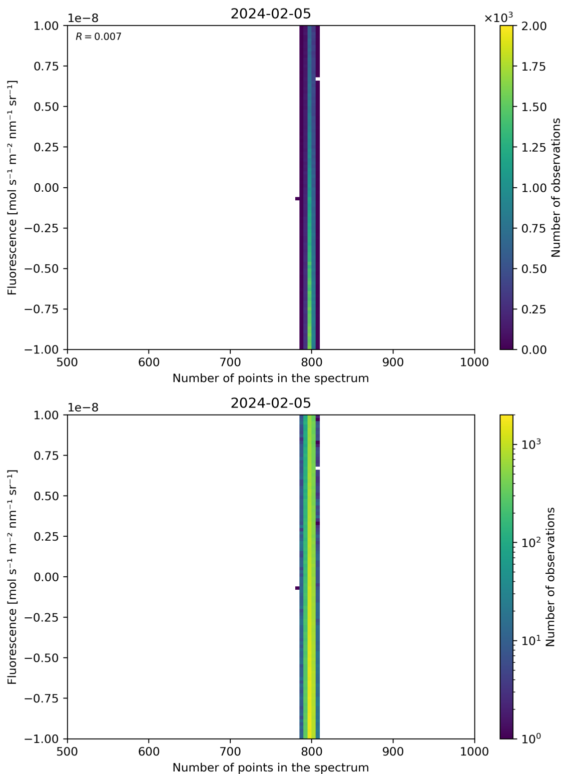
Figure 91: Scatter density plot of “Number of points in the spectrum” against “Fluorescence” for 2024-02-04 to 2024-02-06.
