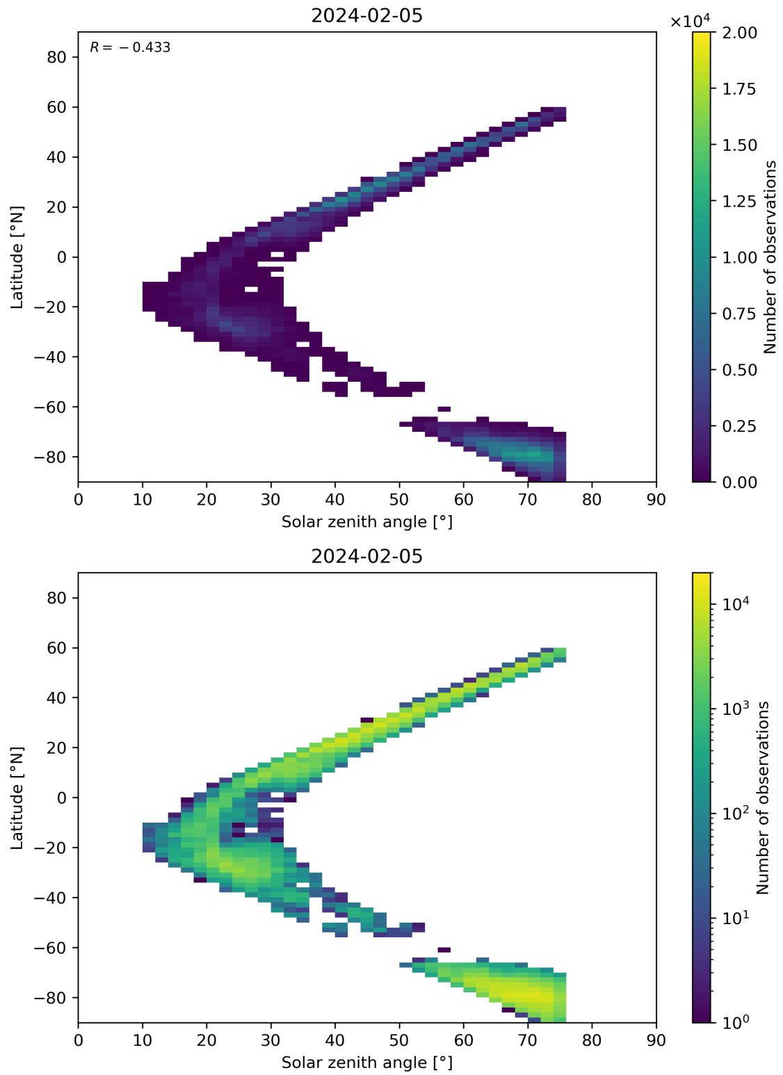
Figure 98: Scatter density plot of “Solar zenith angle” against “Latitude” for 2024-02-04 to 2024-02-06.
