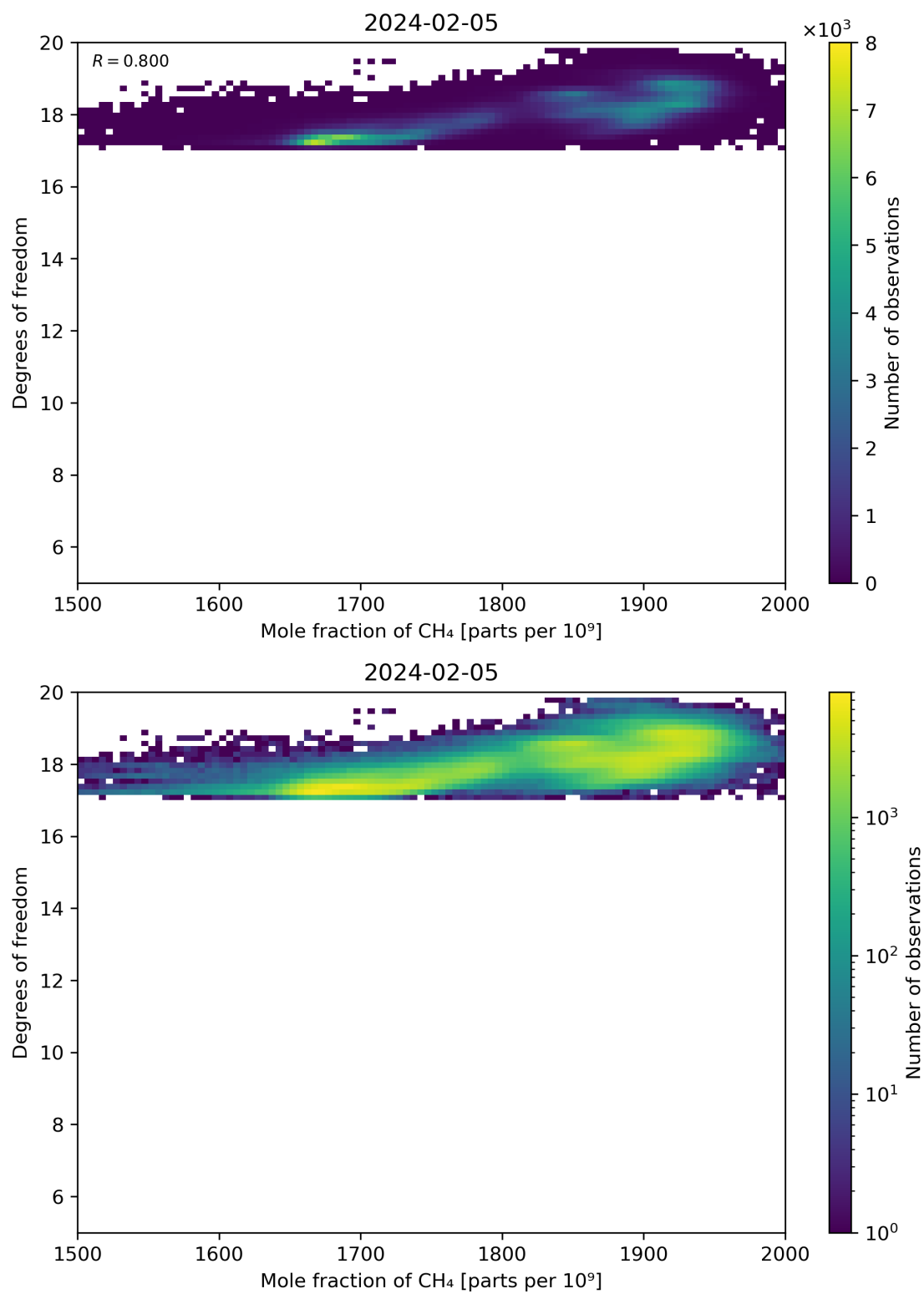
Figure 72: Scatter density plot of “Mole fraction of CH 4 ” against “Degrees of freedom” for 2024-02-04 to 2024-02-06.
