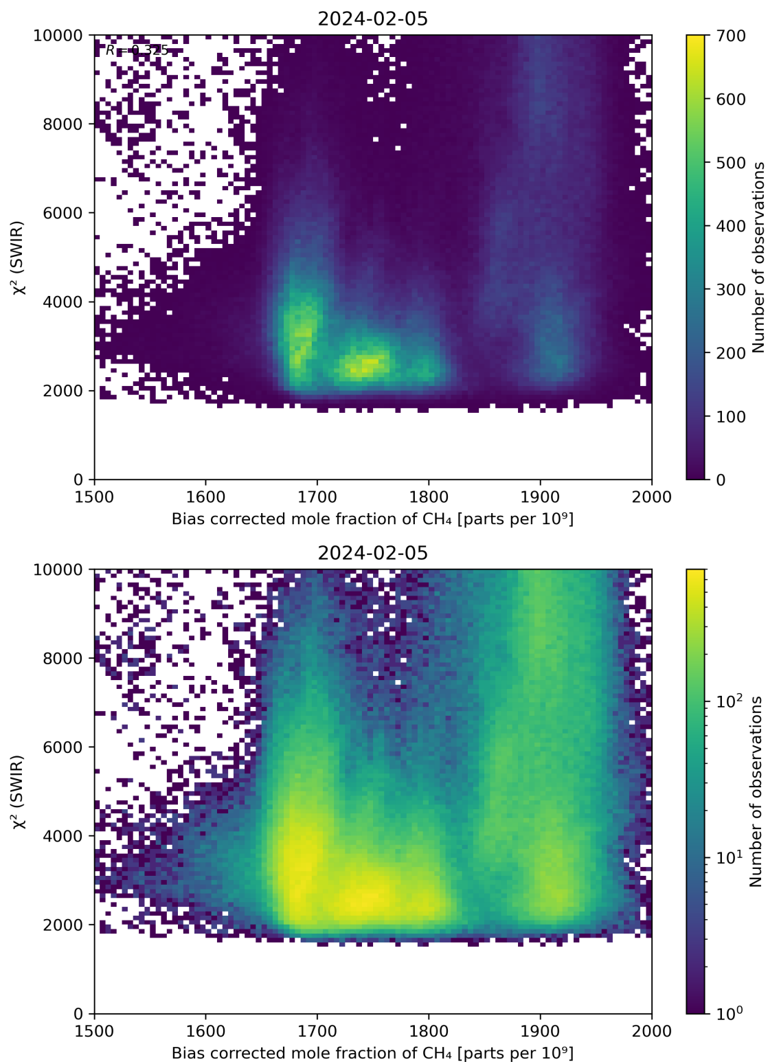
Figure 64: Scatter density plot of “Bias corrected mole fraction of \text{CH}_4 ” against “ \chi^2 (SWIR)” for 2024-02-04 to 2024-02-06.
