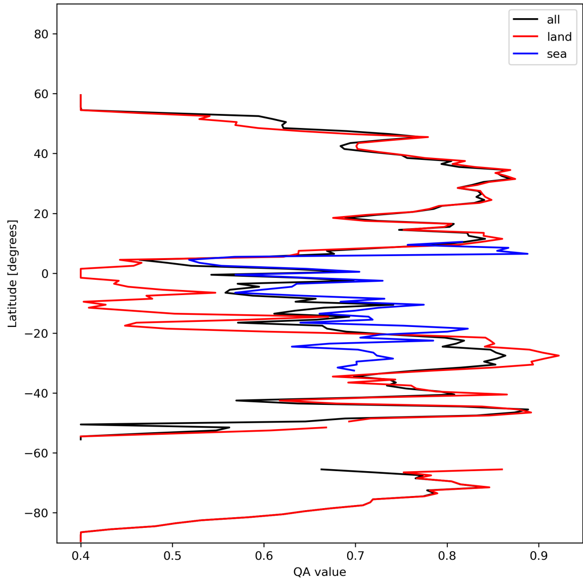
Figure 11: Zonal average of “QA value” for 2024-02-04 to 2024-02-06.
