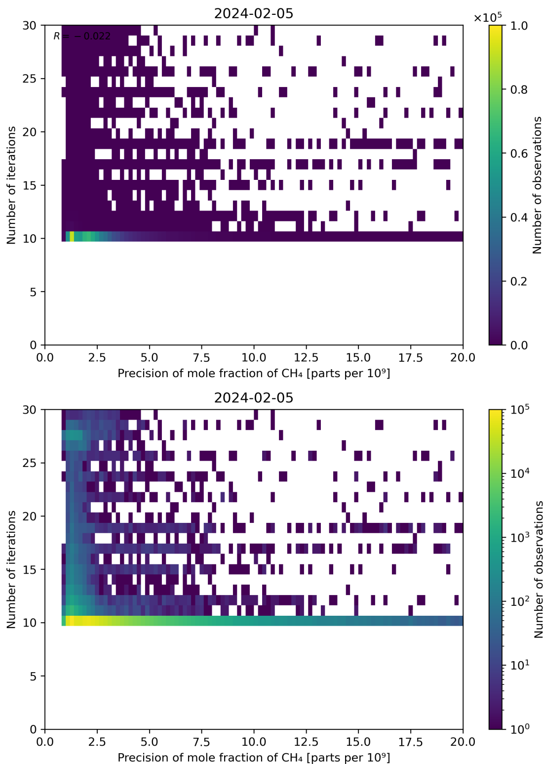
Figure 83: Scatter density plot of “Precision of mole fraction of CH 4 ” against “Number of iterations” for 2024-02-04 to 2024-02-06.
