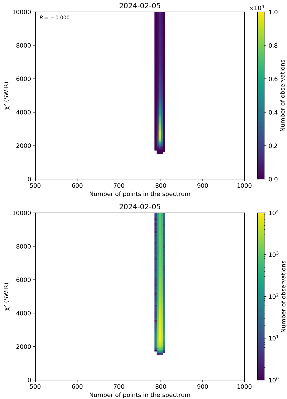
Figure 89: Scatter density plot of “Number of points in the spectrum” against “ \chi^2 (SWIR)” for 2024-02-04 to 2024-02-06.
