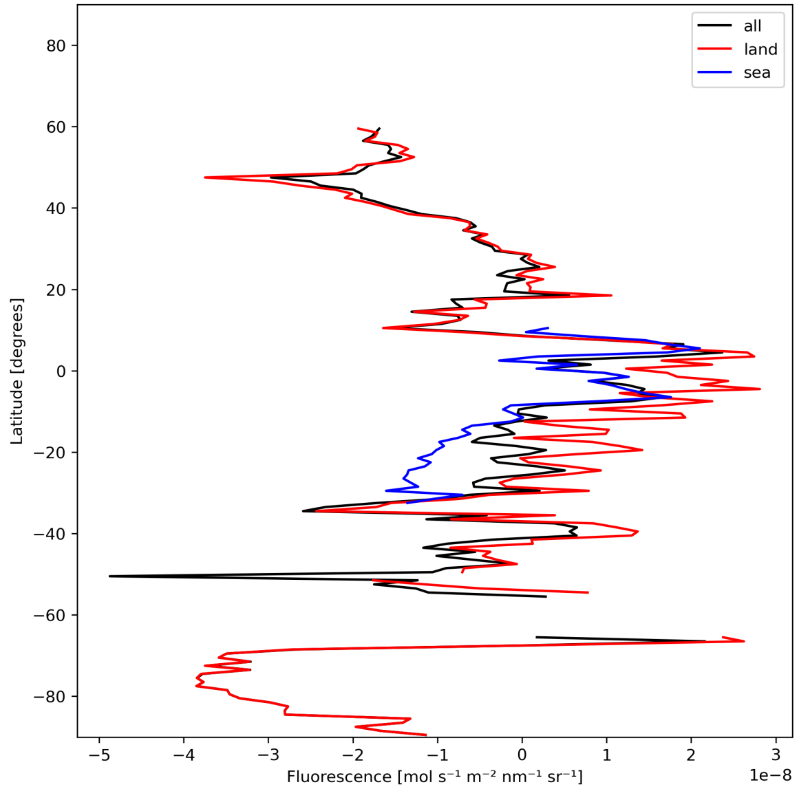
Figure 21: Zonal average of “Fluorescence” for 2024-02-04 to 2024-02-06.
