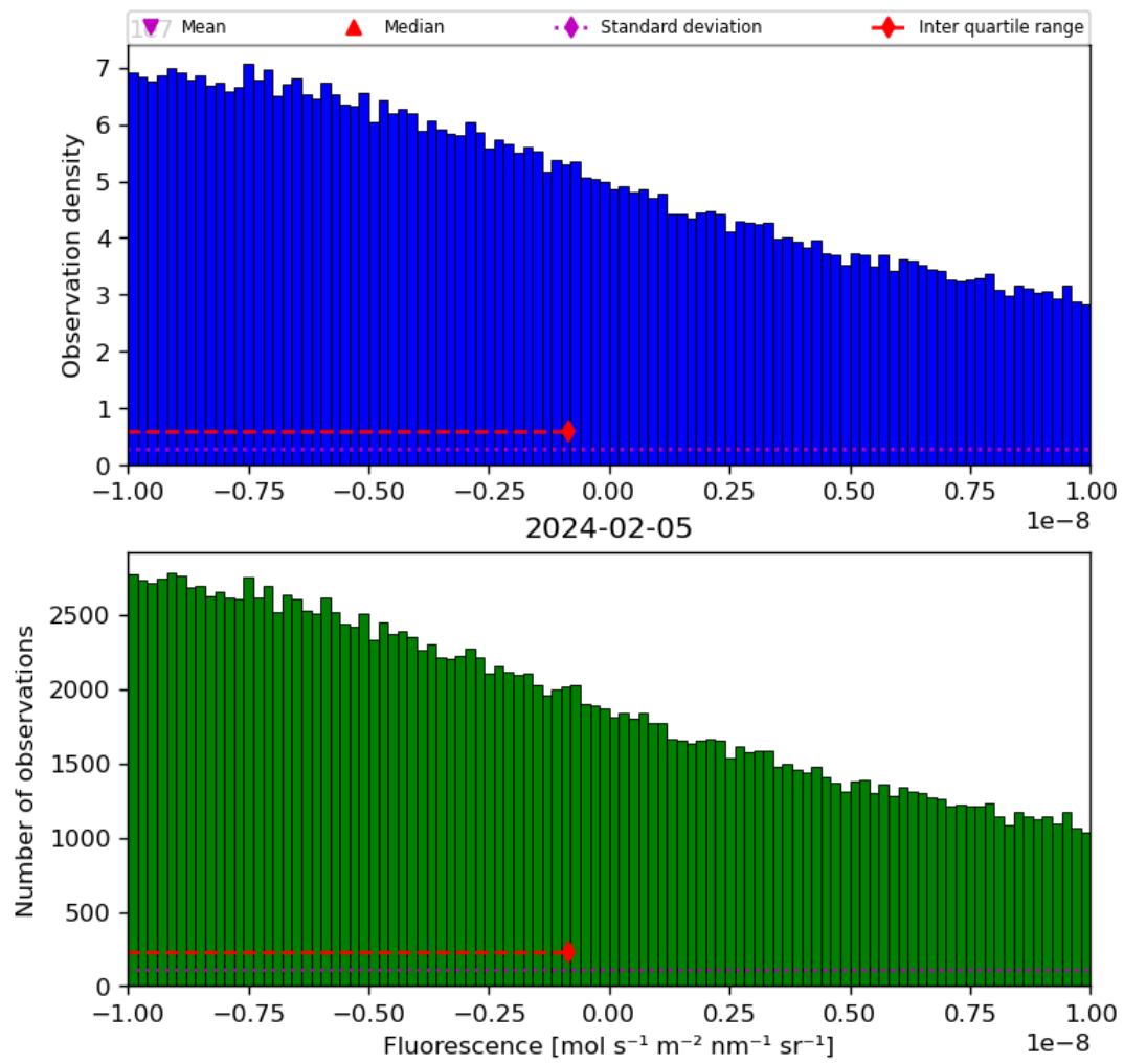
Figure 32: Histogram of “Fluorescence” for 2024-02-04 to 2024-02-06
