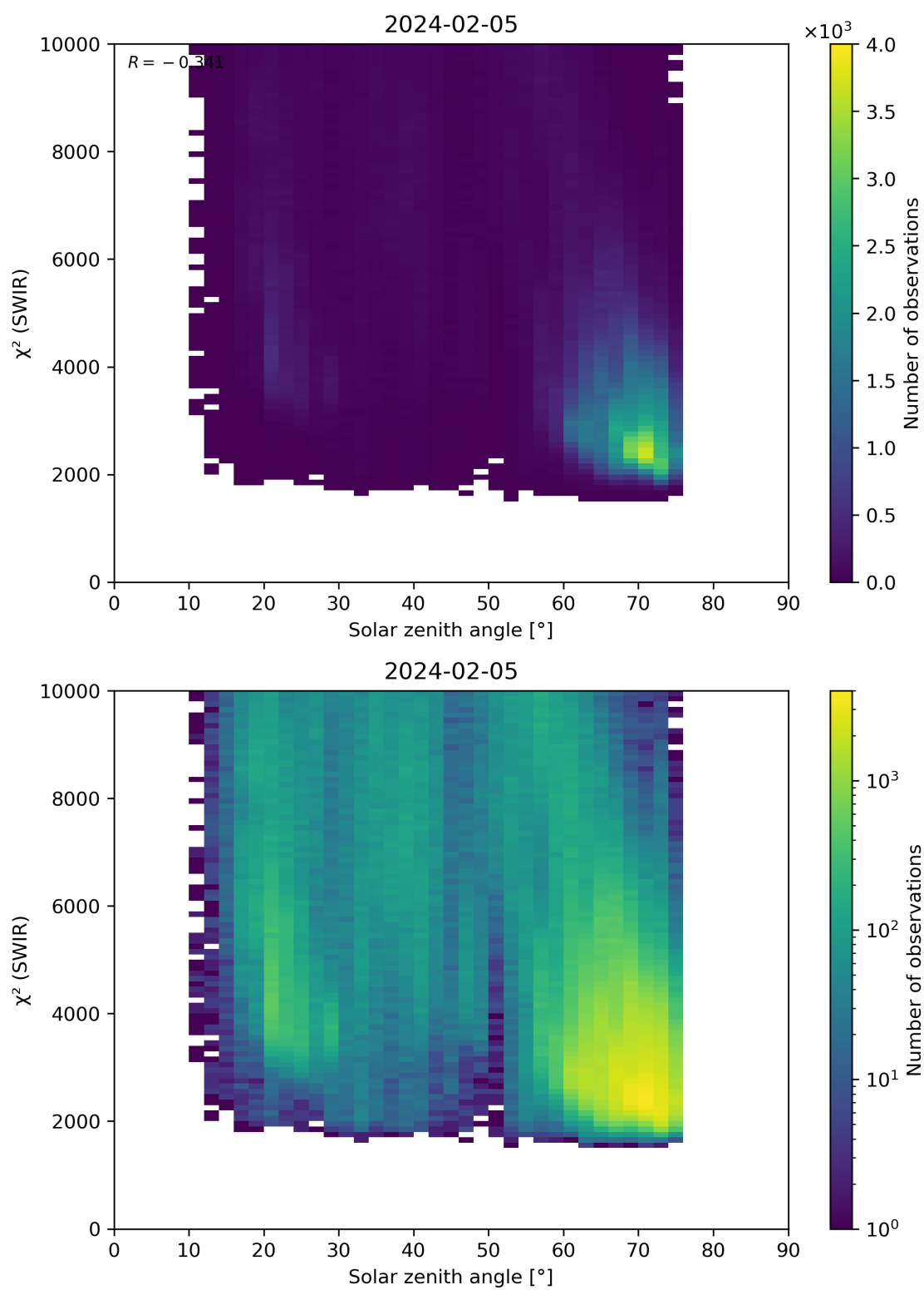
Figure 95: Scatter density plot of “Solar zenith angle” against “ \chi^2 (SWIR)” for 2024-02-04 to 2024-02-06.
