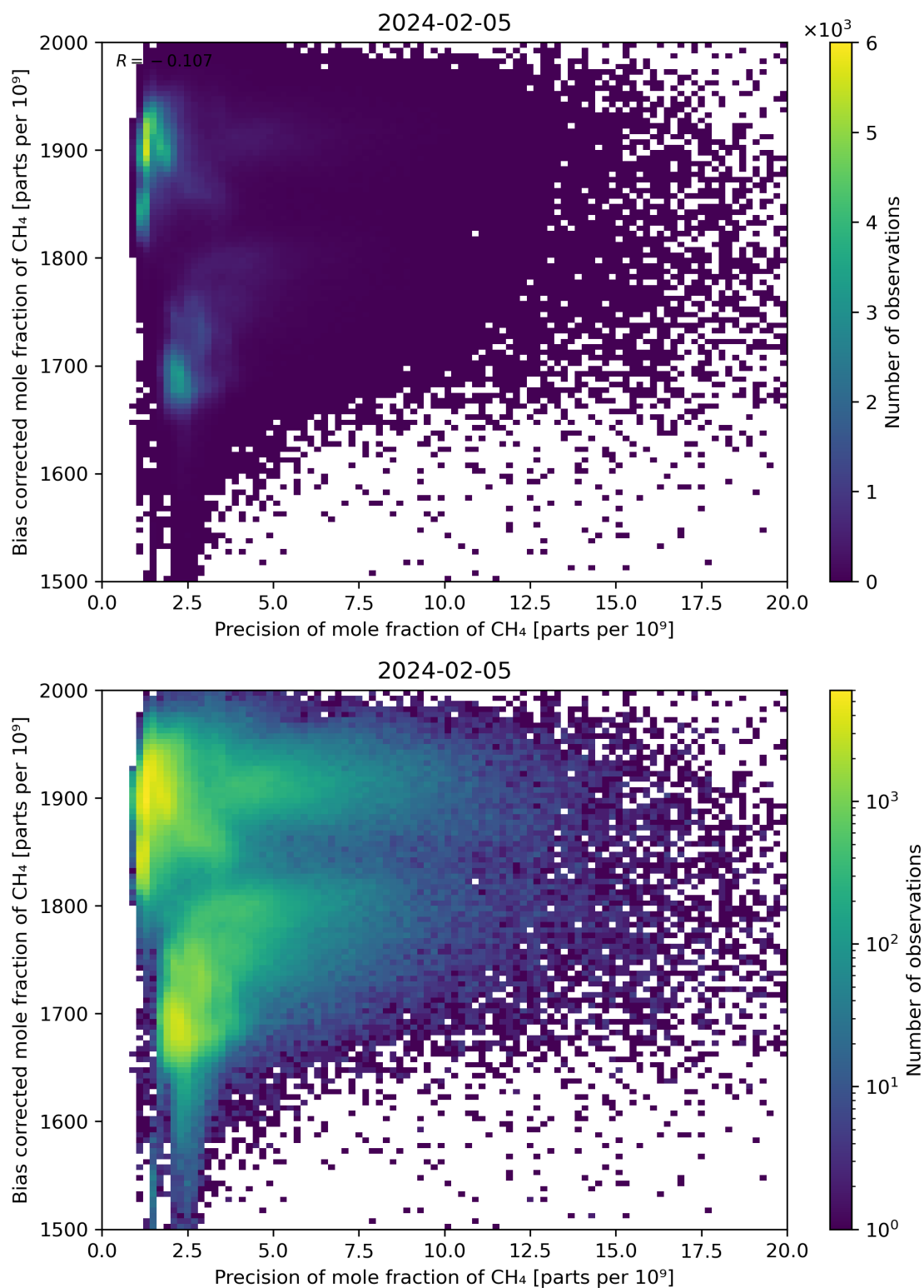
Figure 82: Scatter density plot of “Precision of mole fraction of \text{CH}_4 ” against “Bias corrected mole fraction of \text{CH}_4 ” for 2024-02-04 to 2024-02-06.
