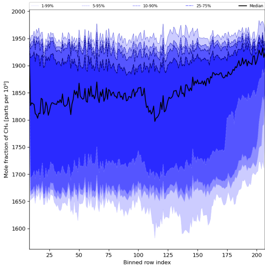
Figure 34: Along track statistics of “Mole fraction of CH 4 ” for 2024-02-04 to 2024-02-06
