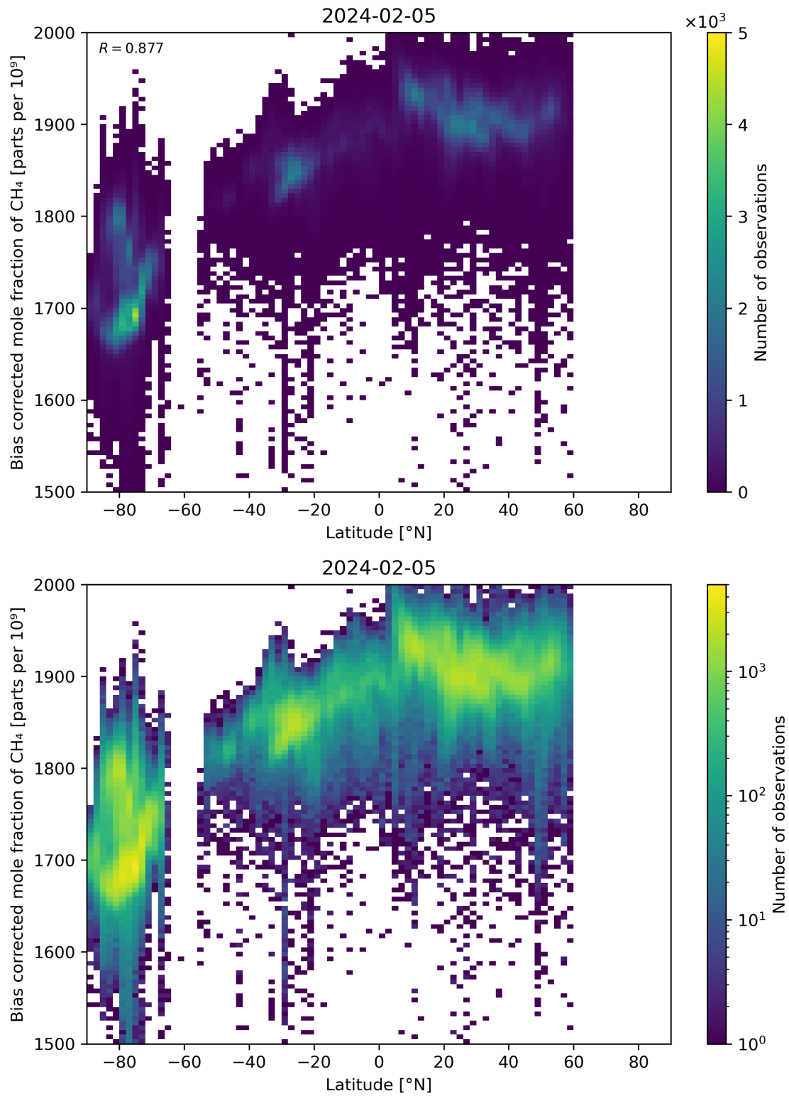
Figure 58: Scatter density plot of “Latitude” against “Bias corrected mole fraction of CH 4 ” for 2024-02-04 to 2024-02-06.
