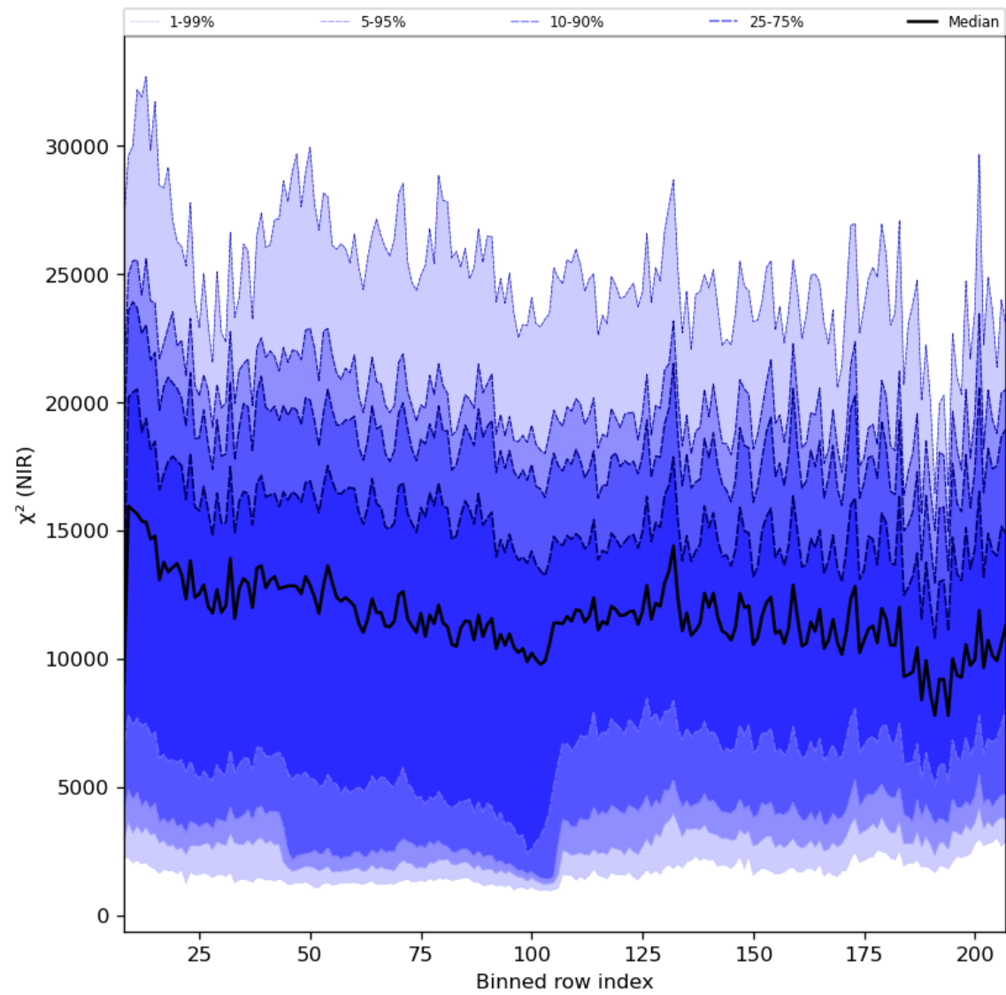
Figure 40: Along track statistics of “ \chi^2 (NIR)” for 2024-02-04 to 2024-02-06
