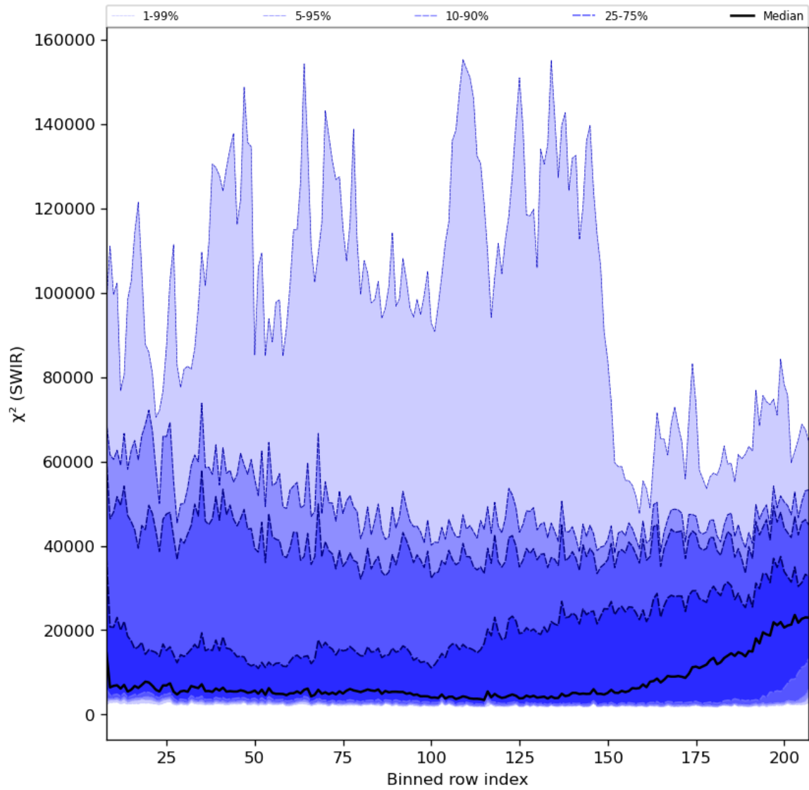
Figure 39: Along track statistics of “ \chi^2 (SWIR)” for 2024-02-04 to 2024-02-06
