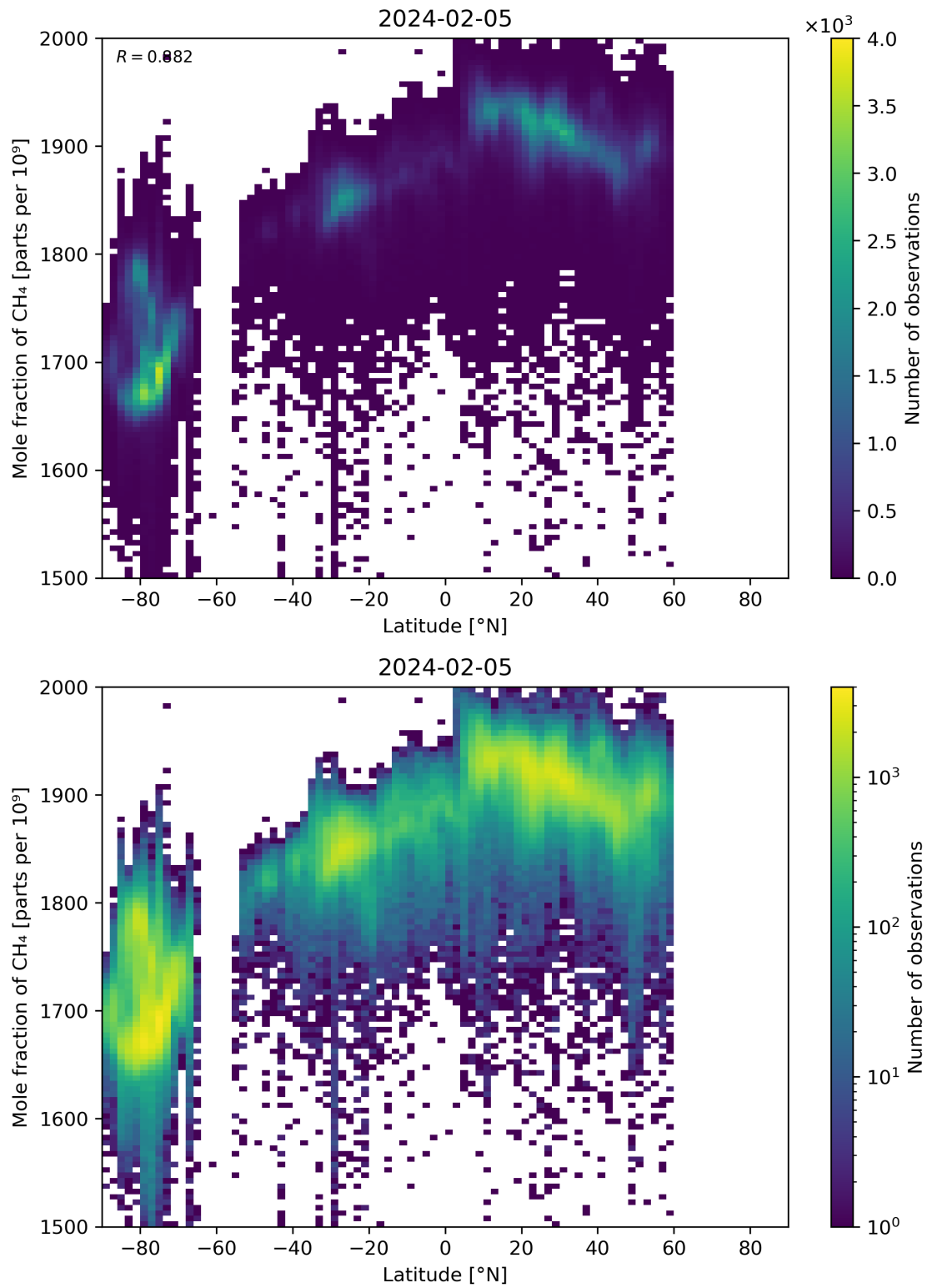
Figure 57: Scatter density plot of “Latitude” against “Mole fraction of CH 4 ” for 2024-02-04 to 2024-02-06.
