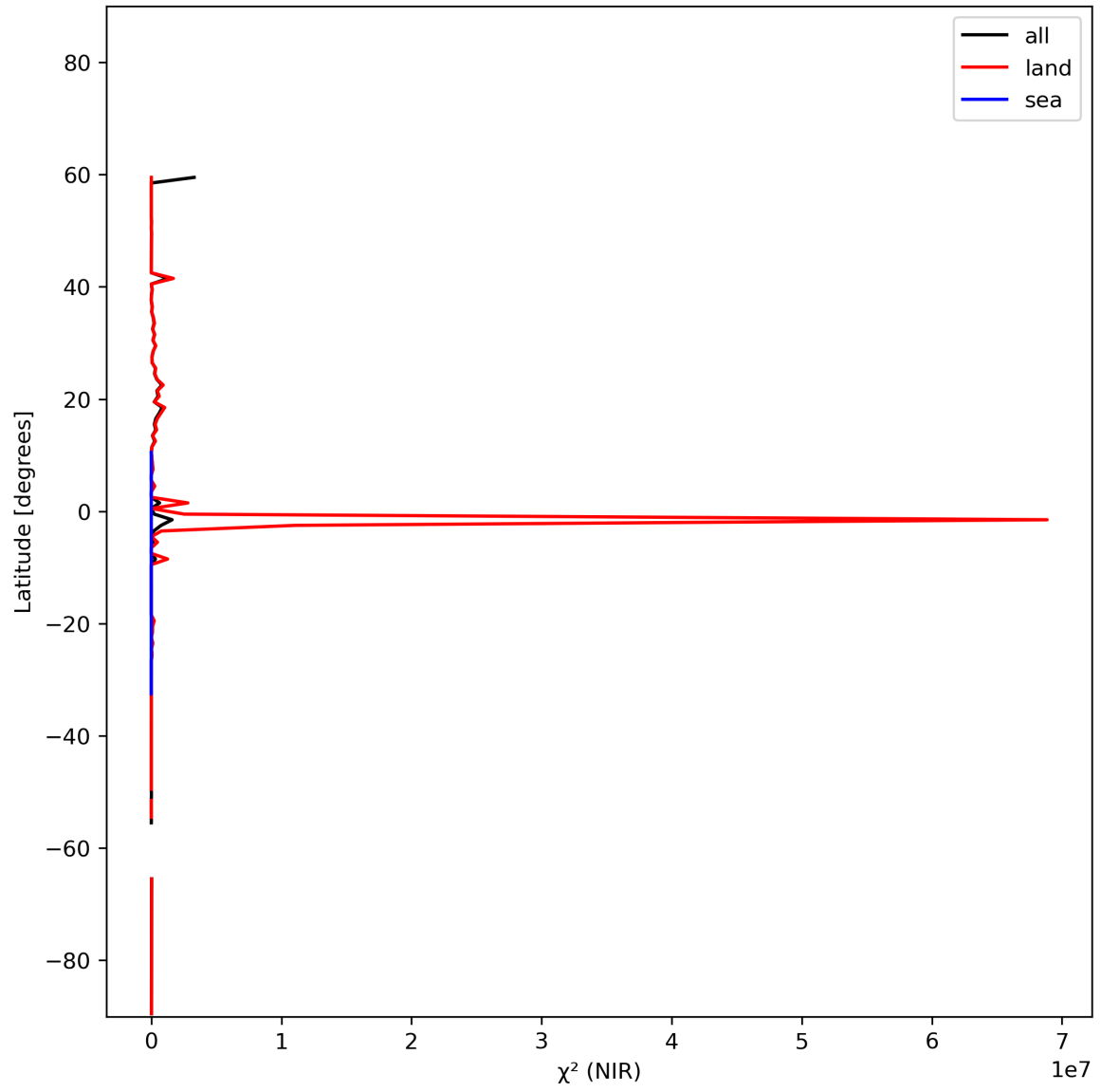
Figure 18: Zonal average of “ \chi^2 (NIR)” for 2024-02-04 to 2024-02-06.
