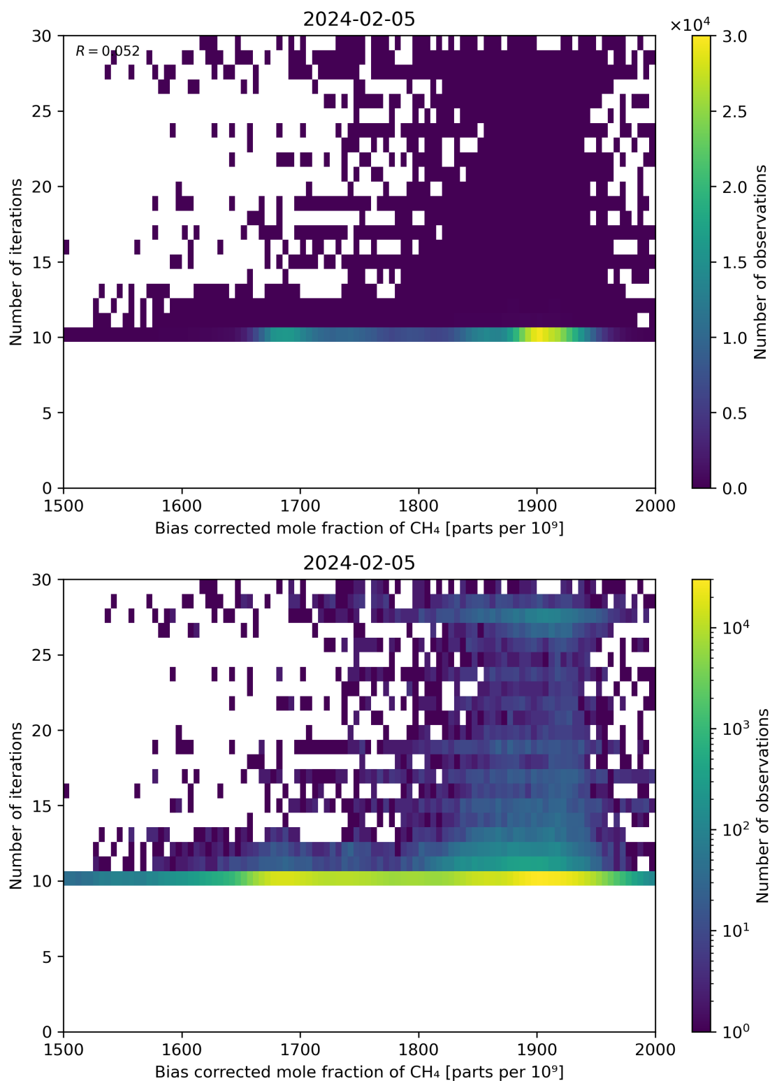
Figure 67: Scatter density plot of “Bias corrected mole fraction of \text{CH}_4 ” against “Number of iterations” for 2024-02-04 to 2024-02-06.
