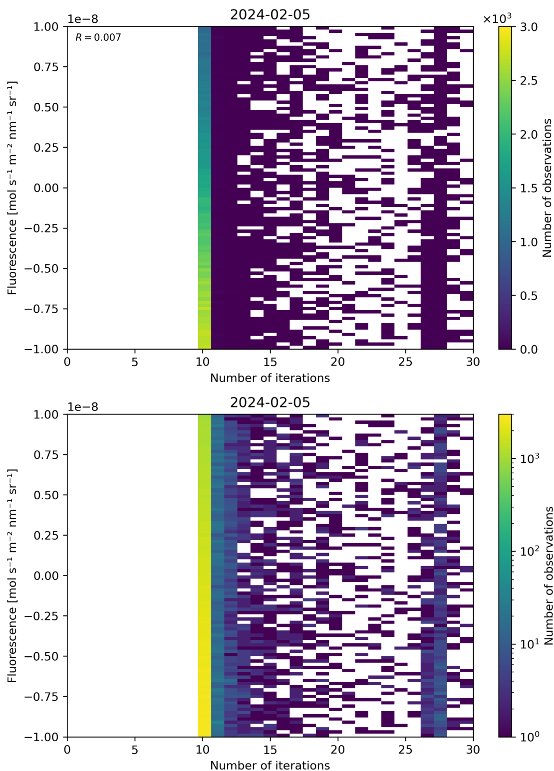
Figure 87: Scatter density plot of “Number of iterations” against “Fluorescence” for 2024-02-04 to 2024-02-06.
