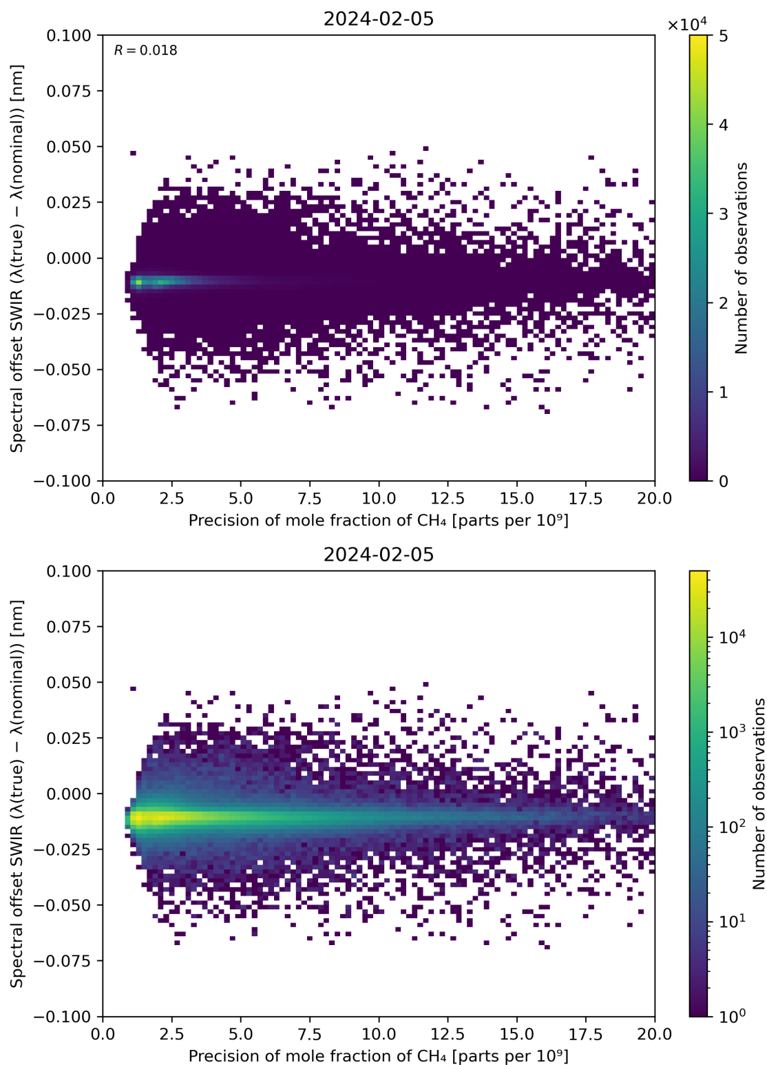
Figure 85: Scatter density plot of “Precision of mole fraction of CH 4 ” against “Spectral offset SWIR ( \lambda(\text{true}) - \lambda(\text{nominal}) )” for 2024-02-04 to 2024-02-06.
