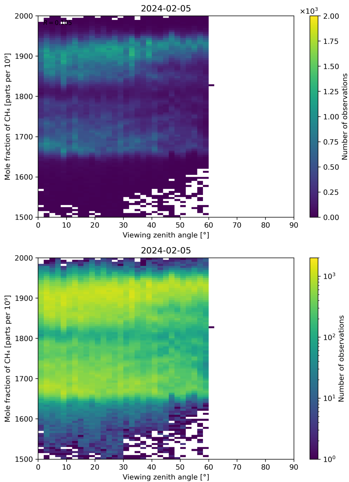
Figure 110: Scatter density plot of “Viewing zenith angle” against “Mole fraction of \text{CH}_4 ” for 2024-02-04 to 2024-02-06.
