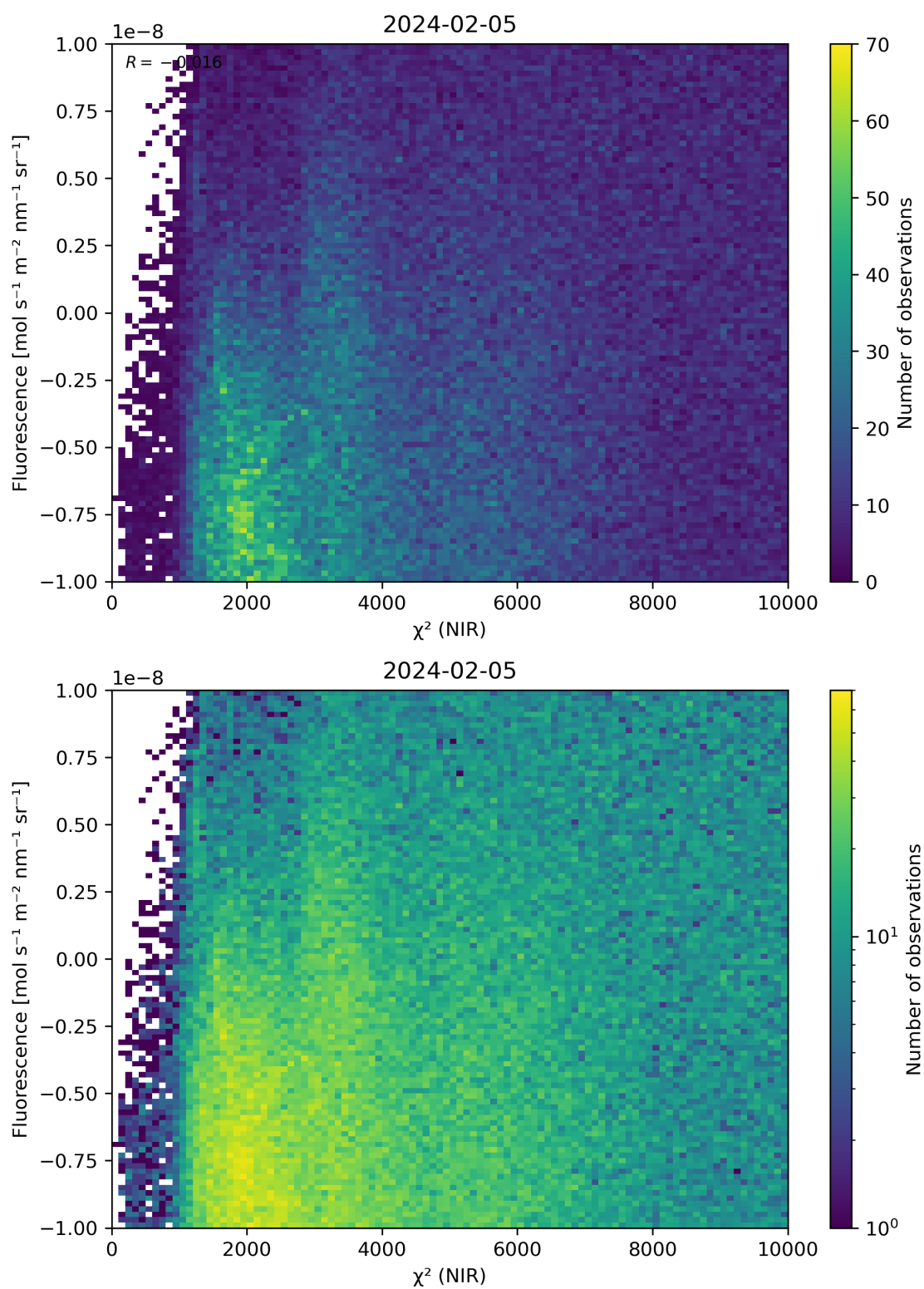
Figure 45: Scatter density plot of “ \chi^2 (NIR)” against “Fluorescence” for 2024-02-04 to 2024-02-06.
