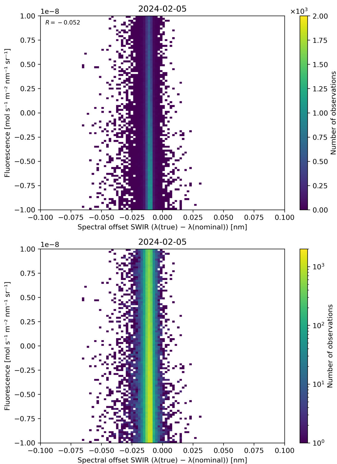
Figure 120: Scatter density plot of “Spectral offset SWIR ( \lambda(\text{true}) - \lambda(\text{nominal}) )” against “Fluorescence” for 2024-02-04 to 2024-02-06.
