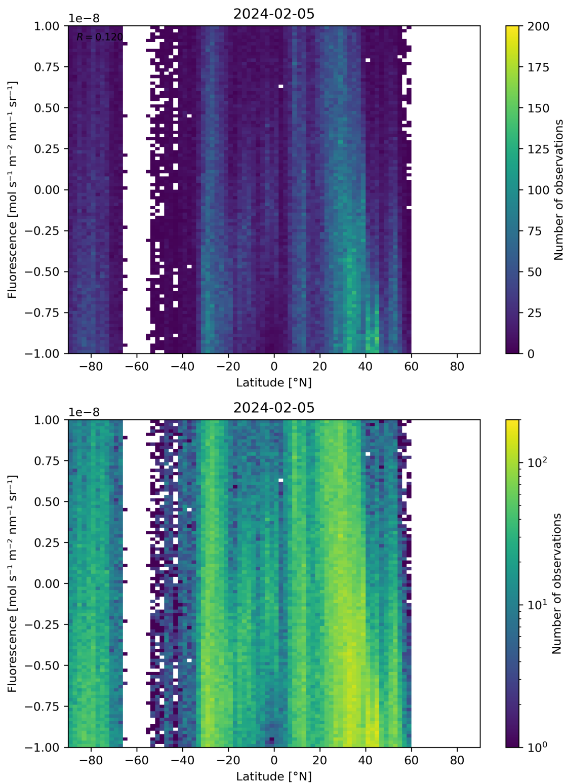
Figure 56: Scatter density plot of “Latitude” against “Fluorescence” for 2024-02-04 to 2024-02-06.
