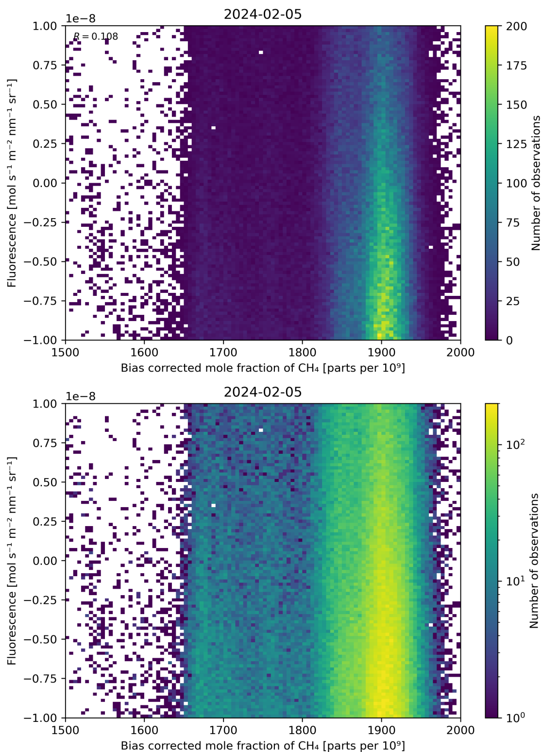
Figure 66: Scatter density plot of “Bias corrected mole fraction of \text{CH}_4 ” against “Fluorescence” for 2024-02-04 to 2024-02-06.
