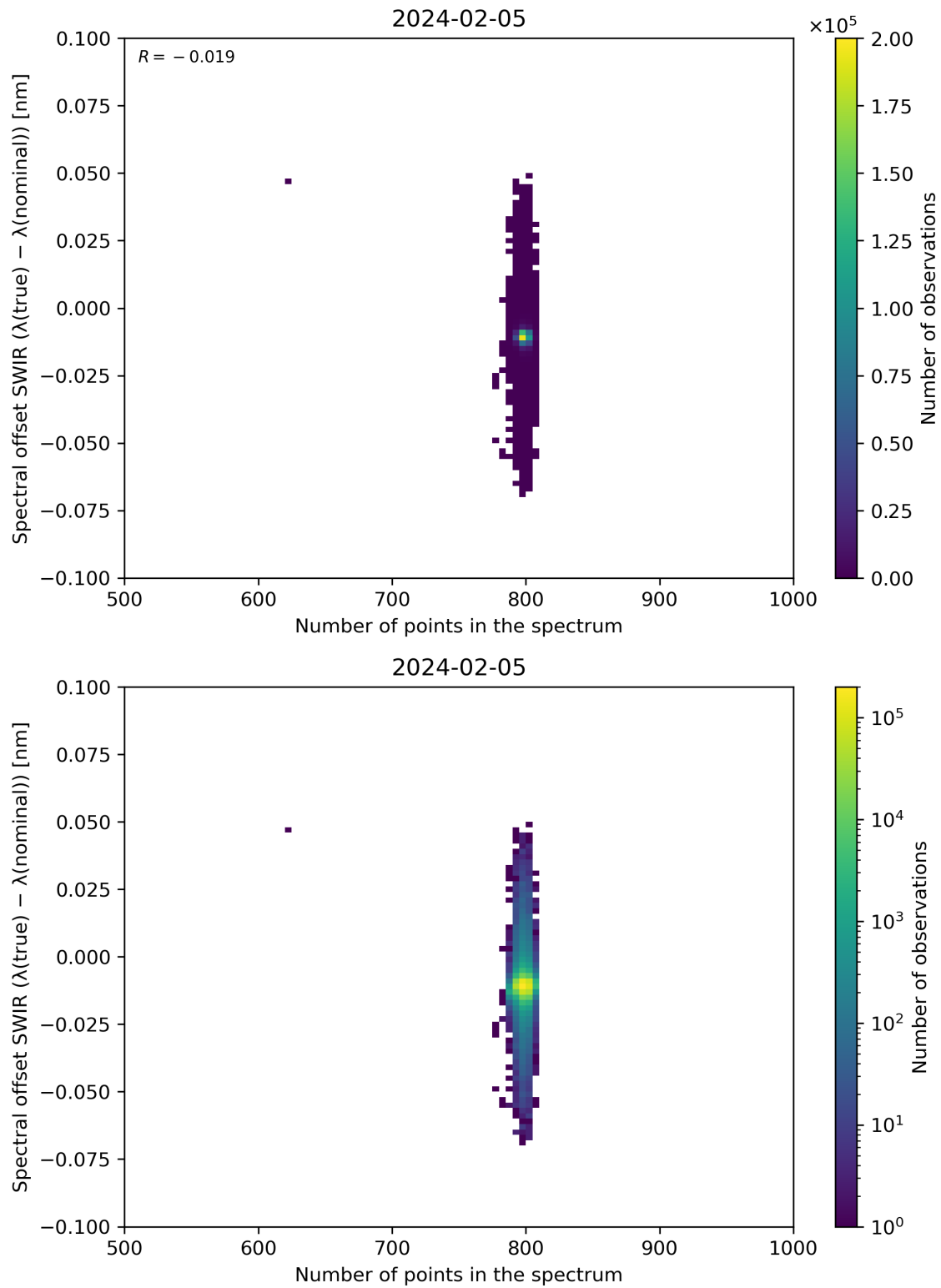
Figure 93: Scatter density plot of “Number of points in the spectrum” against “Spectral offset SWIR ( \lambda(\text{true}) - \lambda(\text{nominal}) )” for 2024-02-04 to 2024-02-06.
