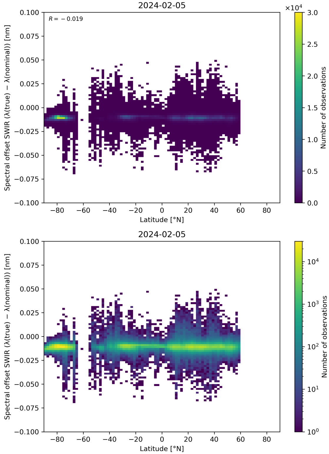
Figure 62: Scatter density plot of “Latitude” against “Spectral offset SWIR ( \lambda(\text{true}) - \lambda(\text{nominal}) )” for 2024-02-04 to 2024-02-06.
