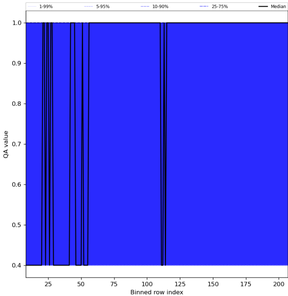
Figure 33: Along track statistics of “QA value” for 2024-02-04 to 2024-02-06
