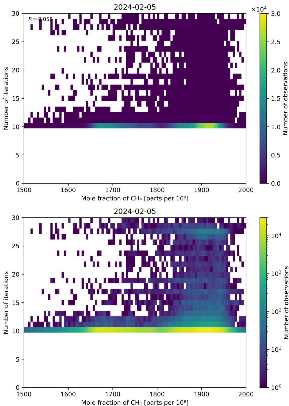
Figure 76: Scatter density plot of “Mole fraction of CH 4 ” against “Number of iterations” for 2024-02-04 to 2024-02-06.
