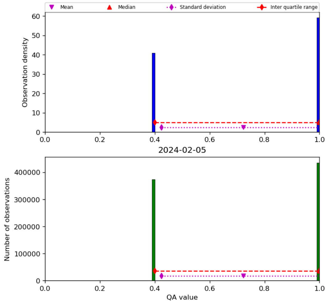
Figure 22: Histogram of “QA value” for 2024-02-04 to 2024-02-06
