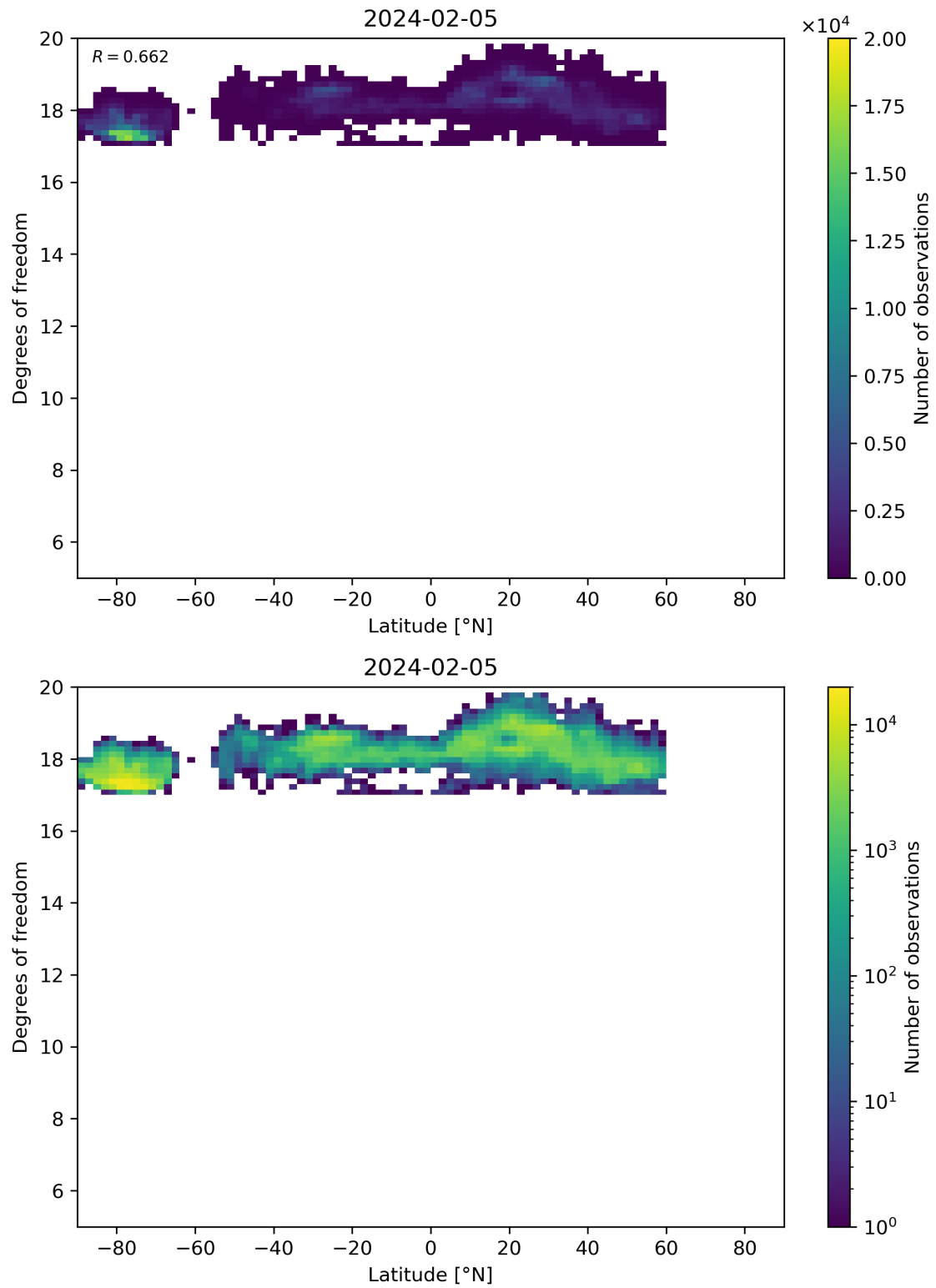
Figure 55: Scatter density plot of “Latitude” against “Degrees of freedom” for 2024-02-04 to 2024-02-06.
