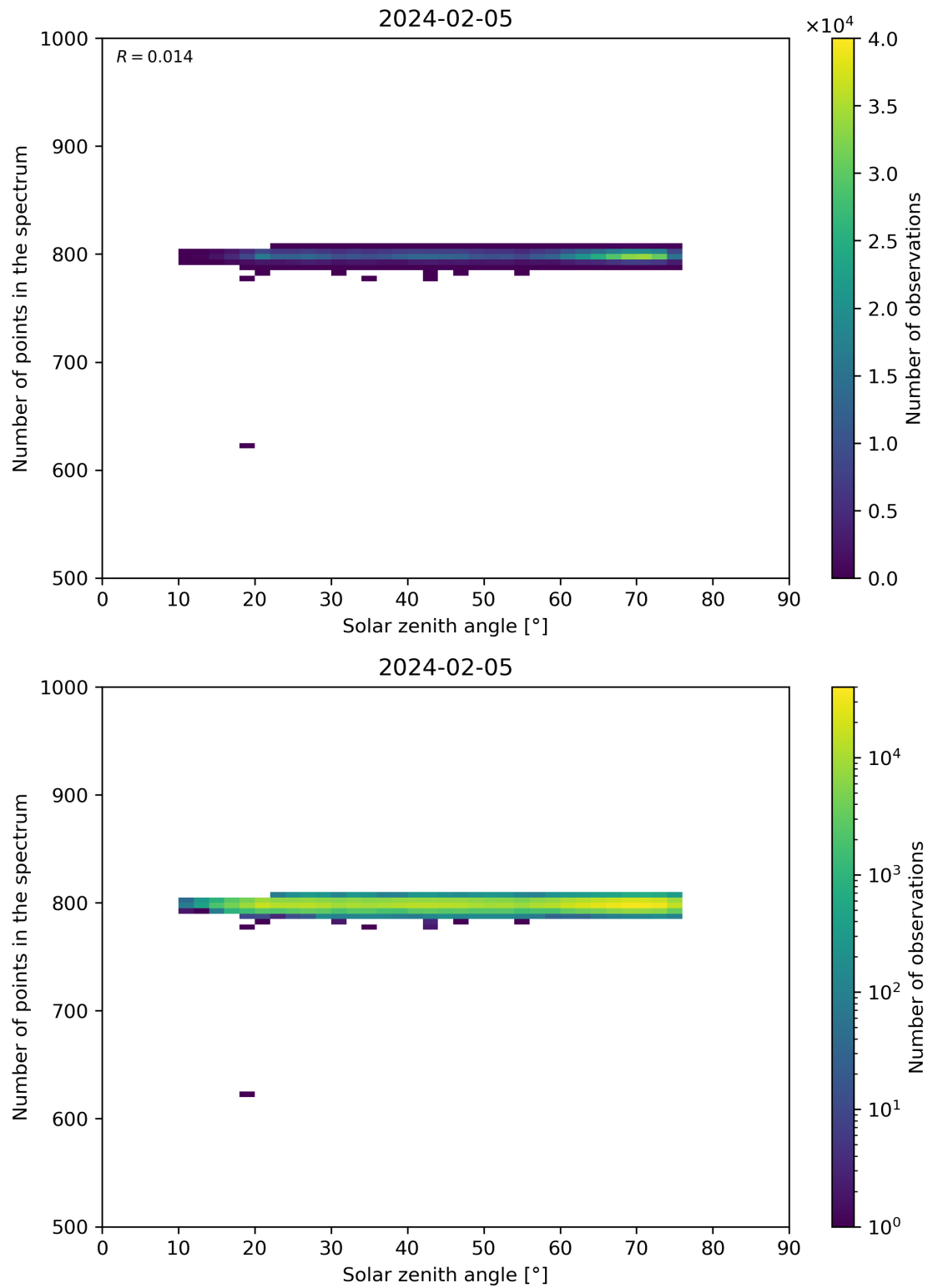
Figure 103: Scatter density plot of “Solar zenith angle” against “Number of points in the spectrum” for 2024-02-04 to 2024-02-06.
