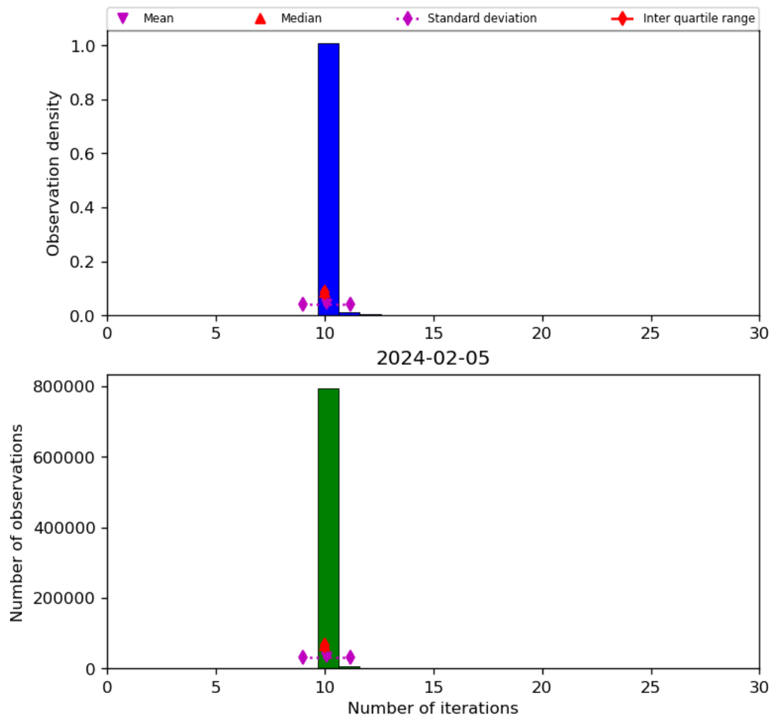
Figure 31: Histogram of “Number of iterations” for 2024-02-04 to 2024-02-06
