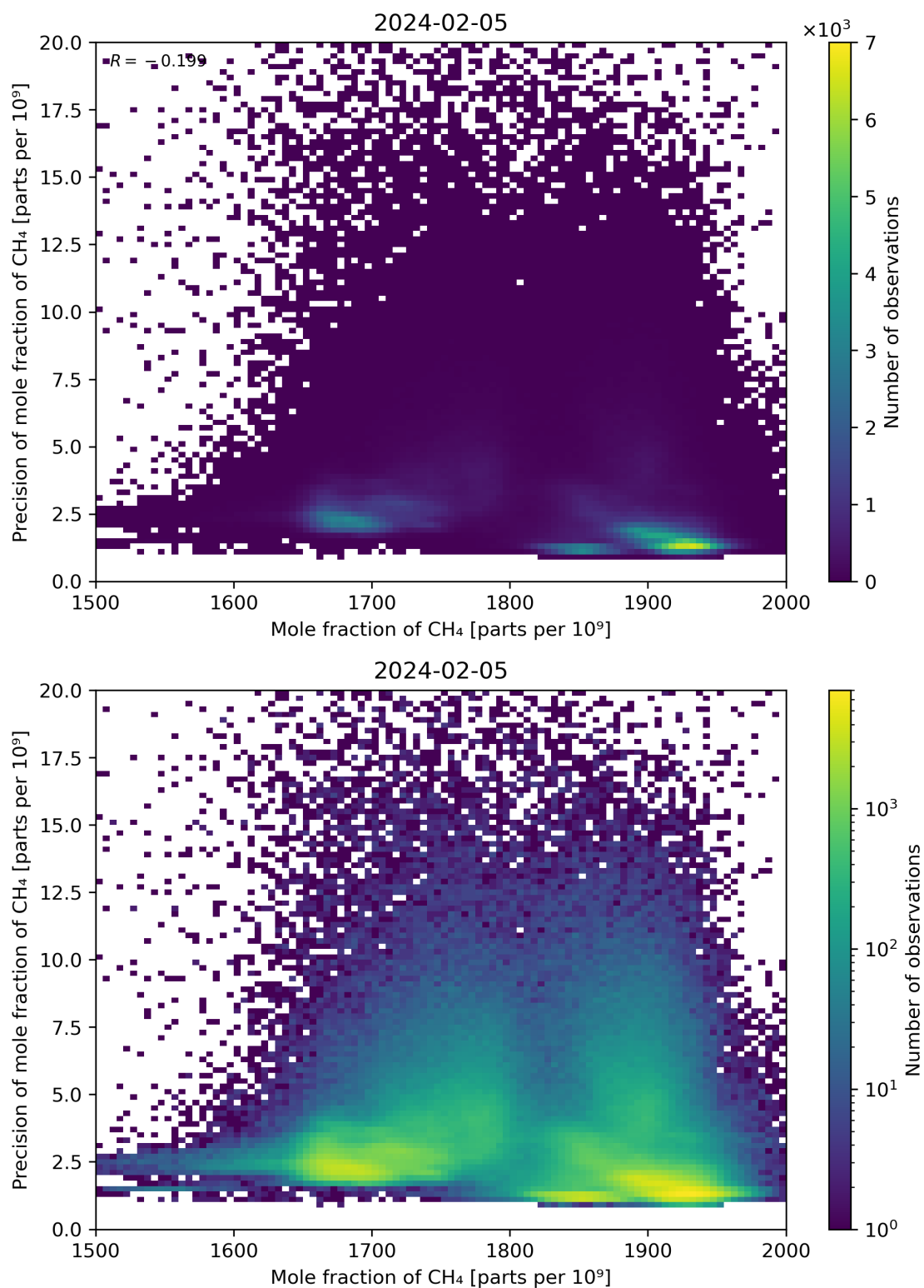
Figure 75: Scatter density plot of “Mole fraction of CH 4 ” against “Precision of mole fraction of CH 4 ” for 2024-02-04 to 2024-02-06.
