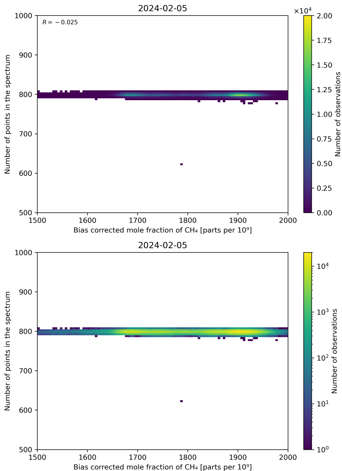
Figure 68: Scatter density plot of “Bias corrected mole fraction of CH 4 ” against “Number of points in the spectrum” for 2024-02-04 to 2024-02-06.
