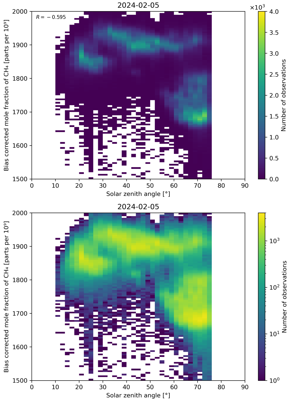
Figure 100: Scatter density plot of “Solar zenith angle” against “Bias corrected mole fraction of CH 4 ” for 2024-02-04 to 2024-02-06.
