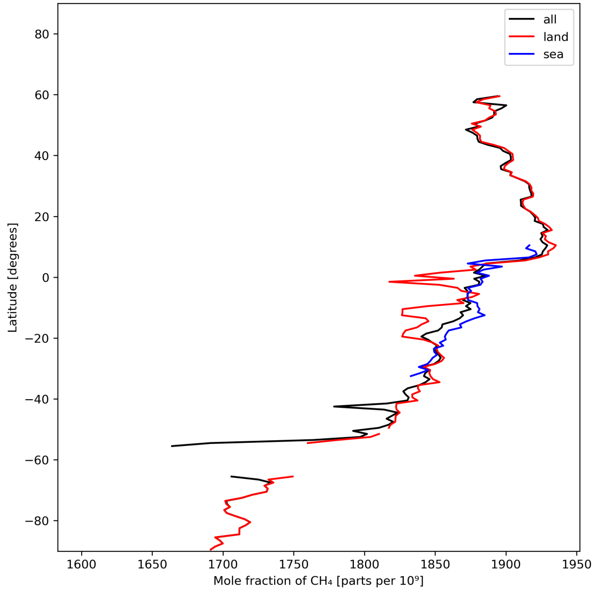
Figure 12: Zonal average of “Mole fraction of \text{CH}_4 ” for 2024-02-04 to 2024-02-06.
