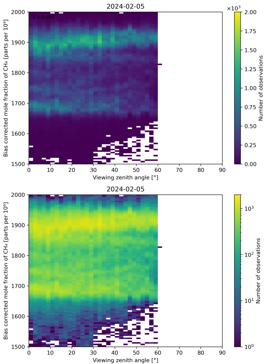
Figure 111: Scatter density plot of “Viewing zenith angle” against “Bias corrected mole fraction of CH 4 ” for 2024-02-04 to 2024-02-06.
