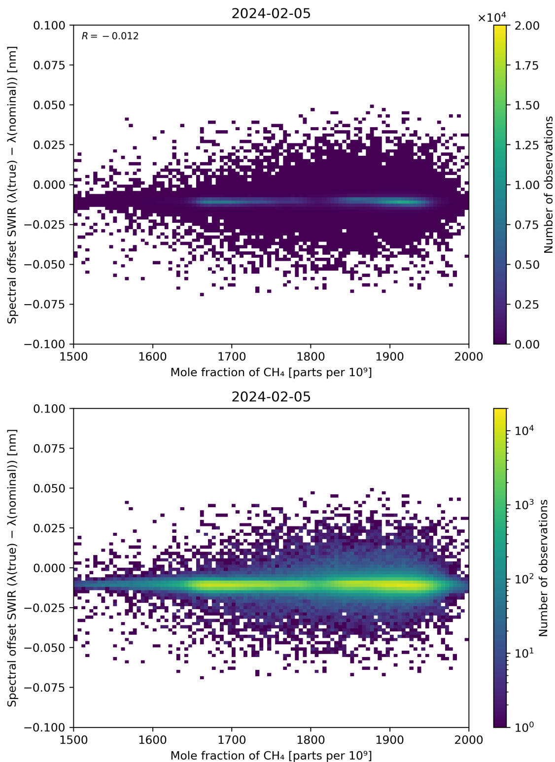
Figure 86: Scatter density plot of “Mole fraction of CH 4 ” against “Spectral offset SWIR ( \lambda(\text{true}) - \lambda(\text{nominal}) )” for 2024-02-04 to 2024-02-06.
