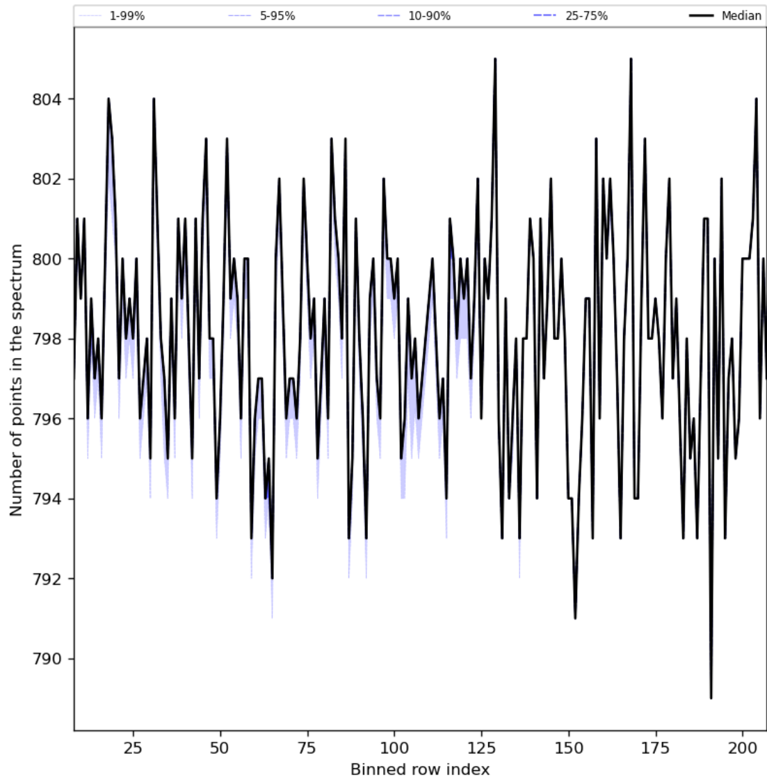
Figure 37: Along track statistics of “Number of points in the spectrum” for 2024-02-04 to 2024-02-06
