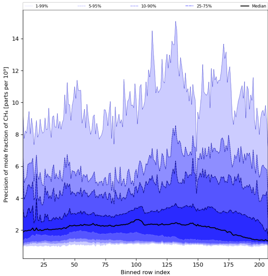
Figure 35: Along track statistics of “Precision of mole fraction of CH 4 ” for 2024-02-04 to 2024-02-06
