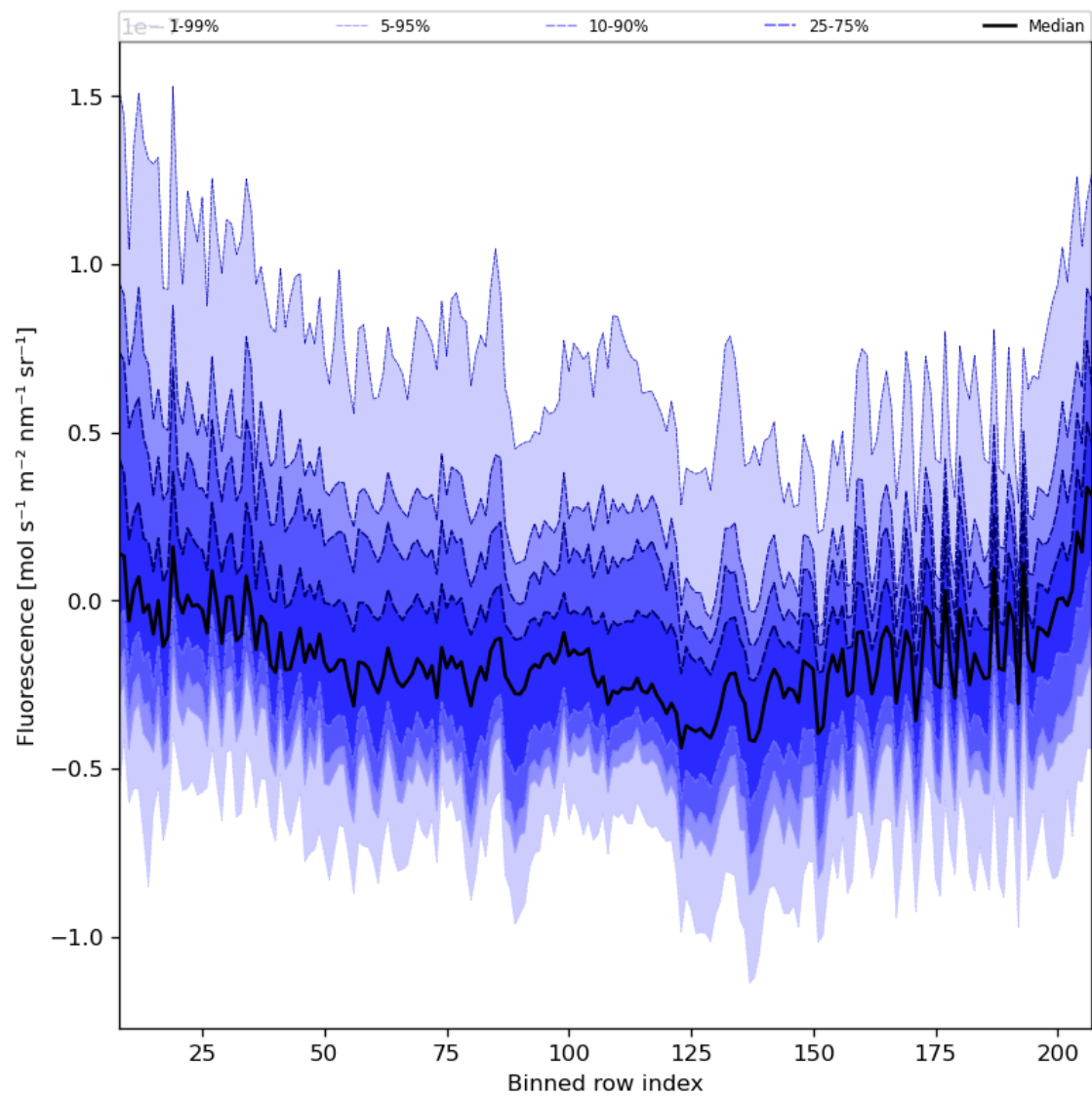
Figure 43: Along track statistics of “Fluorescence” for 2024-02-04 to 2024-02-06
