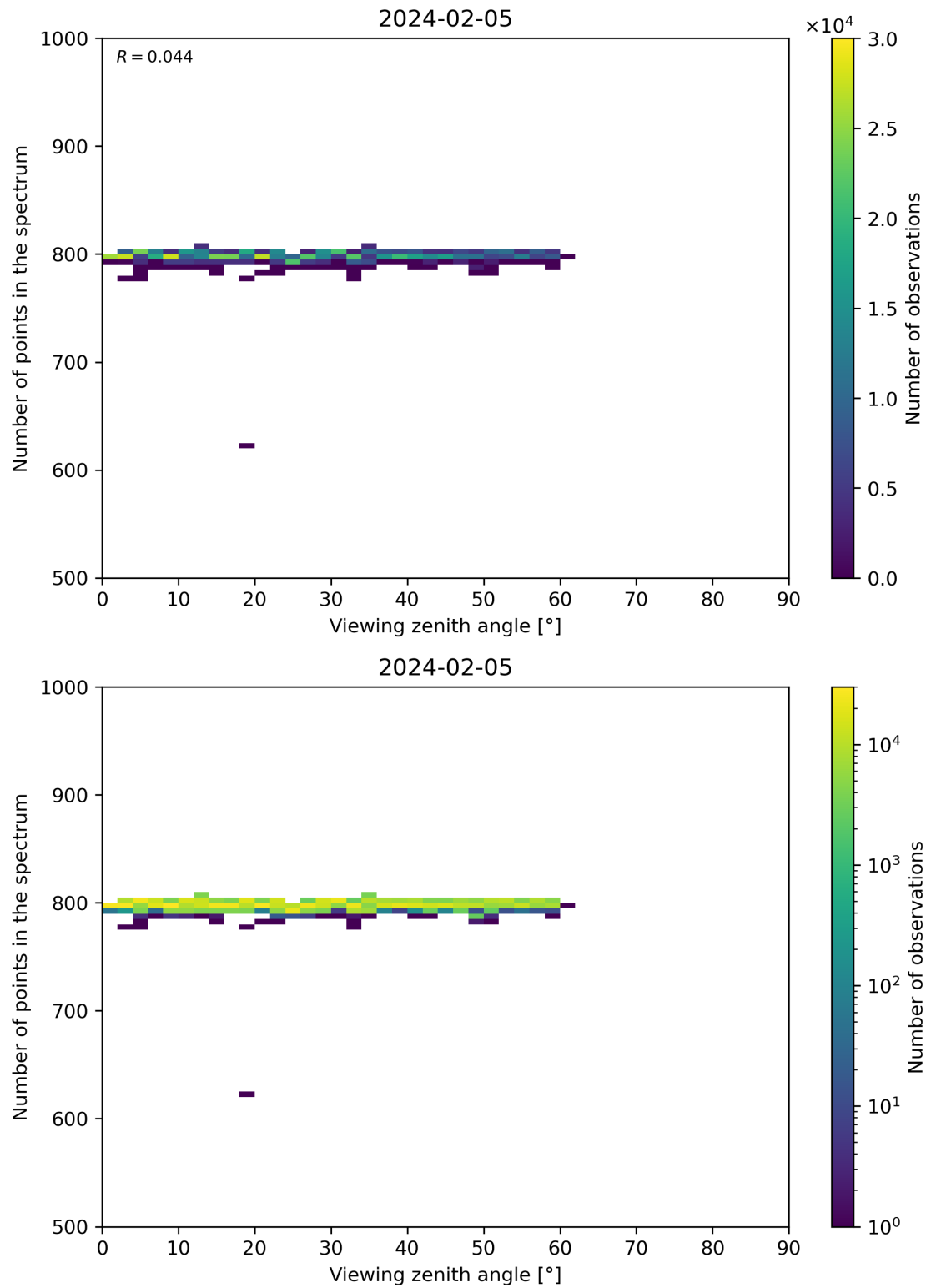
Figure 114: Scatter density plot of “Viewing zenith angle” against “Number of points in the spectrum” for 2024-02-04 to 2024-02-06.
