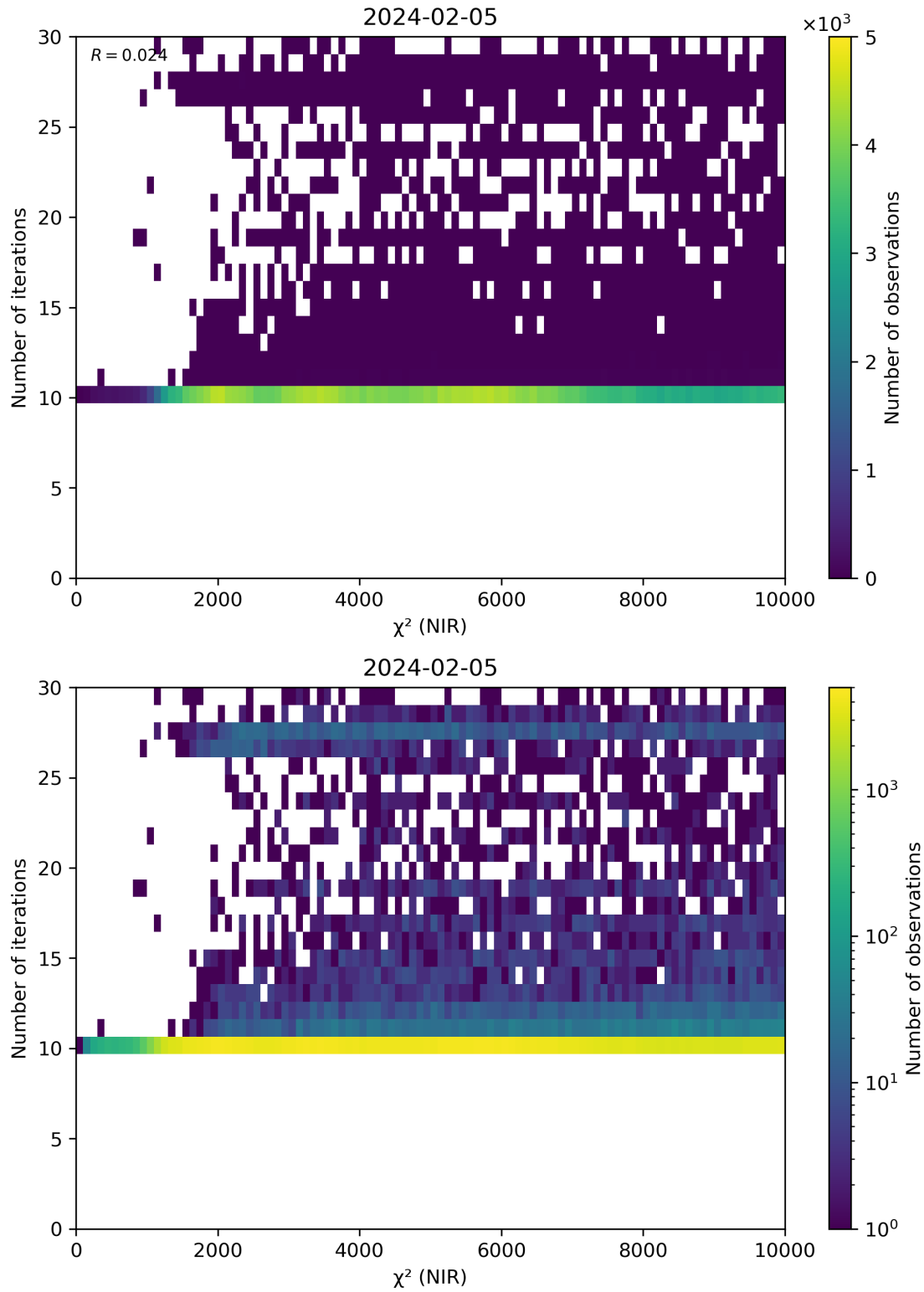
Figure 46: Scatter density plot of “ \chi^2 (NIR)” against “Number of iterations” for 2024-02-04 to 2024-02-06.
