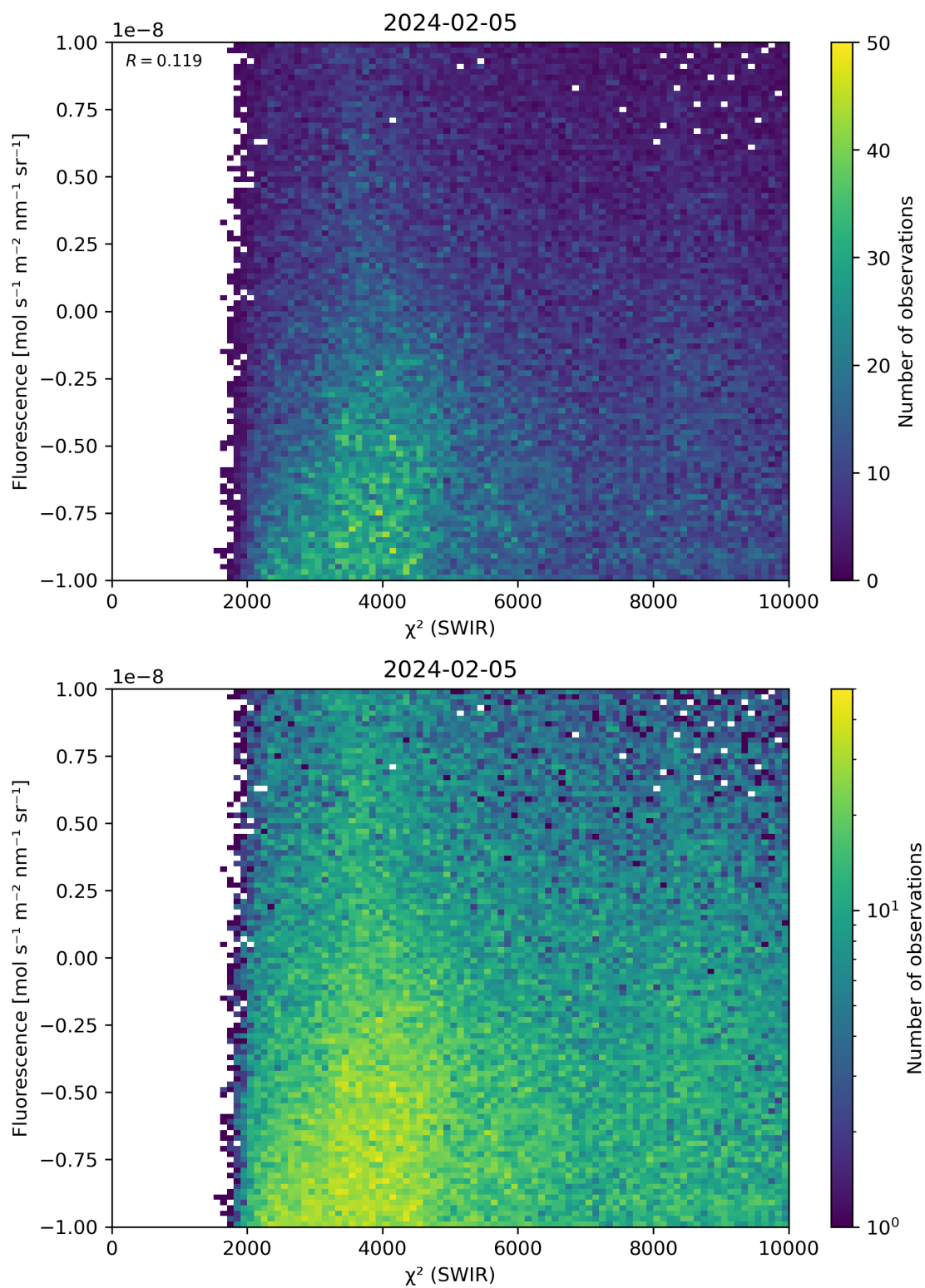
Figure 49: Scatter density plot of “ \chi^2 (SWIR)” against “Fluorescence” for 2024-02-04 to 2024-02-06.
