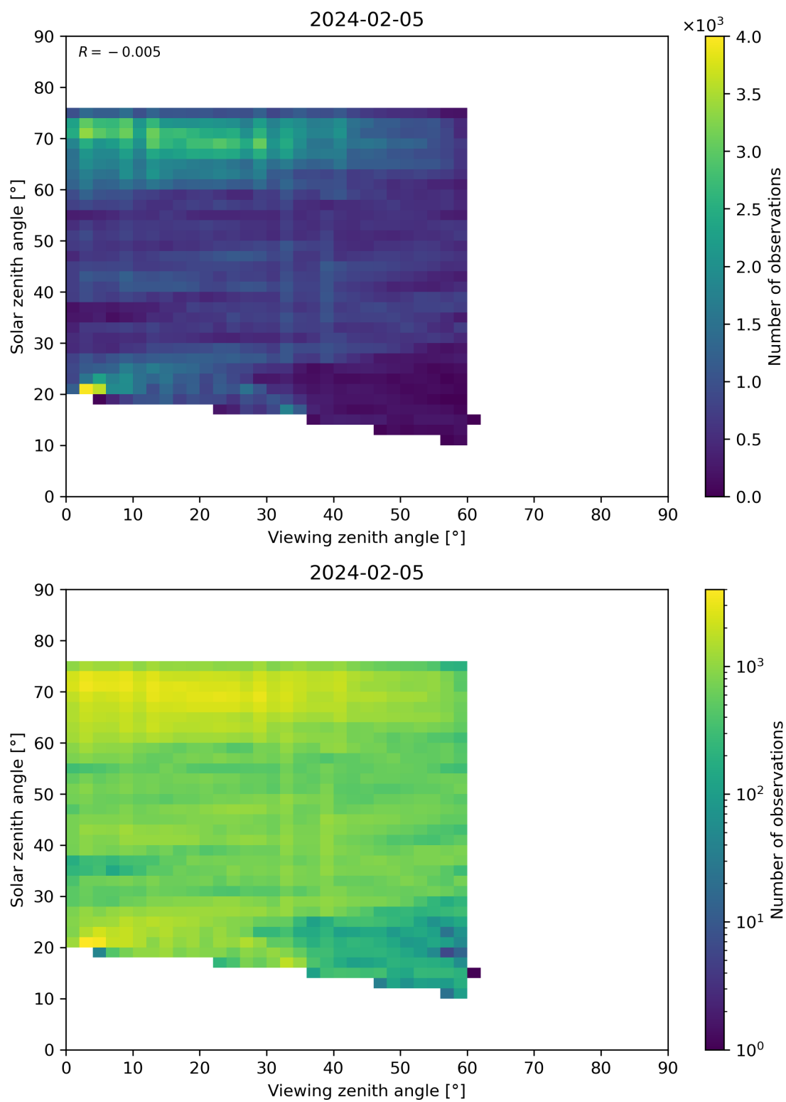
Figure 115: Scatter density plot of “Viewing zenith angle” against “Solar zenith angle” for 2024-02-04 to 2024-02-06.
