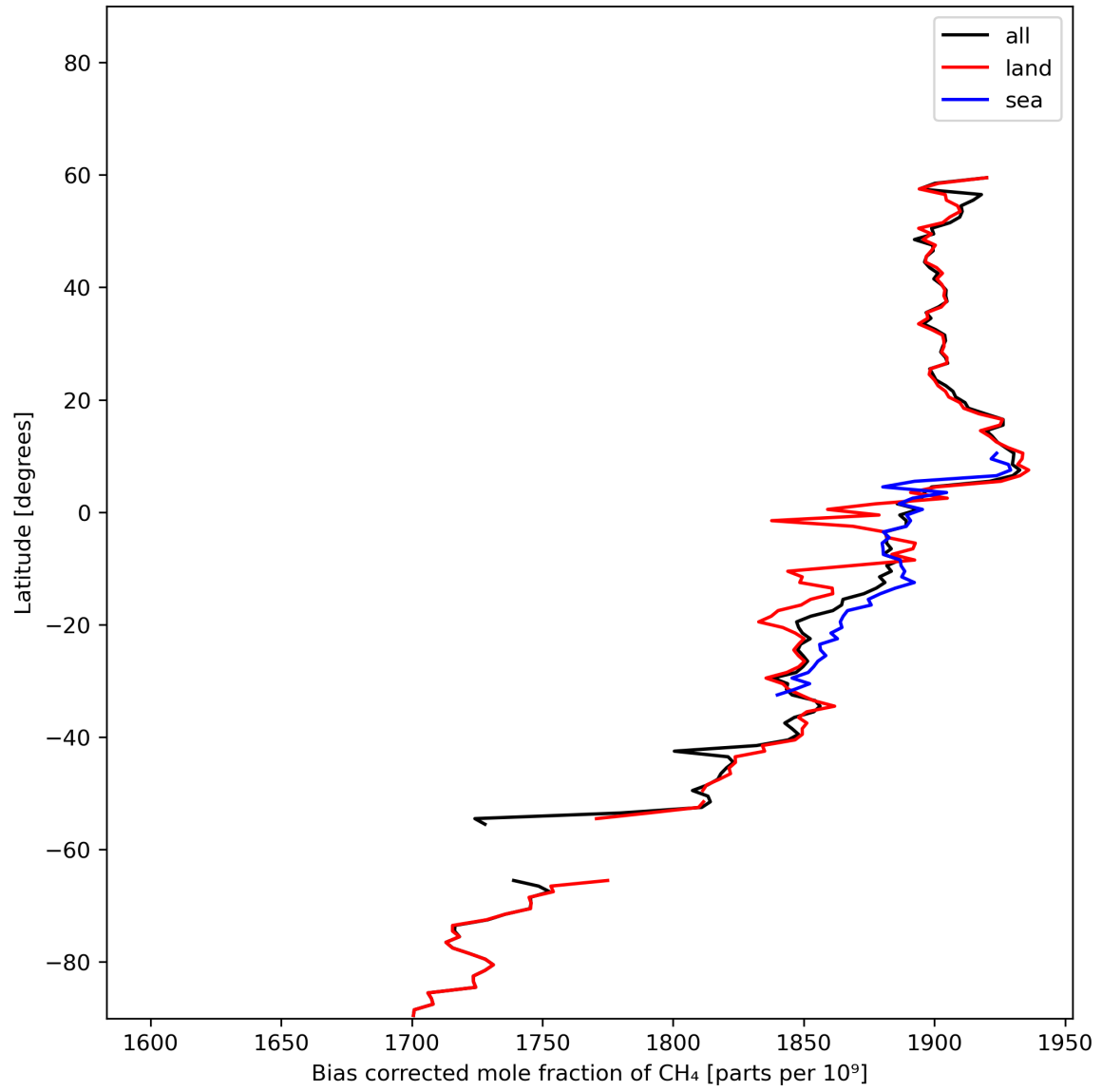
Figure 14: Zonal average of “Bias corrected mole fraction of CH 4 ” for 2024-02-04 to 2024-02-06.
