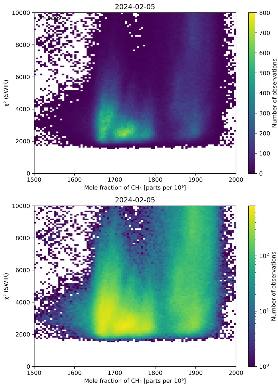
Figure 71: Scatter density plot of “Mole fraction of CH 4 ” against “ \chi^2 (SWIR)” for 2024-02-04 to 2024-02-06.
