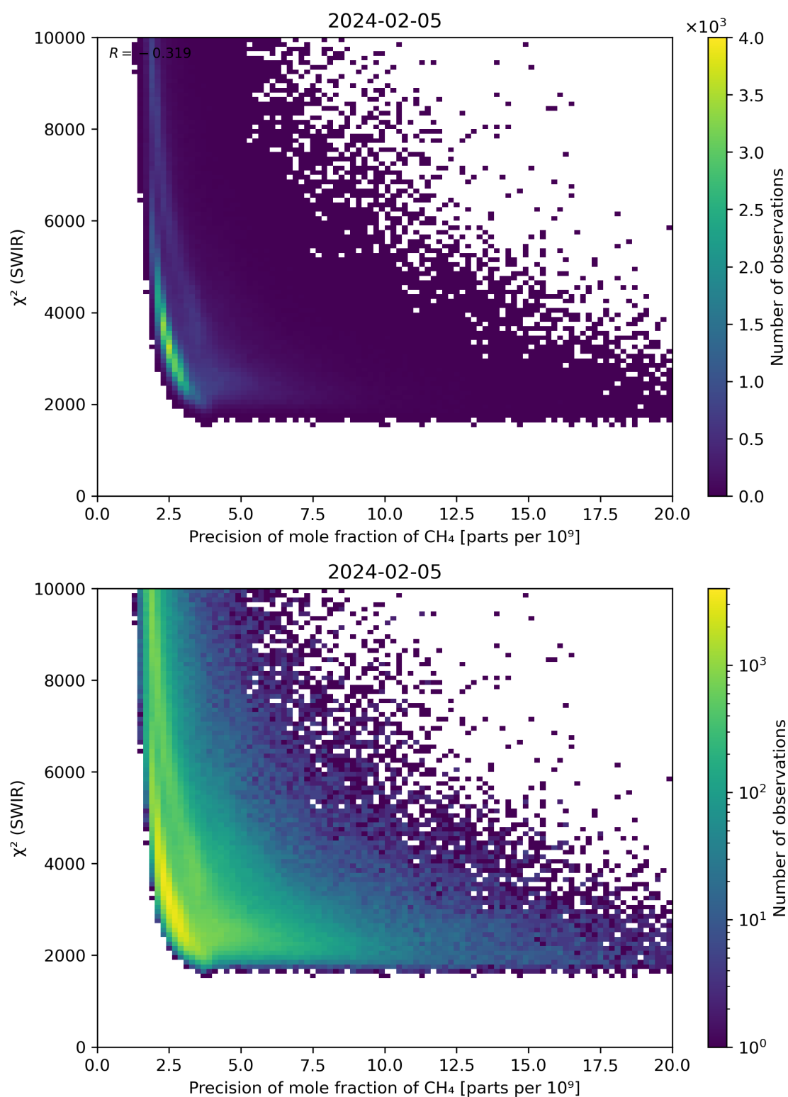
Figure 79: Scatter density plot of “Precision of mole fraction of CH 4 ” against “ \chi^2 (SWIR)” for 2024-02-04 to 2024-02-06.
