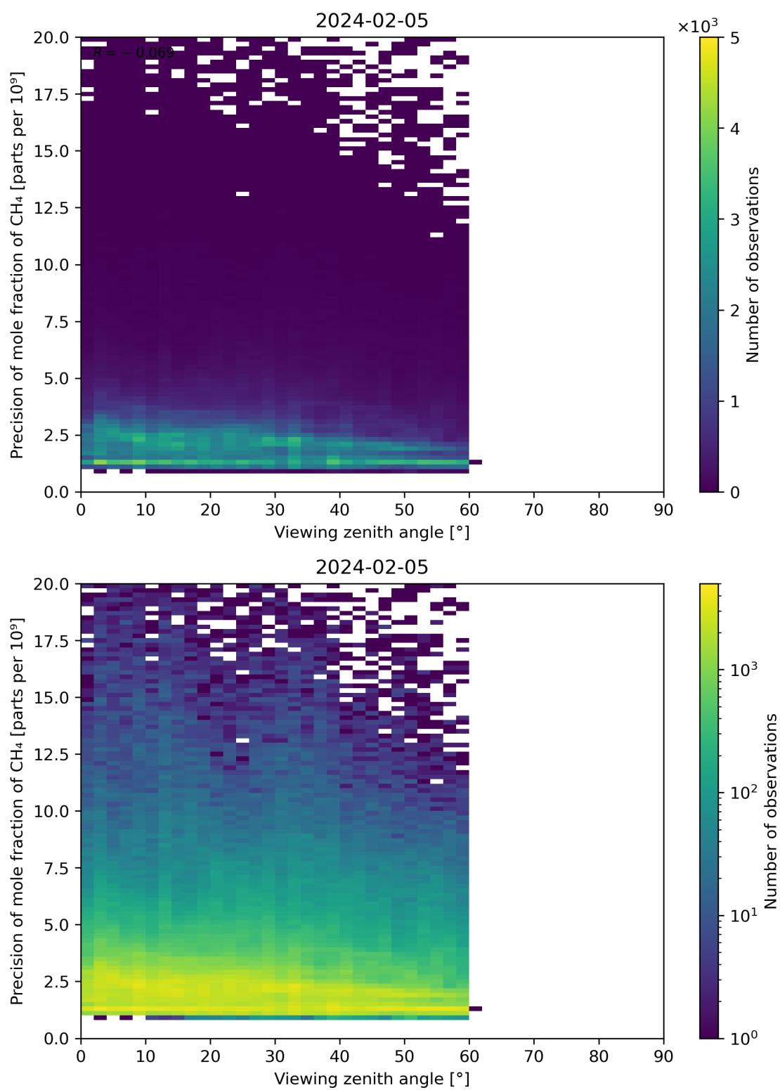
Figure 112: Scatter density plot of “Viewing zenith angle” against “Precision of mole fraction of CH 4 ” for 2024-02-04 to 2024-02-06.
