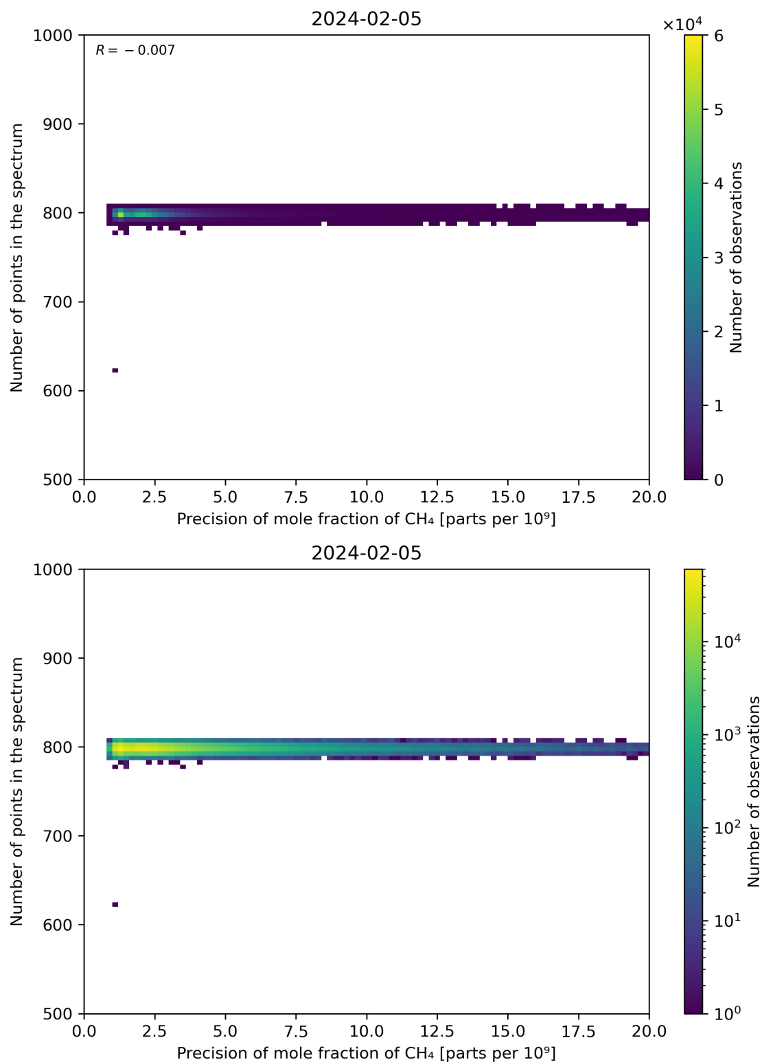
Figure 84: Scatter density plot of “Precision of mole fraction of CH 4 ” against “Number of points in the spectrum” for 2024-02-04 to 2024-02-06.
