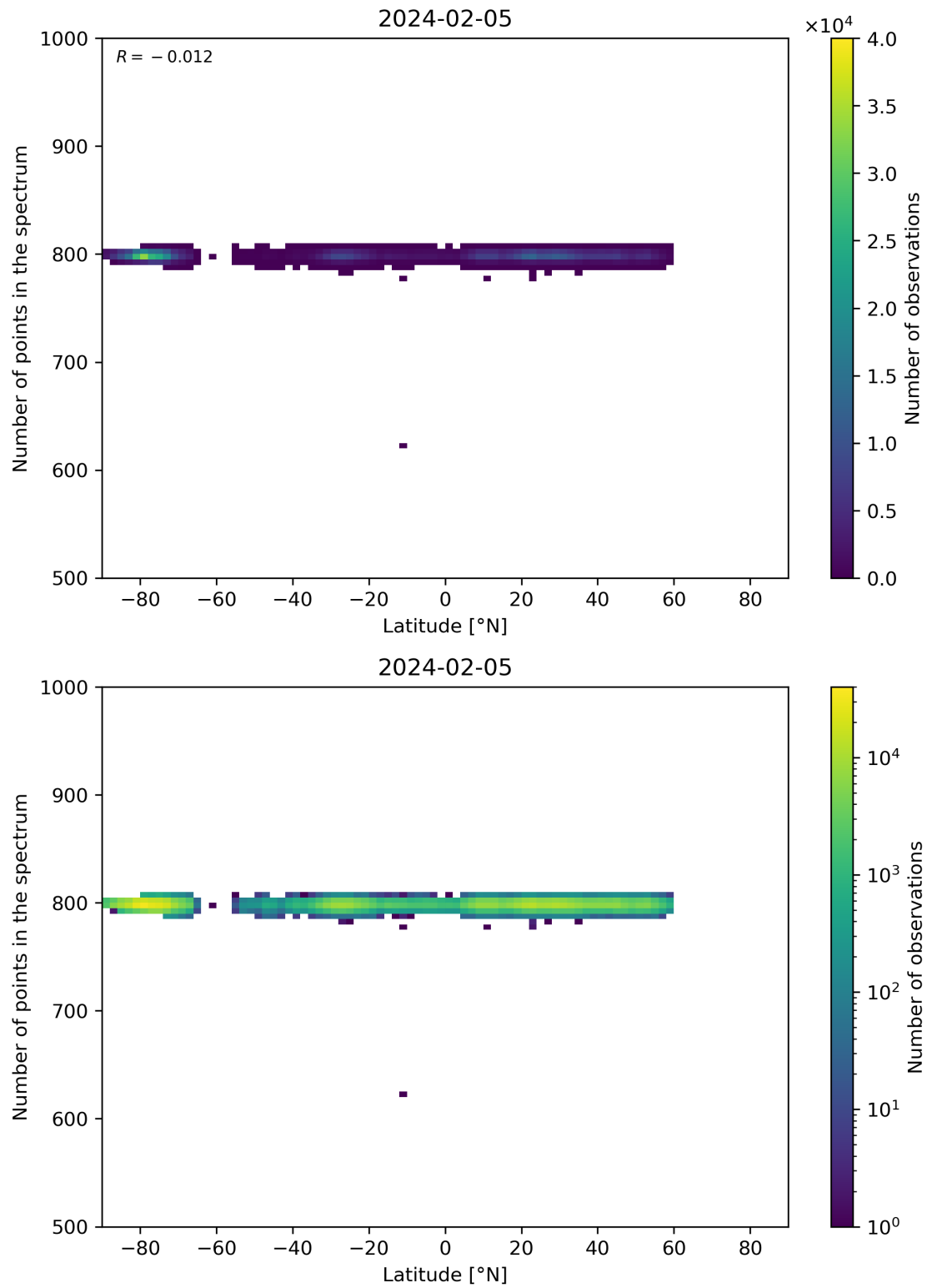
Figure 61: Scatter density plot of “Latitude” against “Number of points in the spectrum” for 2024-02-04 to 2024-02-06.
