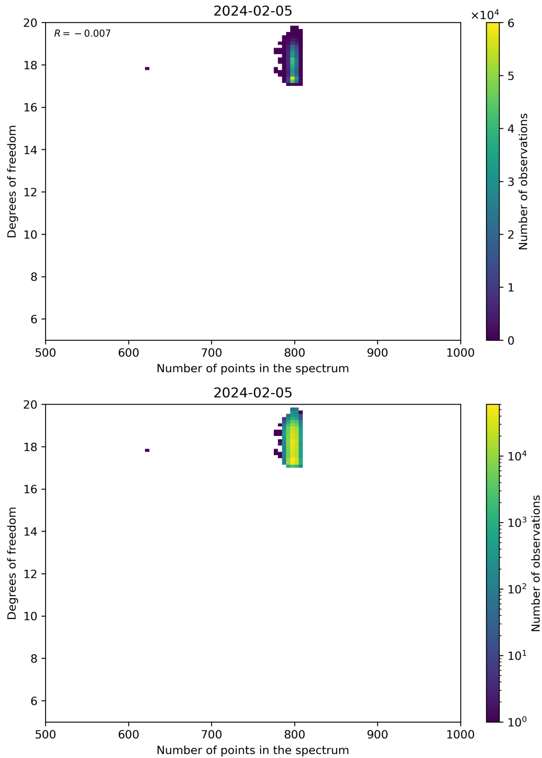
Figure 90: Scatter density plot of “Number of points in the spectrum” against “Degrees of freedom” for 2024-02-04 to 2024-02-06.
