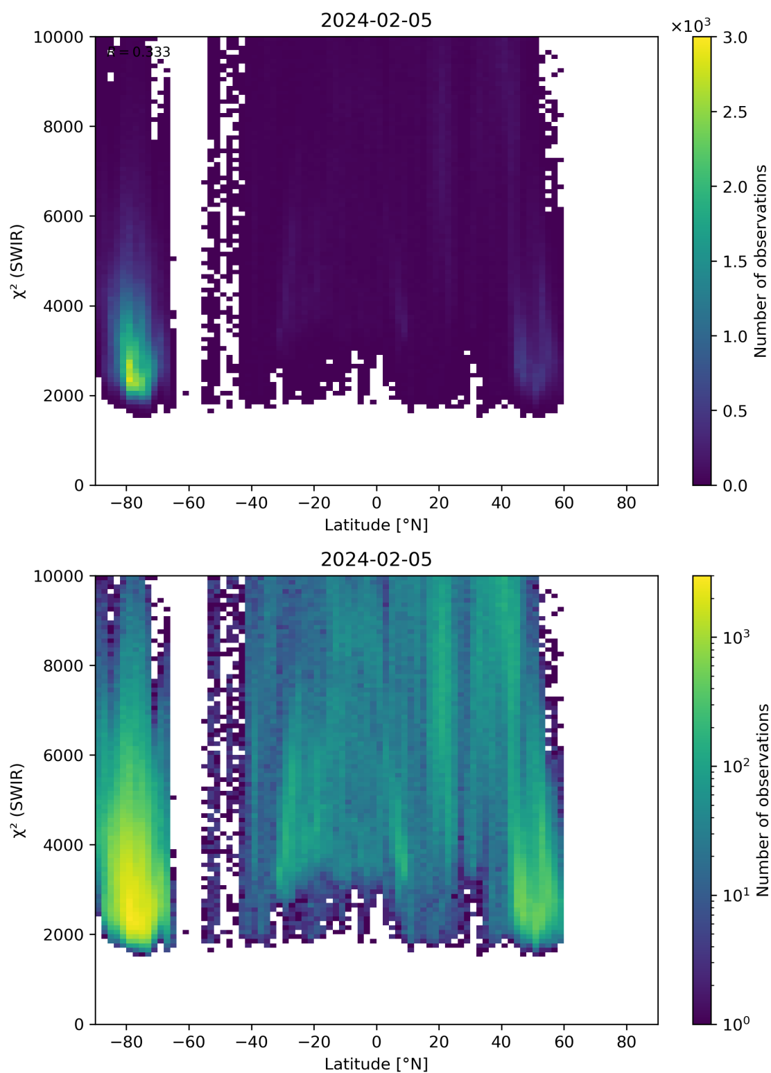
Figure 54: Scatter density plot of “Latitude” against “ \chi^2 (SWIR)” for 2024-02-04 to 2024-02-06.
