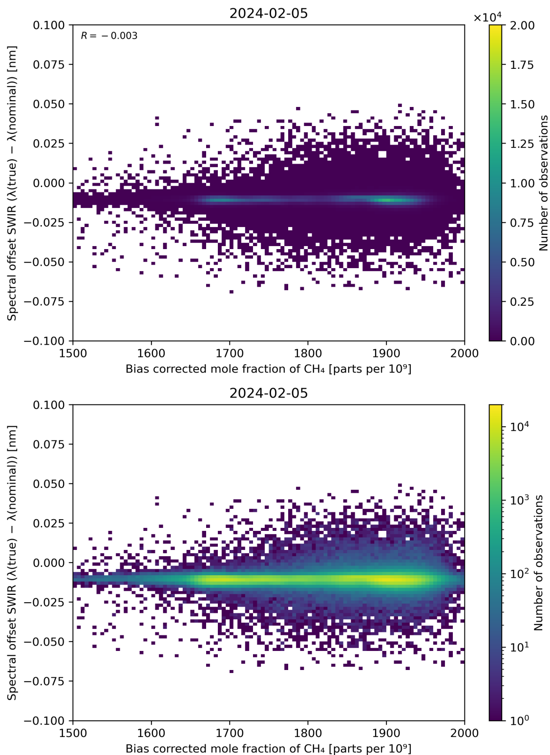
Figure 69: Scatter density plot of “Bias corrected mole fraction of \text{CH}_4 ” against “Spectral offset SWIR ( \lambda(\text{true}) - \lambda(\text{nominal}) )” for 2024-02-04 to 2024-02-06.
