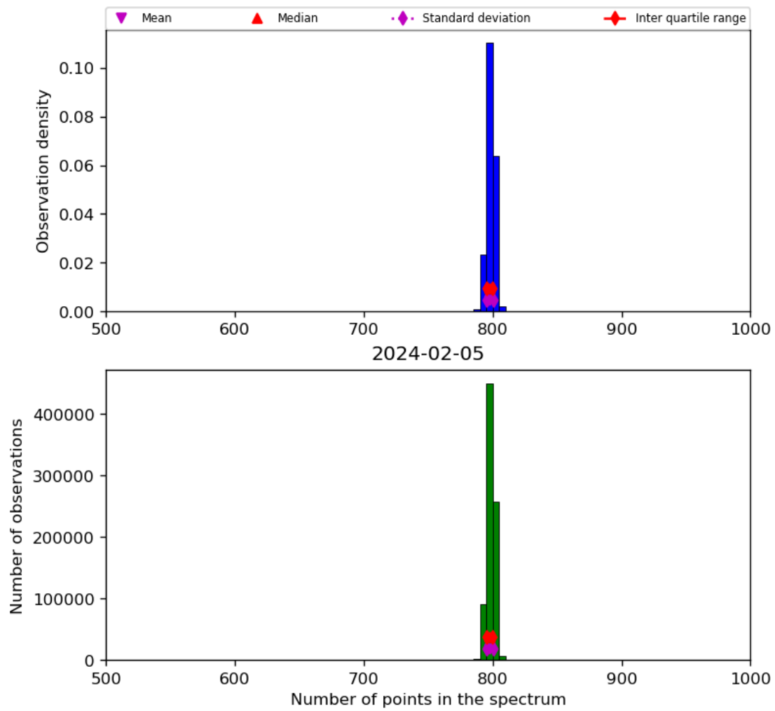
Figure 26: Histogram of “Number of points in the spectrum” for 2024-02-04 to 2024-02-06
