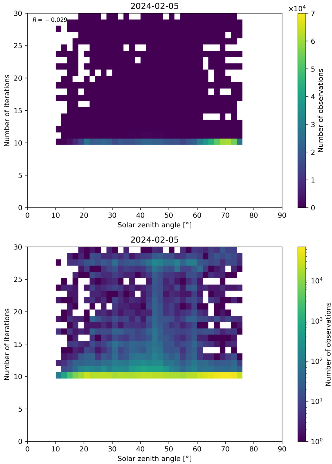
Figure 102: Scatter density plot of “Solar zenith angle” against “Number of iterations” for 2024-02-04 to 2024-02-06.
