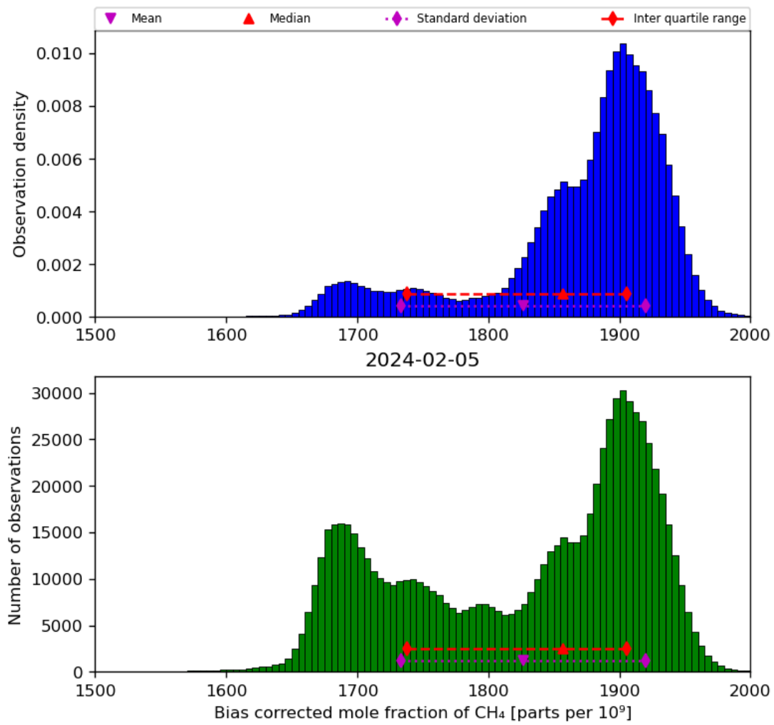
Figure 25: Histogram of “Bias corrected mole fraction of CH 4 ” for 2024-02-04 to 2024-02-06
