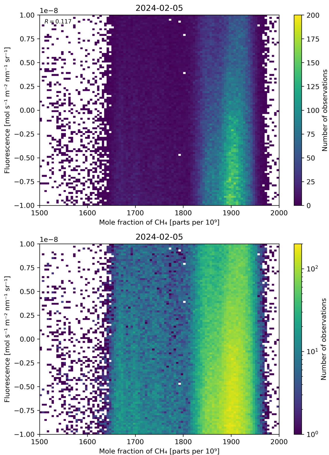
Figure 73: Scatter density plot of “Mole fraction of \text{CH}_4 ” against “Fluorescence” for 2024-02-04 to 2024-02-06.
