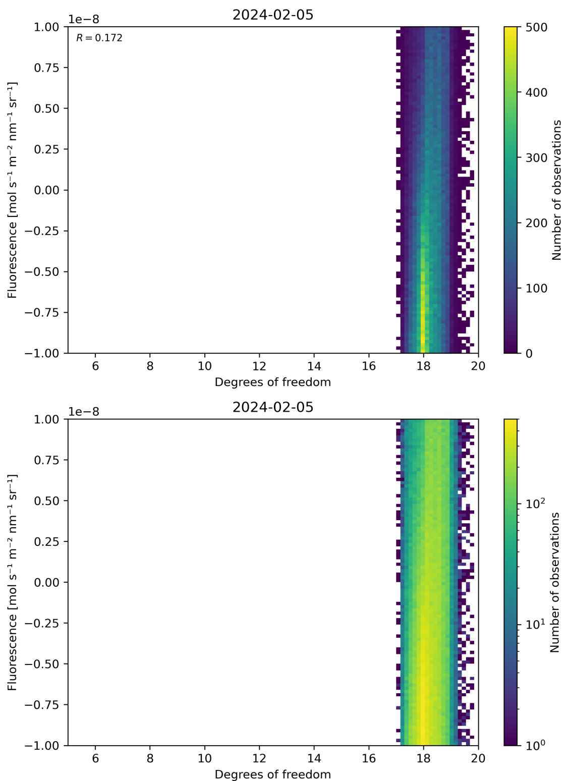
Figure 51: Scatter density plot of “Degrees of freedom” against “Fluorescence” for 2024-02-04 to 2024-02-06.
