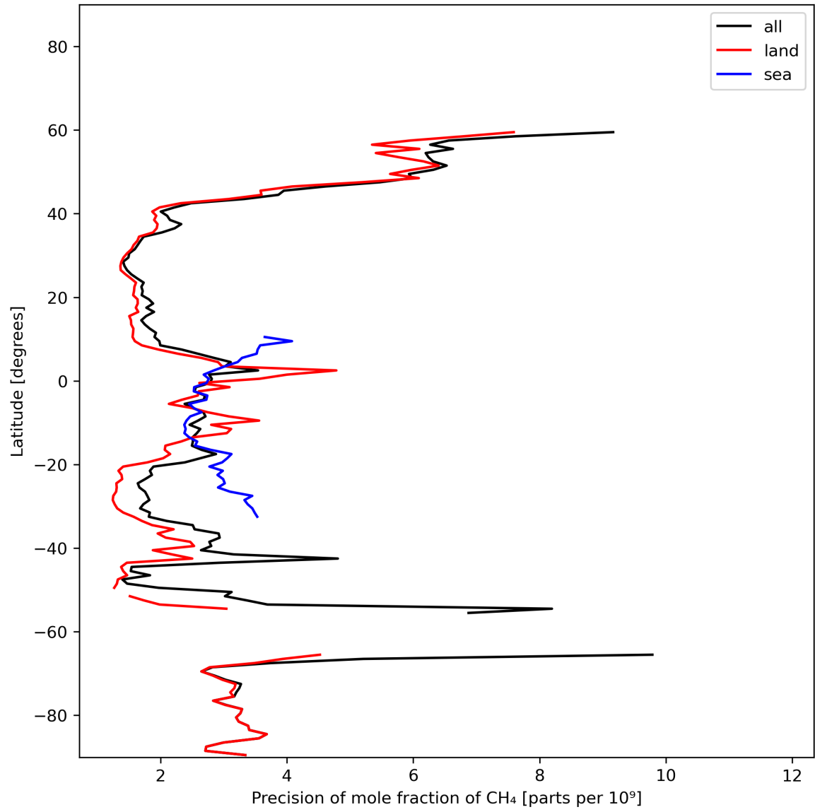
Figure 13: Zonal average of “Precision of mole fraction of CH 4 ” for 2024-02-04 to 2024-02-06.
