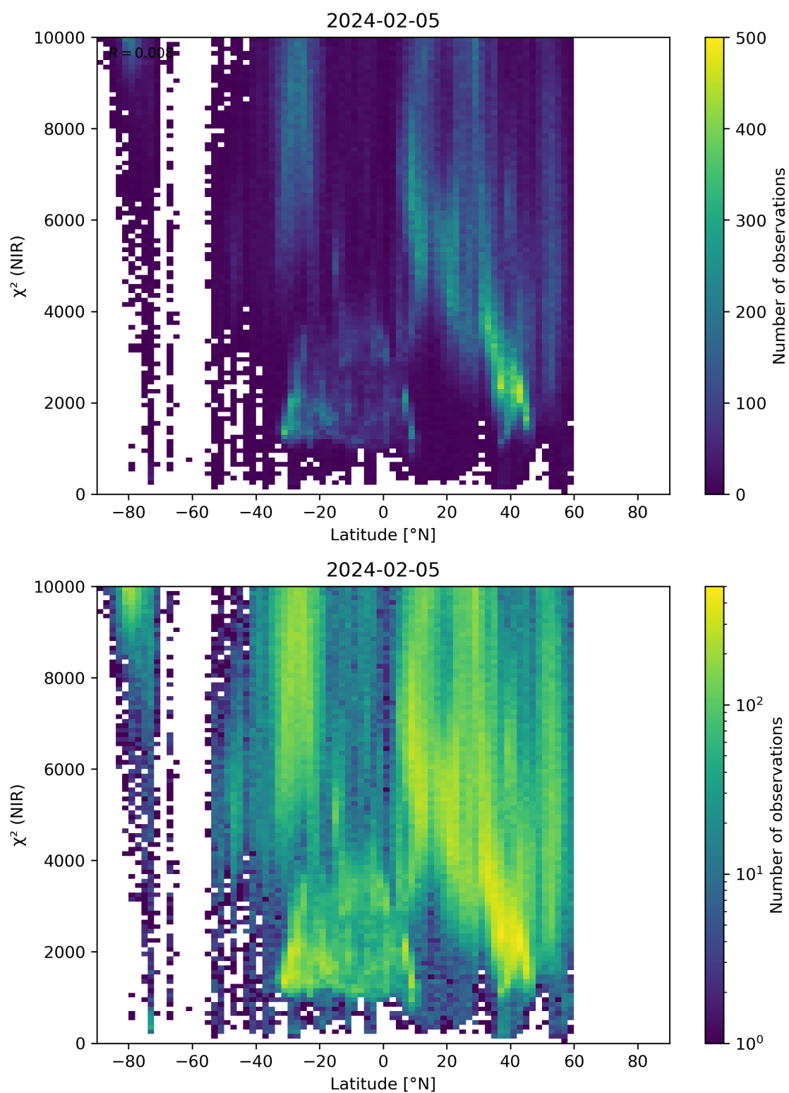
Figure 53: Scatter density plot of “Latitude” against “ \chi^2 (NIR)” for 2024-02-04 to 2024-02-06.
