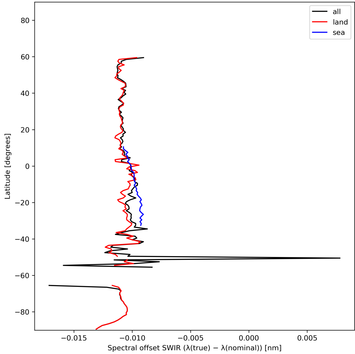
Figure 16: Zonal average of “Spectral offset SWIR ( \lambda(\text{true}) - \lambda(\text{nominal}) )” for 2024-02-04 to 2024-02-06.
