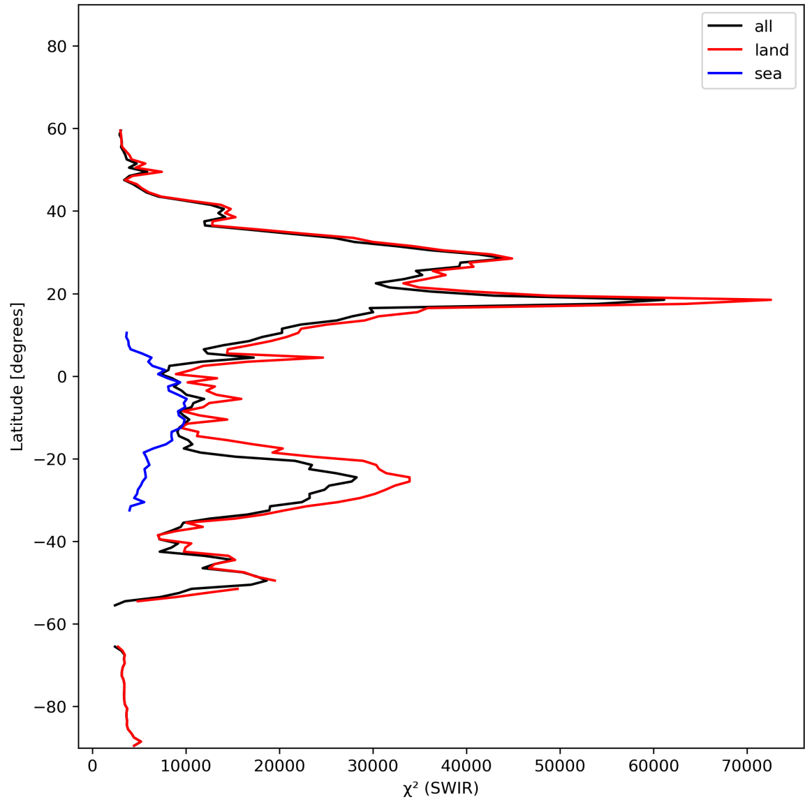
Figure 17: Zonal average of “ \chi^2 (SWIR)” for 2024-02-04 to 2024-02-06.
