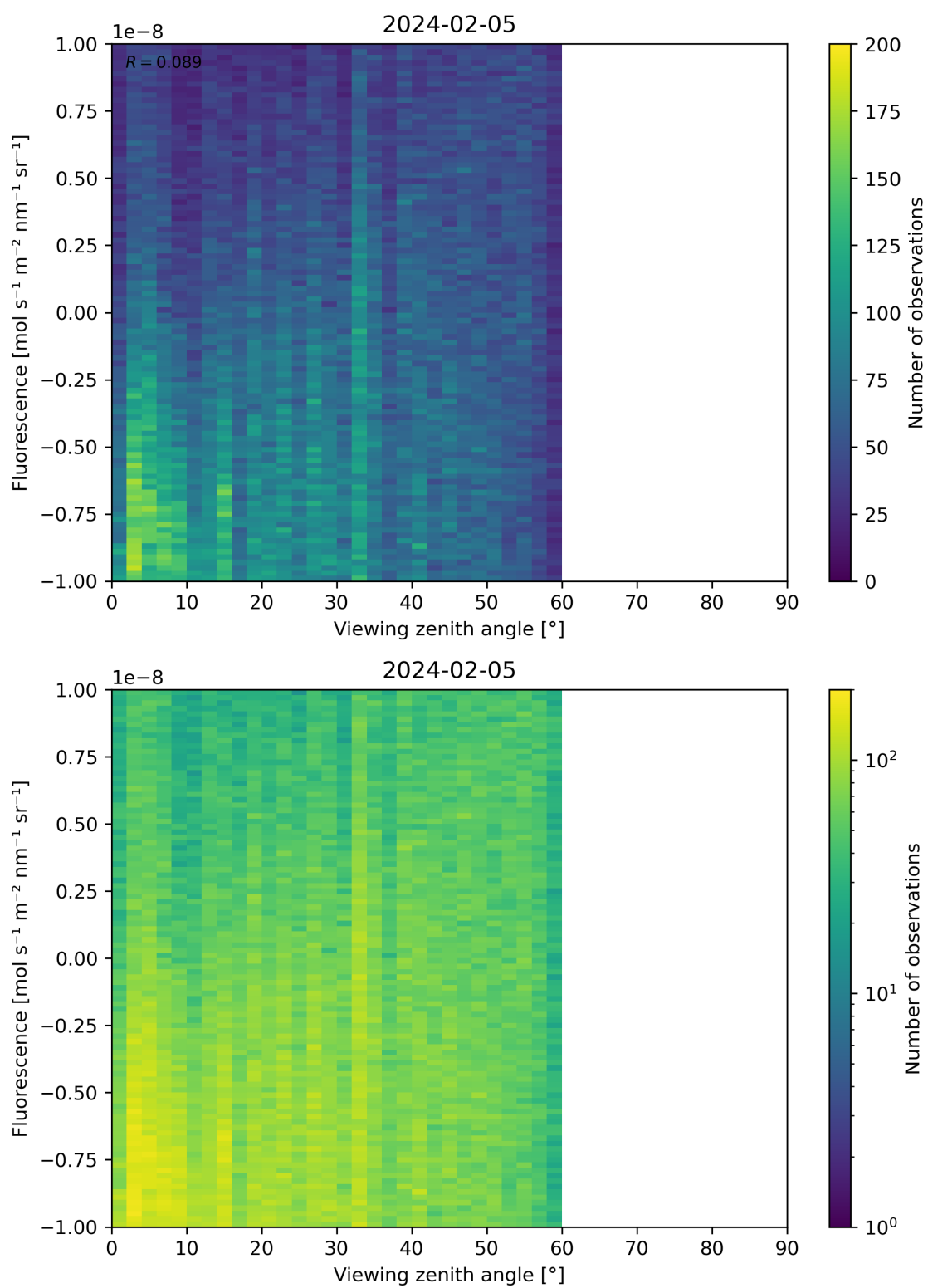
Figure 108: Scatter density plot of “Viewing zenith angle” against “Fluorescence” for 2024-02-04 to 2024-02-06.
