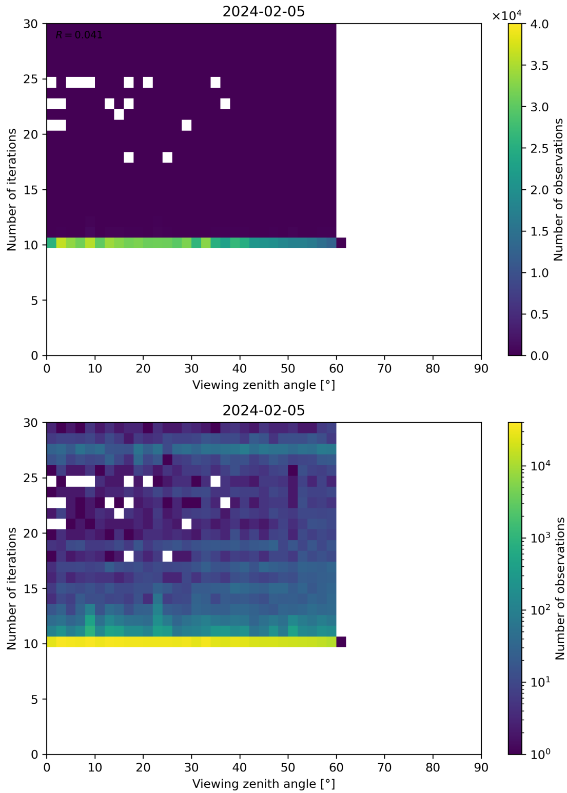
Figure 113: Scatter density plot of “Viewing zenith angle” against “Number of iterations” for 2024-02-04 to 2024-02-06.
