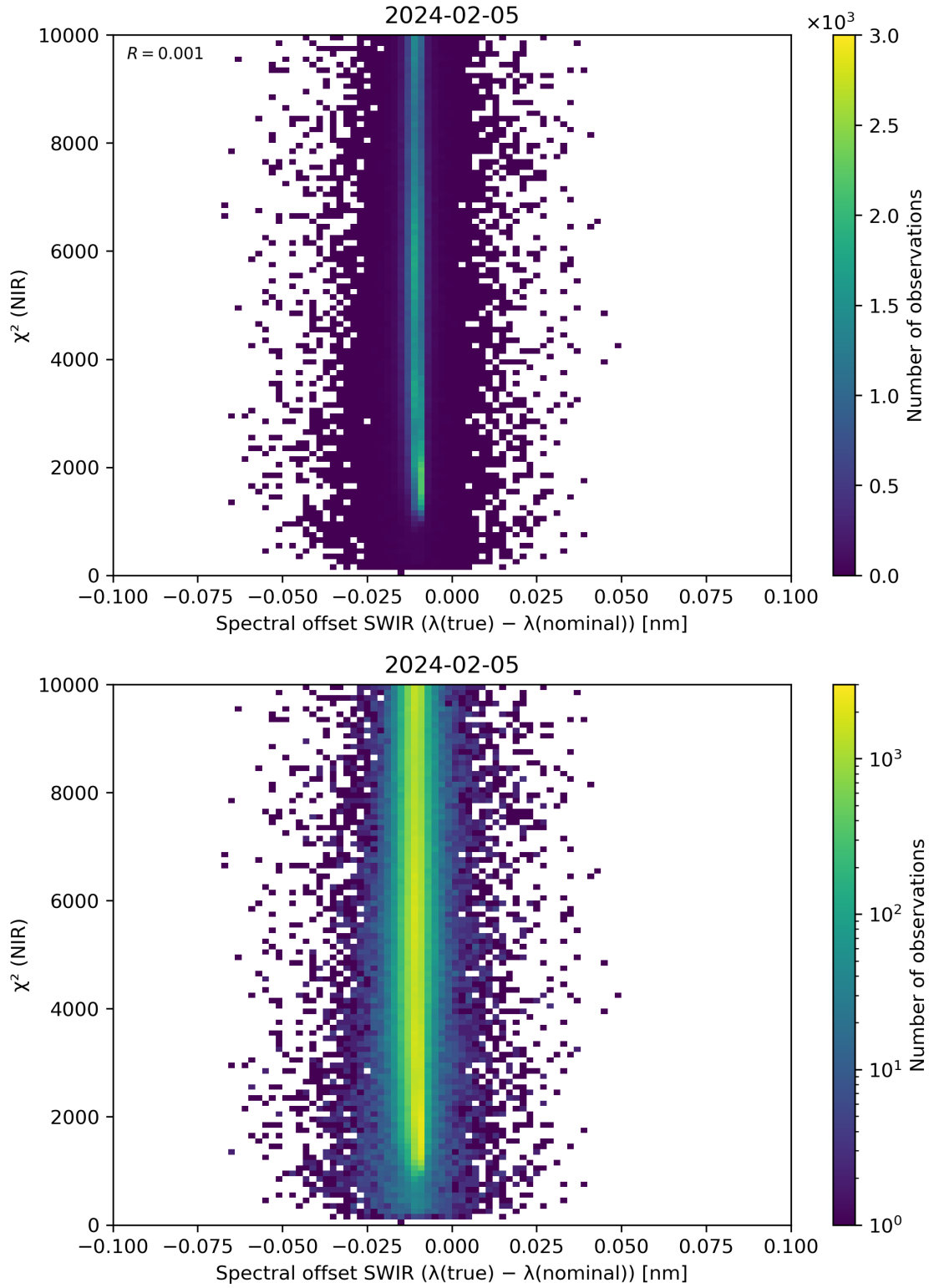
Figure 117: Scatter density plot of “Spectral offset SWIR ( \lambda(\text{true}) - \lambda(\text{nominal}) )” against “ \chi^2 (NIR)” for 2024-02-04 to 2024-02-06.
