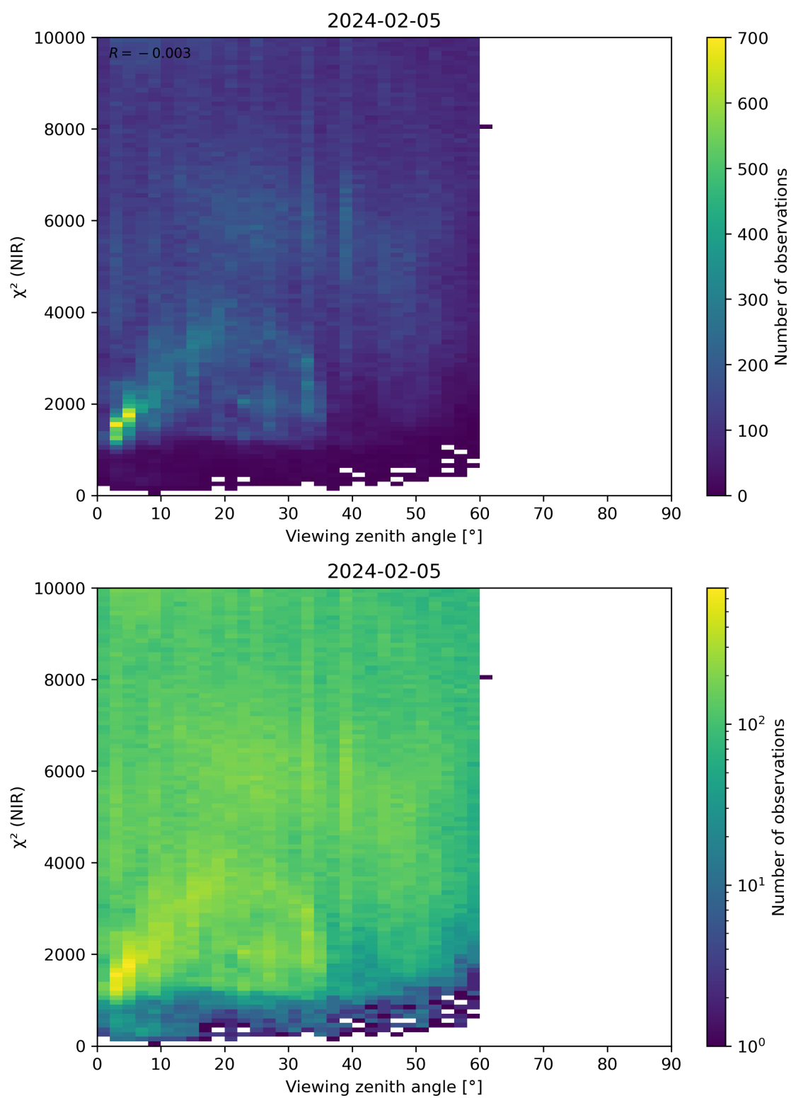
Figure 105: Scatter density plot of “Viewing zenith angle” against “ \chi^2 (NIR)” for 2024-02-04 to 2024-02-06.
