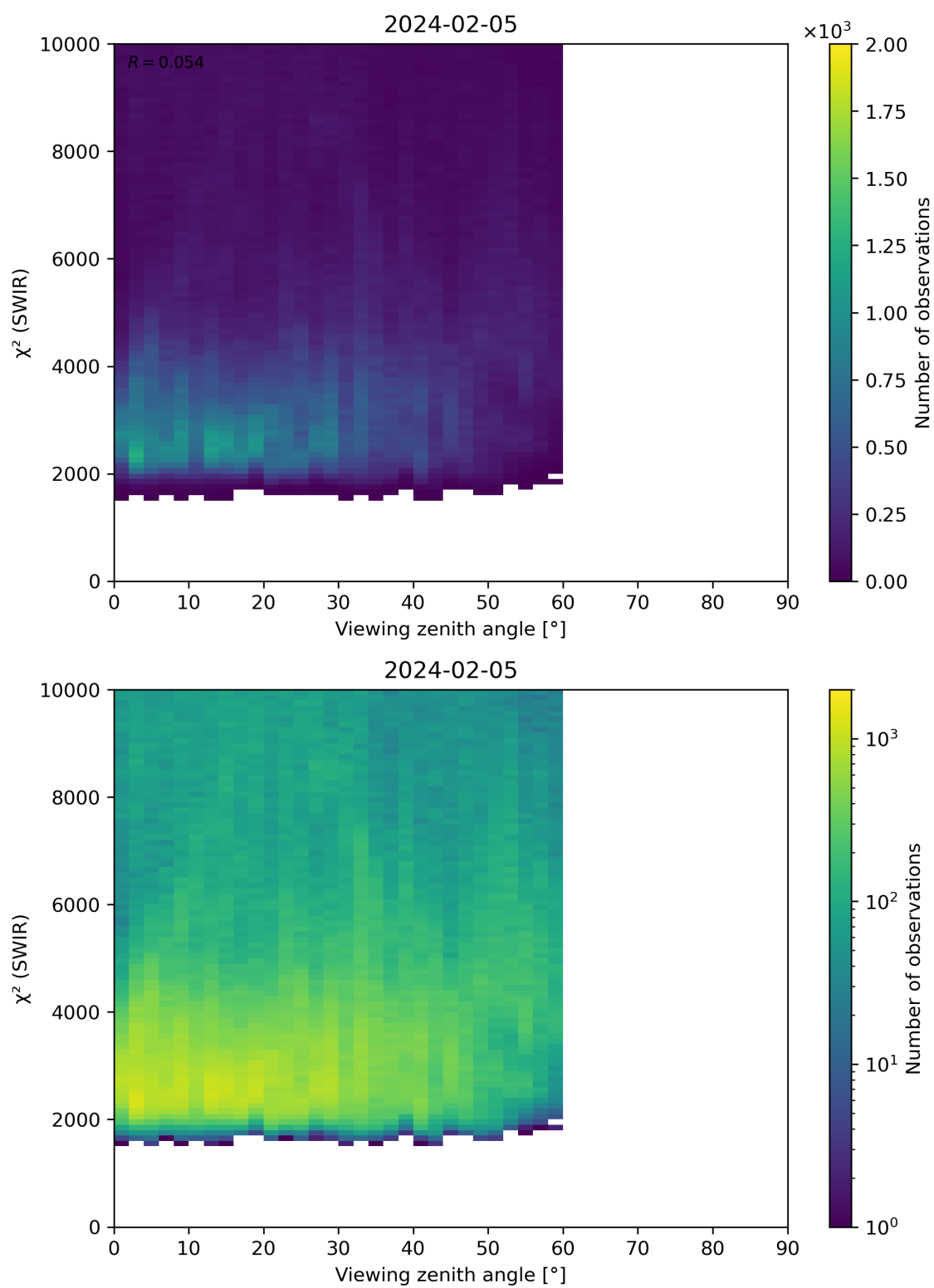
Figure 106: Scatter density plot of “Viewing zenith angle” against “ \chi^2 (SWIR)” for 2024-02-04 to 2024-02-06.
