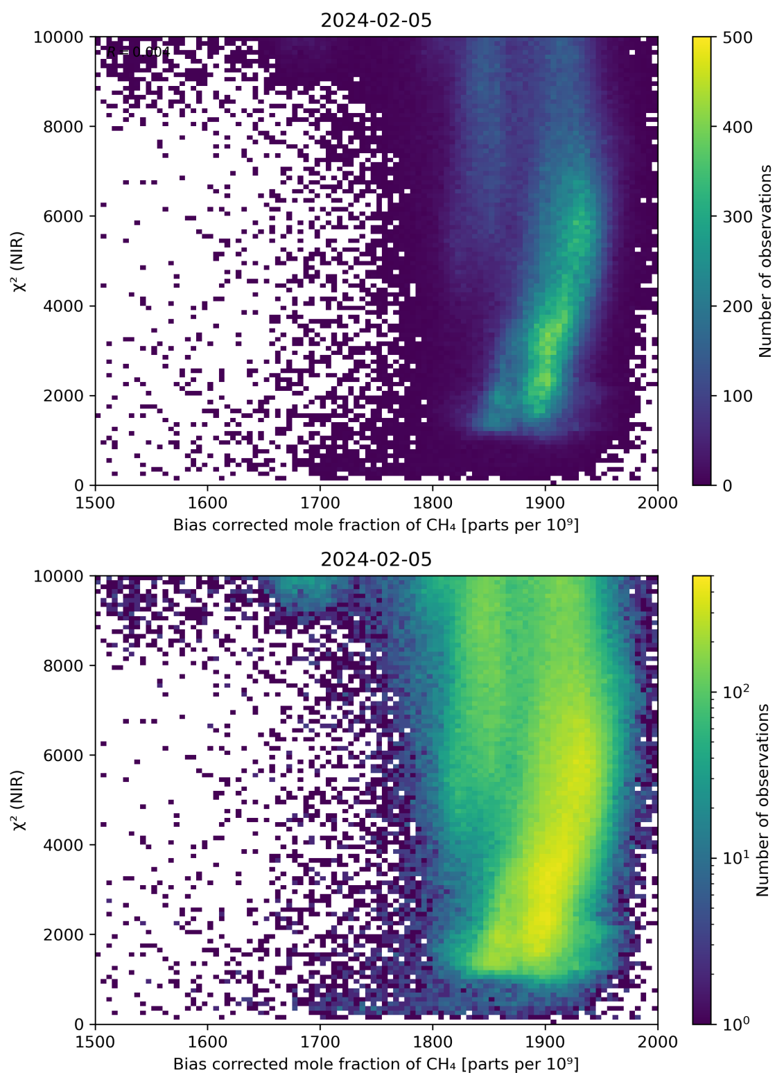
Figure 63: Scatter density plot of “Bias corrected mole fraction of CH 4 ” against “ \chi^2 (NIR)” for 2024-02-04 to 2024-02-06.
