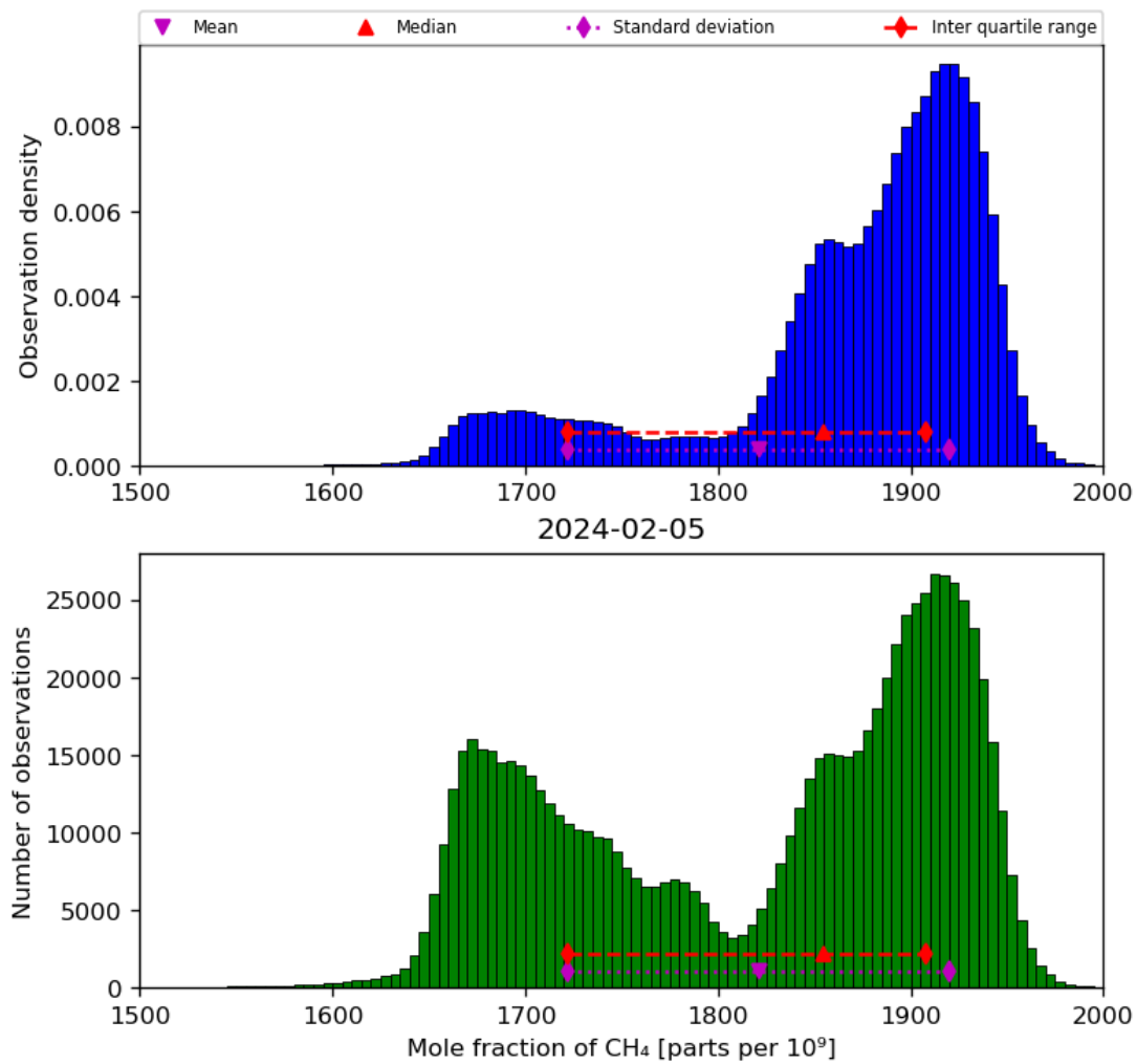
Figure 23: Histogram of “Mole fraction of CH 4 ” for 2024-02-04 to 2024-02-06
