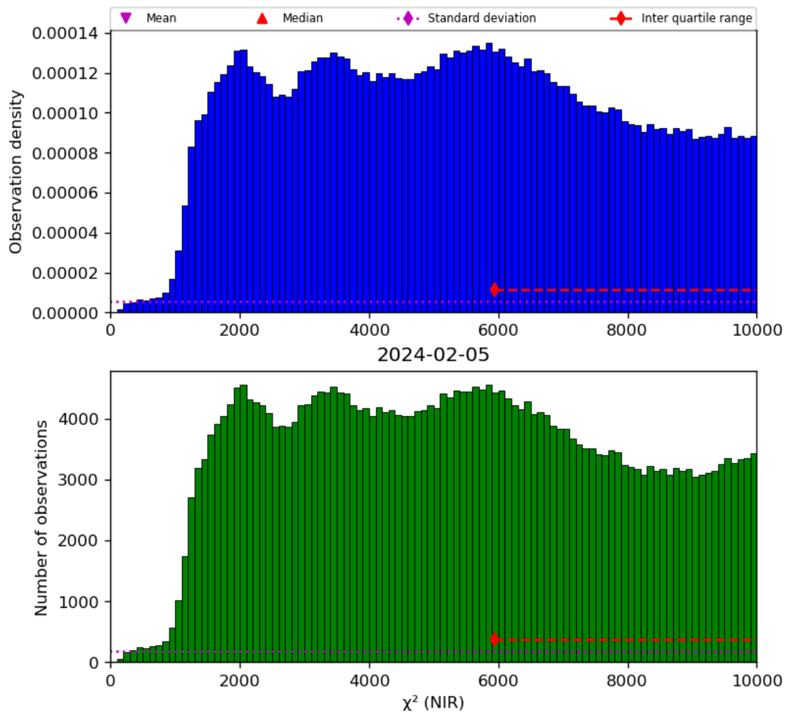
Figure 29: Histogram of " \chi^2 (NIR)" for 2024-02-04 to 2024-02-06
