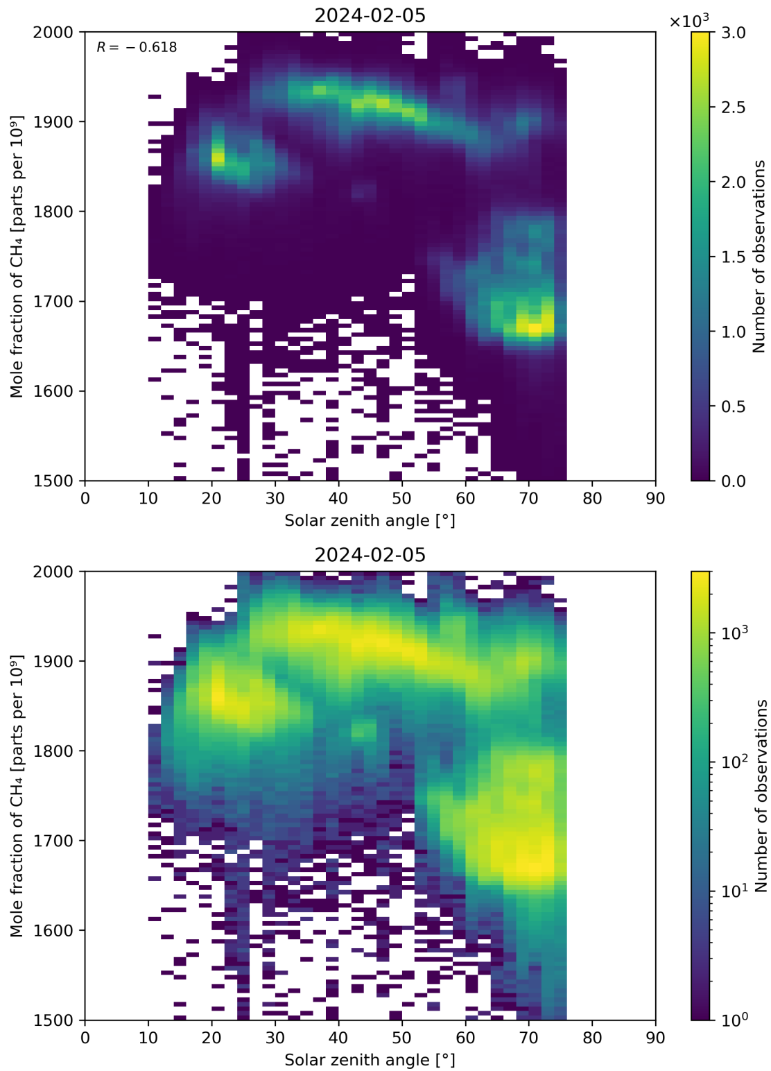
Figure 99: Scatter density plot of “Solar zenith angle” against “Mole fraction of CH 4 ” for 2024-02-04 to 2024-02-06.
