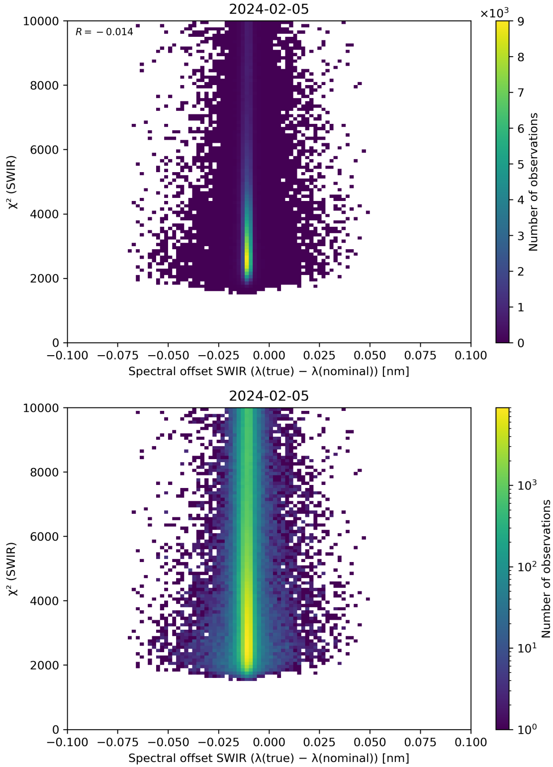
Figure 118: Scatter density plot of “Spectral offset SWIR ( \lambda(\text{true}) - \lambda(\text{nominal}) )” against “ \chi^2 (SWIR)” for 2024-02-04 to 2024-02-06.
