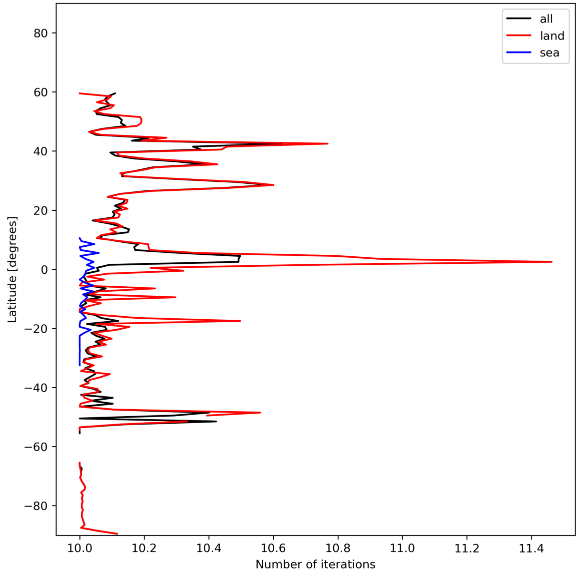
Figure 20: Zonal average of “Number of iterations” for 2024-02-04 to 2024-02-06.
