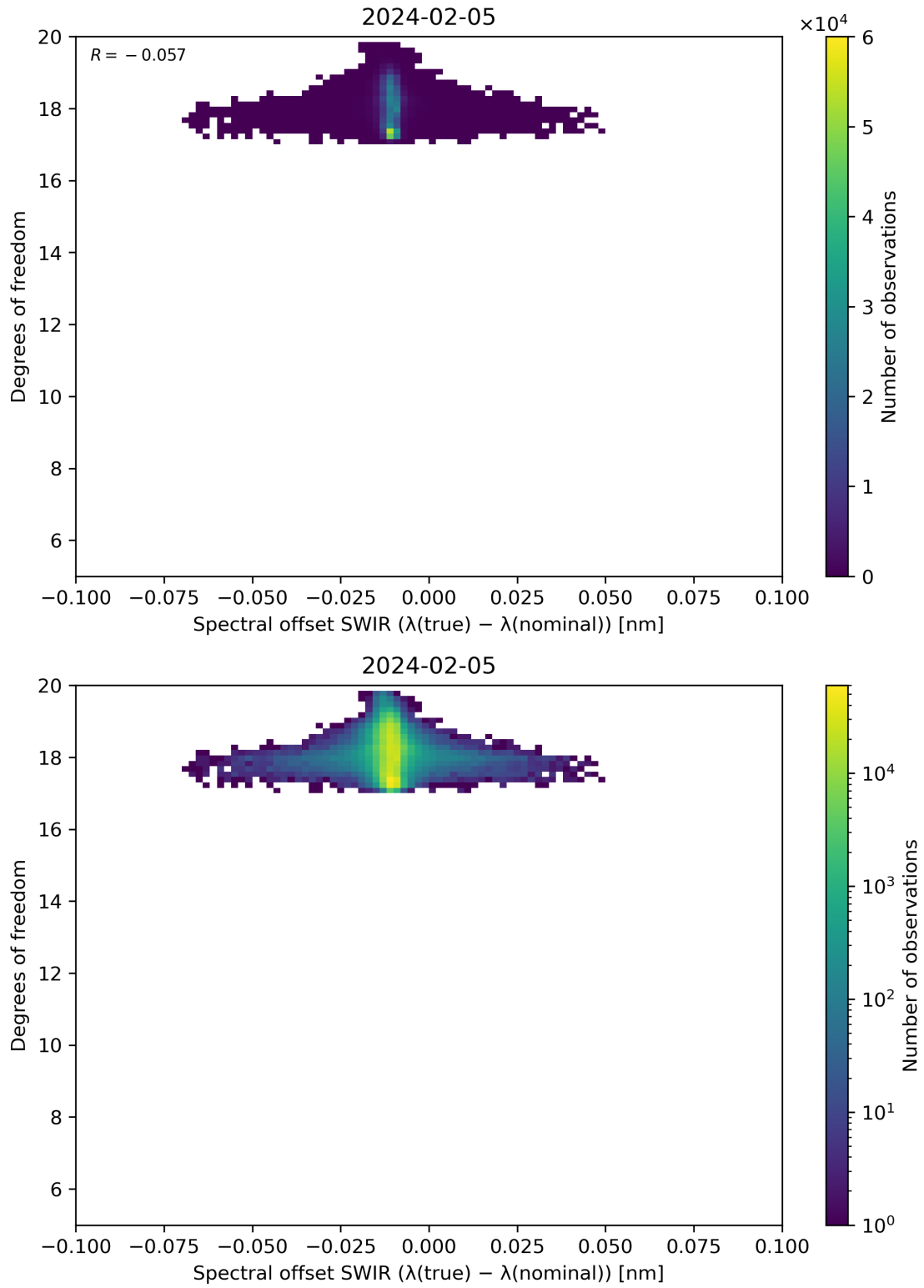
Figure 119: Scatter density plot of “Spectral offset SWIR ( \lambda(\text{true}) - \lambda(\text{nominal}) )” against “Degrees of freedom” for 2024-02-04 to 2024-02-06.
