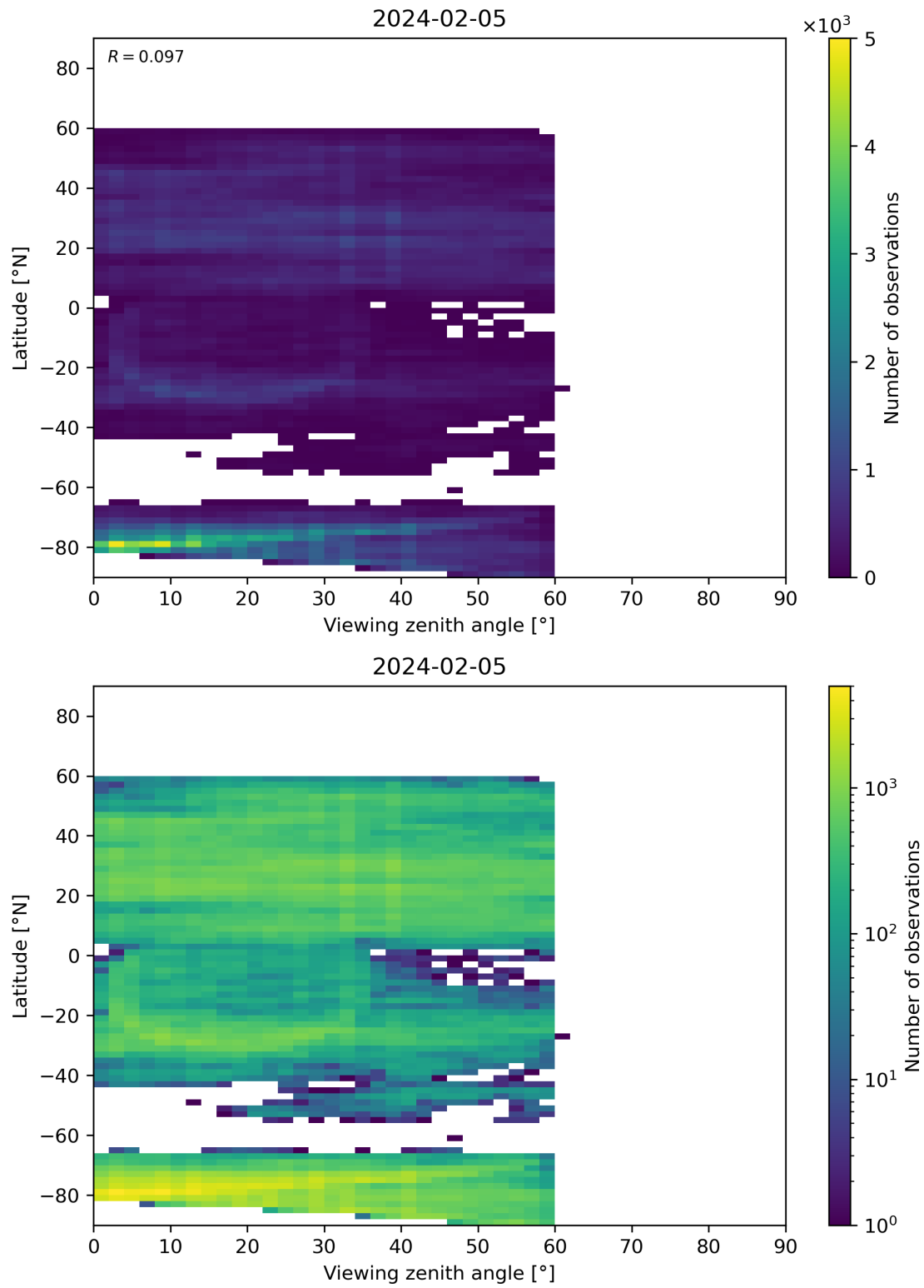
Figure 109: Scatter density plot of “Viewing zenith angle” against “Latitude” for 2024-02-04 to 2024-02-06.
