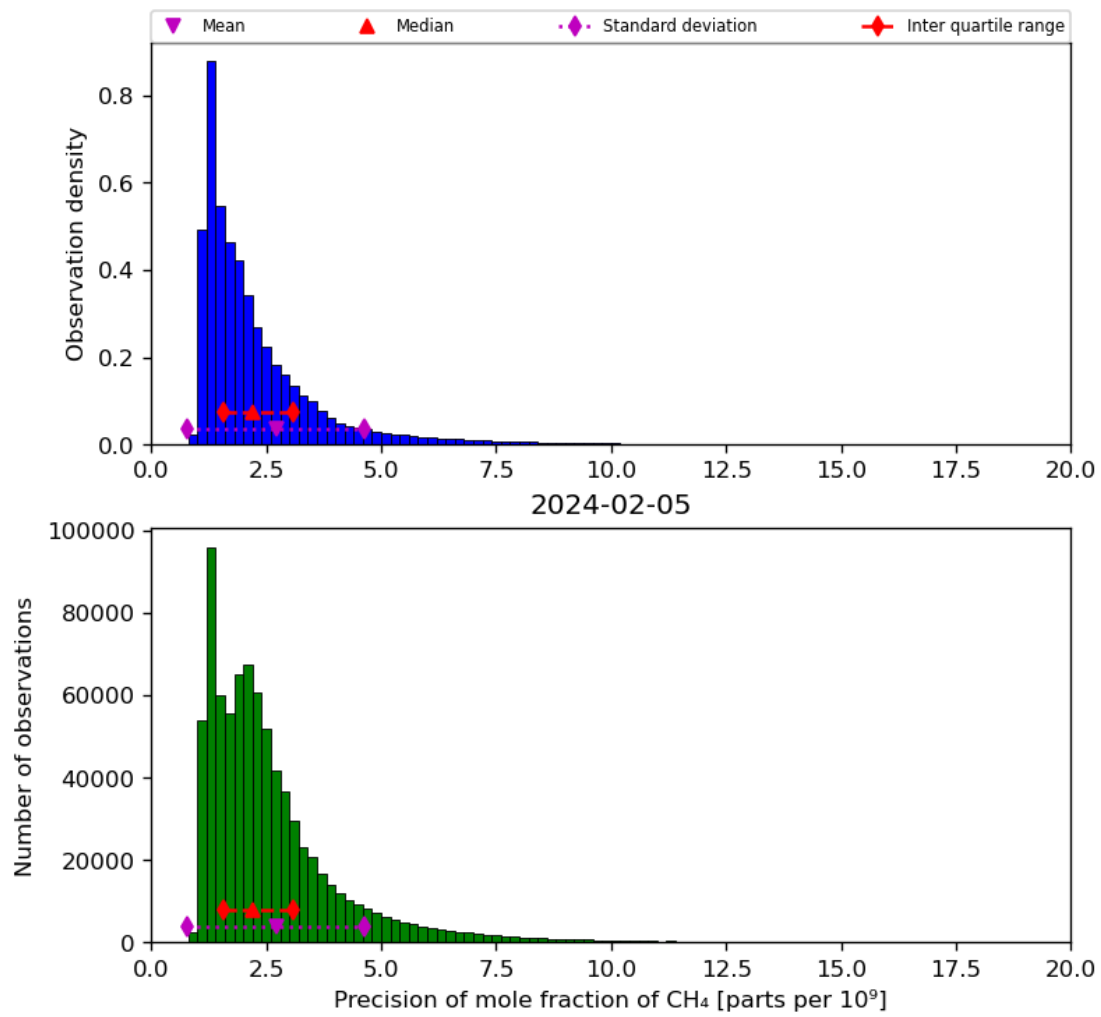
Figure 24: Histogram of “Precision of mole fraction of CH 4 ” for 2024-02-04 to 2024-02-06
