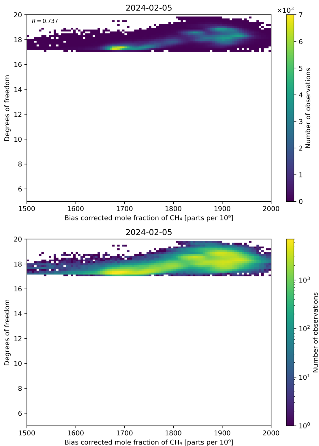
Figure 65: Scatter density plot of “Bias corrected mole fraction of CH 4 ” against “Degrees of freedom” for 2024-02-04 to 2024-02-06.
