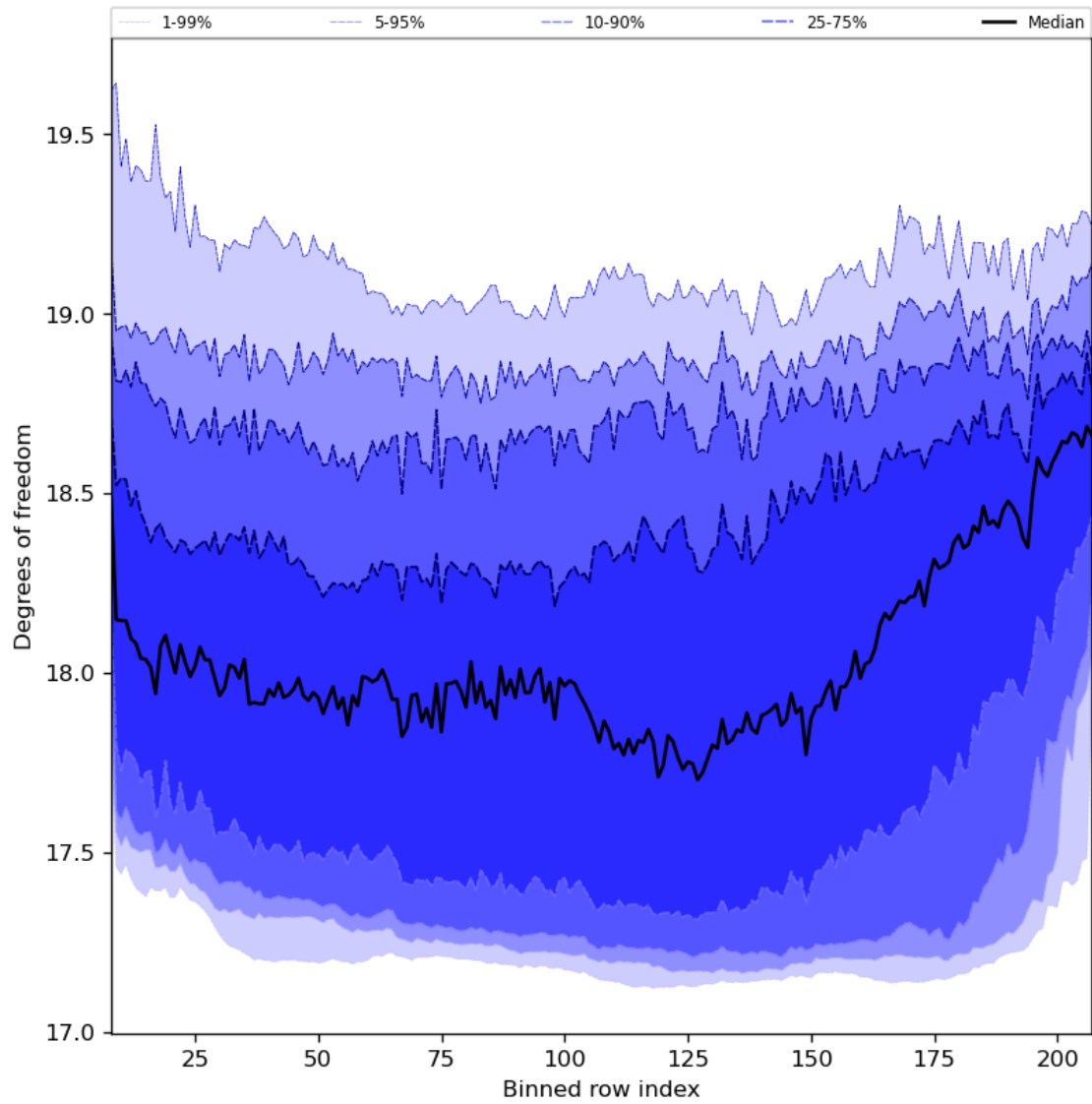
Figure 41: Along track statistics of “Degrees of freedom” for 2024-02-04 to 2024-02-06
