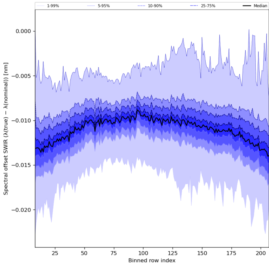
Figure 38: Along track statistics of “Spectral offset SWIR ( \lambda(\text{true}) - \lambda(\text{nominal}) )” for 2024-02-04 to 2024-02-06
