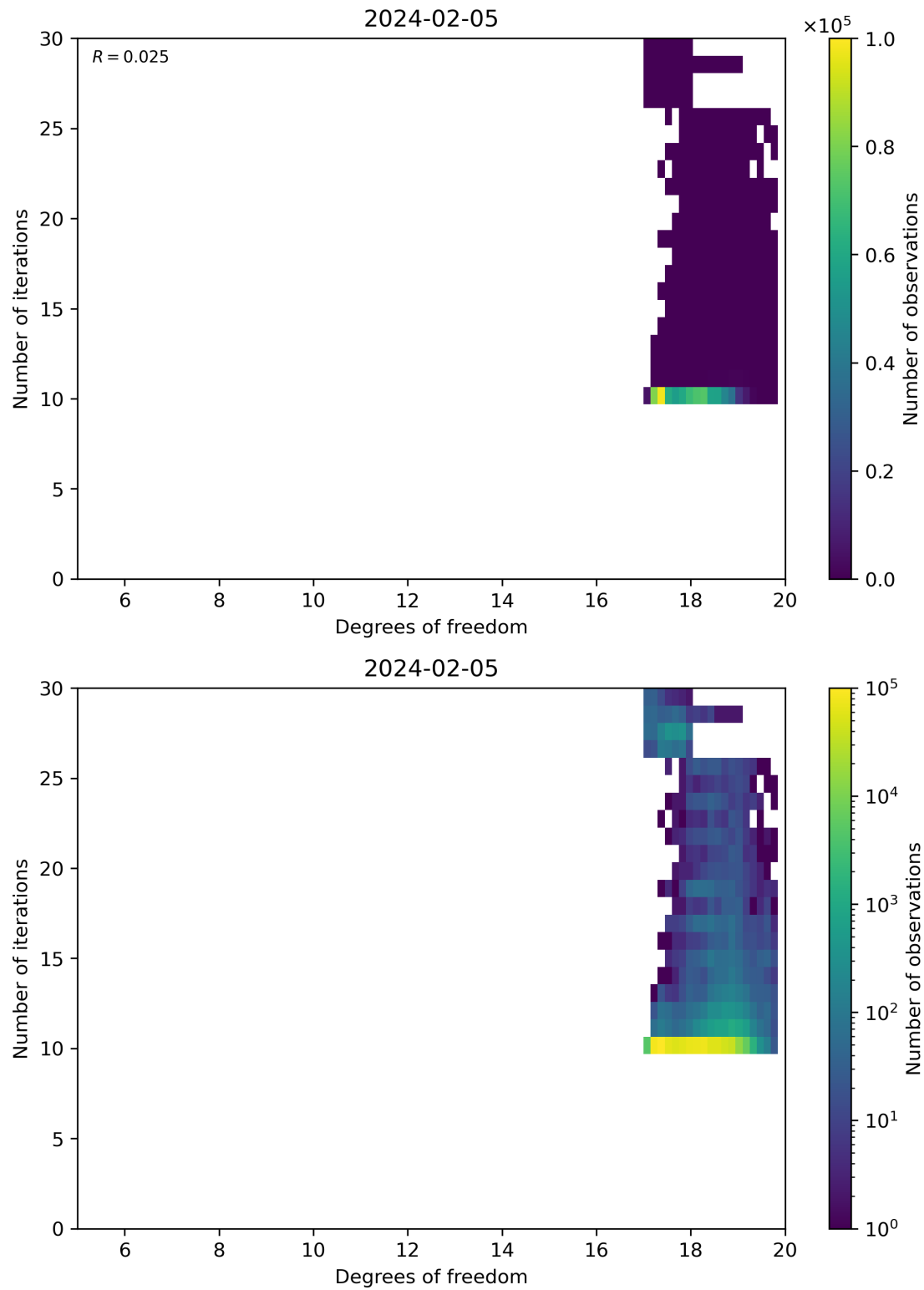
Figure 52: Scatter density plot of “Degrees of freedom” against “Number of iterations” for 2024-02-04 to 2024-02-06.
