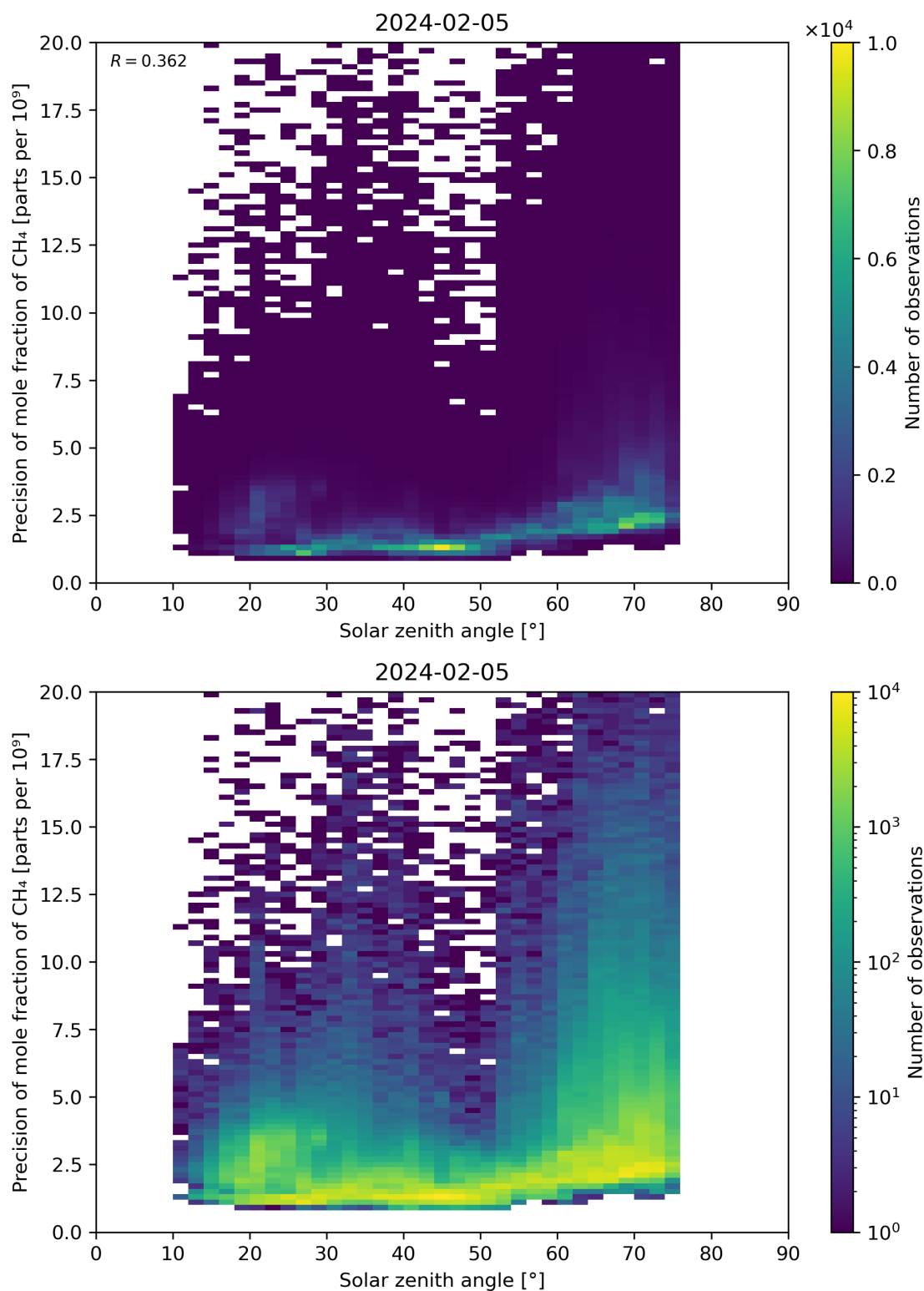
Figure 101: Scatter density plot of “Solar zenith angle” against “Precision of mole fraction of CH 4 ” for 2024-02-04 to 2024-02-06.
