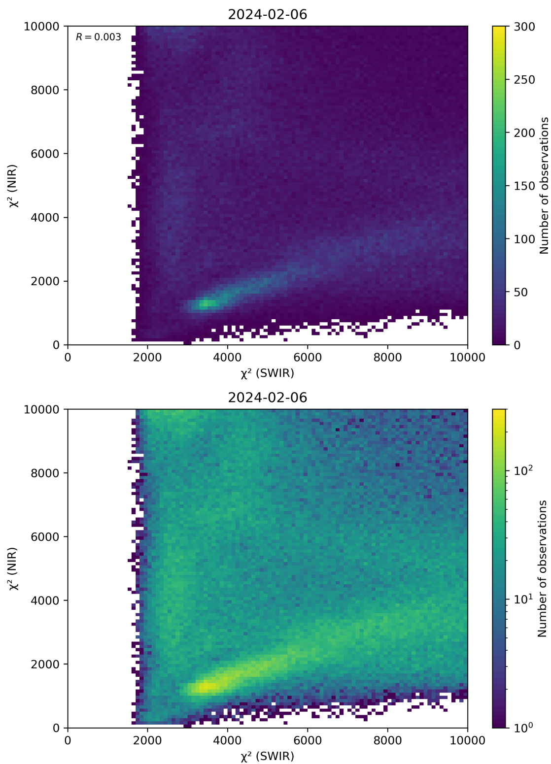
Figure 47: Scatter density plot of “ \chi^2 (SWIR)” against “ \chi^2 (NIR)” for 2024-02-06 to 2024-02-07.
