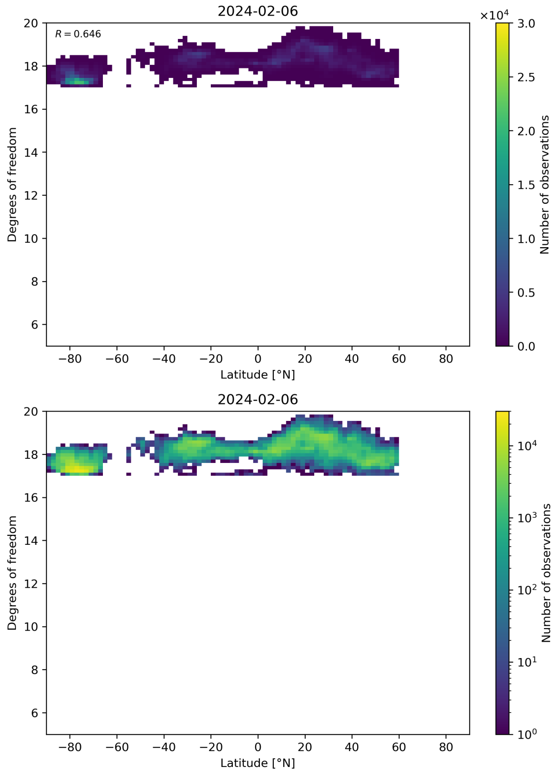
Figure 55: Scatter density plot of “Latitude” against “Degrees of freedom” for 2024-02-06 to 2024-02-07.
