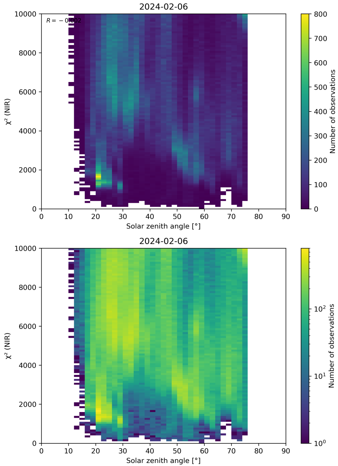
Figure 94: Scatter density plot of “Solar zenith angle” against “ \chi^2 (NIR)” for 2024-02-06 to 2024-02-07.
