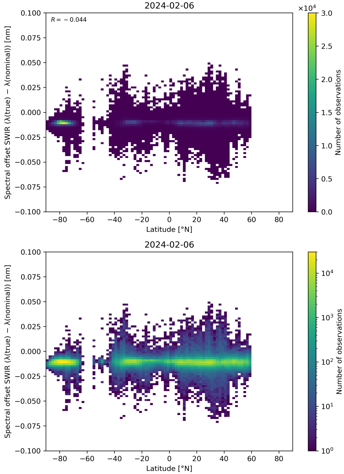
Figure 62: Scatter density plot of “Latitude” against “Spectral offset SWIR ( \lambda(\text{true}) - \lambda(\text{nominal}) )” for 2024-02-06 to 2024-02-07.
