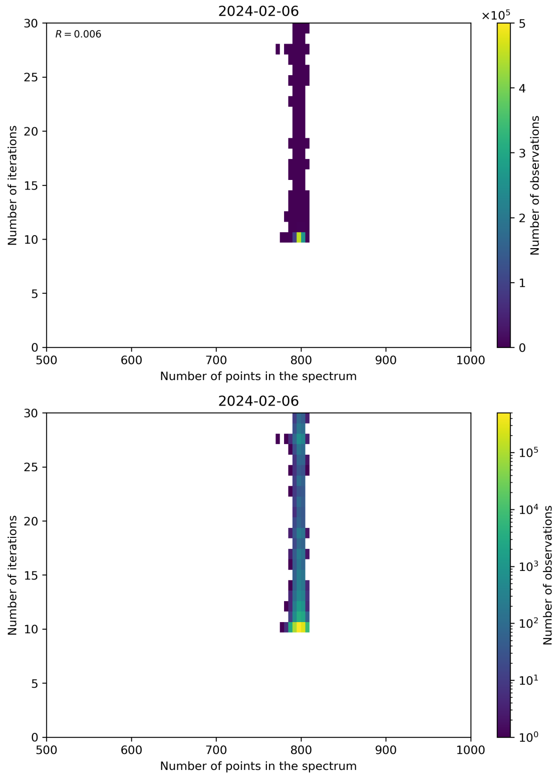
Figure 92: Scatter density plot of “Number of points in the spectrum” against “Number of iterations” for 2024-02-06 to 2024-02-07.
