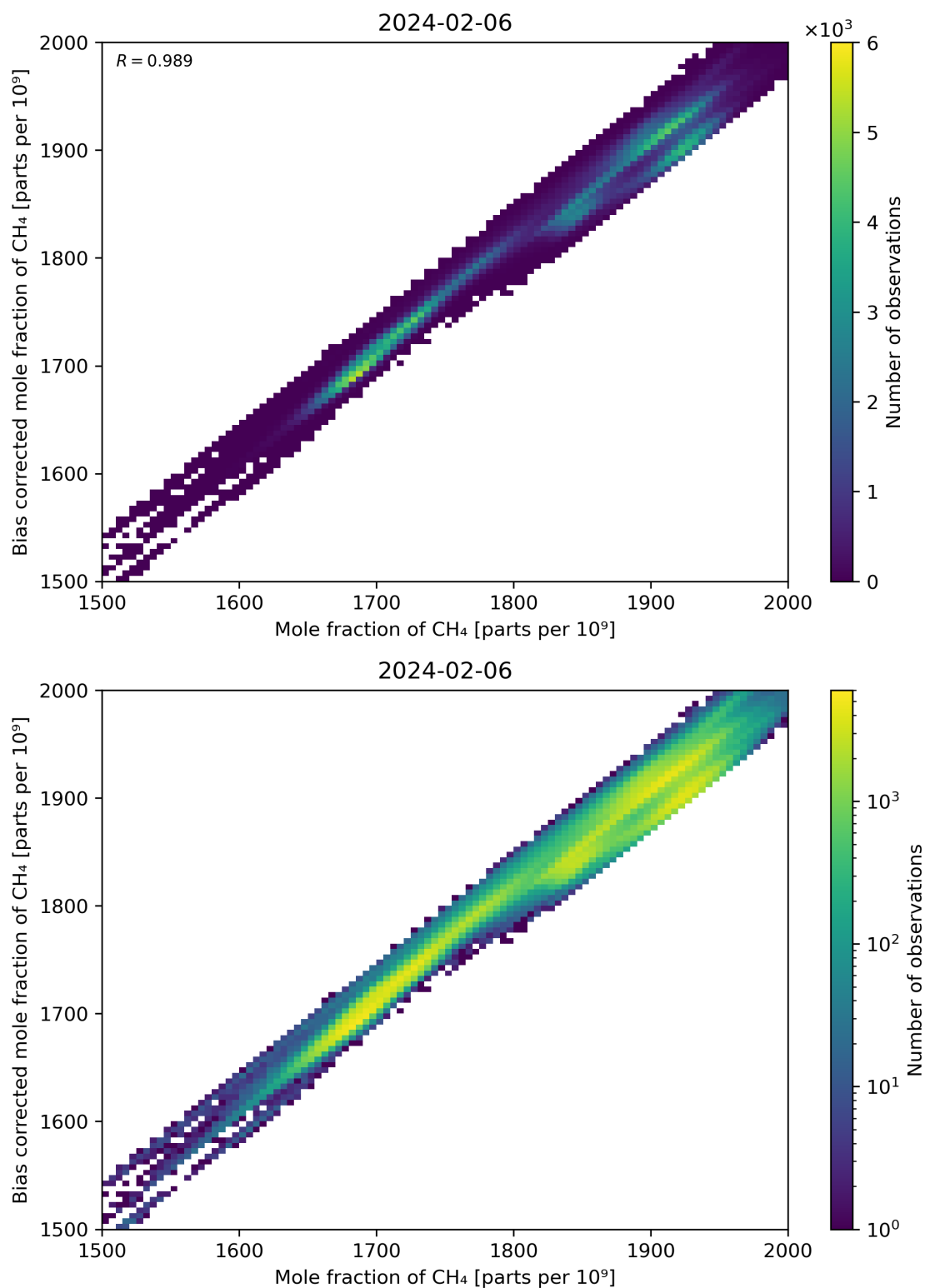
Figure 74: Scatter density plot of “Mole fraction of CH 4 ” against “Bias corrected mole fraction of CH 4 ” for 2024-02-06 to 2024-02-07.
