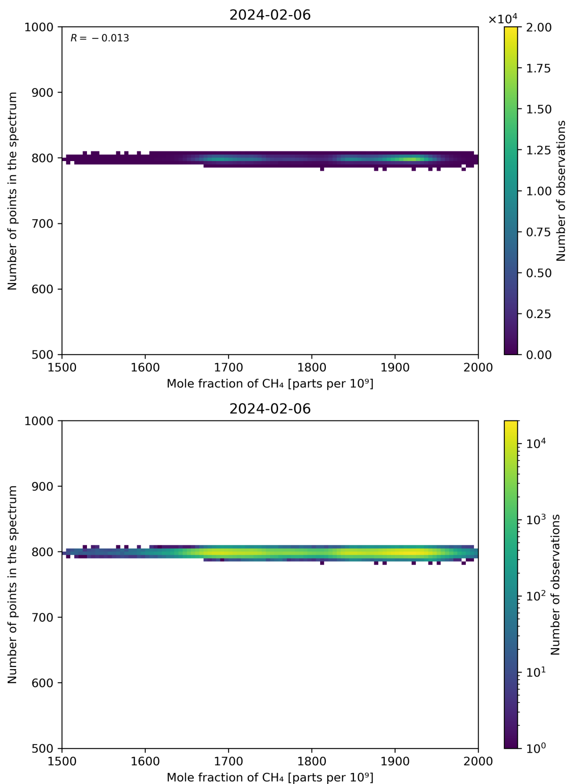
Figure 77: Scatter density plot of “Mole fraction of CH 4 ” against “Number of points in the spectrum” for 2024-02-06 to 2024-02-07.
