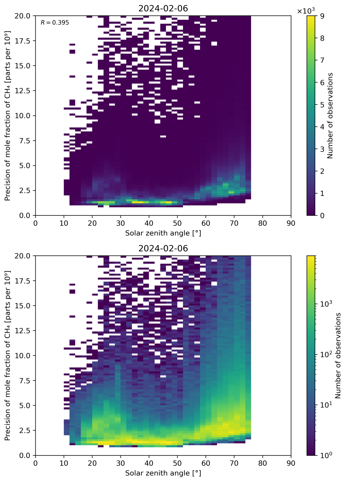
Figure 101: Scatter density plot of “Solar zenith angle” against “Precision of mole fraction of CH 4 ” for 2024-02-06 to 2024-02-07.
