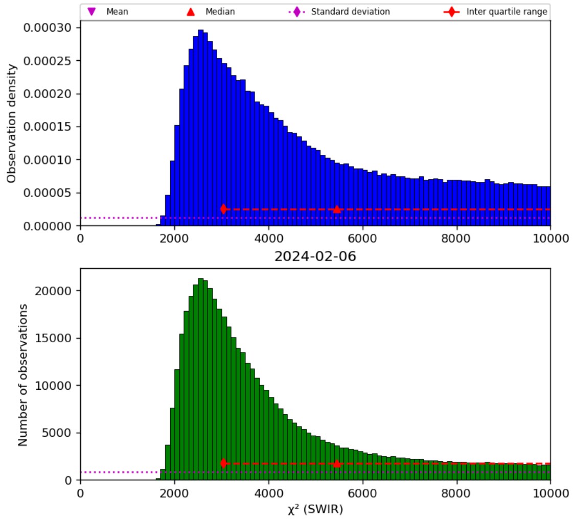
Figure 28: Histogram of “ \chi^2 (SWIR)” for 2024-02-06 to 2024-02-07
