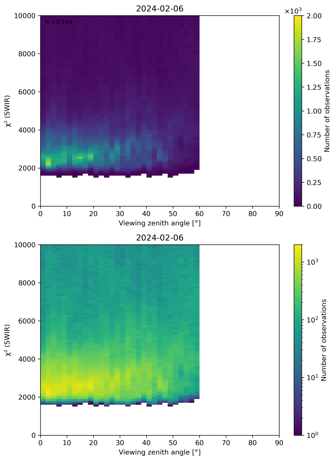
Figure 106: Scatter density plot of “Viewing zenith angle” against “ \chi^2 (SWIR)” for 2024-02-06 to 2024-02-07.
