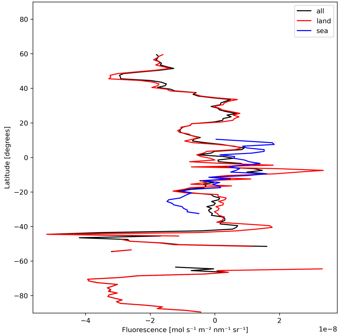
Figure 21: Zonal average of “Fluorescence” for 2024-02-06 to 2024-02-07.
