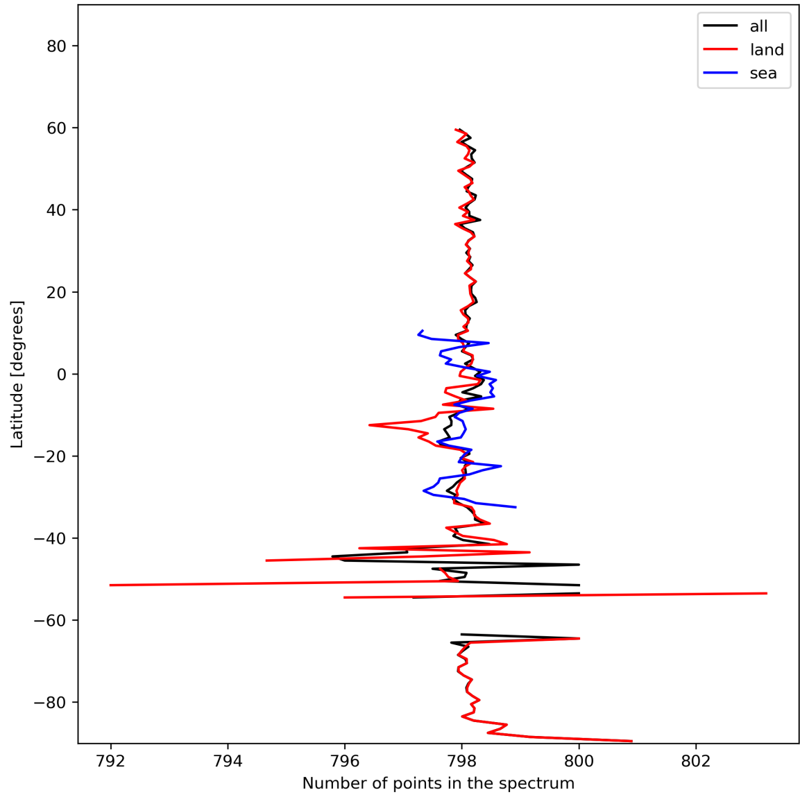
Figure 15: Zonal average of “Number of points in the spectrum” for 2024-02-06 to 2024-02-07.
