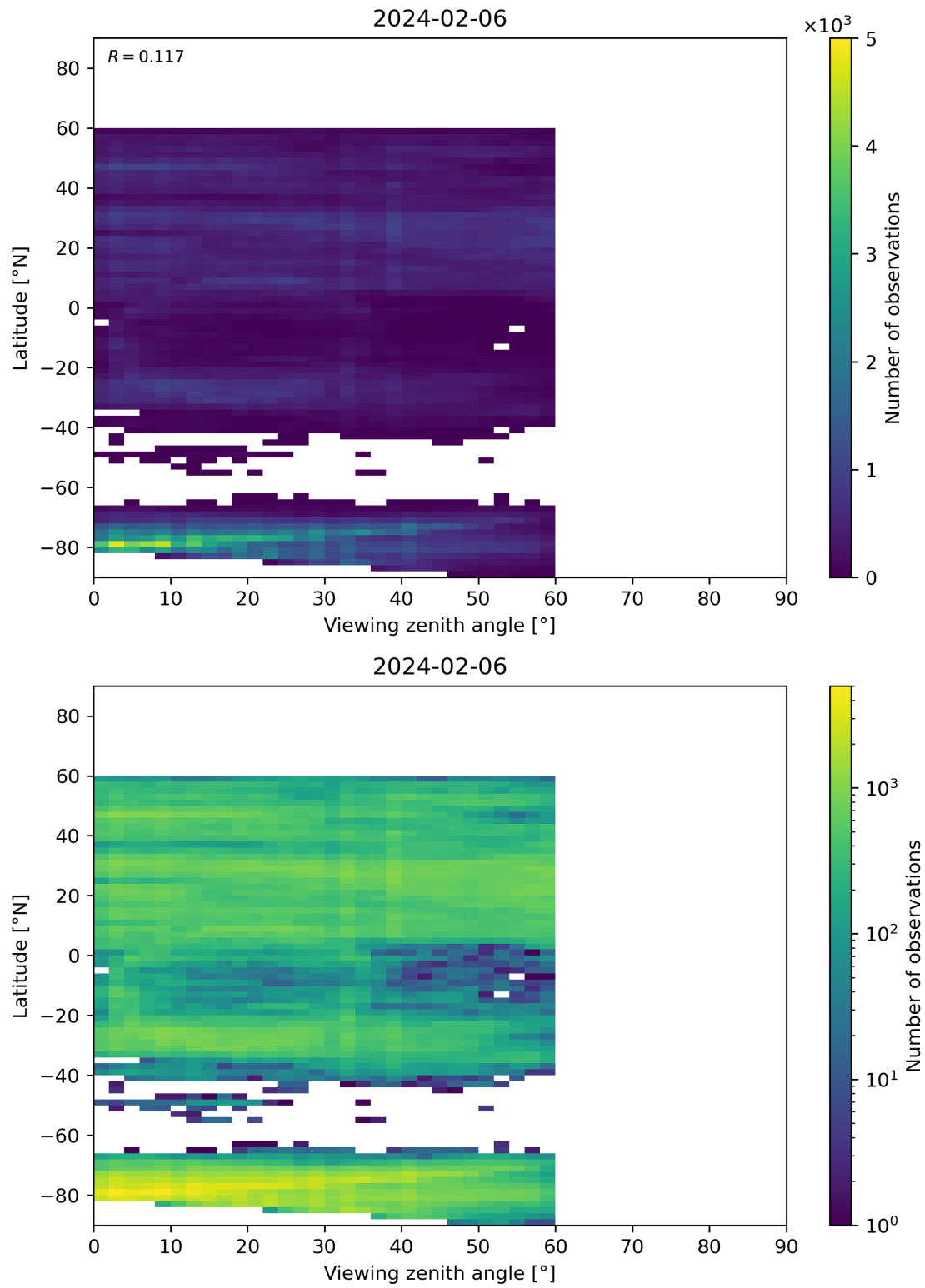
Figure 109: Scatter density plot of “Viewing zenith angle” against “Latitude” for 2024-02-06 to 2024-02-07.
