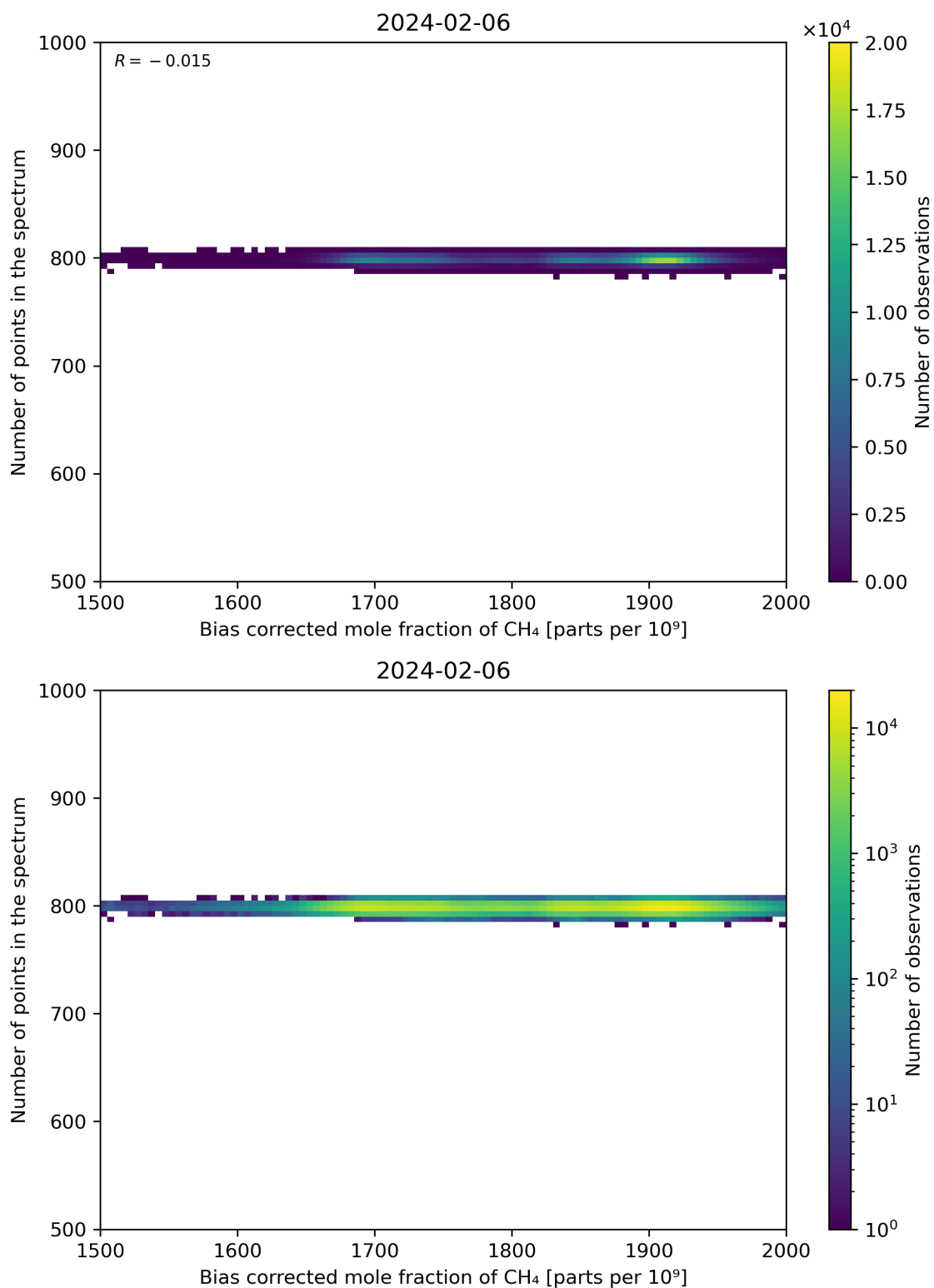
Figure 68: Scatter density plot of “Bias corrected mole fraction of CH 4 ” against “Number of points in the spectrum” for 2024-02-06 to 2024-02-07.
