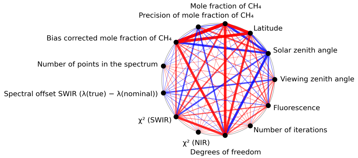
Figure 1: Map of correlation graph for 2024-02-06 to 2024-02-07.
