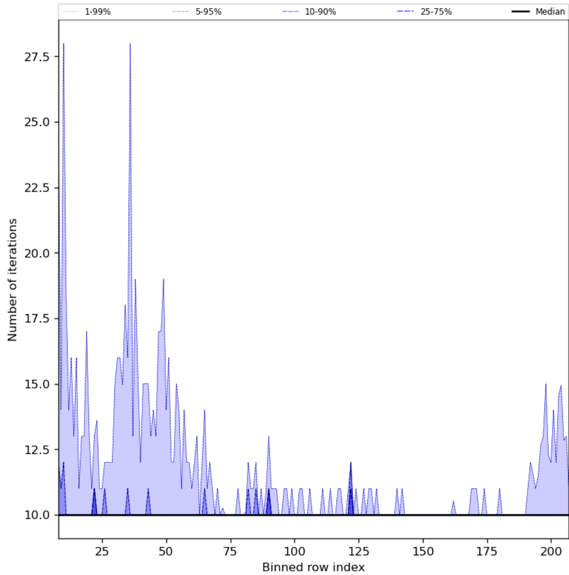
Figure 42: Along track statistics of “Number of iterations” for 2024-02-06 to 2024-02-07
