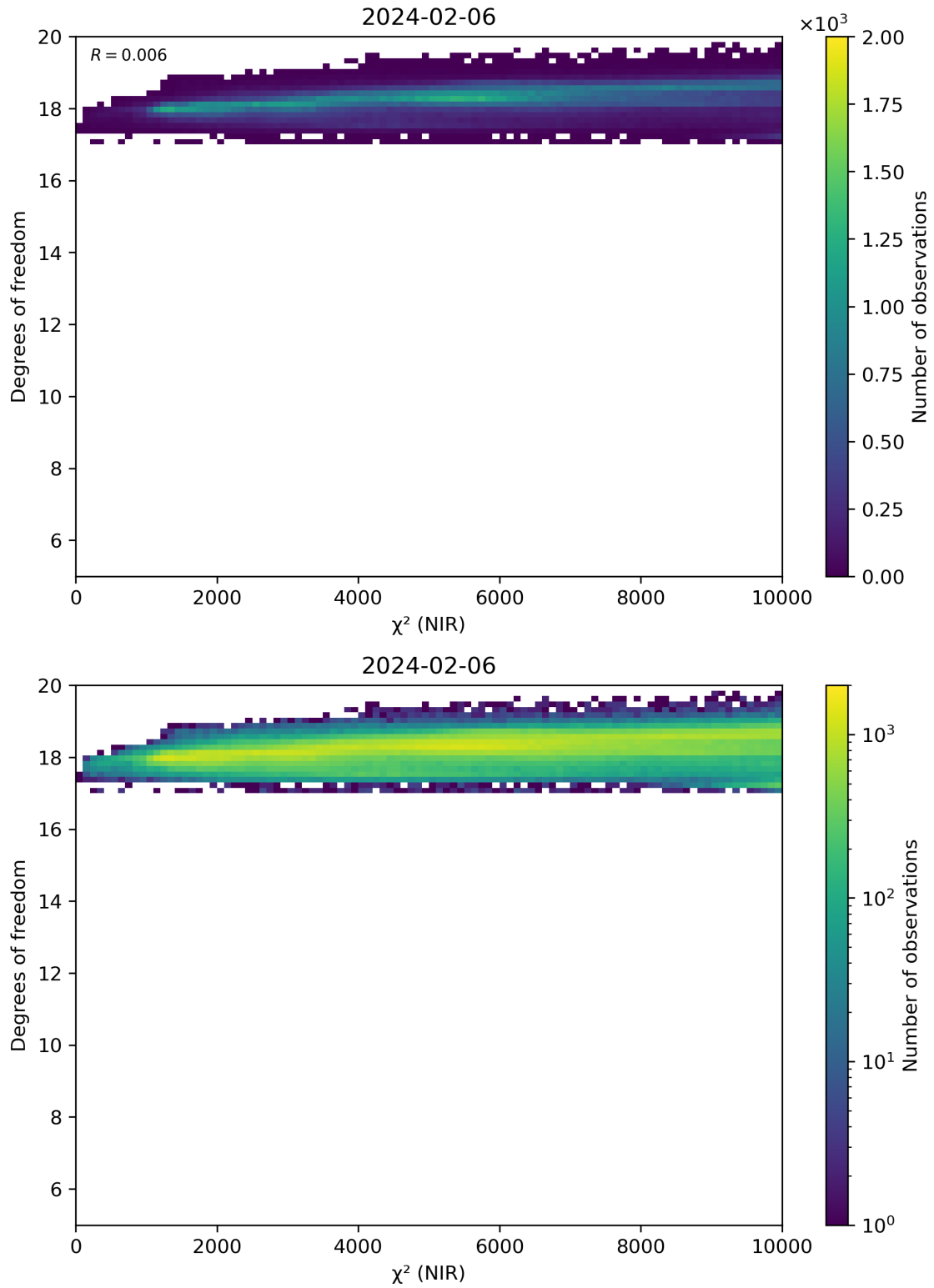
Figure 44: Scatter density plot of “ \chi^2 (NIR)” against “Degrees of freedom” for 2024-02-06 to 2024-02-07.
