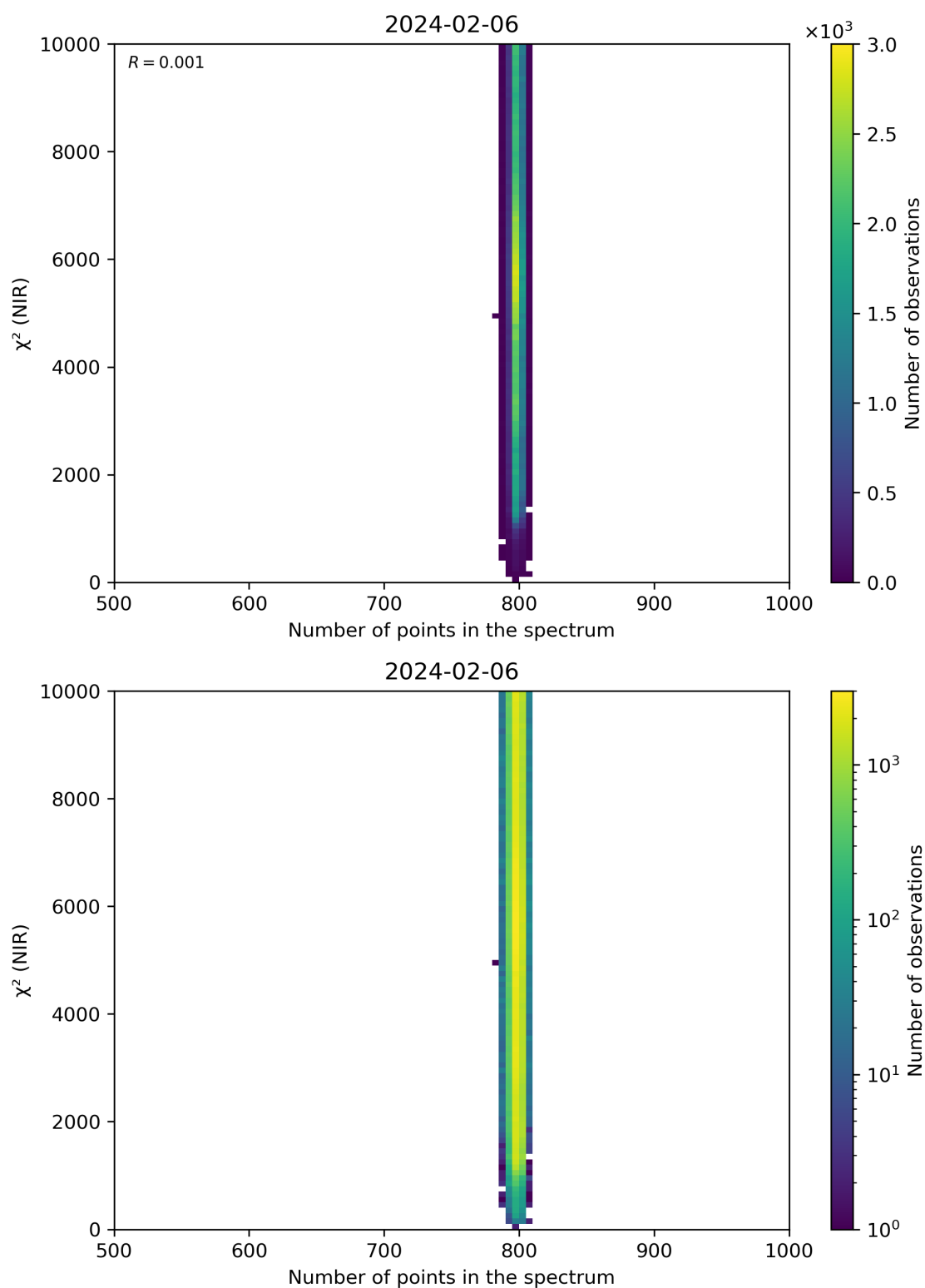
Figure 88: Scatter density plot of “Number of points in the spectrum” against “ \chi^2 (NIR)” for 2024-02-06 to 2024-02-07.
