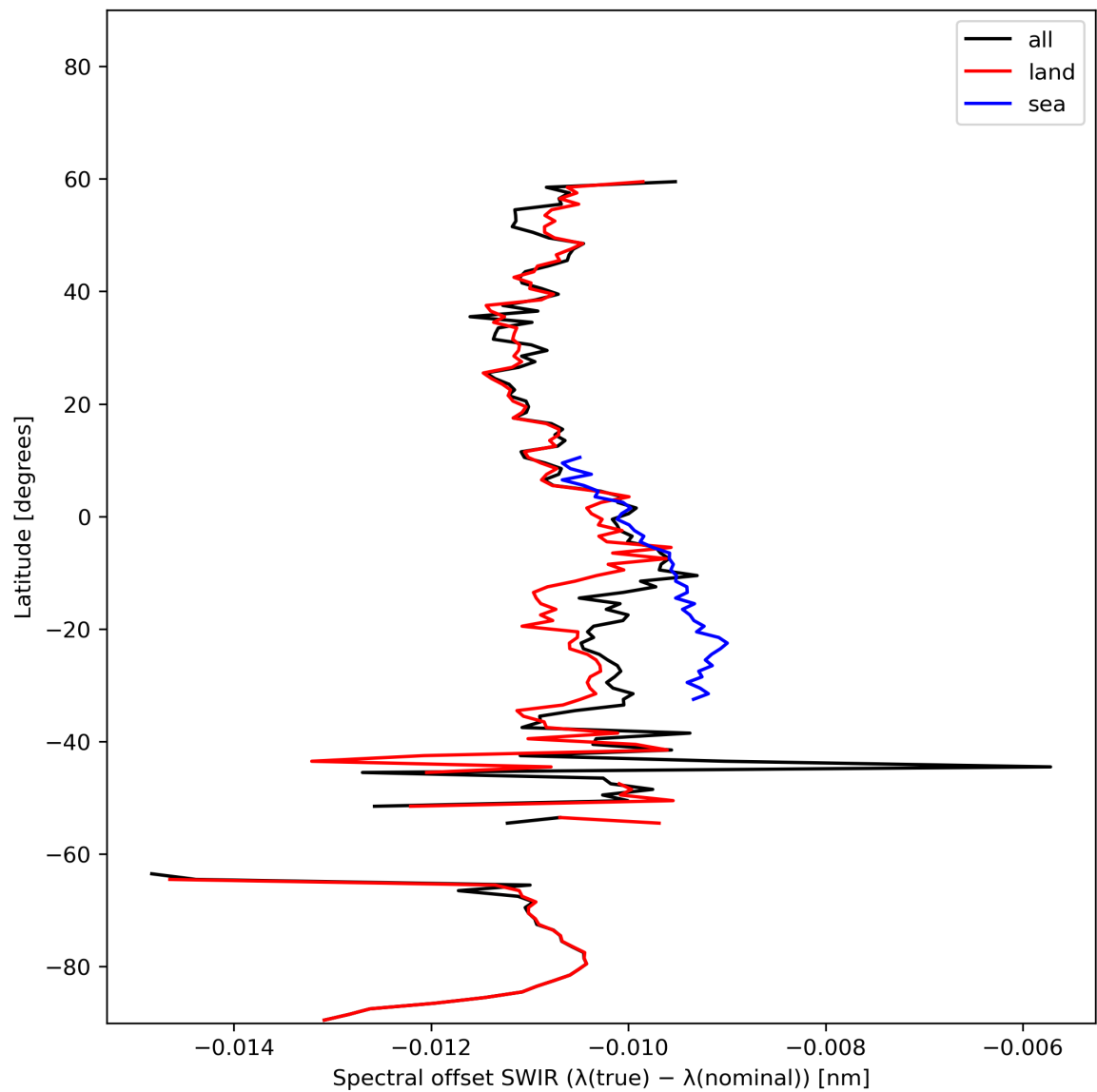
Figure 16: Zonal average of “Spectral offset SWIR ( \lambda(\text{true}) - \lambda(\text{nominal}) )” for 2024-02-06 to 2024-02-07.
