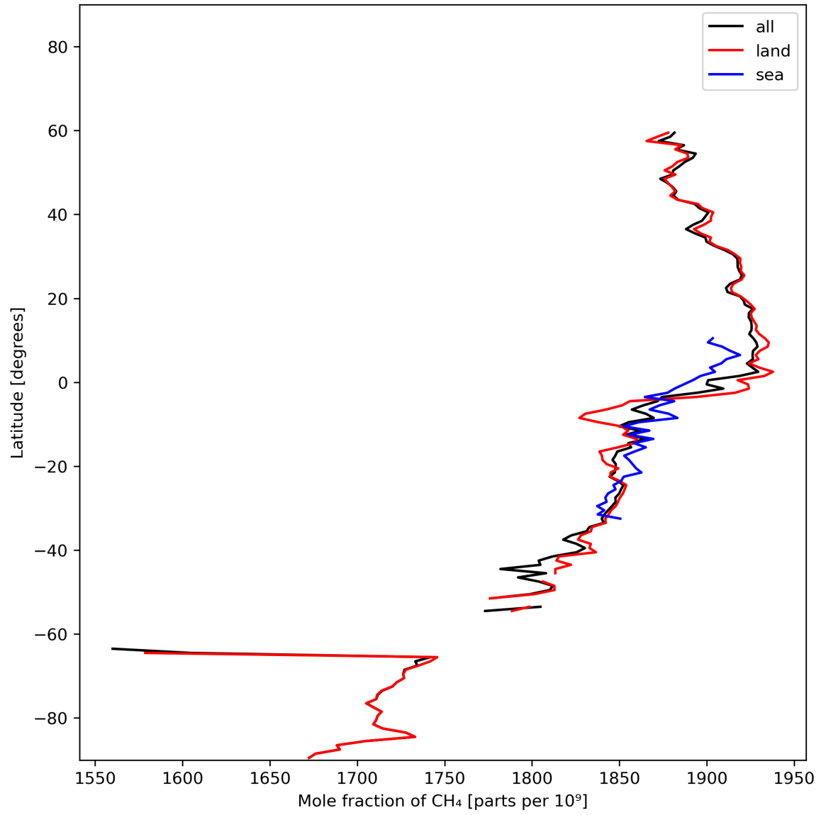
Figure 12: Zonal average of “Mole fraction of CH 4 ” for 2024-02-06 to 2024-02-07.
