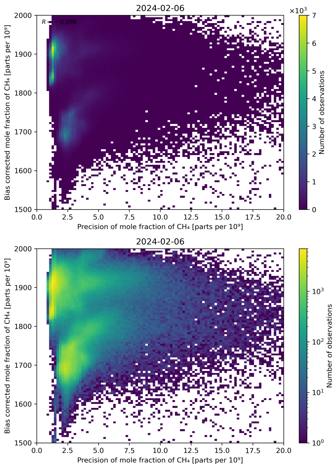
Figure 82: Scatter density plot of “Precision of mole fraction of CH 4 ” against “Bias corrected mole fraction of CH 4 ” for 2024-02-06 to 2024-02-07.
