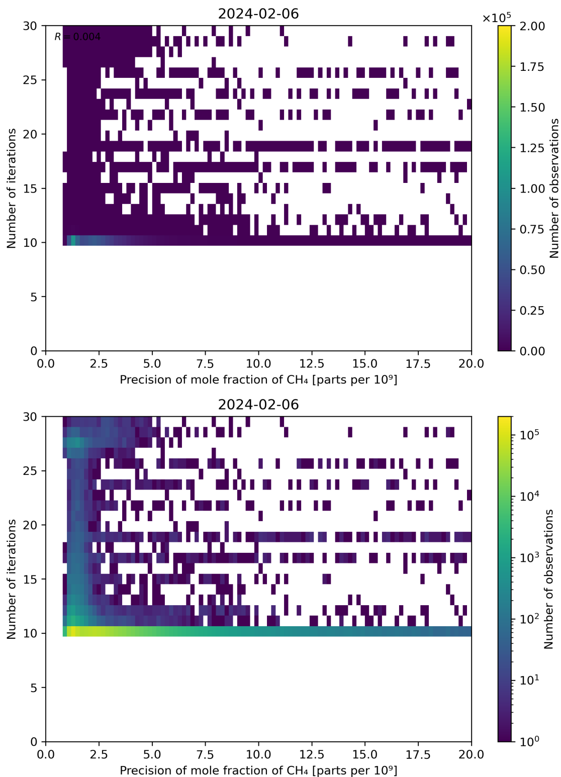
Figure 83: Scatter density plot of “Precision of mole fraction of CH 4 ” against “Number of iterations” for 2024-02-06 to 2024-02-07.
