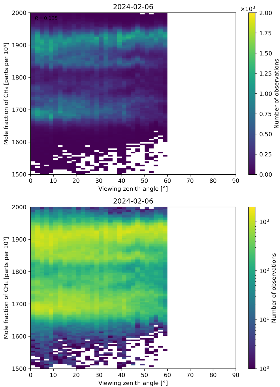
Figure 110: Scatter density plot of “Viewing zenith angle” against “Mole fraction of \text{CH}_4 ” for 2024-02-06 to 2024-02-07.
