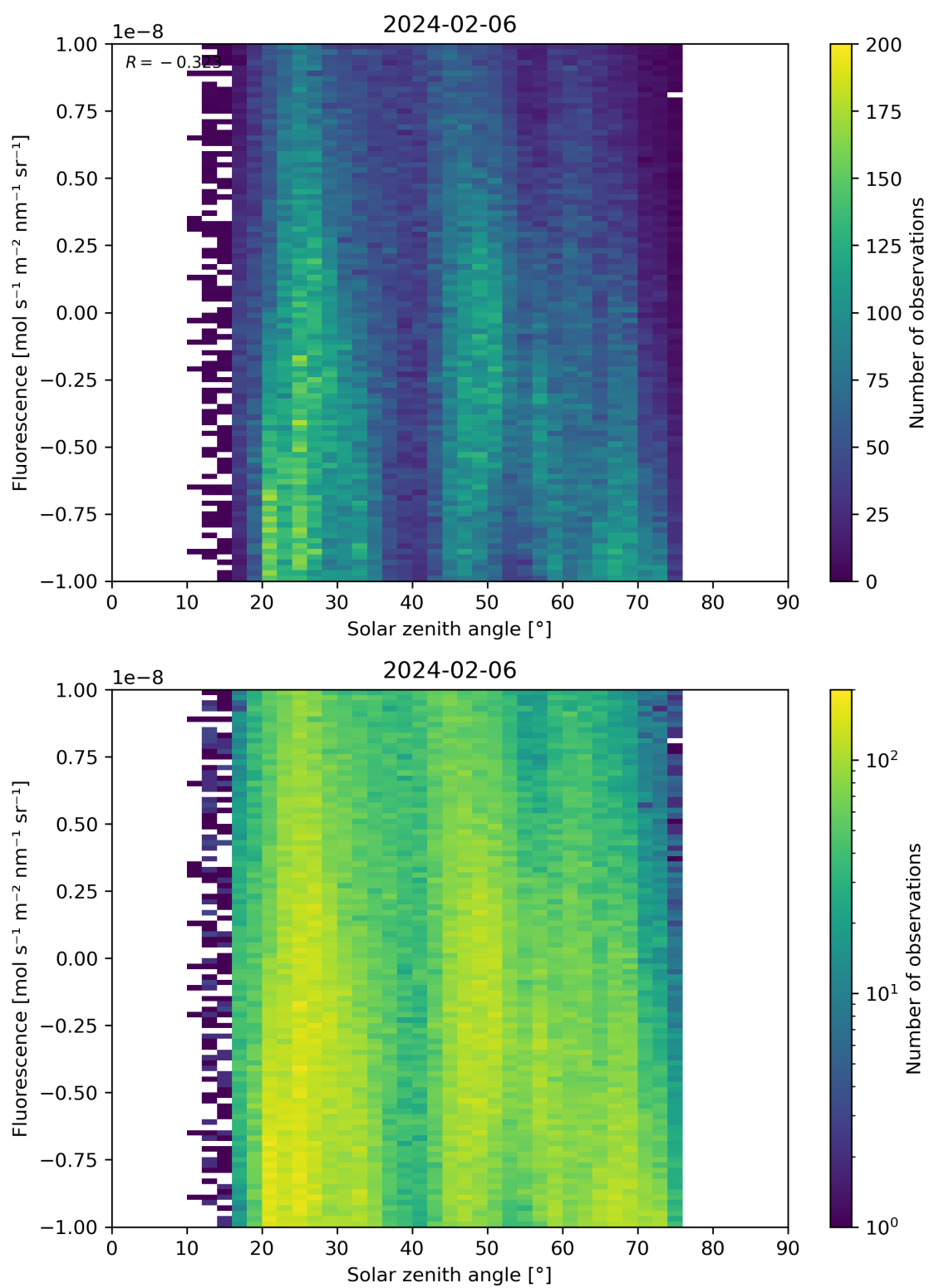
Figure 97: Scatter density plot of “Solar zenith angle” against “Fluorescence” for 2024-02-06 to 2024-02-07.
