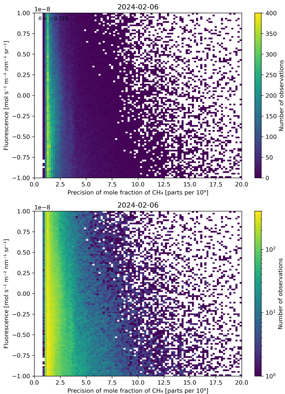
Figure 81: Scatter density plot of “Precision of mole fraction of \text{CH}_4 ” against “Fluorescence” for 2024-02-06 to 2024-02-07.
