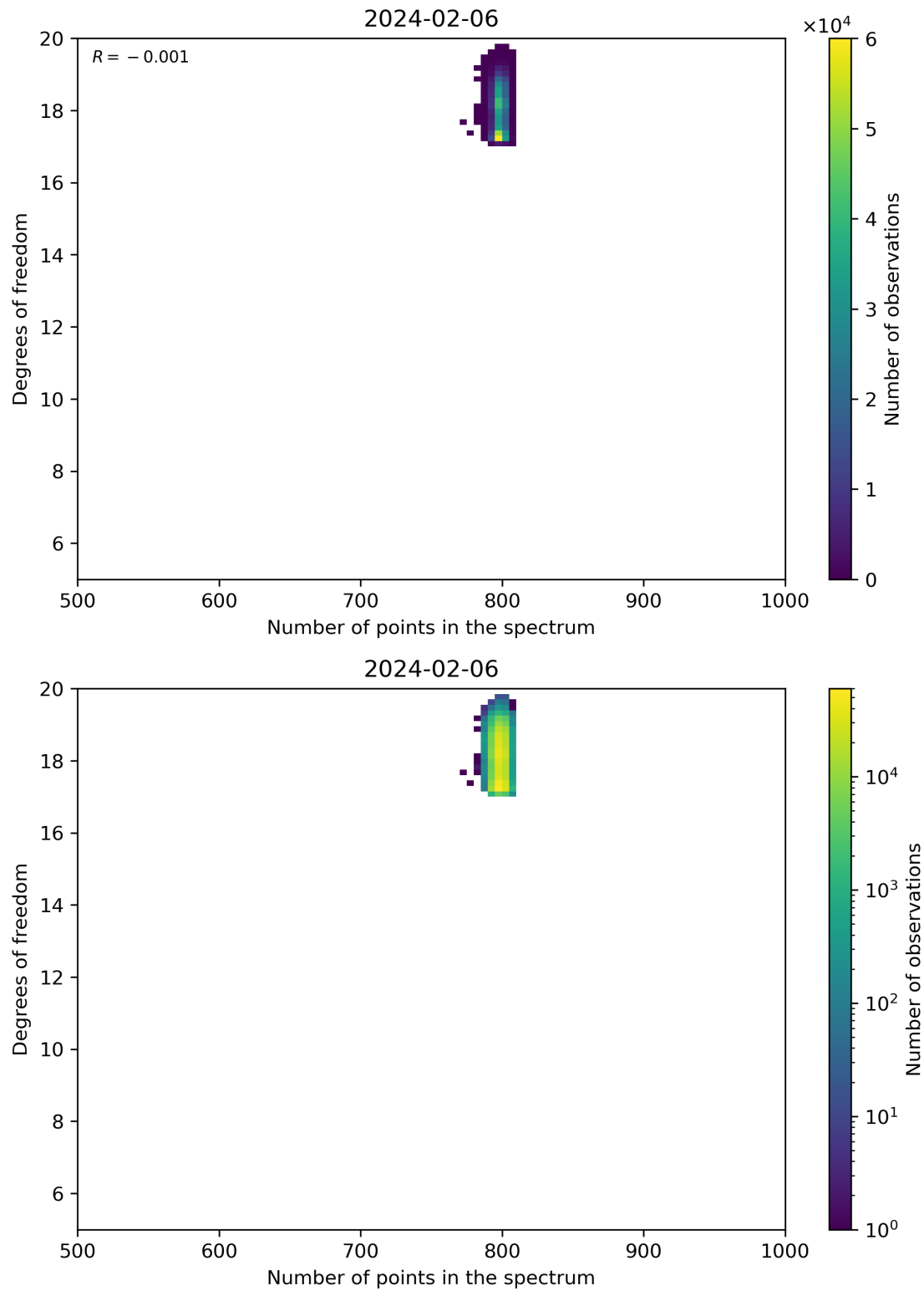
Figure 90: Scatter density plot of “Number of points in the spectrum” against “Degrees of freedom” for 2024-02-06 to 2024-02-07.
