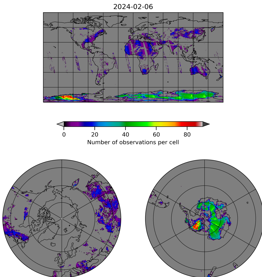
Figure 10: Map of the number of observations for 2024-02-06 to 2024-02-07
