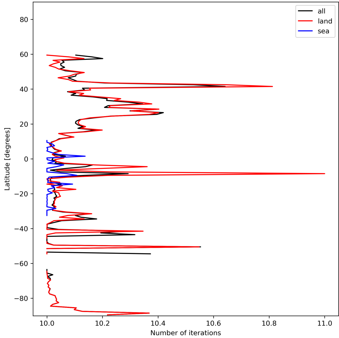
Figure 20: Zonal average of “Number of iterations” for 2024-02-06 to 2024-02-07.
