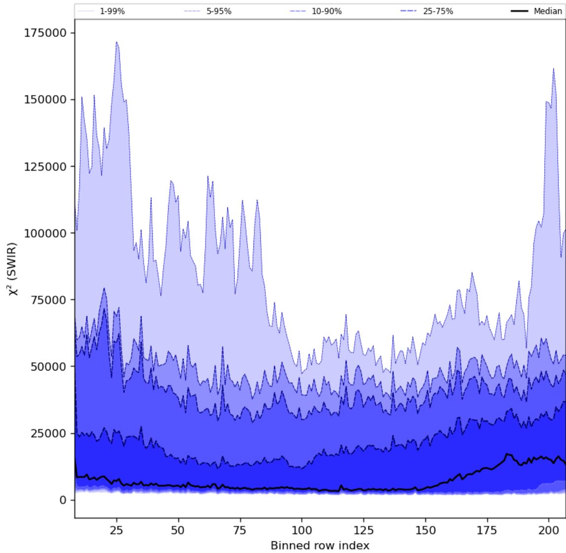
Figure 39: Along track statistics of “ \chi^2 (SWIR)” for 2024-02-06 to 2024-02-07
