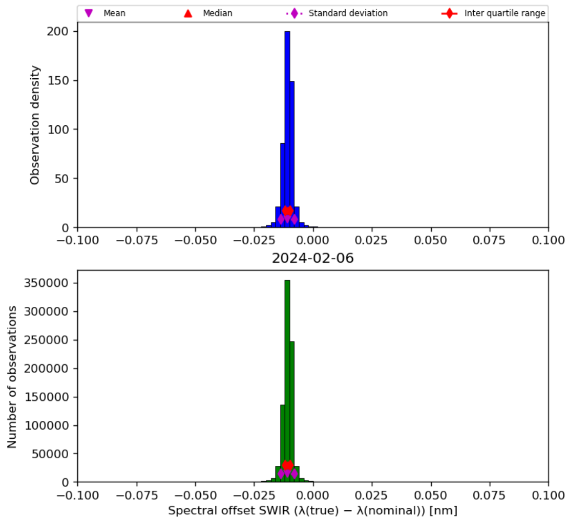
Figure 27: Histogram of “Spectral offset SWIR ( \lambda(\text{true}) - \lambda(\text{nominal}) )” for 2024-02-06 to 2024-02-07
