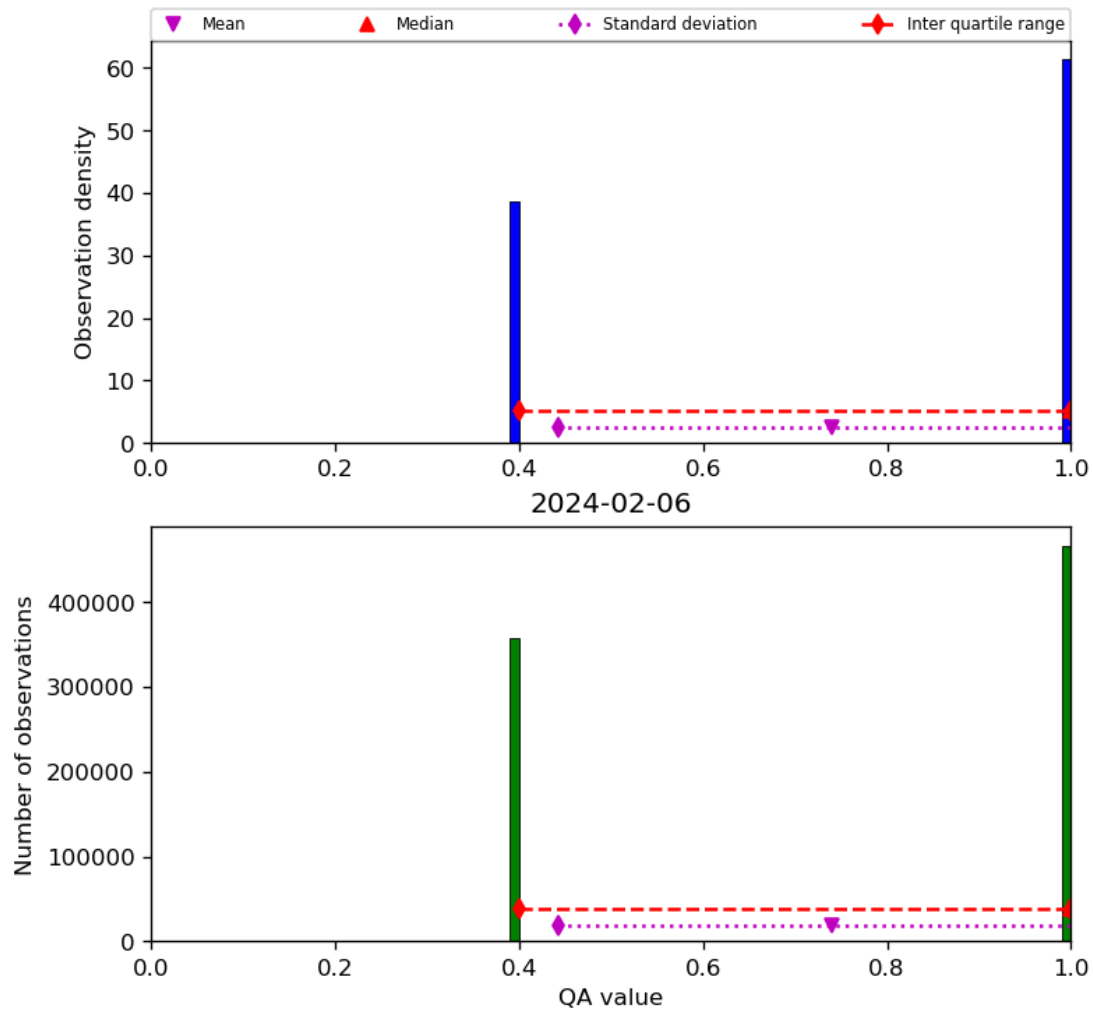
Figure 22: Histogram of “QA value” for 2024-02-06 to 2024-02-07
