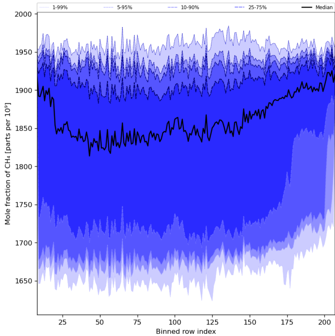
Figure 34: Along track statistics of “Mole fraction of CH 4 ” for 2024-02-06 to 2024-02-07
