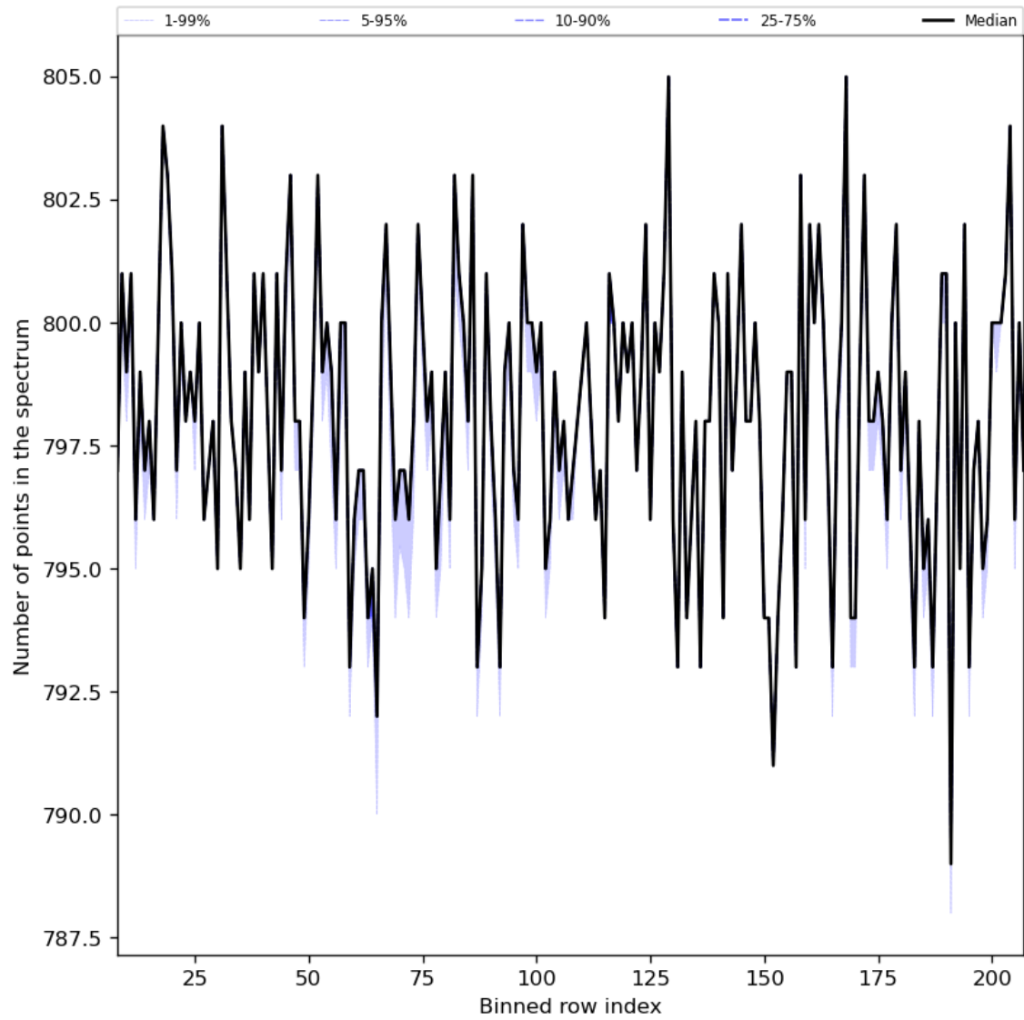
Figure 37: Along track statistics of “Number of points in the spectrum” for 2024-02-06 to 2024-02-07
