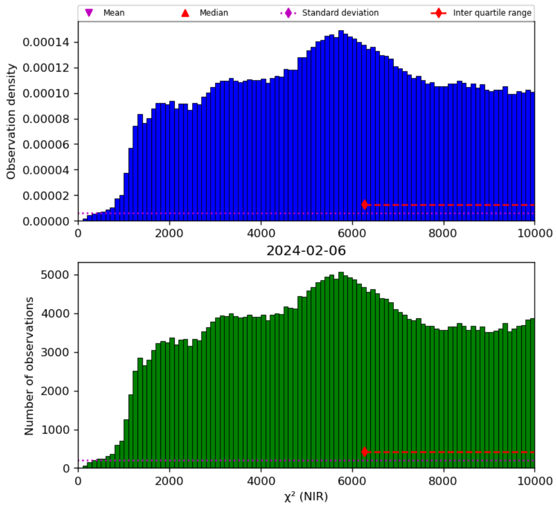
Figure 29: Histogram of “ \chi^2 (NIR)” for 2024-02-06 to 2024-02-07
