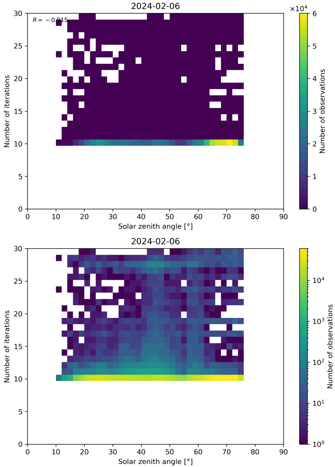
Figure 102: Scatter density plot of “Solar zenith angle” against “Number of iterations” for 2024-02-06 to 2024-02-07.
