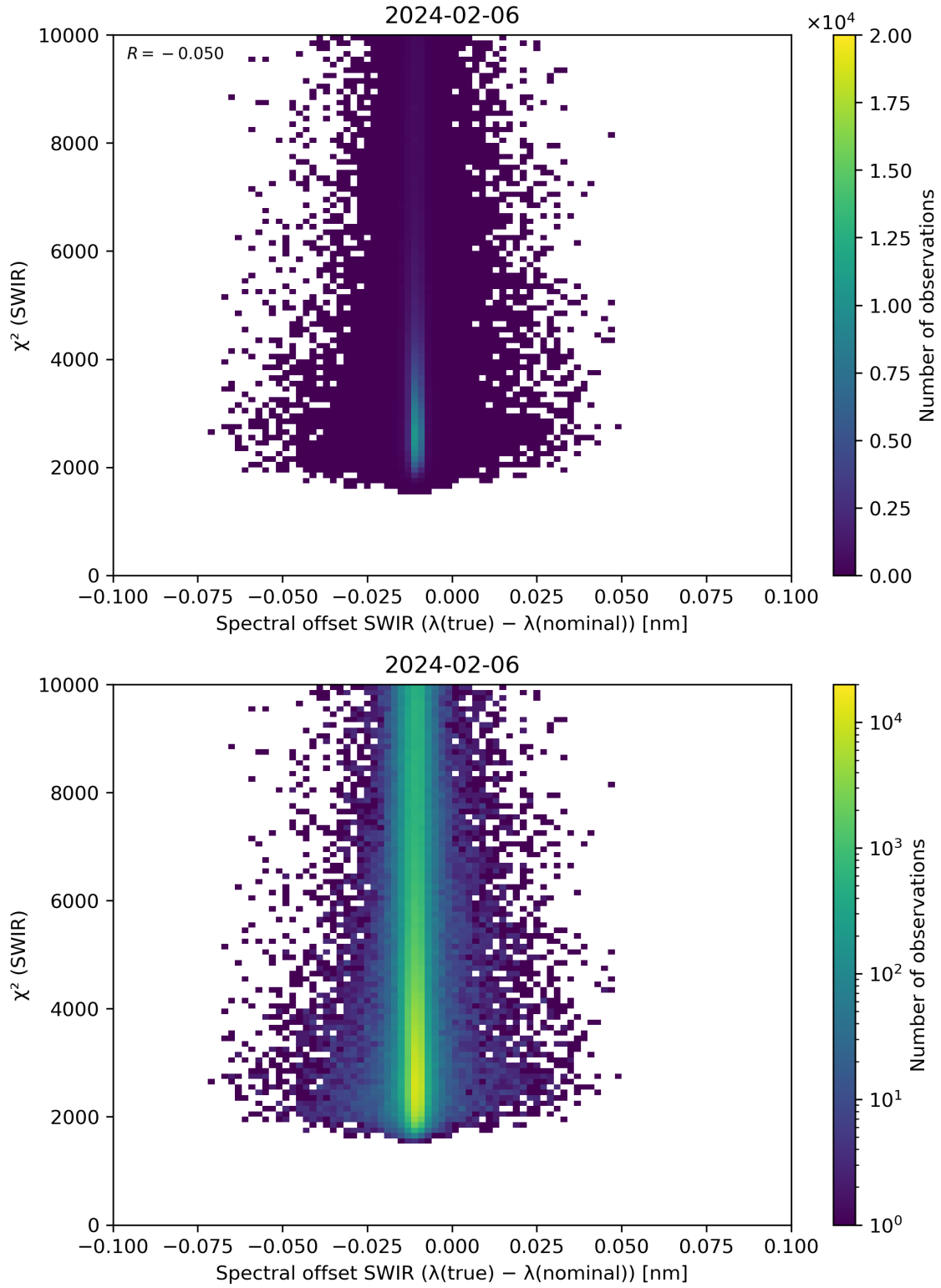
Figure 118: Scatter density plot of “Spectral offset SWIR ( \lambda(\text{true}) - \lambda(\text{nominal}) )” against “ \chi^2 (SWIR)” for 2024-02-06 to 2024-02-07.
