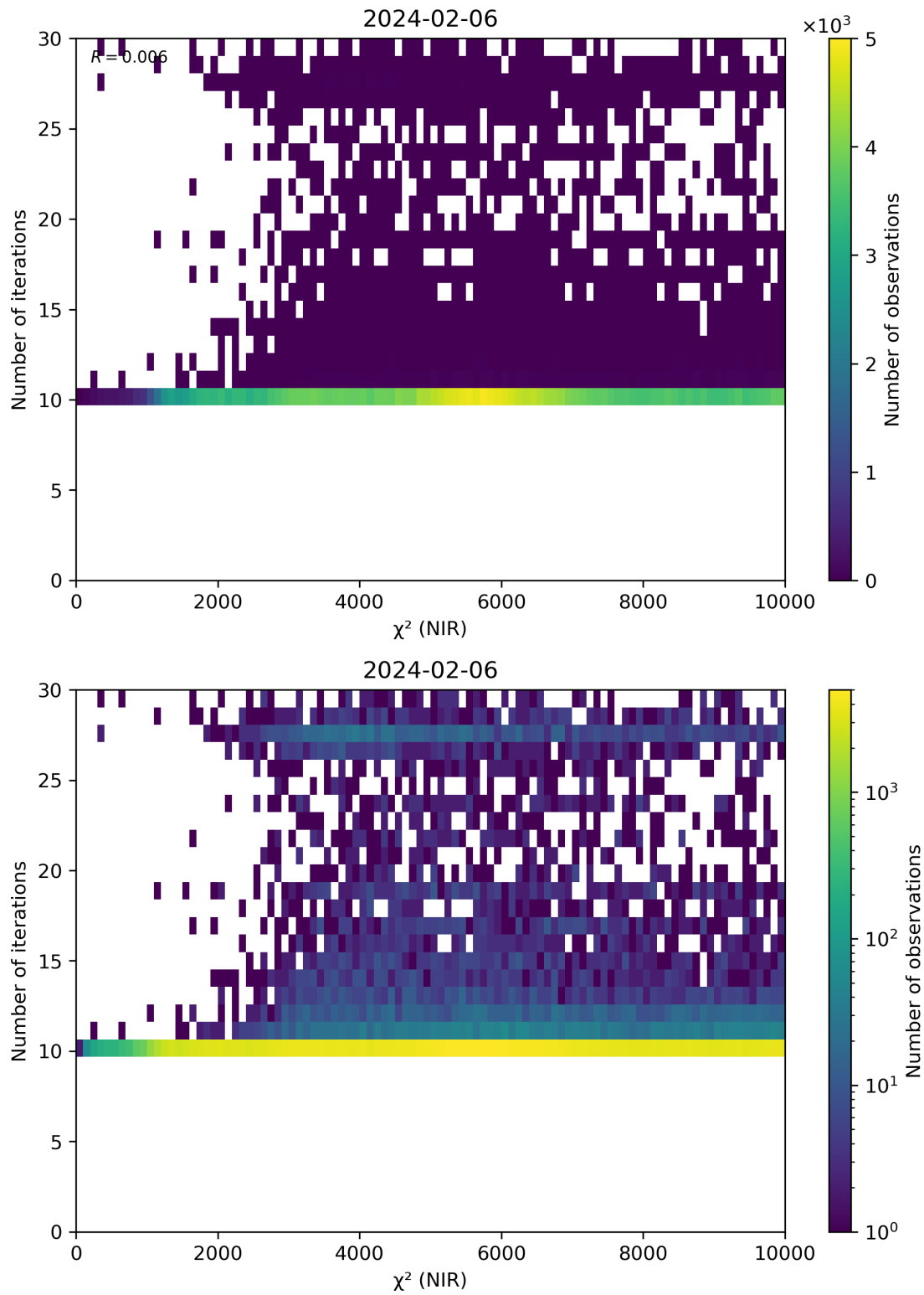
Figure 46: Scatter density plot of “ \chi^2 (NIR)” against “Number of iterations” for 2024-02-06 to 2024-02-07.
