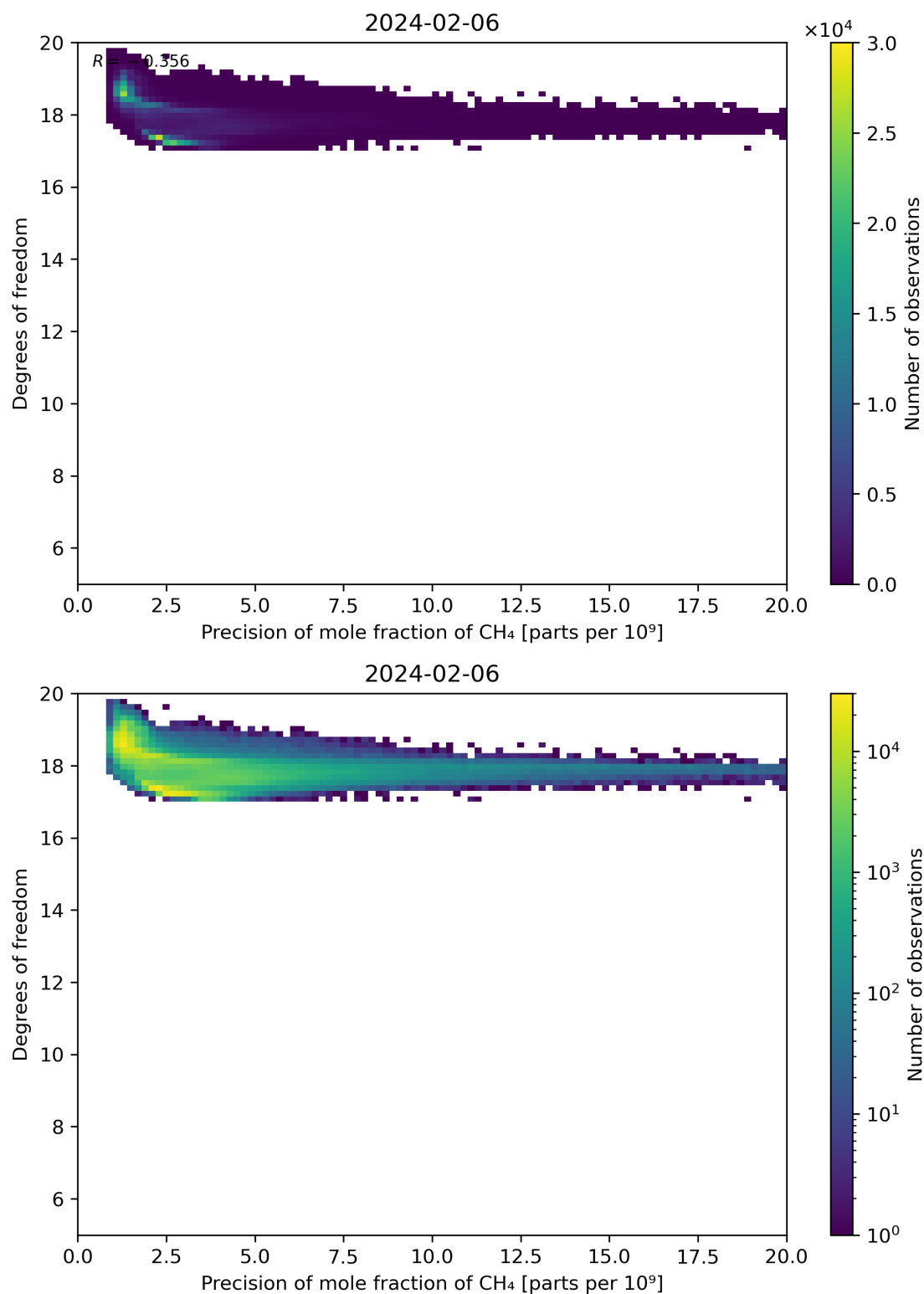
Figure 80: Scatter density plot of “Precision of mole fraction of CH 4 ” against “Degrees of freedom” for 2024-02-06 to 2024-02-07.
