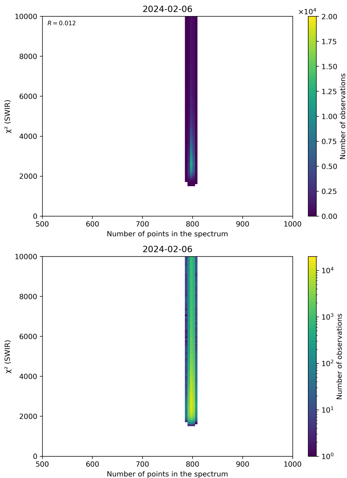
Figure 89: Scatter density plot of “Number of points in the spectrum” against “ \chi^2 (SWIR)” for 2024-02-06 to 2024-02-07.
