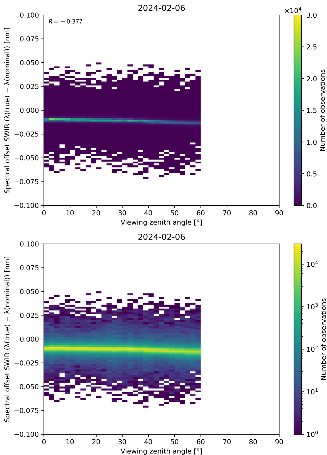
Figure 116: Scatter density plot of “Viewing zenith angle” against “Spectral offset SWIR ( \lambda(\text{true}) - \lambda(\text{nominal}) )” for 2024-02-06 to 2024-02-07.
