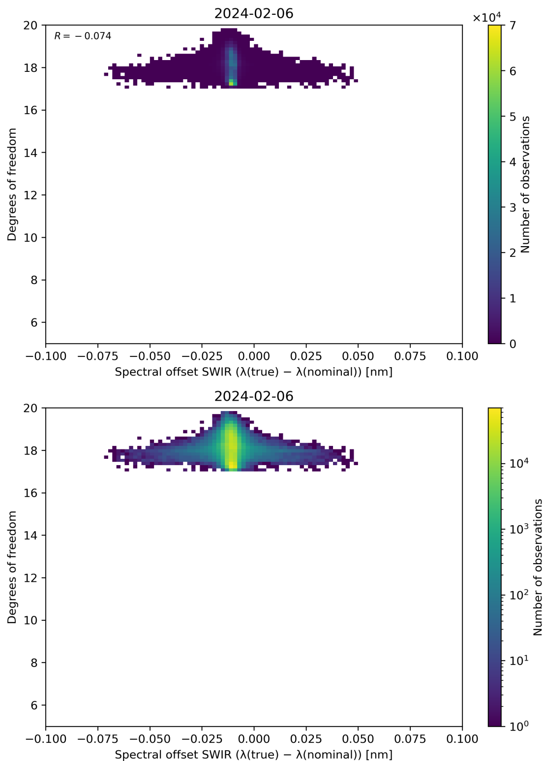
Figure 119: Scatter density plot of “Spectral offset SWIR ( \lambda(\text{true}) - \lambda(\text{nominal}) )” against “Degrees of freedom” for 2024-02-06 to 2024-02-07.
