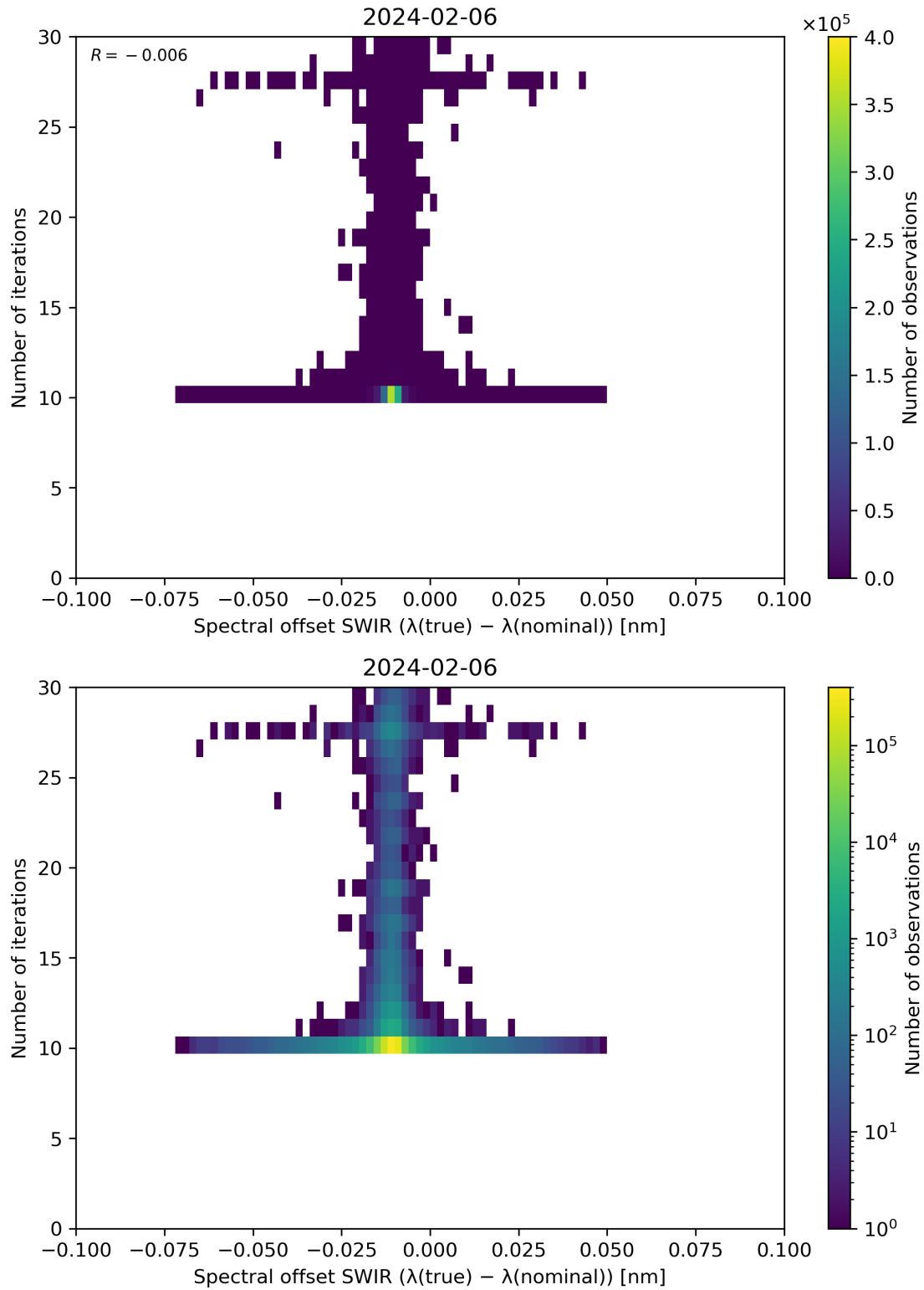
Figure 121: Scatter density plot of “Spectral offset SWIR ( \lambda(\text{true}) - \lambda(\text{nominal}) )” against “Number of iterations” for 2024-02-06 to 2024-02-07.
