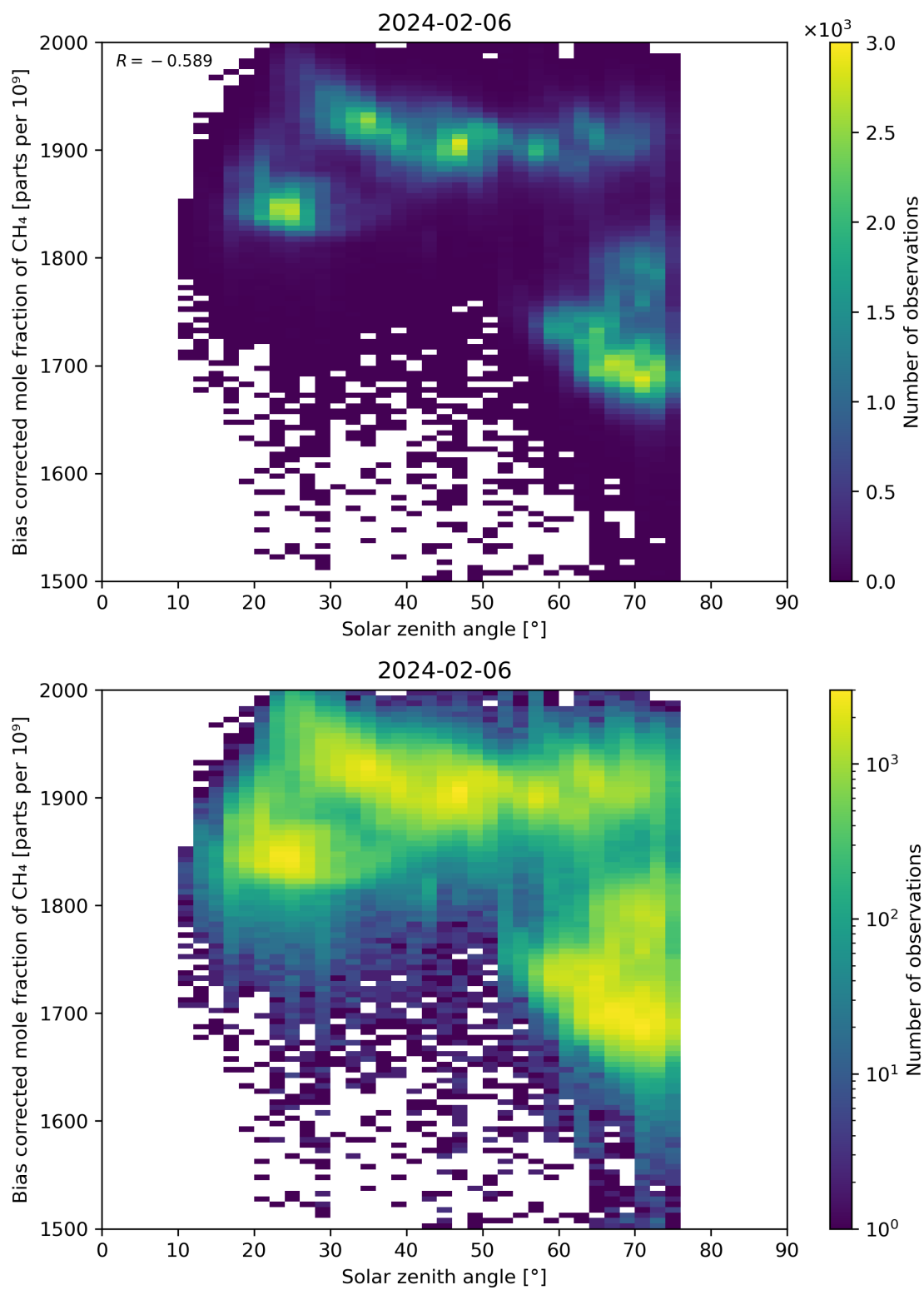
Figure 100: Scatter density plot of “Solar zenith angle” against “Bias corrected mole fraction of CH 4 ” for 2024-02-06 to 2024-02-07.
