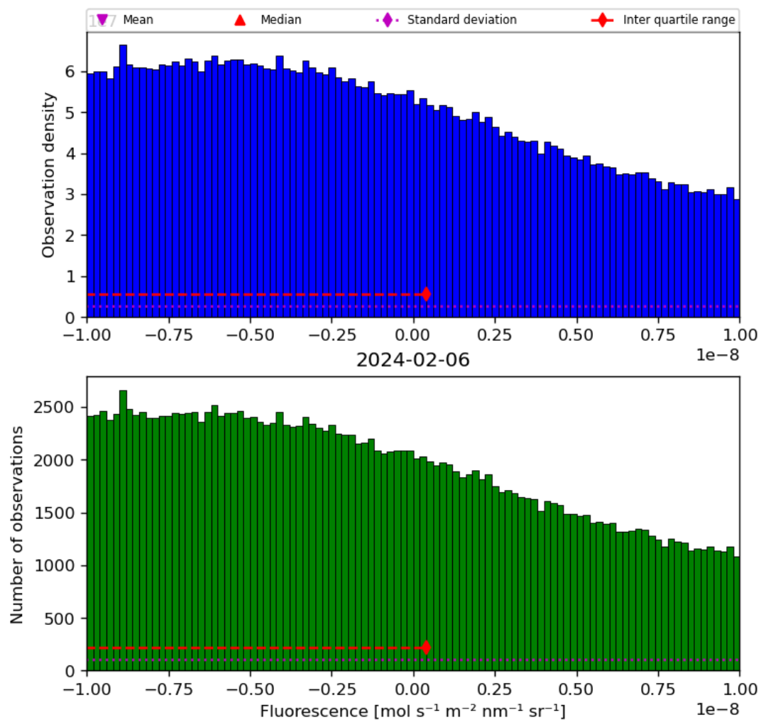
Figure 32: Histogram of “Fluorescence” for 2024-02-06 to 2024-02-07
