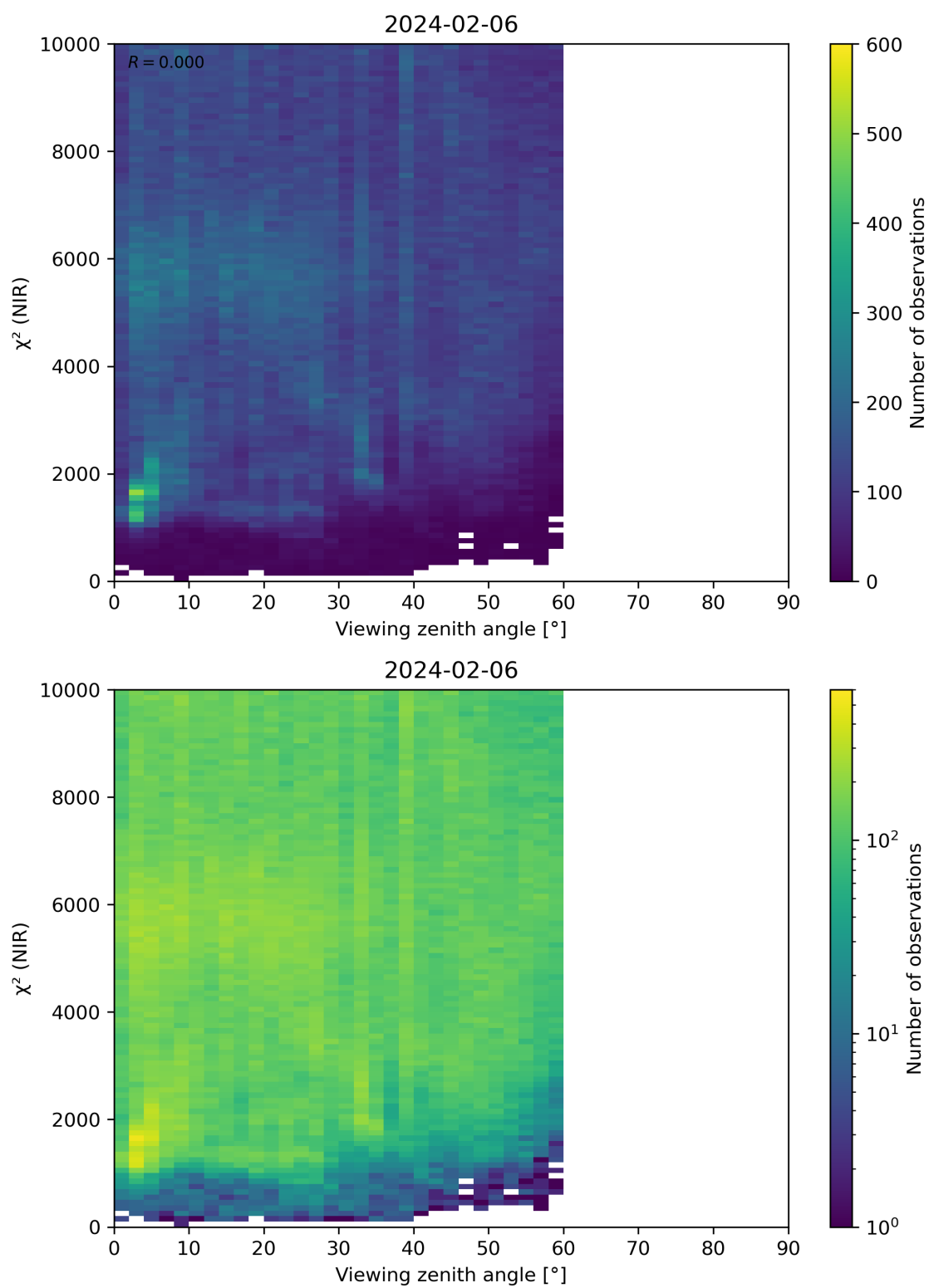
Figure 105: Scatter density plot of “Viewing zenith angle” against “ \chi^2 (NIR)” for 2024-02-06 to 2024-02-07.
