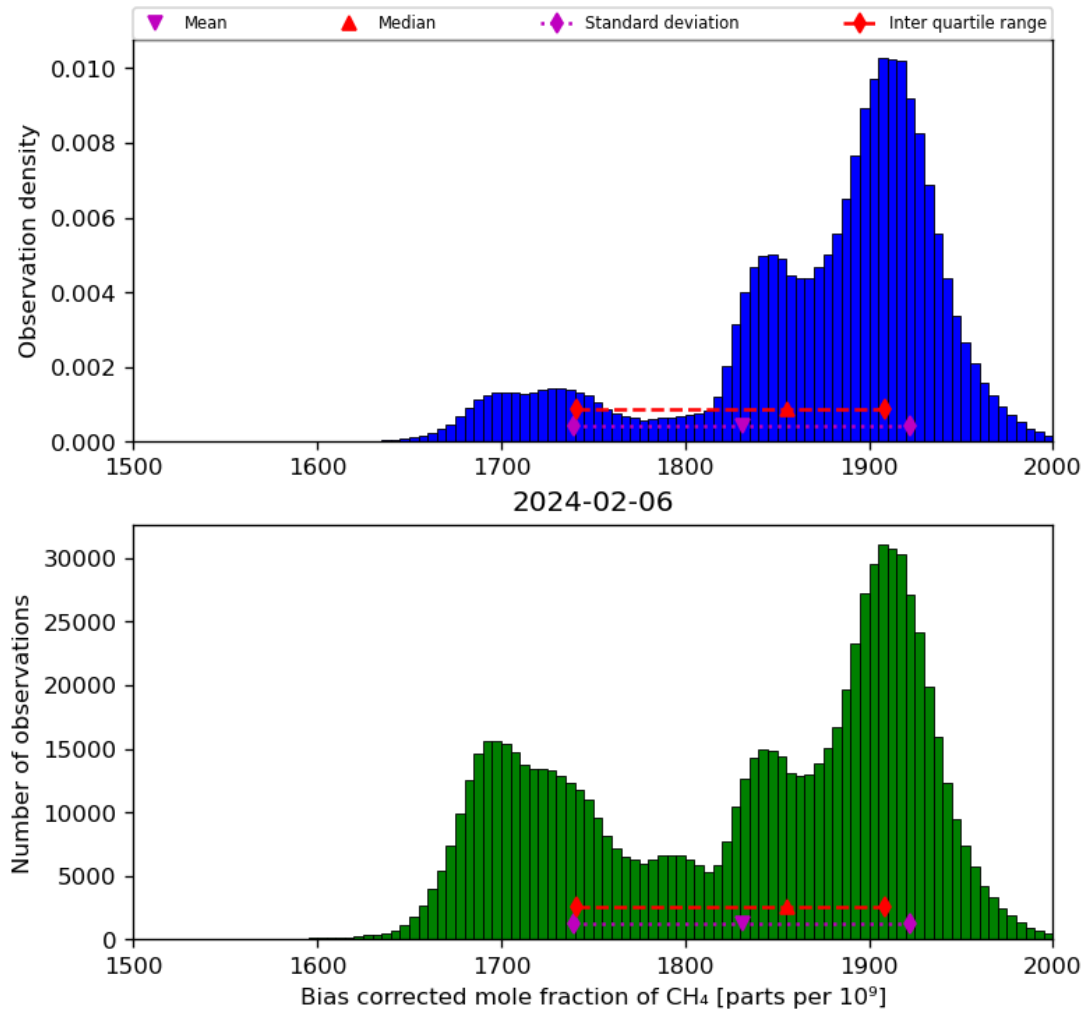
Figure 25: Histogram of “Bias corrected mole fraction of CH 4 ” for 2024-02-06 to 2024-02-07
