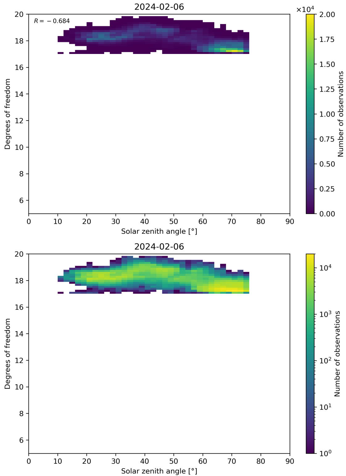
Figure 96: Scatter density plot of “Solar zenith angle” against “Degrees of freedom” for 2024-02-06 to 2024-02-07.
