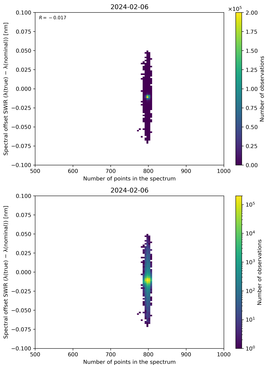
Figure 93: Scatter density plot of “Number of points in the spectrum” against “Spectral offset SWIR ( \lambda(\text{true}) - \lambda(\text{nominal}) )” for 2024-02-06 to 2024-02-07.
