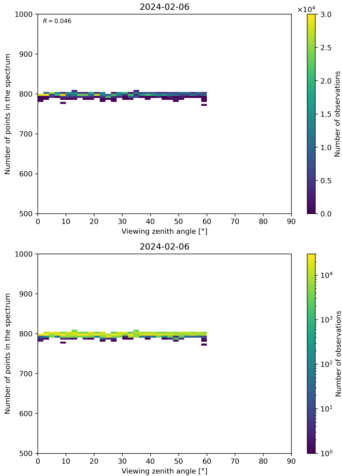
Figure 114: Scatter density plot of “Viewing zenith angle” against “Number of points in the spectrum” for 2024-02-06 to 2024-02-07.
