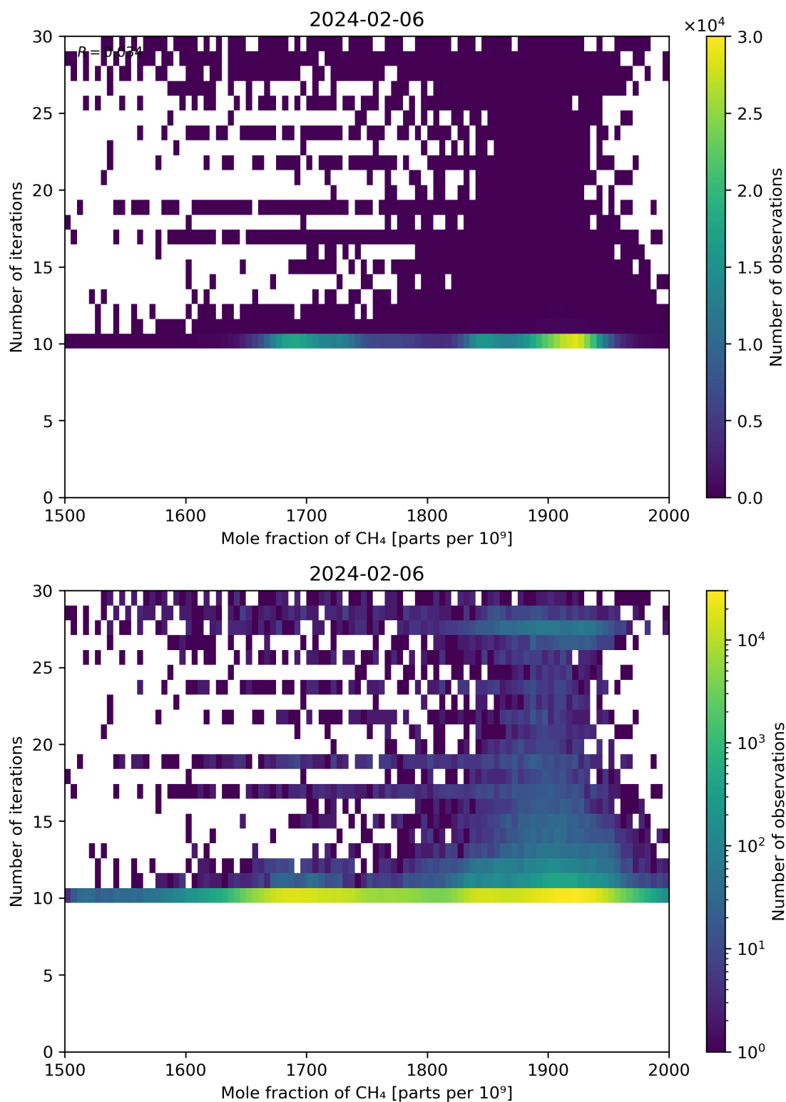
Figure 76: Scatter density plot of “Mole fraction of CH 4 ” against “Number of iterations” for 2024-02-06 to 2024-02-07.
