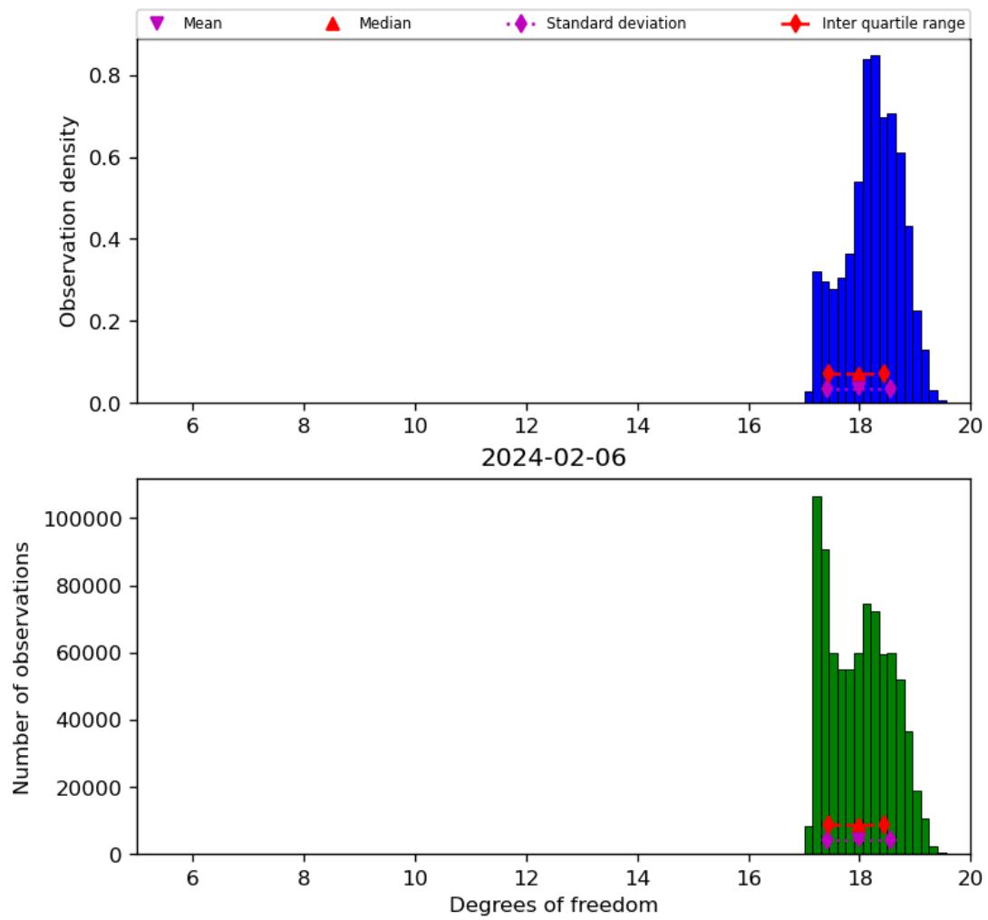
Figure 30: Histogram of “Degrees of freedom” for 2024-02-06 to 2024-02-07
