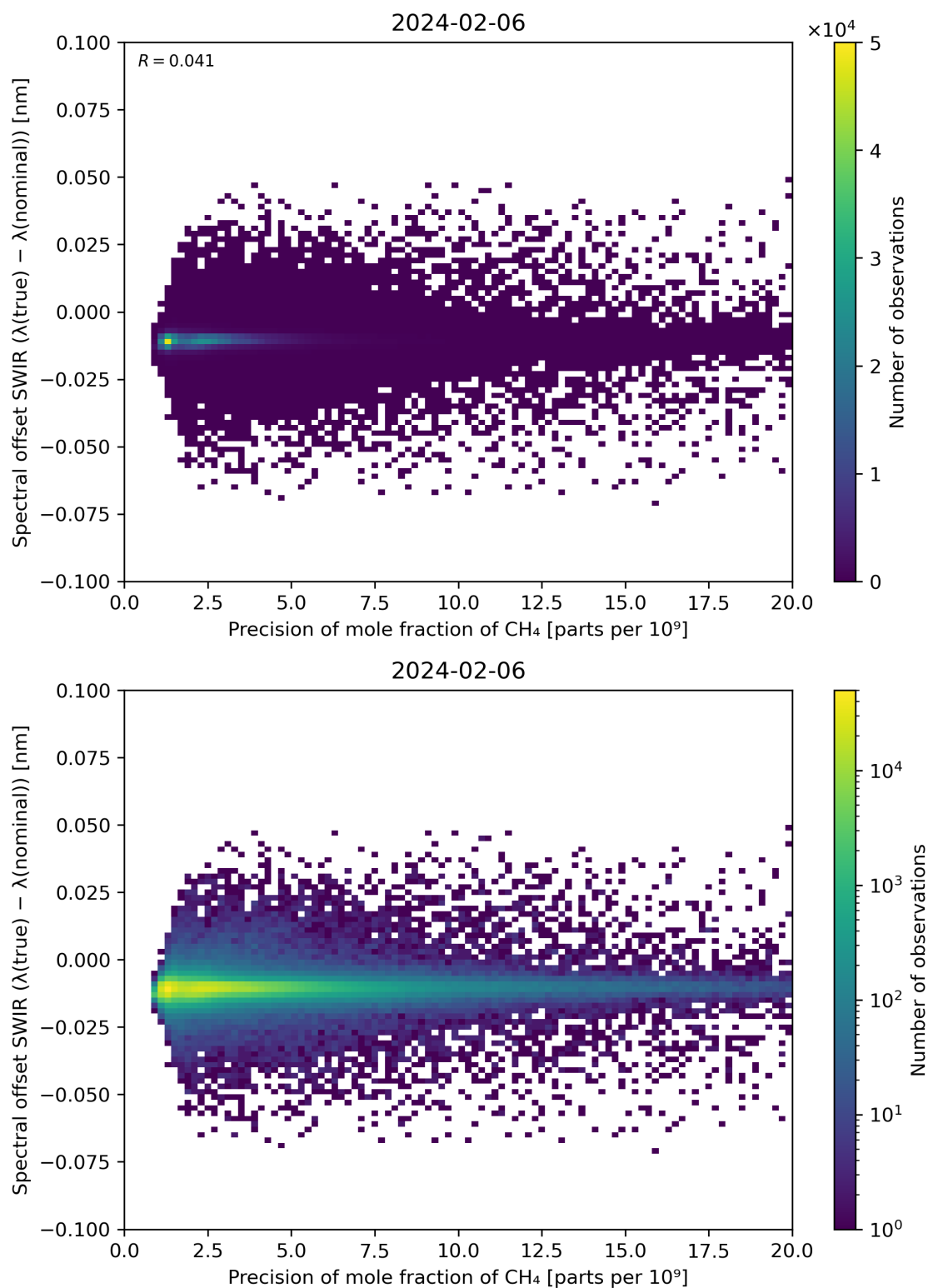
Figure 85: Scatter density plot of “Precision of mole fraction of \text{CH}_4 ” against “Spectral offset SWIR ( \lambda(\text{true}) - \lambda(\text{nominal}) )” for 2024-02-06 to 2024-02-07.
