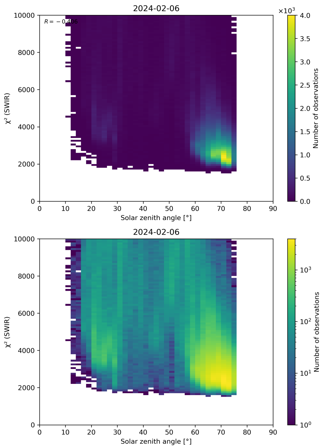
Figure 95: Scatter density plot of “Solar zenith angle” against “ \chi^2 (SWIR)” for 2024-02-06 to 2024-02-07.
