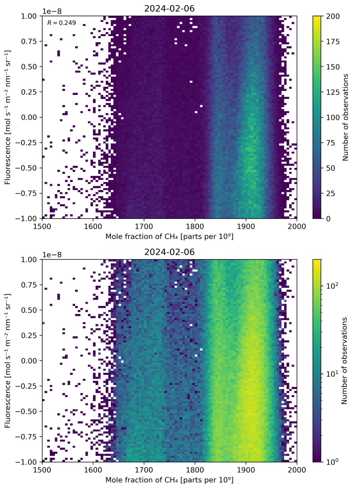
Figure 73: Scatter density plot of “Mole fraction of CH 4 ” against “Fluorescence” for 2024-02-06 to 2024-02-07.
