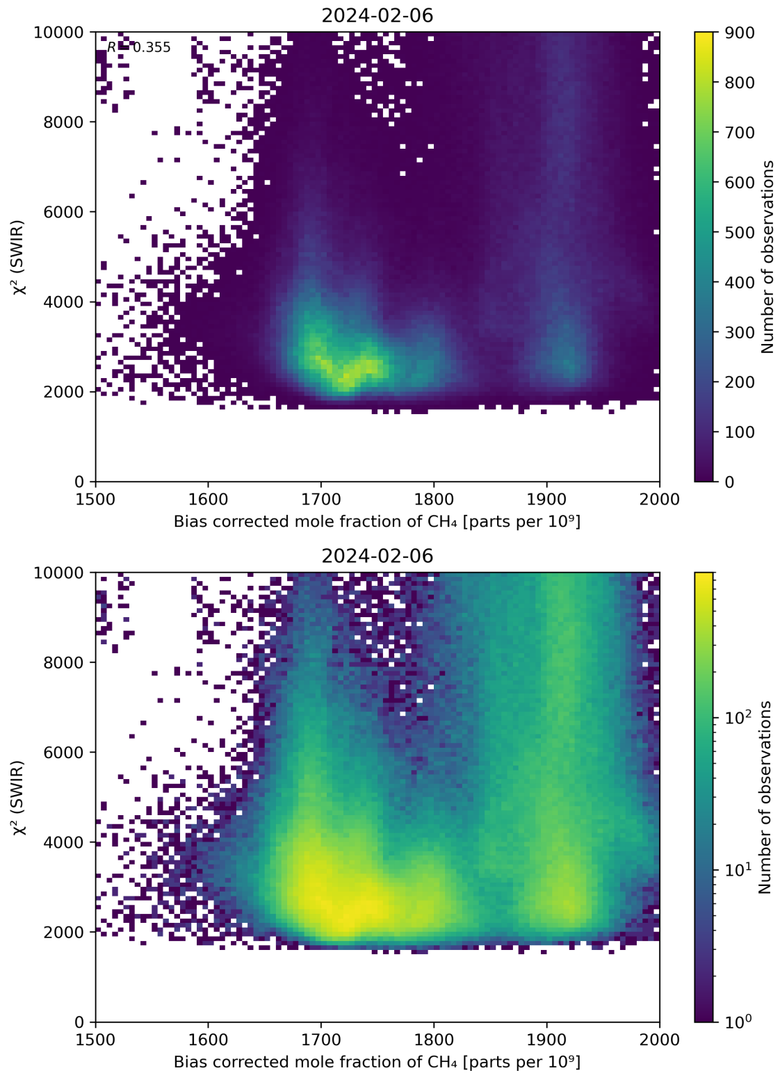
Figure 64: Scatter density plot of “Bias corrected mole fraction of CH 4 ” against “ \chi^2 (SWIR)” for 2024-02-06 to 2024-02-07.
