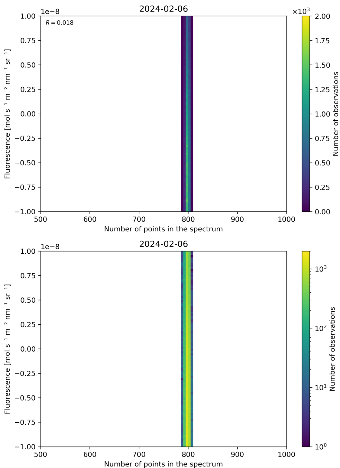
Figure 91: Scatter density plot of “Number of points in the spectrum” against “Fluorescence” for 2024-02-06 to 2024-02-07.
