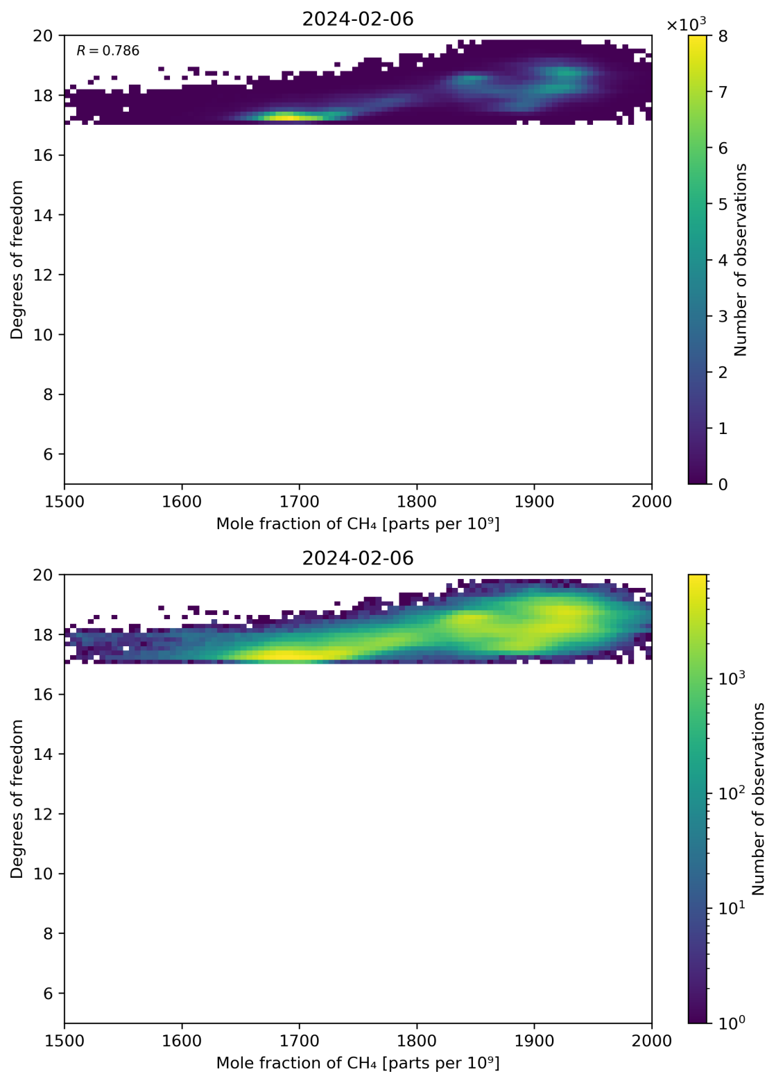
Figure 72: Scatter density plot of “Mole fraction of CH 4 ” against “Degrees of freedom” for 2024-02-06 to 2024-02-07.
