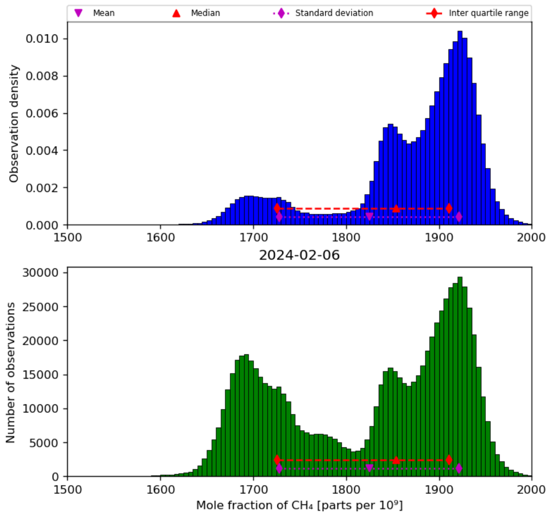
Figure 23: Histogram of “Mole fraction of CH 4 ” for 2024-02-06 to 2024-02-07
