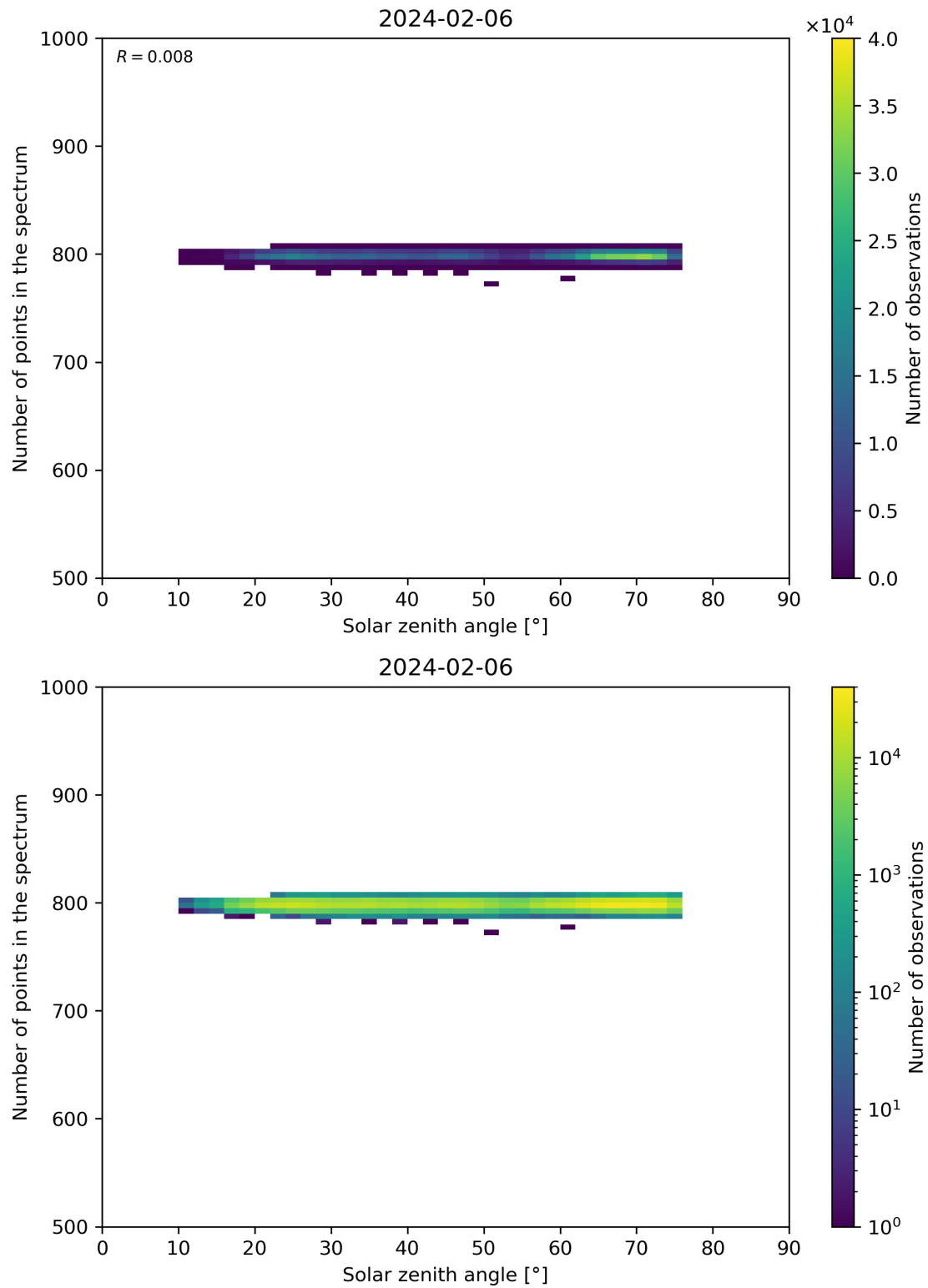
Figure 103: Scatter density plot of “Solar zenith angle” against “Number of points in the spectrum” for 2024-02-06 to 2024-02-07.
