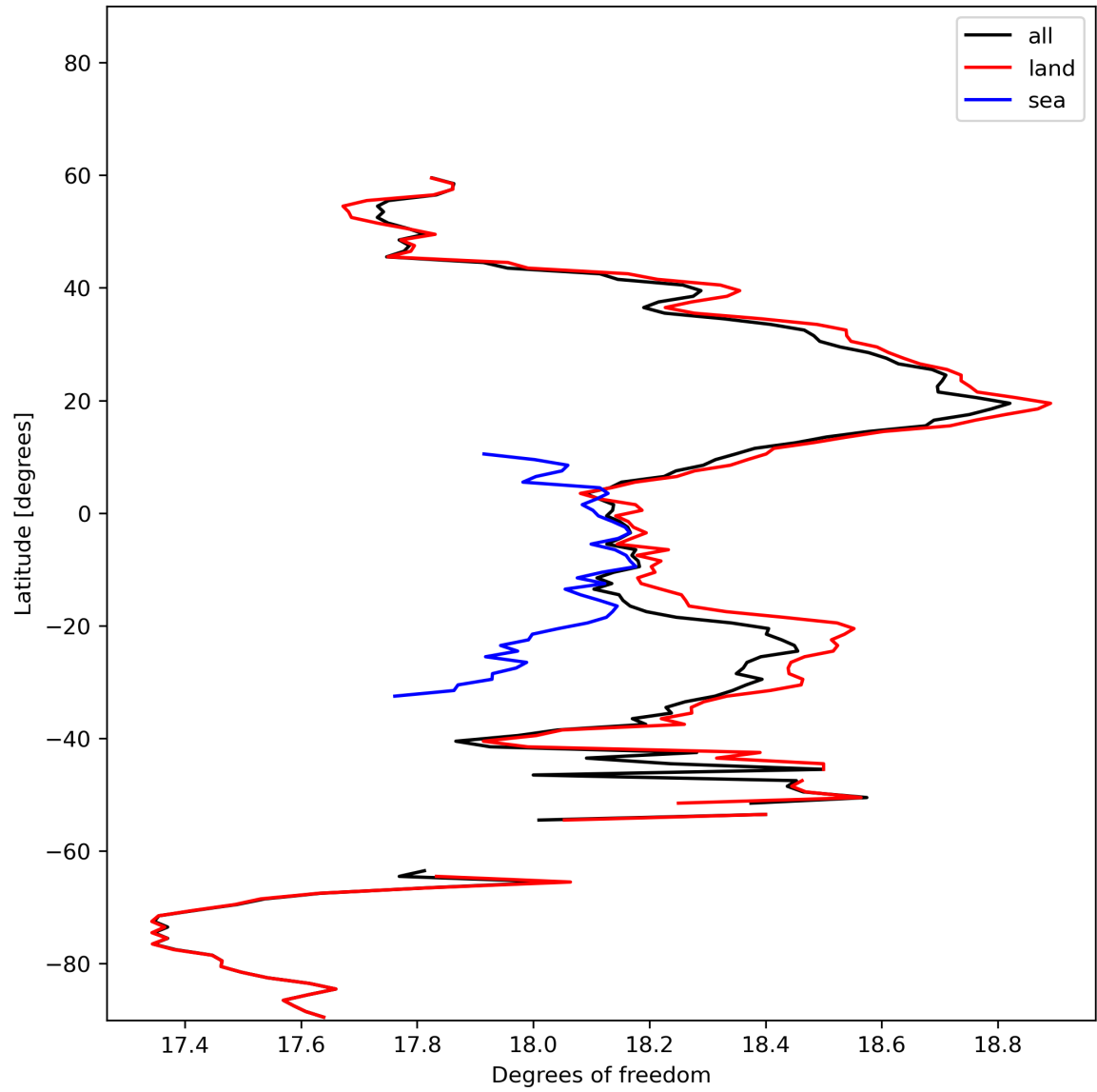
Figure 19: Zonal average of “Degrees of freedom” for 2024-02-06 to 2024-02-07.
