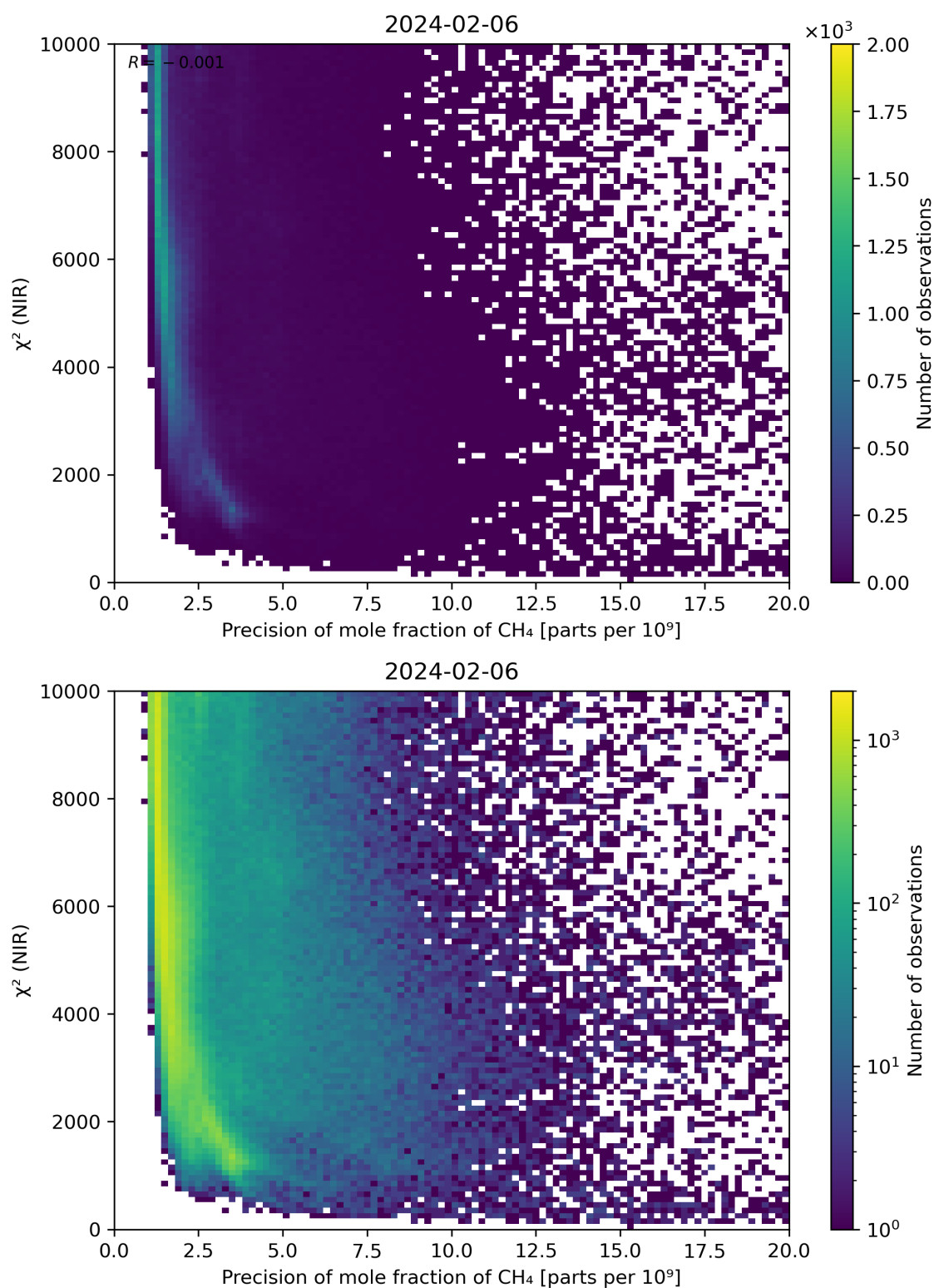
Figure 78: Scatter density plot of “Precision of mole fraction of CH 4 ” against “ \chi^2 (NIR)” for 2024-02-06 to 2024-02-07.
