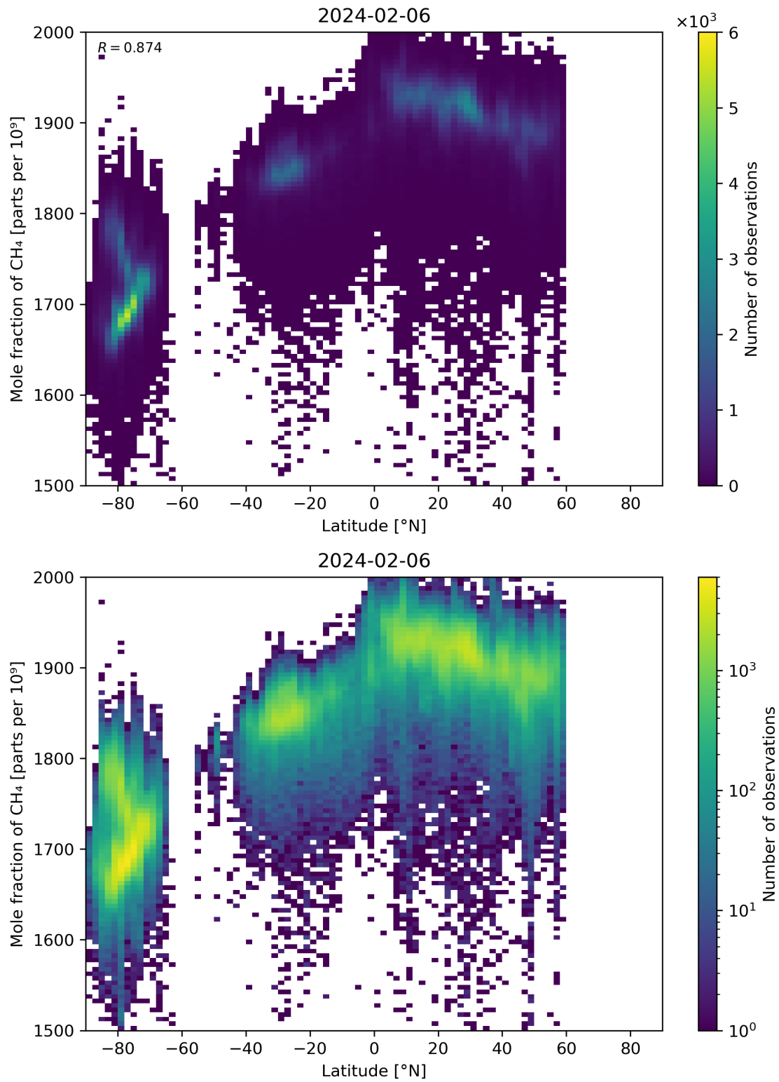
Figure 57: Scatter density plot of “Latitude” against “Mole fraction of \text{CH}_4 ” for 2024-02-06 to 2024-02-07.
