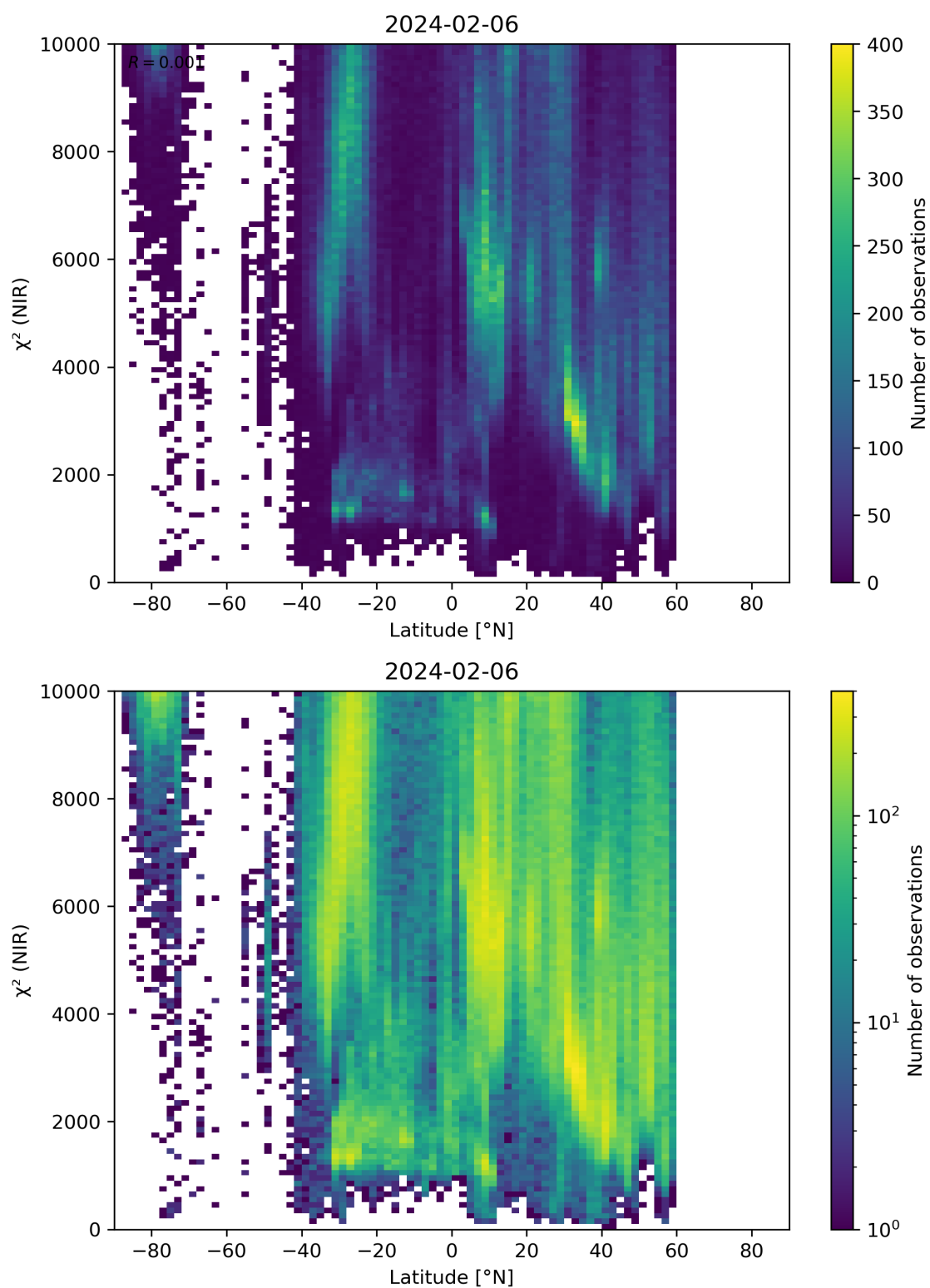
Figure 53: Scatter density plot of “Latitude” against “ \chi^2 (NIR)” for 2024-02-06 to 2024-02-07.
