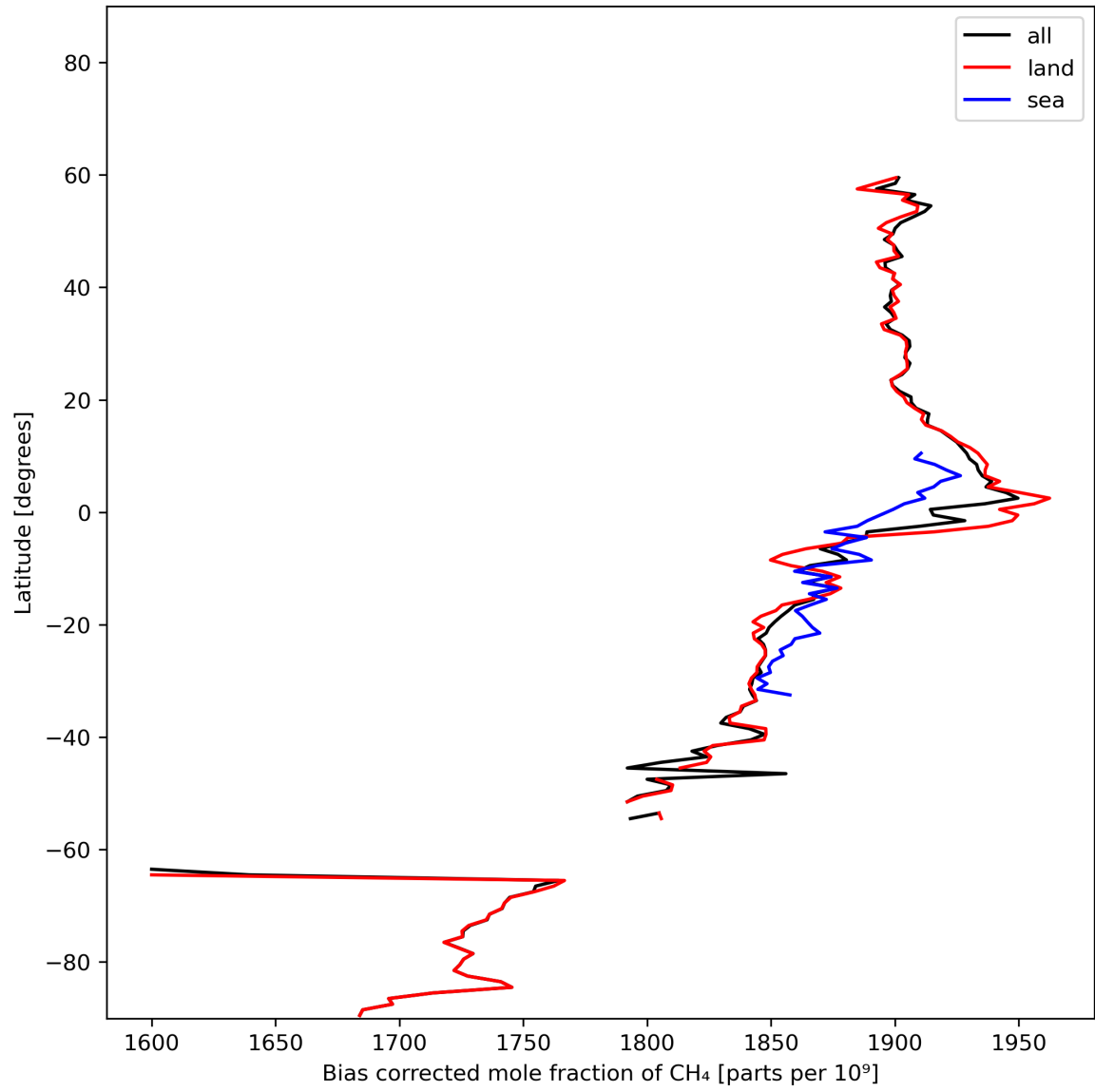
Figure 14: Zonal average of “Bias corrected mole fraction of CH 4 ” for 2024-02-06 to 2024-02-07.
