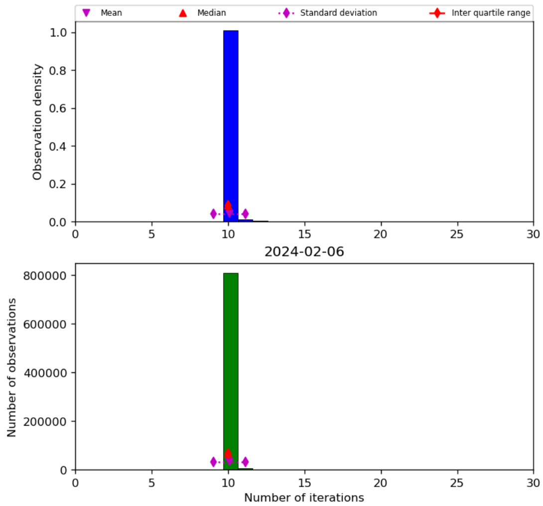
Figure 31: Histogram of “Number of iterations” for 2024-02-06 to 2024-02-07
