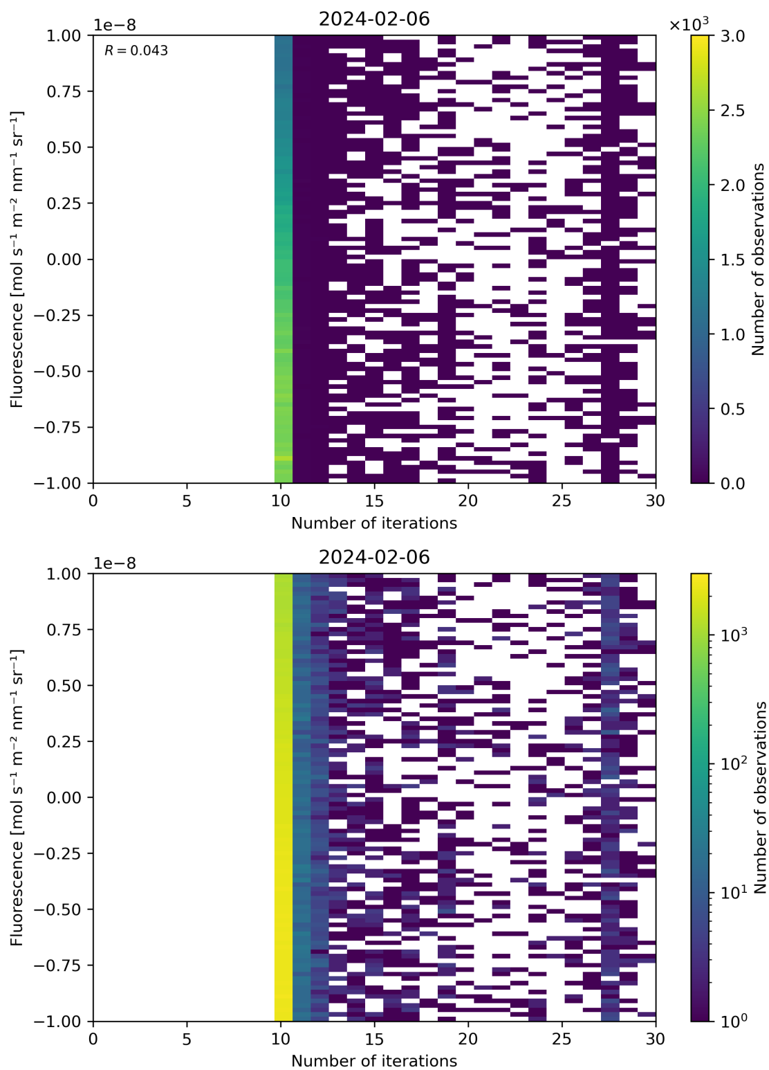
Figure 87: Scatter density plot of "Number of iterations" against "Fluorescence" for 2024-02-06 to 2024-02-07.
