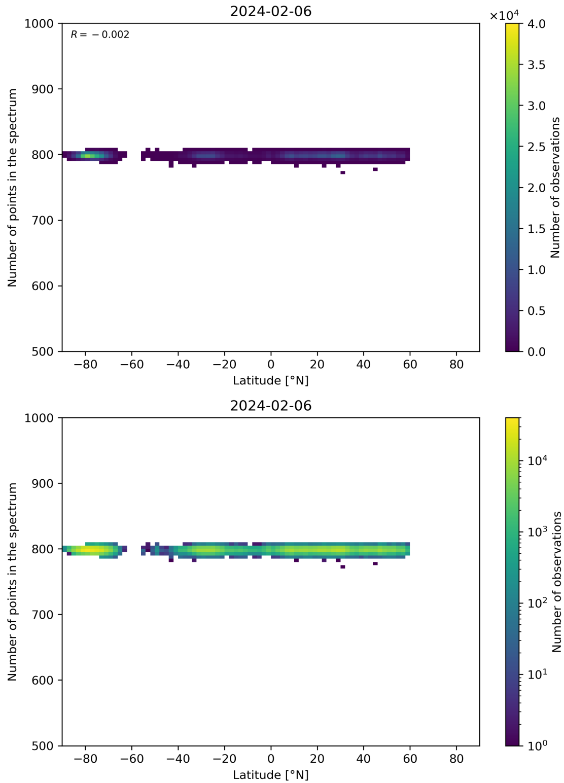
Figure 61: Scatter density plot of “Latitude” against “Number of points in the spectrum” for 2024-02-06 to 2024-02-07.
