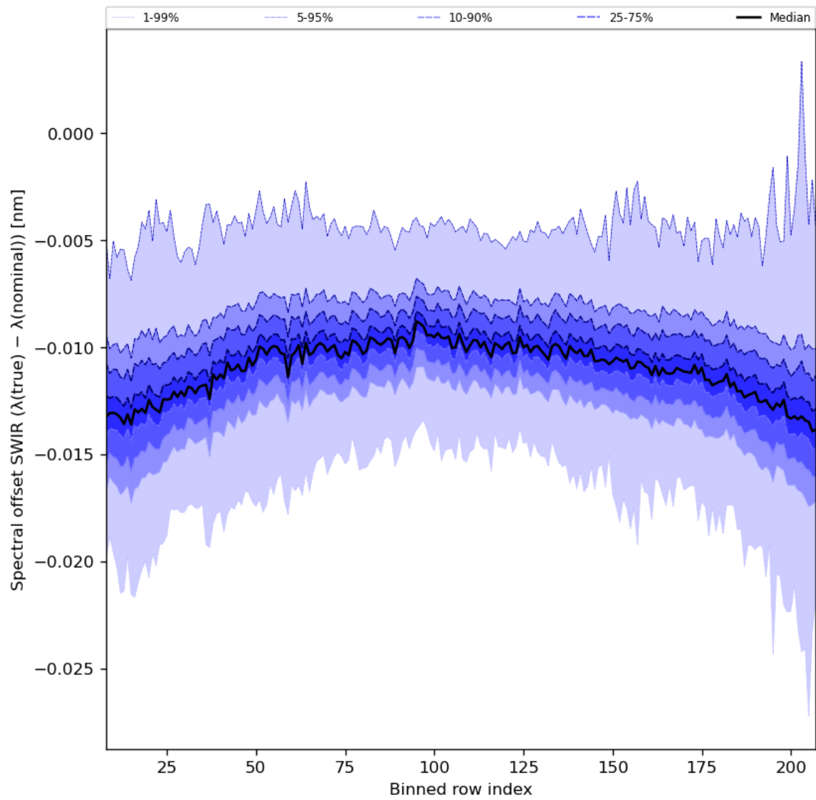
Figure 38: Along track statistics of “Spectral offset SWIR ( \lambda(\text{true}) - \lambda(\text{nominal}) )” for 2024-02-06 to 2024-02-07
