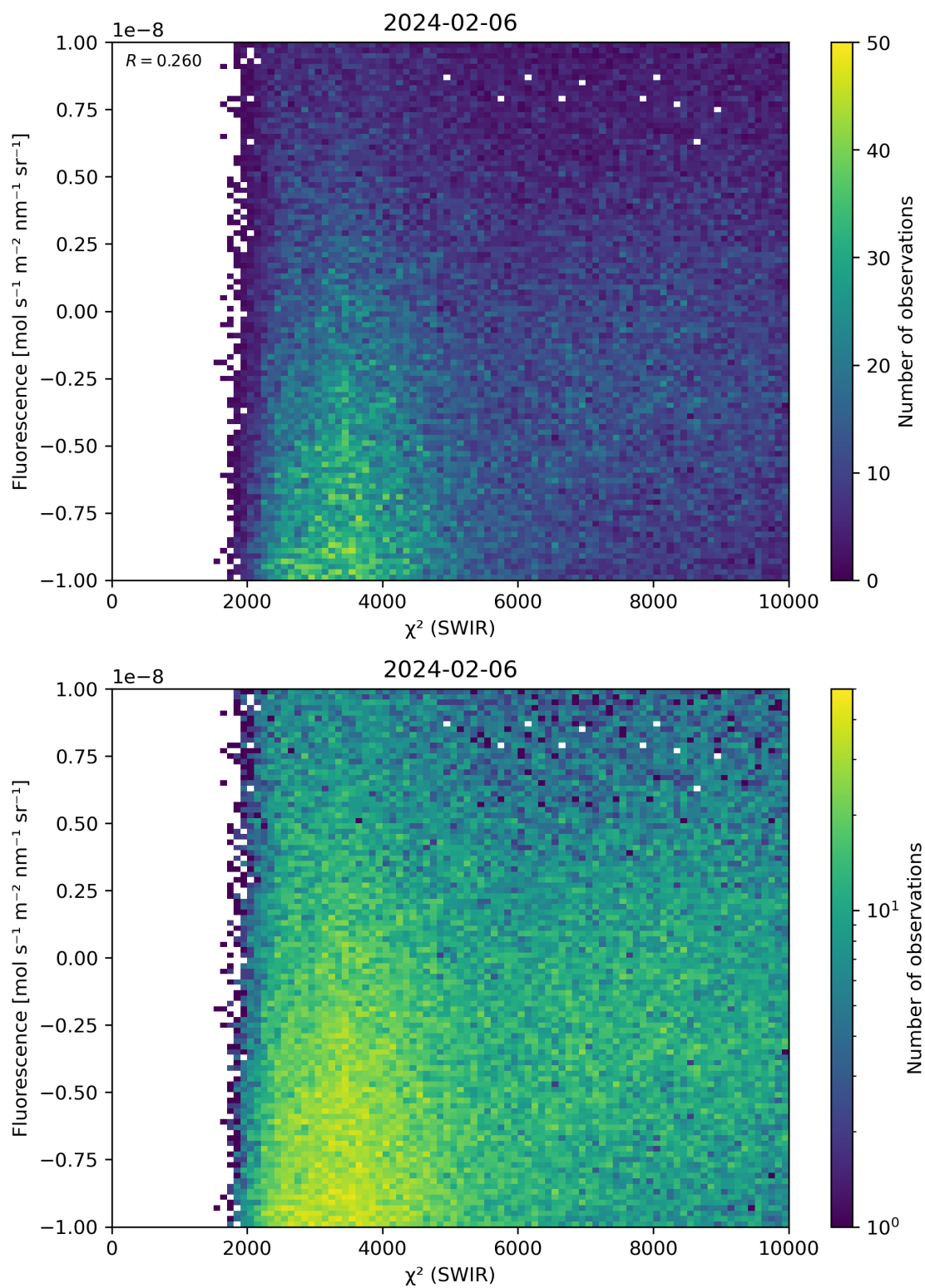
Figure 49: Scatter density plot of “ \chi^2 (SWIR)” against “Fluorescence” for 2024-02-06 to 2024-02-07.
