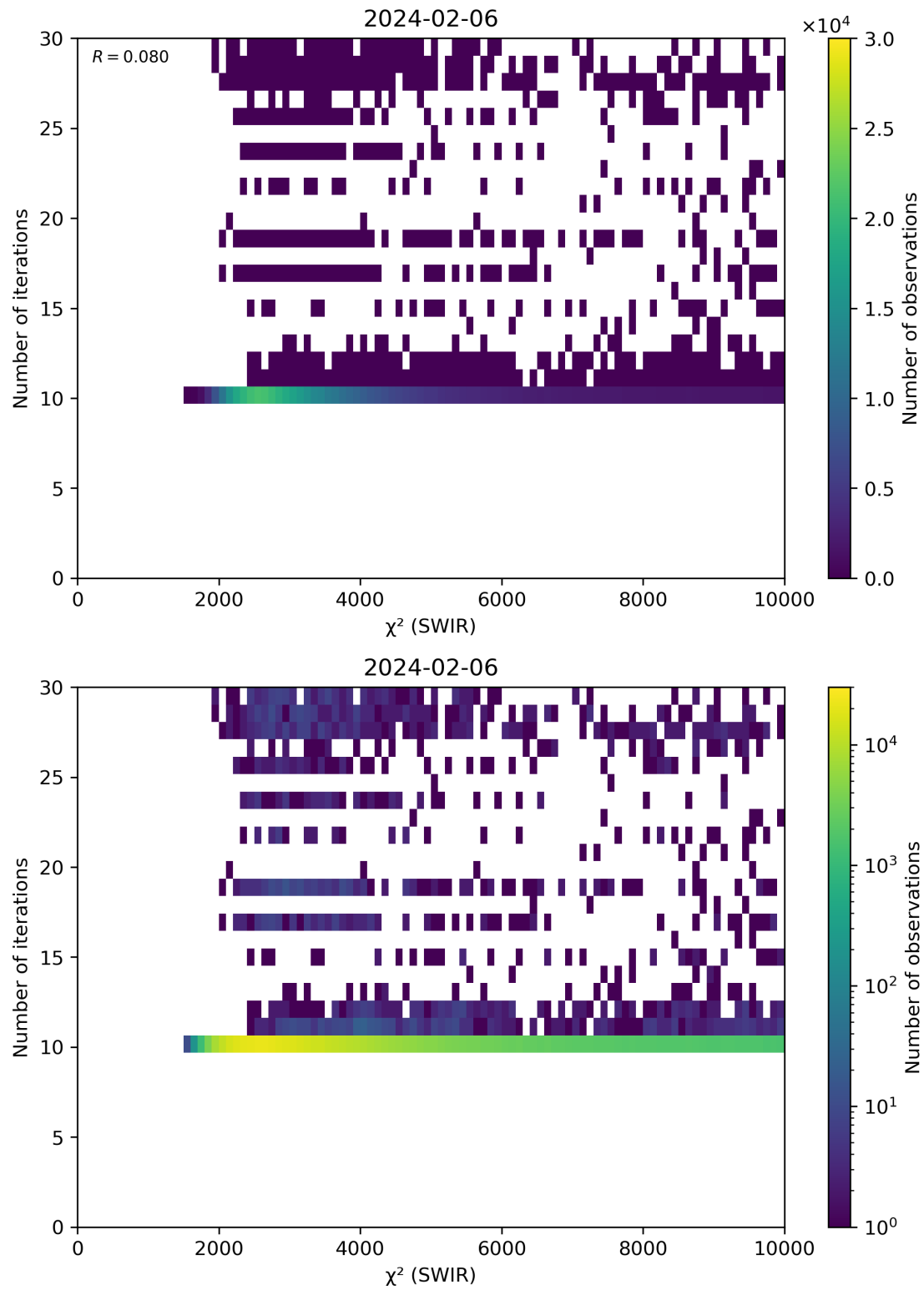
Figure 50: Scatter density plot of “ \chi^2 (SWIR)” against “Number of iterations” for 2024-02-06 to 2024-02-07.
