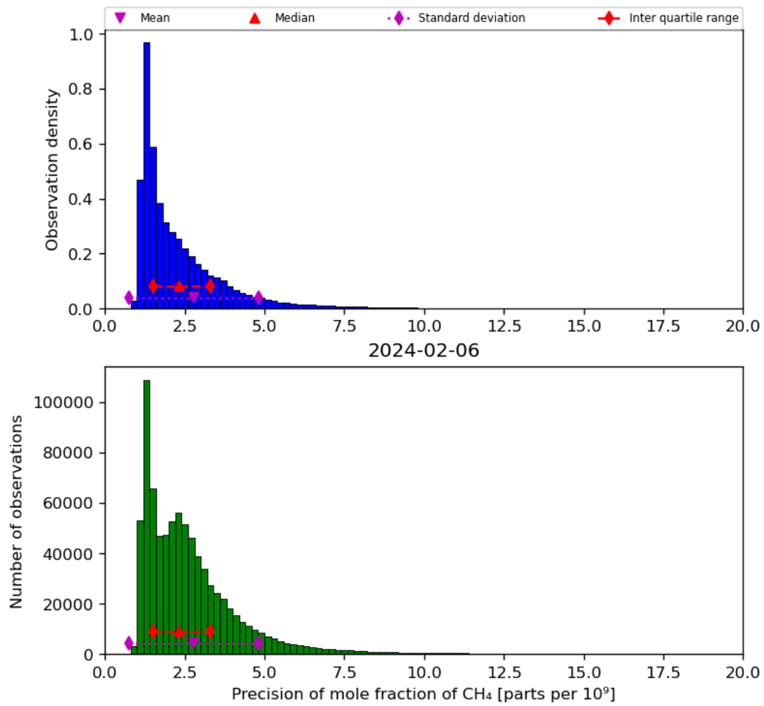
Figure 24: Histogram of “Precision of mole fraction of CH 4 ” for 2024-02-06 to 2024-02-07
