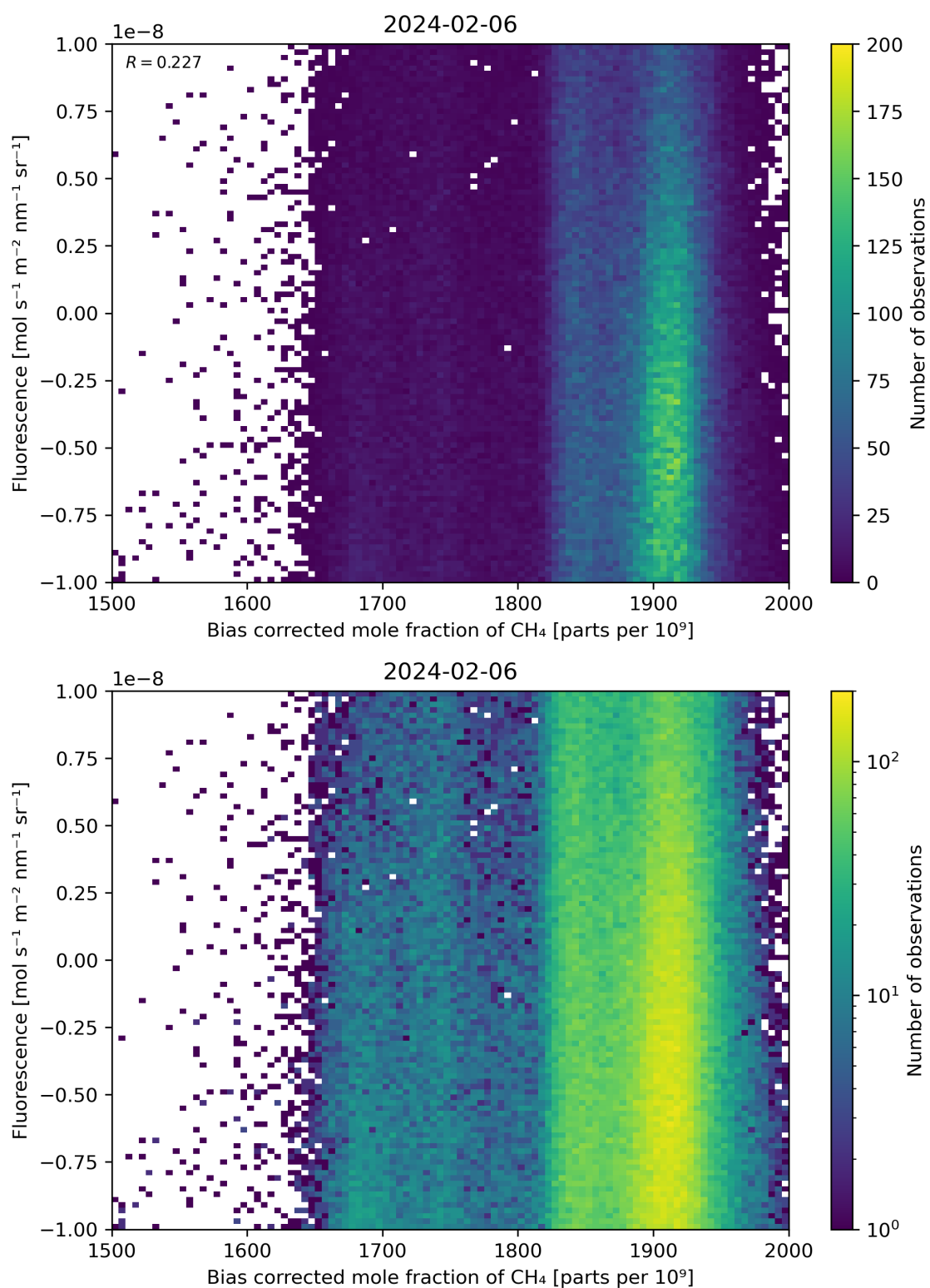
Figure 66: Scatter density plot of “Bias corrected mole fraction of \text{CH}_4 ” against “Fluorescence” for 2024-02-06 to 2024-02-07.
