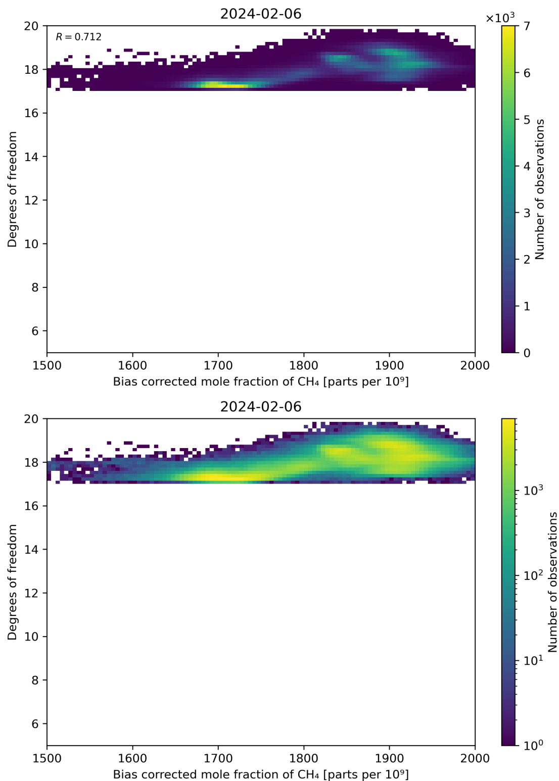
Figure 65: Scatter density plot of “Bias corrected mole fraction of CH 4 ” against “Degrees of freedom” for 2024-02-06 to 2024-02-07.
