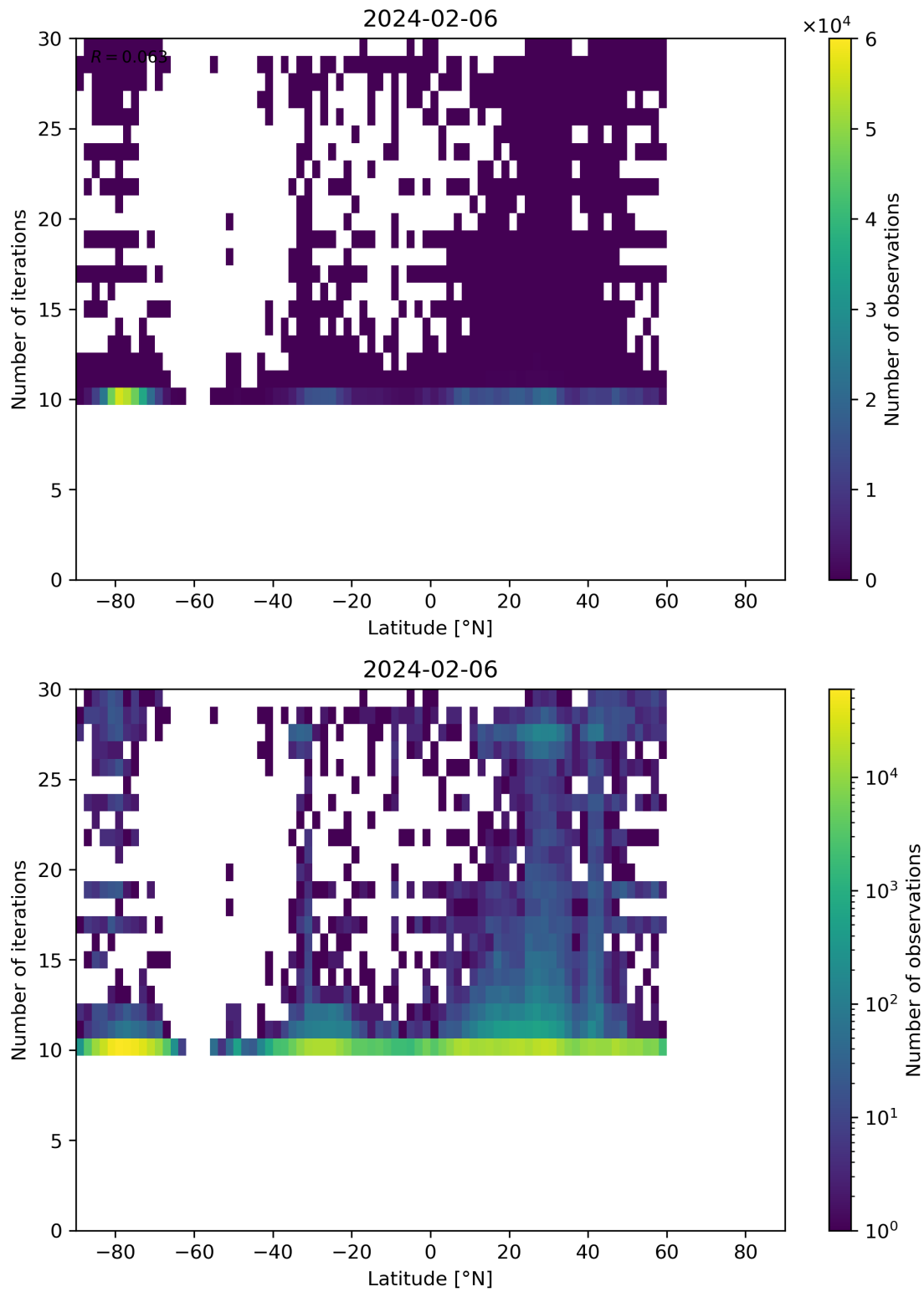
Figure 60: Scatter density plot of “Latitude” against “Number of iterations” for 2024-02-06 to 2024-02-07.
