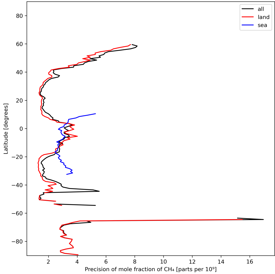
Figure 13: Zonal average of “Precision of mole fraction of CH 4 ” for 2024-02-06 to 2024-02-07.
