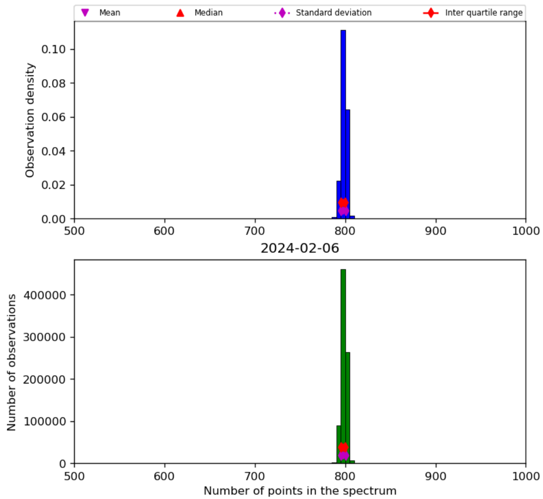
Figure 26: Histogram of “Number of points in the spectrum” for 2024-02-06 to 2024-02-07
