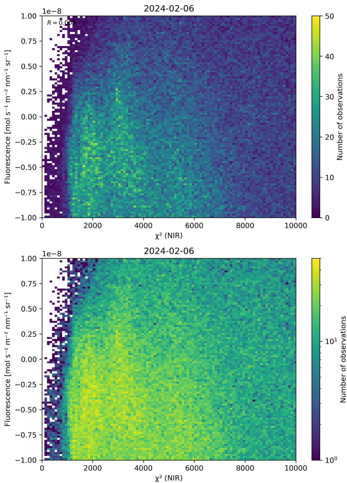
Figure 45: Scatter density plot of “ \chi^2 (NIR)” against “Fluorescence” for 2024-02-06 to 2024-02-07.
