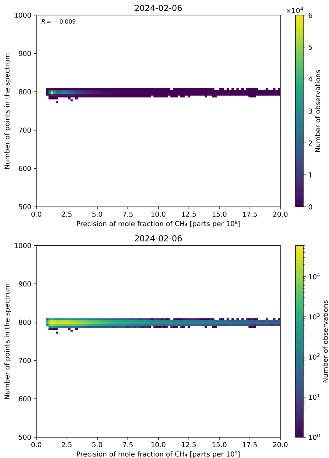
Figure 84: Scatter density plot of “Precision of mole fraction of CH 4 ” against “Number of points in the spectrum” for 2024-02-06 to 2024-02-07.
