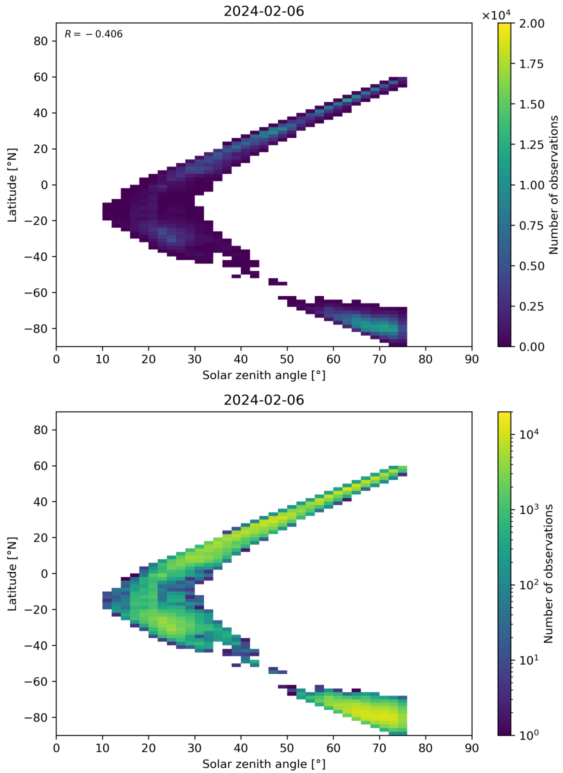
Figure 98: Scatter density plot of “Solar zenith angle” against “Latitude” for 2024-02-06 to 2024-02-07.
