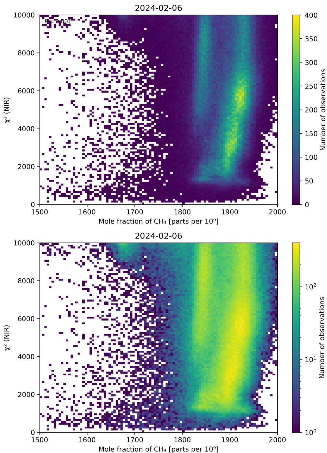
Figure 70: Scatter density plot of “Mole fraction of \text{CH}_4 ” against “ \chi^2 (NIR)” for 2024-02-06 to 2024-02-07.
