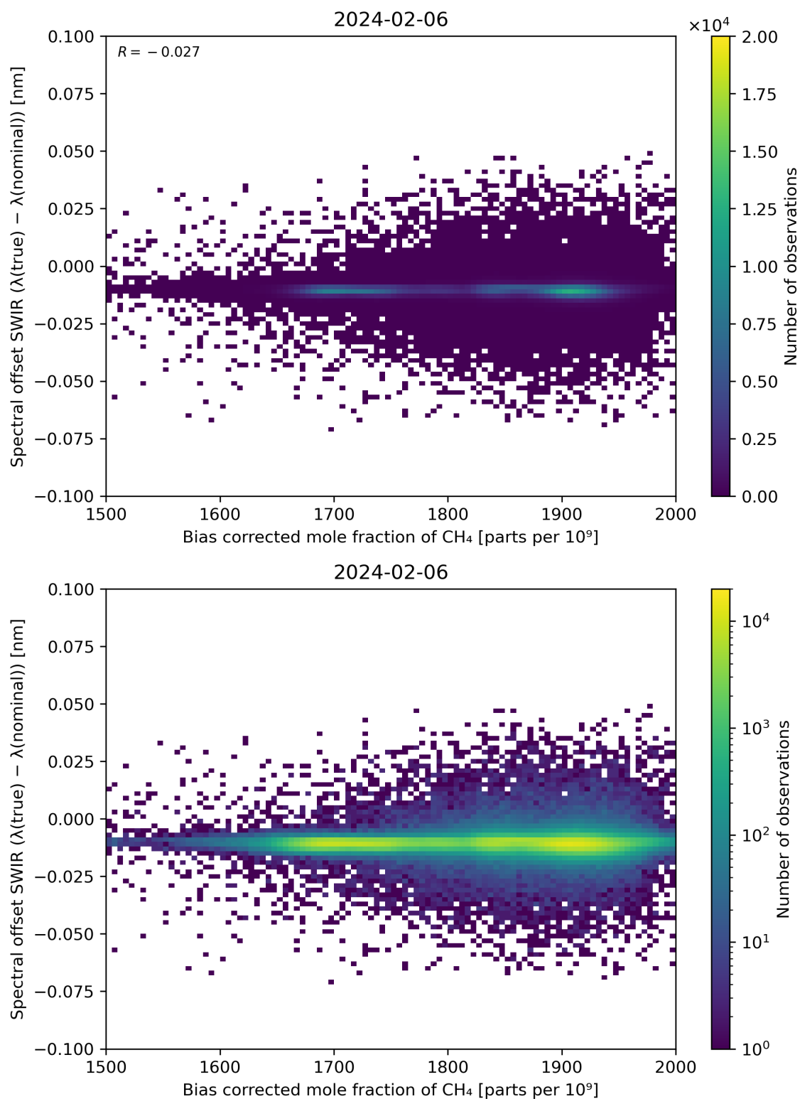
Figure 69: Scatter density plot of “Bias corrected mole fraction of \text{CH}_4 ” against “Spectral offset SWIR ( \lambda(\text{true}) - \lambda(\text{nominal}) )” for 2024-02-06 to 2024-02-07.
