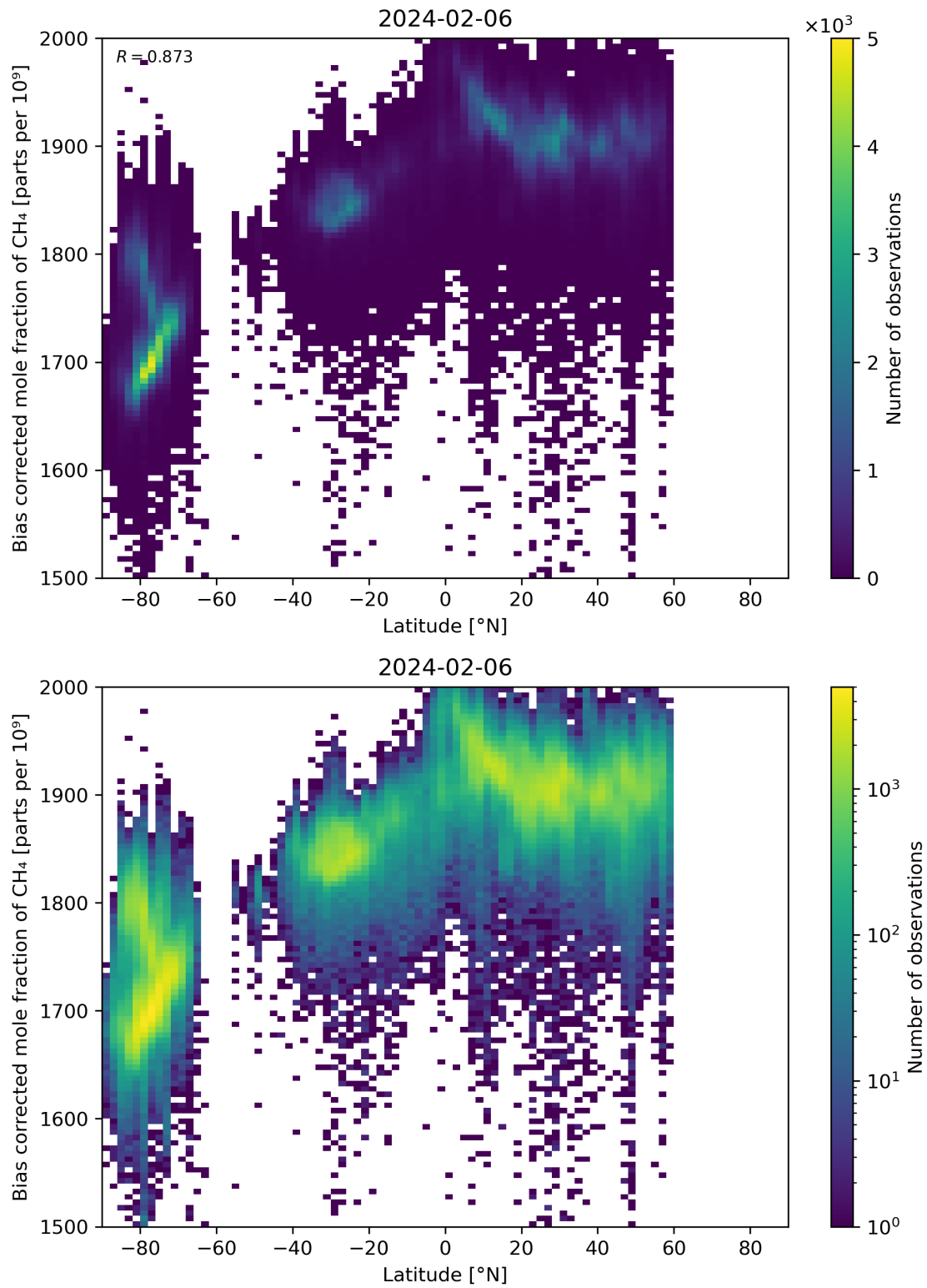
Figure 58: Scatter density plot of “Latitude” against “Bias corrected mole fraction of CH 4 ” for 2024-02-06 to 2024-02-07.
