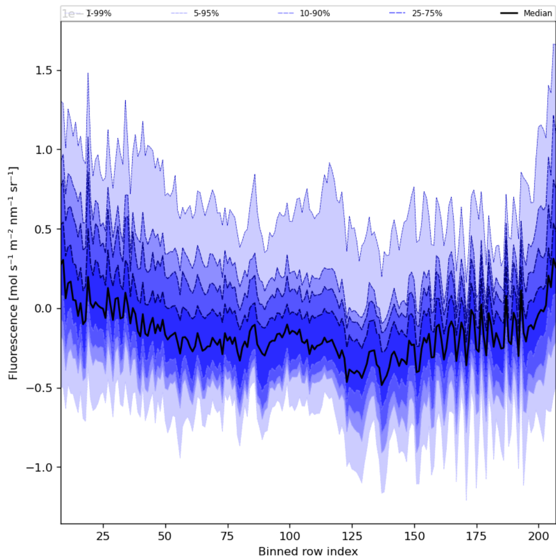
Figure 43: Along track statistics of “Fluorescence” for 2024-02-06 to 2024-02-07
