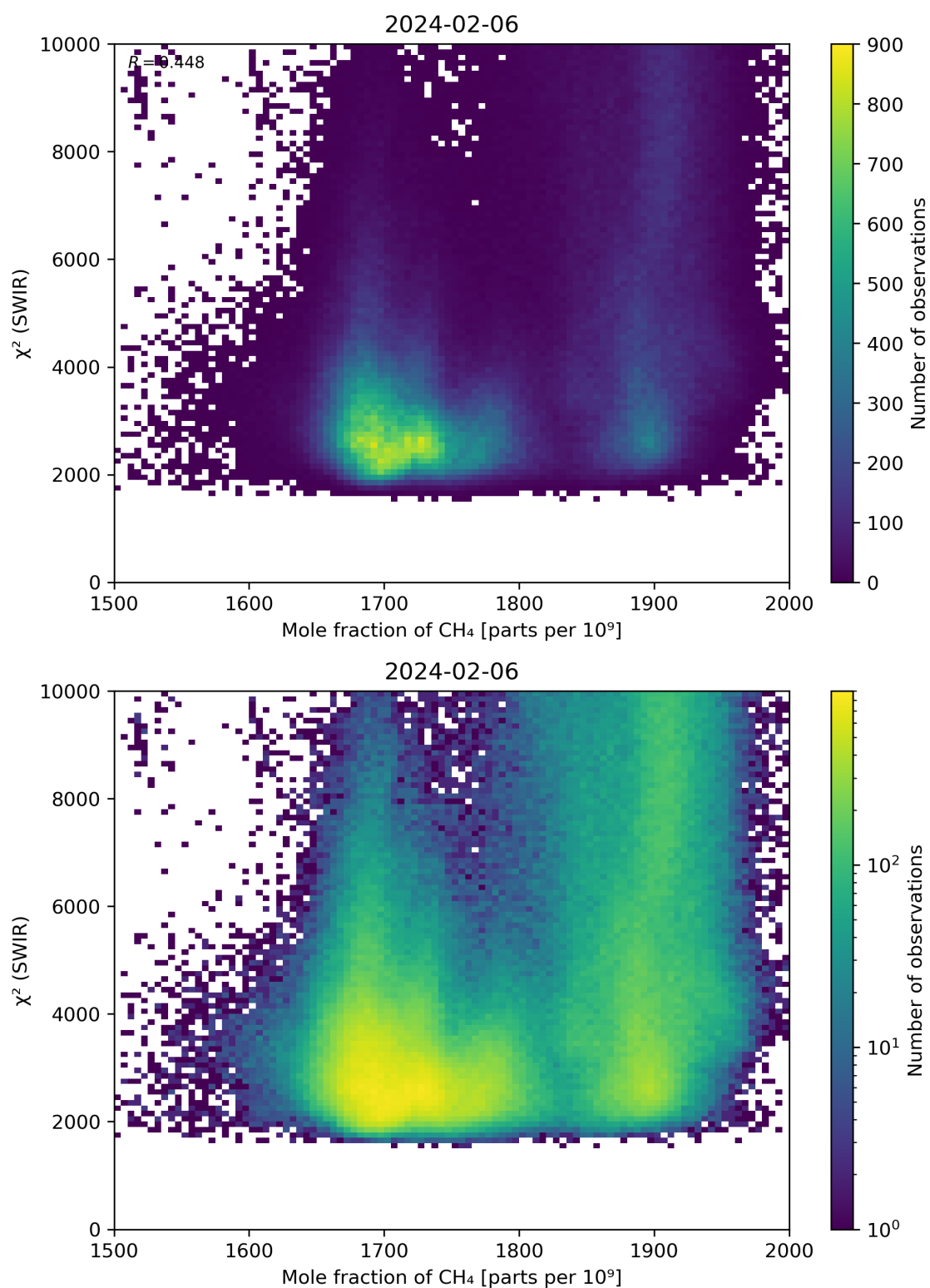
Figure 71: Scatter density plot of “Mole fraction of \text{CH}_4 ” against “ \chi^2 (SWIR)” for 2024-02-06 to 2024-02-07.
