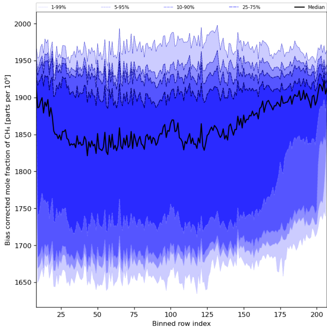
Figure 36: Along track statistics of “Bias corrected mole fraction of CH 4 ” for 2024-02-06 to 2024-02-07
