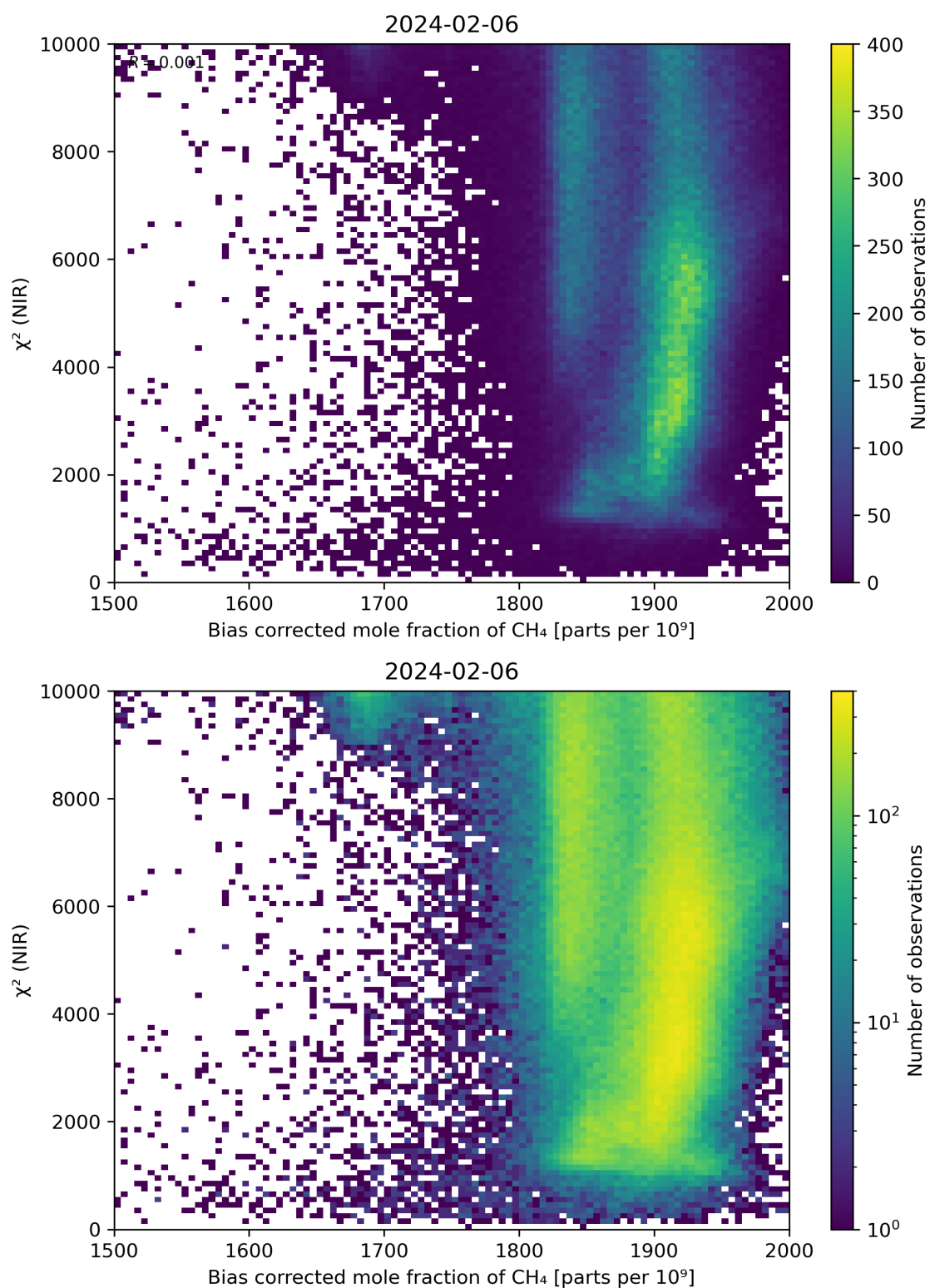
Figure 63: Scatter density plot of “Bias corrected mole fraction of CH 4 ” against “ \chi^2 (NIR)” for 2024-02-06 to 2024-02-07.
