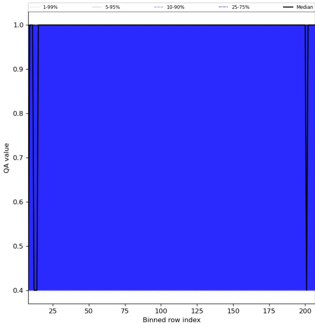
Figure 33: Along track statistics of “QA value” for 2024-02-06 to 2024-02-07
