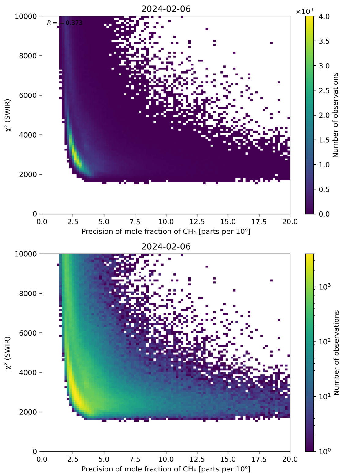
Figure 79: Scatter density plot of “Precision of mole fraction of \text{CH}_4 ” against “ \chi^2 (SWIR)” for 2024-02-06 to 2024-02-07.
