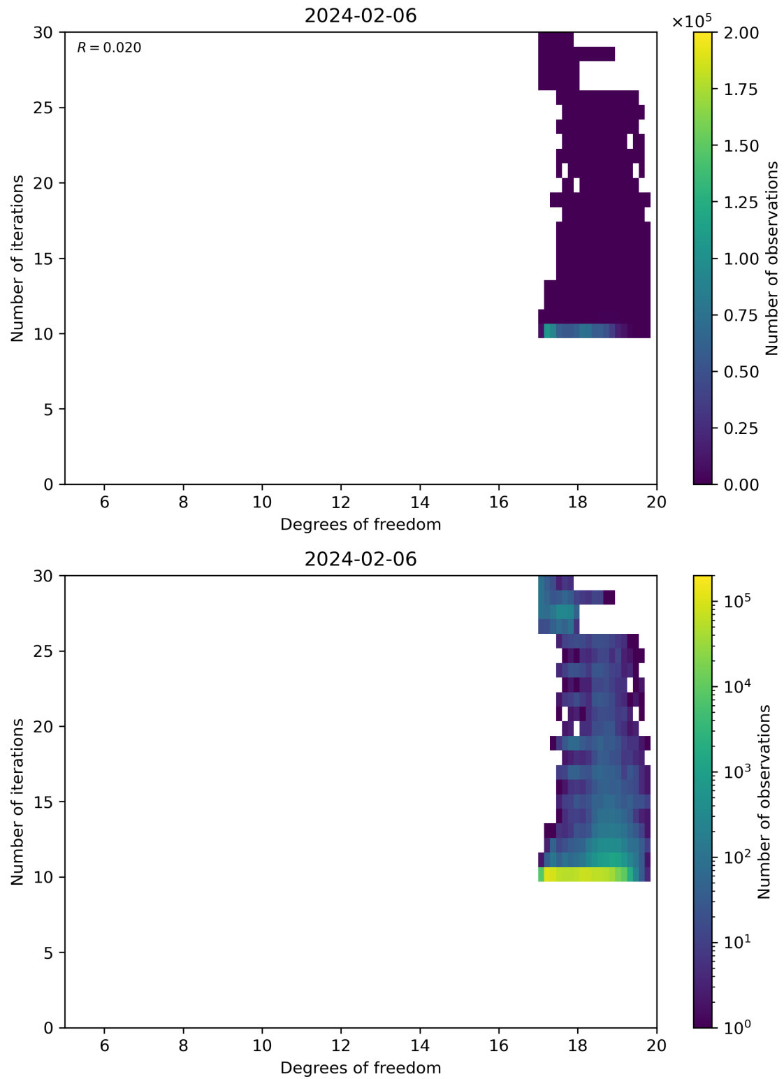
Figure 52: Scatter density plot of “Degrees of freedom” against “Number of iterations” for 2024-02-06 to 2024-02-07.
