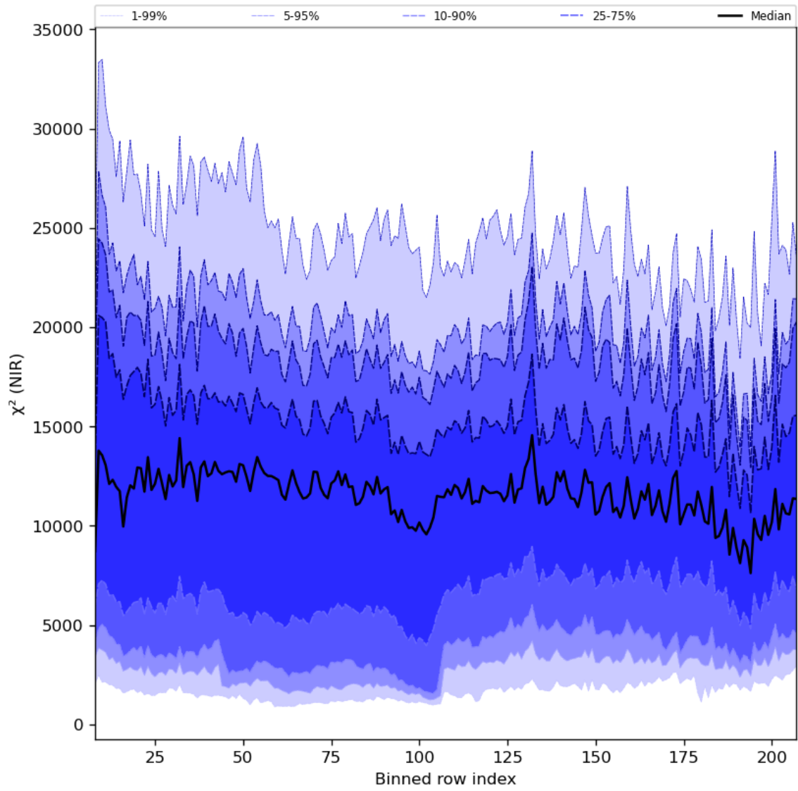
Figure 40: Along track statistics of " \chi^2 (NIR)" for 2024-02-06 to 2024-02-07
