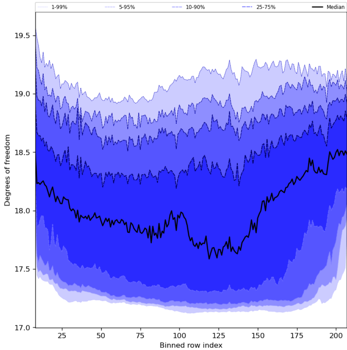
Figure 41: Along track statistics of “Degrees of freedom” for 2024-02-06 to 2024-02-07
