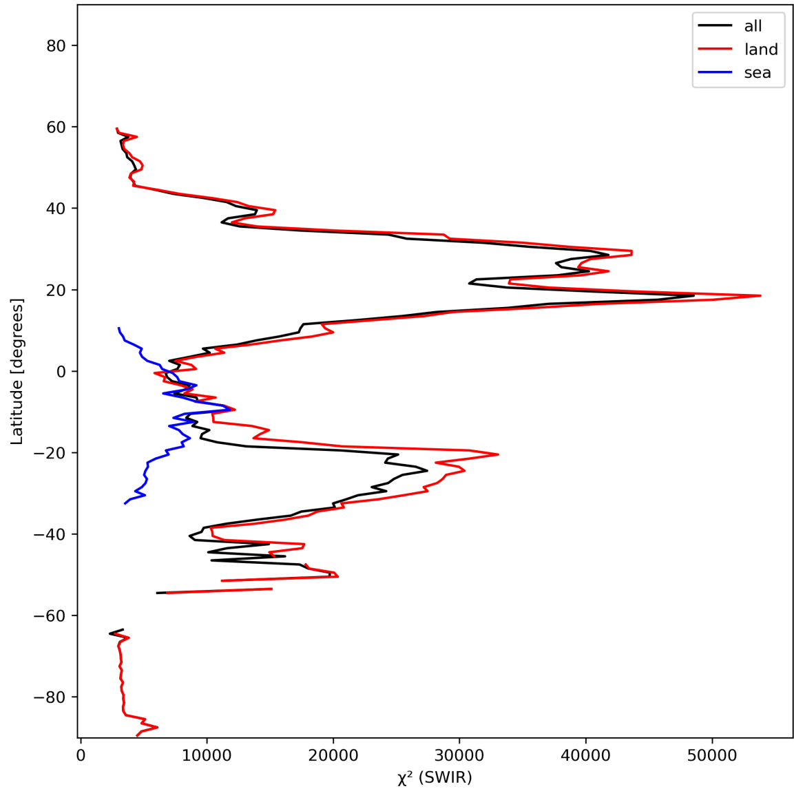
Figure 17: Zonal average of “ \chi^2 (SWIR)” for 2024-02-06 to 2024-02-07.
