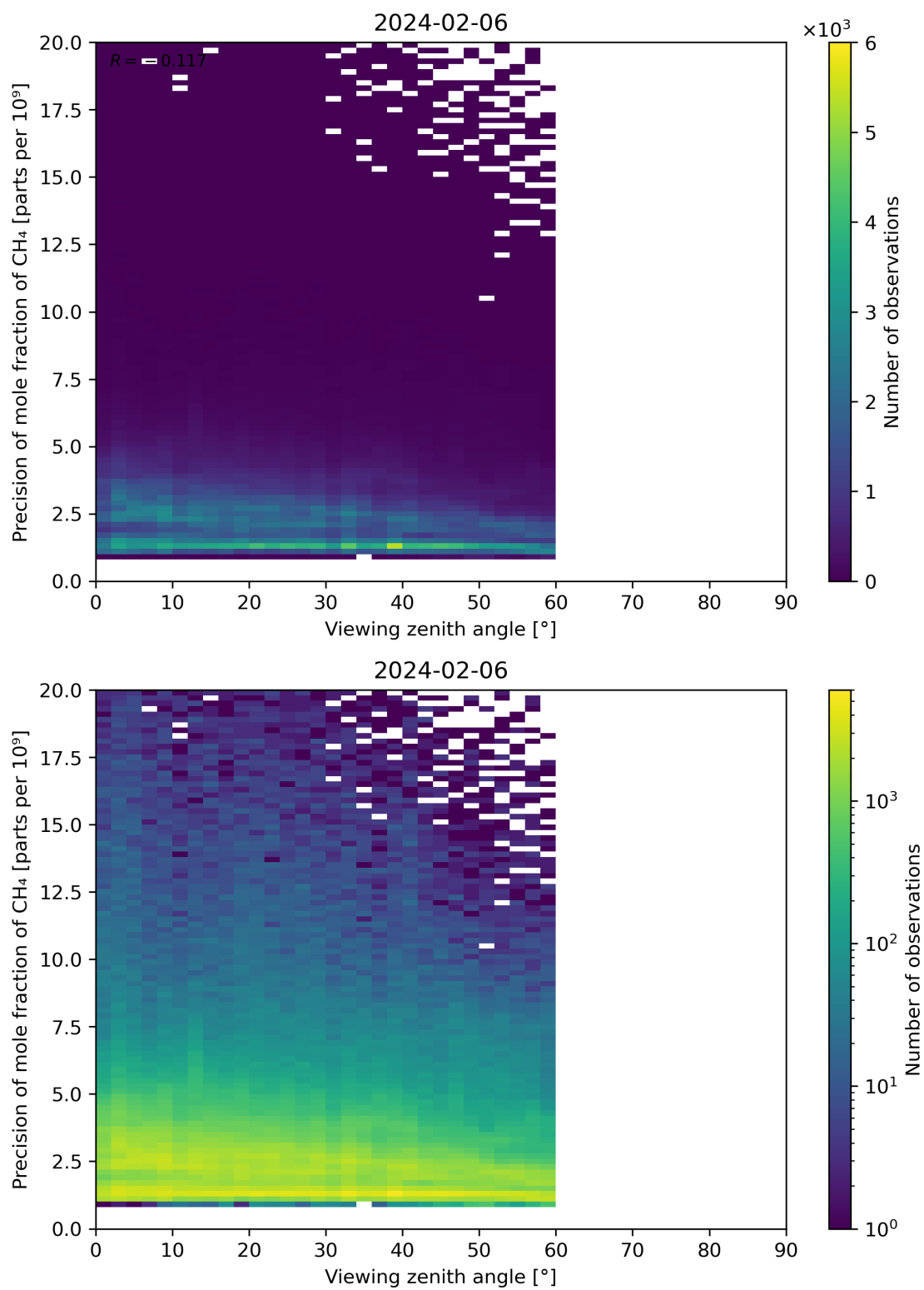
Figure 112: Scatter density plot of “Viewing zenith angle” against “Precision of mole fraction of CH 4 ” for 2024-02-06 to 2024-02-07.
