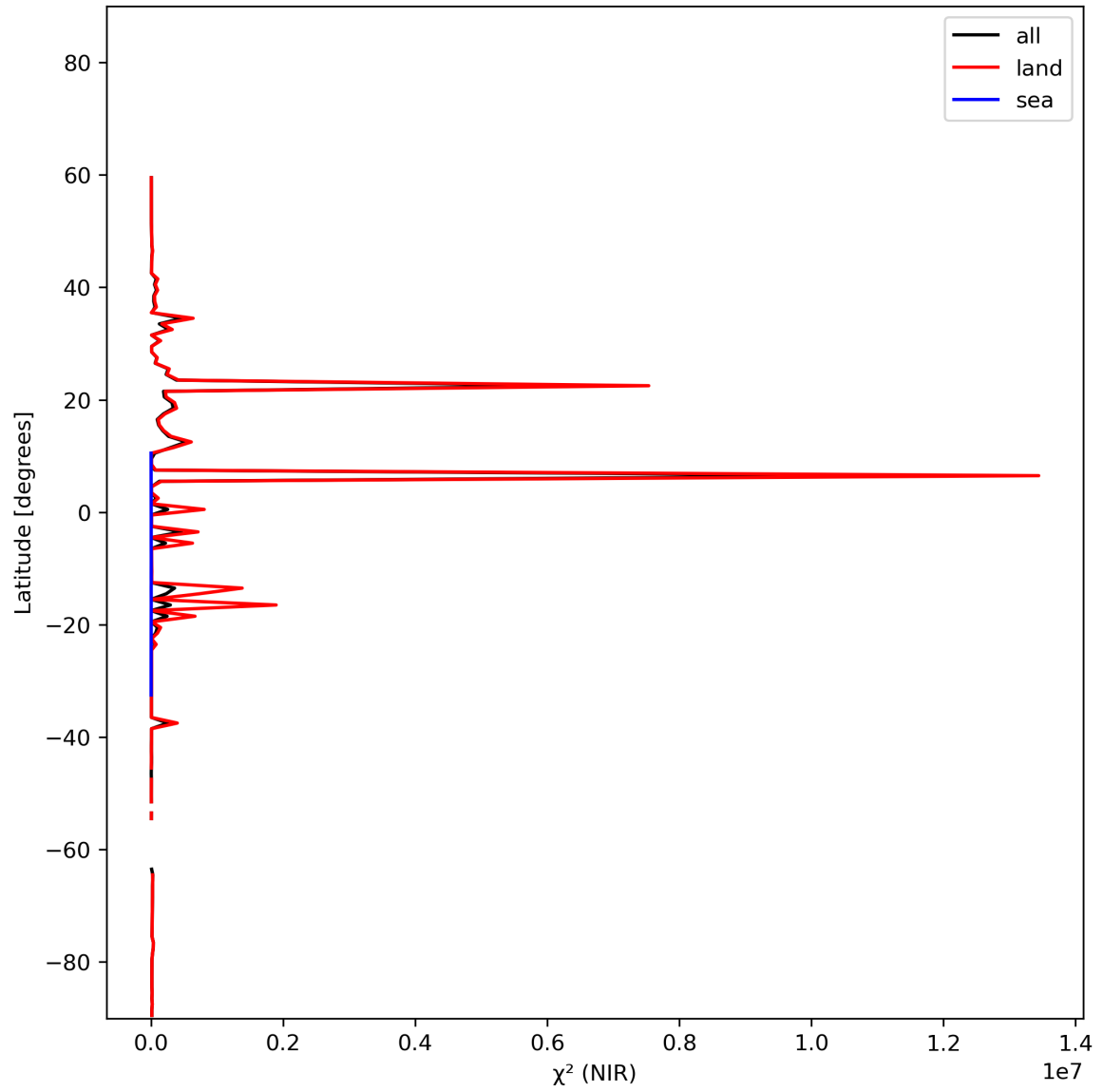
Figure 18: Zonal average of “ \chi^2 (NIR)” for 2024-02-06 to 2024-02-07.
