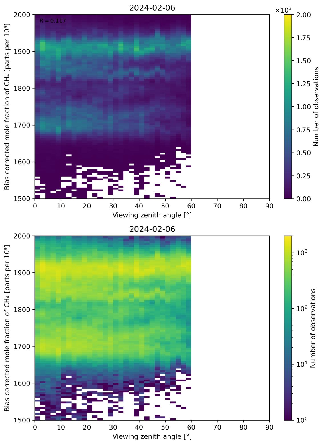
Figure 111: Scatter density plot of “Viewing zenith angle” against “Bias corrected mole fraction of CH 4 ” for 2024-02-06 to 2024-02-07.
