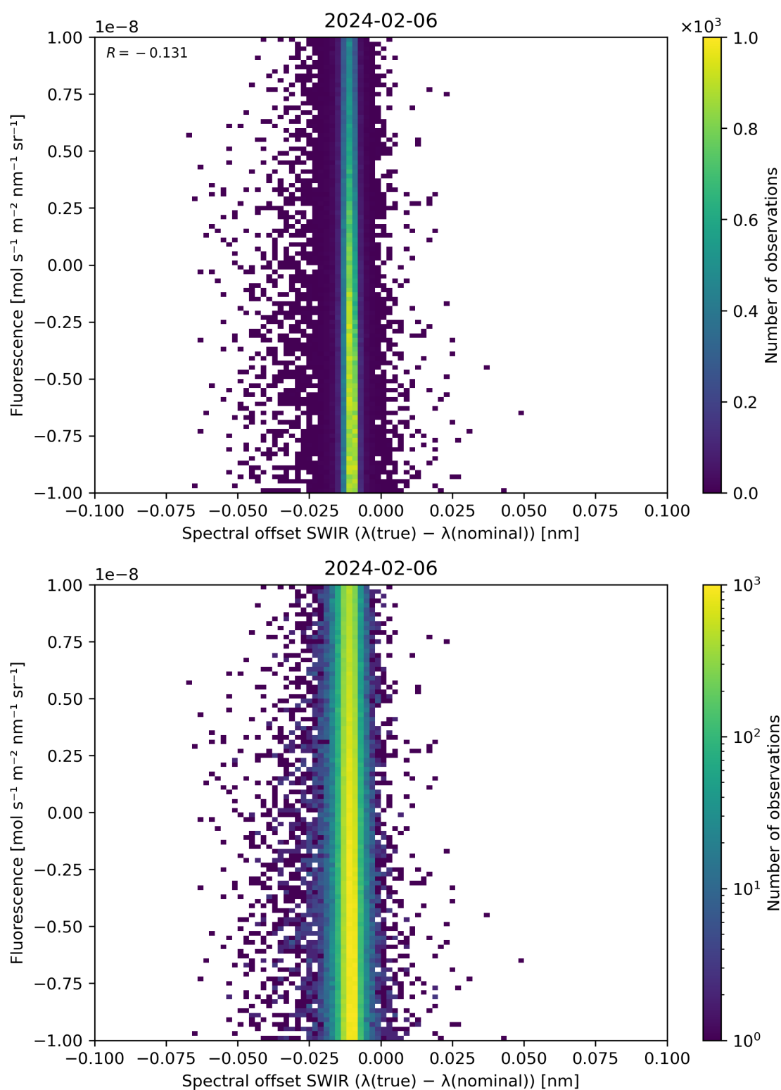
Figure 120: Scatter density plot of “Spectral offset SWIR ( \lambda(\text{true}) - \lambda(\text{nominal}) )” against “Fluorescence” for 2024-02-06 to 2024-02-07.
