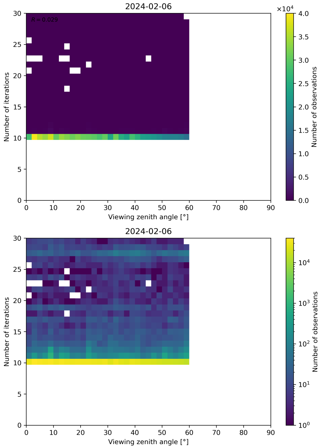
Figure 113: Scatter density plot of “Viewing zenith angle” against “Number of iterations” for 2024-02-06 to 2024-02-07.
