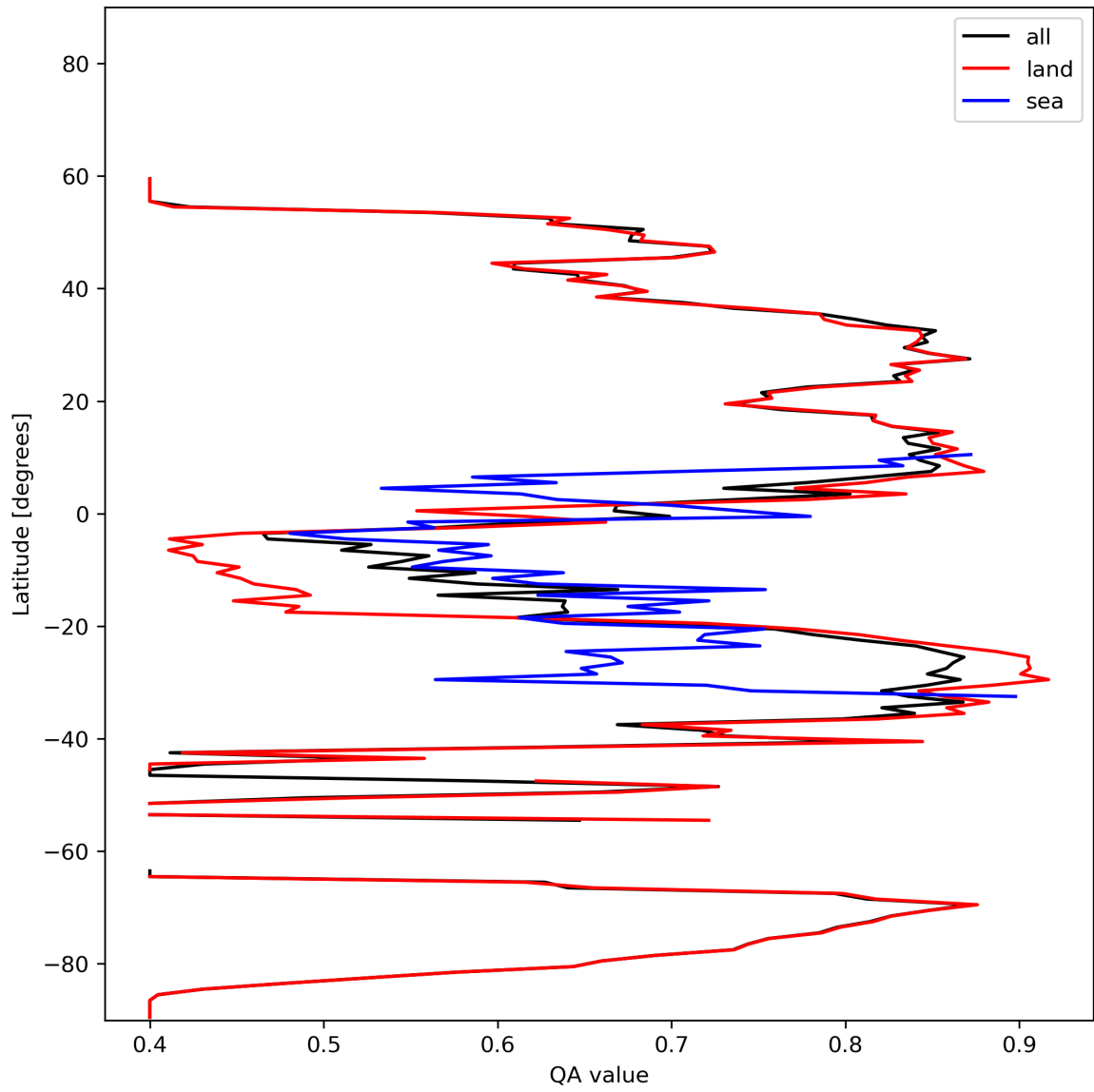
Figure 11: Zonal average of “QA value” for 2024-02-06 to 2024-02-07.
