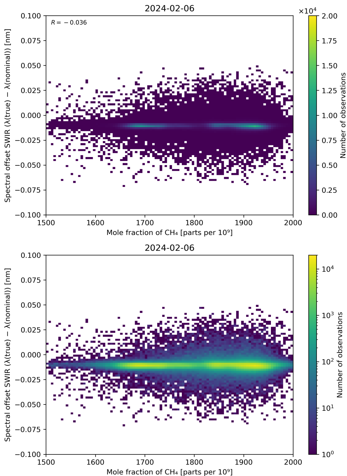
Figure 86: Scatter density plot of “Mole fraction of CH 4 ” against “Spectral offset SWIR ( \lambda(\text{true}) - \lambda(\text{nominal}) )” for 2024-02-06 to 2024-02-07.
