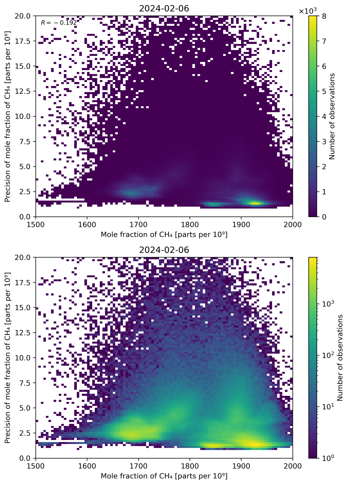
Figure 75: Scatter density plot of “Mole fraction of CH 4 ” against “Precision of mole fraction of CH 4 ” for 2024-02-06 to 2024-02-07.
