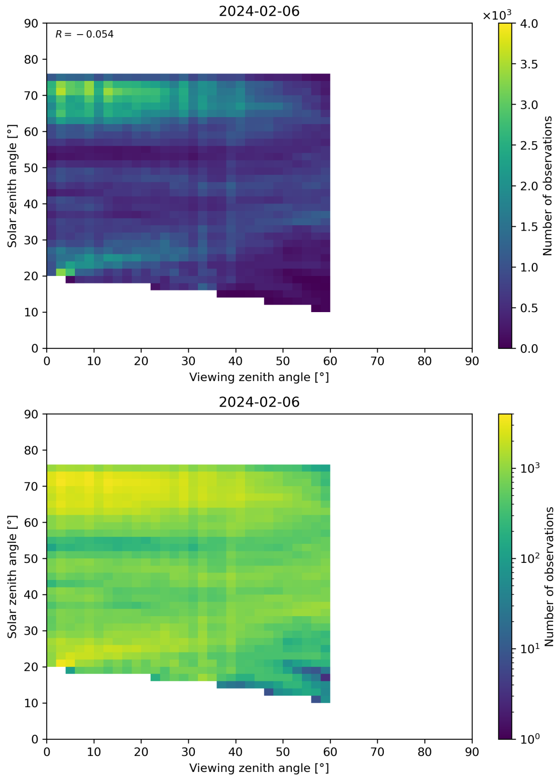
Figure 115: Scatter density plot of “Viewing zenith angle” against “Solar zenith angle” for 2024-02-06 to 2024-02-07.
