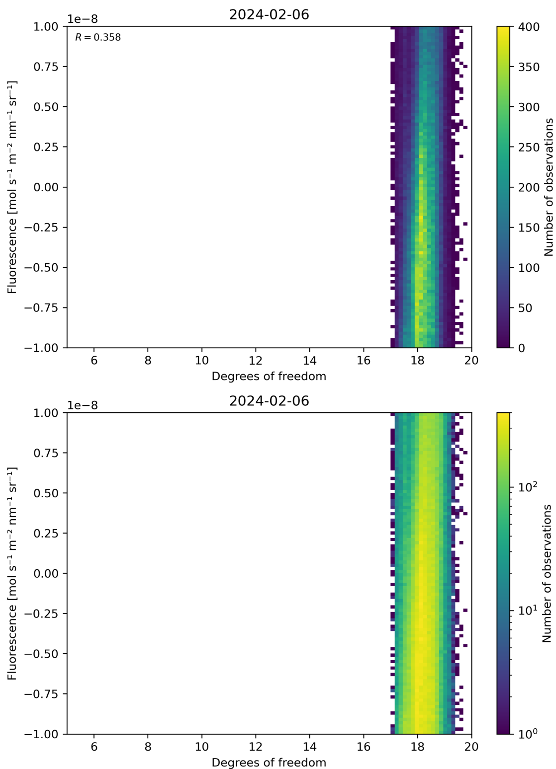
Figure 51: Scatter density plot of “Degrees of freedom” against “Fluorescence” for 2024-02-06 to 2024-02-07.
