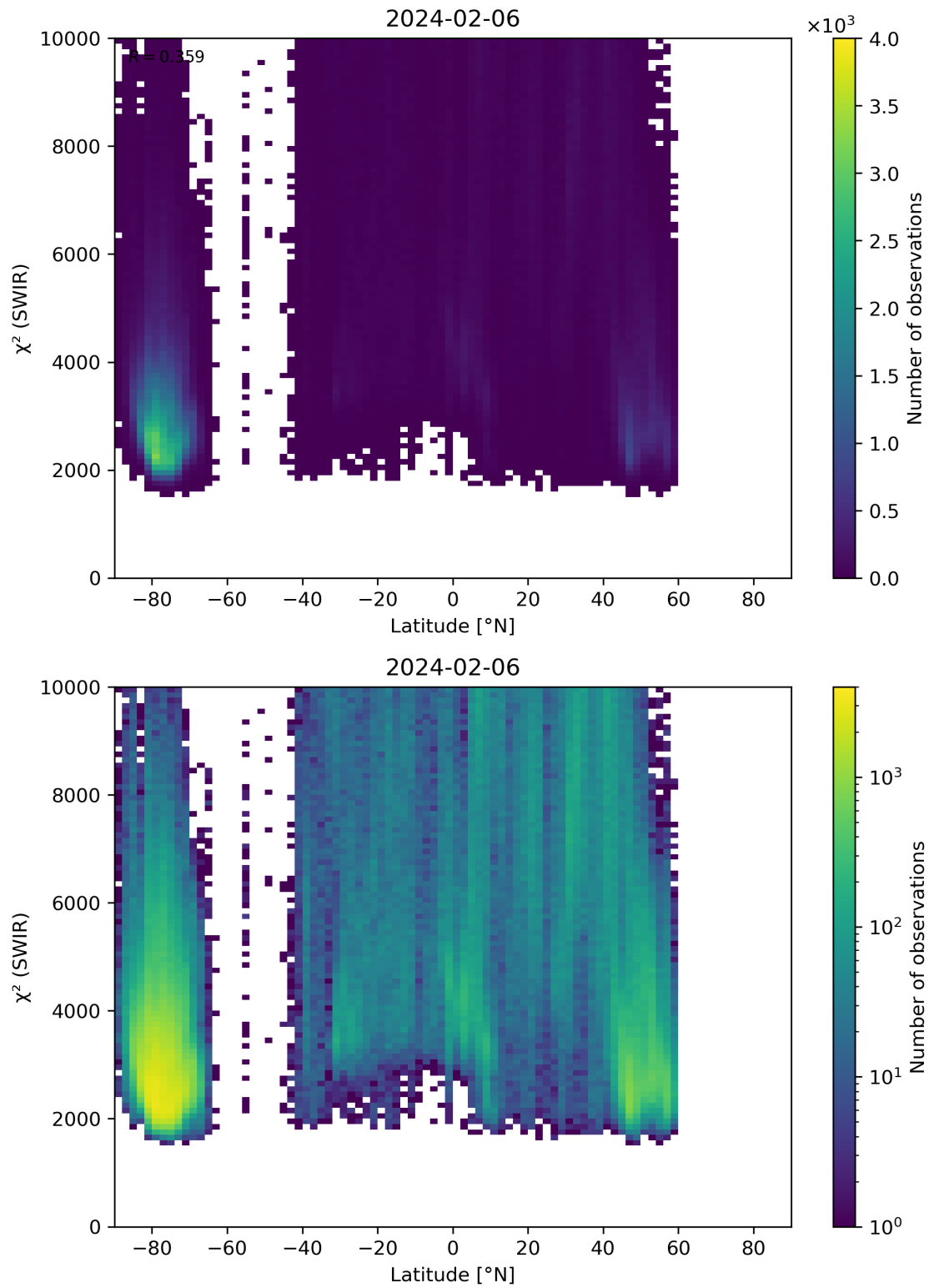
Figure 54: Scatter density plot of “Latitude” against “ \chi^2 (SWIR)” for 2024-02-06 to 2024-02-07.
