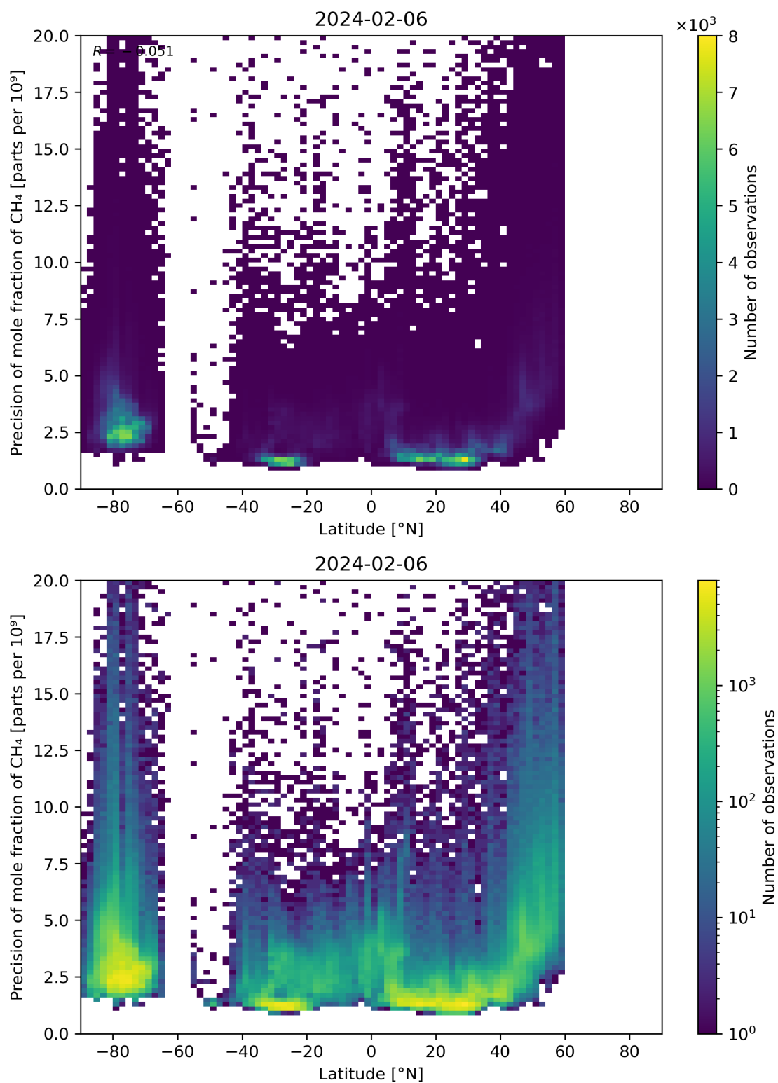
Figure 59: Scatter density plot of “Latitude” against “Precision of mole fraction of CH 4 ” for 2024-02-06 to 2024-02-07.
