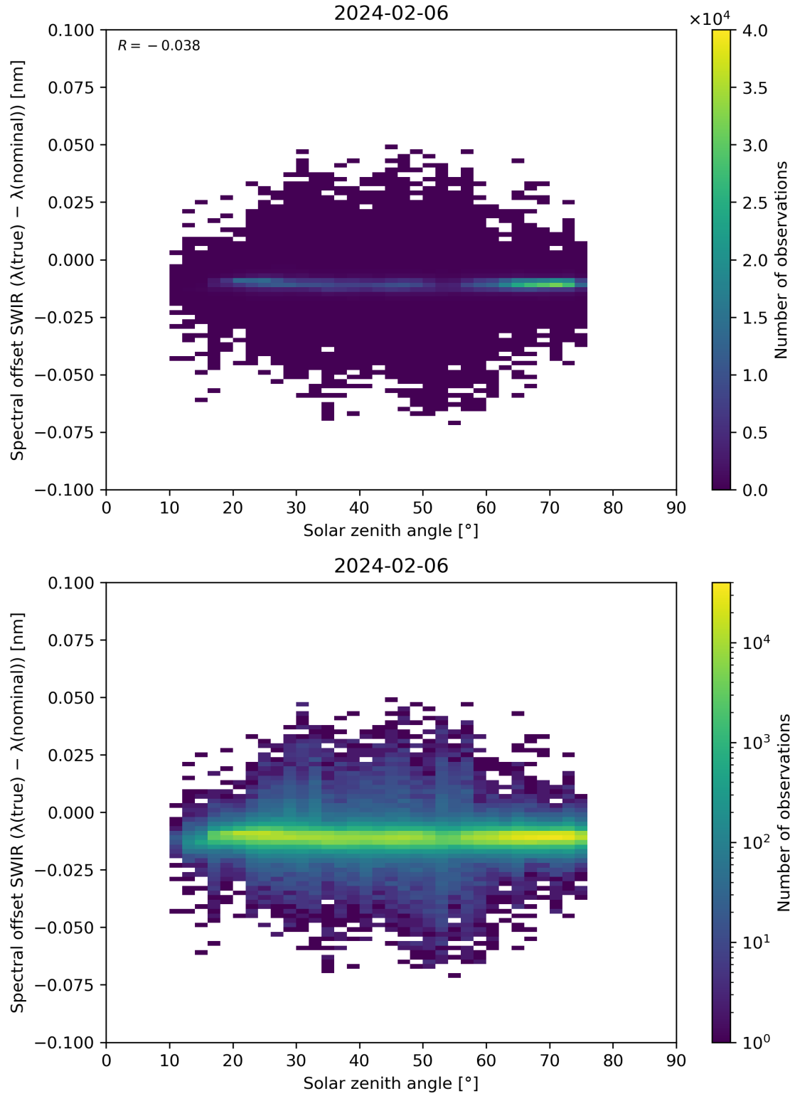
Figure 104: Scatter density plot of “Solar zenith angle” against “Spectral offset SWIR ( \lambda(\text{true}) - \lambda(\text{nominal}) )” for 2024-02-06 to 2024-02-07.
