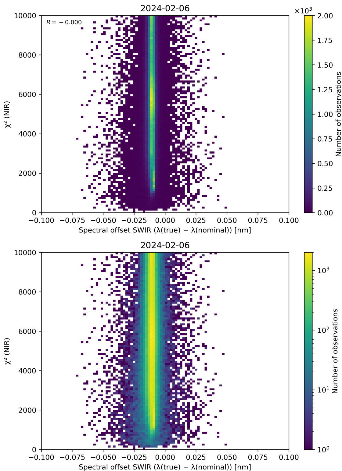
Figure 117: Scatter density plot of “Spectral offset SWIR ( \lambda(\text{true}) - \lambda(\text{nominal}) )” against “ \chi^2 (NIR)” for 2024-02-06 to 2024-02-07.
