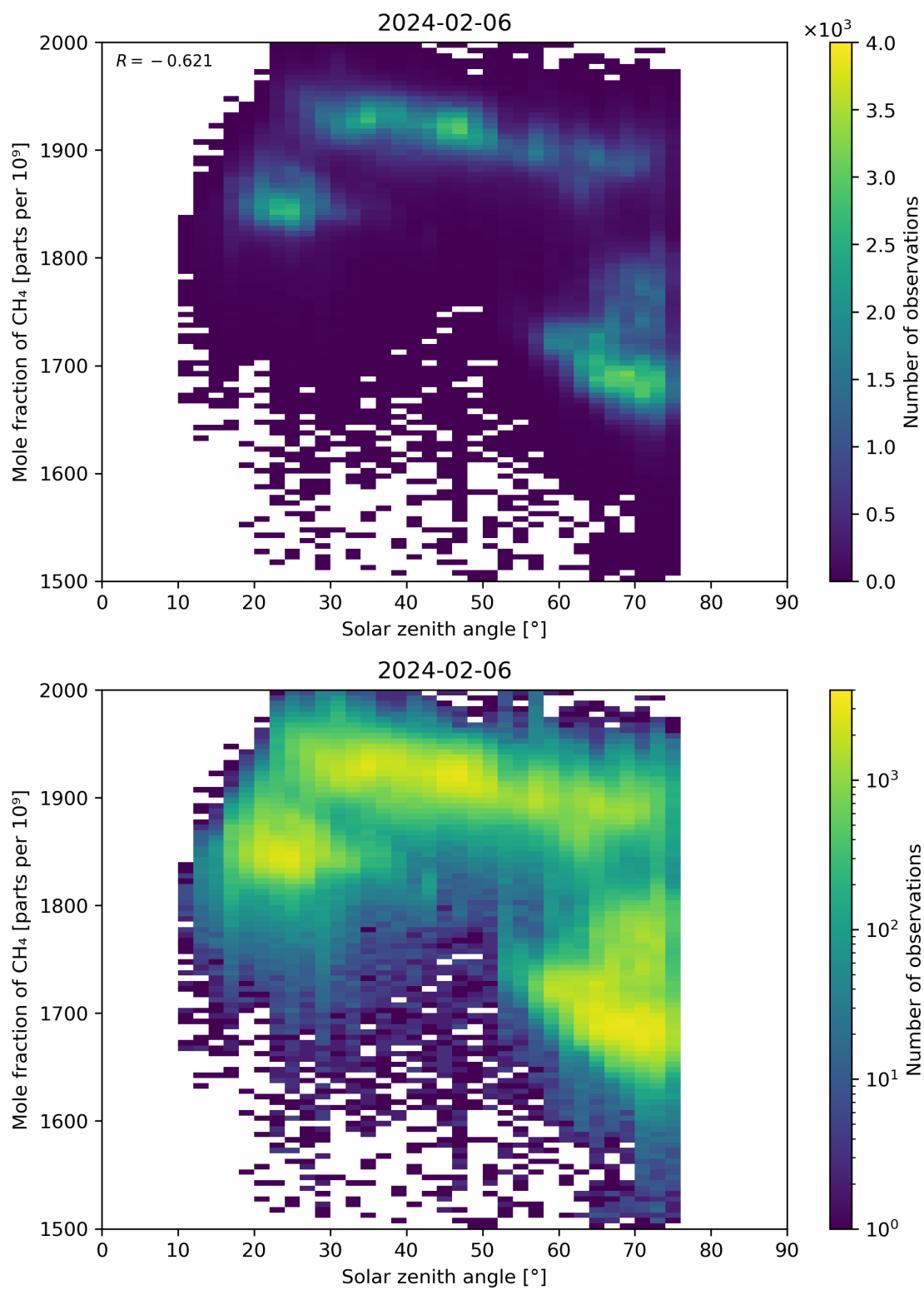
Figure 99: Scatter density plot of “Solar zenith angle” against “Mole fraction of CH 4 ” for 2024-02-06 to 2024-02-07.
