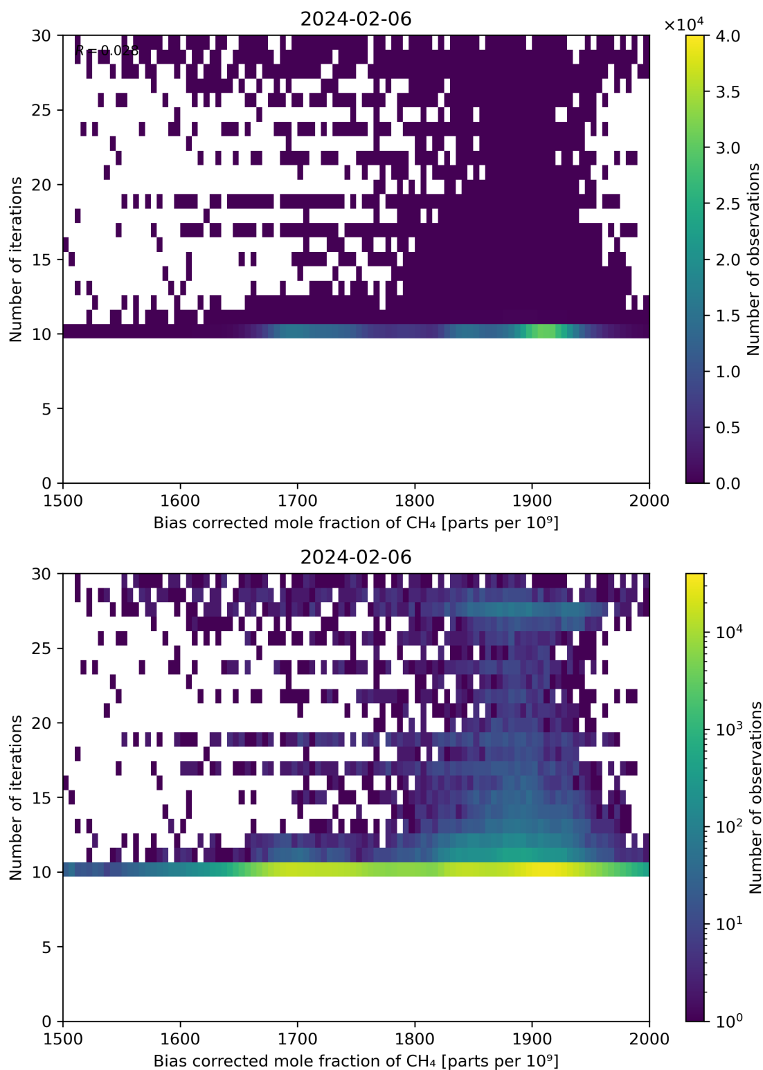
Figure 67: Scatter density plot of “Bias corrected mole fraction of \text{CH}_4 ” against “Number of iterations” for 2024-02-06 to 2024-02-07.
