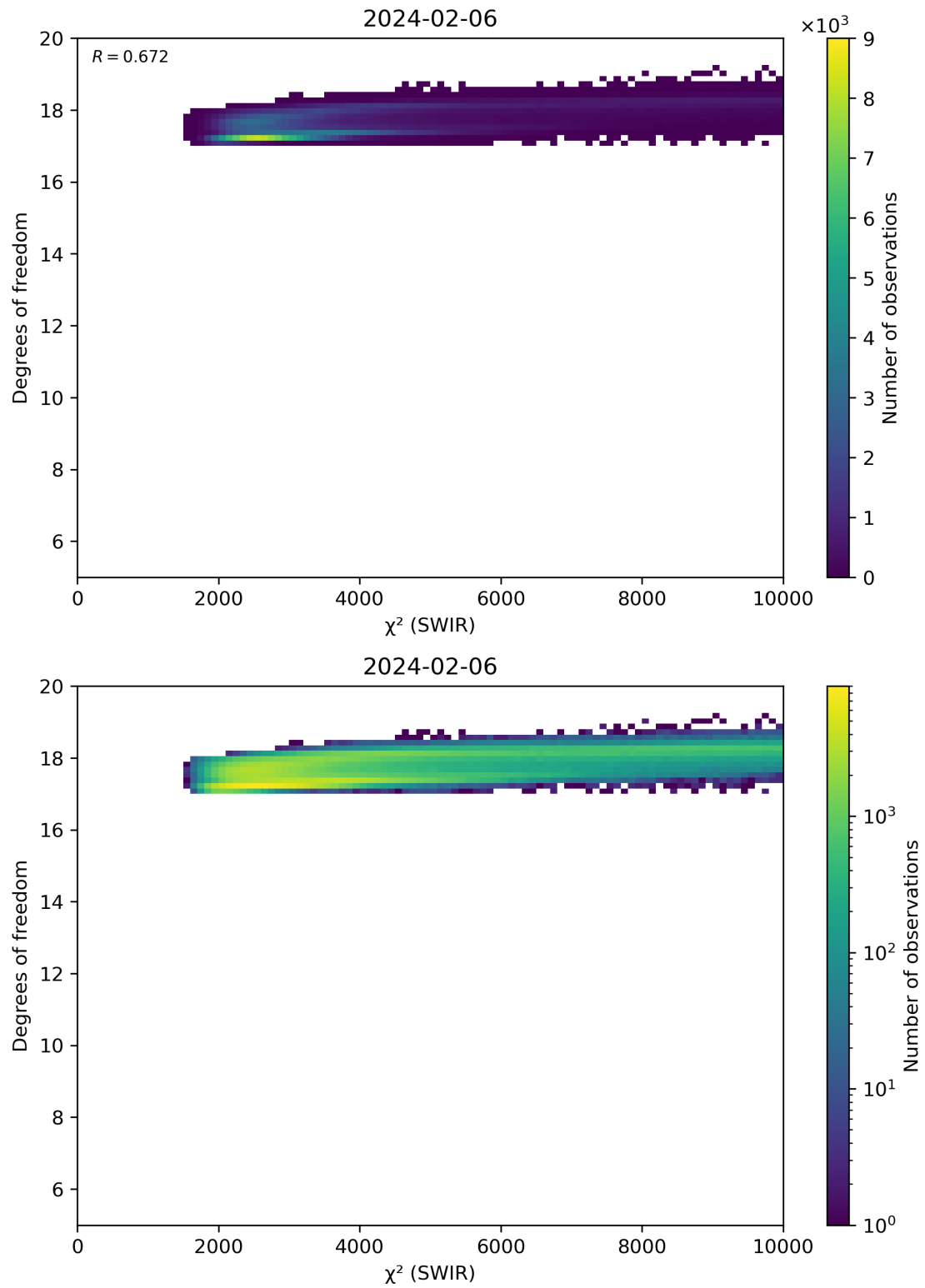
Figure 48: Scatter density plot of “ \chi^2 (SWIR)” against “Degrees of freedom” for 2024-02-06 to 2024-02-07.
