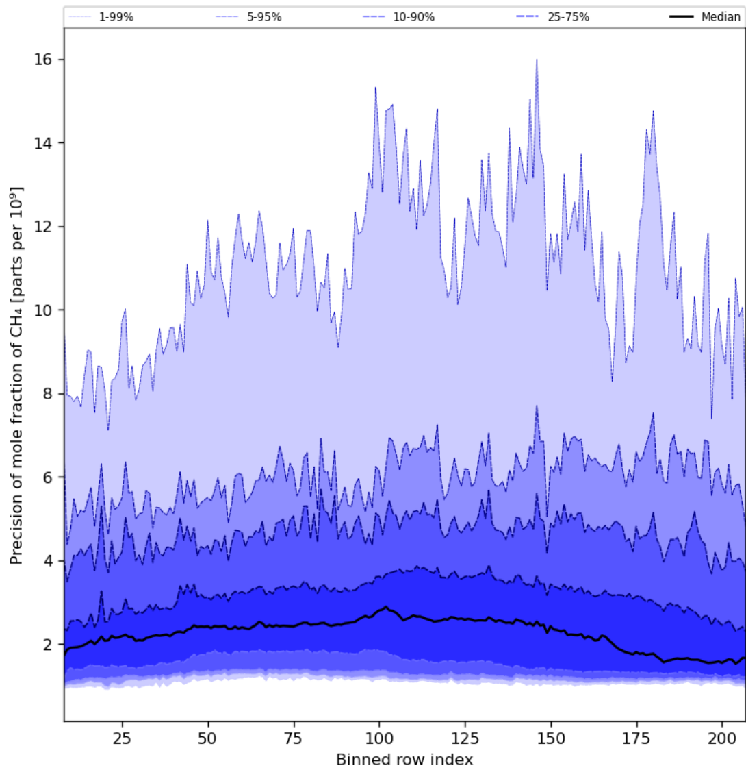
Figure 35: Along track statistics of “Precision of mole fraction of CH 4 ” for 2024-02-06 to 2024-02-07
