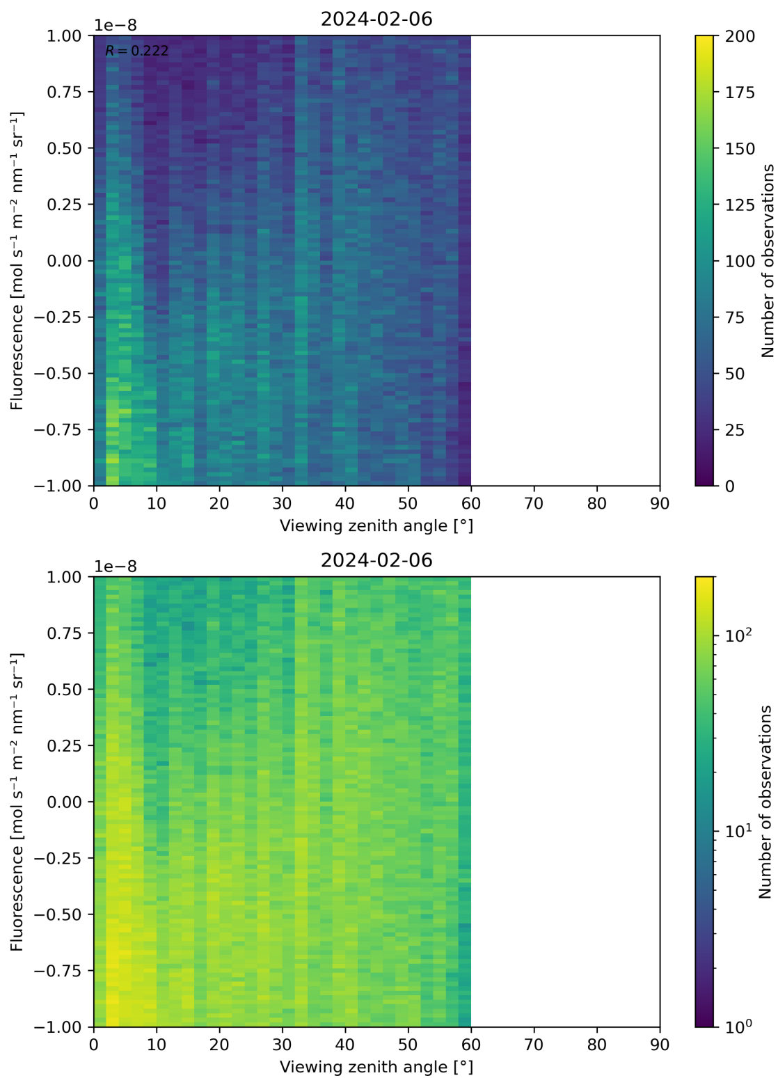
Figure 108: Scatter density plot of “Viewing zenith angle” against “Fluorescence” for 2024-02-06 to 2024-02-07.
