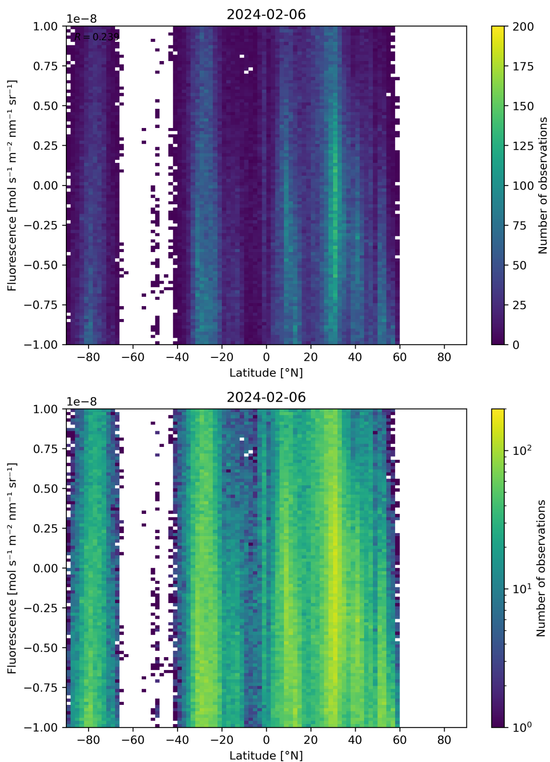
Figure 56: Scatter density plot of “Latitude” against “Fluorescence” for 2024-02-06 to 2024-02-07.
