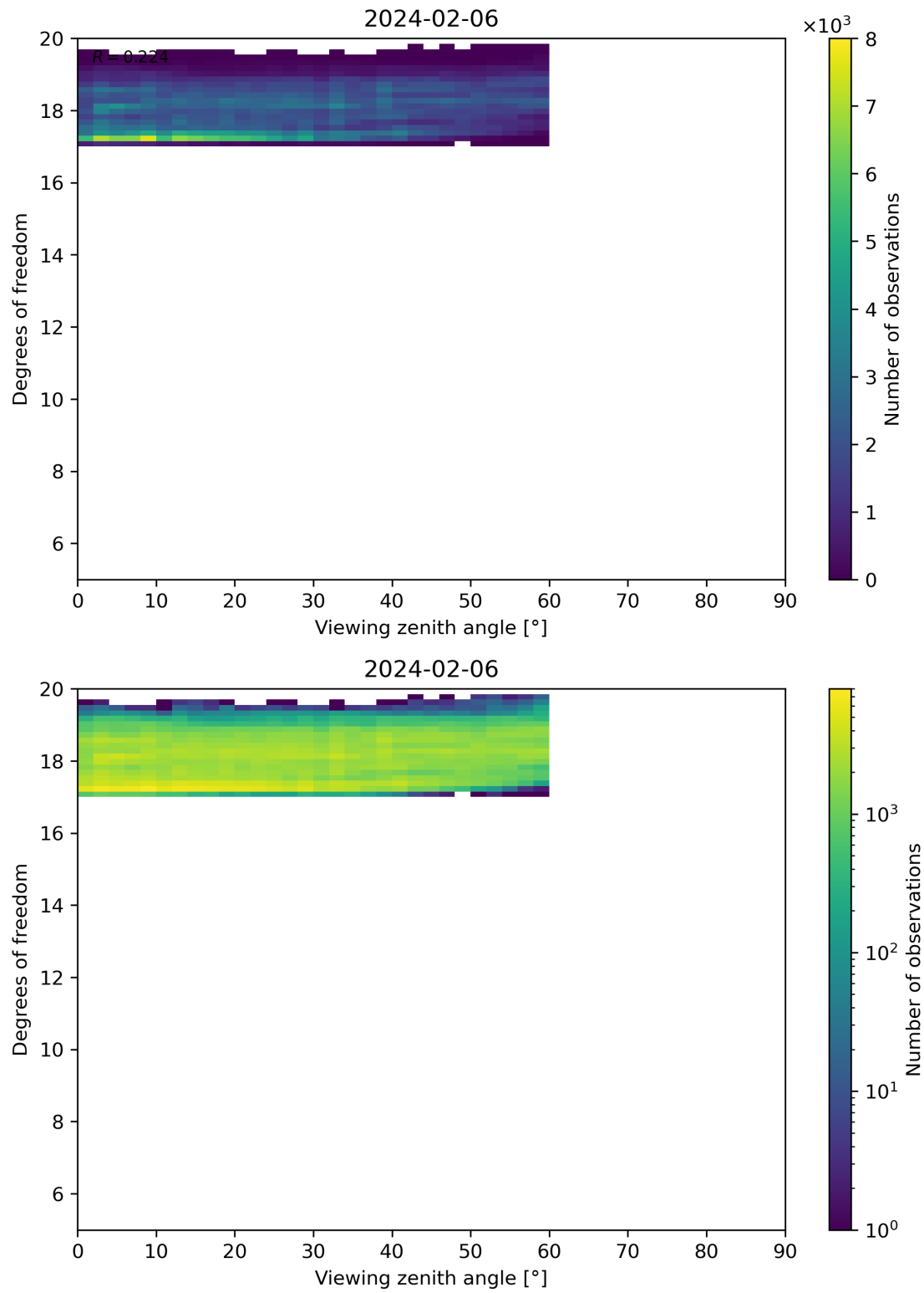
Figure 107: Scatter density plot of “Viewing zenith angle” against “Degrees of freedom” for 2024-02-06 to 2024-02-07.
