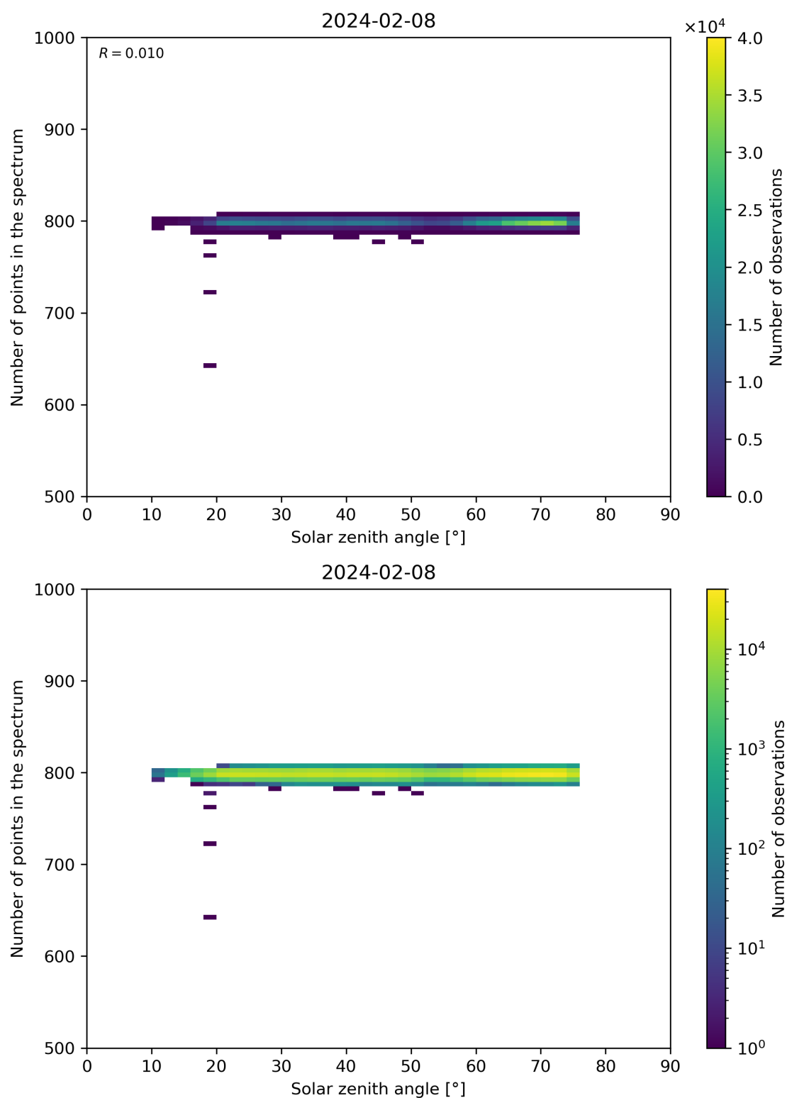
Figure 103: Scatter density plot of “Solar zenith angle” against “Number of points in the spectrum” for 2024-02-07 to 2024-02-09.
