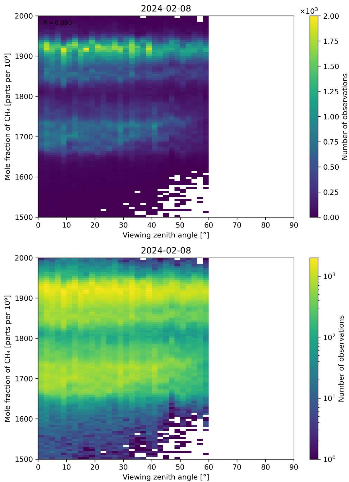
Figure 110: Scatter density plot of “Viewing zenith angle” against “Mole fraction of CH 4 ” for 2024-02-07 to 2024-02-09.
