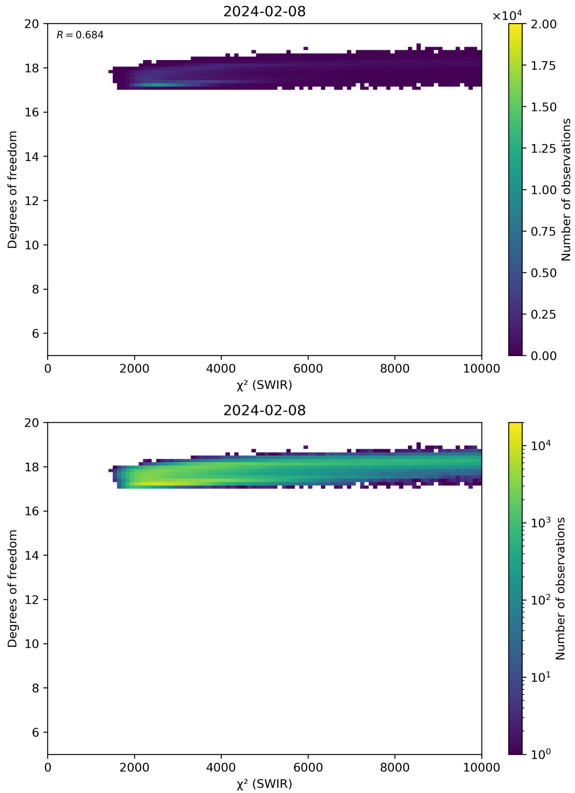
Figure 48: Scatter density plot of “ \chi^2 (SWIR)” against “Degrees of freedom” for 2024-02-07 to 2024-02-09.
