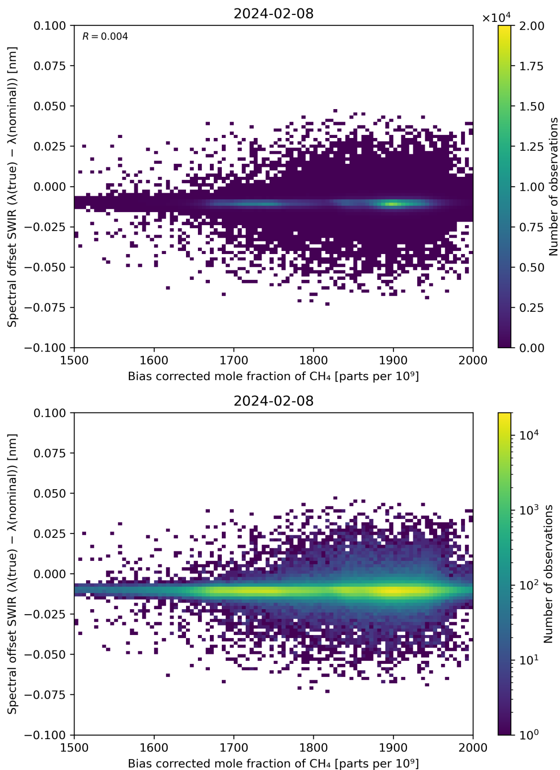
Figure 69: Scatter density plot of “Bias corrected mole fraction of \text{CH}_4 ” against “Spectral offset SWIR ( \lambda(\text{true}) - \lambda(\text{nominal}) )” for 2024-02-07 to 2024-02-09.
