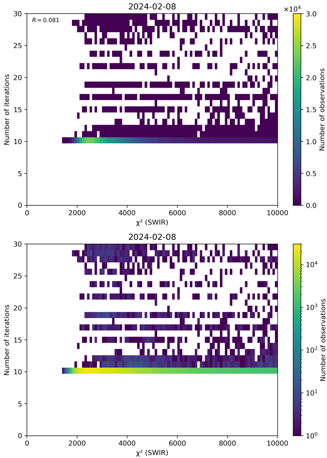
Figure 50: Scatter density plot of “ \chi^2 (SWIR)” against “Number of iterations” for 2024-02-07 to 2024-02-09.
