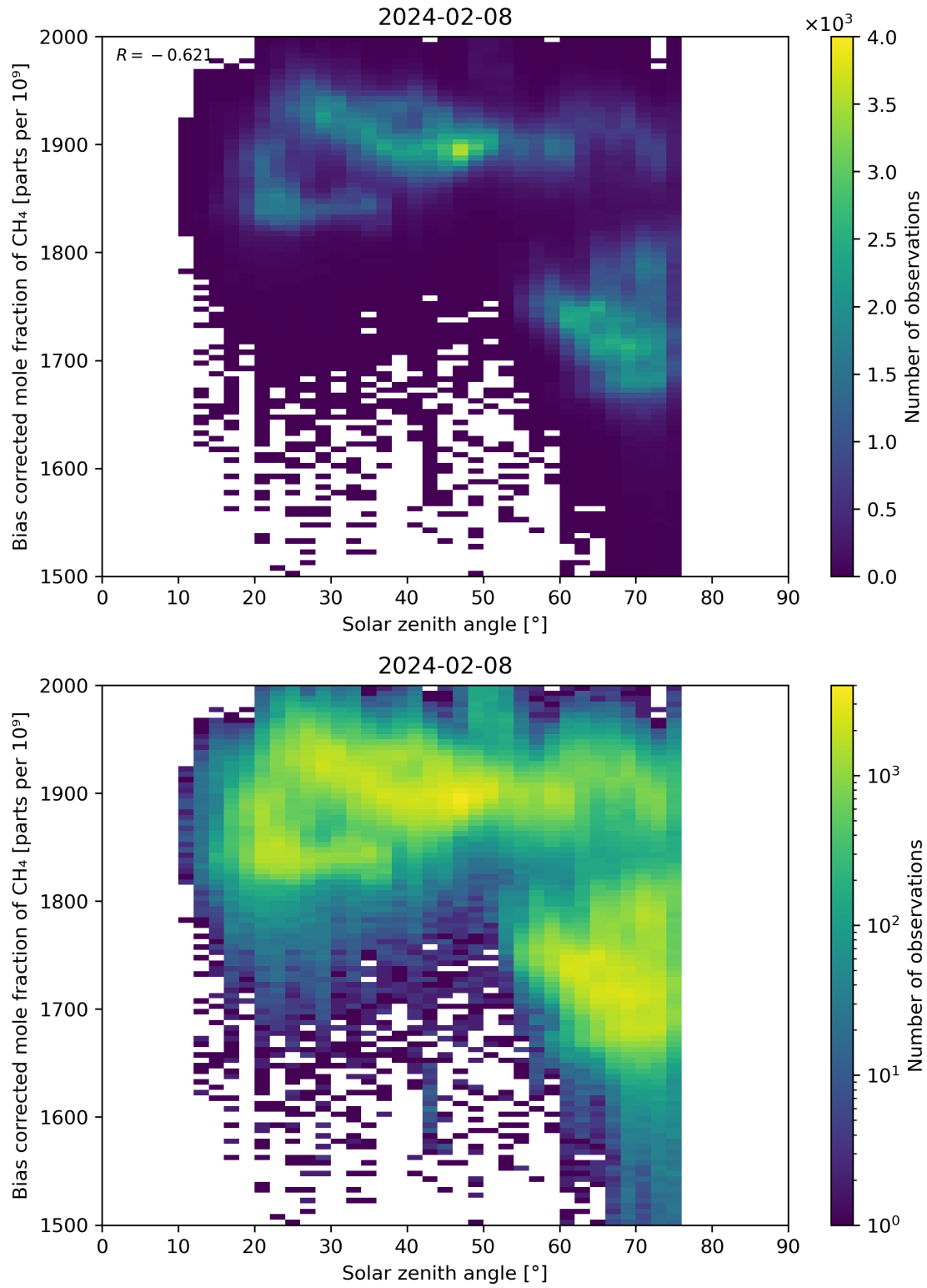
Figure 100: Scatter density plot of “Solar zenith angle” against “Bias corrected mole fraction of CH 4 ” for 2024-02-07 to 2024-02-09.
