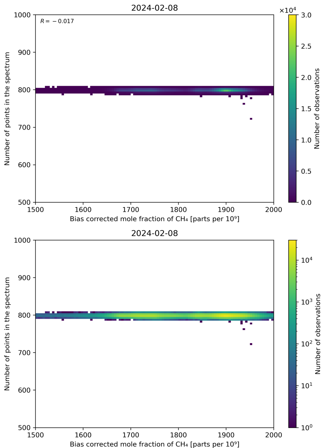
Figure 68: Scatter density plot of “Bias corrected mole fraction of CH 4 ” against “Number of points in the spectrum” for 2024-02-07 to 2024-02-09.
