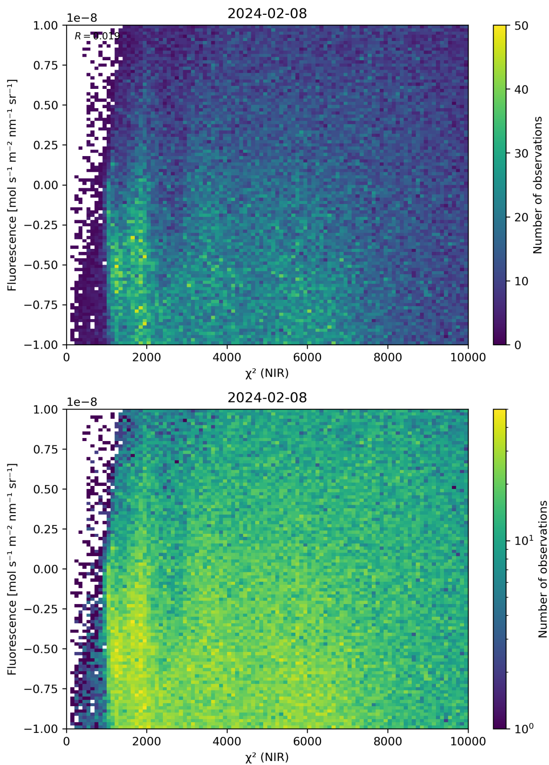
Figure 45: Scatter density plot of “ \chi^2 (NIR)” against “Fluorescence” for 2024-02-07 to 2024-02-09.
