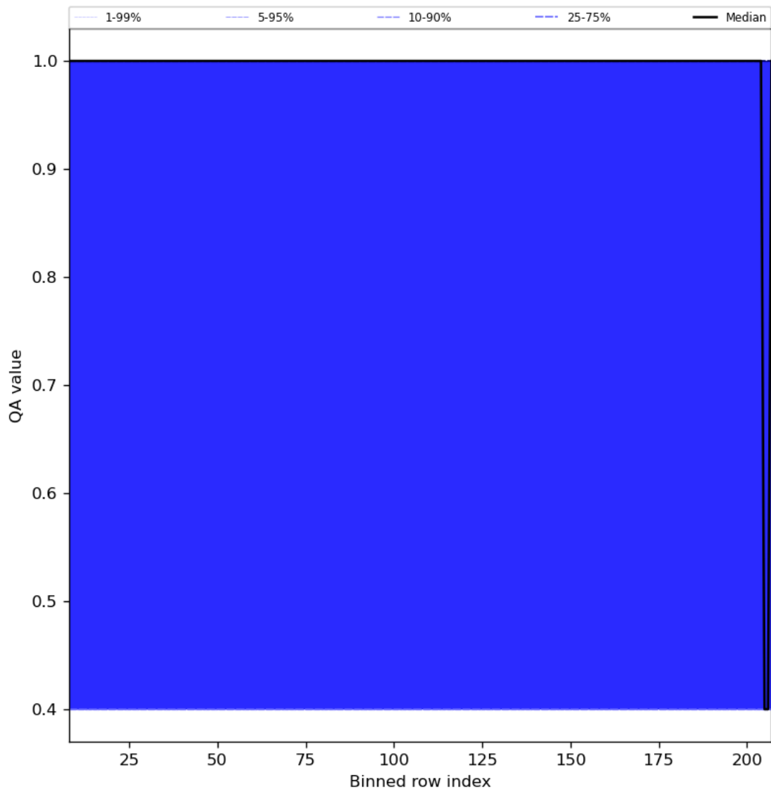
Figure 33: Along track statistics of “QA value” for 2024-02-07 to 2024-02-09
