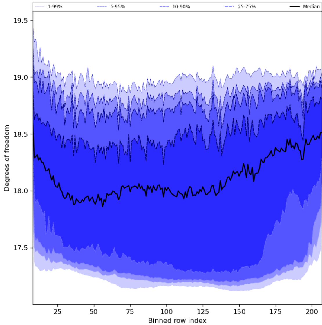
Figure 41: Along track statistics of “Degrees of freedom” for 2024-02-07 to 2024-02-09
