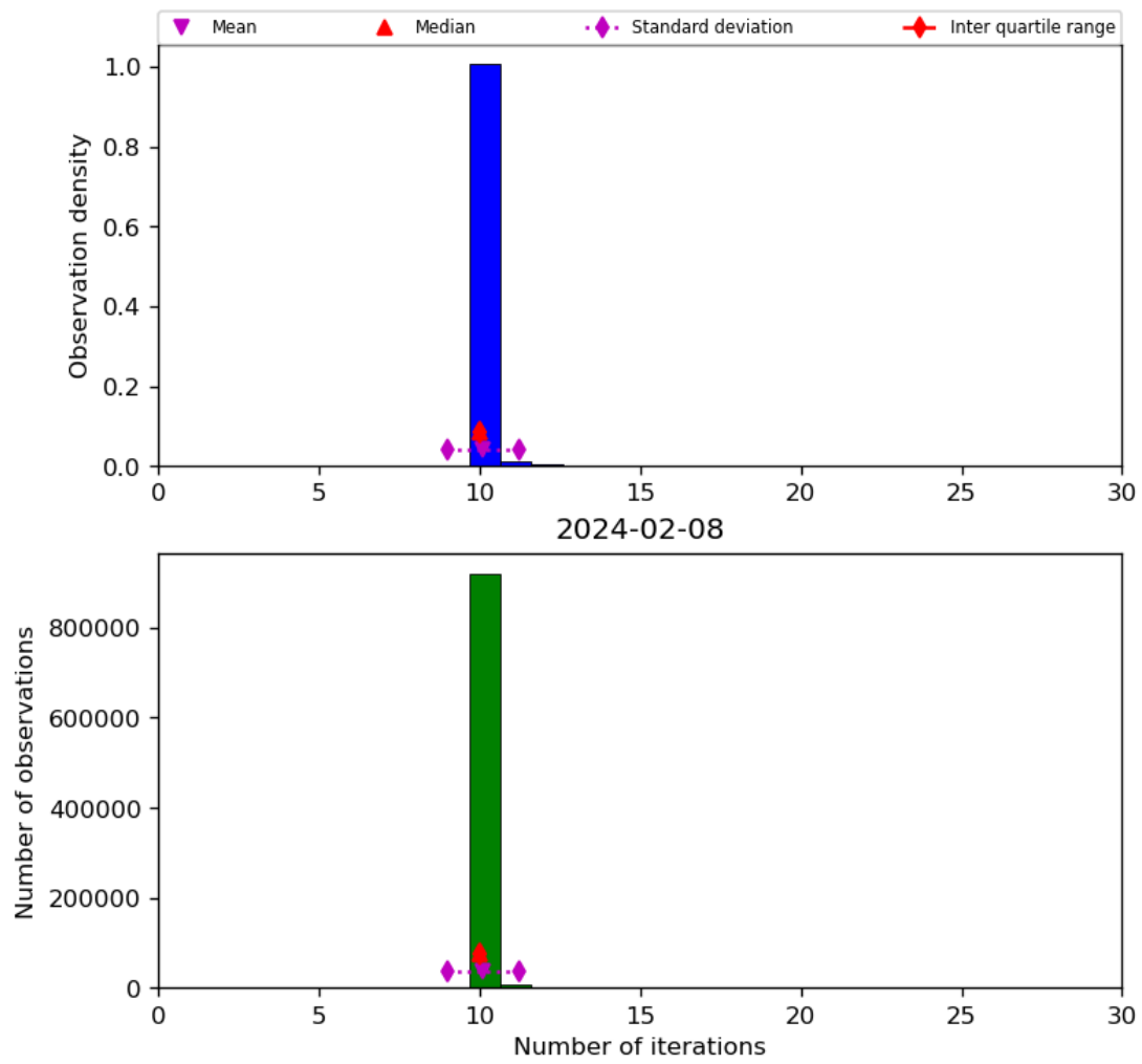
Figure 31: Histogram of “Number of iterations” for 2024-02-07 to 2024-02-09
