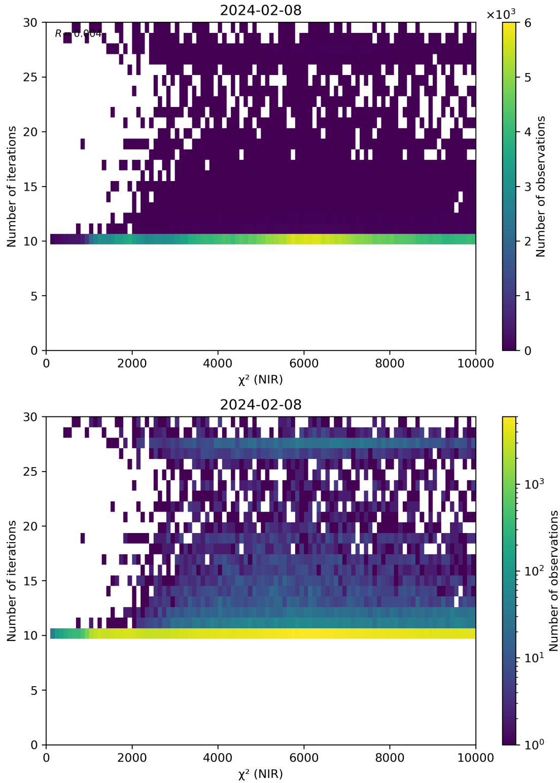
Figure 46: Scatter density plot of “ \chi^2 (NIR)” against “Number of iterations” for 2024-02-07 to 2024-02-09.
