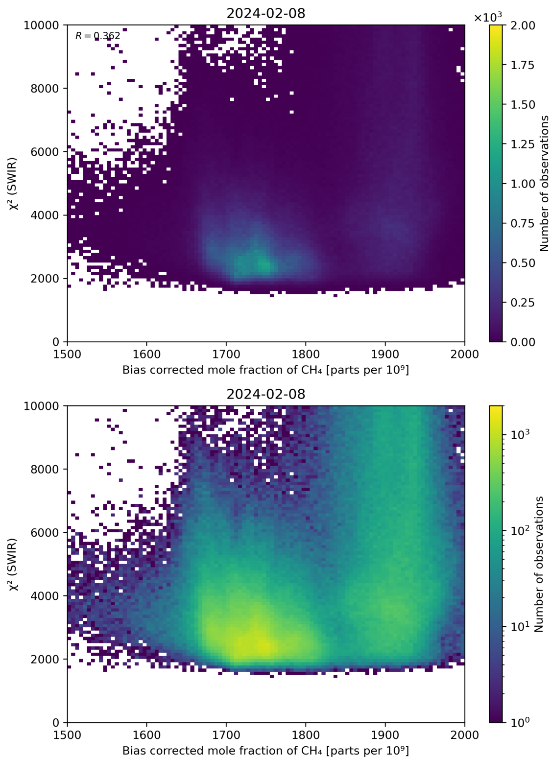
Figure 64: Scatter density plot of “Bias corrected mole fraction of CH 4 ” against “ \chi^2 (SWIR)” for 2024-02-07 to 2024-02-09.
