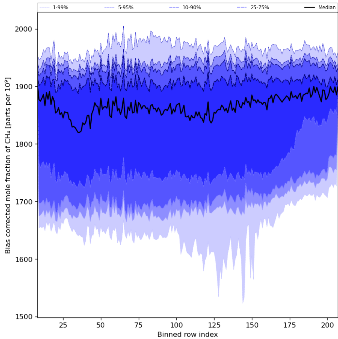
Figure 36: Along track statistics of “Bias corrected mole fraction of \text{CH}_4 ” for 2024-02-07 to 2024-02-09
