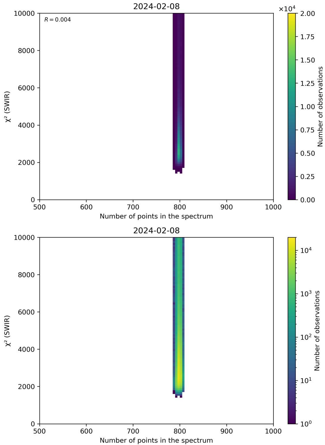
Figure 89: Scatter density plot of “Number of points in the spectrum” against “ \chi^2 (SWIR)” for 2024-02-07 to 2024-02-09.
