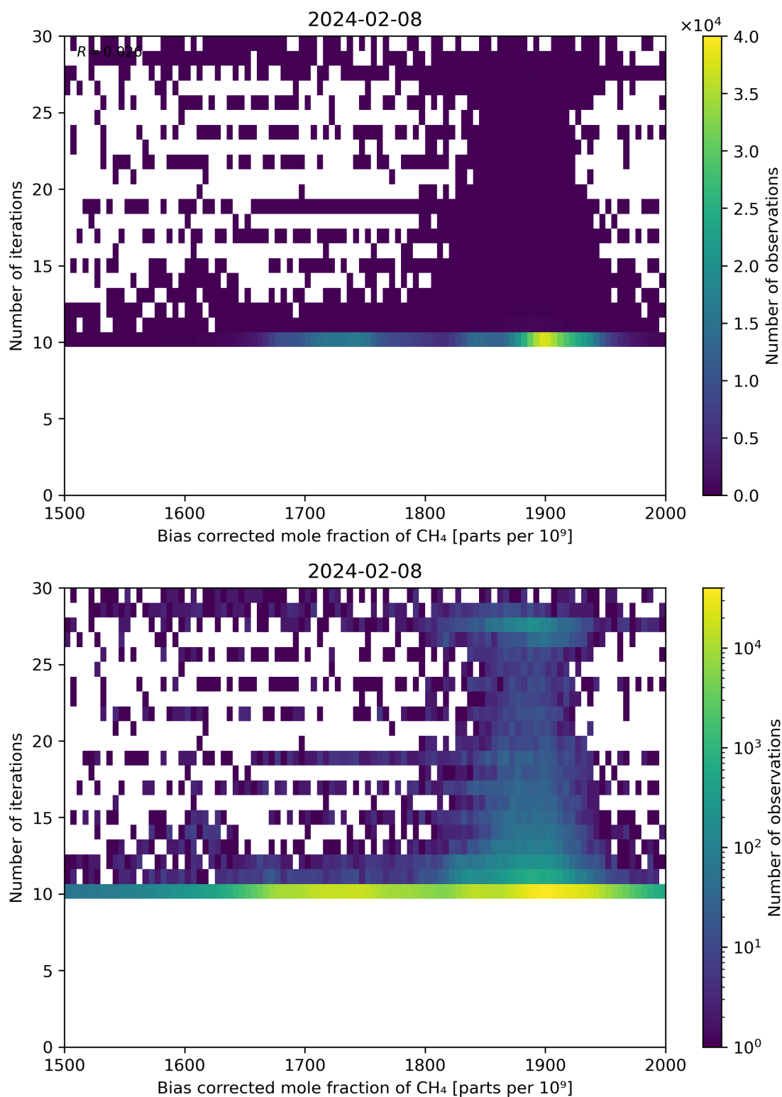
Figure 67: Scatter density plot of “Bias corrected mole fraction of CH 4 ” against “Number of iterations” for 2024-02-07 to 2024-02-09.
