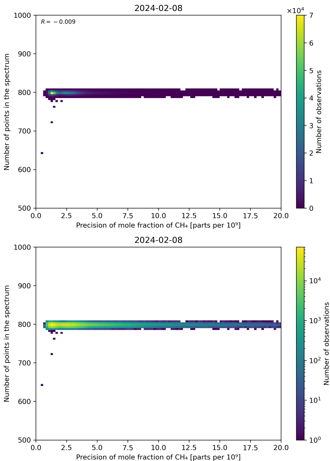
Figure 84: Scatter density plot of “Precision of mole fraction of CH 4 ” against “Number of points in the spectrum” for 2024-02-07 to 2024-02-09.
