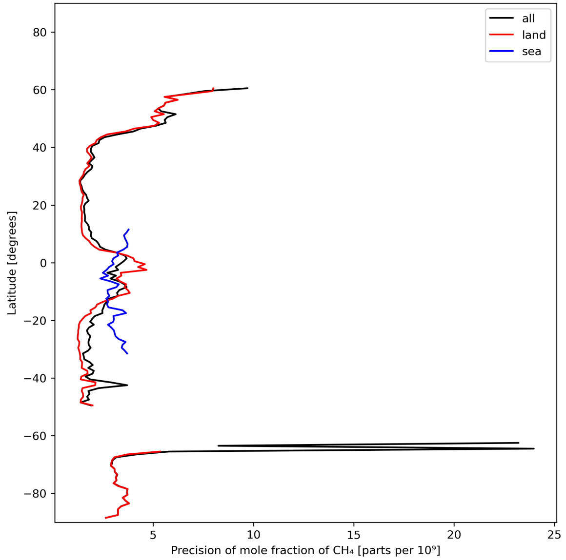
Figure 13: Zonal average of “Precision of mole fraction of CH 4 ” for 2024-02-07 to 2024-02-09.
