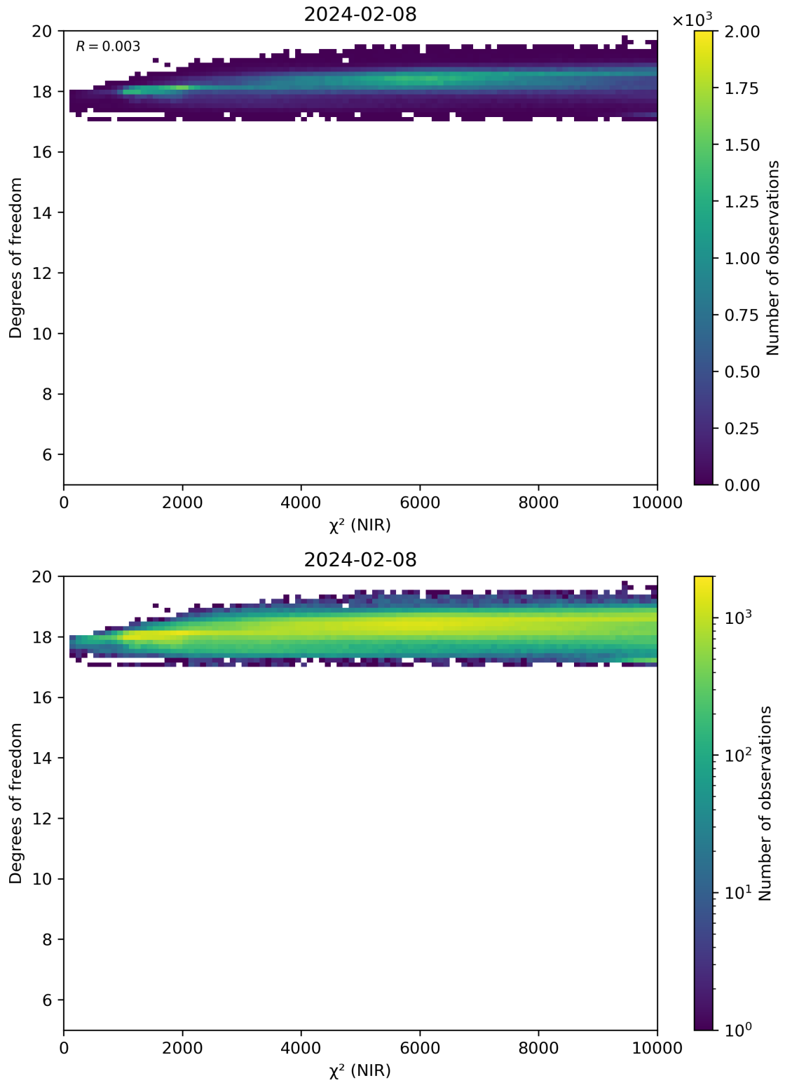
Figure 44: Scatter density plot of “ \chi^2 (NIR)” against “Degrees of freedom” for 2024-02-07 to 2024-02-09.
