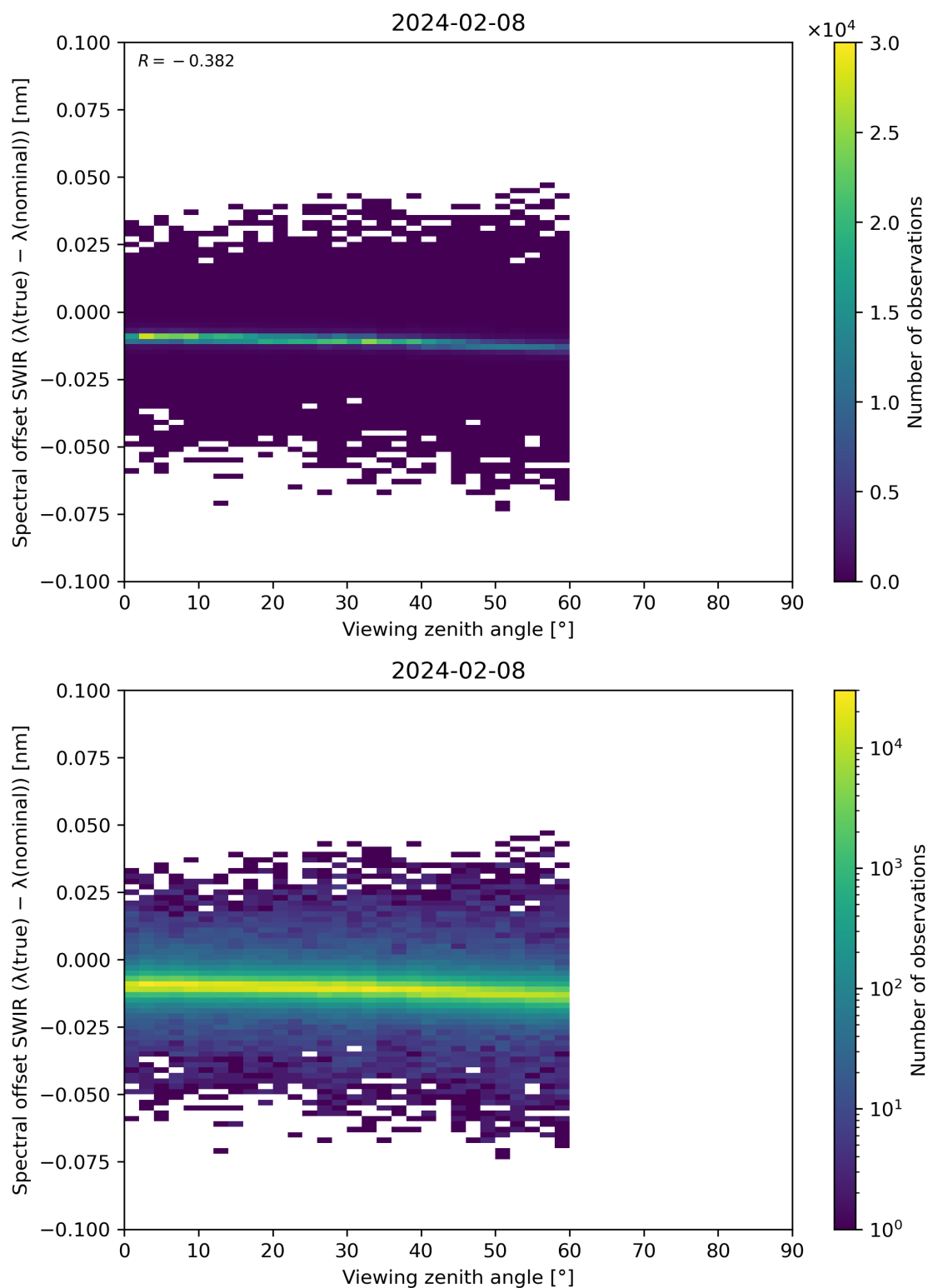
Figure 116: Scatter density plot of “Viewing zenith angle” against “Spectral offset SWIR ( \lambda(\text{true}) - \lambda(\text{nominal}) )” for 2024-02-07 to 2024-02-09.
