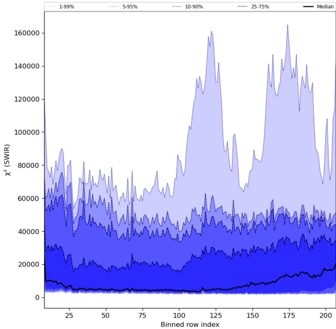
Figure 39: Along track statistics of “ \chi^2 (SWIR)” for 2024-02-07 to 2024-02-09
