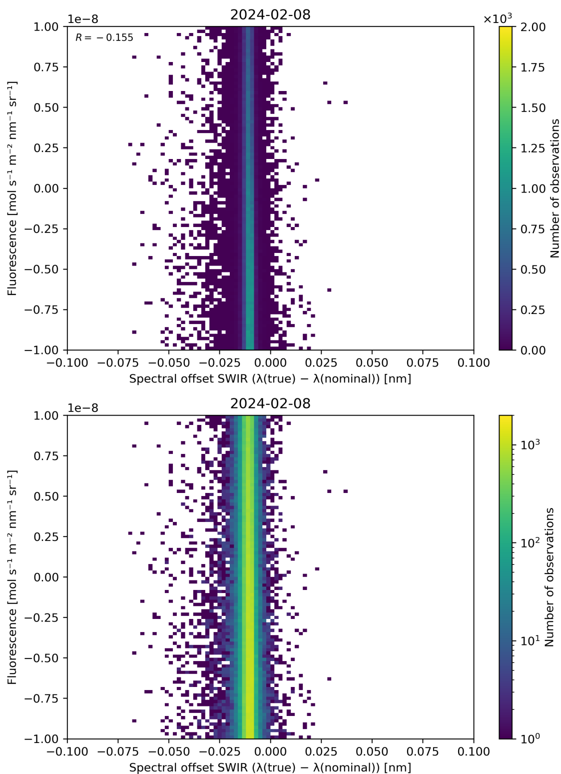
Figure 120: Scatter density plot of “Spectral offset SWIR ( \lambda(\text{true}) - \lambda(\text{nominal}) )” against “Fluorescence” for 2024-02-07 to 2024-02-09.
