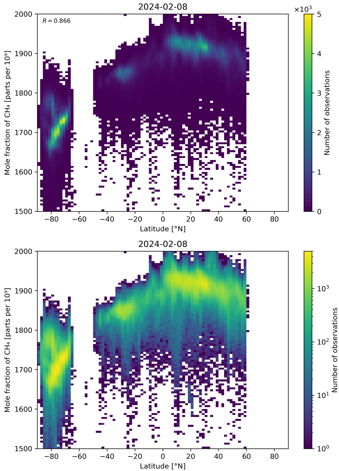
Figure 57: Scatter density plot of “Latitude” against “Mole fraction of \text{CH}_4 ” for 2024-02-07 to 2024-02-09.
