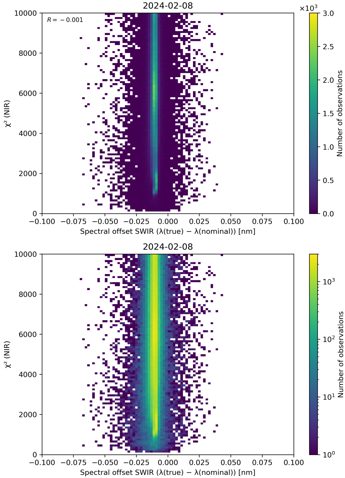
Figure 117: Scatter density plot of “Spectral offset SWIR ( \lambda(\text{true}) - \lambda(\text{nominal}) )” against “ \chi^2 (NIR)” for 2024-02-07 to 2024-02-09.
