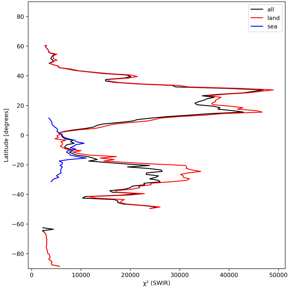
Figure 17: Zonal average of “ \chi^2 (SWIR)” for 2024-02-07 to 2024-02-09.
