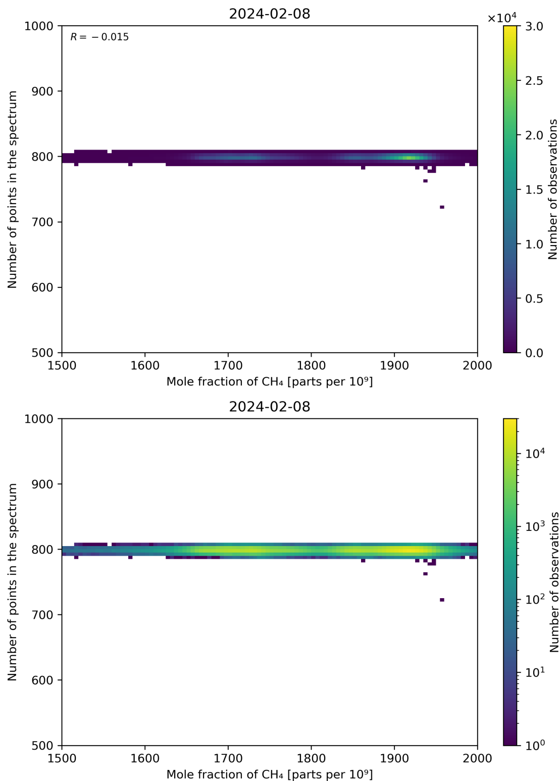
Figure 77: Scatter density plot of “Mole fraction of CH 4 ” against “Number of points in the spectrum” for 2024-02-07 to 2024-02-09.
