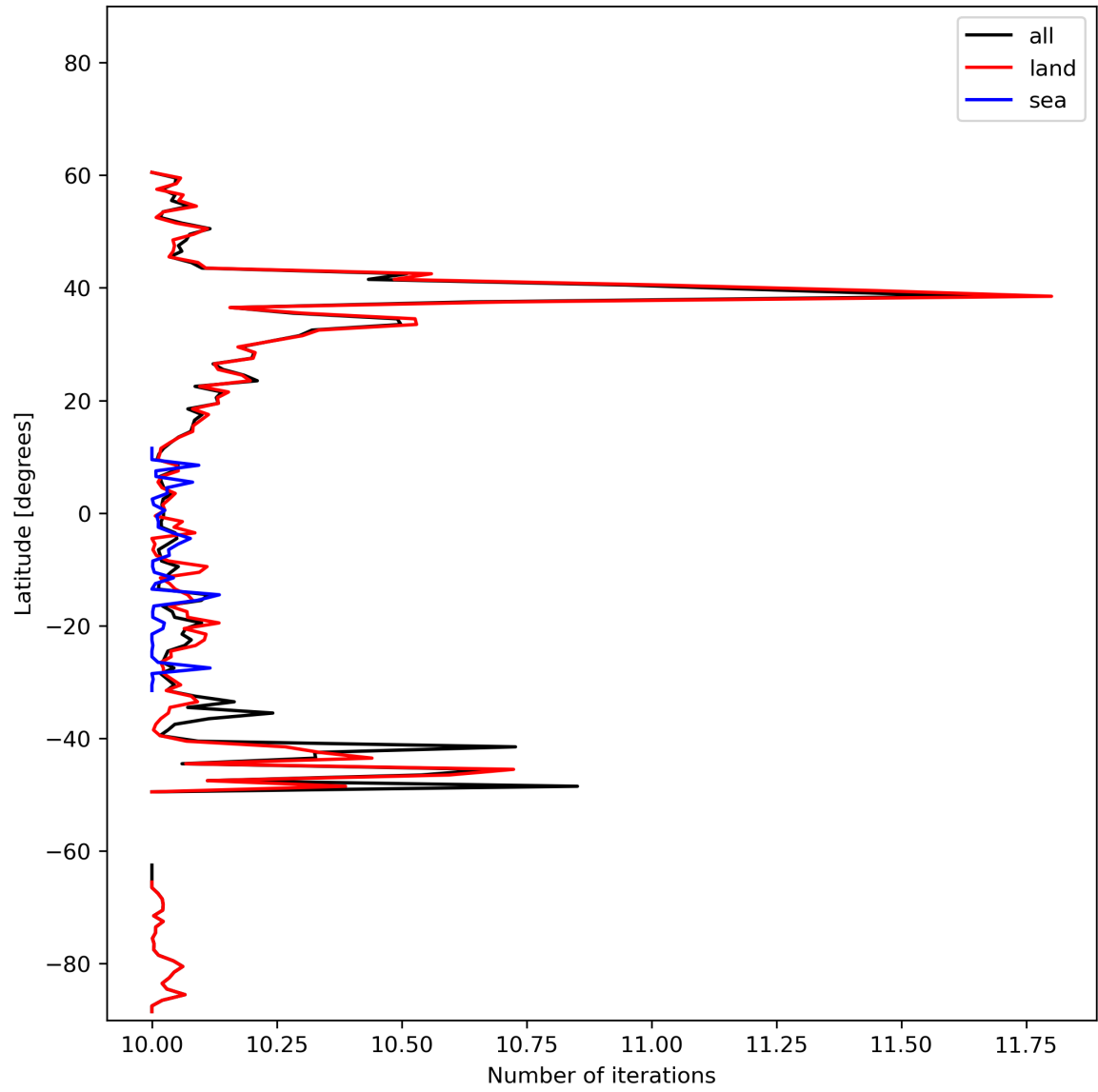
Figure 20: Zonal average of “Number of iterations” for 2024-02-07 to 2024-02-09.
