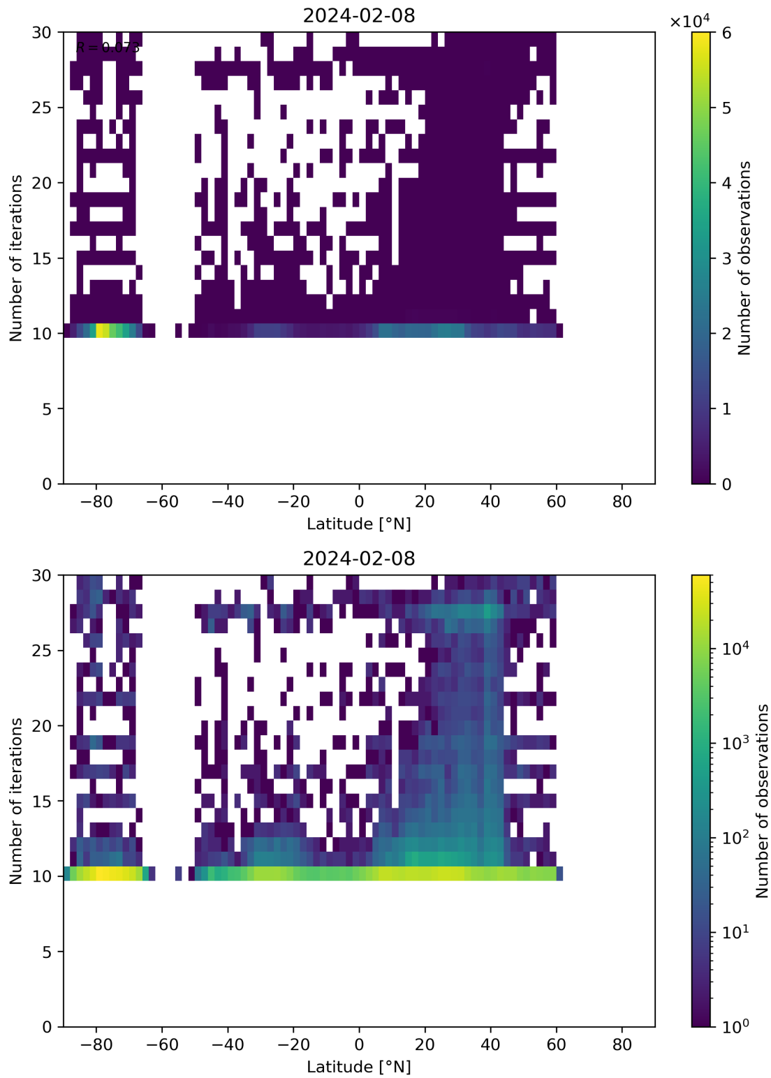
Figure 60: Scatter density plot of “Latitude” against “Number of iterations” for 2024-02-07 to 2024-02-09.
