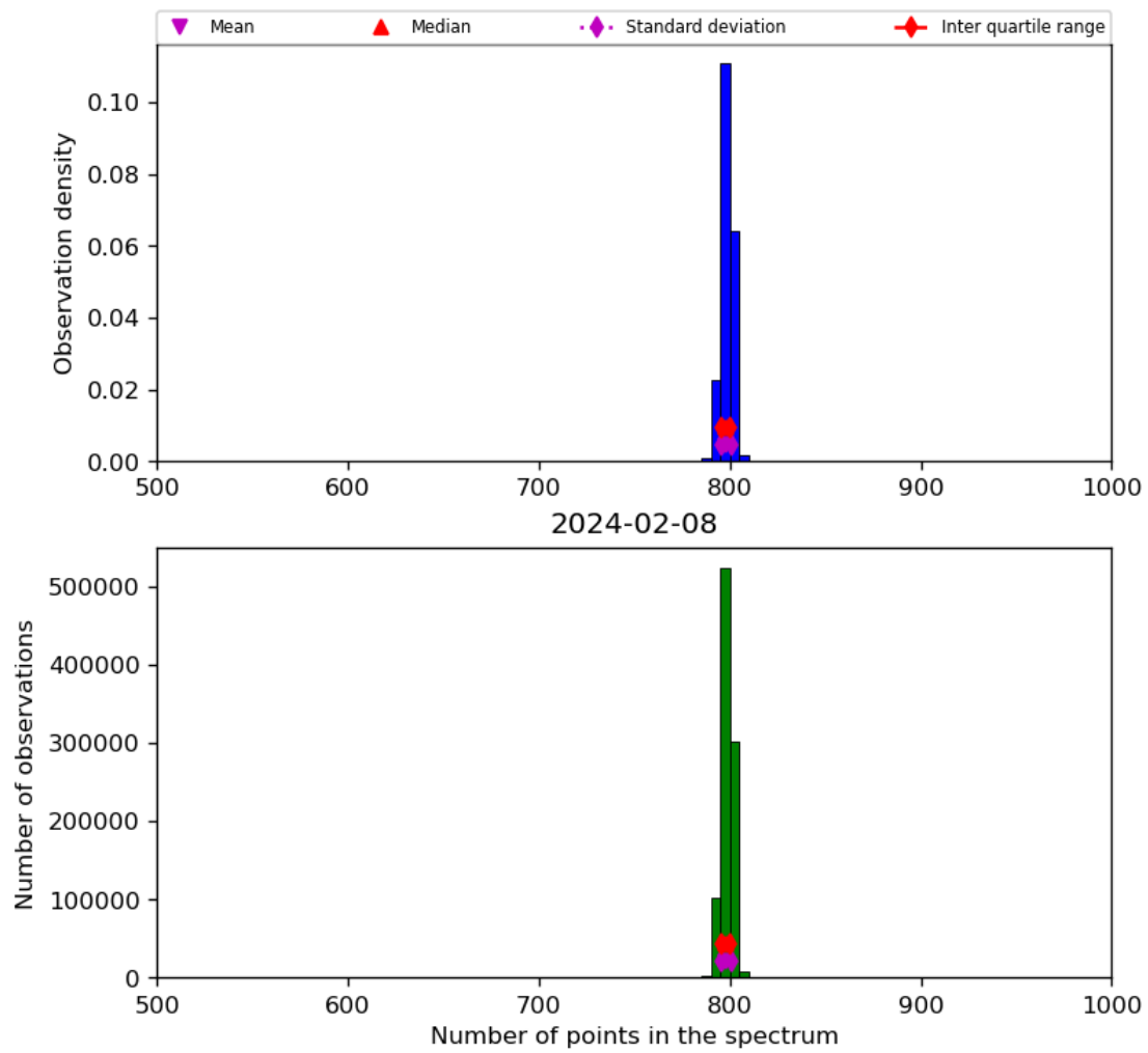
Figure 26: Histogram of “Number of points in the spectrum” for 2024-02-07 to 2024-02-09
