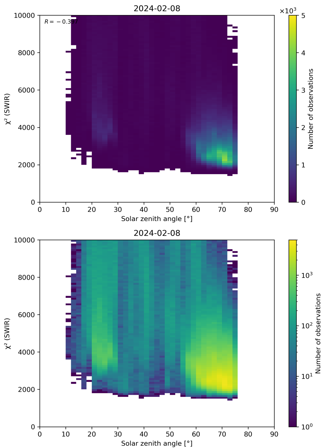
Figure 95: Scatter density plot of “Solar zenith angle” against “ \chi^2 (SWIR)” for 2024-02-07 to 2024-02-09.
