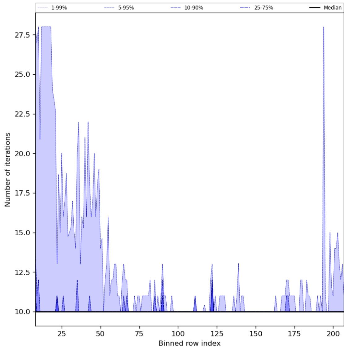
Figure 42: Along track statistics of “Number of iterations” for 2024-02-07 to 2024-02-09
