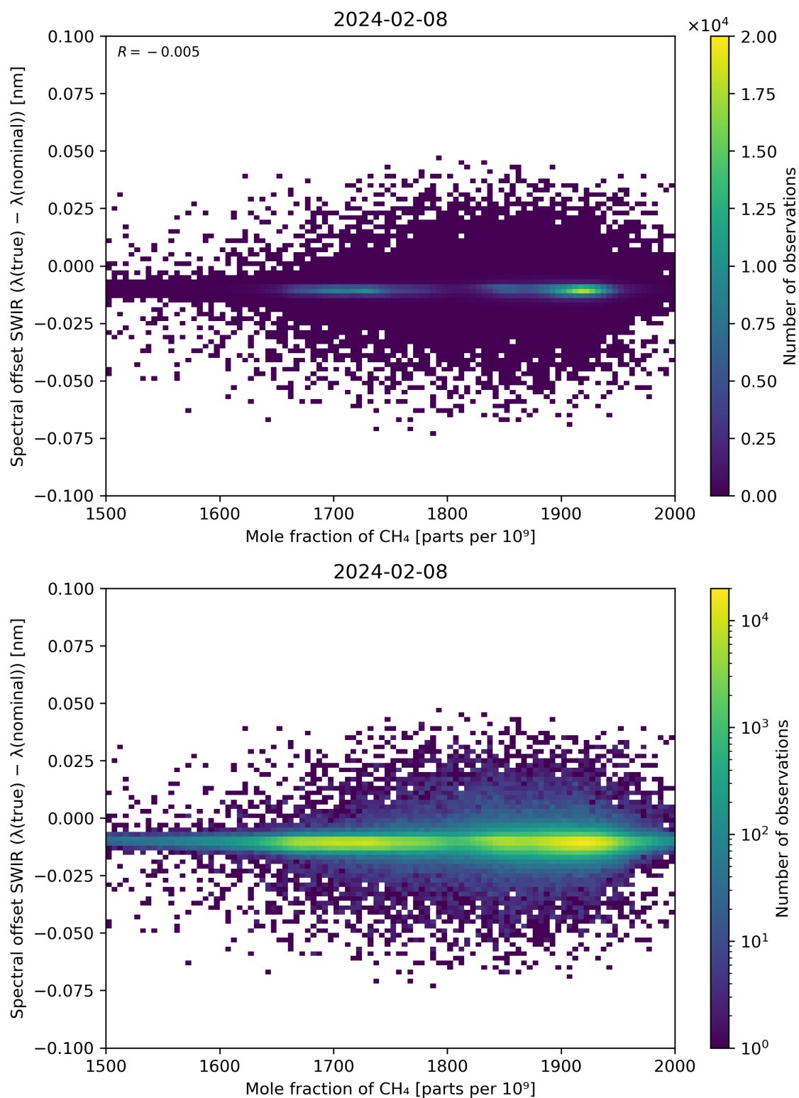
Figure 86: Scatter density plot of “Mole fraction of CH 4 ” against “Spectral offset SWIR ( \lambda(\text{true}) - \lambda(\text{nominal}) )” for 2024-02-07 to 2024-02-09.
