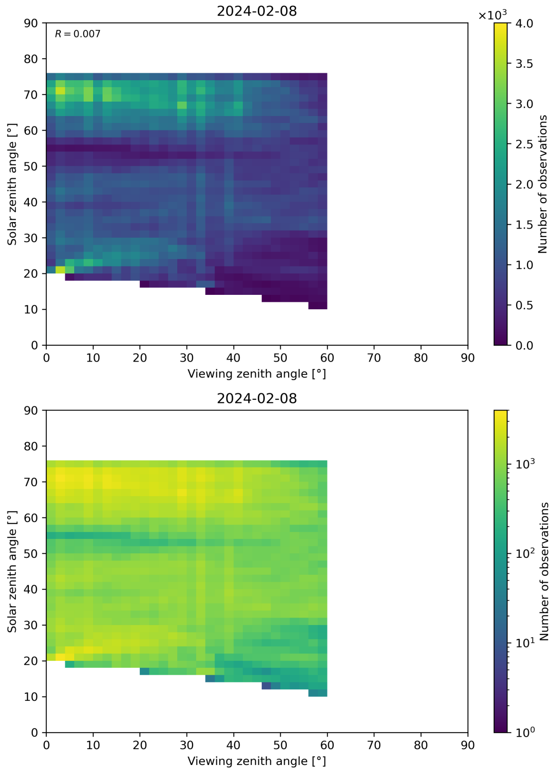
Figure 115: Scatter density plot of “Viewing zenith angle” against “Solar zenith angle” for 2024-02-07 to 2024-02-09.
