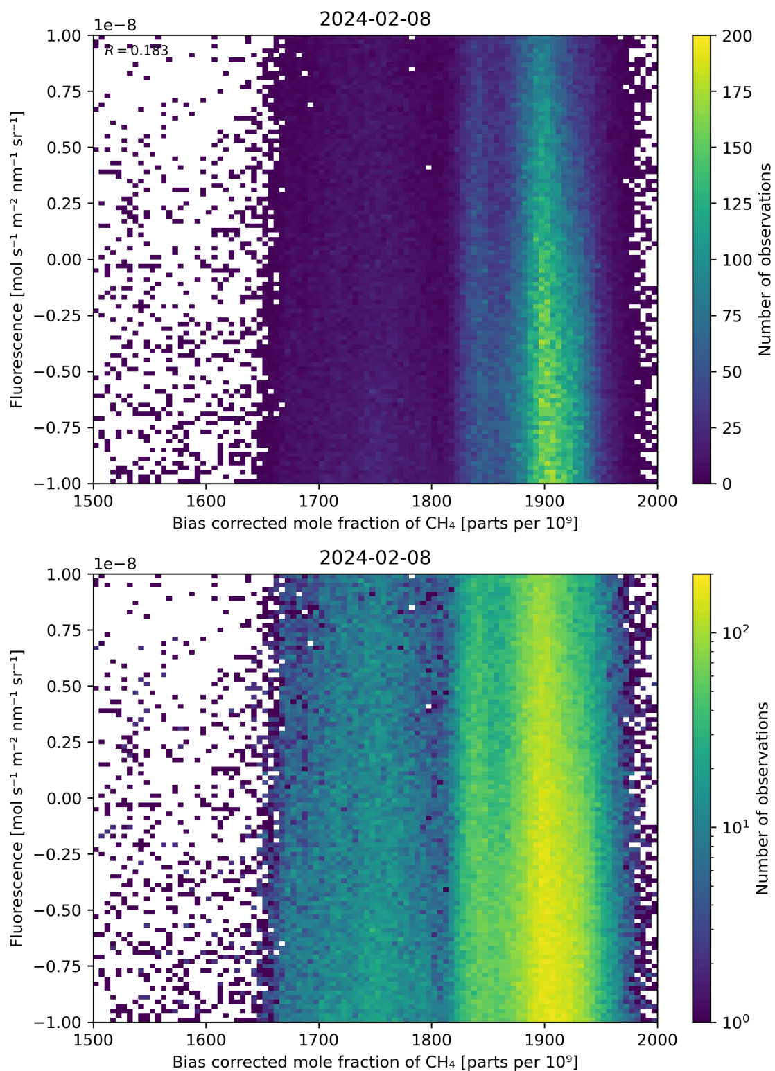
Figure 66: Scatter density plot of “Bias corrected mole fraction of \text{CH}_4 ” against “Fluorescence” for 2024-02-07 to 2024-02-09.
