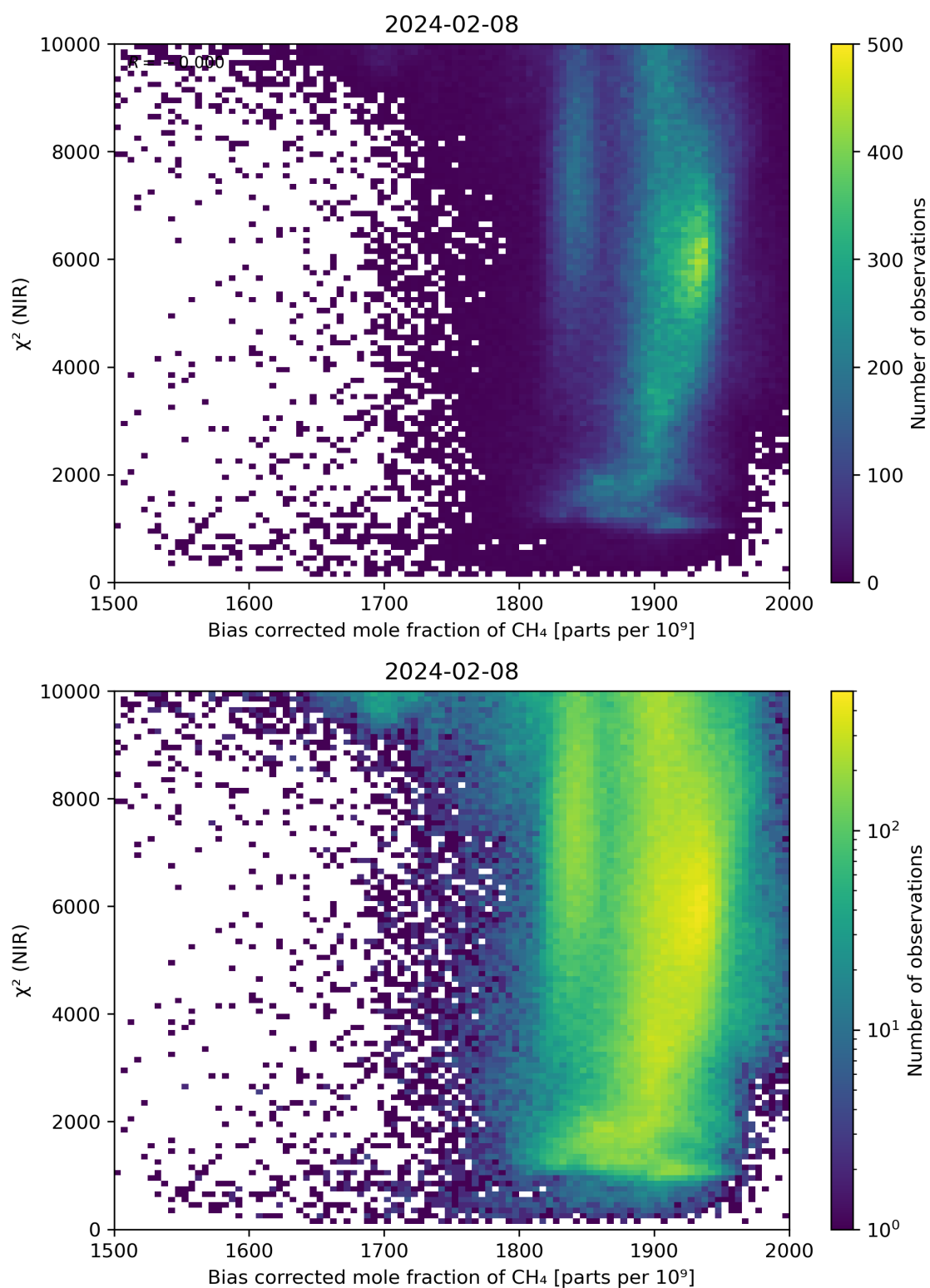
Figure 63: Scatter density plot of “Bias corrected mole fraction of CH 4 ” against “ \chi^2 (NIR)” for 2024-02-07 to 2024-02-09.
