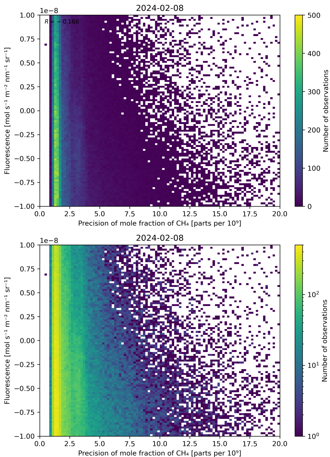
Figure 81: Scatter density plot of “Precision of mole fraction of \text{CH}_4 ” against “Fluorescence” for 2024-02-07 to 2024-02-09.
