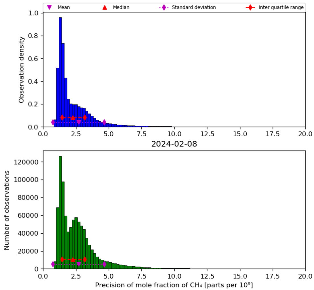
Figure 24: Histogram of “Precision of mole fraction of CH 4 ” for 2024-02-07 to 2024-02-09
