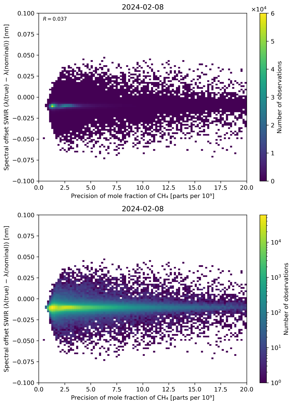
Figure 85: Scatter density plot of “Precision of mole fraction of CH 4 ” against “Spectral offset SWIR ( \lambda(\text{true}) - \lambda(\text{nominal}) )” for 2024-02-07 to 2024-02-09.
