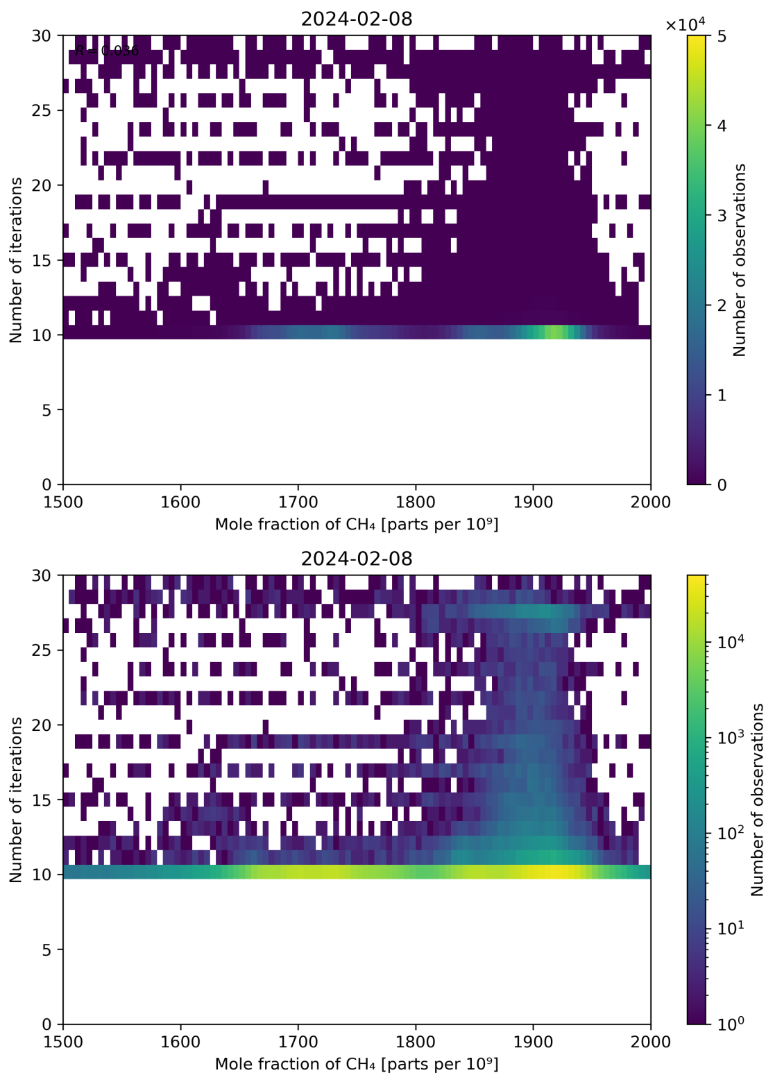
Figure 76: Scatter density plot of “Mole fraction of CH 4 ” against “Number of iterations” for 2024-02-07 to 2024-02-09.
