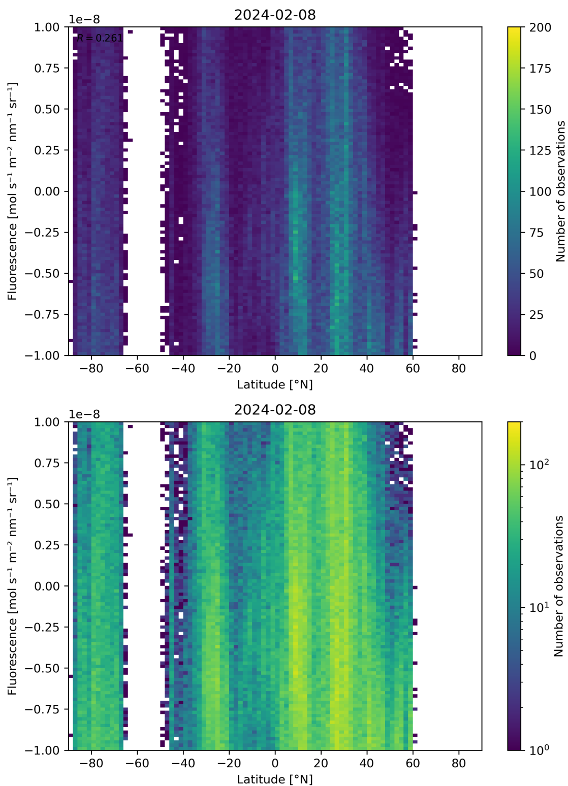
Figure 56: Scatter density plot of “Latitude” against “Fluorescence” for 2024-02-07 to 2024-02-09.
