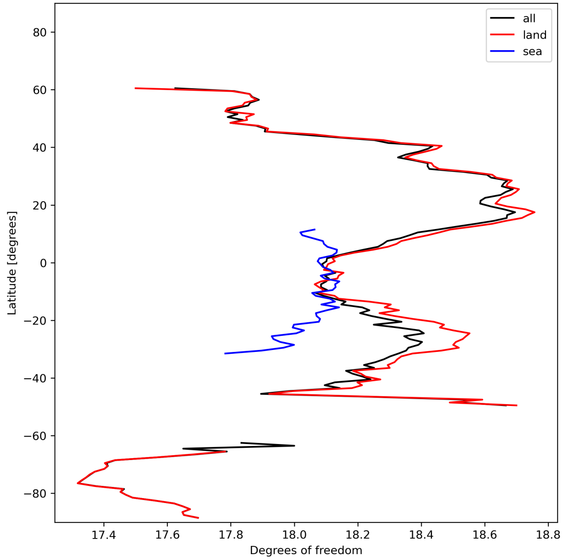
Figure 19: Zonal average of “Degrees of freedom” for 2024-02-07 to 2024-02-09.
