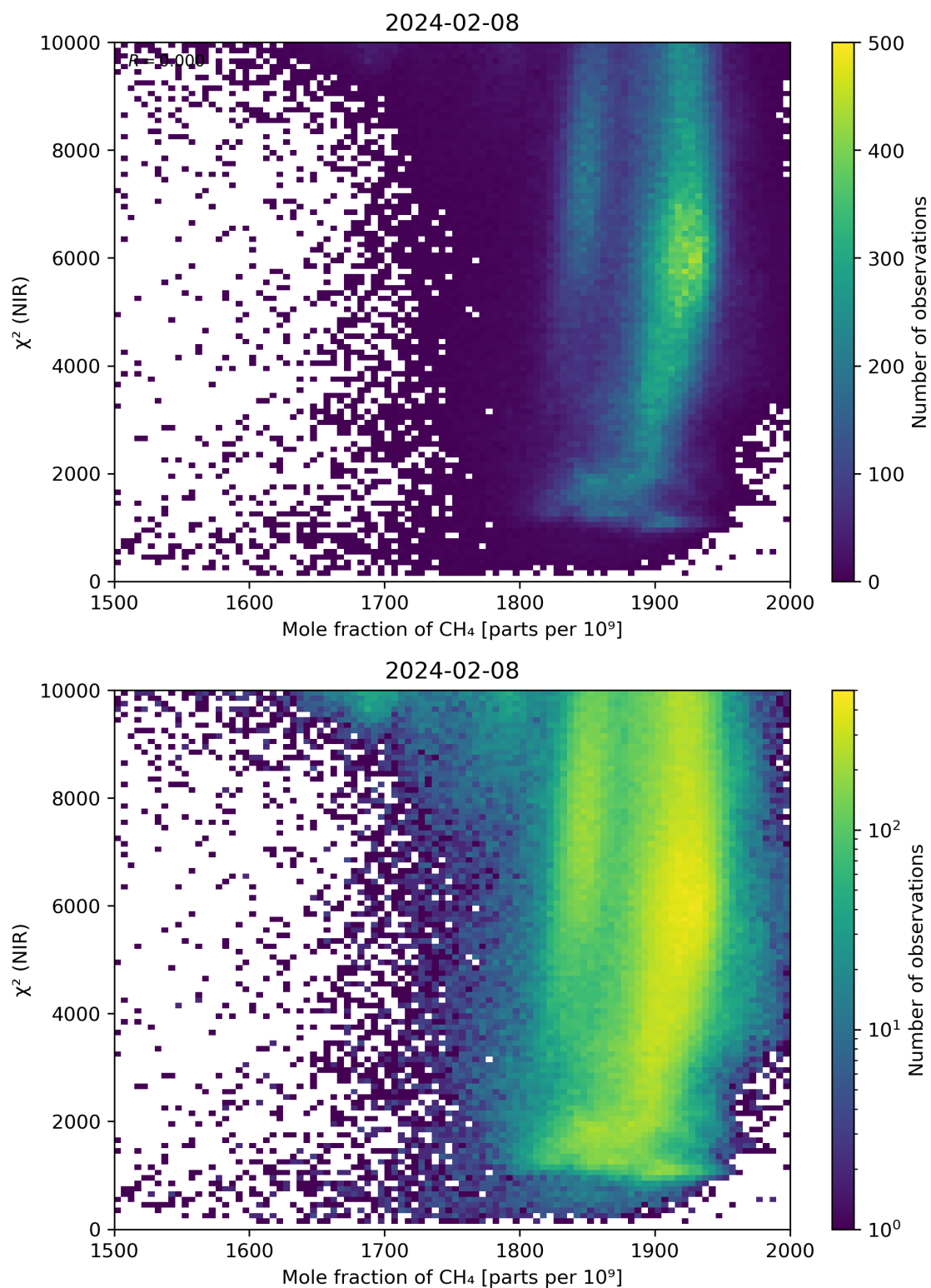
Figure 70: Scatter density plot of “Mole fraction of CH 4 ” against “ \chi^2 (NIR)” for 2024-02-07 to 2024-02-09.
