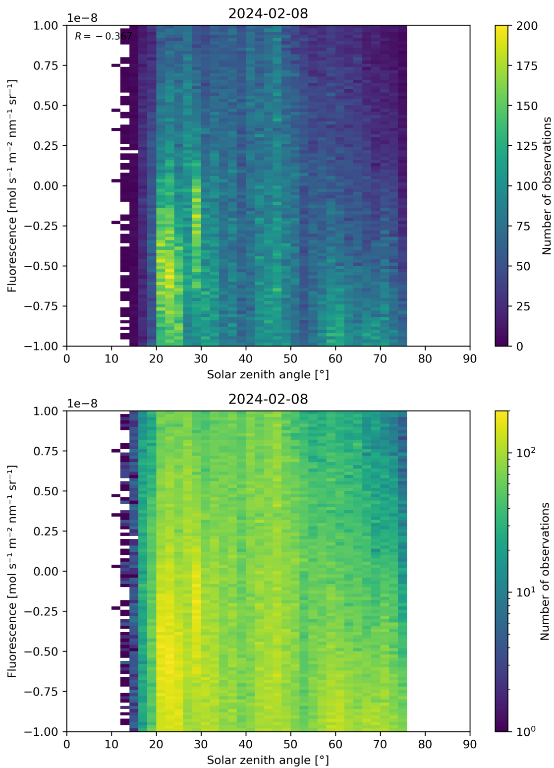
Figure 97: Scatter density plot of “Solar zenith angle” against “Fluorescence” for 2024-02-07 to 2024-02-09.
