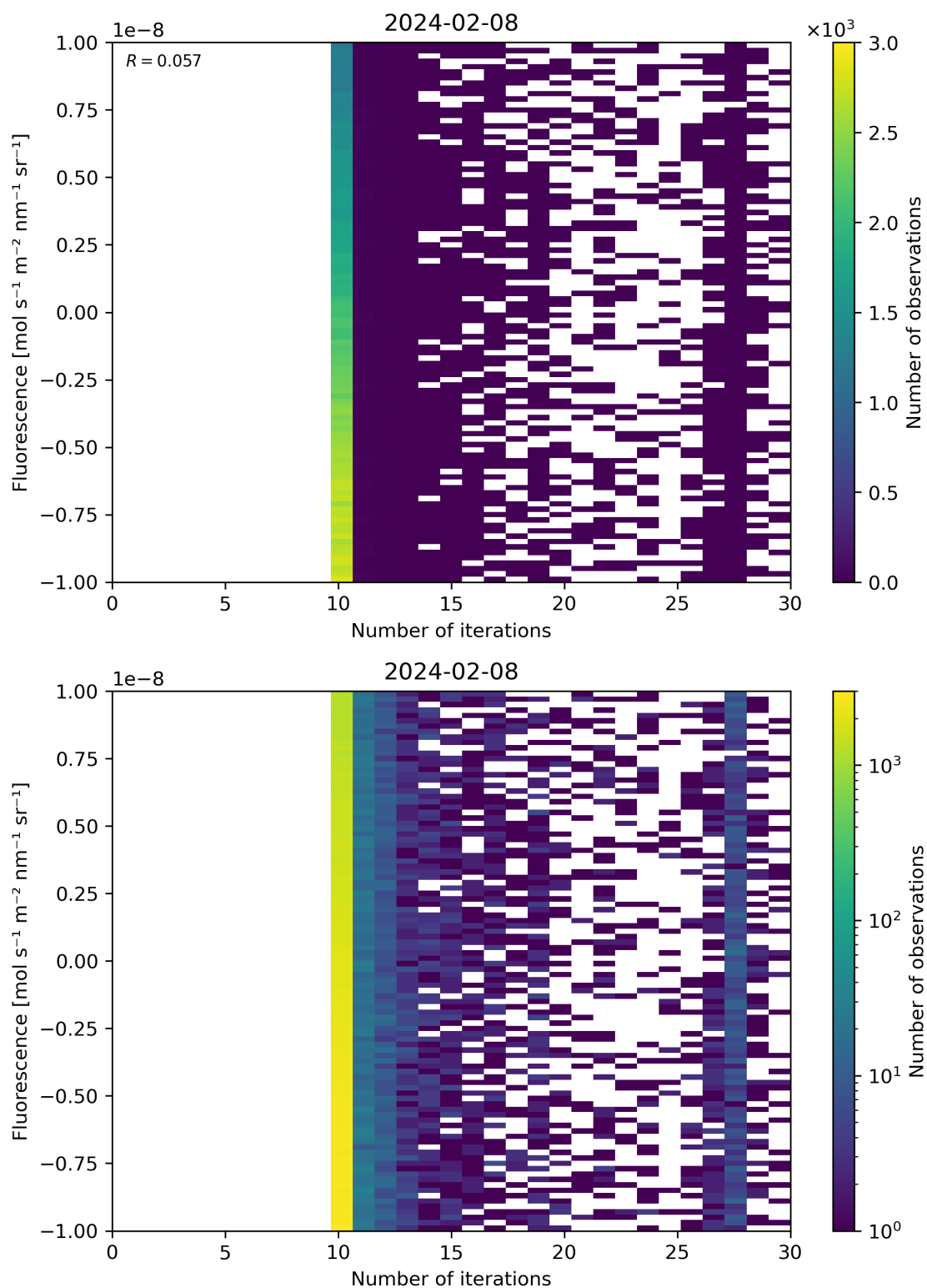
Figure 87: Scatter density plot of “Number of iterations” against “Fluorescence” for 2024-02-07 to 2024-02-09.
