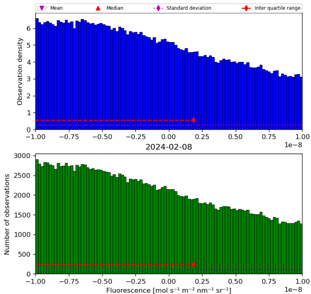
Figure 32: Histogram of “Fluorescence” for 2024-02-07 to 2024-02-09
