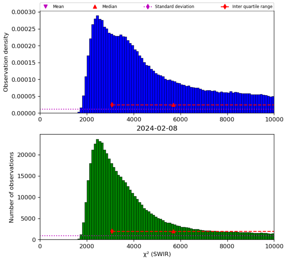
Figure 28: Histogram of “ \chi^2 (SWIR)” for 2024-02-07 to 2024-02-09
