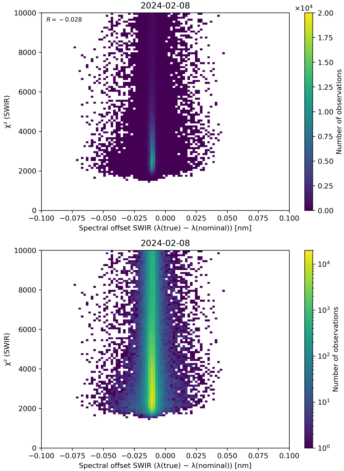
Figure 118: Scatter density plot of “Spectral offset SWIR ( \lambda(\text{true}) - \lambda(\text{nominal}) )” against “ \chi^2 (SWIR)” for 2024-02-07 to 2024-02-09.
