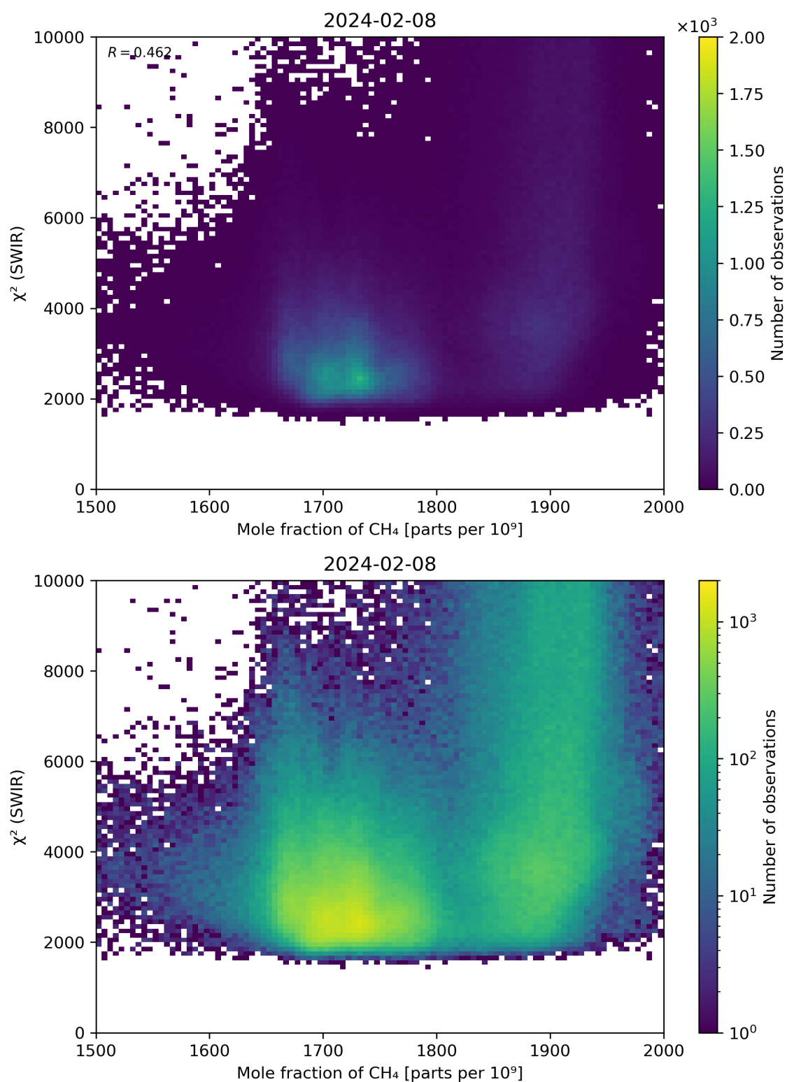
Figure 71: Scatter density plot of “Mole fraction of \text{CH}_4 ” against “ \chi^2 (SWIR)” for 2024-02-07 to 2024-02-09.
