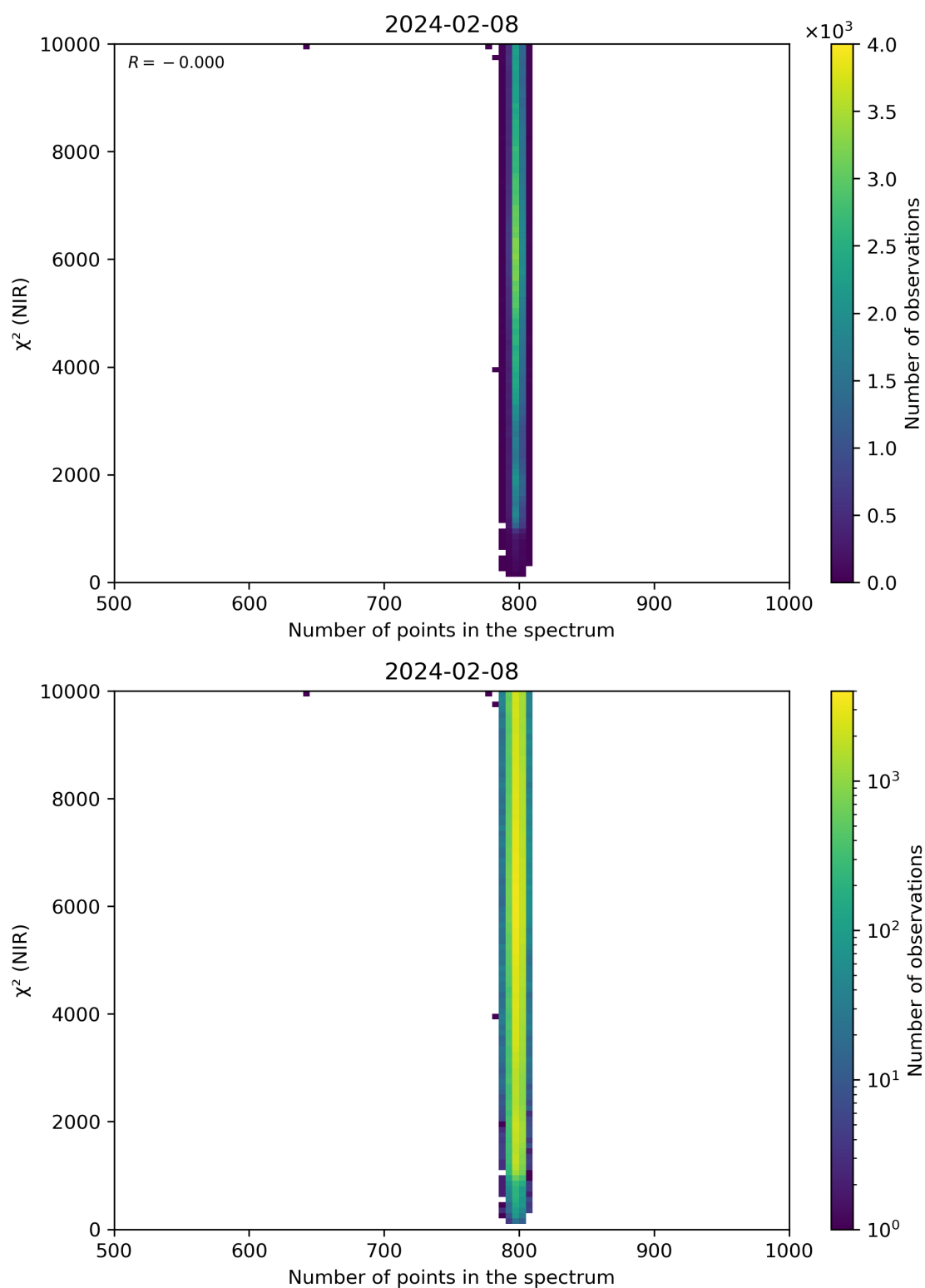
Figure 88: Scatter density plot of “Number of points in the spectrum” against “ \chi^2 (NIR)” for 2024-02-07 to 2024-02-09.
