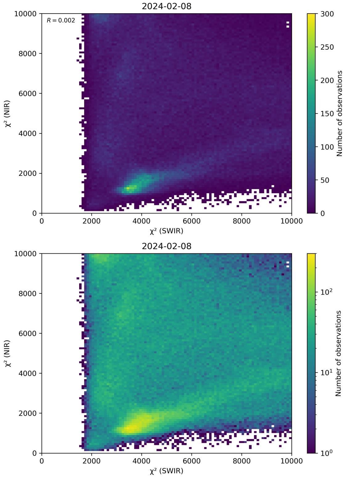
Figure 47: Scatter density plot of “ \chi^2 (SWIR)” against “ \chi^2 (NIR)” for 2024-02-07 to 2024-02-09.
