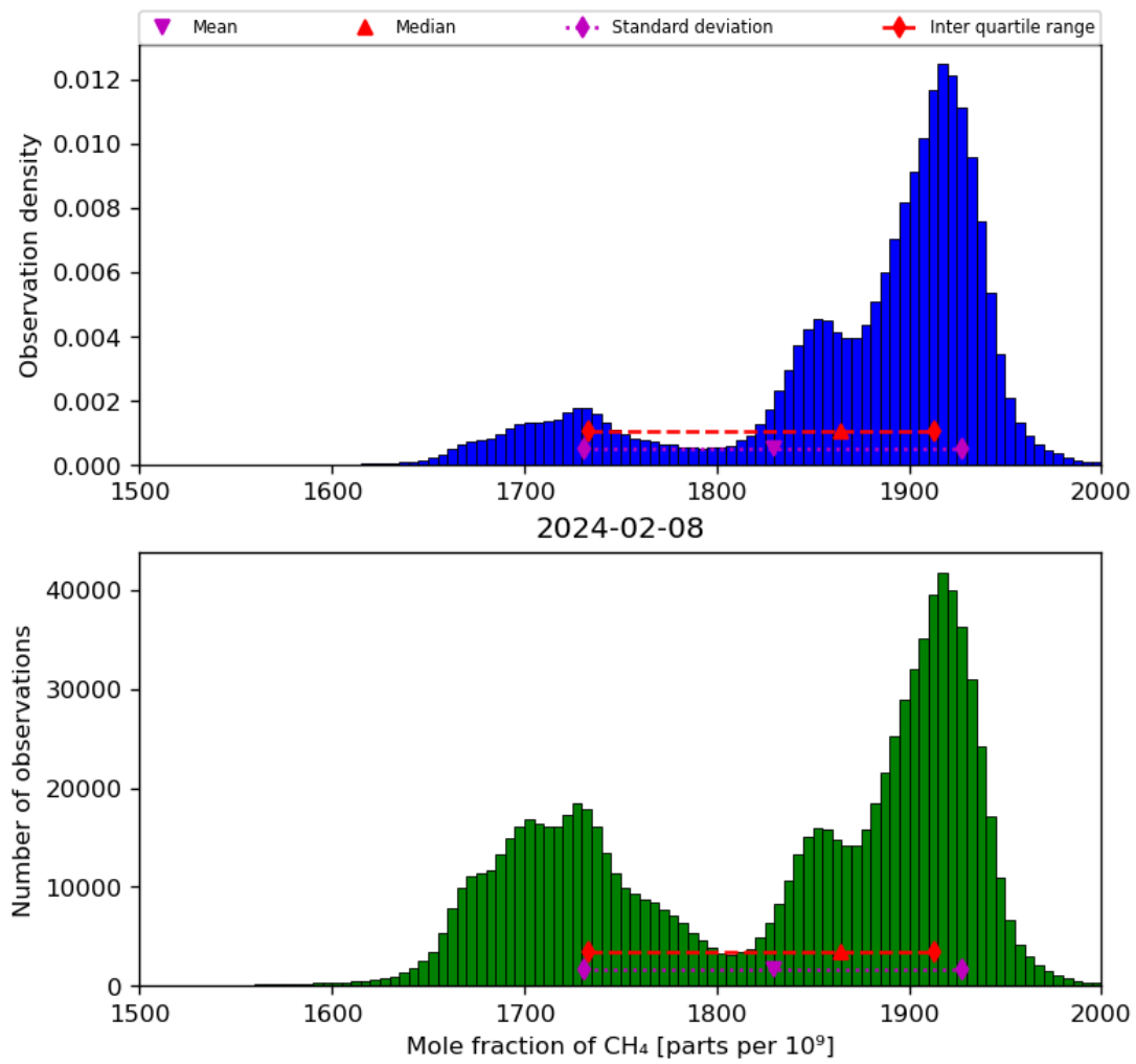
Figure 23: Histogram of “Mole fraction of CH 4 ” for 2024-02-07 to 2024-02-09
