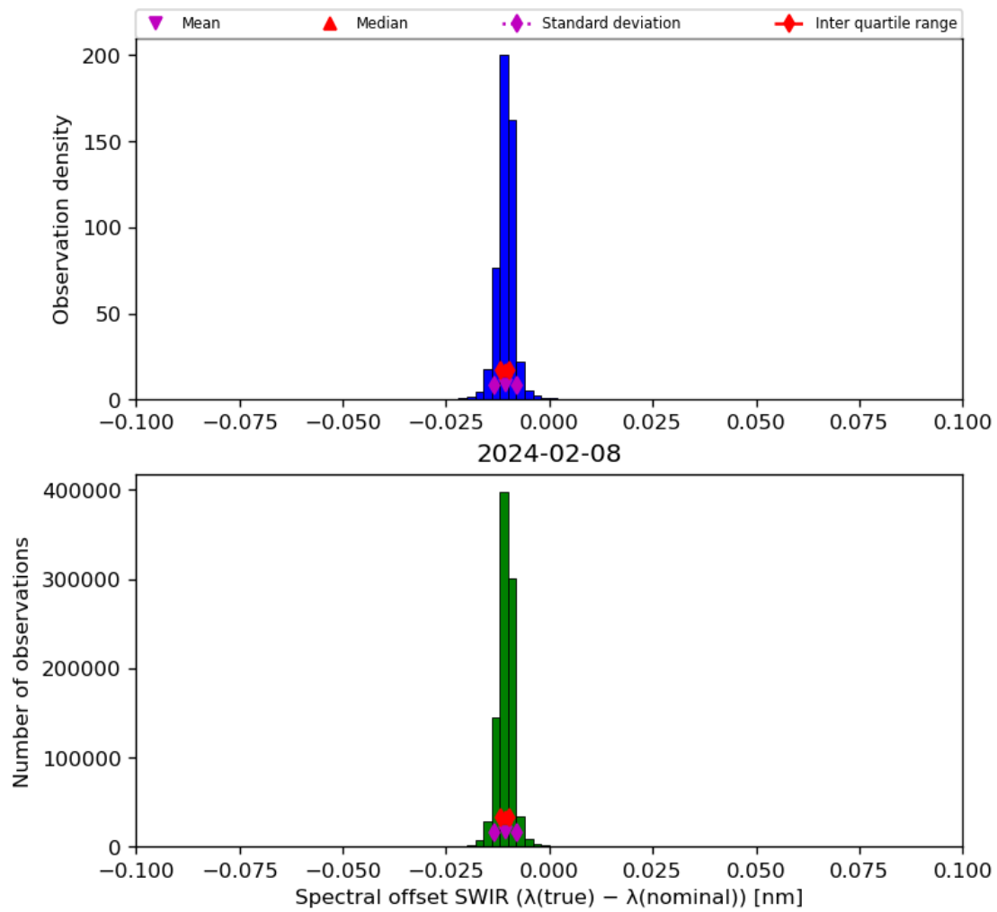
Figure 27: Histogram of “Spectral offset SWIR ( \lambda(\text{true}) - \lambda(\text{nominal}) )” for 2024-02-07 to 2024-02-09
