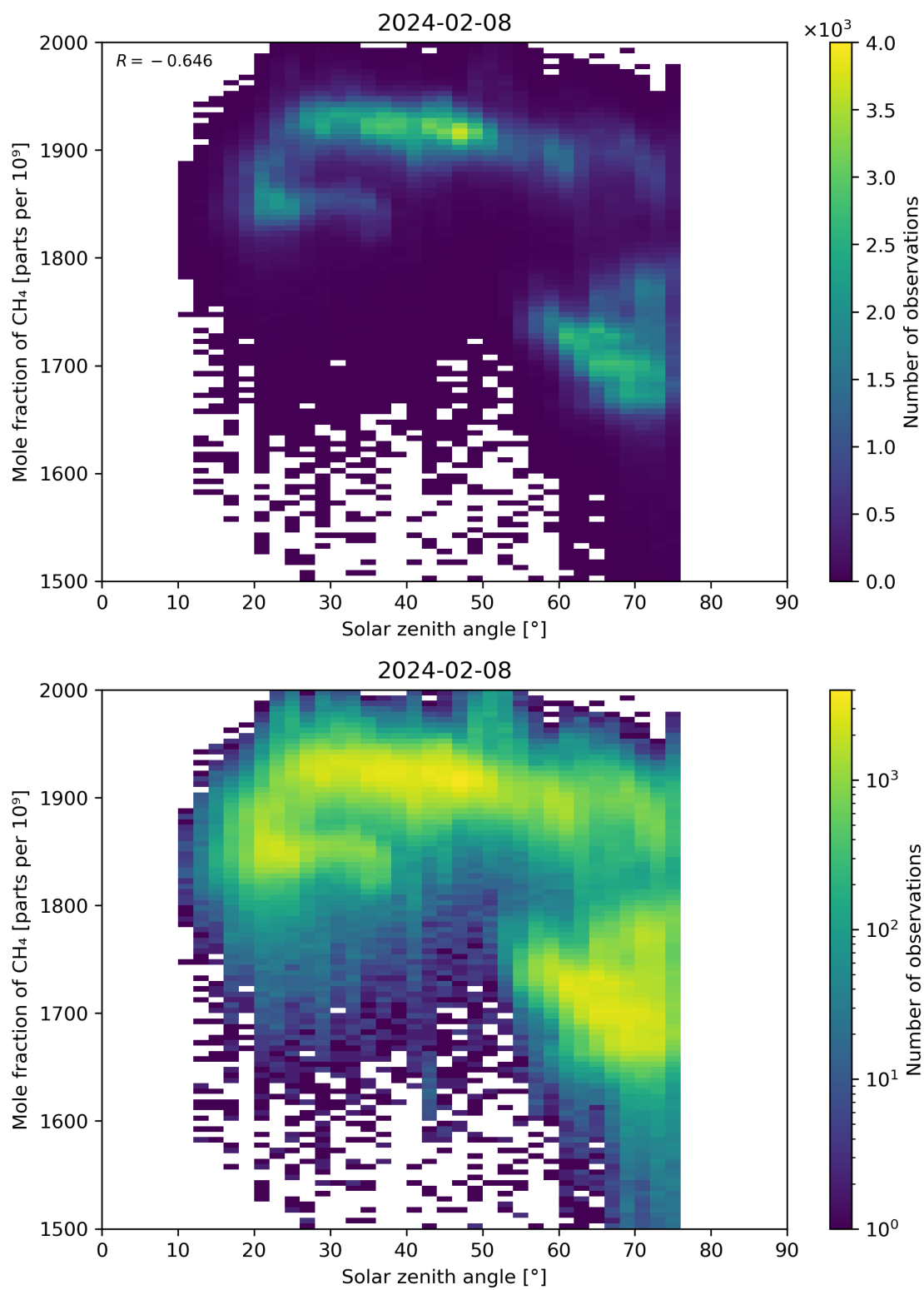
Figure 99: Scatter density plot of “Solar zenith angle” against “Mole fraction of \text{CH}_4 ” for 2024-02-07 to 2024-02-09.
