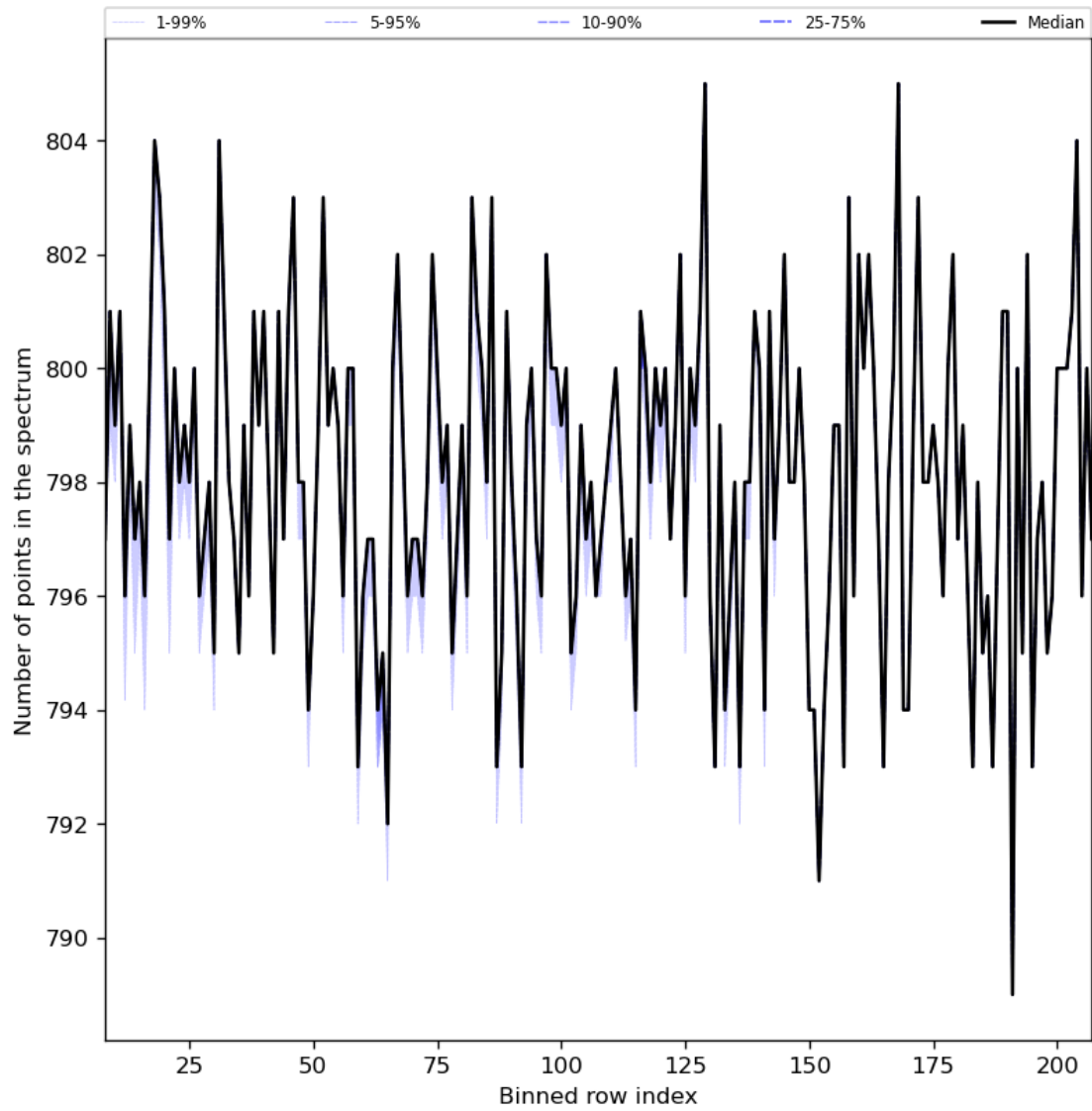
Figure 37: Along track statistics of “Number of points in the spectrum” for 2024-02-07 to 2024-02-09
