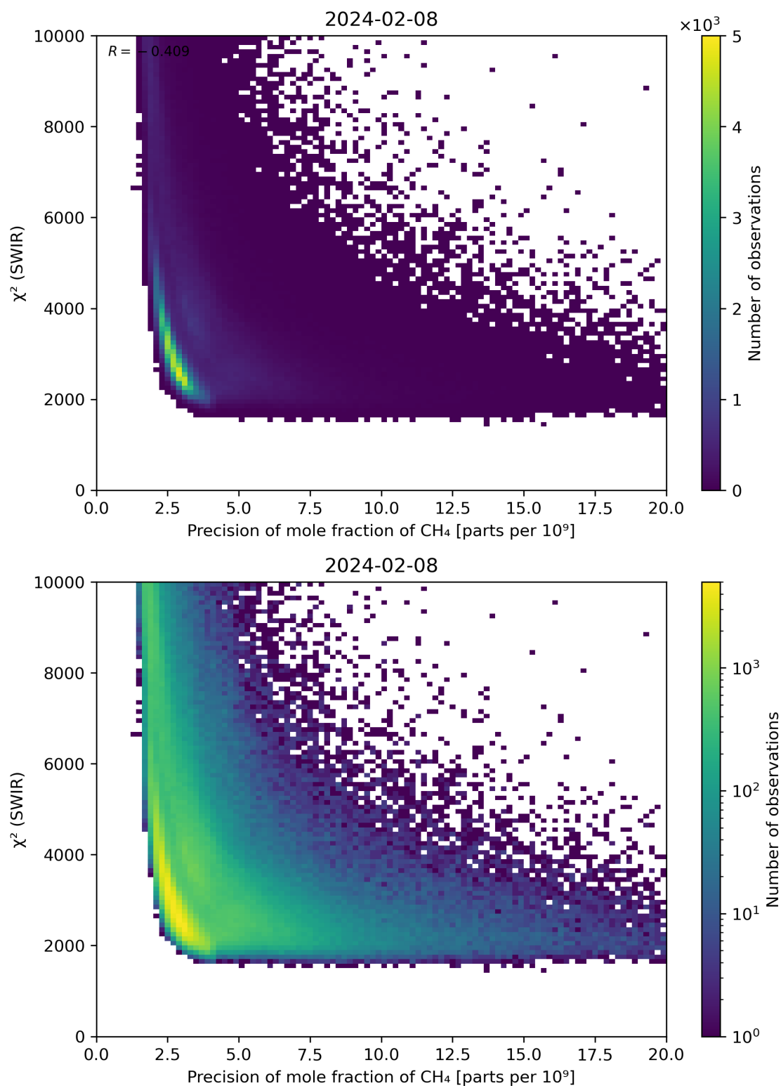
Figure 79: Scatter density plot of “Precision of mole fraction of \text{CH}_4 ” against “ \chi^2 (SWIR)” for 2024-02-07 to 2024-02-09.
