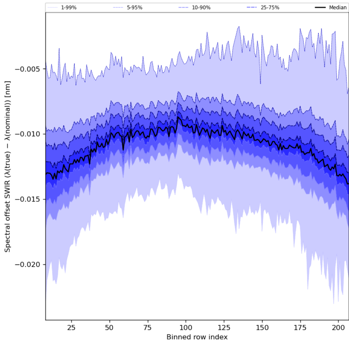
Figure 38: Along track statistics of “Spectral offset SWIR ( \lambda(\text{true}) - \lambda(\text{nominal}) )” for 2024-02-07 to 2024-02-09
