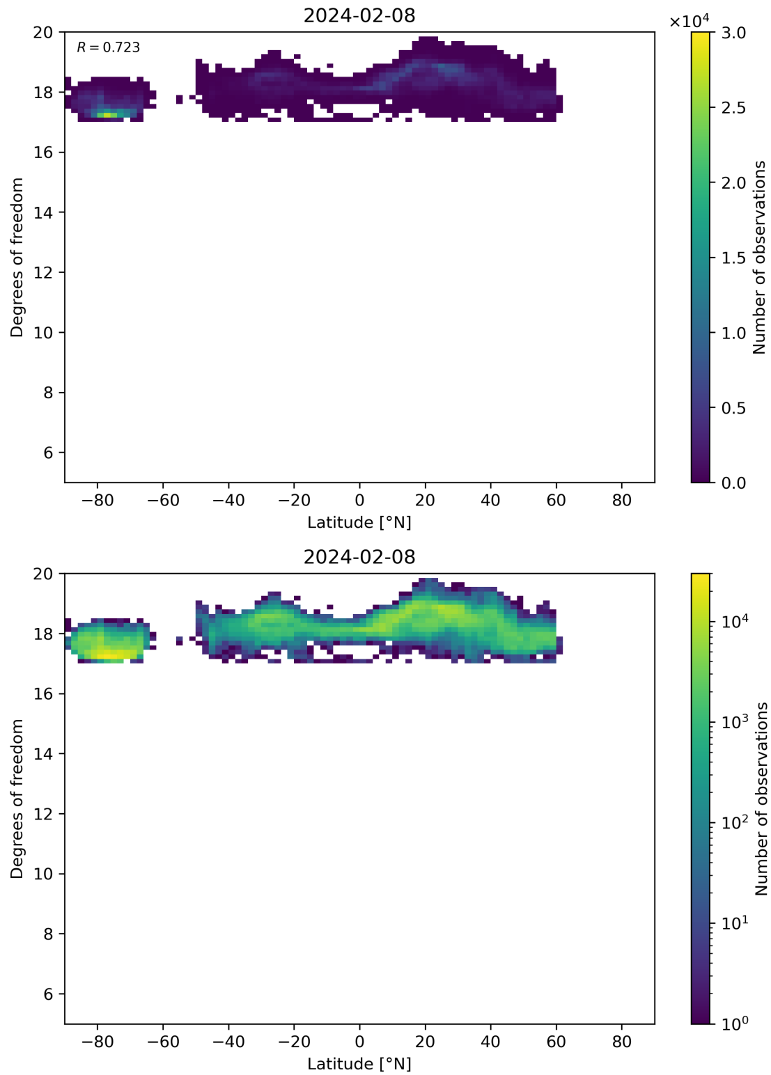
Figure 55: Scatter density plot of “Latitude” against “Degrees of freedom” for 2024-02-07 to 2024-02-09.
