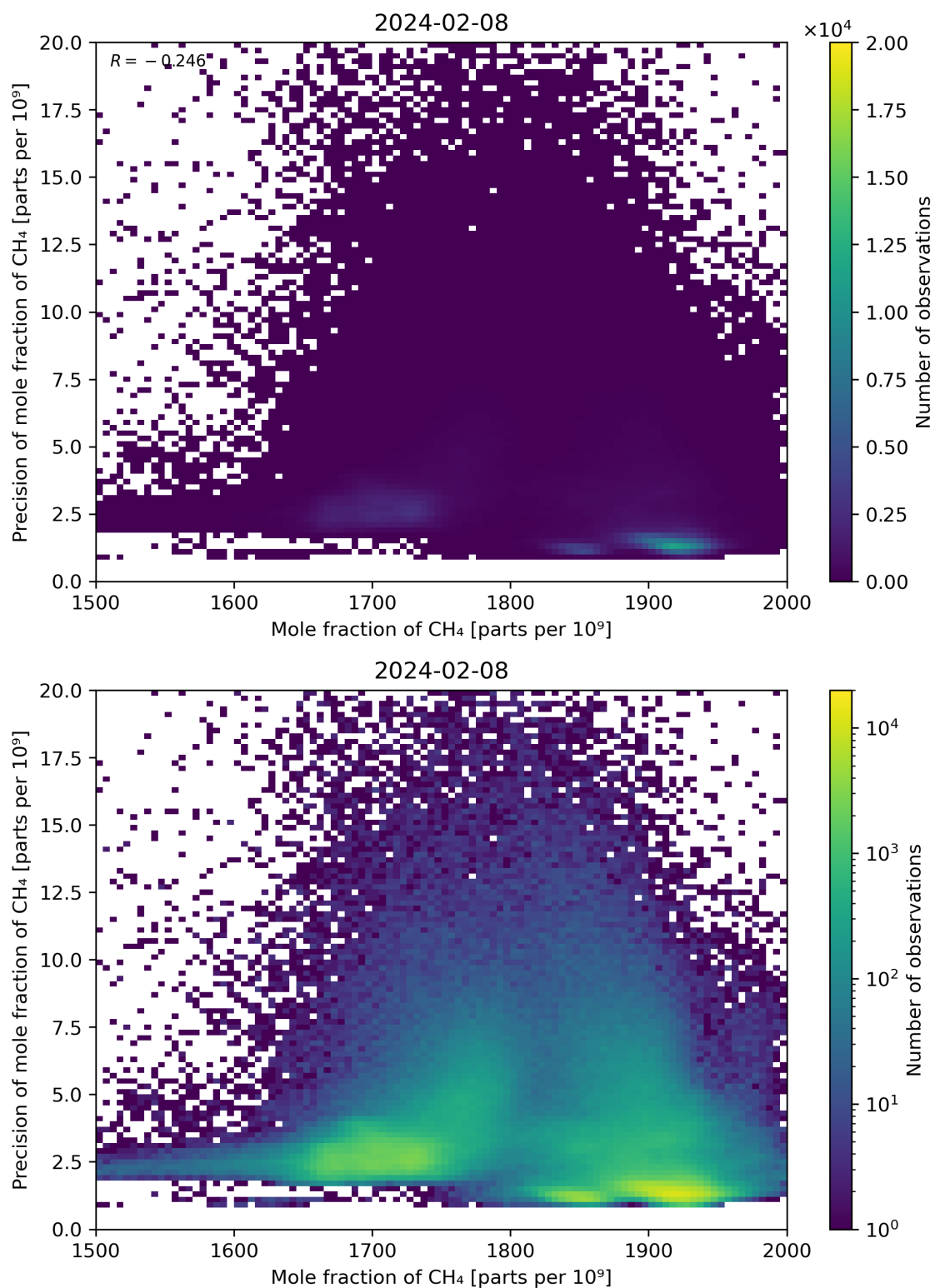
Figure 75: Scatter density plot of “Mole fraction of CH 4 ” against “Precision of mole fraction of CH 4 ” for 2024-02-07 to 2024-02-09.
