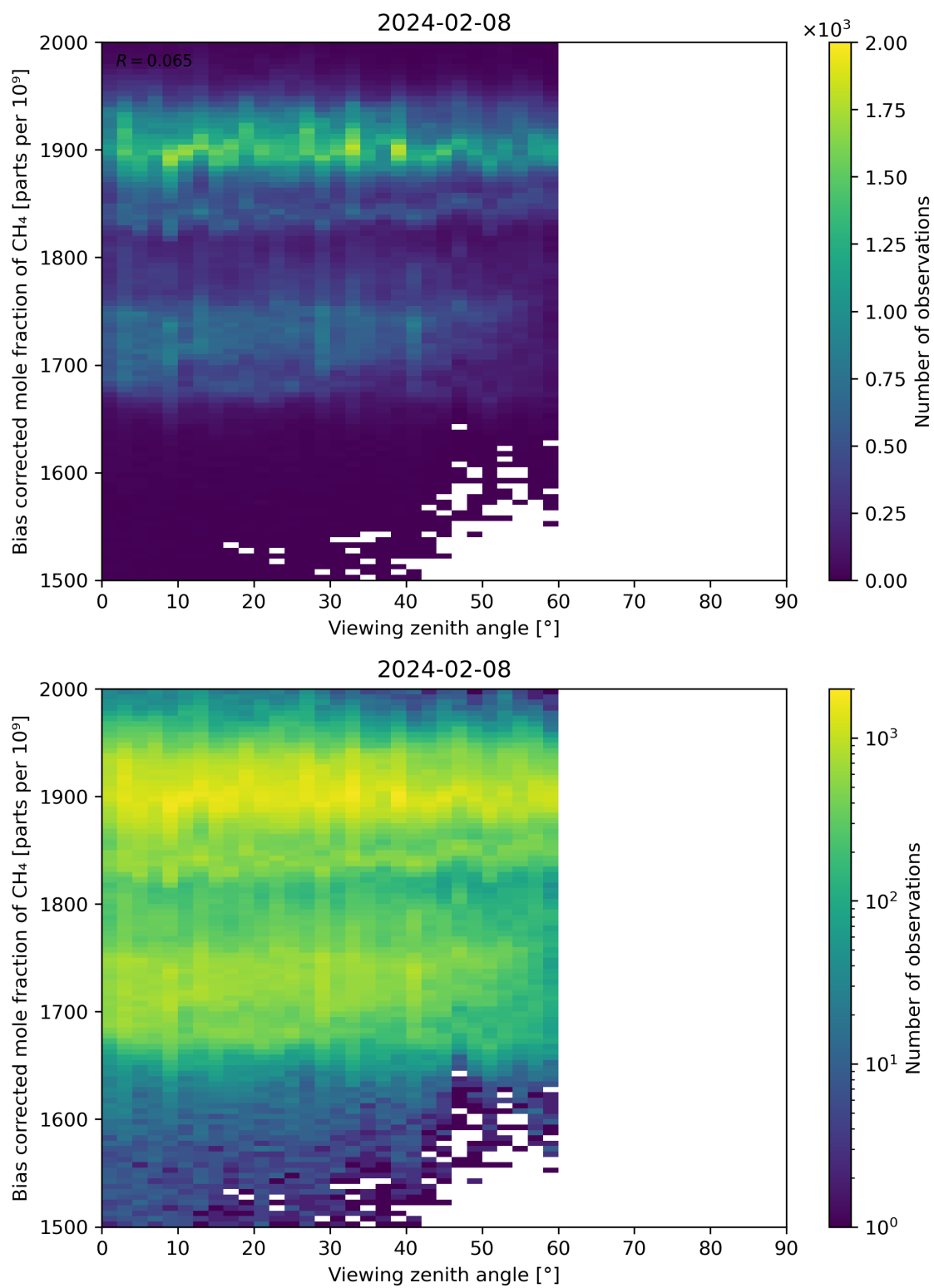
Figure 111: Scatter density plot of “Viewing zenith angle” against “Bias corrected mole fraction of CH 4 ” for 2024-02-07 to 2024-02-09.
