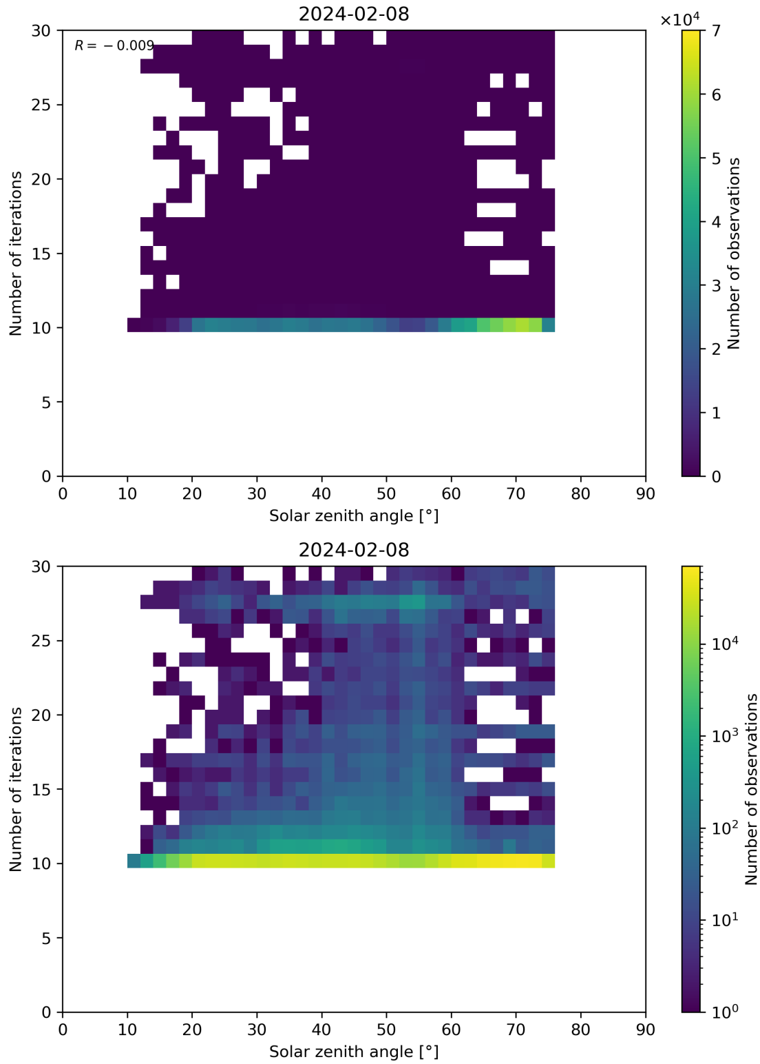
Figure 102: Scatter density plot of “Solar zenith angle” against “Number of iterations” for 2024-02-07 to 2024-02-09.
