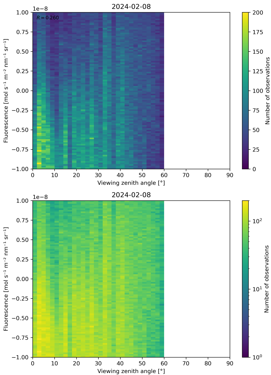
Figure 108: Scatter density plot of “Viewing zenith angle” against “Fluorescence” for 2024-02-07 to 2024-02-09.
