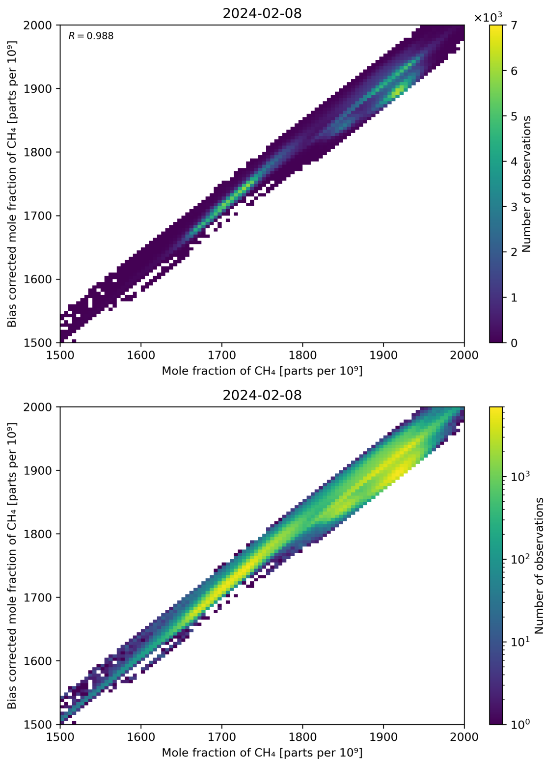
Figure 74: Scatter density plot of “Mole fraction of CH 4 ” against “Bias corrected mole fraction of CH 4 ” for 2024-02-07 to 2024-02-09.
