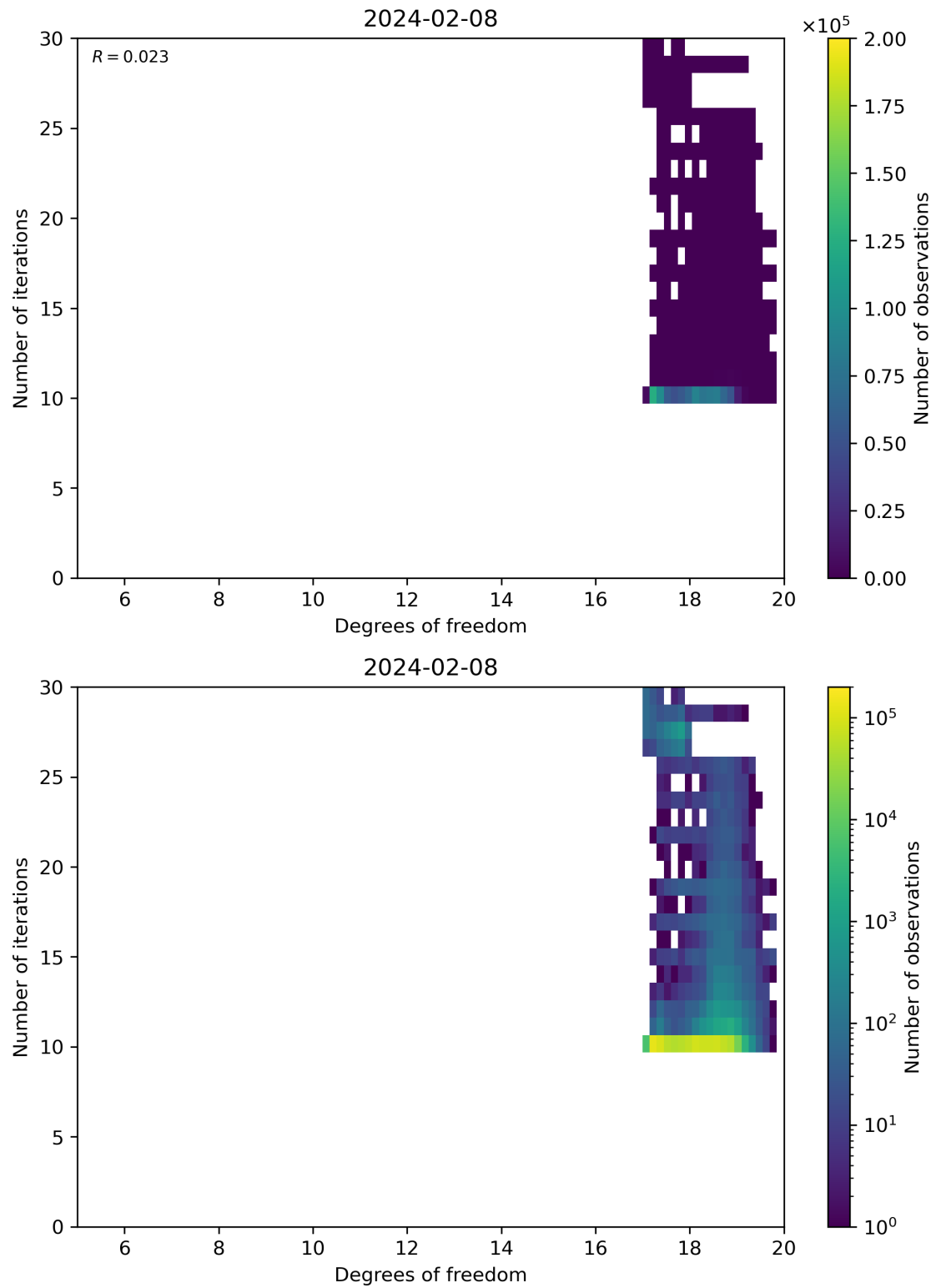
Figure 52: Scatter density plot of “Degrees of freedom” against “Number of iterations” for 2024-02-07 to 2024-02-09.
