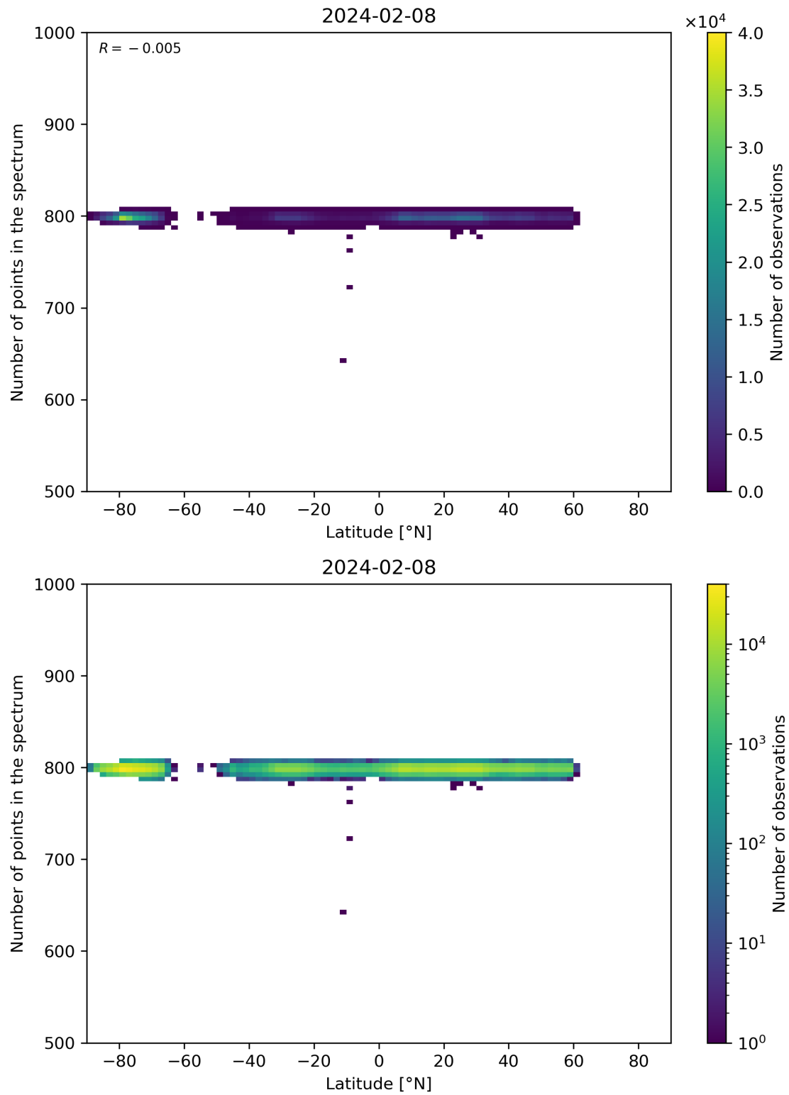
Figure 61: Scatter density plot of “Latitude” against “Number of points in the spectrum” for 2024-02-07 to 2024-02-09.
