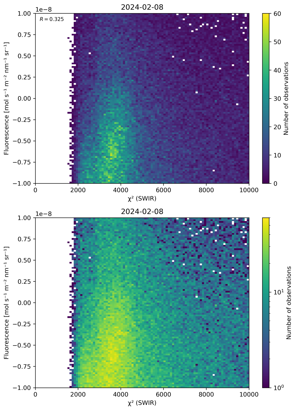
Figure 49: Scatter density plot of “ \chi^2 (SWIR)” against “Fluorescence” for 2024-02-07 to 2024-02-09.
