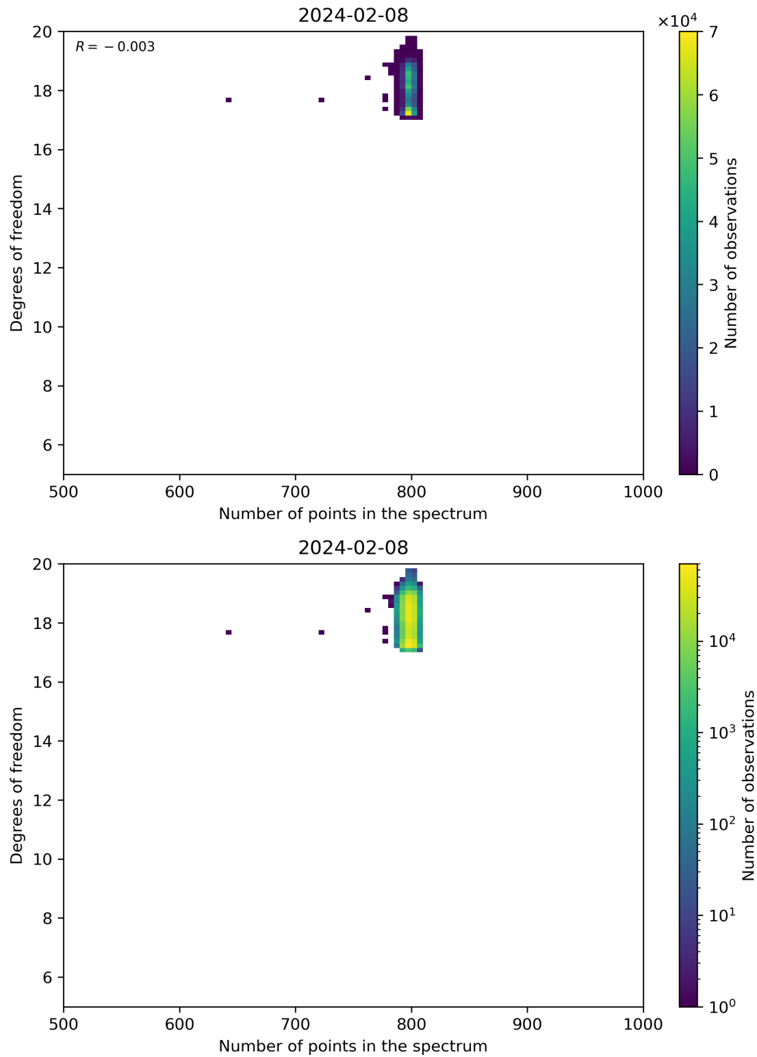
Figure 90: Scatter density plot of “Number of points in the spectrum” against “Degrees of freedom” for 2024-02-07 to 2024-02-09.
