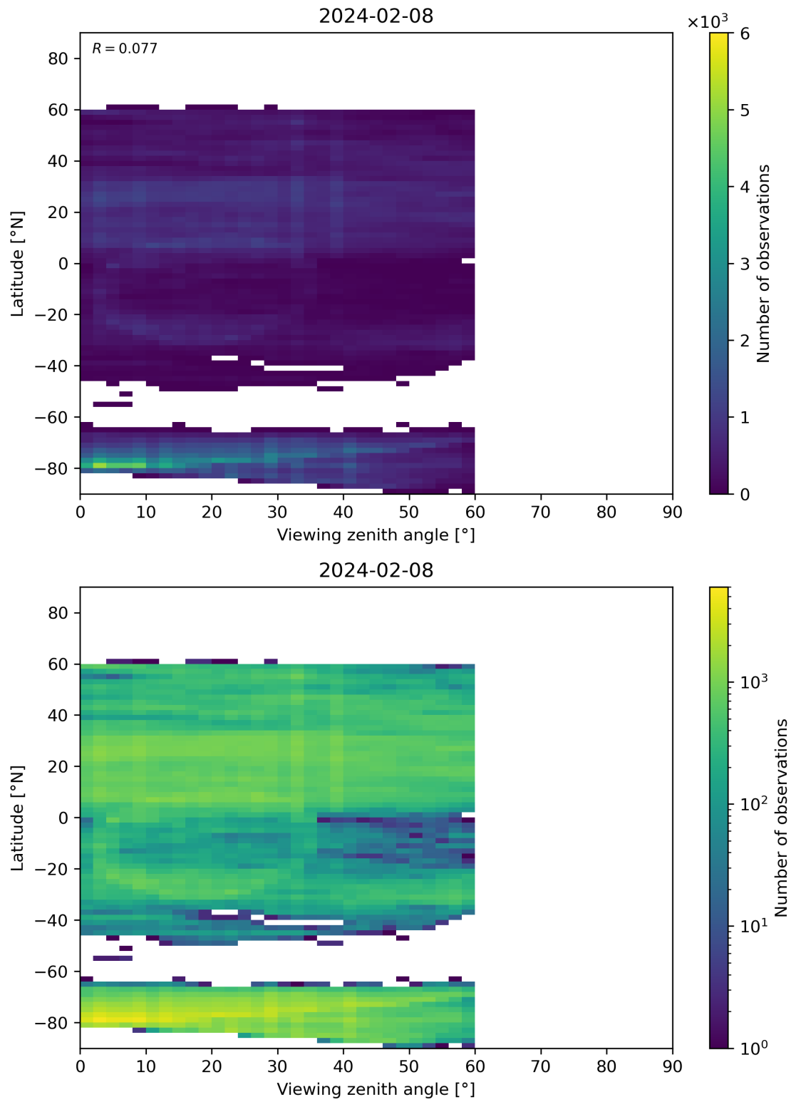
Figure 109: Scatter density plot of “Viewing zenith angle” against “Latitude” for 2024-02-07 to 2024-02-09.
