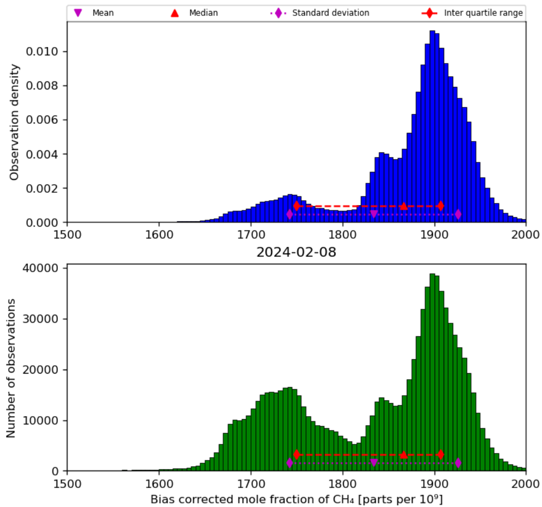
Figure 25: Histogram of “Bias corrected mole fraction of CH 4 ” for 2024-02-07 to 2024-02-09
