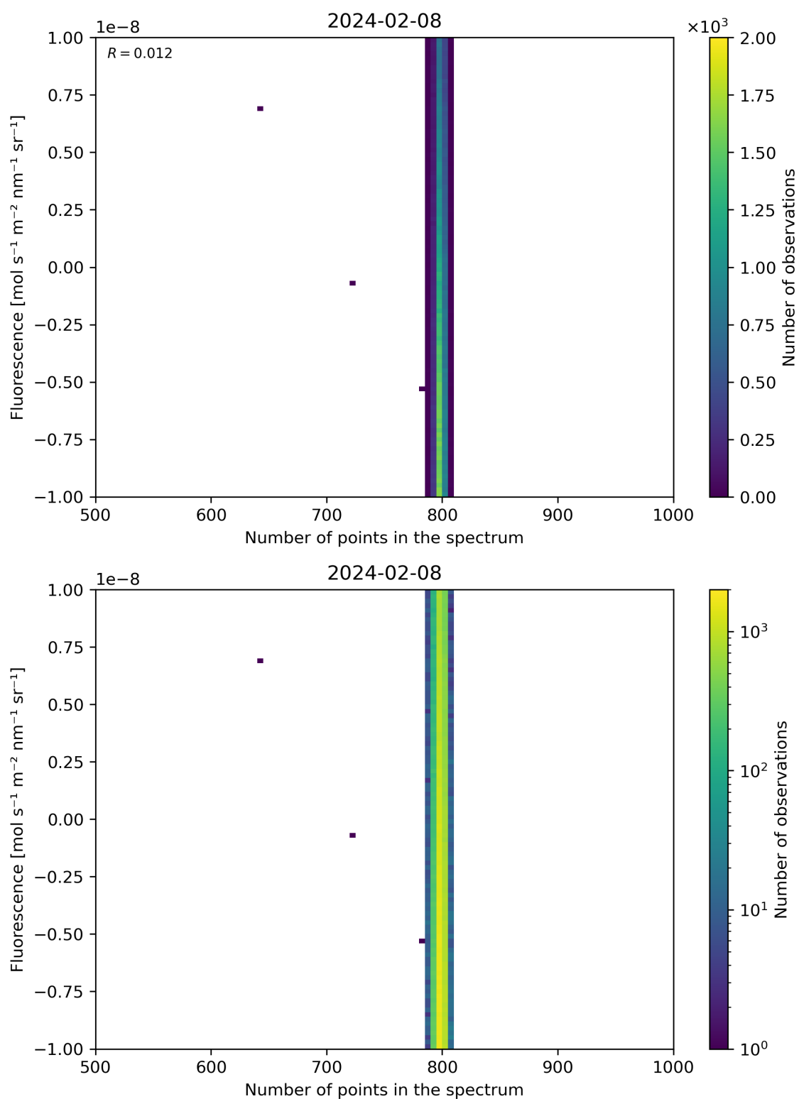
Figure 91: Scatter density plot of “Number of points in the spectrum” against “Fluorescence” for 2024-02-07 to 2024-02-09.
