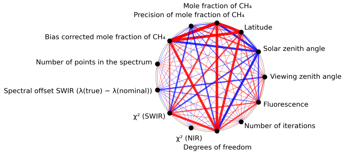
Figure 1: Map of correlation graph for 2024-02-07 to 2024-02-09.
