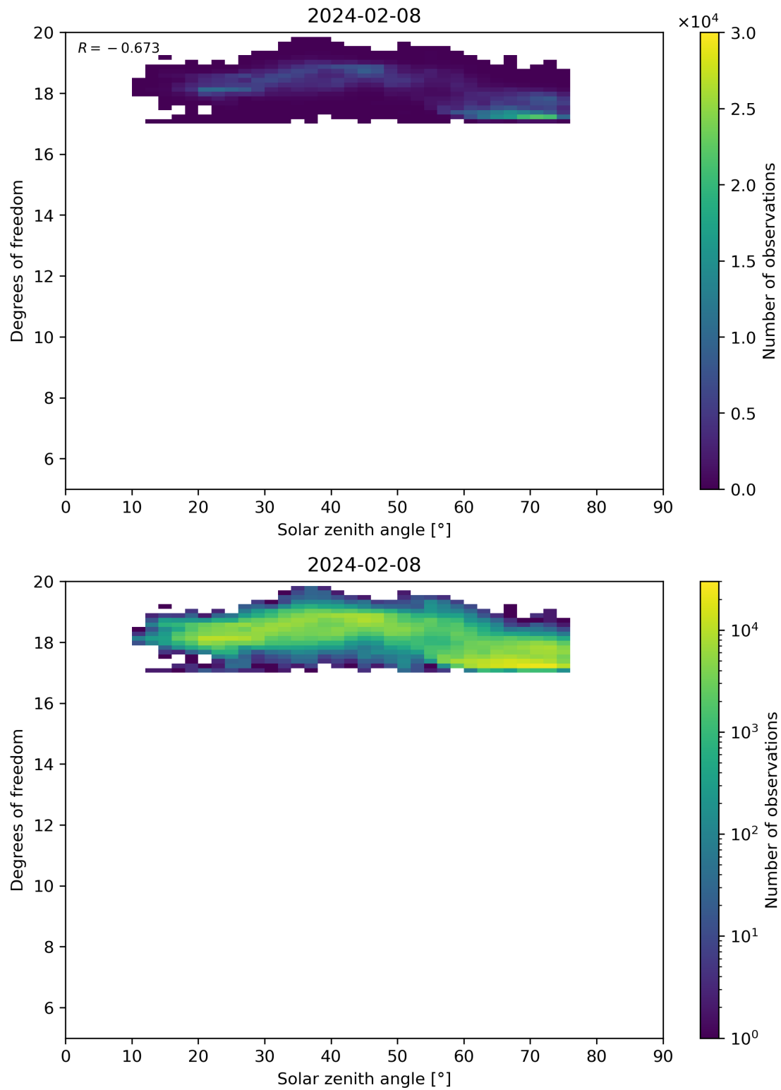
Figure 96: Scatter density plot of “Solar zenith angle” against “Degrees of freedom” for 2024-02-07 to 2024-02-09.
