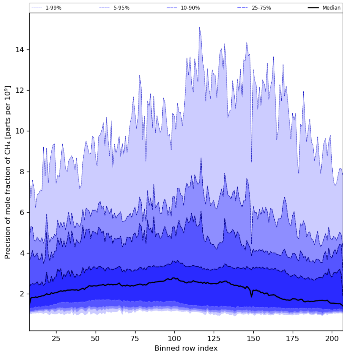
Figure 35: Along track statistics of “Precision of mole fraction of CH 4 ” for 2024-02-07 to 2024-02-09
