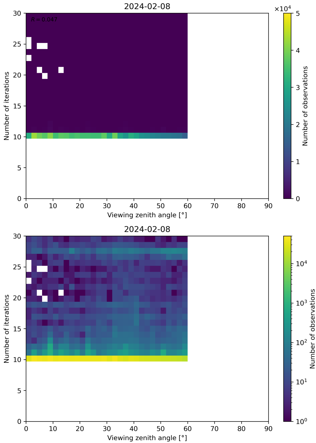
Figure 113: Scatter density plot of “Viewing zenith angle” against “Number of iterations” for 2024-02-07 to 2024-02-09.
