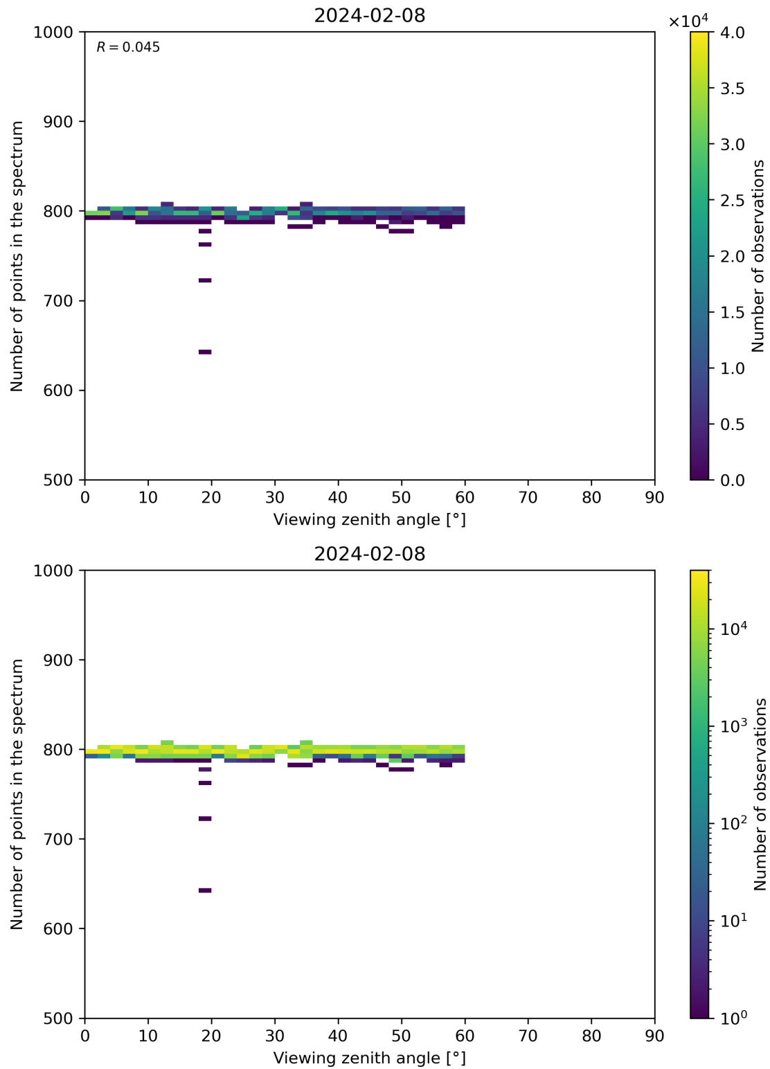
Figure 114: Scatter density plot of “Viewing zenith angle” against “Number of points in the spectrum” for 2024-02-07 to 2024-02-09.
