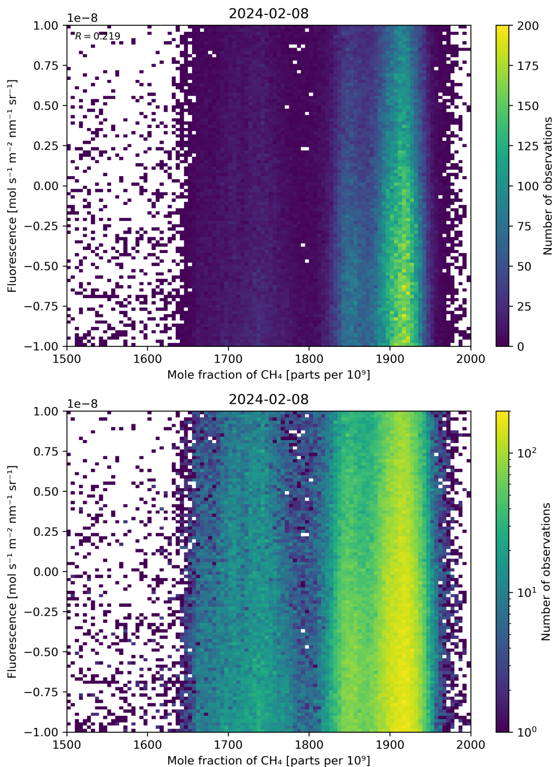
Figure 73: Scatter density plot of “Mole fraction of CH 4 ” against “Fluorescence” for 2024-02-07 to 2024-02-09.
