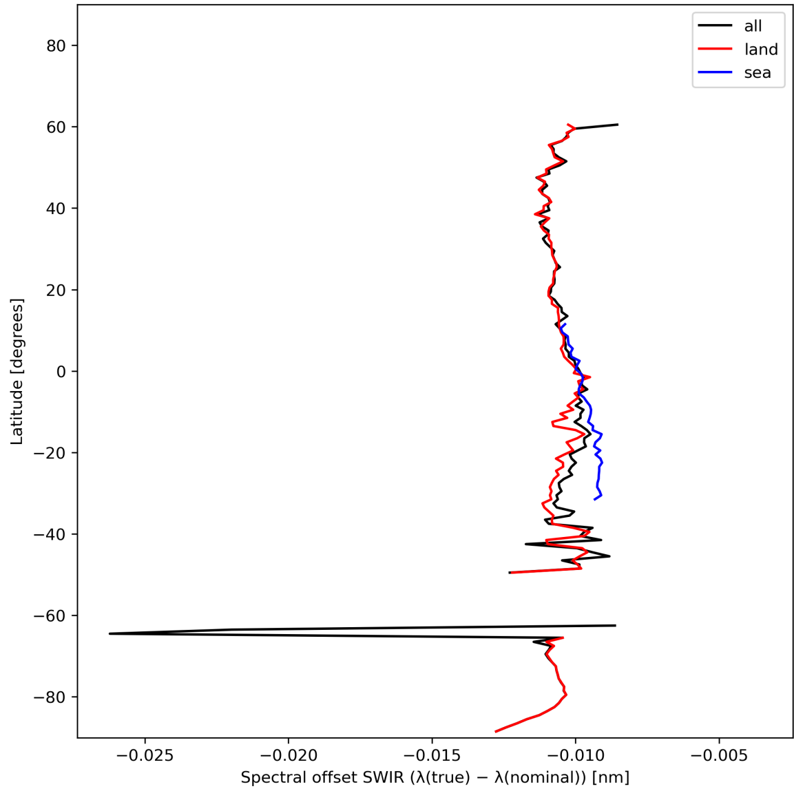
Figure 16: Zonal average of “Spectral offset SWIR ( \lambda(\text{true}) - \lambda(\text{nominal}) )” for 2024-02-07 to 2024-02-09.
