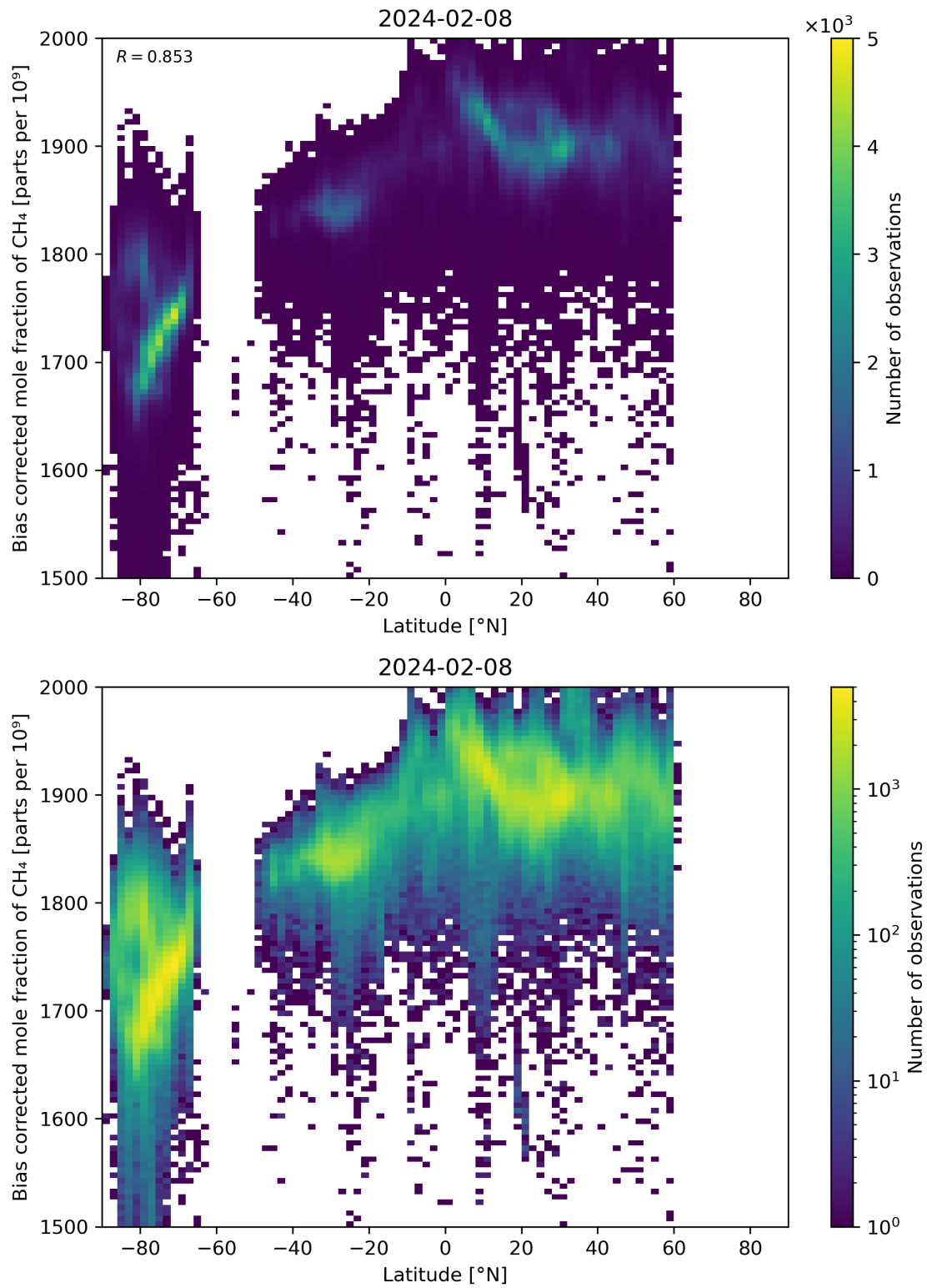
Figure 58: Scatter density plot of “Latitude” against “Bias corrected mole fraction of \text{CH}_4 ” for 2024-02-07 to 2024-02-09.
