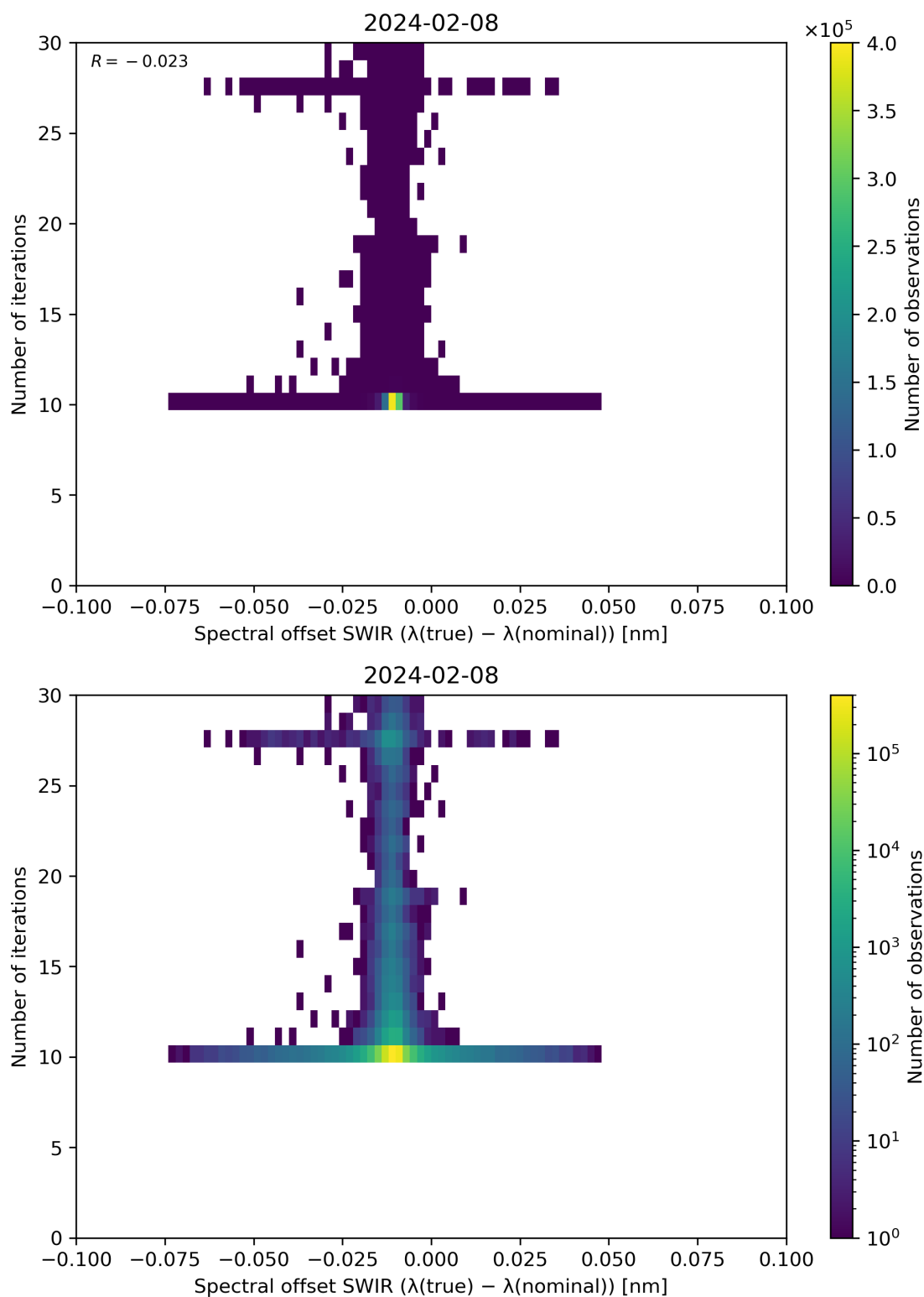
Figure 121: Scatter density plot of “Spectral offset SWIR ( \lambda(\text{true}) - \lambda(\text{nominal}) )” against “Number of iterations” for 2024-02-07 to 2024-02-09.
