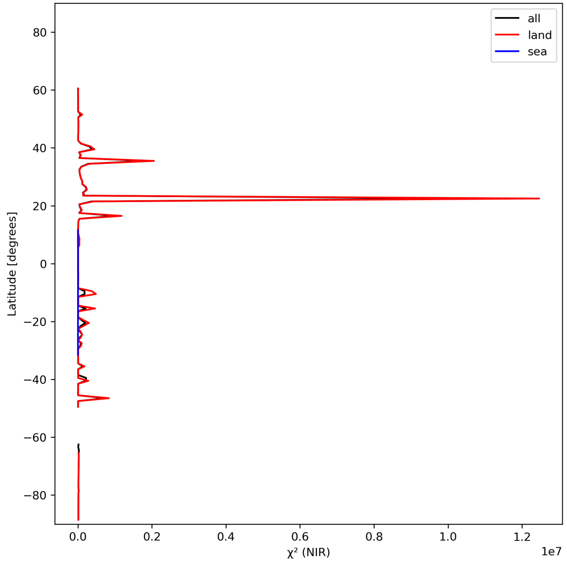
Figure 18: Zonal average of “ \chi^2 (NIR)” for 2024-02-07 to 2024-02-09.
