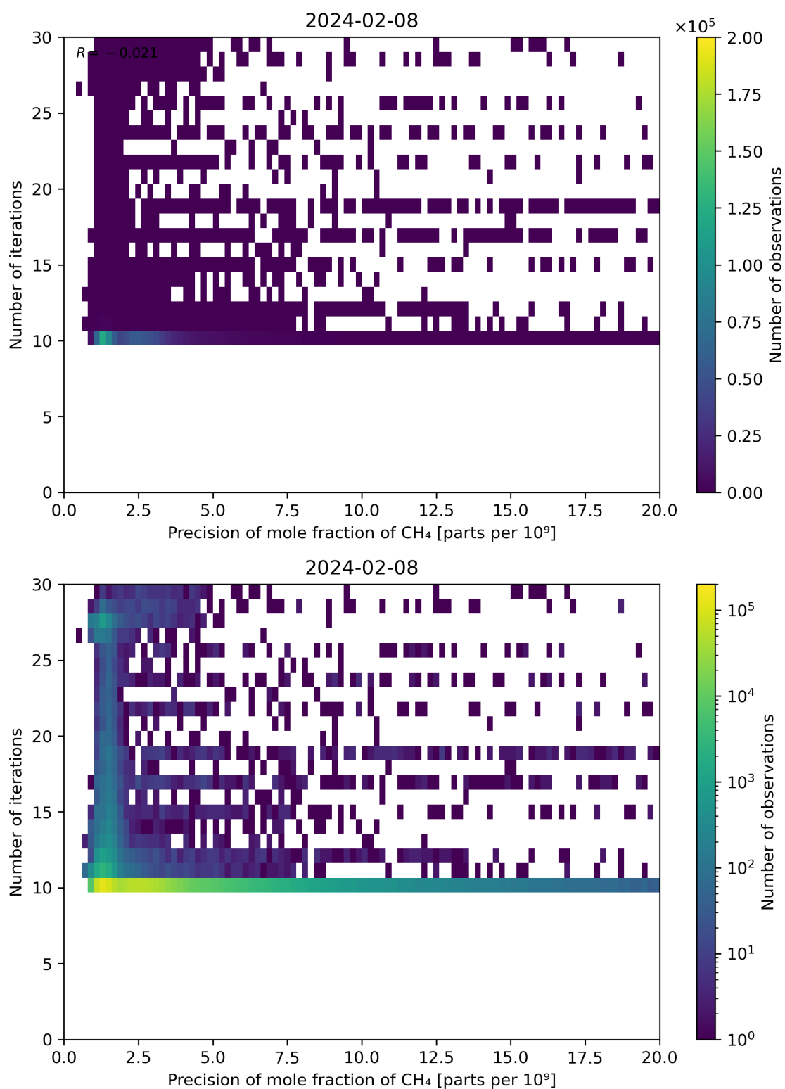
Figure 83: Scatter density plot of “Precision of mole fraction of CH 4 ” against “Number of iterations” for 2024-02-07 to 2024-02-09.
