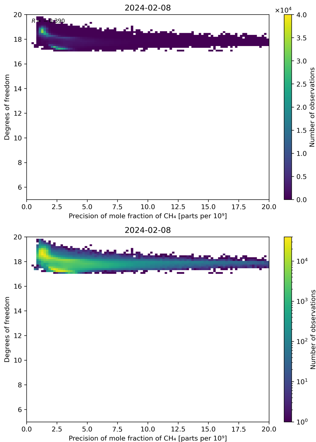
Figure 80: Scatter density plot of “Precision of mole fraction of CH 4 ” against “Degrees of freedom” for 2024-02-07 to 2024-02-09.
