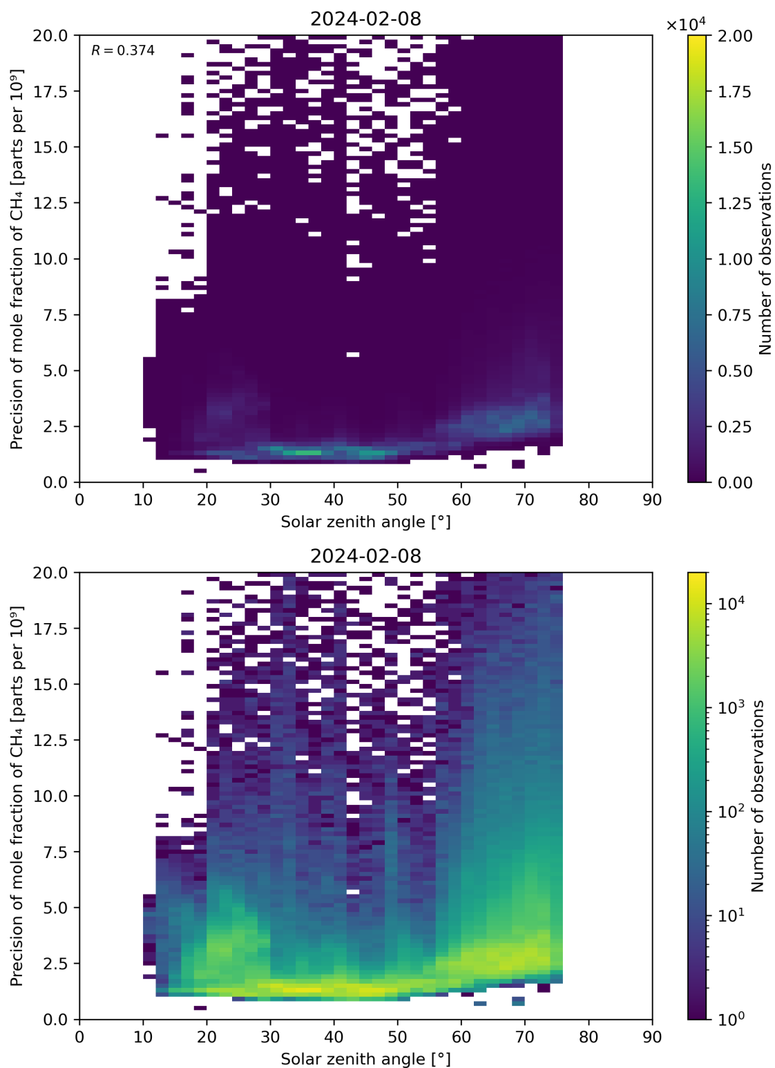
Figure 101: Scatter density plot of “Solar zenith angle” against “Precision of mole fraction of \text{CH}_4 ” for 2024-02-07 to 2024-02-09.
