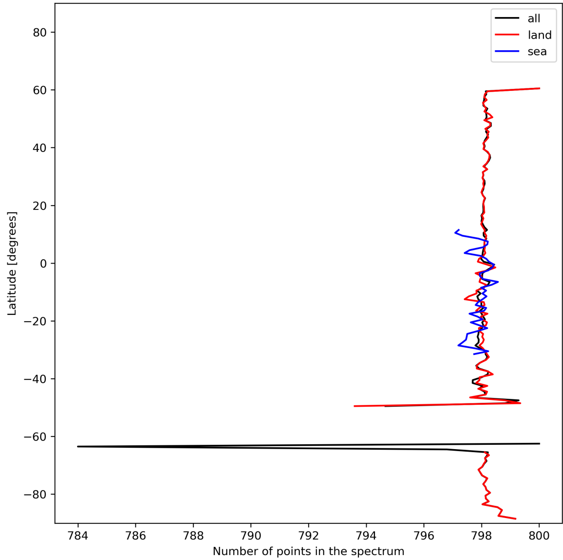
Figure 15: Zonal average of “Number of points in the spectrum” for 2024-02-07 to 2024-02-09.
