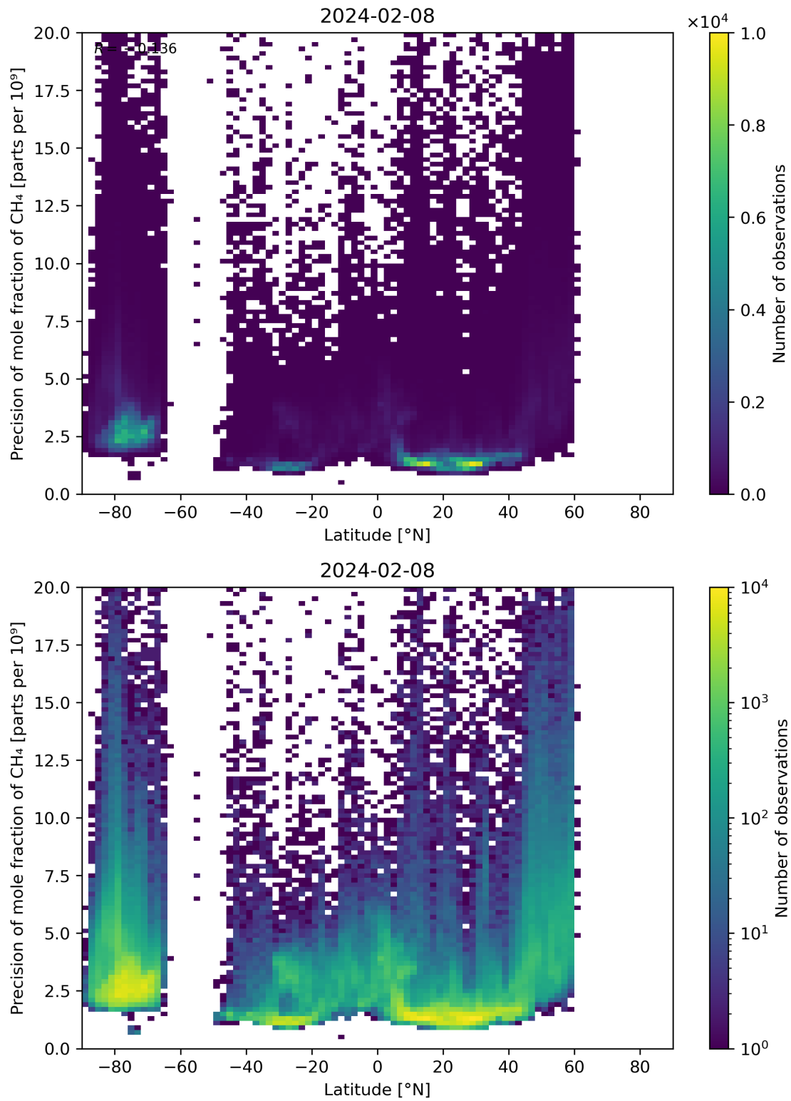
Figure 59: Scatter density plot of “Latitude” against “Precision of mole fraction of CH 4 ” for 2024-02-07 to 2024-02-09.
