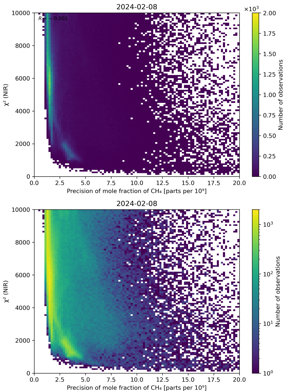
Figure 78: Scatter density plot of “Precision of mole fraction of CH 4 ” against “ \chi^2 (NIR)” for 2024-02-07 to 2024-02-09.
