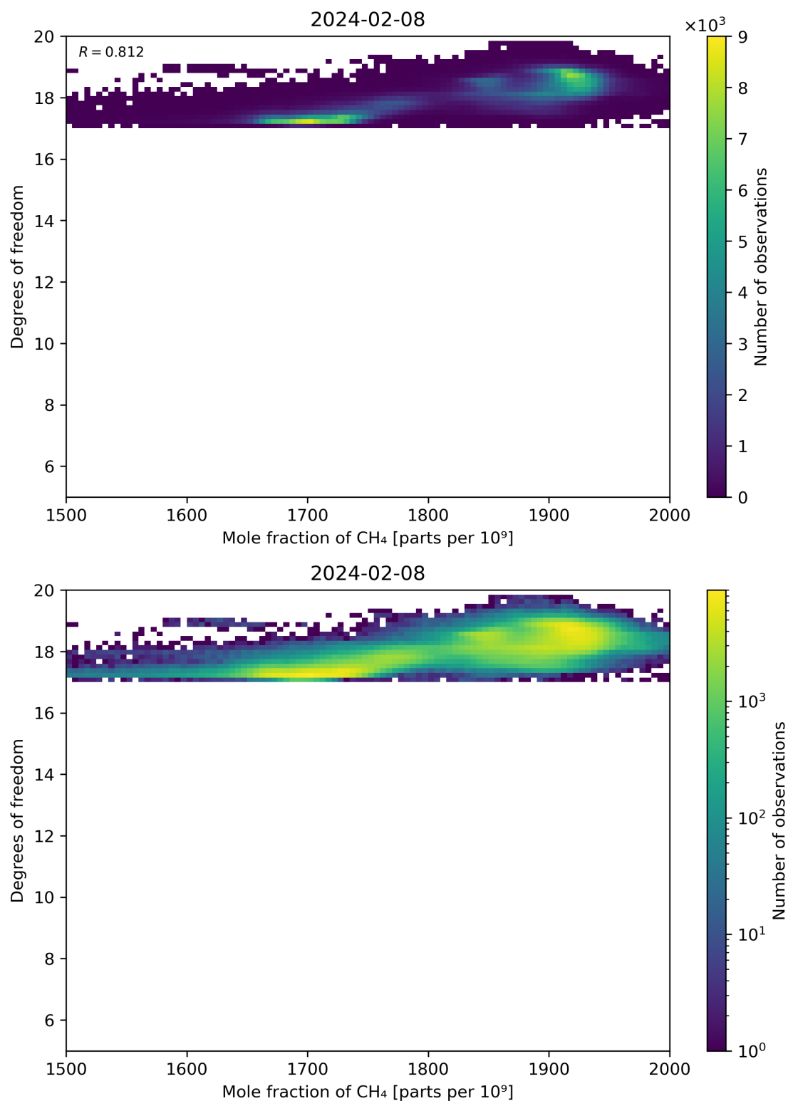
Figure 72: Scatter density plot of “Mole fraction of CH 4 ” against “Degrees of freedom” for 2024-02-07 to 2024-02-09.
