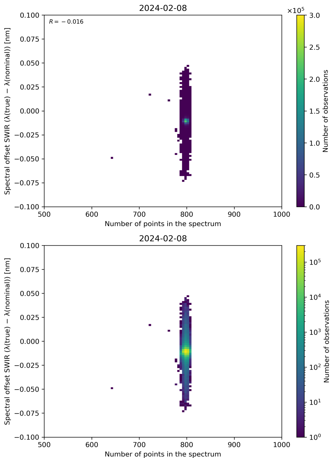
Figure 93: Scatter density plot of “Number of points in the spectrum” against “Spectral offset SWIR ( \lambda(\text{true}) - \lambda(\text{nominal}) )” for 2024-02-07 to 2024-02-09.
