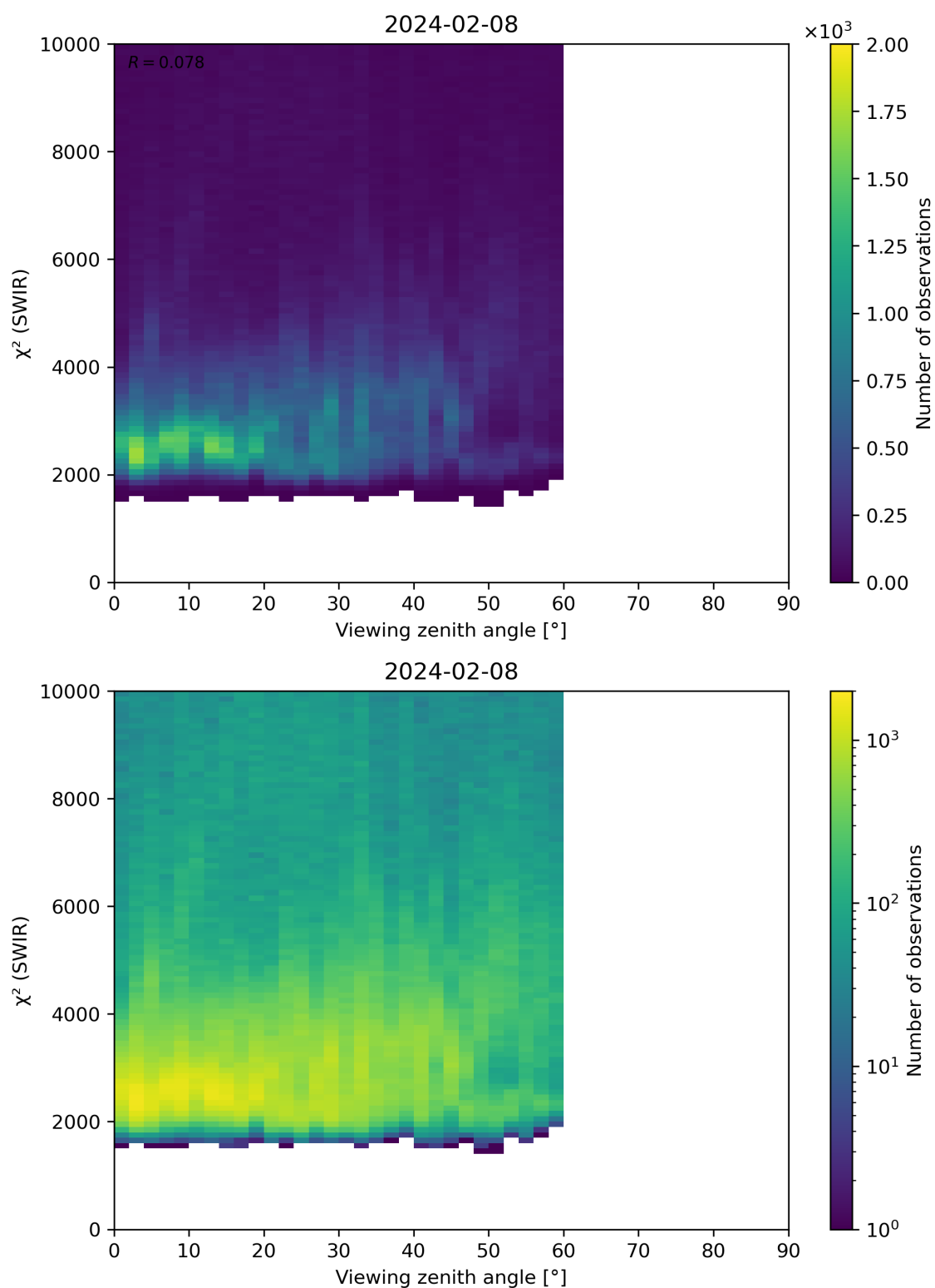
Figure 106: Scatter density plot of “Viewing zenith angle” against “ \chi^2 (SWIR)” for 2024-02-07 to 2024-02-09.
