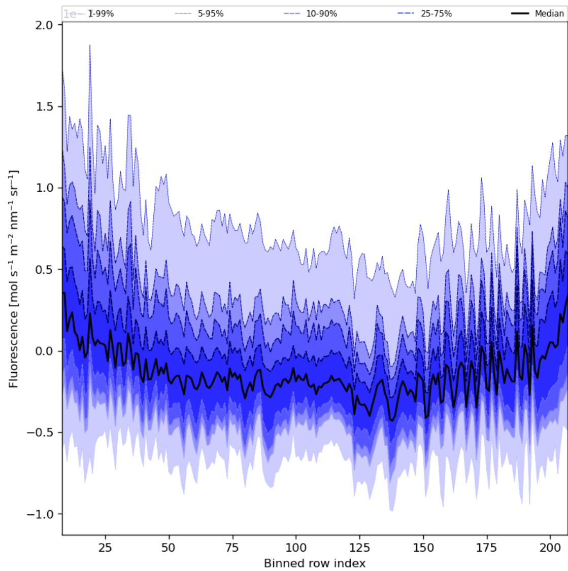
Figure 43: Along track statistics of “Fluorescence” for 2024-02-07 to 2024-02-09
