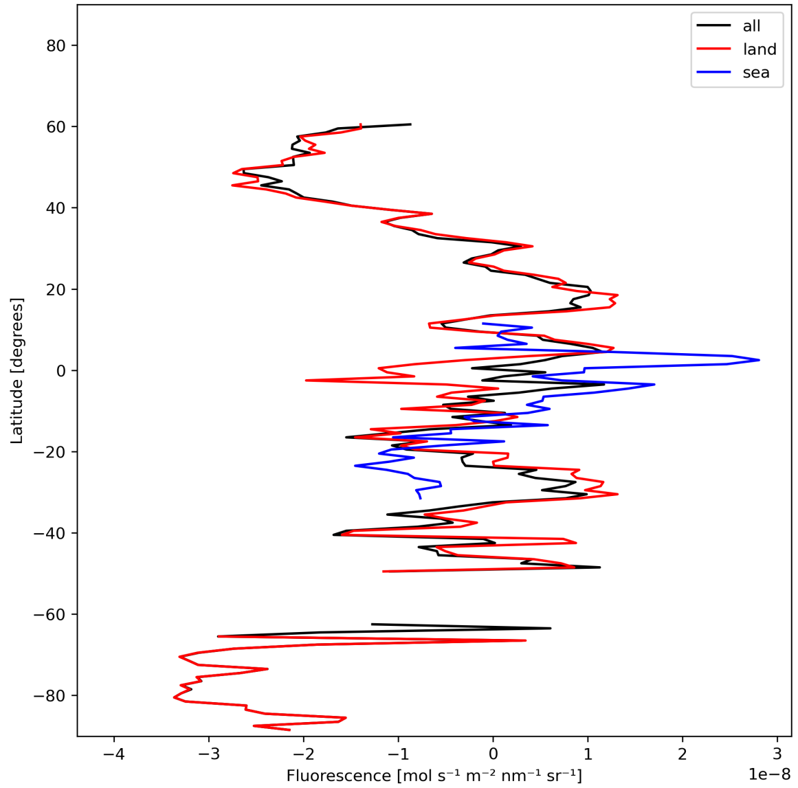
Figure 21: Zonal average of “Fluorescence” for 2024-02-07 to 2024-02-09.
