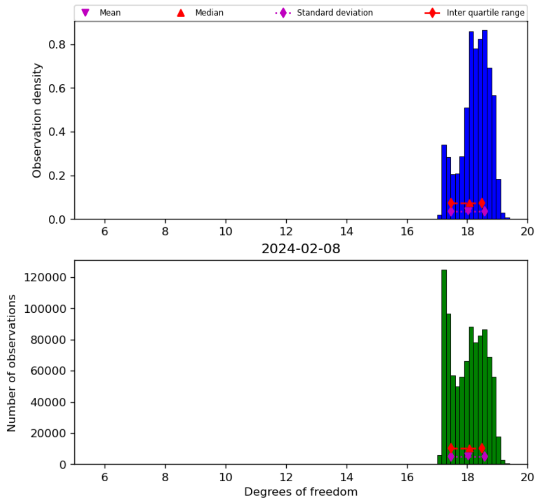
Figure 30: Histogram of “Degrees of freedom” for 2024-02-07 to 2024-02-09
