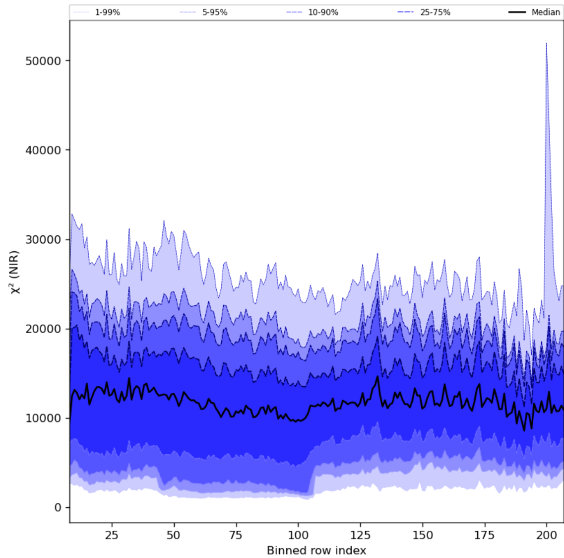
Figure 40: Along track statistics of “ \chi^2 (NIR)” for 2024-02-07 to 2024-02-09
