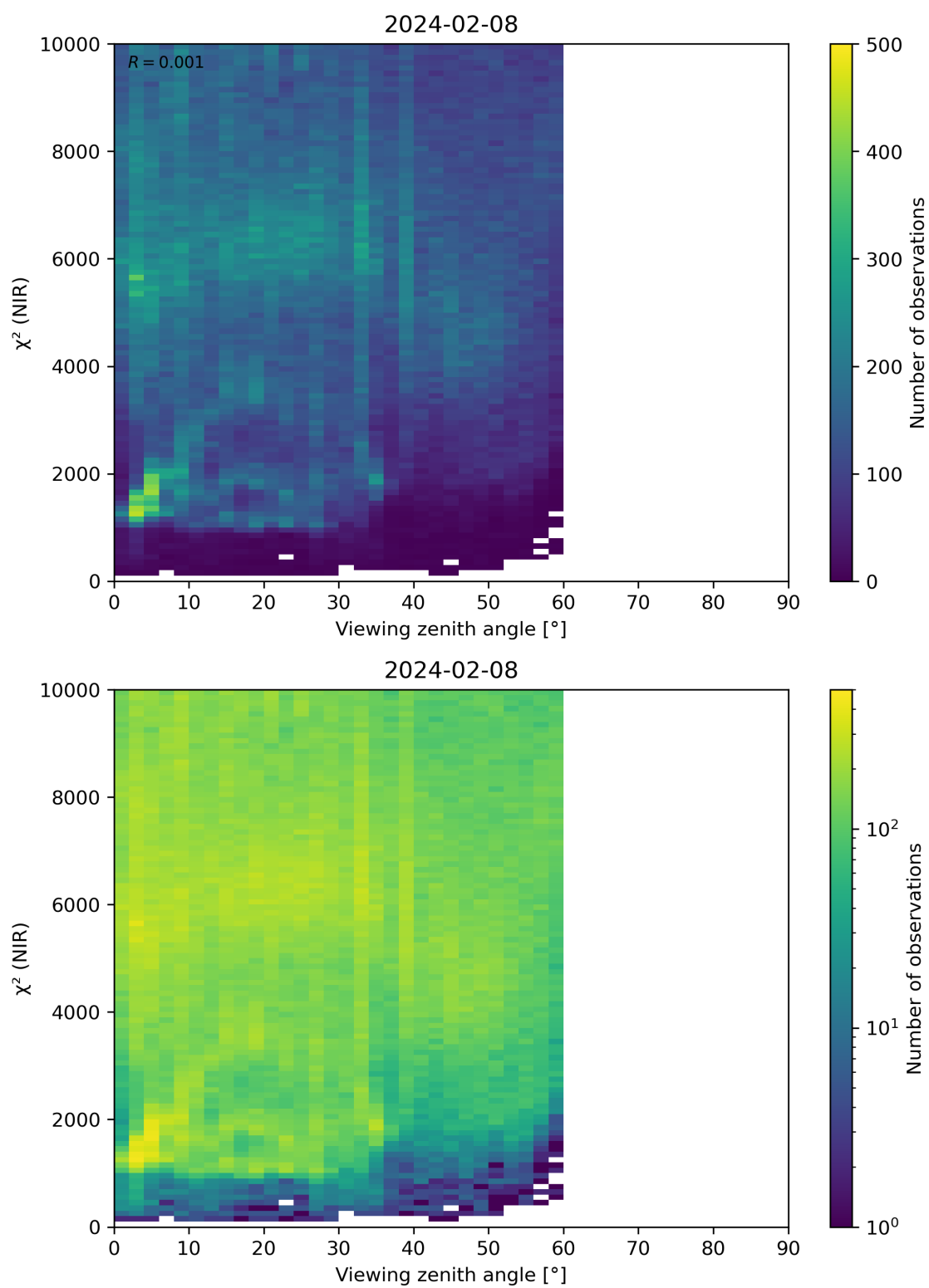
Figure 105: Scatter density plot of “Viewing zenith angle” against “ \chi^2 (NIR)” for 2024-02-07 to 2024-02-09.
