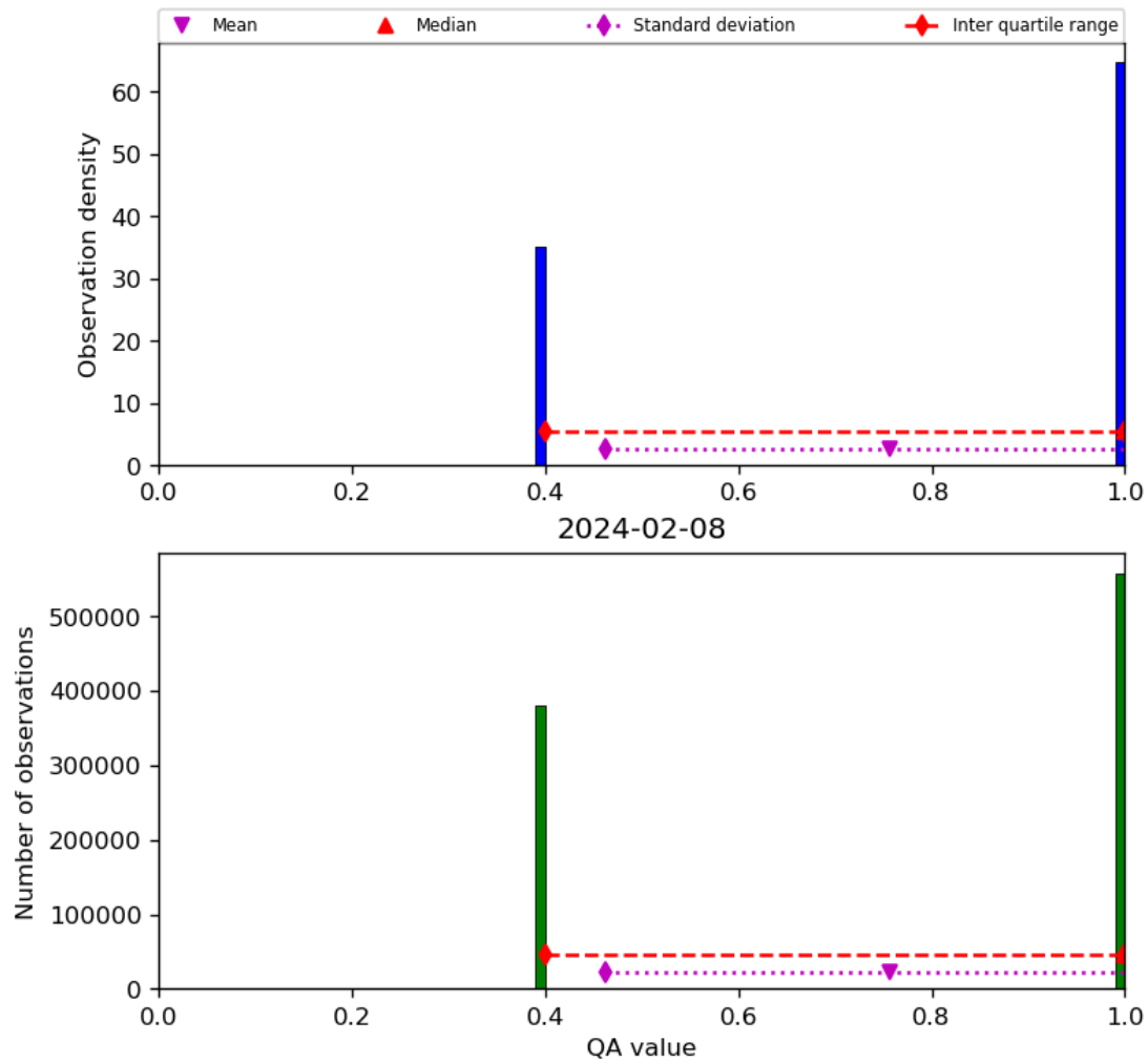
Figure 22: Histogram of “QA value” for 2024-02-07 to 2024-02-09
