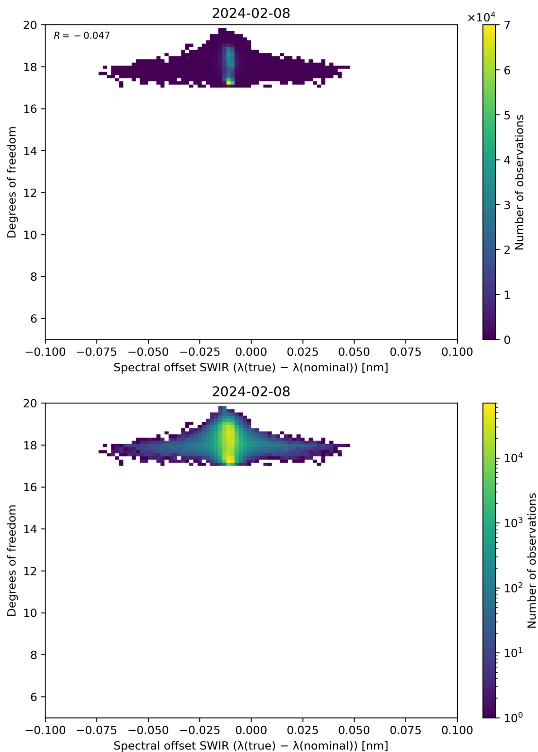
Figure 119: Scatter density plot of “Spectral offset SWIR ( \lambda(\text{true}) - \lambda(\text{nominal}) )” against “Degrees of freedom” for 2024-02-07 to 2024-02-09.
