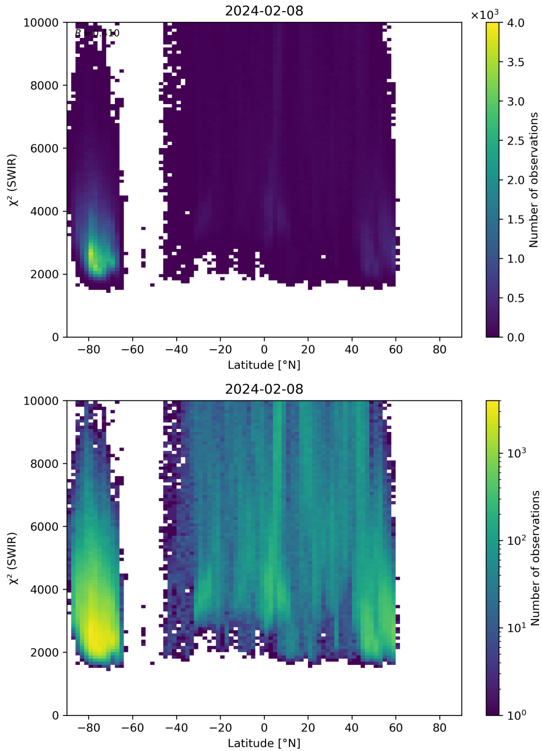
Figure 54: Scatter density plot of “Latitude” against “ \chi^2 (SWIR)” for 2024-02-07 to 2024-02-09.
