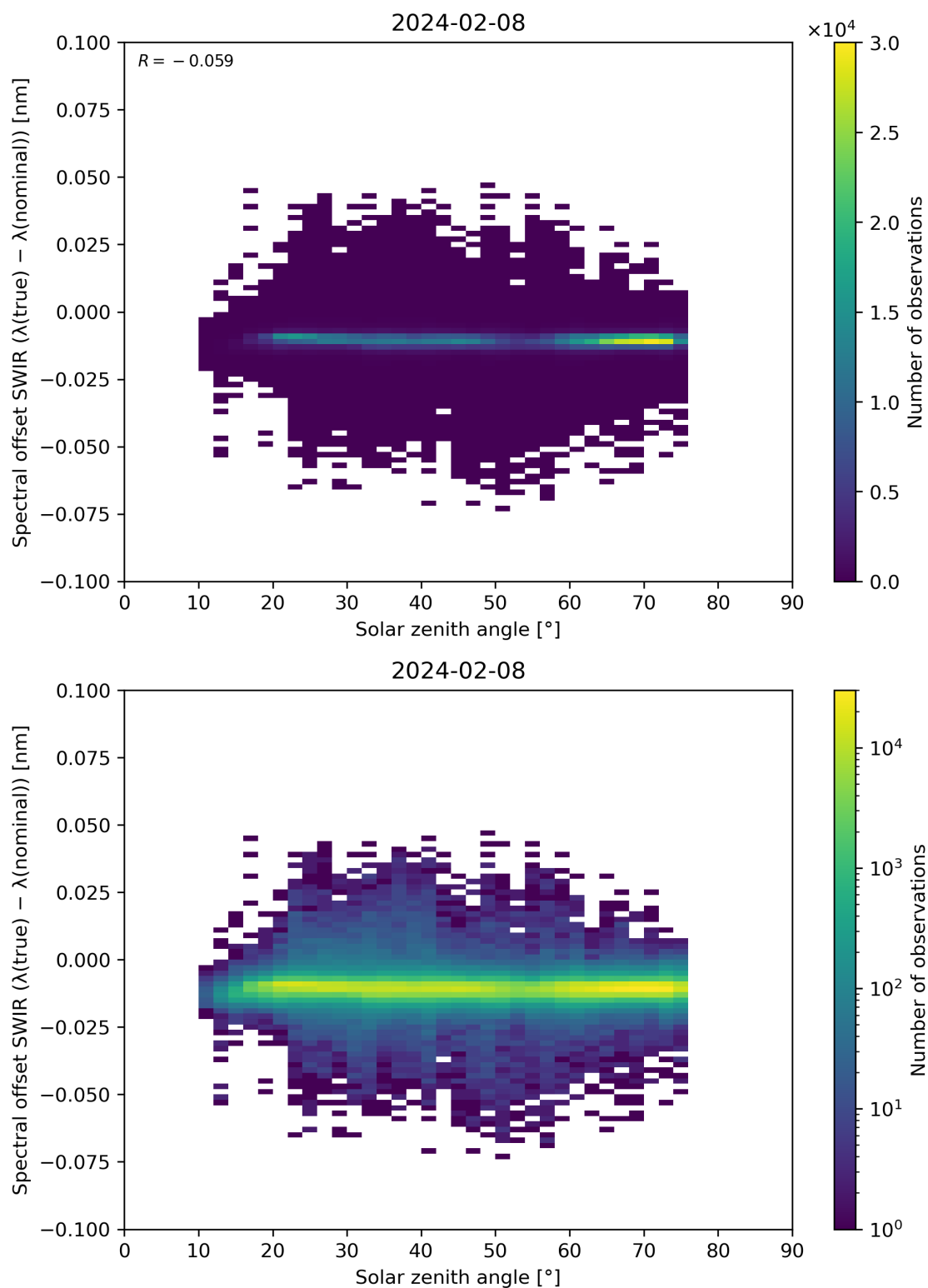
Figure 104: Scatter density plot of “Solar zenith angle” against “Spectral offset SWIR ( \lambda(\text{true}) - \lambda(\text{nominal}) )” for 2024-02-07 to 2024-02-09.
