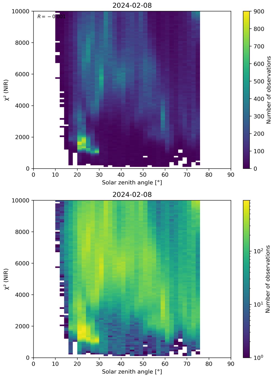
Figure 94: Scatter density plot of “Solar zenith angle” against “ \chi^2 (NIR)” for 2024-02-07 to 2024-02-09.
