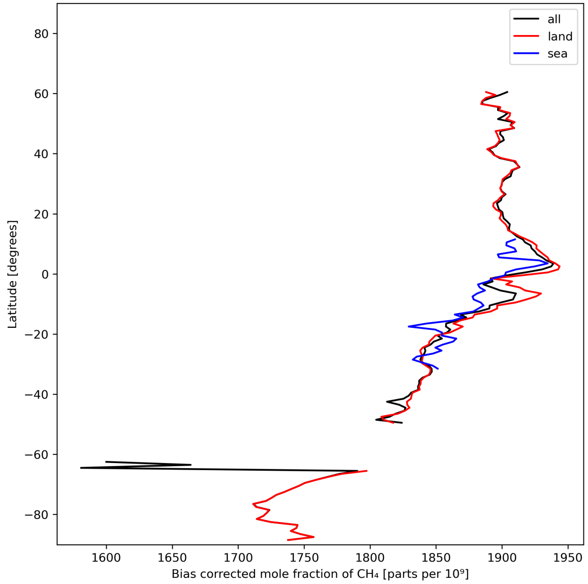
Figure 14: Zonal average of “Bias corrected mole fraction of CH 4 ” for 2024-02-07 to 2024-02-09.
