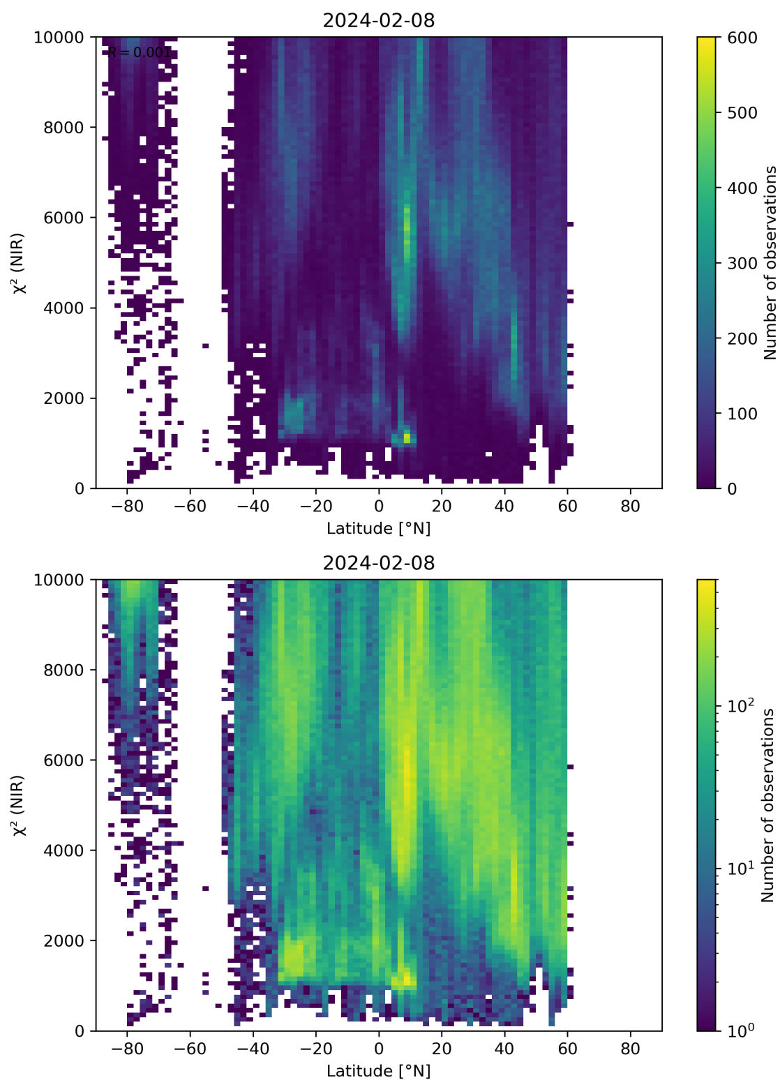
Figure 53: Scatter density plot of “Latitude” against “ \chi^2 (NIR)” for 2024-02-07 to 2024-02-09.
