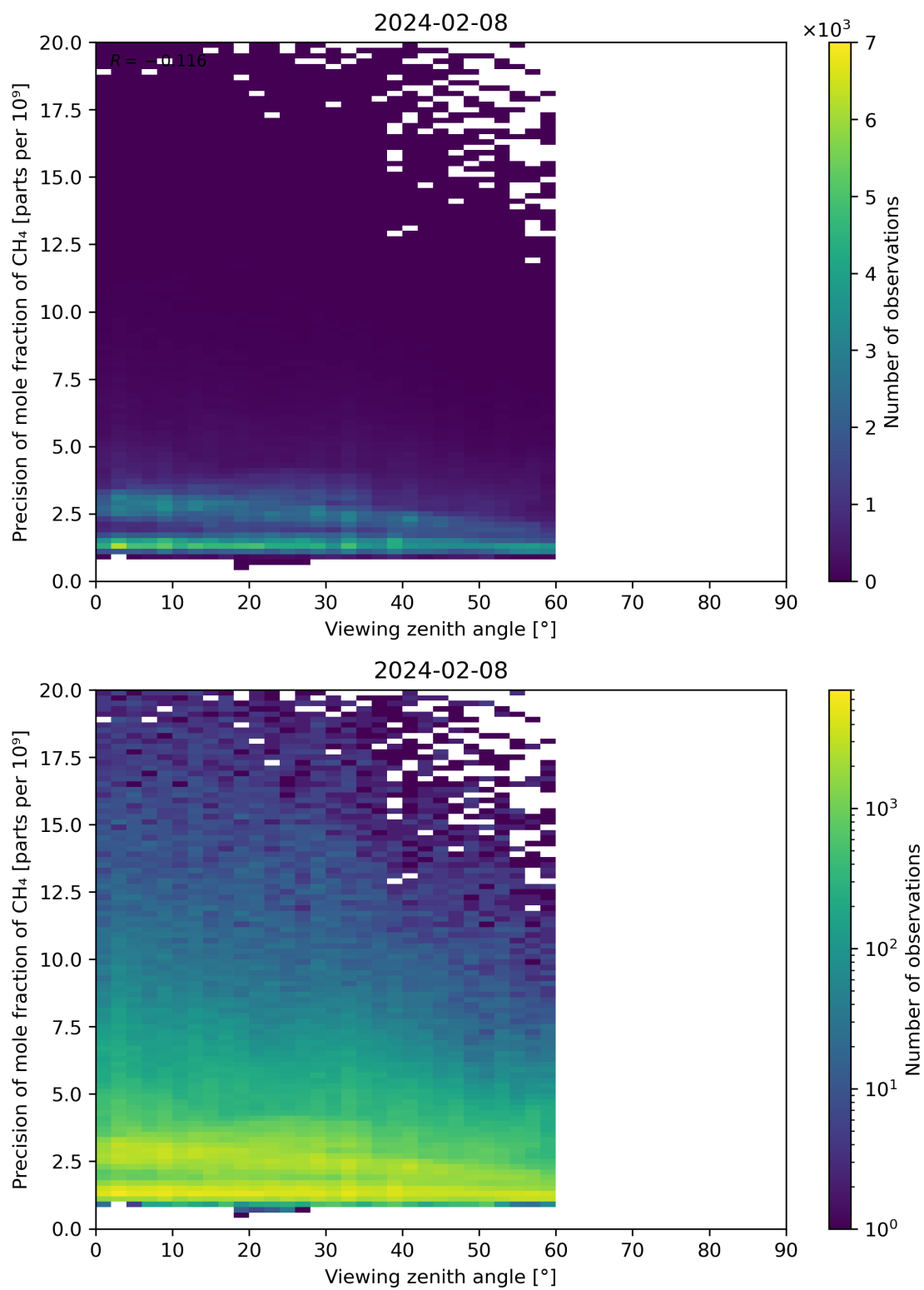
Figure 112: Scatter density plot of “Viewing zenith angle” against “Precision of mole fraction of CH 4 ” for 2024-02-07 to 2024-02-09.
