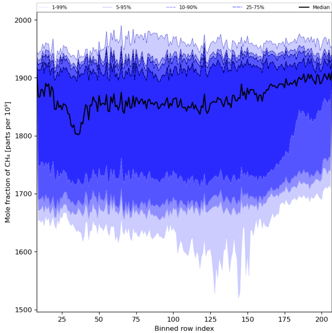
Figure 34: Along track statistics of “Mole fraction of CH 4 ” for 2024-02-07 to 2024-02-09
