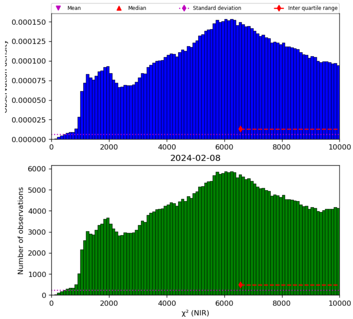
Figure 29: Histogram of “ \chi^2 (NIR)” for 2024-02-07 to 2024-02-09
