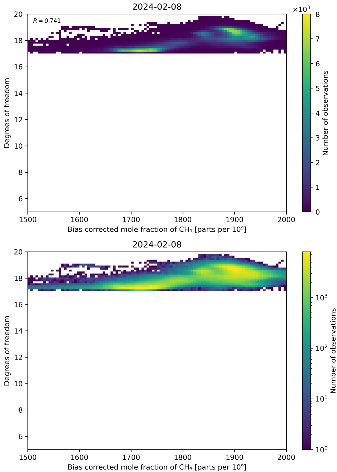
Figure 65: Scatter density plot of “Bias corrected mole fraction of CH 4 ” against “Degrees of freedom” for 2024-02-07 to 2024-02-09.
