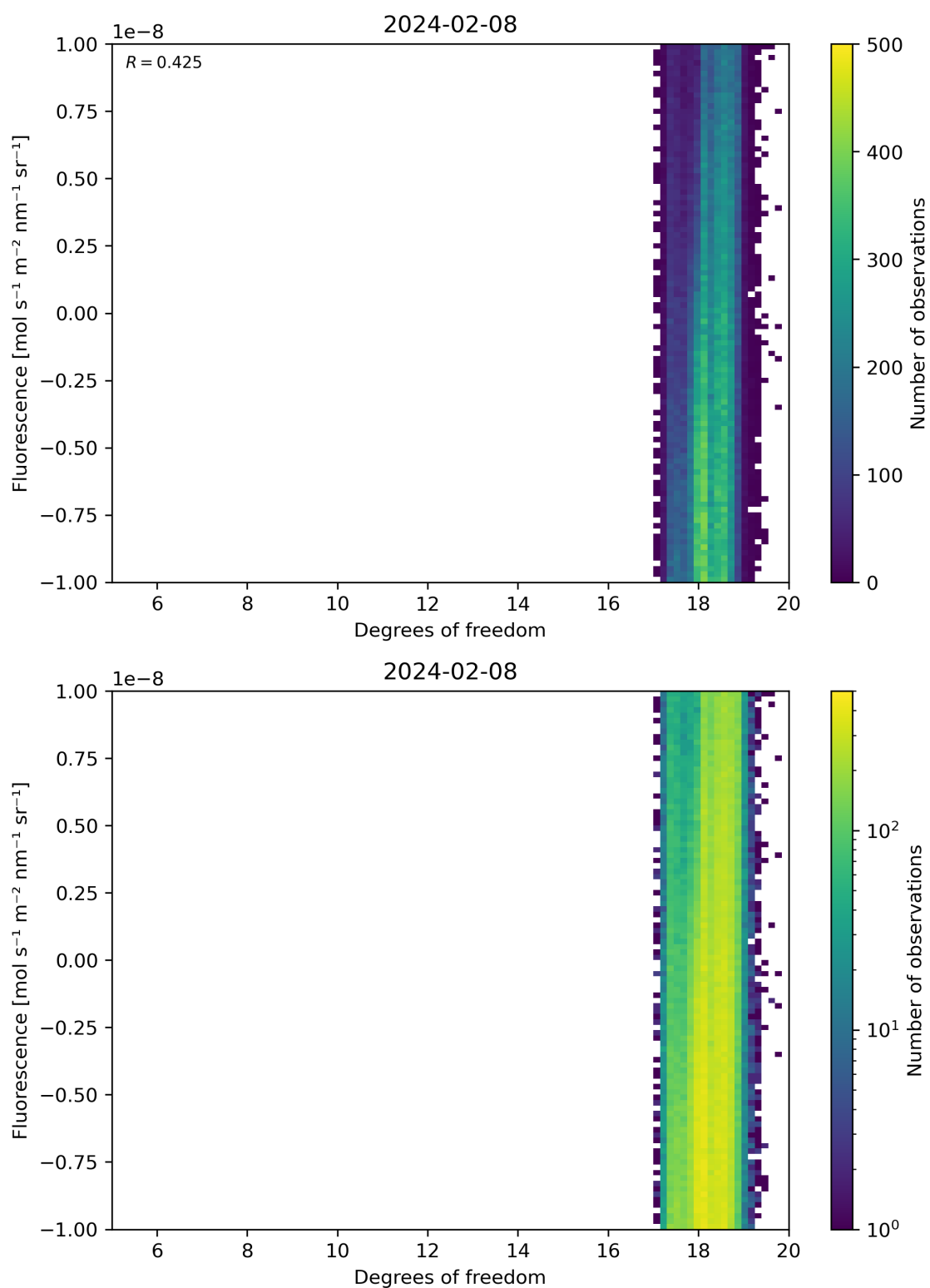
Figure 51: Scatter density plot of “Degrees of freedom” against “Fluorescence” for 2024-02-07 to 2024-02-09.
