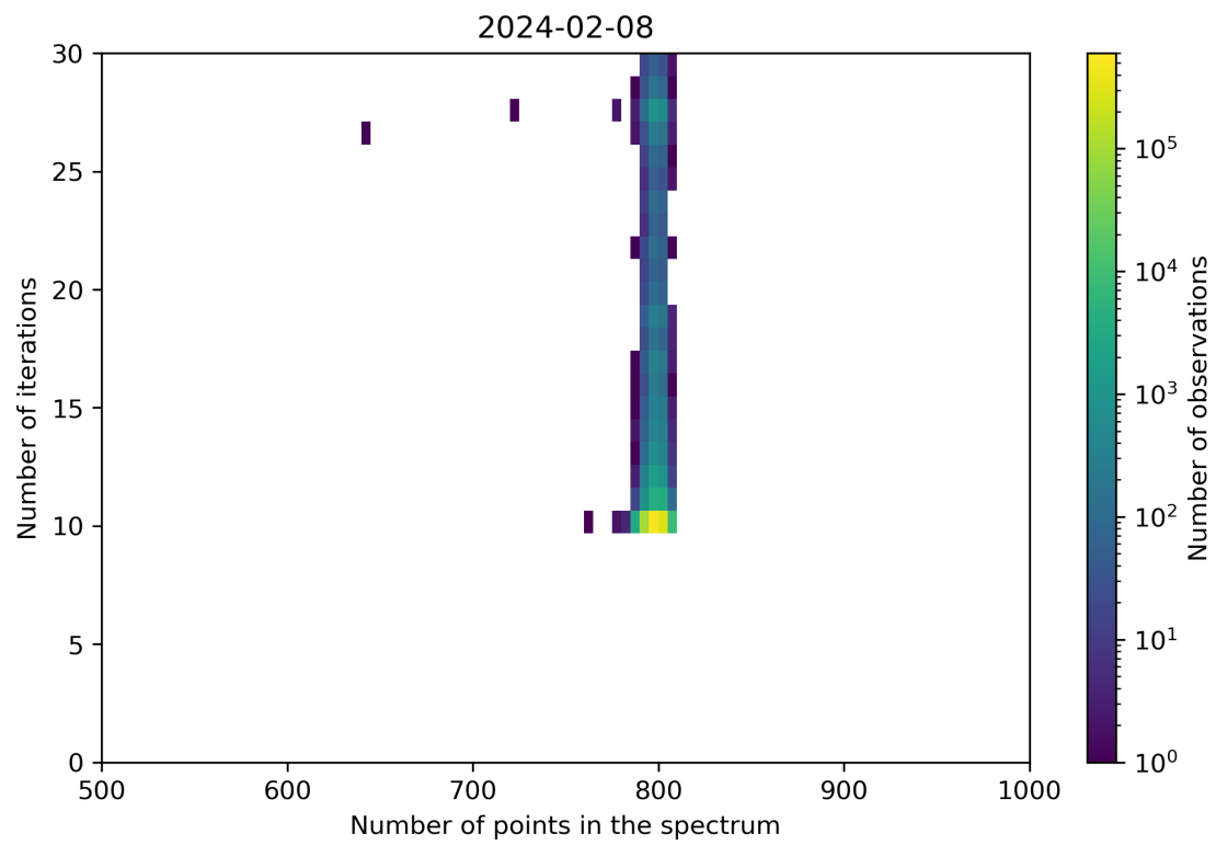
Figure 92: Scatter density plot of “Number of points in the spectrum” against “Number of iterations” for 2024-02-07 to 2024-02-09.
