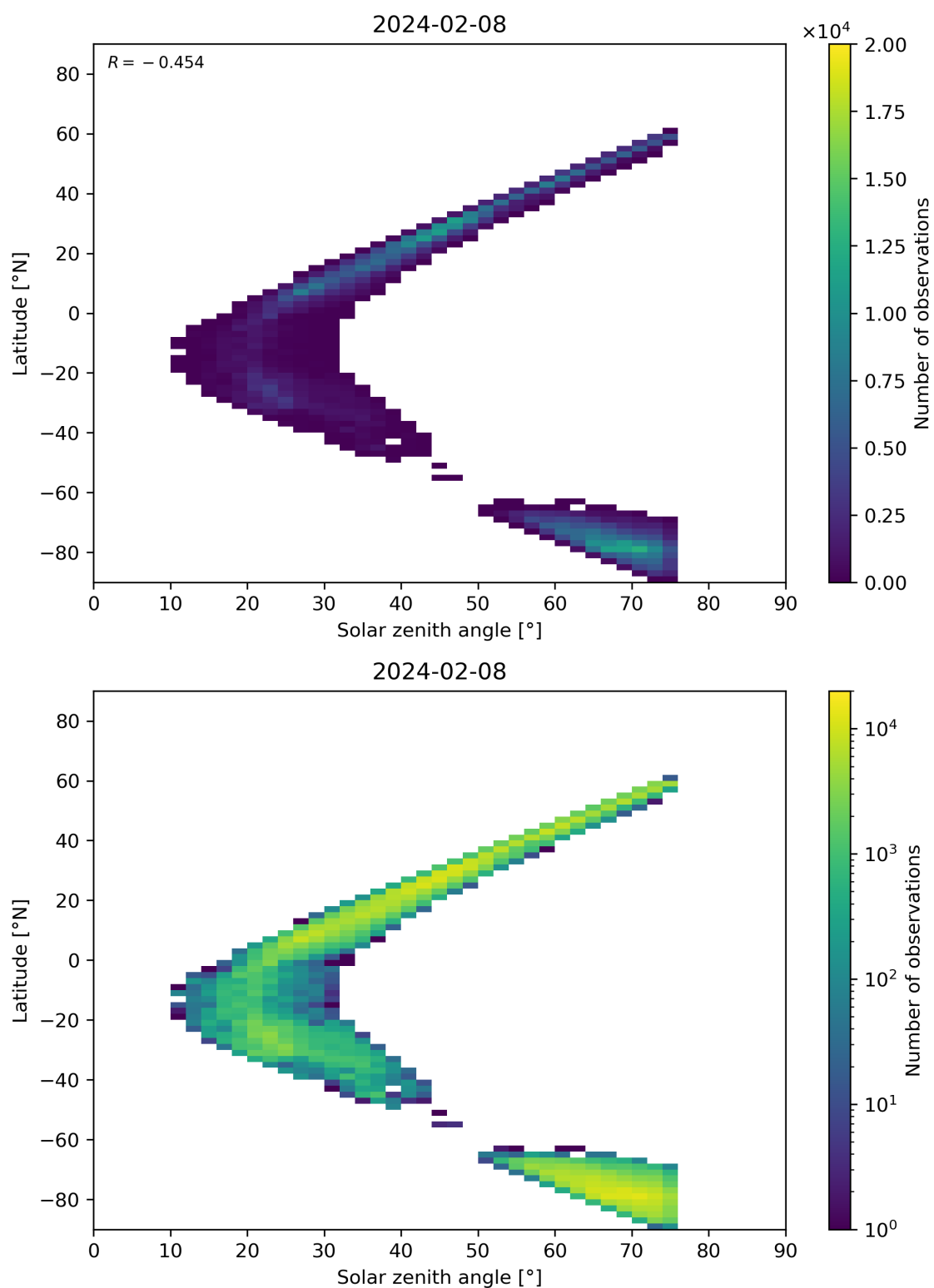
Figure 98: Scatter density plot of “Solar zenith angle” against “Latitude” for 2024-02-07 to 2024-02-09.
