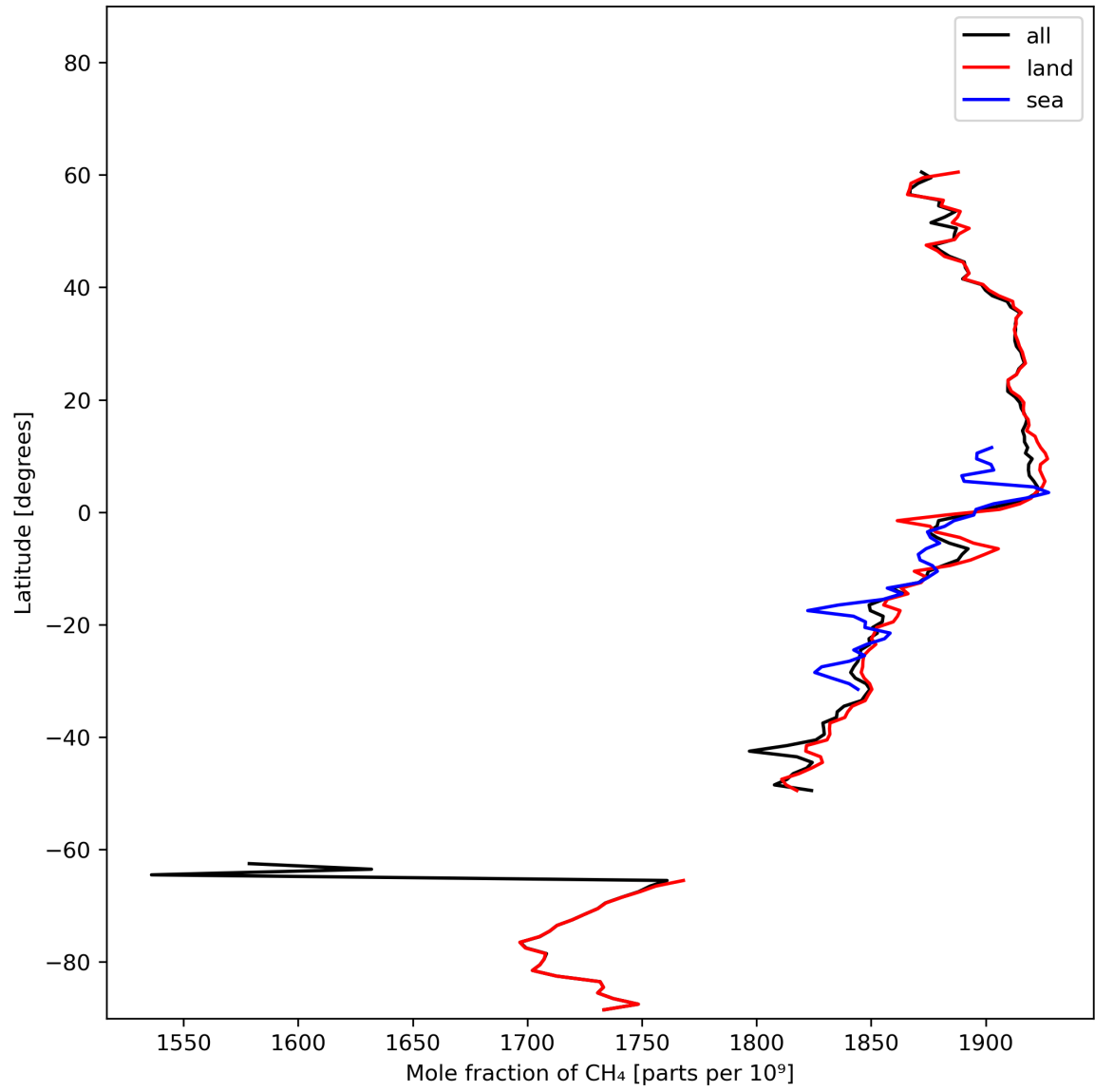
Figure 12: Zonal average of “Mole fraction of CH 4 ” for 2024-02-07 to 2024-02-09.
