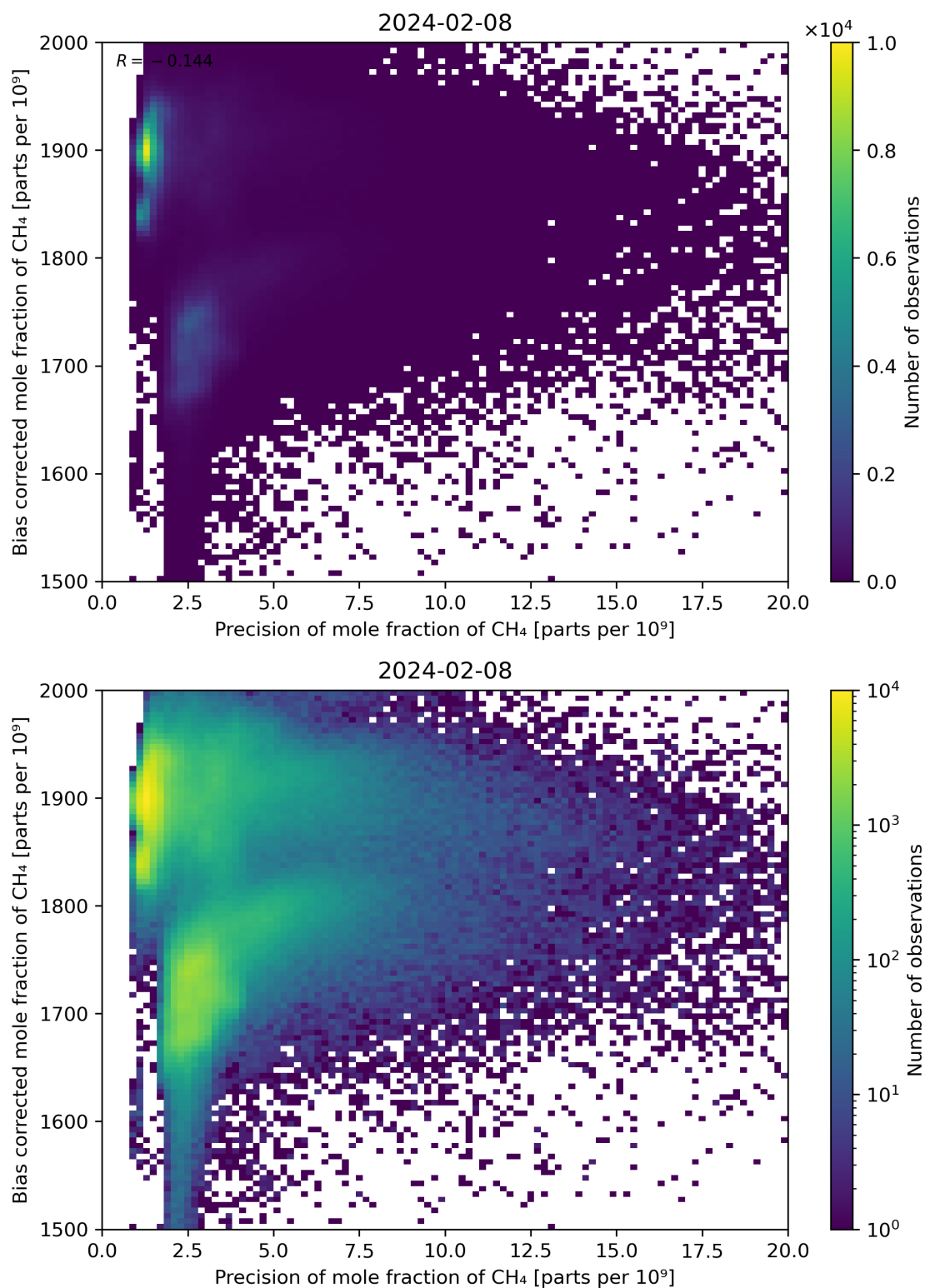
Figure 82: Scatter density plot of “Precision of mole fraction of CH 4 ” against “Bias corrected mole fraction of CH 4 ” for 2024-02-07 to 2024-02-09.
