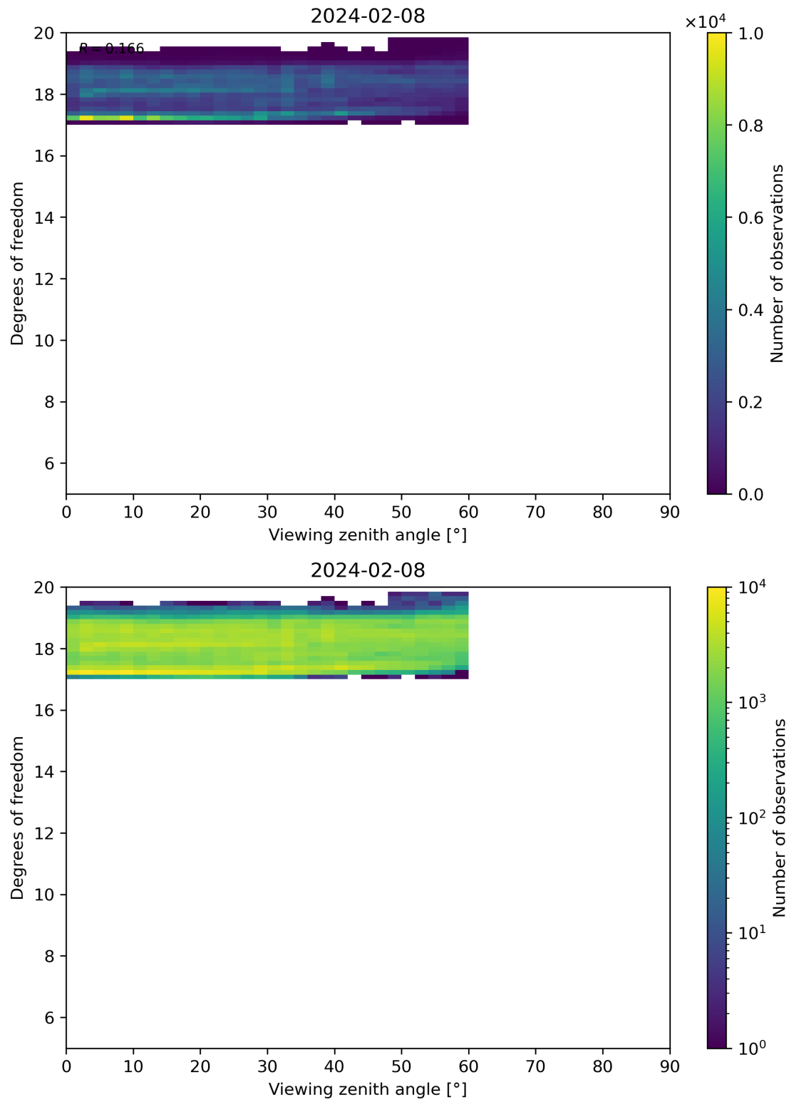
Figure 107: Scatter density plot of “Viewing zenith angle” against “Degrees of freedom” for 2024-02-07 to 2024-02-09.
