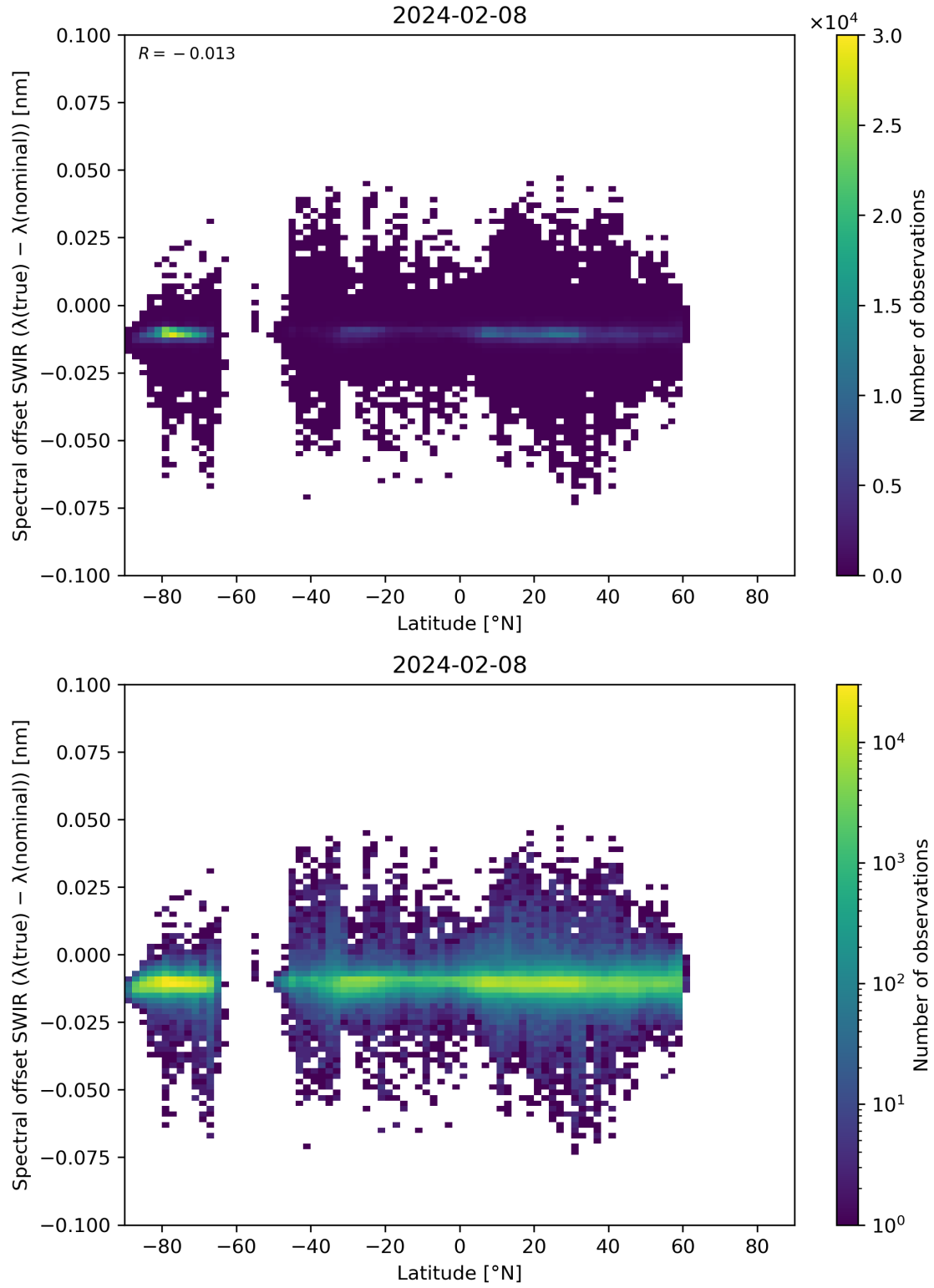
Figure 62: Scatter density plot of “Latitude” against “Spectral offset SWIR ( \lambda(\text{true}) - \lambda(\text{nominal}) )” for 2024-02-07 to 2024-02-09.
