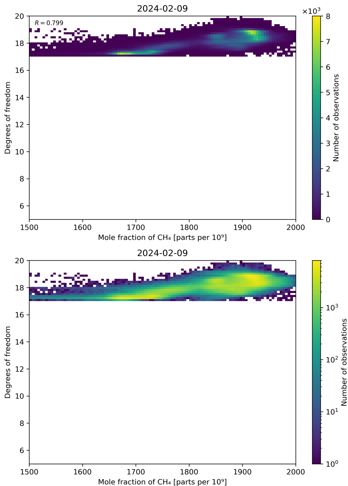
Figure 72: Scatter density plot of “Mole fraction of CH 4 ” against “Degrees of freedom” for 2024-02-08 to 2024-02-10.
