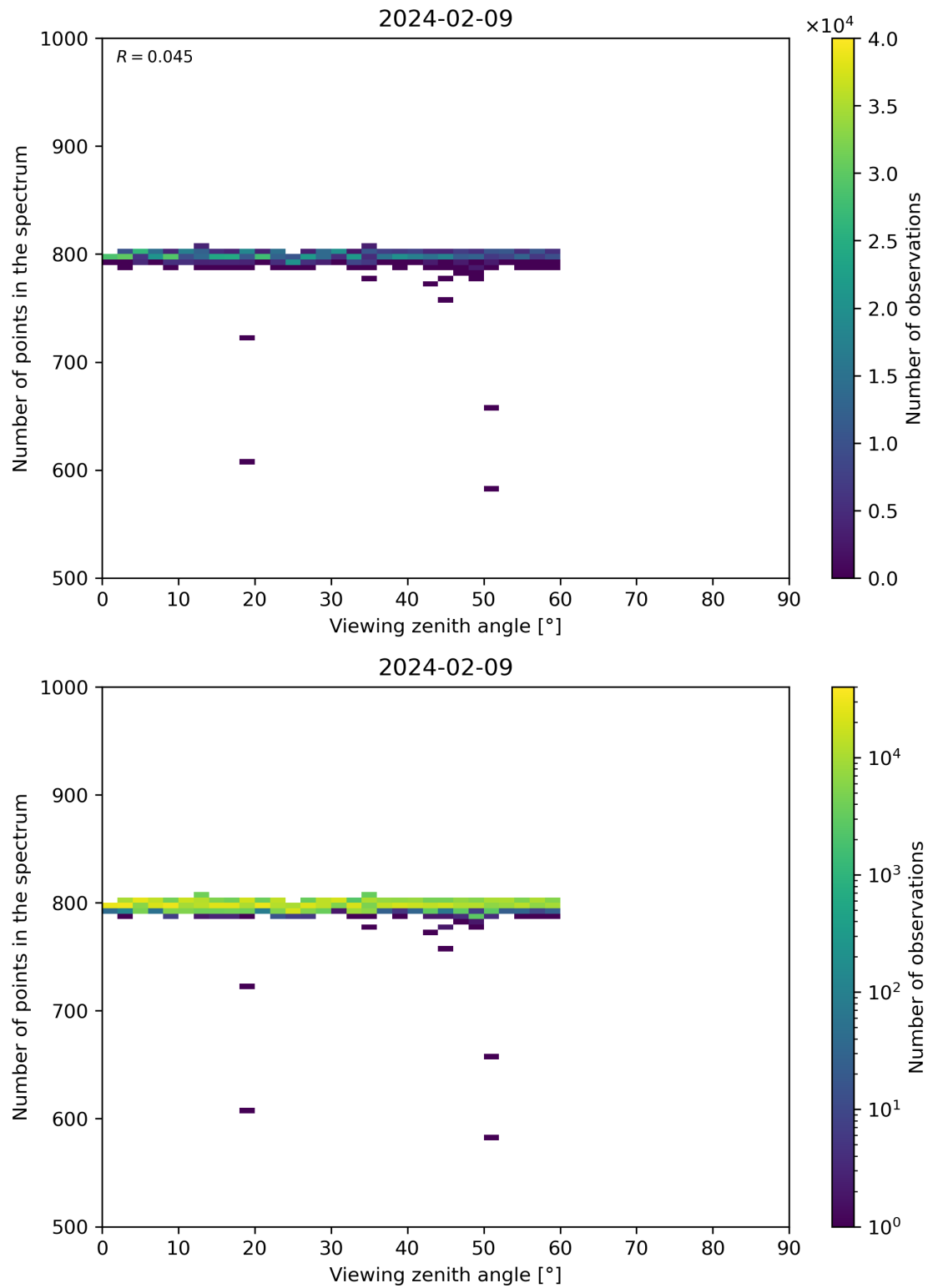
Figure 114: Scatter density plot of “Viewing zenith angle” against “Number of points in the spectrum” for 2024-02-08 to 2024-02-10.
