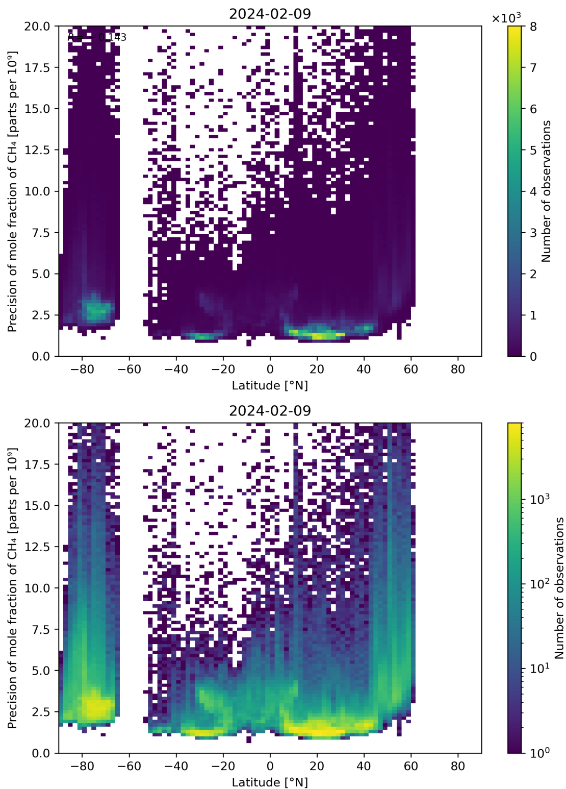
Figure 59: Scatter density plot of “Latitude” against “Precision of mole fraction of CH 4 ” for 2024-02-08 to 2024-02-10.
