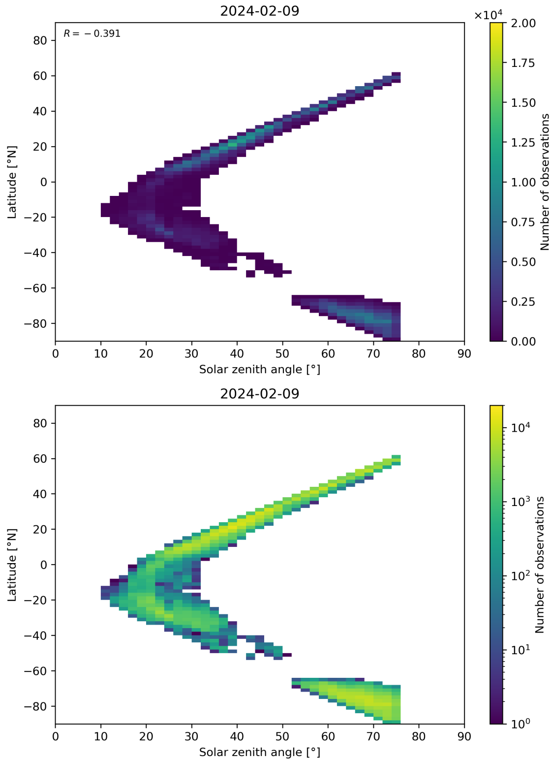
Figure 98: Scatter density plot of “Solar zenith angle” against “Latitude” for 2024-02-08 to 2024-02-10.
