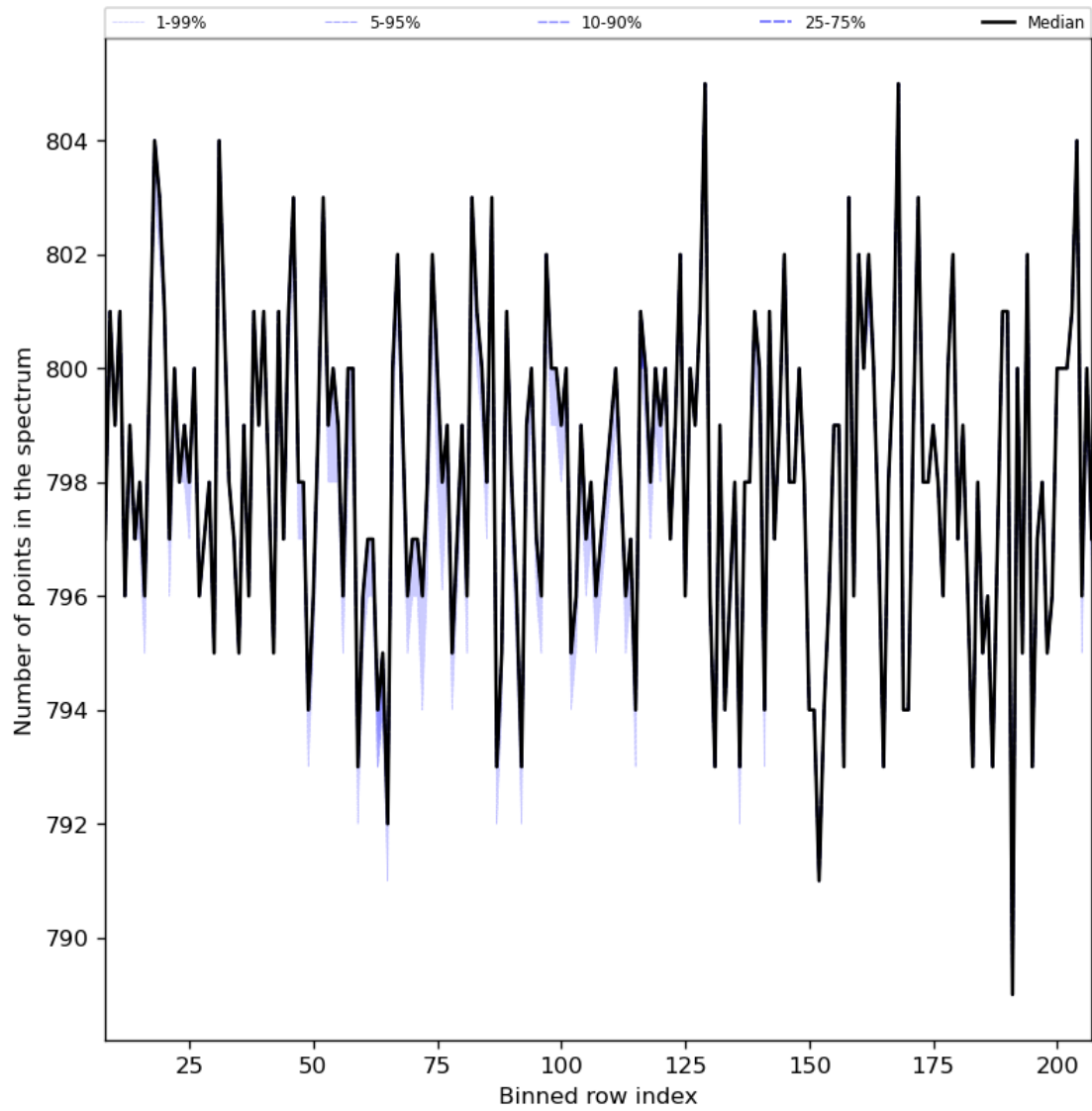
Figure 37: Along track statistics of “Number of points in the spectrum” for 2024-02-08 to 2024-02-10
