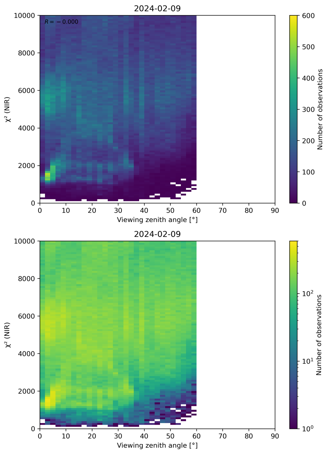
Figure 105: Scatter density plot of “Viewing zenith angle” against “ \chi^2 (NIR)” for 2024-02-08 to 2024-02-10.
