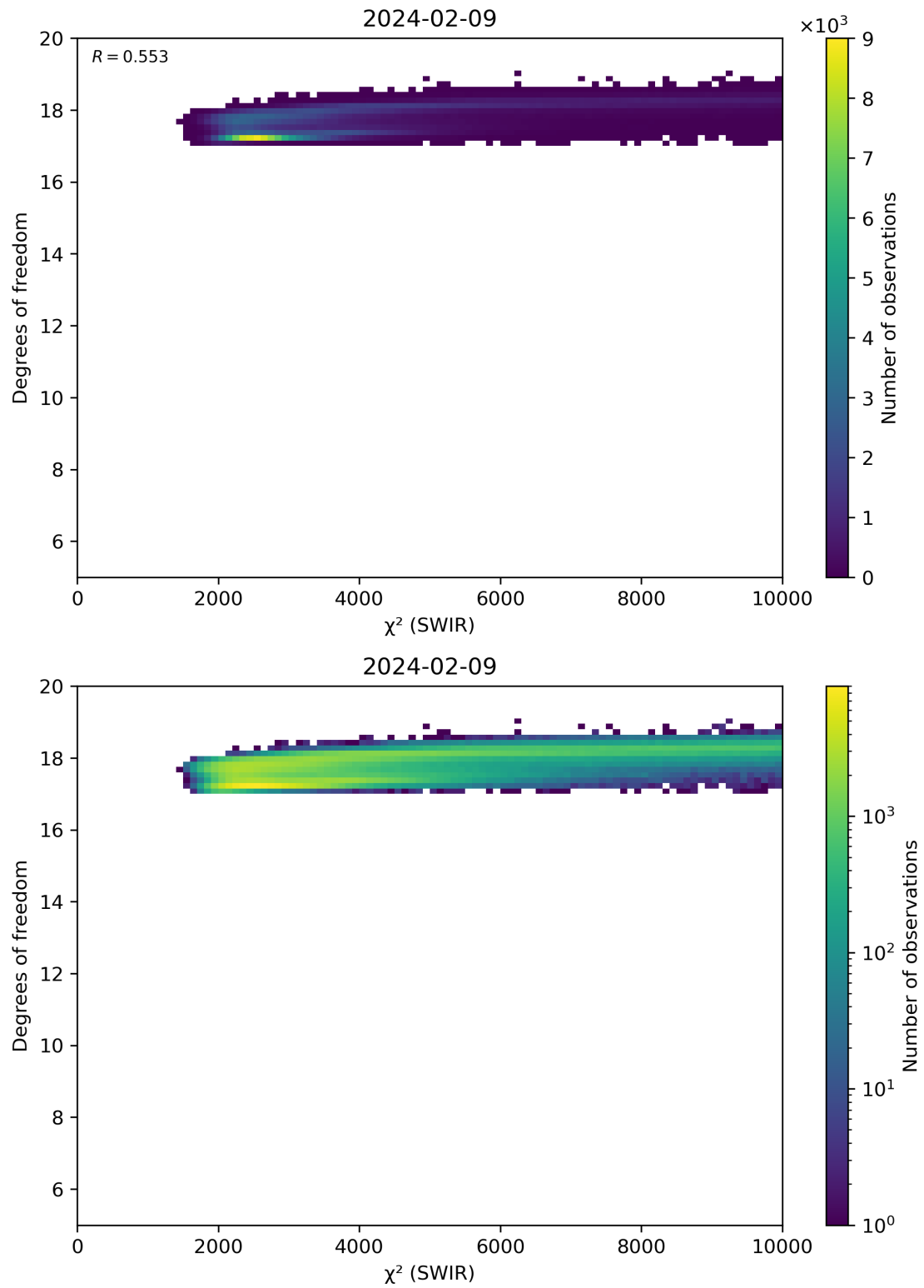
Figure 48: Scatter density plot of “ \chi^2 (SWIR)” against “Degrees of freedom” for 2024-02-08 to 2024-02-10.
