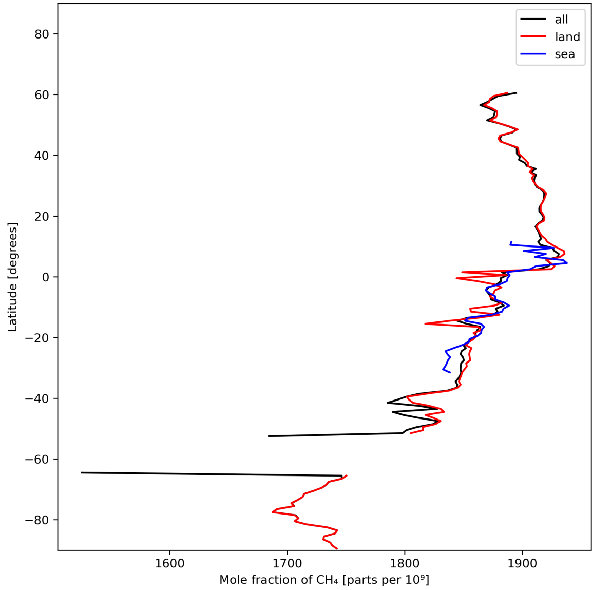
Figure 12: Zonal average of “Mole fraction of \text{CH}_4 ” for 2024-02-08 to 2024-02-10.
