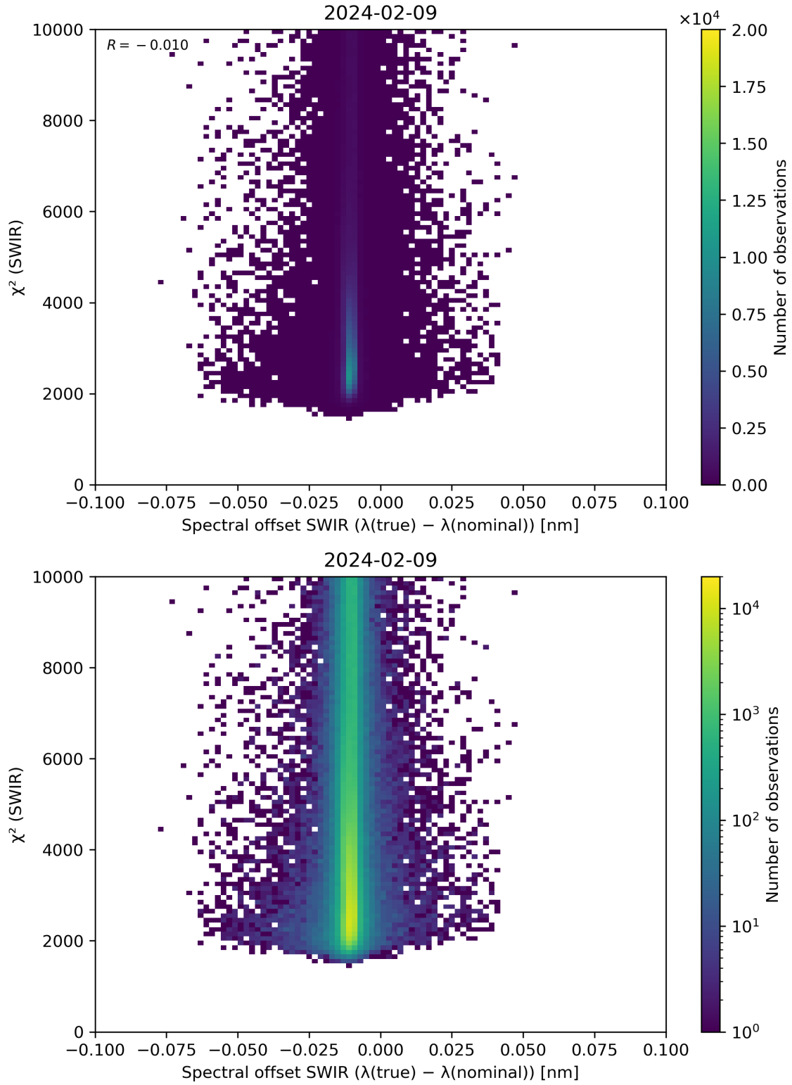
Figure 118: Scatter density plot of “Spectral offset SWIR ( \lambda(\text{true}) - \lambda(\text{nominal}) )” against “ \chi^2 (SWIR)” for 2024-02-08 to 2024-02-10.
