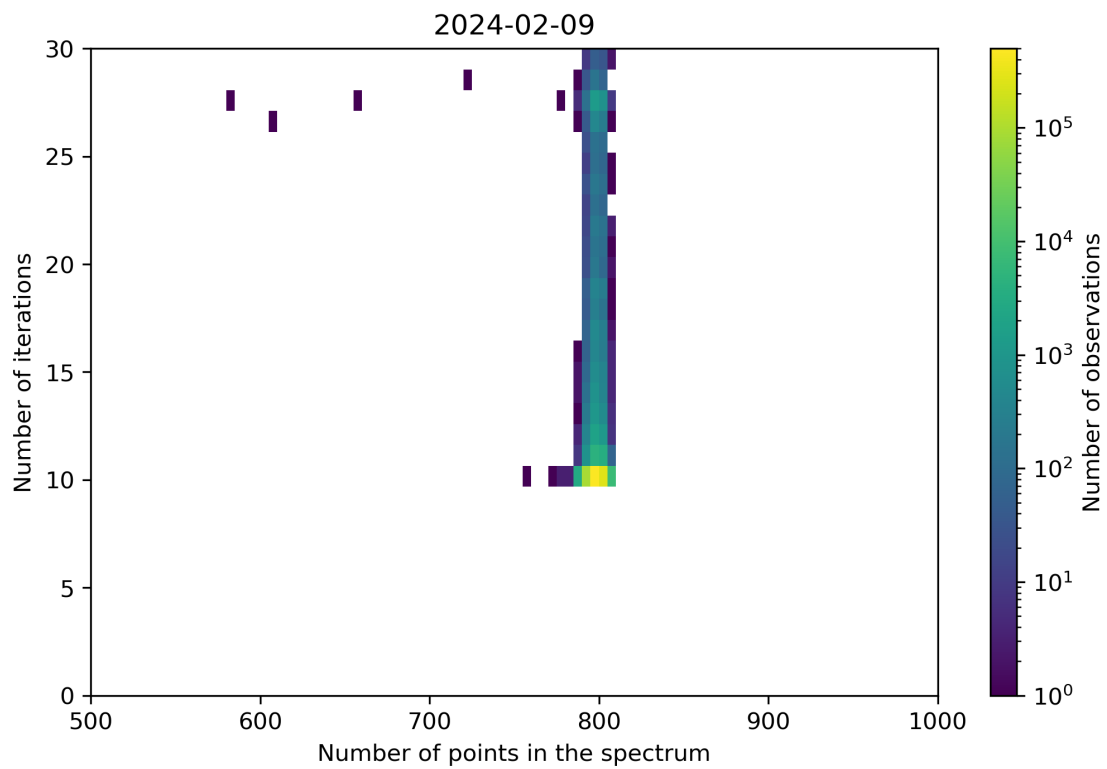
Figure 92: Scatter density plot of “Number of points in the spectrum” against “Number of iterations” for 2024-02-08 to 2024-02-10.
