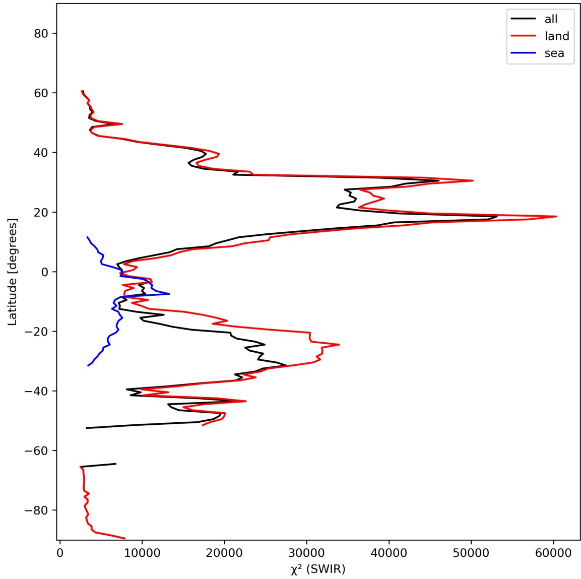
Figure 17: Zonal average of “ \chi^2 (SWIR)” for 2024-02-08 to 2024-02-10.
