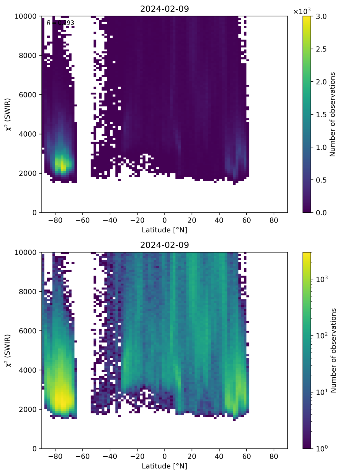
Figure 54: Scatter density plot of “Latitude” against “ \chi^2 (SWIR)” for 2024-02-08 to 2024-02-10.
