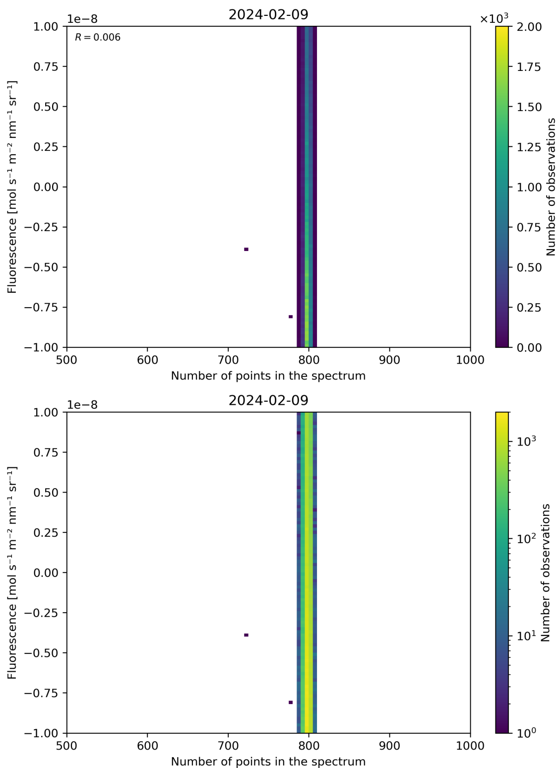
Figure 91: Scatter density plot of “Number of points in the spectrum” against “Fluorescence” for 2024-02-08 to 2024-02-10.
