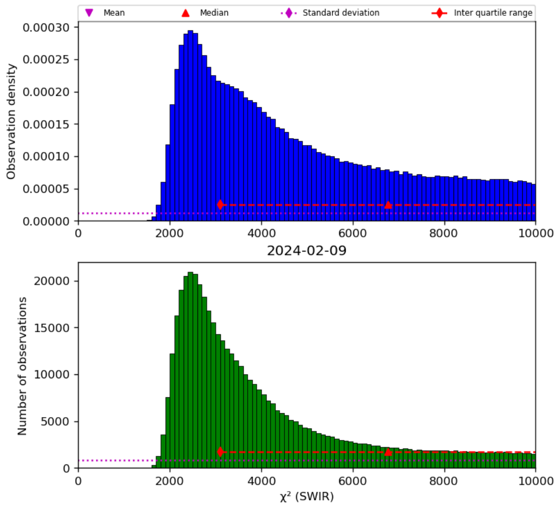
Figure 28: Histogram of “ \chi^2 (SWIR)” for 2024-02-08 to 2024-02-10
