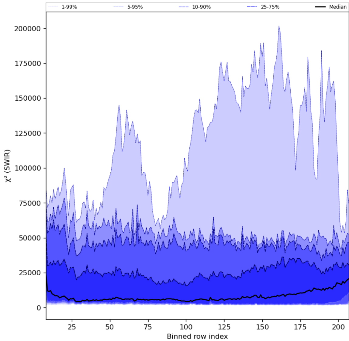
Figure 39: Along track statistics of “ \chi^2 (SWIR)” for 2024-02-08 to 2024-02-10
