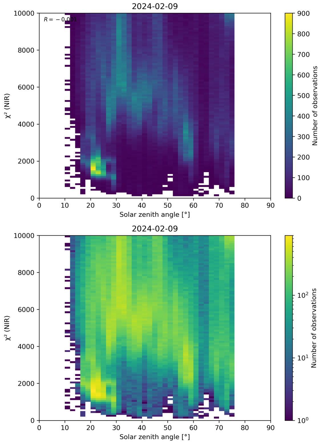
Figure 94: Scatter density plot of “Solar zenith angle” against “ \chi^2 (NIR)” for 2024-02-08 to 2024-02-10.
