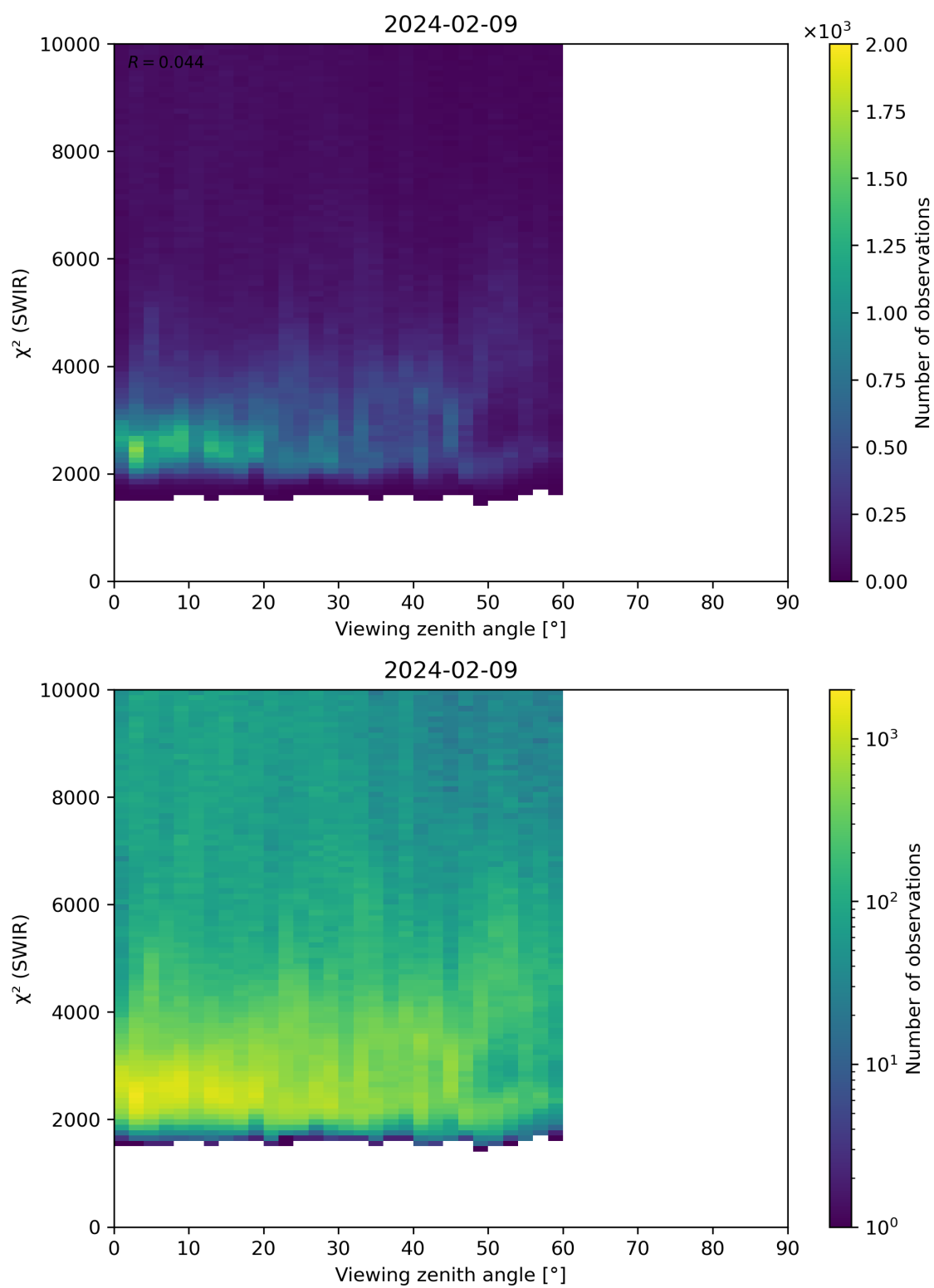
Figure 106: Scatter density plot of “Viewing zenith angle” against “ \chi^2 (SWIR)” for 2024-02-08 to 2024-02-10.
