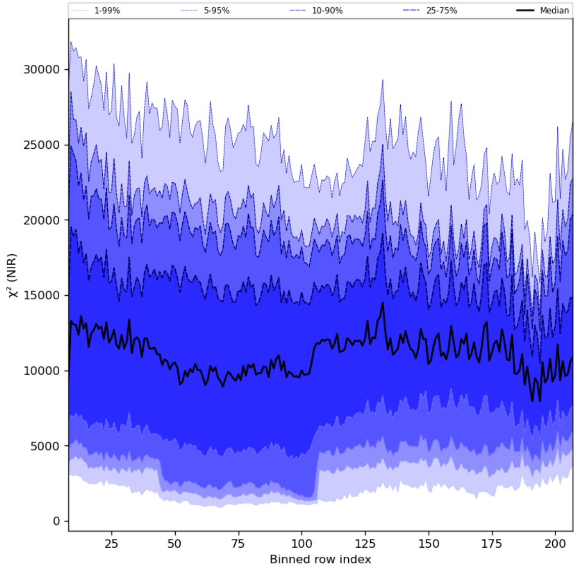
Figure 40: Along track statistics of “ \chi^2 (NIR)” for 2024-02-08 to 2024-02-10
