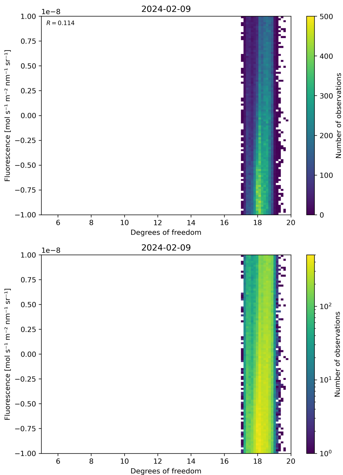
Figure 51: Scatter density plot of “Degrees of freedom” against “Fluorescence” for 2024-02-08 to 2024-02-10.
