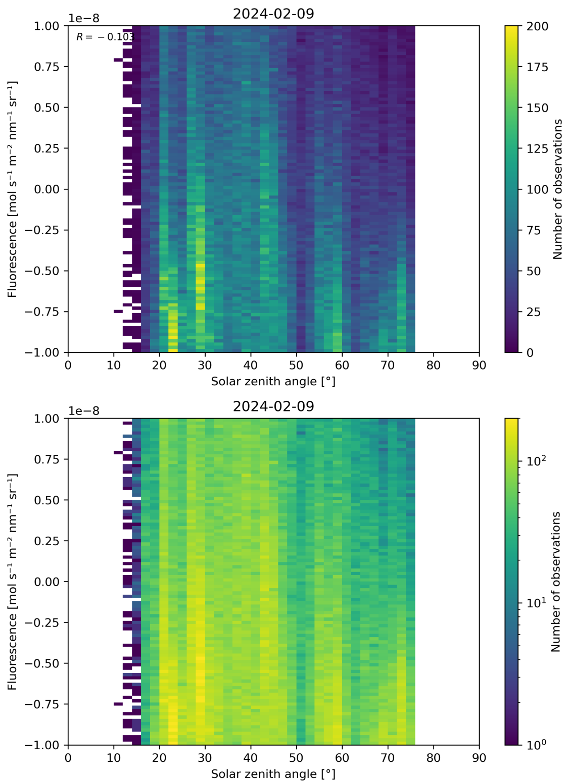
Figure 97: Scatter density plot of “Solar zenith angle” against “Fluorescence” for 2024-02-08 to 2024-02-10.
