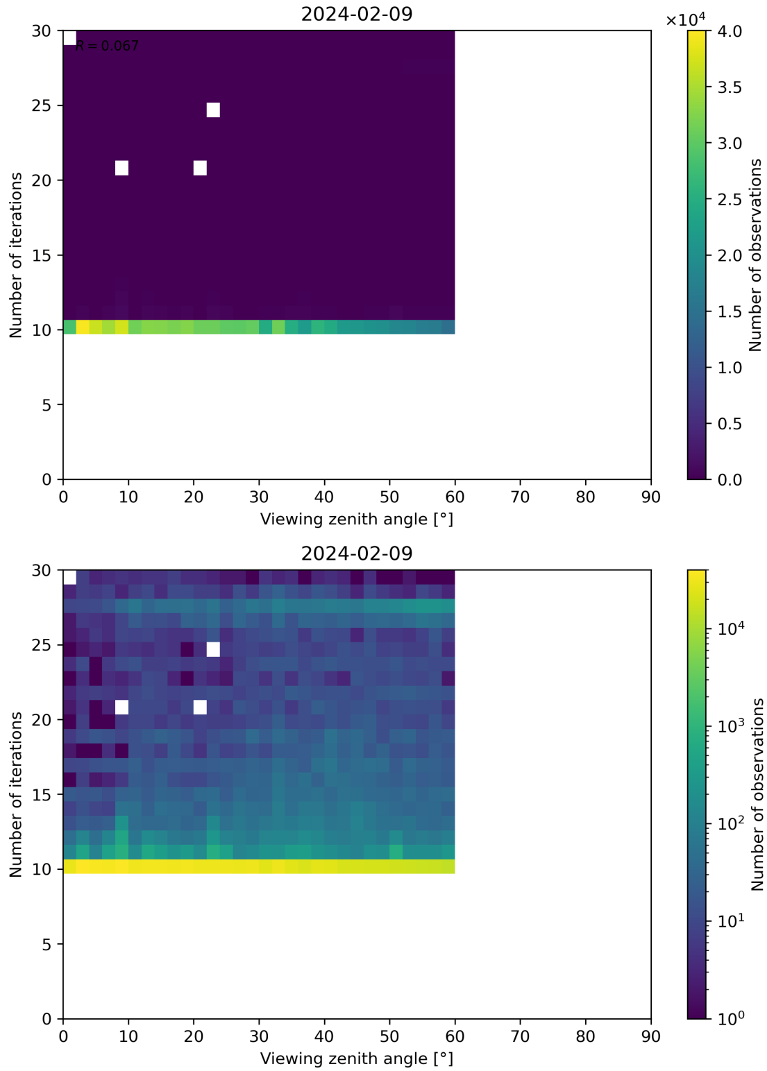
Figure 113: Scatter density plot of “Viewing zenith angle” against “Number of iterations” for 2024-02-08 to 2024-02-10.
