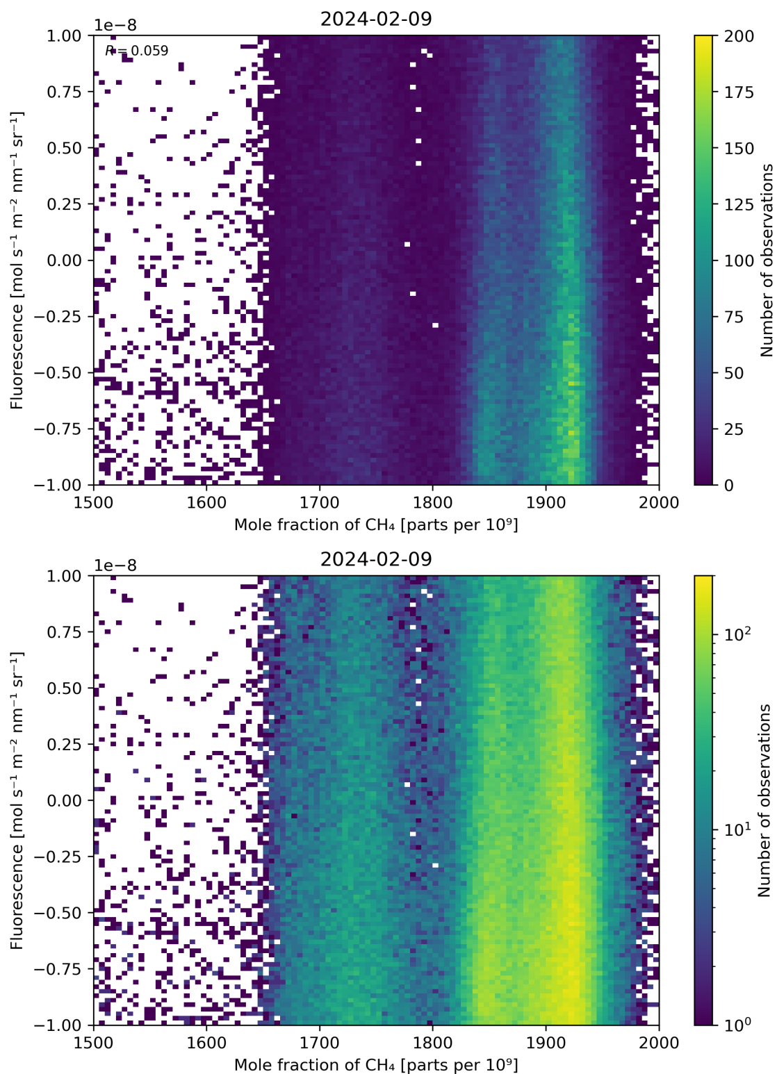
Figure 73: Scatter density plot of “Mole fraction of \text{CH}_4 ” against “Fluorescence” for 2024-02-08 to 2024-02-10.
