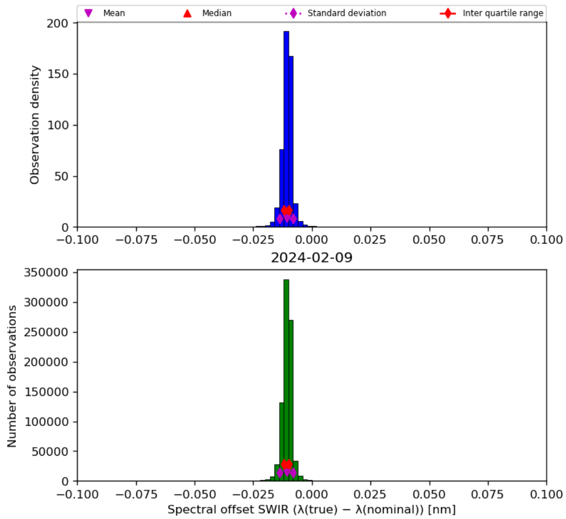
Figure 27: Histogram of “Spectral offset SWIR ( \lambda(\text{true}) - \lambda(\text{nominal}) )” for 2024-02-08 to 2024-02-10
