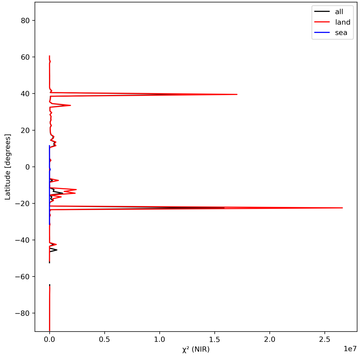
Figure 18: Zonal average of “ \chi^2 (NIR)” for 2024-02-08 to 2024-02-10.
