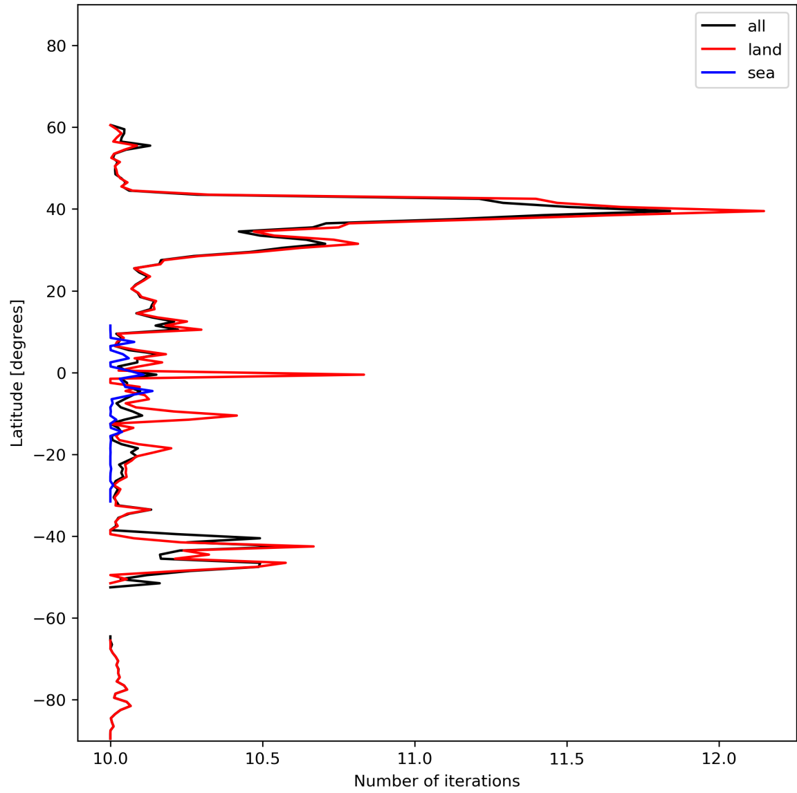
Figure 20: Zonal average of “Number of iterations” for 2024-02-08 to 2024-02-10.
