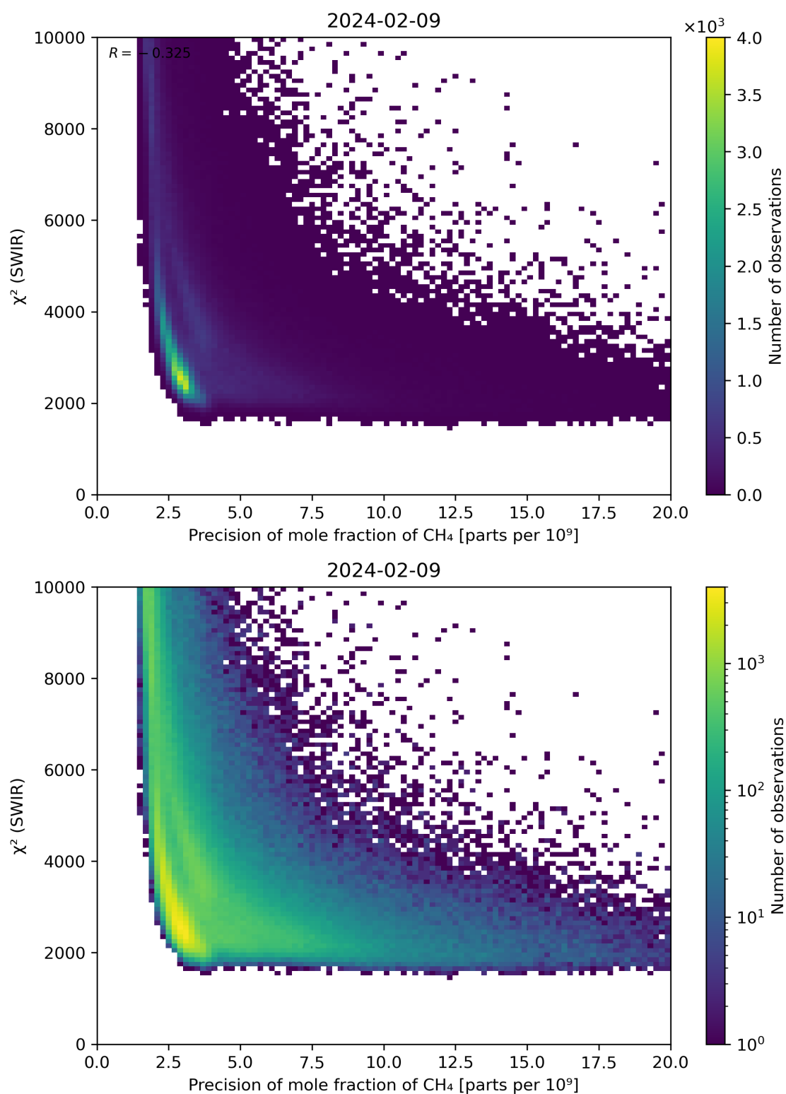
Figure 79: Scatter density plot of “Precision of mole fraction of CH 4 ” against “ \chi^2 (SWIR)” for 2024-02-08 to 2024-02-10.
