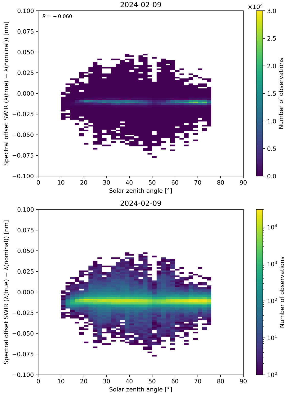
Figure 104: Scatter density plot of “Solar zenith angle” against “Spectral offset SWIR ( \lambda(\text{true}) - \lambda(\text{nominal}) )” for 2024-02-08 to 2024-02-10.
