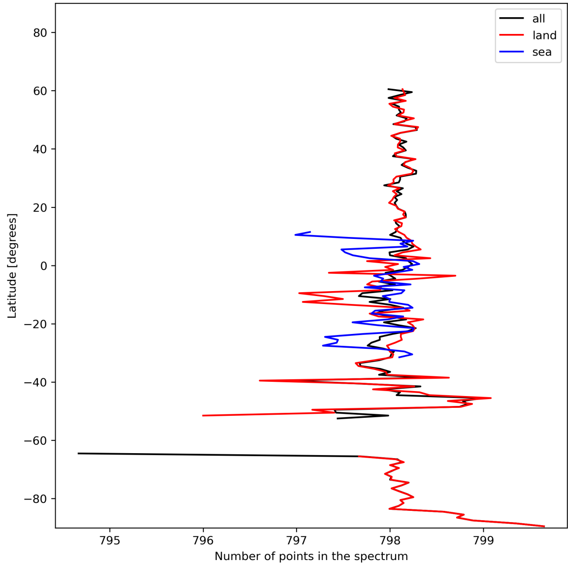
Figure 15: Zonal average of “Number of points in the spectrum” for 2024-02-08 to 2024-02-10.
