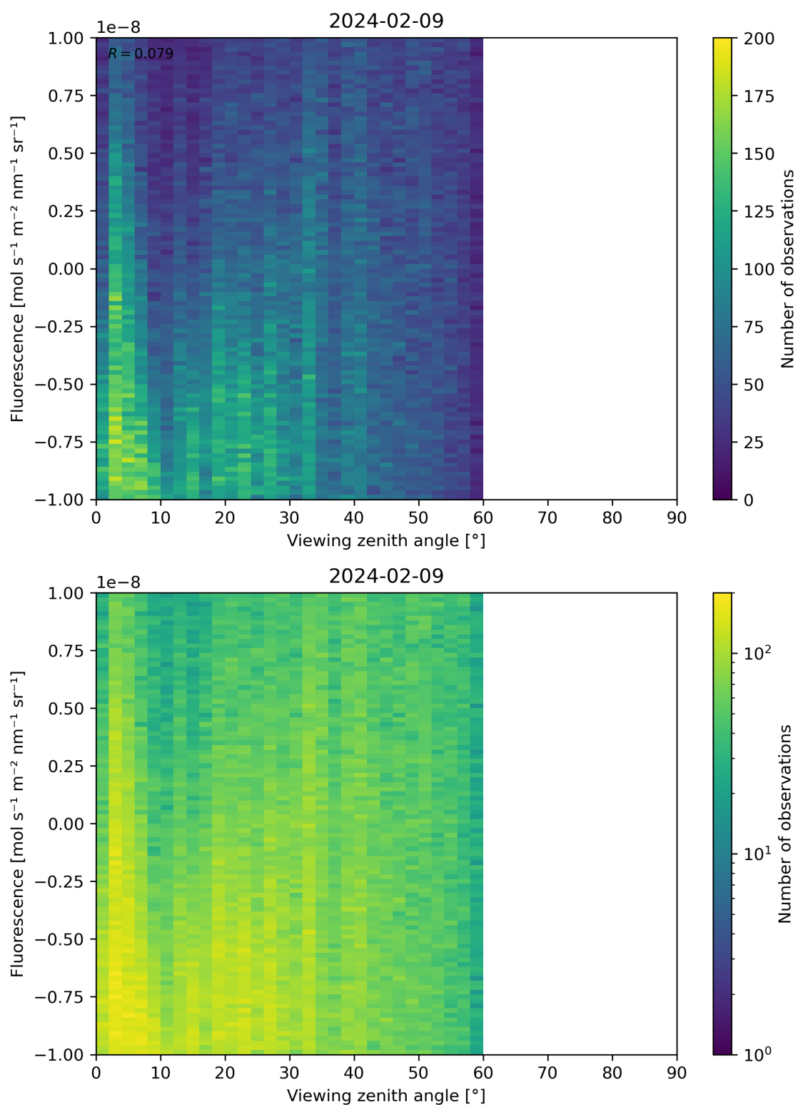
Figure 108: Scatter density plot of “Viewing zenith angle” against “Fluorescence” for 2024-02-08 to 2024-02-10.
