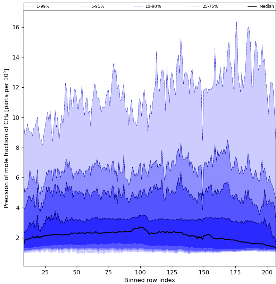
Figure 35: Along track statistics of “Precision of mole fraction of CH 4 ” for 2024-02-08 to 2024-02-10
