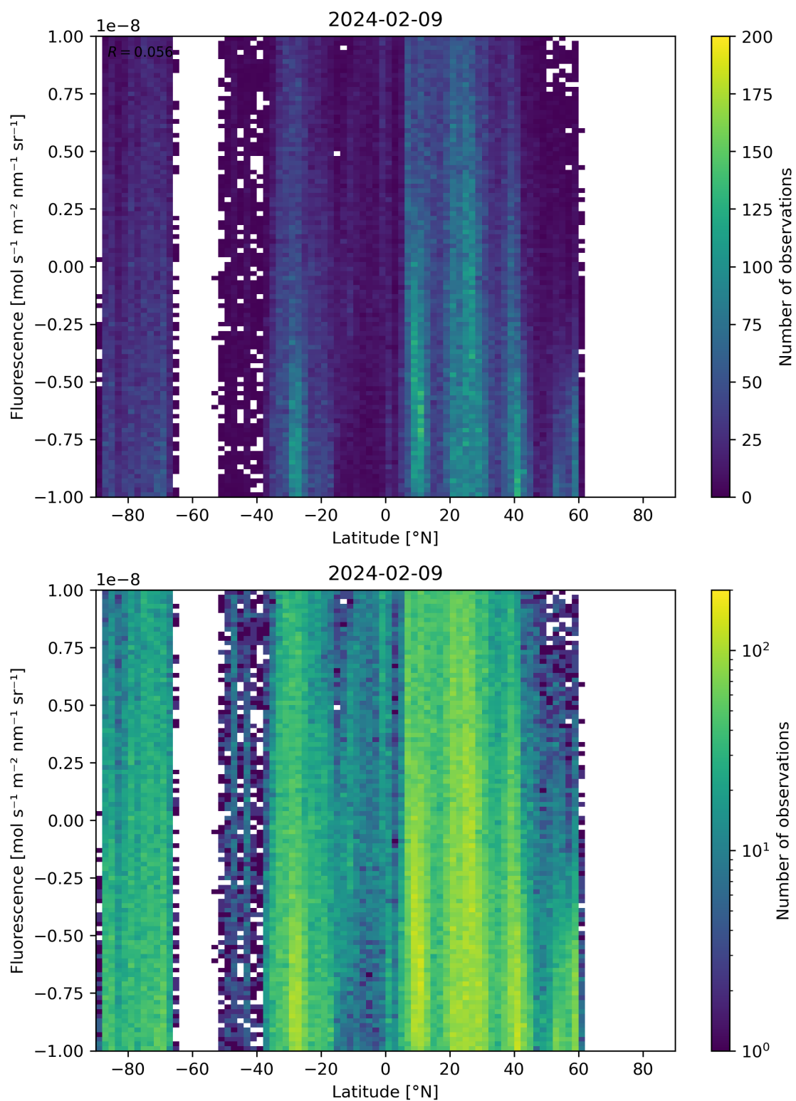
Figure 56: Scatter density plot of “Latitude” against “Fluorescence” for 2024-02-08 to 2024-02-10.
