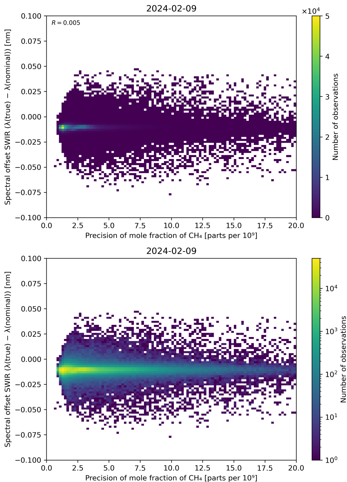
Figure 85: Scatter density plot of “Precision of mole fraction of CH 4 ” against “Spectral offset SWIR ( \lambda(\text{true}) - \lambda(\text{nominal}) )” for 2024-02-08 to 2024-02-10.
