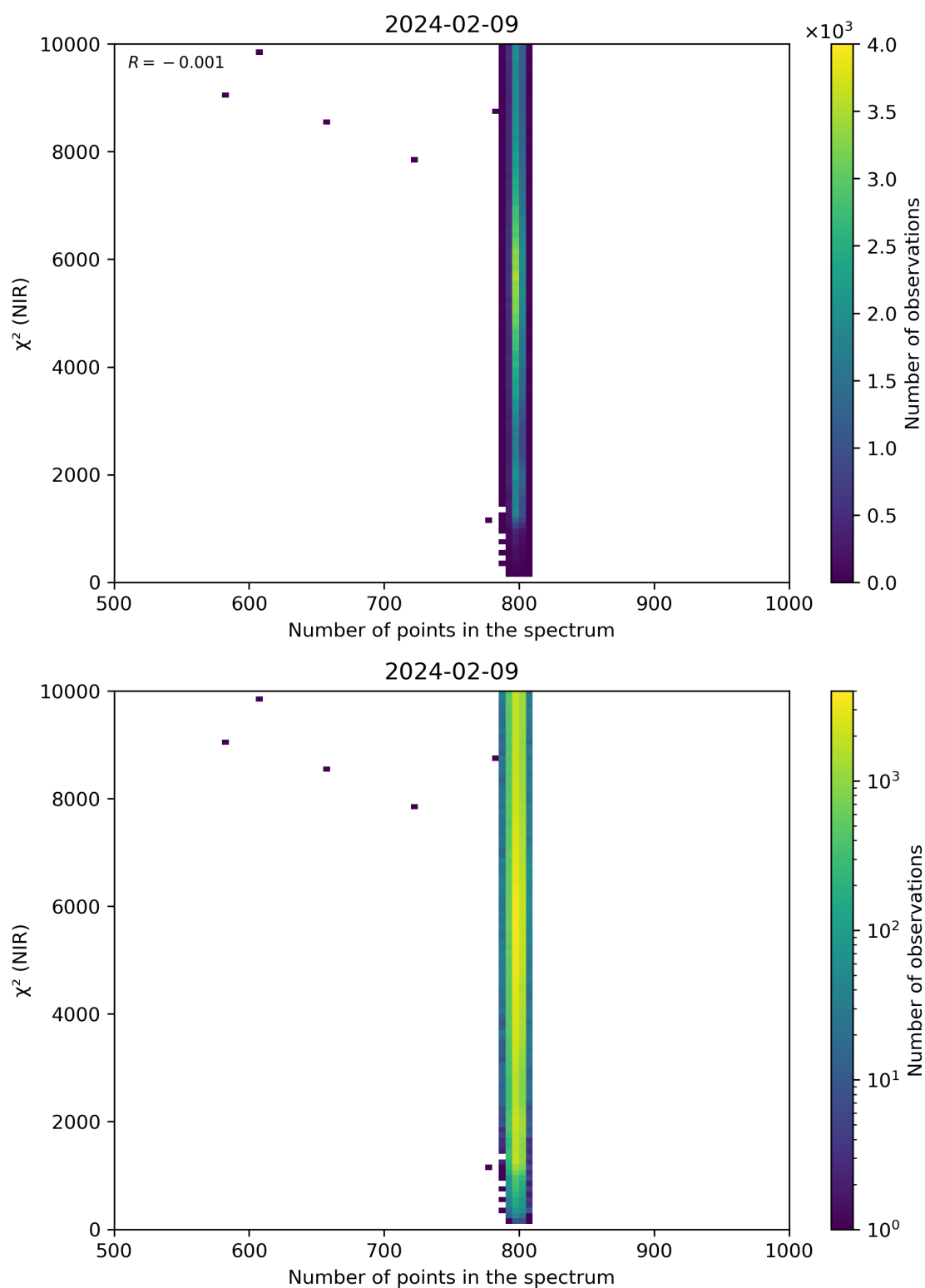
Figure 88: Scatter density plot of “Number of points in the spectrum” against “ \chi^2 (NIR)” for 2024-02-08 to 2024-02-10.
