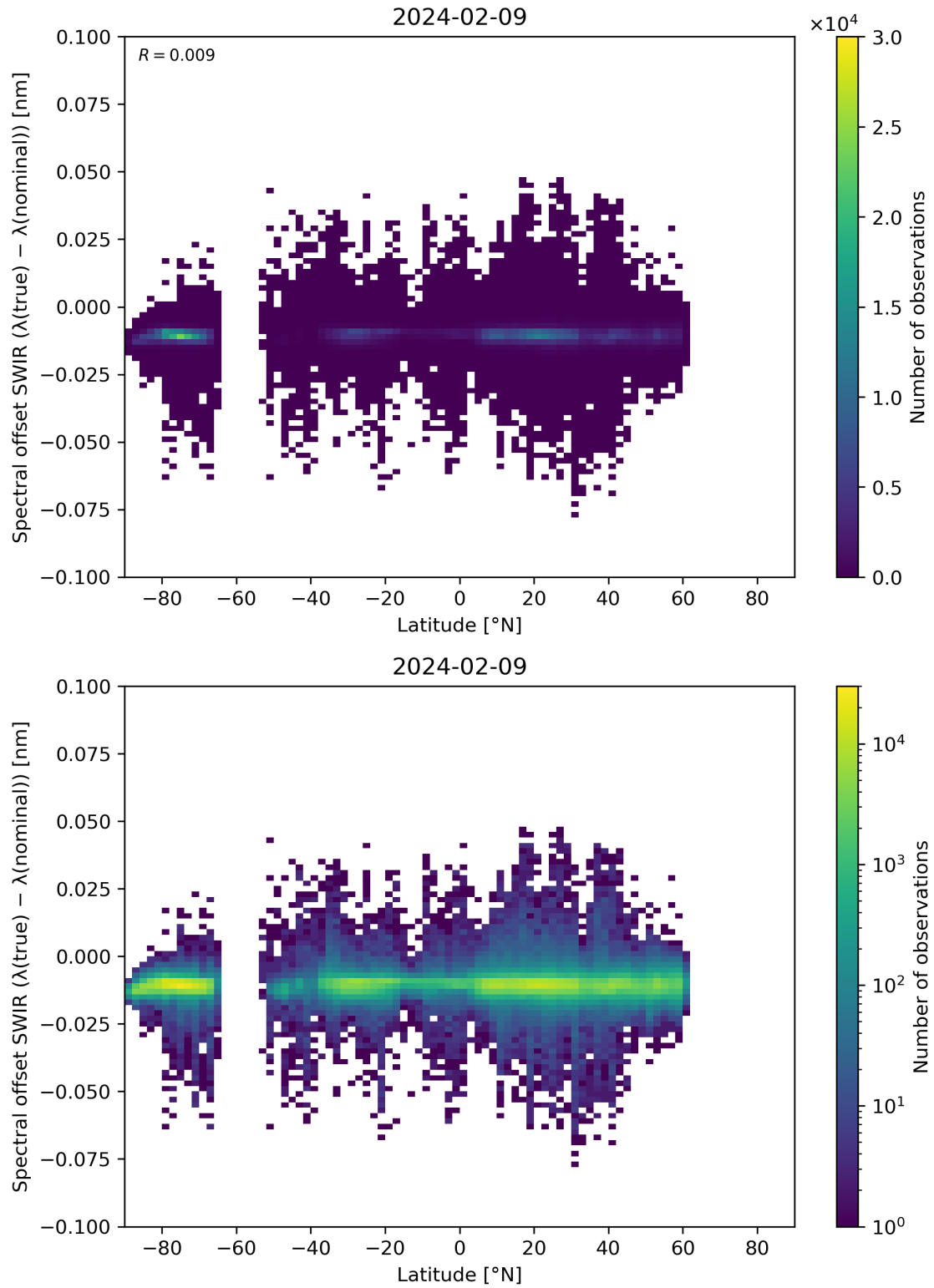
Figure 62: Scatter density plot of “Latitude” against “Spectral offset SWIR ( \lambda(\text{true}) - \lambda(\text{nominal}) )” for 2024-02-08 to 2024-02-10.
