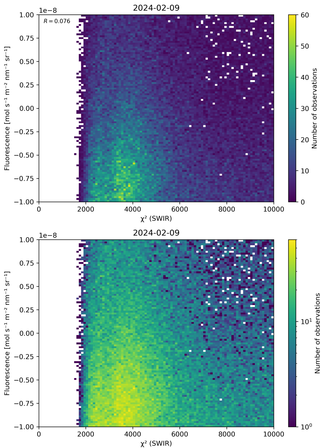
Figure 49: Scatter density plot of “ \chi^2 (SWIR)” against “Fluorescence” for 2024-02-08 to 2024-02-10.
