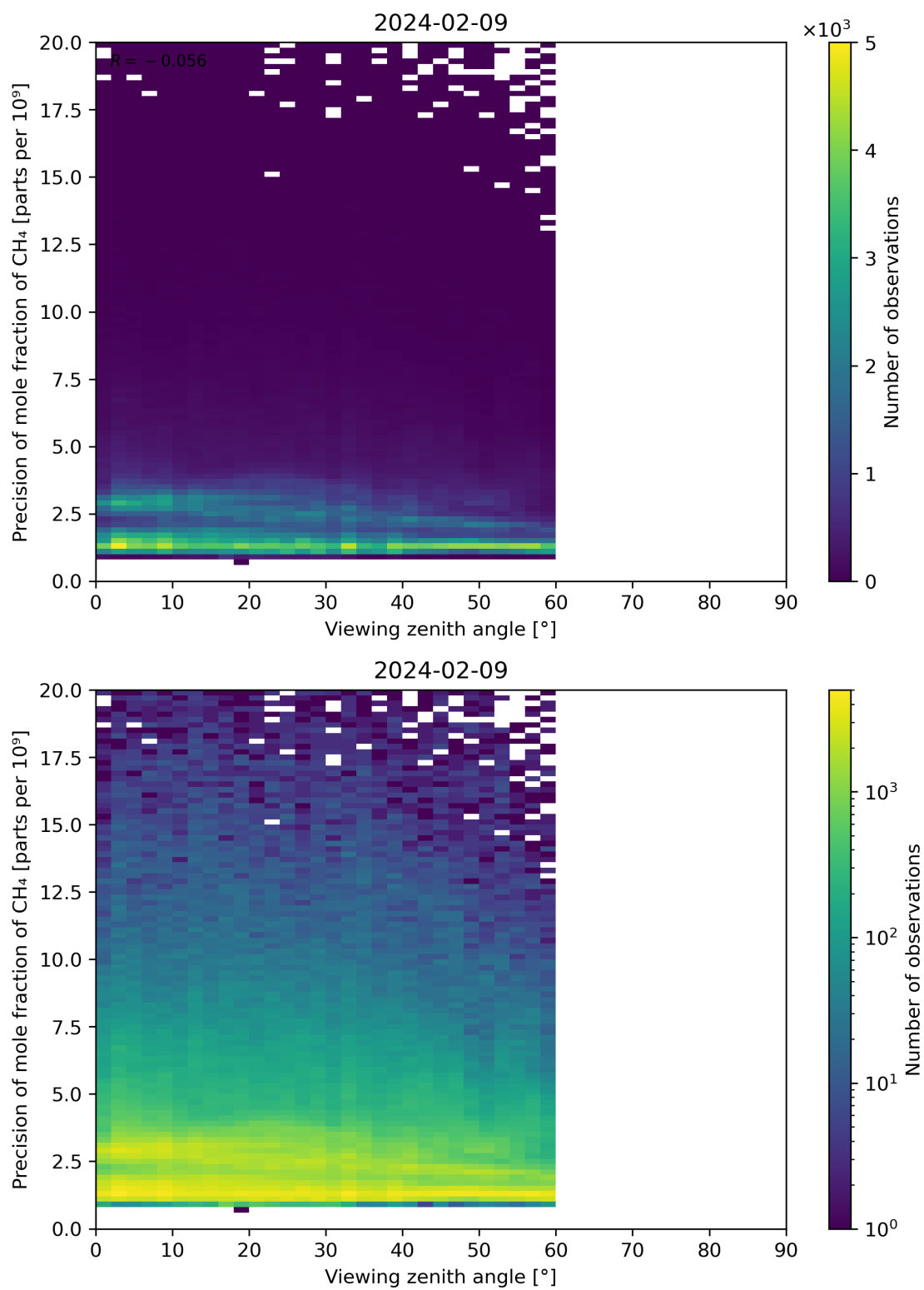
Figure 112: Scatter density plot of “Viewing zenith angle” against “Precision of mole fraction of CH 4 ” for 2024-02-08 to 2024-02-10.
