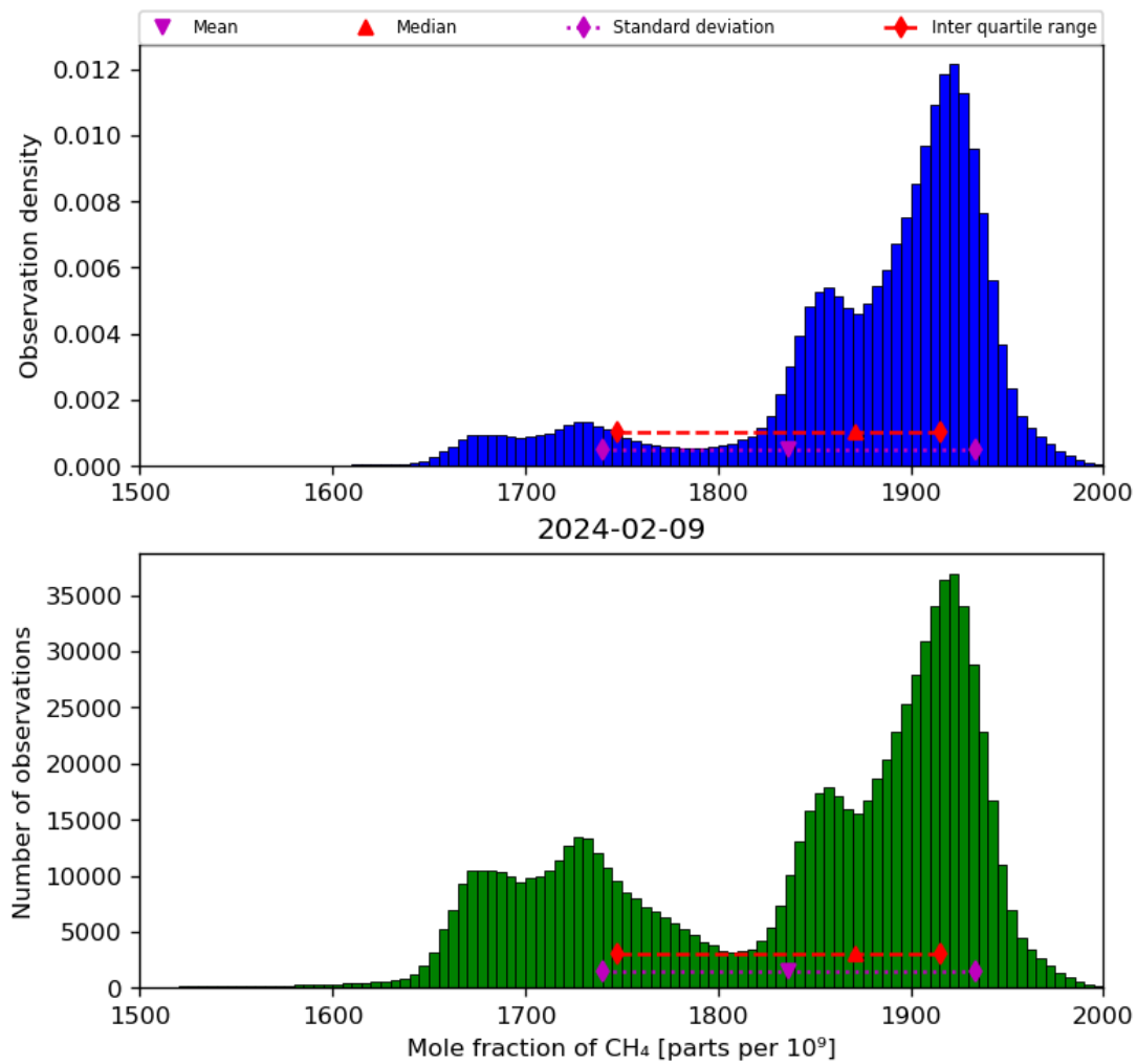
Figure 23: Histogram of “Mole fraction of CH 4 ” for 2024-02-08 to 2024-02-10
