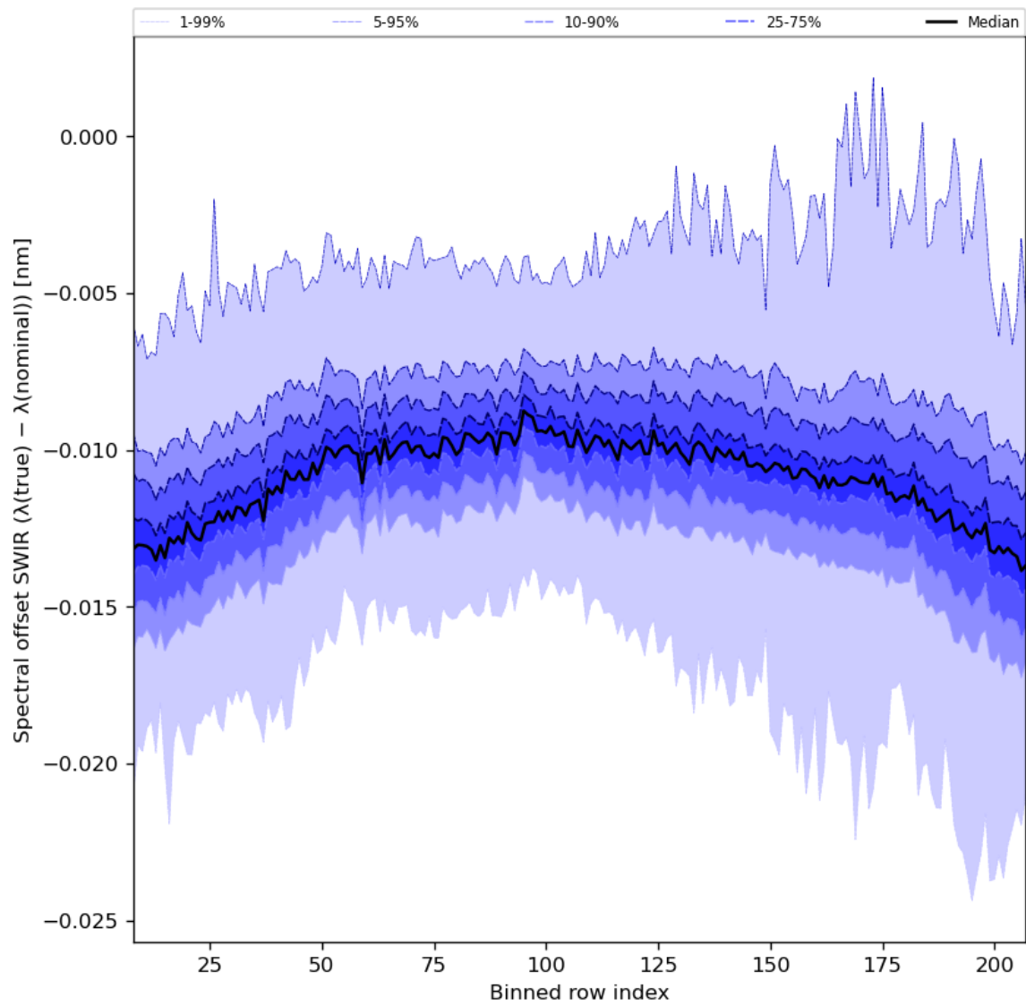
Figure 38: Along track statistics of “Spectral offset SWIR ( \lambda(\text{true}) - \lambda(\text{nominal}) )” for 2024-02-08 to 2024-02-10
