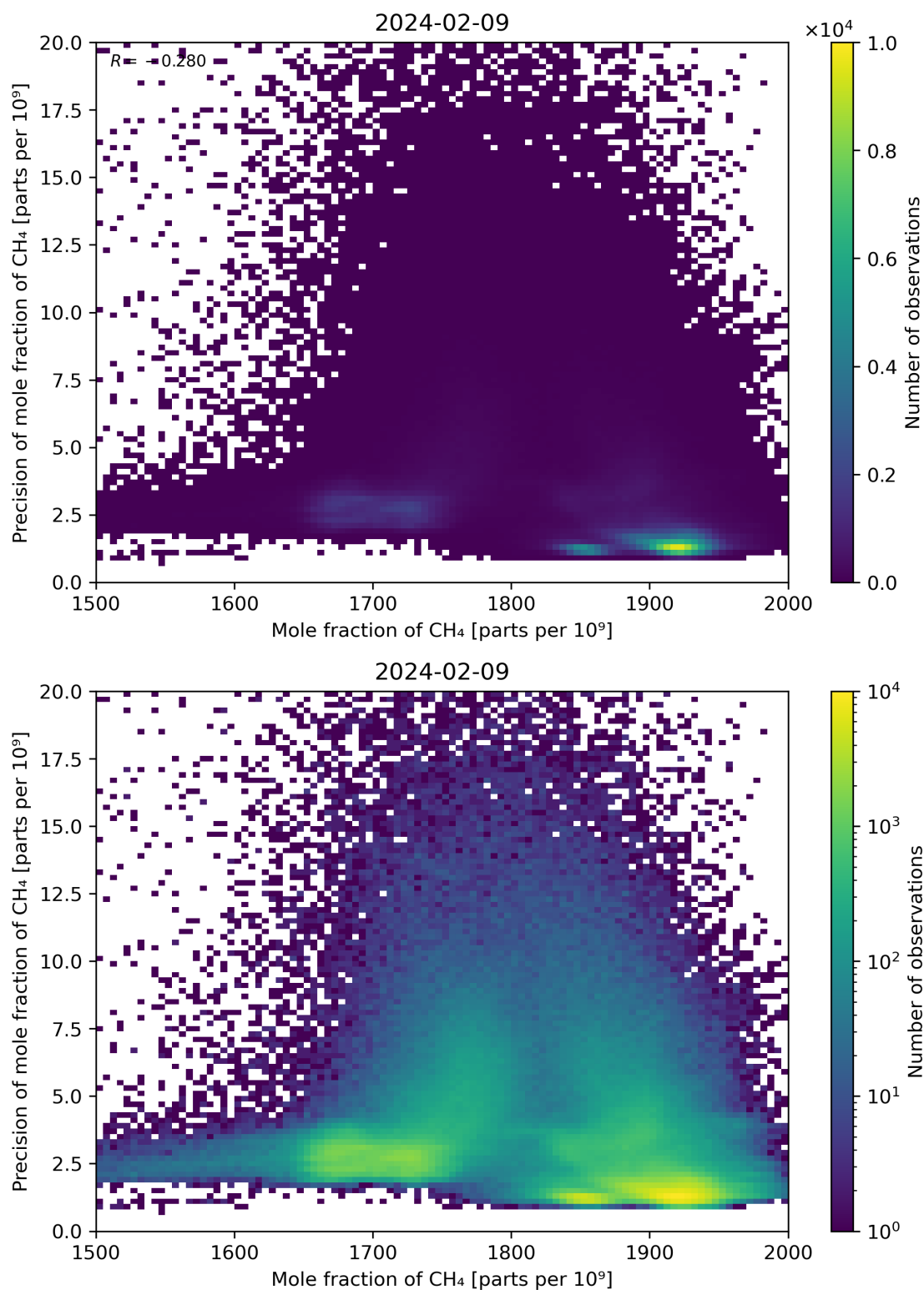
Figure 75: Scatter density plot of “Mole fraction of CH 4 ” against “Precision of mole fraction of CH 4 ” for 2024-02-08 to 2024-02-10.
