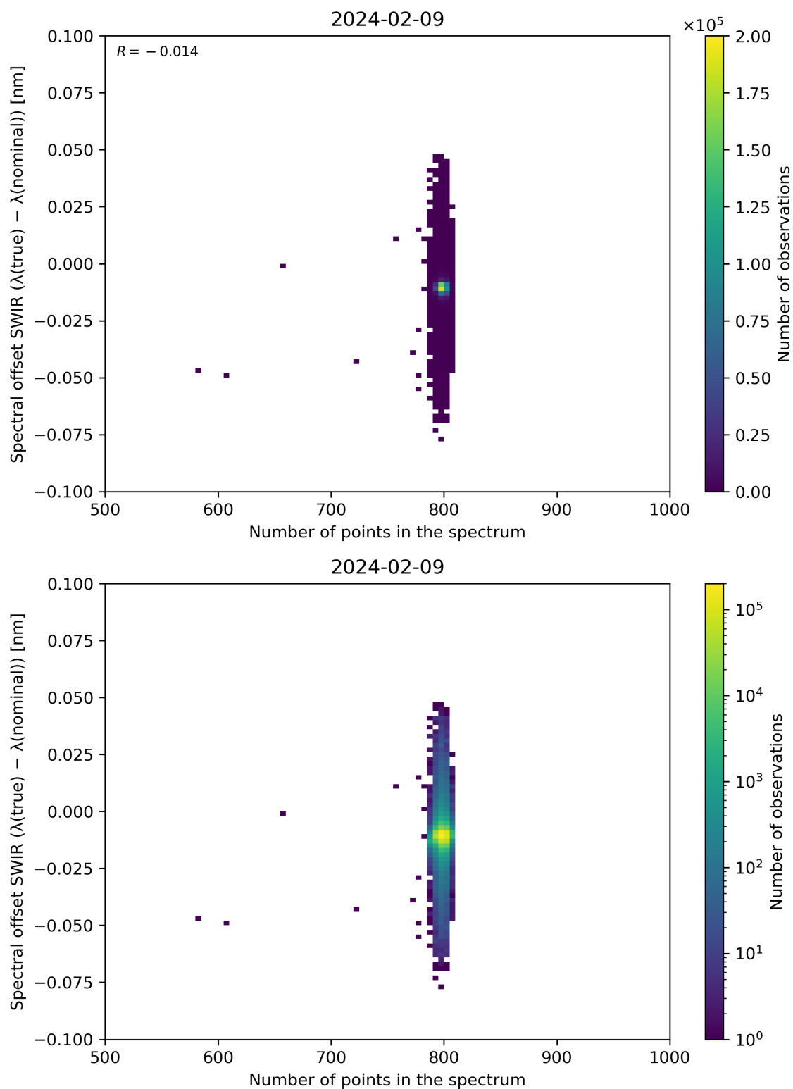
Figure 93: Scatter density plot of “Number of points in the spectrum” against “Spectral offset SWIR ( \lambda(\text{true}) - \lambda(\text{nominal}) )” for 2024-02-08 to 2024-02-10.
