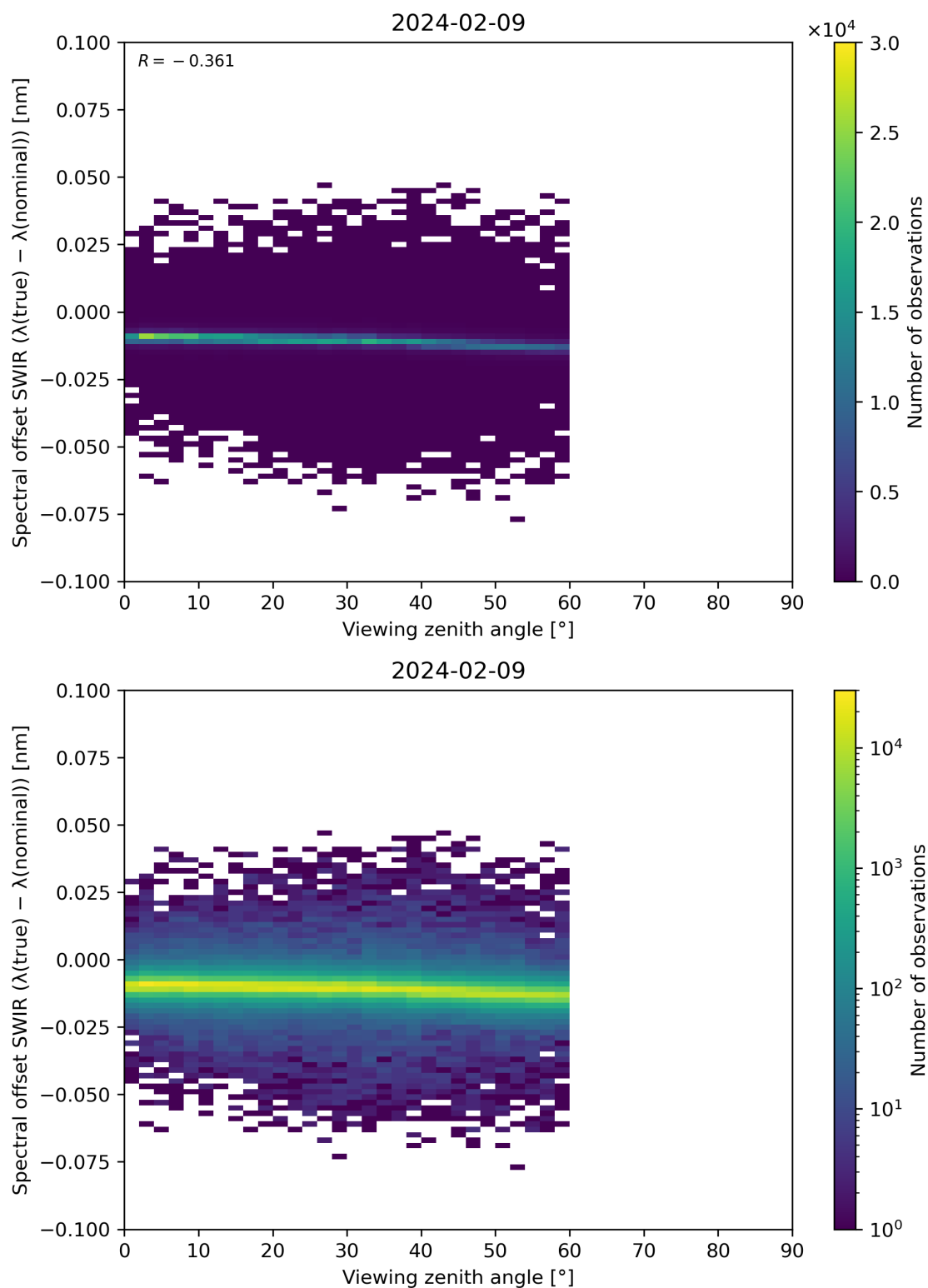
Figure 116: Scatter density plot of “Viewing zenith angle” against “Spectral offset SWIR ( \lambda(\text{true}) - \lambda(\text{nominal}) )” for 2024-02-08 to 2024-02-10.
