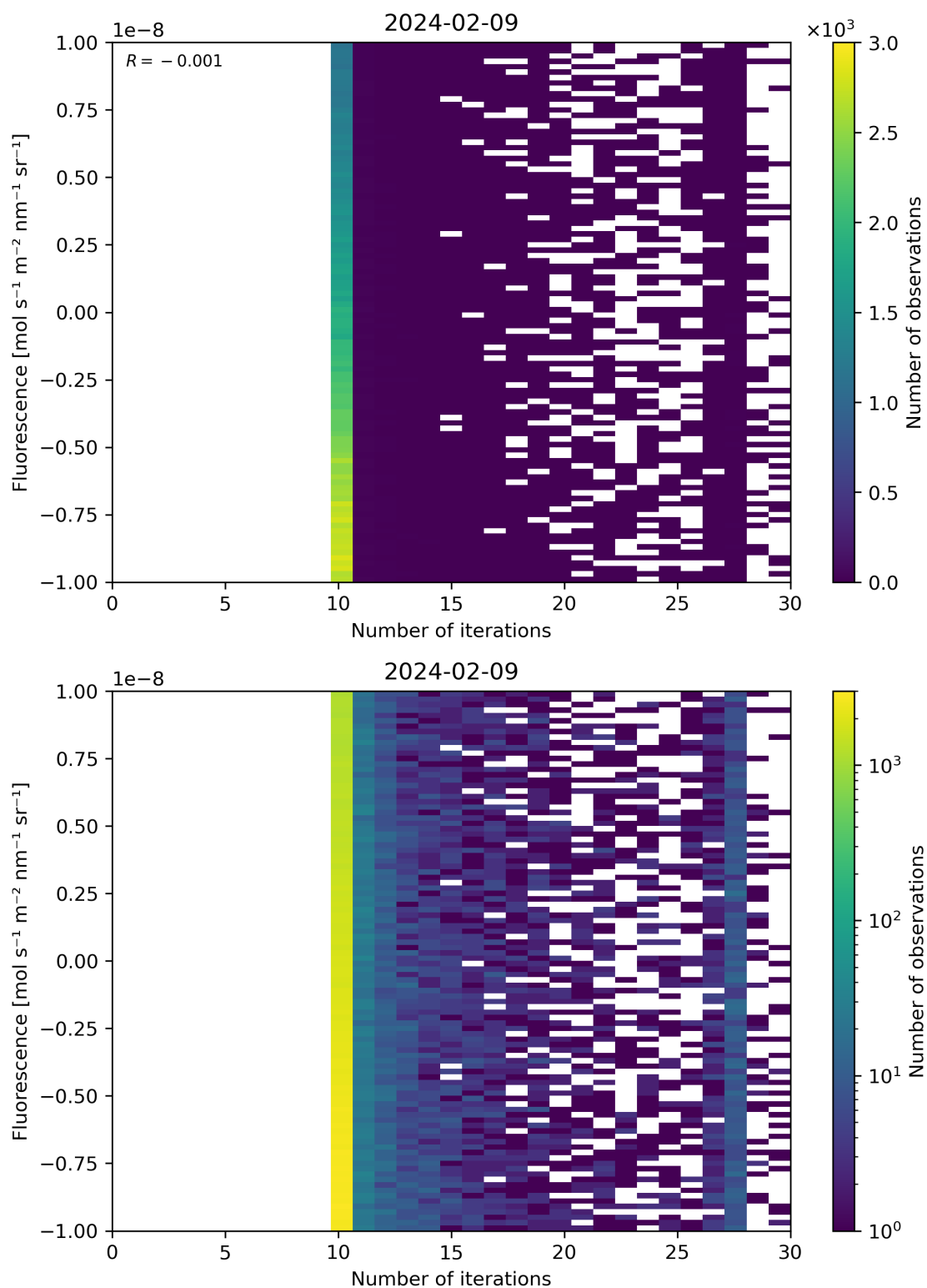
Figure 87: Scatter density plot of “Number of iterations” against “Fluorescence” for 2024-02-08 to 2024-02-10.
