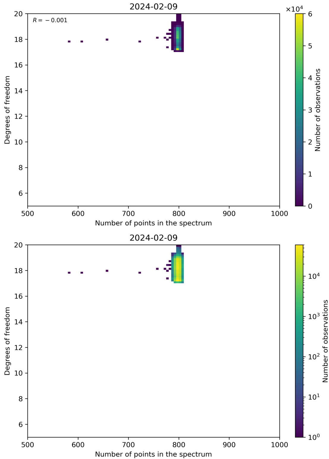
Figure 90: Scatter density plot of “Number of points in the spectrum” against “Degrees of freedom” for 2024-02-08 to 2024-02-10.
