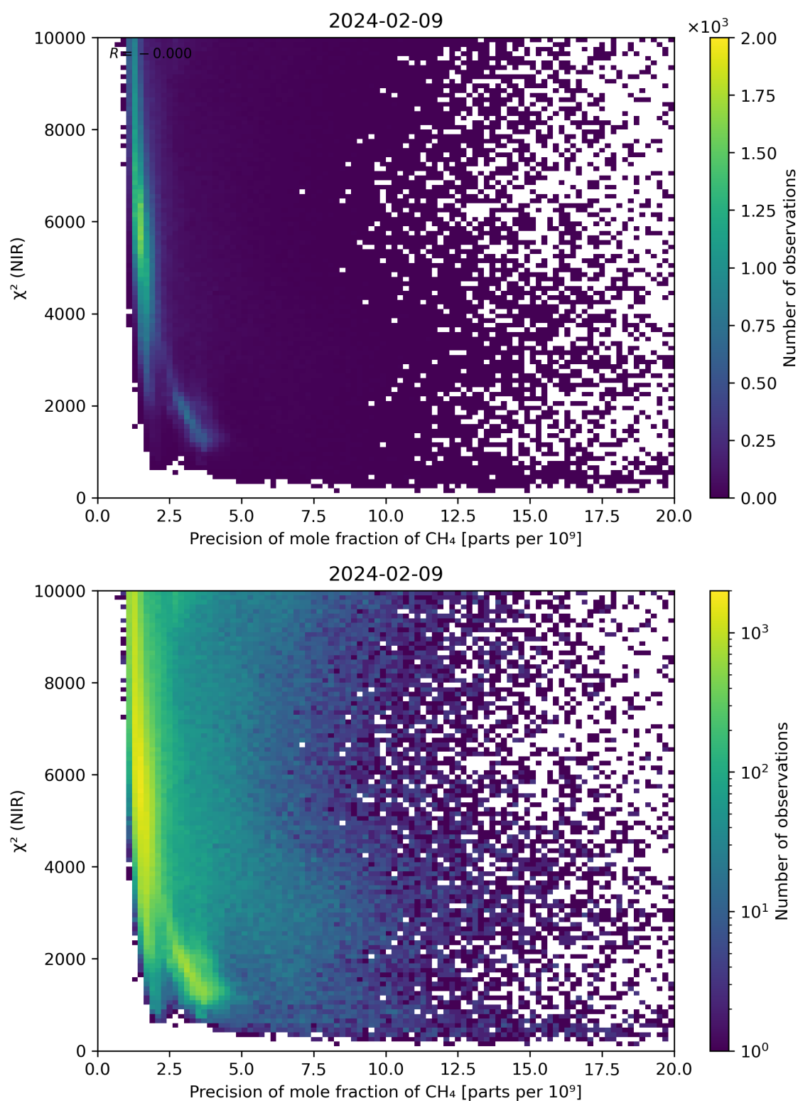
Figure 78: Scatter density plot of “Precision of mole fraction of CH 4 ” against “ \chi^2 (NIR)” for 2024-02-08 to 2024-02-10.
