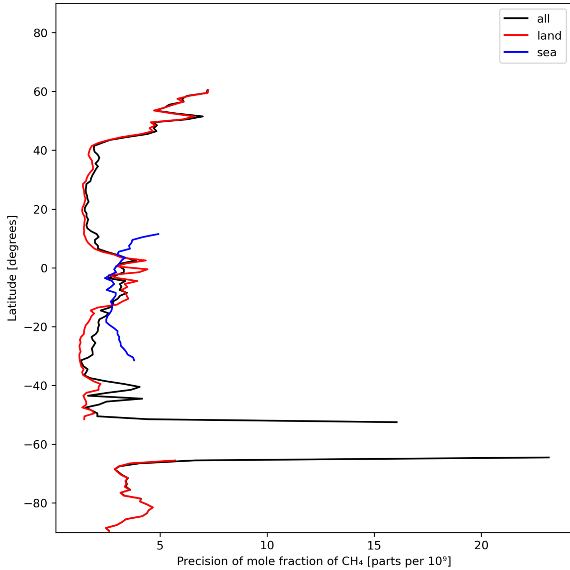
Figure 13: Zonal average of “Precision of mole fraction of CH 4 ” for 2024-02-08 to 2024-02-10.
