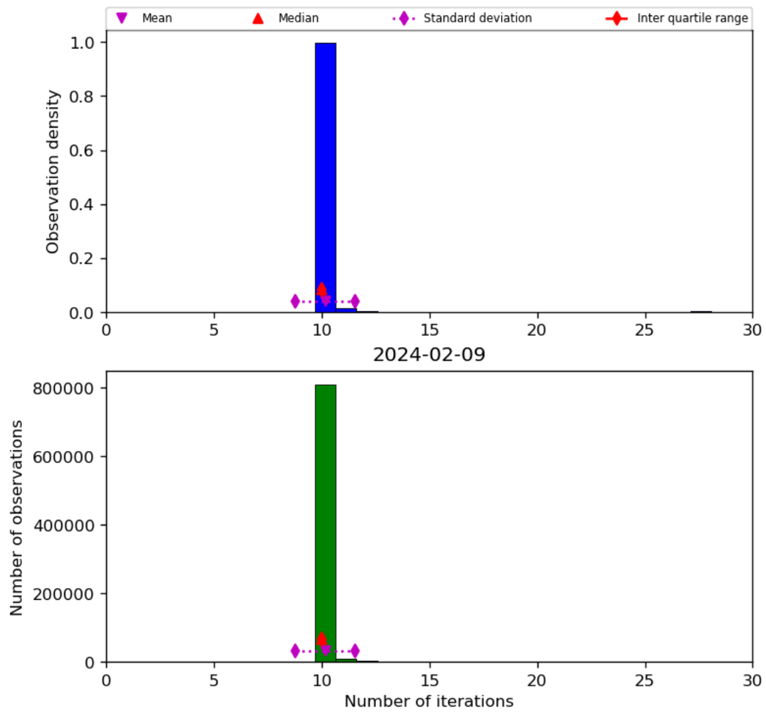
Figure 31: Histogram of "Number of iterations" for 2024-02-08 to 2024-02-10
