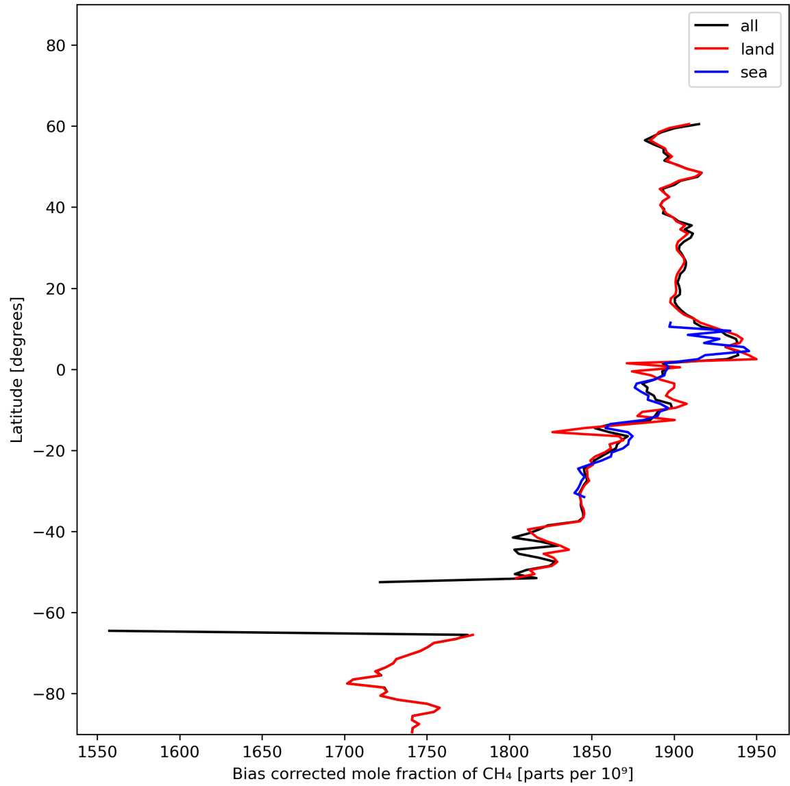
Figure 14: Zonal average of “Bias corrected mole fraction of CH 4 ” for 2024-02-08 to 2024-02-10.
