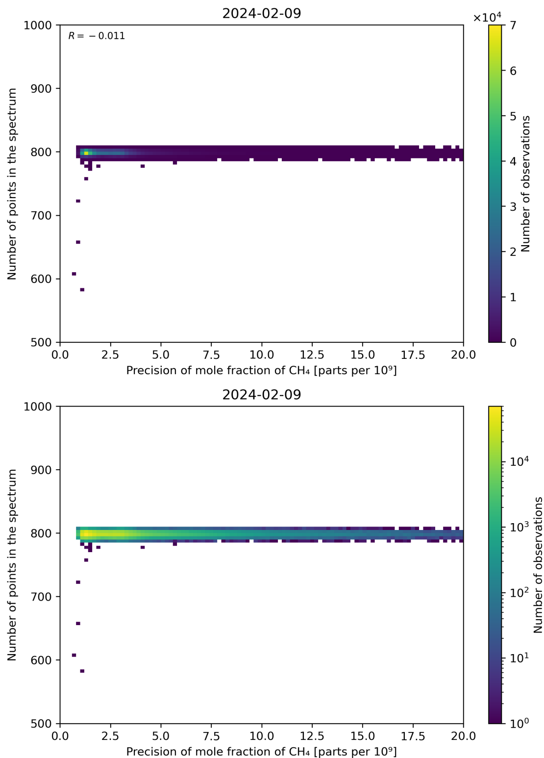
Figure 84: Scatter density plot of “Precision of mole fraction of CH 4 ” against “Number of points in the spectrum” for 2024-02-08 to 2024-02-10.
