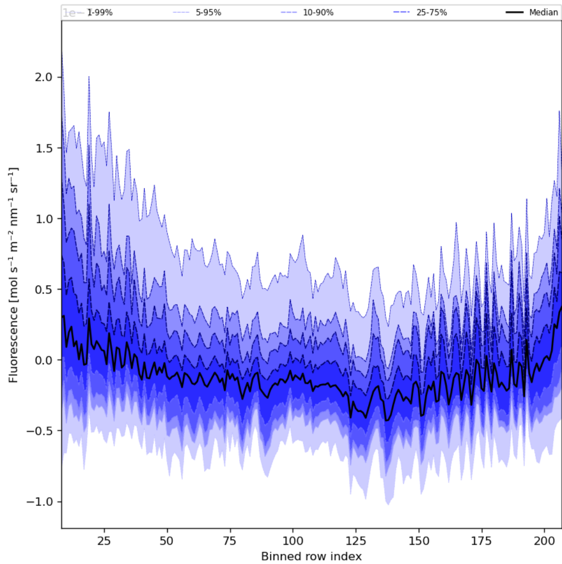
Figure 43: Along track statistics of “Fluorescence” for 2024-02-08 to 2024-02-10
