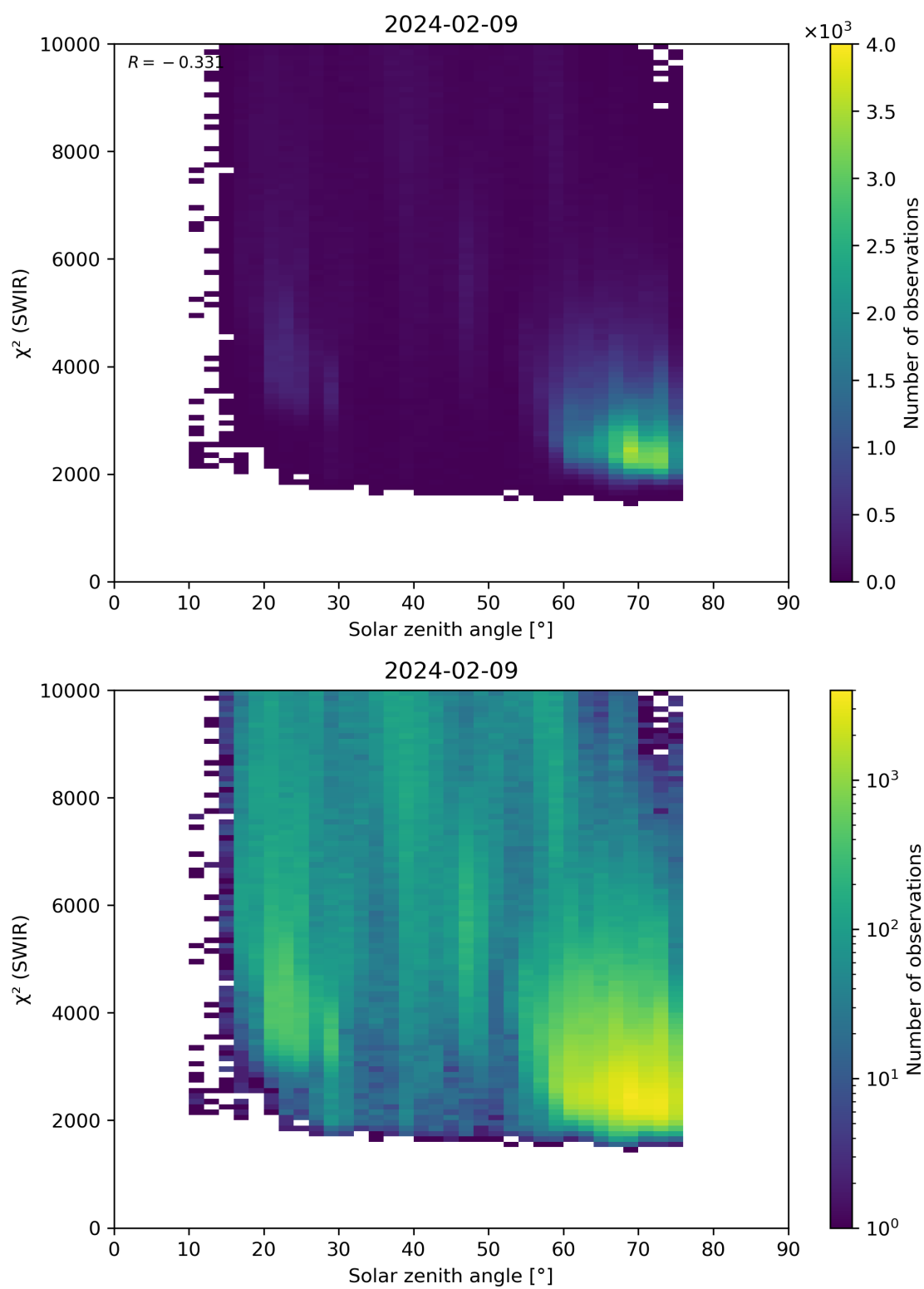
Figure 95: Scatter density plot of “Solar zenith angle” against “ \chi^2 (SWIR)” for 2024-02-08 to 2024-02-10.
