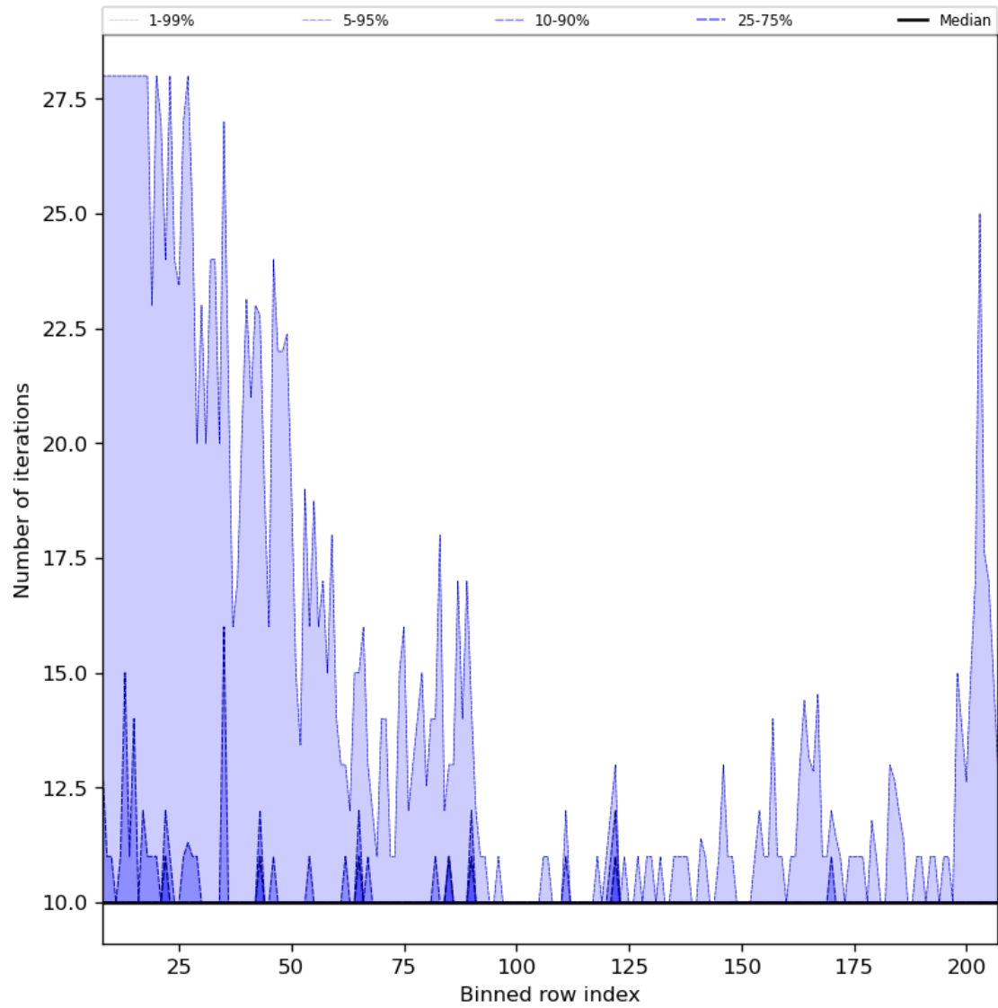
Figure 42: Along track statistics of “Number of iterations” for 2024-02-08 to 2024-02-10
