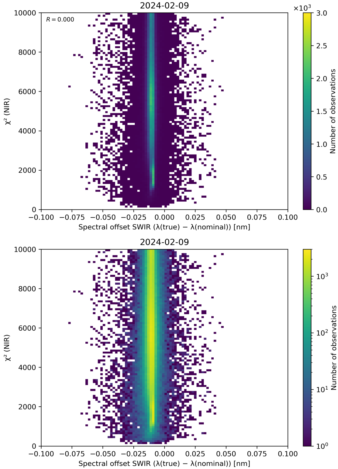
Figure 117: Scatter density plot of “Spectral offset SWIR ( \lambda(\text{true}) - \lambda(\text{nominal}) )” against “ \chi^2 (NIR)” for 2024-02-08 to 2024-02-10.
