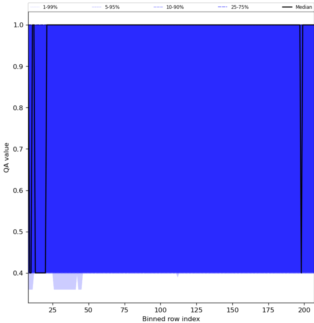
Figure 33: Along track statistics of “QA value” for 2024-02-08 to 2024-02-10
