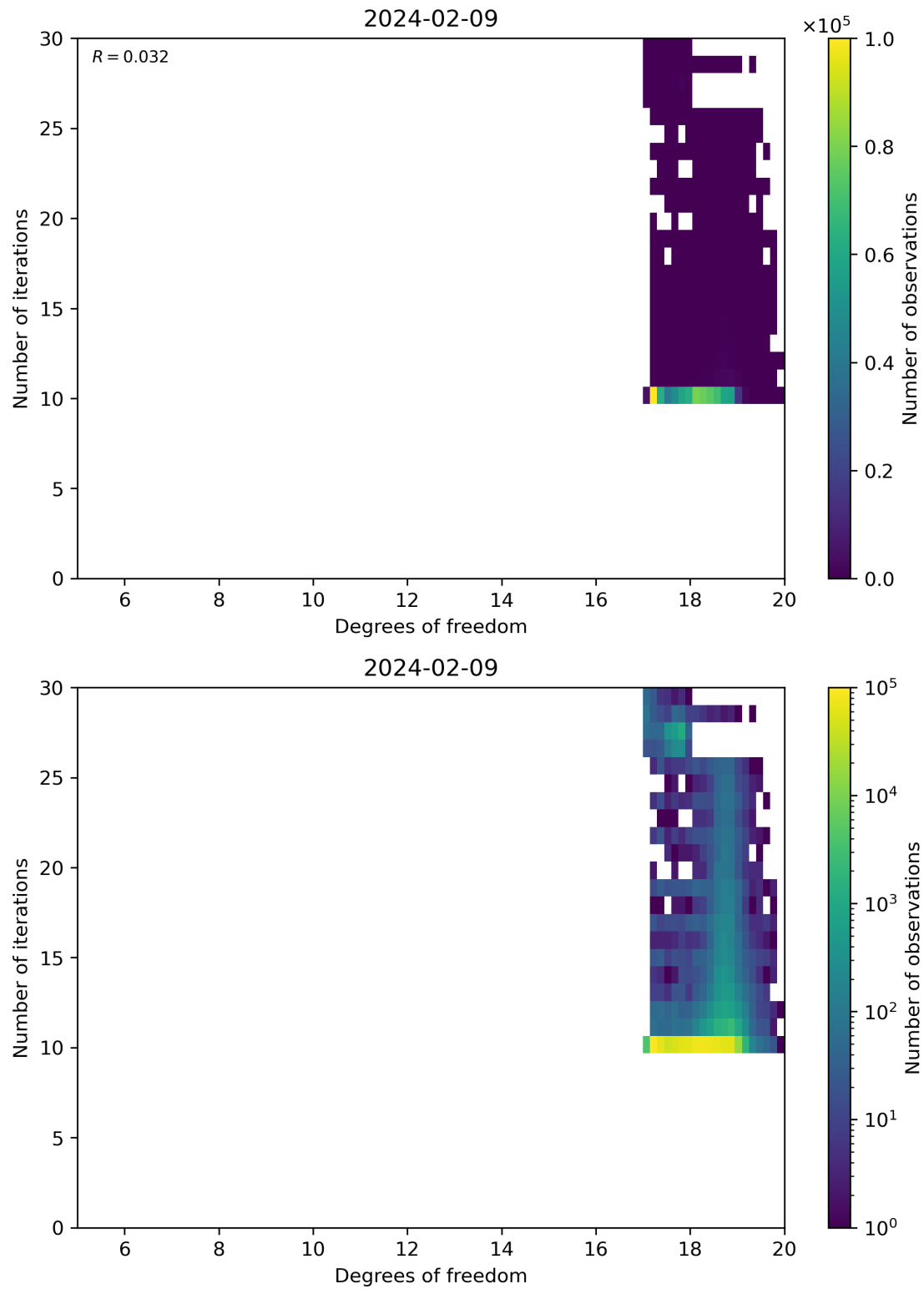
Figure 52: Scatter density plot of “Degrees of freedom” against “Number of iterations” for 2024-02-08 to 2024-02-10.
