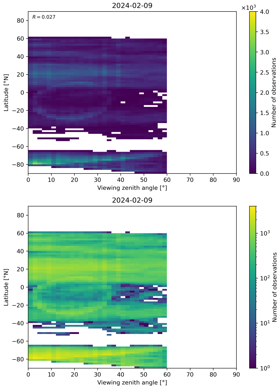
Figure 109: Scatter density plot of “Viewing zenith angle” against “Latitude” for 2024-02-08 to 2024-02-10.
