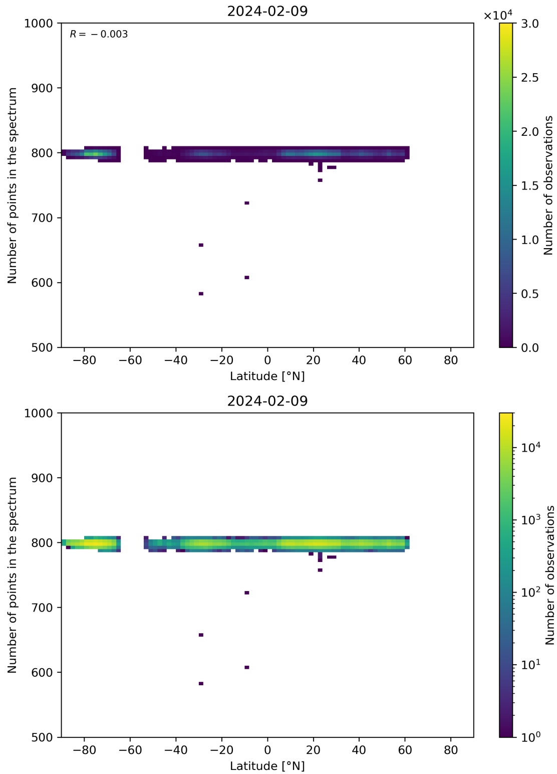
Figure 61: Scatter density plot of “Latitude” against “Number of points in the spectrum” for 2024-02-08 to 2024-02-10.
