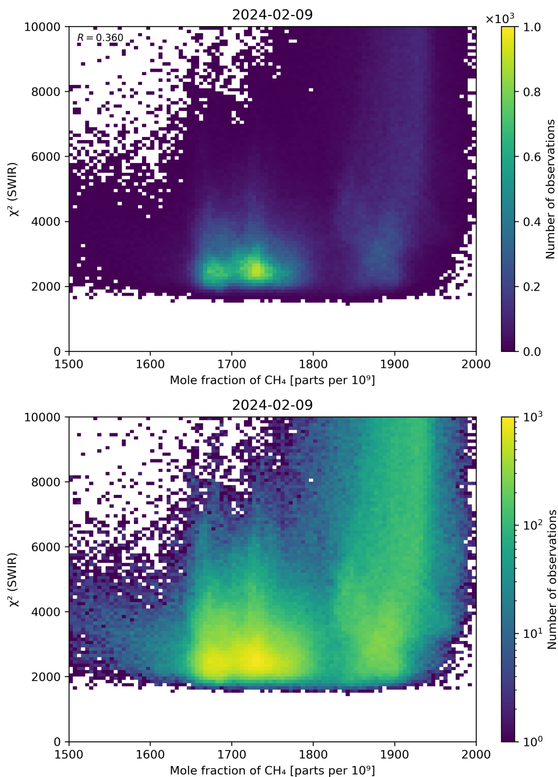
Figure 71: Scatter density plot of “Mole fraction of \text{CH}_4 ” against “ \chi^2 (SWIR)” for 2024-02-08 to 2024-02-10.
