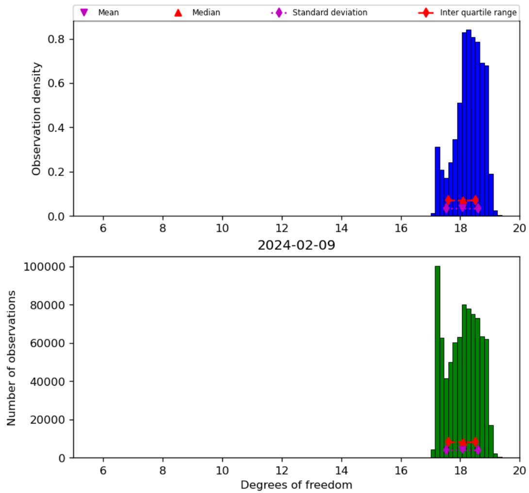
Figure 30: Histogram of “Degrees of freedom” for 2024-02-08 to 2024-02-10
