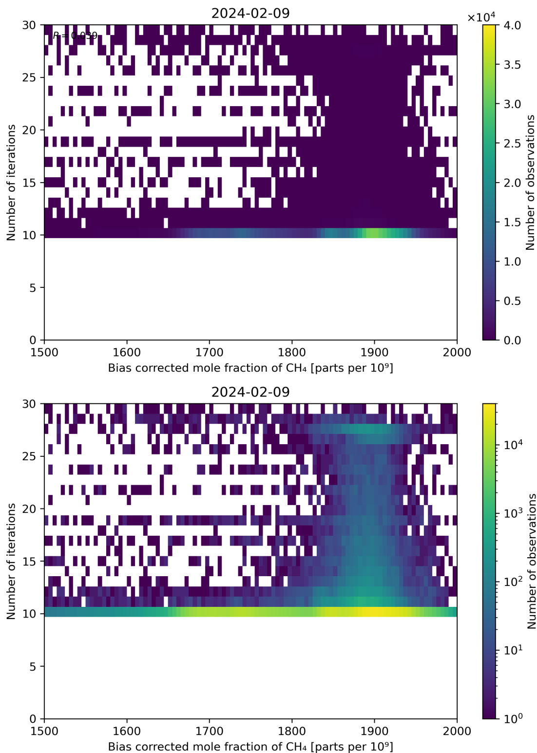
Figure 67: Scatter density plot of “Bias corrected mole fraction of \text{CH}_4 ” against “Number of iterations” for 2024-02-08 to 2024-02-10.
