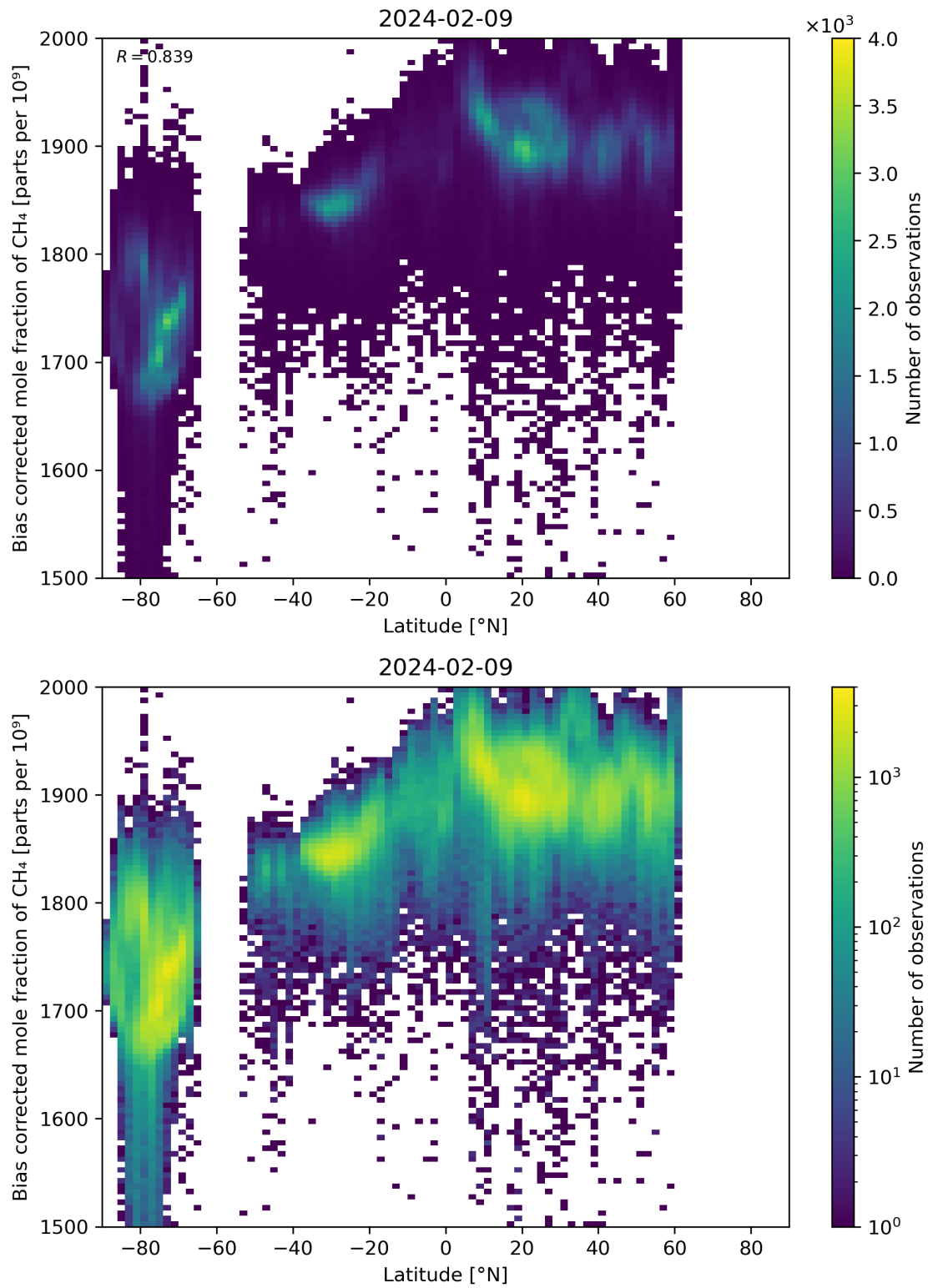
Figure 58: Scatter density plot of “Latitude” against “Bias corrected mole fraction of CH 4 ” for 2024-02-08 to 2024-02-10.
