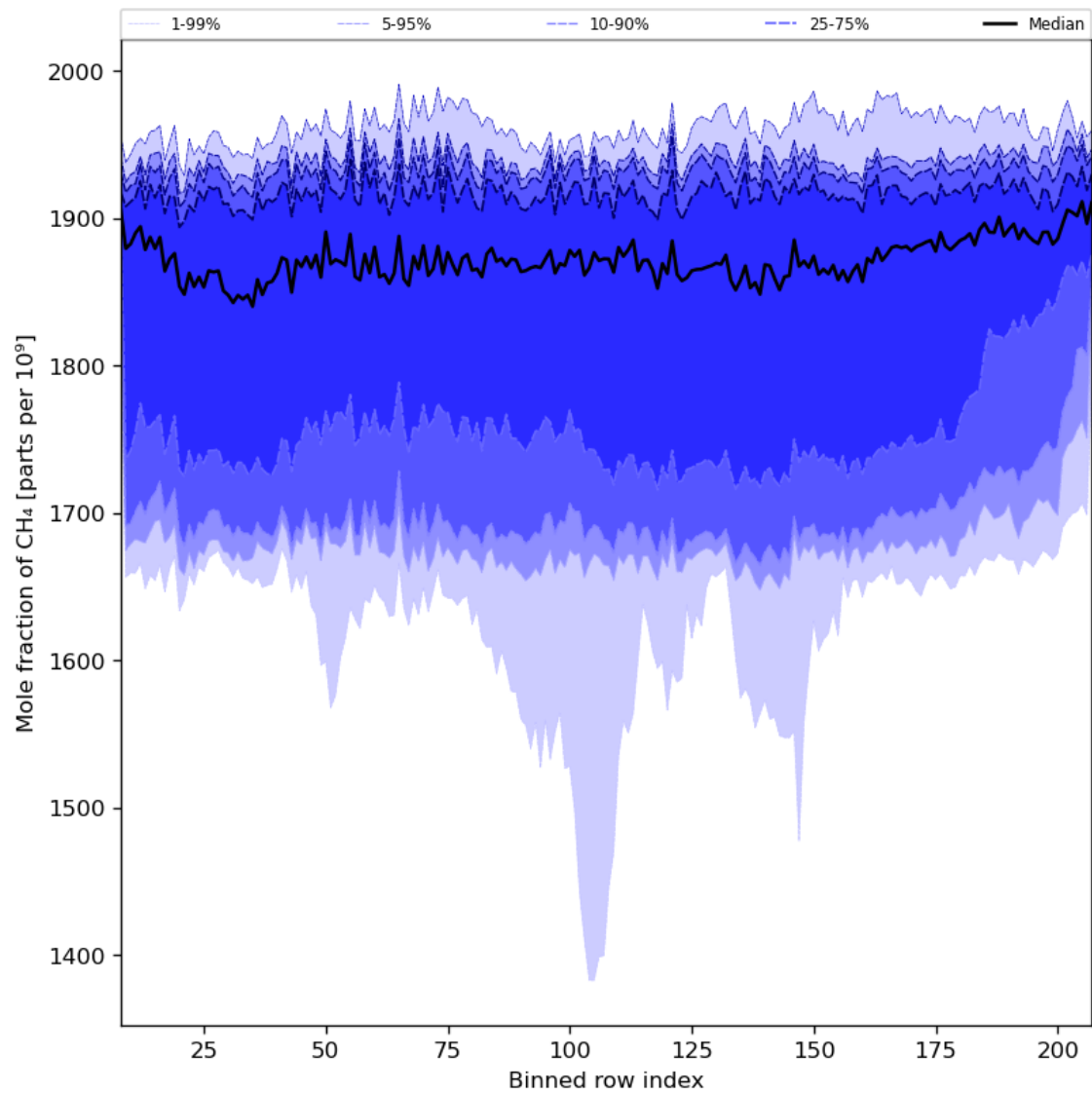
Figure 34: Along track statistics of “Mole fraction of CH 4 ” for 2024-02-08 to 2024-02-10
