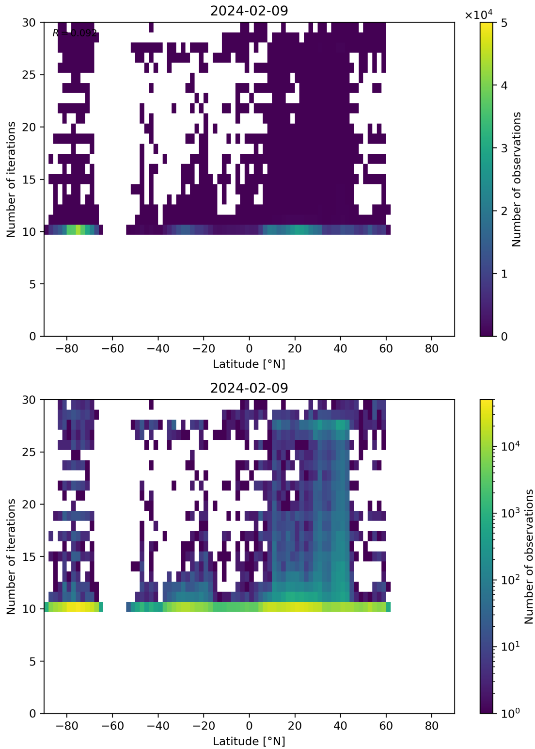
Figure 60: Scatter density plot of “Latitude” against “Number of iterations” for 2024-02-08 to 2024-02-10.
