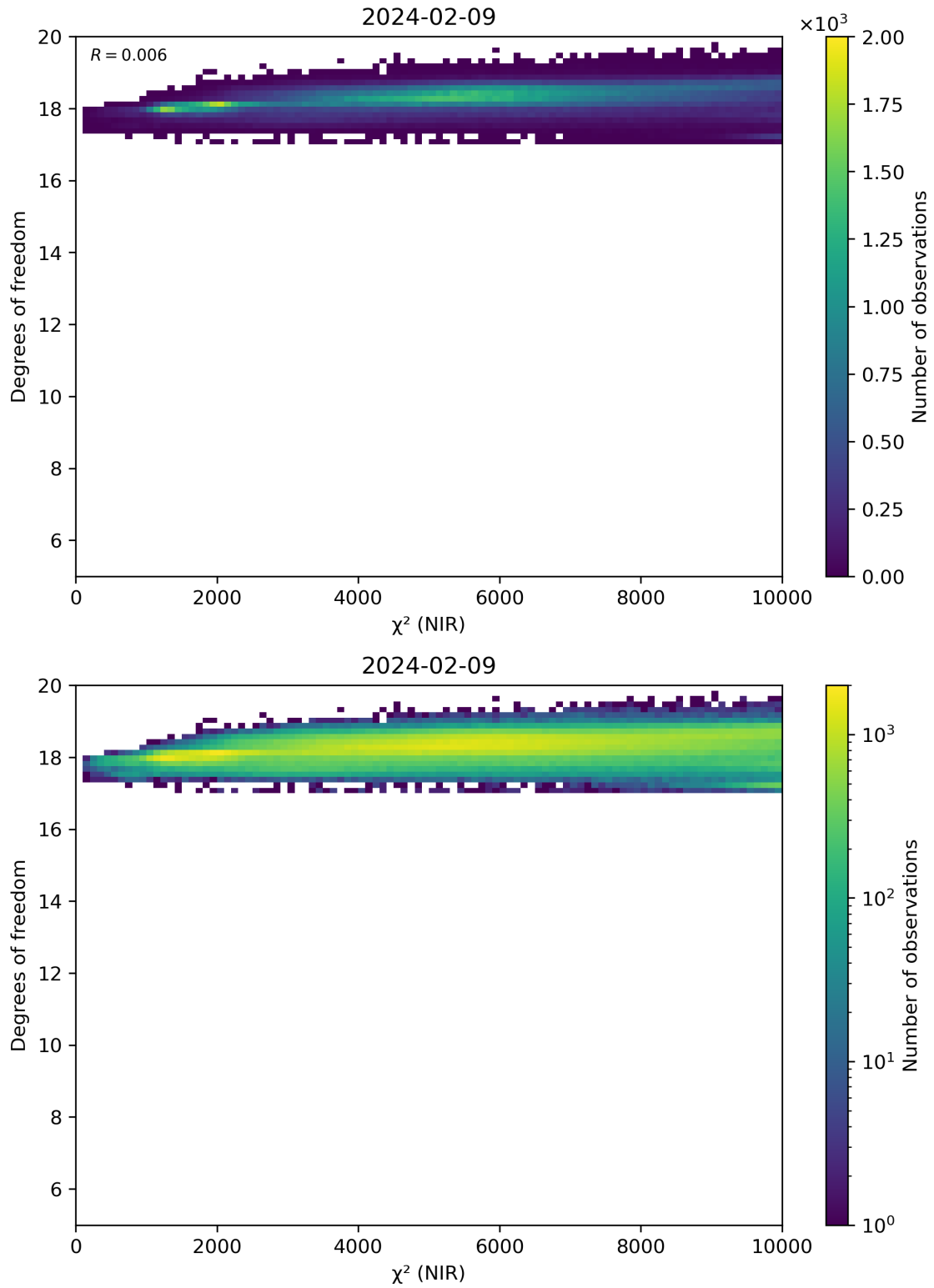
Figure 44: Scatter density plot of “ \chi^2 (NIR)” against “Degrees of freedom” for 2024-02-08 to 2024-02-10.
