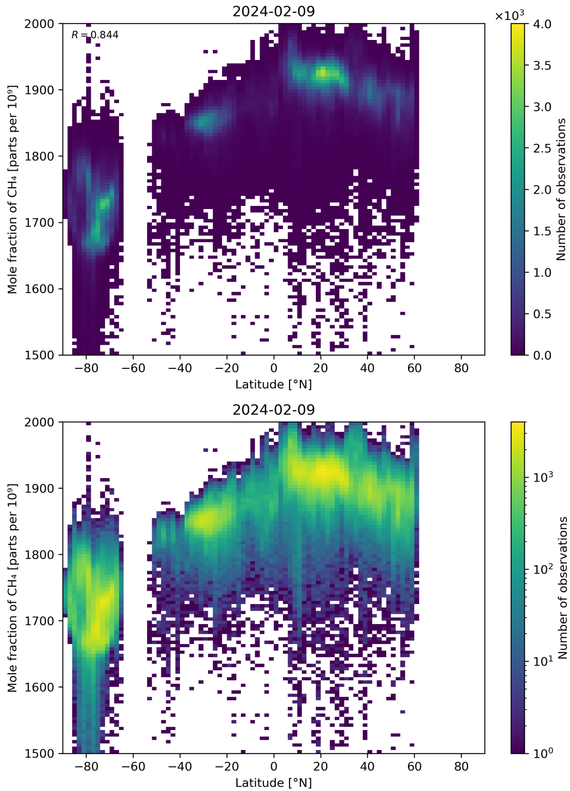
Figure 57: Scatter density plot of “Latitude” against “Mole fraction of CH 4 ” for 2024-02-08 to 2024-02-10.
