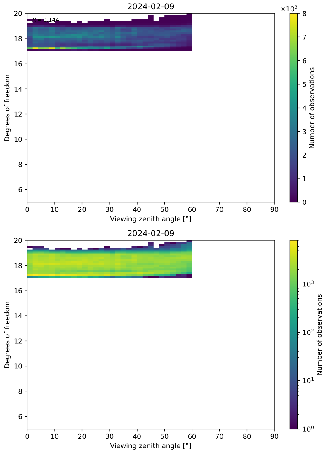
Figure 107: Scatter density plot of “Viewing zenith angle” against “Degrees of freedom” for 2024-02-08 to 2024-02-10.
