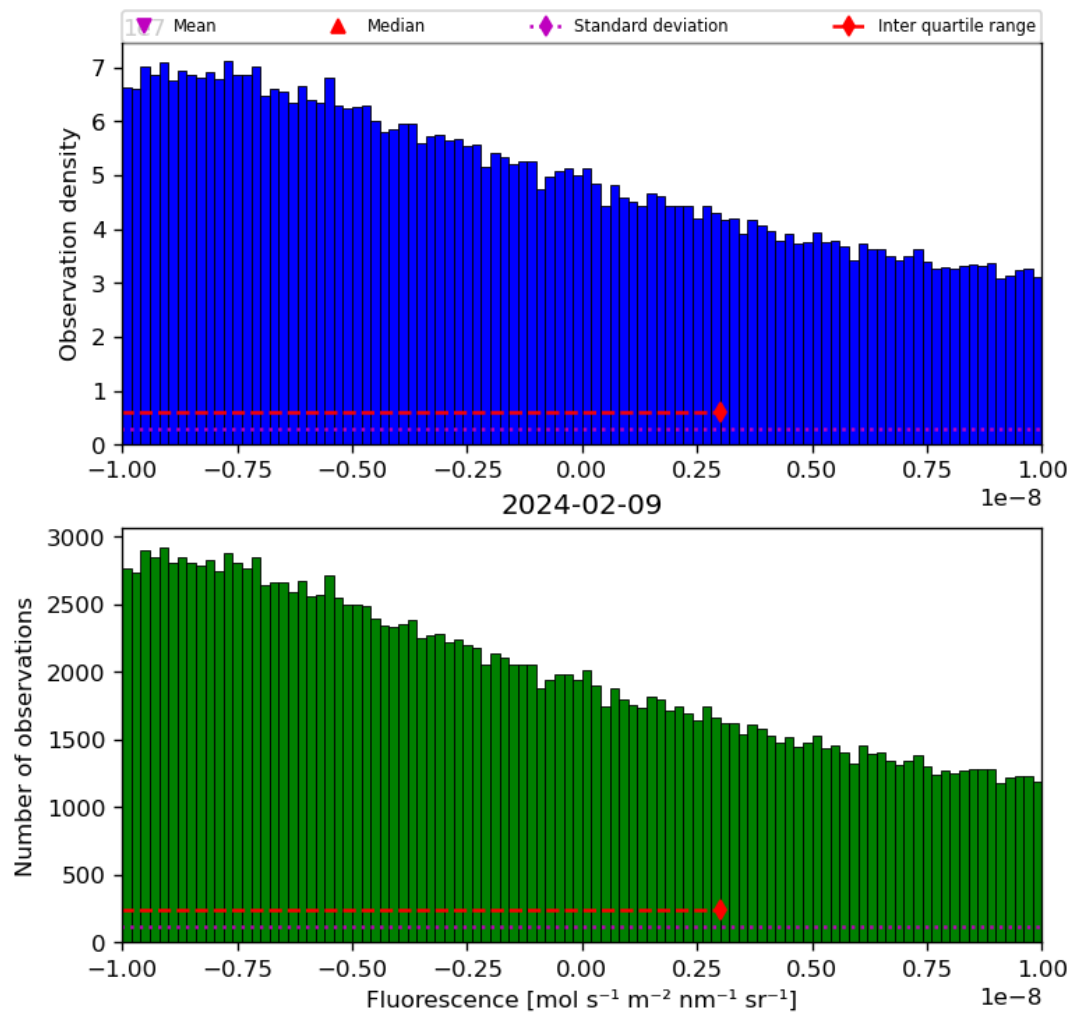
Figure 32: Histogram of “Fluorescence” for 2024-02-08 to 2024-02-10
