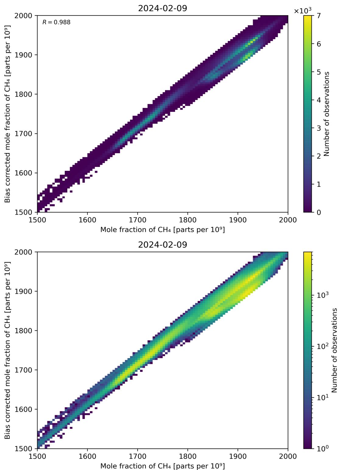
Figure 74: Scatter density plot of “Mole fraction of CH 4 ” against “Bias corrected mole fraction of CH 4 ” for 2024-02-08 to 2024-02-10.
