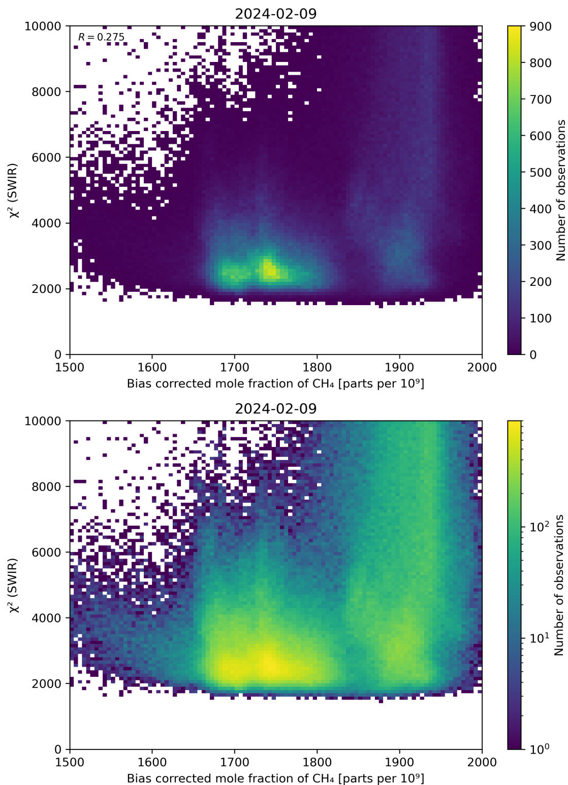
Figure 64: Scatter density plot of “Bias corrected mole fraction of CH 4 ” against “ \chi^2 (SWIR)” for 2024-02-08 to 2024-02-10.
