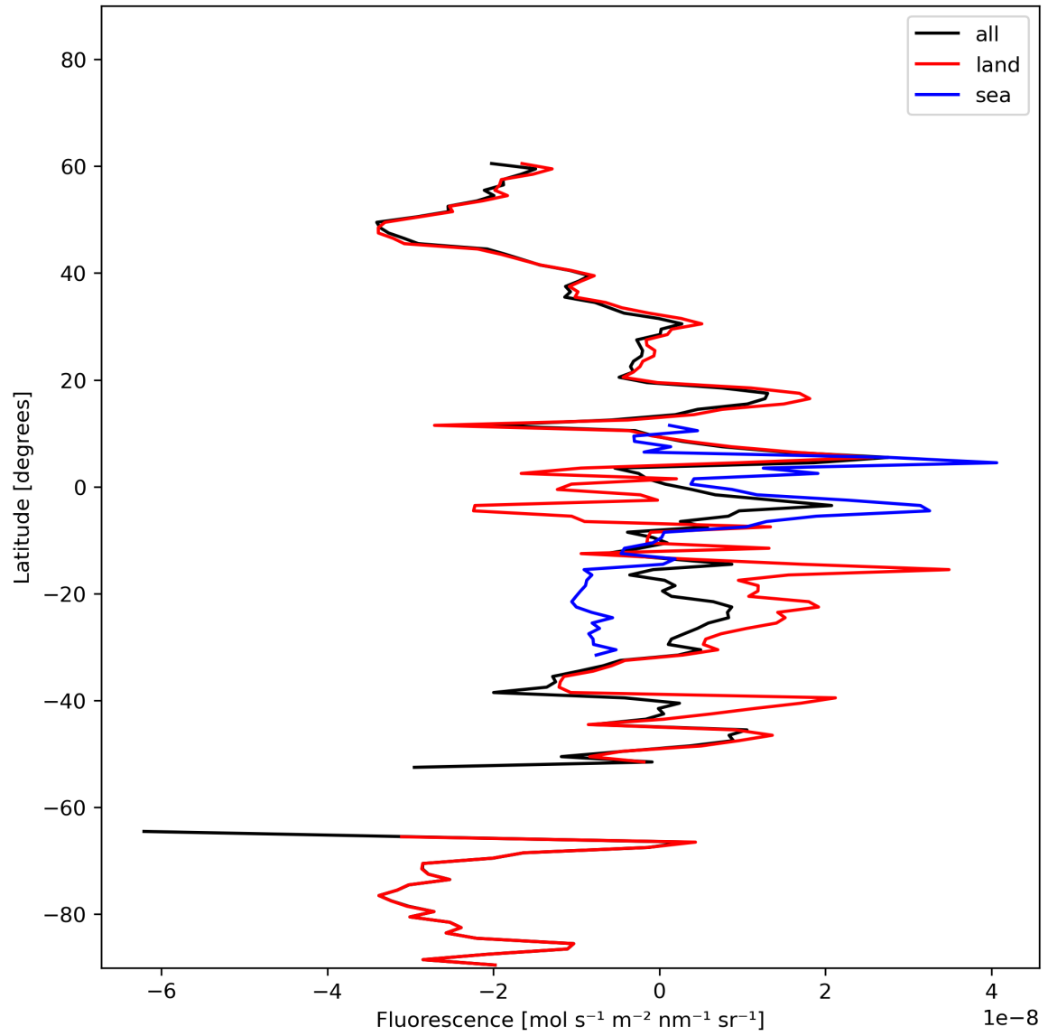
Figure 21: Zonal average of “Fluorescence” for 2024-02-08 to 2024-02-10.
