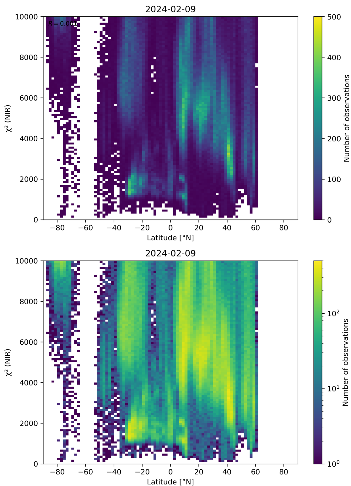
Figure 53: Scatter density plot of “Latitude” against “ \chi^2 (NIR)” for 2024-02-08 to 2024-02-10.
