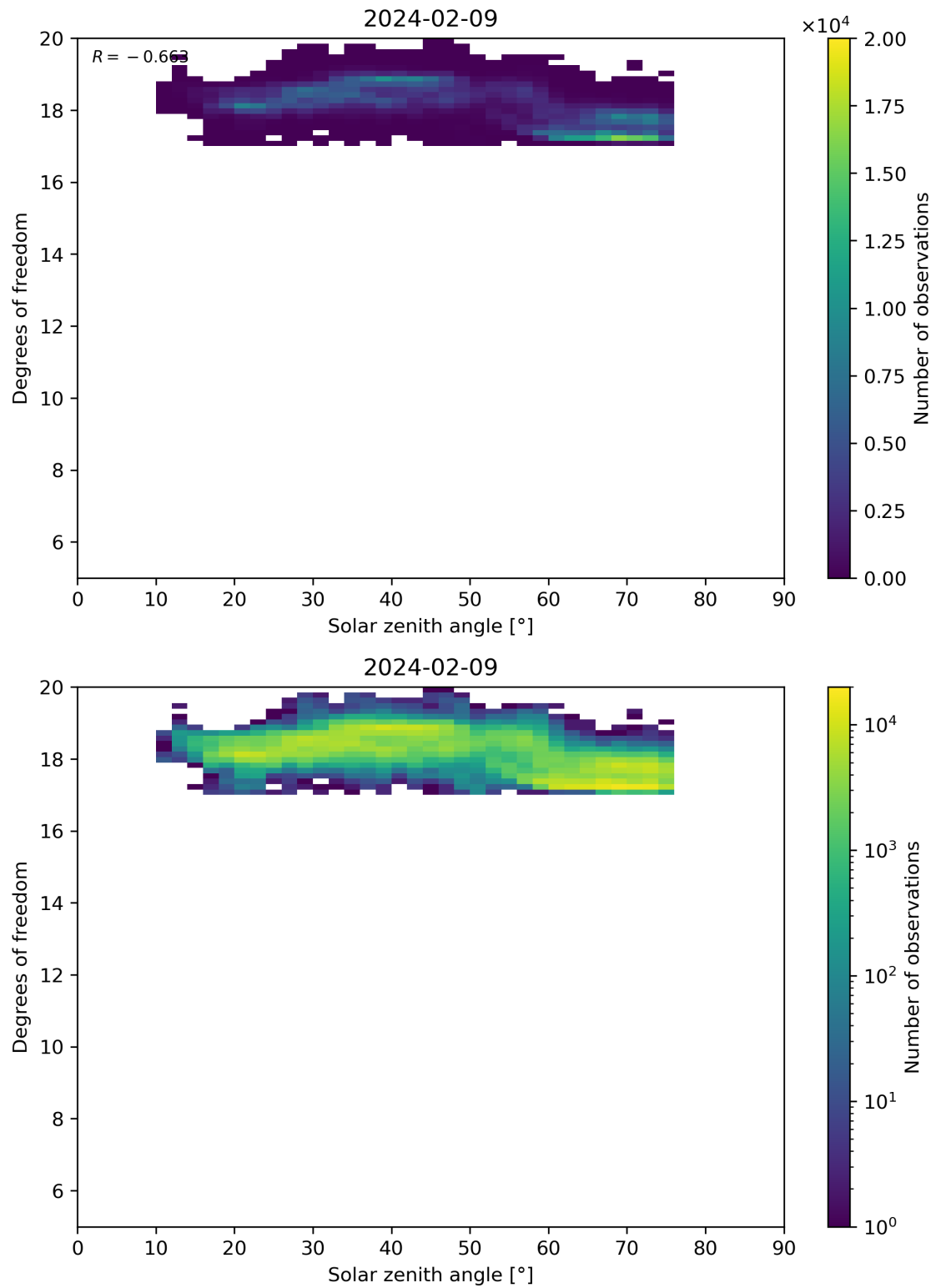
Figure 96: Scatter density plot of “Solar zenith angle” against “Degrees of freedom” for 2024-02-08 to 2024-02-10.
