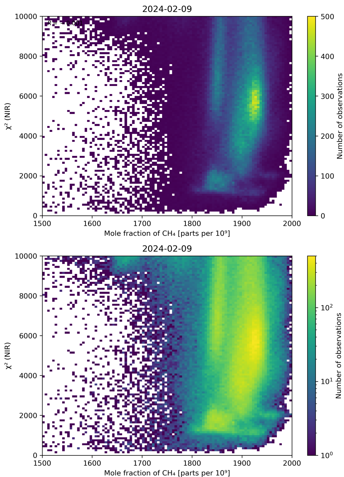
Figure 70: Scatter density plot of “Mole fraction of \text{CH}_4 ” against “ \chi^2 (NIR)” for 2024-02-08 to 2024-02-10.
