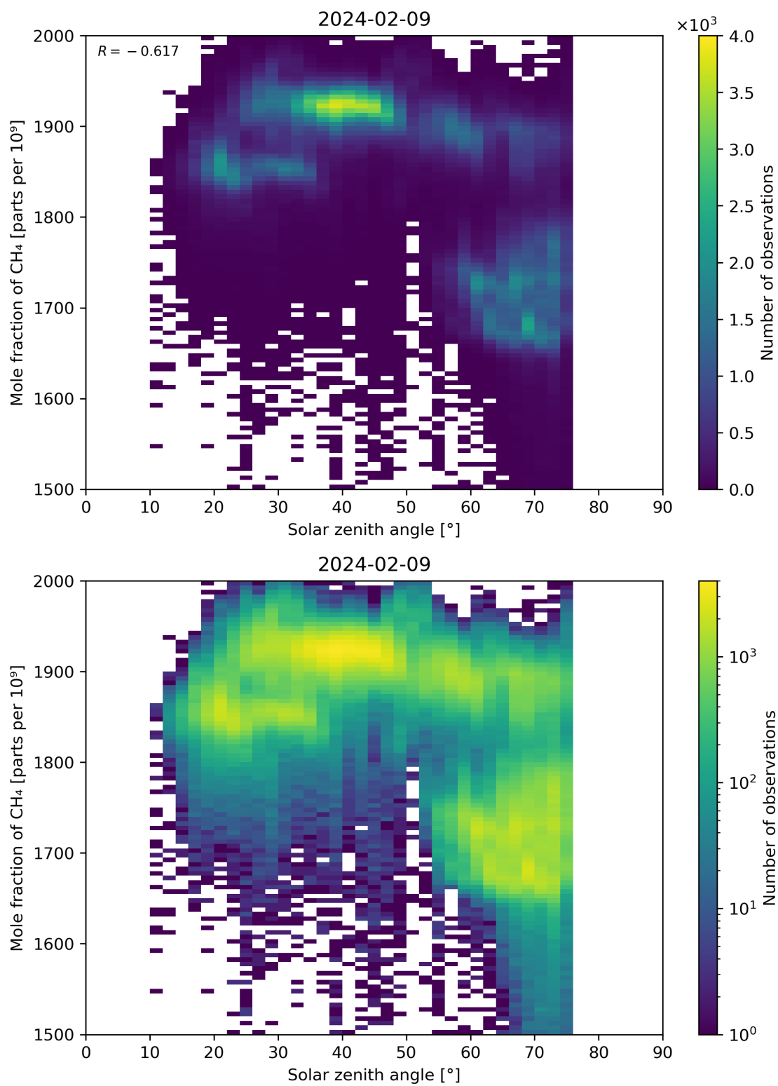
Figure 99: Scatter density plot of “Solar zenith angle” against “Mole fraction of CH 4 ” for 2024-02-08 to 2024-02-10.
