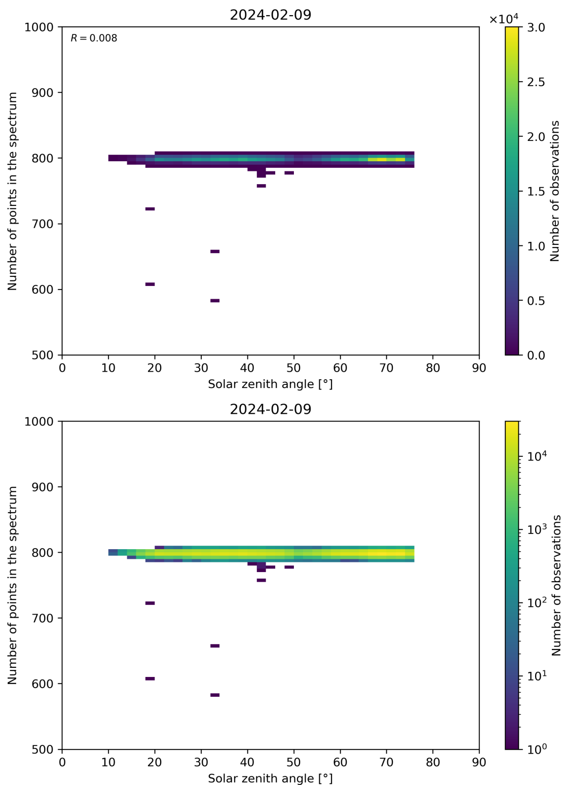
Figure 103: Scatter density plot of “Solar zenith angle” against “Number of points in the spectrum” for 2024-02-08 to 2024-02-10.
