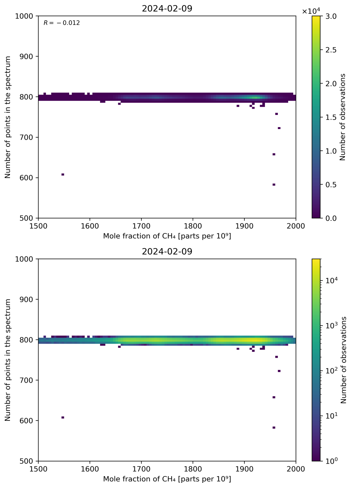
Figure 77: Scatter density plot of “Mole fraction of CH 4 ” against “Number of points in the spectrum” for 2024-02-08 to 2024-02-10.
