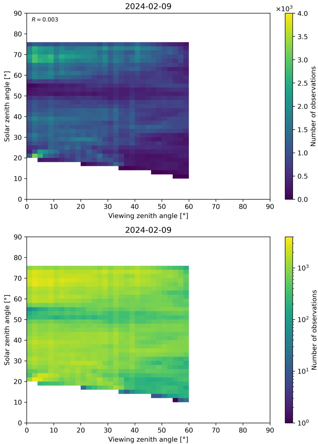
Figure 115: Scatter density plot of “Viewing zenith angle” against “Solar zenith angle” for 2024-02-08 to 2024-02-10.
