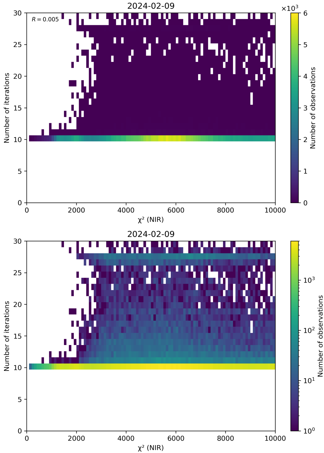
Figure 46: Scatter density plot of “ \chi^2 (NIR)” against “Number of iterations” for 2024-02-08 to 2024-02-10.
