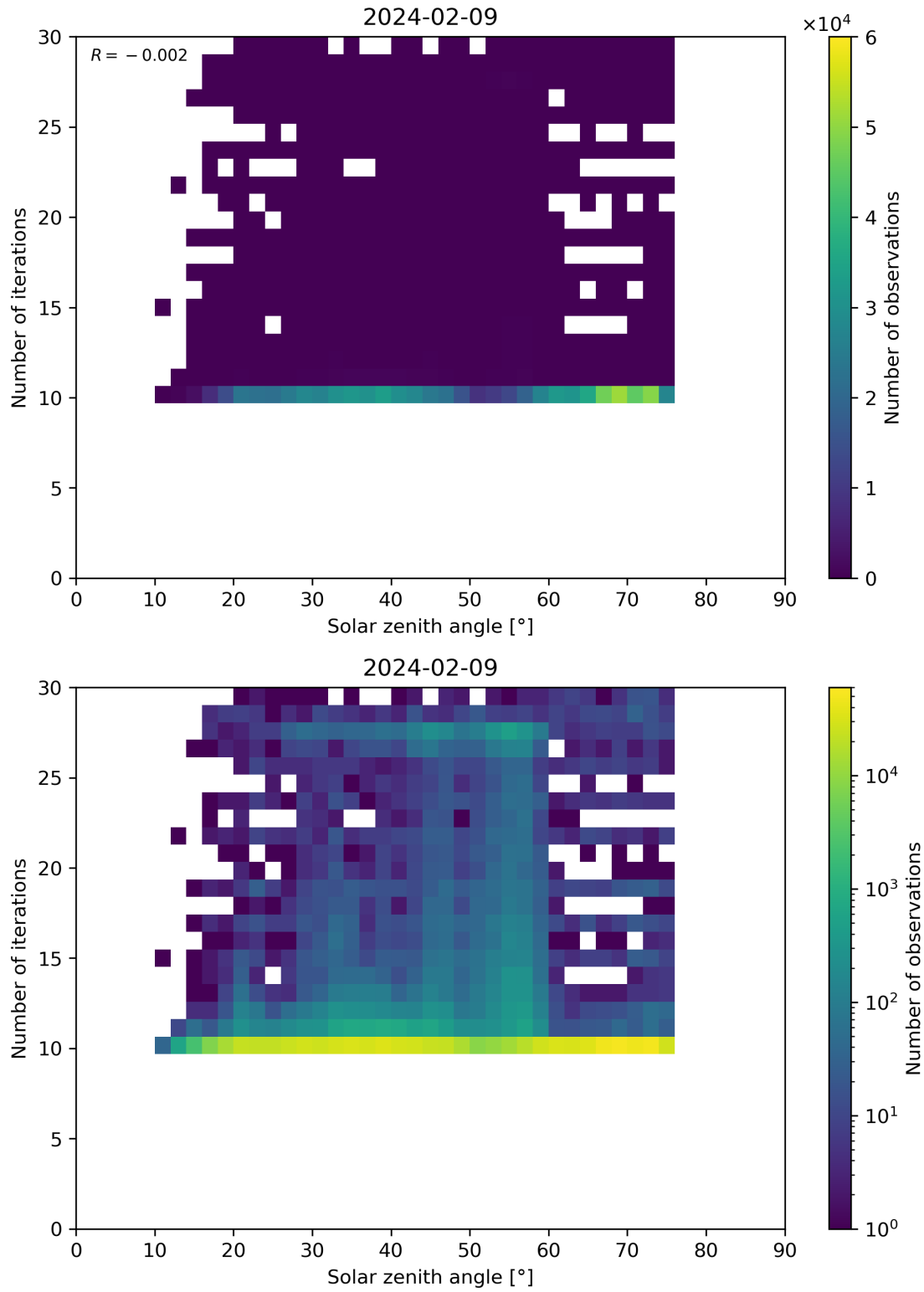
Figure 102: Scatter density plot of “Solar zenith angle” against “Number of iterations” for 2024-02-08 to 2024-02-10.
