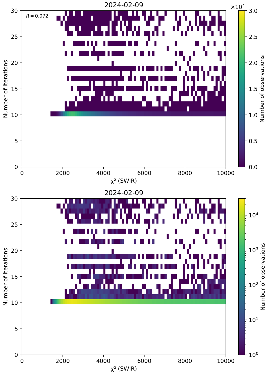
Figure 50: Scatter density plot of “ \chi^2 (SWIR)” against “Number of iterations” for 2024-02-08 to 2024-02-10.
