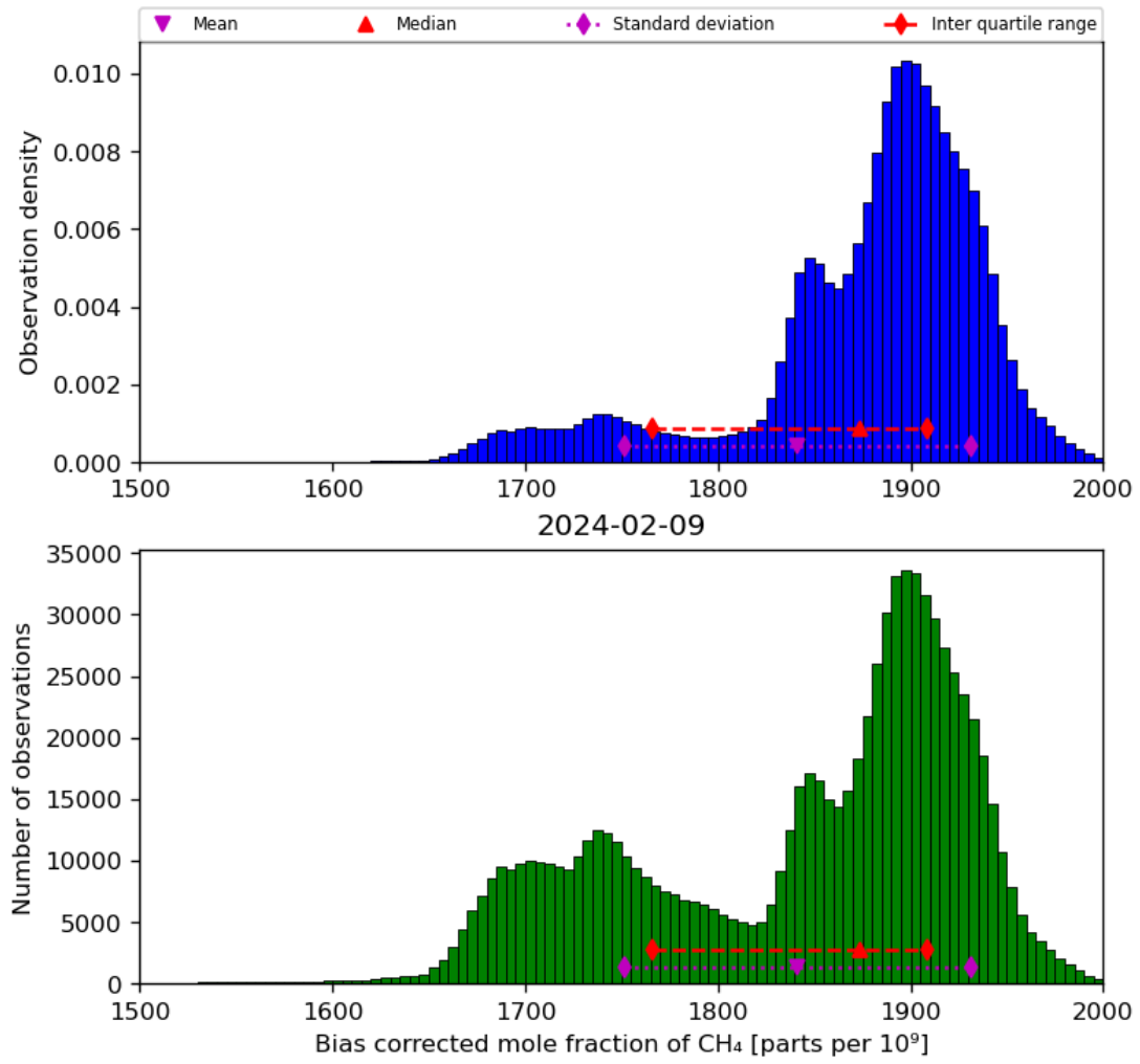
Figure 25: Histogram of “Bias corrected mole fraction of CH 4 ” for 2024-02-08 to 2024-02-10
