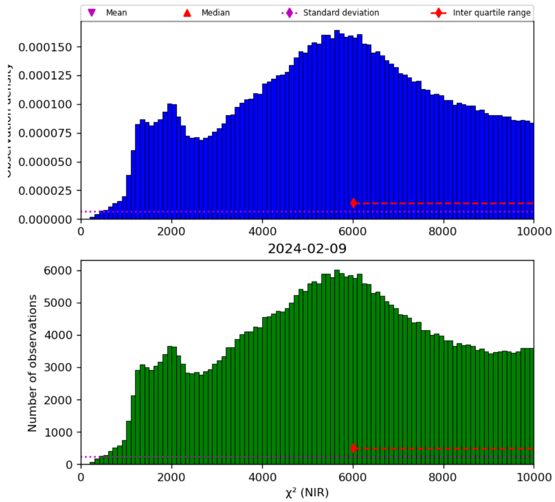
Figure 29: Histogram of “ \chi^2 (NIR)” for 2024-02-08 to 2024-02-10
