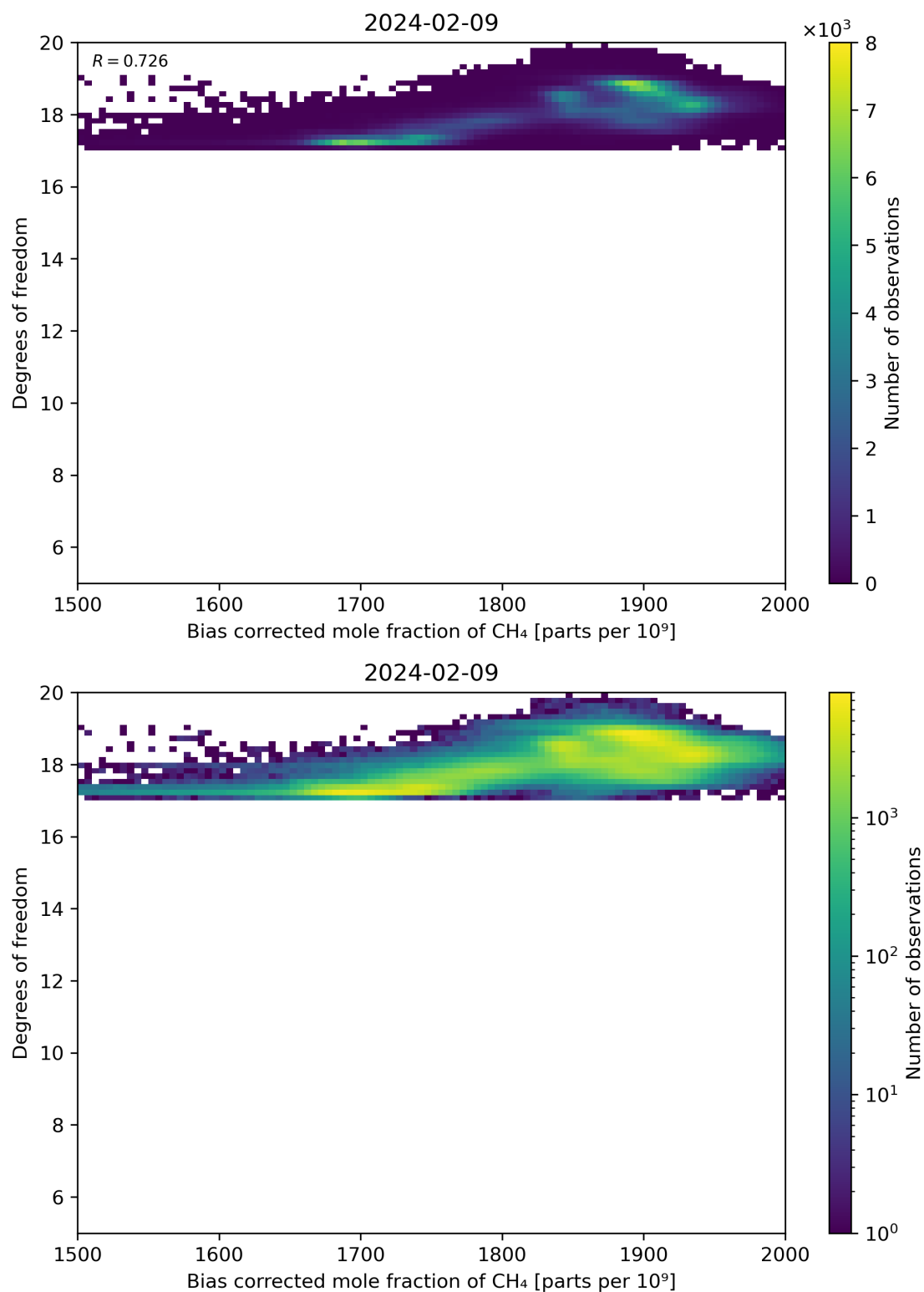
Figure 65: Scatter density plot of “Bias corrected mole fraction of CH 4 ” against “Degrees of freedom” for 2024-02-08 to 2024-02-10.
