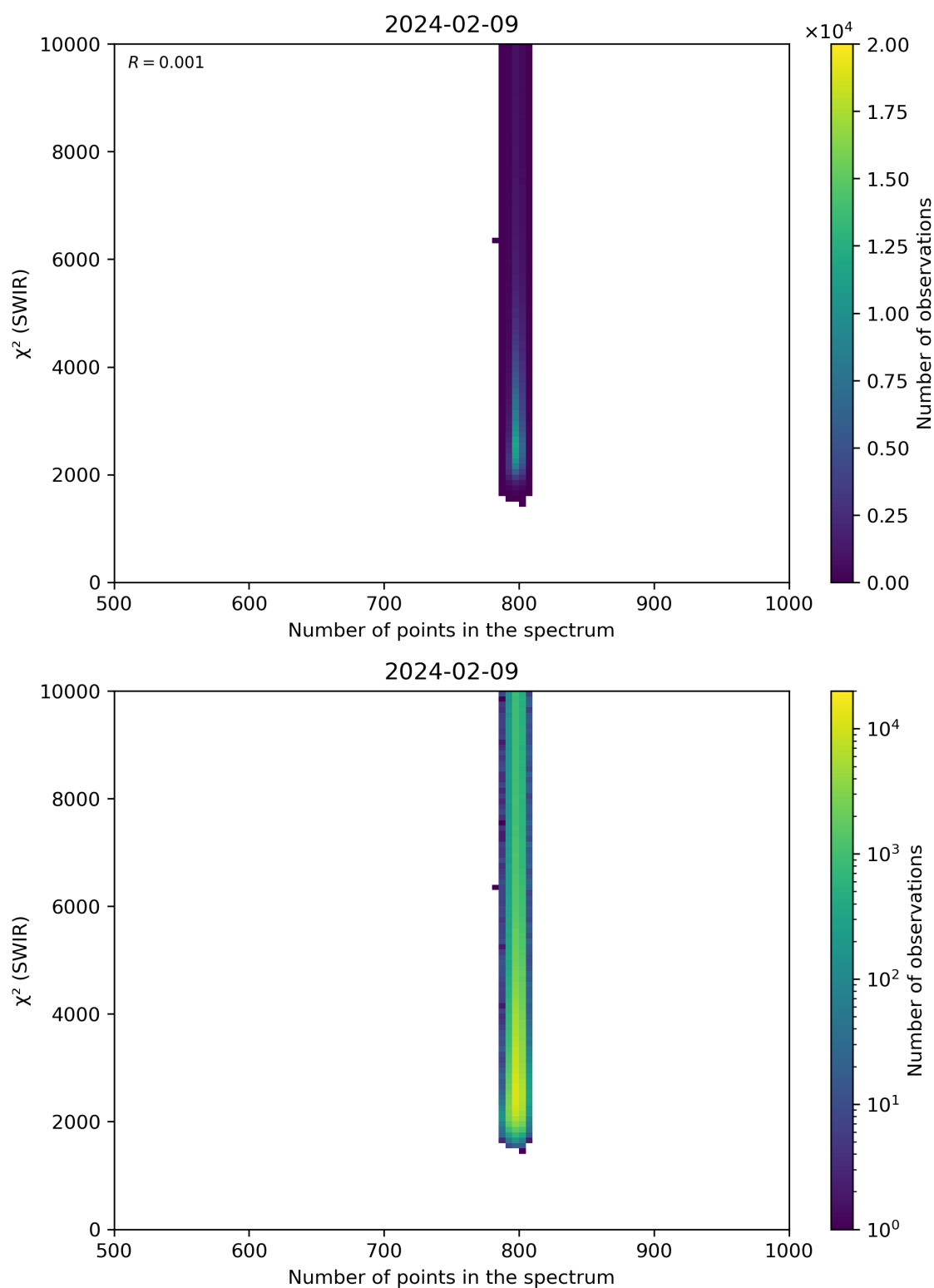
Figure 89: Scatter density plot of “Number of points in the spectrum” against “ \chi^2 (SWIR)” for 2024-02-08 to 2024-02-10.
