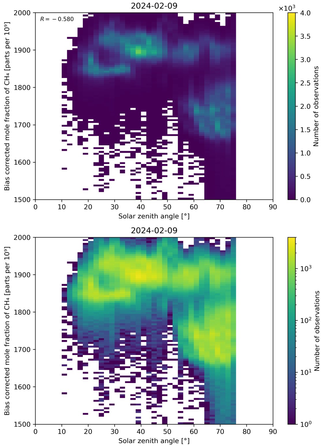
Figure 100: Scatter density plot of “Solar zenith angle” against “Bias corrected mole fraction of CH 4 ” for 2024-02-08 to 2024-02-10.
