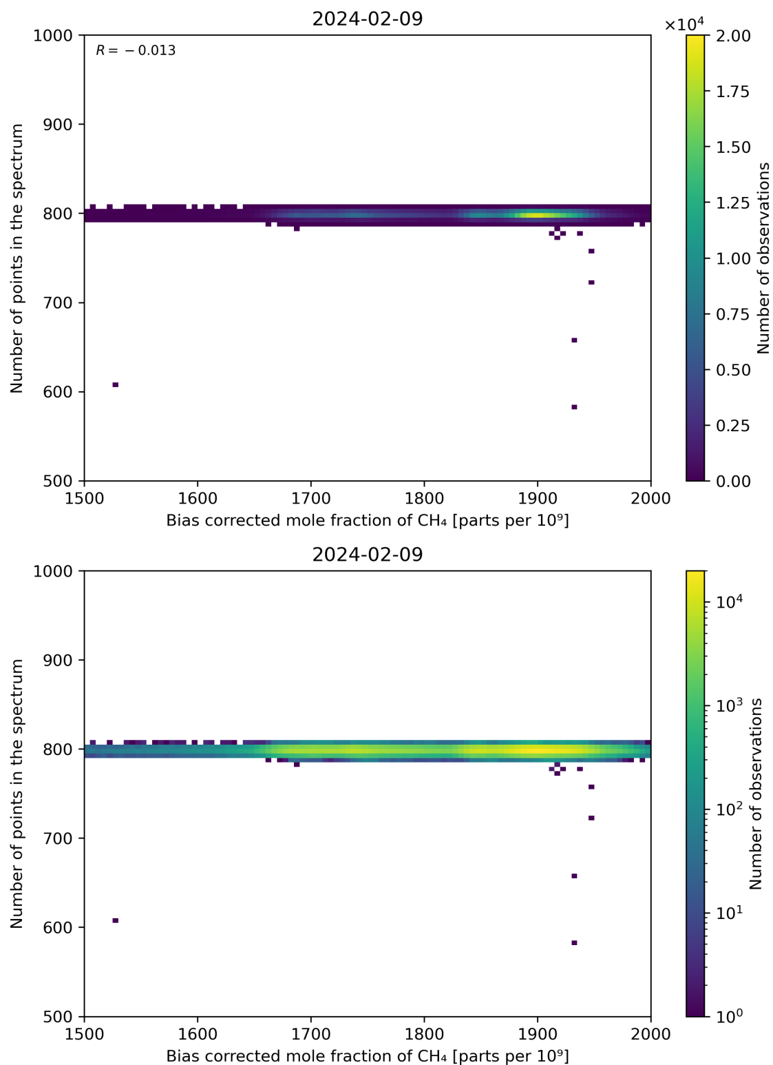
Figure 68: Scatter density plot of “Bias corrected mole fraction of CH 4 ” against “Number of points in the spectrum” for 2024-02-08 to 2024-02-10.
