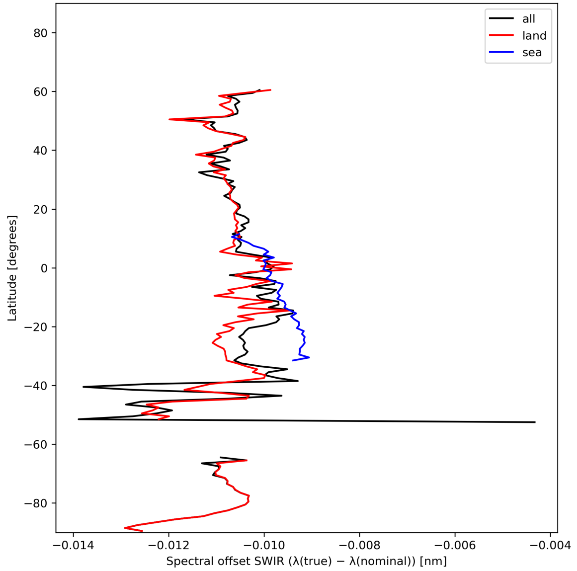
Figure 16: Zonal average of “Spectral offset SWIR ( \lambda(\text{true}) - \lambda(\text{nominal}) )” for 2024-02-08 to 2024-02-10.
