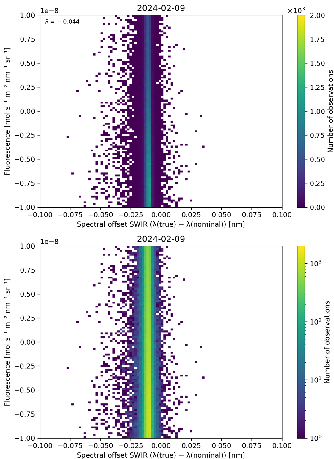
Figure 120: Scatter density plot of “Spectral offset SWIR ( \lambda(\text{true}) - \lambda(\text{nominal}) )” against “Fluorescence” for 2024-02-08 to 2024-02-10.
