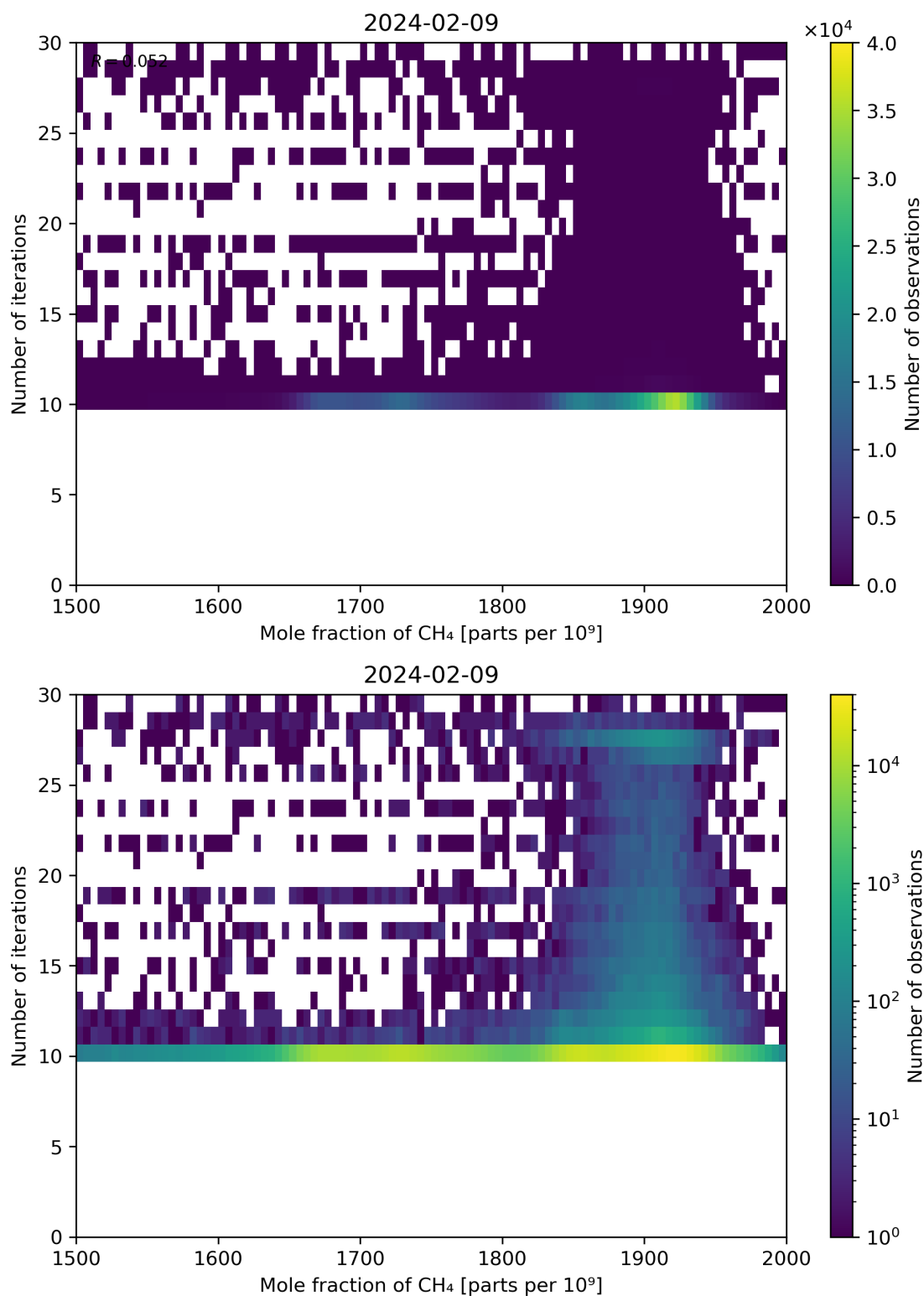
Figure 76: Scatter density plot of “Mole fraction of CH 4 ” against “Number of iterations” for 2024-02-08 to 2024-02-10.
