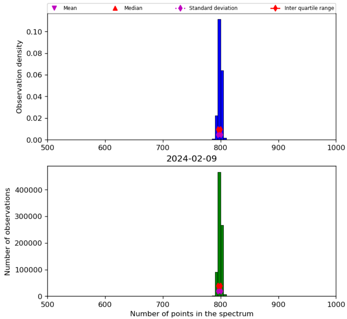
Figure 26: Histogram of “Number of points in the spectrum” for 2024-02-08 to 2024-02-10
