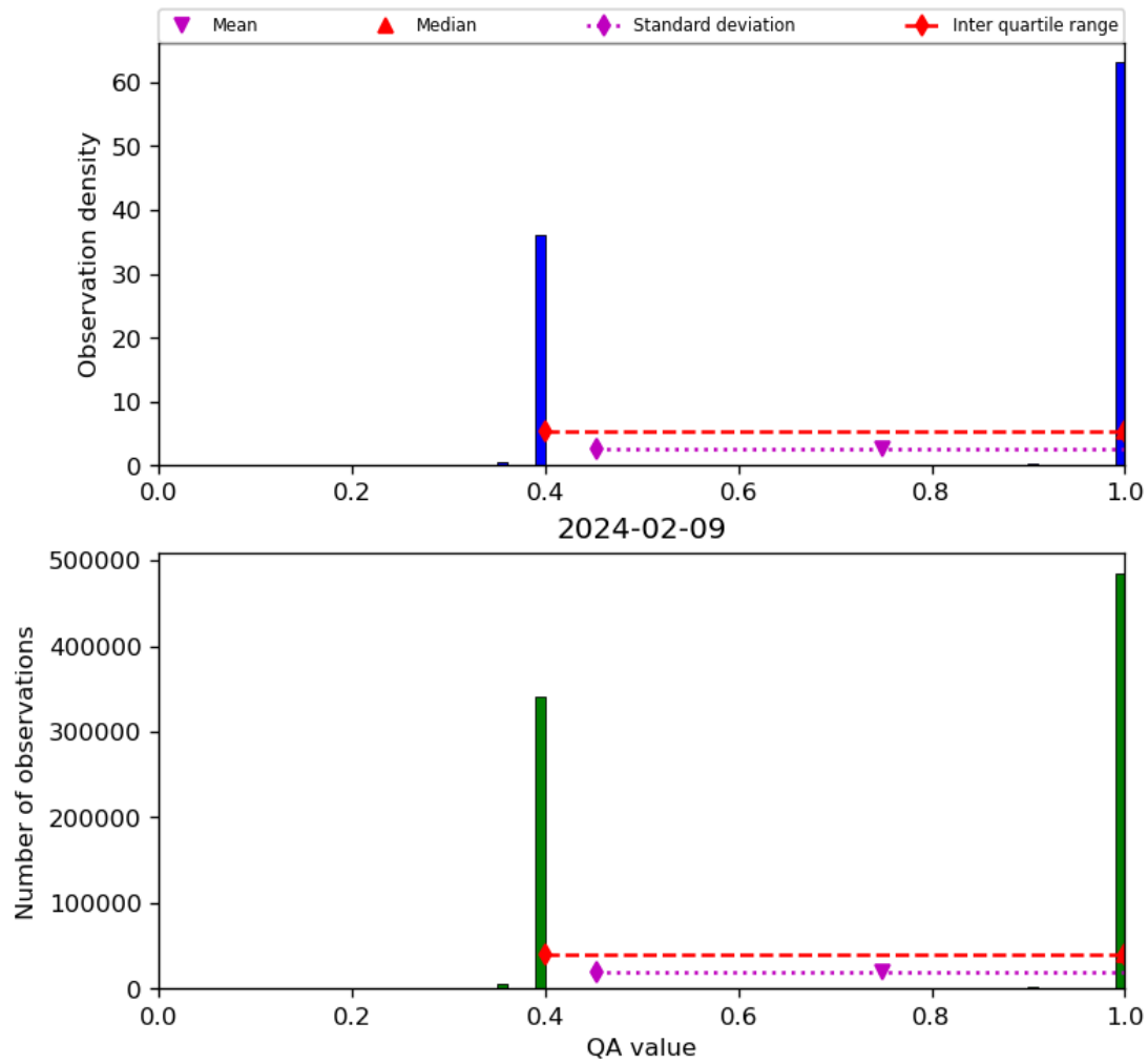
Figure 22: Histogram of “QA value” for 2024-02-08 to 2024-02-10
