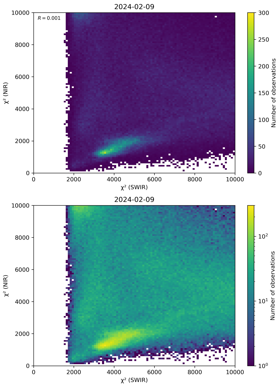
Figure 47: Scatter density plot of “ \chi^2 (SWIR)” against “ \chi^2 (NIR)” for 2024-02-08 to 2024-02-10.
