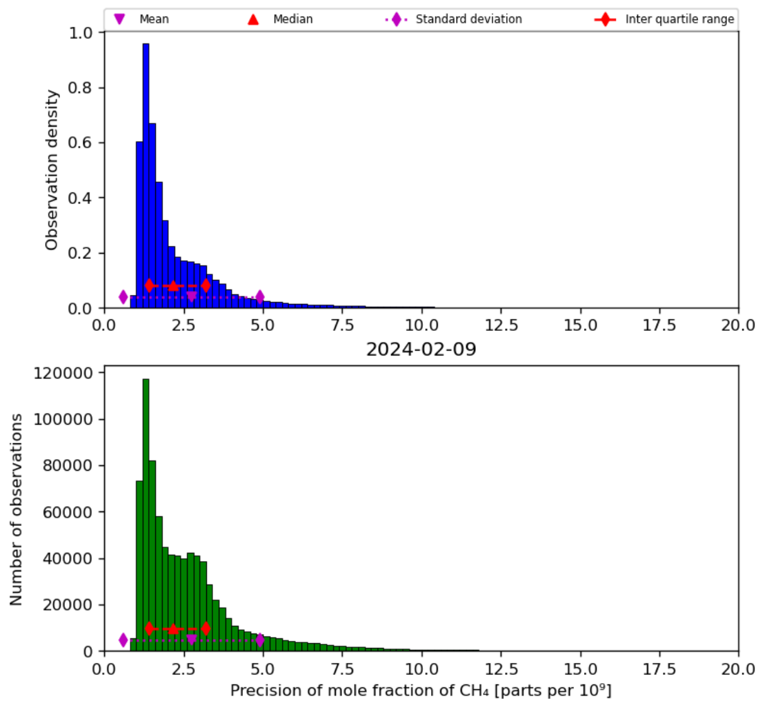
Figure 24: Histogram of “Precision of mole fraction of CH 4 ” for 2024-02-08 to 2024-02-10
