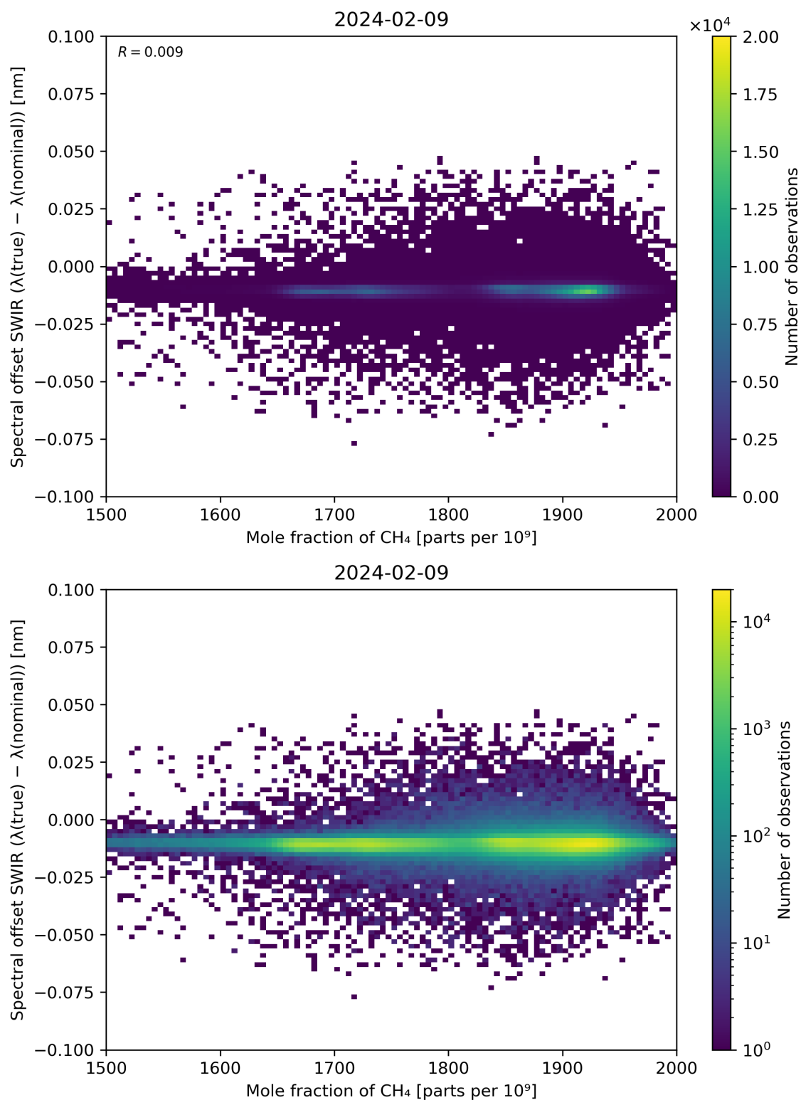
Figure 86: Scatter density plot of “Mole fraction of CH 4 ” against “Spectral offset SWIR ( \lambda(\text{true}) - \lambda(\text{nominal}) )” for 2024-02-08 to 2024-02-10.
