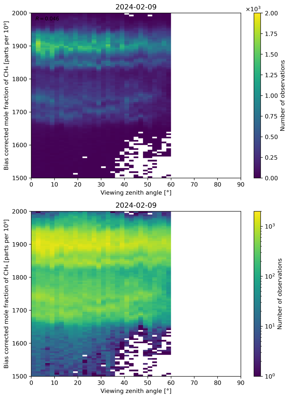
Figure 111: Scatter density plot of “Viewing zenith angle” against “Bias corrected mole fraction of CH 4 ” for 2024-02-08 to 2024-02-10.
