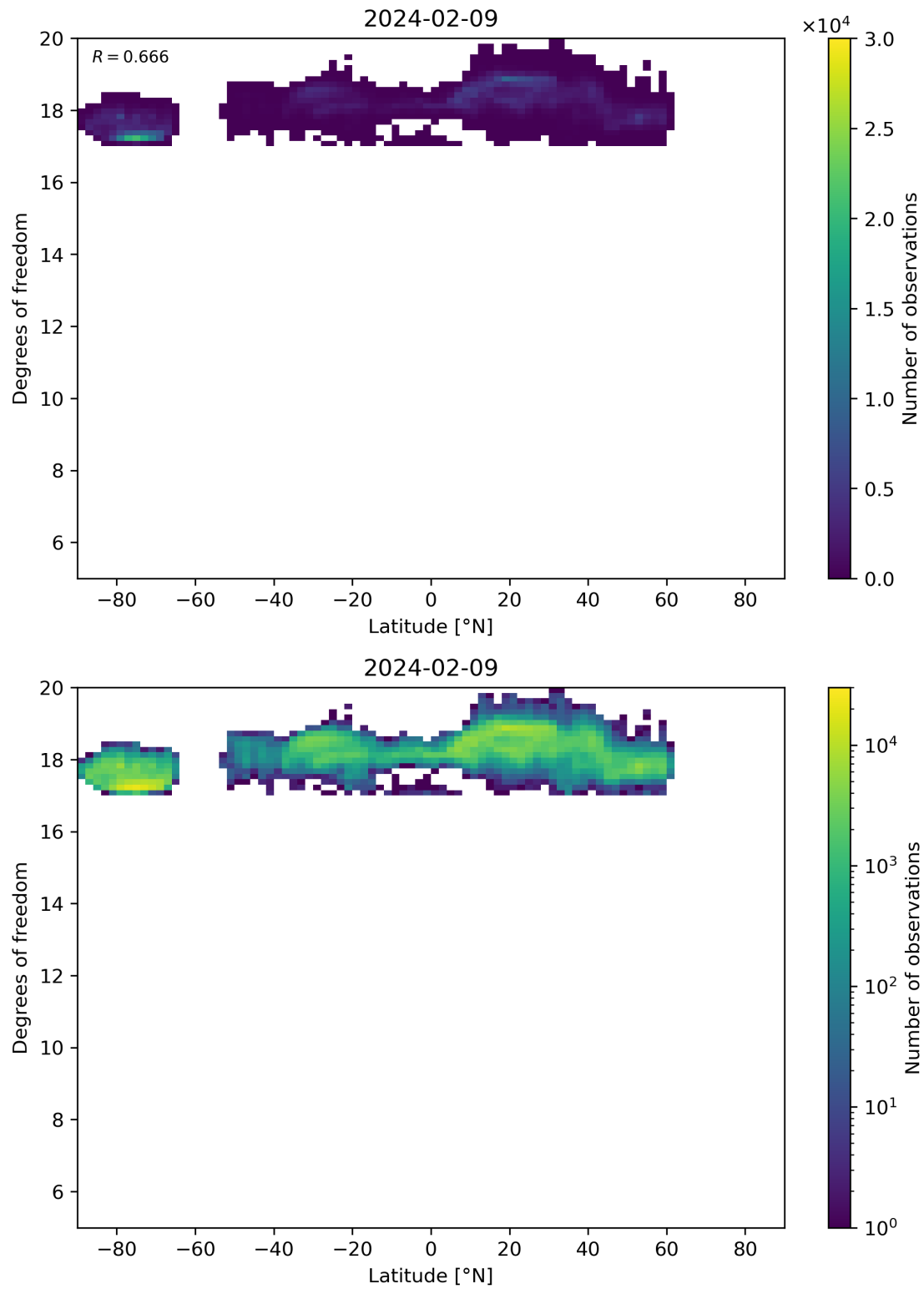
Figure 55: Scatter density plot of “Latitude” against “Degrees of freedom” for 2024-02-08 to 2024-02-10.
