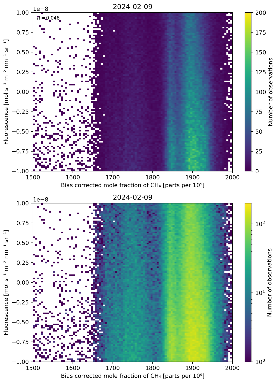
Figure 66: Scatter density plot of “Bias corrected mole fraction of \text{CH}_4 ” against “Fluorescence” for 2024-02-08 to 2024-02-10.
