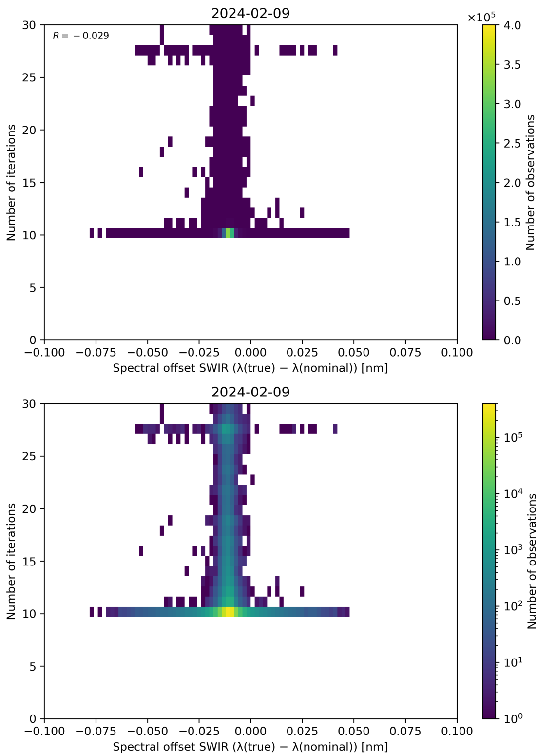
Figure 121: Scatter density plot of “Spectral offset SWIR ( \lambda(\text{true}) - \lambda(\text{nominal}) )” against “Number of iterations” for 2024-02-08 to 2024-02-10.
