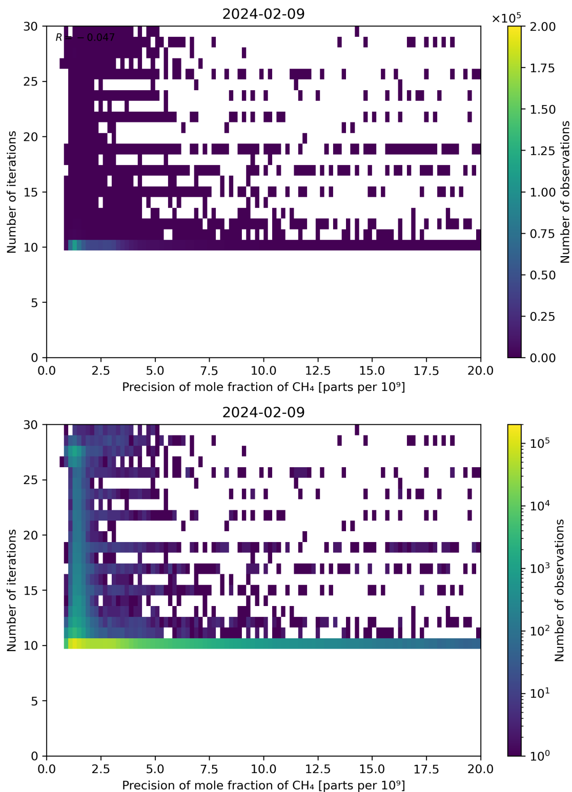
Figure 83: Scatter density plot of “Precision of mole fraction of CH 4 ” against “Number of iterations” for 2024-02-08 to 2024-02-10.
