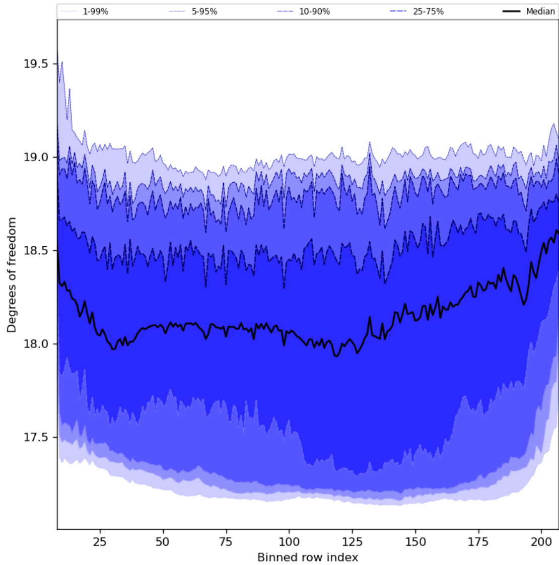
Figure 41: Along track statistics of “Degrees of freedom” for 2024-02-08 to 2024-02-10
