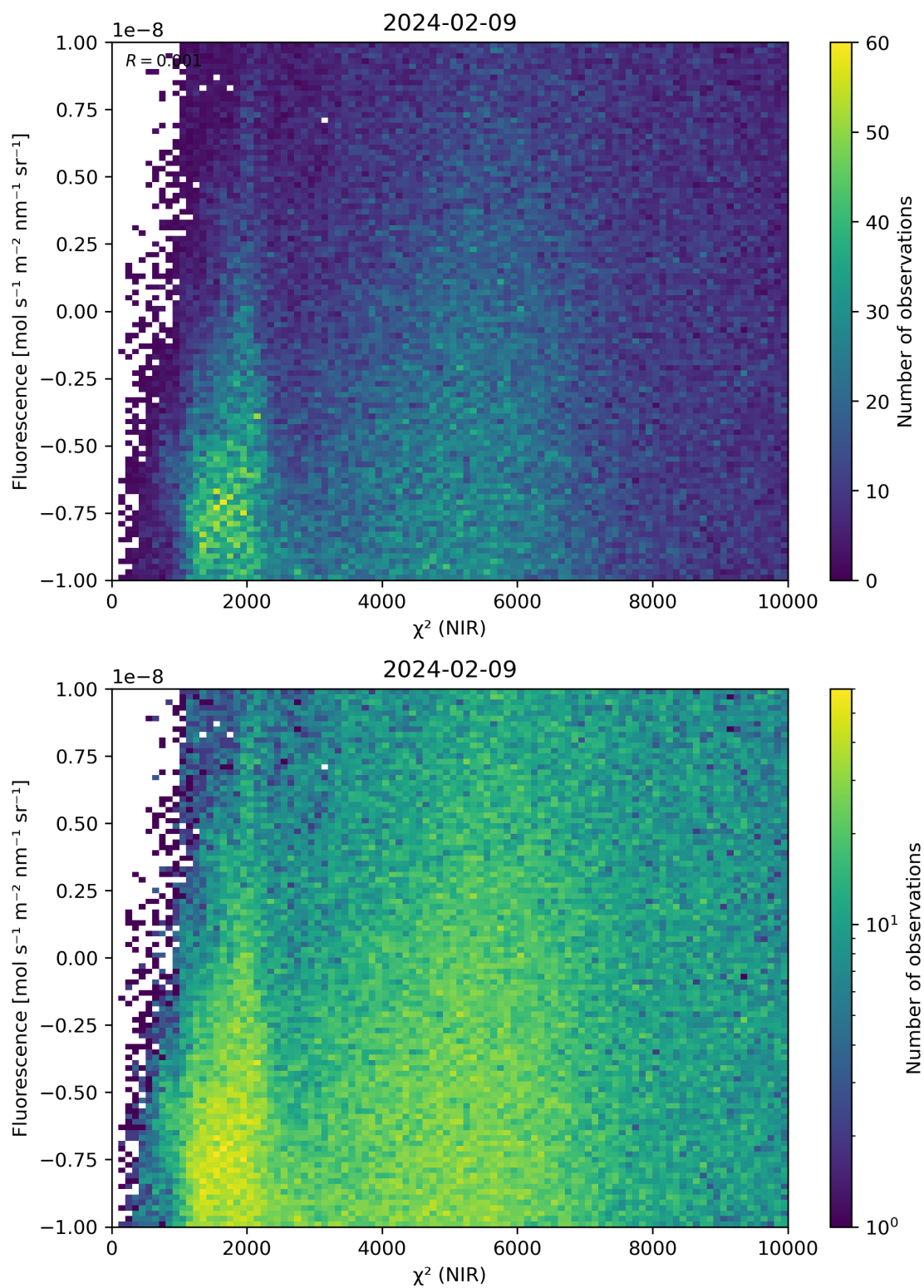
Figure 45: Scatter density plot of “ \chi^2 (NIR)” against “Fluorescence” for 2024-02-08 to 2024-02-10.
