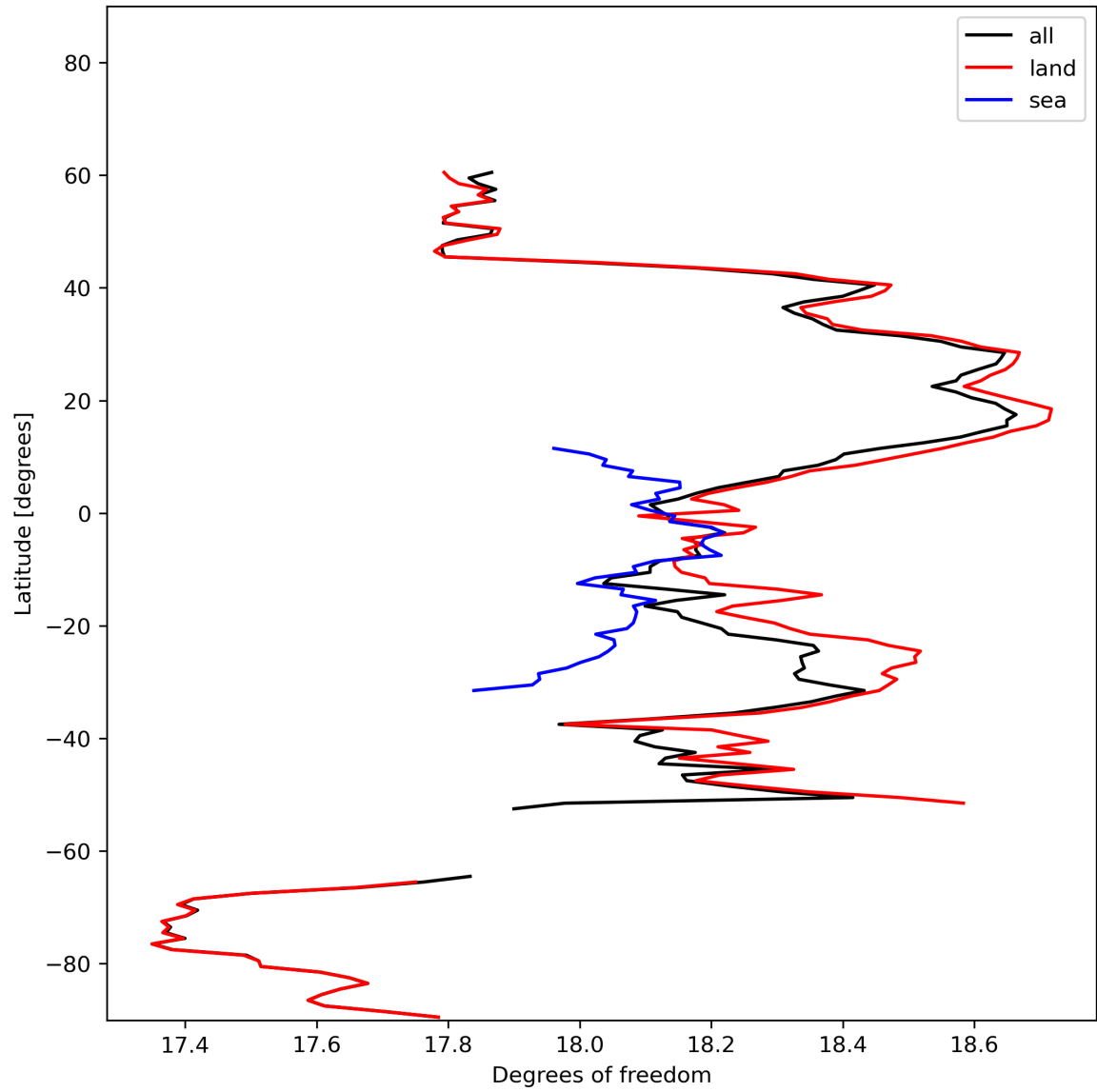
Figure 19: Zonal average of “Degrees of freedom” for 2024-02-08 to 2024-02-10.
