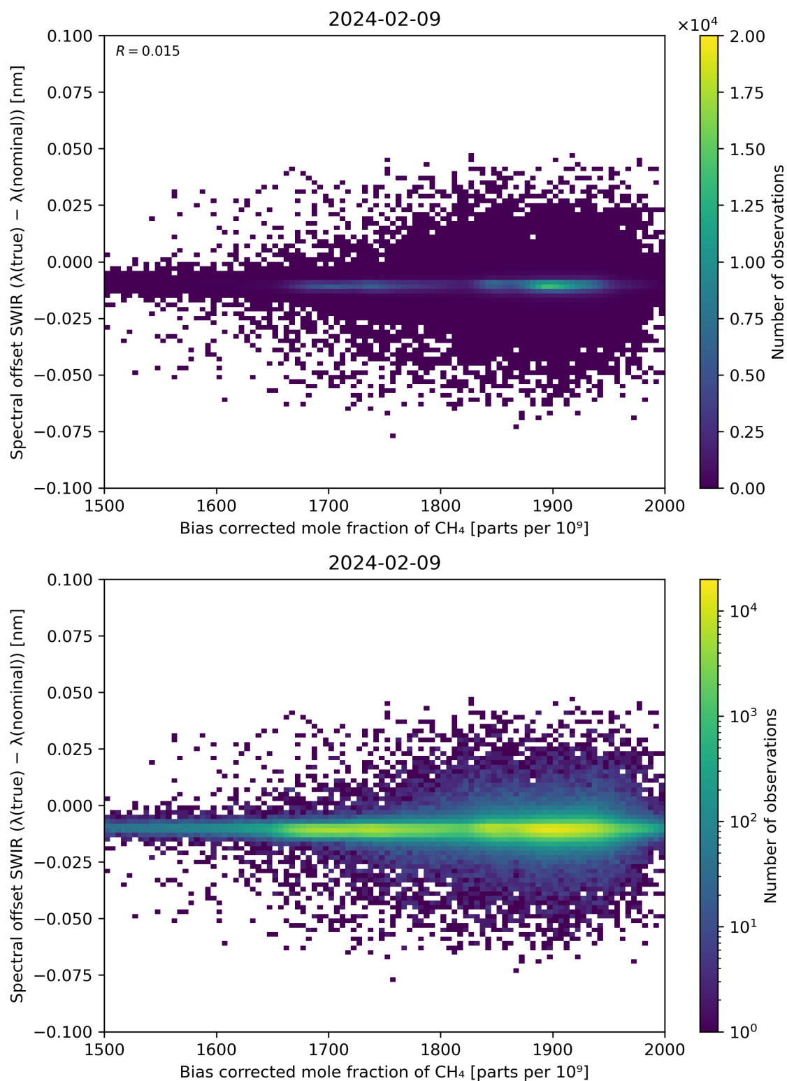
Figure 69: Scatter density plot of “Bias corrected mole fraction of \text{CH}_4 ” against “Spectral offset SWIR ( \lambda(\text{true}) - \lambda(\text{nominal}) )” for 2024-02-08 to 2024-02-10.
