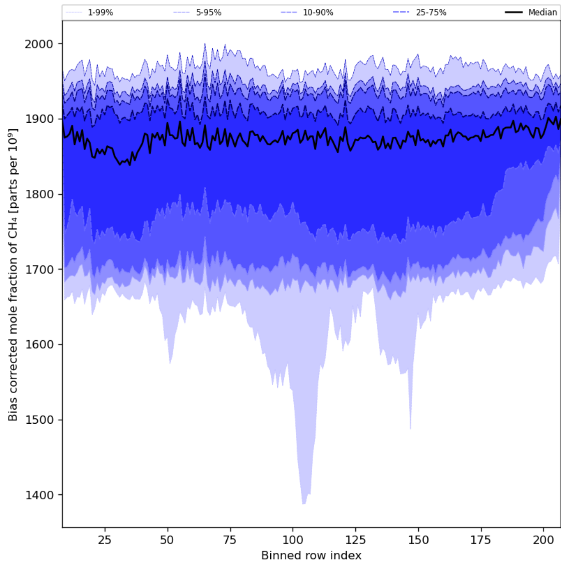
Figure 36: Along track statistics of “Bias corrected mole fraction of CH 4 ” for 2024-02-08 to 2024-02-10
