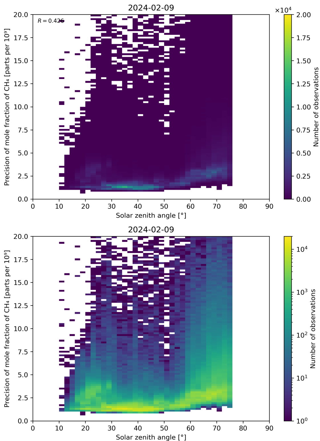
Figure 101: Scatter density plot of “Solar zenith angle” against “Precision of mole fraction of CH 4 ” for 2024-02-08 to 2024-02-10.
