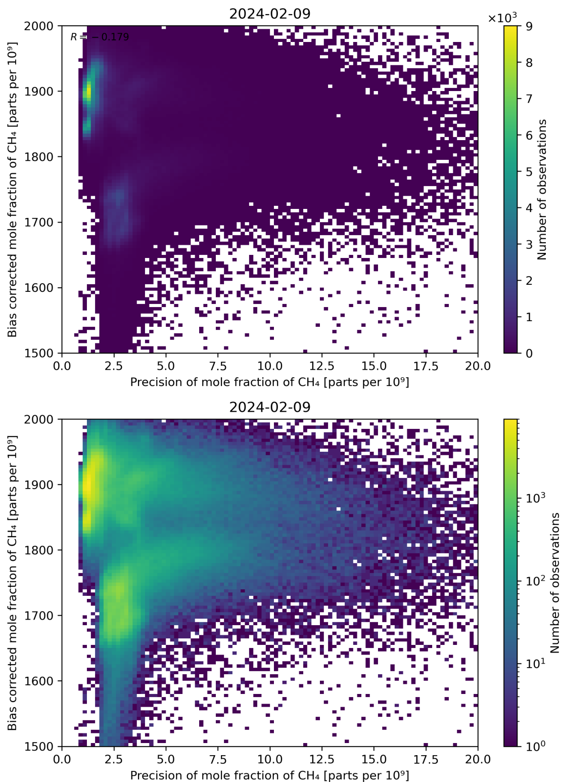
Figure 82: Scatter density plot of “Precision of mole fraction of CH 4 ” against “Bias corrected mole fraction of CH 4 ” for 2024-02-08 to 2024-02-10.
