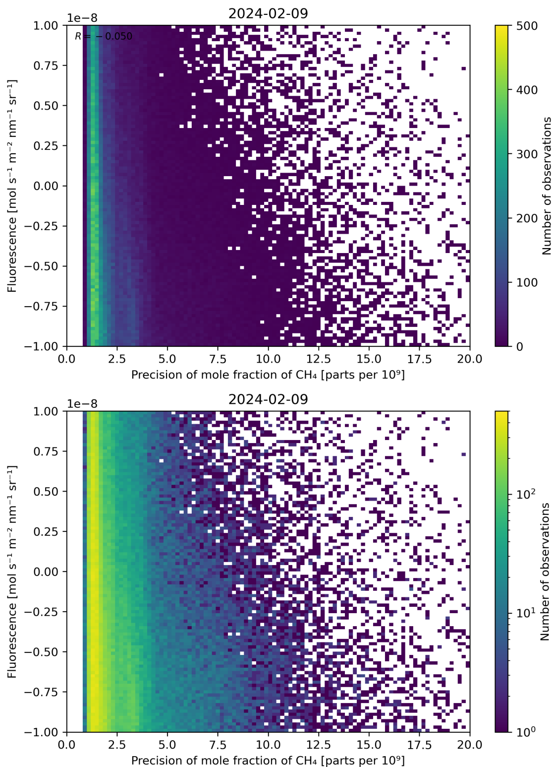
Figure 81: Scatter density plot of “Precision of mole fraction of \text{CH}_4 ” against “Fluorescence” for 2024-02-08 to 2024-02-10.
