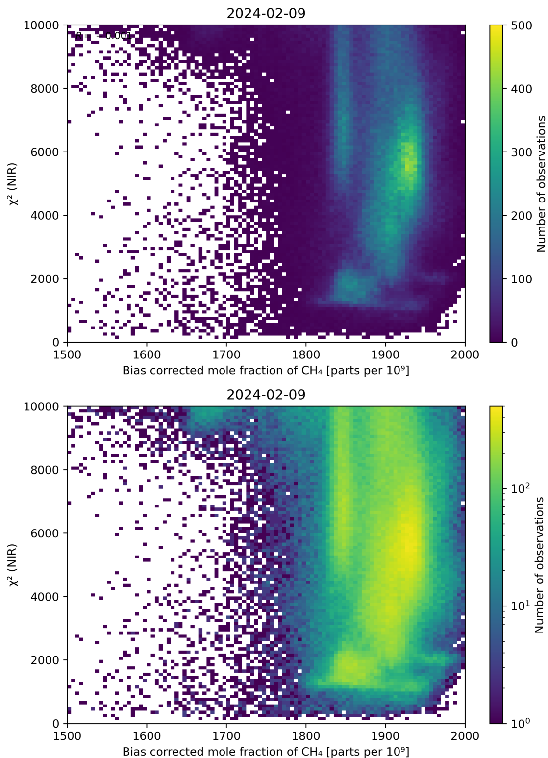
Figure 63: Scatter density plot of “Bias corrected mole fraction of CH 4 ” against “ \chi^2 (NIR)” for 2024-02-08 to 2024-02-10.
