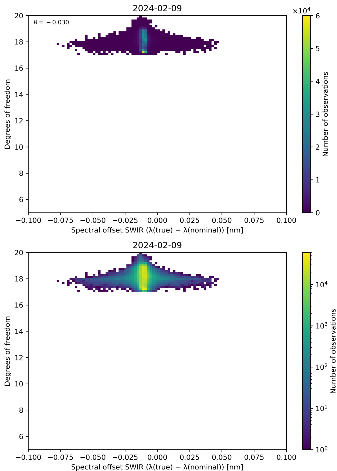
Figure 119: Scatter density plot of “Spectral offset SWIR ( \lambda(\text{true}) - \lambda(\text{nominal}) )” against “Degrees of freedom” for 2024-02-08 to 2024-02-10.
