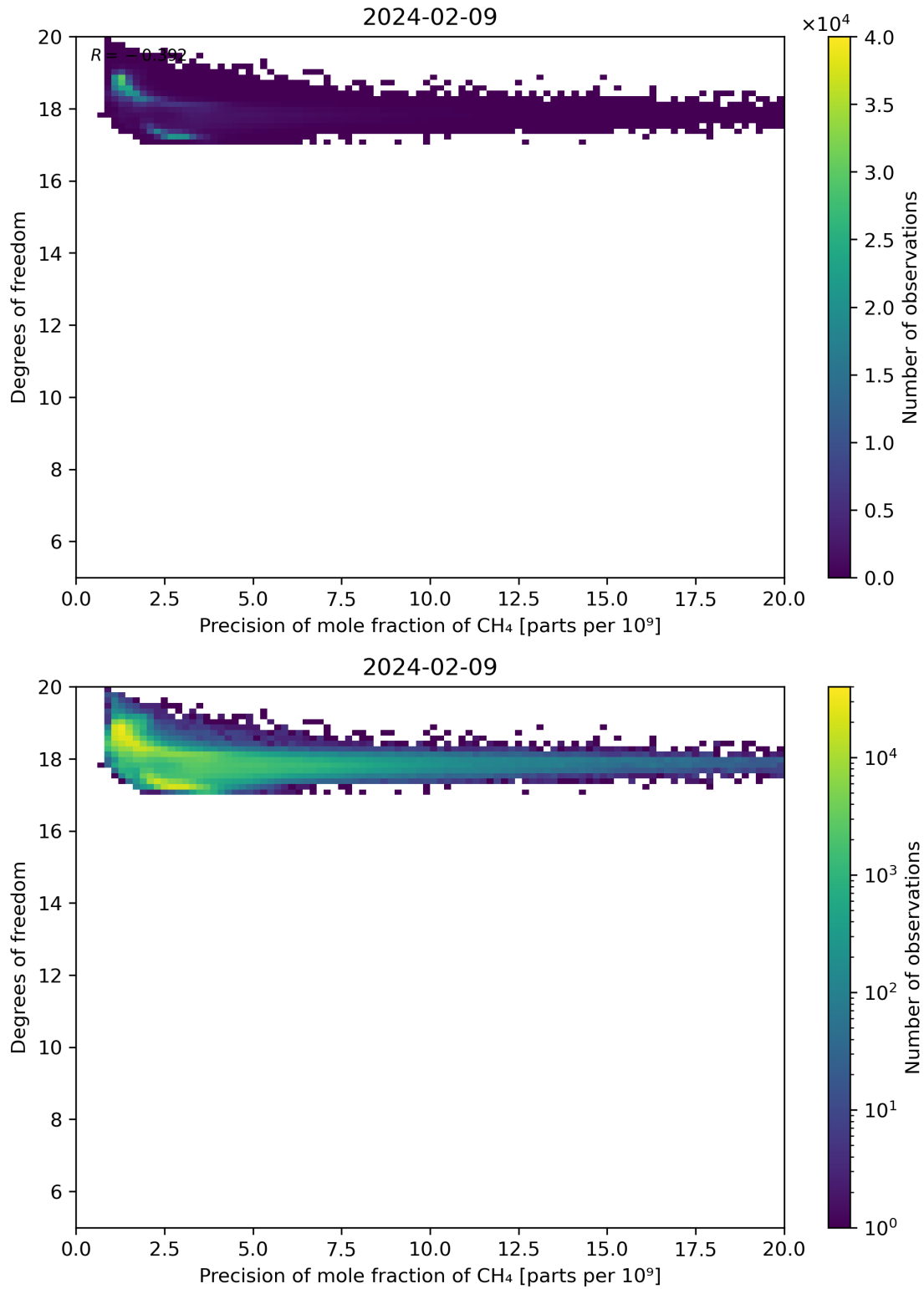
Figure 80: Scatter density plot of “Precision of mole fraction of CH 4 ” against “Degrees of freedom” for 2024-02-08 to 2024-02-10.
