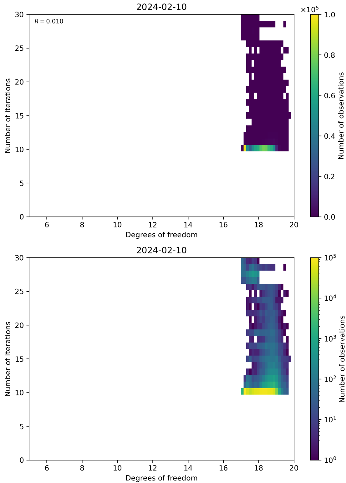
Figure 52: Scatter density plot of “Degrees of freedom” against “Number of iterations” for 2024-02-09 to 2024-02-11.
