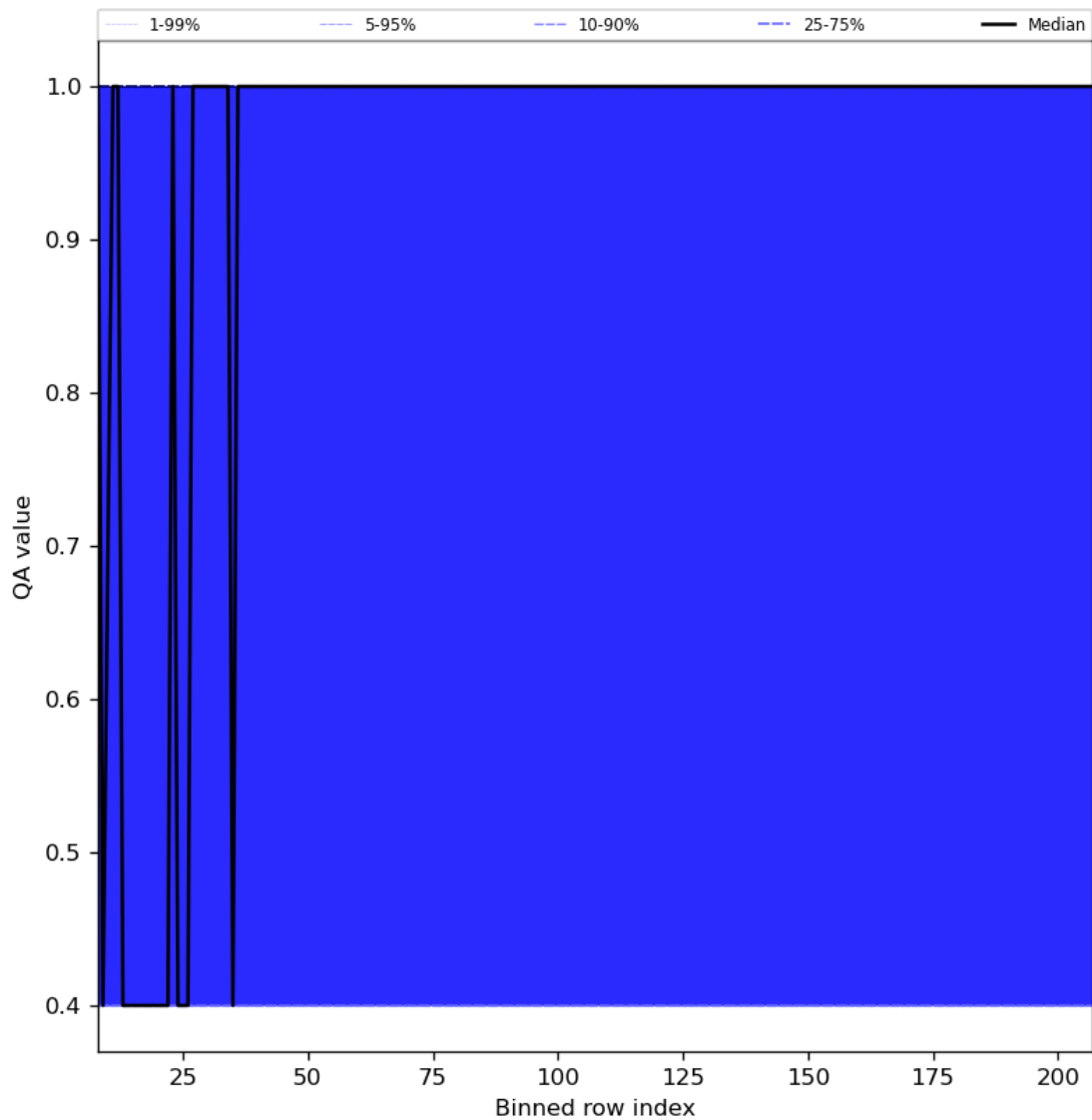
Figure 33: Along track statistics of “QA value” for 2024-02-09 to 2024-02-11
