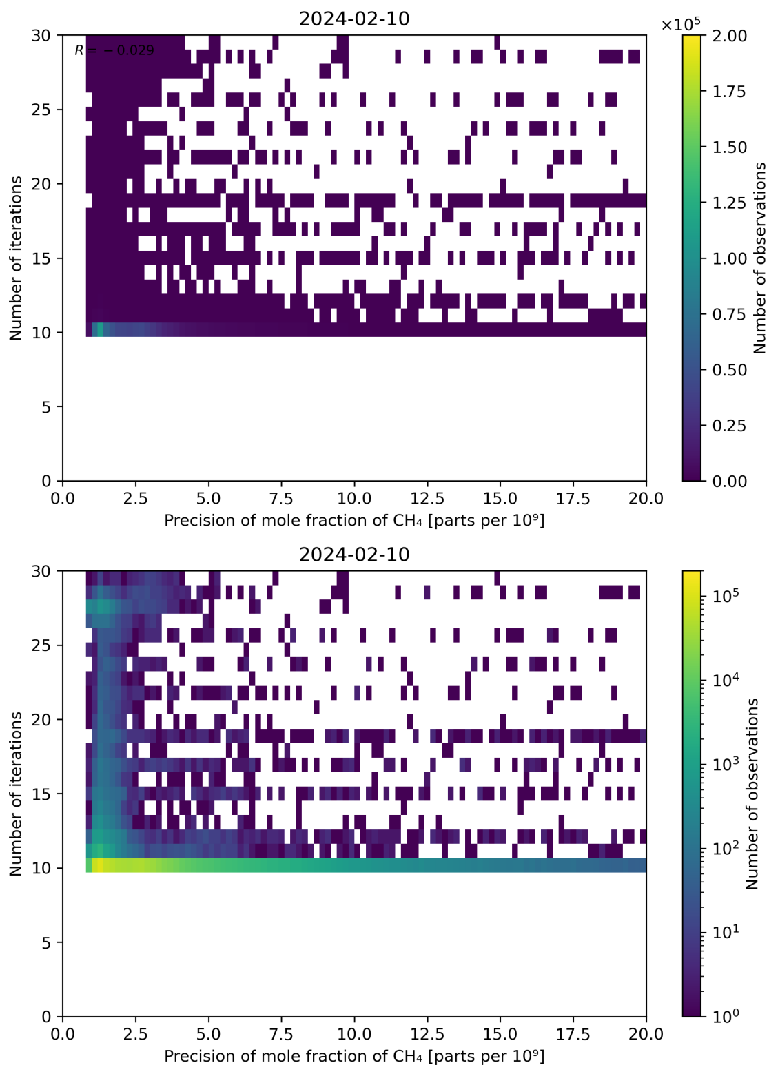
Figure 83: Scatter density plot of “Precision of mole fraction of CH 4 ” against “Number of iterations” for 2024-02-09 to 2024-02-11.
