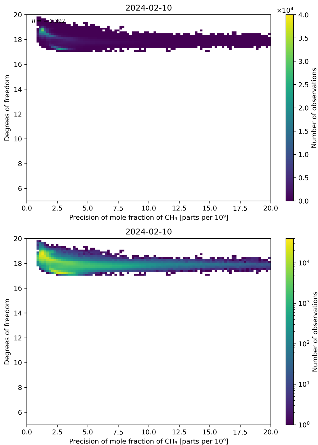
Figure 80: Scatter density plot of “Precision of mole fraction of CH 4 ” against “Degrees of freedom” for 2024-02-09 to 2024-02-11.
