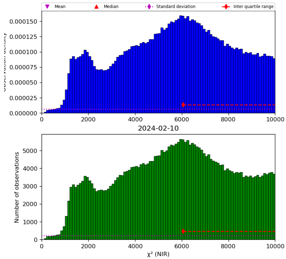
Figure 29: Histogram of “ \chi^2 (NIR)” for 2024-02-09 to 2024-02-11
