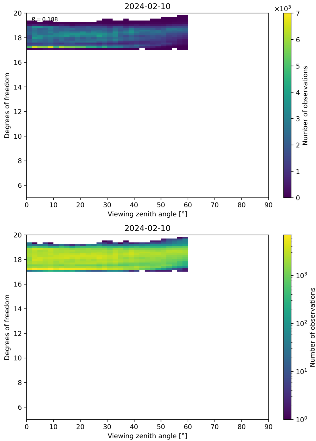
Figure 107: Scatter density plot of “Viewing zenith angle” against “Degrees of freedom” for 2024-02-09 to 2024-02-11.
