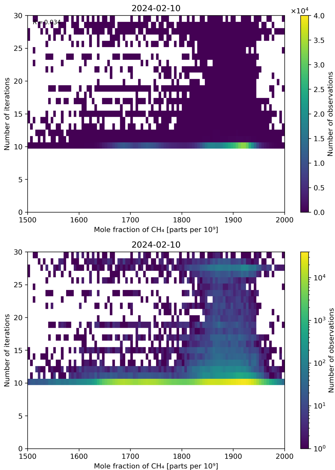
Figure 76: Scatter density plot of “Mole fraction of CH 4 ” against “Number of iterations” for 2024-02-09 to 2024-02-11.
