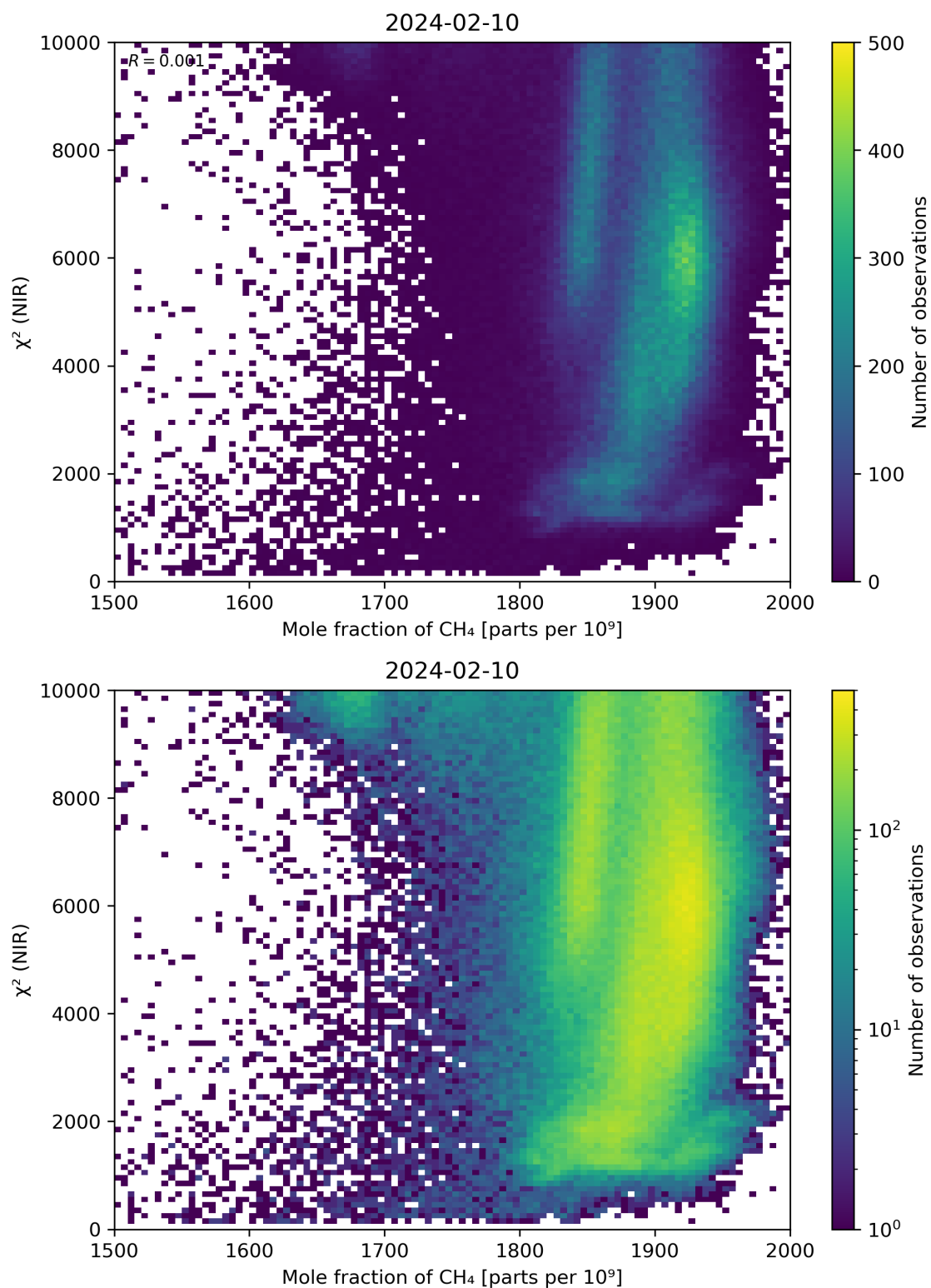
Figure 70: Scatter density plot of “Mole fraction of CH 4 ” against “ \chi^2 (NIR)” for 2024-02-09 to 2024-02-11.
