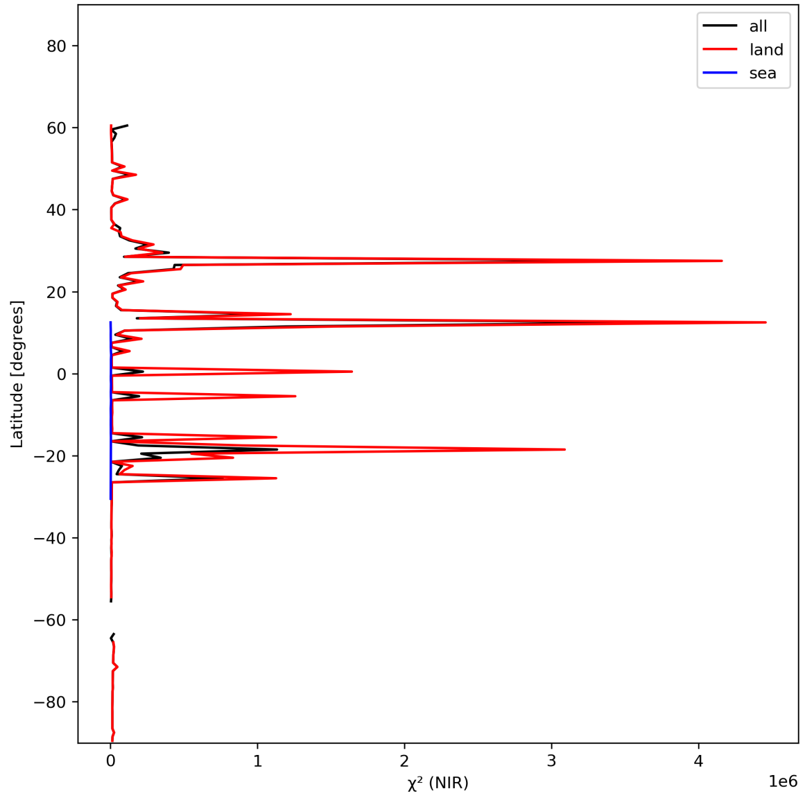
Figure 18: Zonal average of “ \chi^2 (NIR)” for 2024-02-09 to 2024-02-11.
