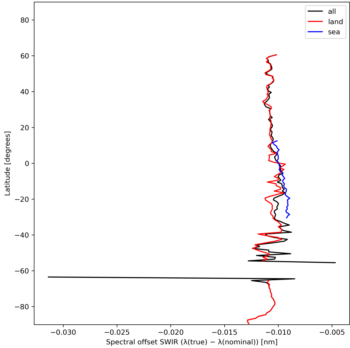
Figure 16: Zonal average of “Spectral offset SWIR ( \lambda(\text{true}) - \lambda(\text{nominal}) )” for 2024-02-09 to 2024-02-11.
