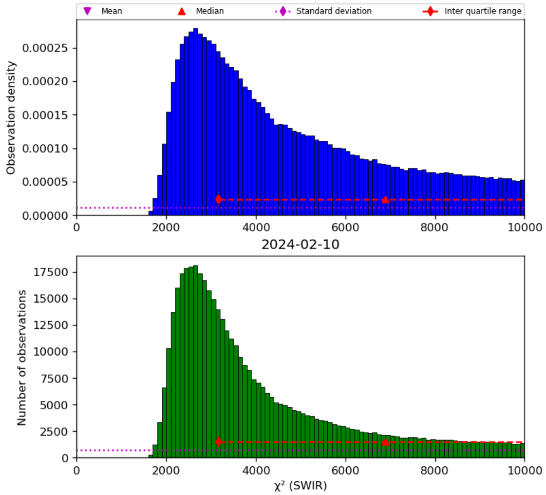
Figure 28: Histogram of “ \chi^2 (SWIR)” for 2024-02-09 to 2024-02-11
