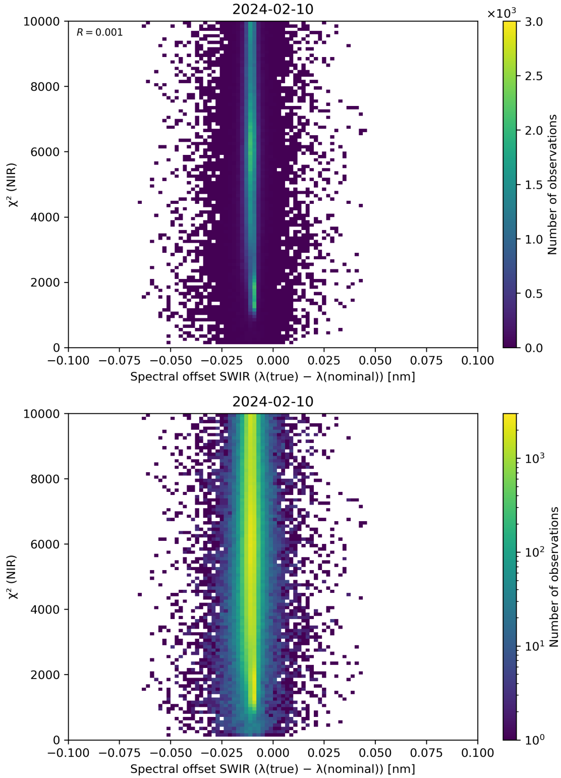
Figure 117: Scatter density plot of “Spectral offset SWIR ( \lambda(\text{true}) - \lambda(\text{nominal}) )” against “ \chi^2 (NIR)” for 2024-02-09 to 2024-02-11.
