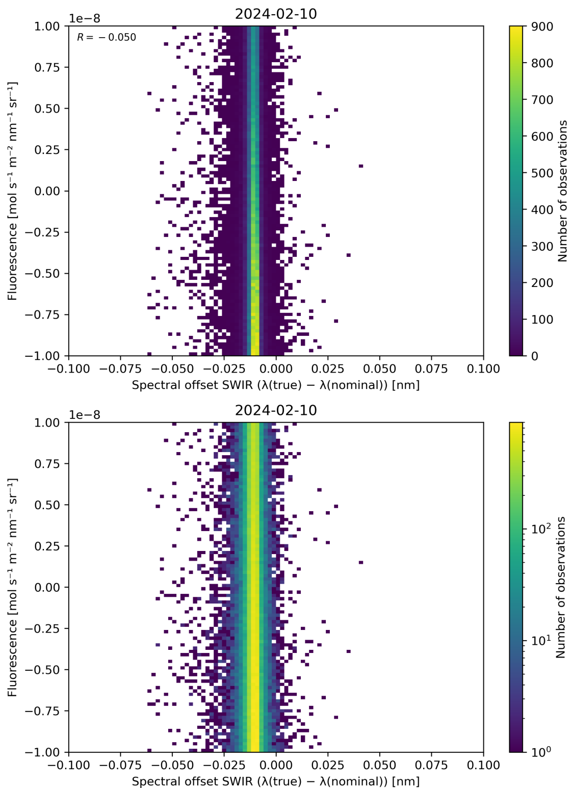
Figure 120: Scatter density plot of “Spectral offset SWIR ( \lambda(\text{true}) - \lambda(\text{nominal}) )” against “Fluorescence” for 2024-02-09 to 2024-02-11.
