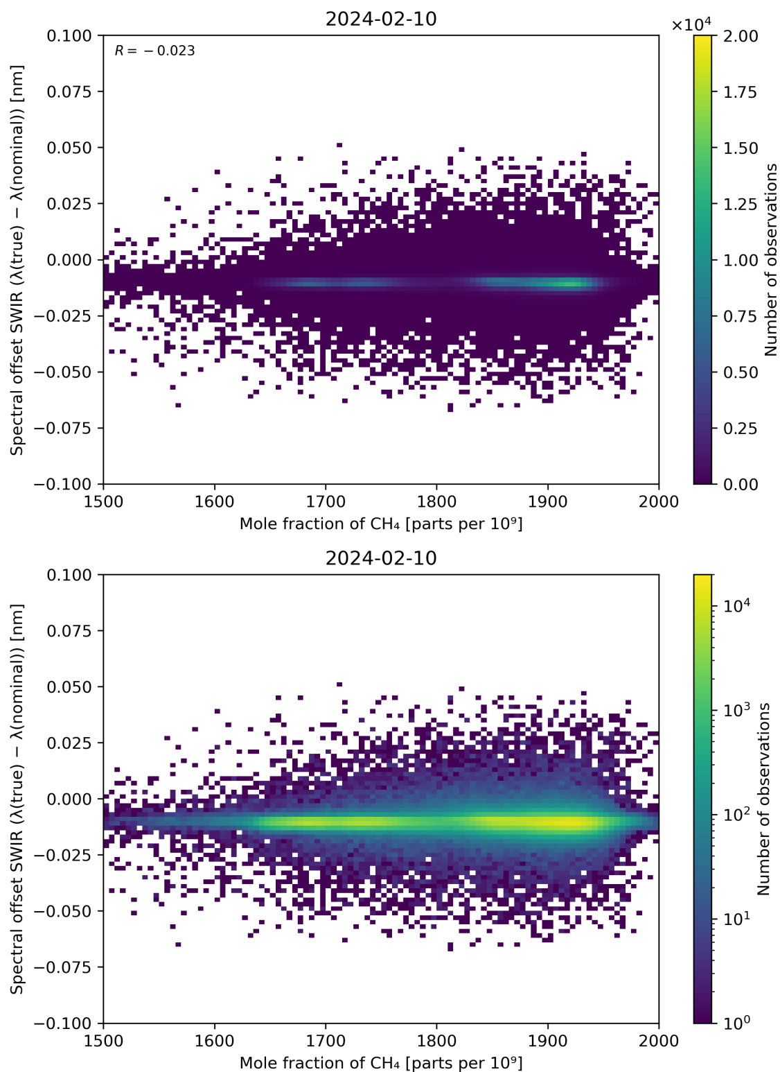
Figure 86: Scatter density plot of “Mole fraction of CH 4 ” against “Spectral offset SWIR ( \lambda(\text{true}) - \lambda(\text{nominal}) )” for 2024-02-09 to 2024-02-11.
