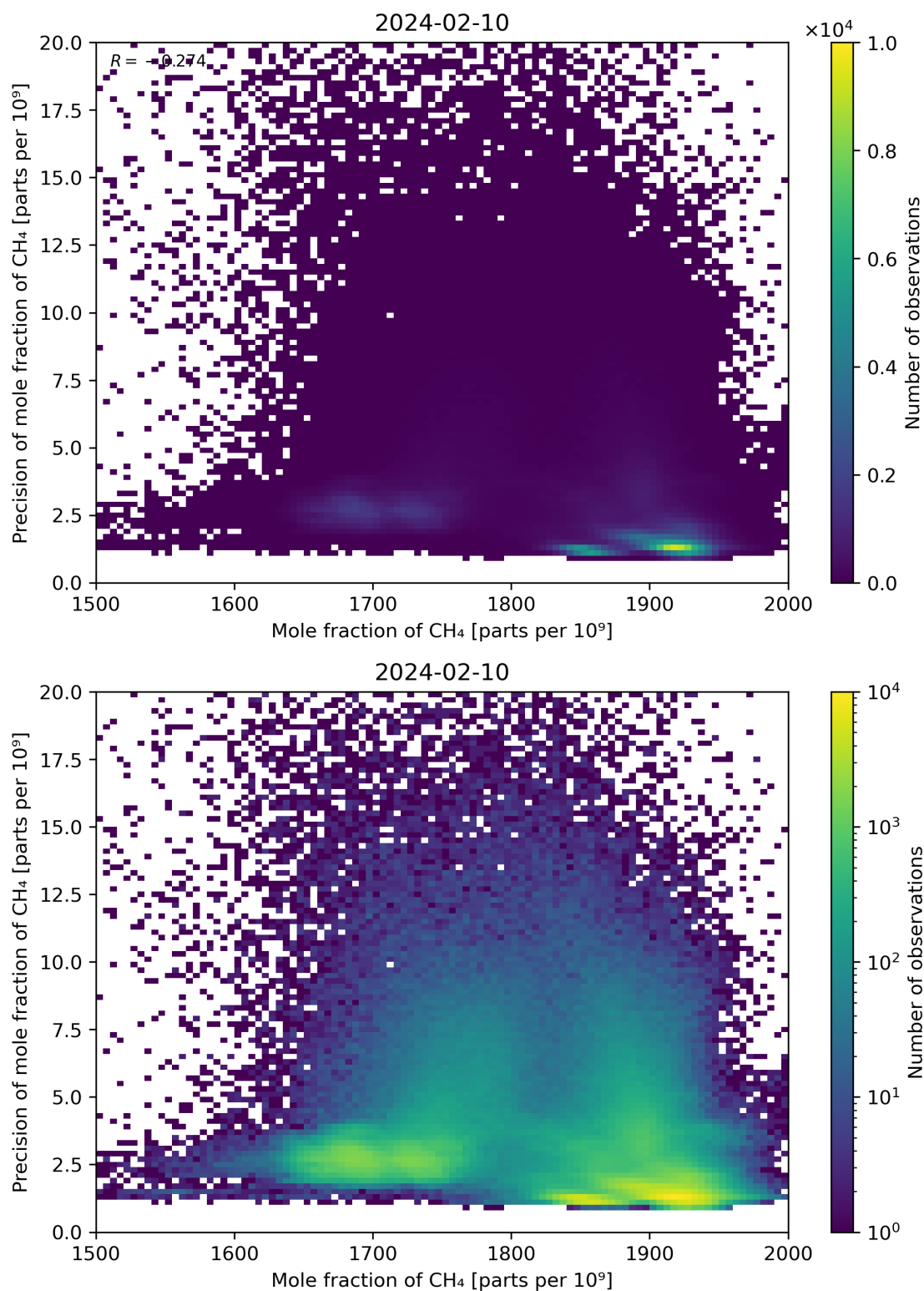
Figure 75: Scatter density plot of “Mole fraction of CH 4 ” against “Precision of mole fraction of CH 4 ” for 2024-02-09 to 2024-02-11.
