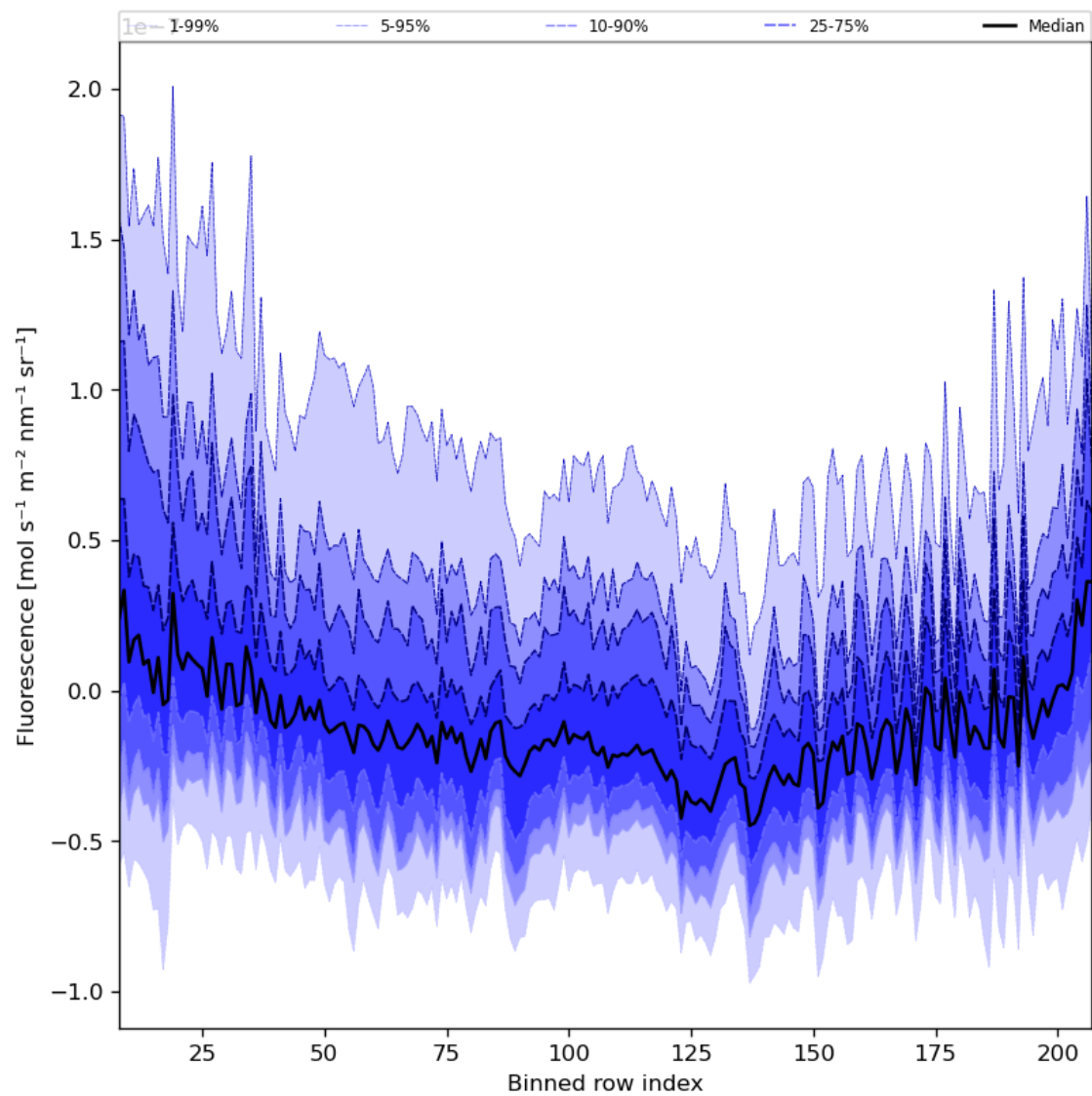
Figure 43: Along track statistics of “Fluorescence” for 2024-02-09 to 2024-02-11
