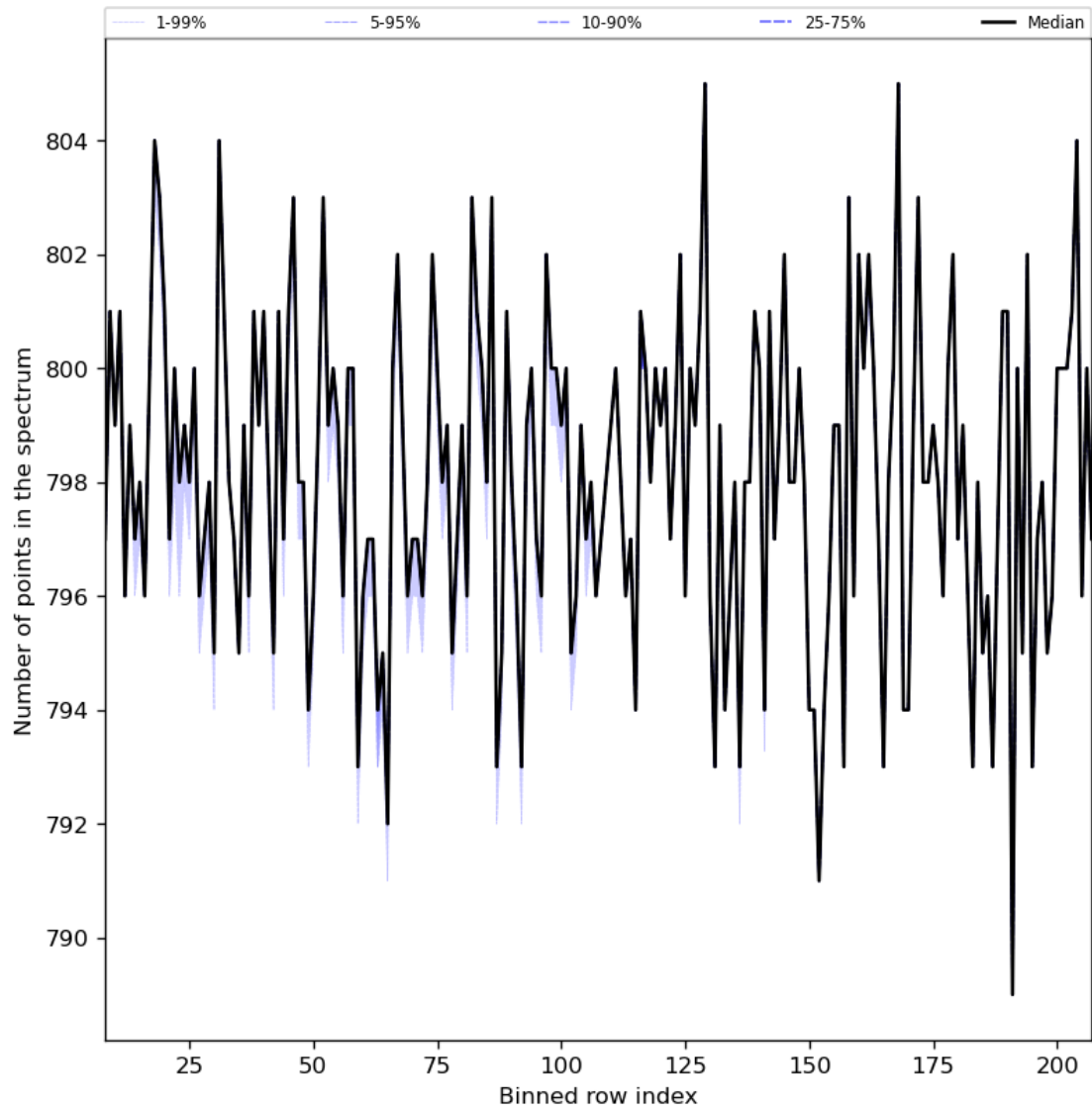
Figure 37: Along track statistics of “Number of points in the spectrum” for 2024-02-09 to 2024-02-11
