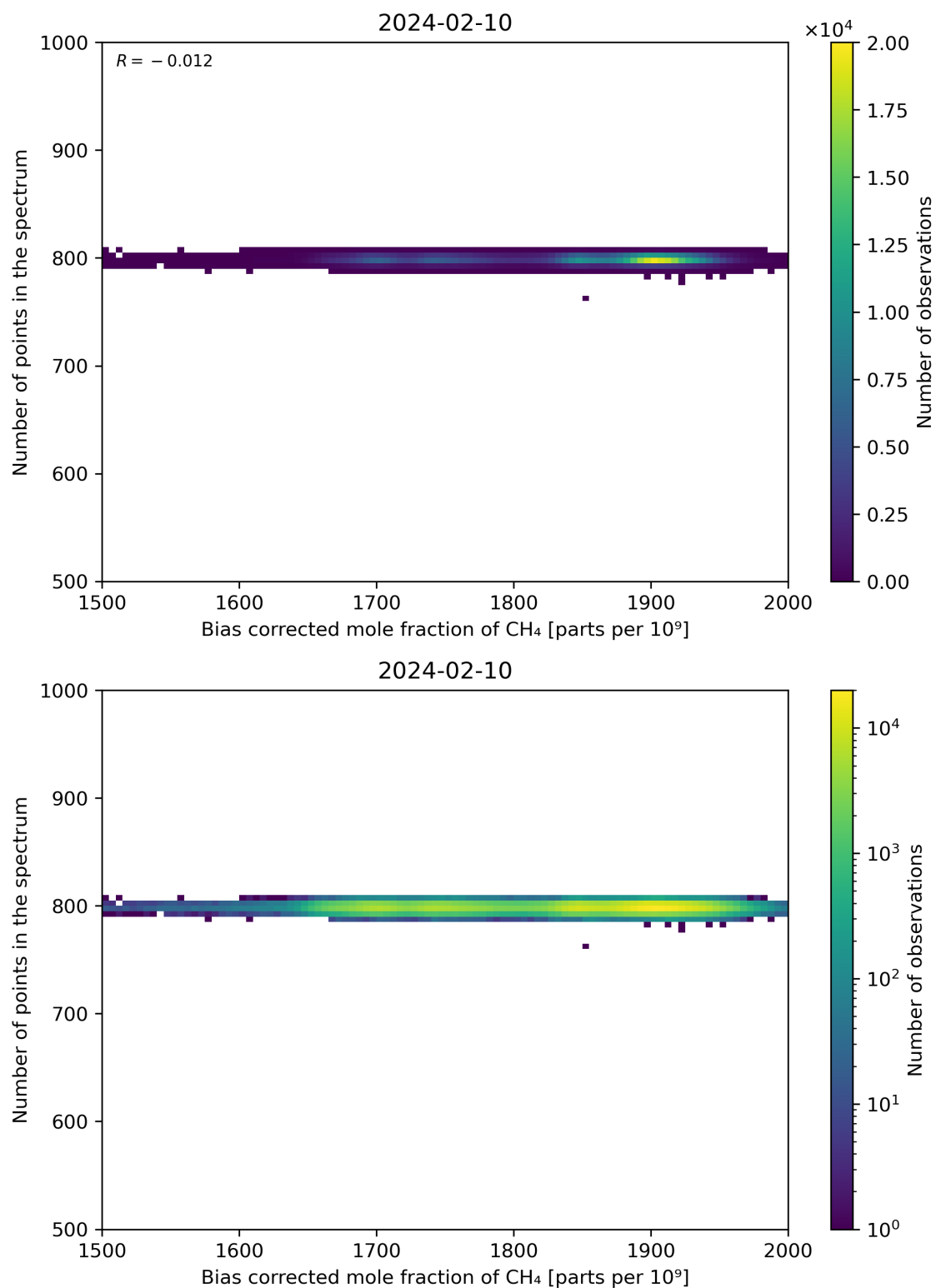
Figure 68: Scatter density plot of “Bias corrected mole fraction of CH 4 ” against “Number of points in the spectrum” for 2024-02-09 to 2024-02-11.
