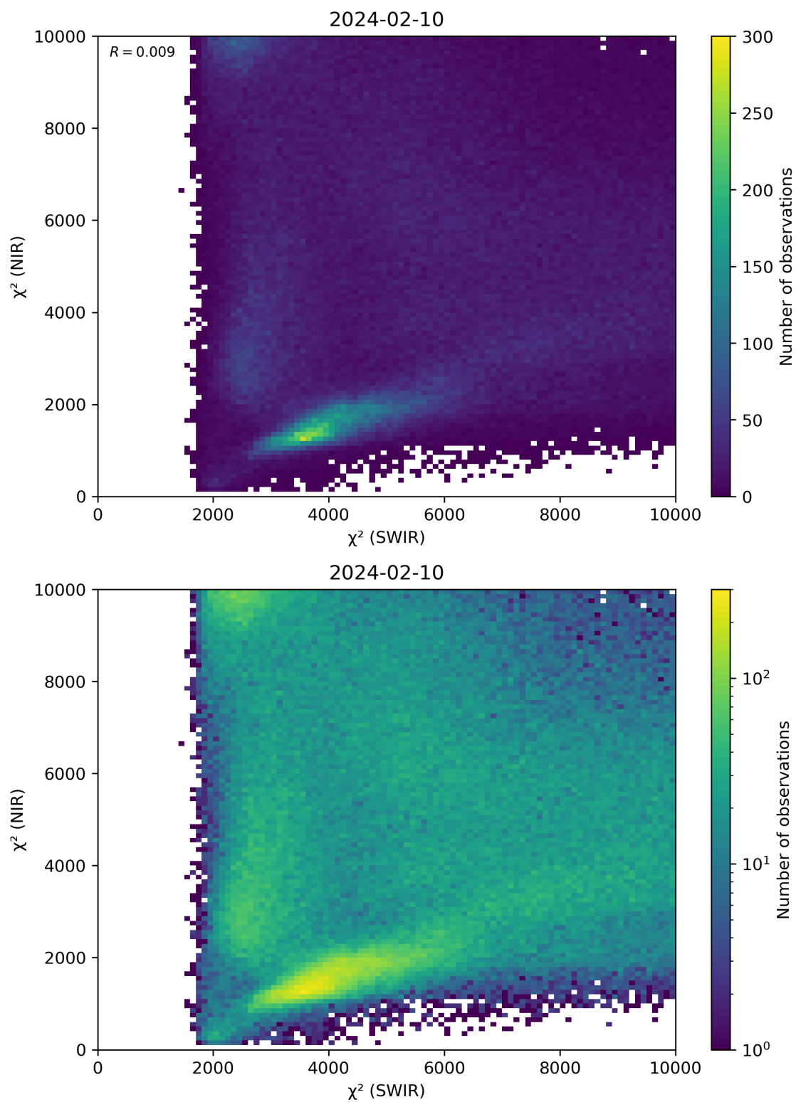
Figure 47: Scatter density plot of “ \chi^2 (SWIR)” against “ \chi^2 (NIR)” for 2024-02-09 to 2024-02-11.
