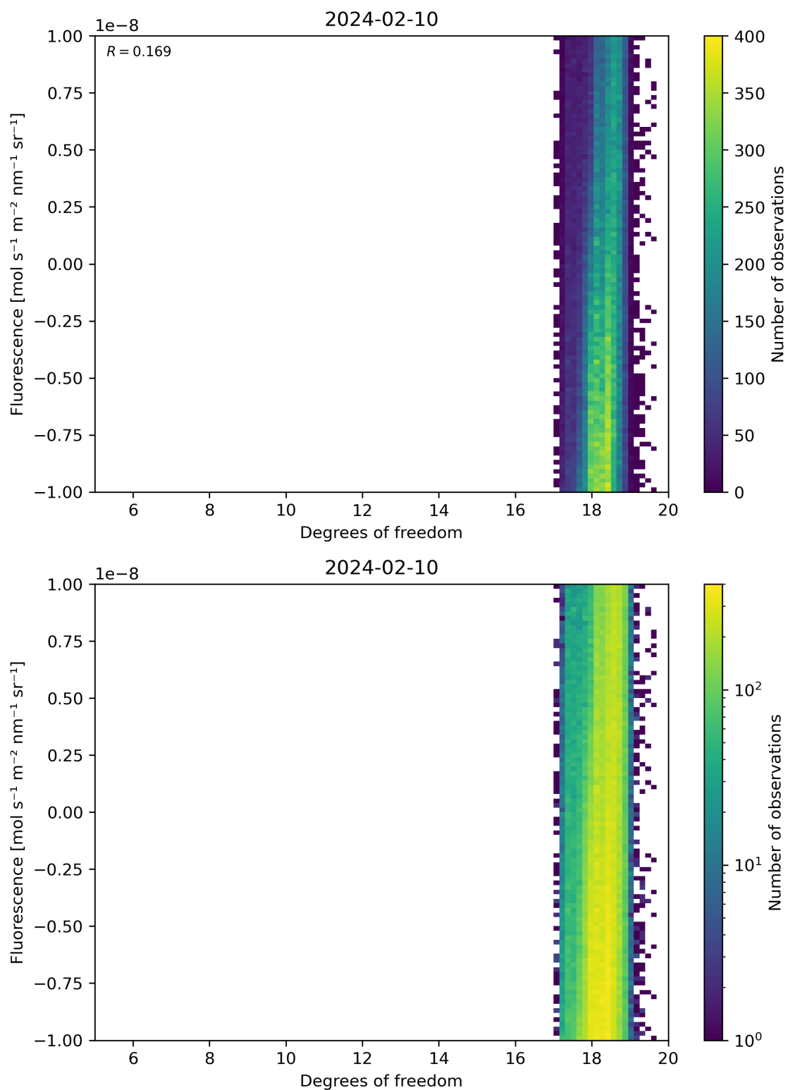
Figure 51: Scatter density plot of “Degrees of freedom” against “Fluorescence” for 2024-02-09 to 2024-02-11.
