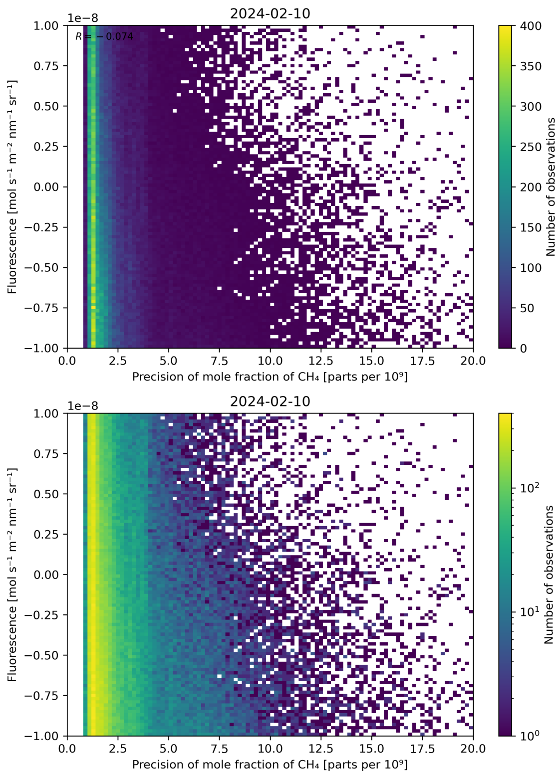
Figure 81: Scatter density plot of “Precision of mole fraction of \text{CH}_4 ” against “Fluorescence” for 2024-02-09 to 2024-02-11.
