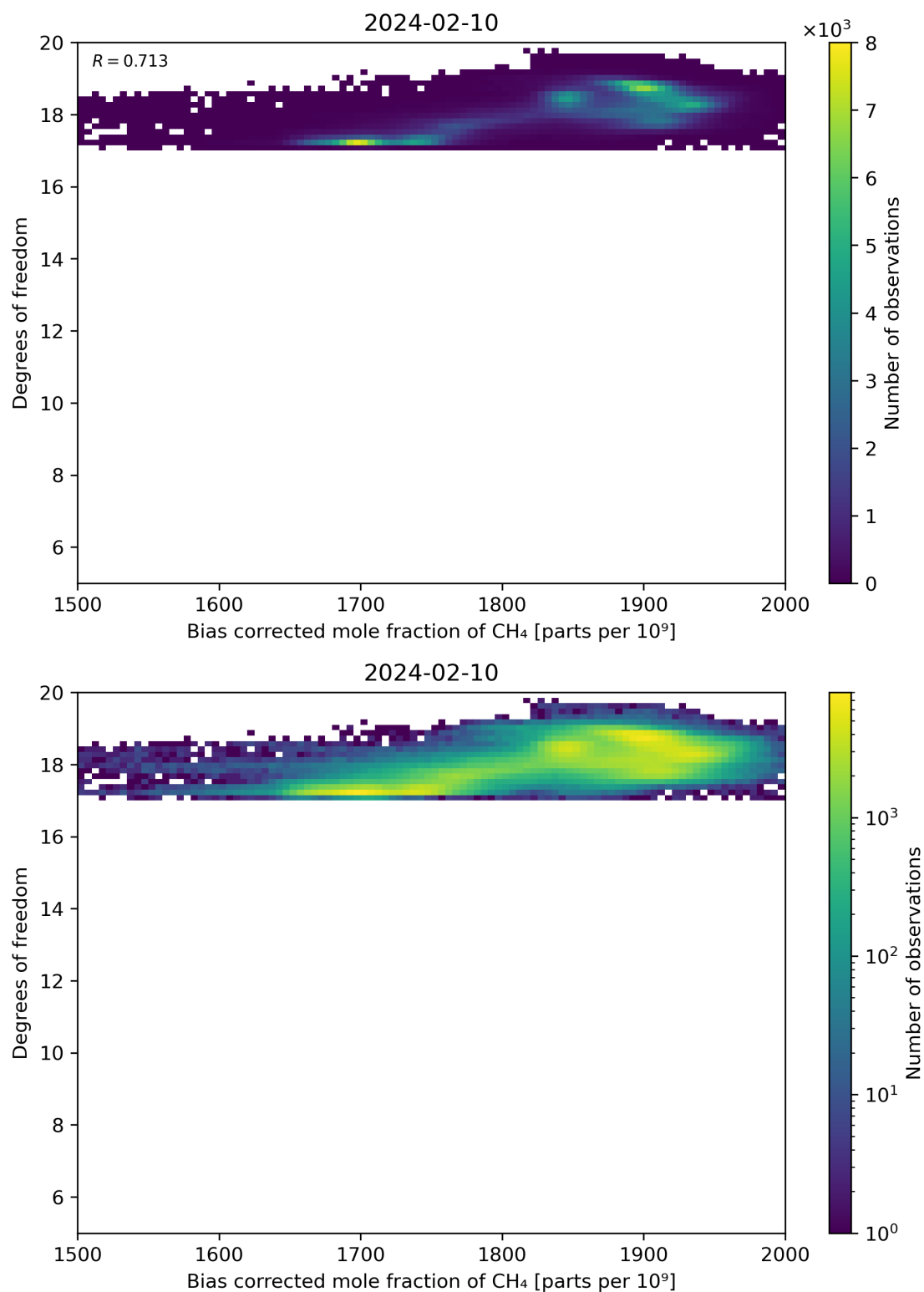
Figure 65: Scatter density plot of “Bias corrected mole fraction of CH 4 ” against “Degrees of freedom” for 2024-02-09 to 2024-02-11.
