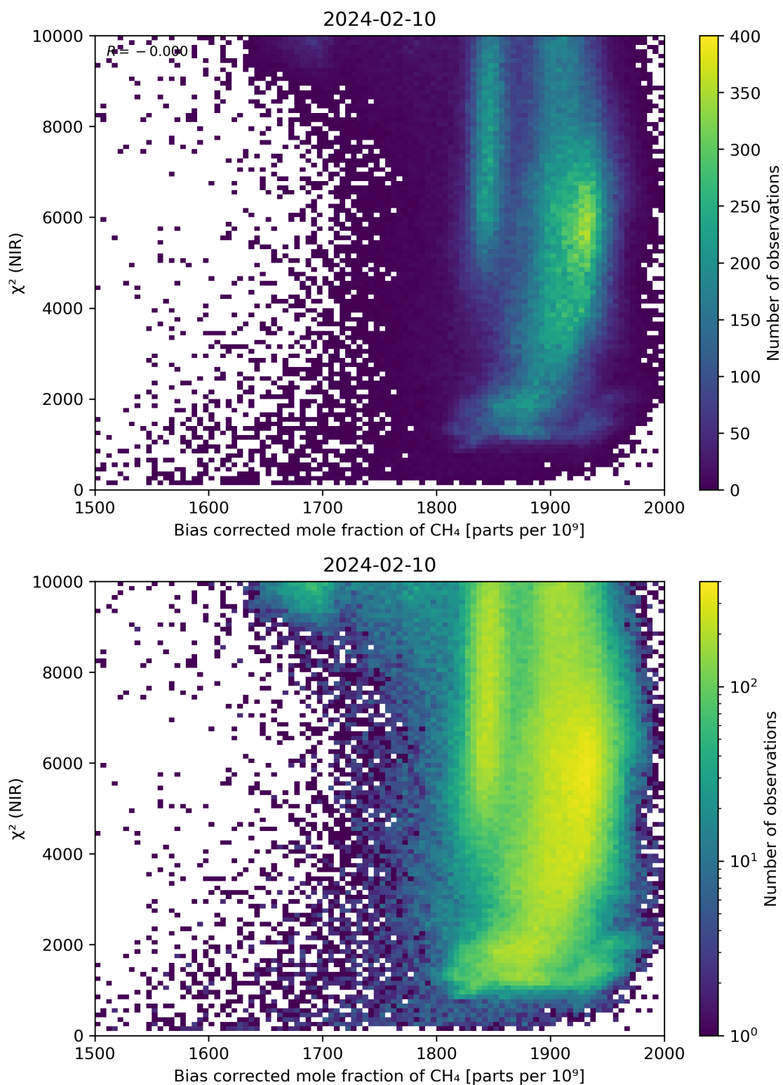
Figure 63: Scatter density plot of “Bias corrected mole fraction of CH 4 ” against “ \chi^2 (NIR)” for 2024-02-09 to 2024-02-11.
