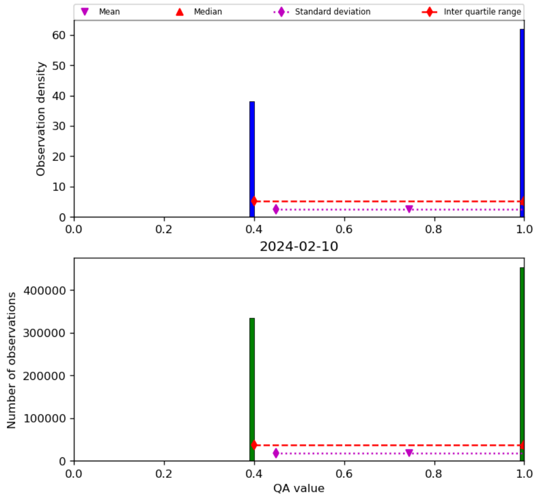
Figure 22: Histogram of “QA value” for 2024-02-09 to 2024-02-11
