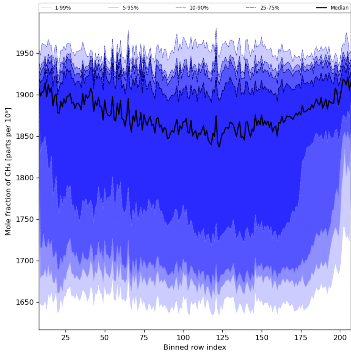
Figure 34: Along track statistics of “Mole fraction of CH 4 ” for 2024-02-09 to 2024-02-11
