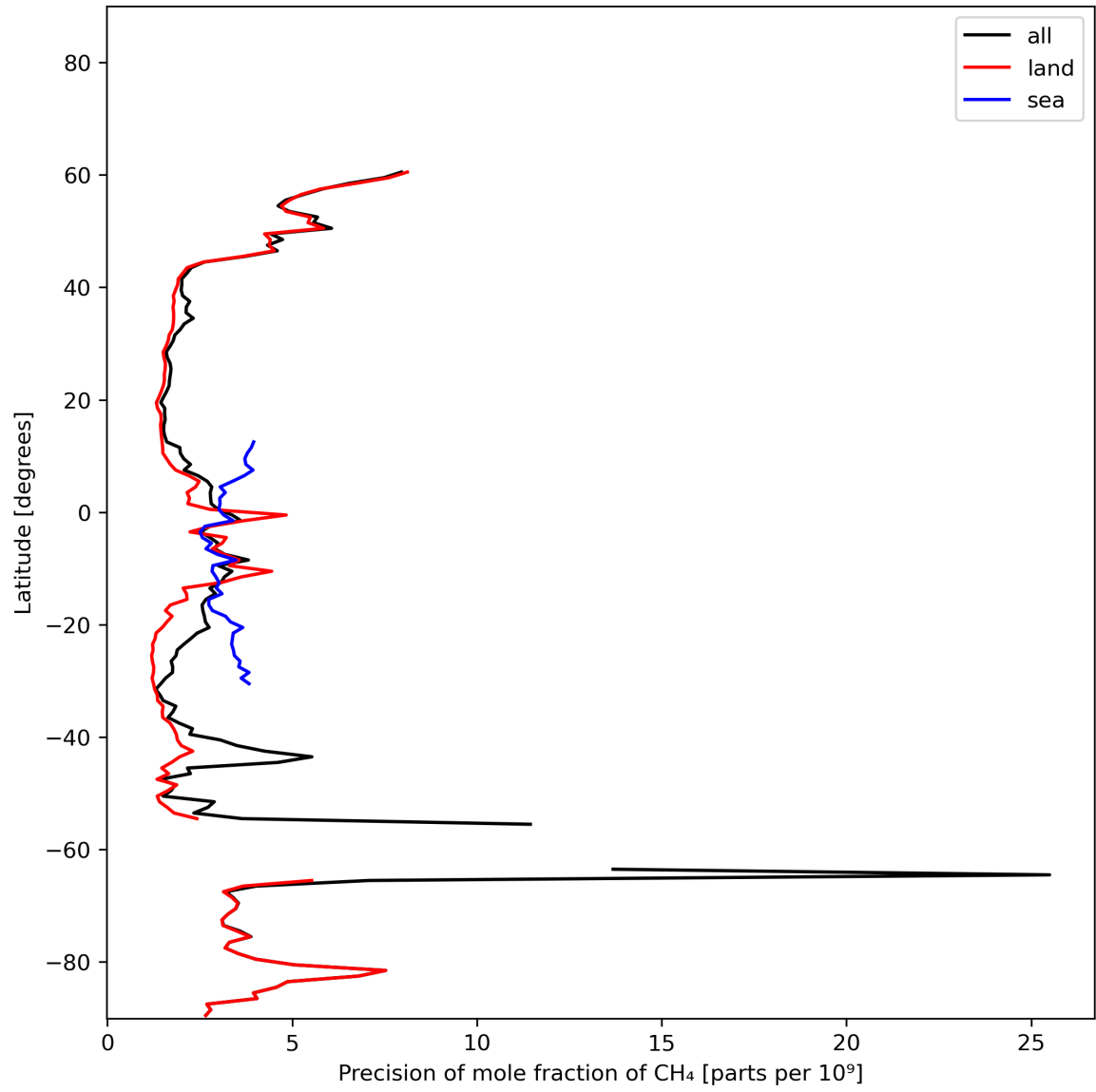
Figure 13: Zonal average of “Precision of mole fraction of CH 4 ” for 2024-02-09 to 2024-02-11.
