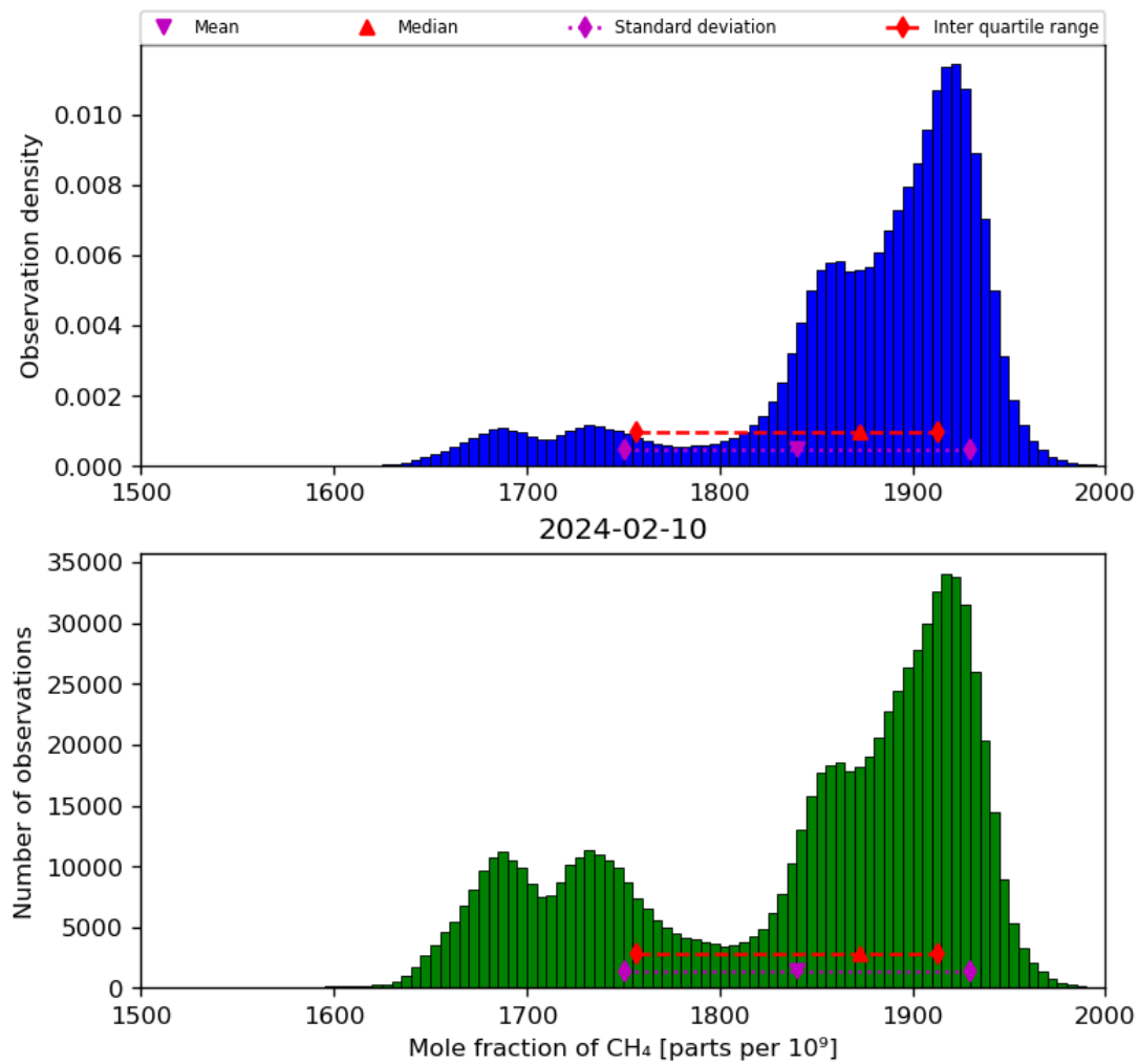
Figure 23: Histogram of “Mole fraction of CH 4 ” for 2024-02-09 to 2024-02-11
