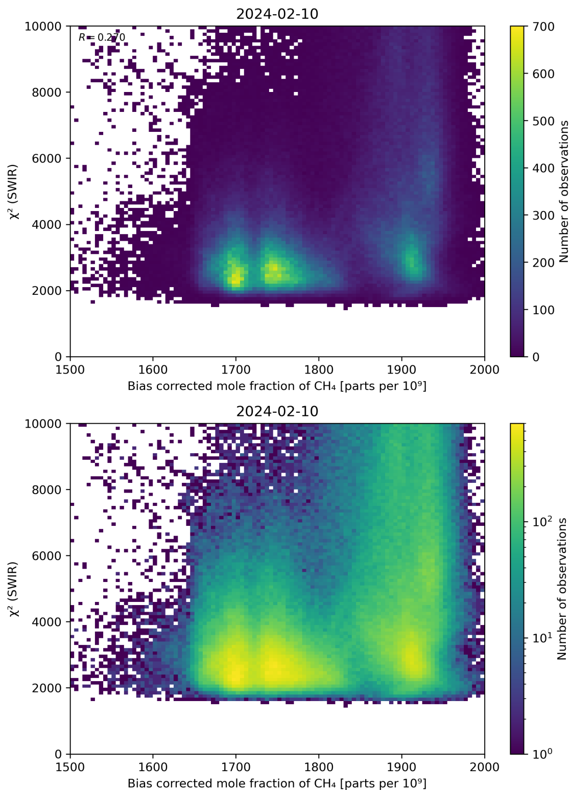
Figure 64: Scatter density plot of “Bias corrected mole fraction of \text{CH}_4 ” against “ \chi^2 (SWIR)” for 2024-02-09 to 2024-02-11.
