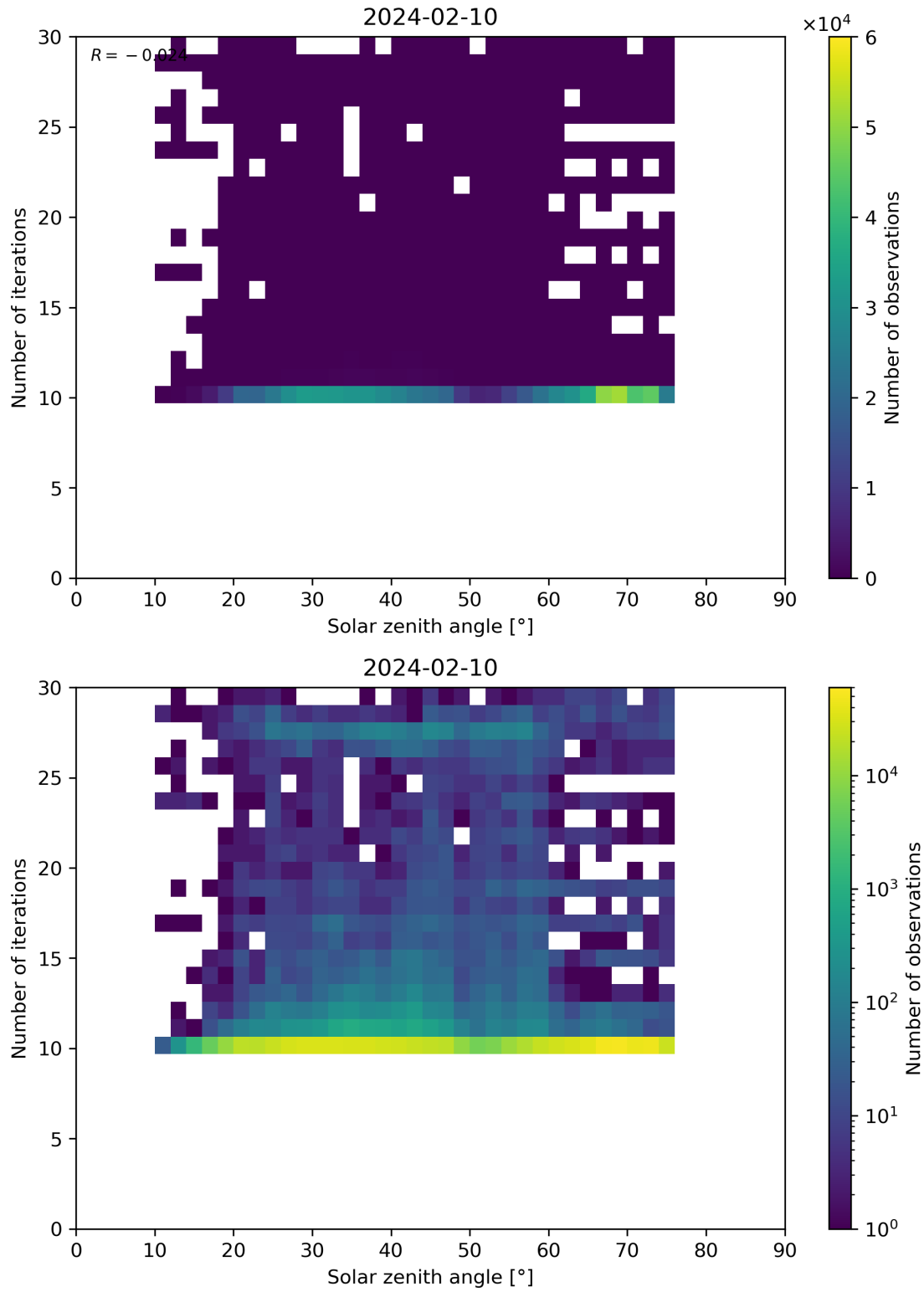
Figure 102: Scatter density plot of “Solar zenith angle” against “Number of iterations” for 2024-02-09 to 2024-02-11.
