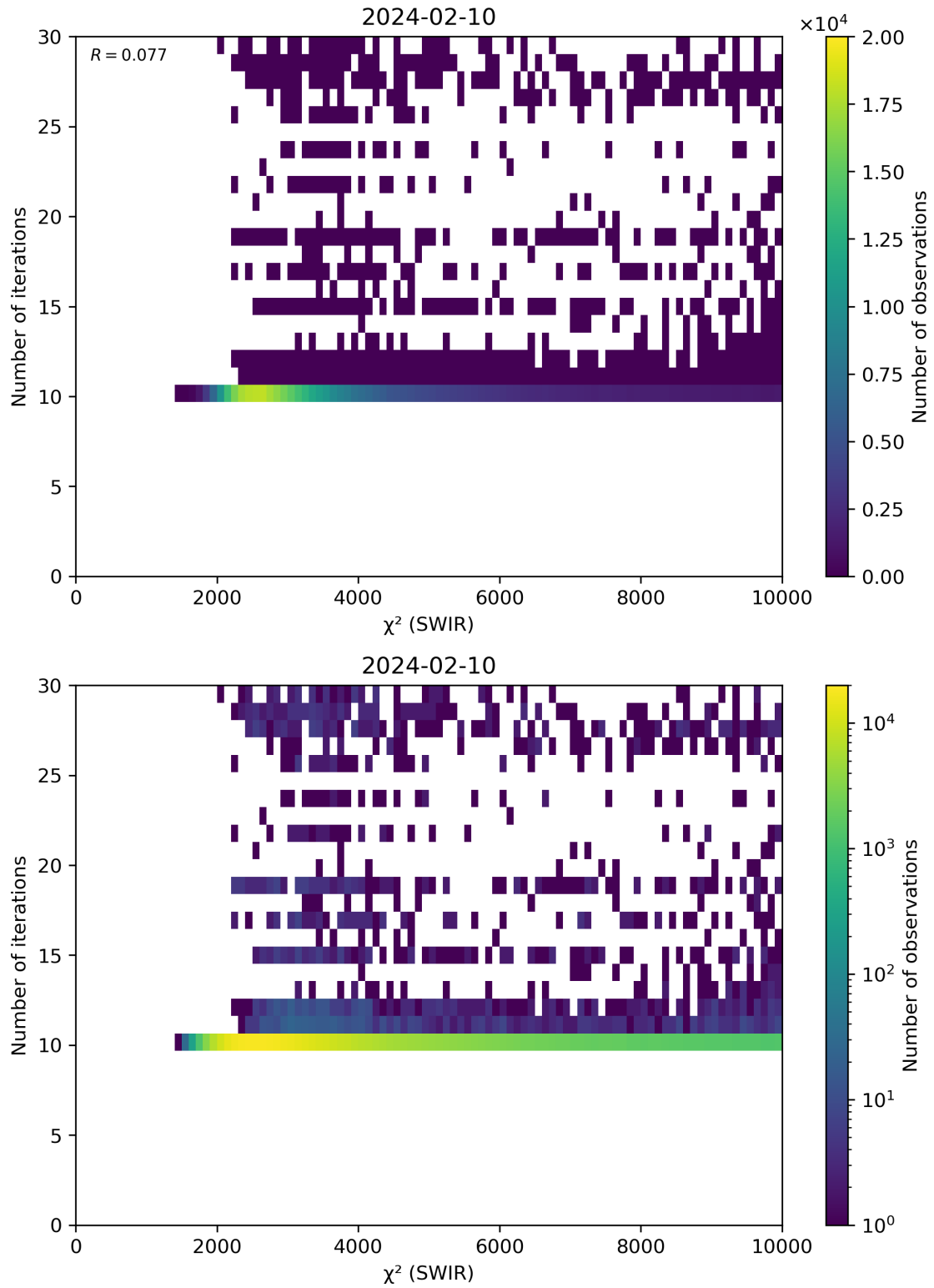
Figure 50: Scatter density plot of " \chi^2 (SWIR)" against "Number of iterations" for 2024-02-09 to 2024-02-11.
