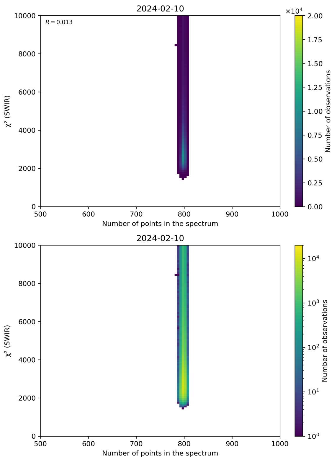
Figure 89: Scatter density plot of “Number of points in the spectrum” against “ \chi^2 (SWIR)” for 2024-02-09 to 2024-02-11.
