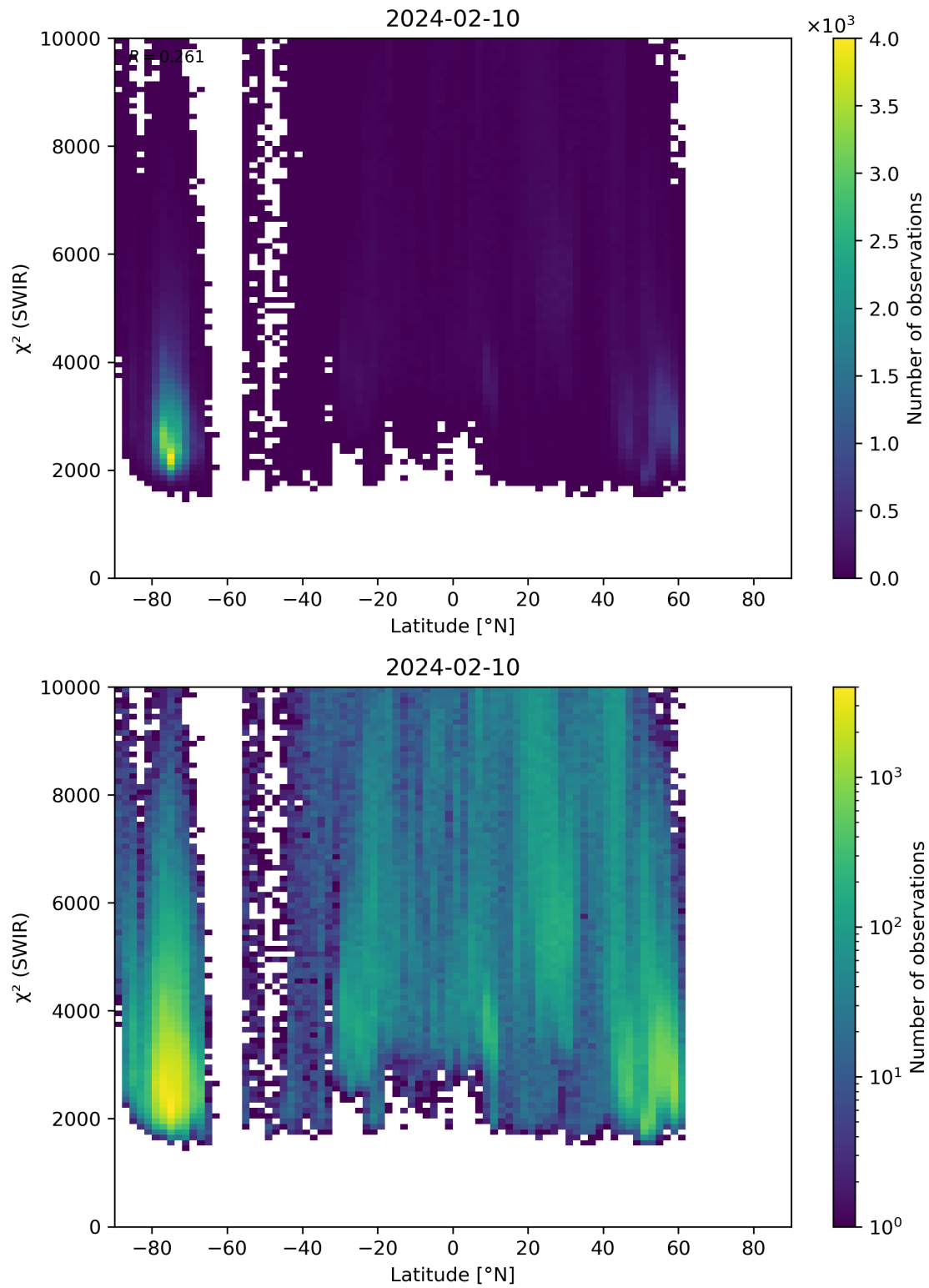
Figure 54: Scatter density plot of “Latitude” against “ \chi^2 (SWIR)” for 2024-02-09 to 2024-02-11.
