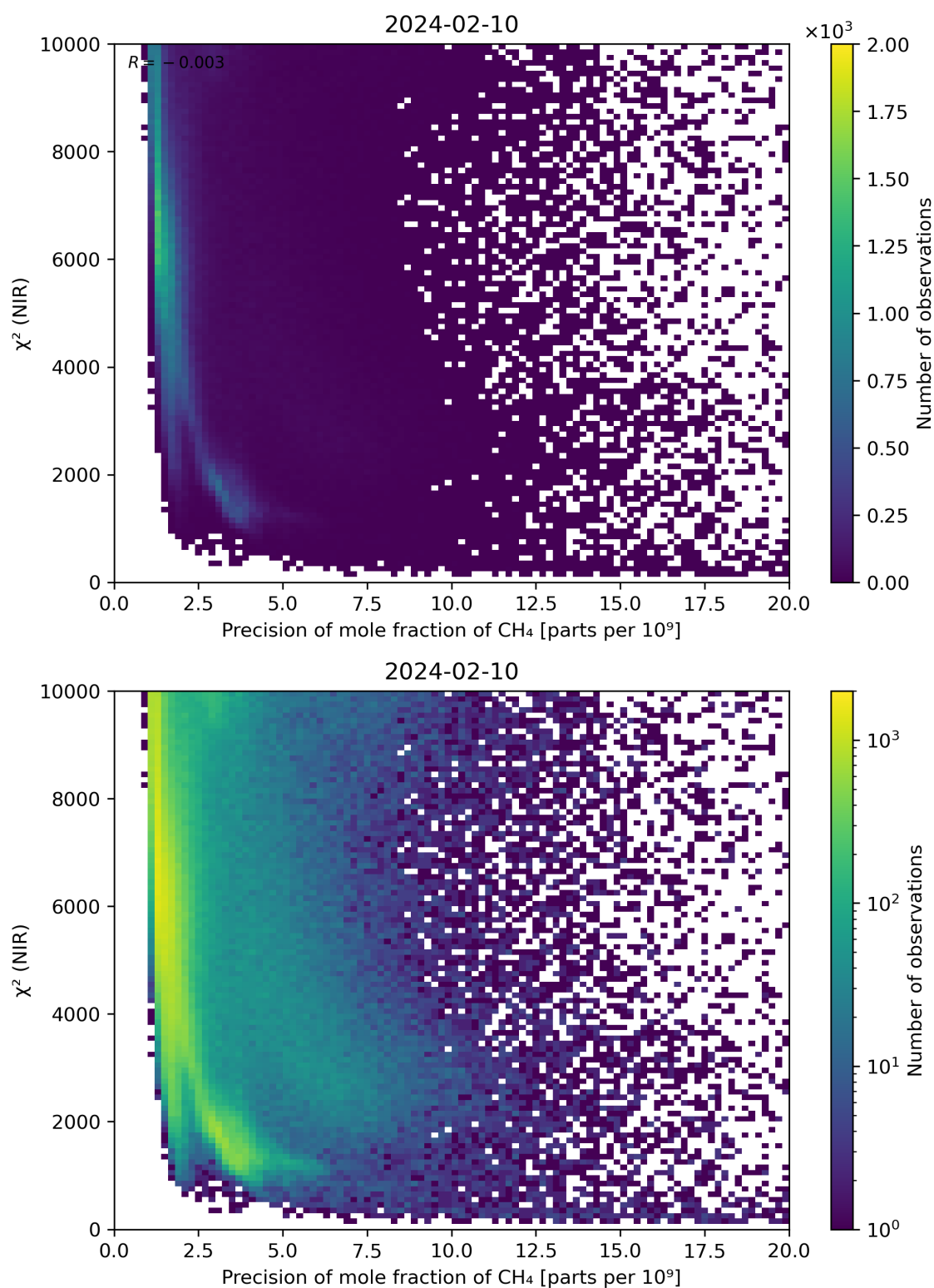
Figure 78: Scatter density plot of “Precision of mole fraction of \text{CH}_4 ” against “ \chi^2 (NIR)” for 2024-02-09 to 2024-02-11.
