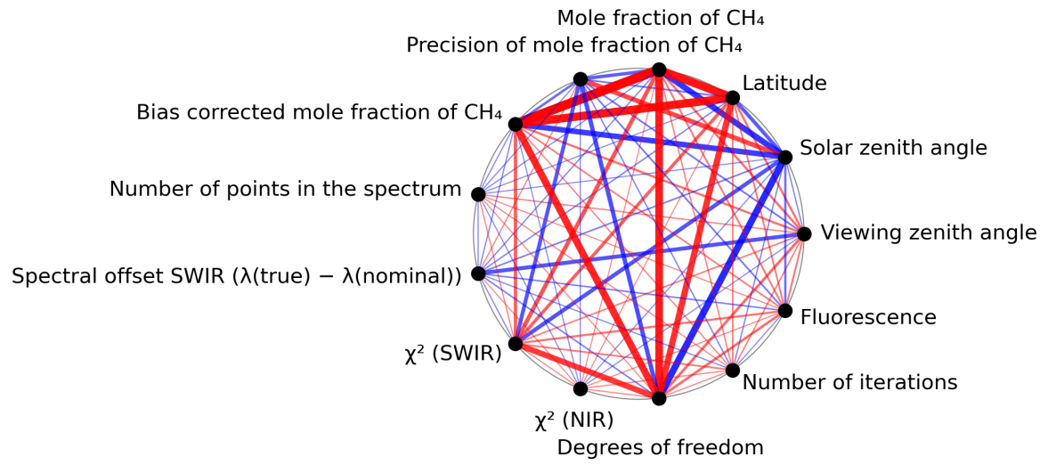
Figure 1: Map of correlation graph for 2024-02-09 to 2024-02-11.
