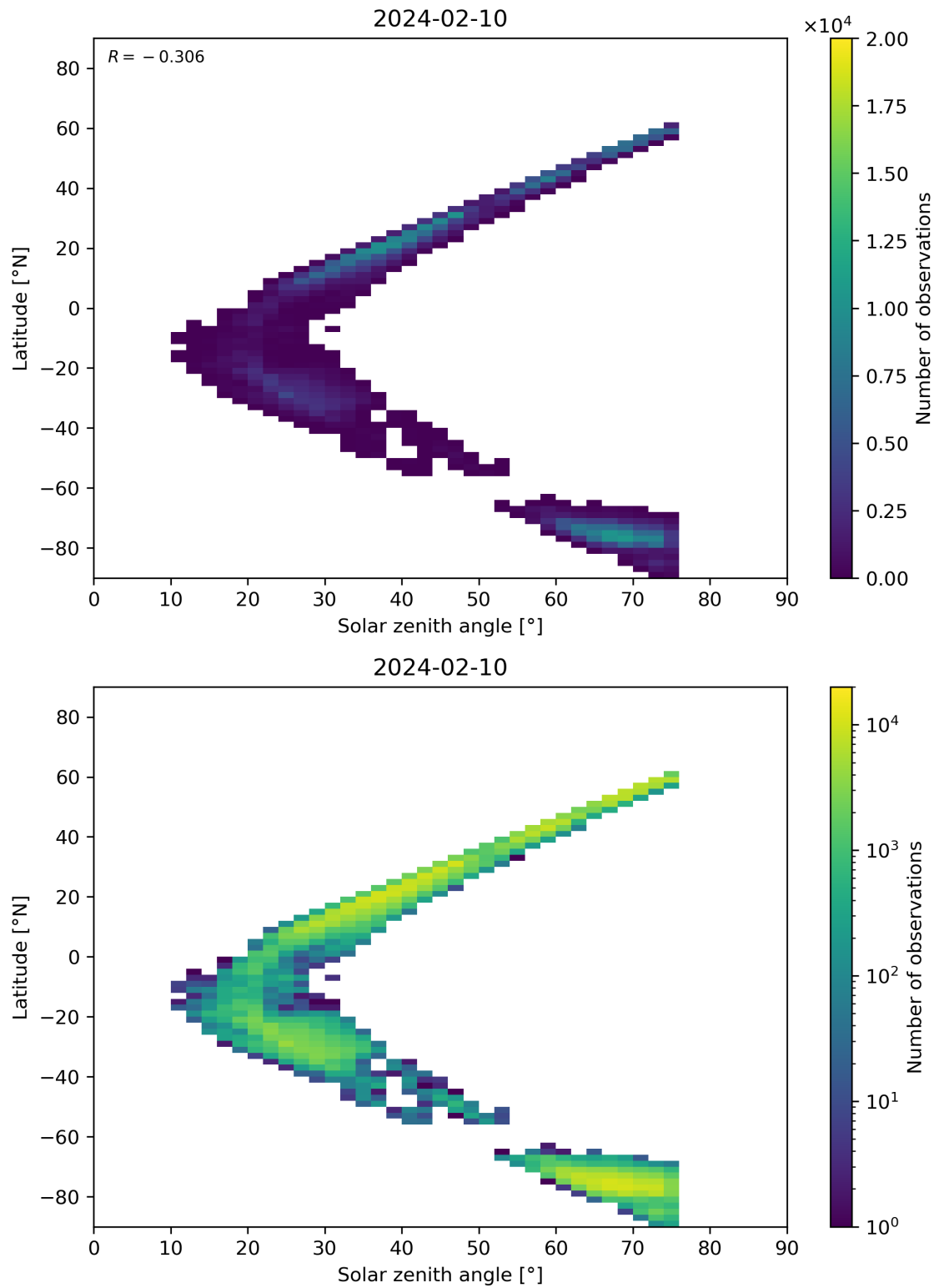
Figure 98: Scatter density plot of “Solar zenith angle” against “Latitude” for 2024-02-09 to 2024-02-11.
