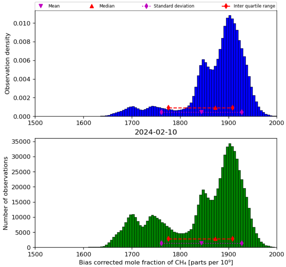
Figure 25: Histogram of “Bias corrected mole fraction of CH 4 ” for 2024-02-09 to 2024-02-11
