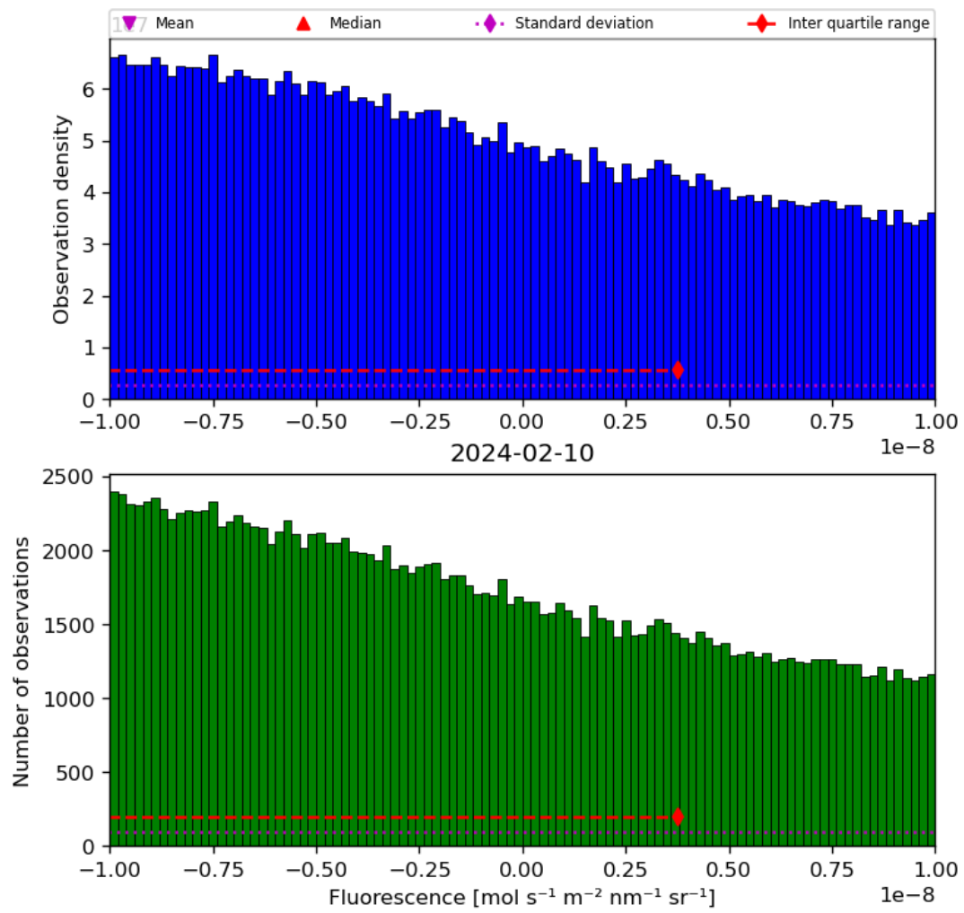
Figure 32: Histogram of “Fluorescence” for 2024-02-09 to 2024-02-11
