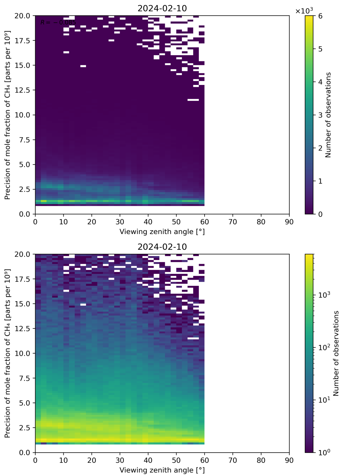
Figure 112: Scatter density plot of “Viewing zenith angle” against “Precision of mole fraction of CH 4 ” for 2024-02-09 to 2024-02-11.
