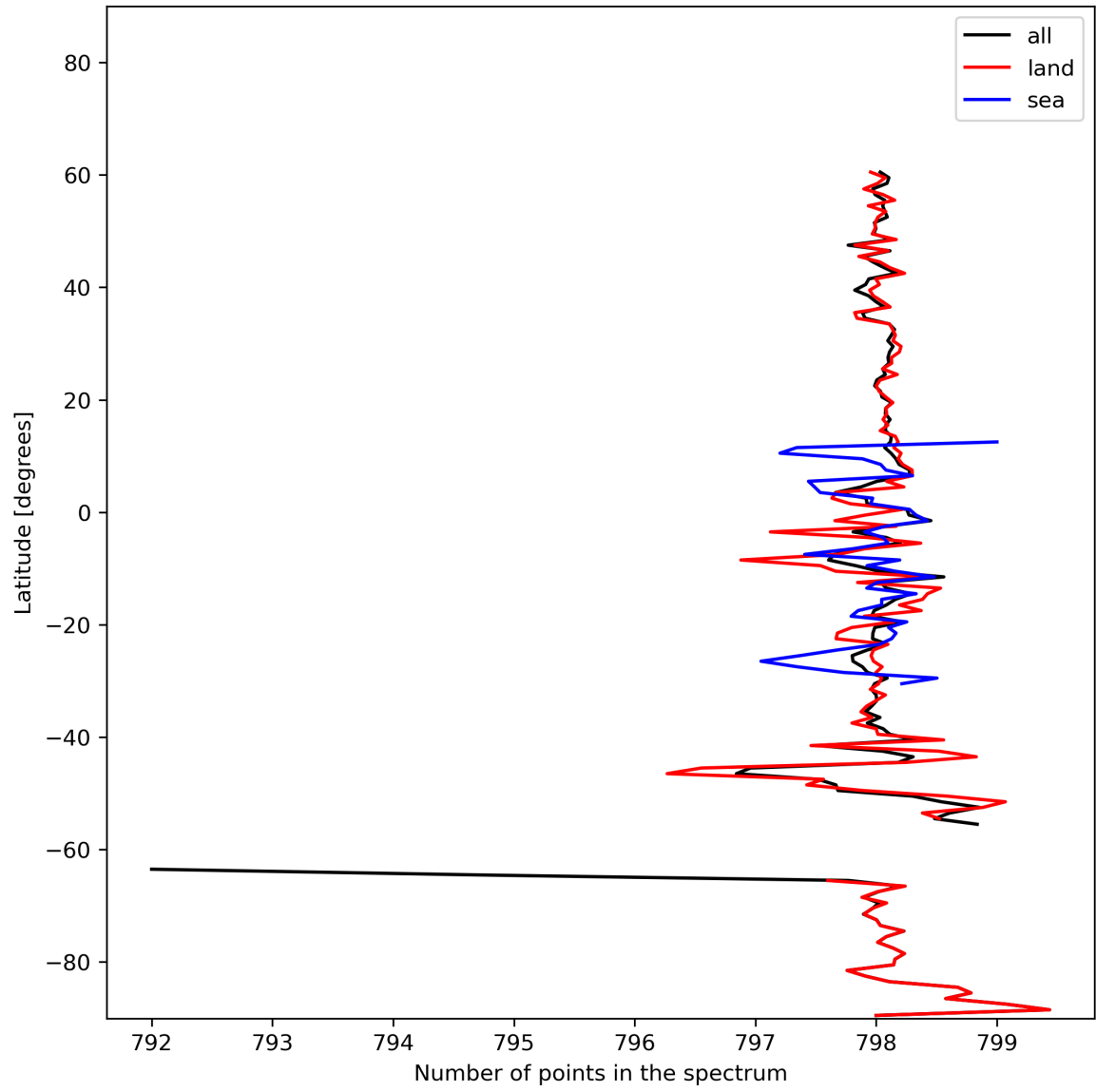
Figure 15: Zonal average of “Number of points in the spectrum” for 2024-02-09 to 2024-02-11.
