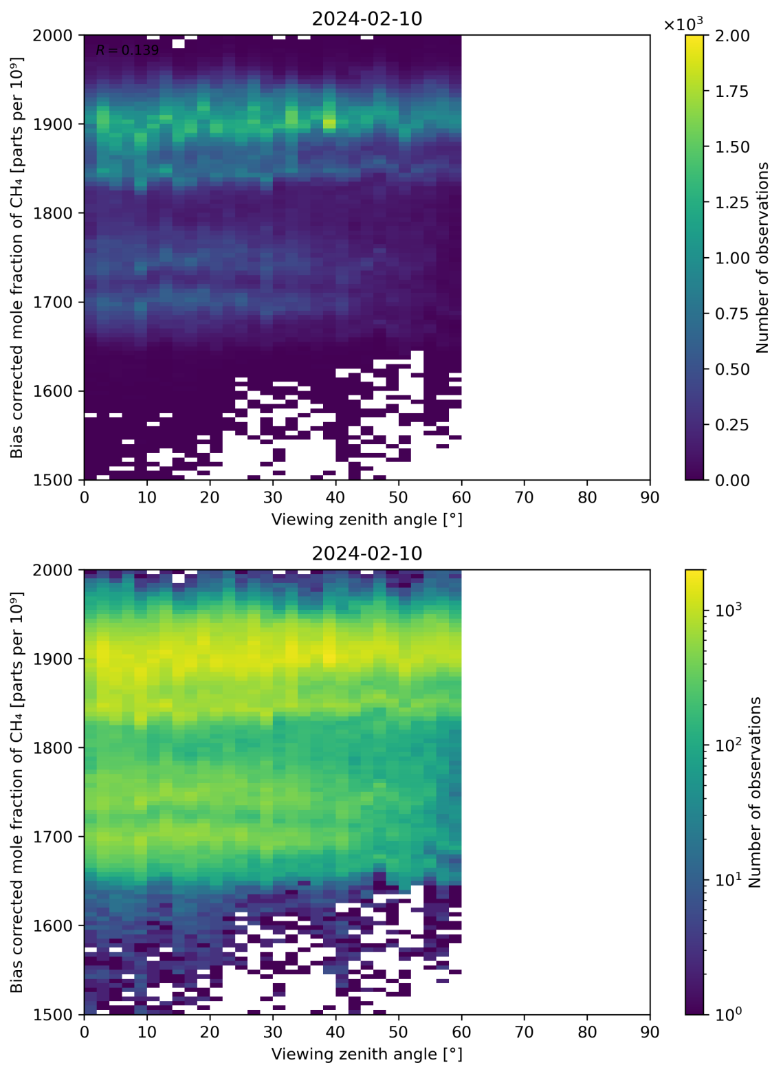
Figure 111: Scatter density plot of “Viewing zenith angle” against “Bias corrected mole fraction of CH 4 ” for 2024-02-09 to 2024-02-11.
