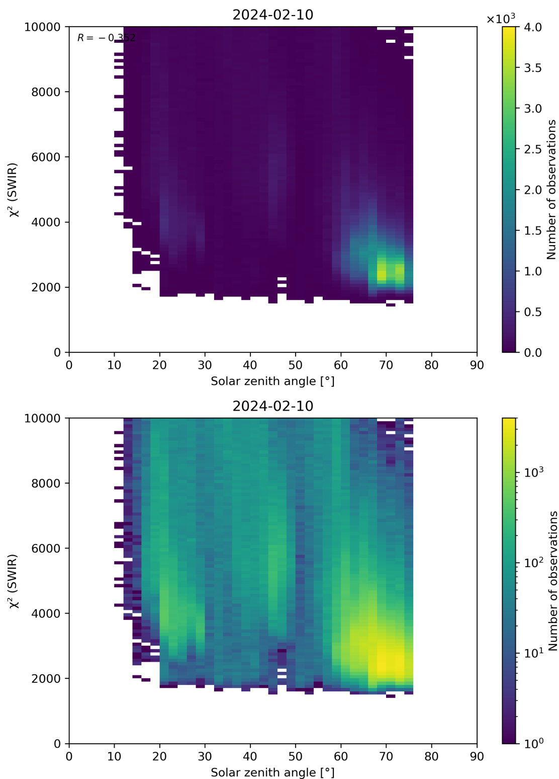
Figure 95: Scatter density plot of “Solar zenith angle” against “ \chi^2 (SWIR)” for 2024-02-09 to 2024-02-11.
