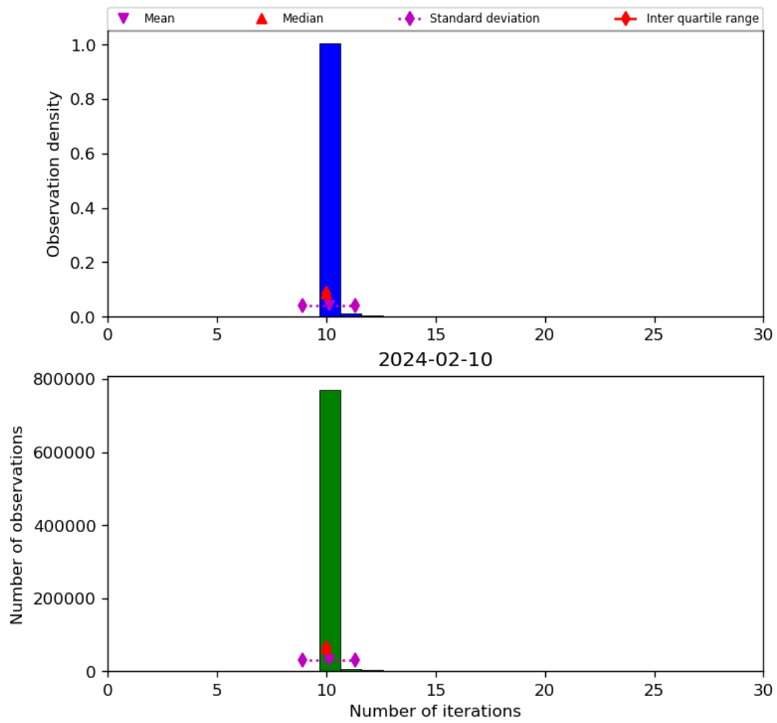
Figure 31: Histogram of “Number of iterations” for 2024-02-09 to 2024-02-11
