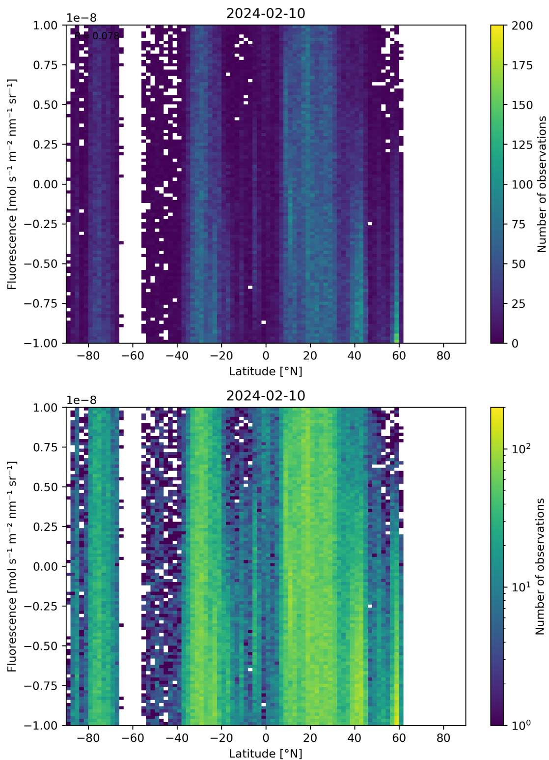
Figure 56: Scatter density plot of “Latitude” against “Fluorescence” for 2024-02-09 to 2024-02-11.
