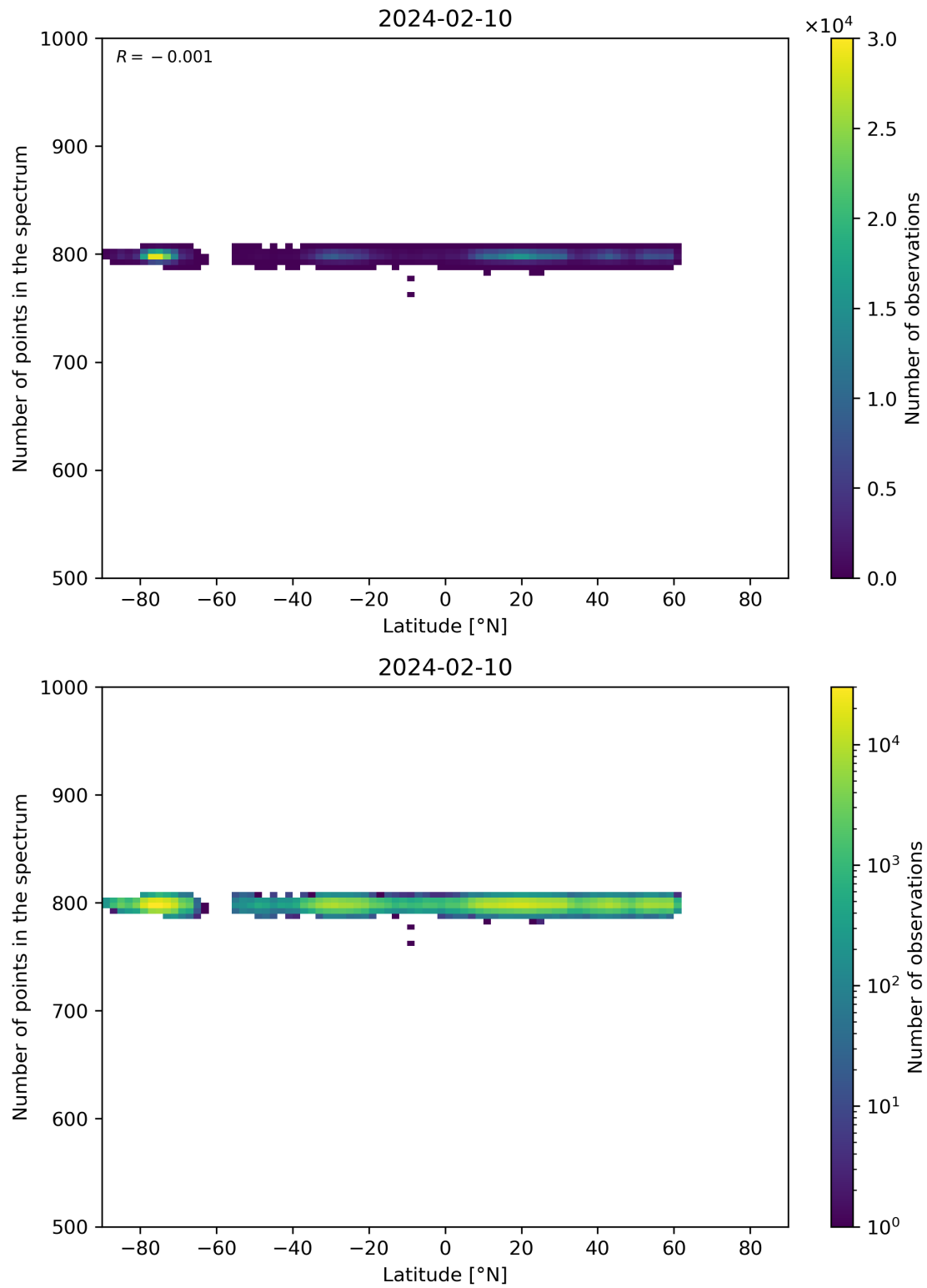
Figure 61: Scatter density plot of “Latitude” against “Number of points in the spectrum” for 2024-02-09 to 2024-02-11.
