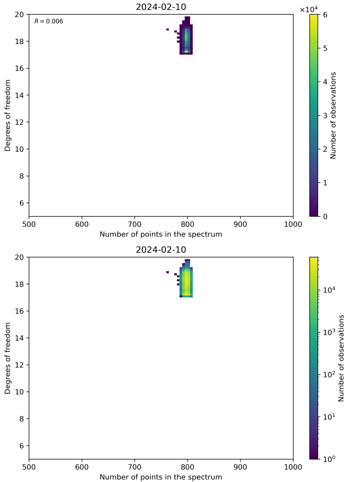
Figure 90: Scatter density plot of “Number of points in the spectrum” against “Degrees of freedom” for 2024-02-09 to 2024-02-11.
