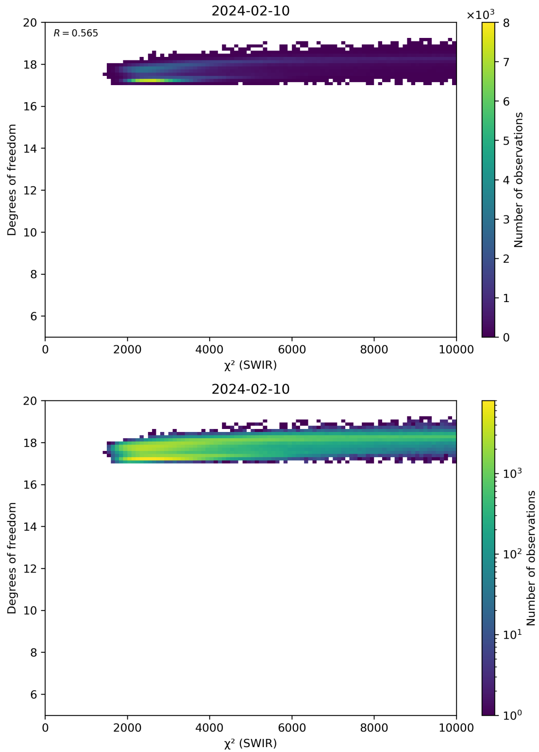
Figure 48: Scatter density plot of “ \chi^2 (SWIR)” against “Degrees of freedom” for 2024-02-09 to 2024-02-11.
