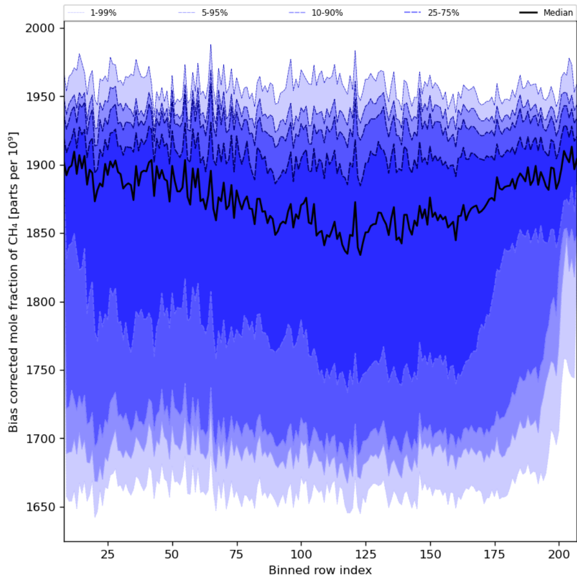
Figure 36: Along track statistics of “Bias corrected mole fraction of CH 4 ” for 2024-02-09 to 2024-02-11
