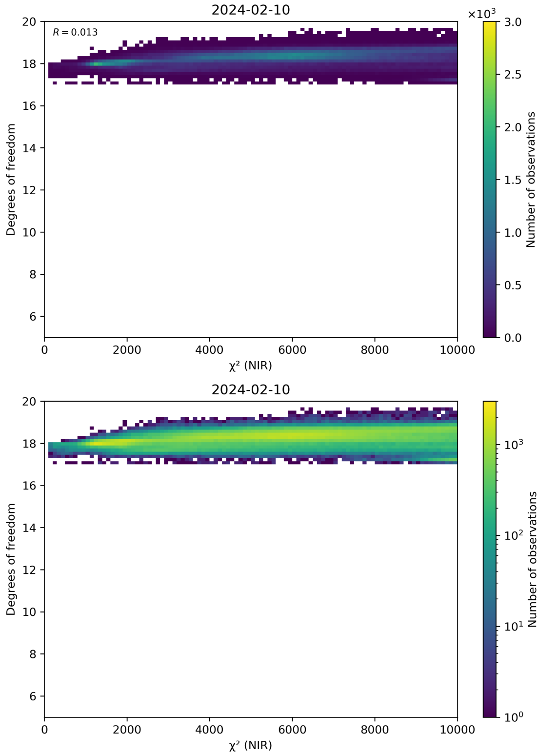
Figure 44: Scatter density plot of “ \chi^2 (NIR)” against “Degrees of freedom” for 2024-02-09 to 2024-02-11.
