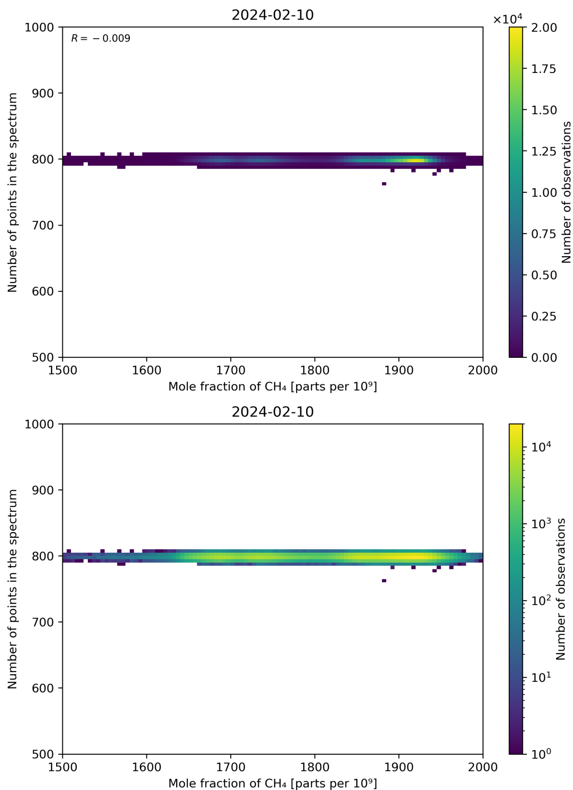
Figure 77: Scatter density plot of “Mole fraction of CH 4 ” against “Number of points in the spectrum” for 2024-02-09 to 2024-02-11.
