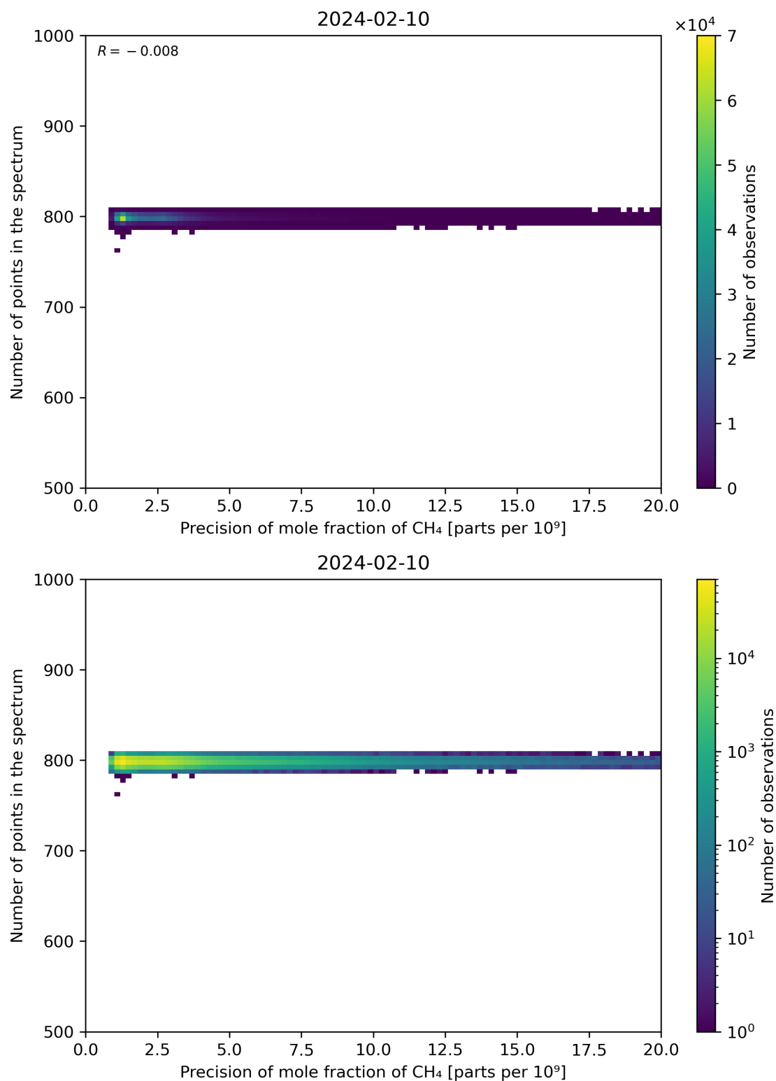
Figure 84: Scatter density plot of “Precision of mole fraction of CH 4 ” against “Number of points in the spectrum” for 2024-02-09 to 2024-02-11.
