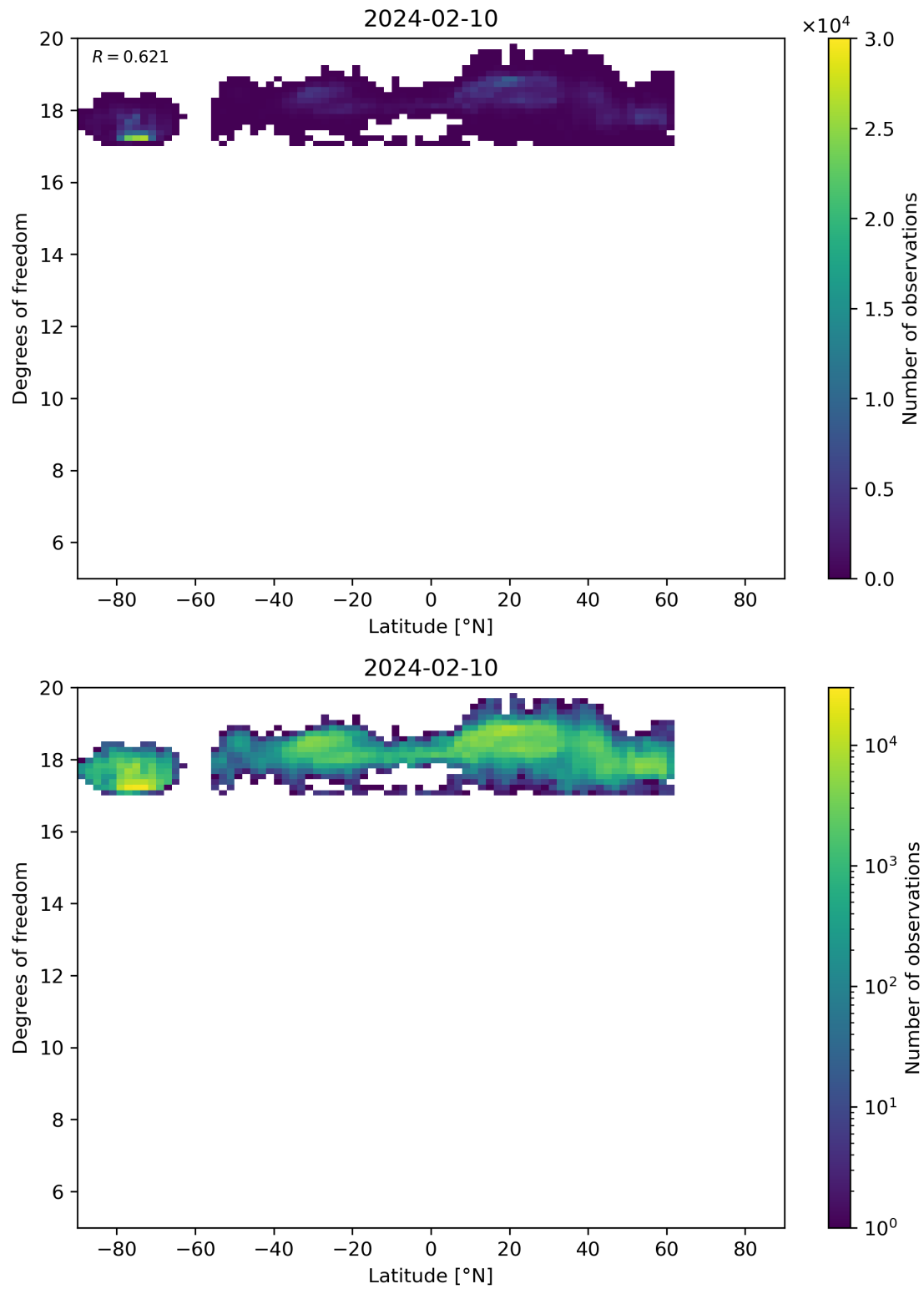
Figure 55: Scatter density plot of “Latitude” against “Degrees of freedom” for 2024-02-09 to 2024-02-11.
