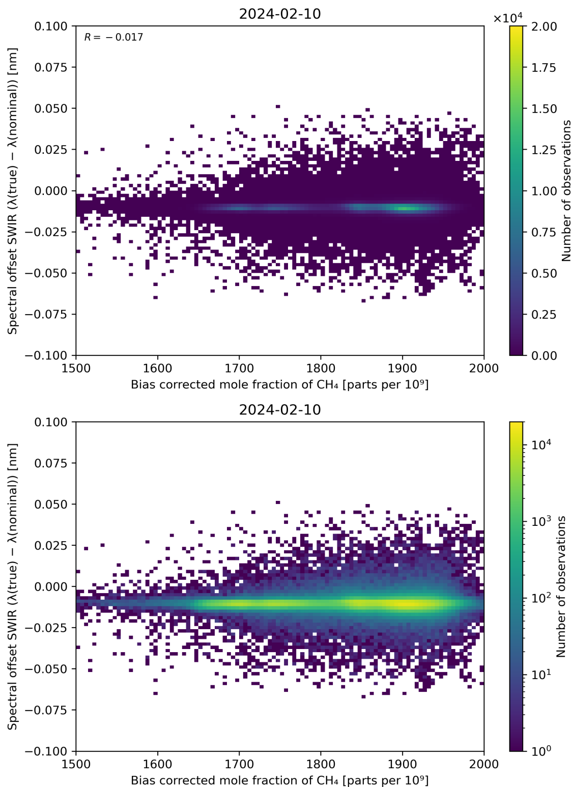
Figure 69: Scatter density plot of “Bias corrected mole fraction of \text{CH}_4 ” against “Spectral offset SWIR ( \lambda(\text{true}) - \lambda(\text{nominal}) )” for 2024-02-09 to 2024-02-11.
