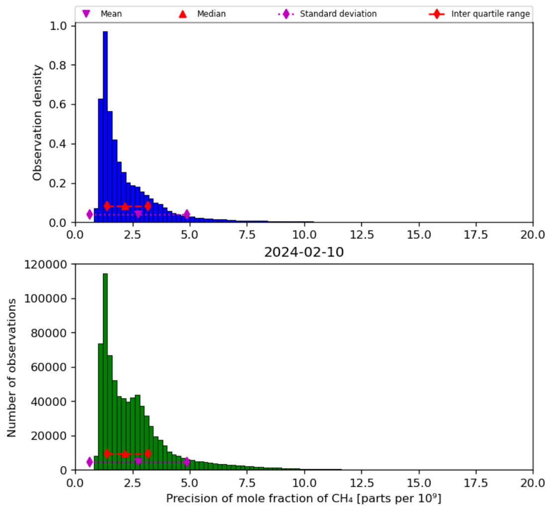
Figure 24: Histogram of “Precision of mole fraction of CH 4 ” for 2024-02-09 to 2024-02-11
