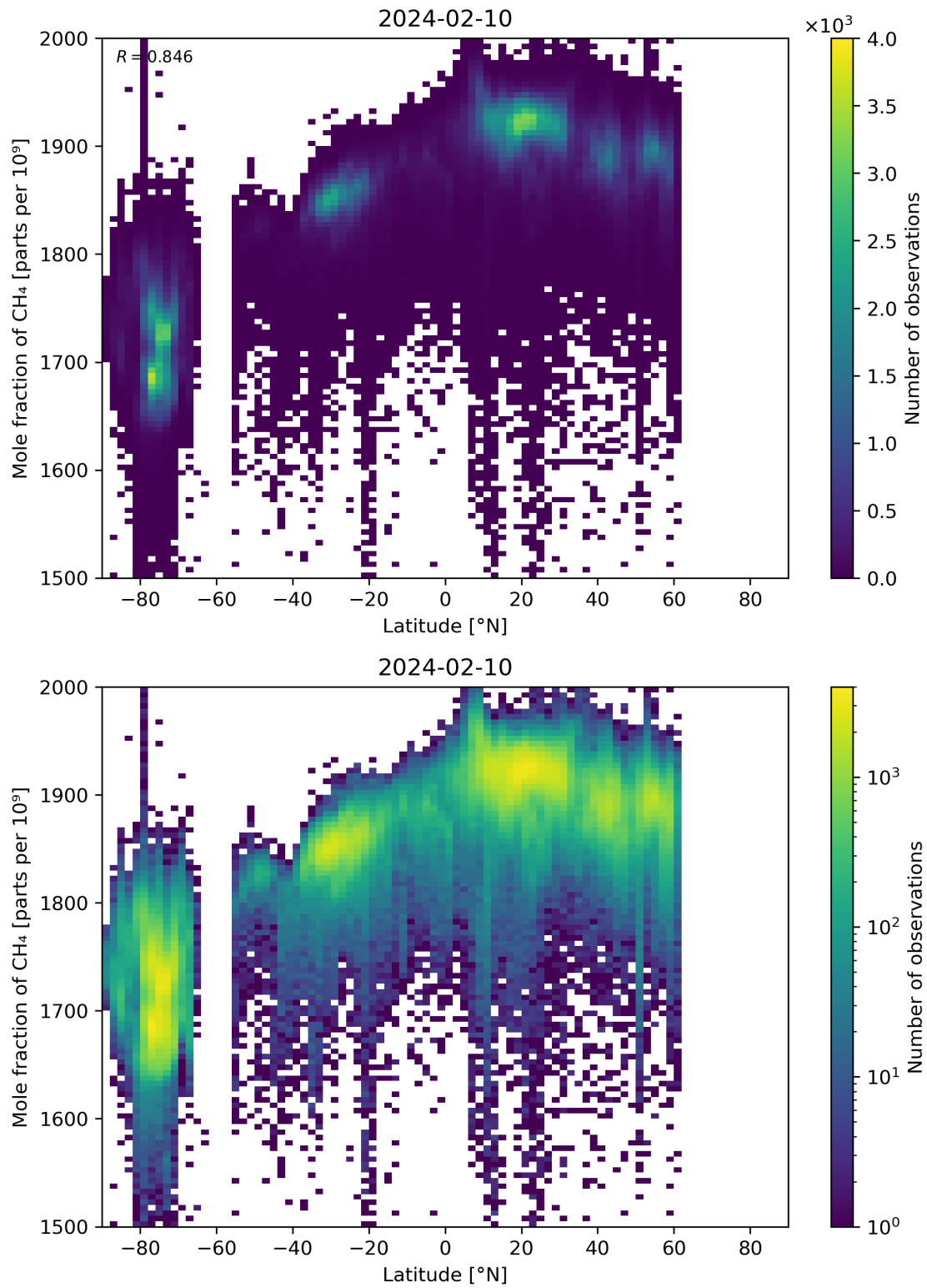
Figure 57: Scatter density plot of “Latitude” against “Mole fraction of CH 4 ” for 2024-02-09 to 2024-02-11.
