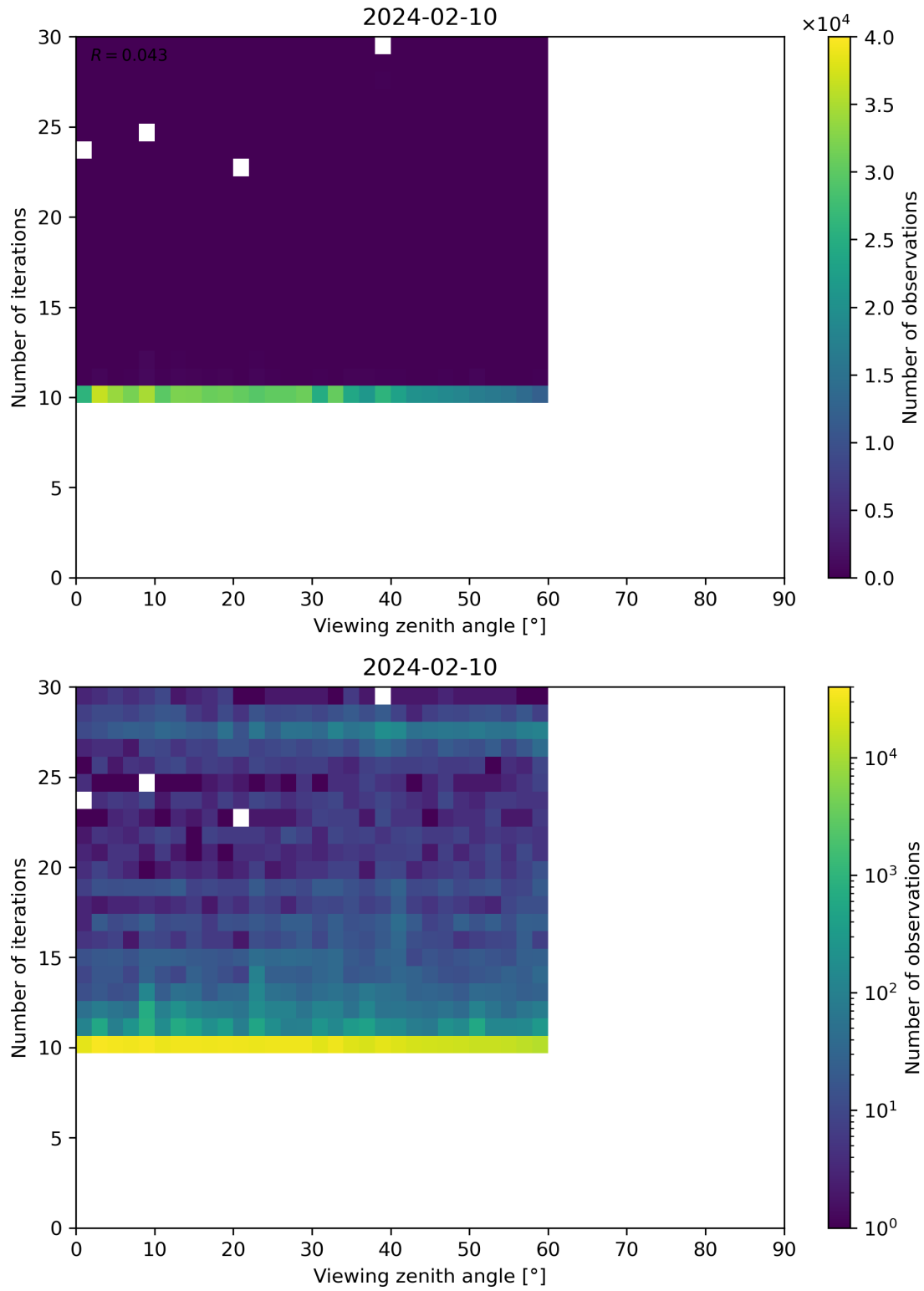
Figure 113: Scatter density plot of “Viewing zenith angle” against “Number of iterations” for 2024-02-09 to 2024-02-11.
