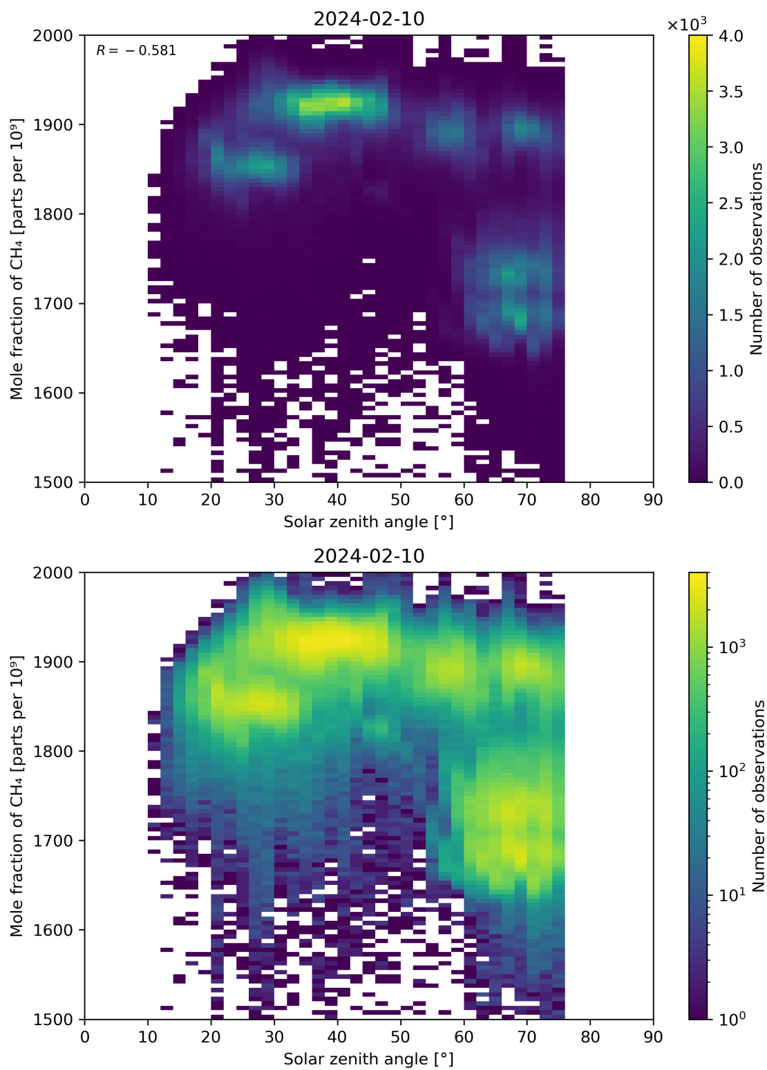
Figure 99: Scatter density plot of “Solar zenith angle” against “Mole fraction of \text{CH}_4 ” for 2024-02-09 to 2024-02-11.
