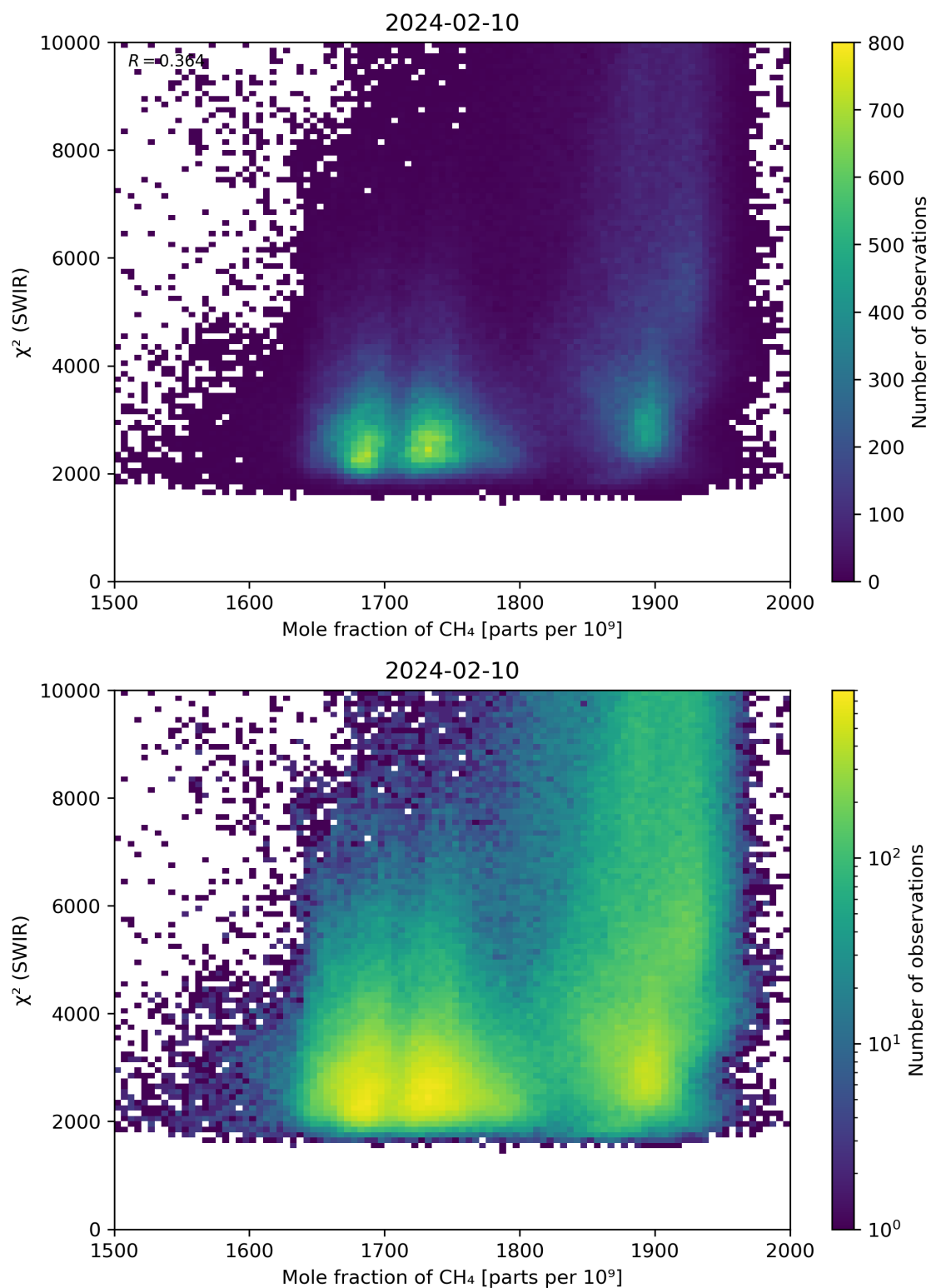
Figure 71: Scatter density plot of “Mole fraction of \text{CH}_4 ” against “ \chi^2 (SWIR)” for 2024-02-09 to 2024-02-11.
