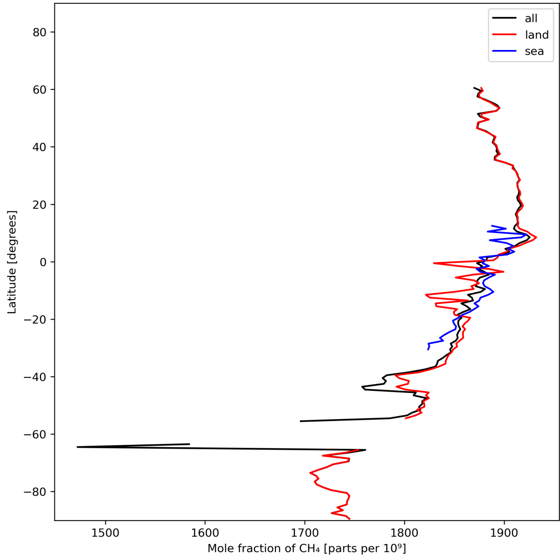
Figure 12: Zonal average of “Mole fraction of CH 4 ” for 2024-02-09 to 2024-02-11.
