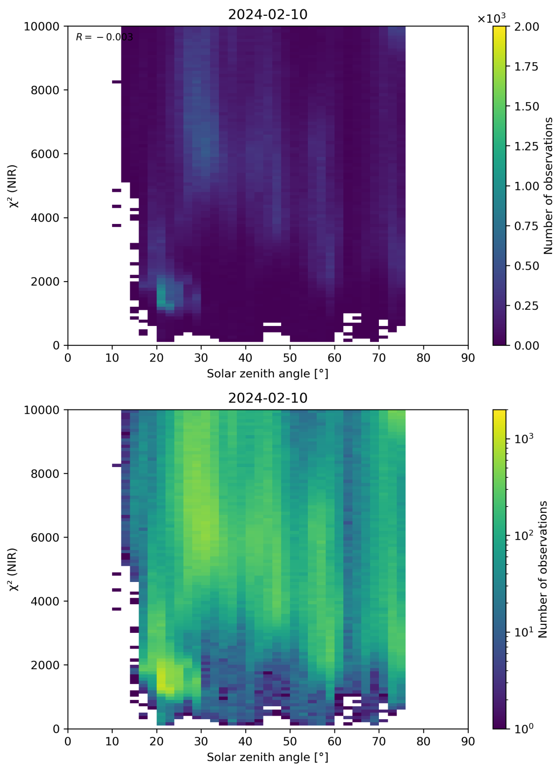
Figure 94: Scatter density plot of “Solar zenith angle” against “ \chi^2 (NIR)” for 2024-02-09 to 2024-02-11.
