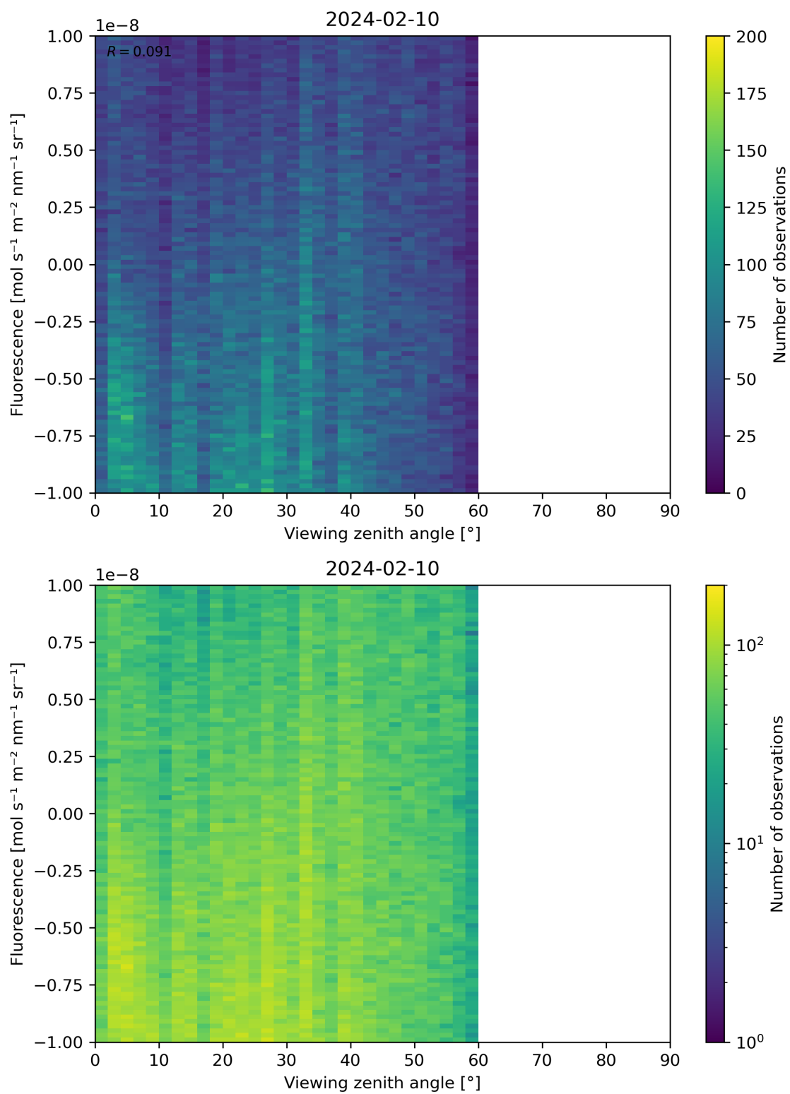
Figure 108: Scatter density plot of “Viewing zenith angle” against “Fluorescence” for 2024-02-09 to 2024-02-11.
