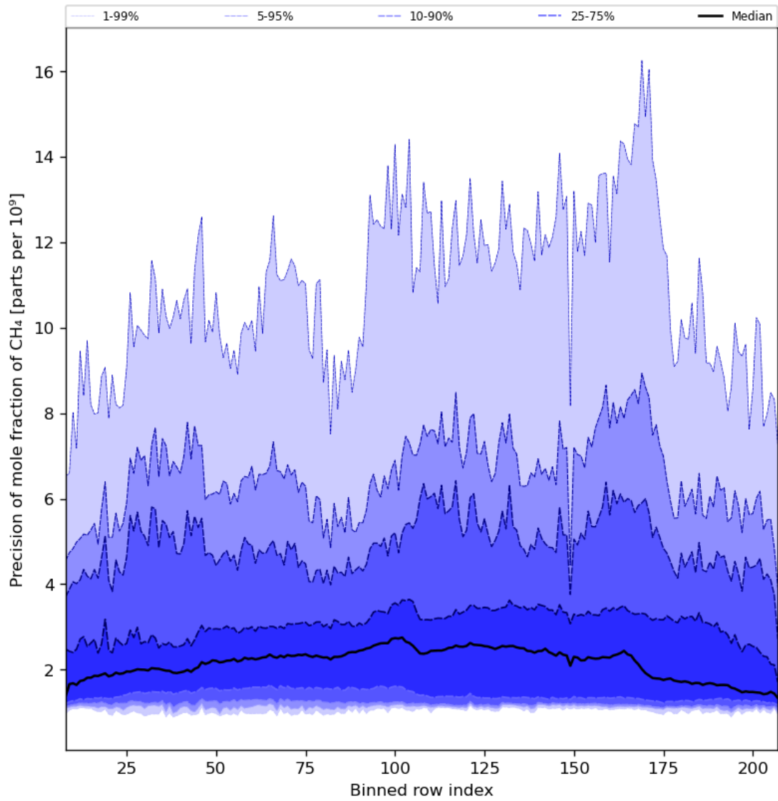
Figure 35: Along track statistics of “Precision of mole fraction of CH 4 ” for 2024-02-09 to 2024-02-11
