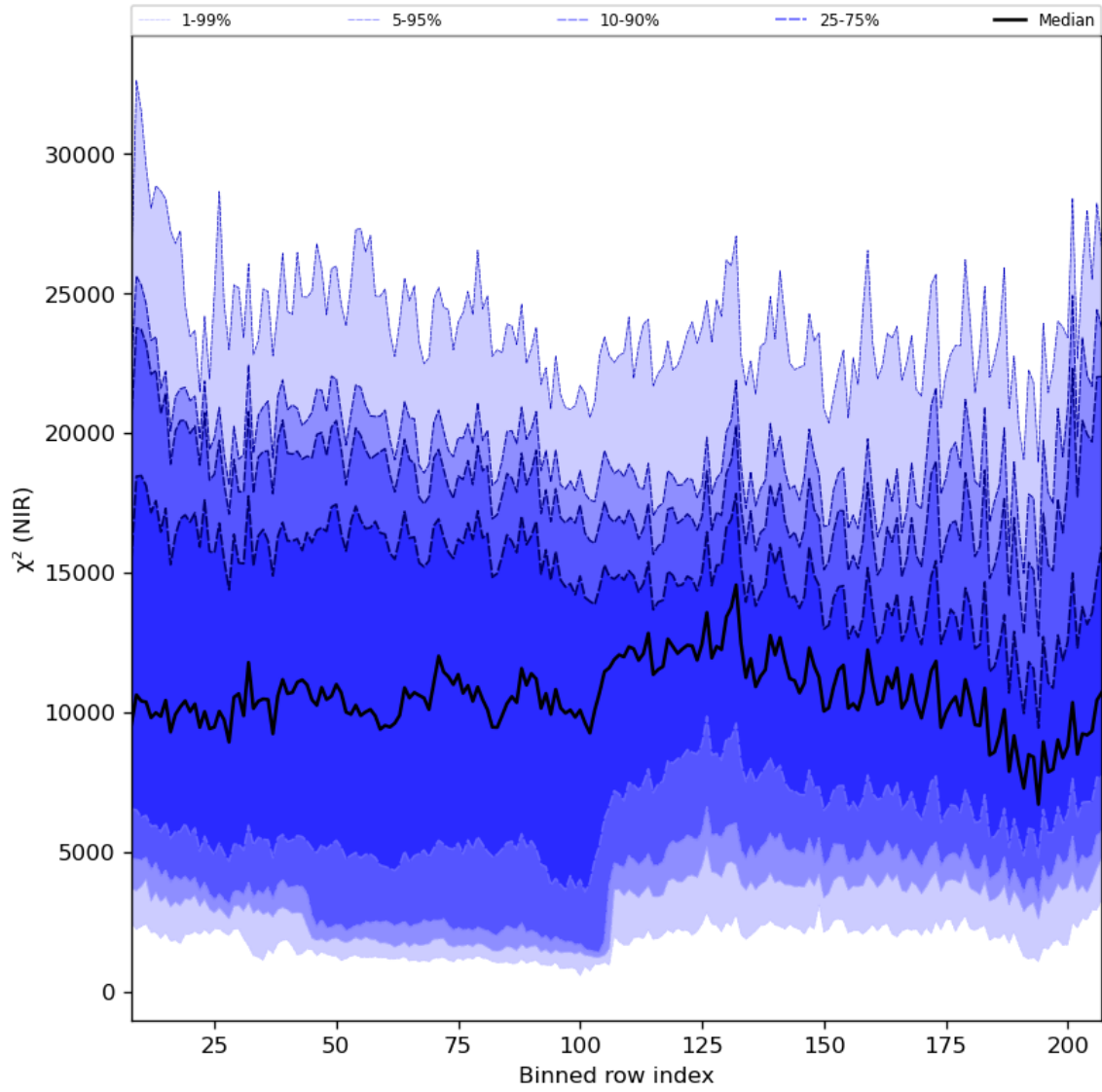
Figure 40: Along track statistics of " \chi^2 (NIR)" for 2024-02-09 to 2024-02-11
