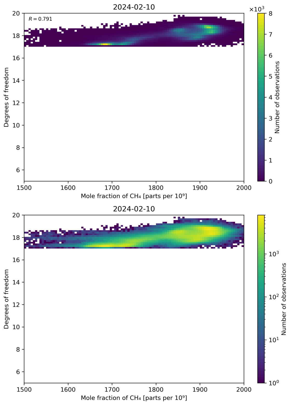
Figure 72: Scatter density plot of “Mole fraction of CH 4 ” against “Degrees of freedom” for 2024-02-09 to 2024-02-11.
