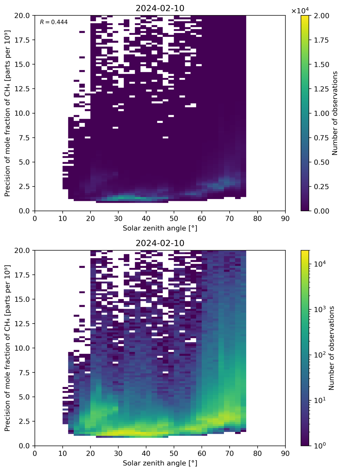
Figure 101: Scatter density plot of “Solar zenith angle” against “Precision of mole fraction of CH 4 ” for 2024-02-09 to 2024-02-11.
