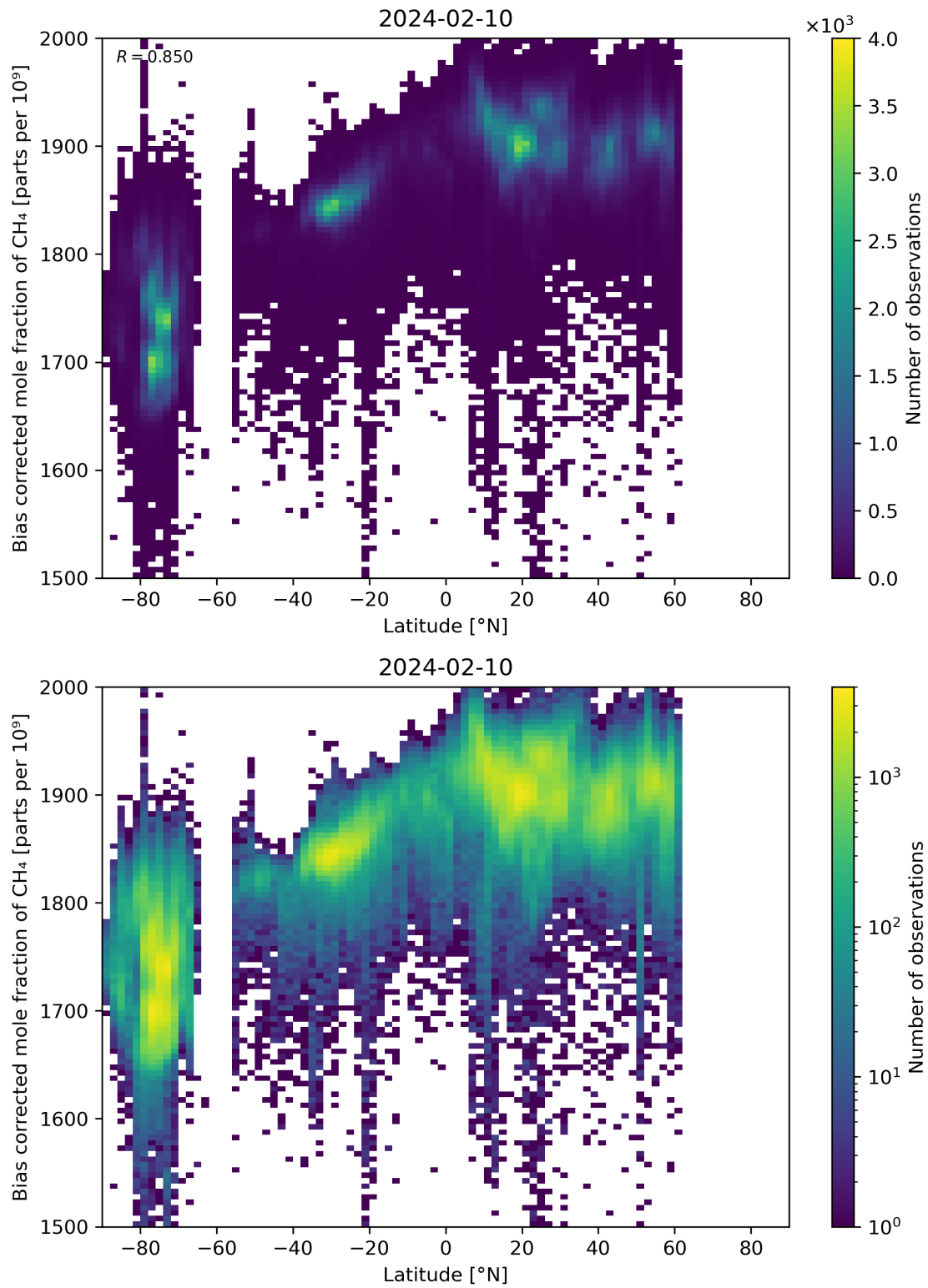
Figure 58: Scatter density plot of “Latitude” against “Bias corrected mole fraction of CH 4 ” for 2024-02-09 to 2024-02-11.
