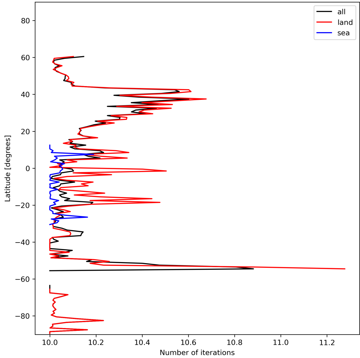
Figure 20: Zonal average of “Number of iterations” for 2024-02-09 to 2024-02-11.
