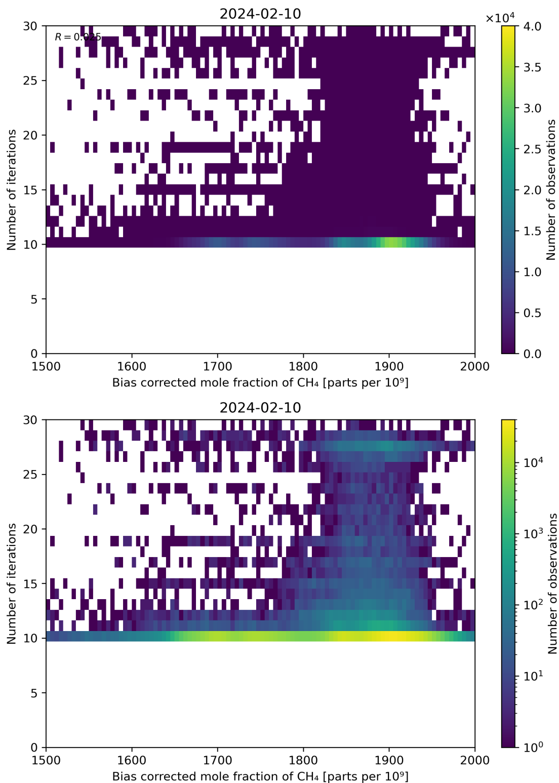
Figure 67: Scatter density plot of “Bias corrected mole fraction of \text{CH}_4 ” against “Number of iterations” for 2024-02-09 to 2024-02-11.
