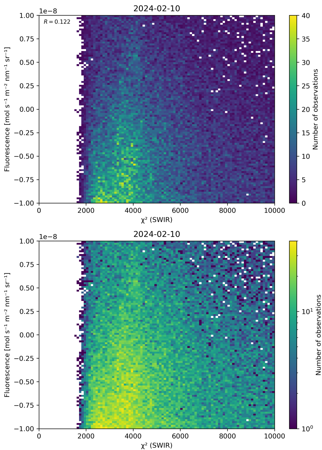
Figure 49: Scatter density plot of “ \chi^2 (SWIR)” against “Fluorescence” for 2024-02-09 to 2024-02-11.
