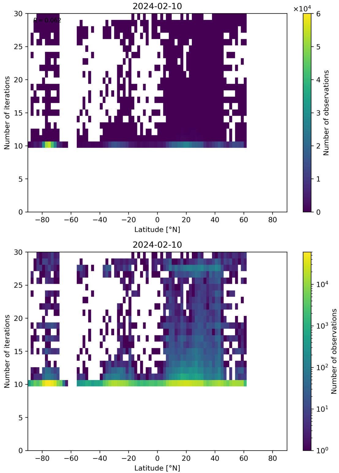
Figure 60: Scatter density plot of “Latitude” against “Number of iterations” for 2024-02-09 to 2024-02-11.
