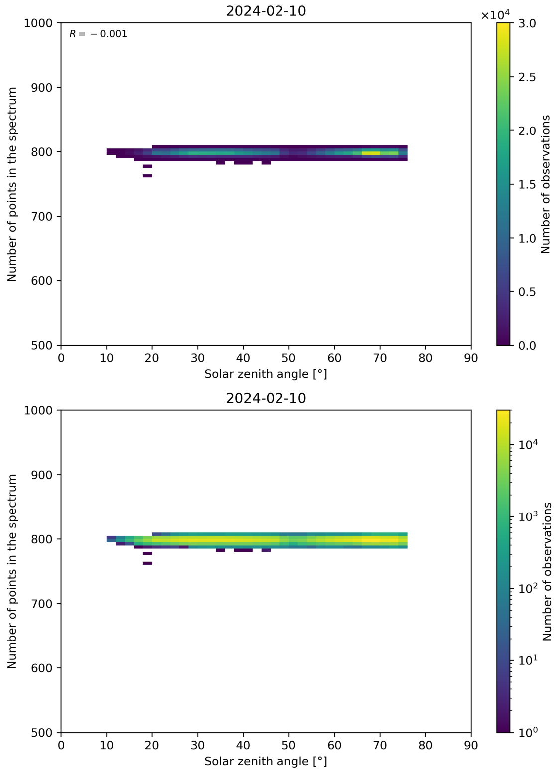
Figure 103: Scatter density plot of “Solar zenith angle” against “Number of points in the spectrum” for 2024-02-09 to 2024-02-11.
