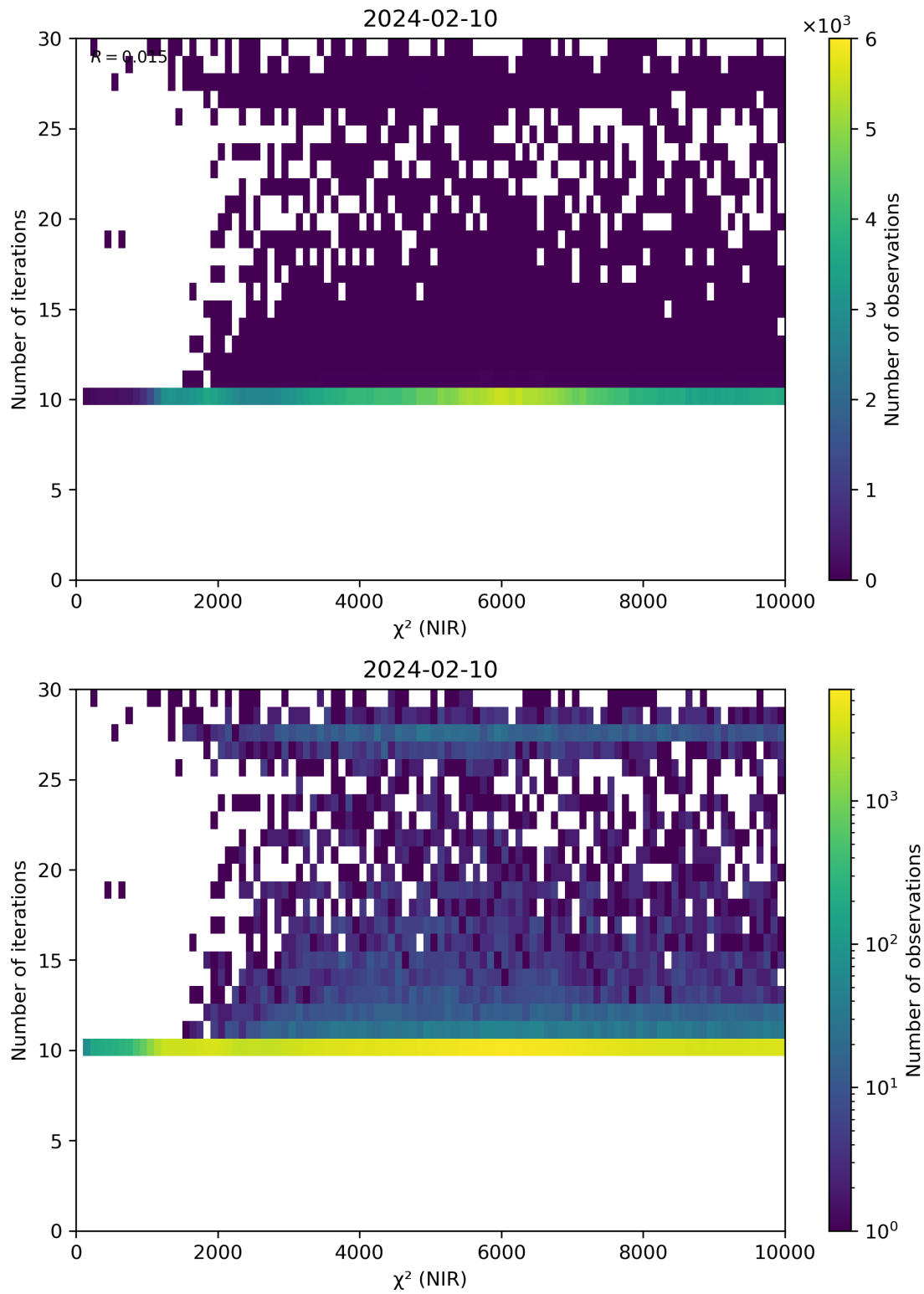
Figure 46: Scatter density plot of “ \chi^2 (NIR)” against “Number of iterations” for 2024-02-09 to 2024-02-11.
