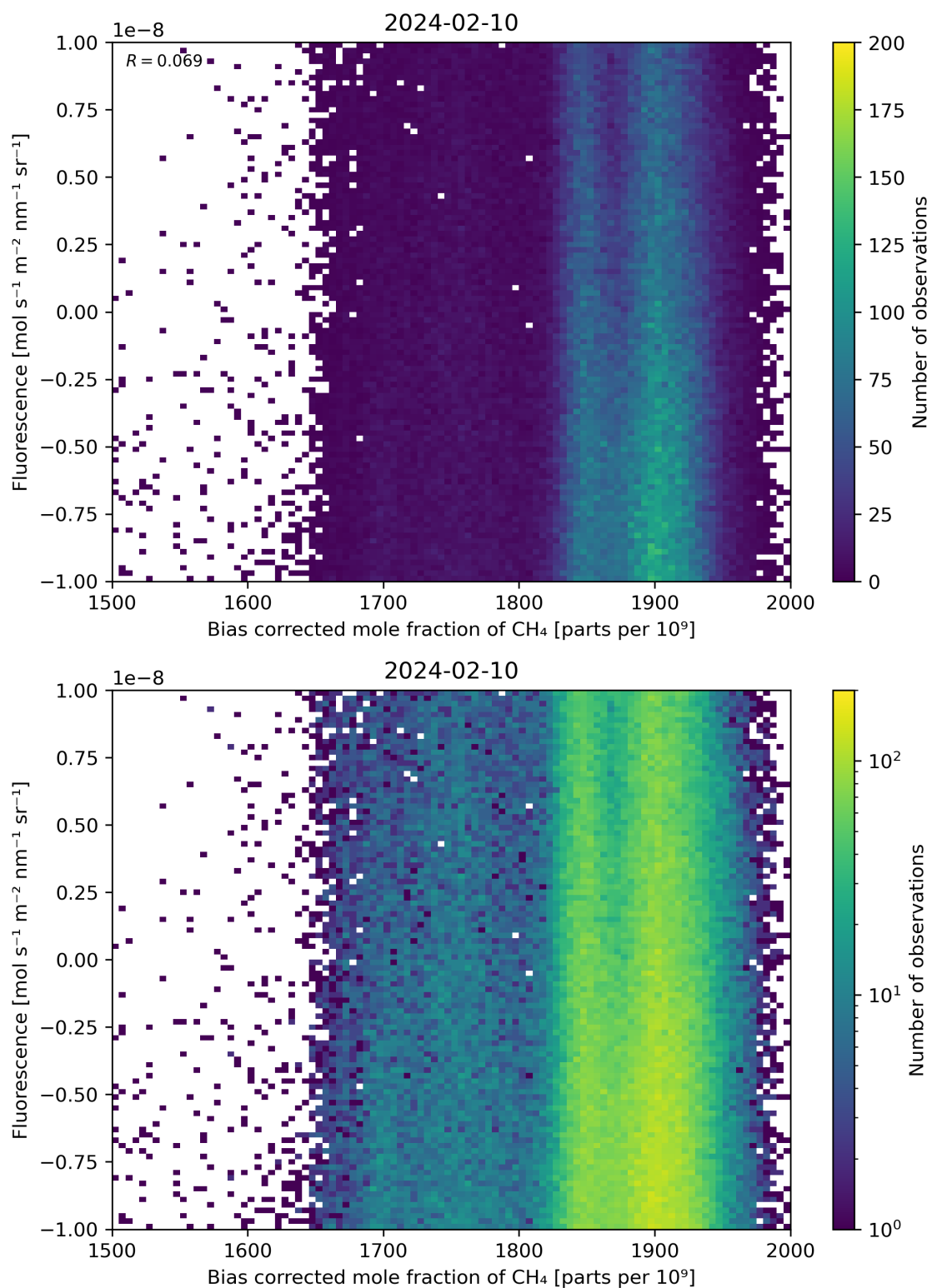
Figure 66: Scatter density plot of “Bias corrected mole fraction of \text{CH}_4 ” against “Fluorescence” for 2024-02-09 to 2024-02-11.
