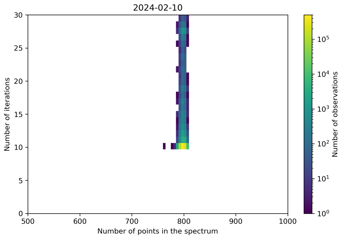
Figure 92: Scatter density plot of “Number of points in the spectrum” against “Number of iterations” for 2024-02-09 to 2024-02-11.
