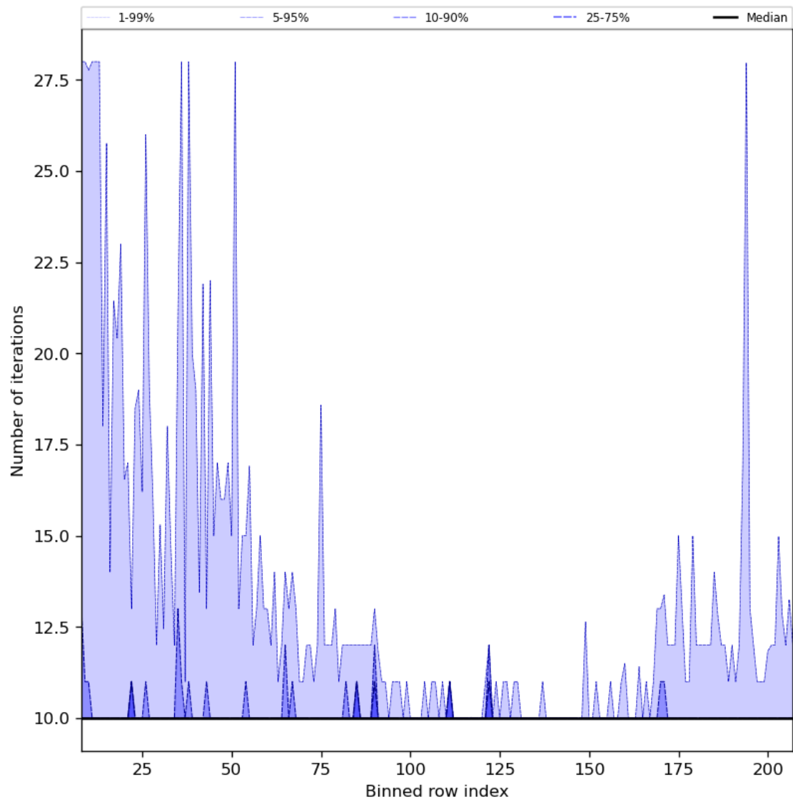
Figure 42: Along track statistics of “Number of iterations” for 2024-02-09 to 2024-02-11
