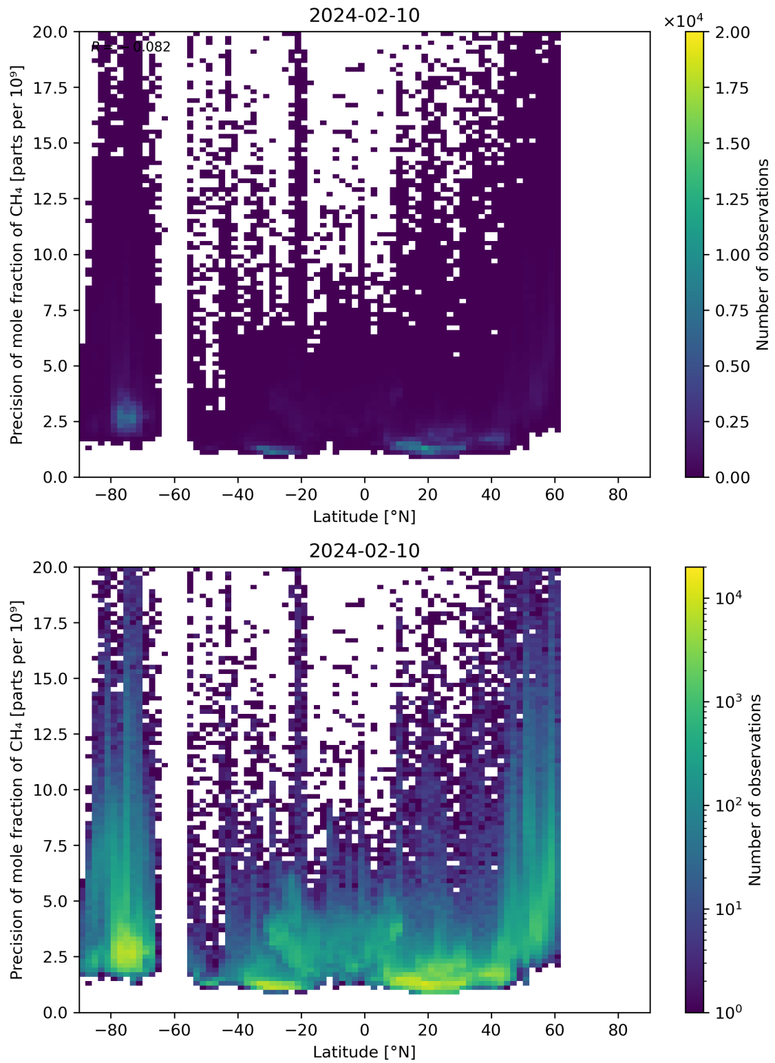
Figure 59: Scatter density plot of “Latitude” against “Precision of mole fraction of CH 4 ” for 2024-02-09 to 2024-02-11.
