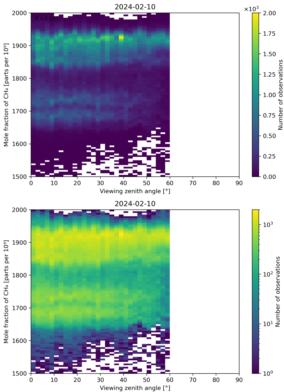
Figure 110: Scatter density plot of “Viewing zenith angle” against “Mole fraction of CH 4 ” for 2024-02-09 to 2024-02-11.
