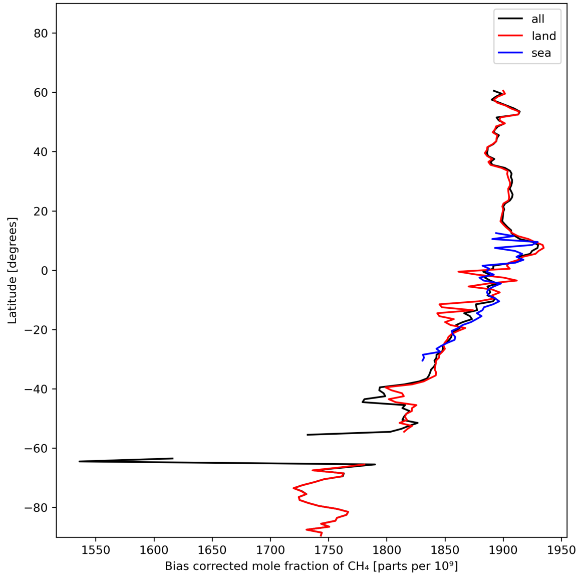
Figure 14: Zonal average of “Bias corrected mole fraction of CH 4 ” for 2024-02-09 to 2024-02-11.
