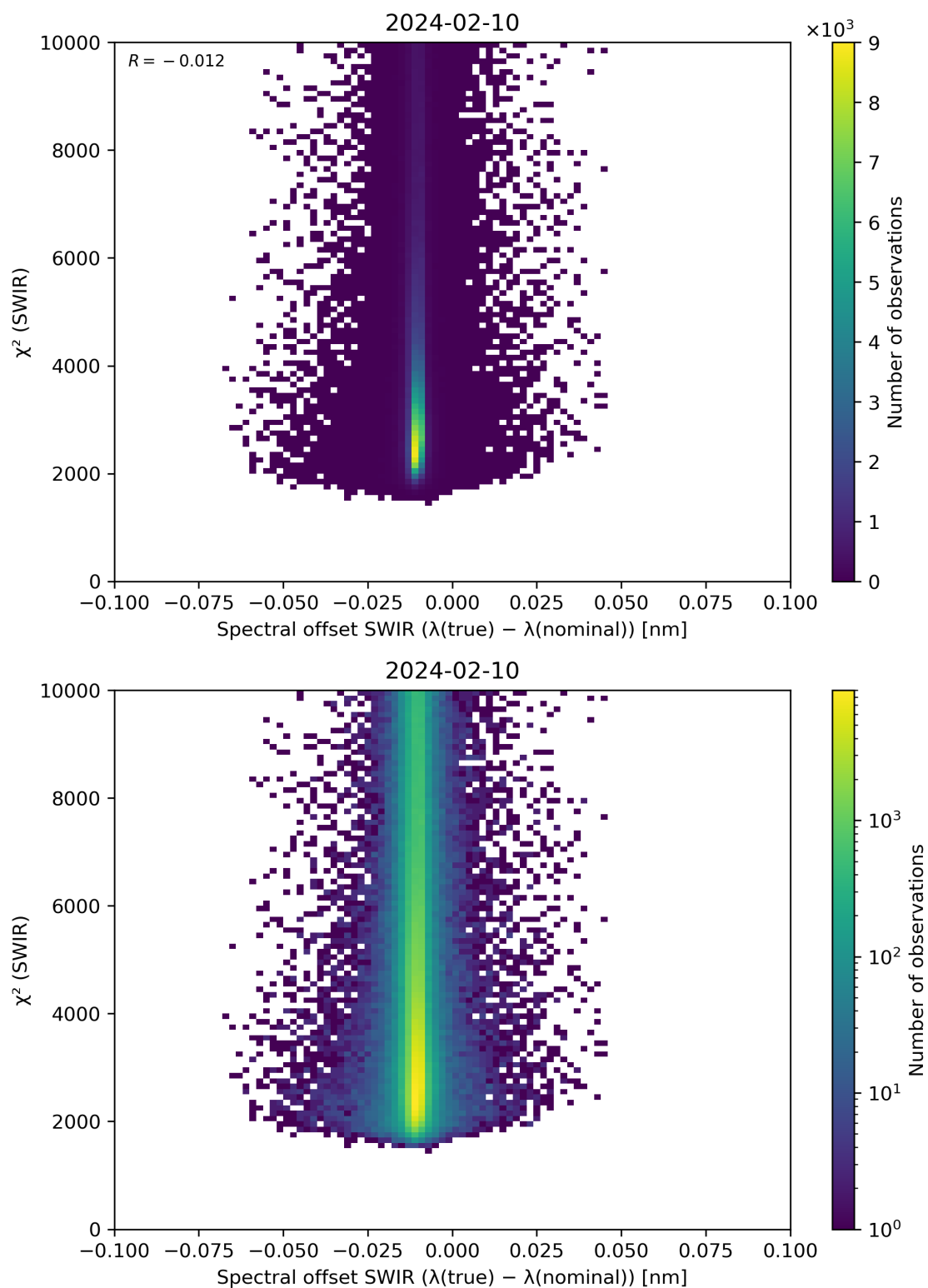
Figure 118: Scatter density plot of “Spectral offset SWIR ( \lambda(\text{true}) - \lambda(\text{nominal}) )” against “ \chi^2 (SWIR)” for 2024-02-09 to 2024-02-11.
