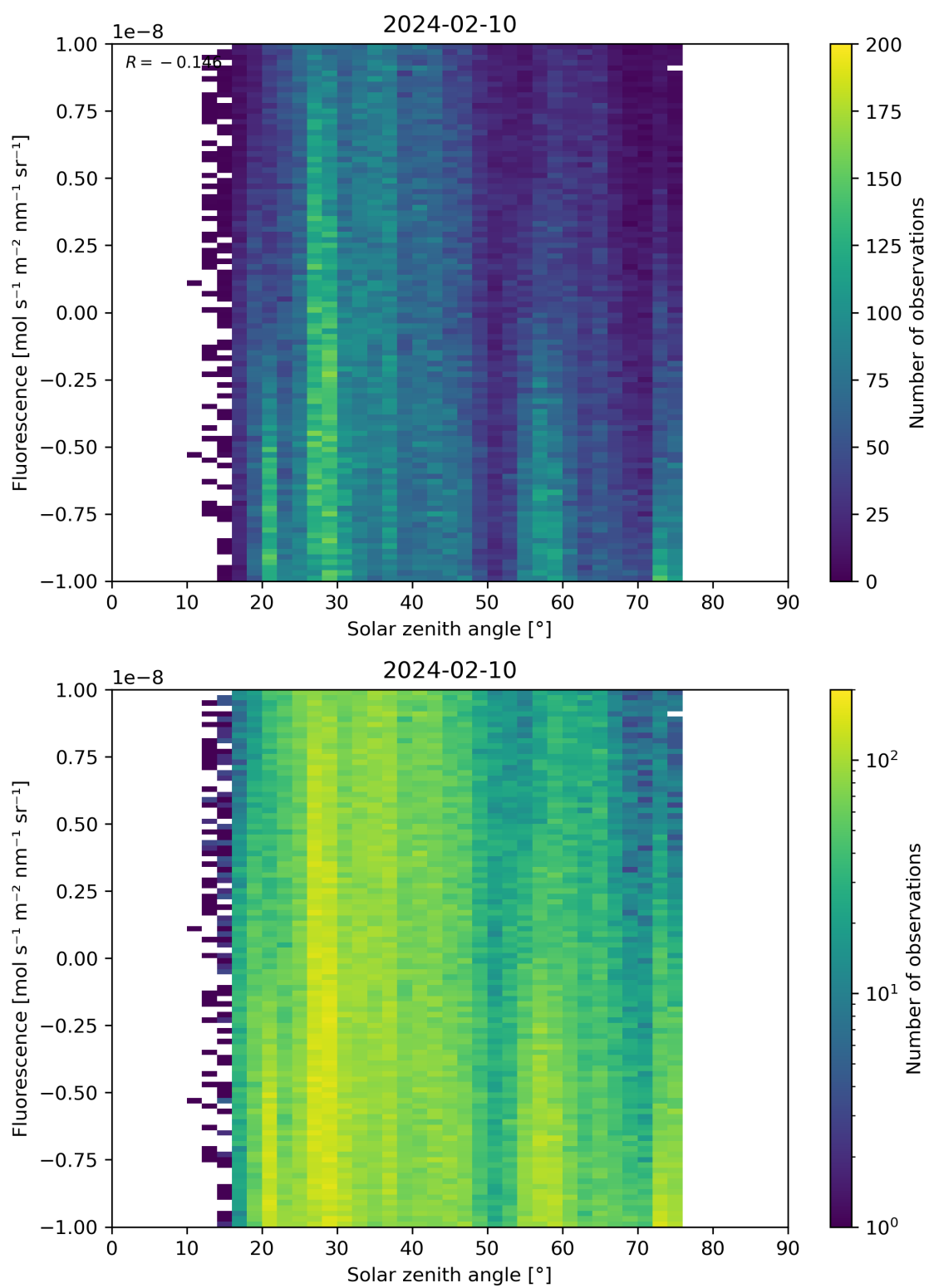
Figure 97: Scatter density plot of “Solar zenith angle” against “Fluorescence” for 2024-02-09 to 2024-02-11.
