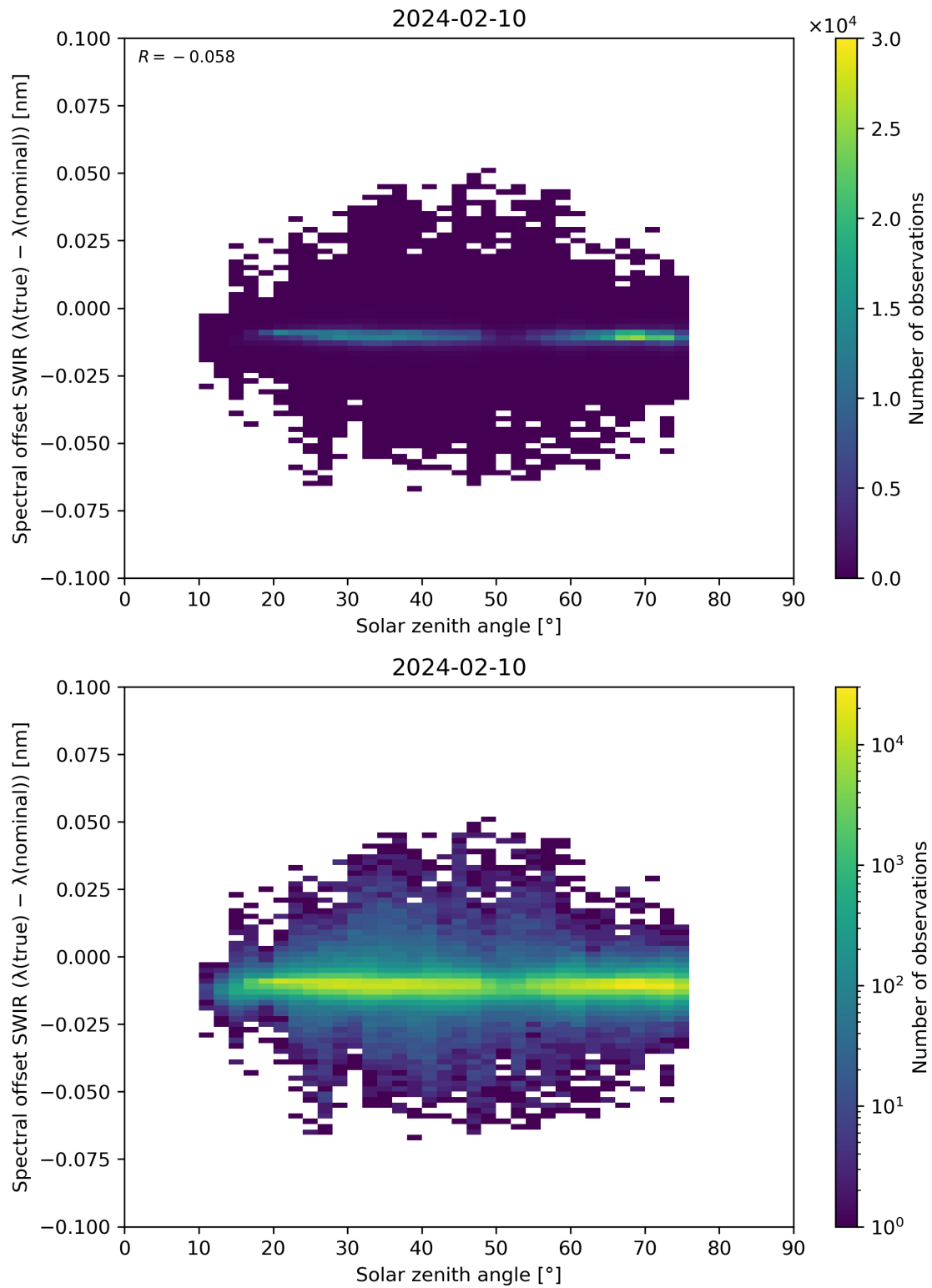
Figure 104: Scatter density plot of “Solar zenith angle” against “Spectral offset SWIR ( \lambda(\text{true}) - \lambda(\text{nominal}) )” for 2024-02-09 to 2024-02-11.
