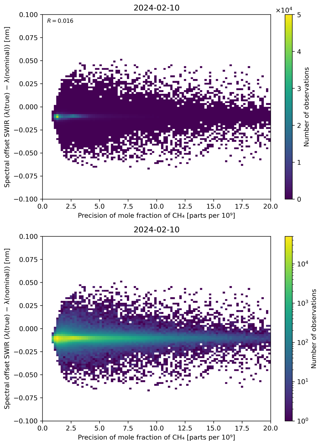
Figure 85: Scatter density plot of “Precision of mole fraction of CH 4 ” against “Spectral offset SWIR ( \lambda(\text{true}) - \lambda(\text{nominal}) )” for 2024-02-09 to 2024-02-11.
