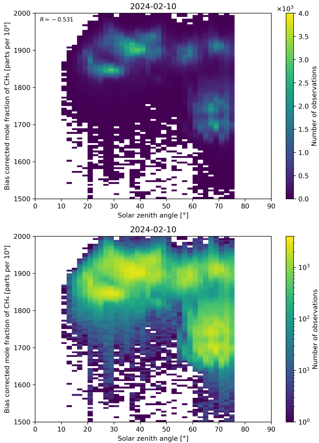
Figure 100: Scatter density plot of “Solar zenith angle” against “Bias corrected mole fraction of CH 4 ” for 2024-02-09 to 2024-02-11.
