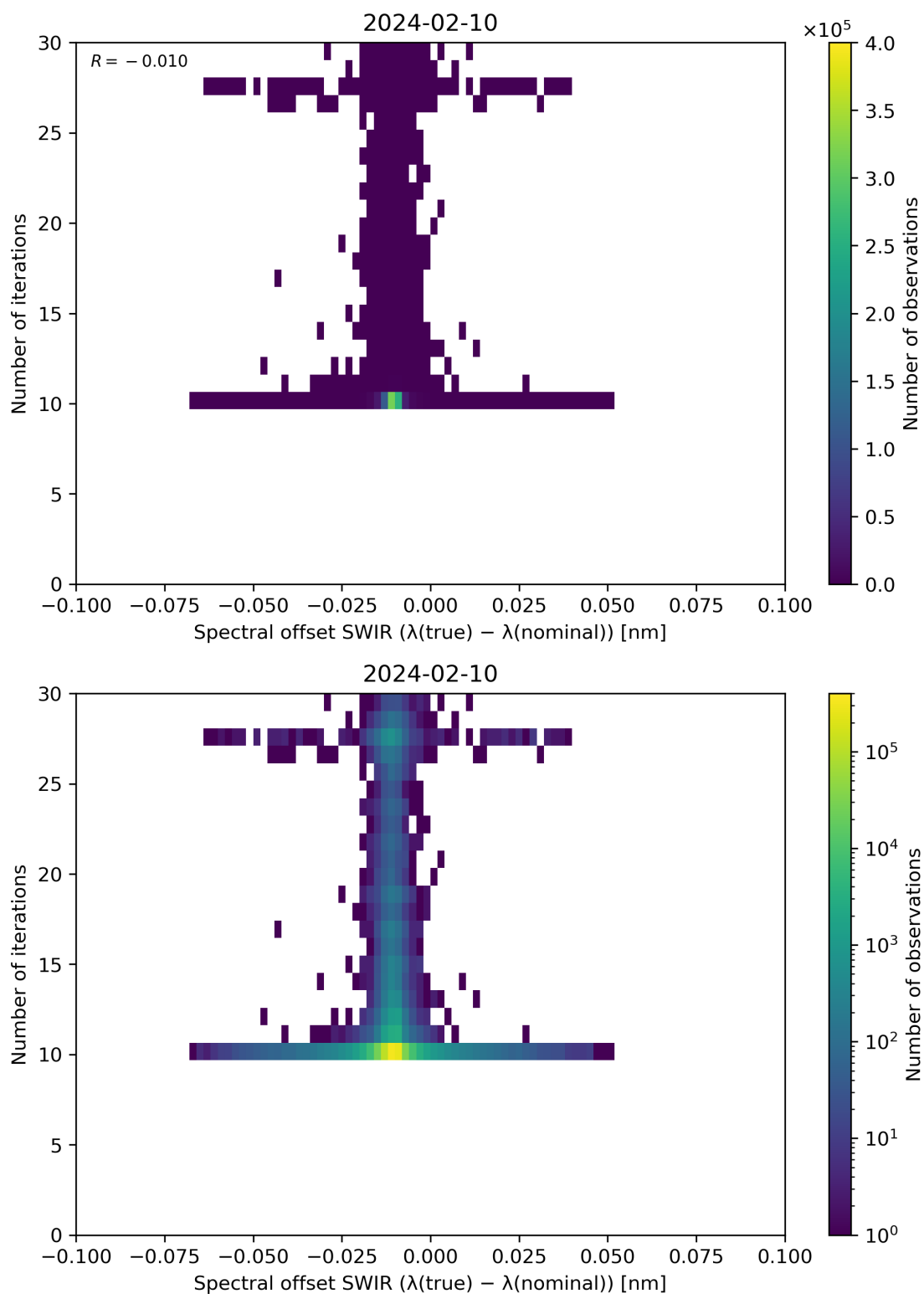
Figure 121: Scatter density plot of “Spectral offset SWIR ( \lambda(\text{true}) - \lambda(\text{nominal}) )” against “Number of iterations” for 2024-02-09 to 2024-02-11.
