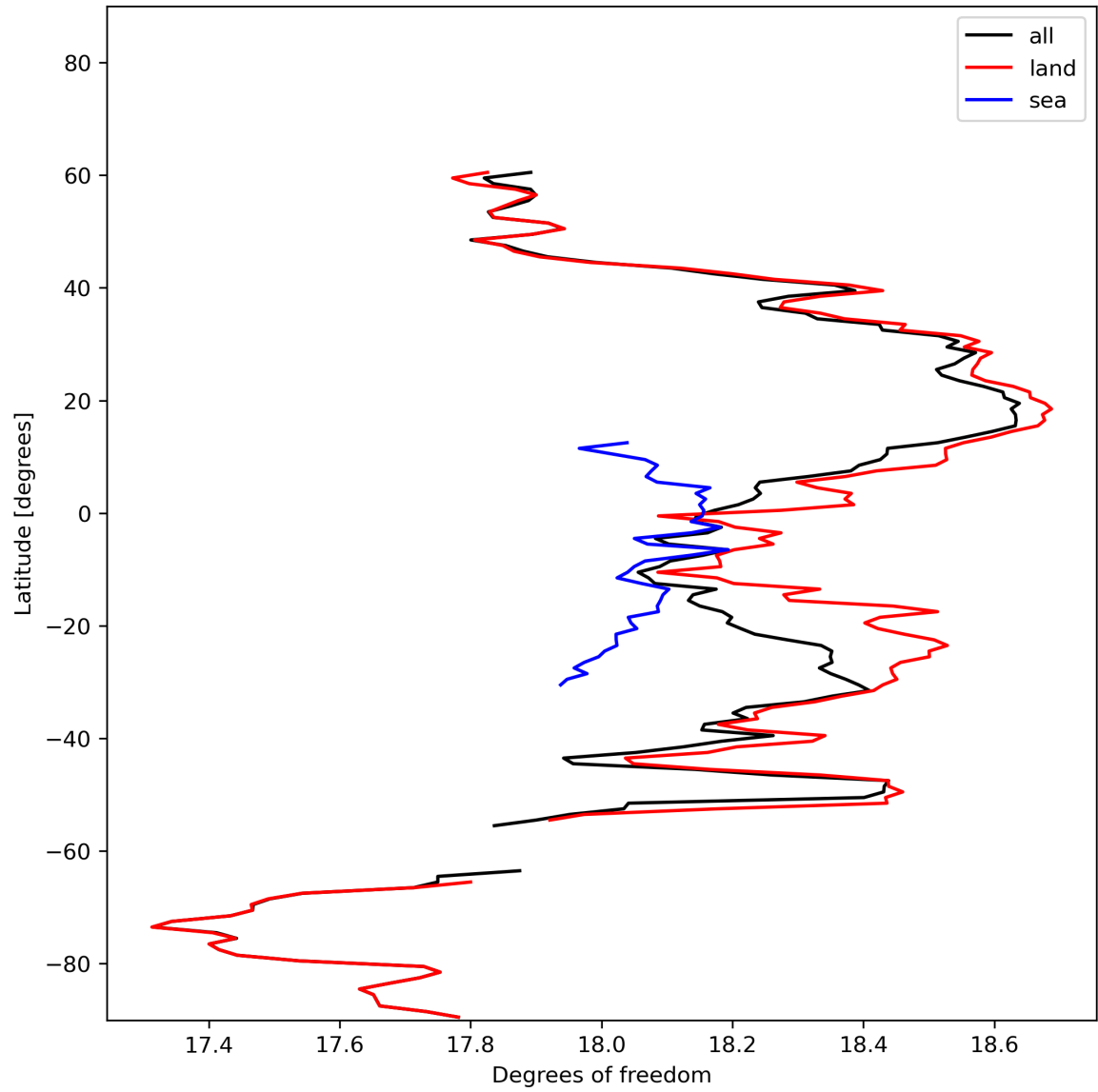
Figure 19: Zonal average of “Degrees of freedom” for 2024-02-09 to 2024-02-11.
