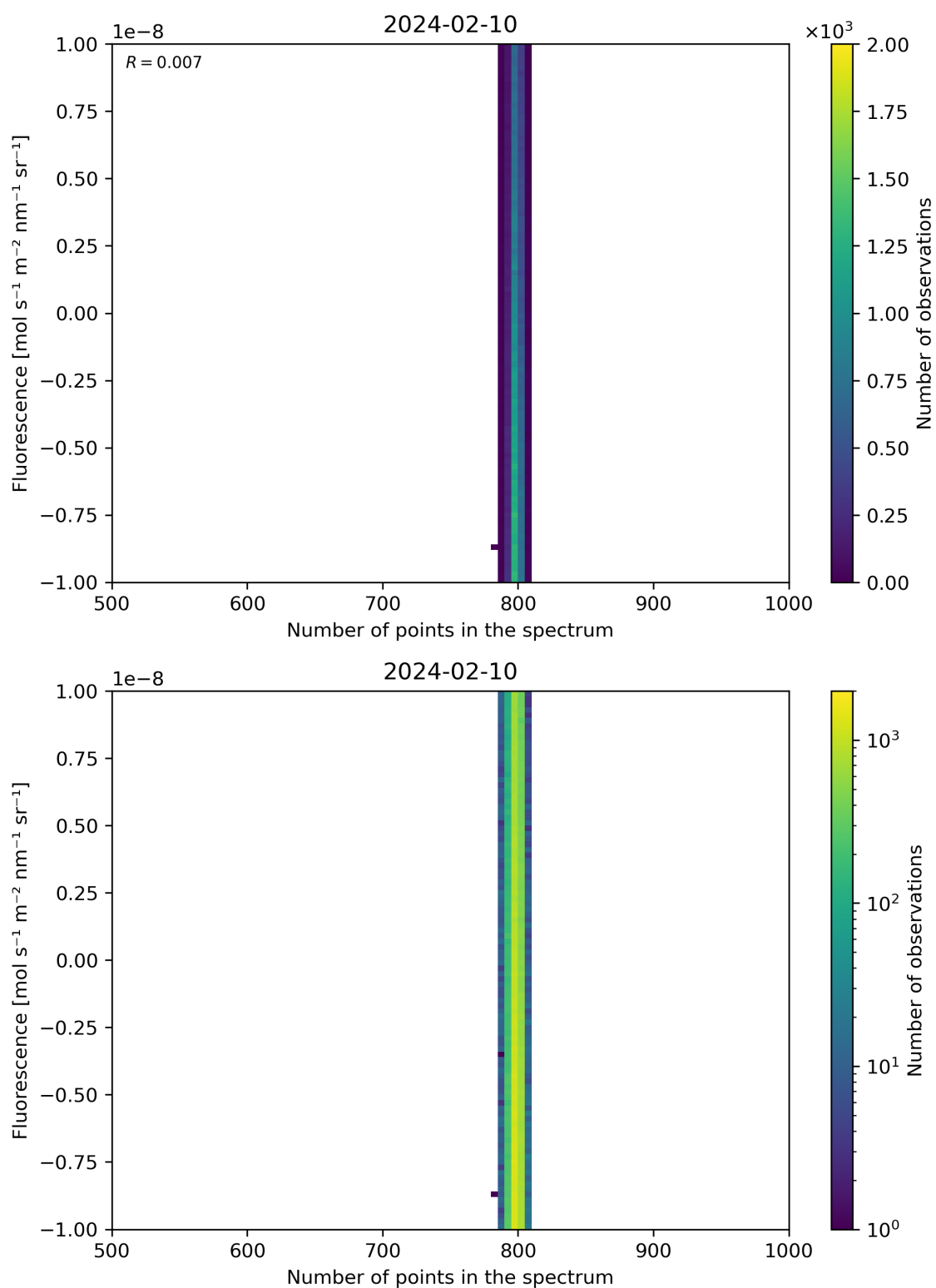
Figure 91: Scatter density plot of “Number of points in the spectrum” against “Fluorescence” for 2024-02-09 to 2024-02-11.
