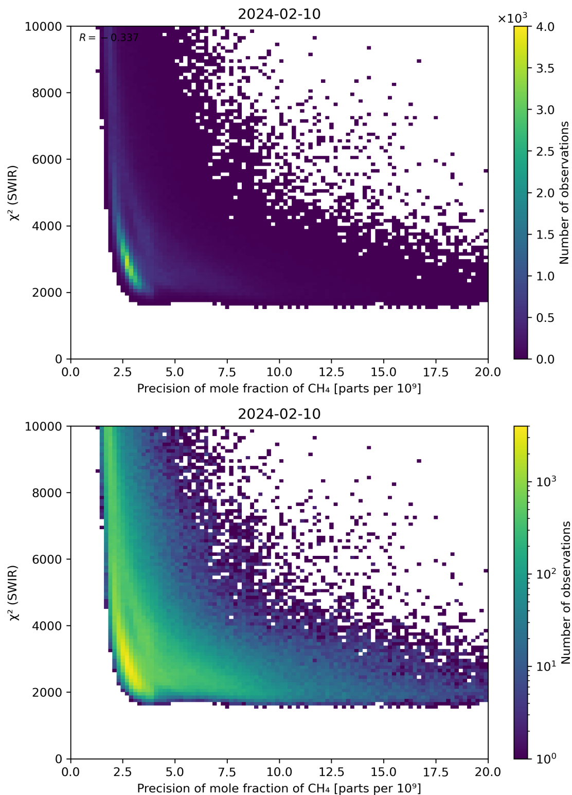
Figure 79: Scatter density plot of “Precision of mole fraction of CH 4 ” against “ \chi^2 (SWIR)” for 2024-02-09 to 2024-02-11.
