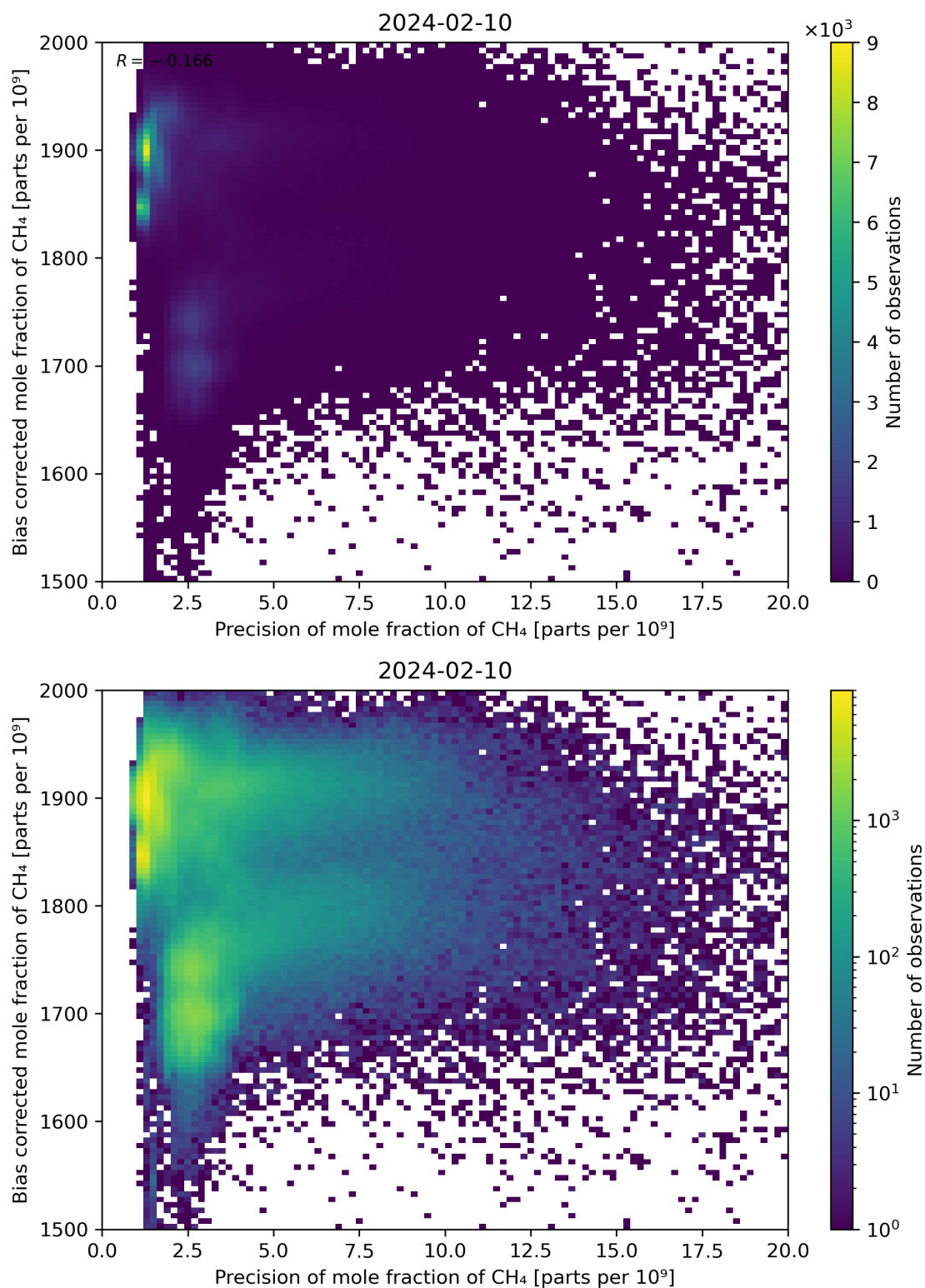
Figure 82: Scatter density plot of “Precision of mole fraction of CH 4 ” against “Bias corrected mole fraction of CH 4 ” for 2024-02-09 to 2024-02-11.
