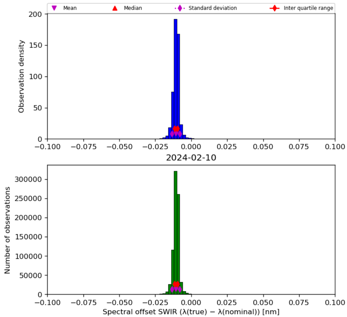
Figure 27: Histogram of “Spectral offset SWIR ( \lambda(\text{true}) - \lambda(\text{nominal}) )” for 2024-02-09 to 2024-02-11
