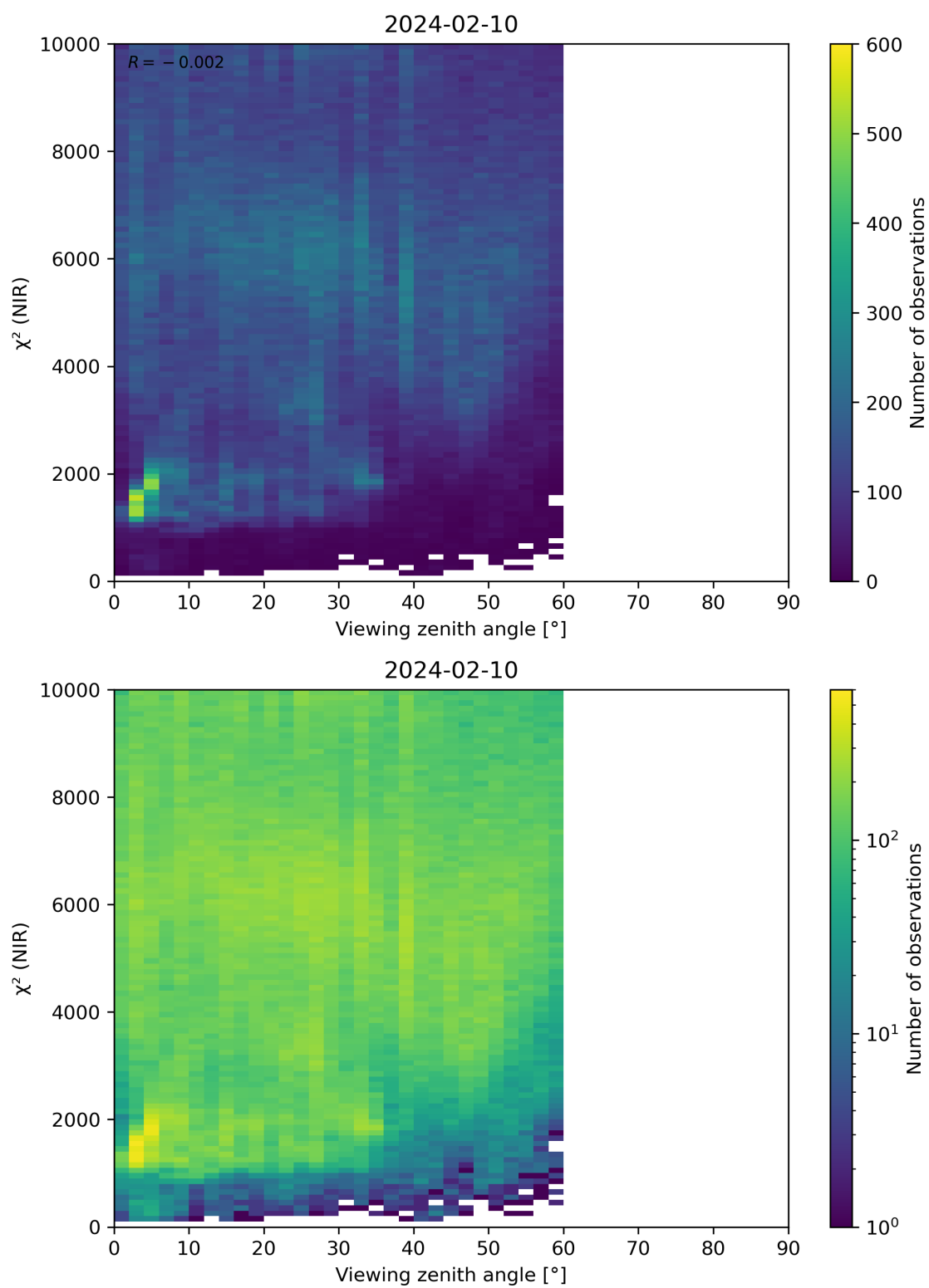
Figure 105: Scatter density plot of “Viewing zenith angle” against “ \chi^2 (NIR)” for 2024-02-09 to 2024-02-11.
