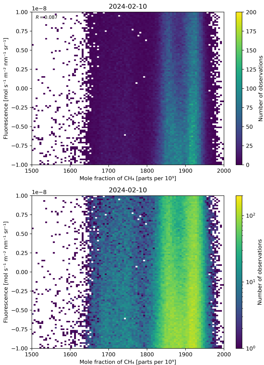
Figure 73: Scatter density plot of “Mole fraction of \text{CH}_4 ” against “Fluorescence” for 2024-02-09 to 2024-02-11.
