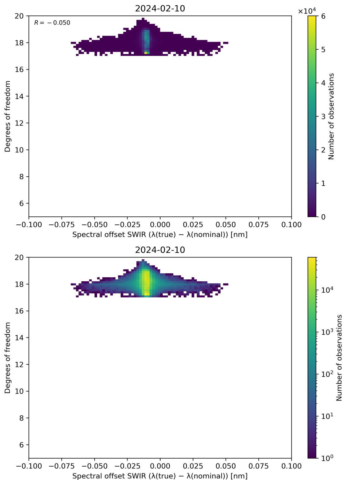
Figure 119: Scatter density plot of “Spectral offset SWIR ( \lambda(\text{true}) - \lambda(\text{nominal}) )” against “Degrees of freedom” for 2024-02-09 to 2024-02-11.
