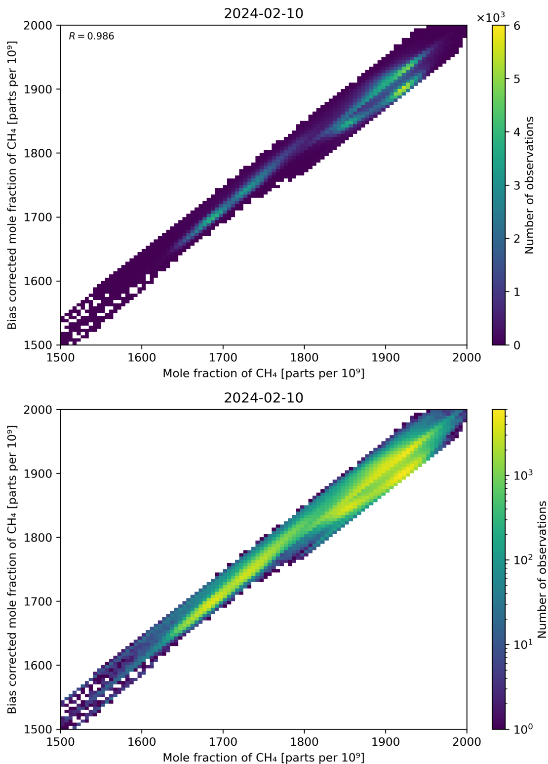
Figure 74: Scatter density plot of “Mole fraction of CH 4 ” against “Bias corrected mole fraction of CH 4 ” for 2024-02-09 to 2024-02-11.
