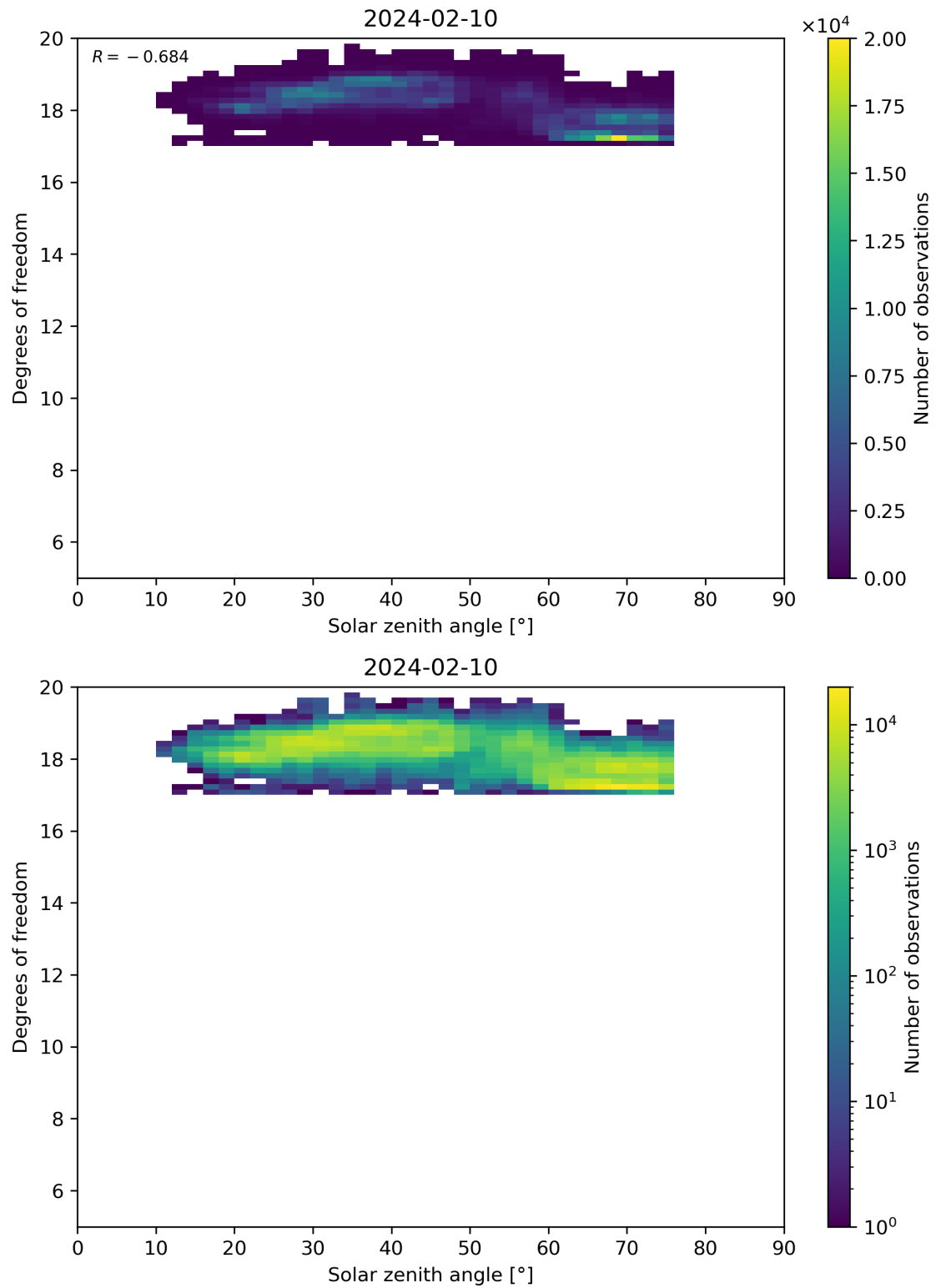
Figure 96: Scatter density plot of “Solar zenith angle” against “Degrees of freedom” for 2024-02-09 to 2024-02-11.
