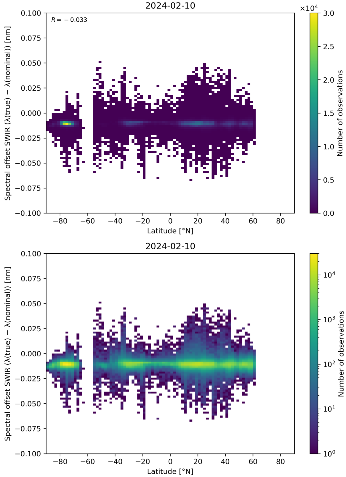
Figure 62: Scatter density plot of “Latitude” against “Spectral offset SWIR ( \lambda(\text{true}) - \lambda(\text{nominal}) )” for 2024-02-09 to 2024-02-11.
