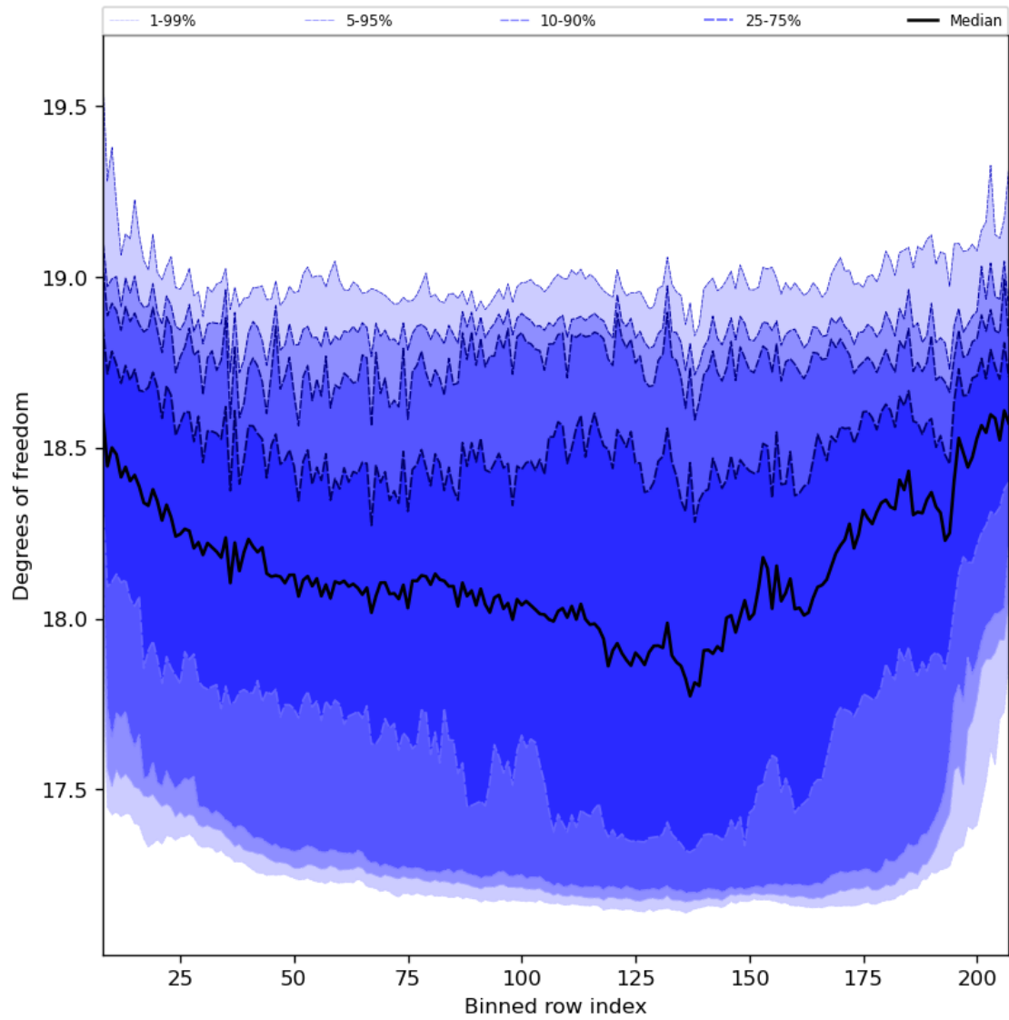
Figure 41: Along track statistics of “Degrees of freedom” for 2024-02-09 to 2024-02-11
