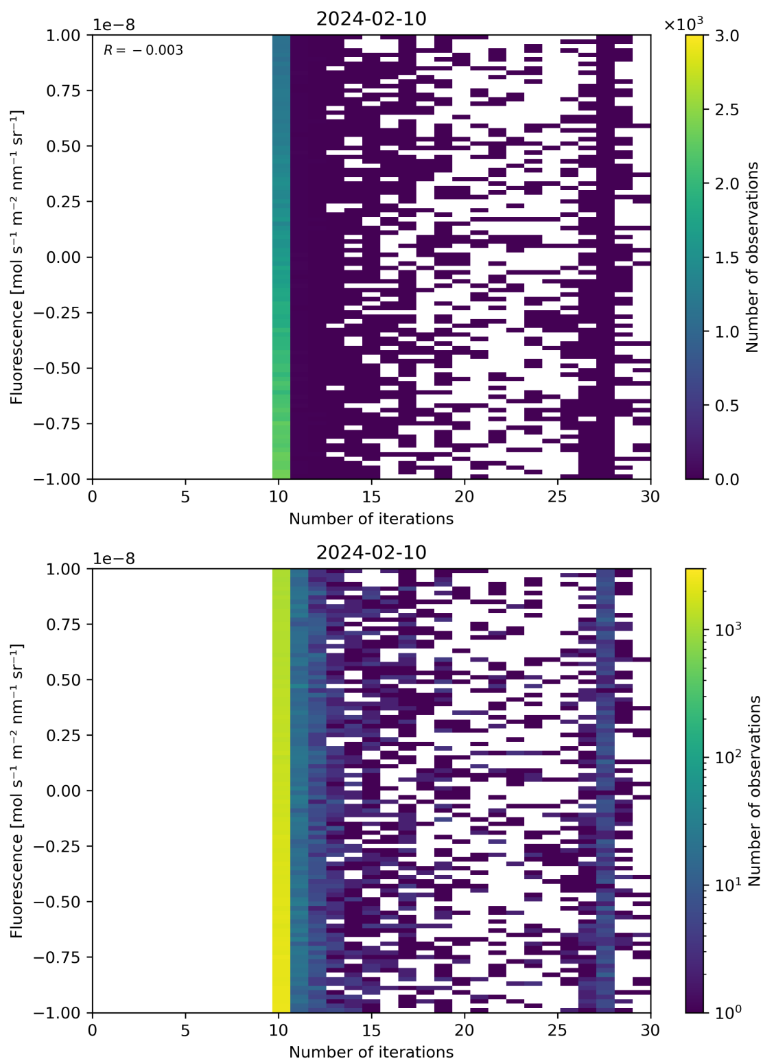
Figure 87: Scatter density plot of “Number of iterations” against “Fluorescence” for 2024-02-09 to 2024-02-11.
