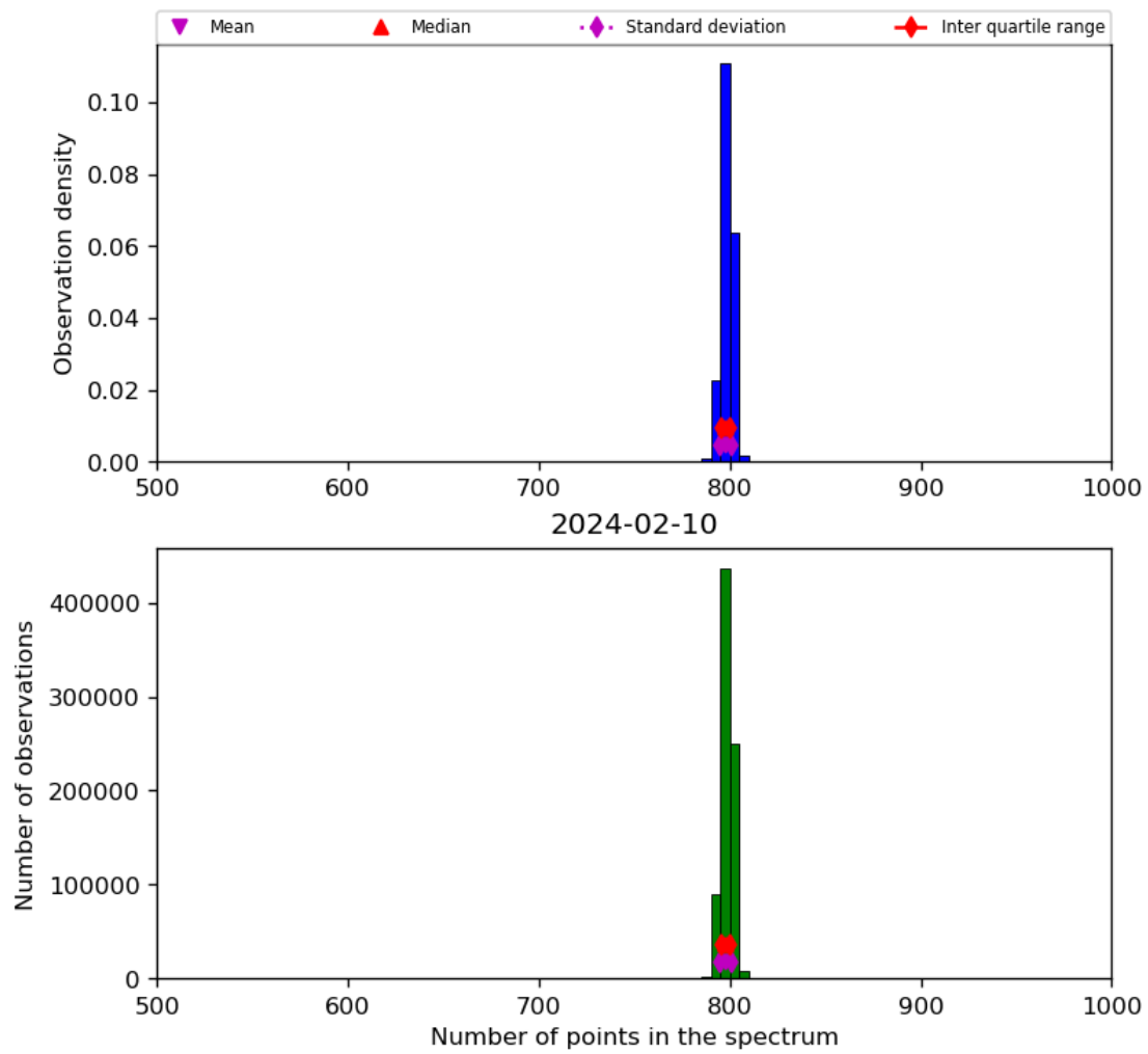
Figure 26: Histogram of “Number of points in the spectrum” for 2024-02-09 to 2024-02-11
