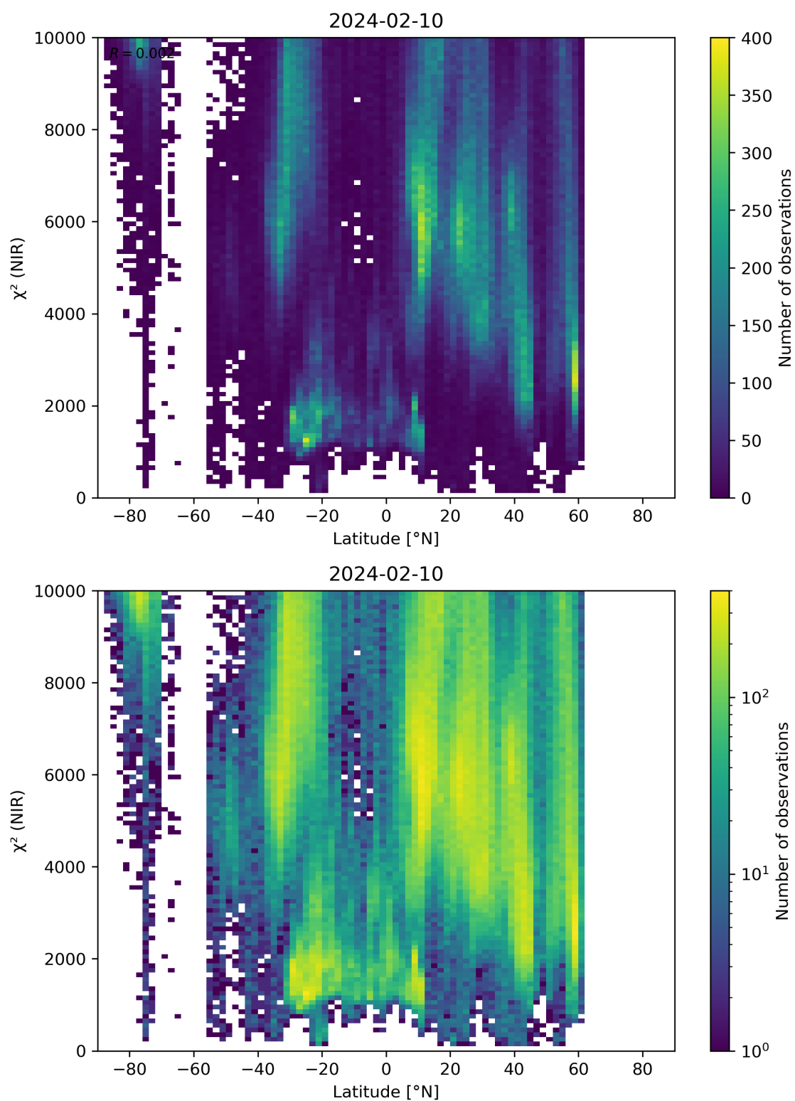
Figure 53: Scatter density plot of “Latitude” against “ \chi^2 (NIR)” for 2024-02-09 to 2024-02-11.
