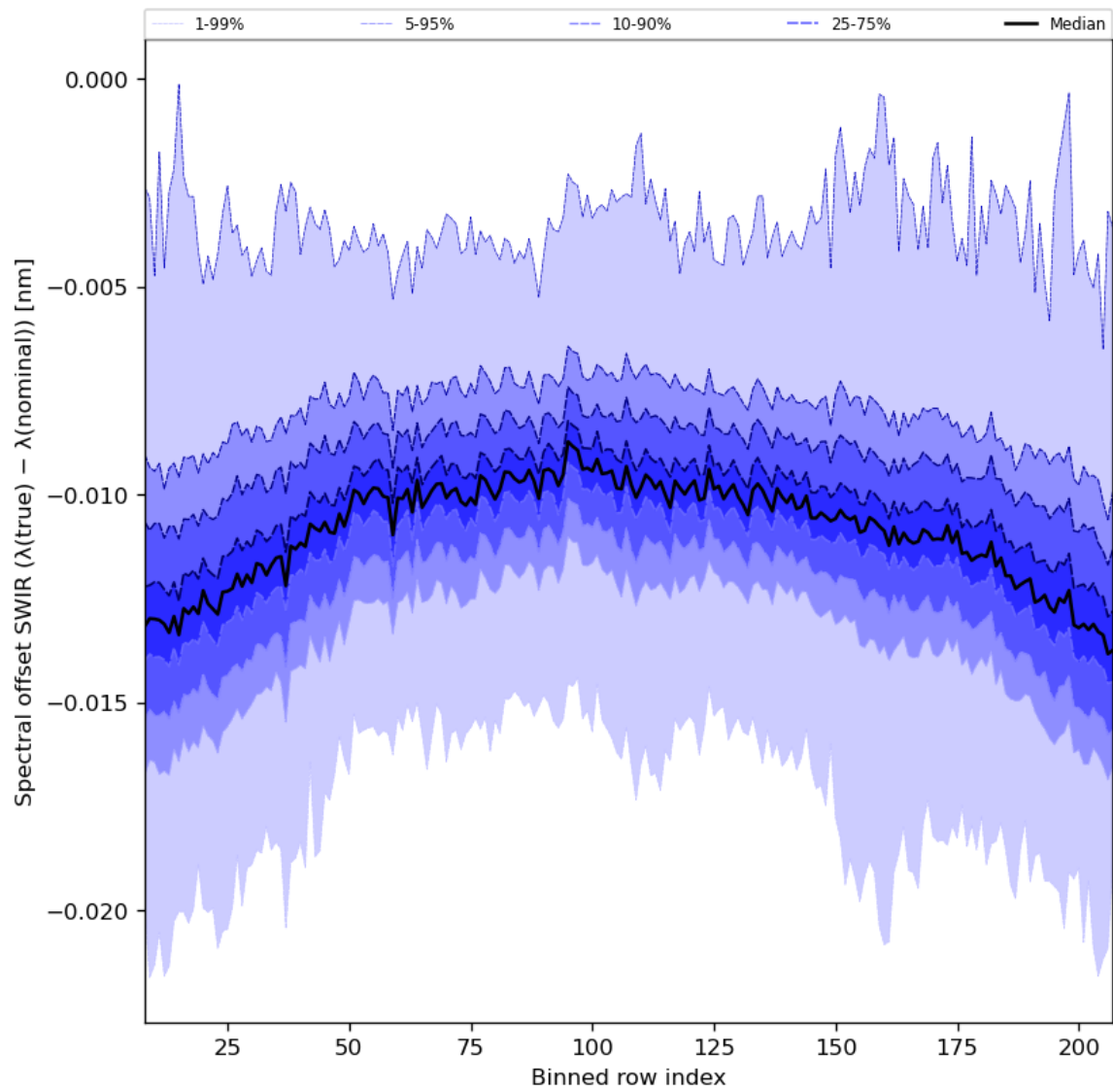
Figure 38: Along track statistics of “Spectral offset SWIR ( \lambda(\text{true}) - \lambda(\text{nominal}) )” for 2024-02-09 to 2024-02-11
