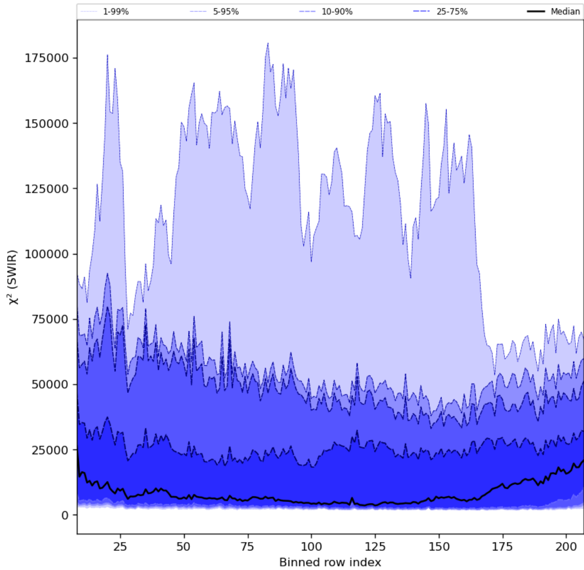
Figure 39: Along track statistics of “ \chi^2 (SWIR)” for 2024-02-09 to 2024-02-11
