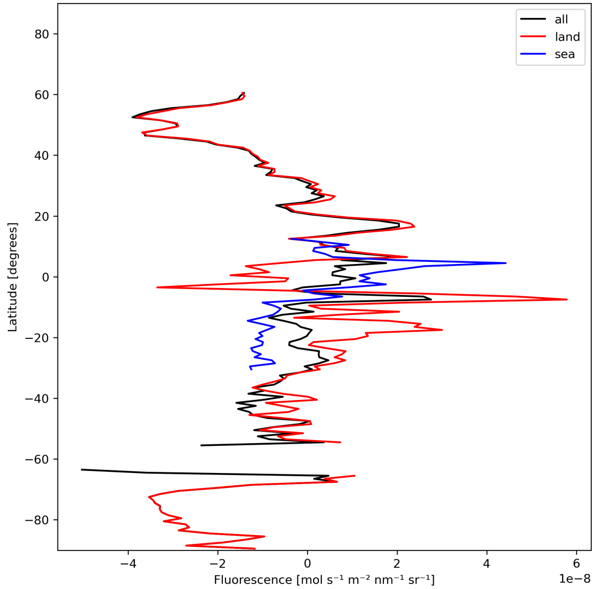
Figure 21: Zonal average of “Fluorescence” for 2024-02-09 to 2024-02-11.
