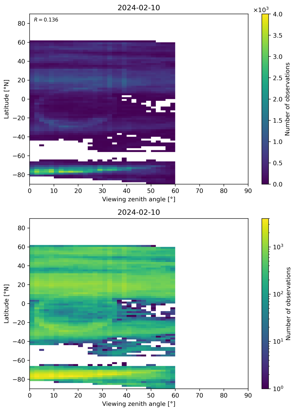
Figure 109: Scatter density plot of “Viewing zenith angle” against “Latitude” for 2024-02-09 to 2024-02-11.
