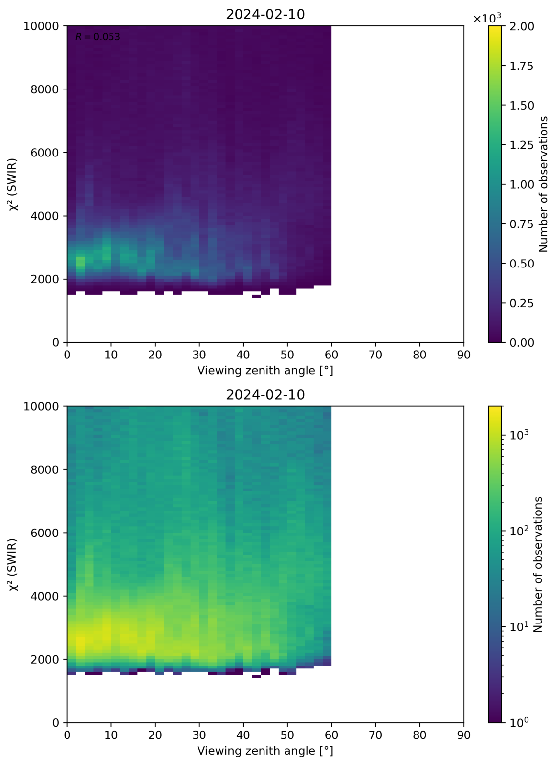
Figure 106: Scatter density plot of “Viewing zenith angle” against “ \chi^2 (SWIR)” for 2024-02-09 to 2024-02-11.
