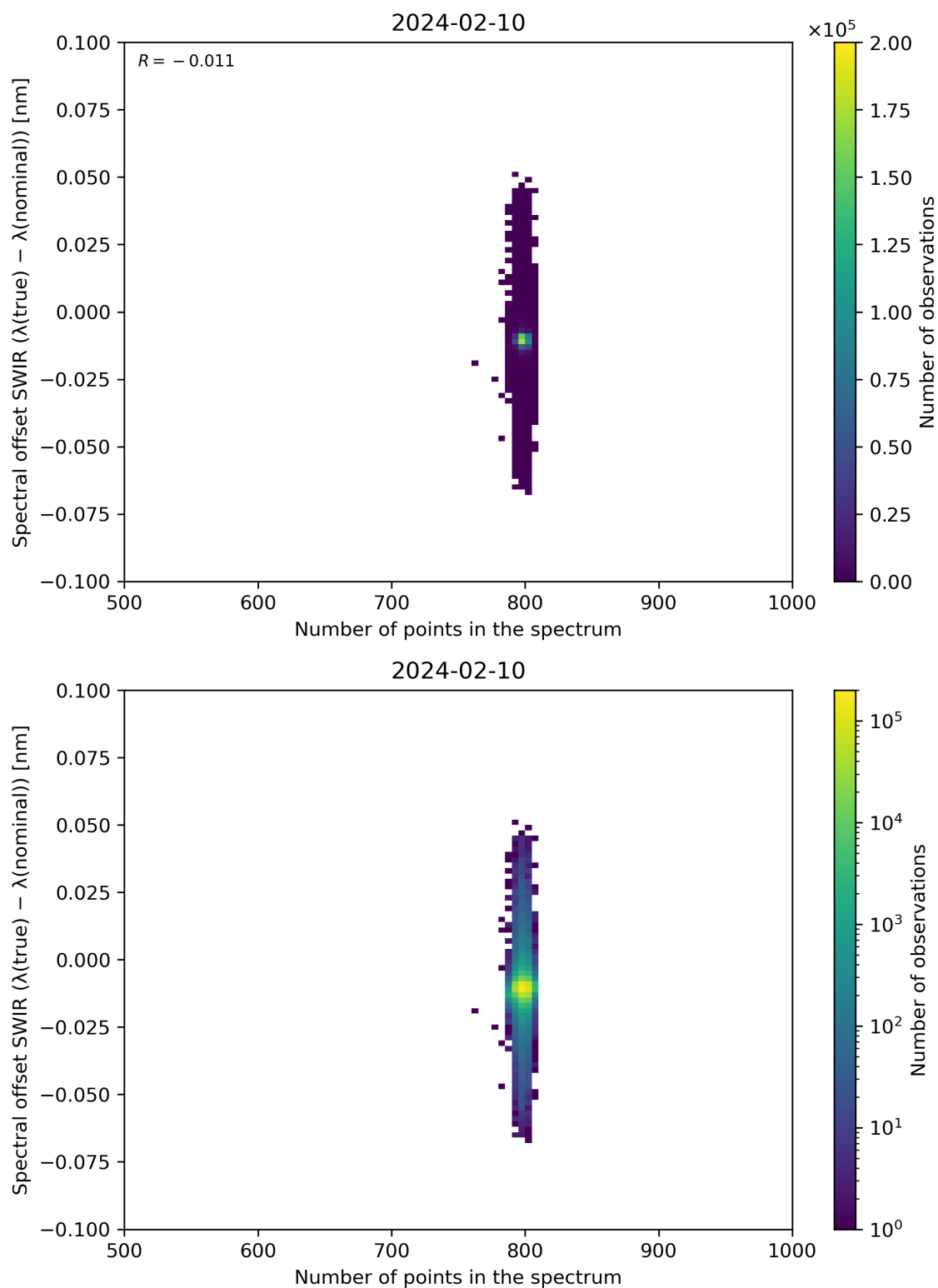
Figure 93: Scatter density plot of “Number of points in the spectrum” against “Spectral offset SWIR ( \lambda(\text{true}) - \lambda(\text{nominal}) )” for 2024-02-09 to 2024-02-11.
