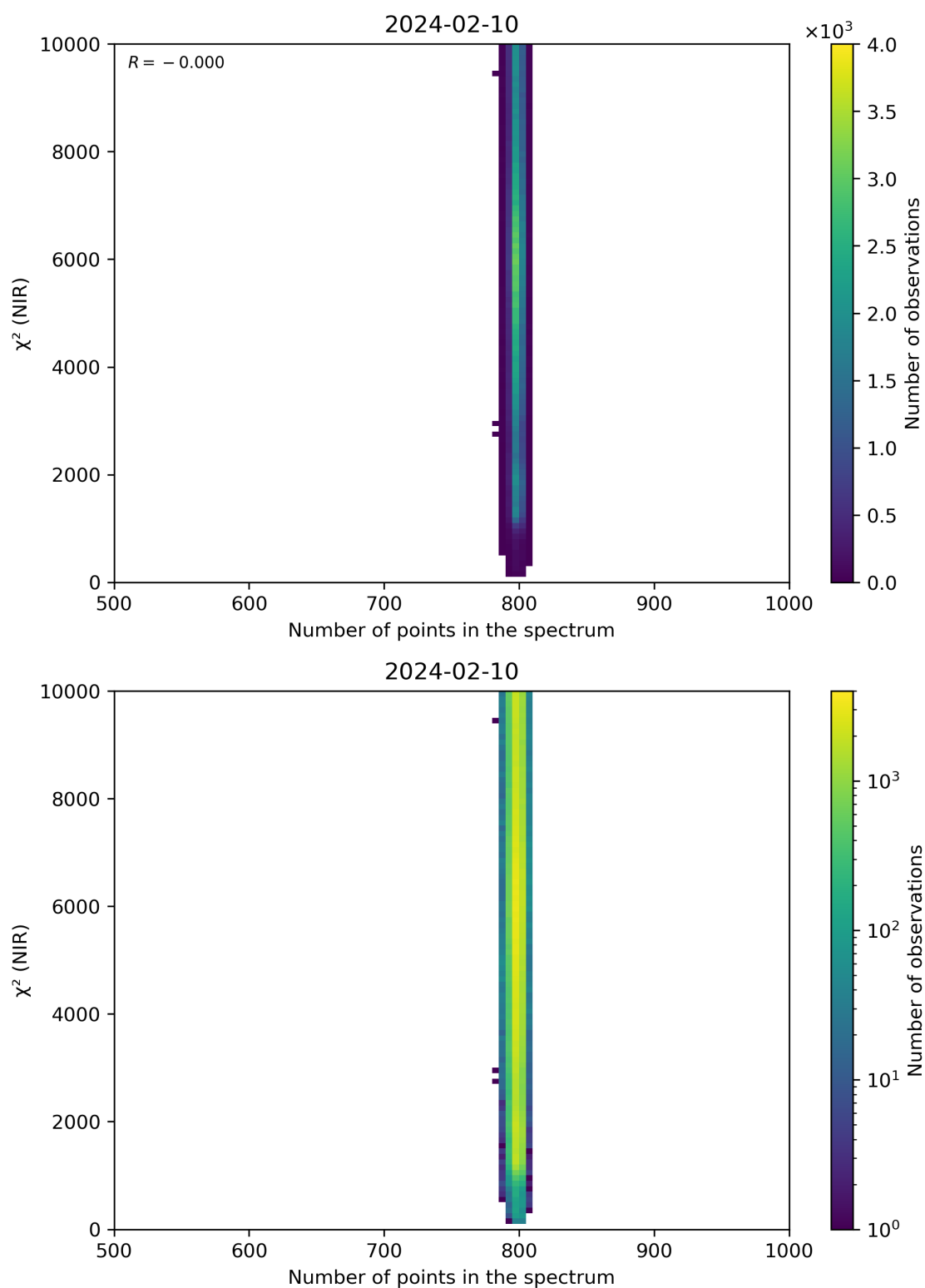
Figure 88: Scatter density plot of “Number of points in the spectrum” against “ \chi^2 (NIR)” for 2024-02-09 to 2024-02-11.
