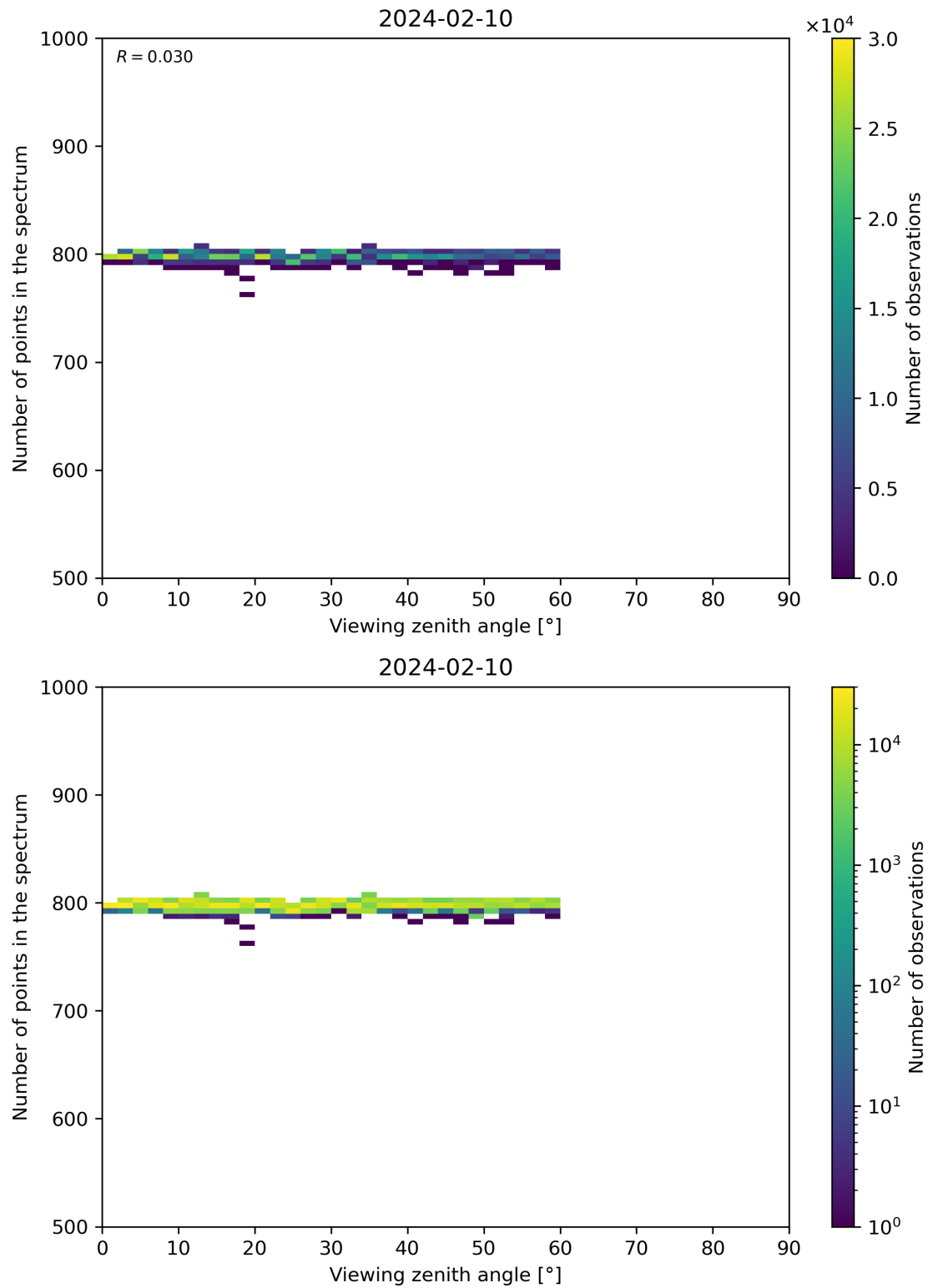
Figure 114: Scatter density plot of “Viewing zenith angle” against “Number of points in the spectrum” for 2024-02-09 to 2024-02-11.
