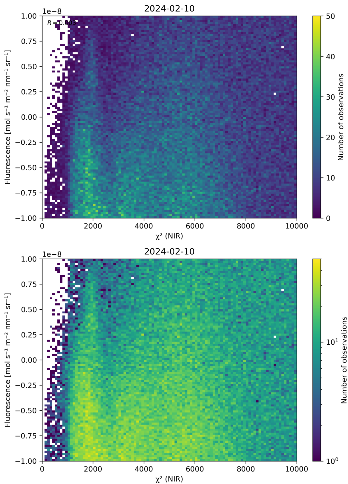
Figure 45: Scatter density plot of “ \chi^2 (NIR)” against “Fluorescence” for 2024-02-09 to 2024-02-11.
