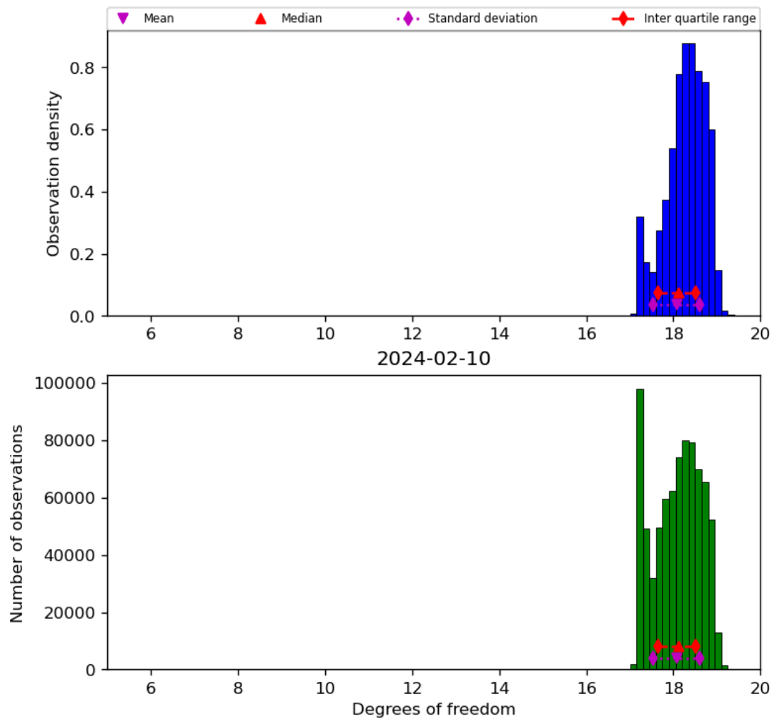
Figure 30: Histogram of “Degrees of freedom” for 2024-02-09 to 2024-02-11
