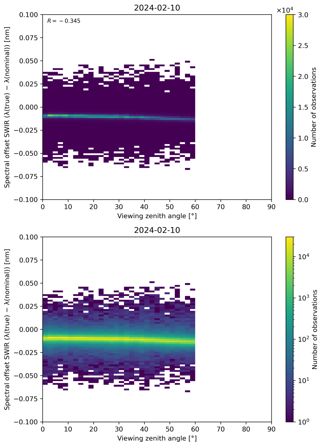
Figure 116: Scatter density plot of “Viewing zenith angle” against “Spectral offset SWIR ( \lambda(\text{true}) - \lambda(\text{nominal}) )” for 2024-02-09 to 2024-02-11.
