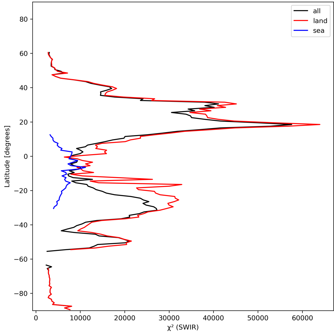
Figure 17: Zonal average of “ \chi^2 (SWIR)” for 2024-02-09 to 2024-02-11.
