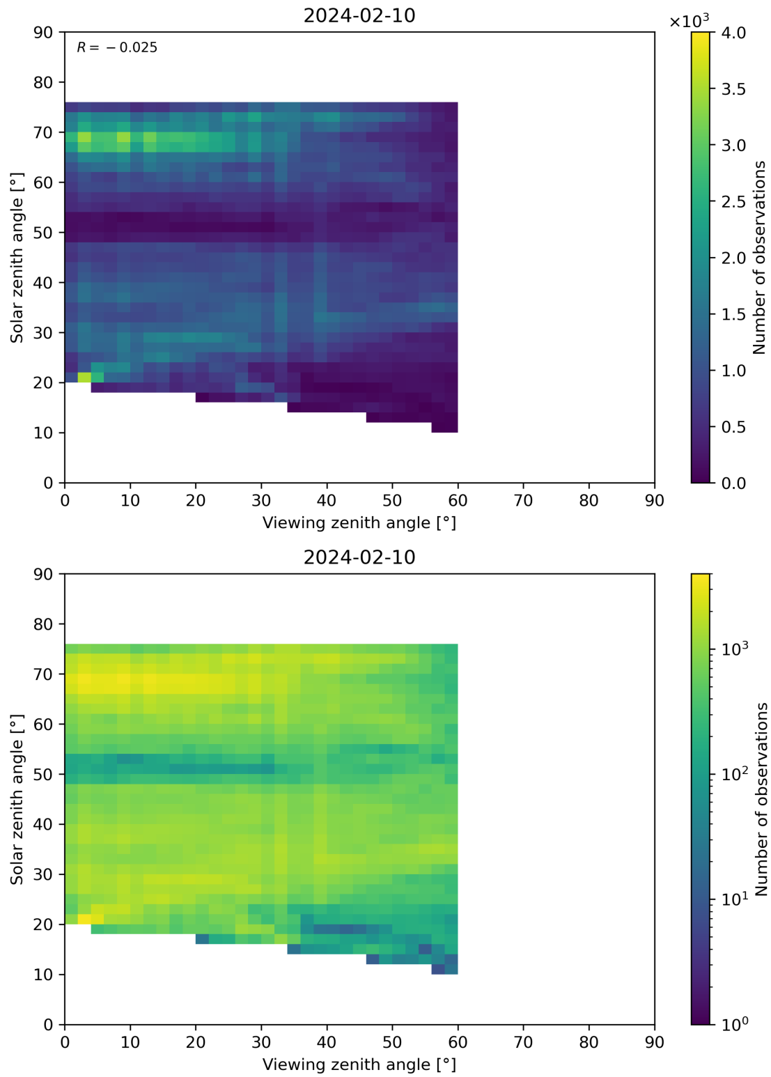
Figure 115: Scatter density plot of “Viewing zenith angle” against “Solar zenith angle” for 2024-02-09 to 2024-02-11.
