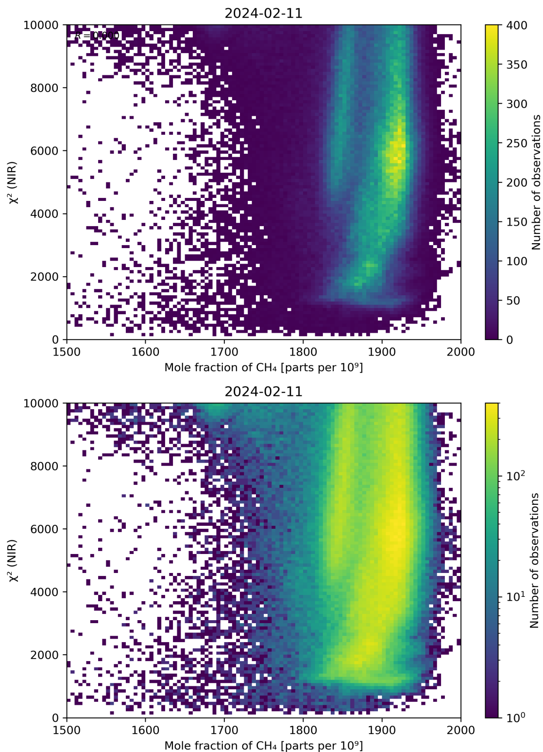
Figure 70: Scatter density plot of “Mole fraction of \text{CH}_4 ” against “ \chi^2 (NIR)” for 2024-02-11 to 2024-02-12.
