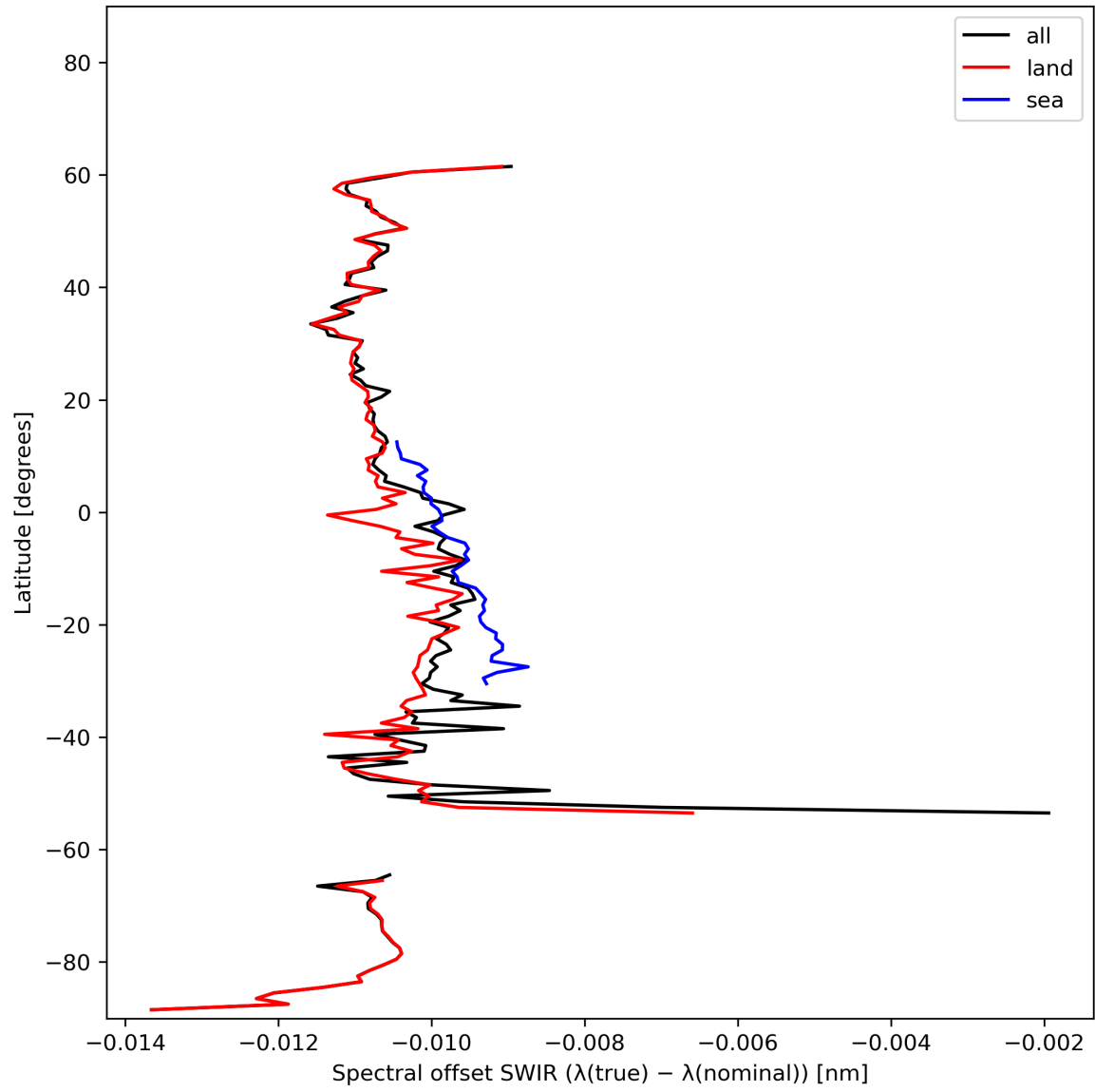
Figure 16: Zonal average of “Spectral offset SWIR ( \lambda(\text{true}) - \lambda(\text{nominal}) )” for 2024-02-11 to 2024-02-12.
