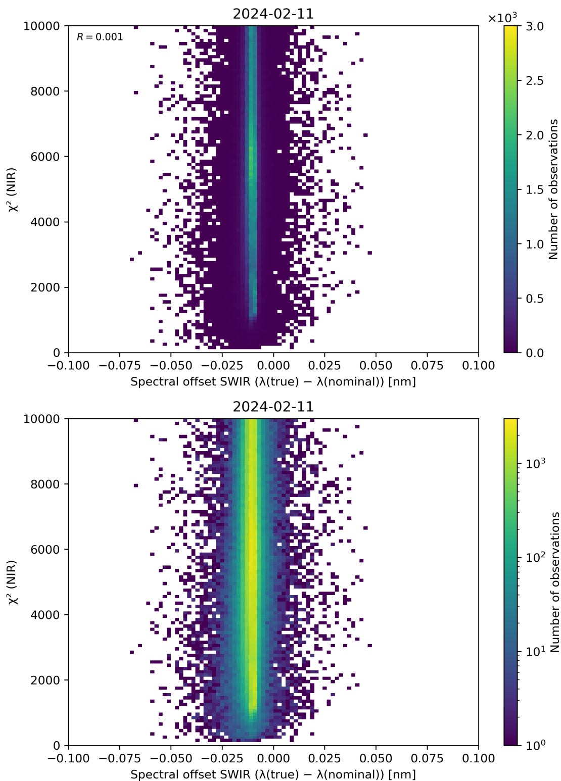
Figure 117: Scatter density plot of “Spectral offset SWIR ( \lambda(\text{true}) - \lambda(\text{nominal}) )” against “ \chi^2 (NIR)” for 2024-02-11 to 2024-02-12.
