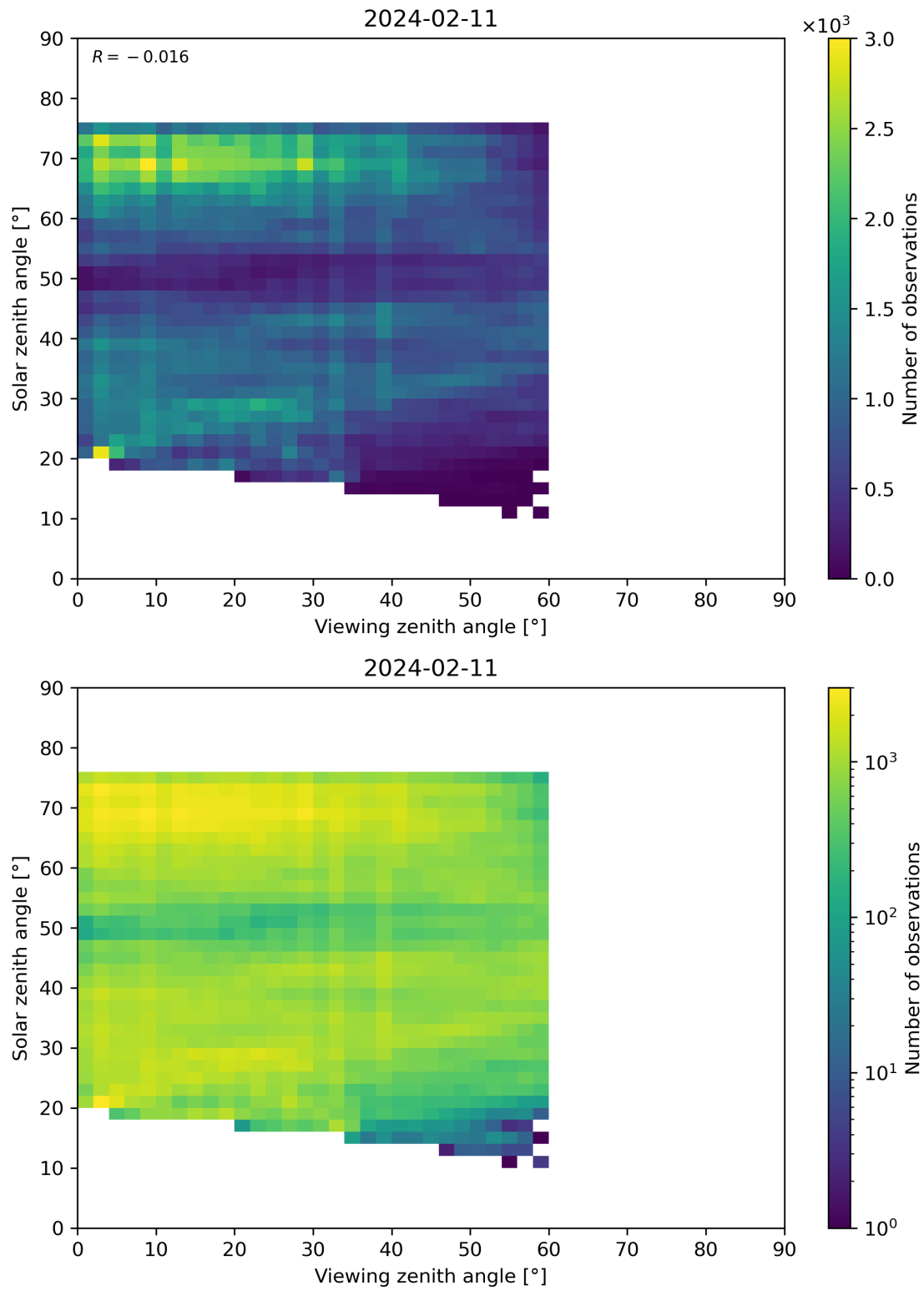
Figure 115: Scatter density plot of “Viewing zenith angle” against “Solar zenith angle” for 2024-02-11 to 2024-02-12.
