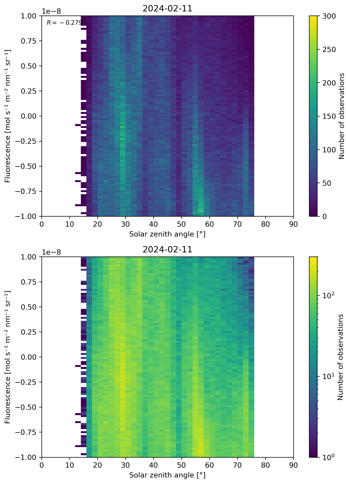
Figure 97: Scatter density plot of “Solar zenith angle” against “Fluorescence” for 2024-02-11 to 2024-02-12.
