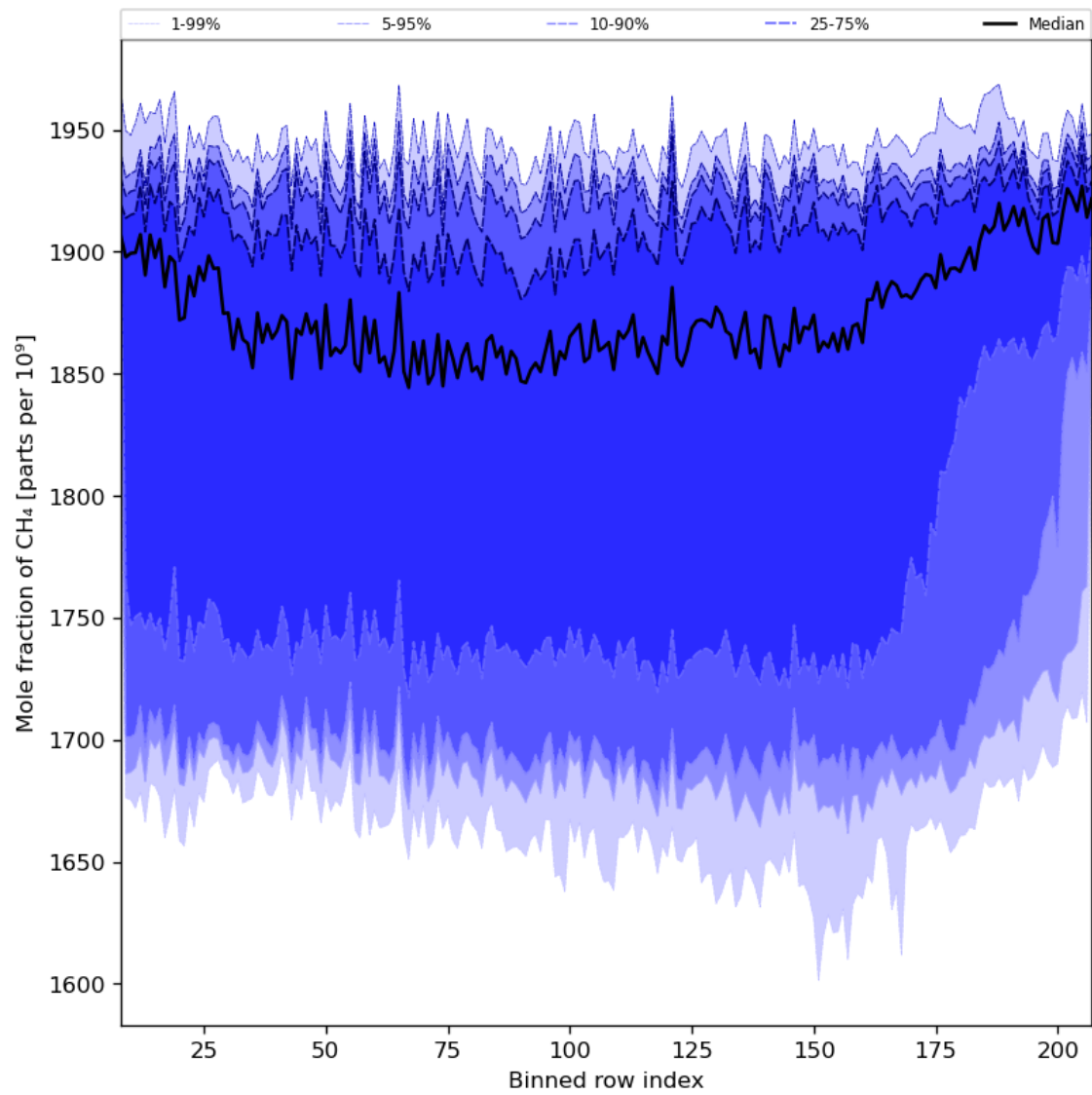
Figure 34: Along track statistics of “Mole fraction of CH 4 ” for 2024-02-11 to 2024-02-12
