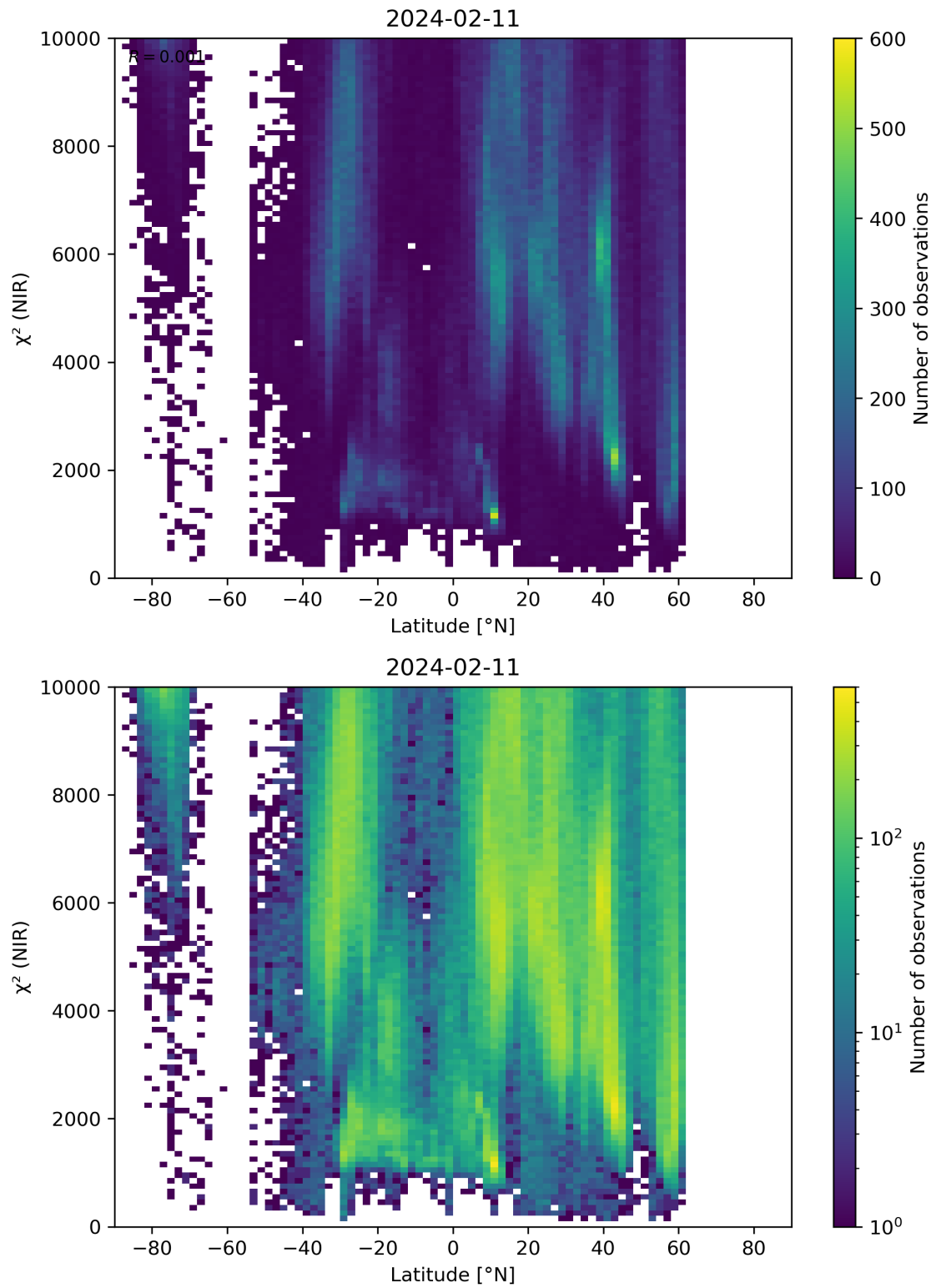
Figure 53: Scatter density plot of “Latitude” against “ \chi^2 (NIR)” for 2024-02-11 to 2024-02-12.
