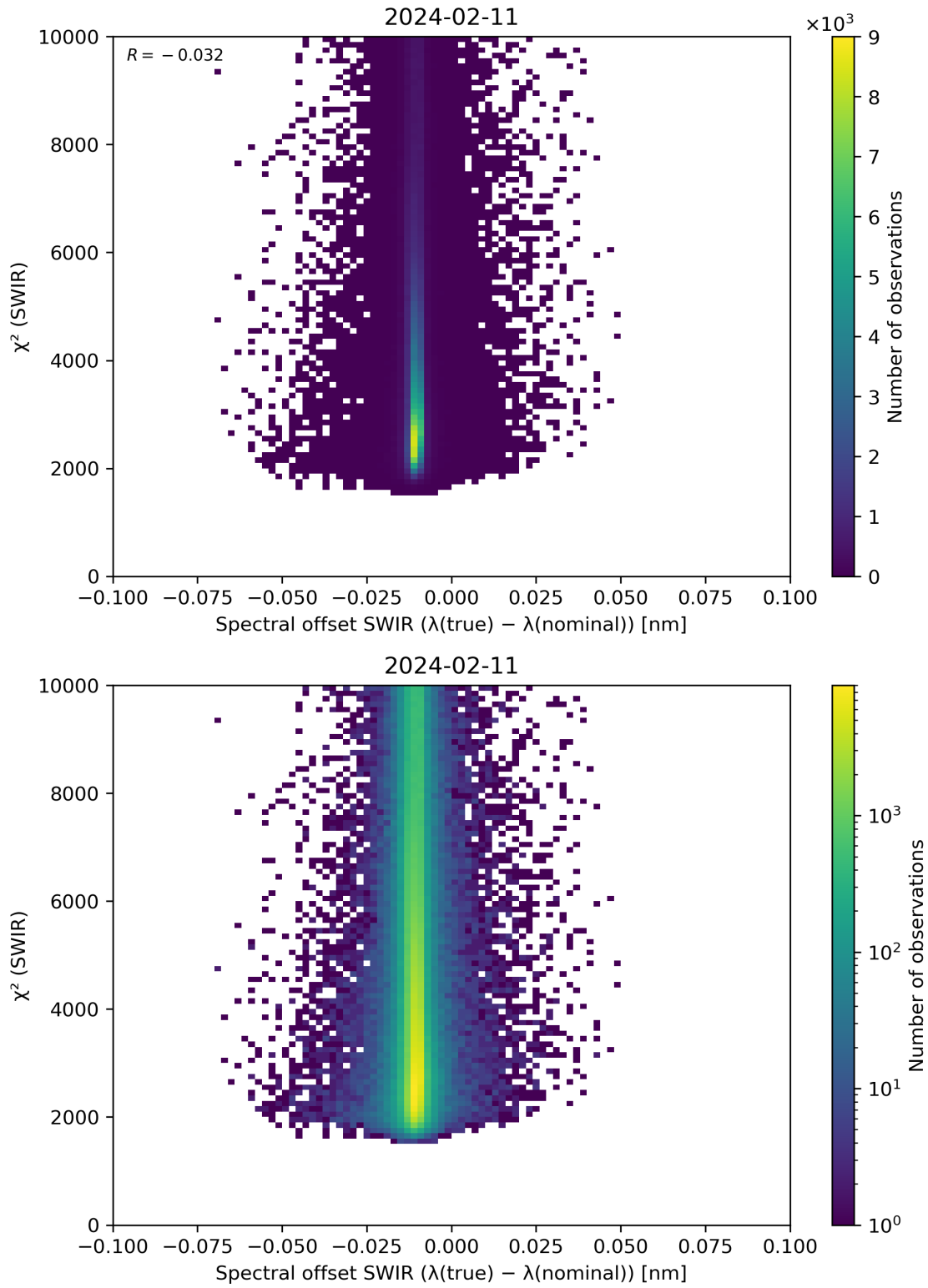
Figure 118: Scatter density plot of “Spectral offset SWIR ( \lambda(\text{true}) - \lambda(\text{nominal}) )” against “ \chi^2 (SWIR)” for 2024-02-11 to 2024-02-12.
