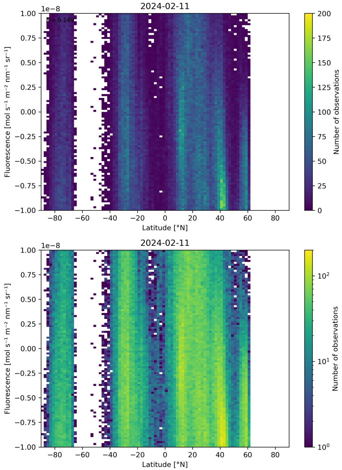
Figure 56: Scatter density plot of “Latitude” against “Fluorescence” for 2024-02-11 to 2024-02-12.
