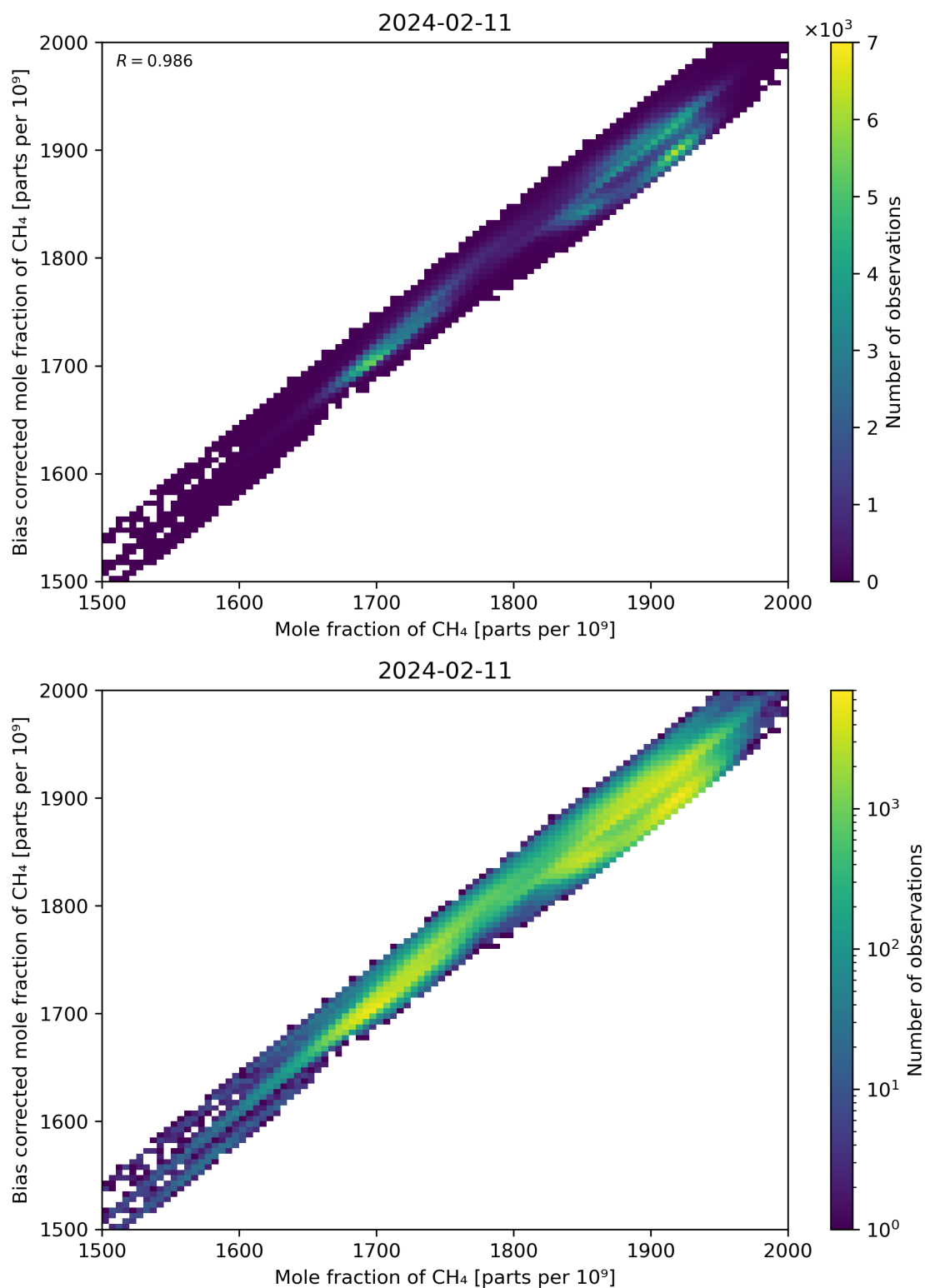
Figure 74: Scatter density plot of “Mole fraction of CH 4 ” against “Bias corrected mole fraction of CH 4 ” for 2024-02-11 to 2024-02-12.
