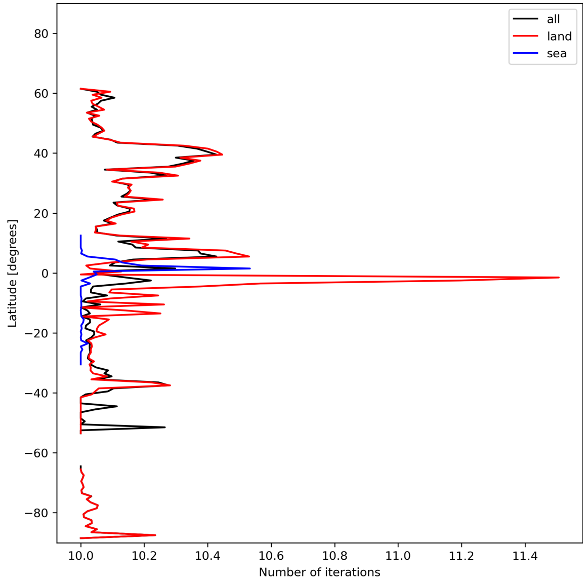
Figure 20: Zonal average of “Number of iterations” for 2024-02-11 to 2024-02-12.
