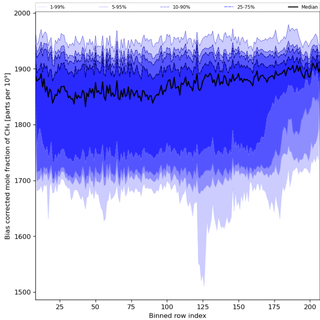
Figure 36: Along track statistics of “Bias corrected mole fraction of CH 4 ” for 2024-02-11 to 2024-02-13
