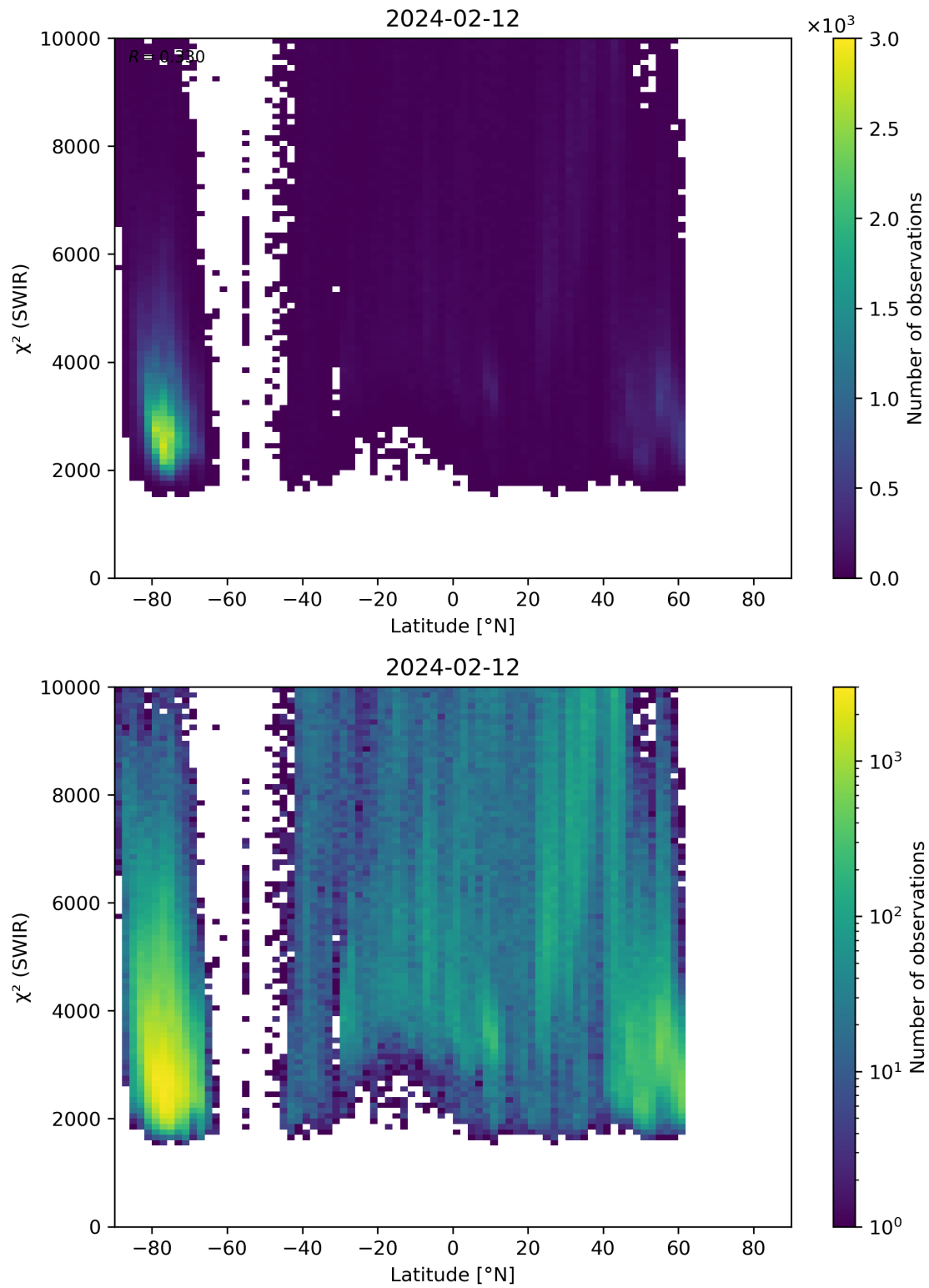
Figure 54: Scatter density plot of “Latitude” against “ \chi^2 (SWIR)” for 2024-02-11 to 2024-02-13.
