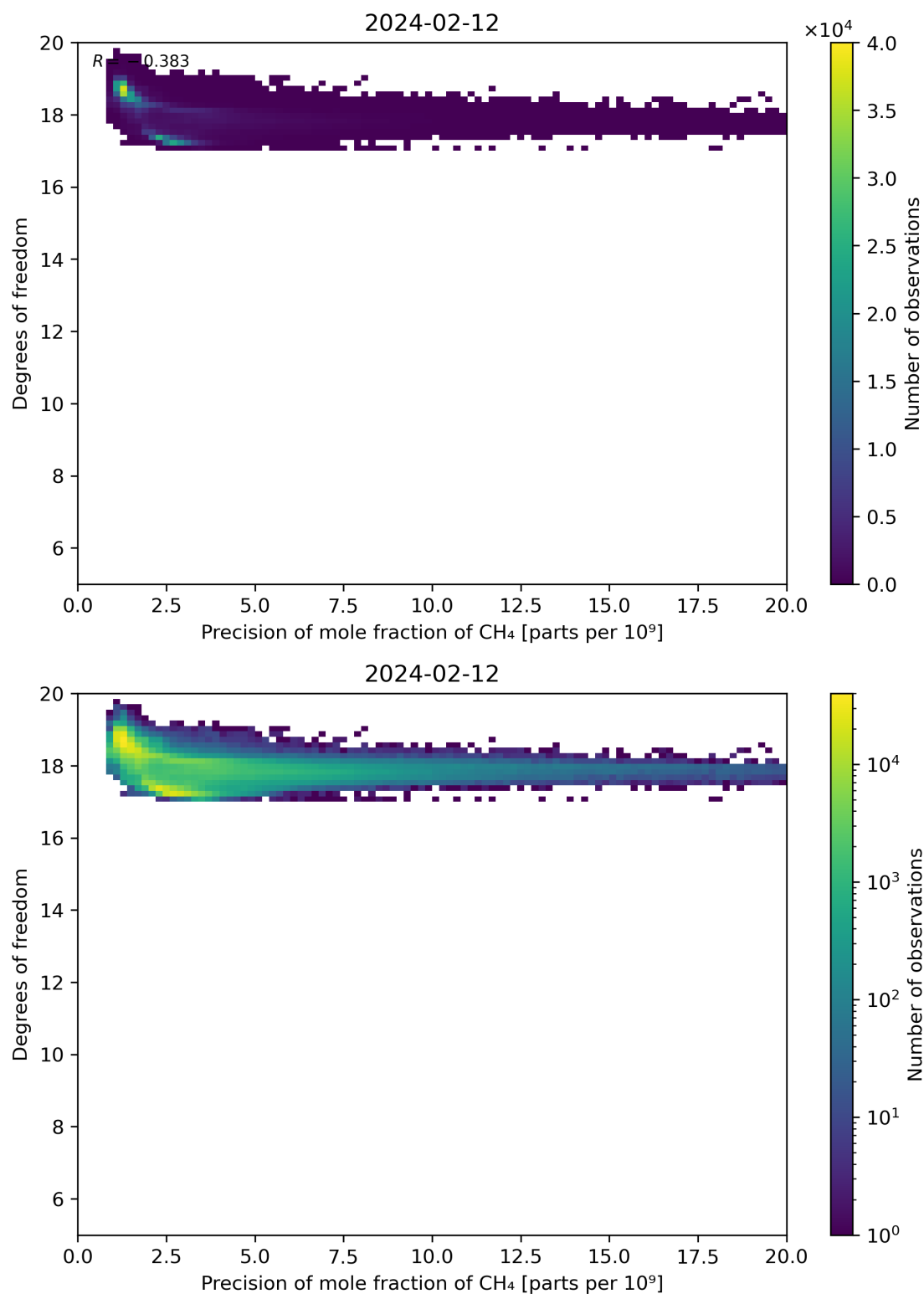
Figure 80: Scatter density plot of “Precision of mole fraction of CH 4 ” against “Degrees of freedom” for 2024-02-11 to 2024-02-13.
