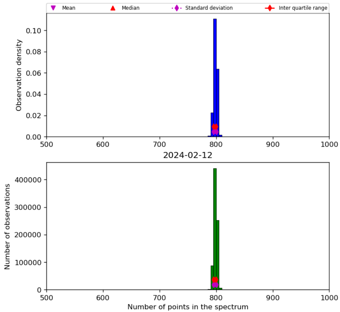
Figure 26: Histogram of “Number of points in the spectrum” for 2024-02-11 to 2024-02-13
