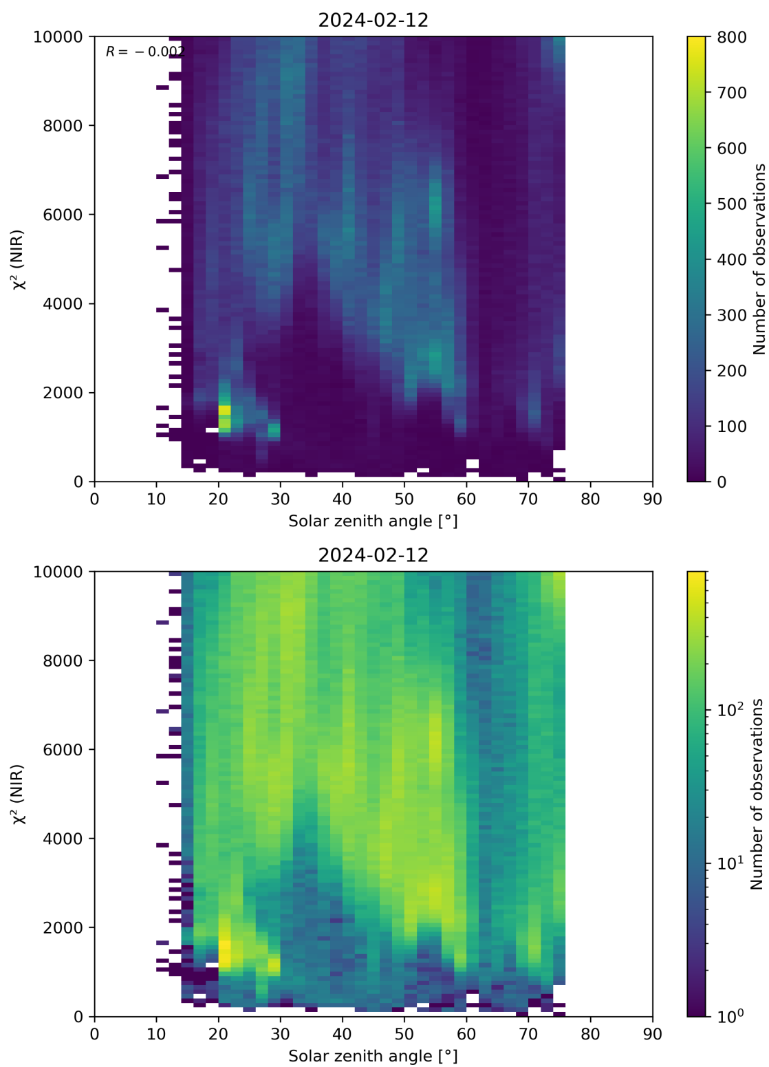
Figure 94: Scatter density plot of “Solar zenith angle” against “ \chi^2 (NIR)” for 2024-02-11 to 2024-02-13.
