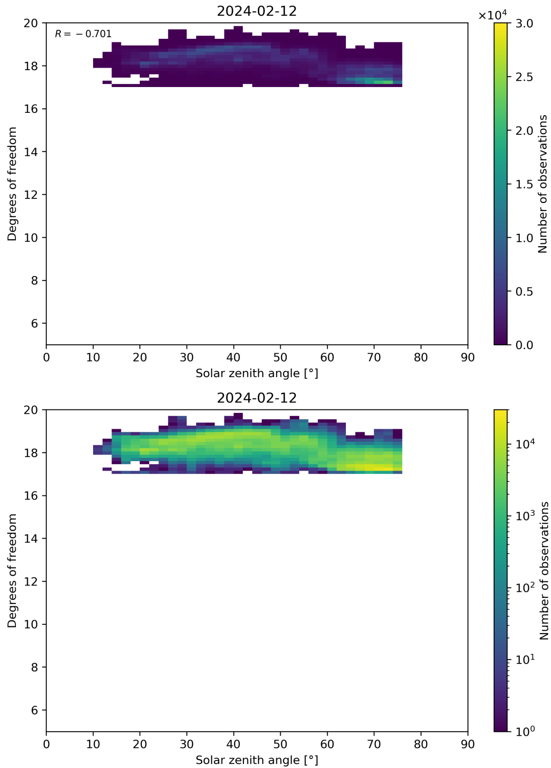
Figure 96: Scatter density plot of “Solar zenith angle” against “Degrees of freedom” for 2024-02-11 to 2024-02-13.
