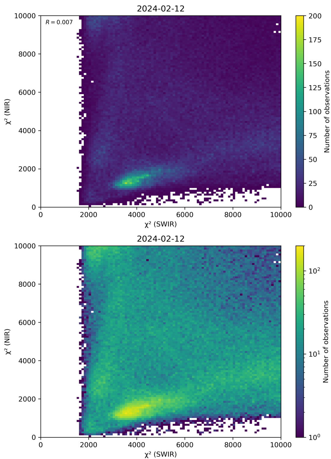
Figure 47: Scatter density plot of “ \chi^2 (SWIR)” against “ \chi^2 (NIR)” for 2024-02-11 to 2024-02-13.
