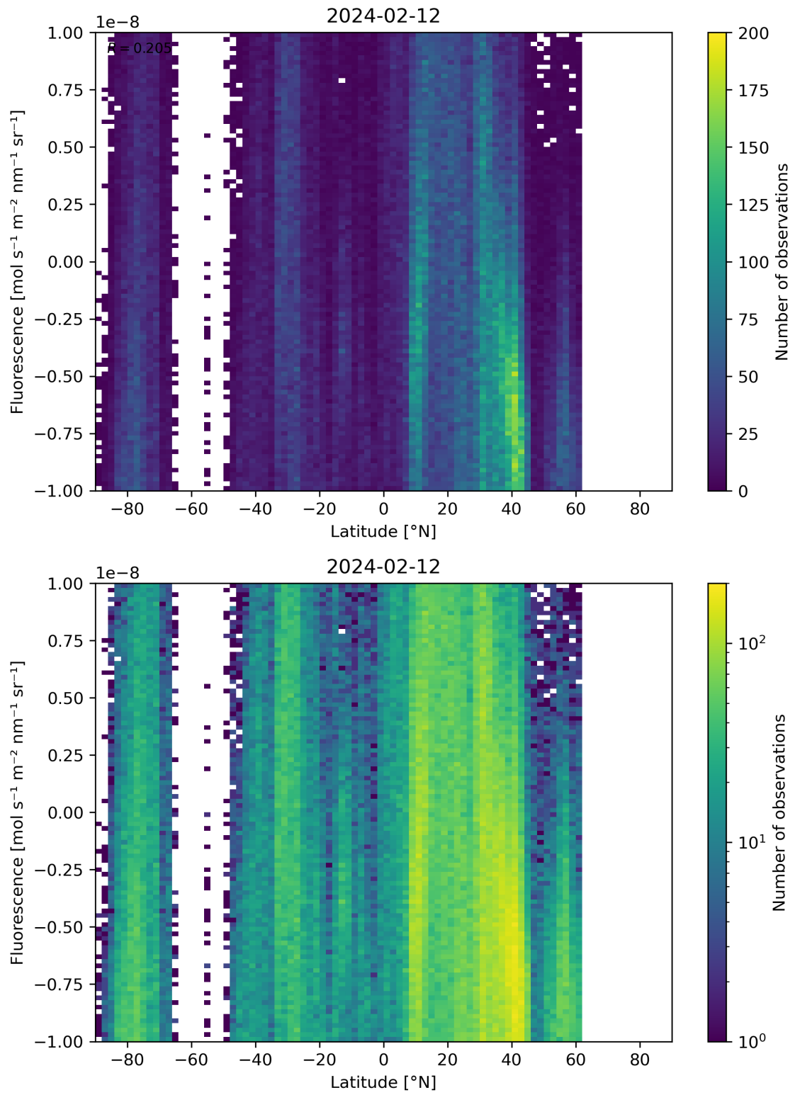
Figure 56: Scatter density plot of “Latitude” against “Fluorescence” for 2024-02-11 to 2024-02-13.
