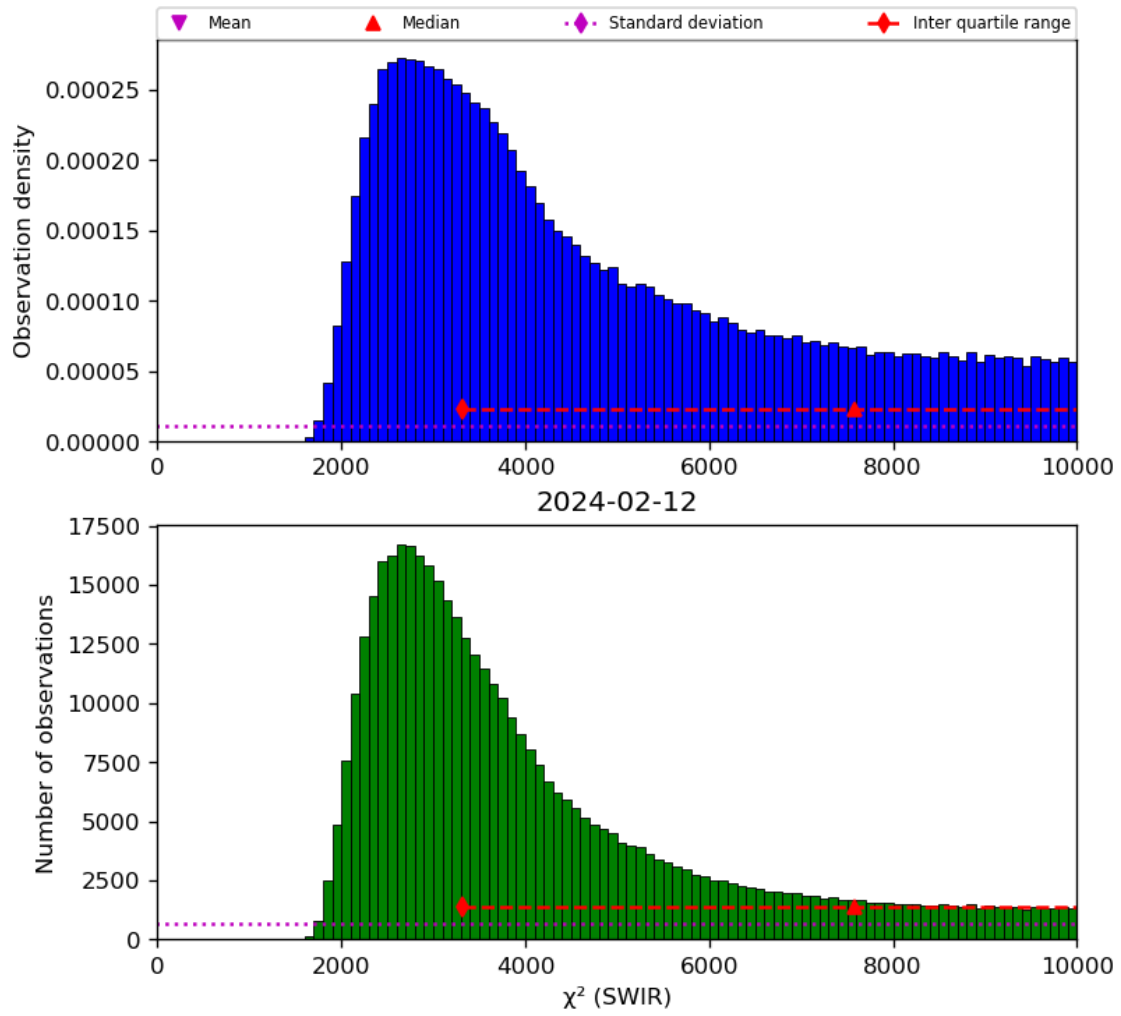
Figure 28: Histogram of “ \chi^2 (SWIR)” for 2024-02-11 to 2024-02-13
