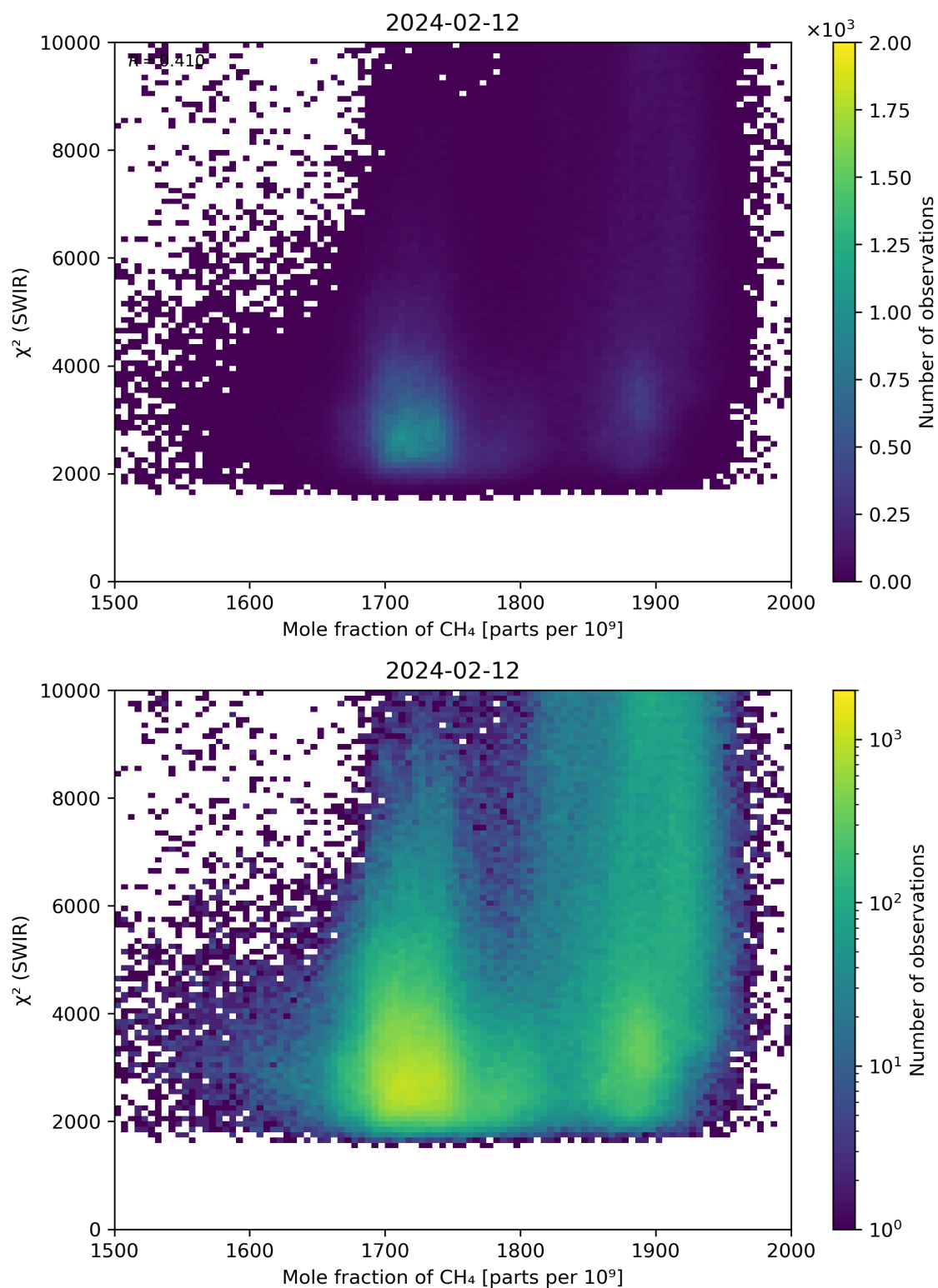
Figure 71: Scatter density plot of “Mole fraction of CH 4 ” against “ \chi^2 (SWIR)” for 2024-02-11 to 2024-02-13.
