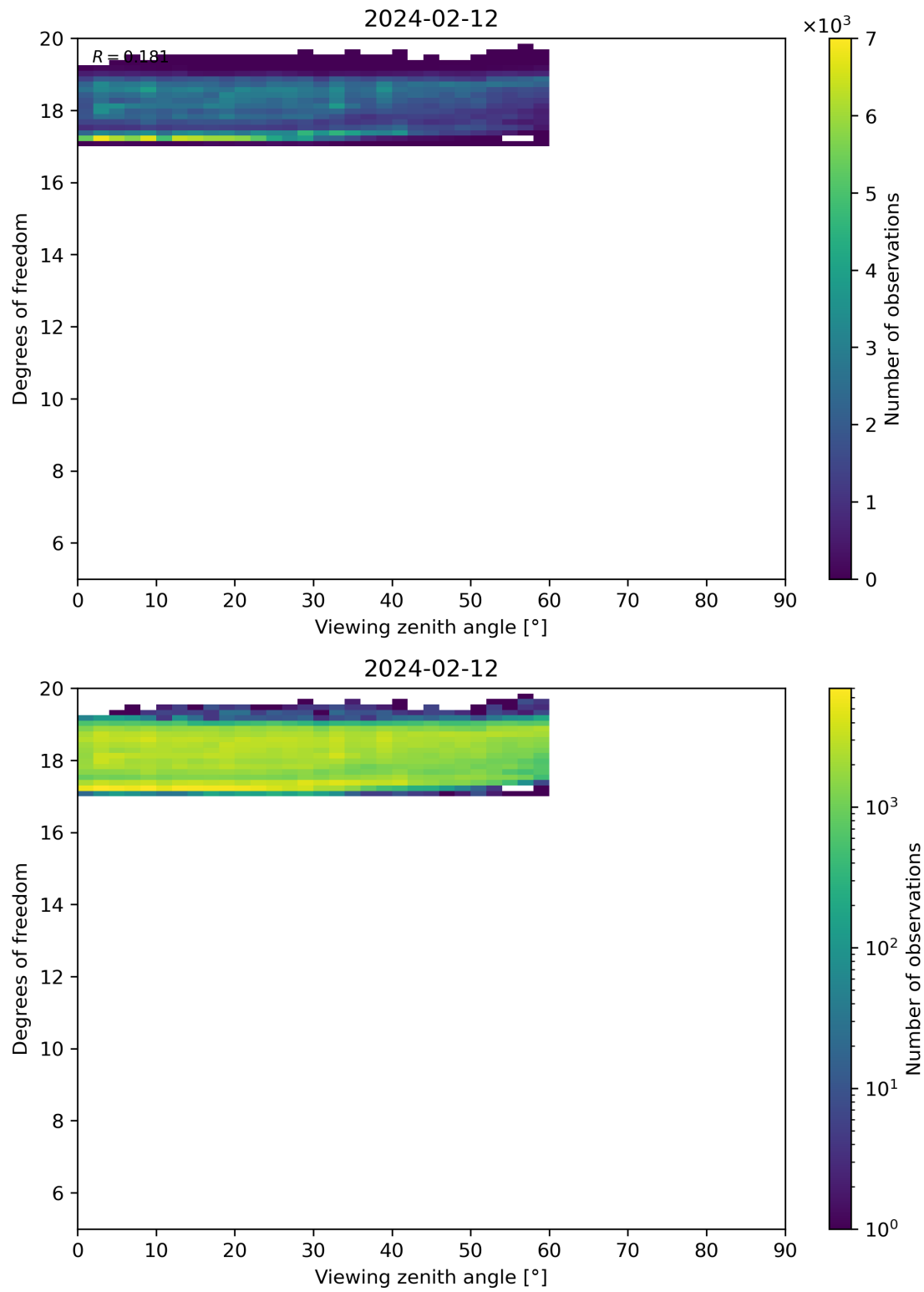
Figure 107: Scatter density plot of “Viewing zenith angle” against “Degrees of freedom” for 2024-02-11 to 2024-02-13.
