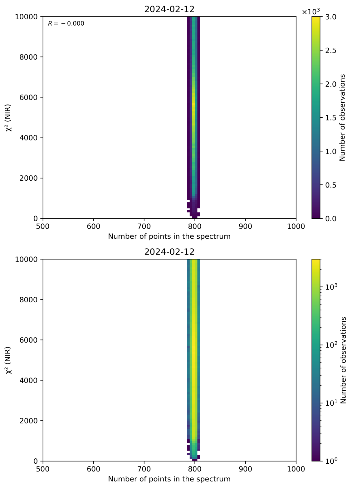
Figure 88: Scatter density plot of “Number of points in the spectrum” against “ \chi^2 (NIR)” for 2024-02-11 to 2024-02-13.
