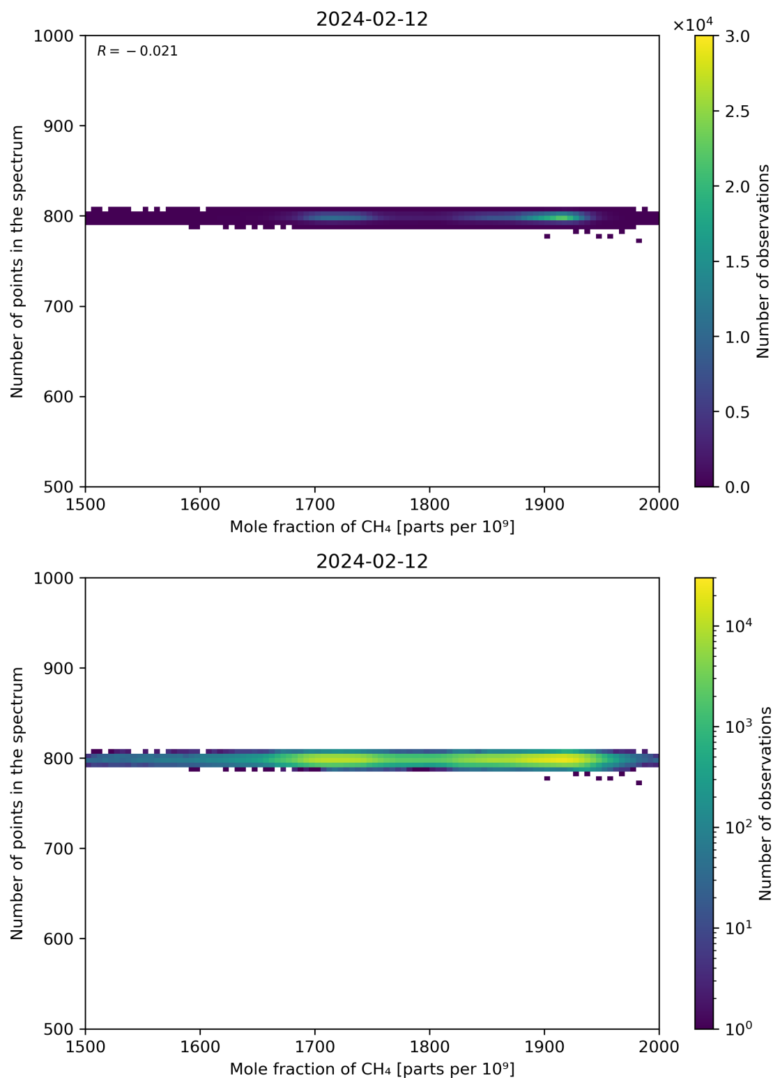
Figure 77: Scatter density plot of “Mole fraction of CH 4 ” against “Number of points in the spectrum” for 2024-02-11 to 2024-02-13.
