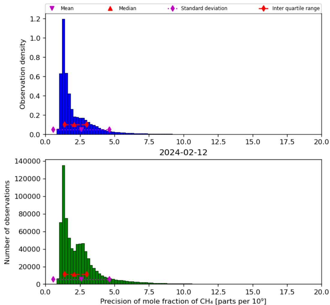
Figure 24: Histogram of “Precision of mole fraction of CH 4 ” for 2024-02-11 to 2024-02-13
