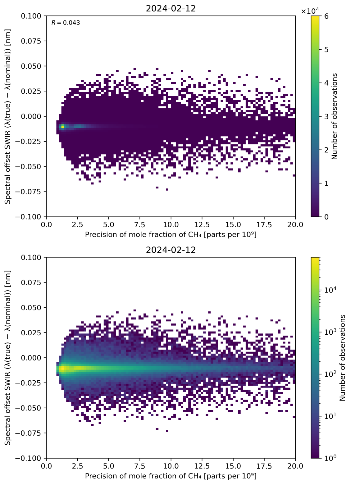
Figure 85: Scatter density plot of “Precision of mole fraction of \text{CH}_4 ” against “Spectral offset SWIR ( \lambda(\text{true}) - \lambda(\text{nominal}) )” for 2024-02-11 to 2024-02-13.
