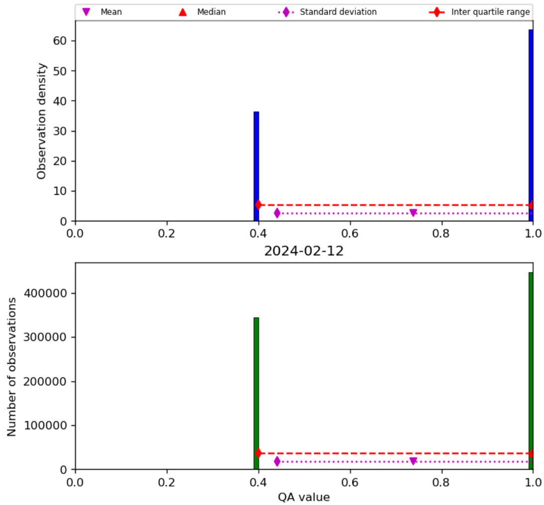
Figure 22: Histogram of “QA value” for 2024-02-11 to 2024-02-13
