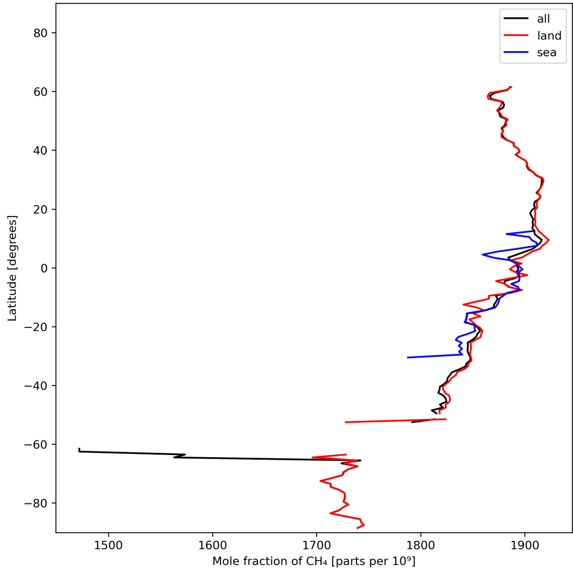
Figure 12: Zonal average of “Mole fraction of \text{CH}_4 ” for 2024-02-11 to 2024-02-13.
