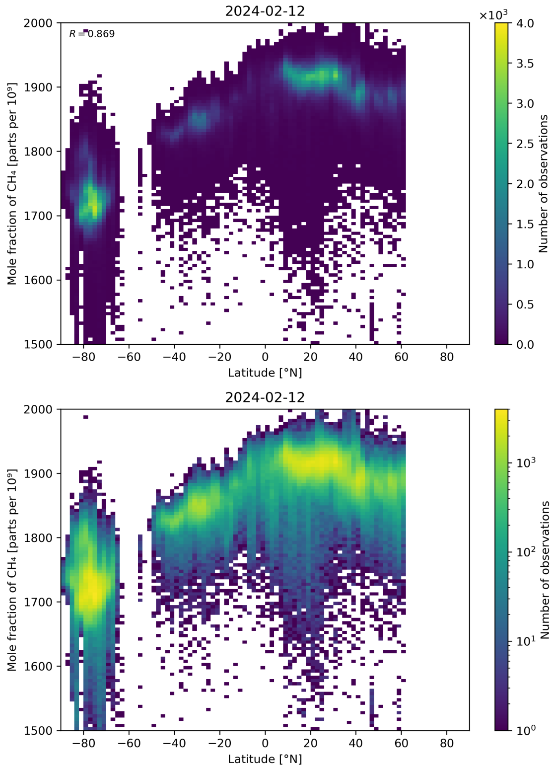
Figure 57: Scatter density plot of “Latitude” against “Mole fraction of CH 4 ” for 2024-02-11 to 2024-02-13.
