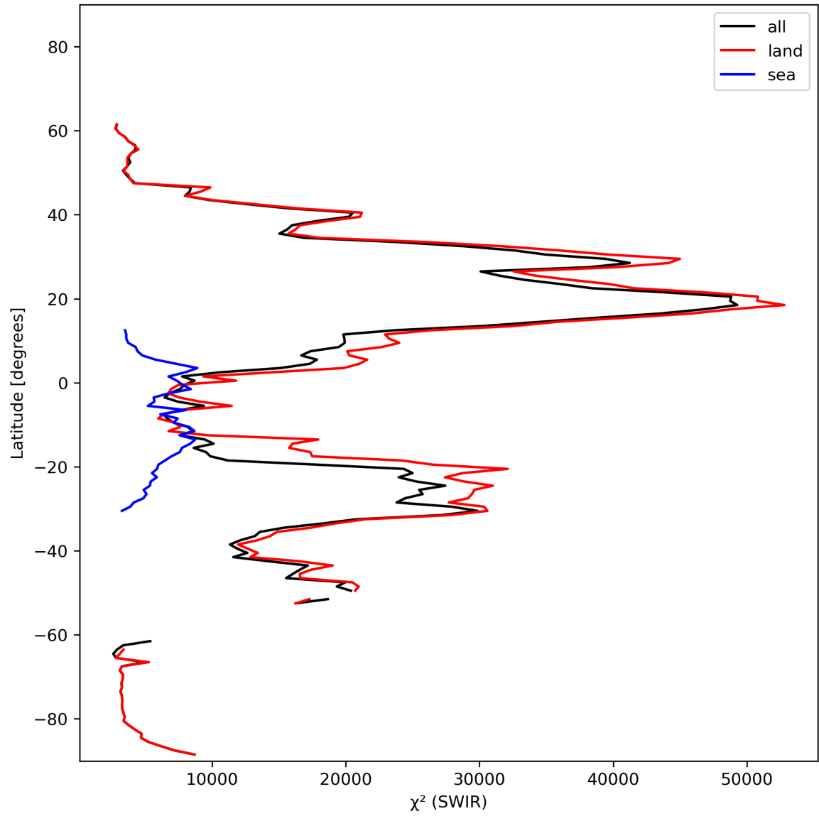
Figure 17: Zonal average of “ \chi^2 (SWIR)” for 2024-02-11 to 2024-02-13.
