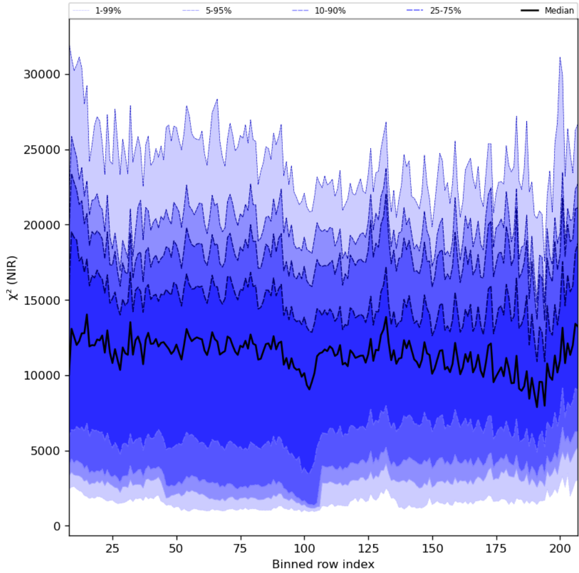
Figure 40: Along track statistics of “ \chi^2 (NIR)” for 2024-02-11 to 2024-02-13
