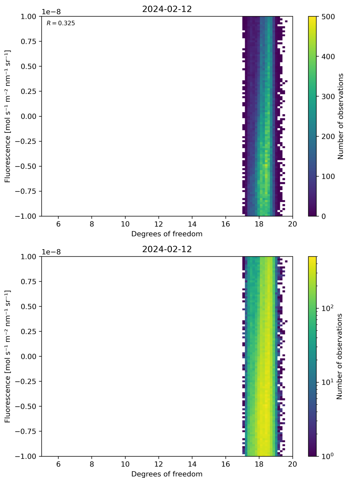
Figure 51: Scatter density plot of “Degrees of freedom” against “Fluorescence” for 2024-02-11 to 2024-02-13.
