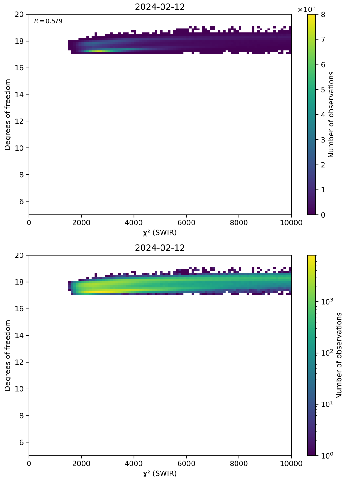
Figure 48: Scatter density plot of “ \chi^2 (SWIR)” against “Degrees of freedom” for 2024-02-11 to 2024-02-13.
