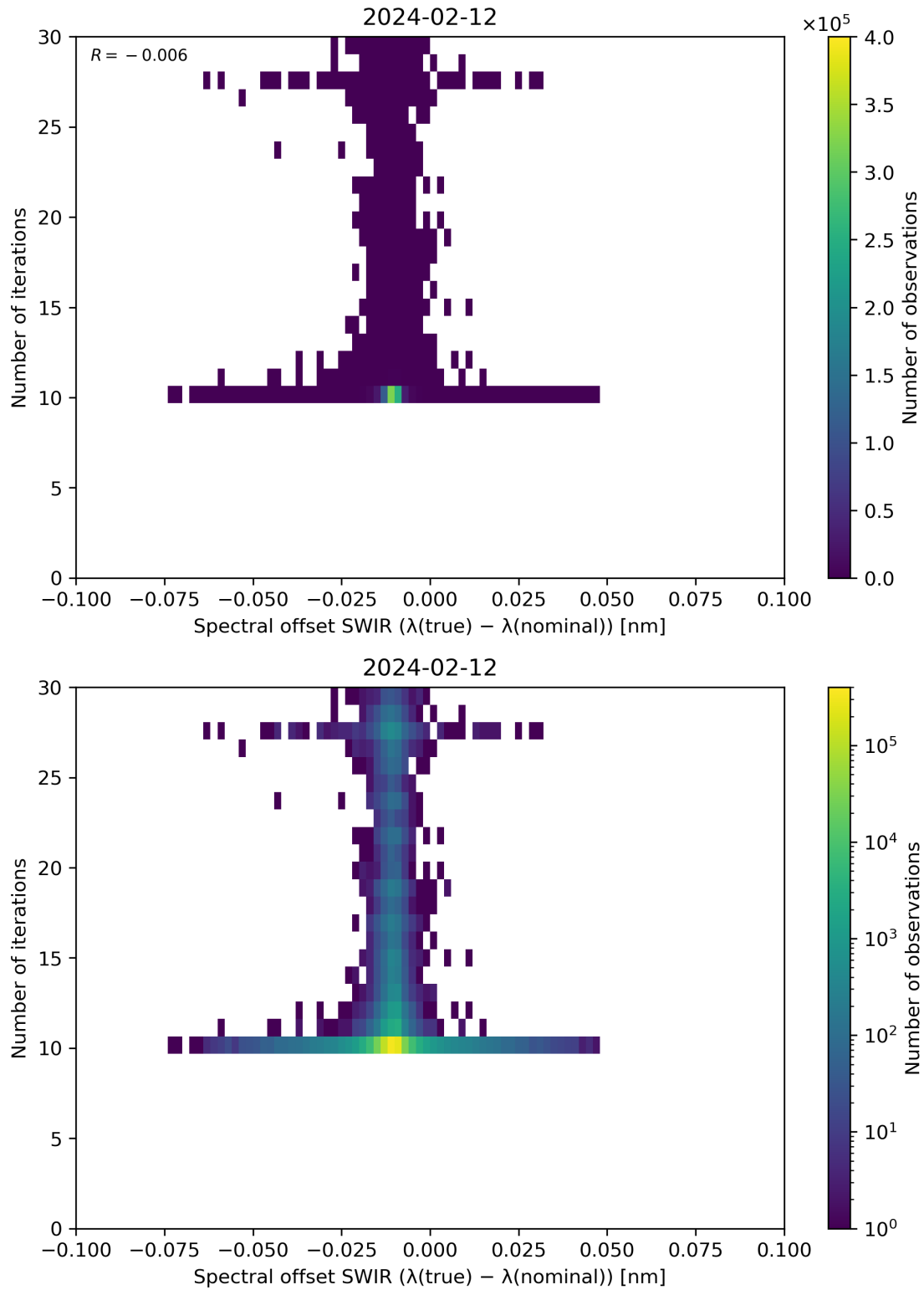
Figure 121: Scatter density plot of “Spectral offset SWIR ( \lambda(\text{true}) - \lambda(\text{nominal}) )” against “Number of iterations” for 2024-02-11 to 2024-02-13.
