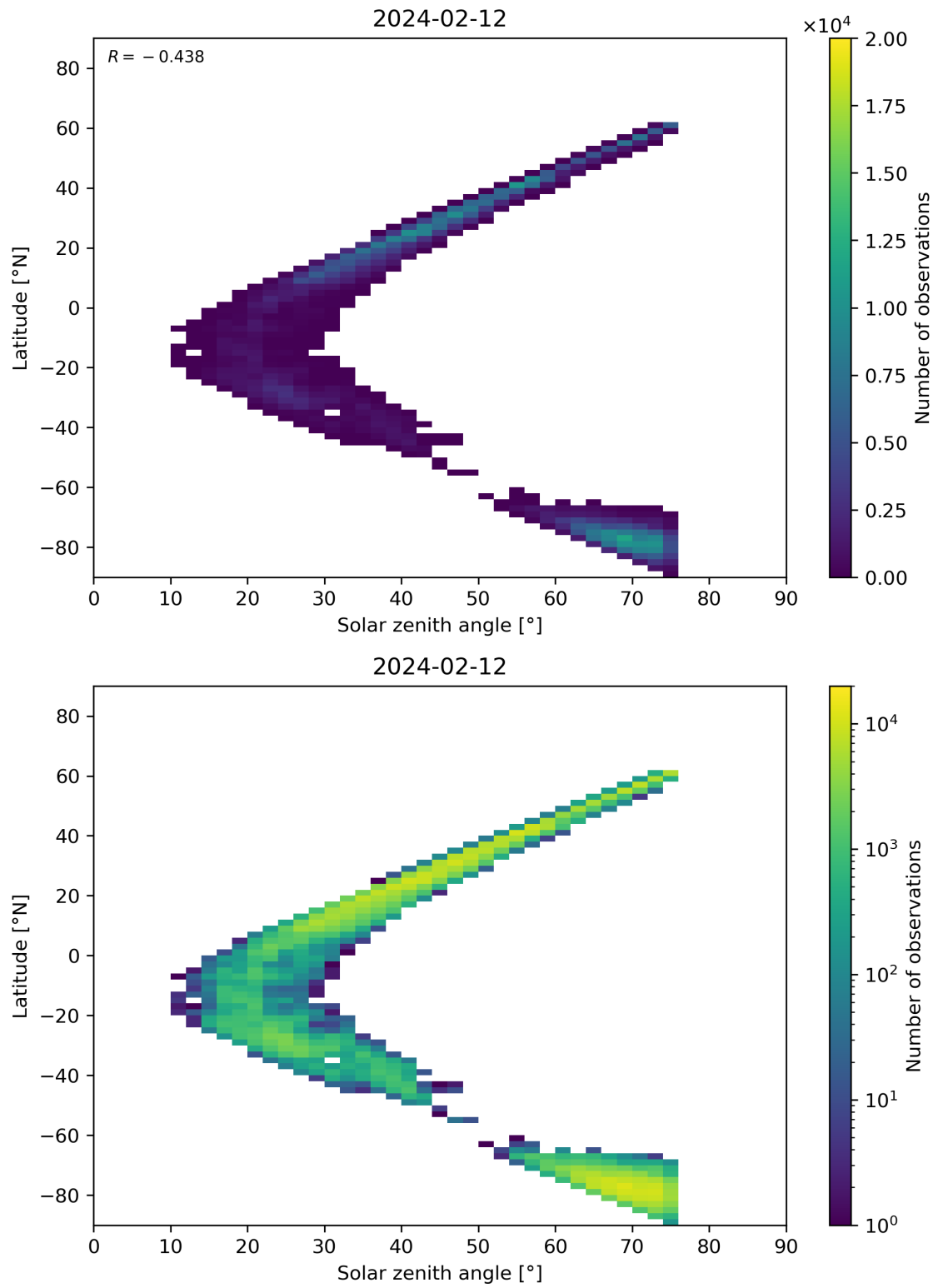
Figure 98: Scatter density plot of “Solar zenith angle” against “Latitude” for 2024-02-11 to 2024-02-13.
