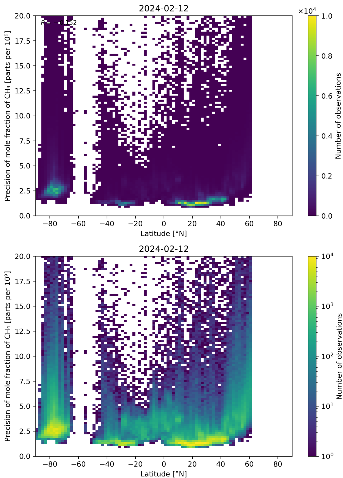
Figure 59: Scatter density plot of “Latitude” against “Precision of mole fraction of CH 4 ” for 2024-02-11 to 2024-02-13.
