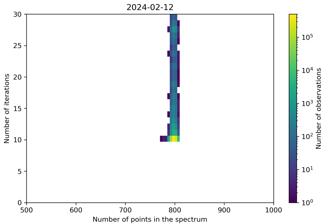
Figure 92: Scatter density plot of “Number of points in the spectrum” against “Number of iterations” for 2024-02-11 to 2024-02-13.
