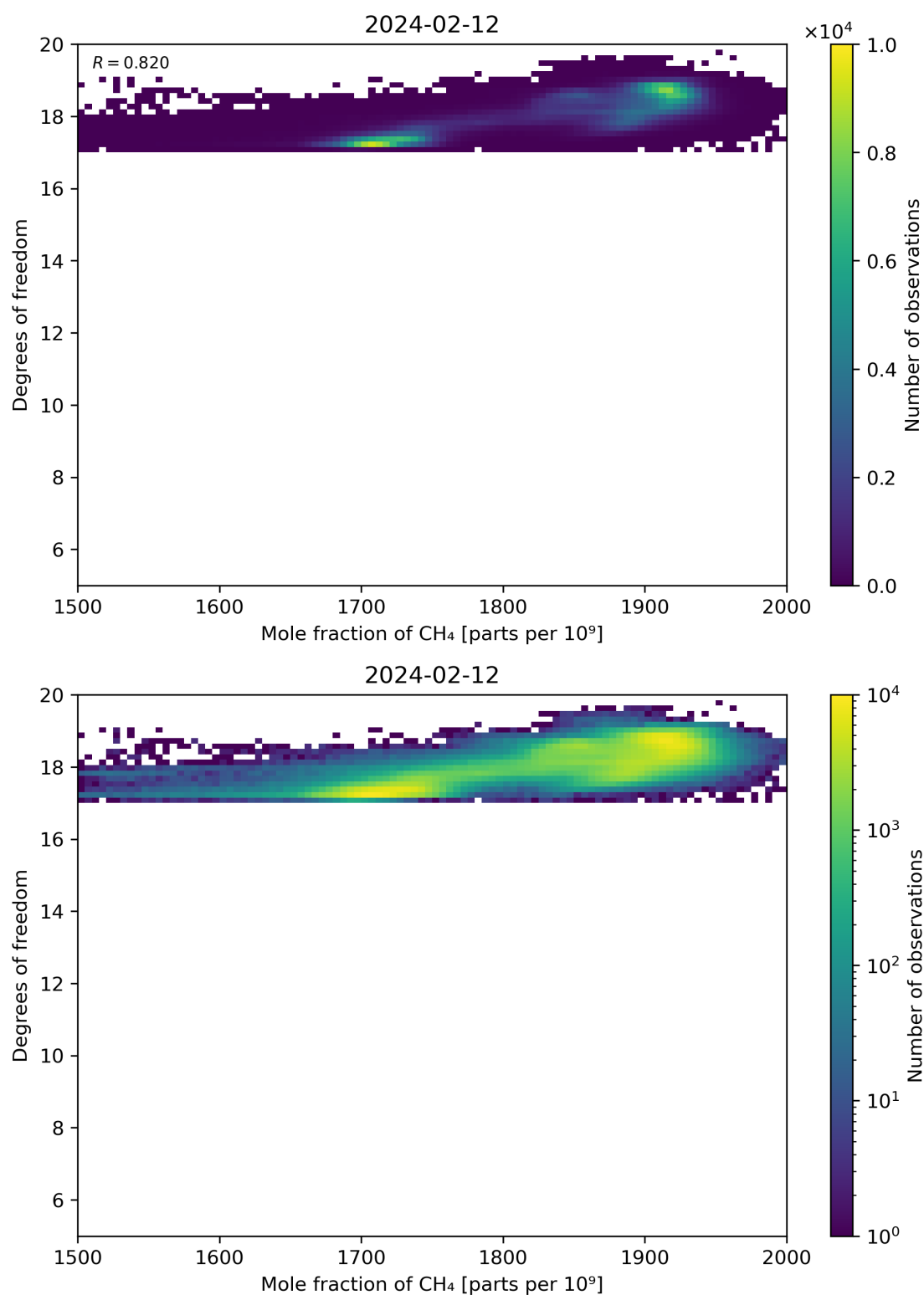
Figure 72: Scatter density plot of “Mole fraction of CH 4 ” against “Degrees of freedom” for 2024-02-11 to 2024-02-13.
