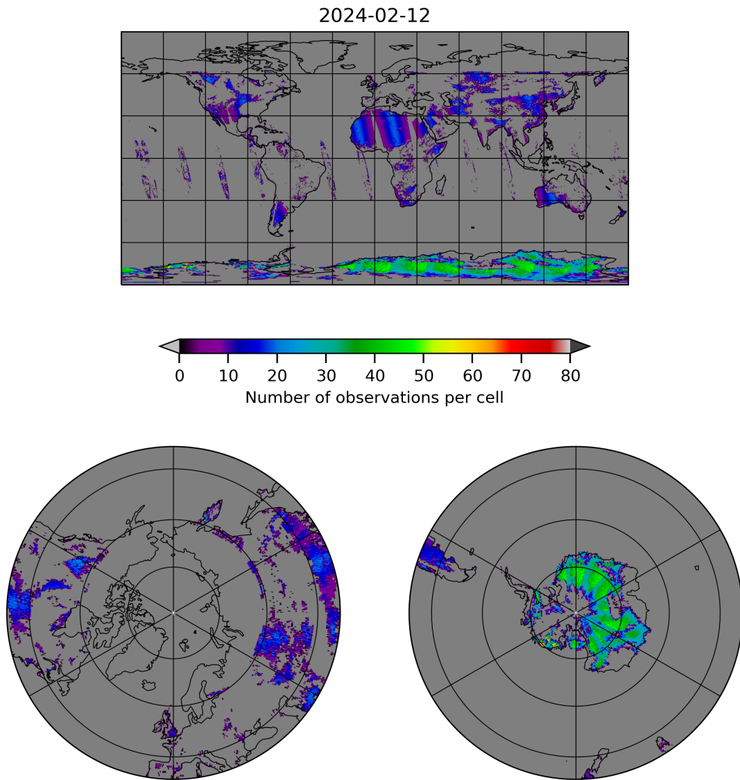
Figure 10: Map of the number of observations for 2024-02-11 to 2024-02-13
