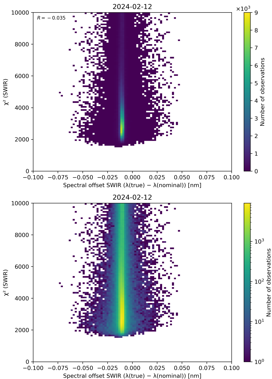
Figure 118: Scatter density plot of “Spectral offset SWIR ( \lambda(\text{true}) - \lambda(\text{nominal}) )” against “ \chi^2 (SWIR)” for 2024-02-11 to 2024-02-13.
