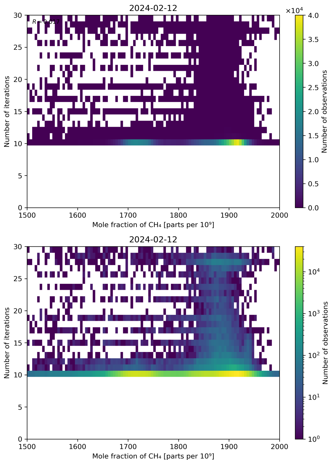
Figure 76: Scatter density plot of “Mole fraction of CH 4 ” against “Number of iterations” for 2024-02-11 to 2024-02-13.
