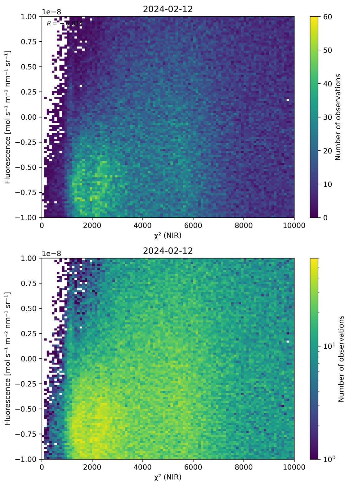
Figure 45: Scatter density plot of “ \chi^2 (NIR)” against “Fluorescence” for 2024-02-11 to 2024-02-13.
