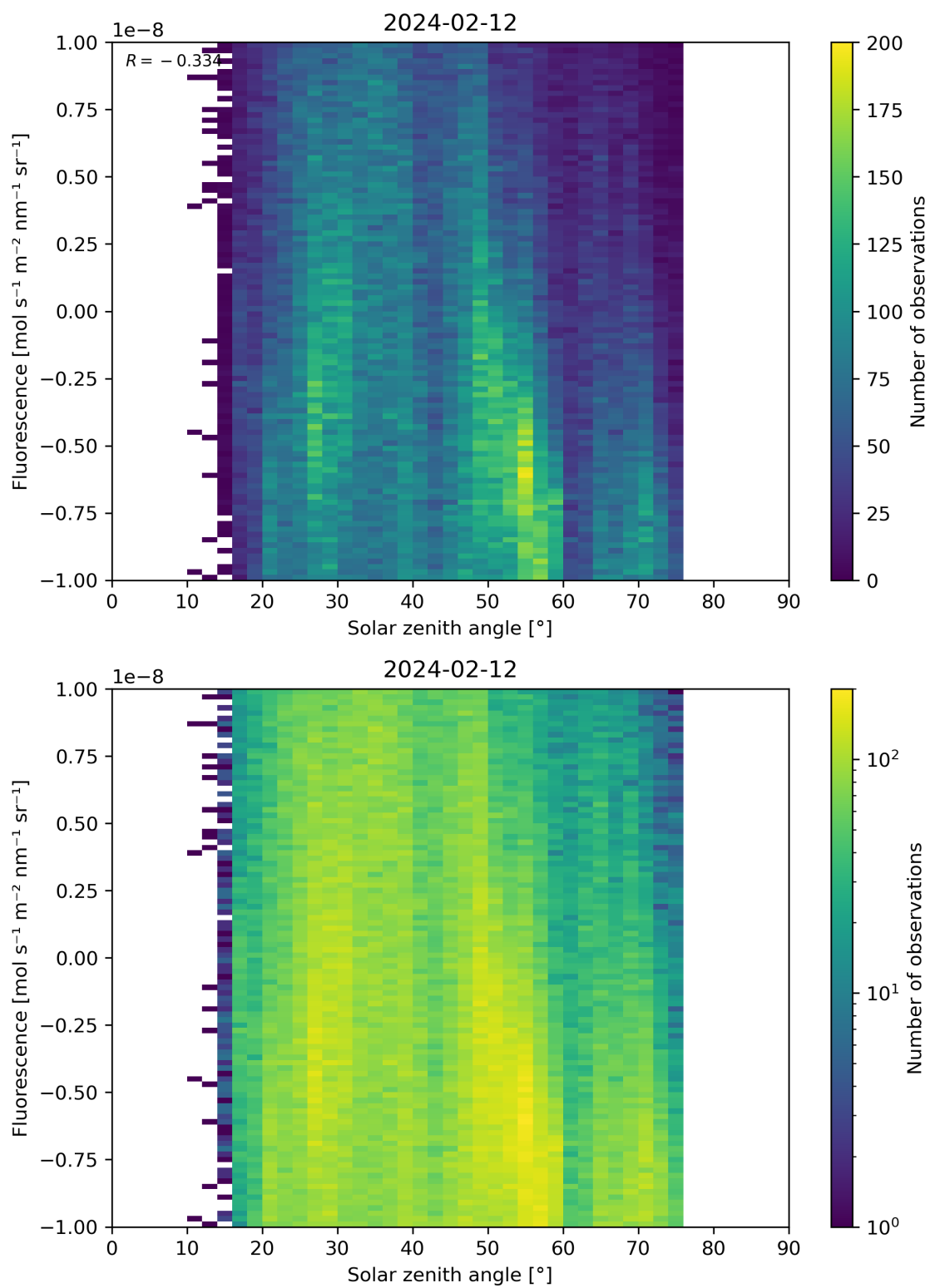
Figure 97: Scatter density plot of “Solar zenith angle” against “Fluorescence” for 2024-02-11 to 2024-02-13.
