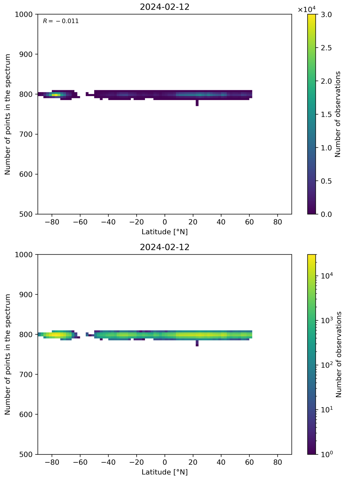
Figure 61: Scatter density plot of “Latitude” against “Number of points in the spectrum” for 2024-02-11 to 2024-02-13.
