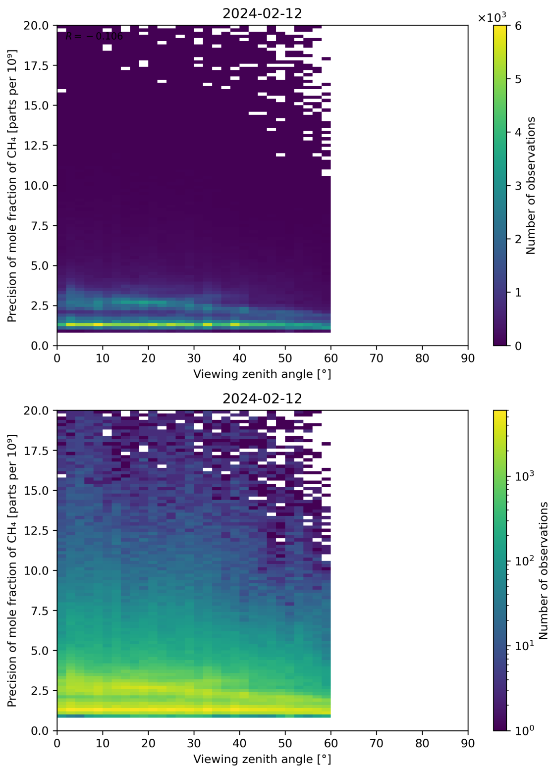
Figure 112: Scatter density plot of “Viewing zenith angle” against “Precision of mole fraction of CH 4 ” for 2024-02-11 to 2024-02-13.
