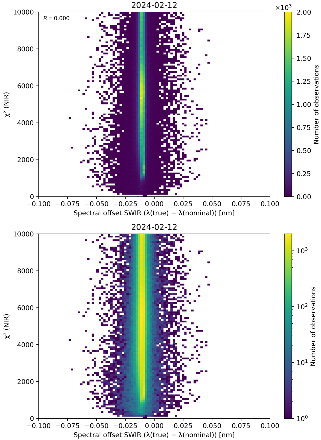
Figure 117: Scatter density plot of “Spectral offset SWIR ( \lambda(\text{true}) - \lambda(\text{nominal}) )” against “ \chi^2 (NIR)” for 2024-02-11 to 2024-02-13.
