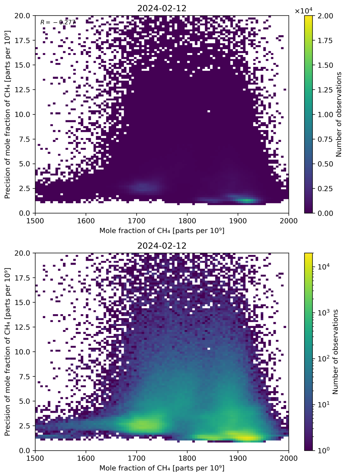
Figure 75: Scatter density plot of “Mole fraction of CH 4 ” against “Precision of mole fraction of CH 4 ” for 2024-02-11 to 2024-02-13.
