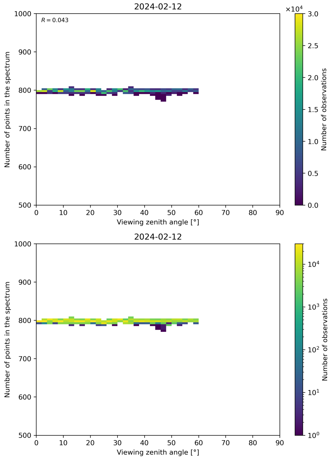
Figure 114: Scatter density plot of “Viewing zenith angle” against “Number of points in the spectrum” for 2024-02-11 to 2024-02-13.
