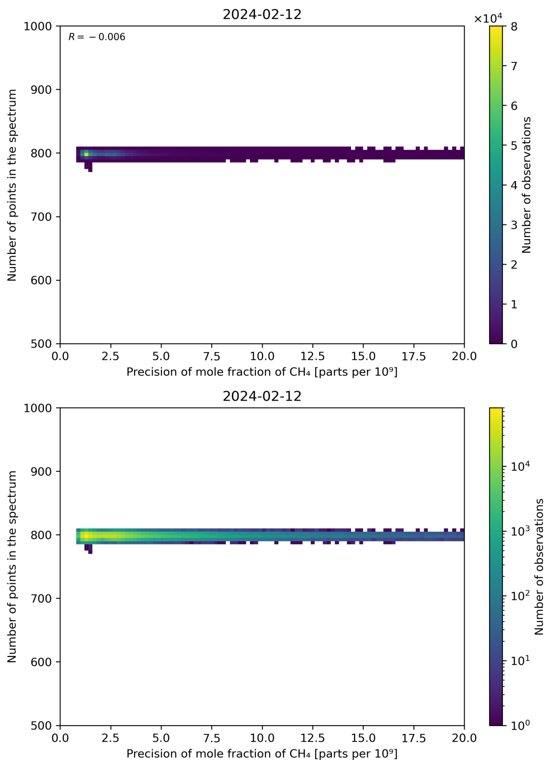
Figure 84: Scatter density plot of “Precision of mole fraction of CH 4 ” against “Number of points in the spectrum” for 2024-02-11 to 2024-02-13.
