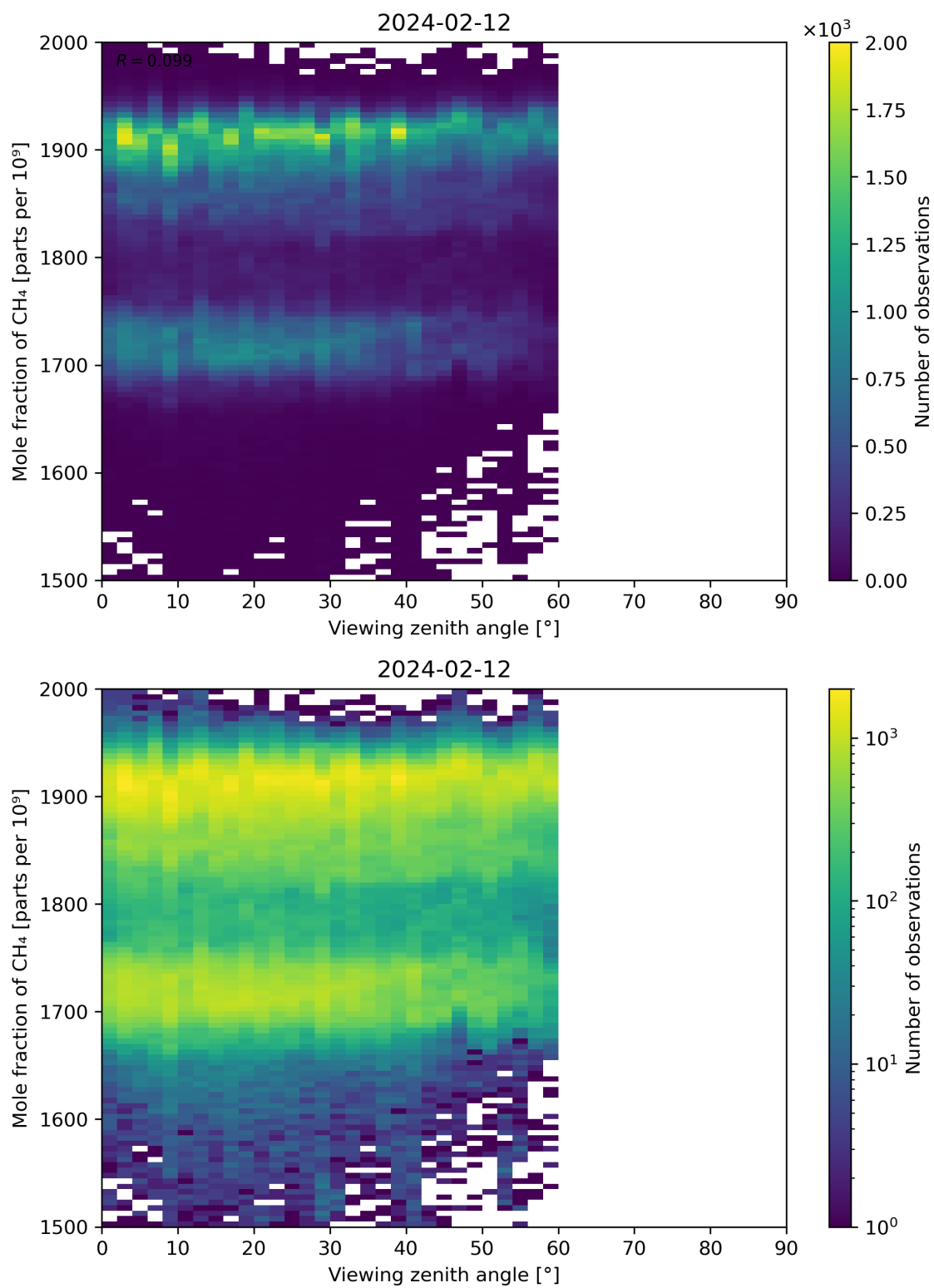
Figure 110: Scatter density plot of “Viewing zenith angle” against “Mole fraction of CH 4 ” for 2024-02-11 to 2024-02-13.
