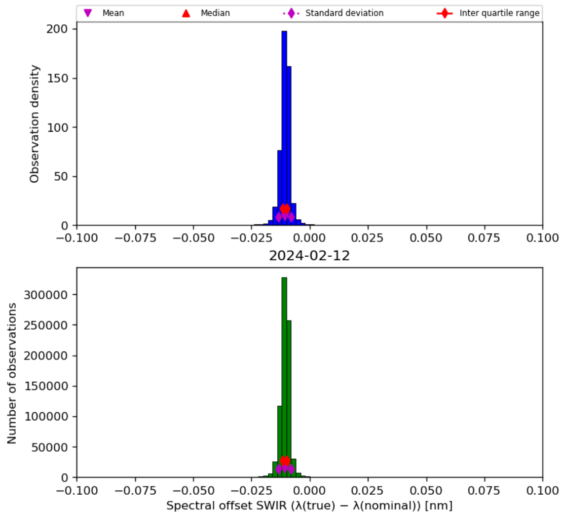
Figure 27: Histogram of “Spectral offset SWIR ( \lambda(\text{true}) - \lambda(\text{nominal}) )” for 2024-02-11 to 2024-02-13
