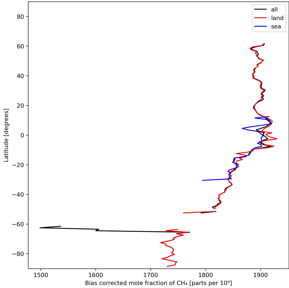
Figure 14: Zonal average of “Bias corrected mole fraction of CH 4 ” for 2024-02-11 to 2024-02-13.
