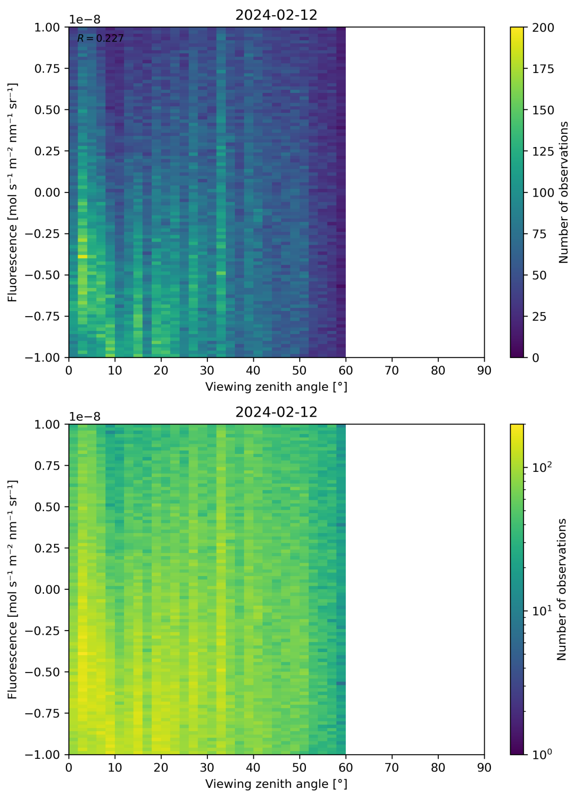
Figure 108: Scatter density plot of “Viewing zenith angle” against “Fluorescence” for 2024-02-11 to 2024-02-13.
