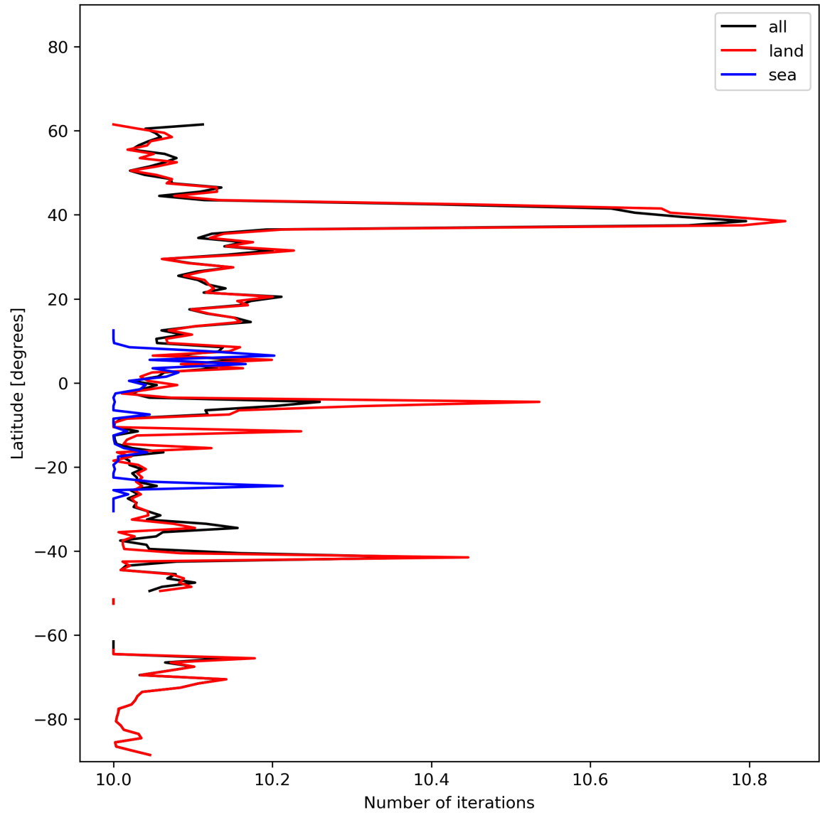
Figure 20: Zonal average of “Number of iterations” for 2024-02-11 to 2024-02-13.
