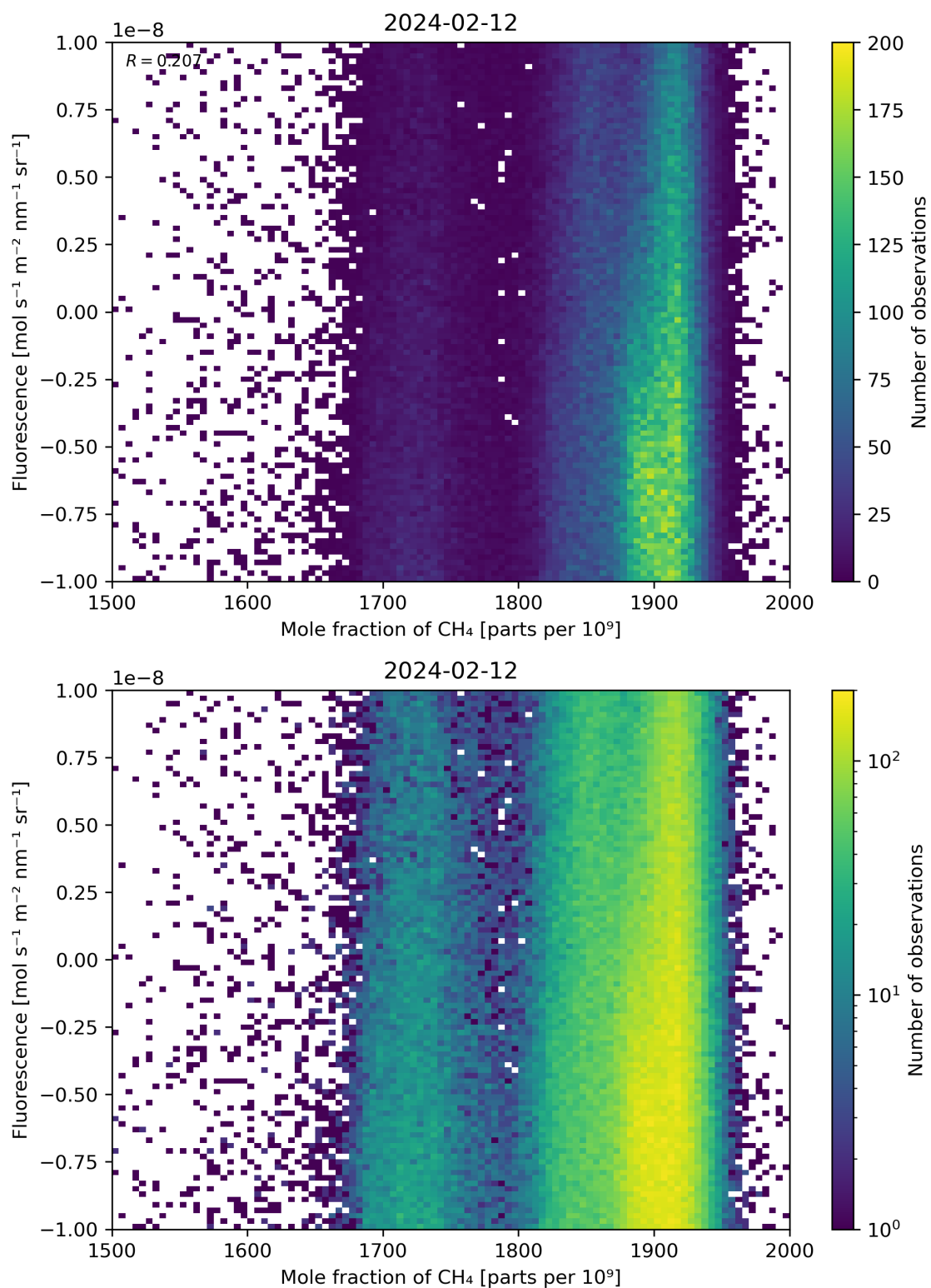
Figure 73: Scatter density plot of “Mole fraction of \text{CH}_4 ” against “Fluorescence” for 2024-02-11 to 2024-02-13.
