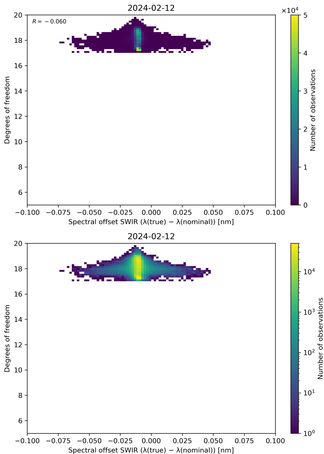
Figure 119: Scatter density plot of “Spectral offset SWIR ( \lambda(\text{true}) - \lambda(\text{nominal}) )” against “Degrees of freedom” for 2024-02-11 to 2024-02-13.
