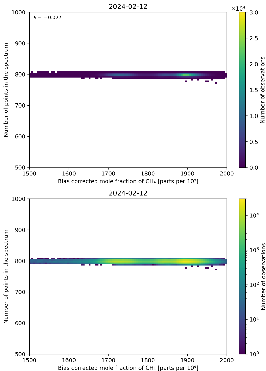
Figure 68: Scatter density plot of “Bias corrected mole fraction of CH 4 ” against “Number of points in the spectrum” for 2024-02-11 to 2024-02-13.
