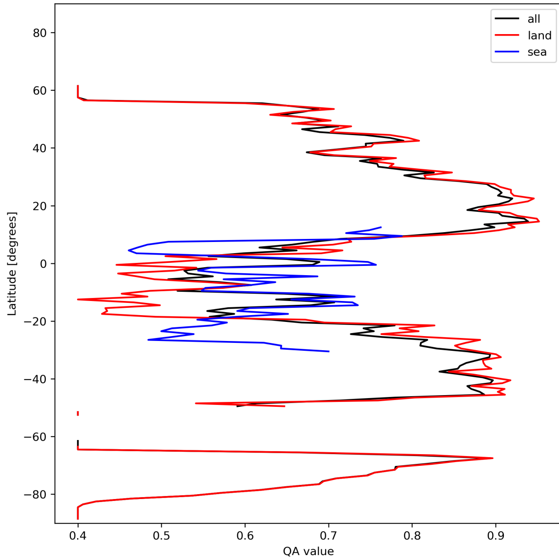
Figure 11: Zonal average of “QA value” for 2024-02-11 to 2024-02-13.
