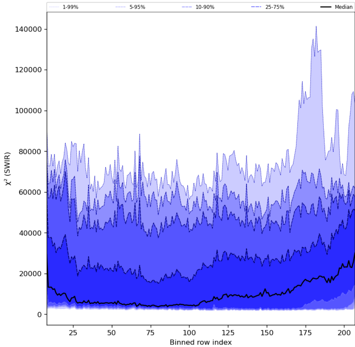
Figure 39: Along track statistics of “ \chi^2 (SWIR)” for 2024-02-11 to 2024-02-13
