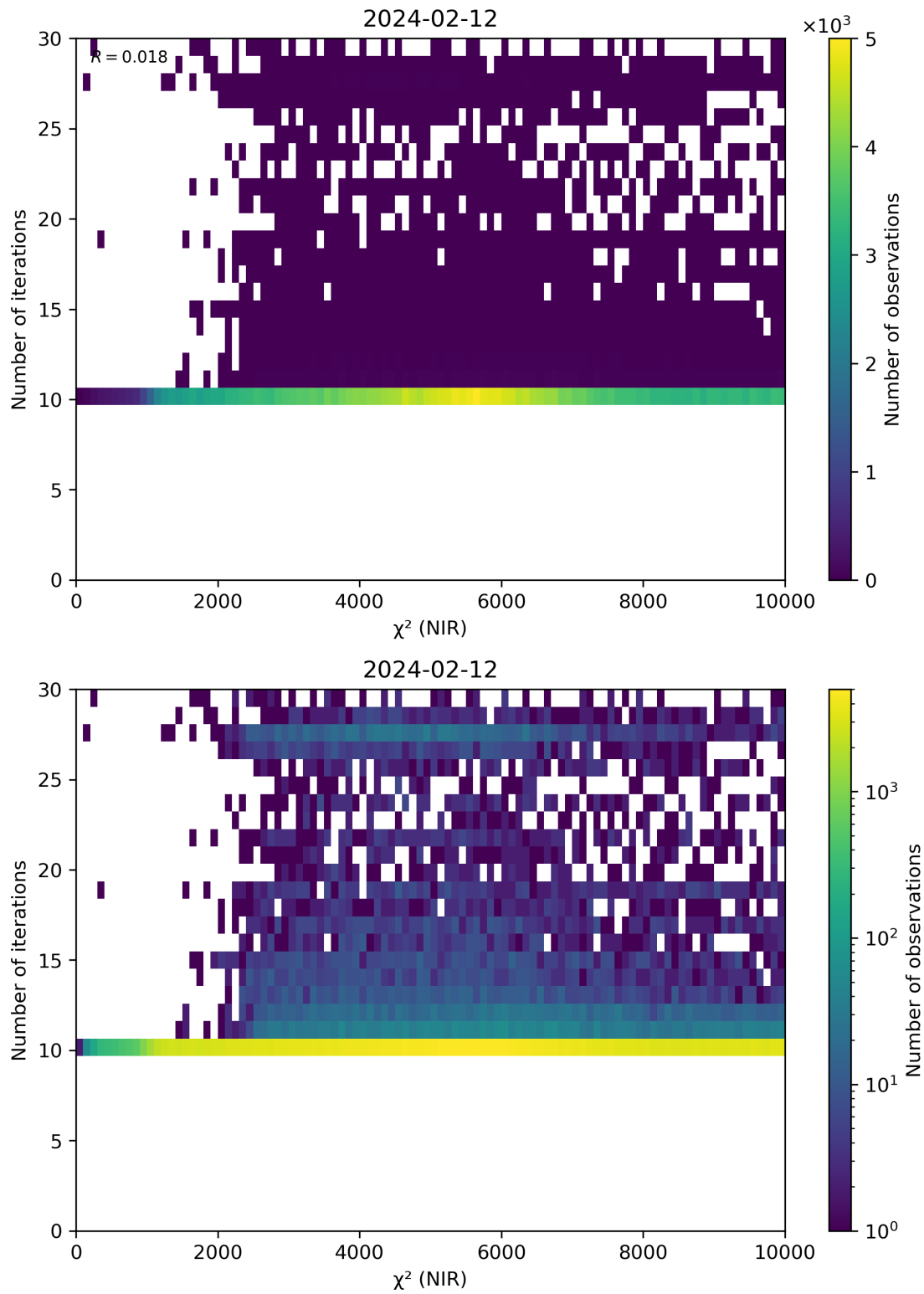
Figure 46: Scatter density plot of “ \chi^2 (NIR)” against “Number of iterations” for 2024-02-11 to 2024-02-13.
