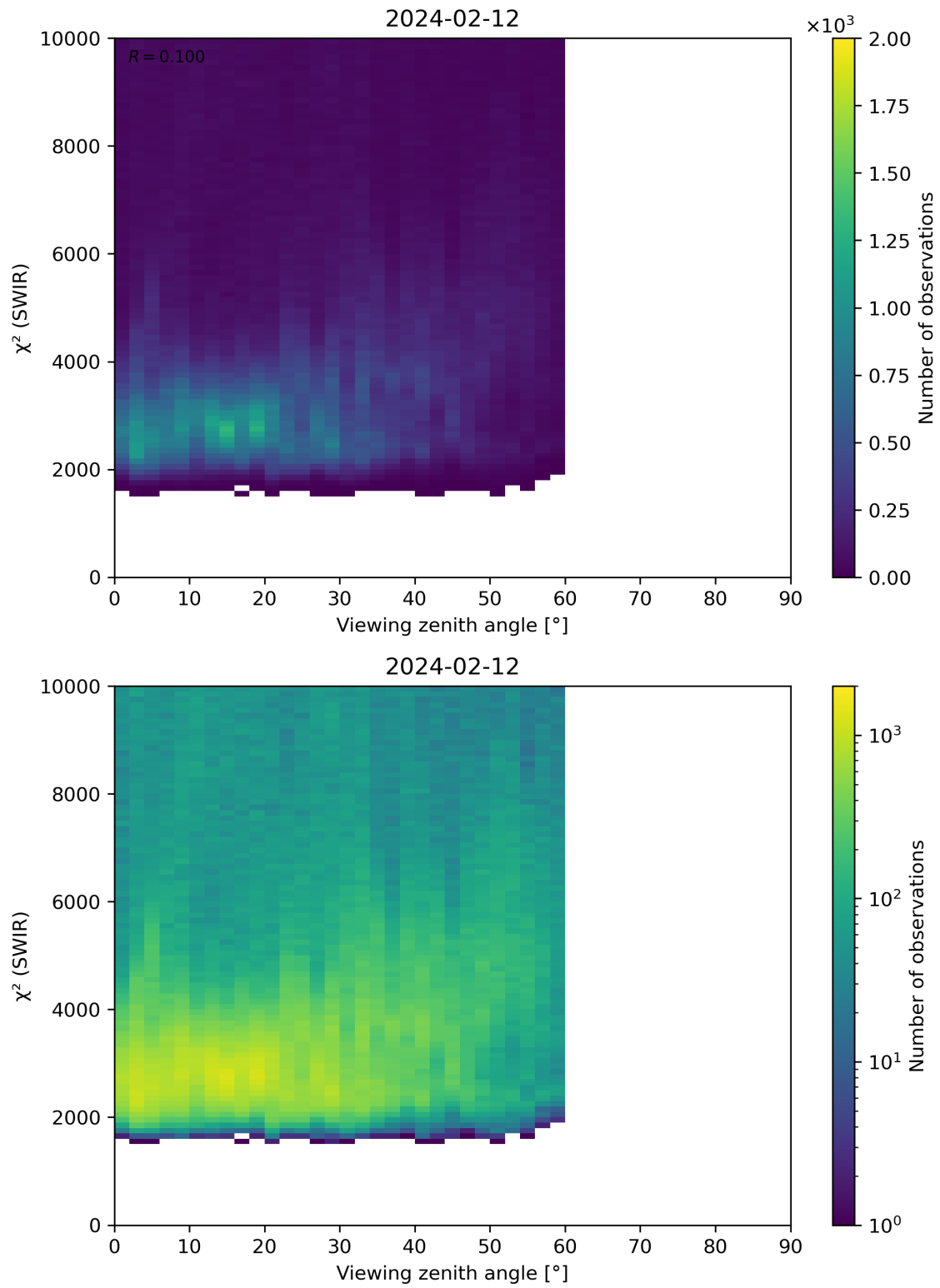
Figure 106: Scatter density plot of “Viewing zenith angle” against “ \chi^2 (SWIR)” for 2024-02-11 to 2024-02-13.
