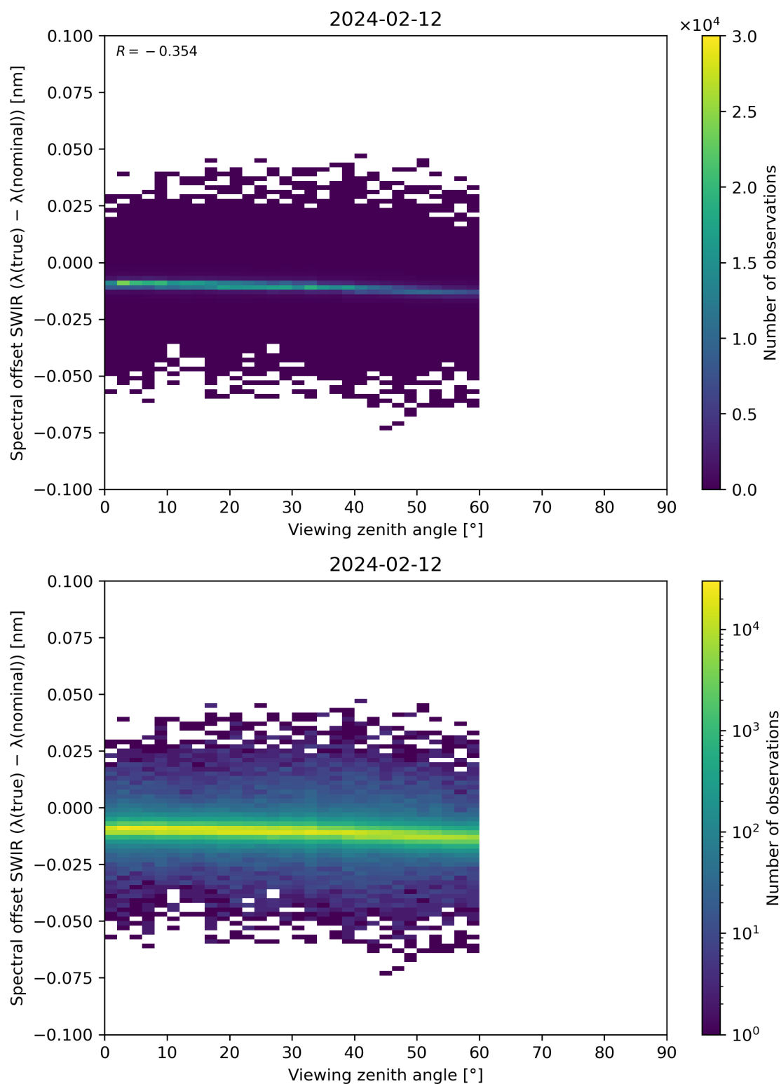
Figure 116: Scatter density plot of “Viewing zenith angle” against “Spectral offset SWIR ( \lambda(\text{true}) - \lambda(\text{nominal}) )” for 2024-02-11 to 2024-02-13.
