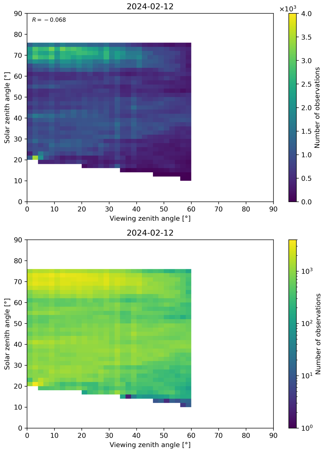
Figure 115: Scatter density plot of “Viewing zenith angle” against “Solar zenith angle” for 2024-02-11 to 2024-02-13.
