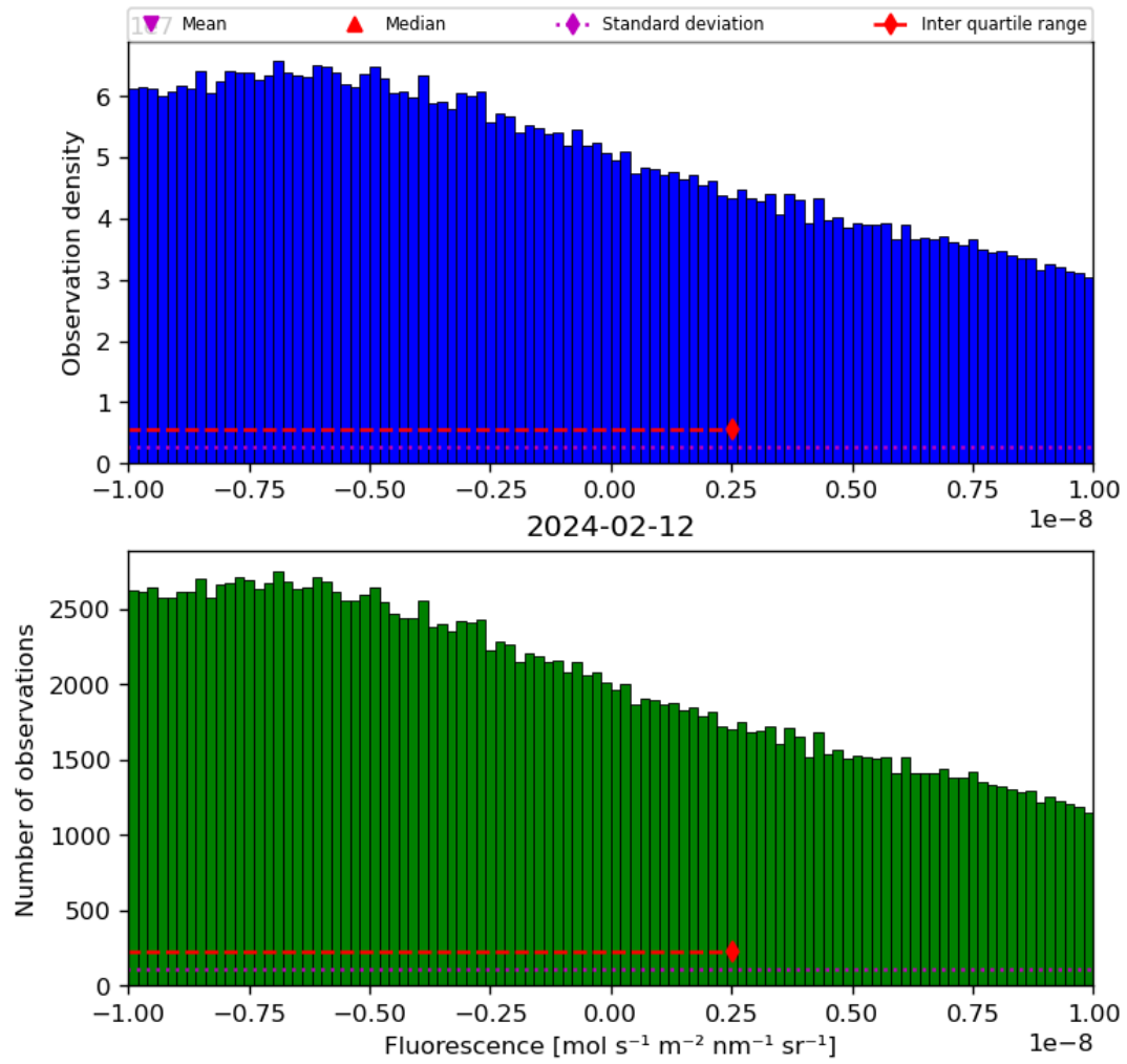
Figure 32: Histogram of “Fluorescence” for 2024-02-11 to 2024-02-13
