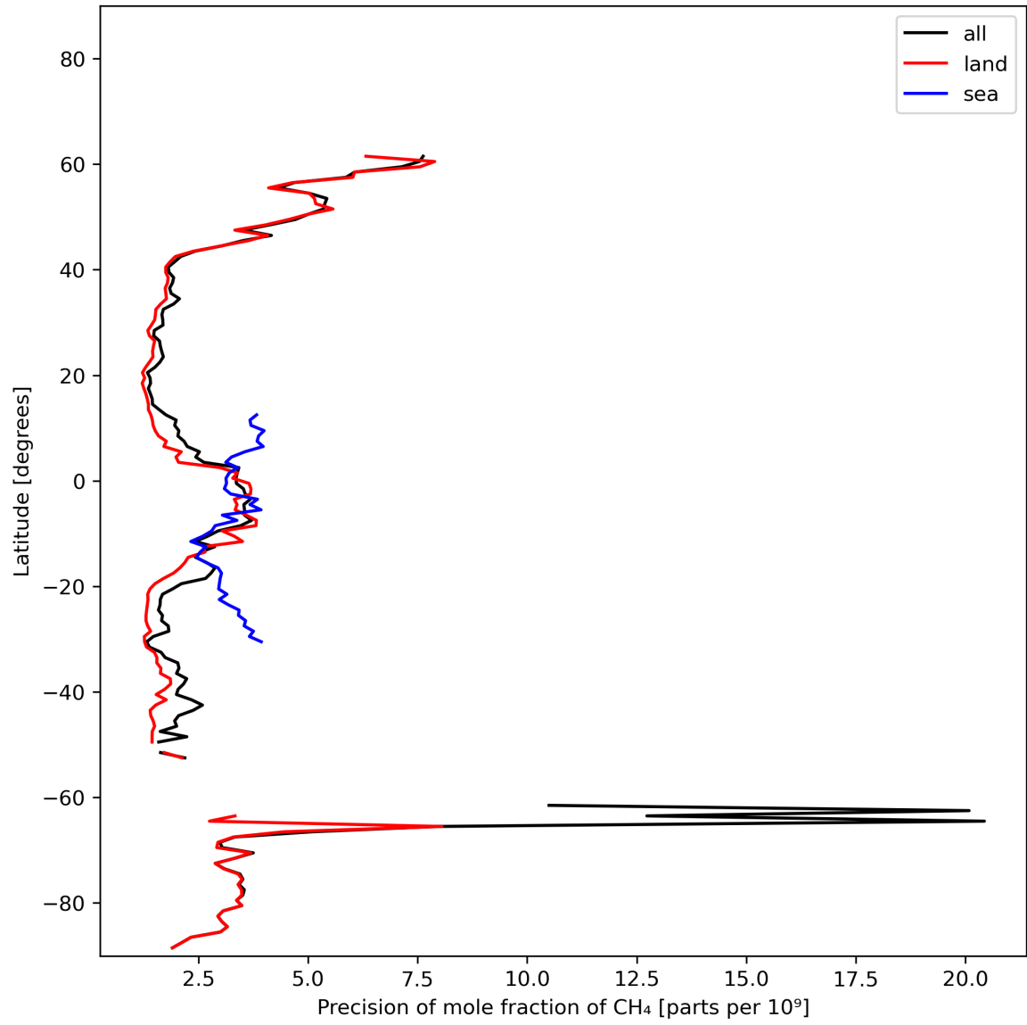
Figure 13: Zonal average of “Precision of mole fraction of CH 4 ” for 2024-02-11 to 2024-02-13.
