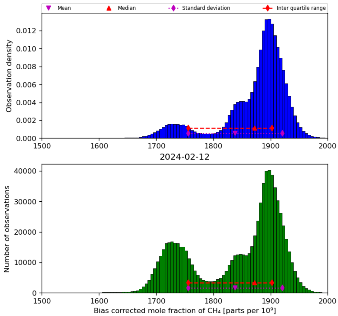
Figure 25: Histogram of “Bias corrected mole fraction of CH 4 ” for 2024-02-11 to 2024-02-13
