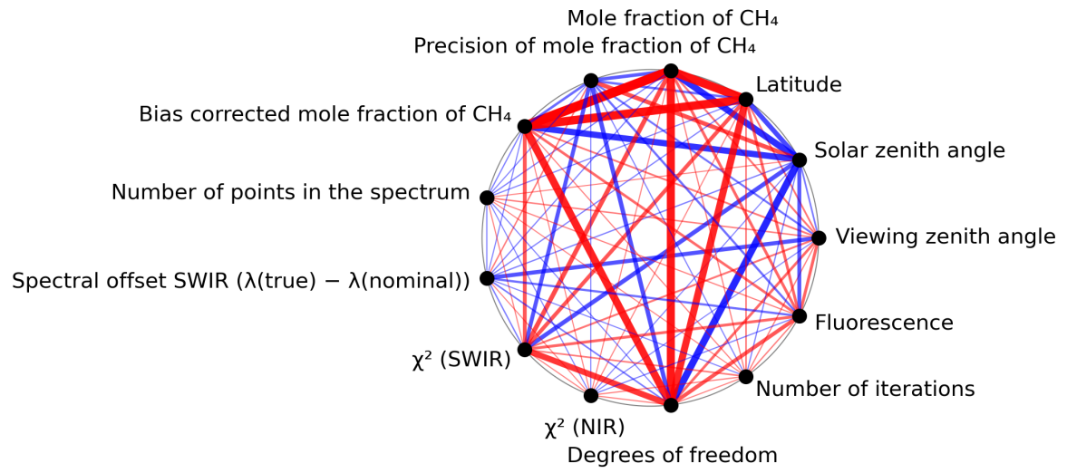
Figure 1: Map of correlation graph for 2024-02-11 to 2024-02-13.
