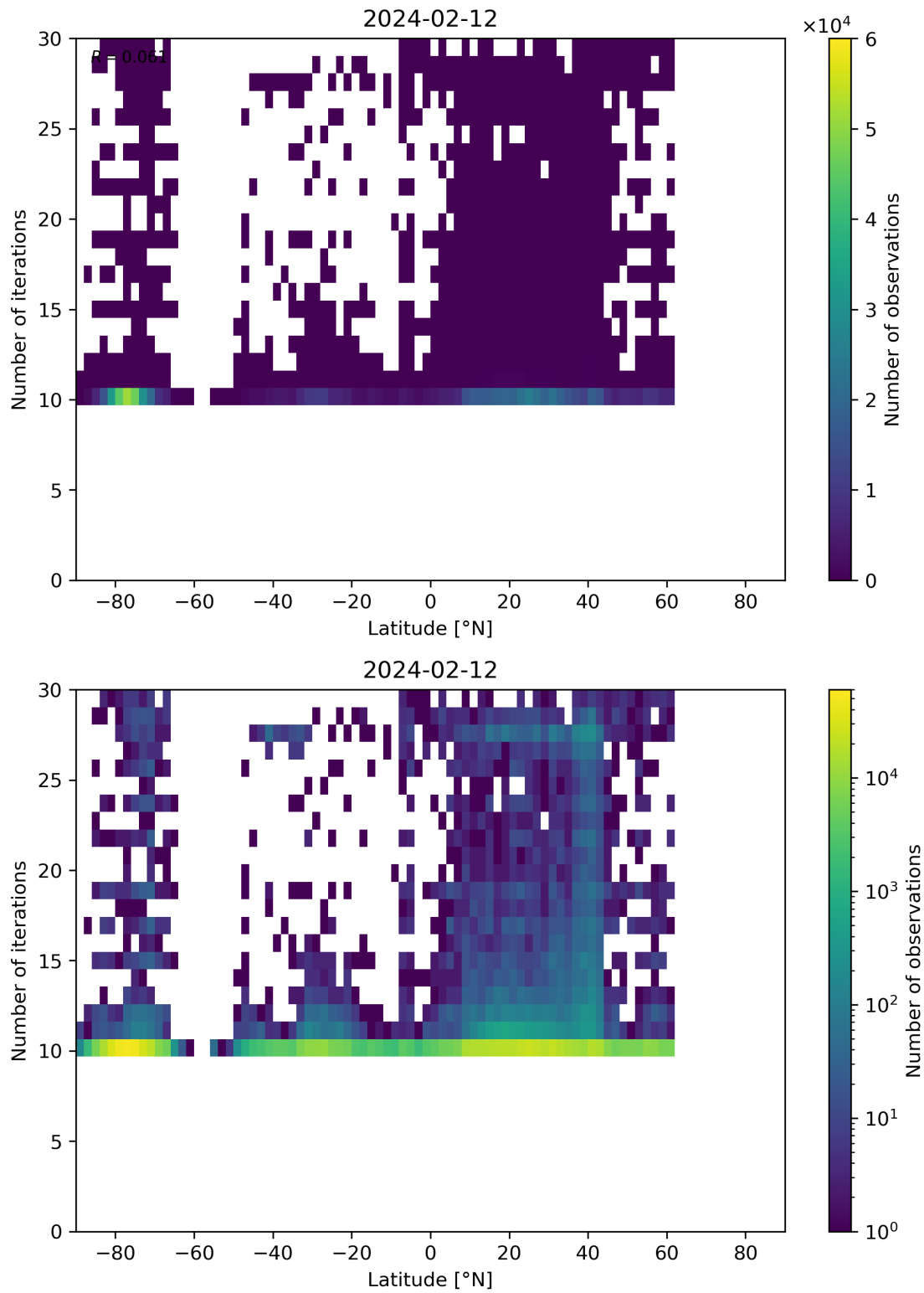
Figure 60: Scatter density plot of “Latitude” against “Number of iterations” for 2024-02-11 to 2024-02-13.
