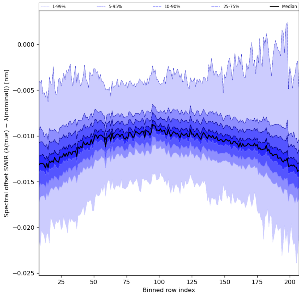
Figure 38: Along track statistics of “Spectral offset SWIR ( \lambda(\text{true}) - \lambda(\text{nominal}) )” for 2024-02-11 to 2024-02-13
