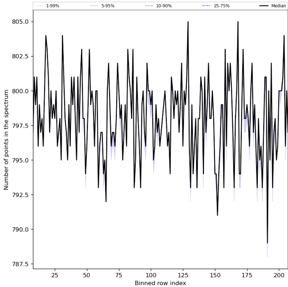
Figure 37: Along track statistics of “Number of points in the spectrum” for 2024-02-11 to 2024-02-13
