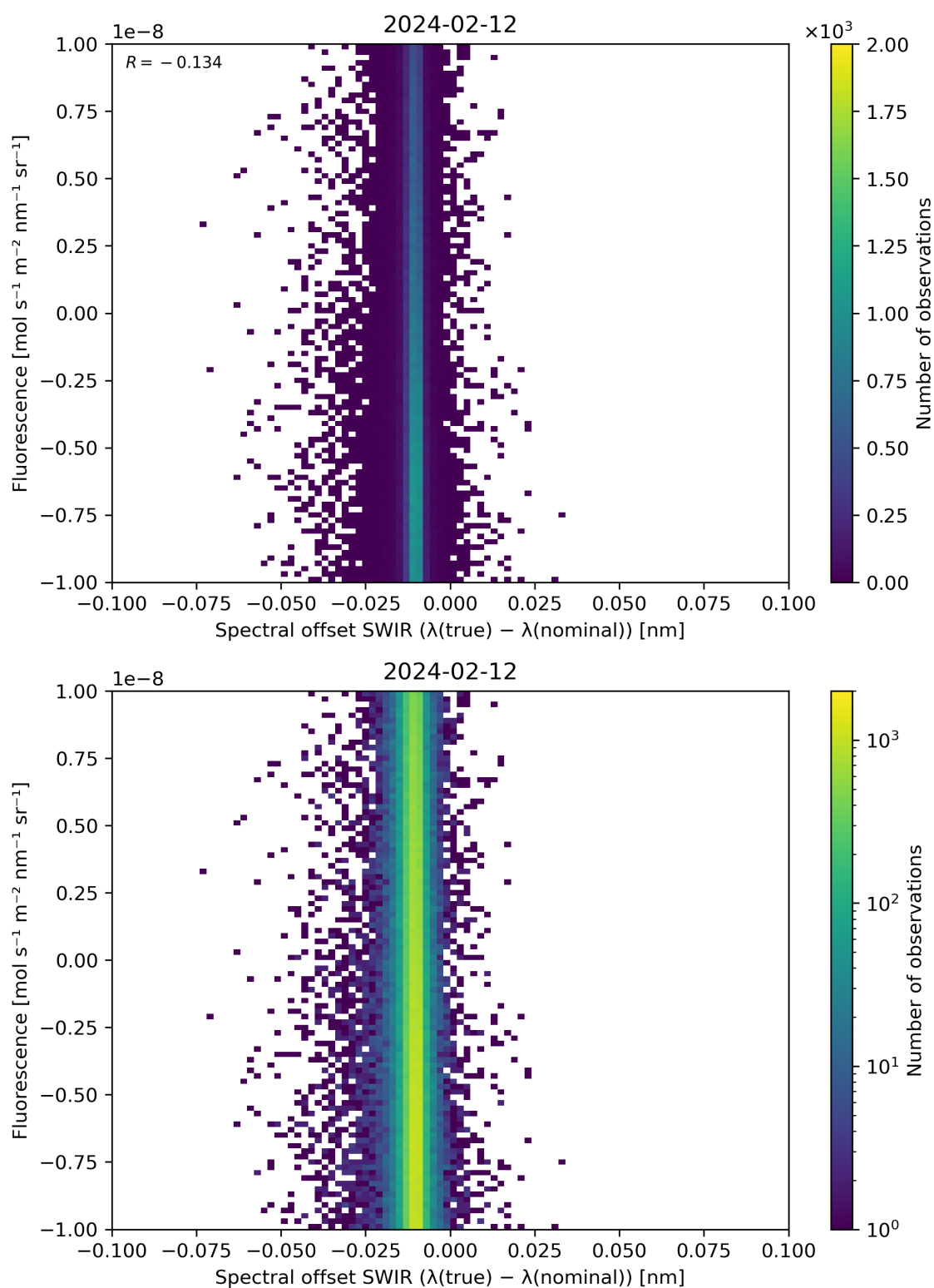
Figure 120: Scatter density plot of “Spectral offset SWIR ( \lambda(\text{true}) - \lambda(\text{nominal}) )” against “Fluorescence” for 2024-02-11 to 2024-02-13.
