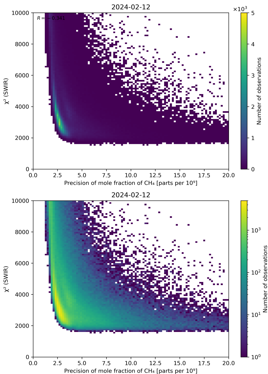
Figure 79: Scatter density plot of “Precision of mole fraction of \text{CH}_4 ” against “ \chi^2 (SWIR)” for 2024-02-11 to 2024-02-13.
