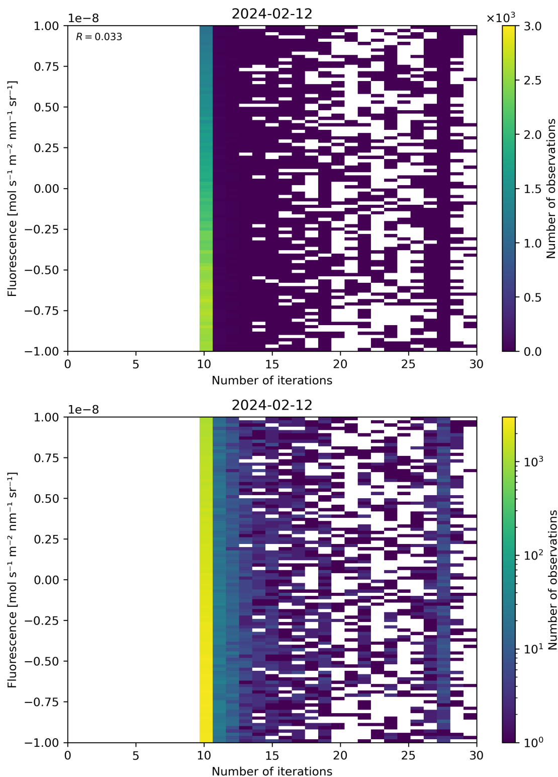
Figure 87: Scatter density plot of “Number of iterations” against “Fluorescence” for 2024-02-11 to 2024-02-13.
