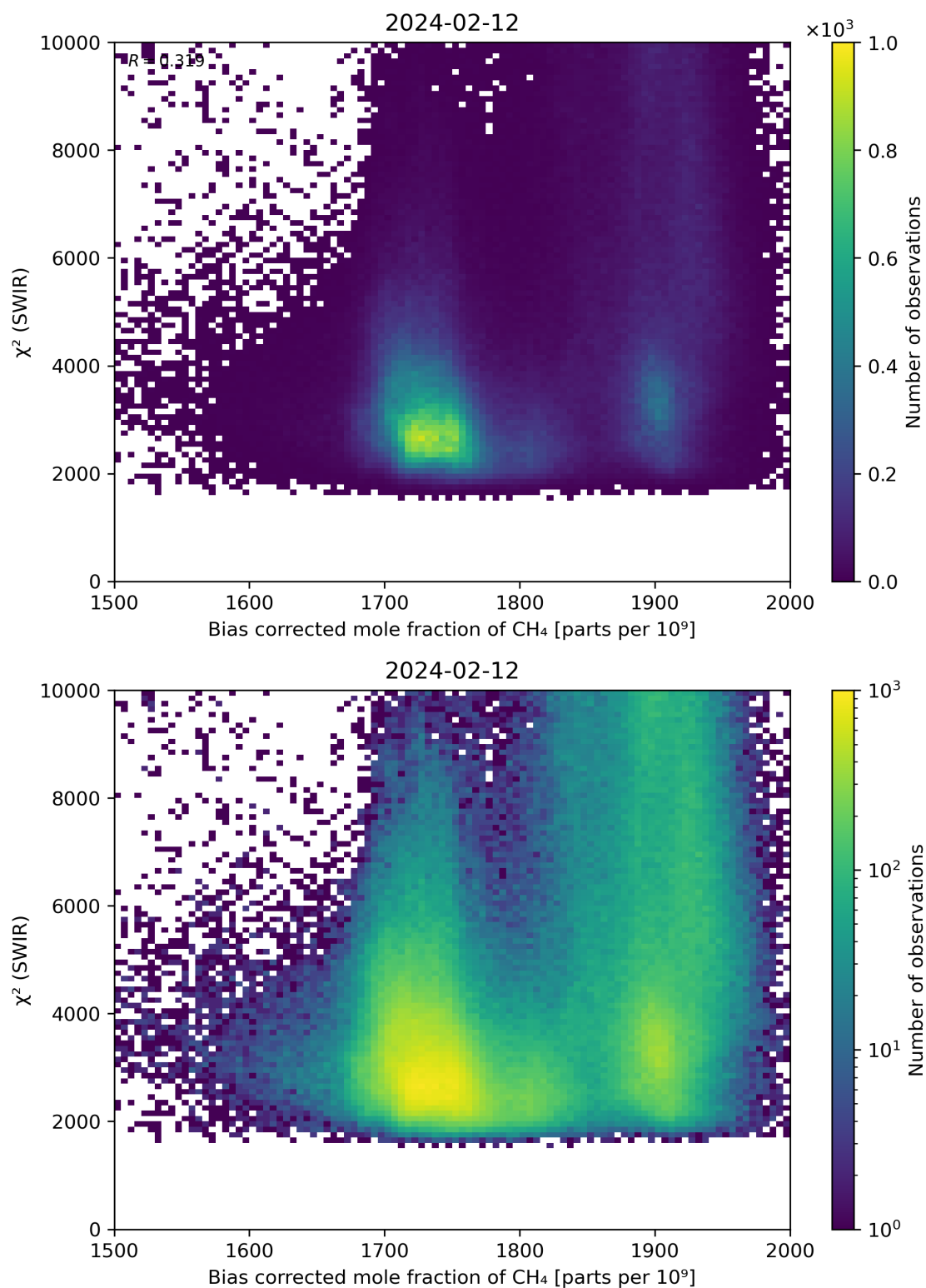
Figure 64: Scatter density plot of “Bias corrected mole fraction of \text{CH}_4 ” against “ \chi^2 (SWIR)” for 2024-02-11 to 2024-02-13.
