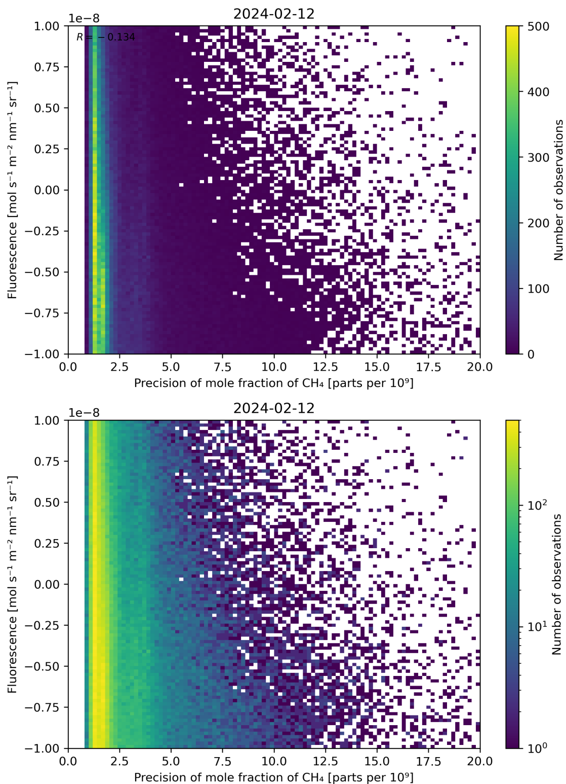
Figure 81: Scatter density plot of “Precision of mole fraction of \text{CH}_4 ” against “Fluorescence” for 2024-02-11 to 2024-02-13.
