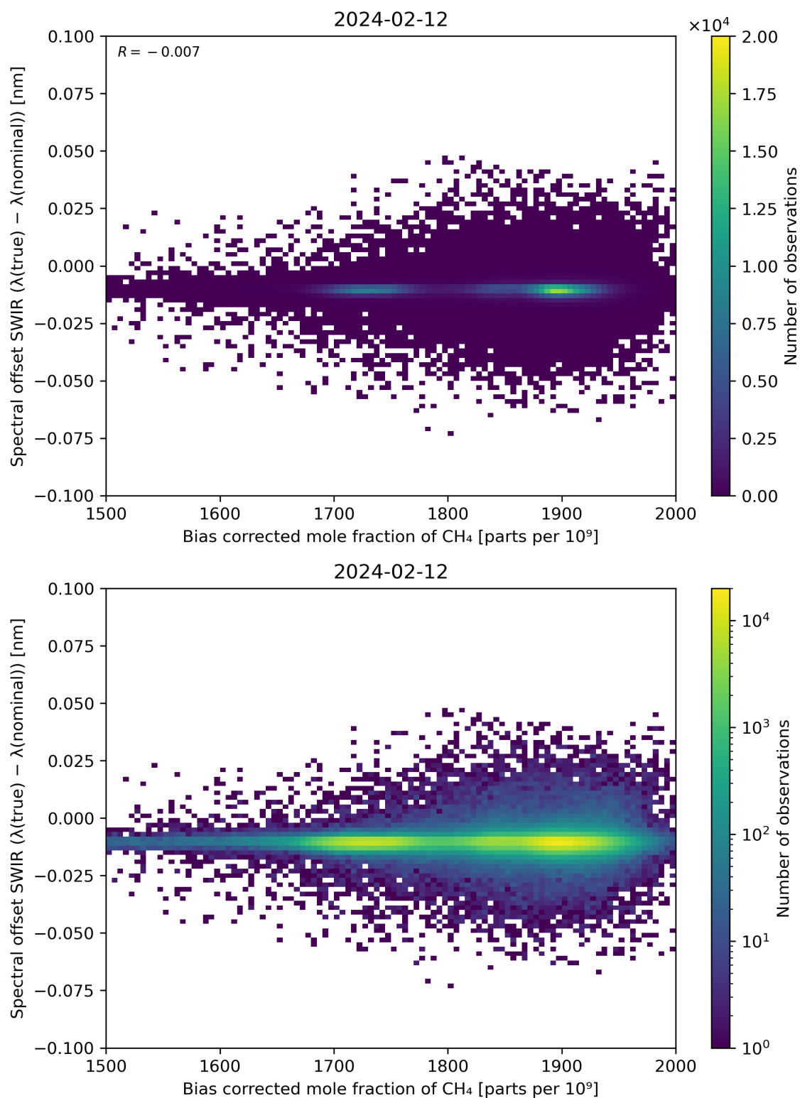
Figure 69: Scatter density plot of “Bias corrected mole fraction of \text{CH}_4 ” against “Spectral offset SWIR ( \lambda(\text{true}) - \lambda(\text{nominal}) )” for 2024-02-11 to 2024-02-13.
