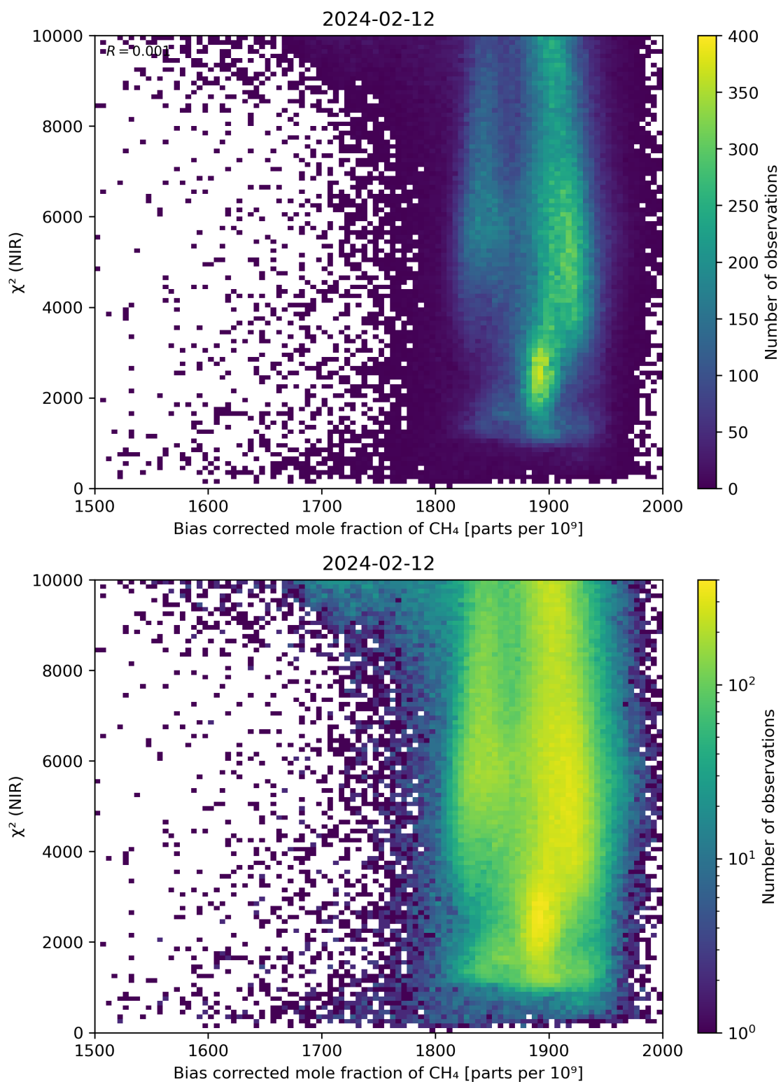
Figure 63: Scatter density plot of “Bias corrected mole fraction of CH 4 ” against “ \chi^2 (NIR)” for 2024-02-11 to 2024-02-13.
