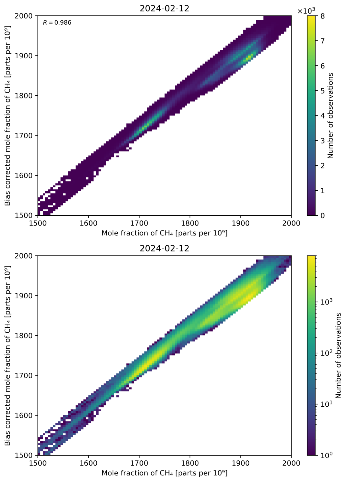
Figure 74: Scatter density plot of “Mole fraction of CH 4 ” against “Bias corrected mole fraction of CH 4 ” for 2024-02-11 to 2024-02-13.
