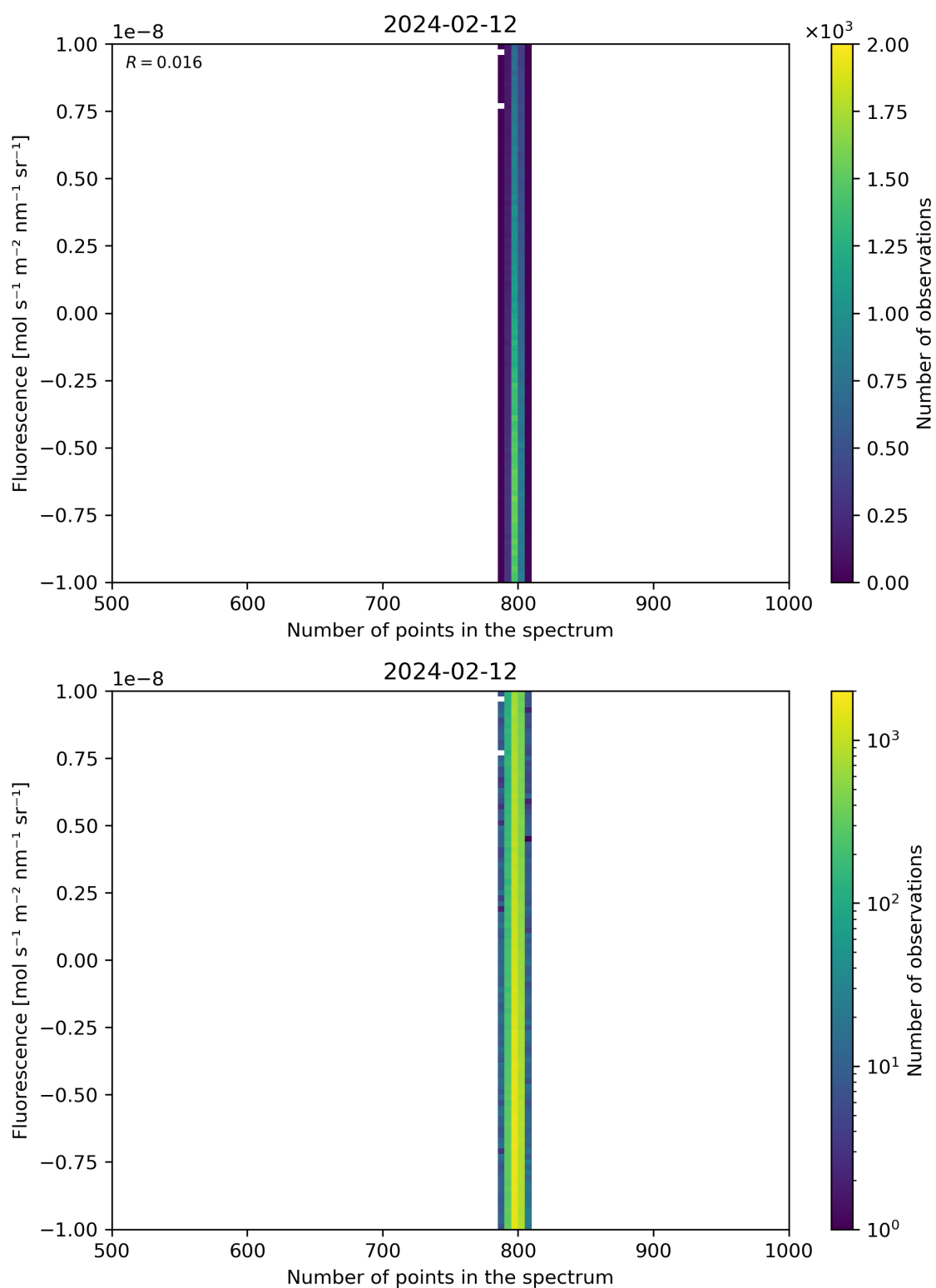
Figure 91: Scatter density plot of “Number of points in the spectrum” against “Fluorescence” for 2024-02-11 to 2024-02-13.
