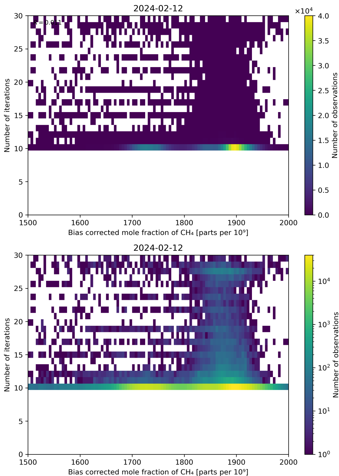
Figure 67: Scatter density plot of “Bias corrected mole fraction of CH 4 ” against “Number of iterations” for 2024-02-11 to 2024-02-13.
