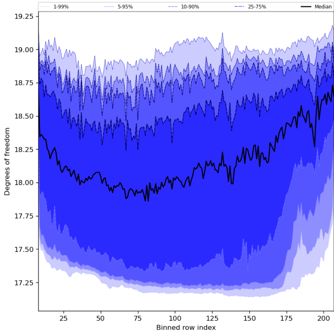
Figure 41: Along track statistics of “Degrees of freedom” for 2024-02-11 to 2024-02-13
