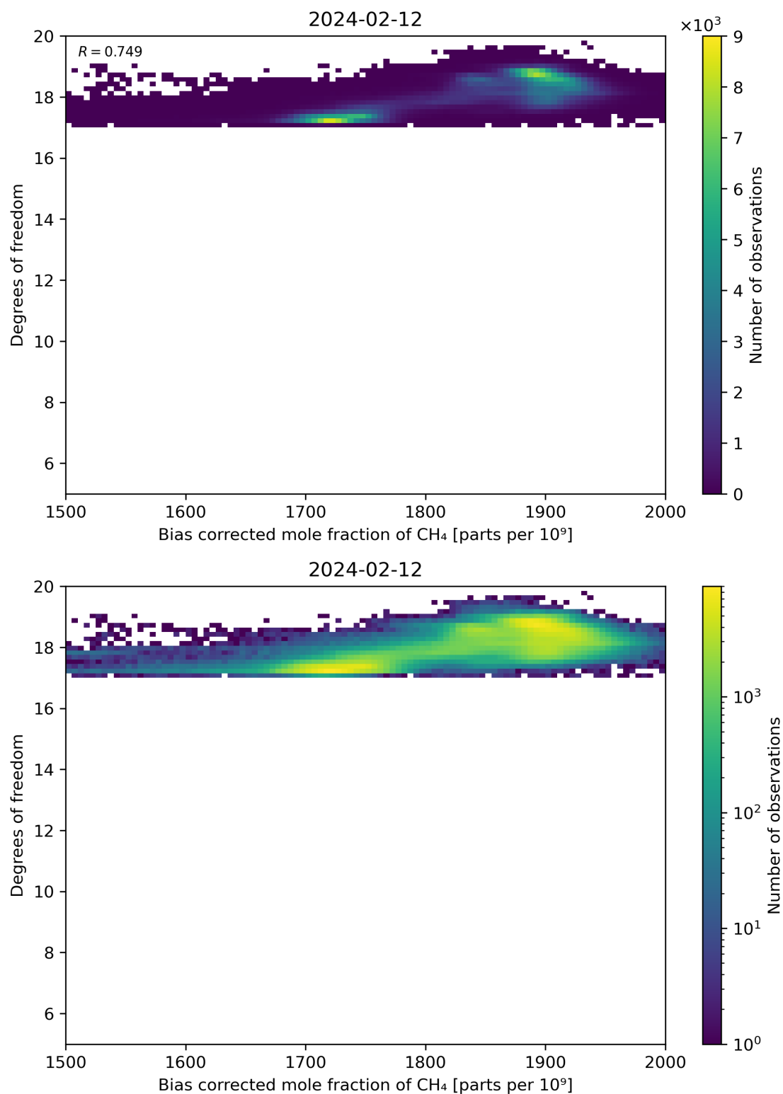
Figure 65: Scatter density plot of “Bias corrected mole fraction of CH 4 ” against “Degrees of freedom” for 2024-02-11 to 2024-02-13.
