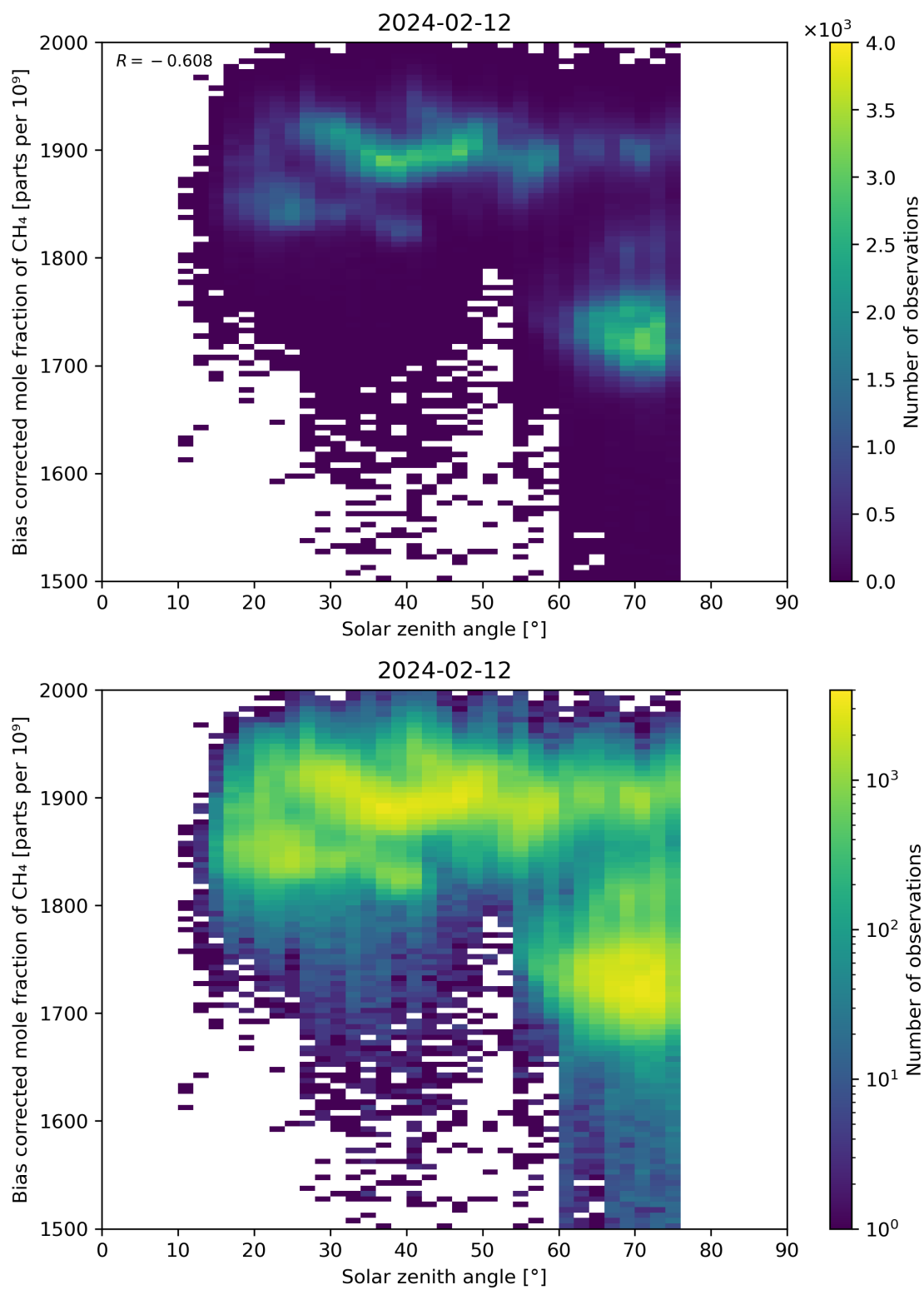
Figure 100: Scatter density plot of “Solar zenith angle” against “Bias corrected mole fraction of \text{CH}_4 ” for 2024-02-11 to 2024-02-13.
