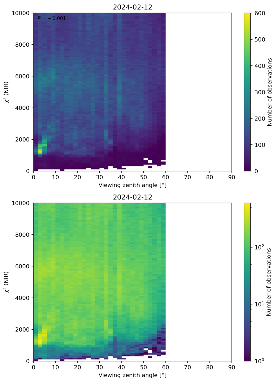
Figure 105: Scatter density plot of “Viewing zenith angle” against “ \chi^2 (NIR)” for 2024-02-11 to 2024-02-13.
