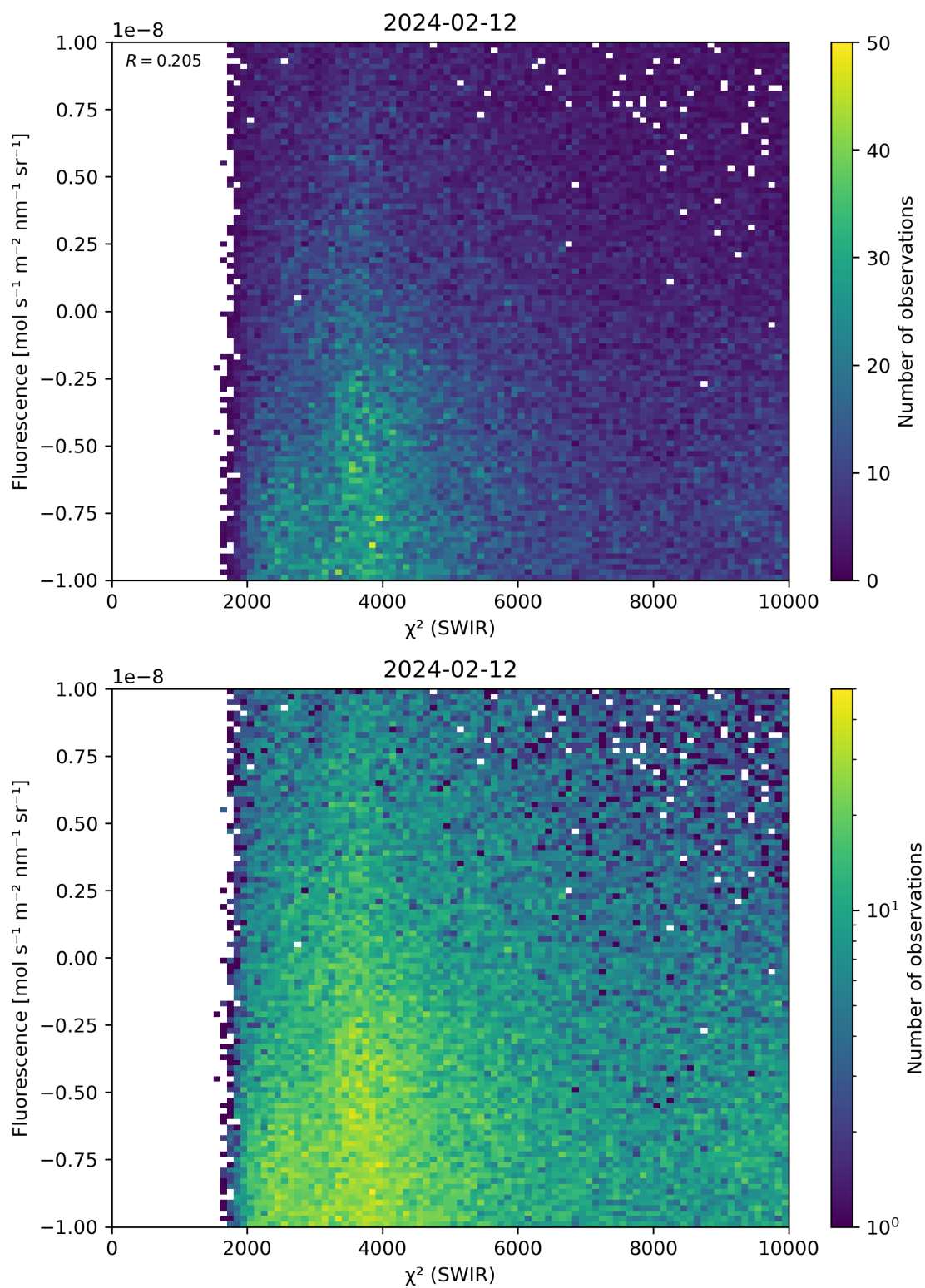
Figure 49: Scatter density plot of “ \chi^2 (SWIR)” against “Fluorescence” for 2024-02-11 to 2024-02-13.
