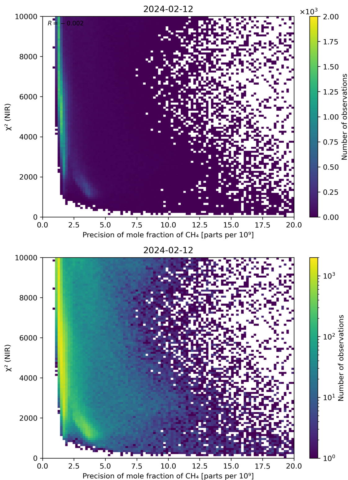
Figure 78: Scatter density plot of “Precision of mole fraction of CH 4 ” against “ \chi^2 (NIR)” for 2024-02-11 to 2024-02-13.
