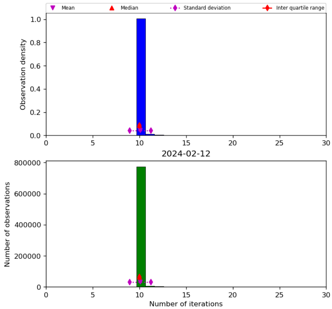
Figure 31: Histogram of “Number of iterations” for 2024-02-11 to 2024-02-13
