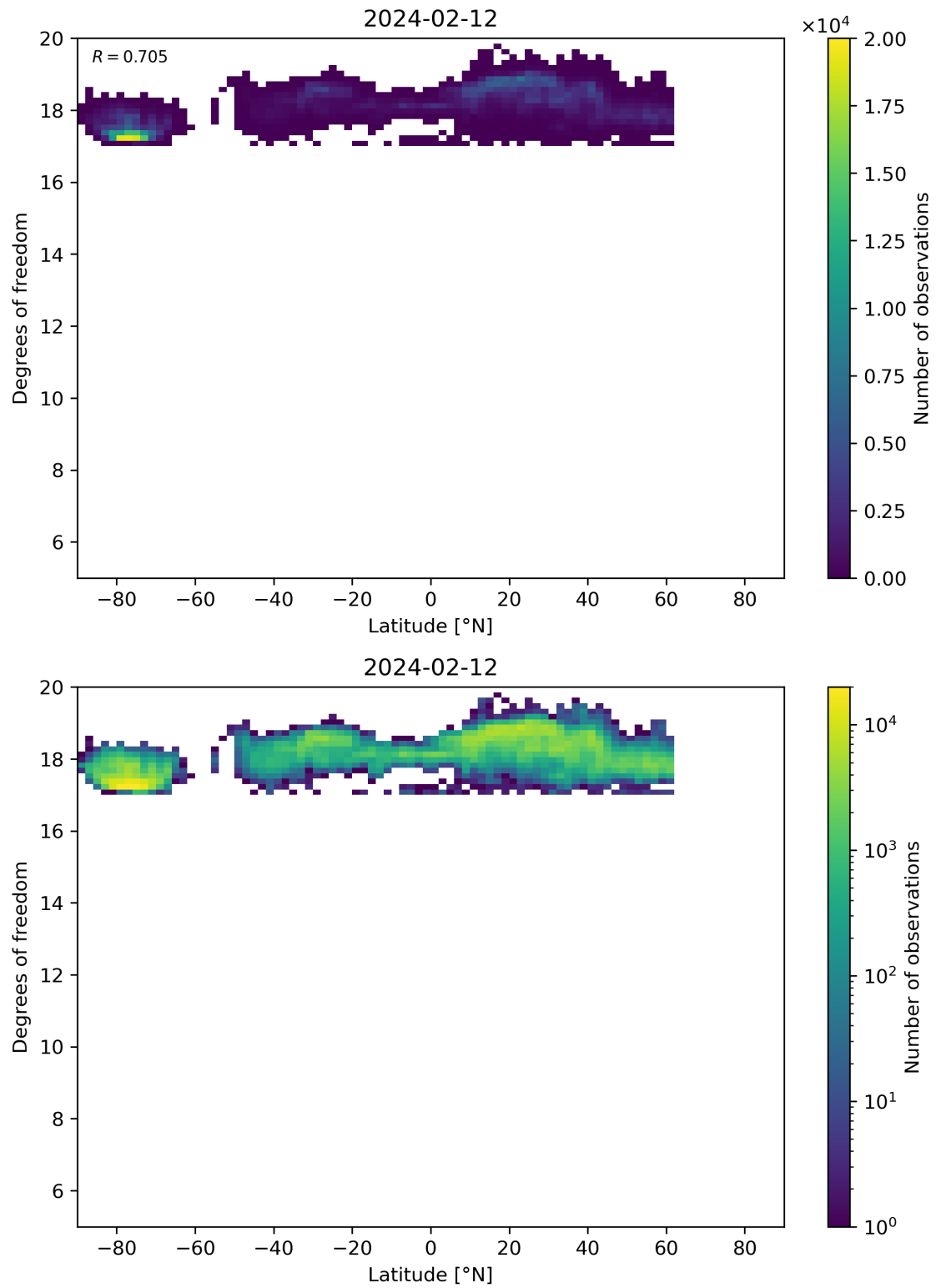
Figure 55: Scatter density plot of “Latitude” against “Degrees of freedom” for 2024-02-11 to 2024-02-13.
