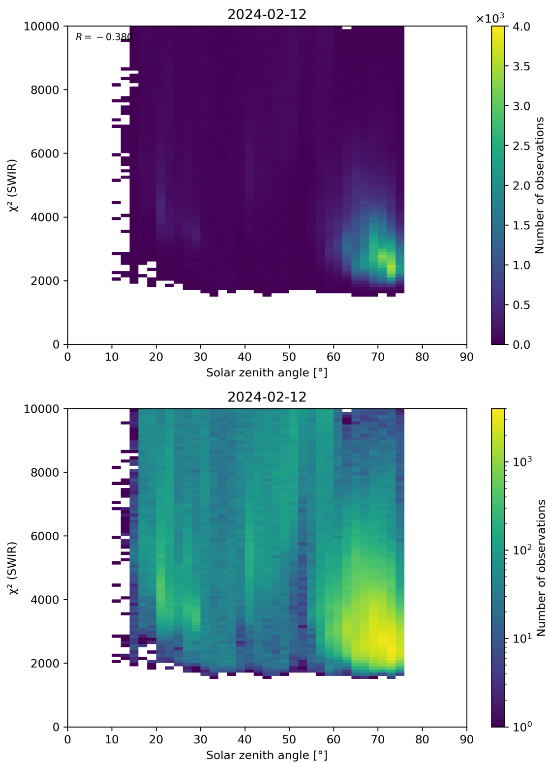
Figure 95: Scatter density plot of “Solar zenith angle” against “ \chi^2 (SWIR)” for 2024-02-11 to 2024-02-13.
