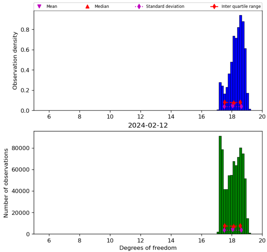
Figure 30: Histogram of “Degrees of freedom” for 2024-02-11 to 2024-02-13
