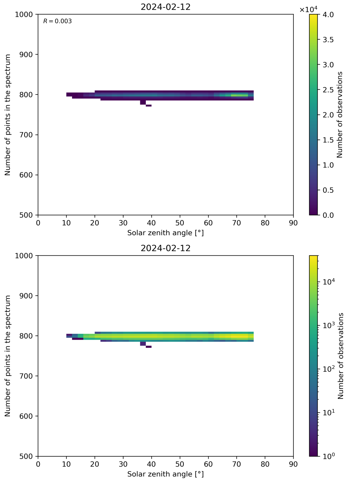
Figure 103: Scatter density plot of “Solar zenith angle” against “Number of points in the spectrum” for 2024-02-11 to 2024-02-13.
