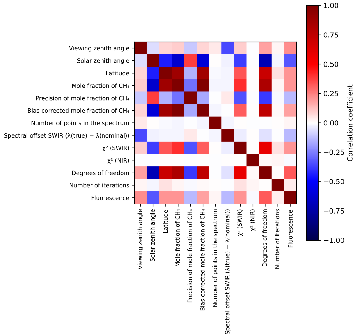
Figure 2: Map of correlation matrix for 2024-02-11 to 2024-02-13.
