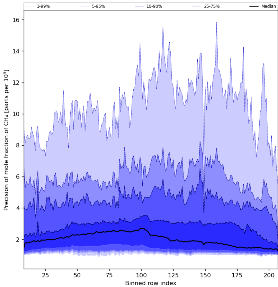
Figure 35: Along track statistics of “Precision of mole fraction of CH 4 ” for 2024-02-11 to 2024-02-13
