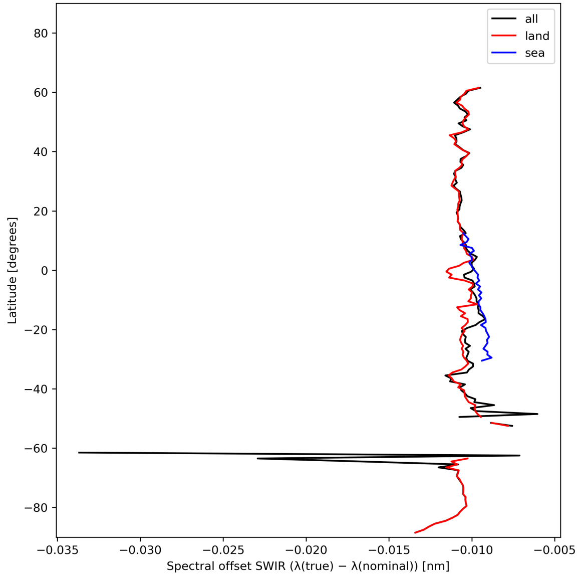
Figure 16: Zonal average of “Spectral offset SWIR ( \lambda(\text{true}) - \lambda(\text{nominal}) )” for 2024-02-11 to 2024-02-13.
