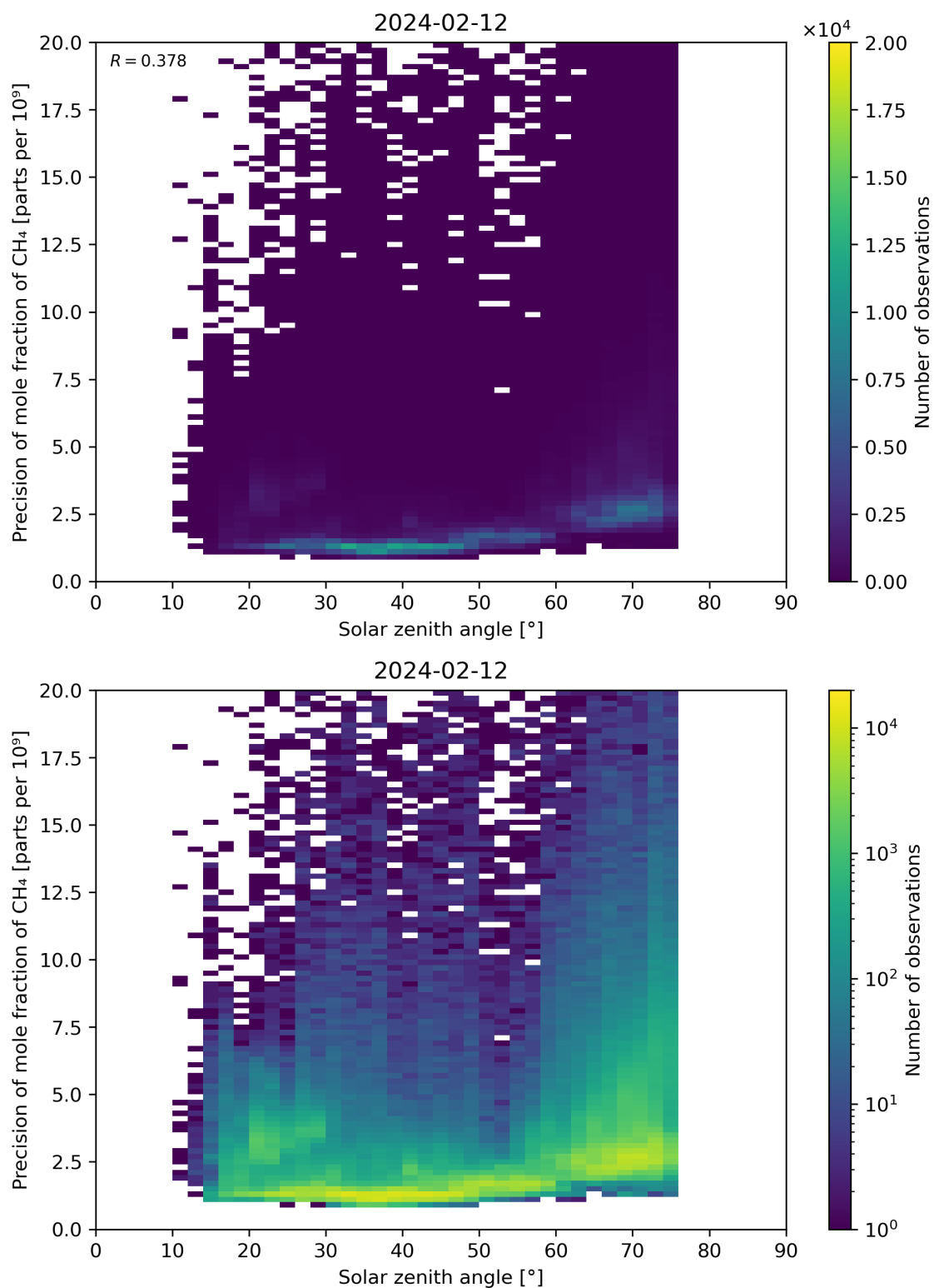
Figure 101: Scatter density plot of “Solar zenith angle” against “Precision of mole fraction of CH 4 ” for 2024-02-11 to 2024-02-13.
