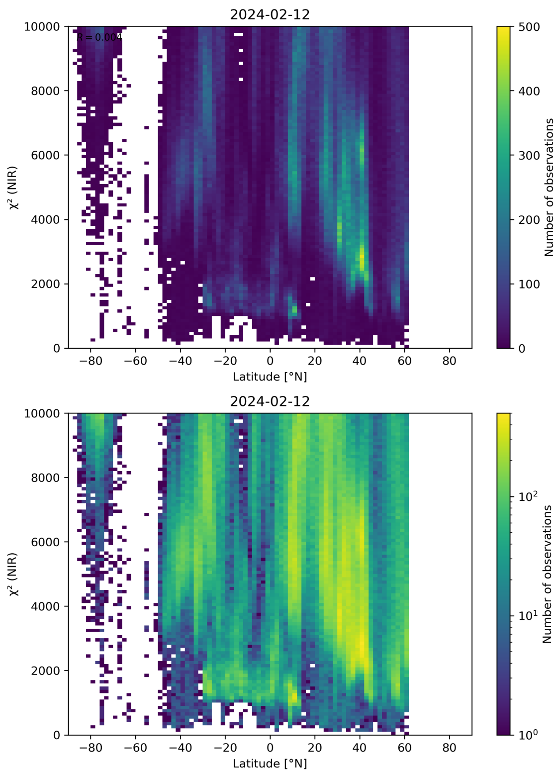
Figure 53: Scatter density plot of “Latitude” against “ \chi^2 (NIR)” for 2024-02-11 to 2024-02-13.
