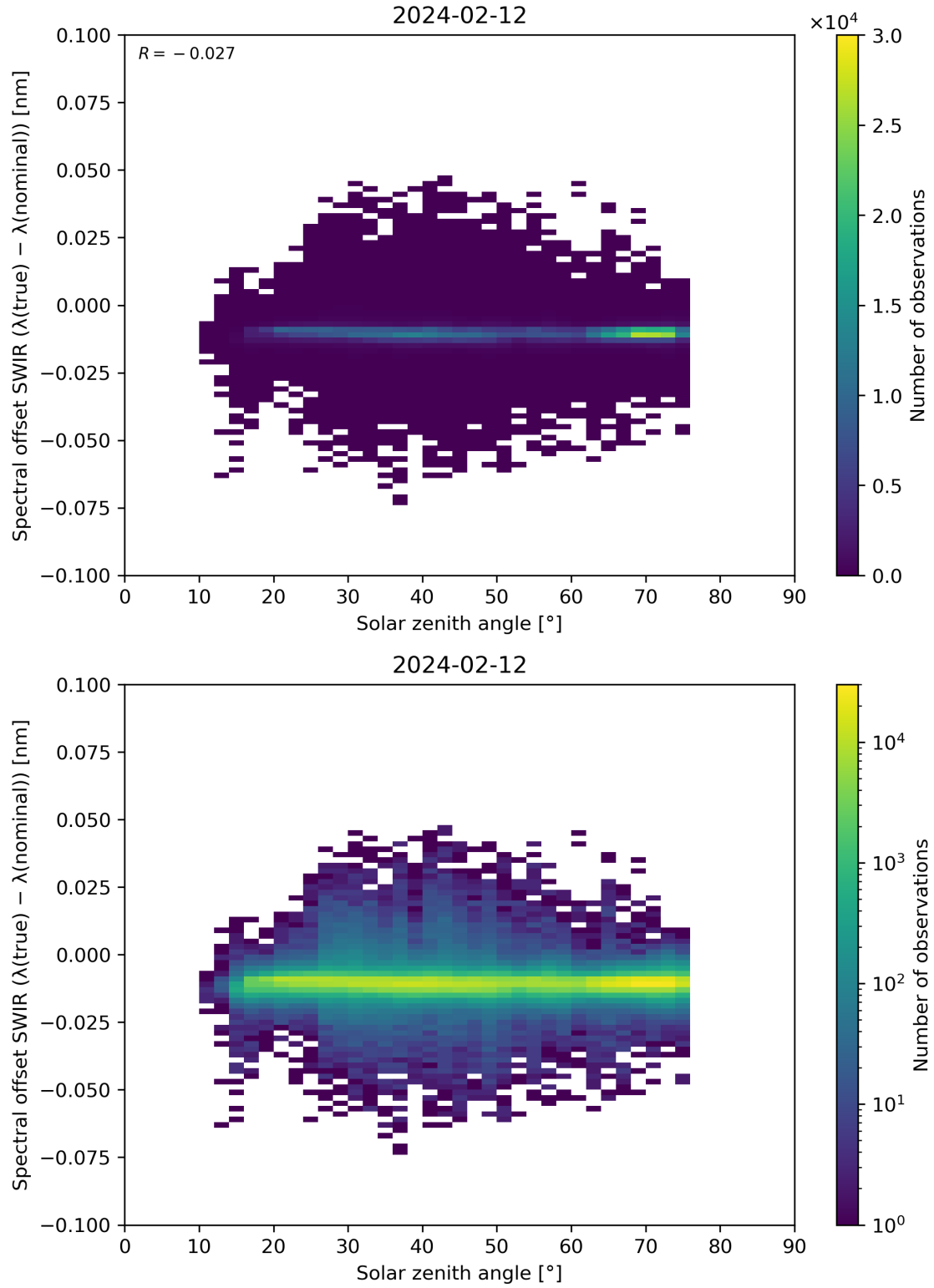
Figure 104: Scatter density plot of “Solar zenith angle” against “Spectral offset SWIR ( \lambda(\text{true}) - \lambda(\text{nominal}) )” for 2024-02-11 to 2024-02-13.
