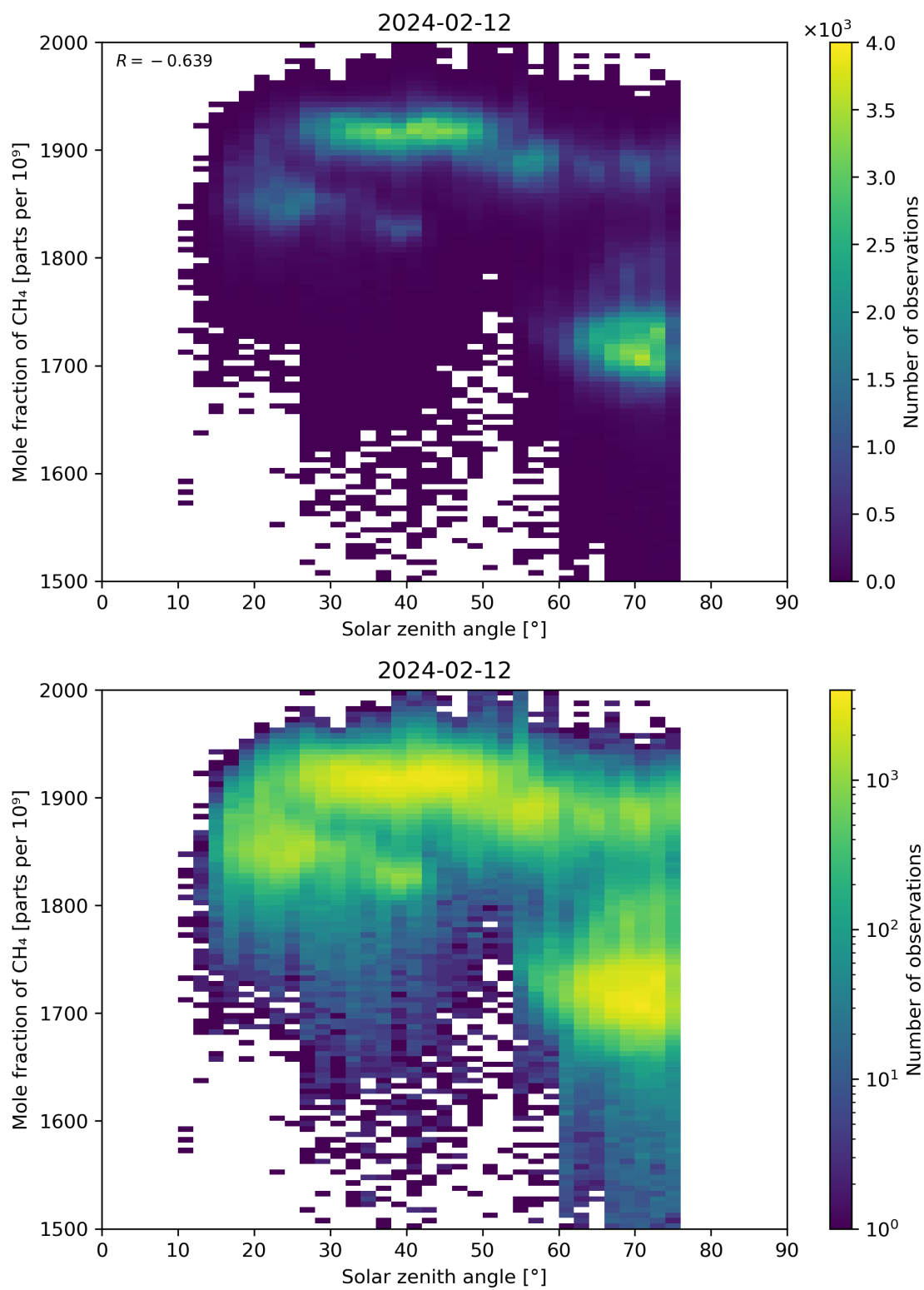
Figure 99: Scatter density plot of “Solar zenith angle” against “Mole fraction of CH 4 ” for 2024-02-11 to 2024-02-13.
