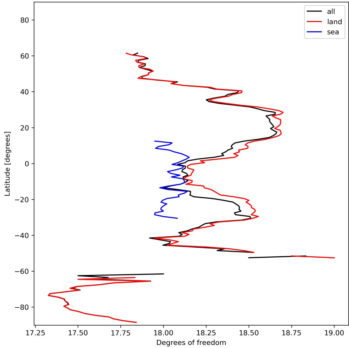
Figure 19: Zonal average of “Degrees of freedom” for 2024-02-11 to 2024-02-13.
