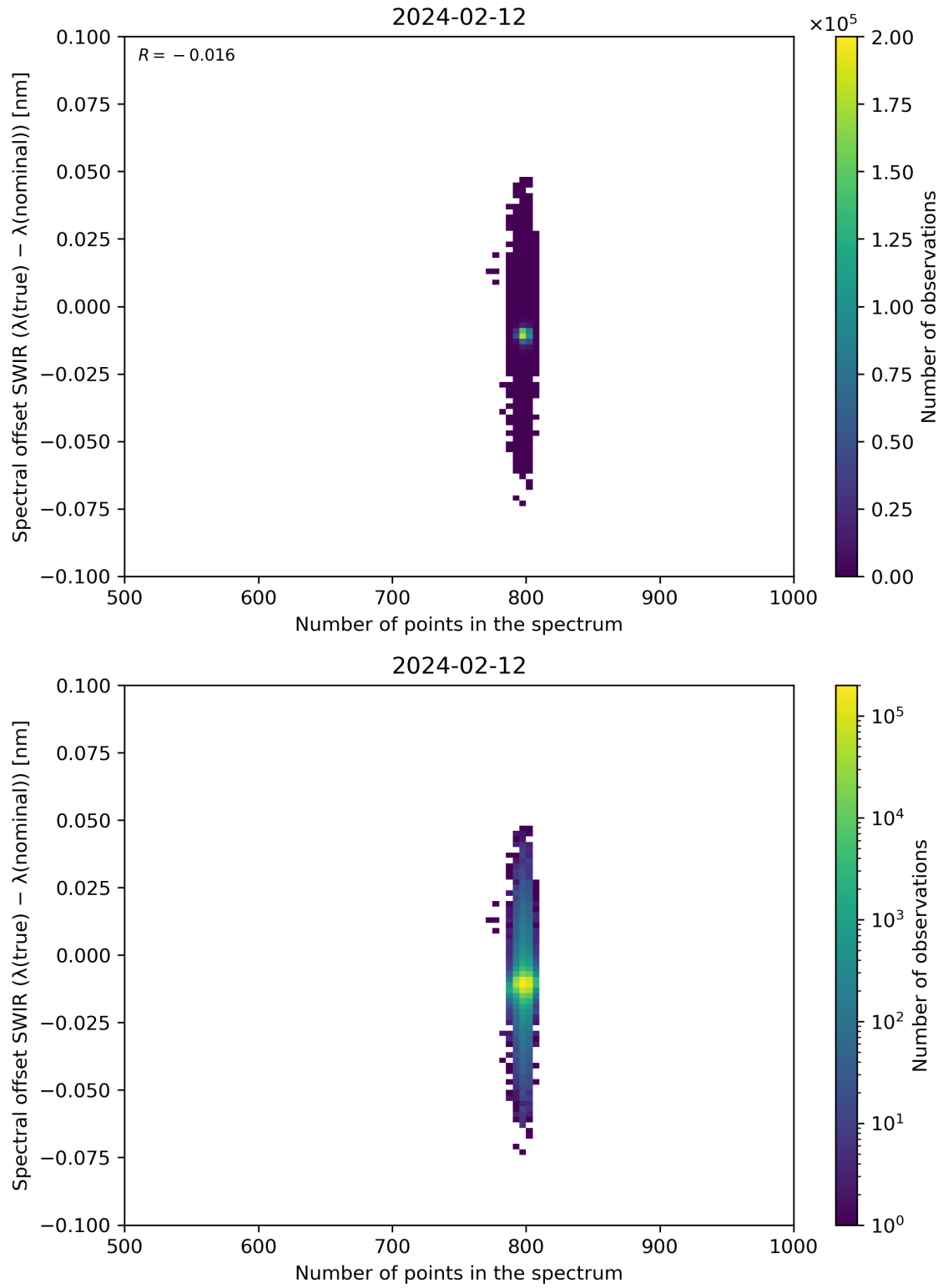
Figure 93: Scatter density plot of “Number of points in the spectrum” against “Spectral offset SWIR ( \lambda(\text{true}) - \lambda(\text{nominal}) )” for 2024-02-11 to 2024-02-13.
