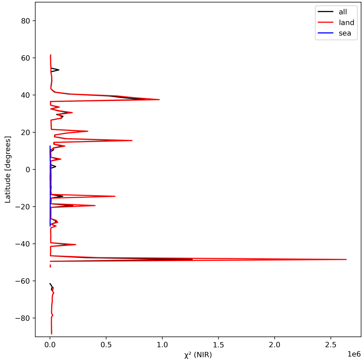
Figure 18: Zonal average of “ \chi^2 (NIR)” for 2024-02-11 to 2024-02-13.
