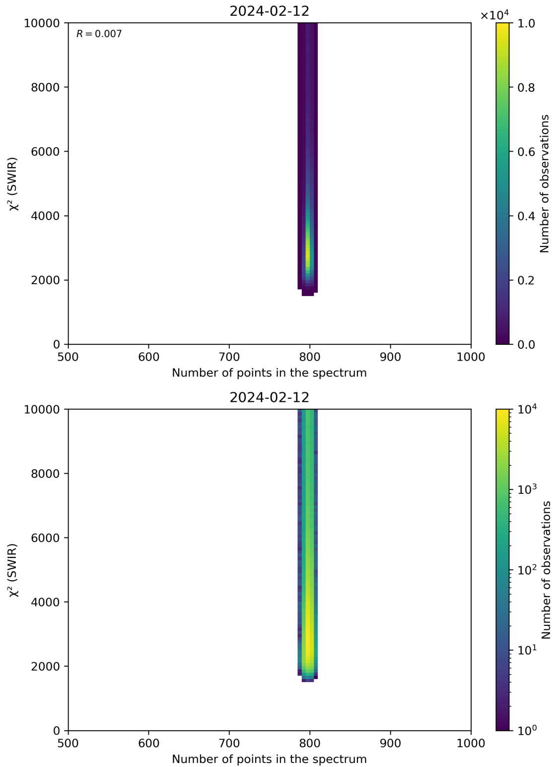
Figure 89: Scatter density plot of “Number of points in the spectrum” against “ \chi^2 (SWIR)” for 2024-02-11 to 2024-02-13.
