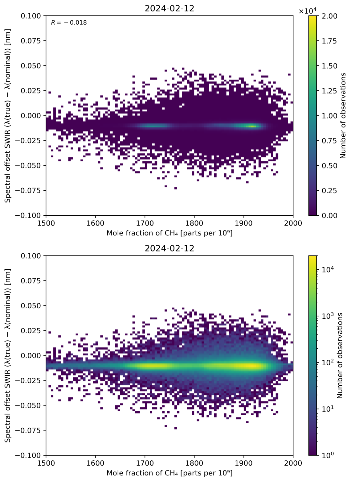
Figure 86: Scatter density plot of “Mole fraction of CH 4 ” against “Spectral offset SWIR ( \lambda(\text{true}) - \lambda(\text{nominal}) )” for 2024-02-11 to 2024-02-13.
