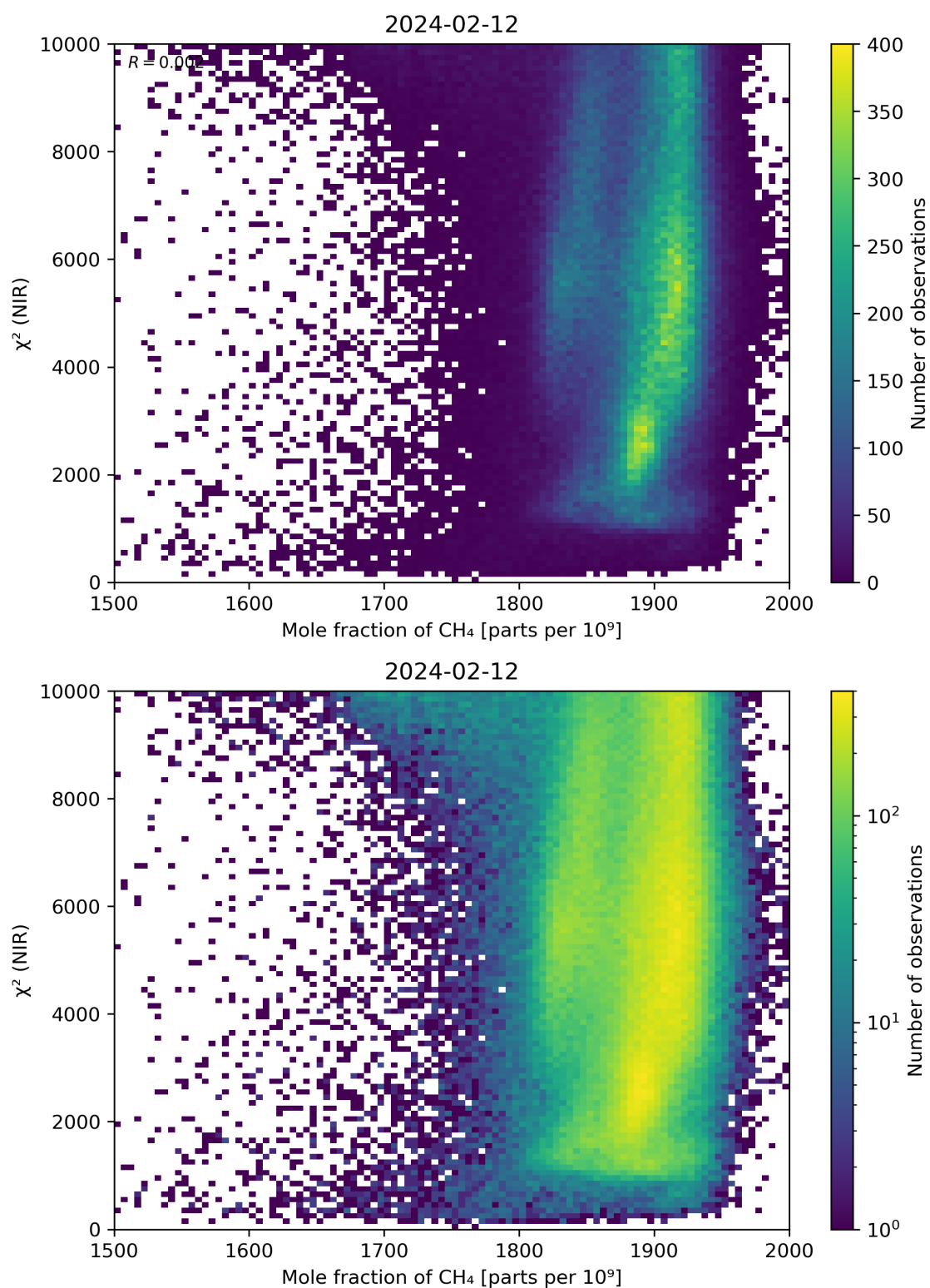
Figure 70: Scatter density plot of “Mole fraction of \text{CH}_4 ” against “ \chi^2 (NIR)” for 2024-02-11 to 2024-02-13.
