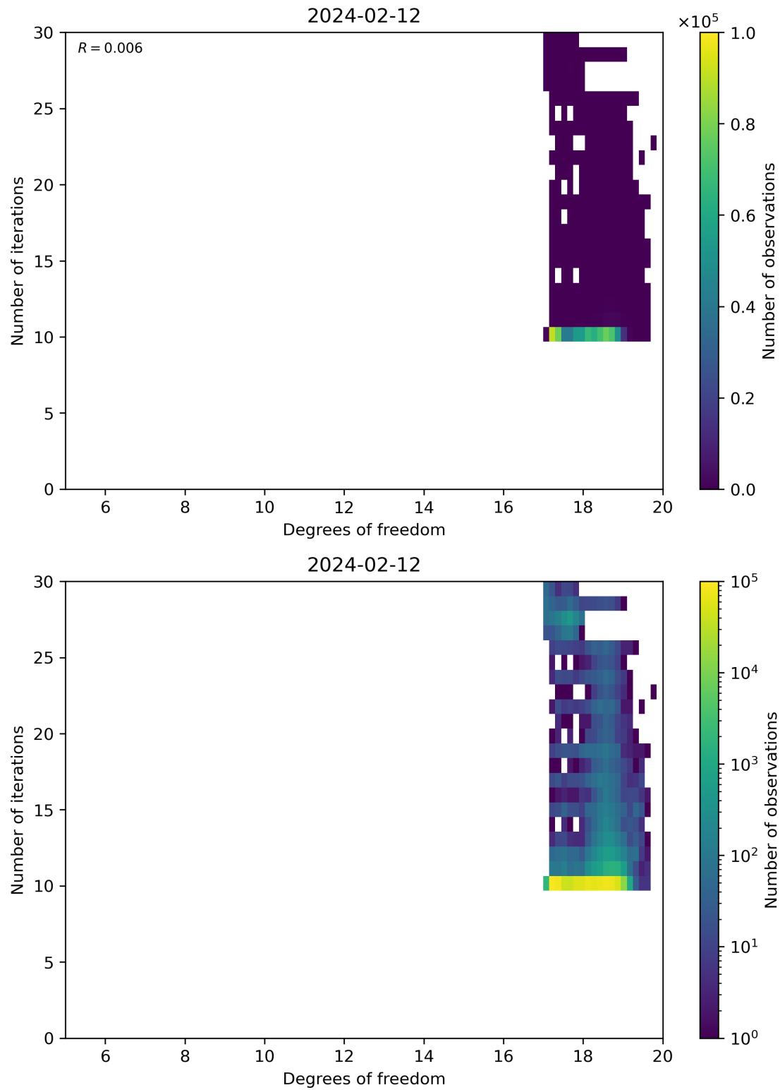
Figure 52: Scatter density plot of “Degrees of freedom” against “Number of iterations” for 2024-02-11 to 2024-02-13.
