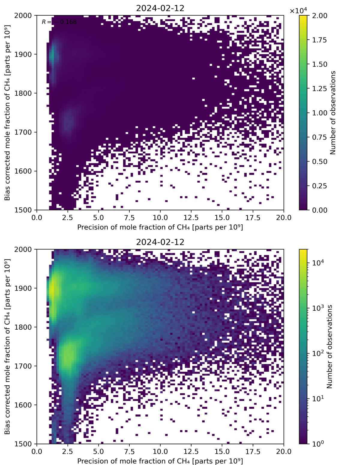
Figure 82: Scatter density plot of “Precision of mole fraction of \text{CH}_4 ” against “Bias corrected mole fraction of \text{CH}_4 ” for 2024-02-11 to 2024-02-13.
