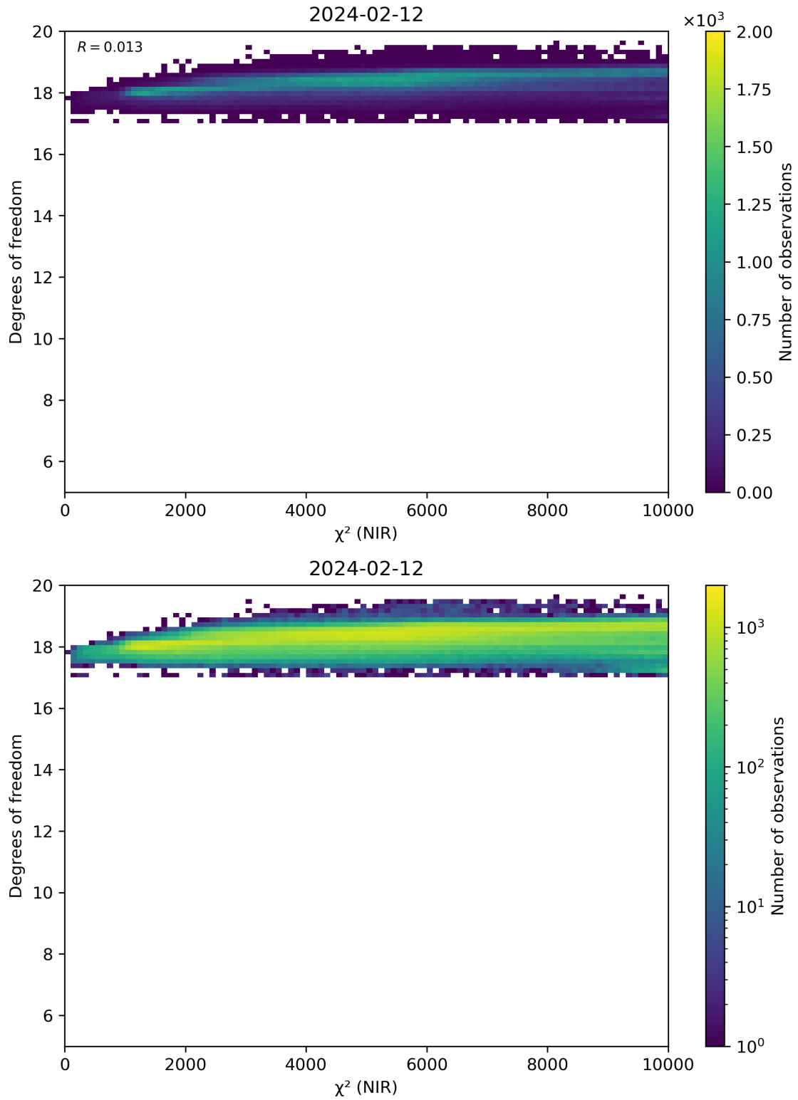
Figure 44: Scatter density plot of “ \chi^2 (NIR)” against “Degrees of freedom” for 2024-02-11 to 2024-02-13.
