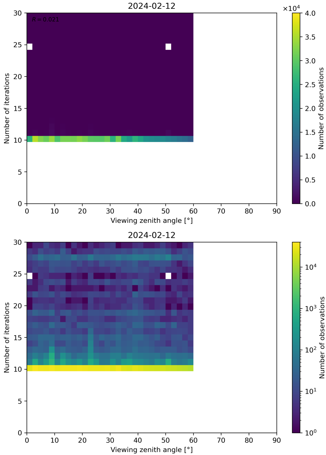
Figure 113: Scatter density plot of “Viewing zenith angle” against “Number of iterations” for 2024-02-11 to 2024-02-13.
