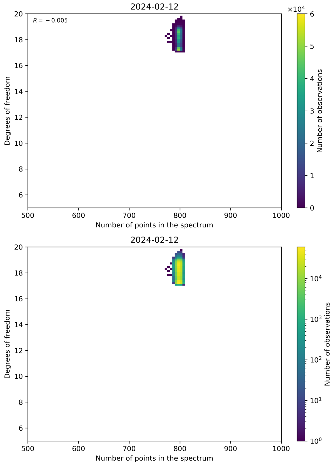
Figure 90: Scatter density plot of “Number of points in the spectrum” against “Degrees of freedom” for 2024-02-11 to 2024-02-13.
