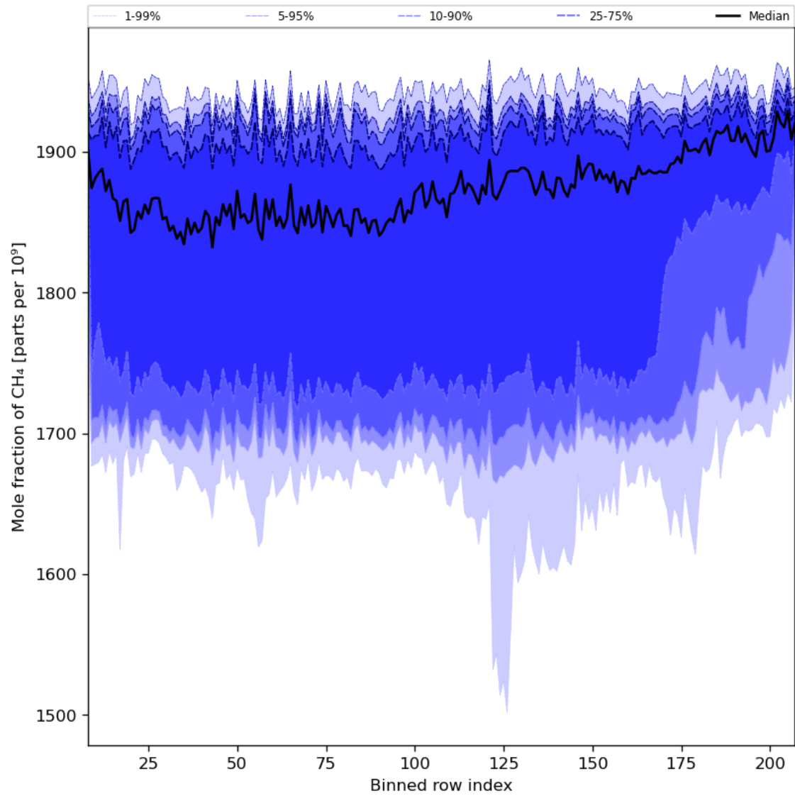
Figure 34: Along track statistics of “Mole fraction of CH 4 ” for 2024-02-11 to 2024-02-13
