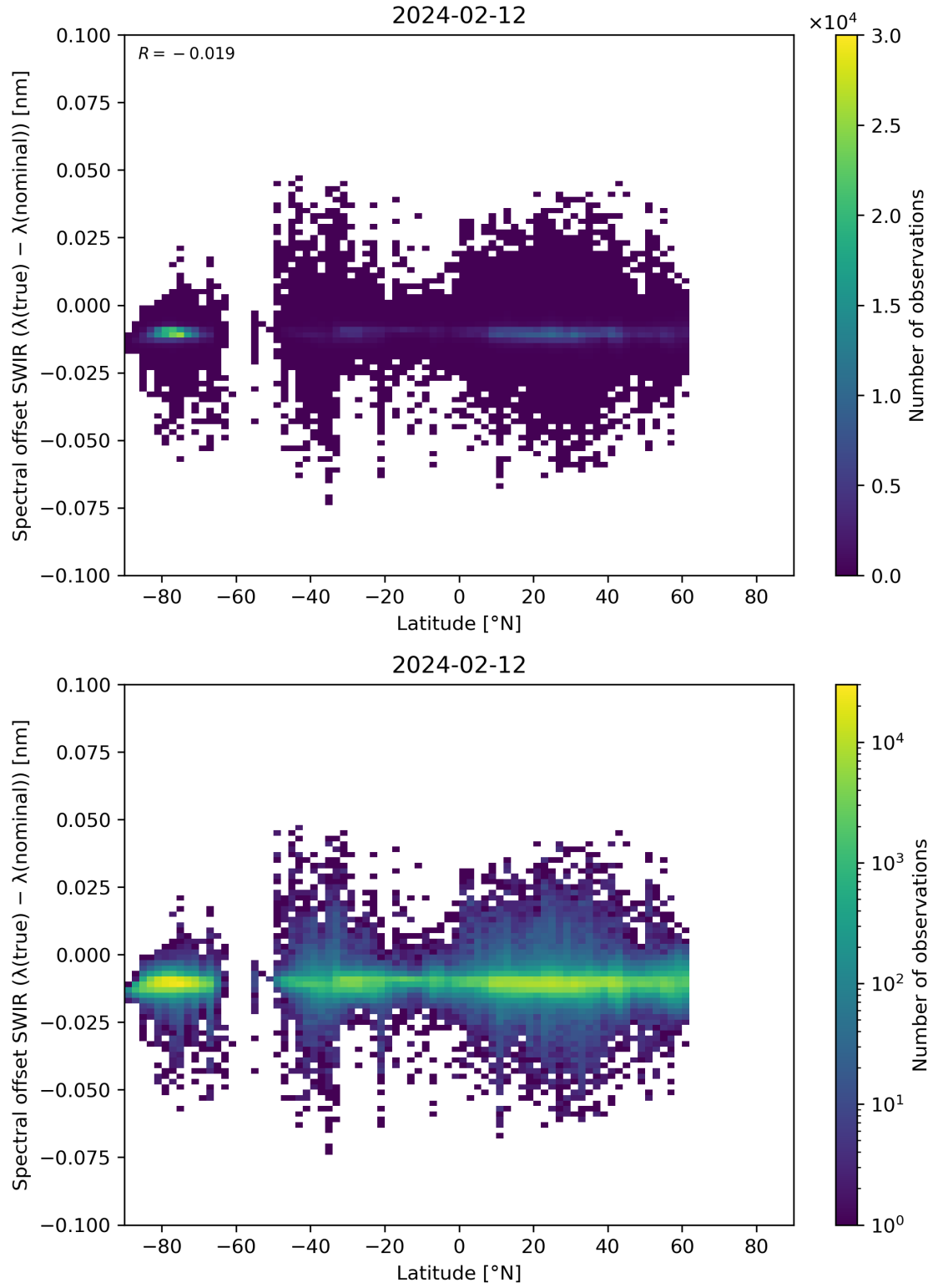
Figure 62: Scatter density plot of “Latitude” against “Spectral offset SWIR ( \lambda(\text{true}) - \lambda(\text{nominal}) )” for 2024-02-11 to 2024-02-13.
