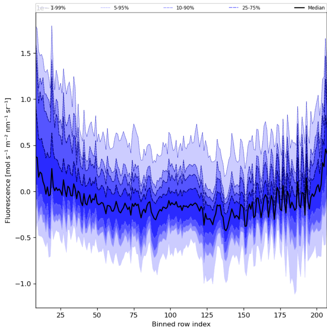
Figure 43: Along track statistics of “Fluorescence” for 2024-02-11 to 2024-02-13
