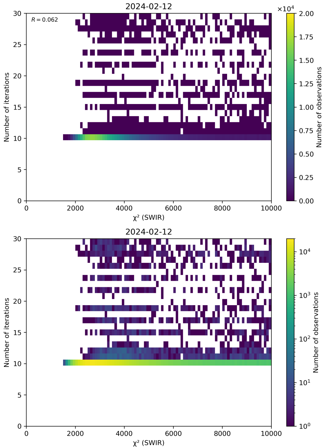
Figure 50: Scatter density plot of “ \chi^2 (SWIR)” against “Number of iterations” for 2024-02-11 to 2024-02-13.
