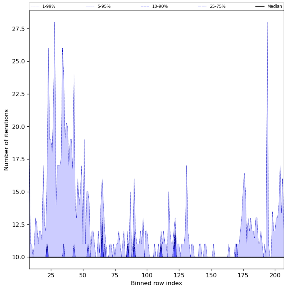
Figure 42: Along track statistics of “Number of iterations” for 2024-02-11 to 2024-02-13
