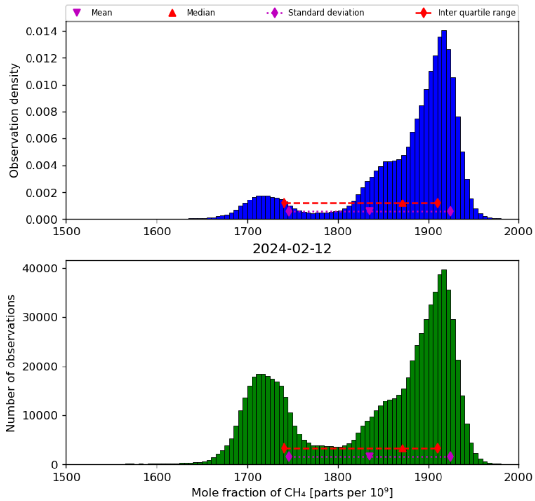
Figure 23: Histogram of “Mole fraction of CH 4 ” for 2024-02-11 to 2024-02-13
