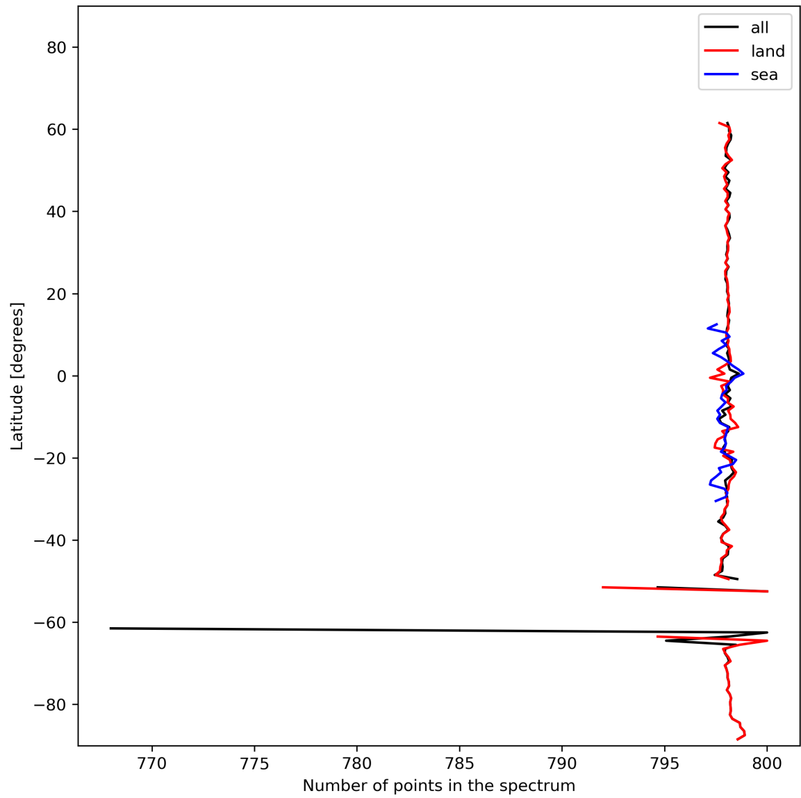
Figure 15: Zonal average of “Number of points in the spectrum” for 2024-02-11 to 2024-02-13.
