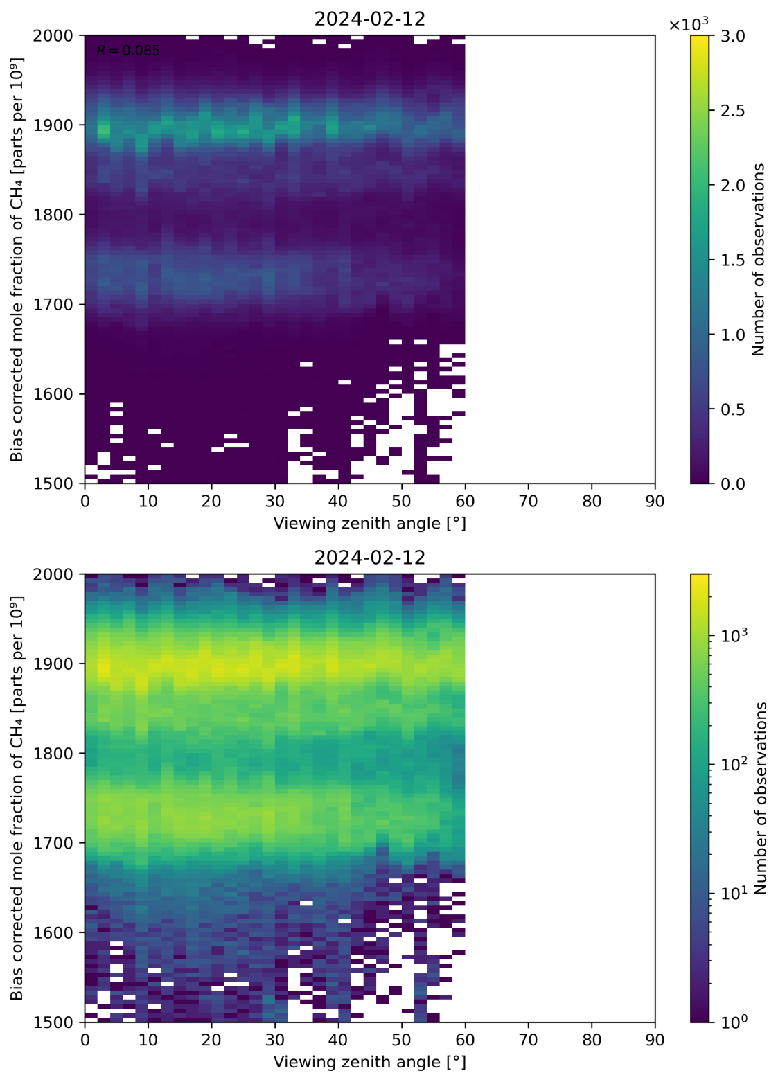
Figure 111: Scatter density plot of “Viewing zenith angle” against “Bias corrected mole fraction of CH 4 ” for 2024-02-11 to 2024-02-13.
