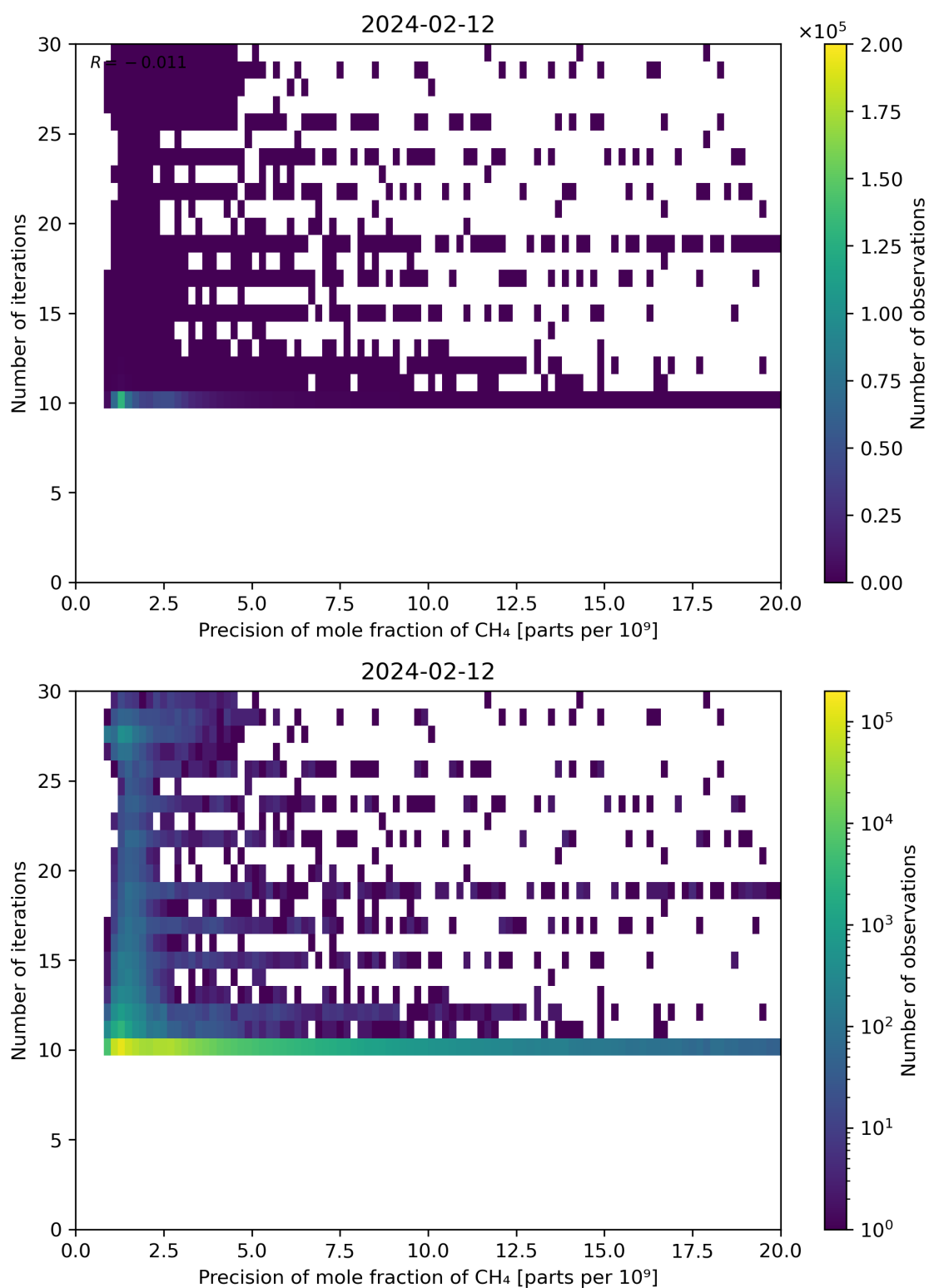
Figure 83: Scatter density plot of “Precision of mole fraction of CH 4 ” against “Number of iterations” for 2024-02-11 to 2024-02-13.
