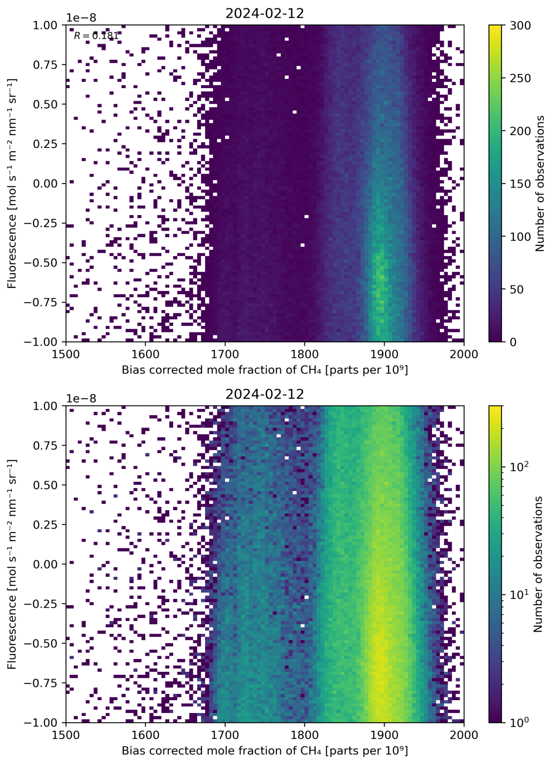
Figure 66: Scatter density plot of “Bias corrected mole fraction of \text{CH}_4 ” against “Fluorescence” for 2024-02-11 to 2024-02-13.
