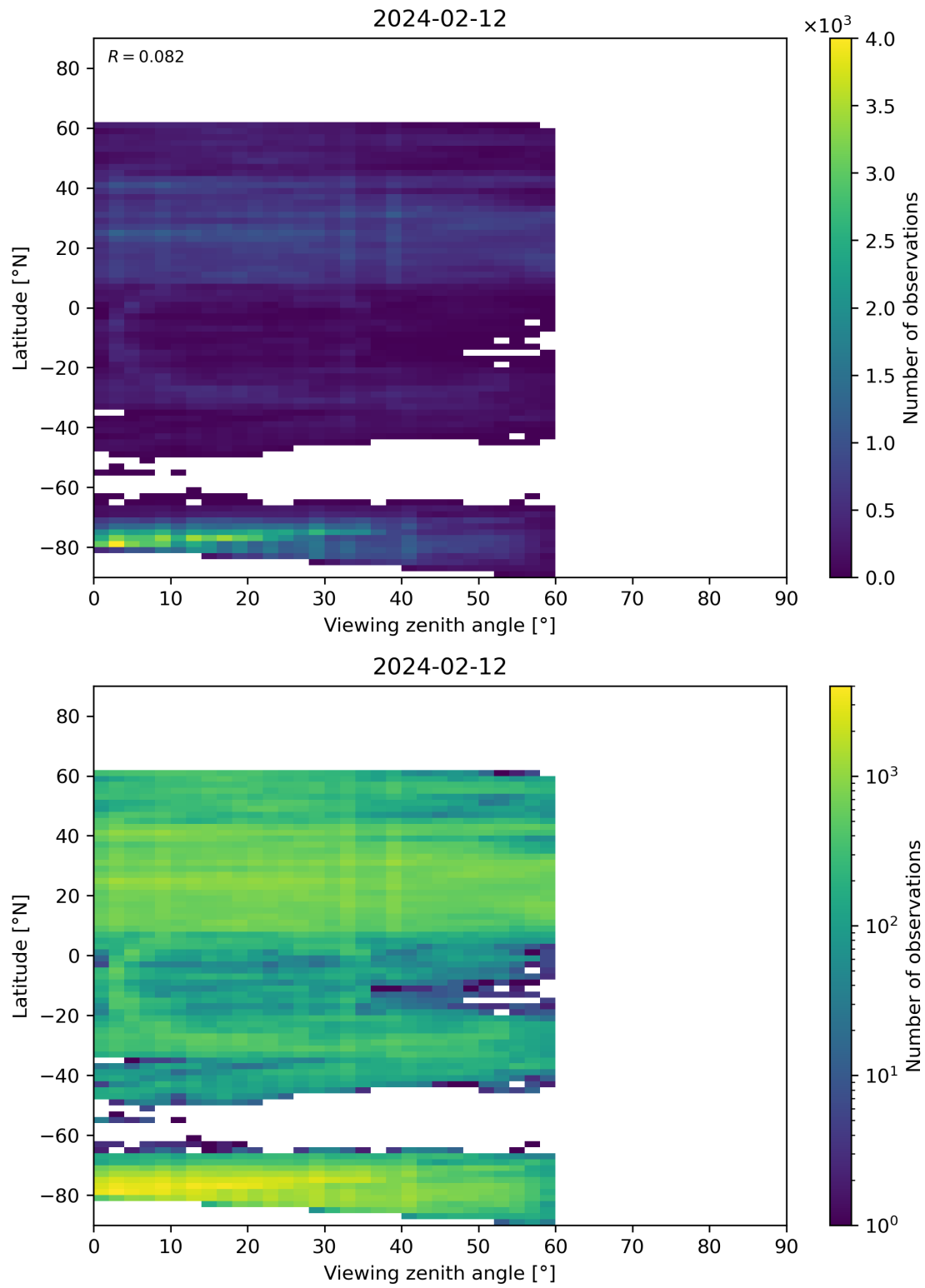
Figure 109: Scatter density plot of “Viewing zenith angle” against “Latitude” for 2024-02-11 to 2024-02-13.
