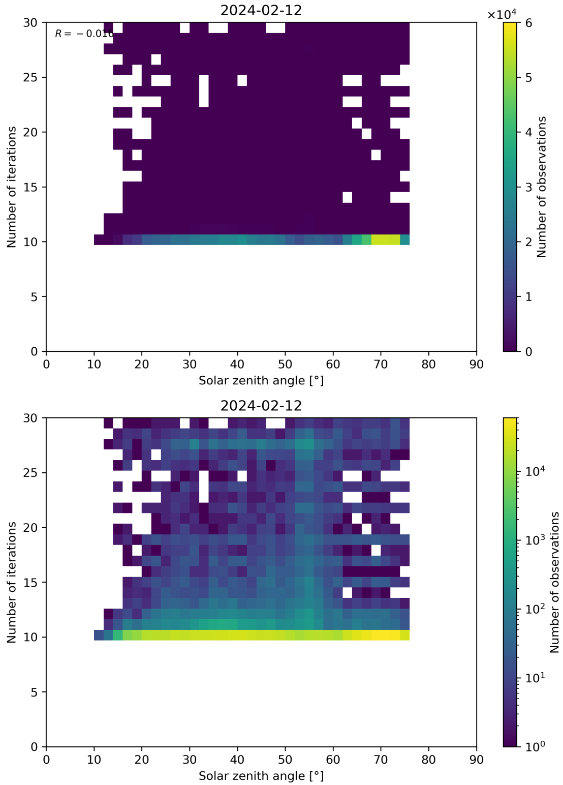
Figure 102: Scatter density plot of “Solar zenith angle” against “Number of iterations” for 2024-02-11 to 2024-02-13.
