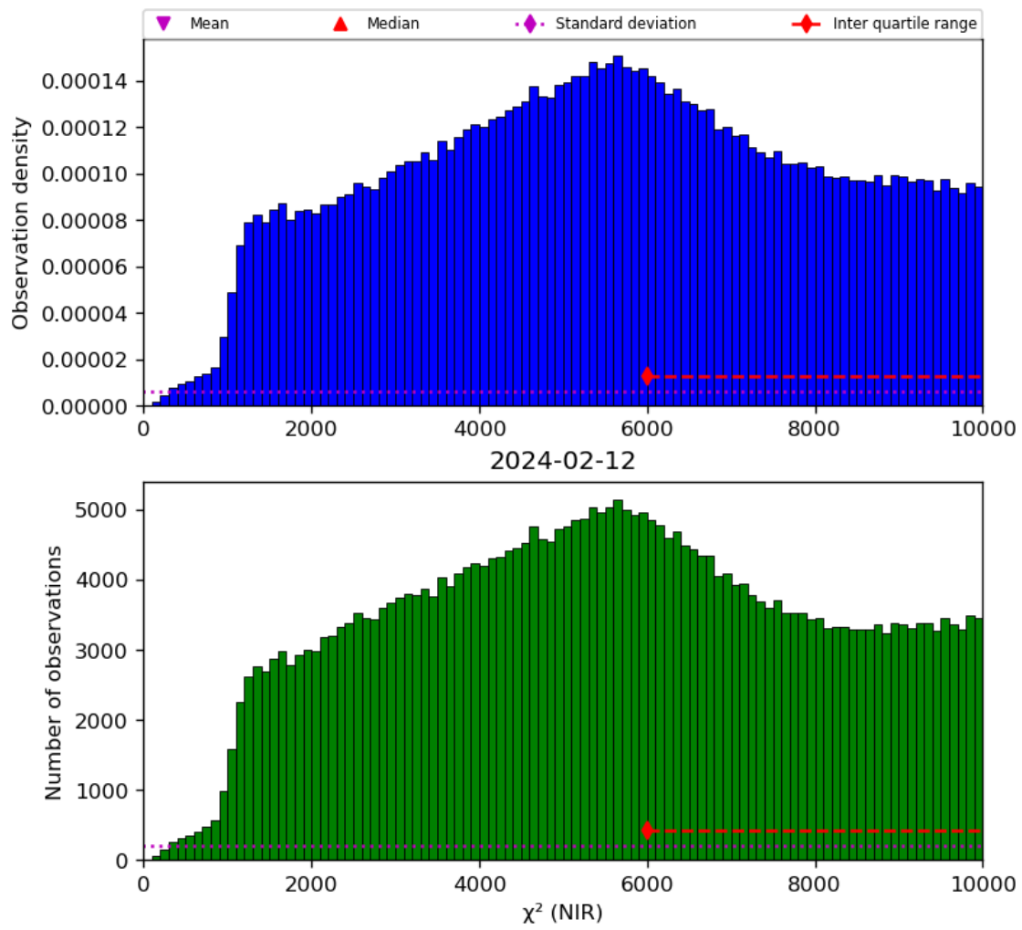
Figure 29: Histogram of “ \chi^2 (NIR)” for 2024-02-11 to 2024-02-13
