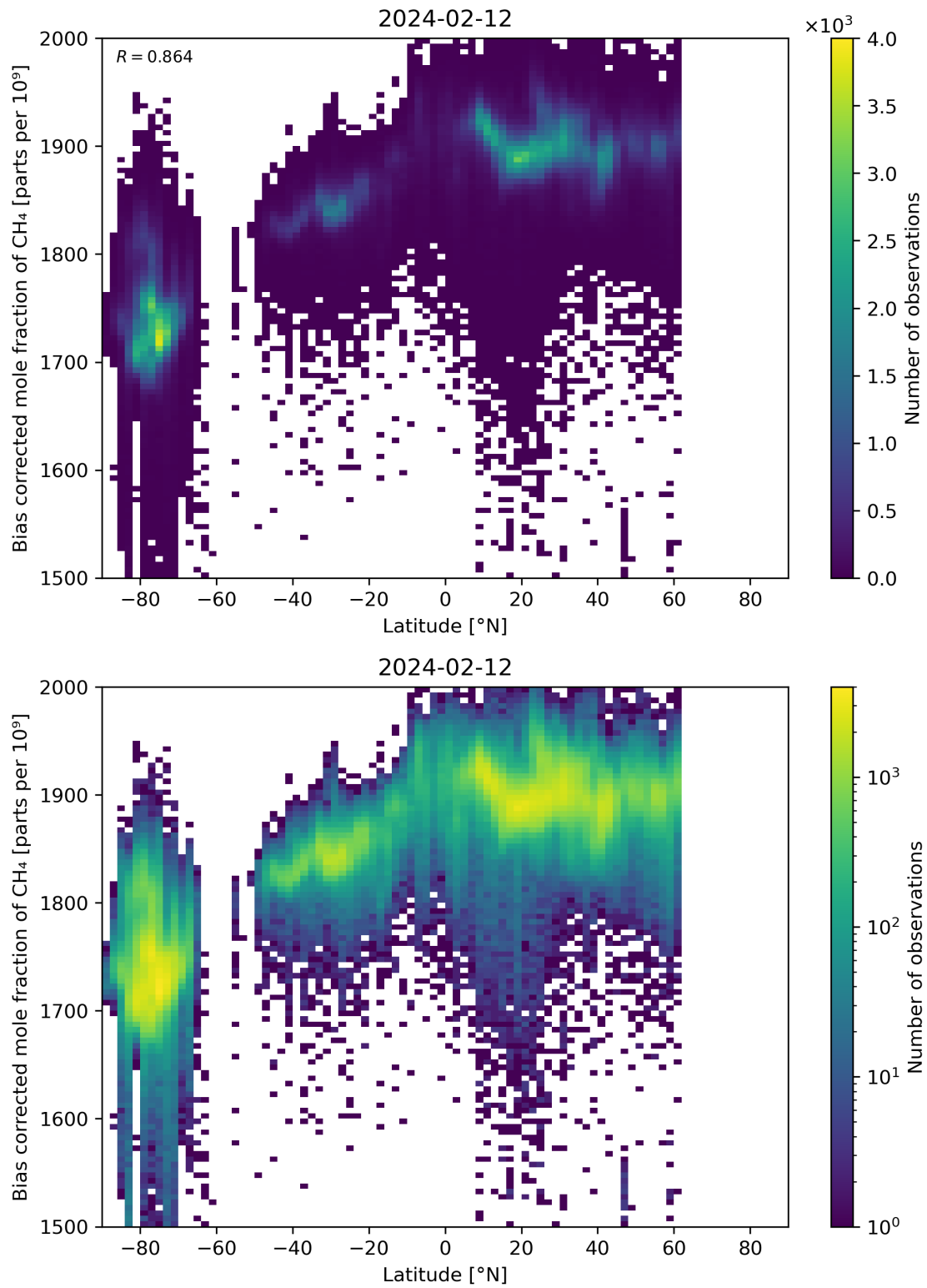
Figure 58: Scatter density plot of “Latitude” against “Bias corrected mole fraction of CH 4 ” for 2024-02-11 to 2024-02-13.
