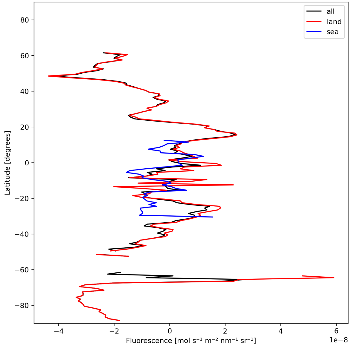
Figure 21: Zonal average of “Fluorescence” for 2024-02-11 to 2024-02-13.
