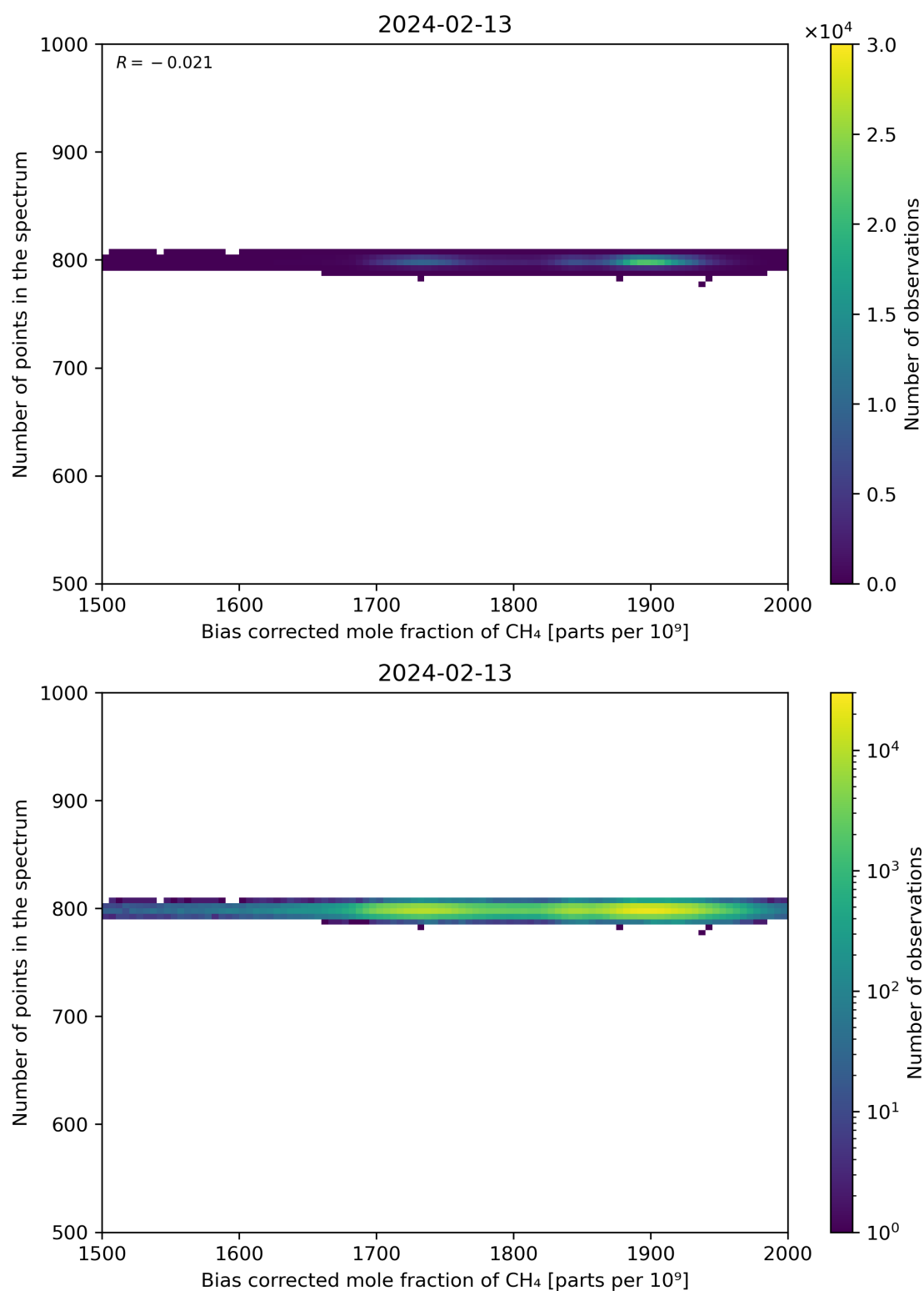
Figure 68: Scatter density plot of “Bias corrected mole fraction of CH 4 ” against “Number of points in the spectrum” for 2024-02-12 to 2024-02-14.
