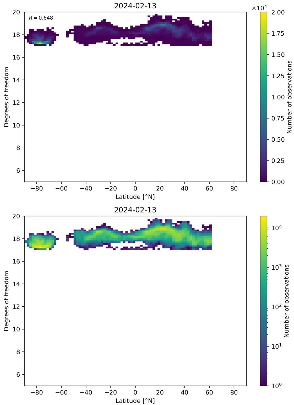
Figure 55: Scatter density plot of “Latitude” against “Degrees of freedom” for 2024-02-12 to 2024-02-14.
