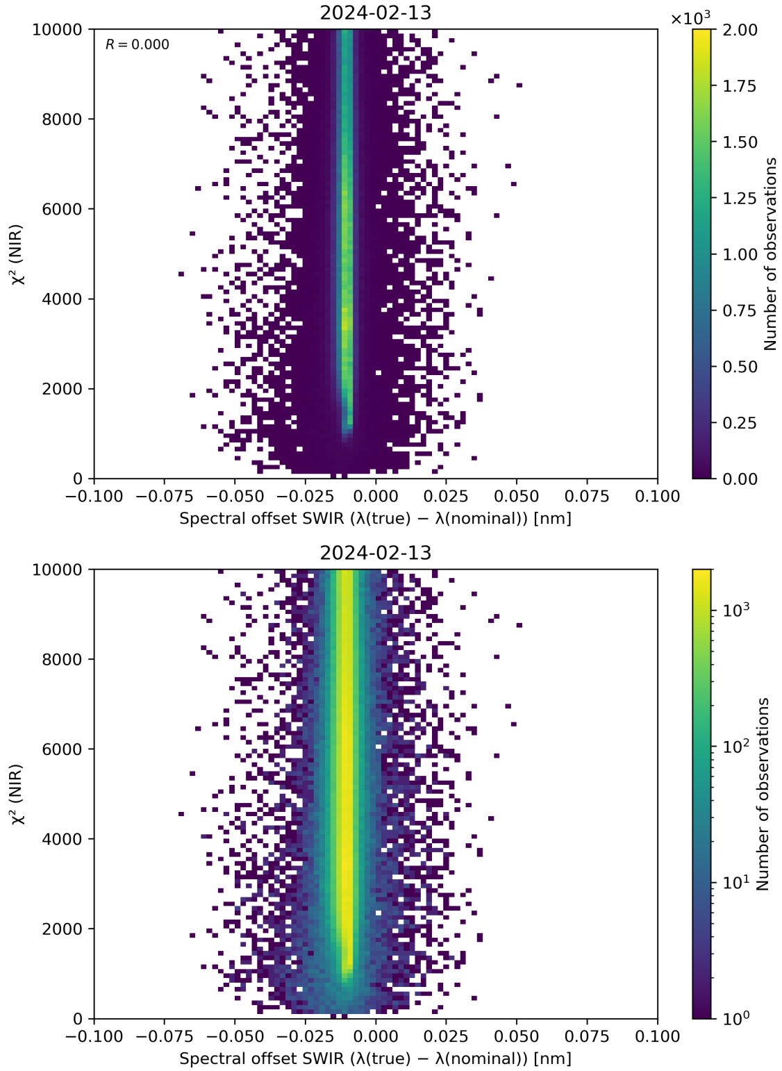
Figure 117: Scatter density plot of “Spectral offset SWIR ( \lambda(\text{true}) - \lambda(\text{nominal}) )” against “ \chi^2 (NIR)” for 2024-02-12 to 2024-02-14.
