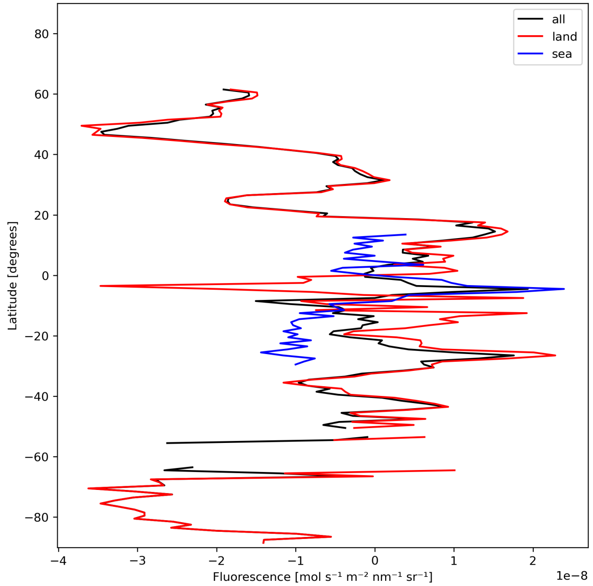
Figure 21: Zonal average of “Fluorescence” for 2024-02-12 to 2024-02-14.
