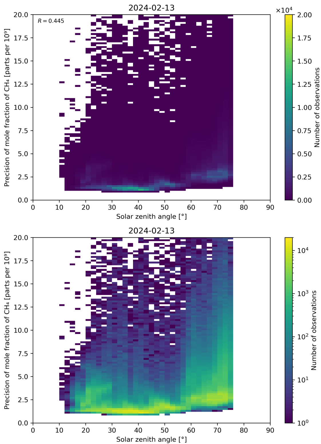
Figure 101: Scatter density plot of “Solar zenith angle” against “Precision of mole fraction of CH 4 ” for 2024-02-12 to 2024-02-14.
