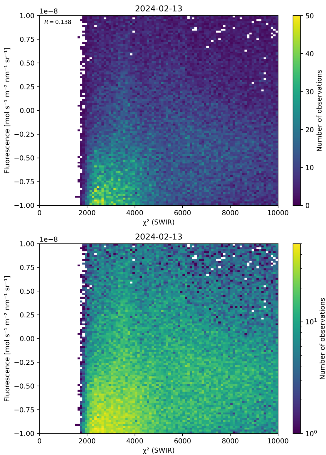
Figure 49: Scatter density plot of “ \chi^2 (SWIR)” against “Fluorescence” for 2024-02-12 to 2024-02-14.
