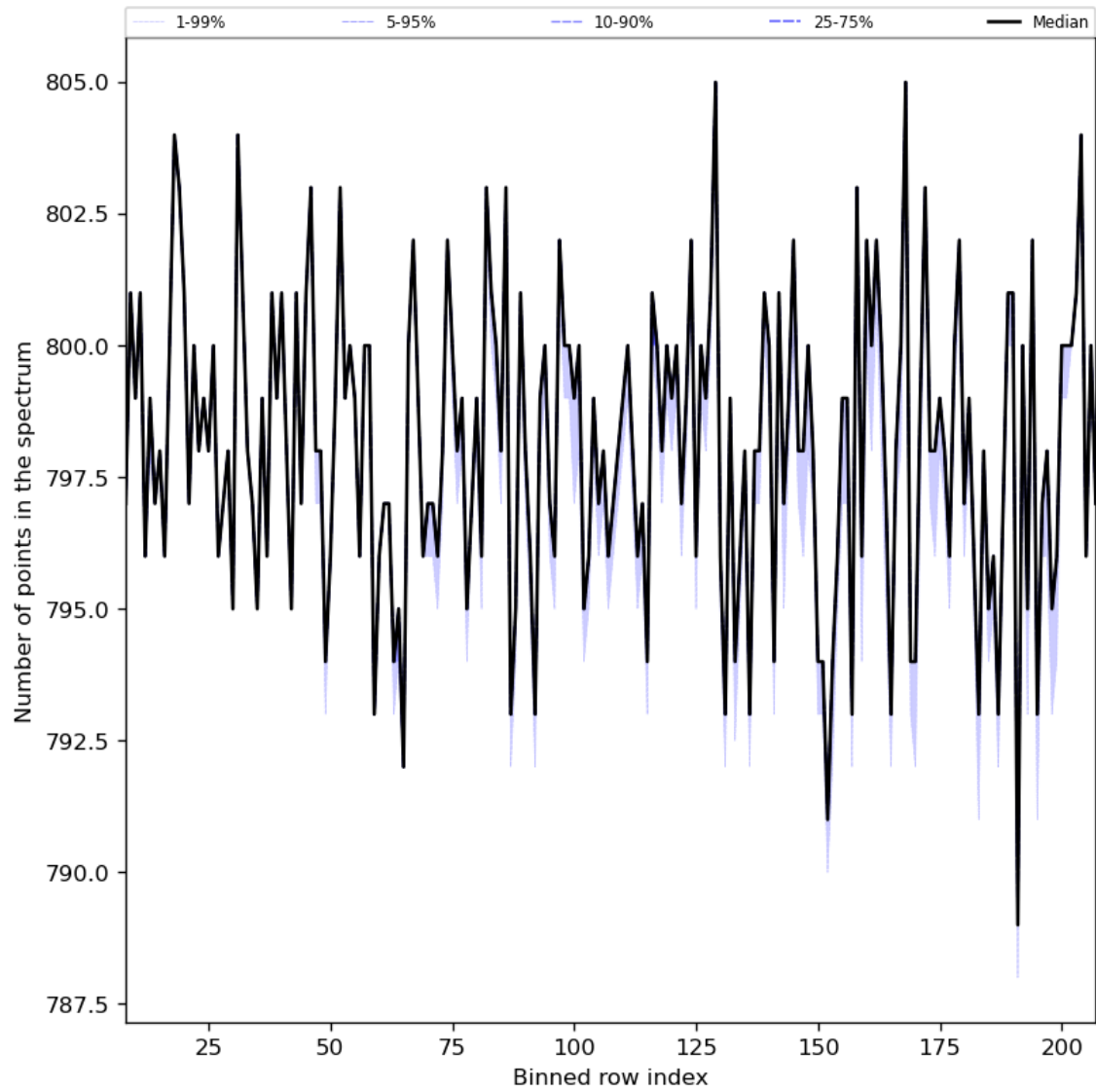
Figure 37: Along track statistics of “Number of points in the spectrum” for 2024-02-12 to 2024-02-14
