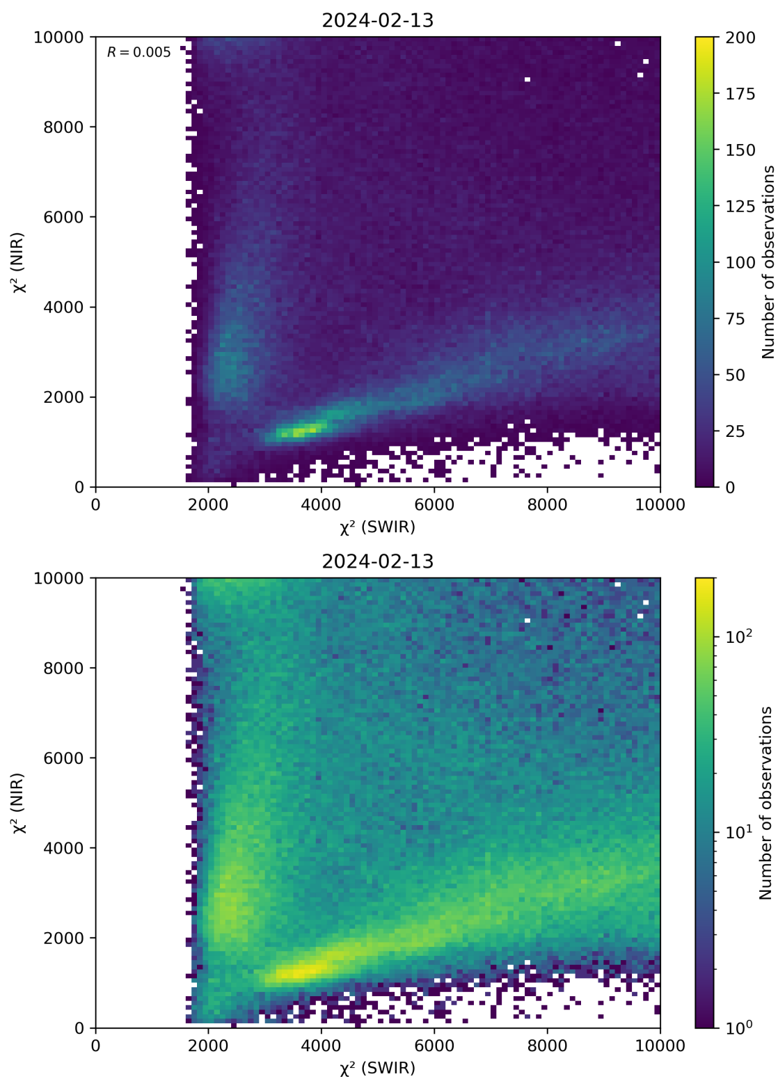
Figure 47: Scatter density plot of “ \chi^2 (SWIR)” against “ \chi^2 (NIR)” for 2024-02-12 to 2024-02-14.
