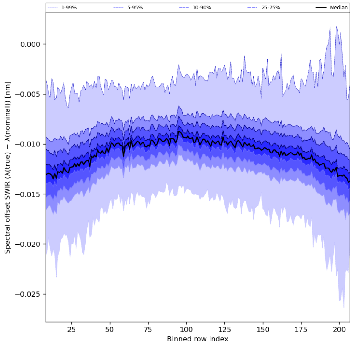
Figure 38: Along track statistics of “Spectral offset SWIR ( \lambda(\text{true}) - \lambda(\text{nominal}) )” for 2024-02-12 to 2024-02-14
