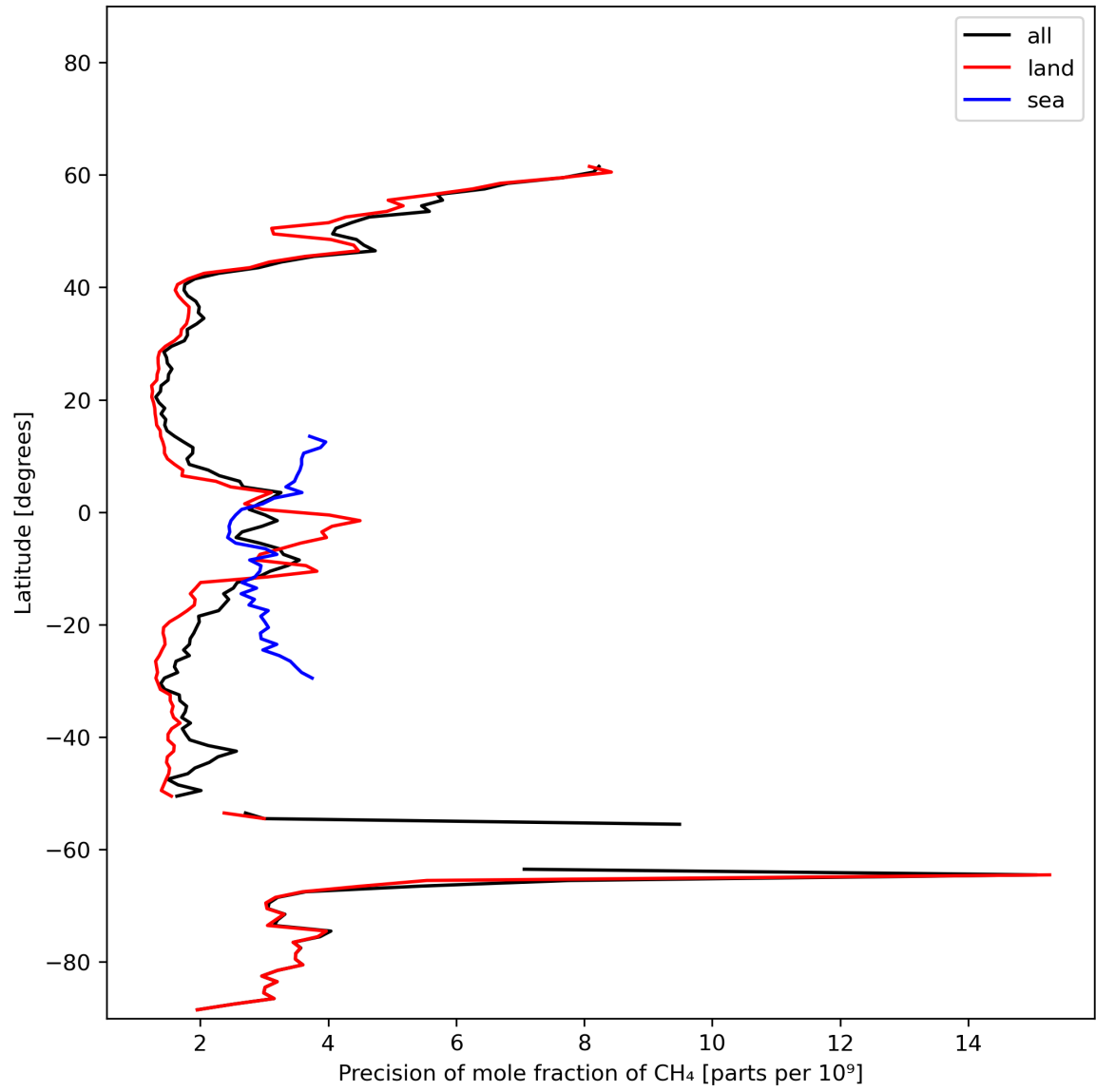
Figure 13: Zonal average of “Precision of mole fraction of CH 4 ” for 2024-02-12 to 2024-02-14.
