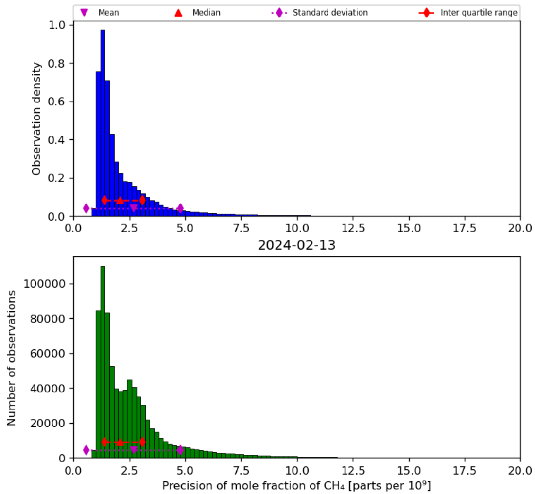
Figure 24: Histogram of “Precision of mole fraction of CH 4 ” for 2024-02-12 to 2024-02-14
