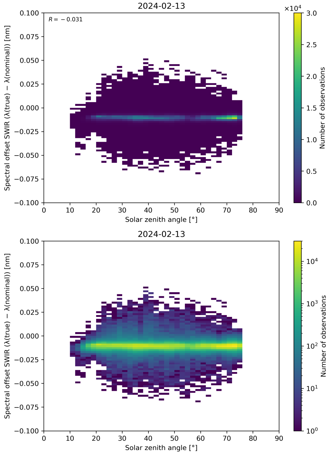
Figure 104: Scatter density plot of “Solar zenith angle” against “Spectral offset SWIR ( \lambda(\text{true}) - \lambda(\text{nominal}) )” for 2024-02-12 to 2024-02-14.
