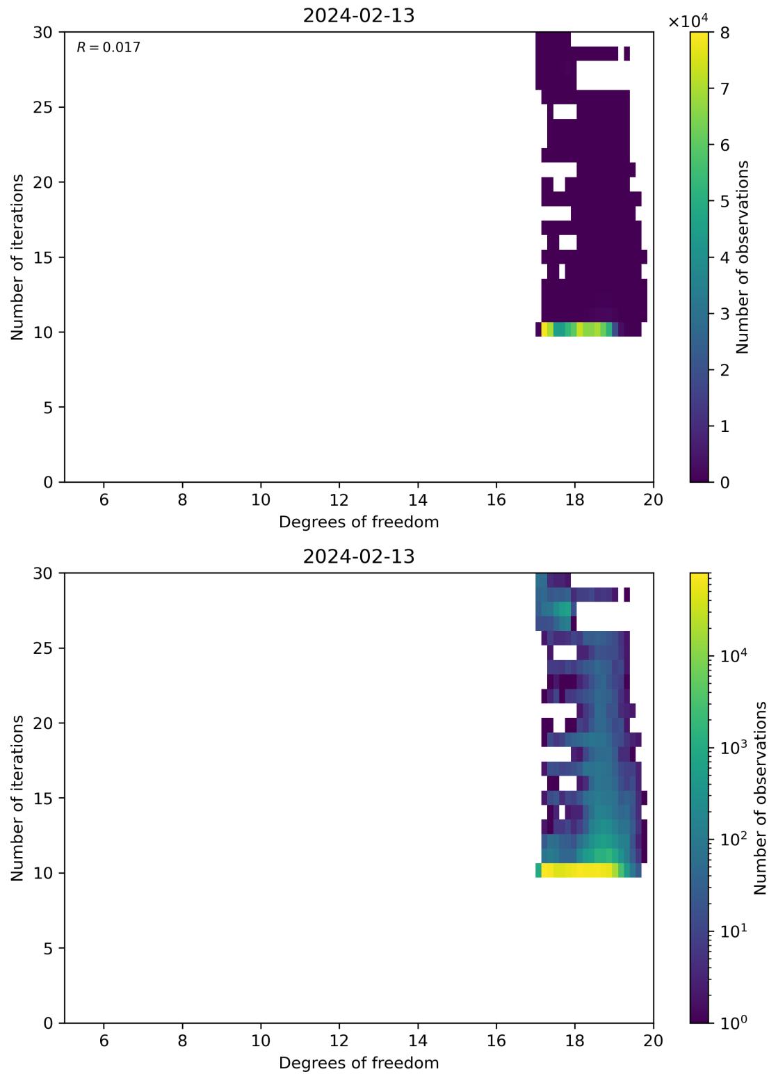
Figure 52: Scatter density plot of “Degrees of freedom” against “Number of iterations” for 2024-02-12 to 2024-02-14.
