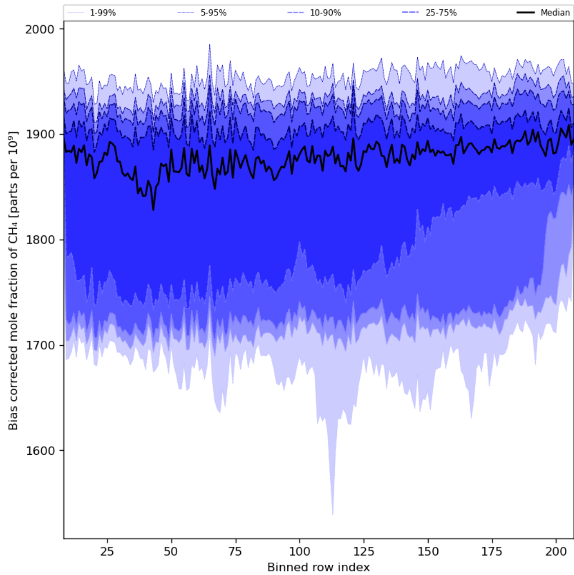
Figure 36: Along track statistics of “Bias corrected mole fraction of \text{CH}_4 ” for 2024-02-12 to 2024-02-14
