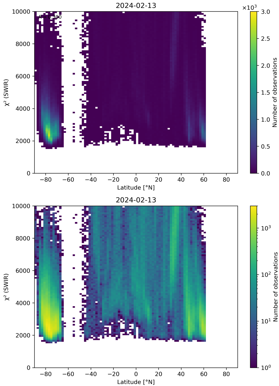
Figure 54: Scatter density plot of “Latitude” against “ \chi^2 (SWIR)” for 2024-02-12 to 2024-02-14.
