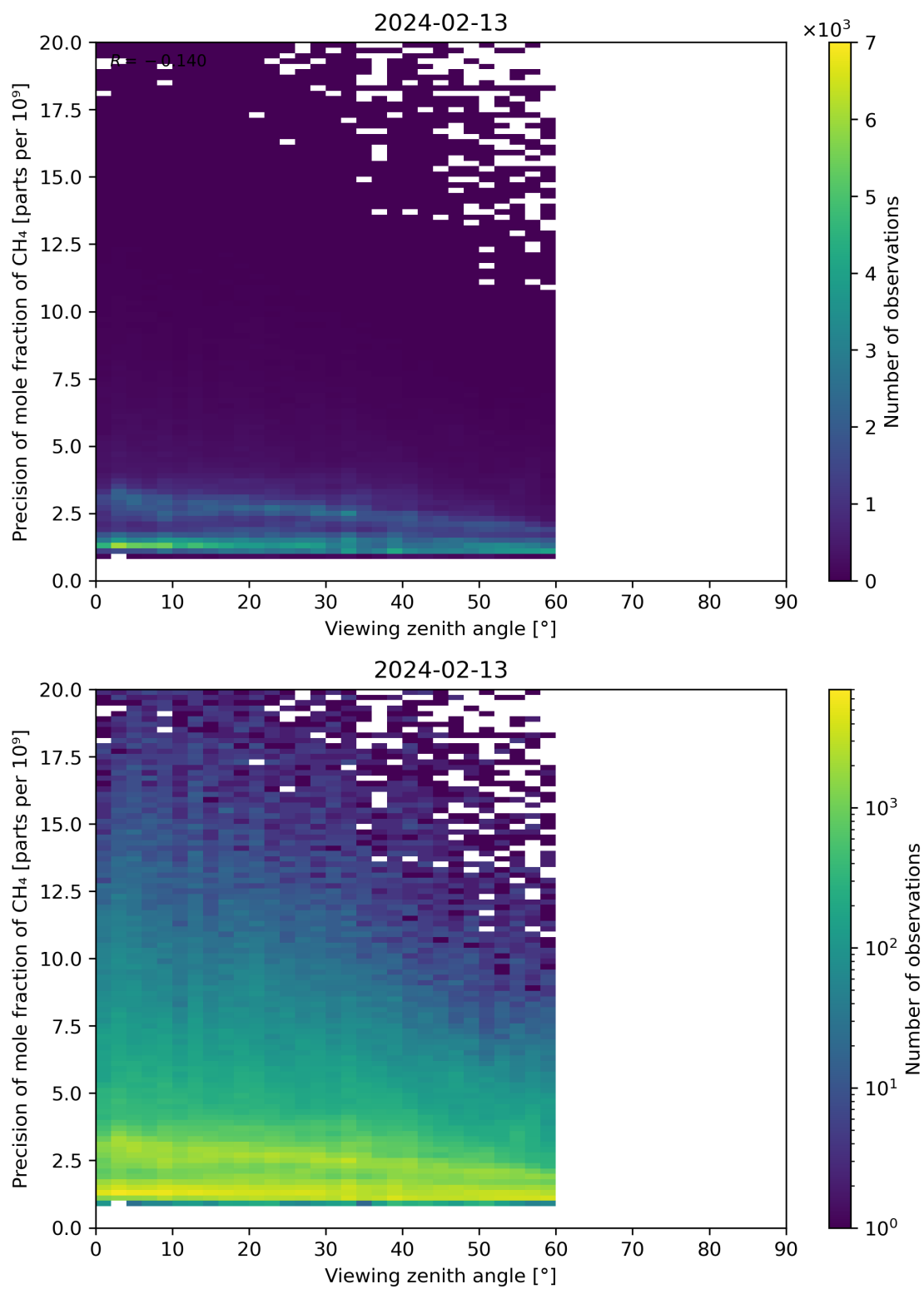
Figure 112: Scatter density plot of “Viewing zenith angle” against “Precision of mole fraction of CH 4 ” for 2024-02-12 to 2024-02-14.
