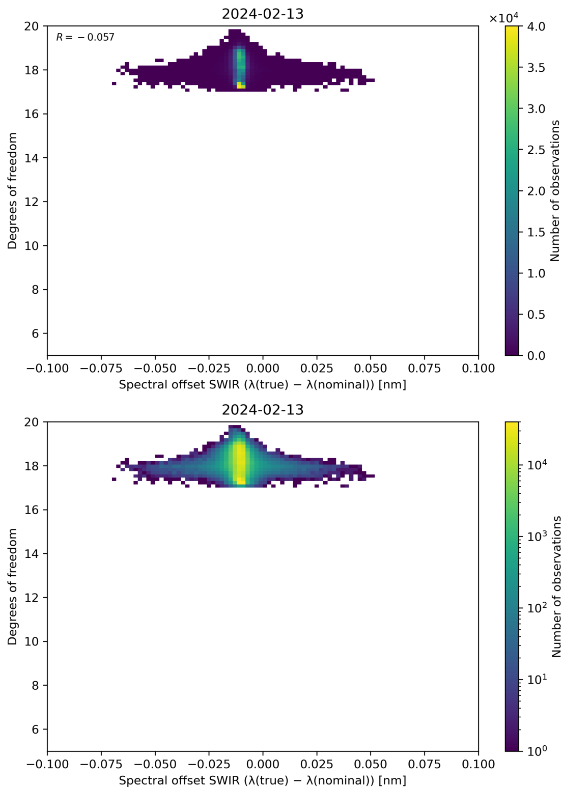
Figure 119: Scatter density plot of “Spectral offset SWIR ( \lambda(\text{true}) - \lambda(\text{nominal}) )” against “Degrees of freedom” for 2024-02-12 to 2024-02-14.
