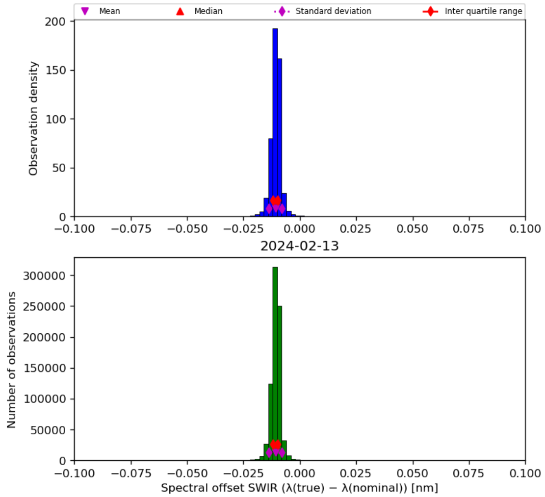
Figure 27: Histogram of “Spectral offset SWIR ( \lambda(\text{true}) - \lambda(\text{nominal}) )” for 2024-02-12 to 2024-02-14
