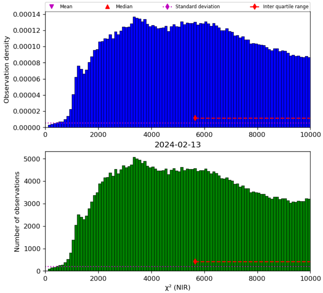
Figure 29: Histogram of “ \chi^2 (NIR)” for 2024-02-12 to 2024-02-14
