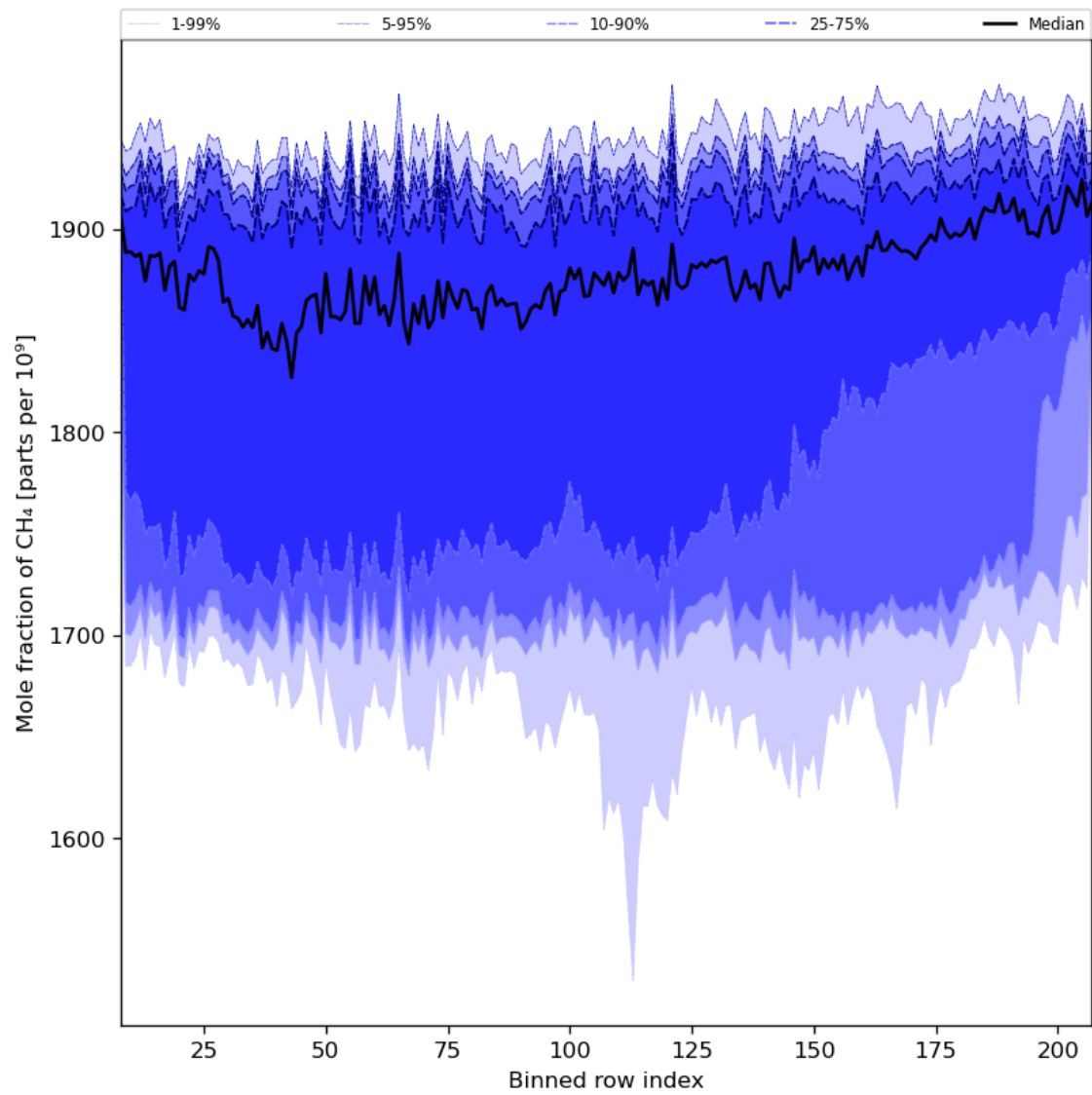
Figure 34: Along track statistics of “Mole fraction of CH 4 ” for 2024-02-12 to 2024-02-14
