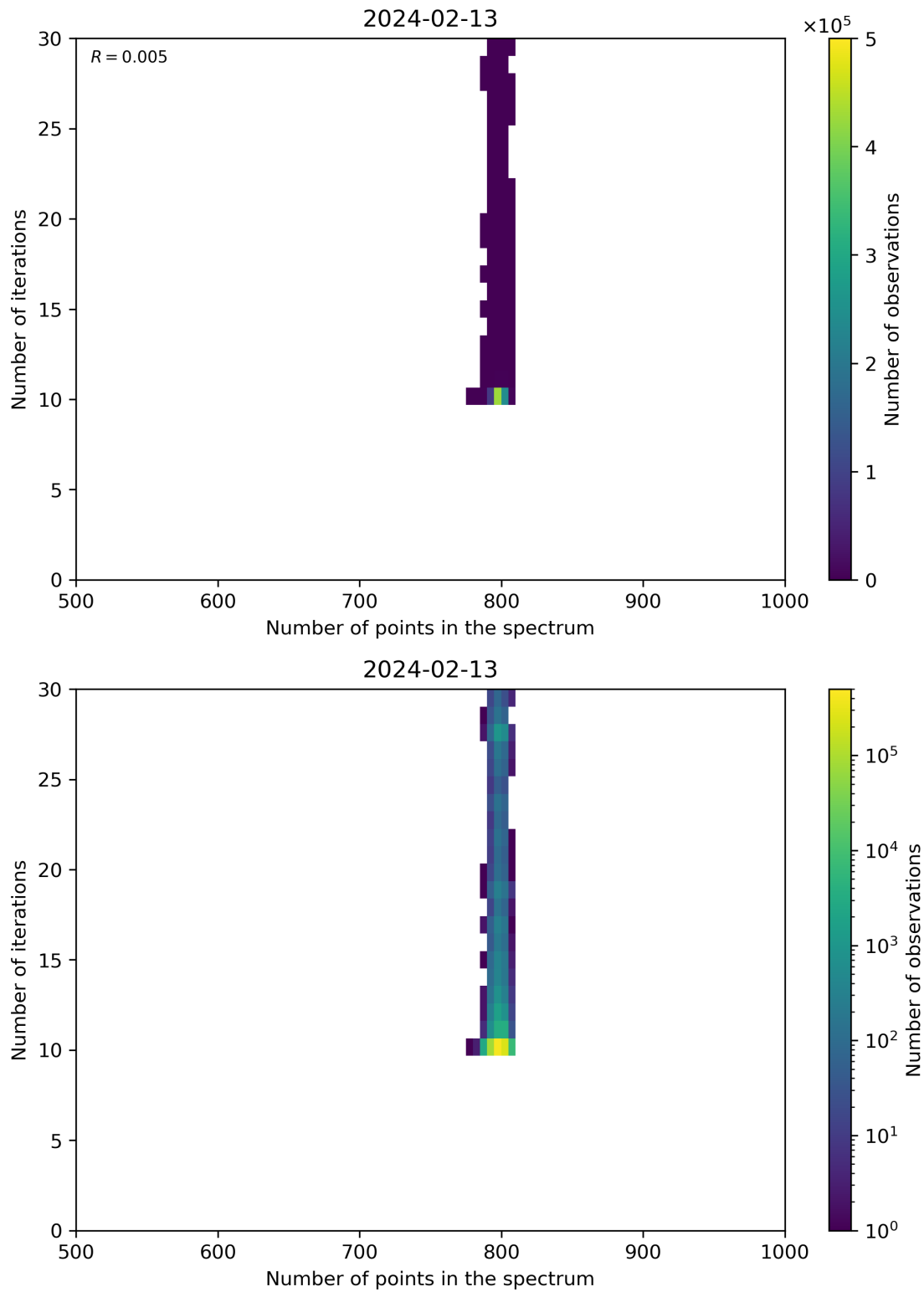
Figure 92: Scatter density plot of “Number of points in the spectrum” against “Number of iterations” for 2024-02-12 to 2024-02-14.
