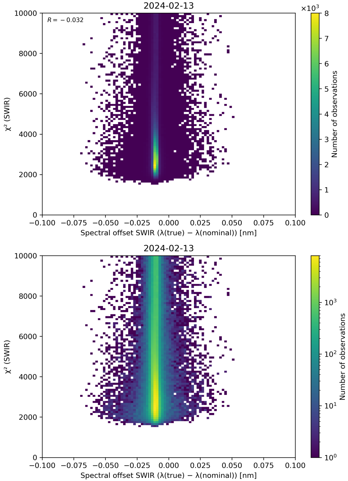
Figure 118: Scatter density plot of “Spectral offset SWIR ( \lambda(\text{true}) - \lambda(\text{nominal}) )” against “ \chi^2 (SWIR)” for 2024-02-12 to 2024-02-14.
