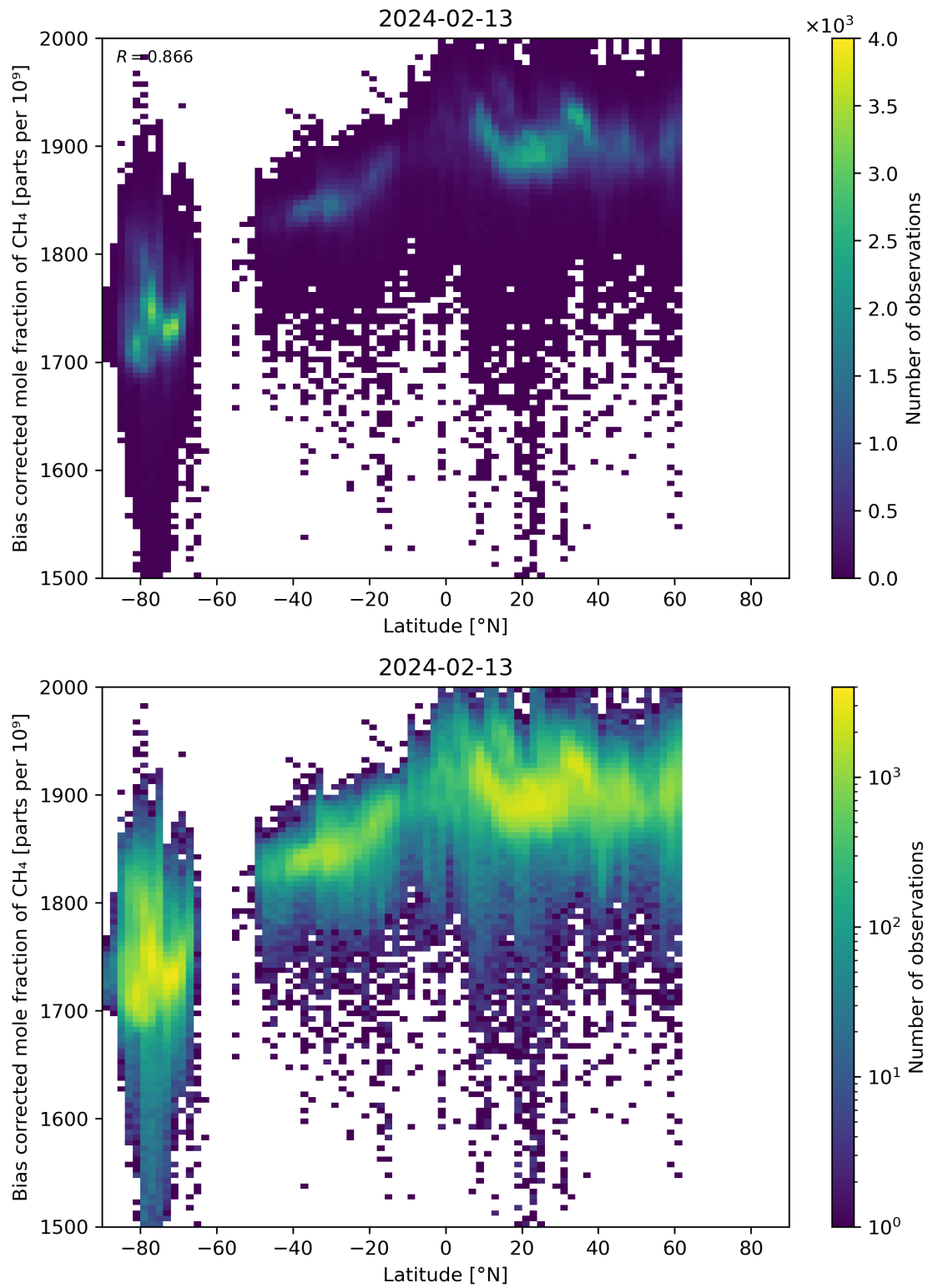
Figure 58: Scatter density plot of “Latitude” against “Bias corrected mole fraction of CH 4 ” for 2024-02-12 to 2024-02-14.
