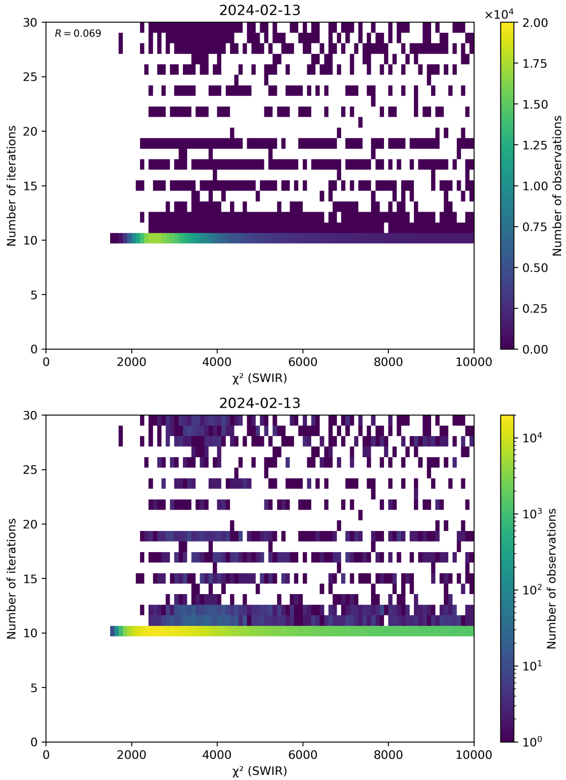
Figure 50: Scatter density plot of “ \chi^2 (SWIR)” against “Number of iterations” for 2024-02-12 to 2024-02-14.
