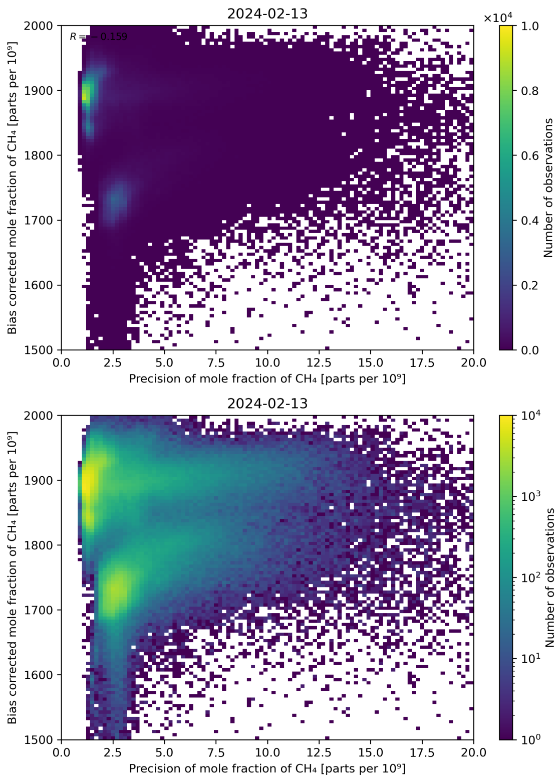
Figure 82: Scatter density plot of “Precision of mole fraction of CH 4 ” against “Bias corrected mole fraction of CH 4 ” for 2024-02-12 to 2024-02-14.
