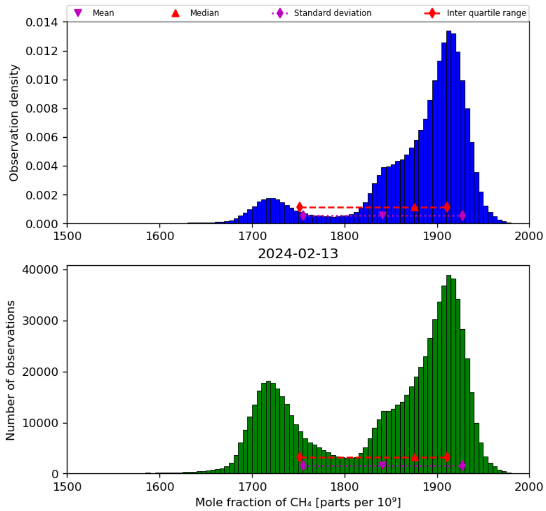
Figure 23: Histogram of “Mole fraction of CH 4 ” for 2024-02-12 to 2024-02-14
