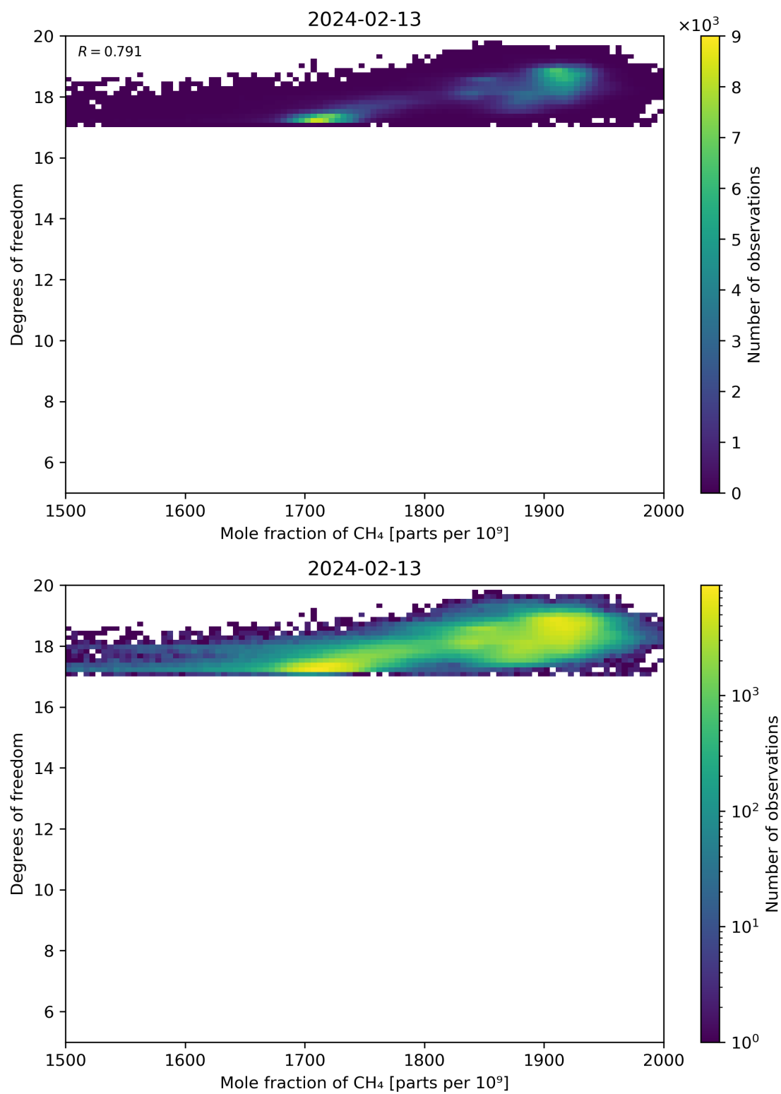
Figure 72: Scatter density plot of “Mole fraction of CH 4 ” against “Degrees of freedom” for 2024-02-12 to 2024-02-14.
