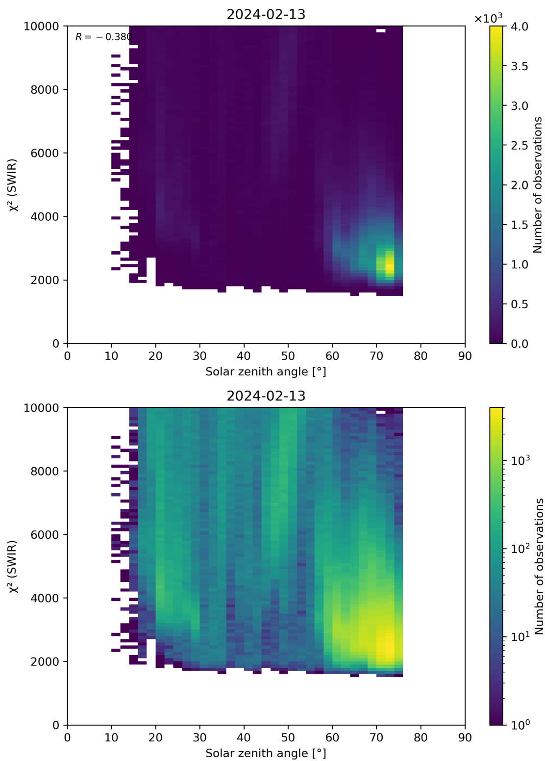
Figure 95: Scatter density plot of “Solar zenith angle” against “ \chi^2 (SWIR)” for 2024-02-12 to 2024-02-14.
