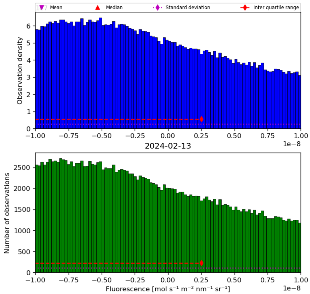
Figure 32: Histogram of “Fluorescence” for 2024-02-12 to 2024-02-14
