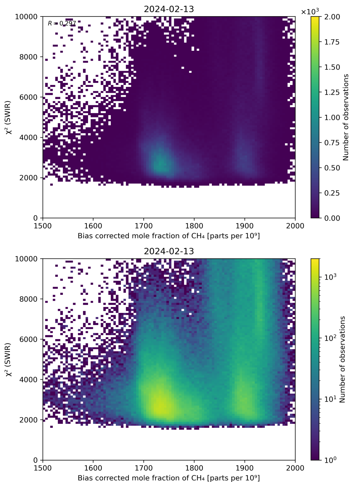
Figure 64: Scatter density plot of “Bias corrected mole fraction of \text{CH}_4 ” against “ \chi^2 (SWIR)” for 2024-02-12 to 2024-02-14.
