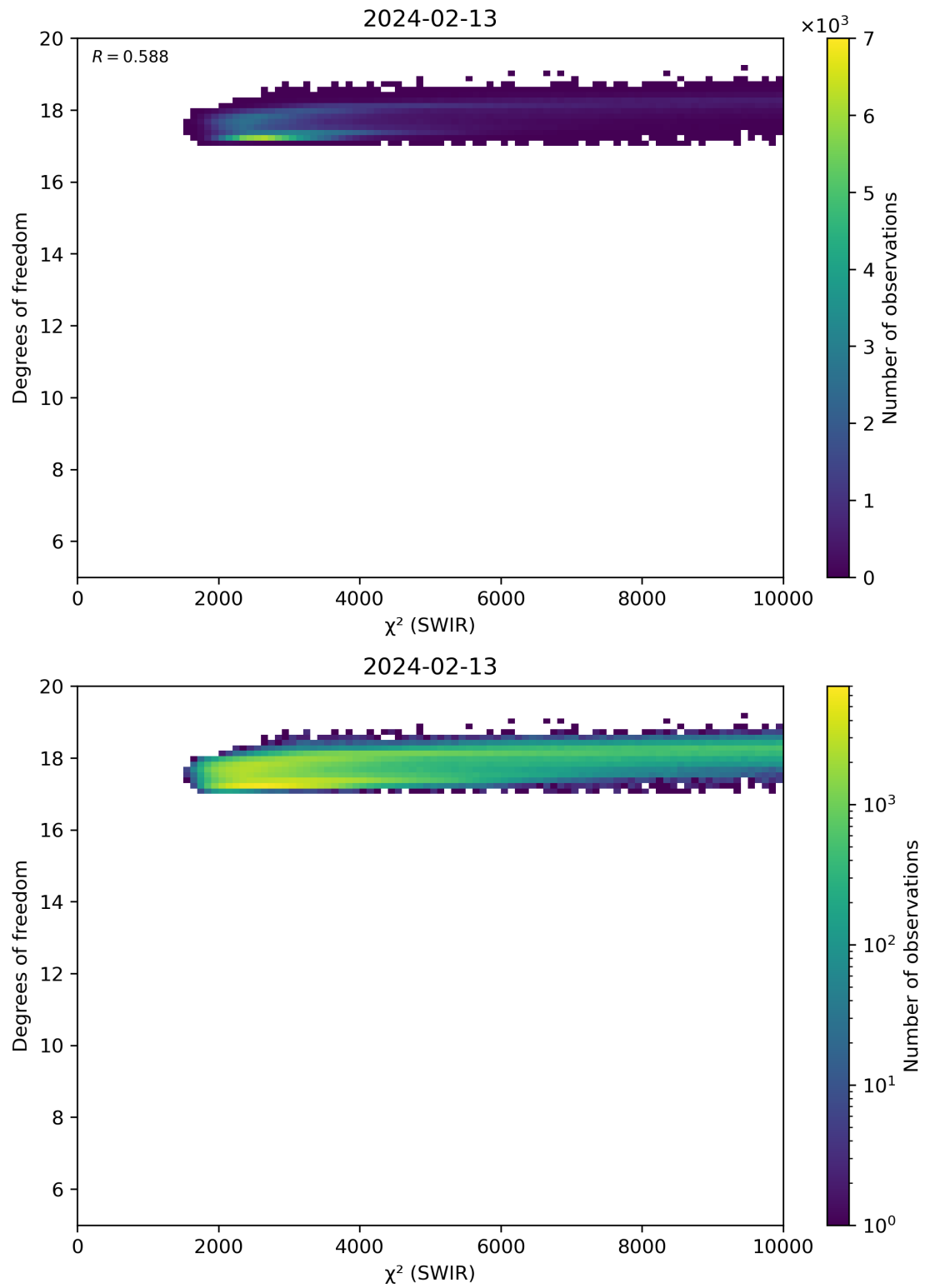
Figure 48: Scatter density plot of “ \chi^2 (SWIR)” against “Degrees of freedom” for 2024-02-12 to 2024-02-14.
