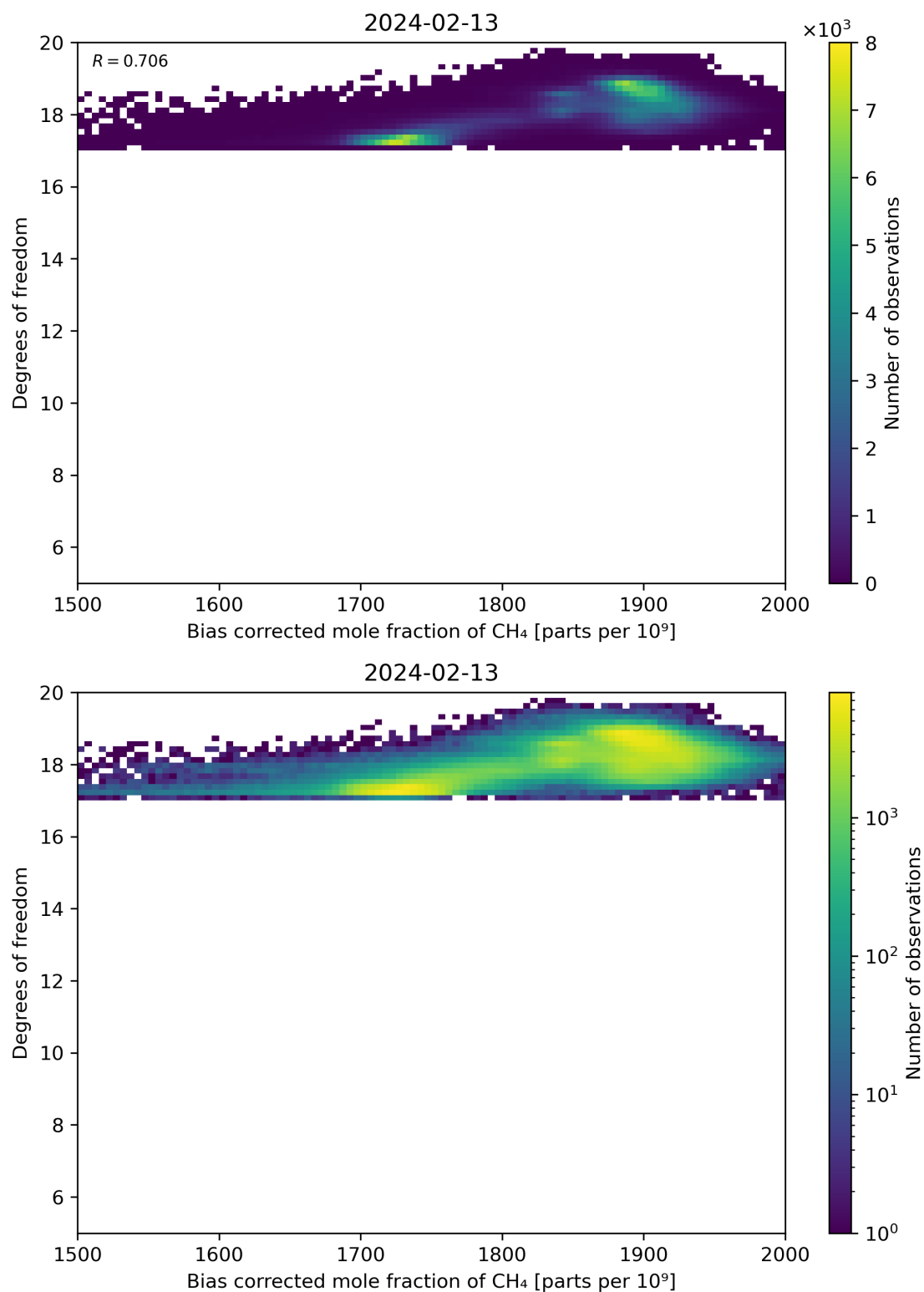
Figure 65: Scatter density plot of “Bias corrected mole fraction of CH 4 ” against “Degrees of freedom” for 2024-02-12 to 2024-02-14.
