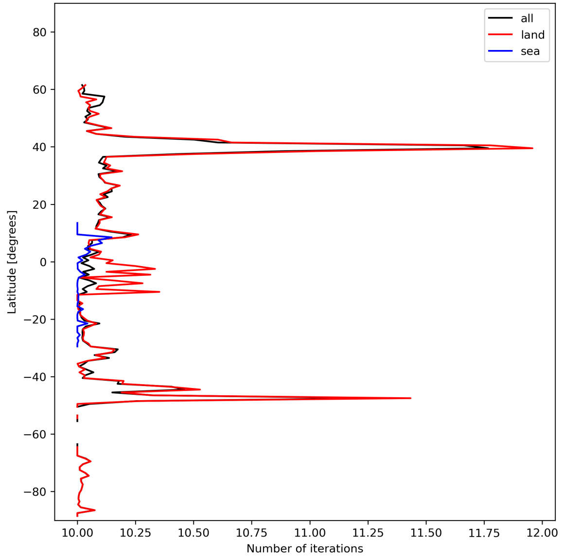
Figure 20: Zonal average of “Number of iterations” for 2024-02-12 to 2024-02-14.
