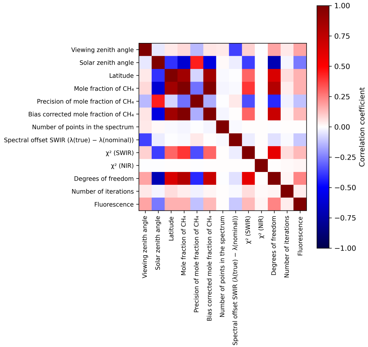
Figure 2: Map of correlation matrix for 2024-02-12 to 2024-02-14.
