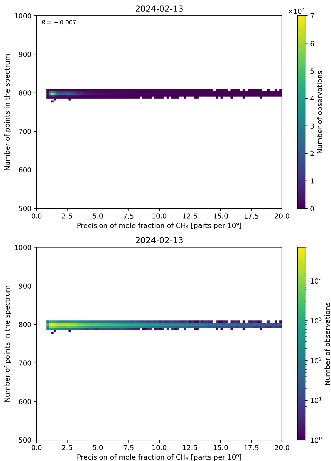
Figure 84: Scatter density plot of “Precision of mole fraction of CH 4 ” against “Number of points in the spectrum” for 2024-02-12 to 2024-02-14.
