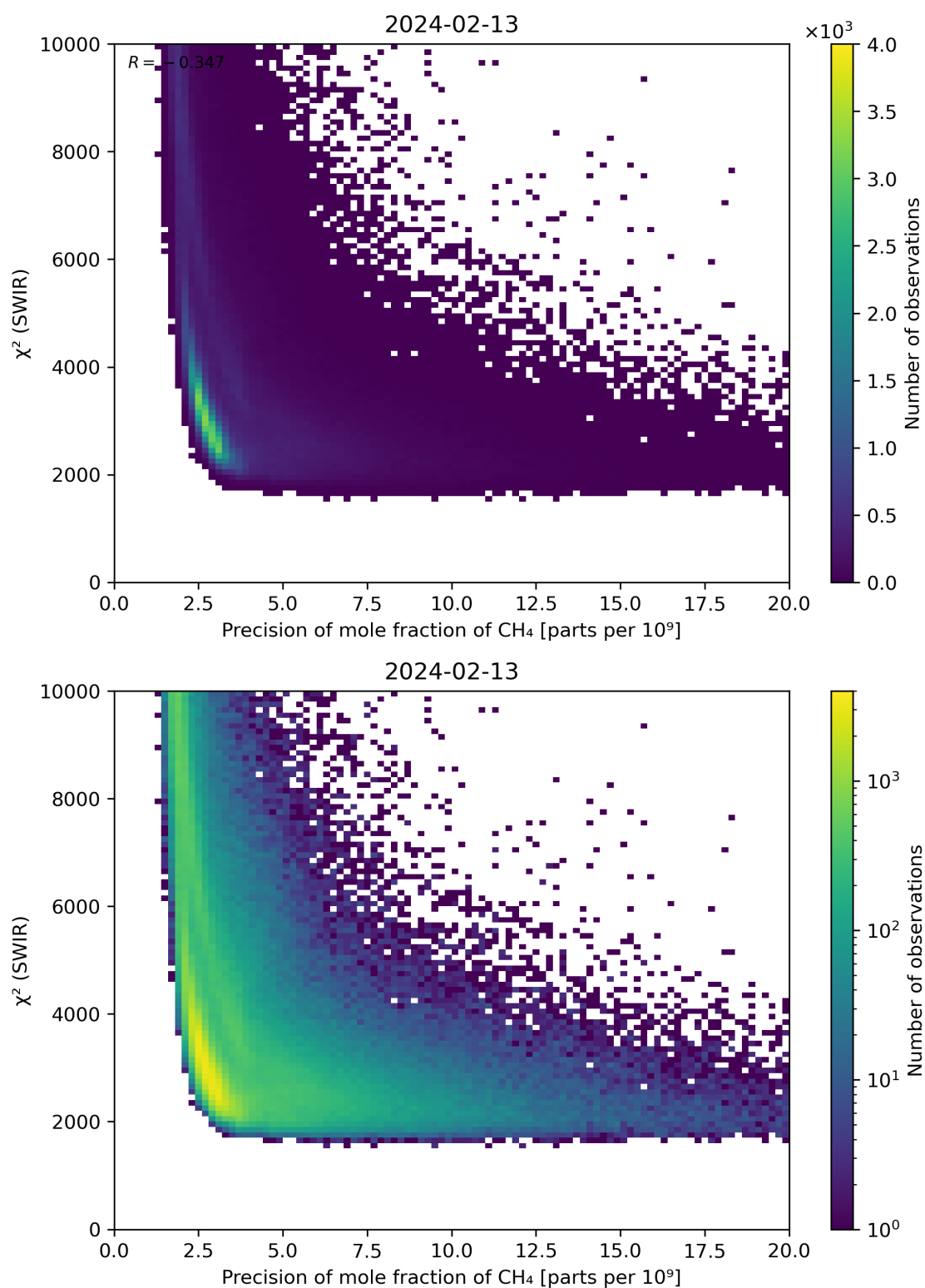
Figure 79: Scatter density plot of “Precision of mole fraction of CH 4 ” against “ \chi^2 (SWIR)” for 2024-02-12 to 2024-02-14.
