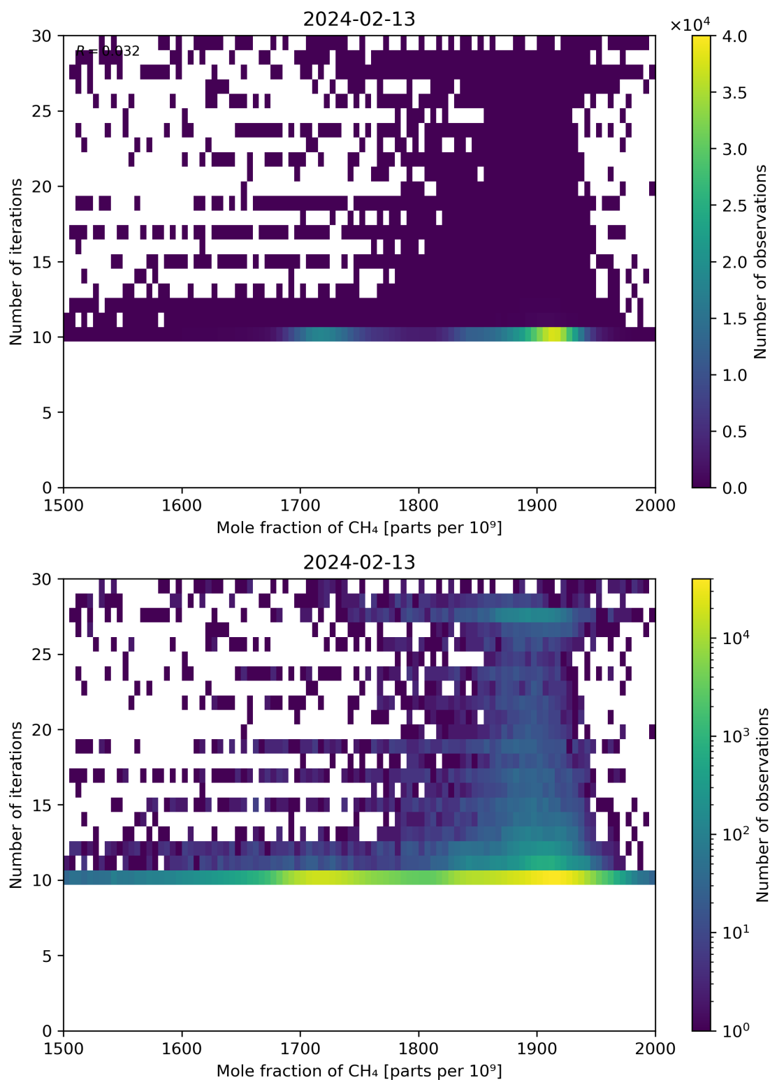
Figure 76: Scatter density plot of “Mole fraction of CH 4 ” against “Number of iterations” for 2024-02-12 to 2024-02-14.
