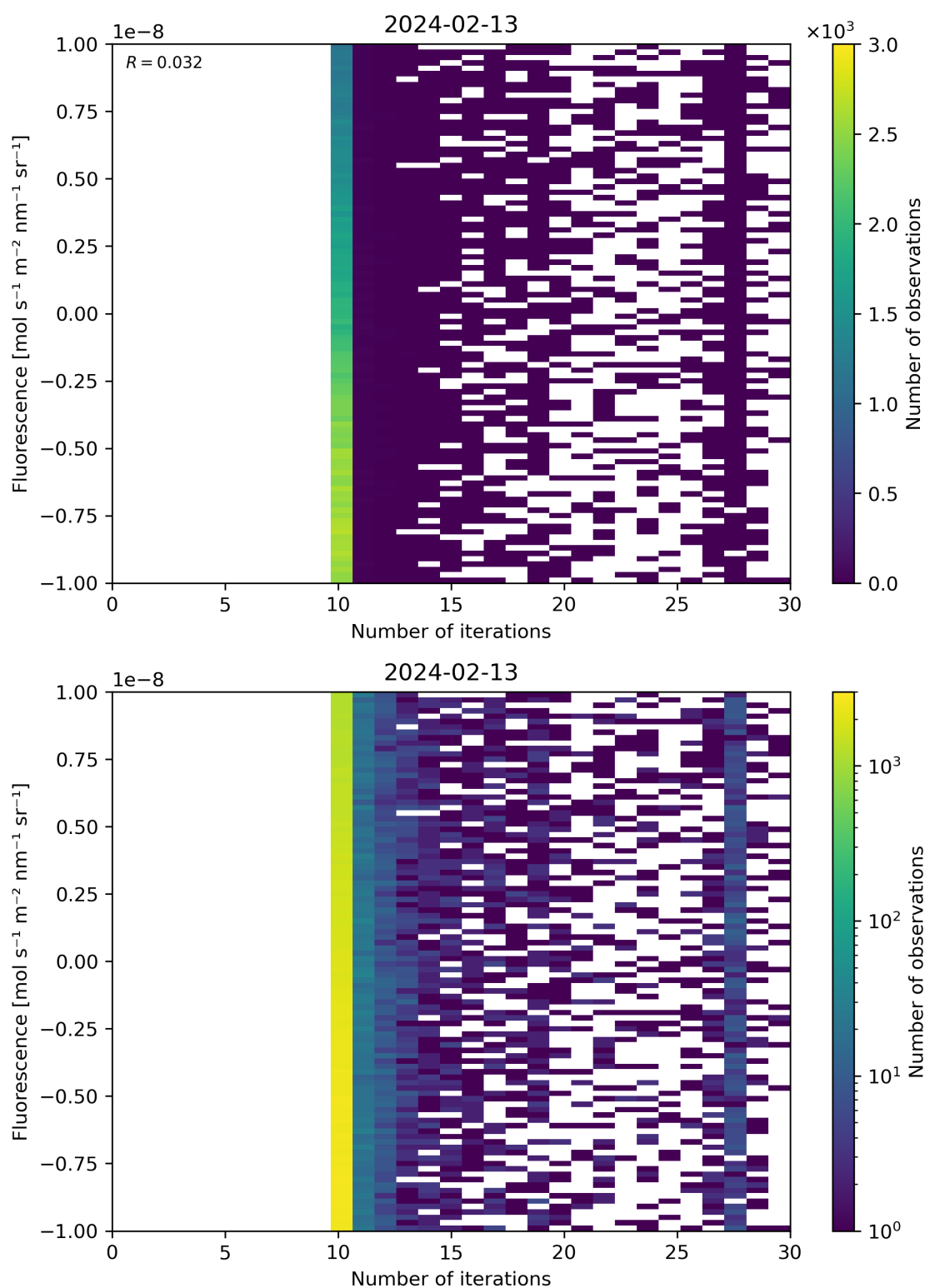
Figure 87: Scatter density plot of “Number of iterations” against “Fluorescence” for 2024-02-12 to 2024-02-14.
