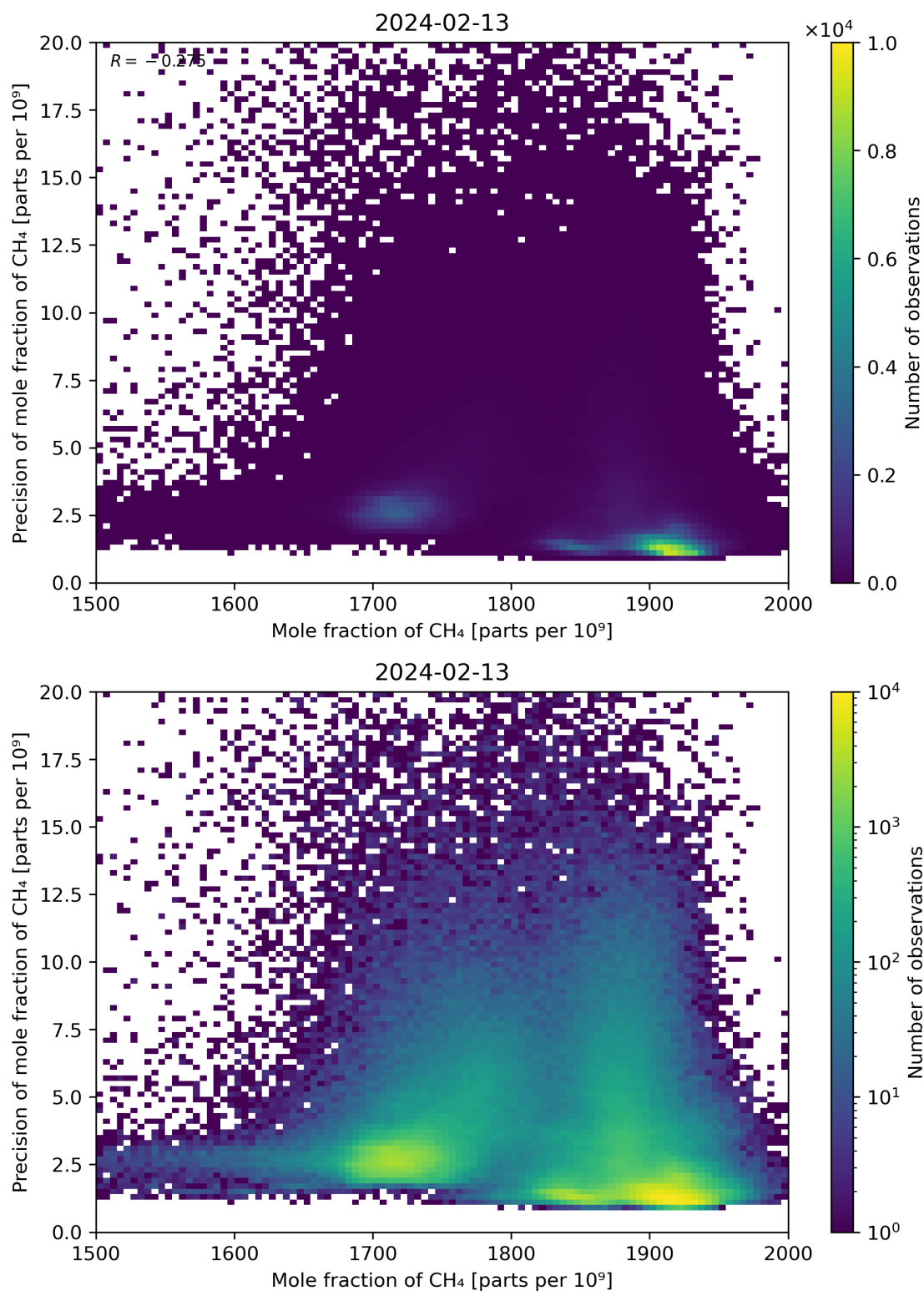
Figure 75: Scatter density plot of “Mole fraction of CH 4 ” against “Precision of mole fraction of CH 4 ” for 2024-02-12 to 2024-02-14.
