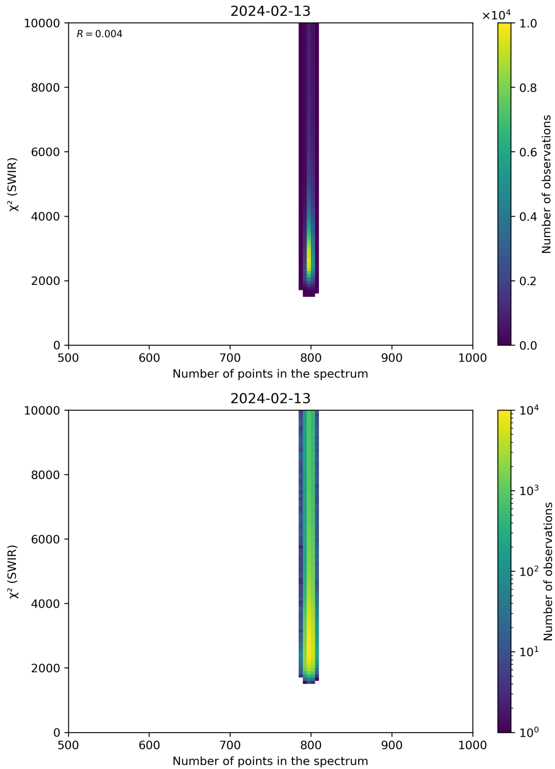
Figure 89: Scatter density plot of “Number of points in the spectrum” against “ \chi^2 (SWIR)” for 2024-02-12 to 2024-02-14.
