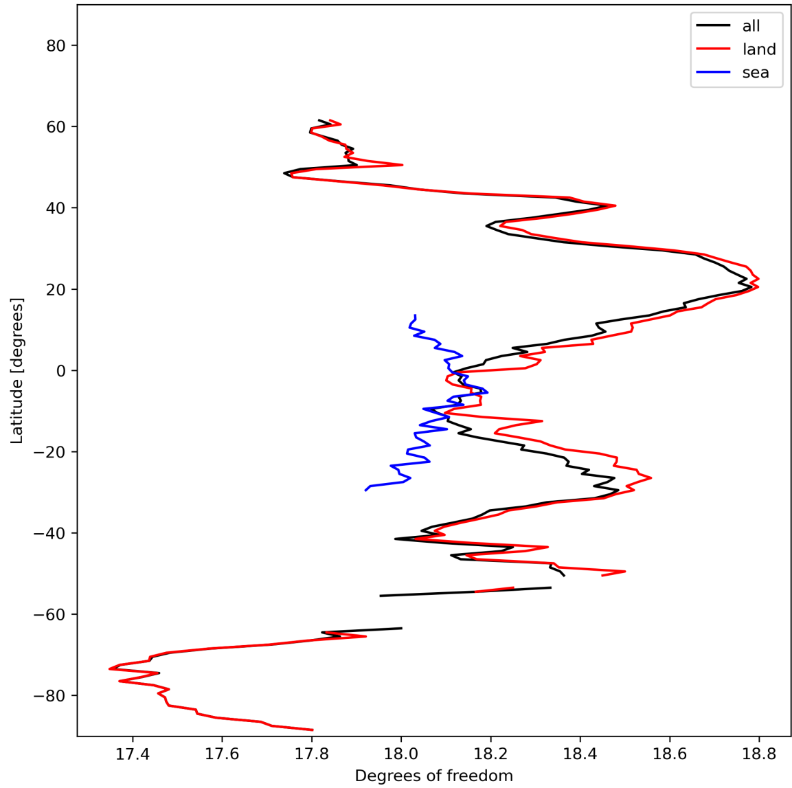
Figure 19: Zonal average of “Degrees of freedom” for 2024-02-12 to 2024-02-14.
