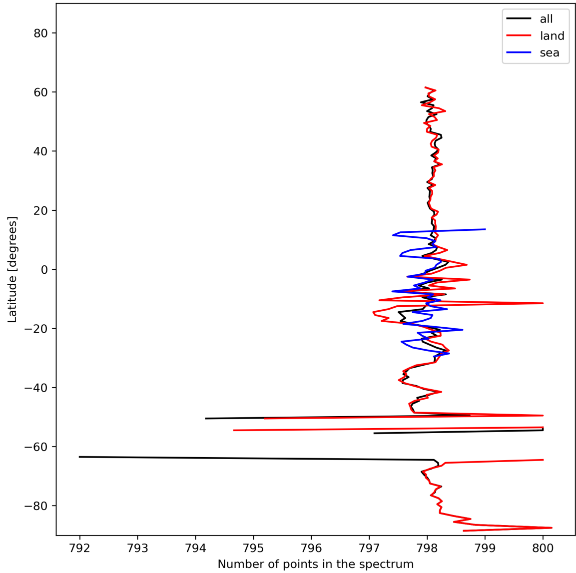
Figure 15: Zonal average of “Number of points in the spectrum” for 2024-02-12 to 2024-02-14.
