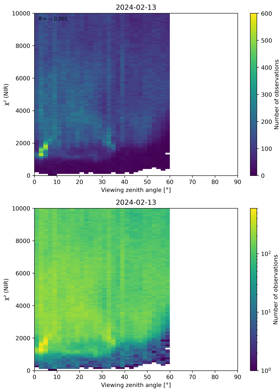
Figure 105: Scatter density plot of “Viewing zenith angle” against “ \chi^2 (NIR)” for 2024-02-12 to 2024-02-14.
