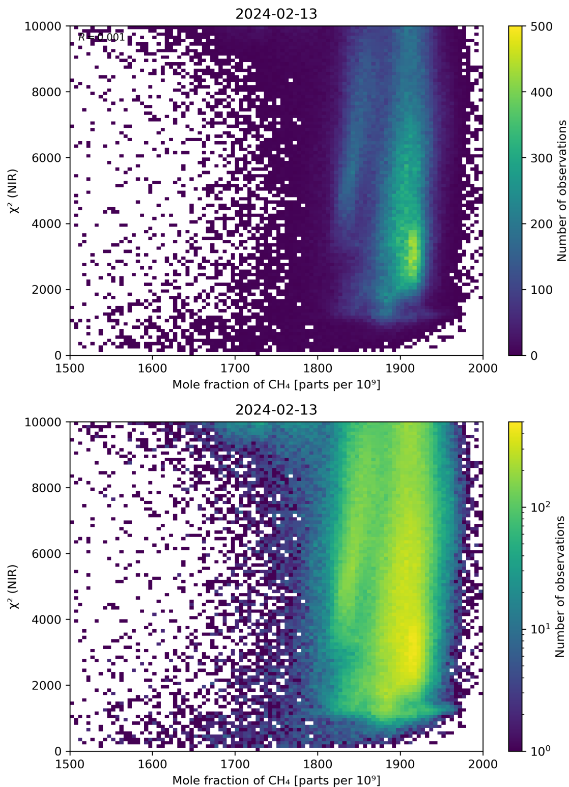
Figure 70: Scatter density plot of “Mole fraction of CH 4 ” against “ \chi^2 (NIR)” for 2024-02-12 to 2024-02-14.
