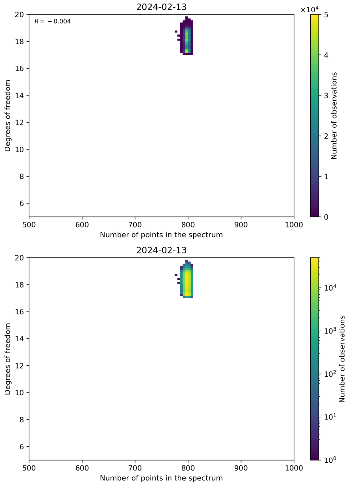
Figure 90: Scatter density plot of “Number of points in the spectrum” against “Degrees of freedom” for 2024-02-12 to 2024-02-14.
