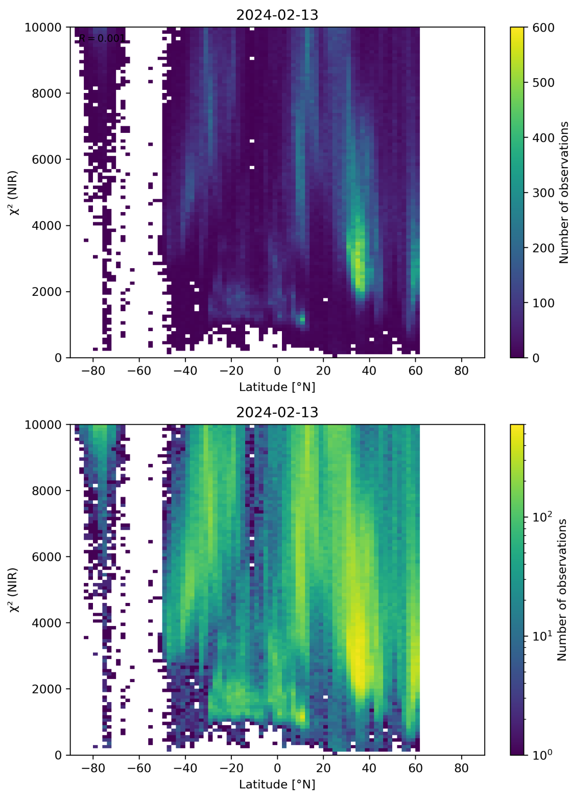
Figure 53: Scatter density plot of “Latitude” against “ \chi^2 (NIR)” for 2024-02-12 to 2024-02-14.
