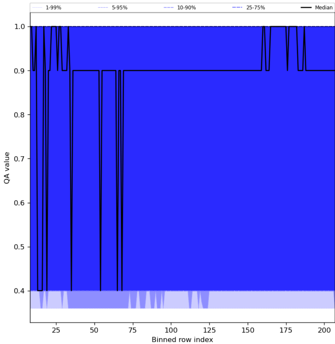
Figure 33: Along track statistics of “QA value” for 2024-02-12 to 2024-02-14
