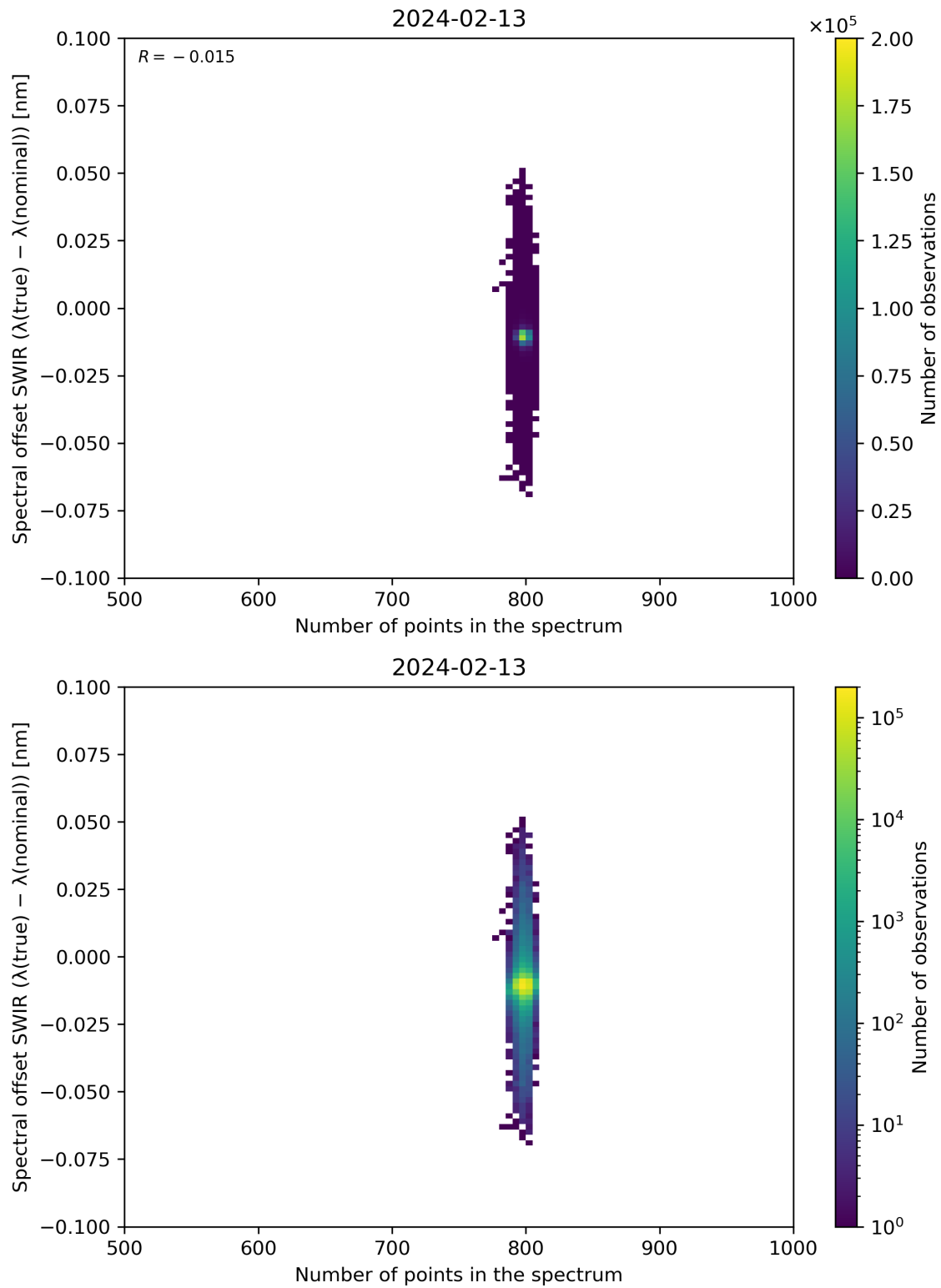
Figure 93: Scatter density plot of “Number of points in the spectrum” against “Spectral offset SWIR ( \lambda(\text{true}) - \lambda(\text{nominal}) )” for 2024-02-12 to 2024-02-14.
