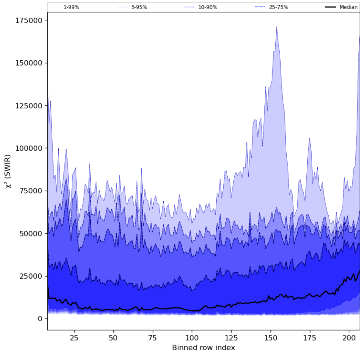
Figure 39: Along track statistics of “ \chi^2 (SWIR)” for 2024-02-12 to 2024-02-14
