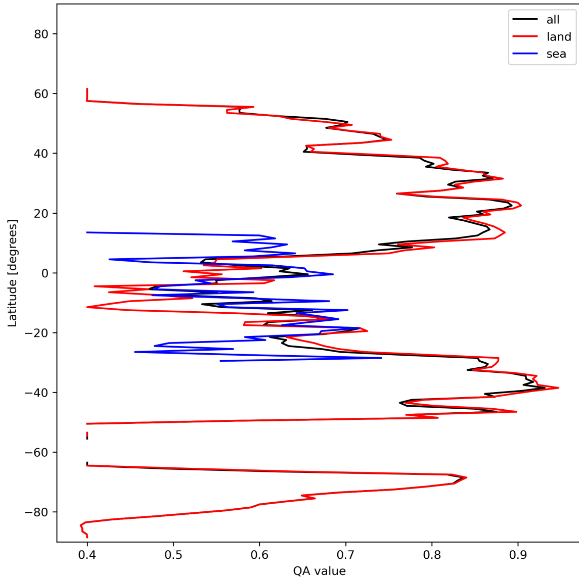
Figure 11: Zonal average of “QA value” for 2024-02-12 to 2024-02-14.
