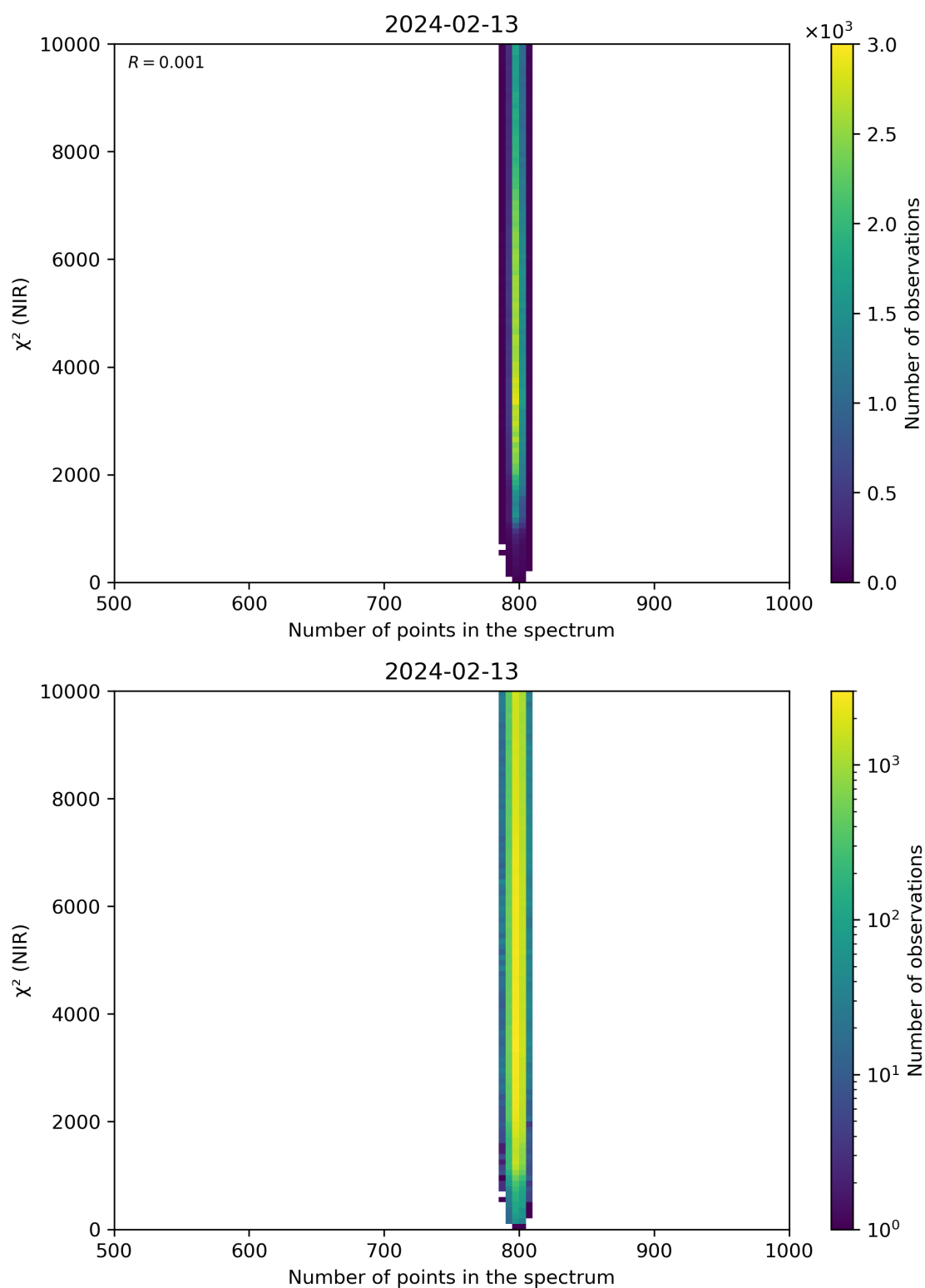
Figure 88: Scatter density plot of “Number of points in the spectrum” against “ \chi^2 (NIR)” for 2024-02-12 to 2024-02-14.
