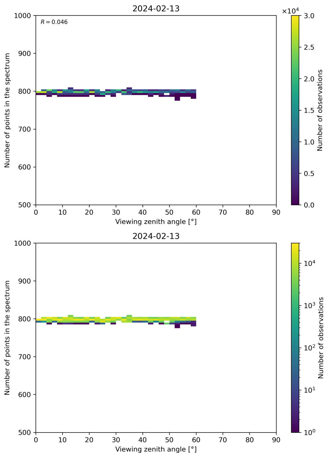
Figure 114: Scatter density plot of “Viewing zenith angle” against “Number of points in the spectrum” for 2024-02-12 to 2024-02-14.
