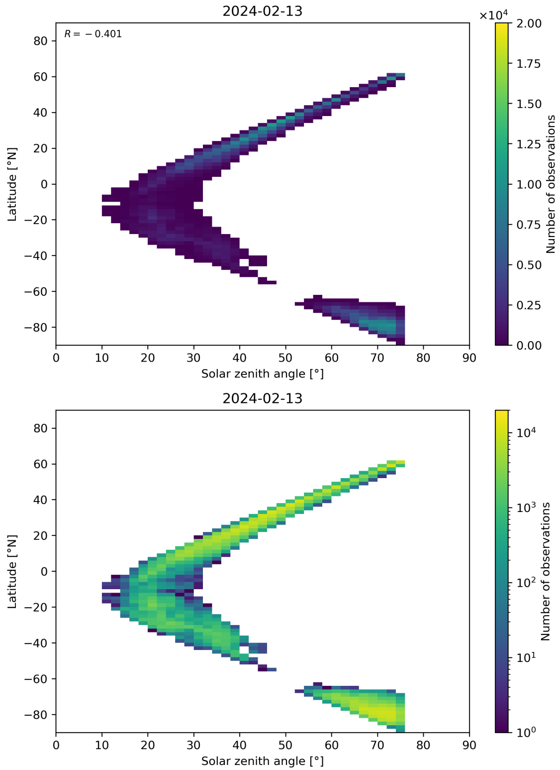
Figure 98: Scatter density plot of “Solar zenith angle” against “Latitude” for 2024-02-12 to 2024-02-14.
