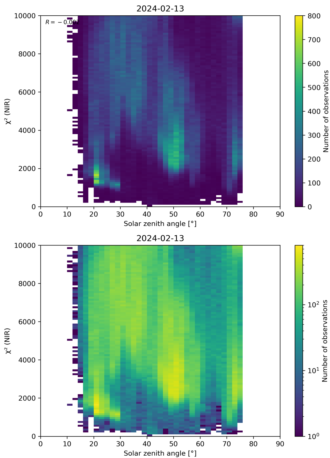
Figure 94: Scatter density plot of “Solar zenith angle” against “ \chi^2 (NIR)” for 2024-02-12 to 2024-02-14.
