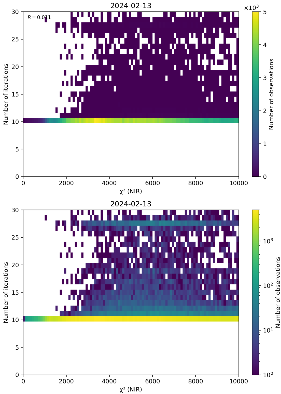
Figure 46: Scatter density plot of “ \chi^2 (NIR)” against “Number of iterations” for 2024-02-12 to 2024-02-14.
