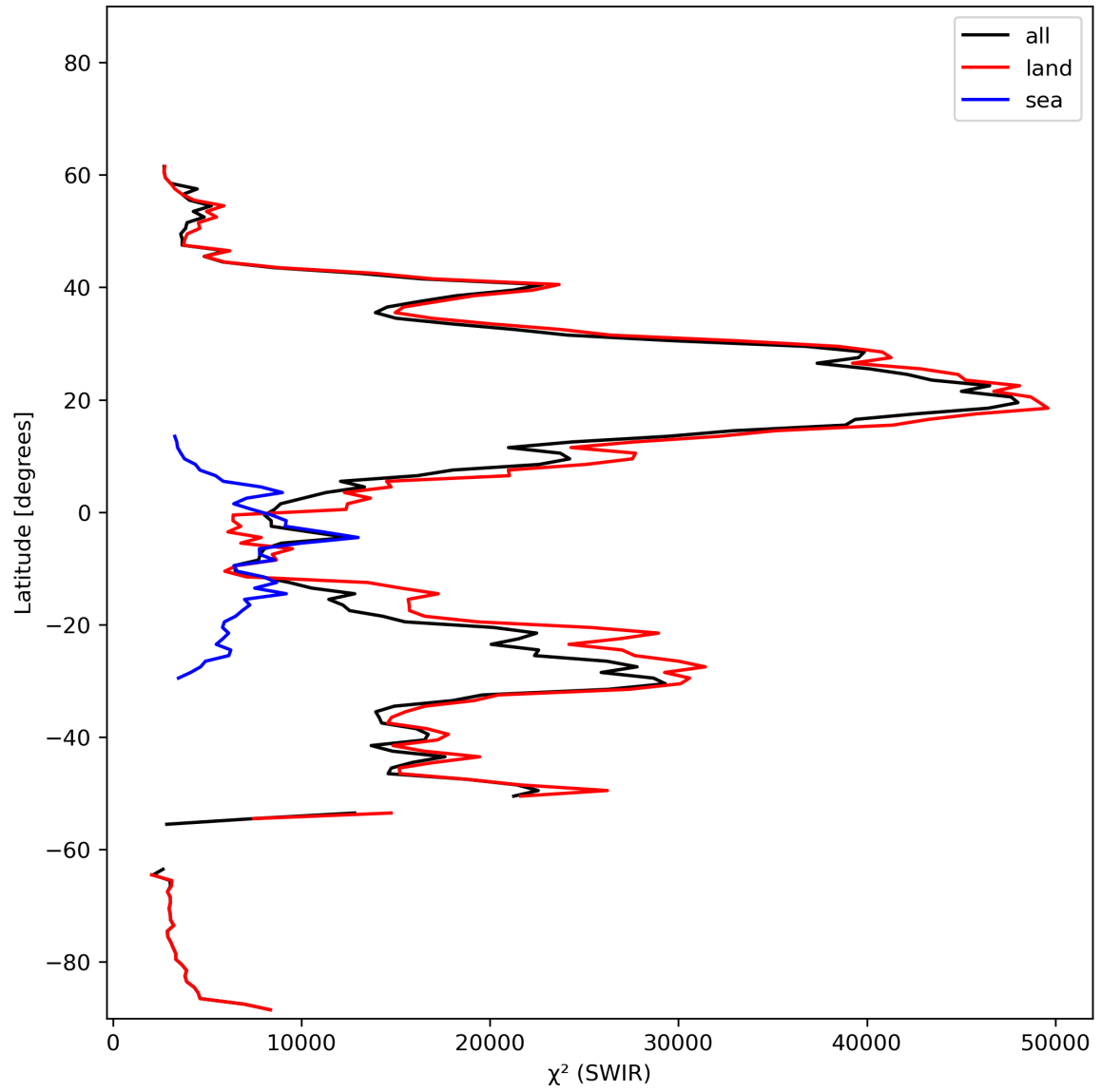
Figure 17: Zonal average of “ \chi^2 (SWIR)” for 2024-02-12 to 2024-02-14.
