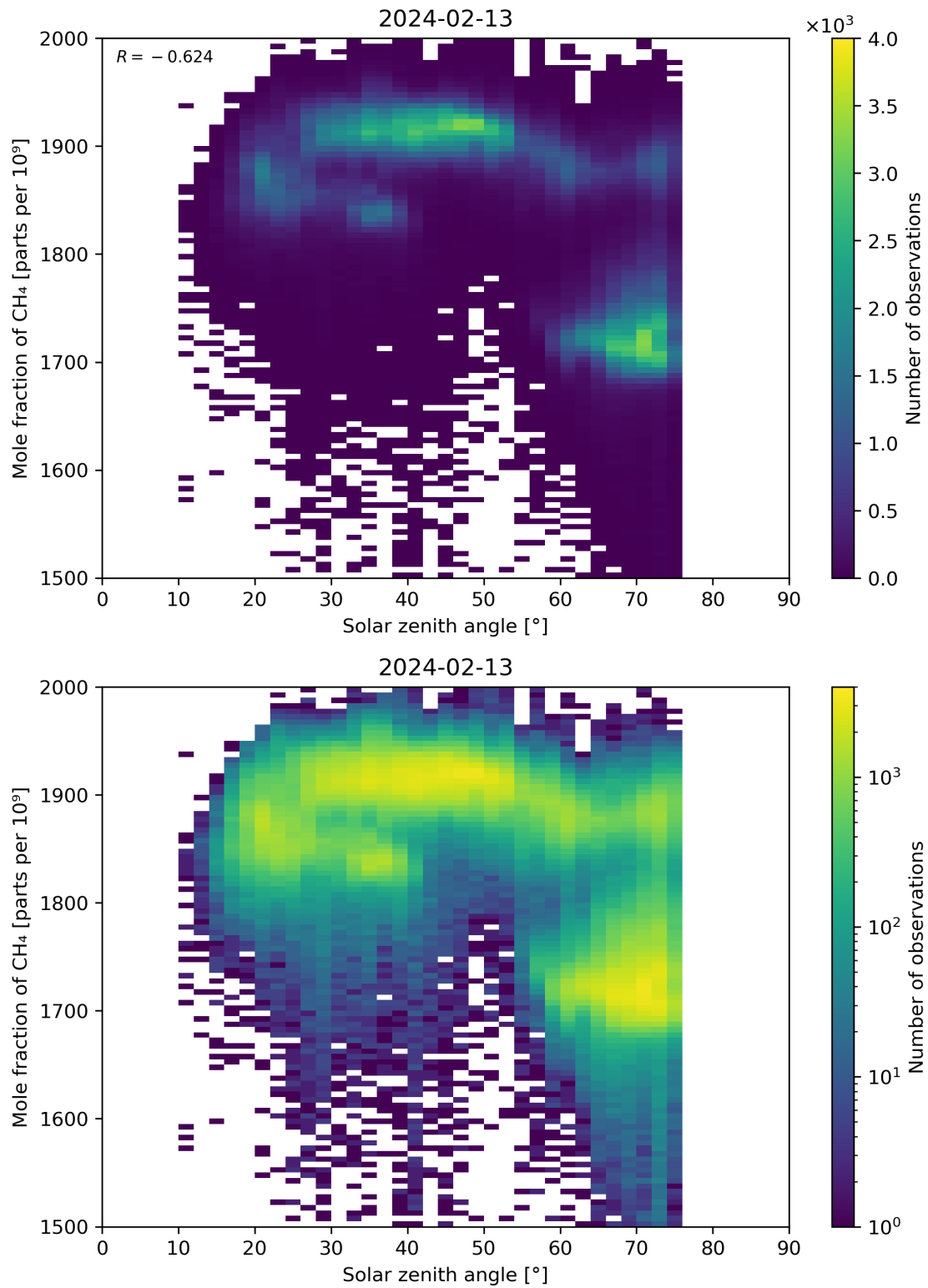
Figure 99: Scatter density plot of “Solar zenith angle” against “Mole fraction of CH 4 ” for 2024-02-12 to 2024-02-14.
