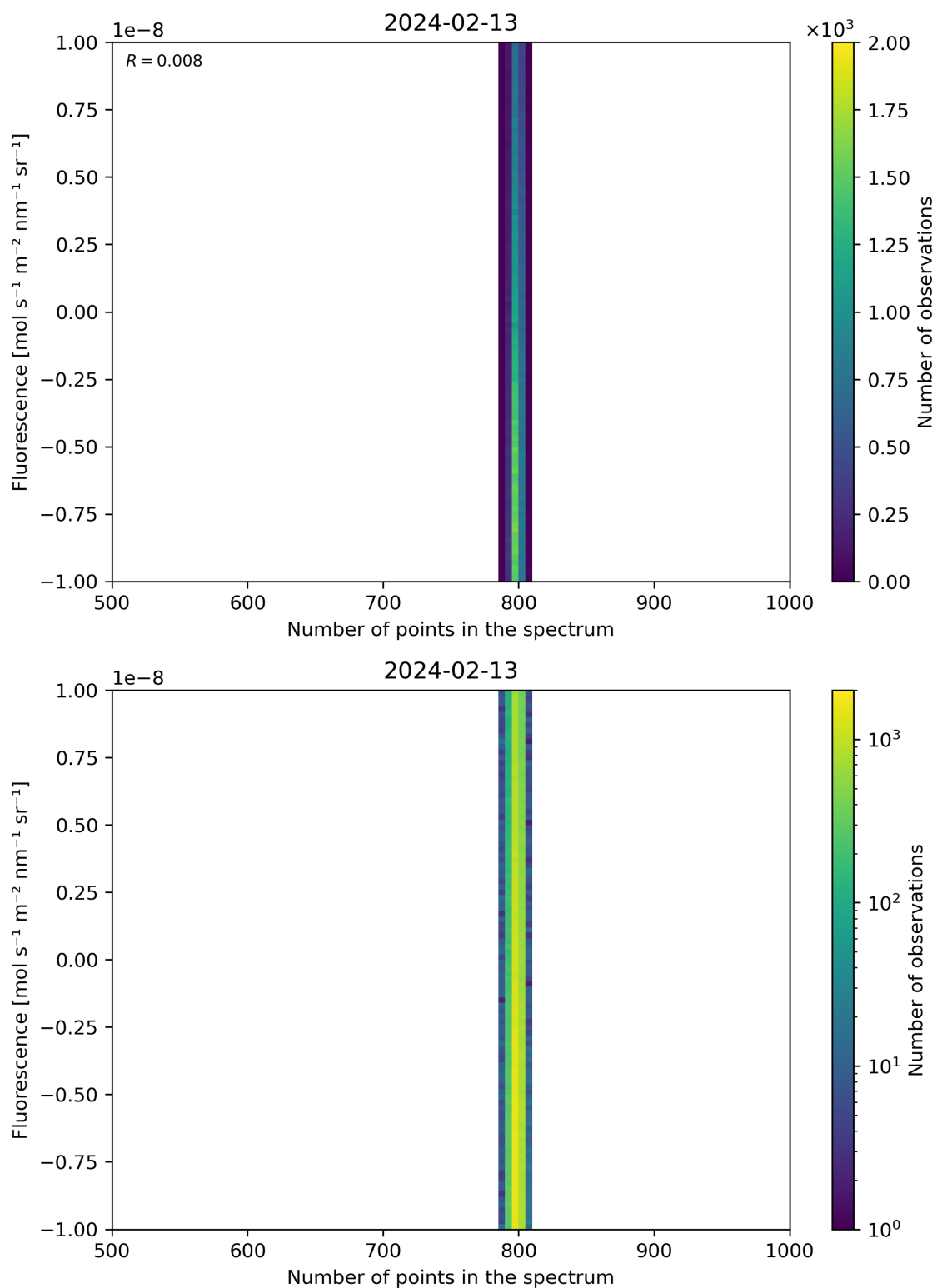
Figure 91: Scatter density plot of “Number of points in the spectrum” against “Fluorescence” for 2024-02-12 to 2024-02-14.
