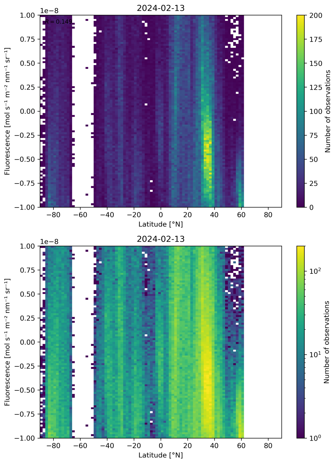
Figure 56: Scatter density plot of “Latitude” against “Fluorescence” for 2024-02-12 to 2024-02-14.
