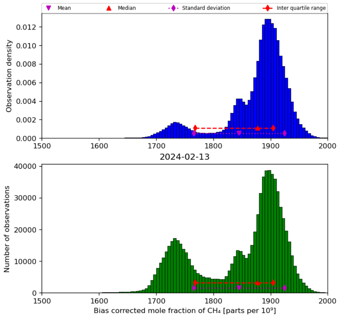
Figure 25: Histogram of “Bias corrected mole fraction of CH 4 ” for 2024-02-12 to 2024-02-14
