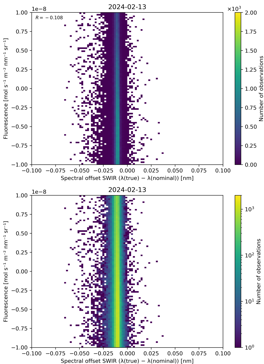
Figure 120: Scatter density plot of “Spectral offset SWIR ( \lambda(\text{true}) - \lambda(\text{nominal}) )” against “Fluorescence” for 2024-02-12 to 2024-02-14.
