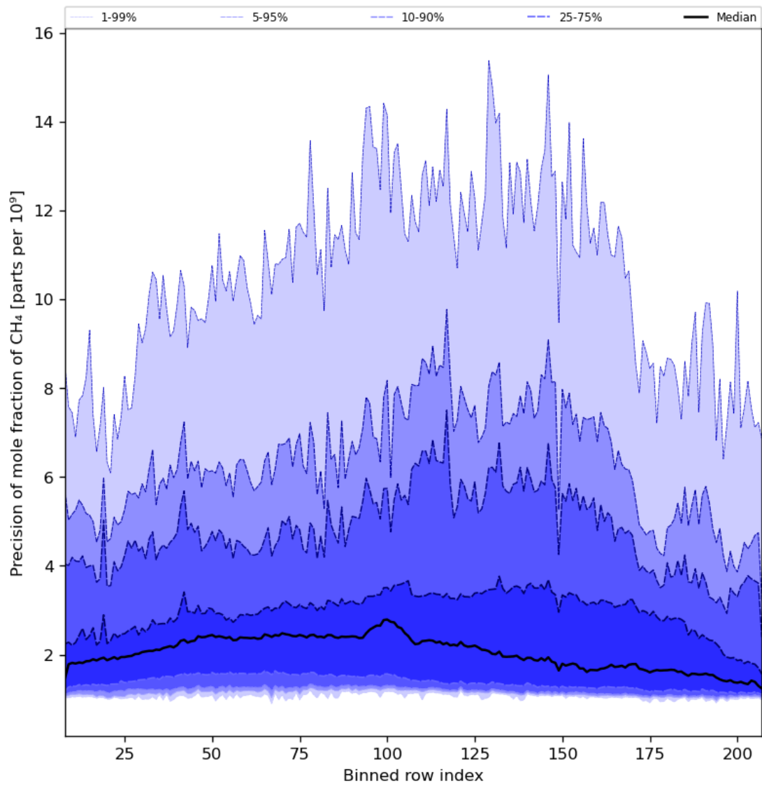
Figure 35: Along track statistics of “Precision of mole fraction of CH 4 ” for 2024-02-12 to 2024-02-14
