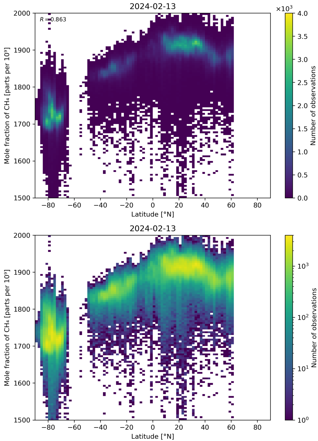
Figure 57: Scatter density plot of “Latitude” against “Mole fraction of CH 4 ” for 2024-02-12 to 2024-02-14.
