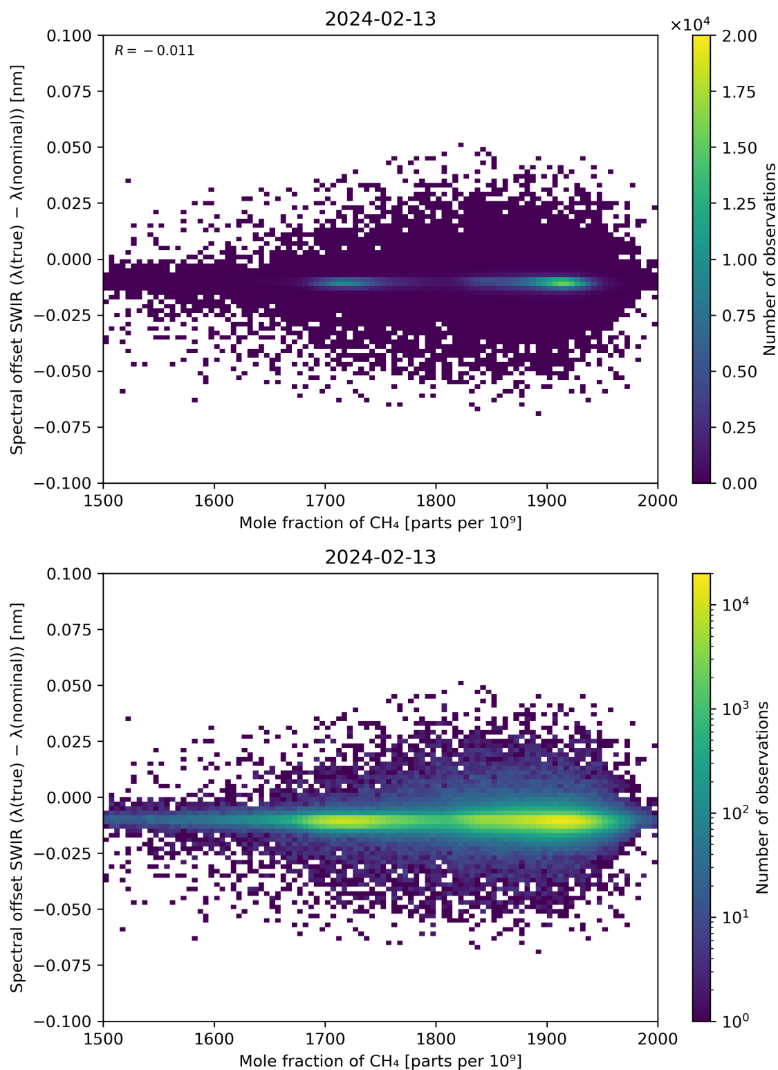
Figure 86: Scatter density plot of “Mole fraction of CH 4 ” against “Spectral offset SWIR ( \lambda(\text{true}) - \lambda(\text{nominal}) )” for 2024-02-12 to 2024-02-14.
