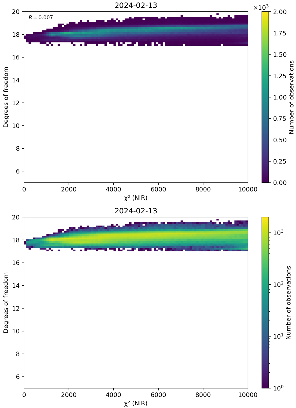
Figure 44: Scatter density plot of “ \chi^2 (NIR)” against “Degrees of freedom” for 2024-02-12 to 2024-02-14.
