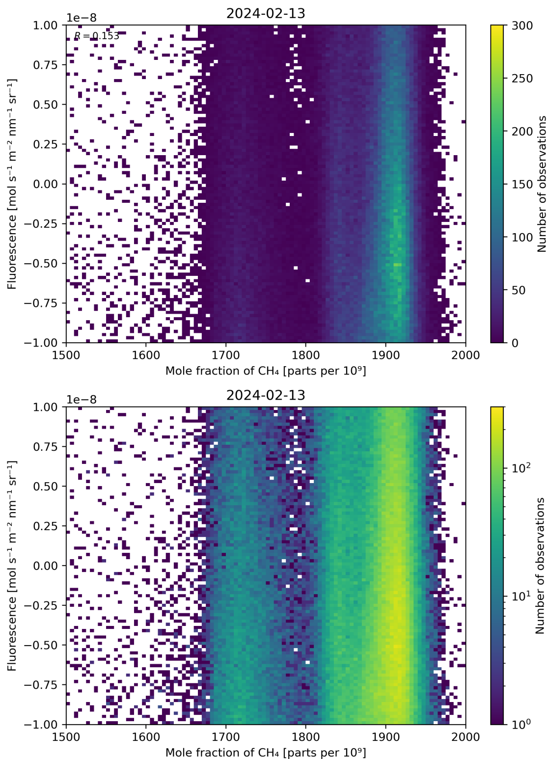
Figure 73: Scatter density plot of “Mole fraction of CH 4 ” against “Fluorescence” for 2024-02-12 to 2024-02-14.
