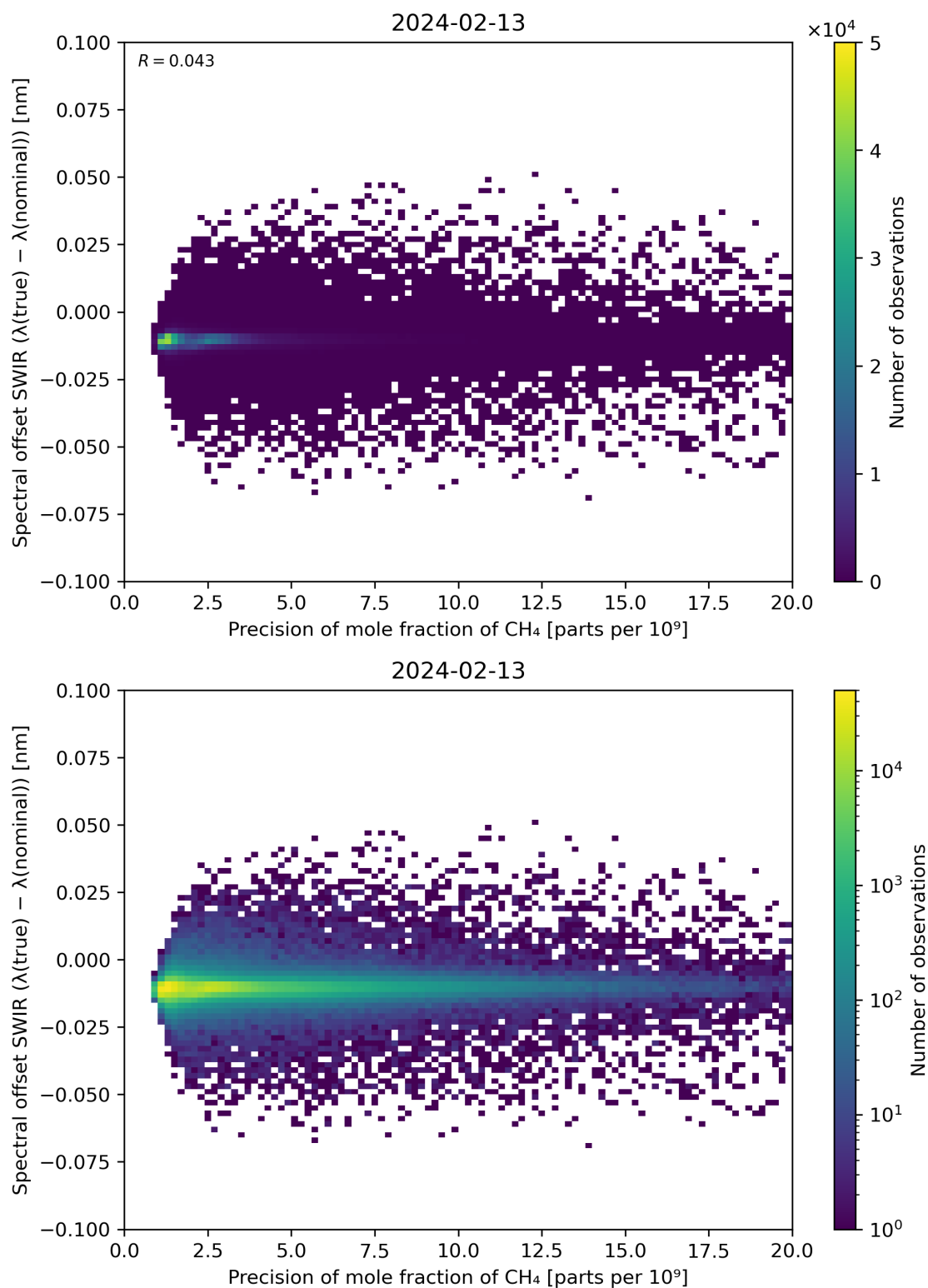
Figure 85: Scatter density plot of “Precision of mole fraction of CH 4 ” against “Spectral offset SWIR ( \lambda(\text{true}) - \lambda(\text{nominal}) )” for 2024-02-12 to 2024-02-14.
