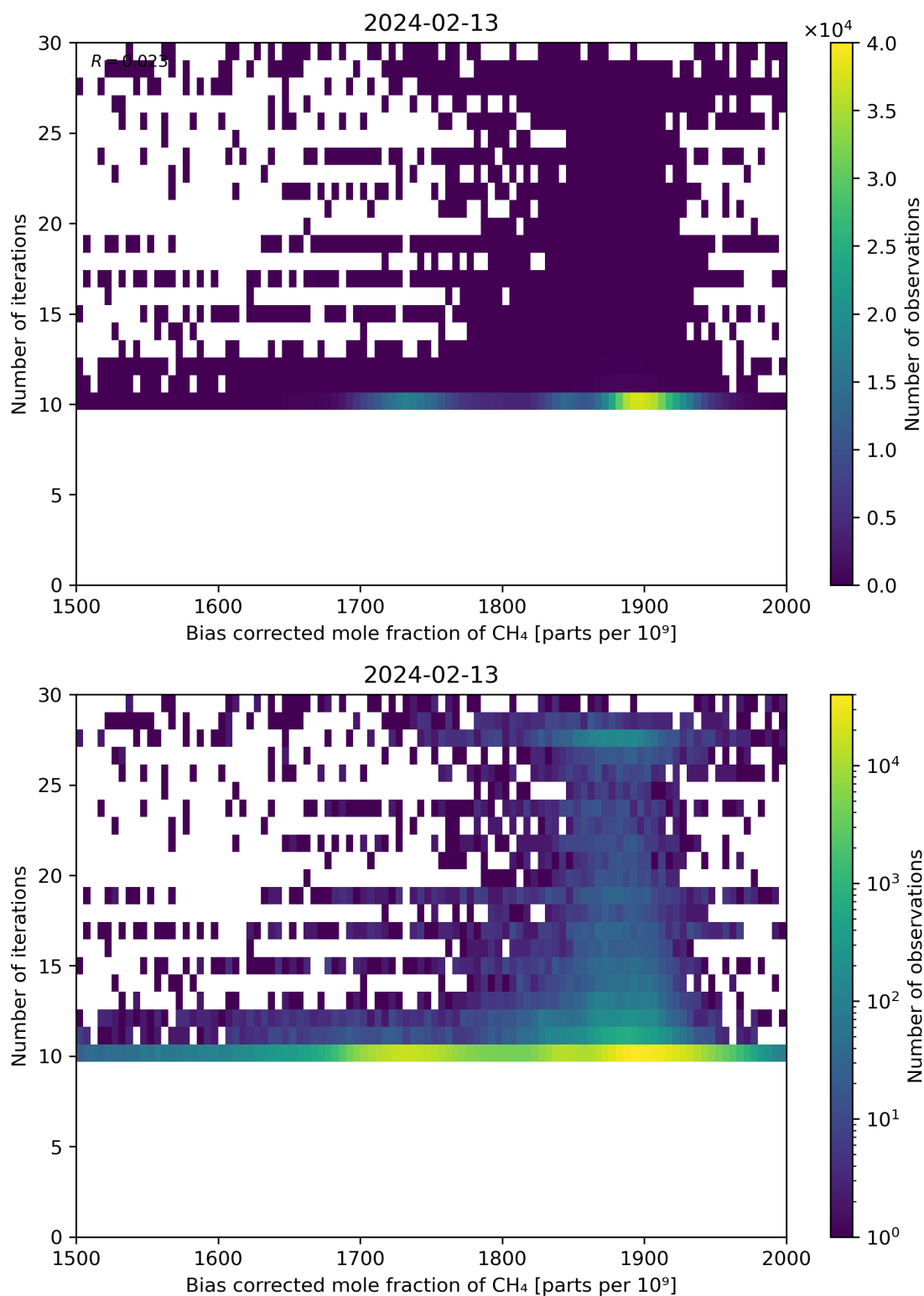
Figure 67: Scatter density plot of “Bias corrected mole fraction of \text{CH}_4 ” against “Number of iterations” for 2024-02-12 to 2024-02-14.
