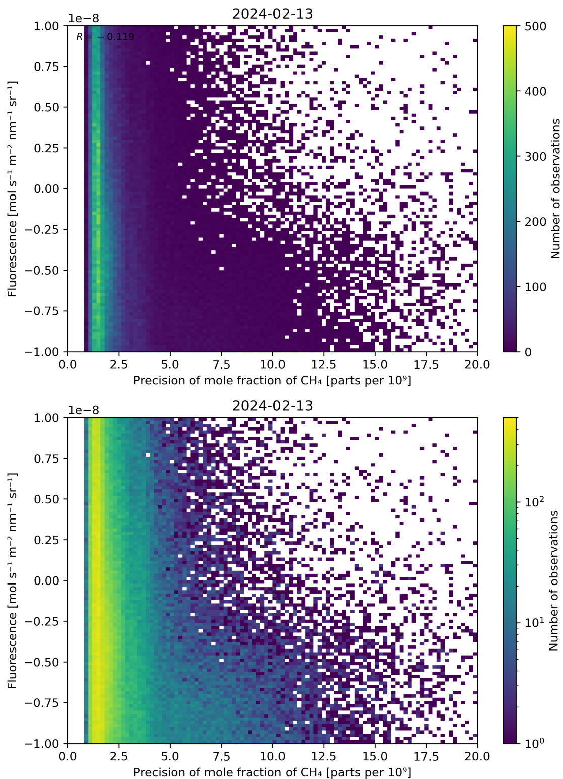
Figure 81: Scatter density plot of “Precision of mole fraction of \text{CH}_4 ” against “Fluorescence” for 2024-02-12 to 2024-02-14.
