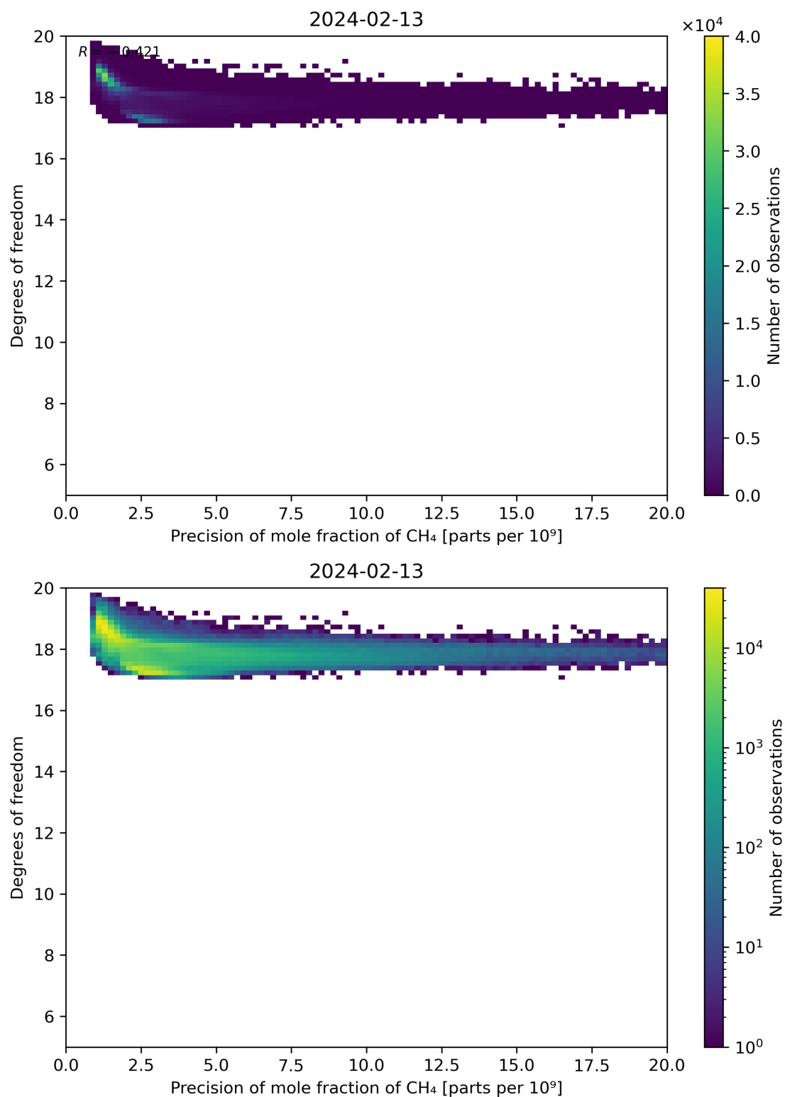
Figure 80: Scatter density plot of “Precision of mole fraction of CH 4 ” against “Degrees of freedom” for 2024-02-12 to 2024-02-14.
