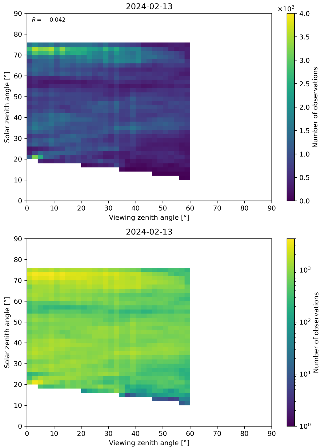
Figure 115: Scatter density plot of “Viewing zenith angle” against “Solar zenith angle” for 2024-02-12 to 2024-02-14.
