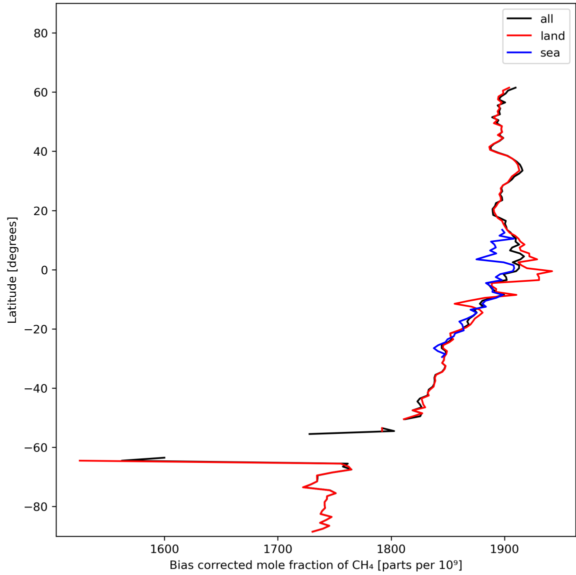
Figure 14: Zonal average of “Bias corrected mole fraction of CH 4 ” for 2024-02-12 to 2024-02-14.
