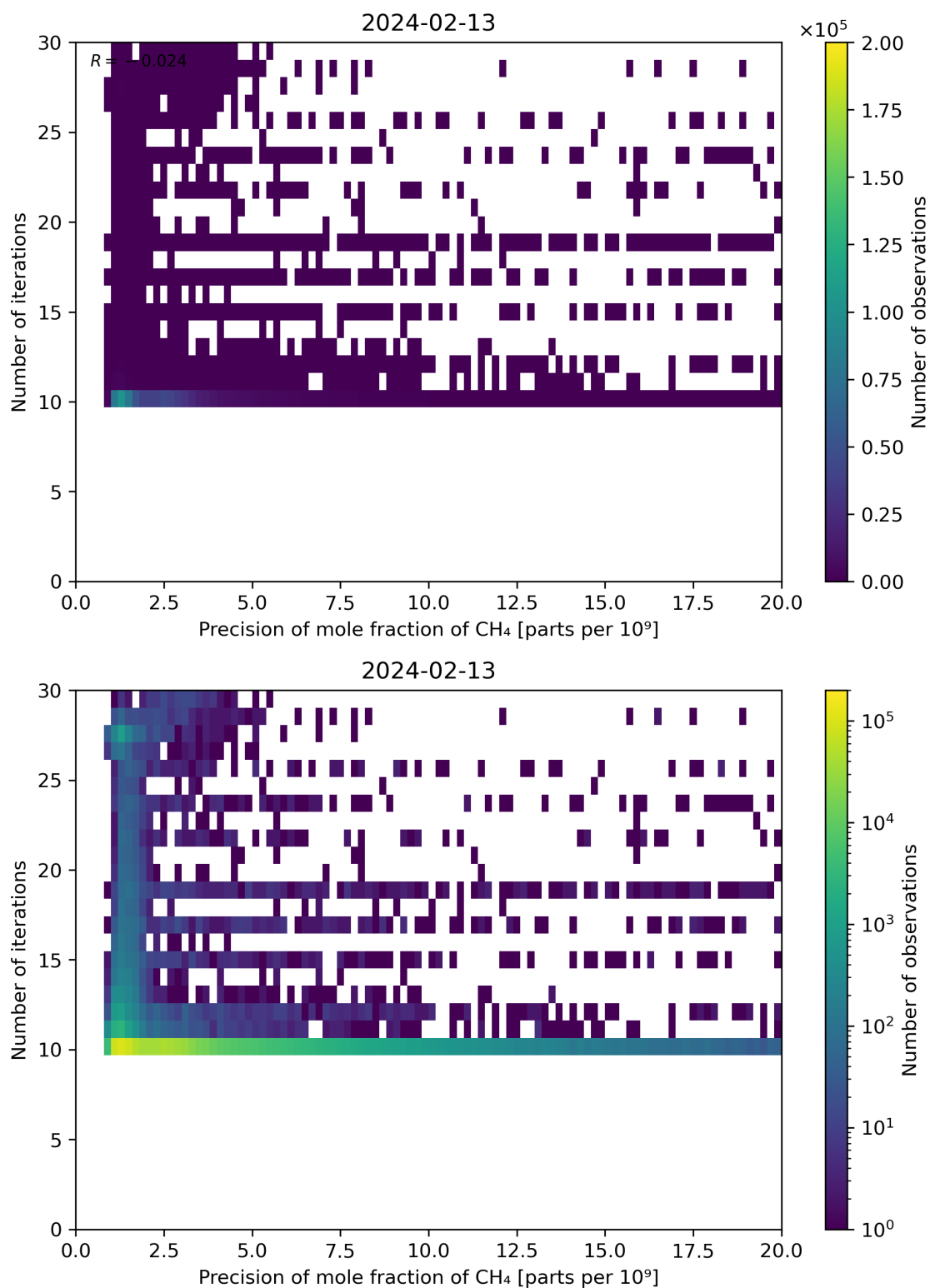
Figure 83: Scatter density plot of “Precision of mole fraction of CH 4 ” against “Number of iterations” for 2024-02-12 to 2024-02-14.
