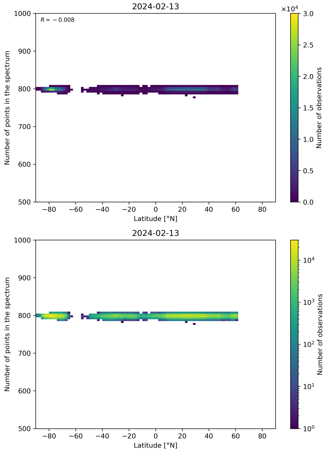
Figure 61: Scatter density plot of “Latitude” against “Number of points in the spectrum” for 2024-02-12 to 2024-02-14.
