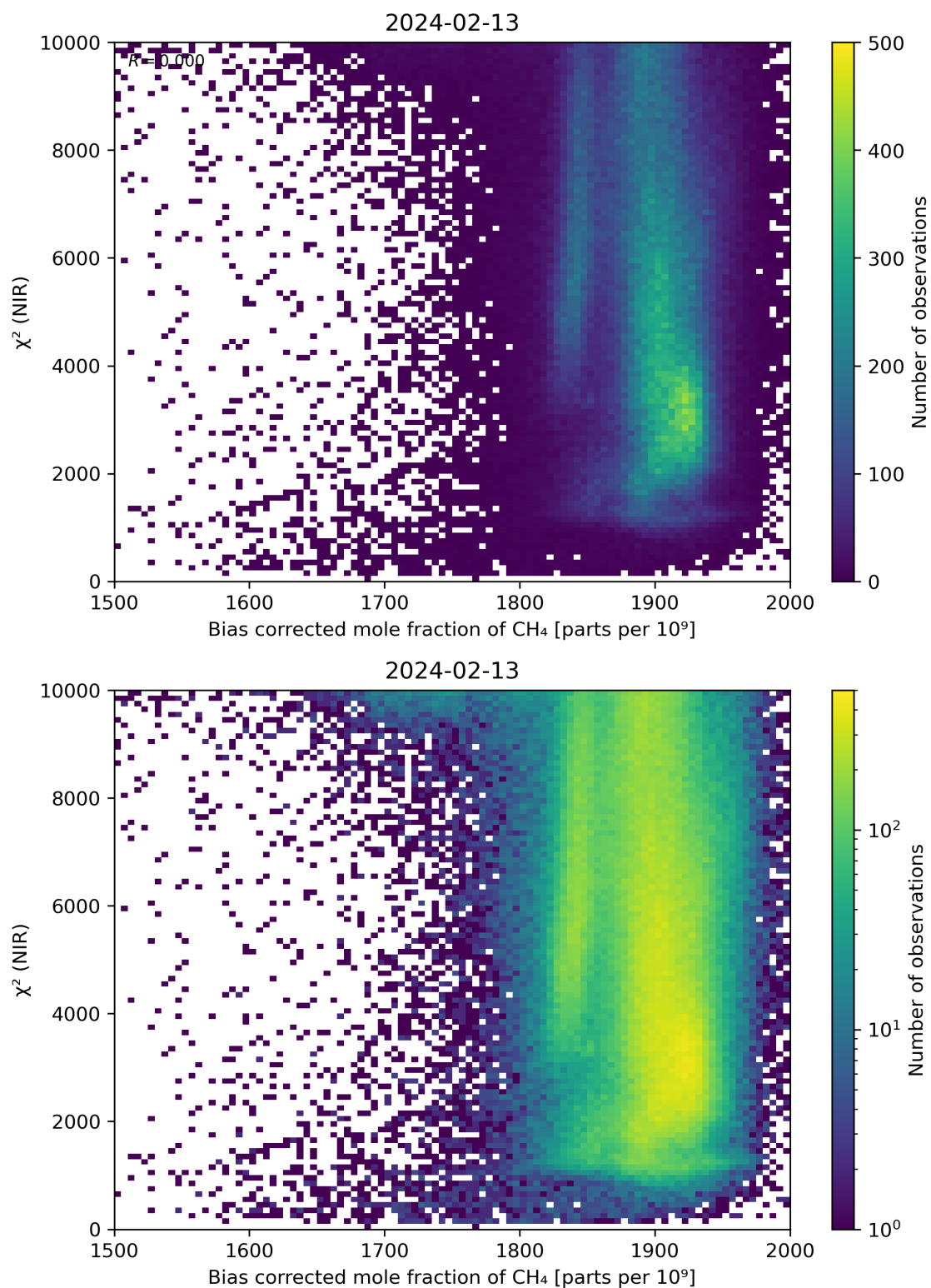
Figure 63: Scatter density plot of “Bias corrected mole fraction of \text{CH}_4 ” against “ \chi^2 (NIR)” for 2024-02-12 to 2024-02-14.
