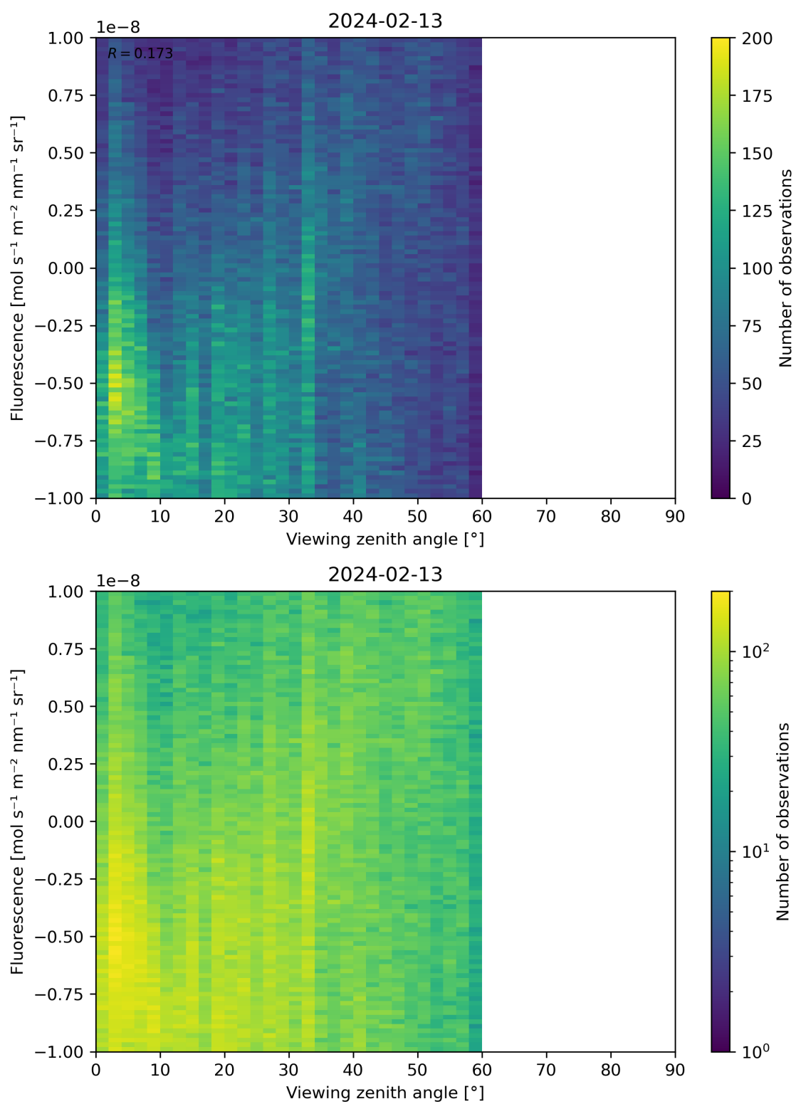
Figure 108: Scatter density plot of “Viewing zenith angle” against “Fluorescence” for 2024-02-12 to 2024-02-14.
