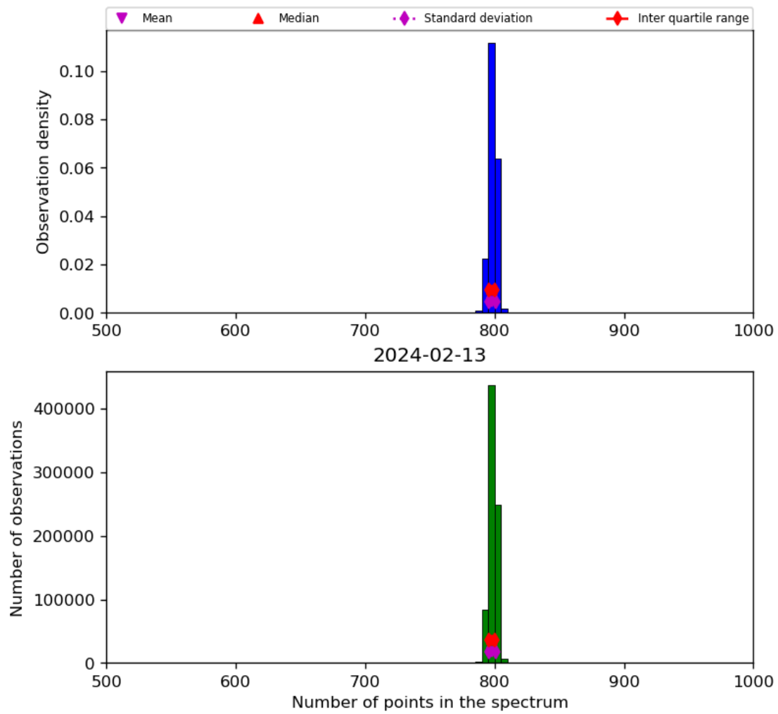
Figure 26: Histogram of “Number of points in the spectrum” for 2024-02-12 to 2024-02-14
