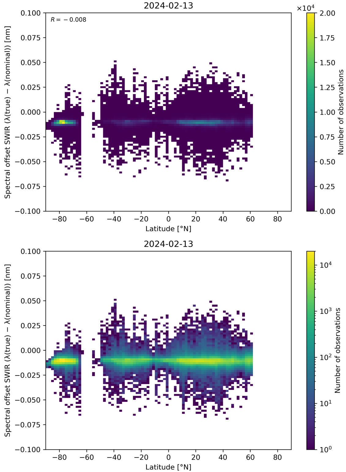
Figure 62: Scatter density plot of “Latitude” against “Spectral offset SWIR ( \lambda(\text{true}) - \lambda(\text{nominal}) )” for 2024-02-12 to 2024-02-14.
