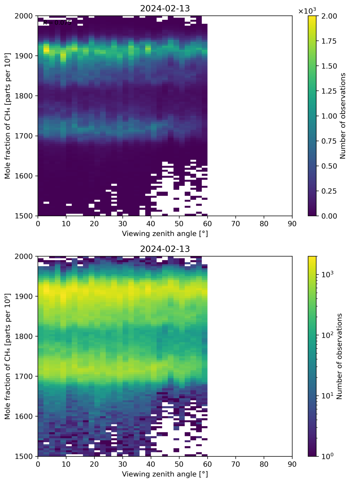
Figure 110: Scatter density plot of “Viewing zenith angle” against “Mole fraction of CH 4 ” for 2024-02-12 to 2024-02-14.
