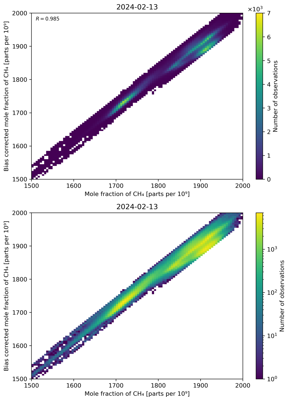
Figure 74: Scatter density plot of “Mole fraction of CH 4 ” against “Bias corrected mole fraction of CH 4 ” for 2024-02-12 to 2024-02-14.
