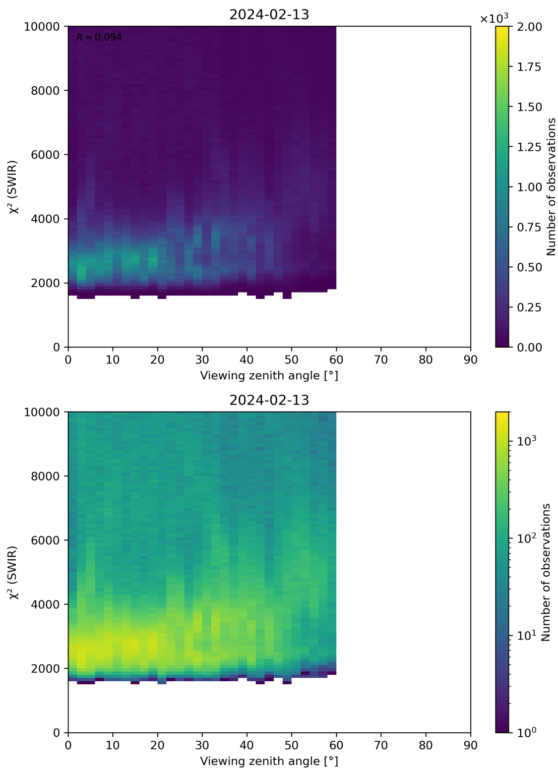
Figure 106: Scatter density plot of “Viewing zenith angle” against “ \chi^2 (SWIR)” for 2024-02-12 to 2024-02-14.
