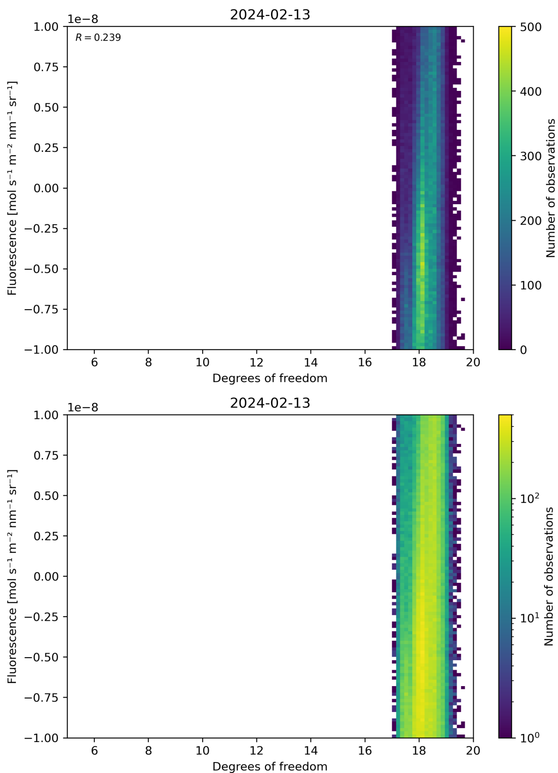
Figure 51: Scatter density plot of “Degrees of freedom” against “Fluorescence” for 2024-02-12 to 2024-02-14.
