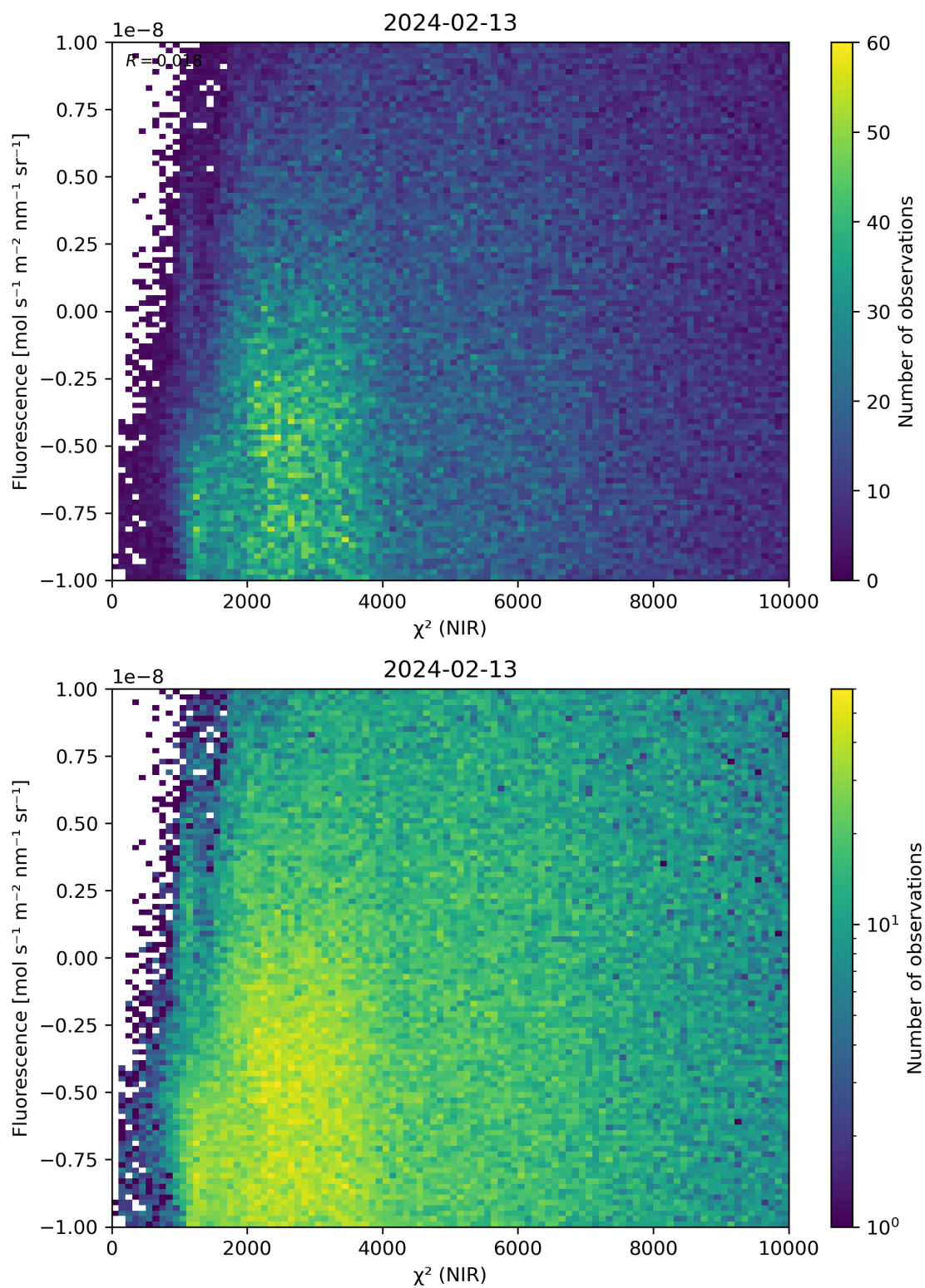
Figure 45: Scatter density plot of “ \chi^2 (NIR)” against “Fluorescence” for 2024-02-12 to 2024-02-14.
