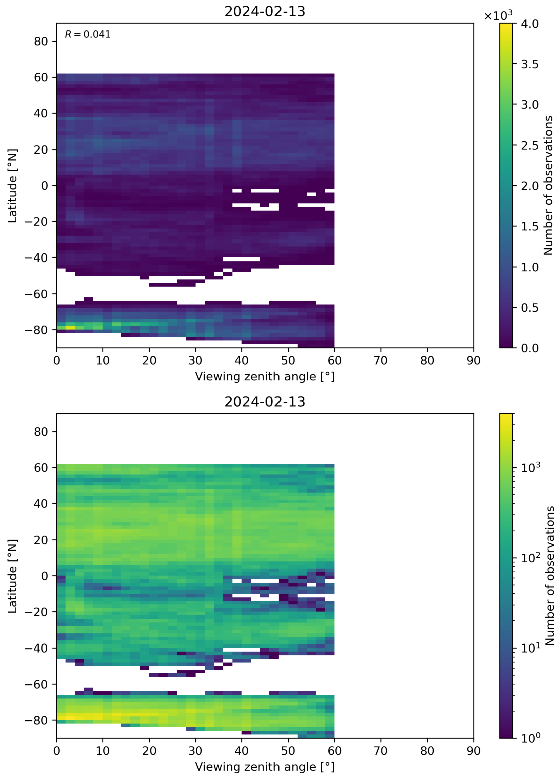
Figure 109: Scatter density plot of “Viewing zenith angle” against “Latitude” for 2024-02-12 to 2024-02-14.
