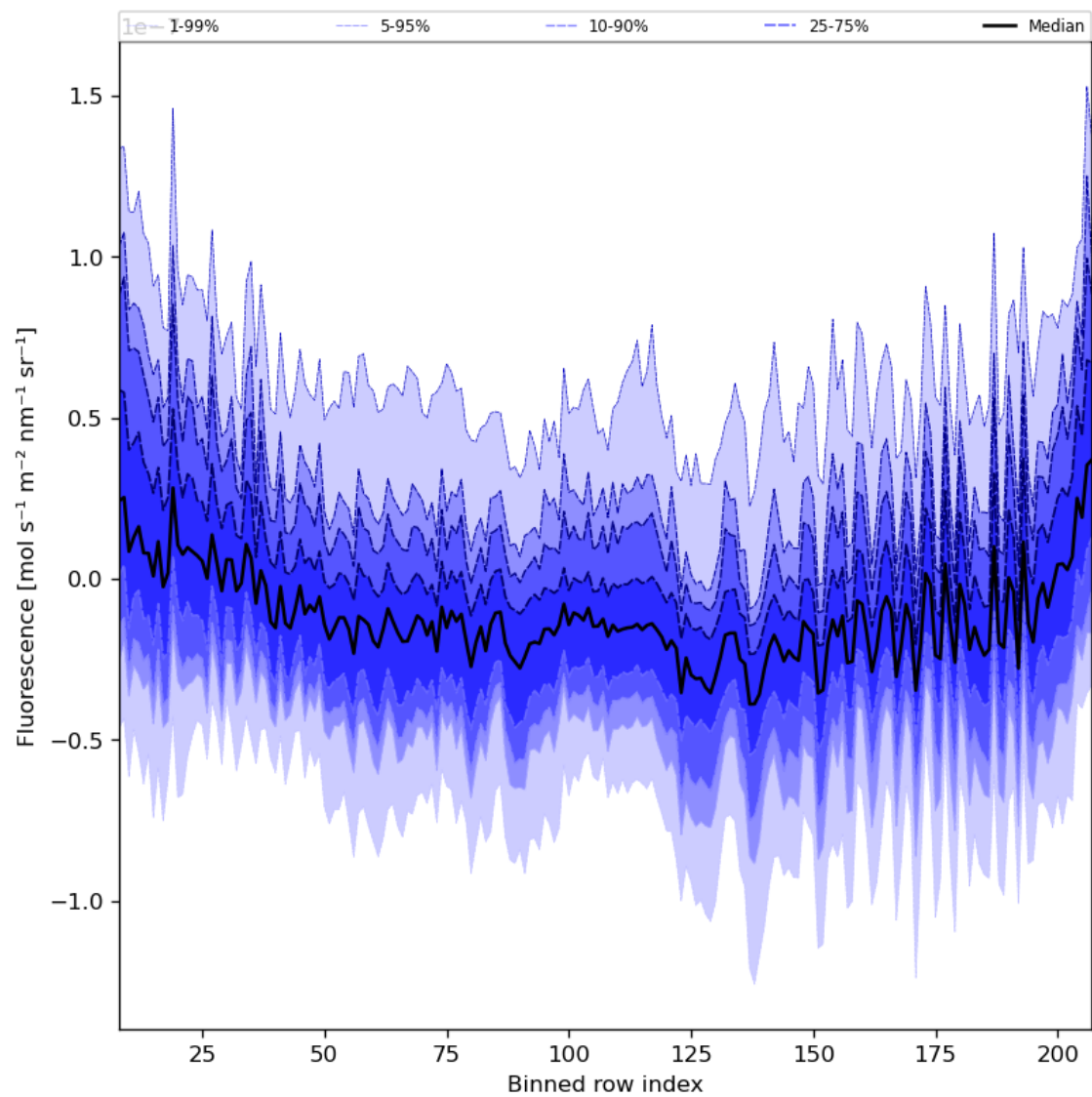
Figure 43: Along track statistics of “Fluorescence” for 2024-02-12 to 2024-02-14
