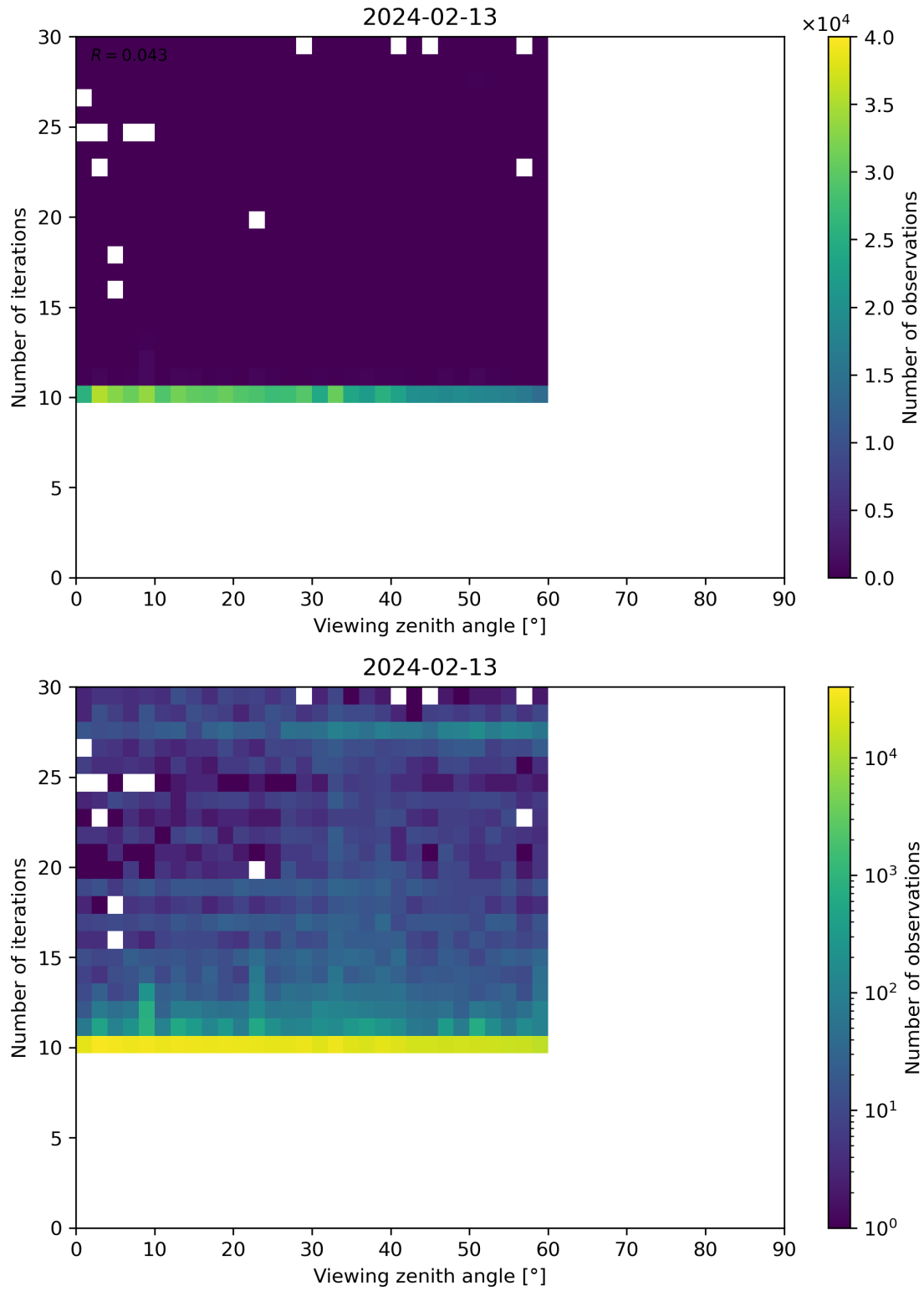
Figure 113: Scatter density plot of “Viewing zenith angle” against “Number of iterations” for 2024-02-12 to 2024-02-14.
