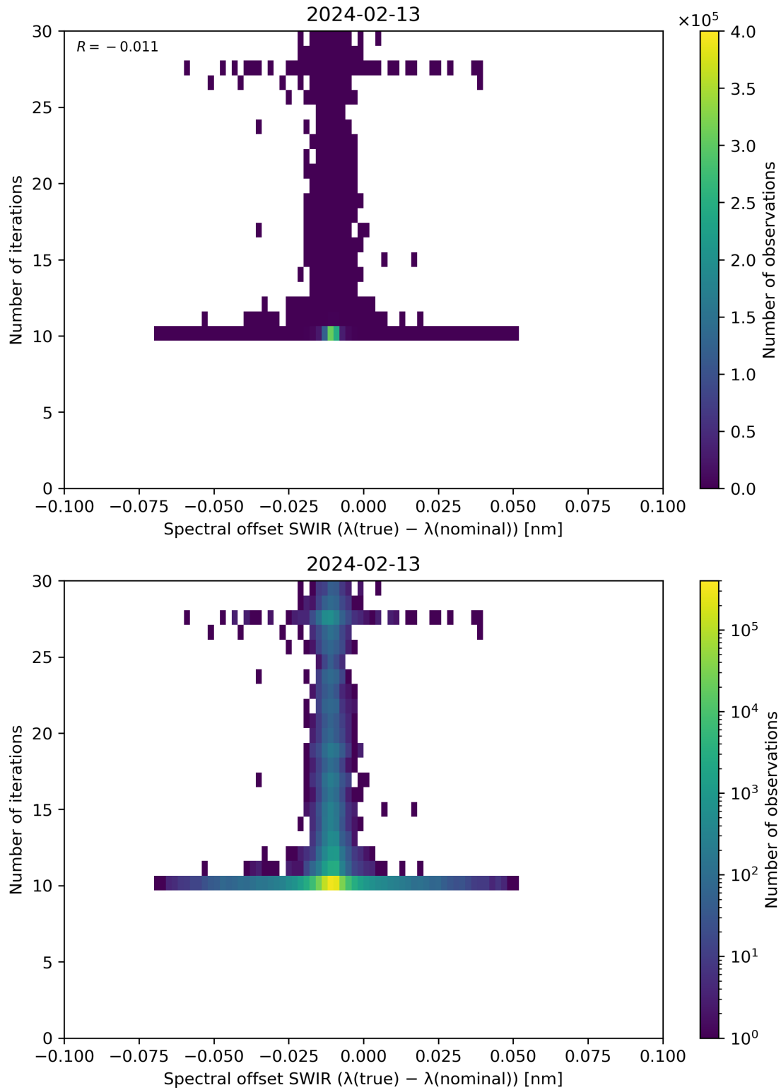
Figure 121: Scatter density plot of “Spectral offset SWIR ( \lambda(\text{true}) - \lambda(\text{nominal}) )” against “Number of iterations” for 2024-02-12 to 2024-02-14.
