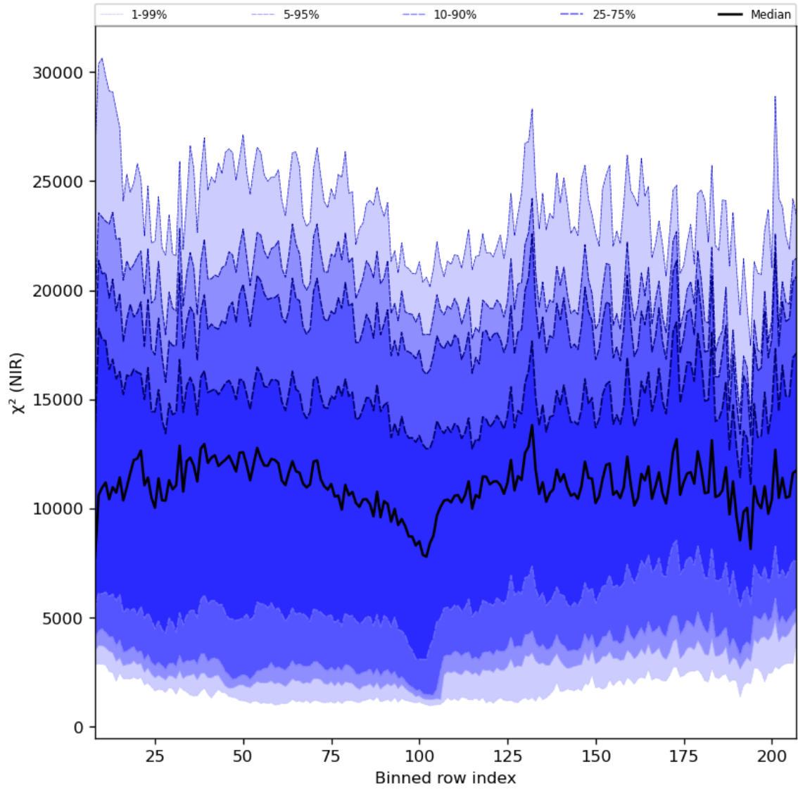
Figure 40: Along track statistics of “ \chi^2 (NIR)” for 2024-02-12 to 2024-02-14
