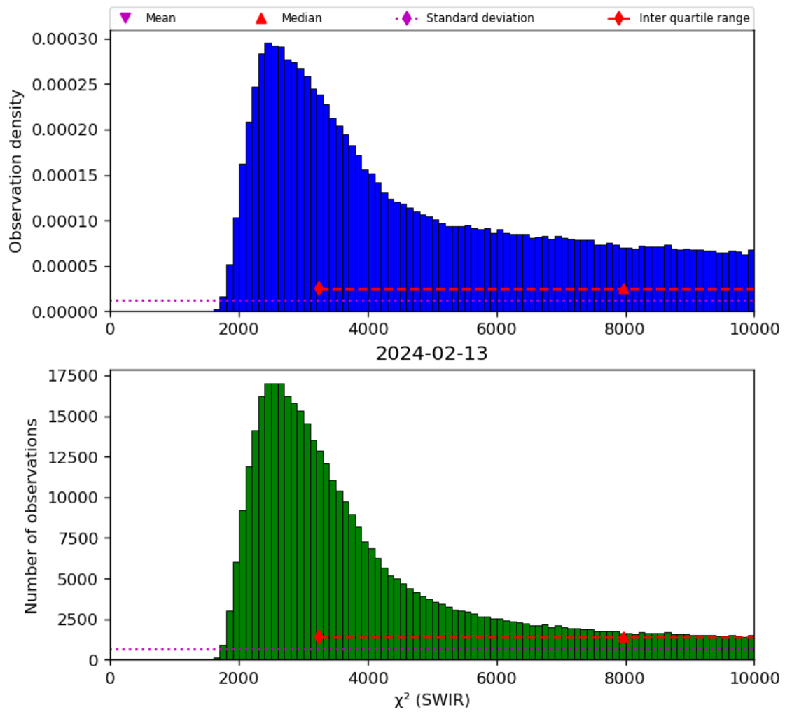
Figure 28: Histogram of “ \chi^2 (SWIR)” for 2024-02-12 to 2024-02-14
