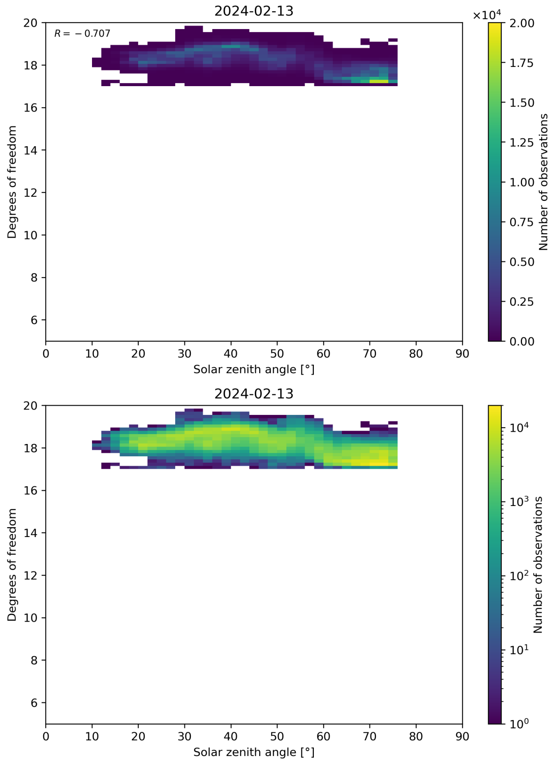
Figure 96: Scatter density plot of “Solar zenith angle” against “Degrees of freedom” for 2024-02-12 to 2024-02-14.
