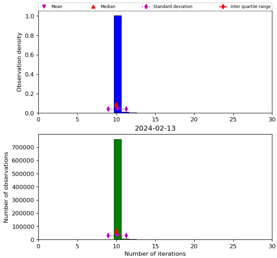
Figure 31: Histogram of “Number of iterations” for 2024-02-12 to 2024-02-14
