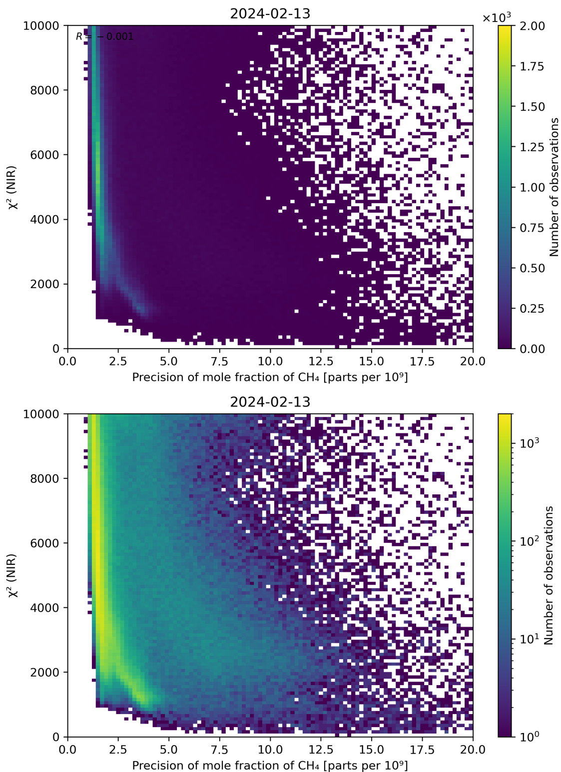
Figure 78: Scatter density plot of “Precision of mole fraction of \text{CH}_4 ” against “ \chi^2 (NIR)” for 2024-02-12 to 2024-02-14.
