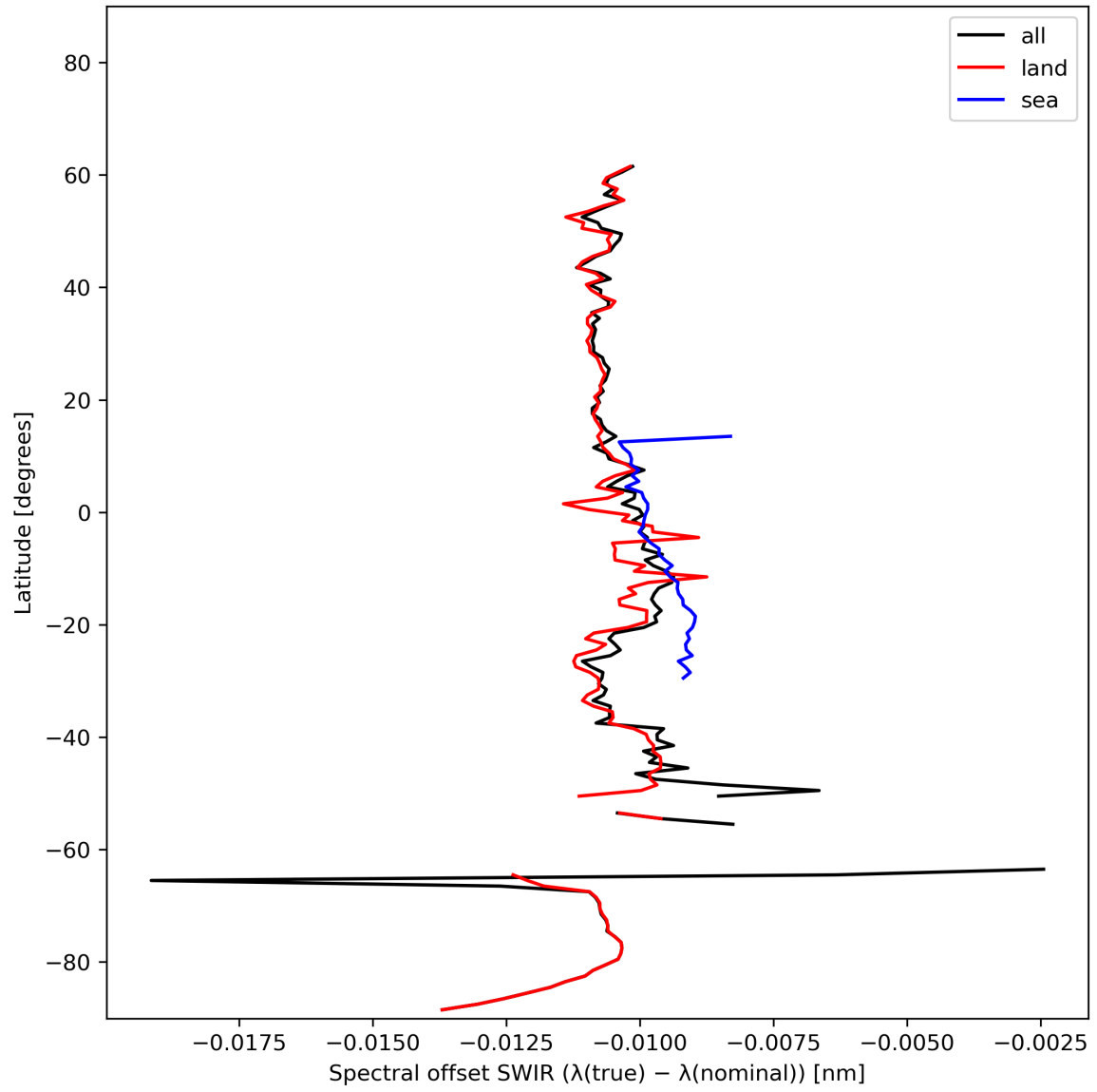
Figure 16: Zonal average of “Spectral offset SWIR ( \lambda(\text{true}) - \lambda(\text{nominal}) )” for 2024-02-12 to 2024-02-14.
