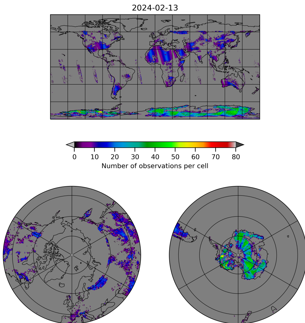
Figure 10: Map of the number of observations for 2024-02-12 to 2024-02-14
