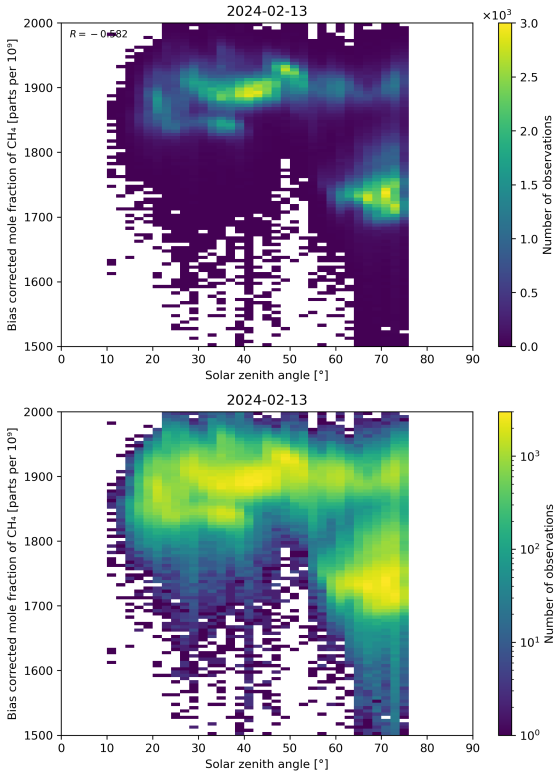
Figure 100: Scatter density plot of “Solar zenith angle” against “Bias corrected mole fraction of CH 4 ” for 2024-02-12 to 2024-02-14.
