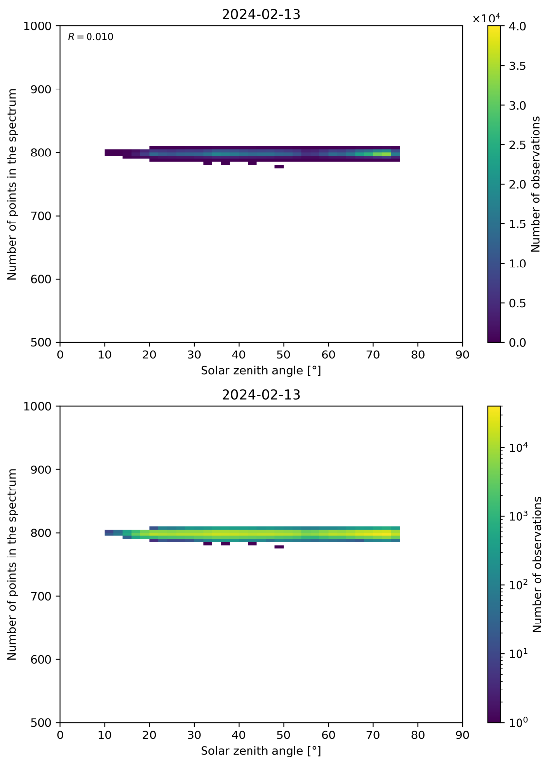
Figure 103: Scatter density plot of “Solar zenith angle” against “Number of points in the spectrum” for 2024-02-12 to 2024-02-14.
