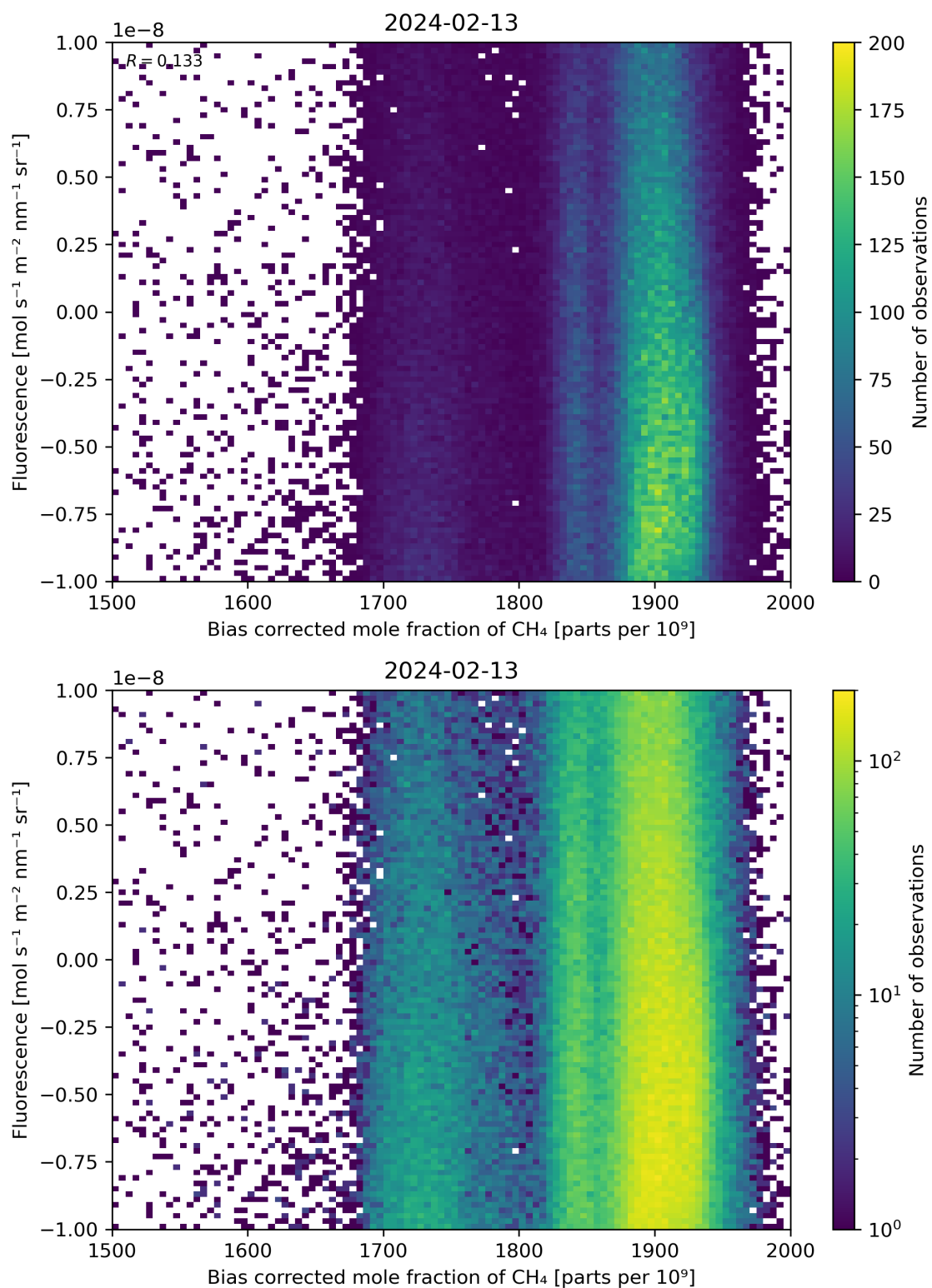
Figure 66: Scatter density plot of “Bias corrected mole fraction of \text{CH}_4 ” against “Fluorescence” for 2024-02-12 to 2024-02-14.
