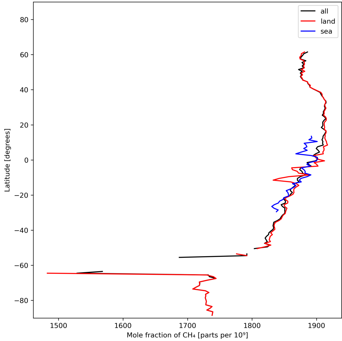
Figure 12: Zonal average of “Mole fraction of \text{CH}_4 ” for 2024-02-12 to 2024-02-14.
