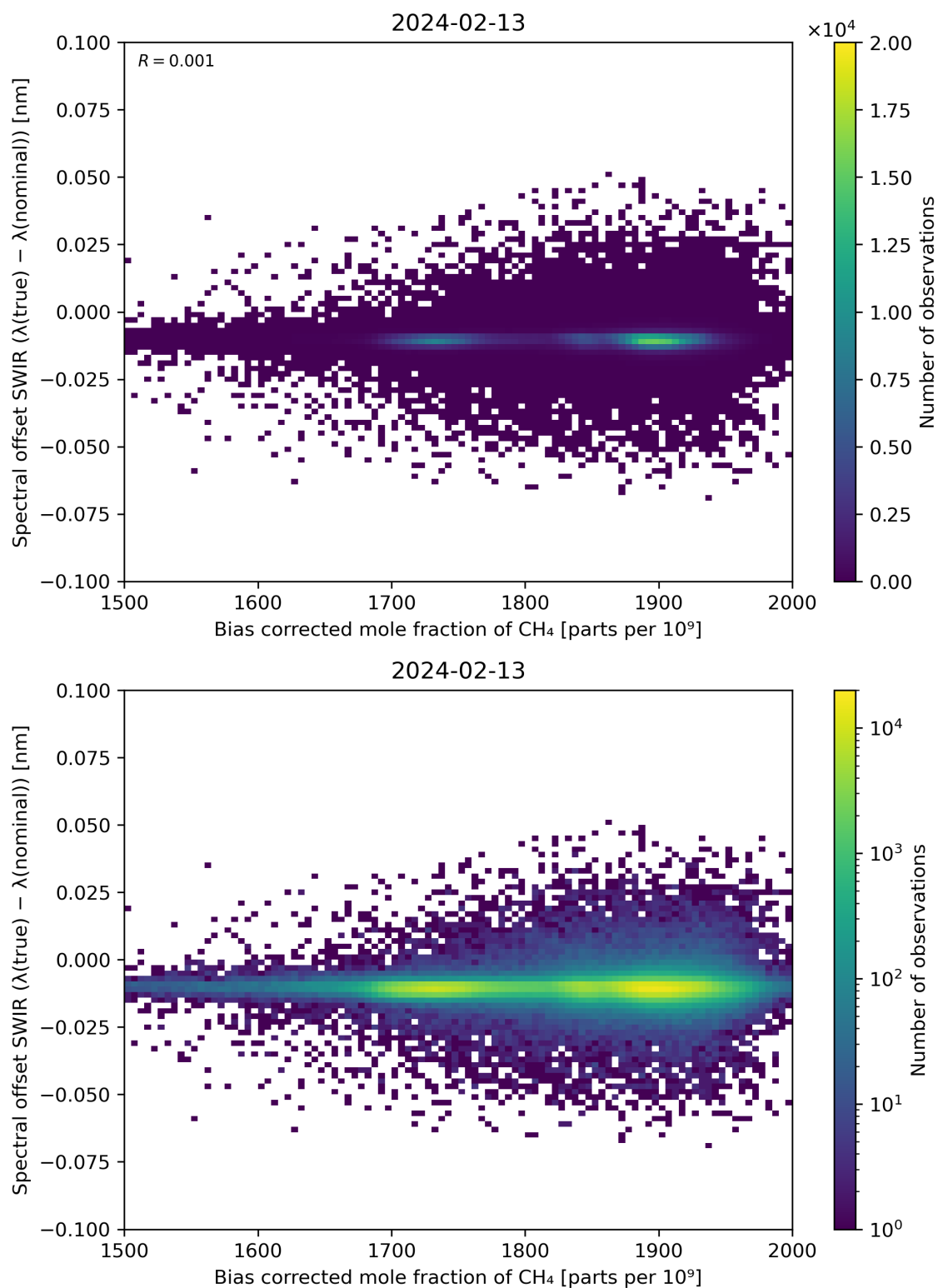
Figure 69: Scatter density plot of “Bias corrected mole fraction of \text{CH}_4 ” against “Spectral offset SWIR ( \lambda(\text{true}) - \lambda(\text{nominal}) )” for 2024-02-12 to 2024-02-14.
