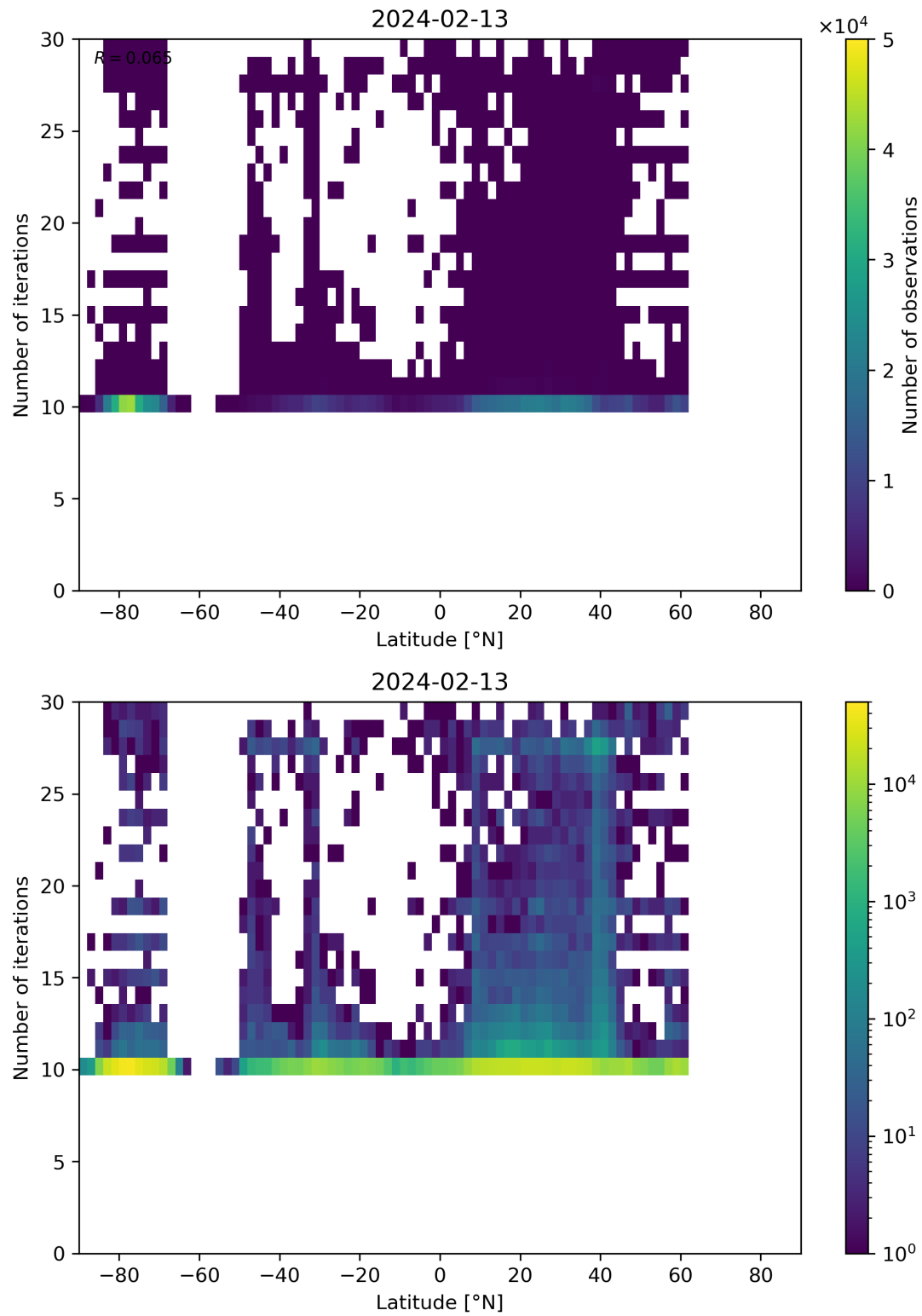
Figure 60: Scatter density plot of “Latitude” against “Number of iterations” for 2024-02-12 to 2024-02-14.
