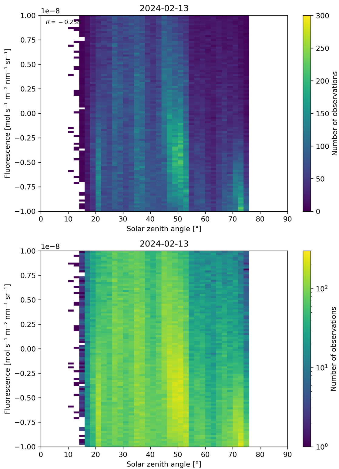
Figure 97: Scatter density plot of “Solar zenith angle” against “Fluorescence” for 2024-02-12 to 2024-02-14.
