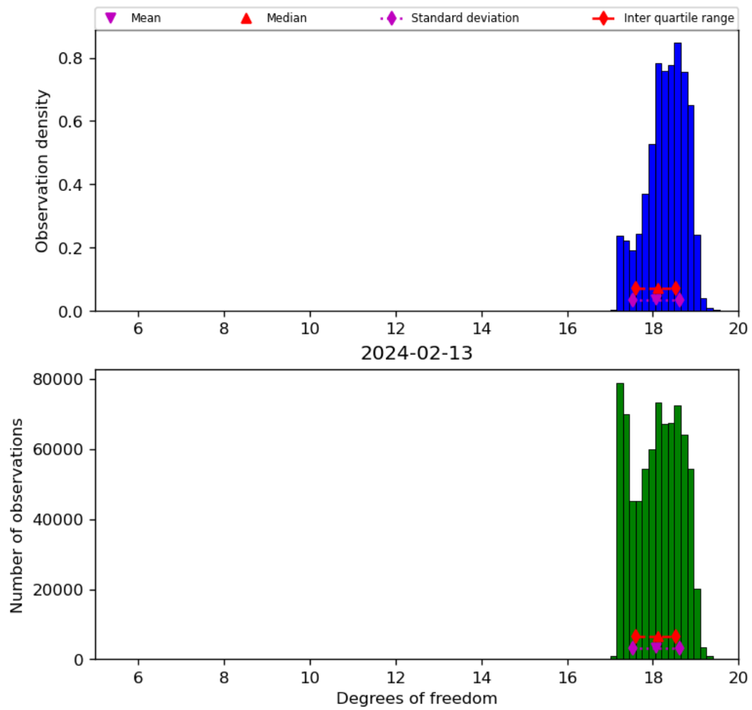
Figure 30: Histogram of “Degrees of freedom” for 2024-02-12 to 2024-02-14
