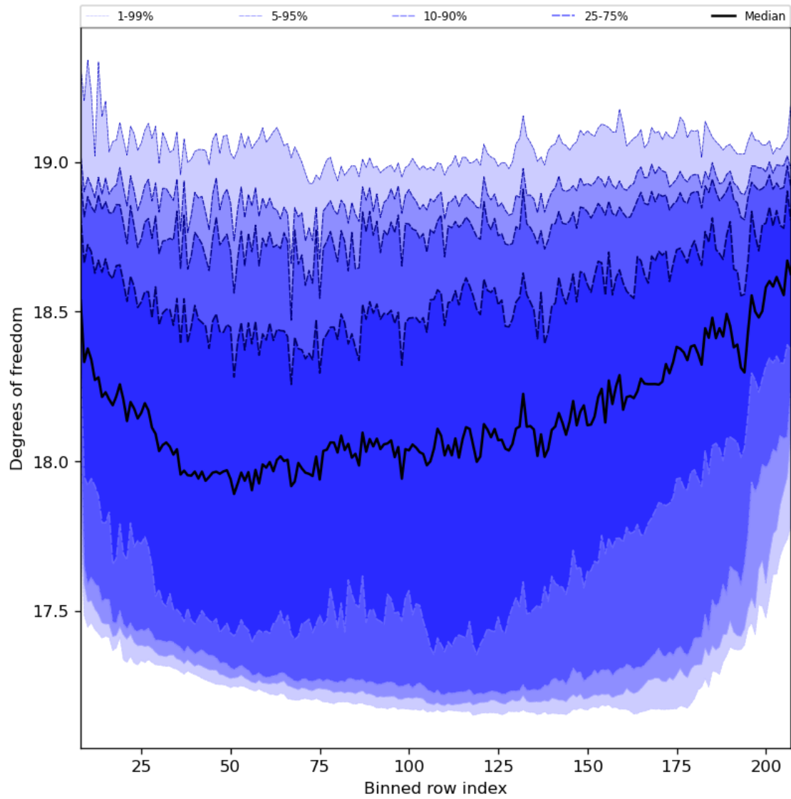
Figure 41: Along track statistics of “Degrees of freedom” for 2024-02-12 to 2024-02-14
