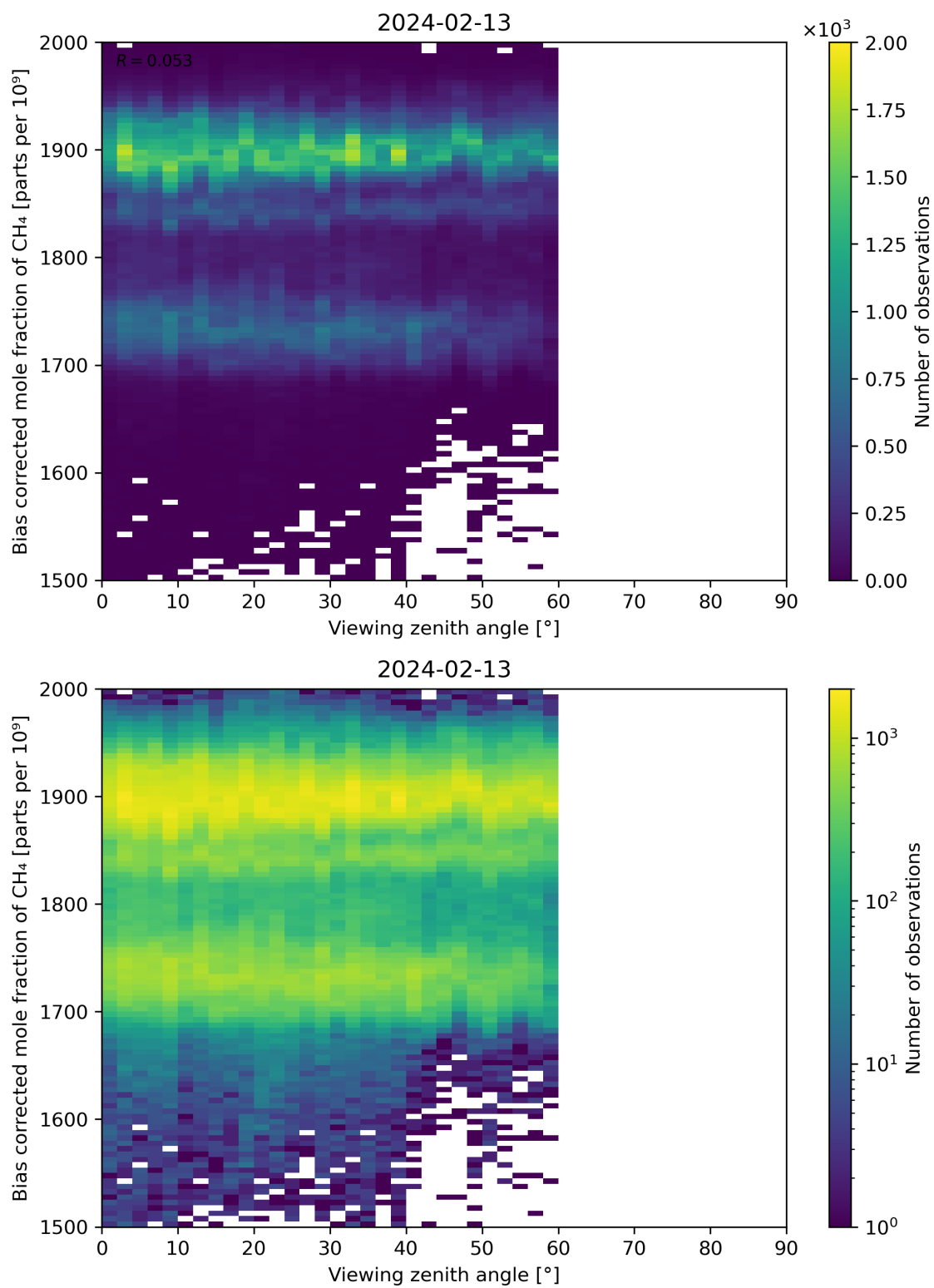
Figure 111: Scatter density plot of “Viewing zenith angle” against “Bias corrected mole fraction of CH 4 ” for 2024-02-12 to 2024-02-14.
