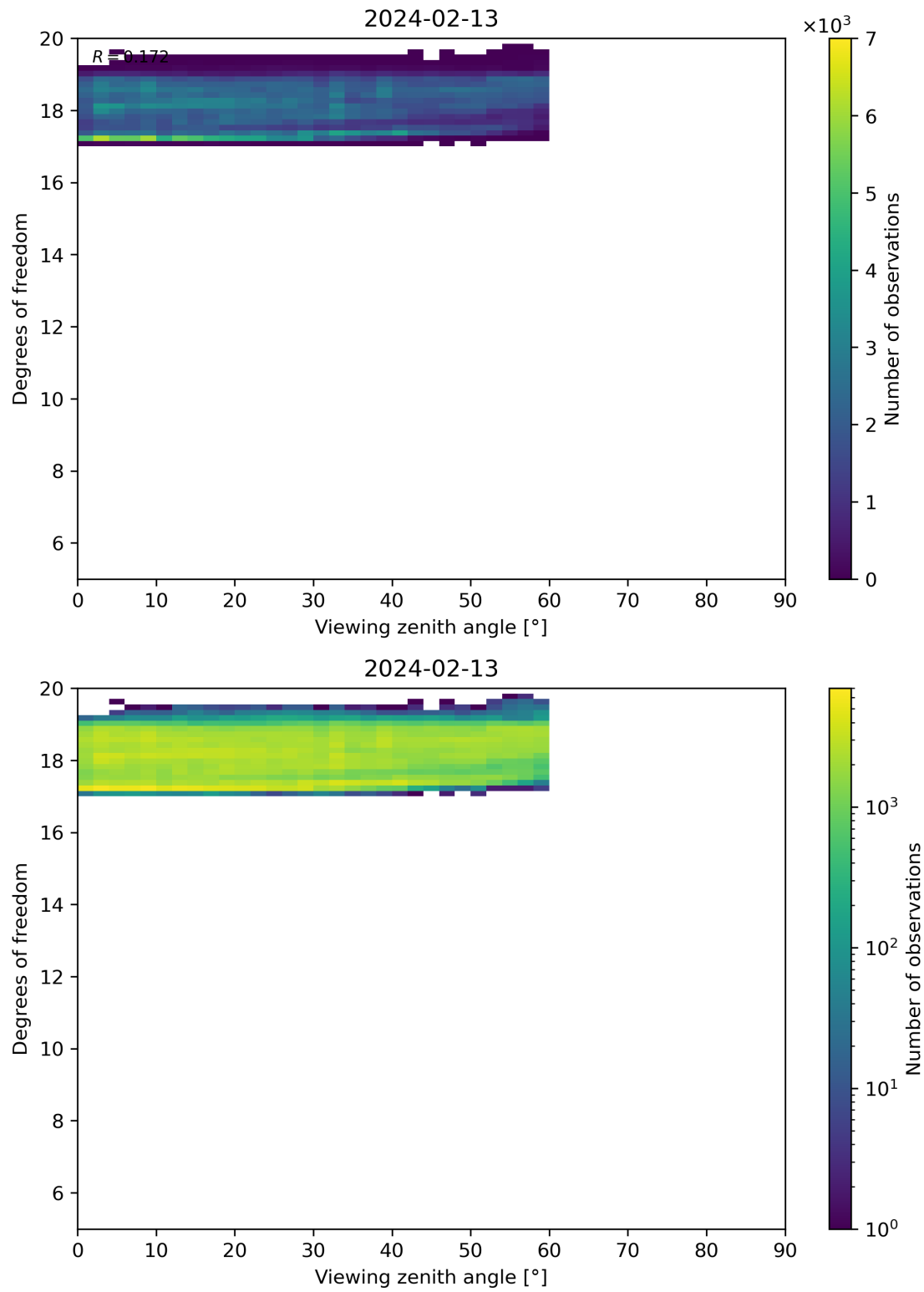
Figure 107: Scatter density plot of “Viewing zenith angle” against “Degrees of freedom” for 2024-02-12 to 2024-02-14.
