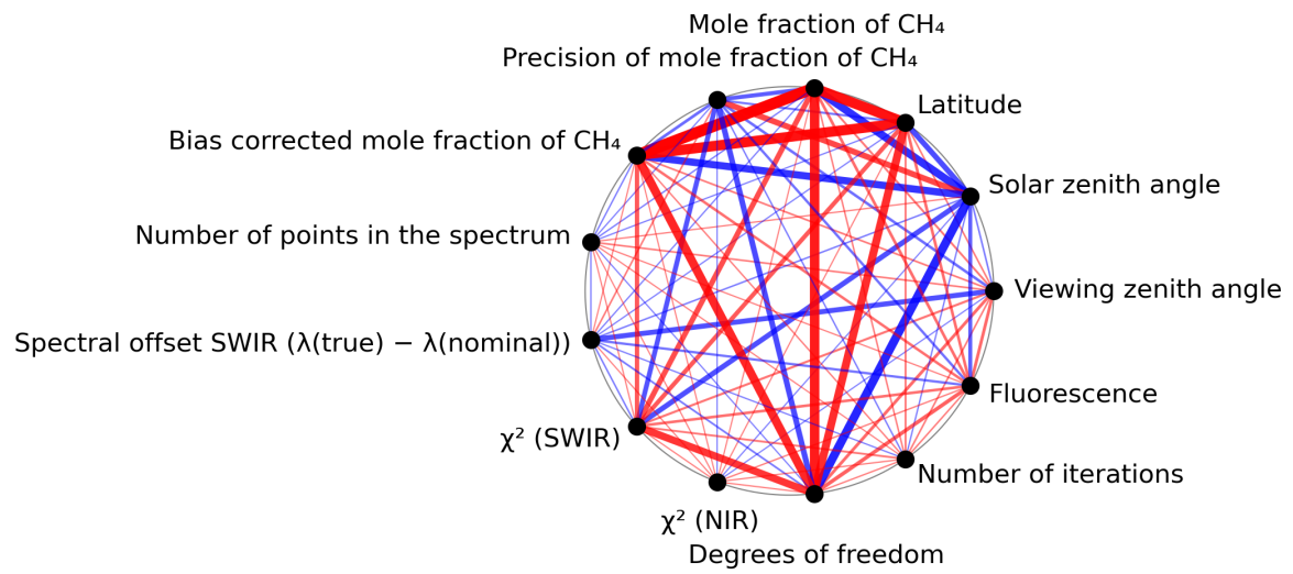
Figure 1: Map of correlation graph for 2024-02-12 to 2024-02-14.
