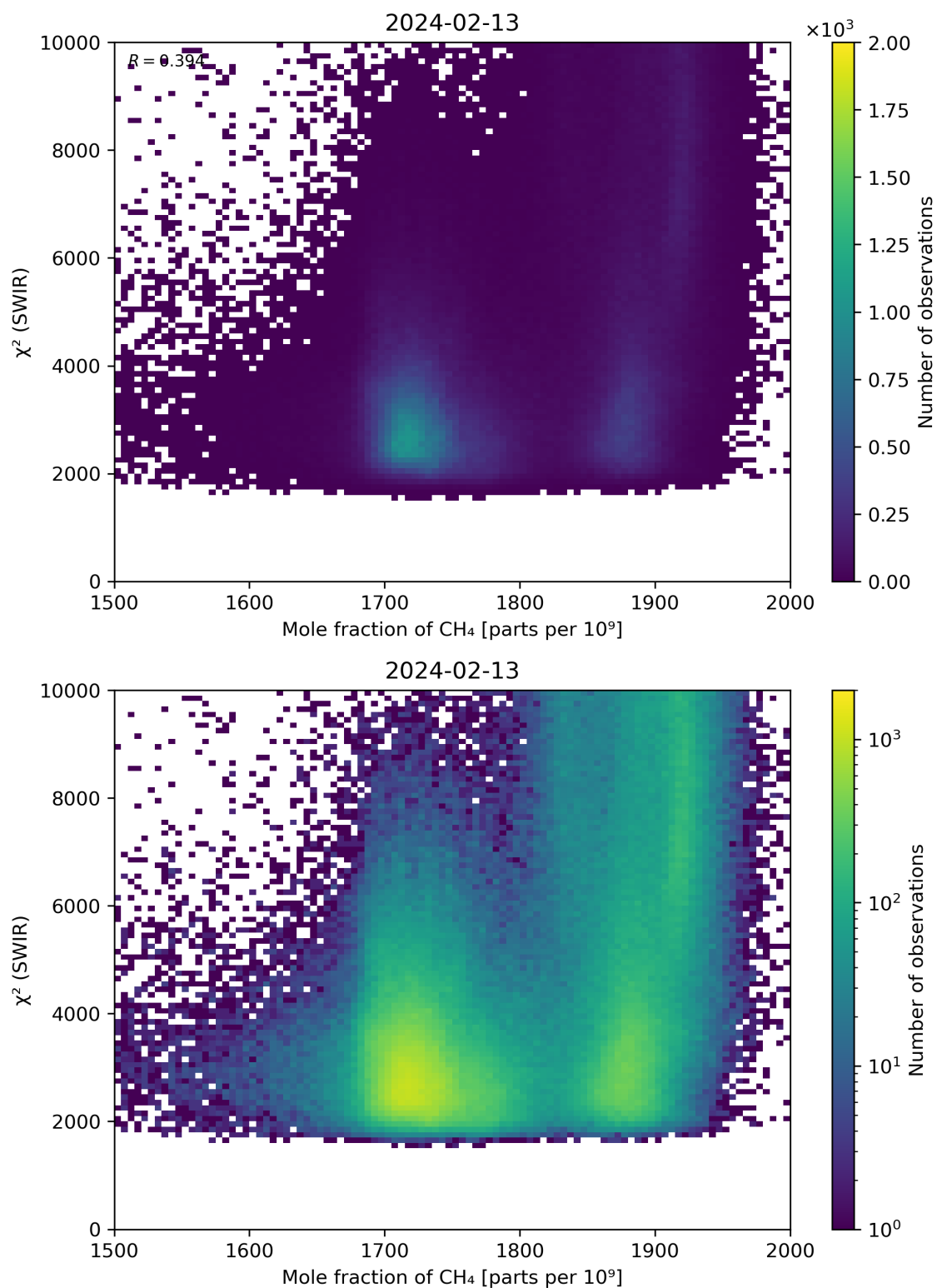
Figure 71: Scatter density plot of “Mole fraction of \text{CH}_4 ” against “ \chi^2 (SWIR)” for 2024-02-12 to 2024-02-14.
