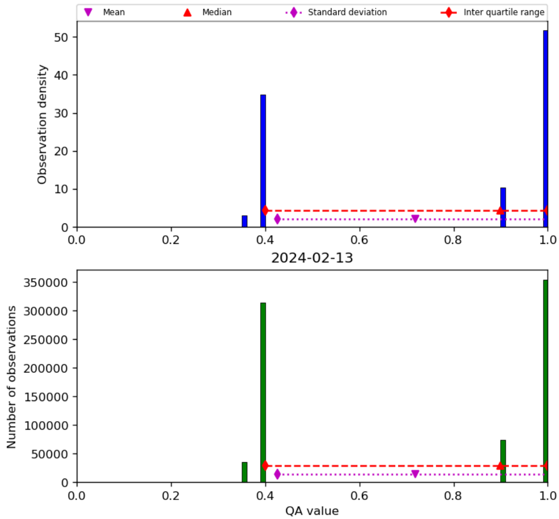
Figure 22: Histogram of “QA value” for 2024-02-12 to 2024-02-14
