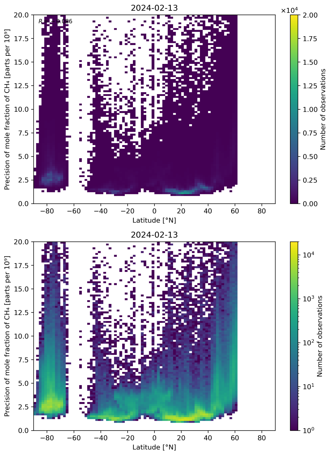
Figure 59: Scatter density plot of “Latitude” against “Precision of mole fraction of CH 4 ” for 2024-02-12 to 2024-02-14.
