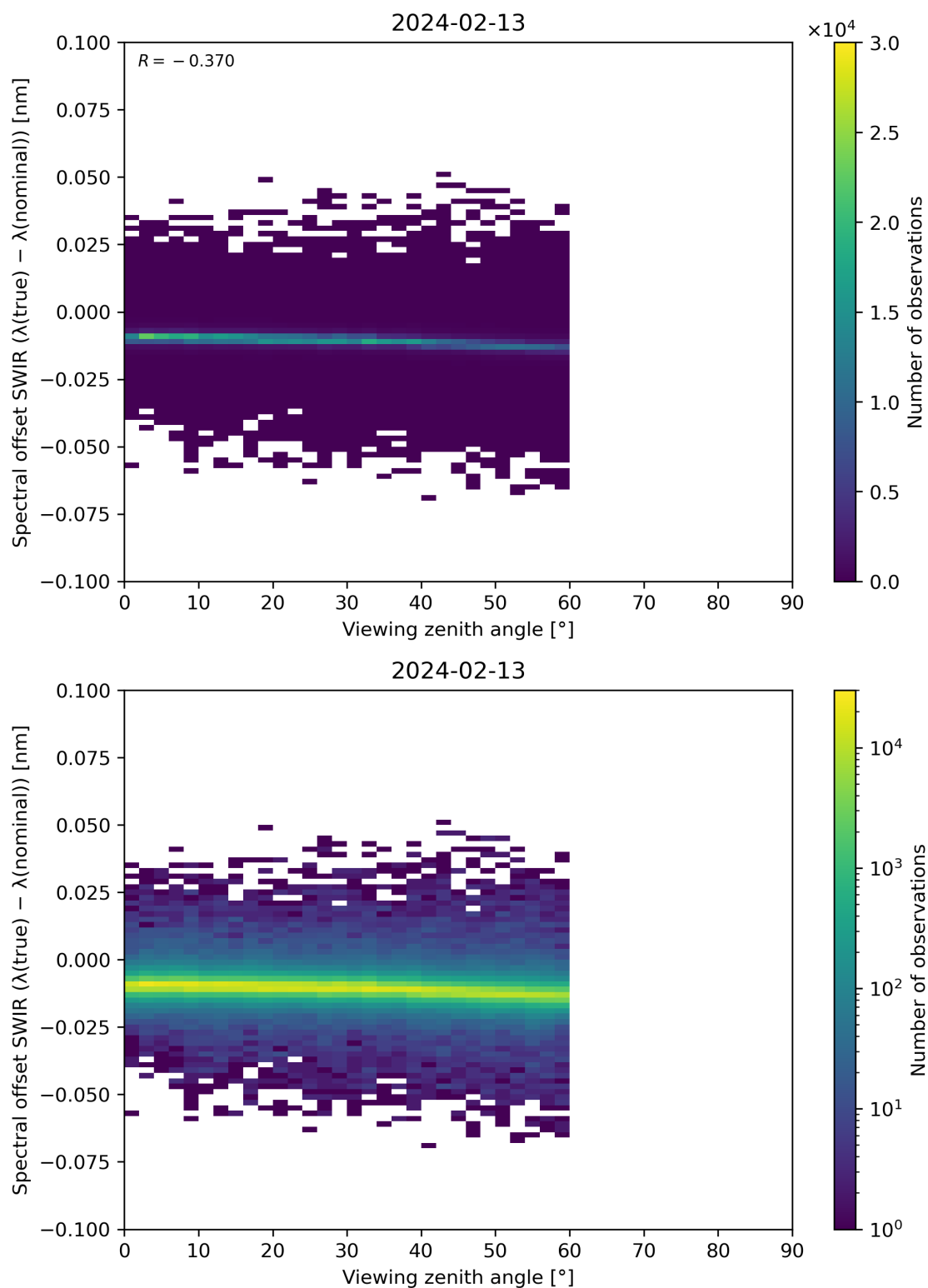
Figure 116: Scatter density plot of “Viewing zenith angle” against “Spectral offset SWIR ( \lambda(\text{true}) - \lambda(\text{nominal}) )” for 2024-02-12 to 2024-02-14.
