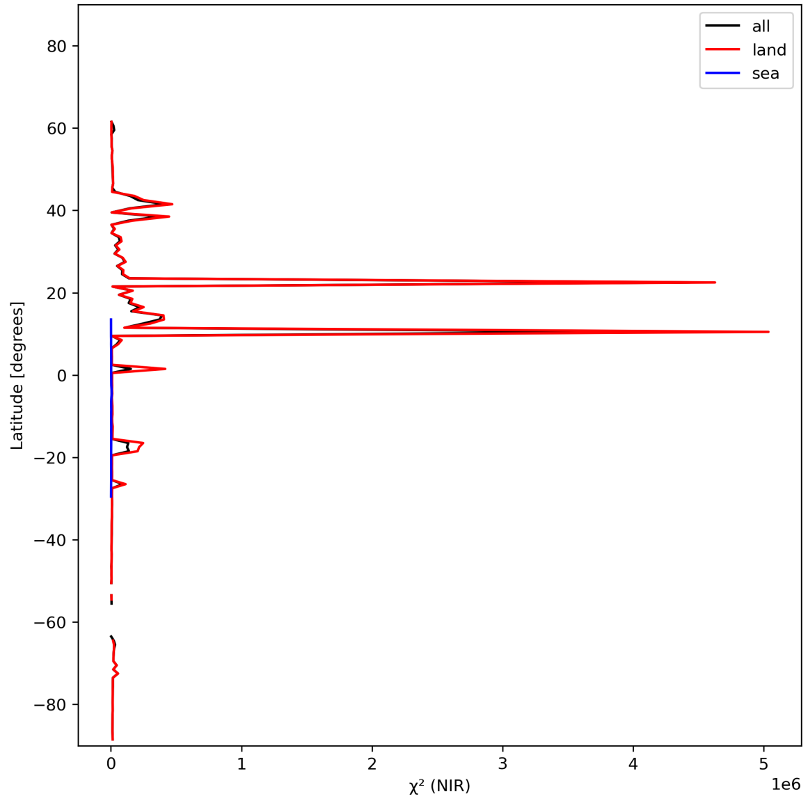
Figure 18: Zonal average of “ \chi^2 (NIR)” for 2024-02-12 to 2024-02-14.
