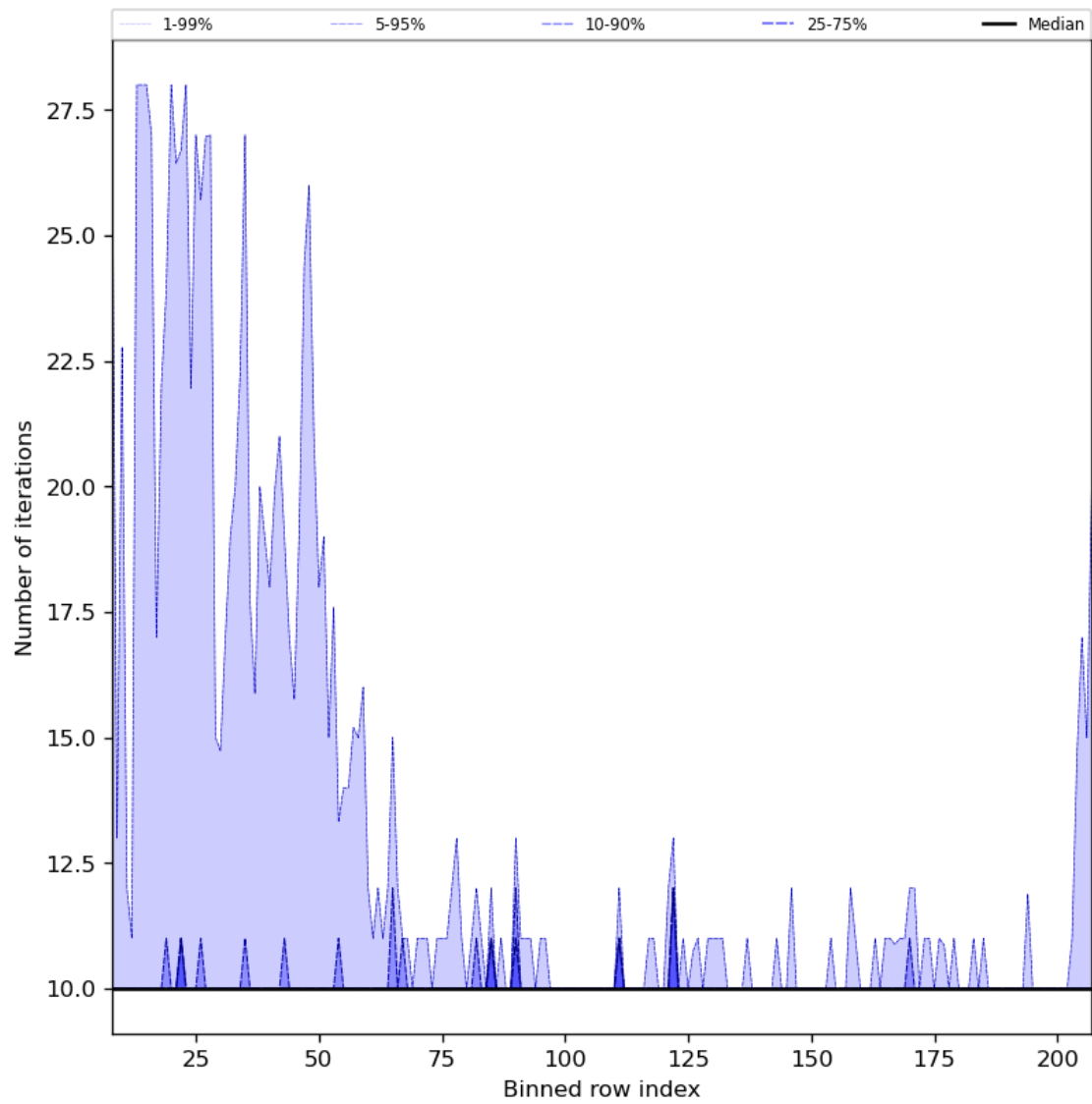
Figure 42: Along track statistics of “Number of iterations” for 2024-02-12 to 2024-02-14
