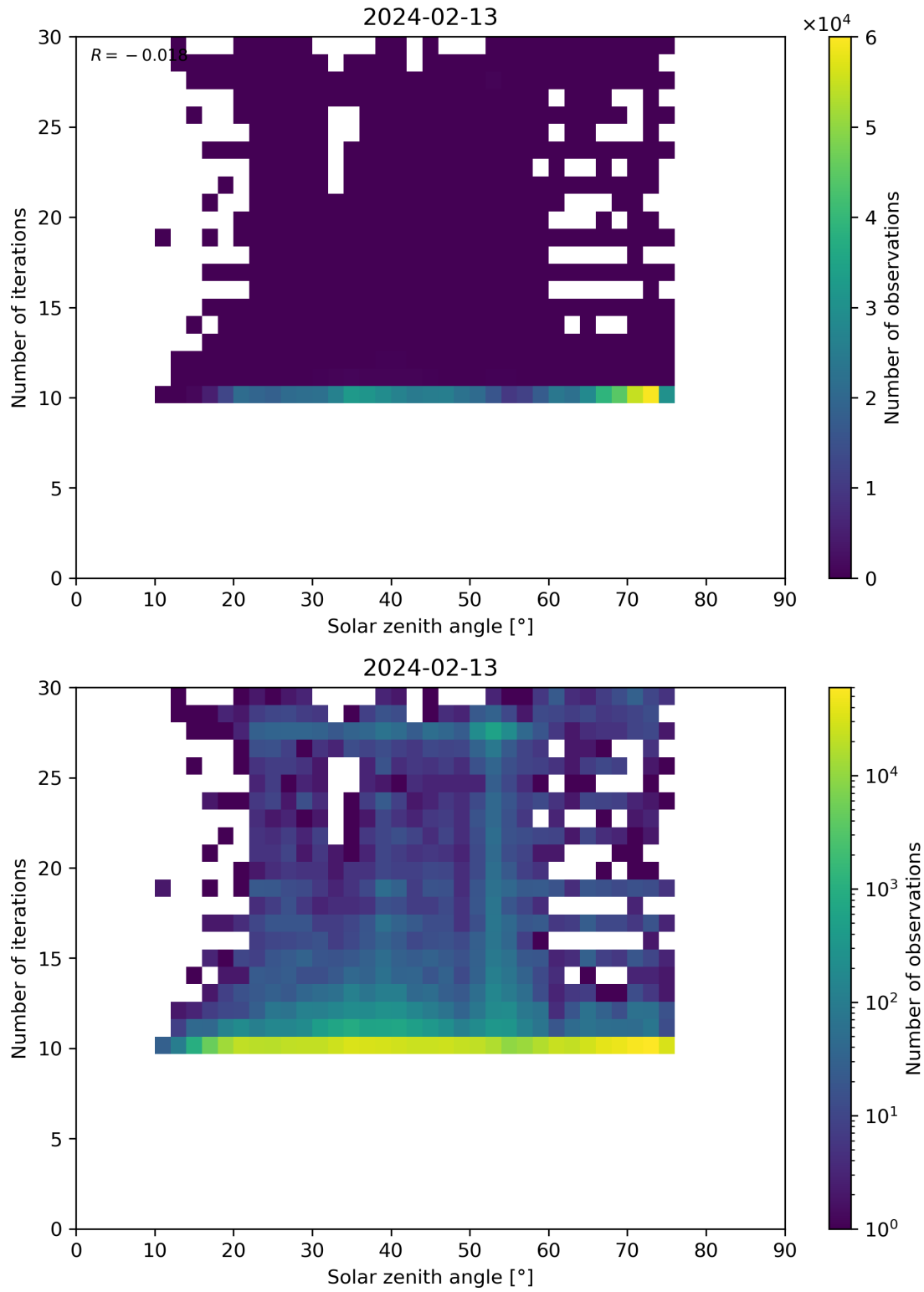
Figure 102: Scatter density plot of “Solar zenith angle” against “Number of iterations” for 2024-02-12 to 2024-02-14.
