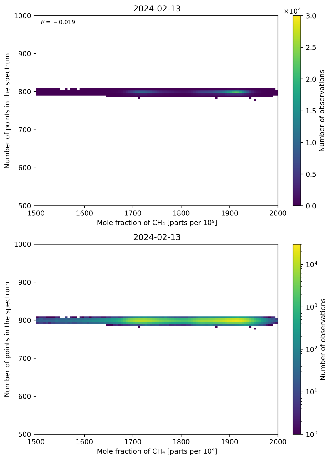
Figure 77: Scatter density plot of “Mole fraction of CH 4 ” against “Number of points in the spectrum” for 2024-02-12 to 2024-02-14.
