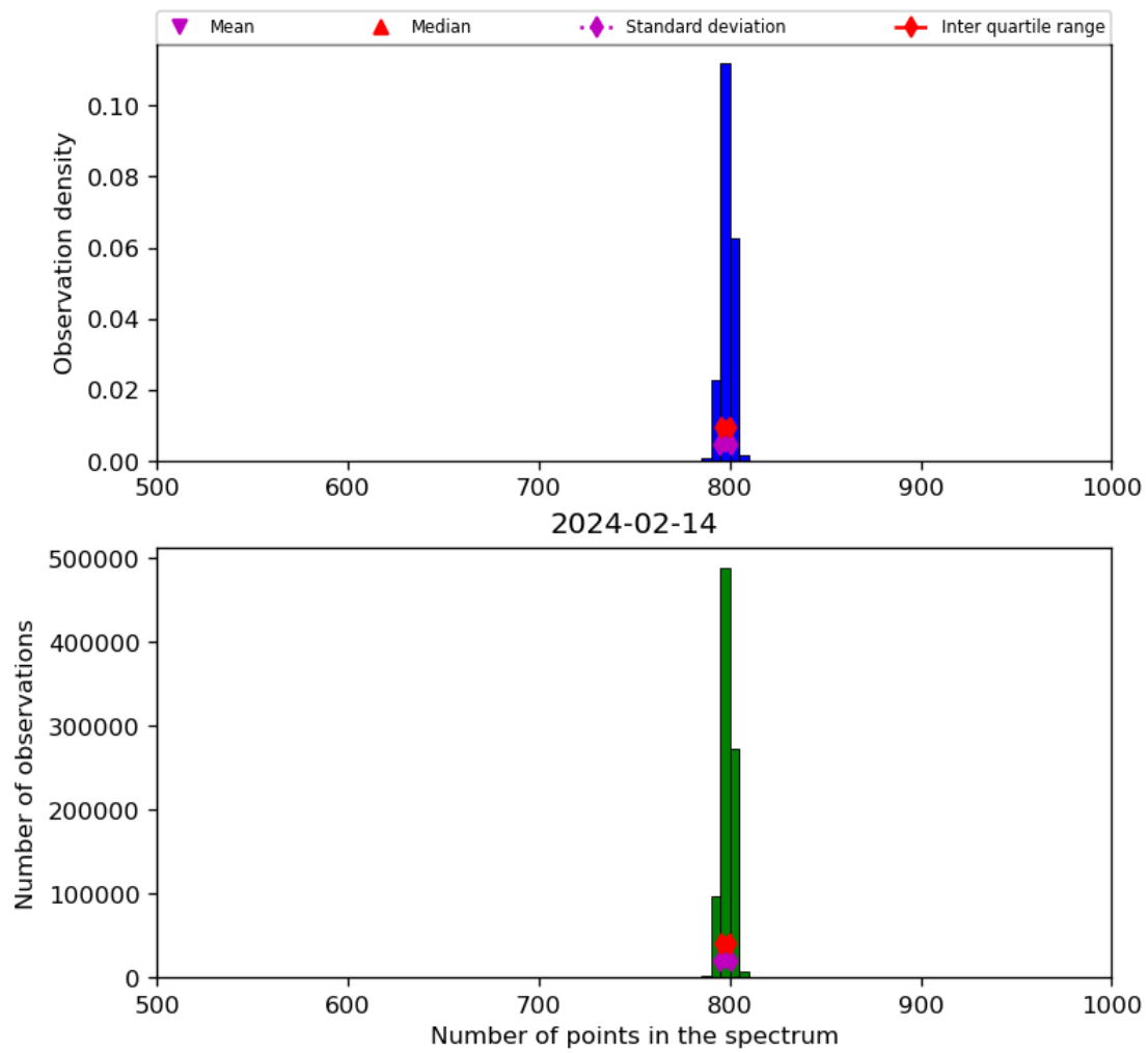
Figure 26: Histogram of “Number of points in the spectrum” for 2024-02-13 to 2024-02-15
