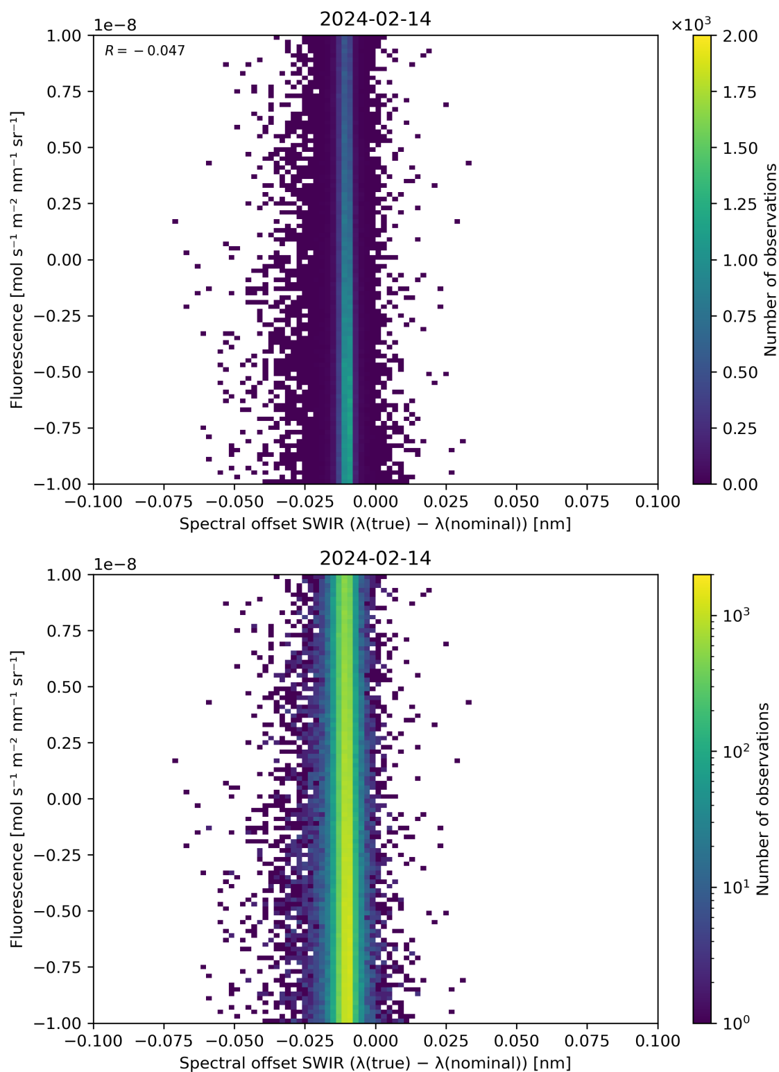
Figure 120: Scatter density plot of “Spectral offset SWIR ( \lambda(\text{true}) - \lambda(\text{nominal}) )” against “Fluorescence” for 2024-02-13 to 2024-02-15.
