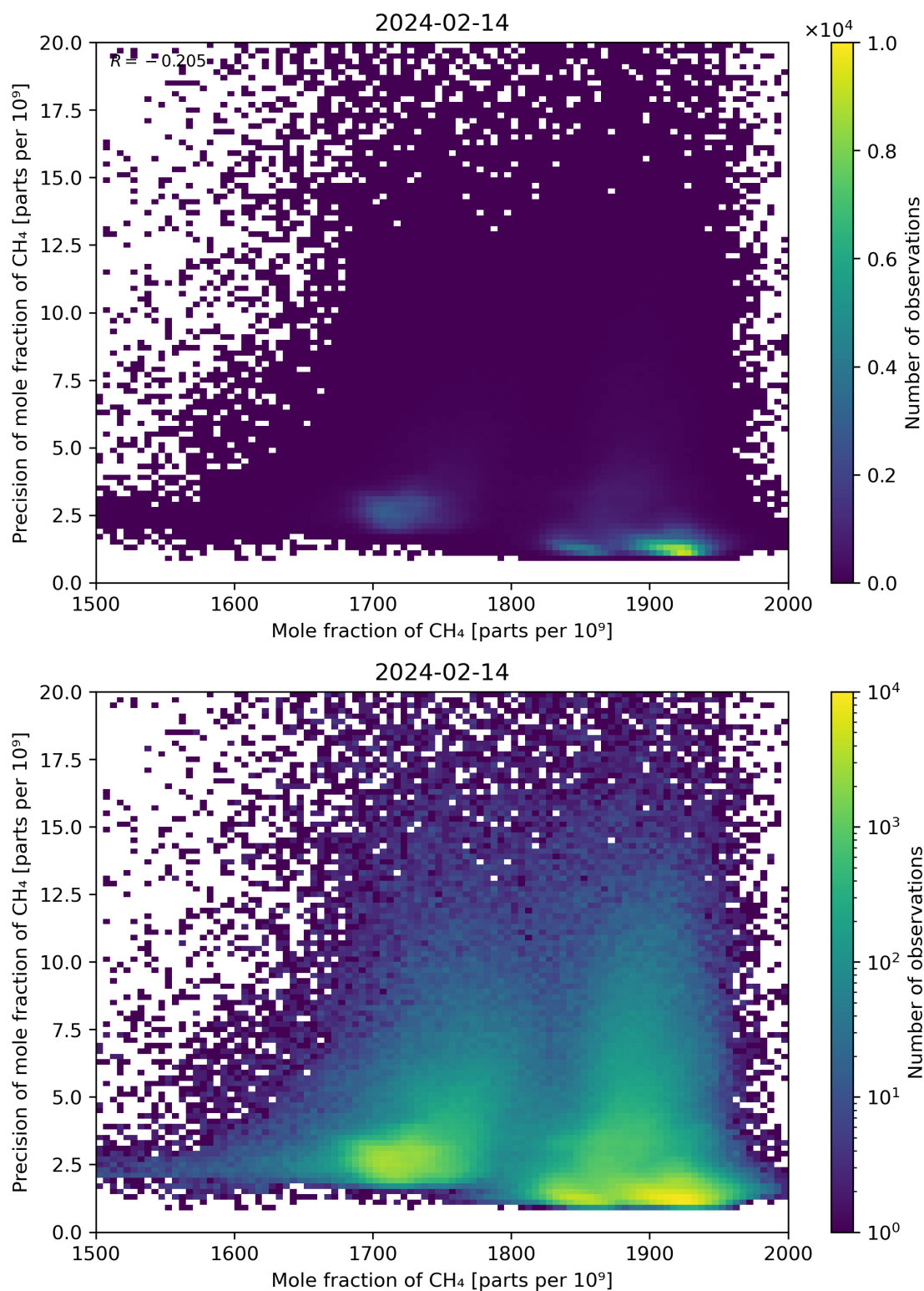
Figure 75: Scatter density plot of “Mole fraction of CH 4 ” against “Precision of mole fraction of CH 4 ” for 2024-02-13 to 2024-02-15.
