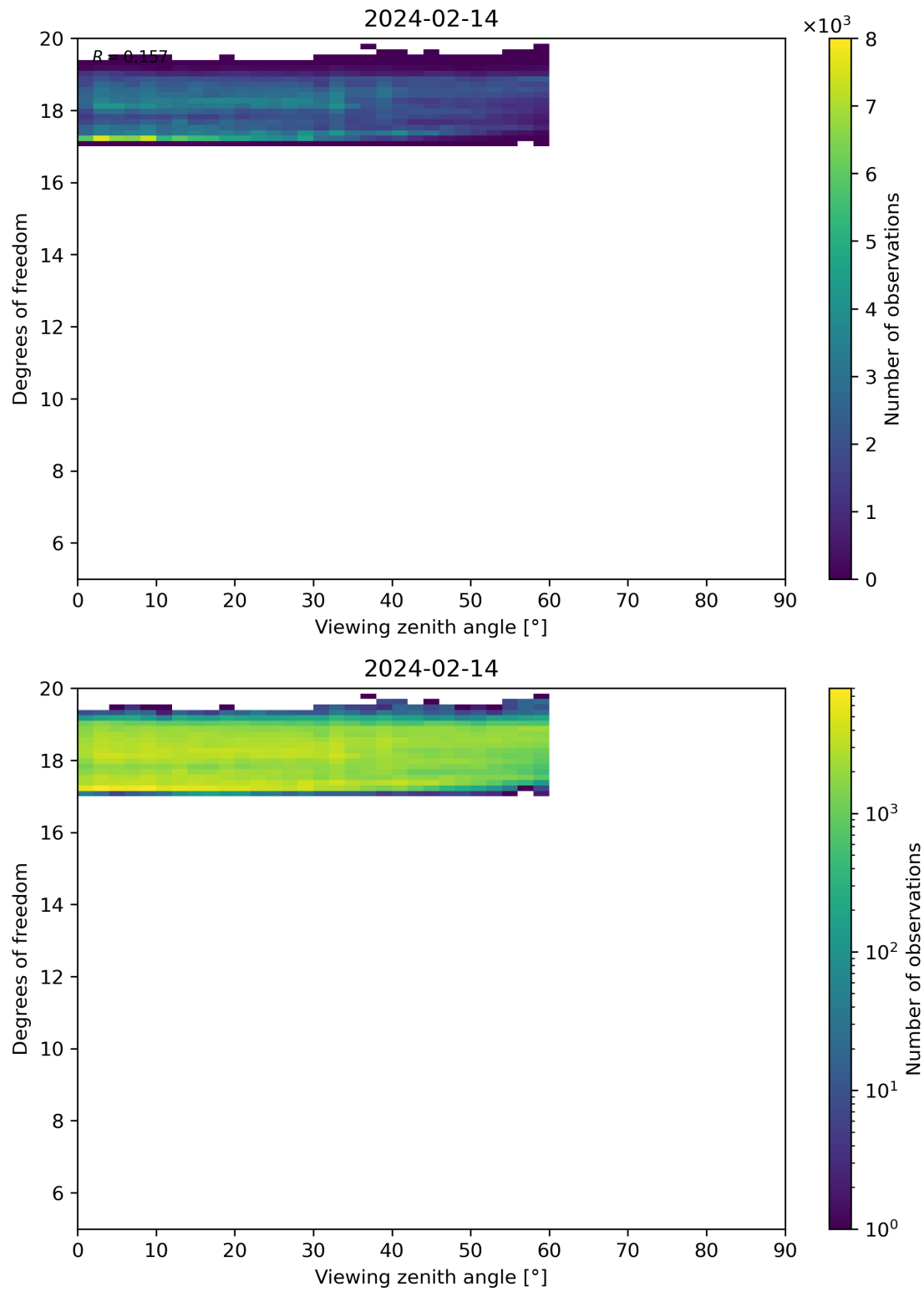
Figure 107: Scatter density plot of “Viewing zenith angle” against “Degrees of freedom” for 2024-02-13 to 2024-02-15.
