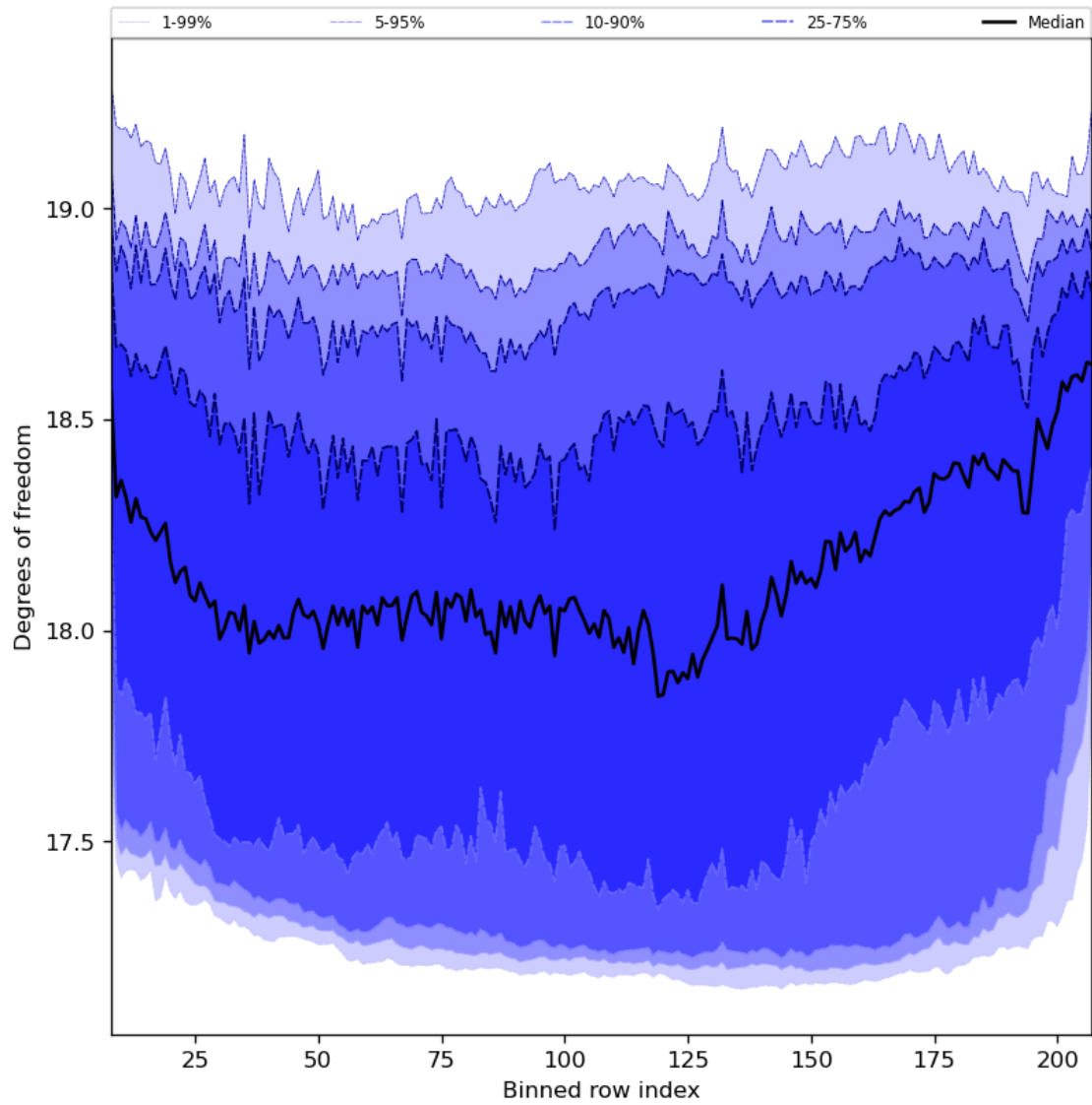
Figure 41: Along track statistics of “Degrees of freedom” for 2024-02-13 to 2024-02-15
