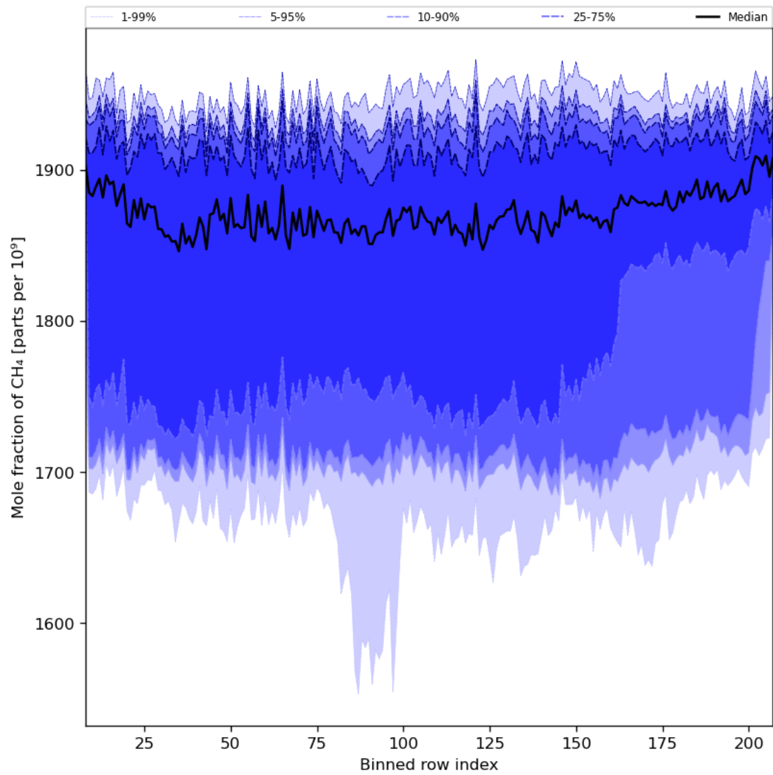
Figure 34: Along track statistics of “Mole fraction of CH 4 ” for 2024-02-13 to 2024-02-15
