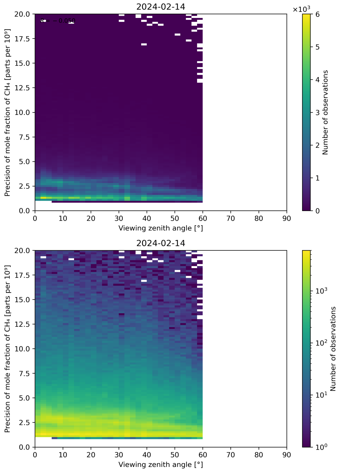
Figure 112: Scatter density plot of “Viewing zenith angle” against “Precision of mole fraction of CH 4 ” for 2024-02-13 to 2024-02-15.
