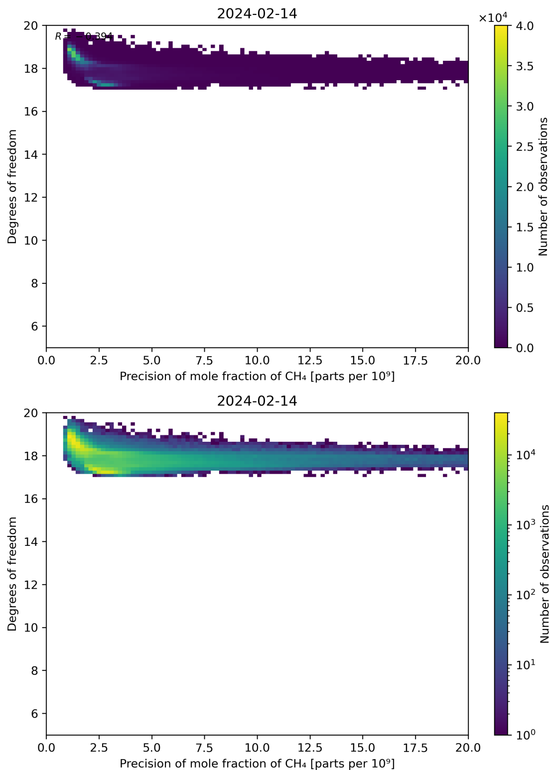
Figure 80: Scatter density plot of “Precision of mole fraction of CH 4 ” against “Degrees of freedom” for 2024-02-13 to 2024-02-15.
