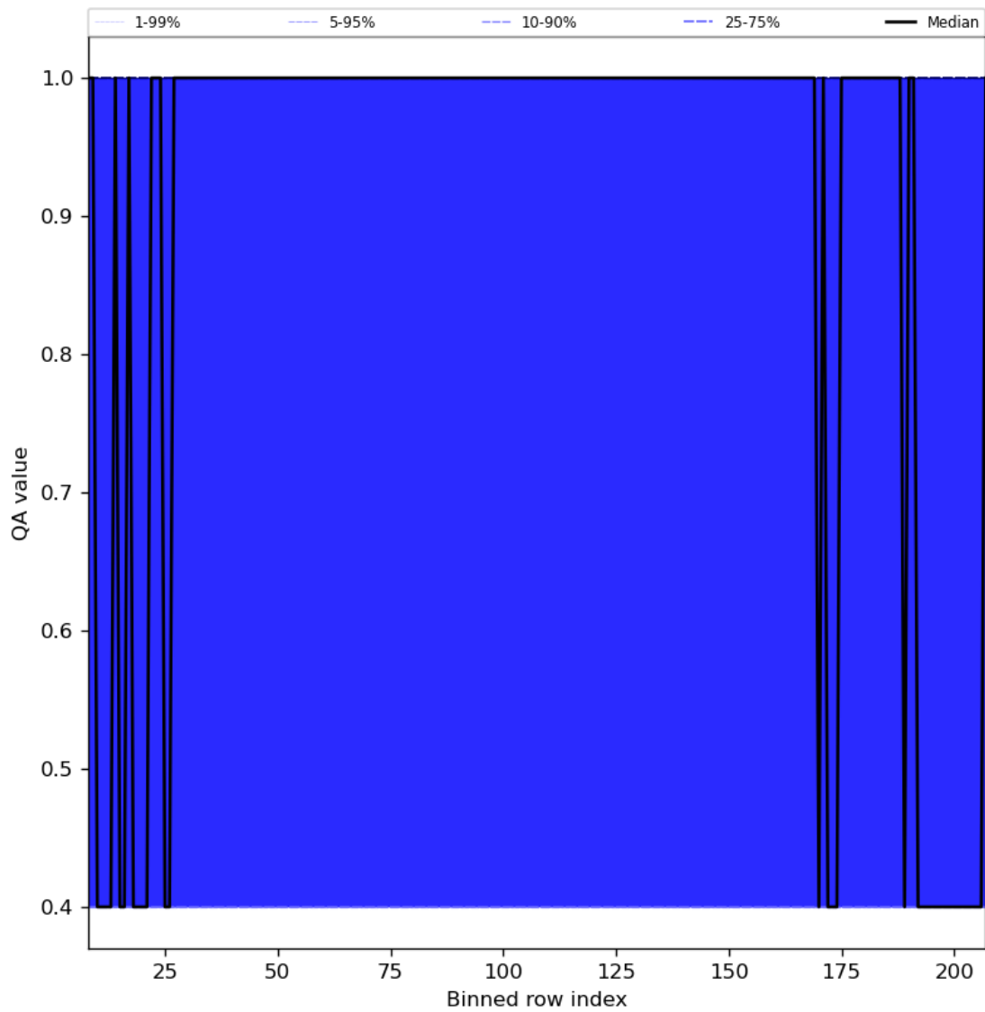
Figure 33: Along track statistics of “QA value” for 2024-02-13 to 2024-02-15
