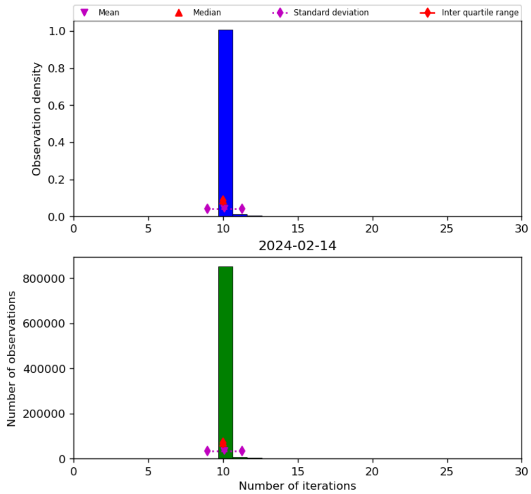
Figure 31: Histogram of “Number of iterations” for 2024-02-13 to 2024-02-15
