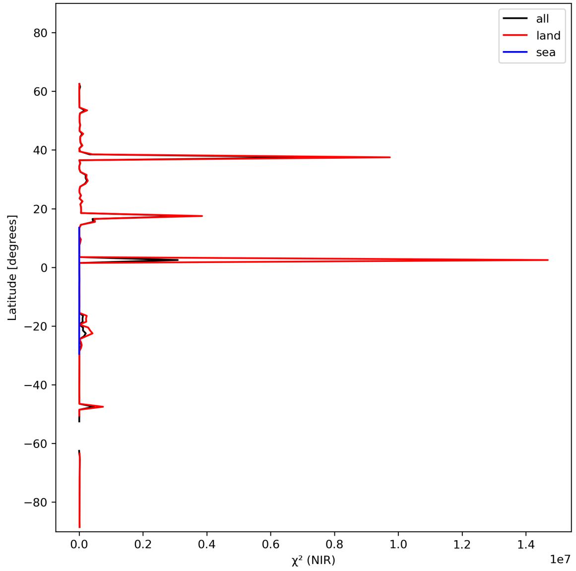
Figure 18: Zonal average of “ \chi^2 (NIR)” for 2024-02-13 to 2024-02-15.
