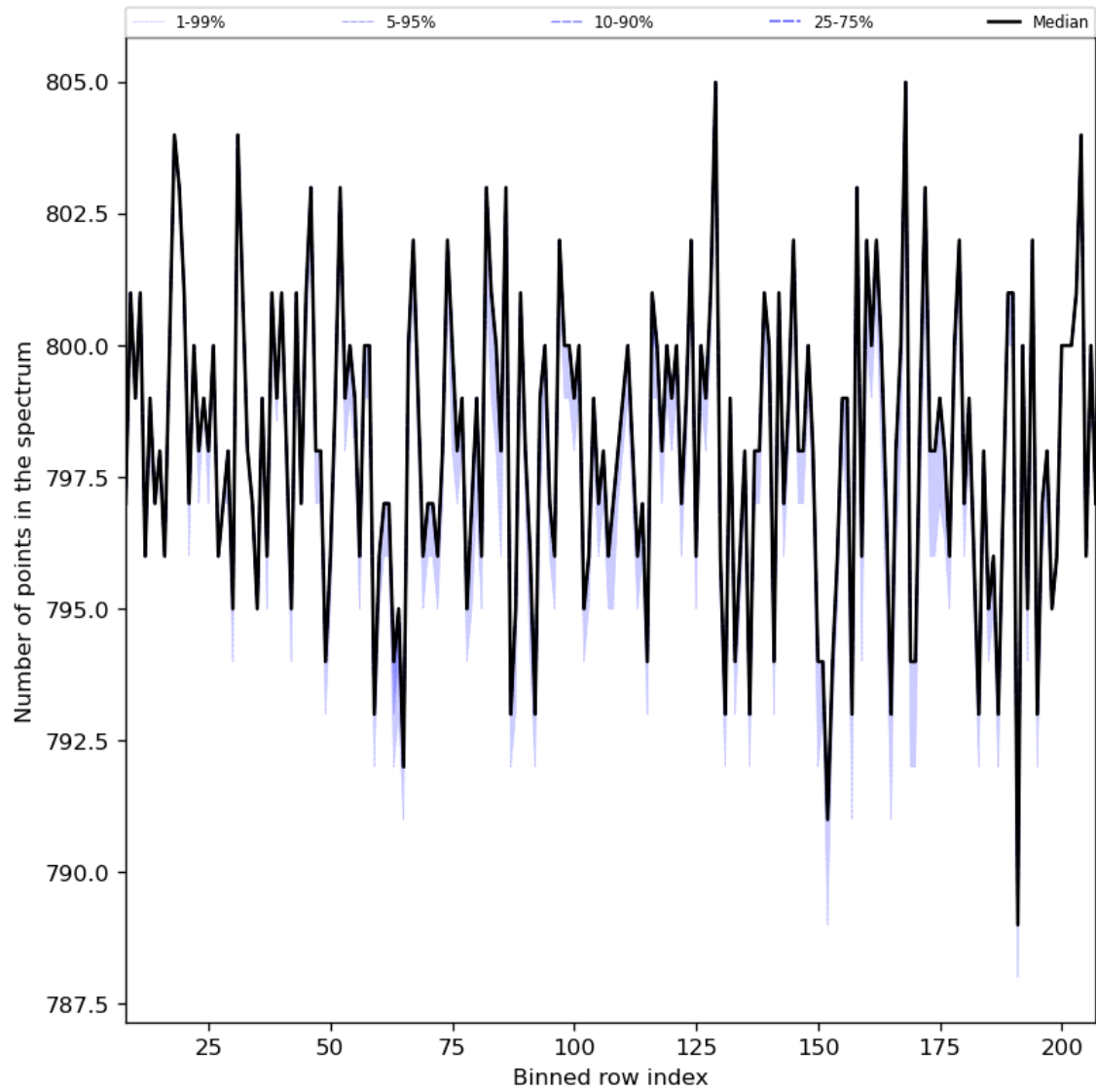
Figure 37: Along track statistics of “Number of points in the spectrum” for 2024-02-13 to 2024-02-15
