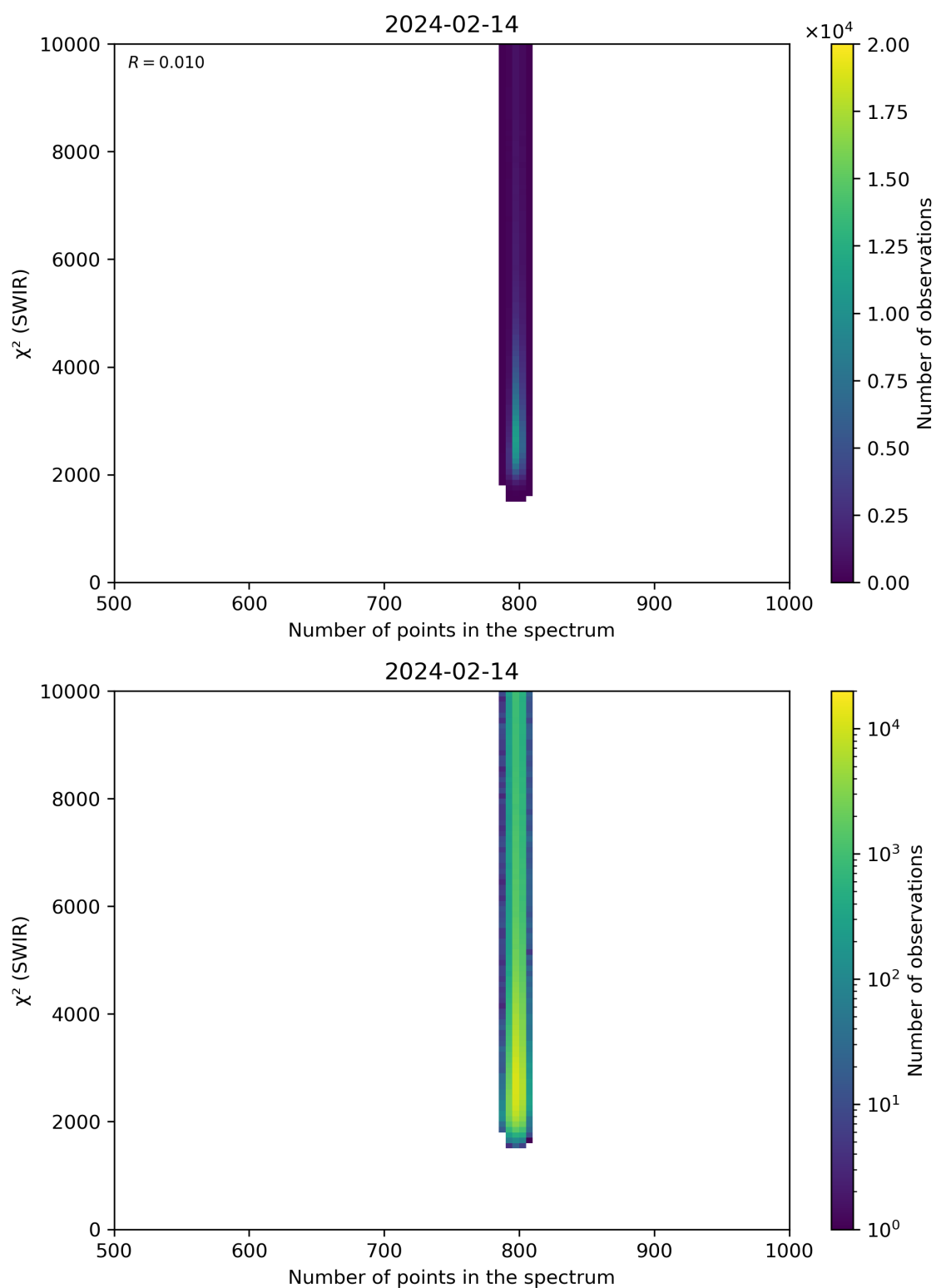
Figure 89: Scatter density plot of “Number of points in the spectrum” against “ \chi^2 (SWIR)” for 2024-02-13 to 2024-02-15.
