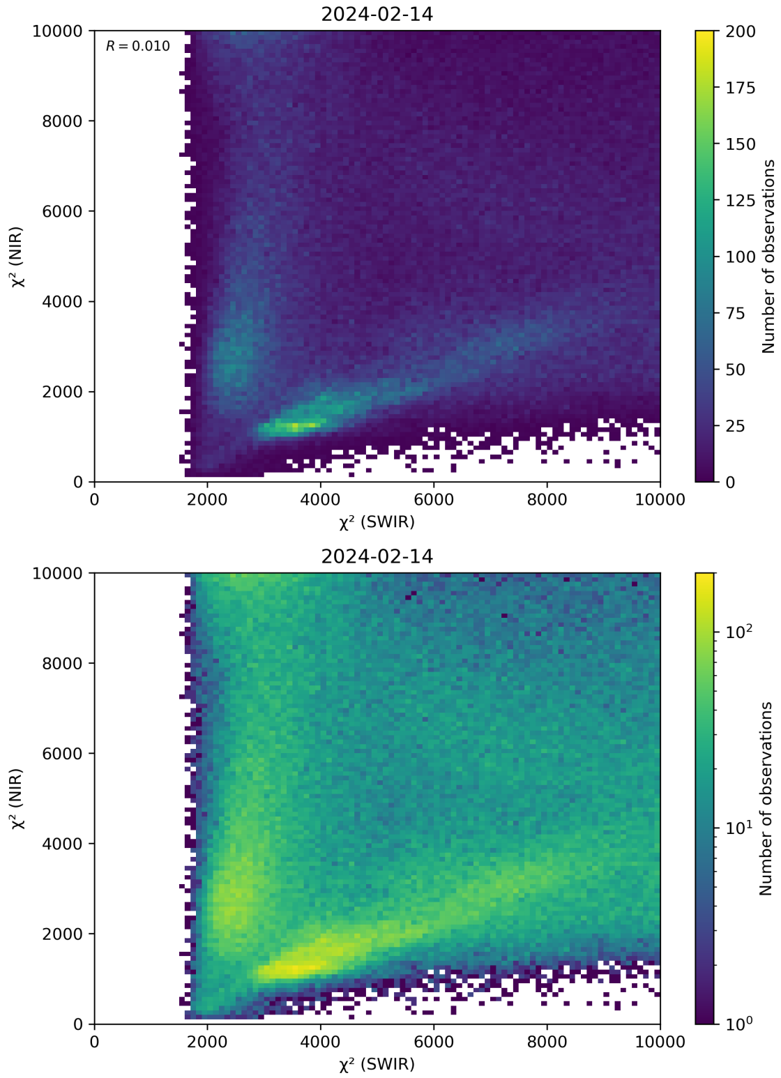
Figure 47: Scatter density plot of “ \chi^2 (SWIR)” against “ \chi^2 (NIR)” for 2024-02-13 to 2024-02-15.
