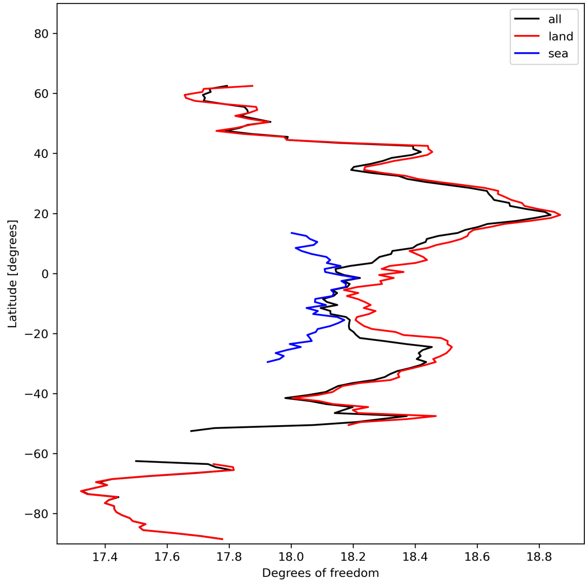
Figure 19: Zonal average of “Degrees of freedom” for 2024-02-13 to 2024-02-15.
