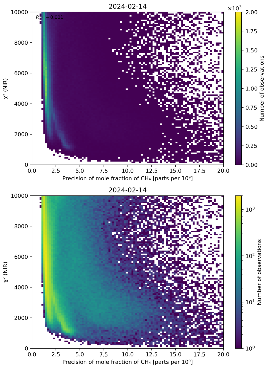
Figure 78: Scatter density plot of “Precision of mole fraction of \text{CH}_4 ” against “ \chi^2 (NIR)” for 2024-02-13 to 2024-02-15.
