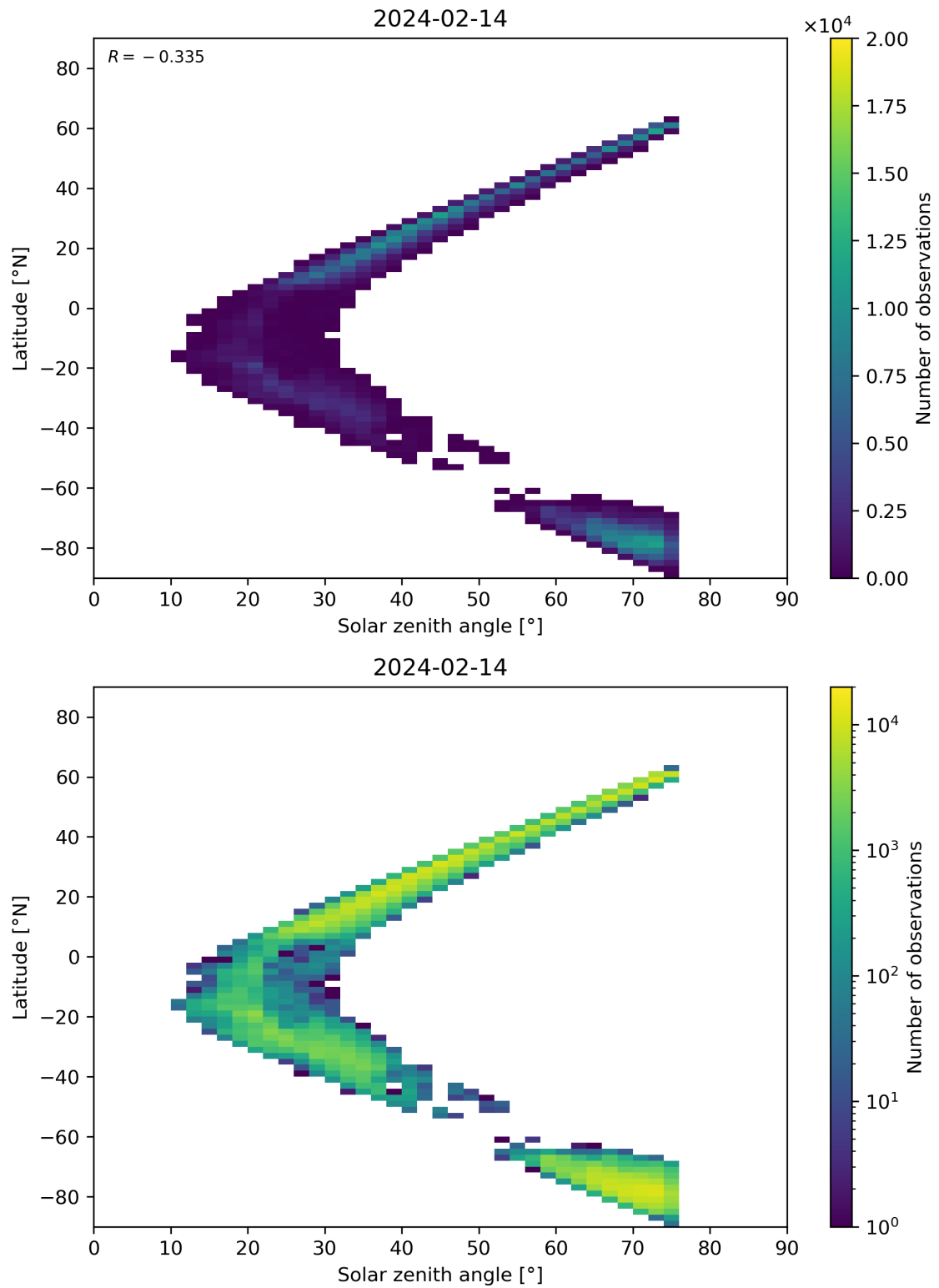
Figure 98: Scatter density plot of “Solar zenith angle” against “Latitude” for 2024-02-13 to 2024-02-15.
