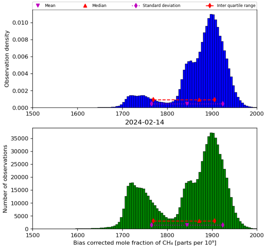
Figure 25: Histogram of “Bias corrected mole fraction of CH 4 ” for 2024-02-13 to 2024-02-15
