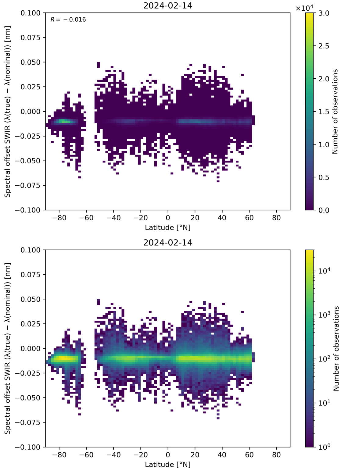
Figure 62: Scatter density plot of “Latitude” against “Spectral offset SWIR ( \lambda(\text{true}) - \lambda(\text{nominal}) )” for 2024-02-13 to 2024-02-15.
