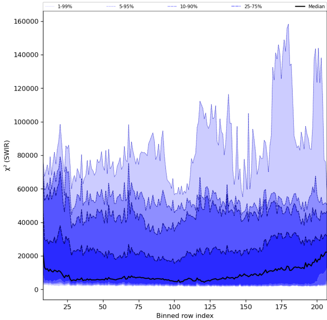
Figure 39: Along track statistics of " \chi^2 (SWIR)" for 2024-02-13 to 2024-02-15
