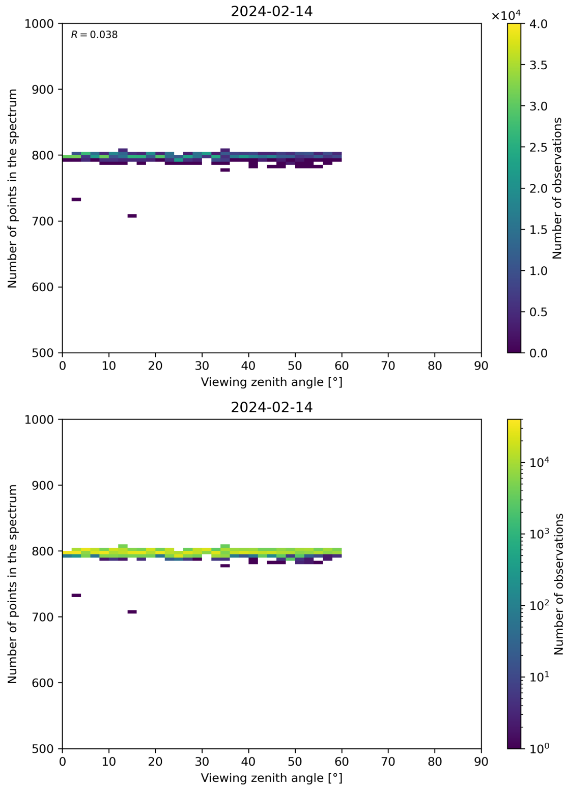
Figure 114: Scatter density plot of “Viewing zenith angle” against “Number of points in the spectrum” for 2024-02-13 to 2024-02-15.
