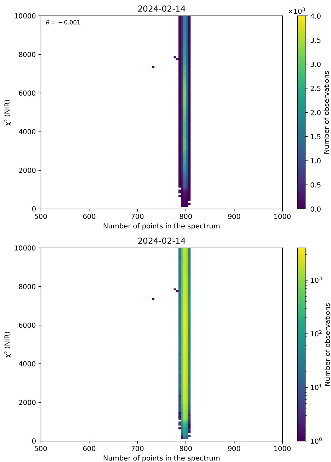
Figure 88: Scatter density plot of “Number of points in the spectrum” against “ \chi^2 (NIR)” for 2024-02-13 to 2024-02-15.
