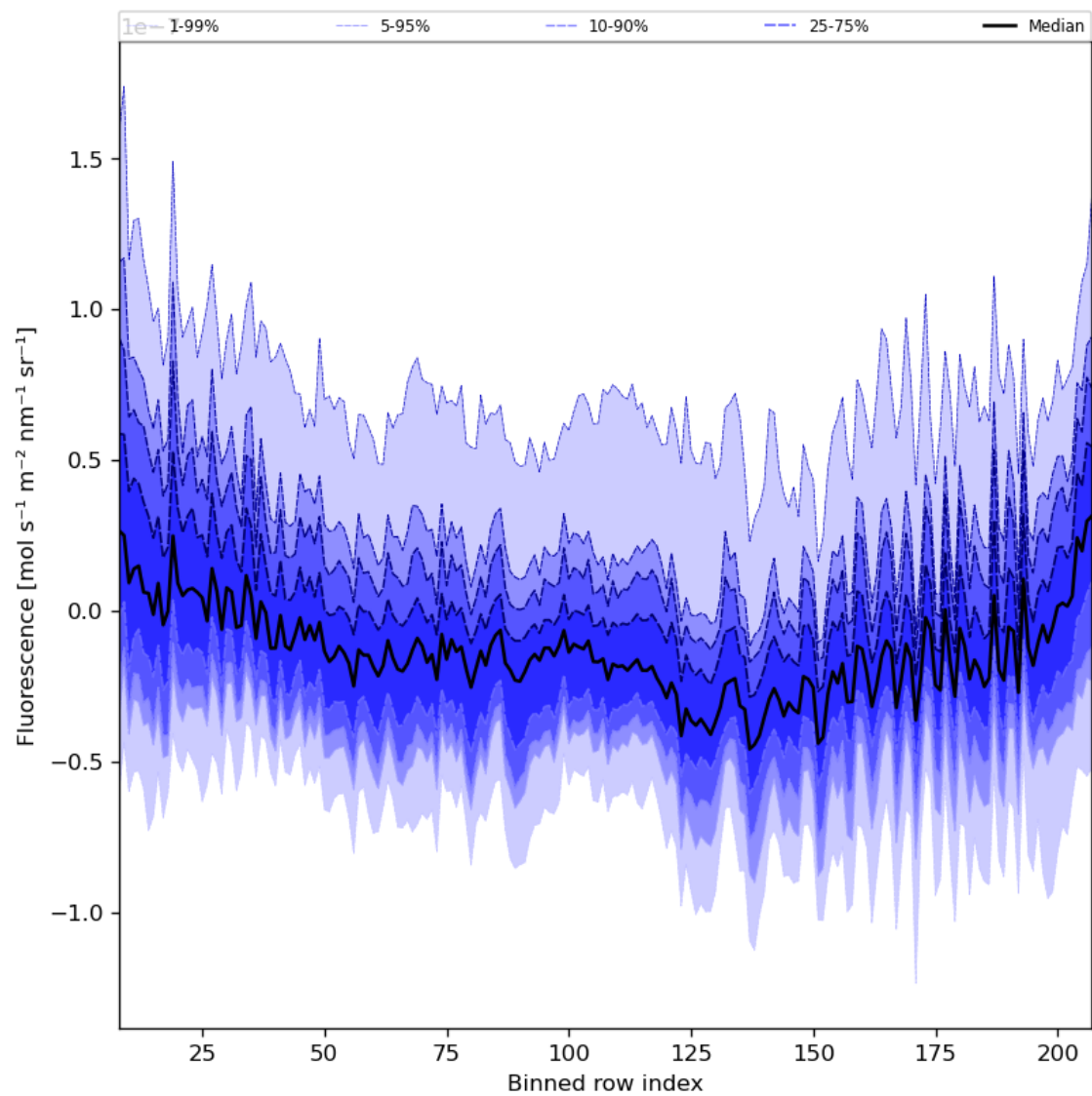
Figure 43: Along track statistics of “Fluorescence” for 2024-02-13 to 2024-02-15
