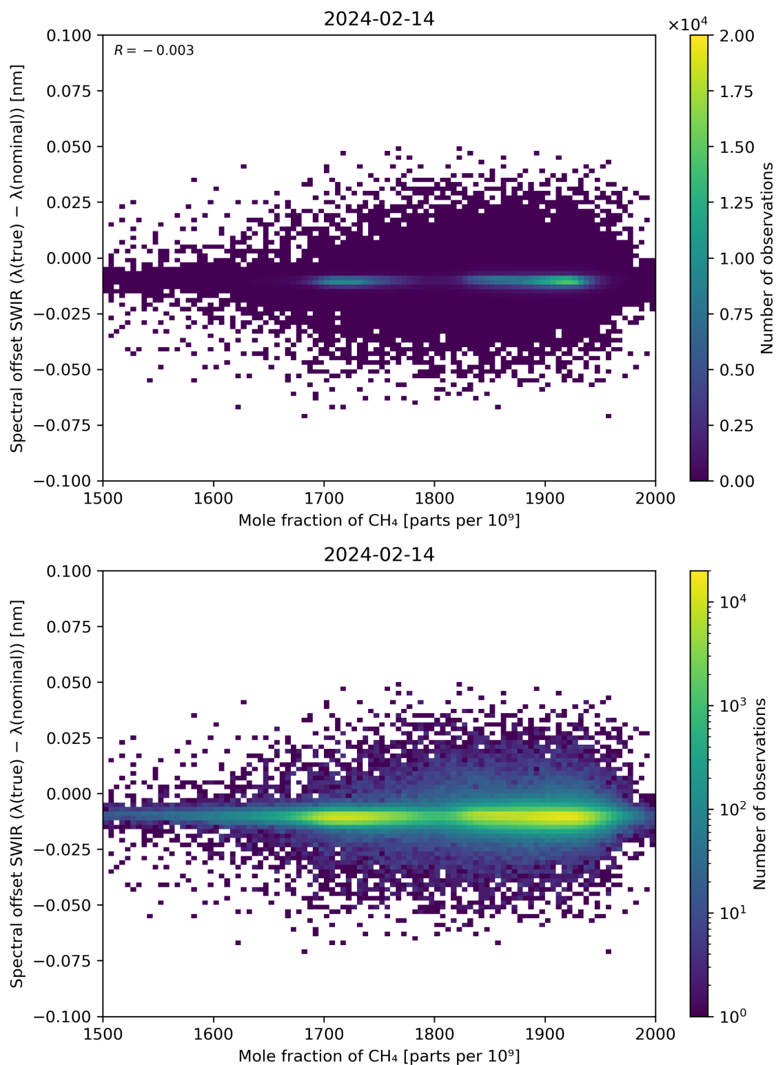
Figure 86: Scatter density plot of “Mole fraction of CH 4 ” against “Spectral offset SWIR ( \lambda(\text{true}) - \lambda(\text{nominal}) )” for 2024-02-13 to 2024-02-15.
