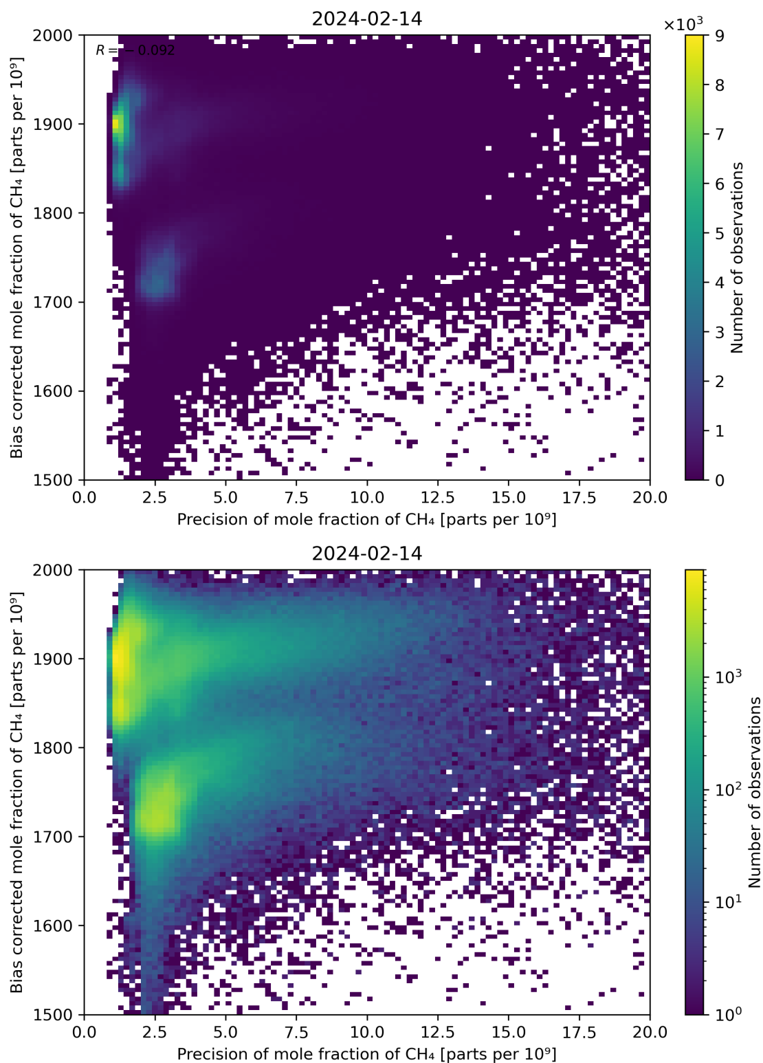
Figure 82: Scatter density plot of “Precision of mole fraction of \text{CH}_4 ” against “Bias corrected mole fraction of \text{CH}_4 ” for 2024-02-13 to 2024-02-15.
