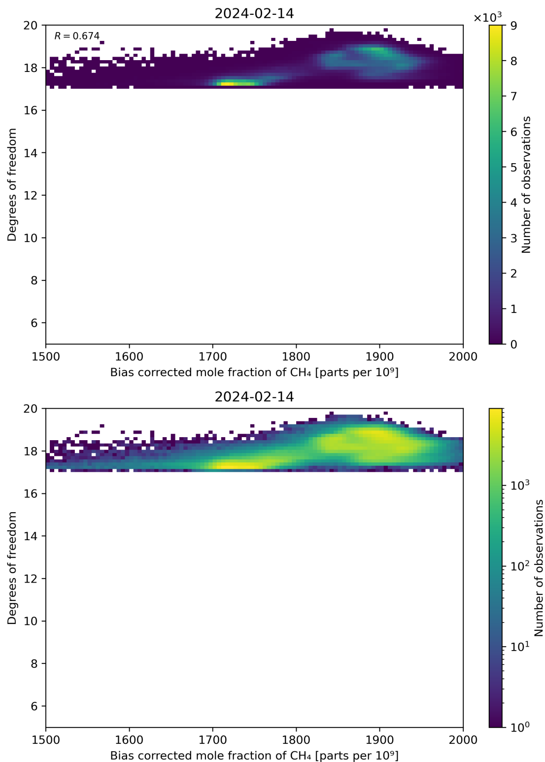
Figure 65: Scatter density plot of “Bias corrected mole fraction of CH 4 ” against “Degrees of freedom” for 2024-02-13 to 2024-02-15.
