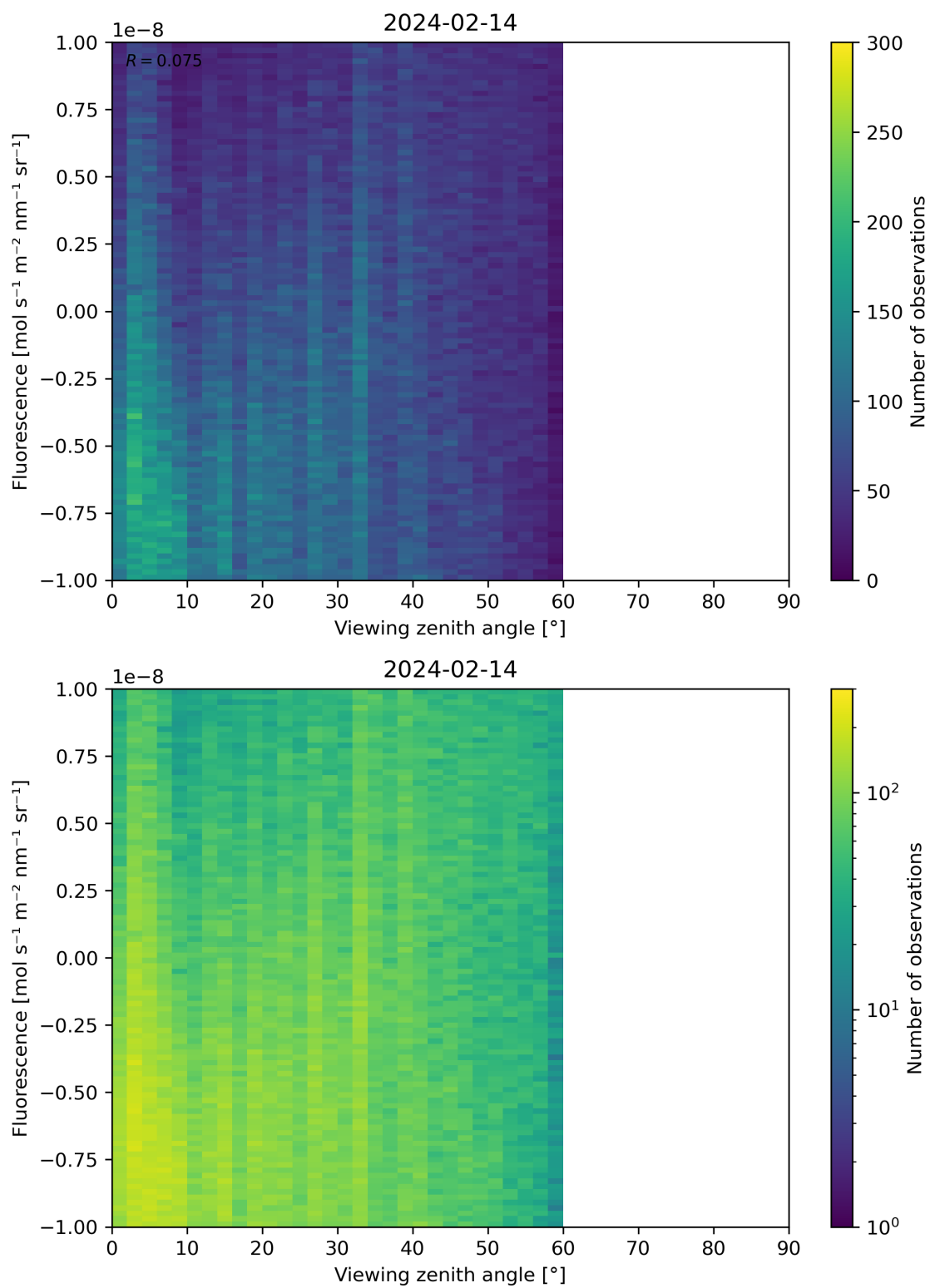
Figure 108: Scatter density plot of “Viewing zenith angle” against “Fluorescence” for 2024-02-13 to 2024-02-15.
