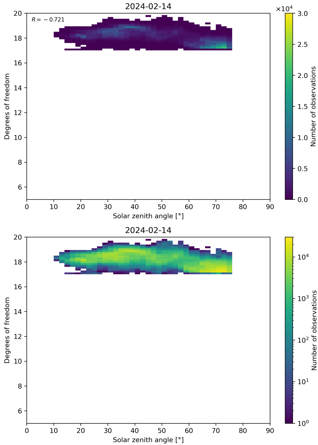
Figure 96: Scatter density plot of “Solar zenith angle” against “Degrees of freedom” for 2024-02-13 to 2024-02-15.
