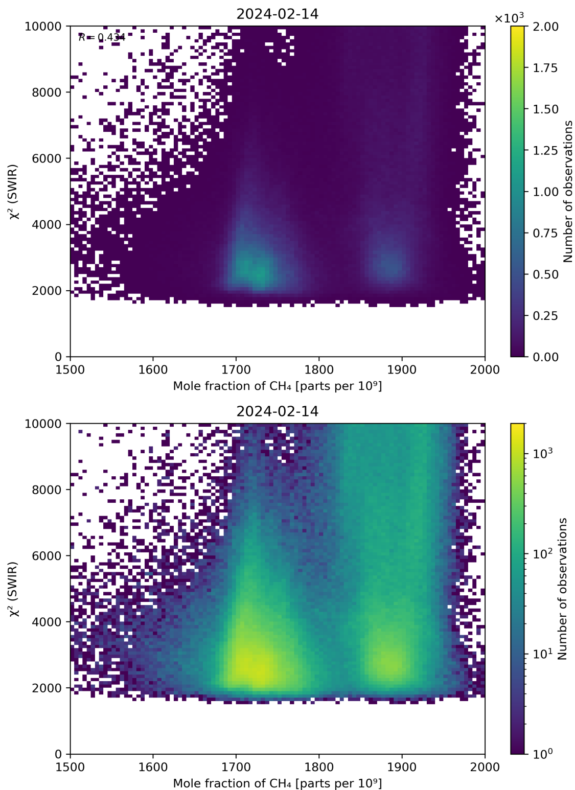
Figure 71: Scatter density plot of “Mole fraction of \text{CH}_4 ” against “ \chi^2 (SWIR)” for 2024-02-13 to 2024-02-15.
