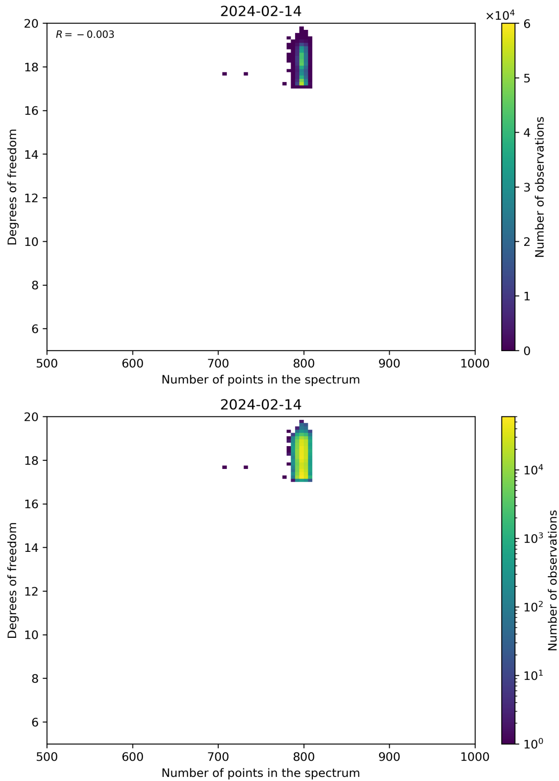
Figure 90: Scatter density plot of “Number of points in the spectrum” against “Degrees of freedom” for 2024-02-13 to 2024-02-15.
