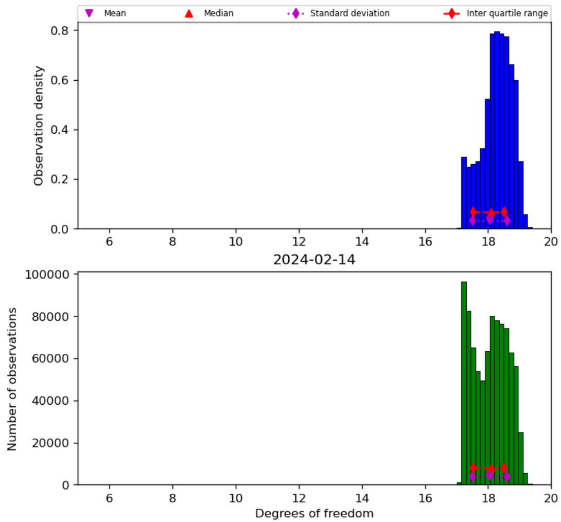
Figure 30: Histogram of “Degrees of freedom” for 2024-02-13 to 2024-02-15
