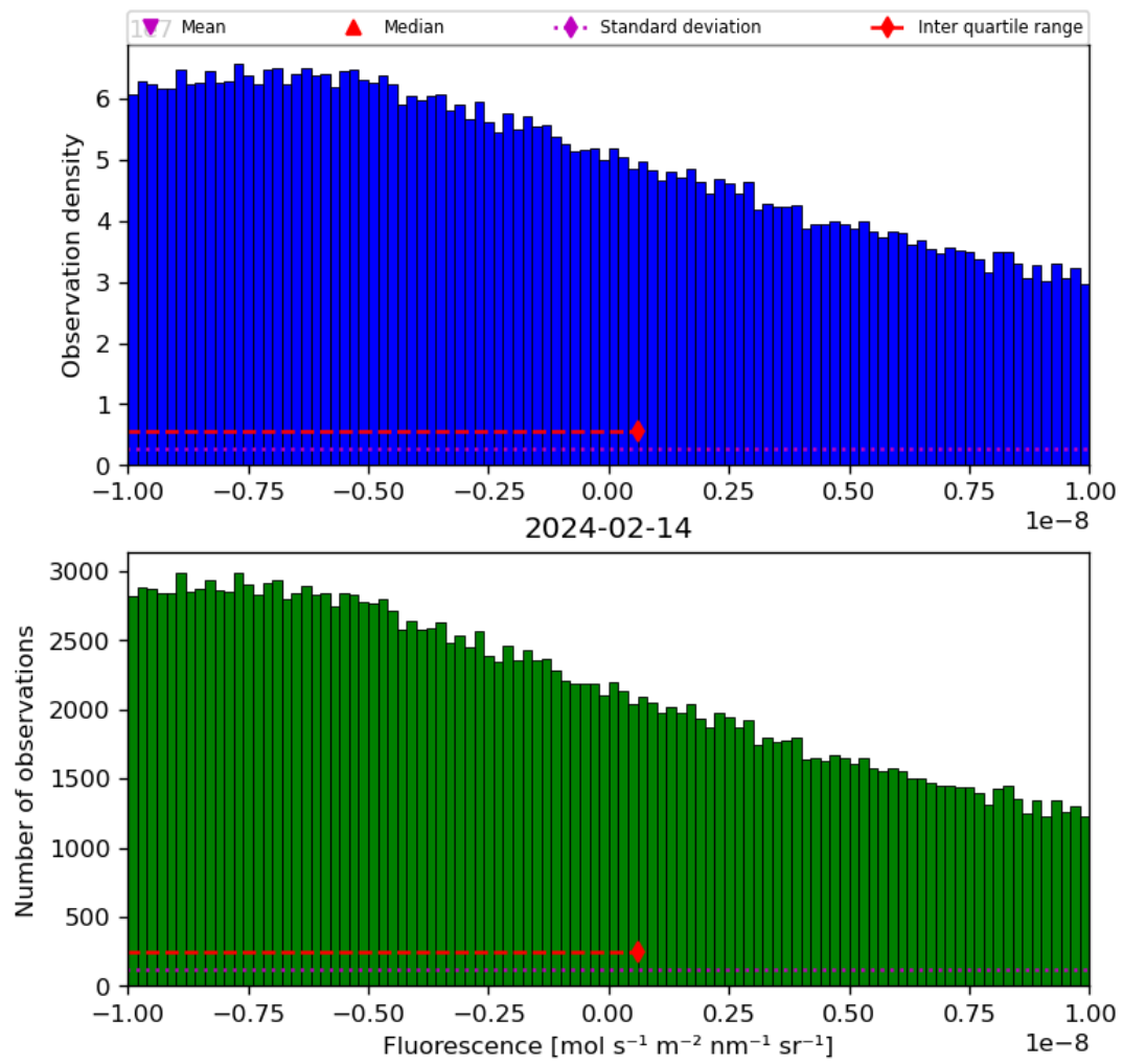
Figure 32: Histogram of “Fluorescence” for 2024-02-13 to 2024-02-15
