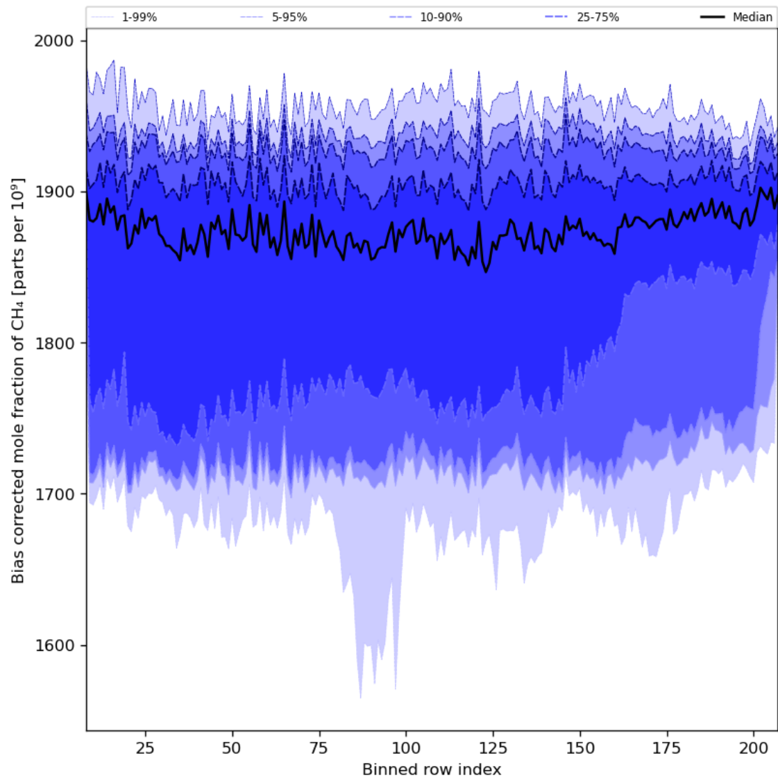
Figure 36: Along track statistics of “Bias corrected mole fraction of CH 4 ” for 2024-02-13 to 2024-02-15
