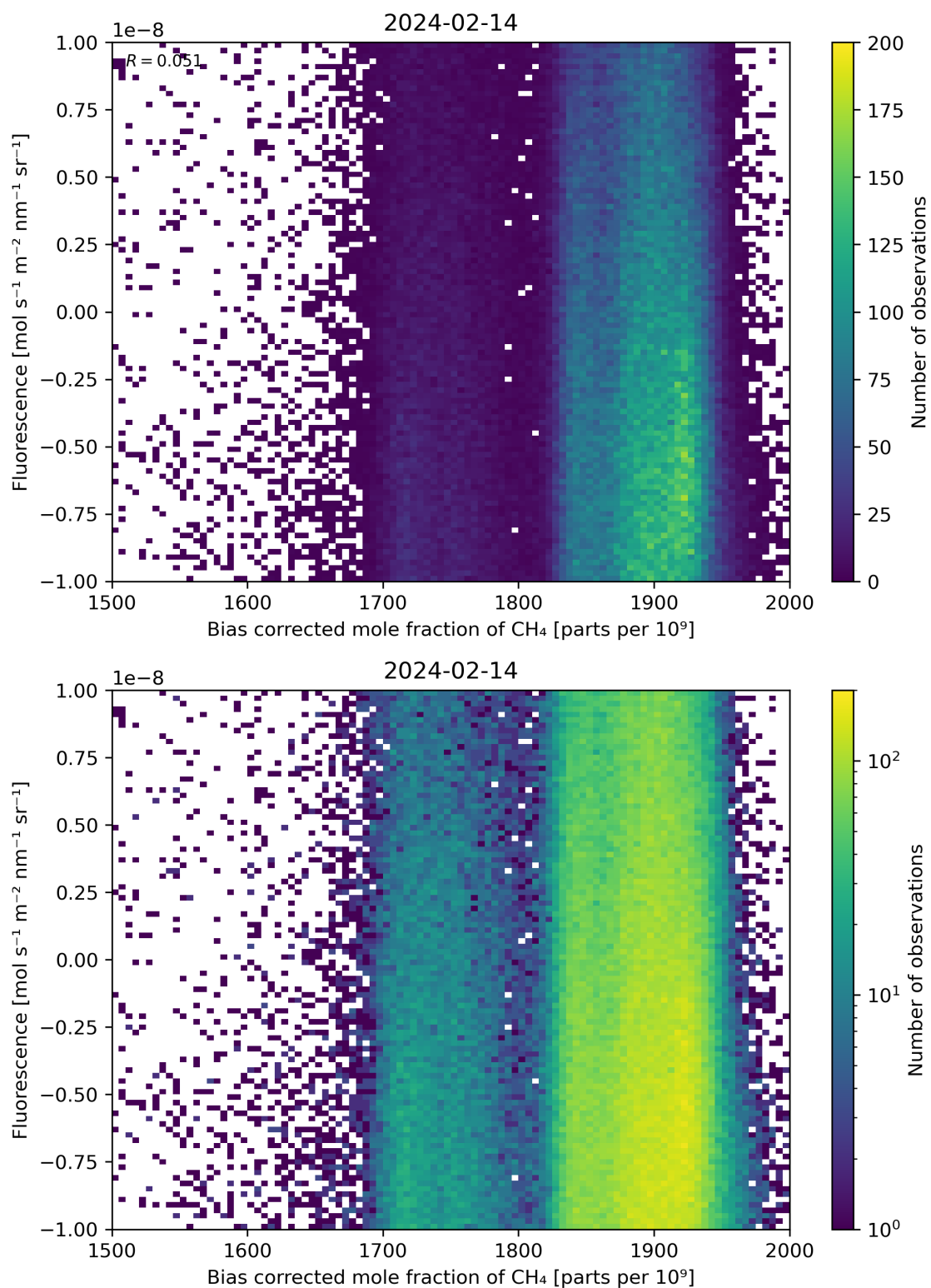
Figure 66: Scatter density plot of “Bias corrected mole fraction of \text{CH}_4 ” against “Fluorescence” for 2024-02-13 to 2024-02-15.
