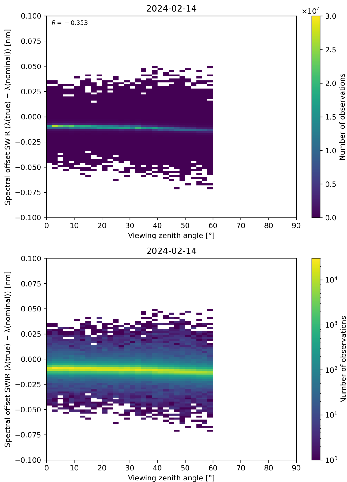
Figure 116: Scatter density plot of “Viewing zenith angle” against “Spectral offset SWIR ( \lambda(\text{true}) - \lambda(\text{nominal}) )” for 2024-02-13 to 2024-02-15.
