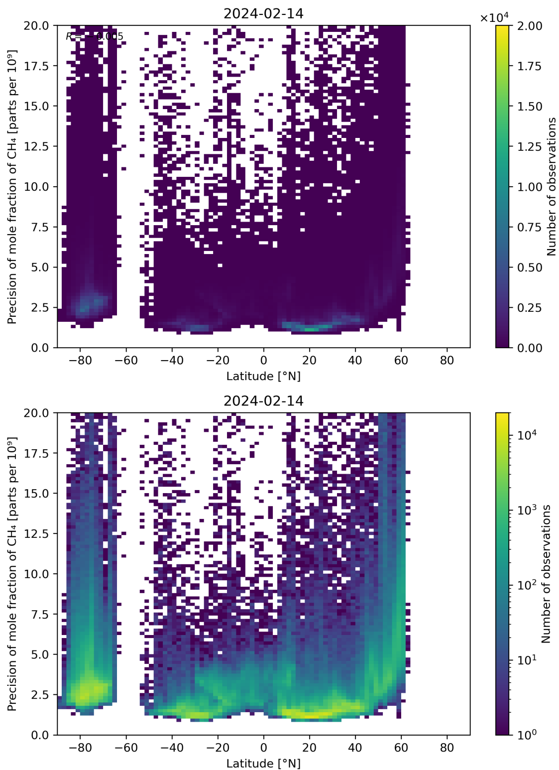
Figure 59: Scatter density plot of “Latitude” against “Precision of mole fraction of CH 4 ” for 2024-02-13 to 2024-02-15.
