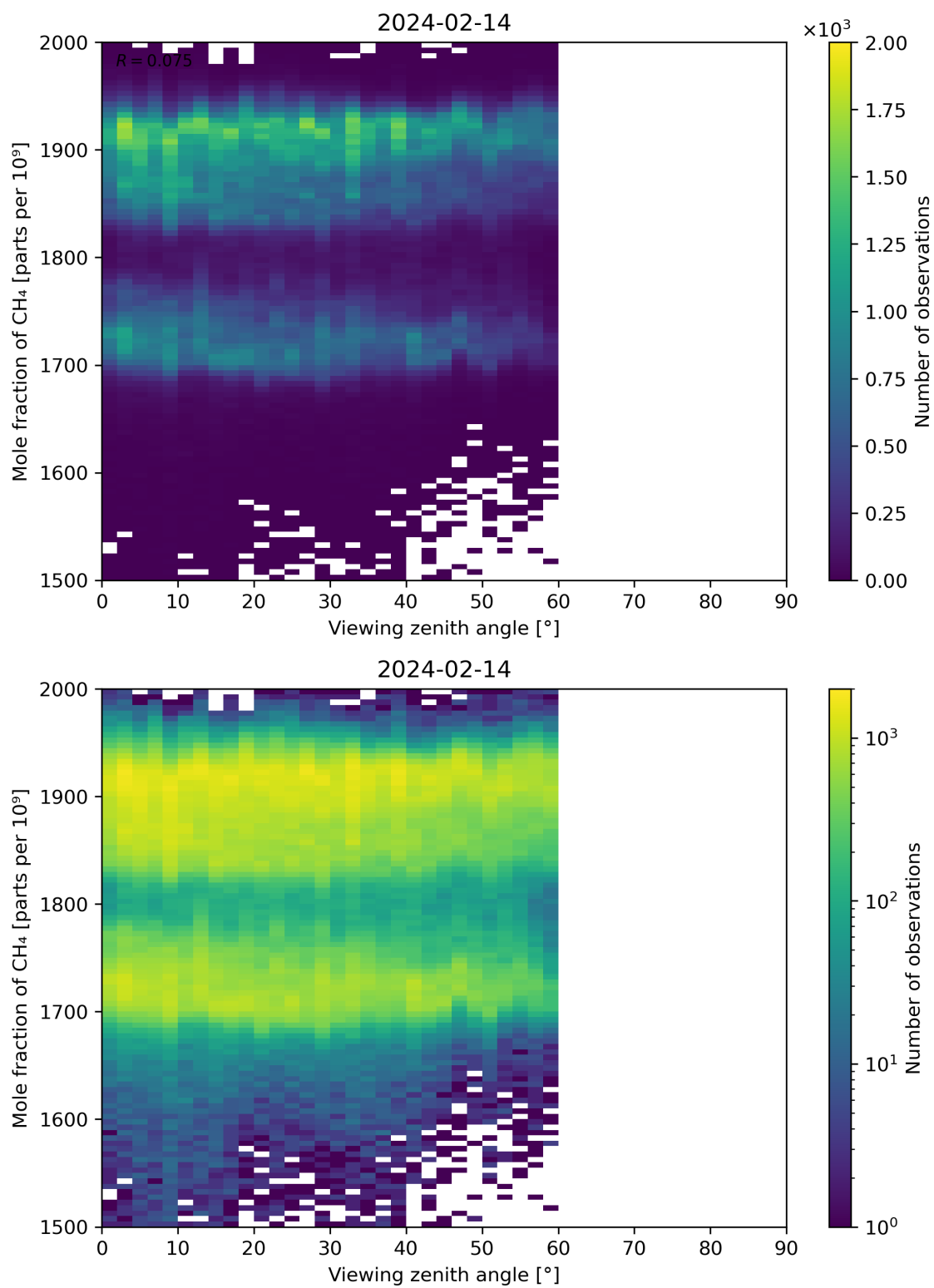
Figure 110: Scatter density plot of “Viewing zenith angle” against “Mole fraction of CH 4 ” for 2024-02-13 to 2024-02-15.
