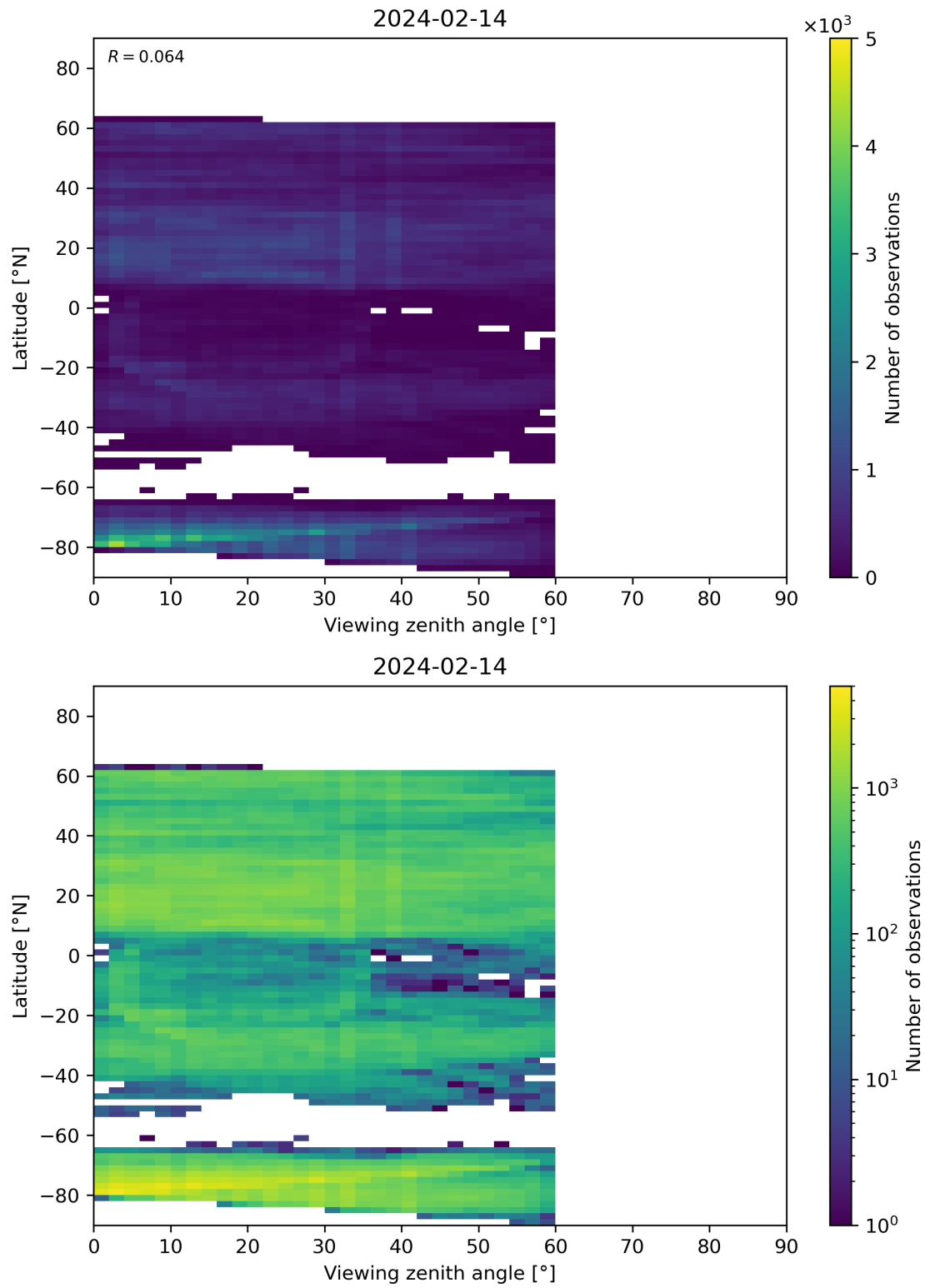
Figure 109: Scatter density plot of “Viewing zenith angle” against “Latitude” for 2024-02-13 to 2024-02-15.
