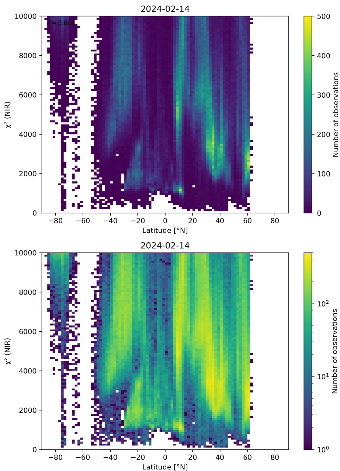
Figure 53: Scatter density plot of “Latitude” against “ \chi^2 (NIR)” for 2024-02-13 to 2024-02-15.
