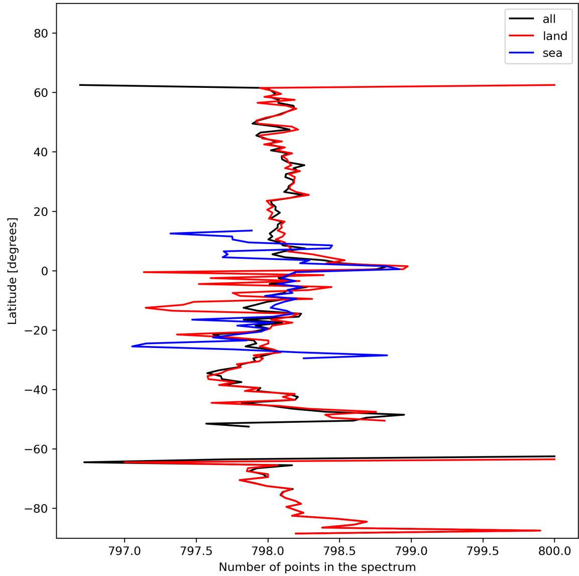
Figure 15: Zonal average of “Number of points in the spectrum” for 2024-02-13 to 2024-02-15.
