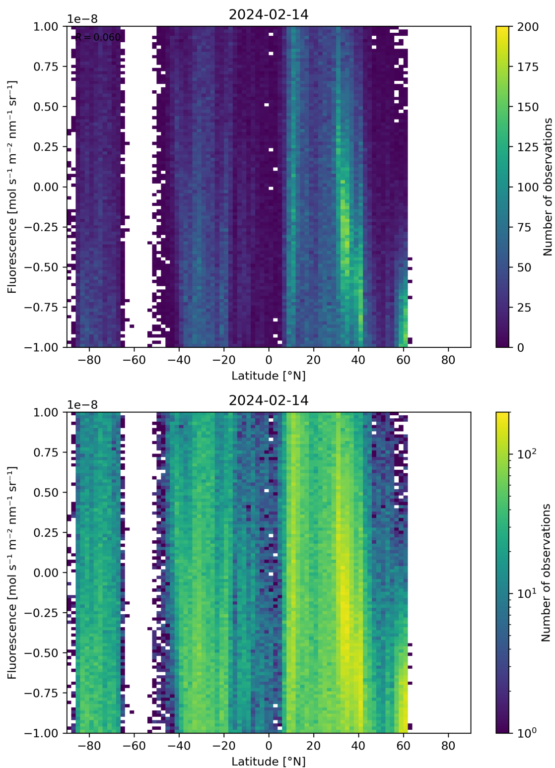
Figure 56: Scatter density plot of “Latitude” against “Fluorescence” for 2024-02-13 to 2024-02-15.
