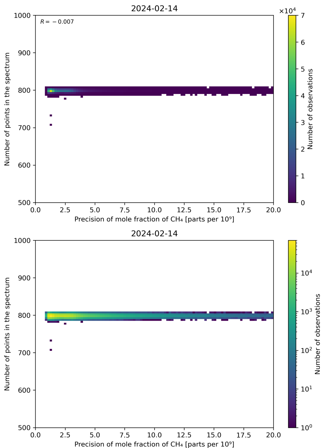
Figure 84: Scatter density plot of “Precision of mole fraction of CH 4 ” against “Number of points in the spectrum” for 2024-02-13 to 2024-02-15.
