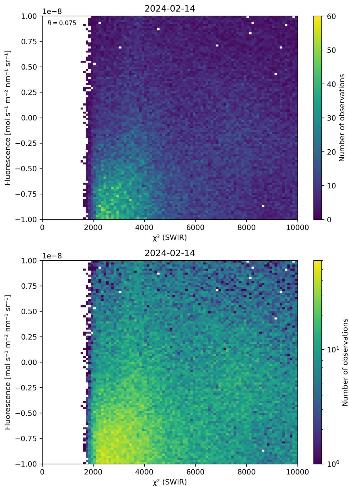
Figure 49: Scatter density plot of “ \chi^2 (SWIR)” against “Fluorescence” for 2024-02-13 to 2024-02-15.
