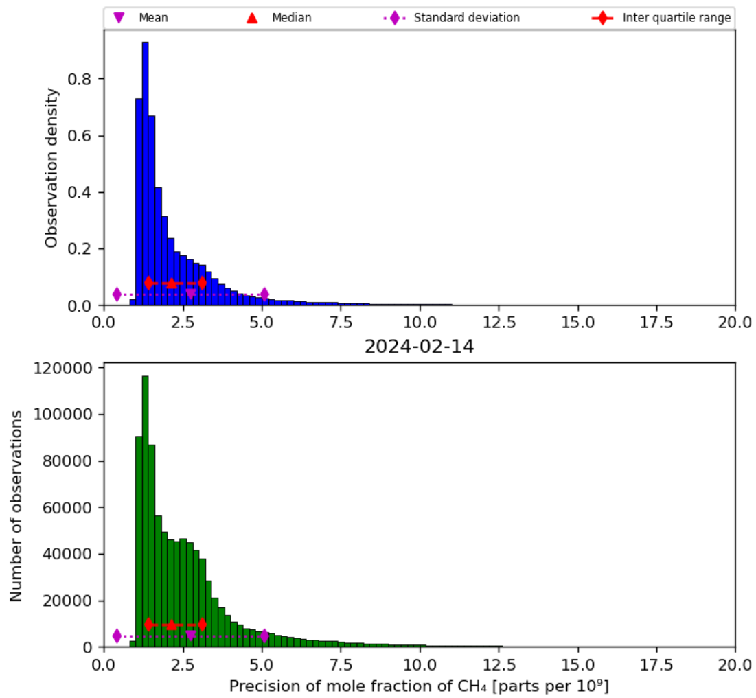
Figure 24: Histogram of “Precision of mole fraction of CH 4 ” for 2024-02-13 to 2024-02-15
