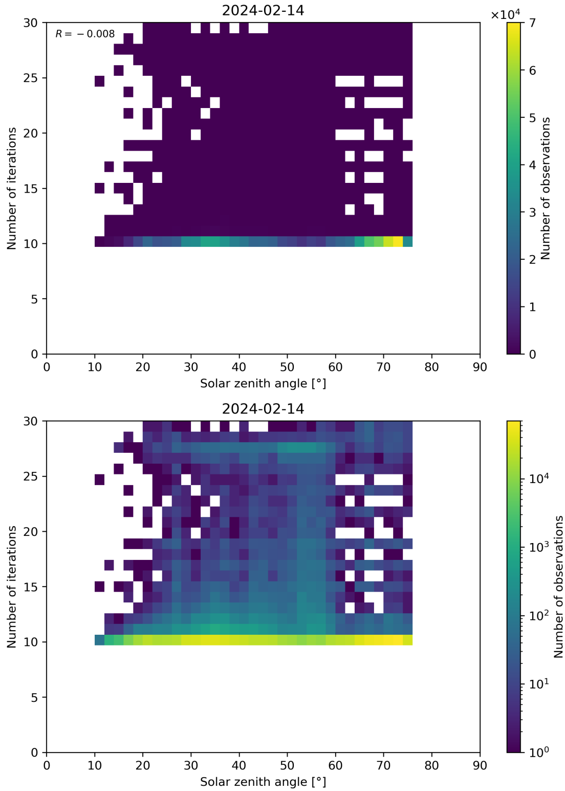
Figure 102: Scatter density plot of “Solar zenith angle” against “Number of iterations” for 2024-02-13 to 2024-02-15.
