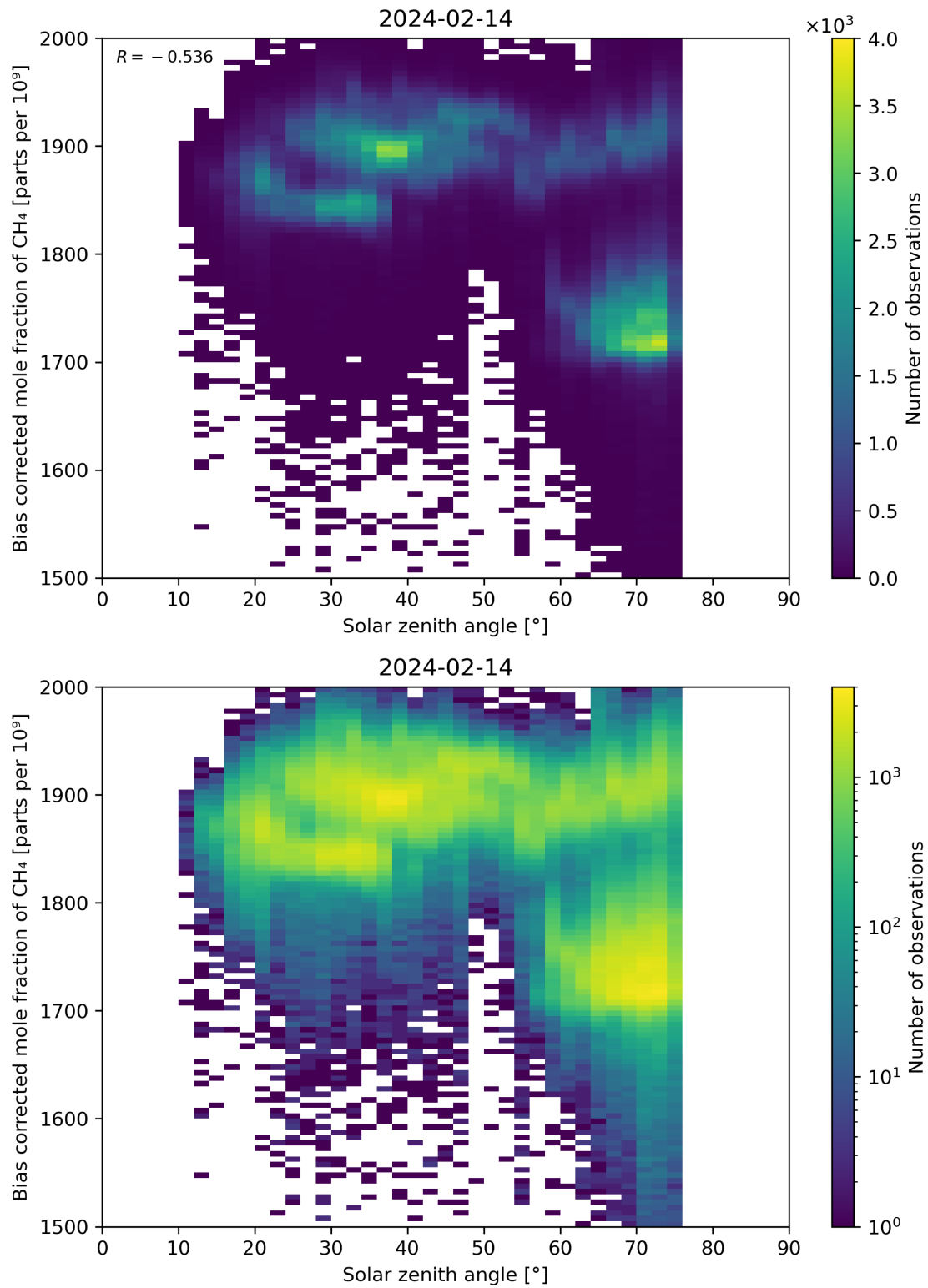
Figure 100: Scatter density plot of “Solar zenith angle” against “Bias corrected mole fraction of CH 4 ” for 2024-02-13 to 2024-02-15.
