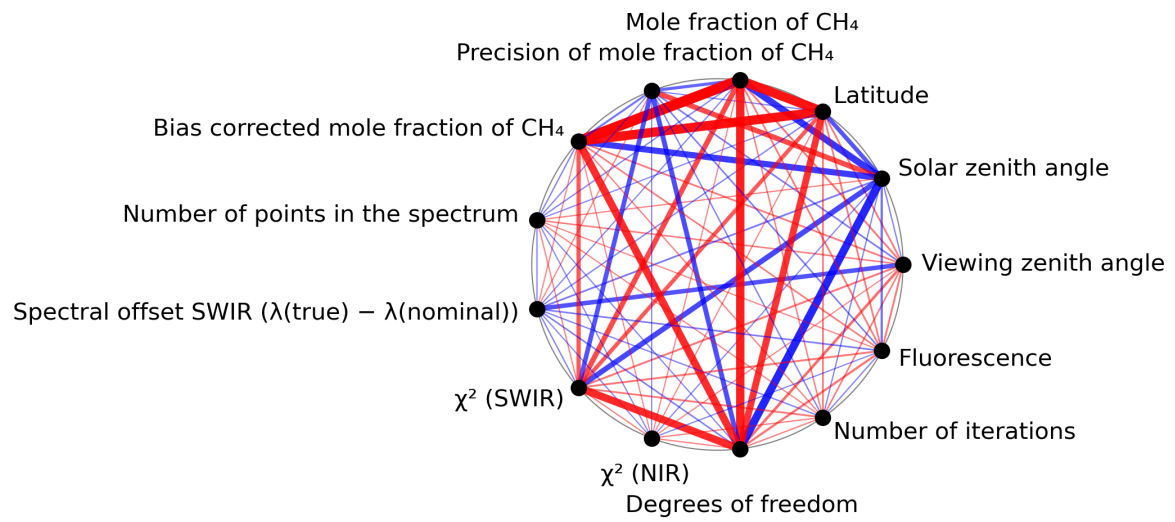
Figure 1: Map of correlation graph for 2024-02-13 to 2024-02-15.
