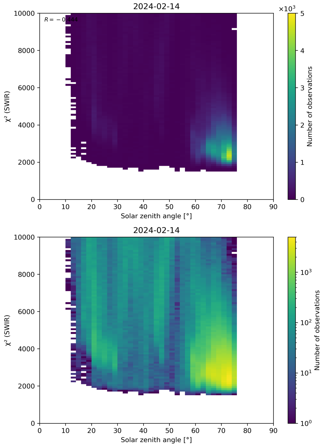
Figure 95: Scatter density plot of “Solar zenith angle” against “ \chi^2 (SWIR)” for 2024-02-13 to 2024-02-15.
