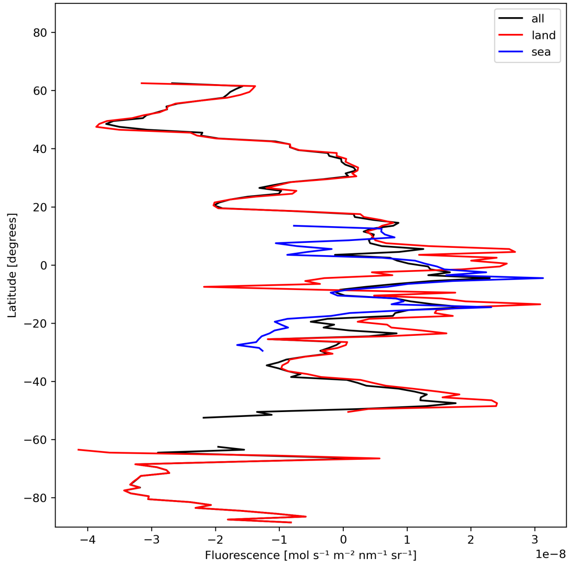
Figure 21: Zonal average of “Fluorescence” for 2024-02-13 to 2024-02-15.
