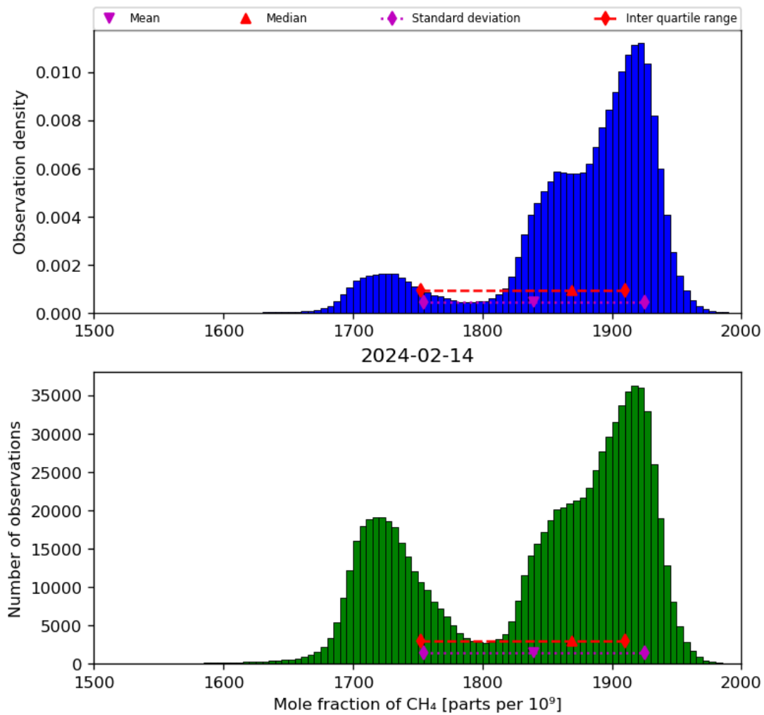
Figure 23: Histogram of “Mole fraction of CH 4 ” for 2024-02-13 to 2024-02-15
