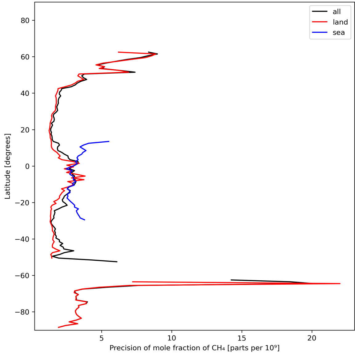
Figure 13: Zonal average of “Precision of mole fraction of CH 4 ” for 2024-02-13 to 2024-02-15.
