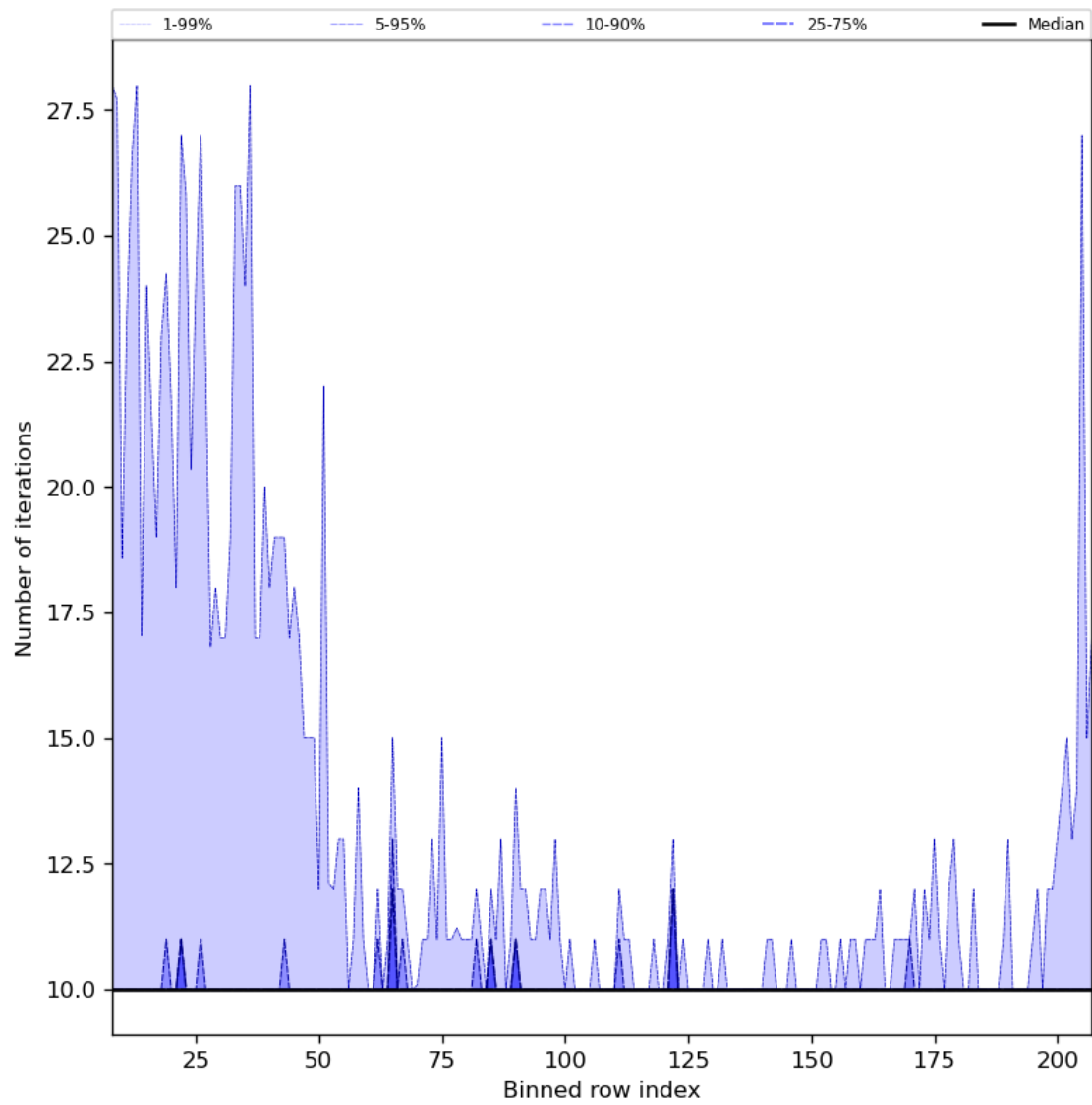
Figure 42: Along track statistics of “Number of iterations” for 2024-02-13 to 2024-02-15
