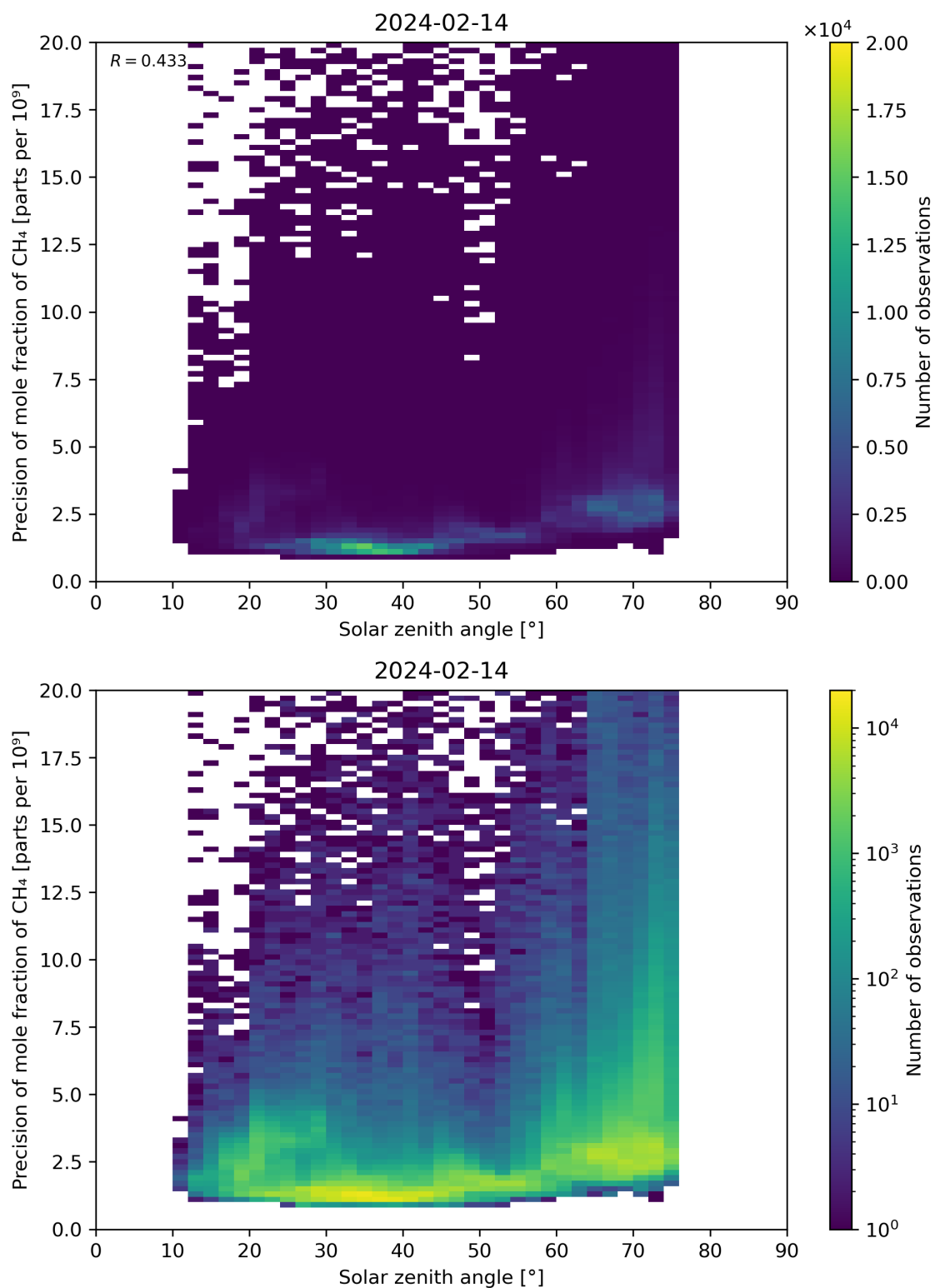
Figure 101: Scatter density plot of “Solar zenith angle” against “Precision of mole fraction of CH 4 ” for 2024-02-13 to 2024-02-15.
