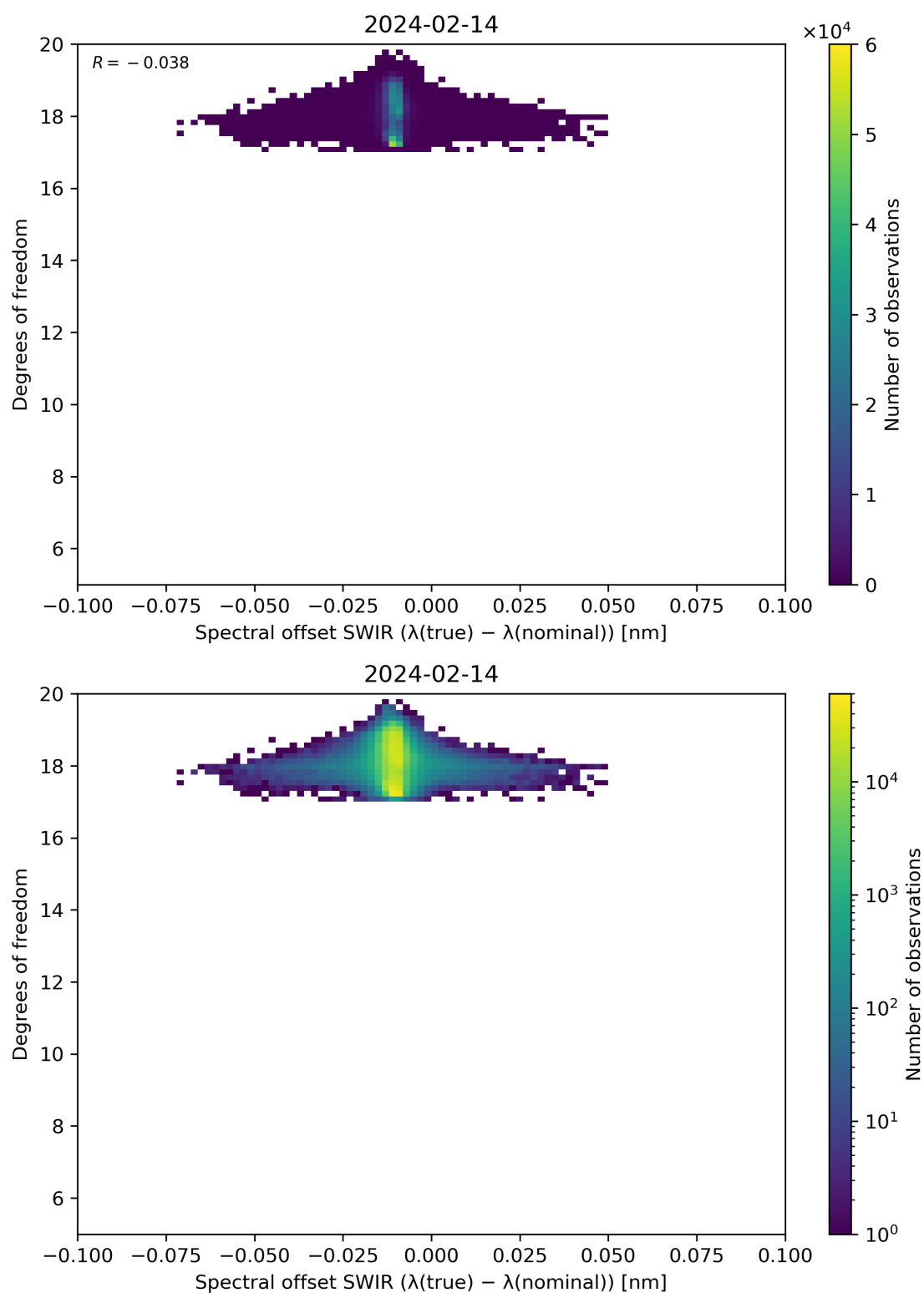
Figure 119: Scatter density plot of “Spectral offset SWIR ( \lambda(\text{true}) - \lambda(\text{nominal}) )” against “Degrees of freedom” for 2024-02-13 to 2024-02-15.
