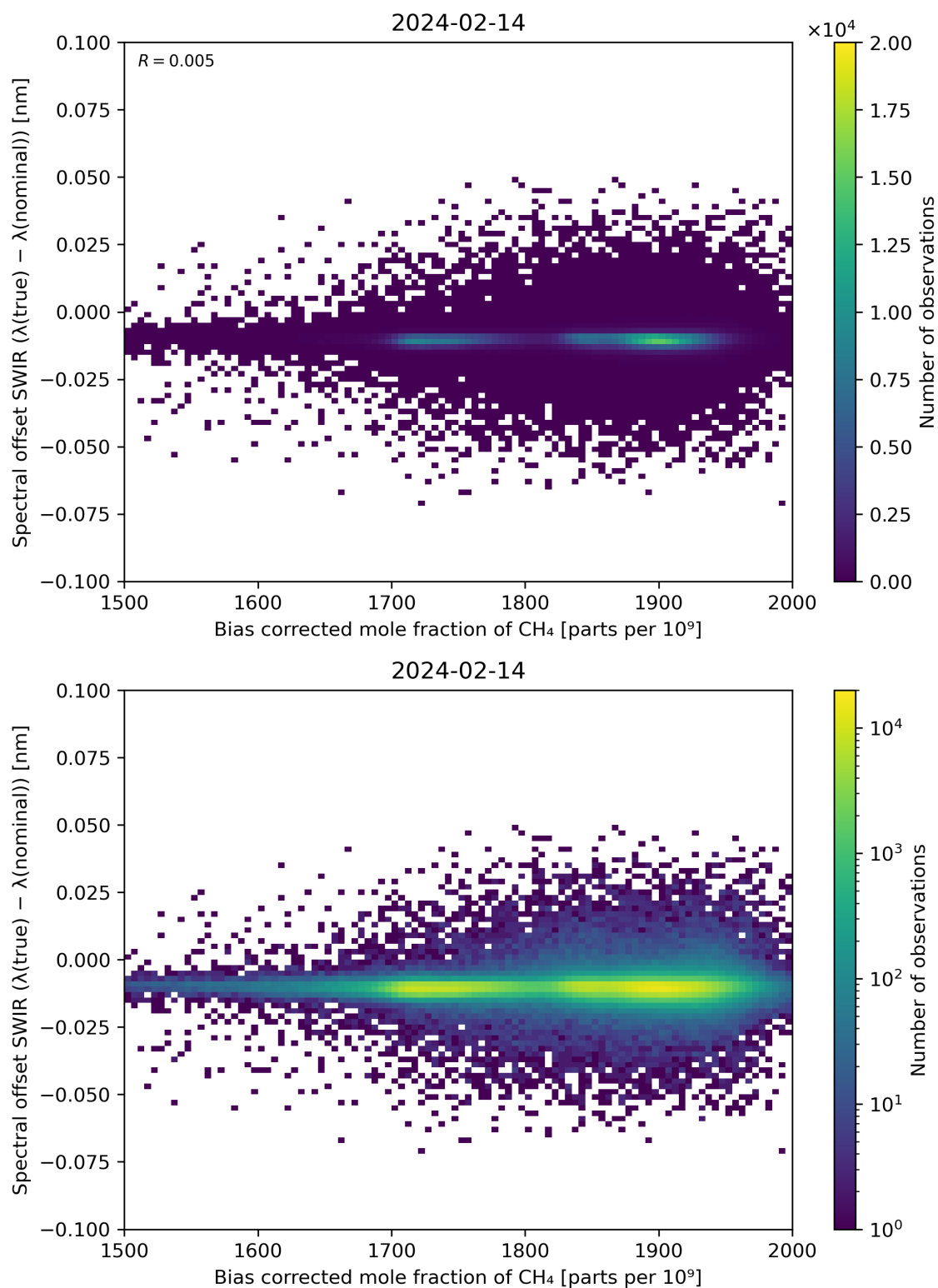
Figure 69: Scatter density plot of “Bias corrected mole fraction of \text{CH}_4 ” against “Spectral offset SWIR ( \lambda(\text{true}) - \lambda(\text{nominal}) )” for 2024-02-13 to 2024-02-15.
