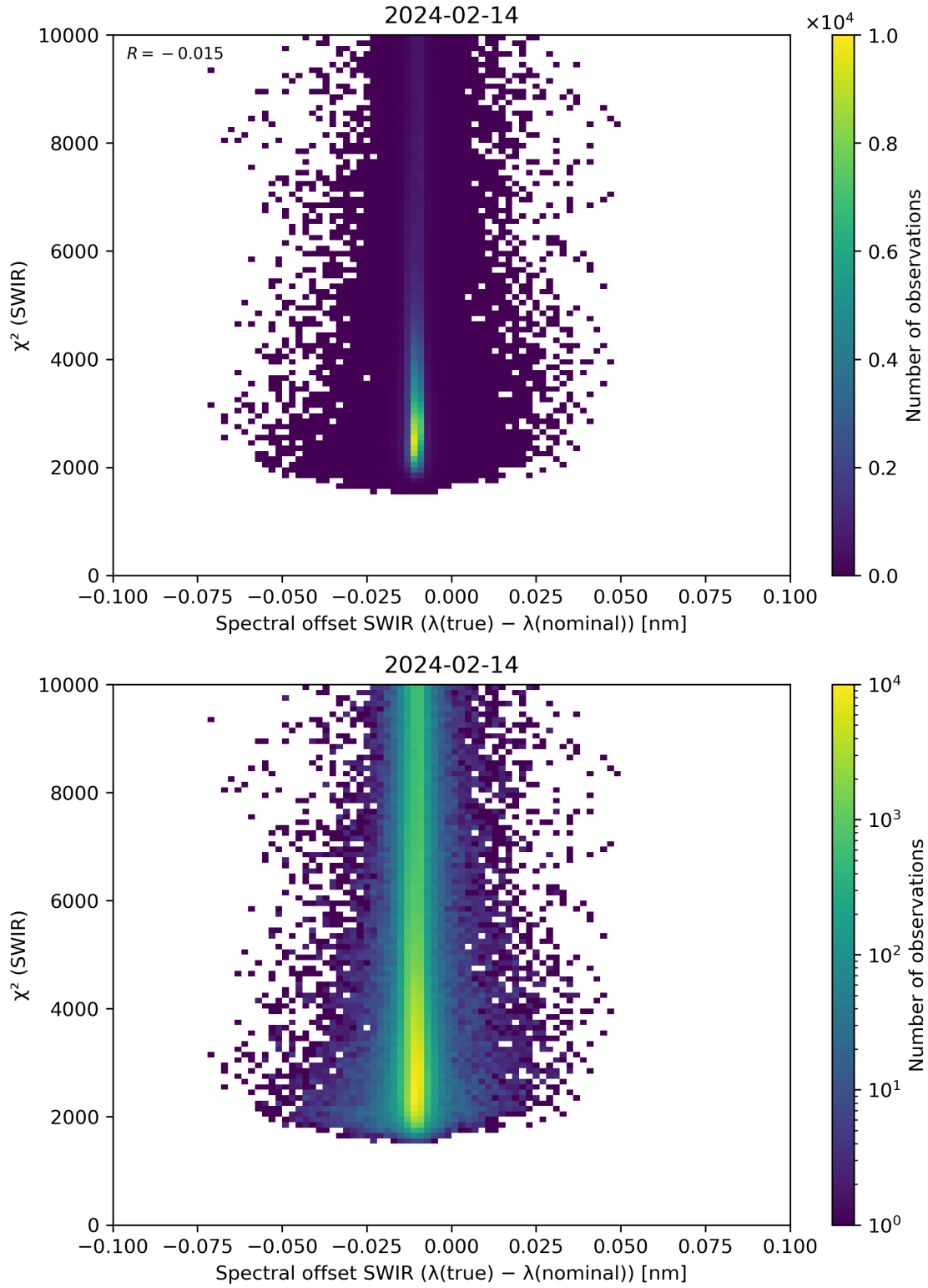
Figure 118: Scatter density plot of “Spectral offset SWIR ( \lambda(\text{true}) - \lambda(\text{nominal}) )” against “ \chi^2 (SWIR)” for 2024-02-13 to 2024-02-15.
