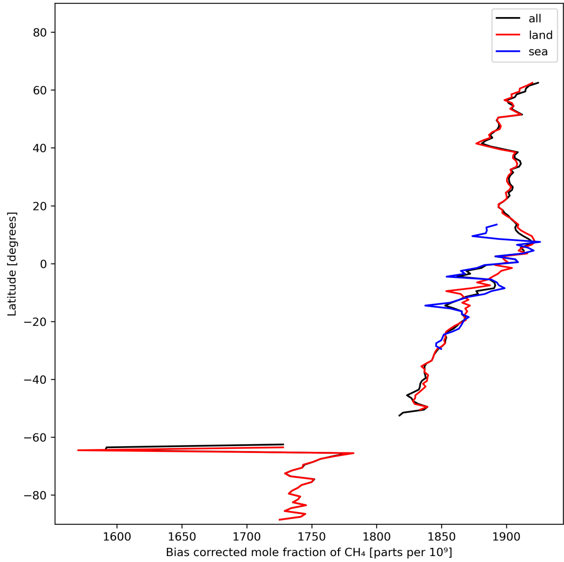
Figure 14: Zonal average of “Bias corrected mole fraction of CH 4 ” for 2024-02-13 to 2024-02-15.
