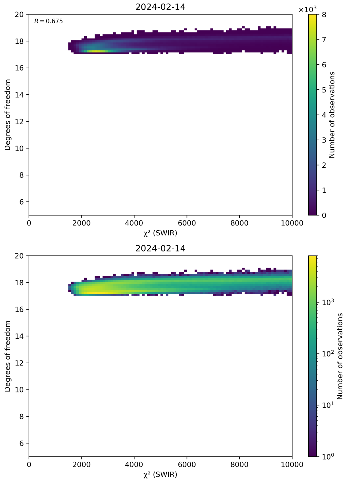
Figure 48: Scatter density plot of “ \chi^2 (SWIR)” against “Degrees of freedom” for 2024-02-13 to 2024-02-15.
