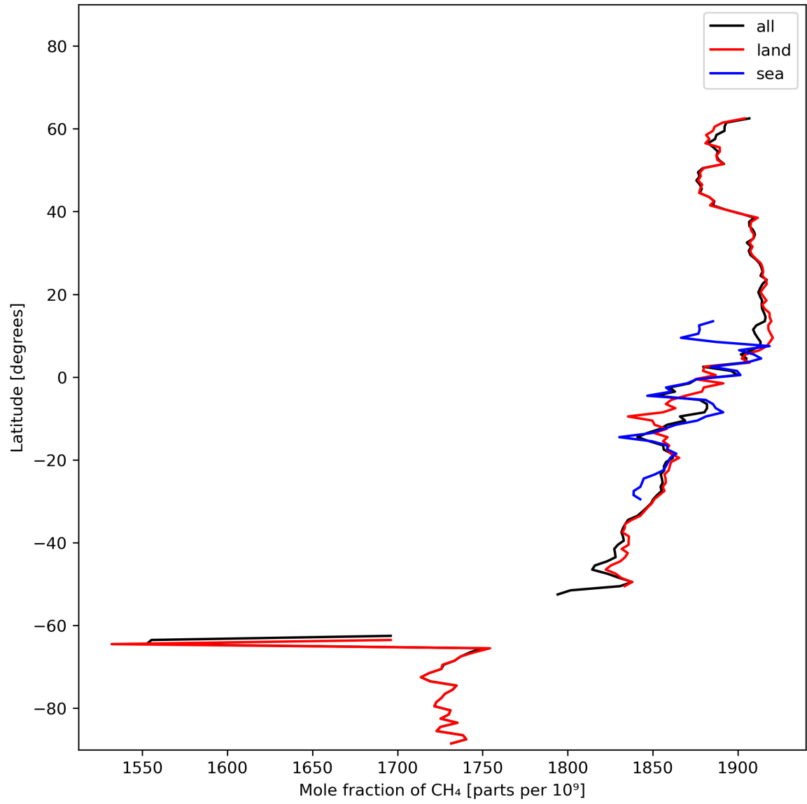
Figure 12: Zonal average of “Mole fraction of \text{CH}_4 ” for 2024-02-13 to 2024-02-15.
