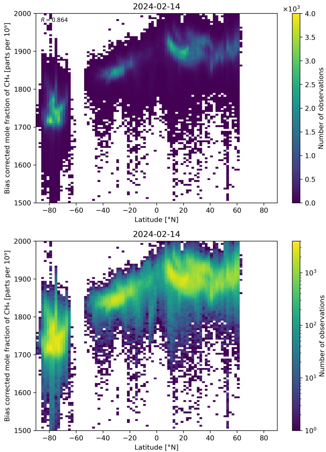
Figure 58: Scatter density plot of “Latitude” against “Bias corrected mole fraction of CH 4 ” for 2024-02-13 to 2024-02-15.
