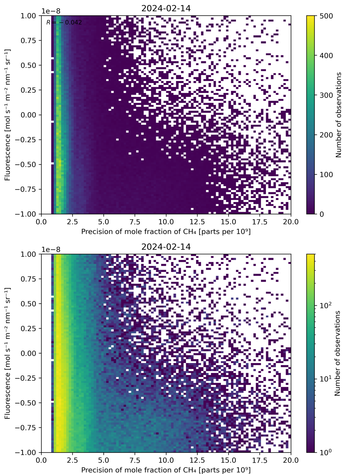
Figure 81: Scatter density plot of “Precision of mole fraction of \text{CH}_4 ” against “Fluorescence” for 2024-02-13 to 2024-02-15.
