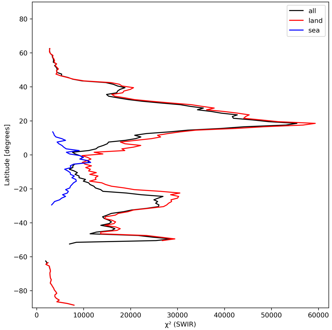
Figure 17: Zonal average of “ \chi^2 (SWIR)” for 2024-02-13 to 2024-02-15.
