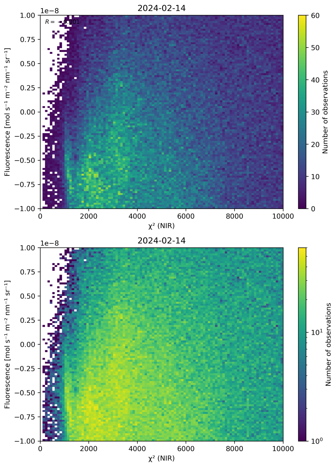
Figure 45: Scatter density plot of “ \chi^2 (NIR)” against “Fluorescence” for 2024-02-13 to 2024-02-15.
