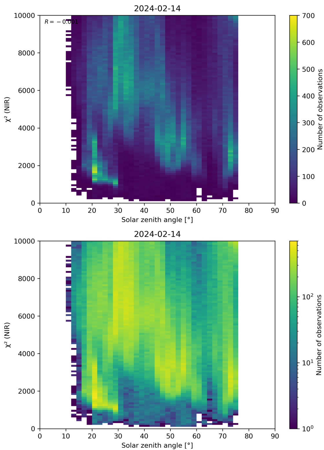
Figure 94: Scatter density plot of “Solar zenith angle” against “ \chi^2 (NIR)” for 2024-02-13 to 2024-02-15.
