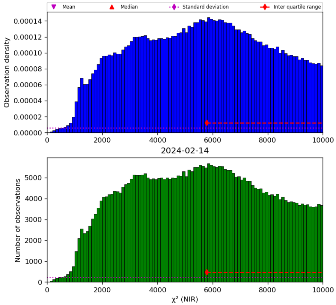
Figure 29: Histogram of “ \chi^2 (NIR)” for 2024-02-13 to 2024-02-15
