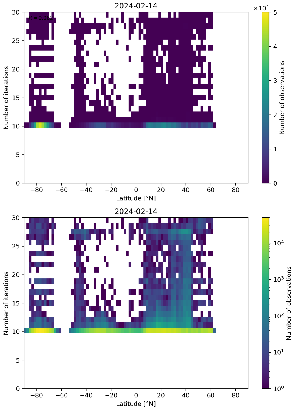
Figure 60: Scatter density plot of “Latitude” against “Number of iterations” for 2024-02-13 to 2024-02-15.
