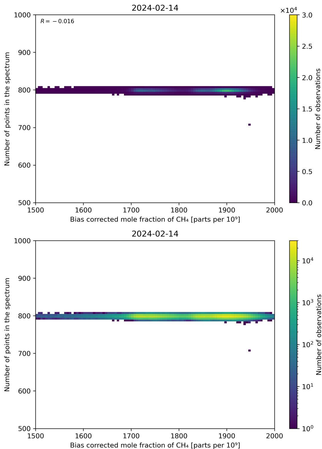
Figure 68: Scatter density plot of “Bias corrected mole fraction of CH 4 ” against “Number of points in the spectrum” for 2024-02-13 to 2024-02-15.
