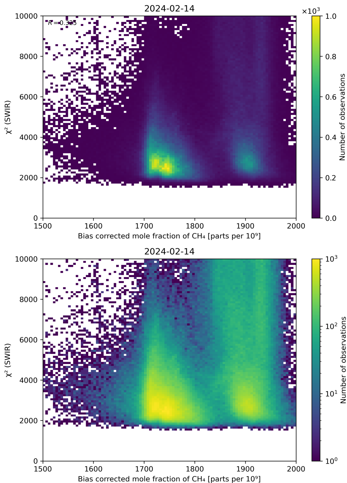
Figure 64: Scatter density plot of “Bias corrected mole fraction of CH 4 ” against “ \chi^2 (SWIR)” for 2024-02-13 to 2024-02-15.
