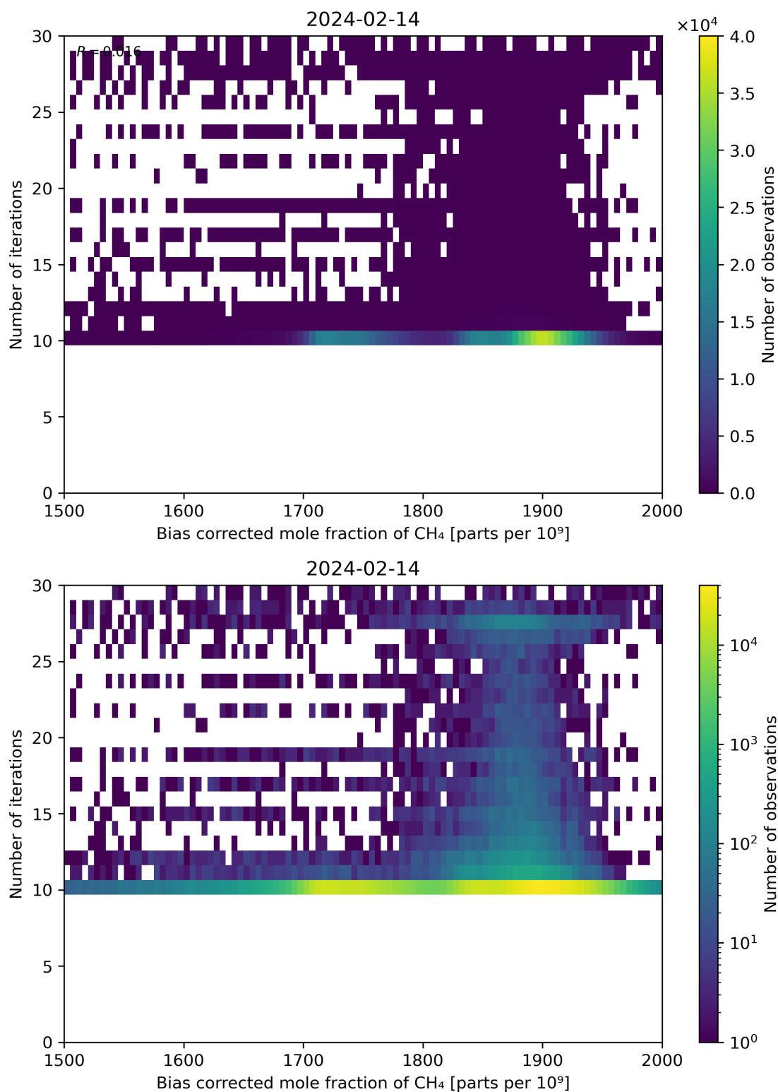
Figure 67: Scatter density plot of “Bias corrected mole fraction of CH 4 ” against “Number of iterations” for 2024-02-13 to 2024-02-15.
