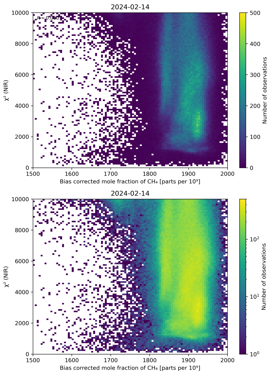
Figure 63: Scatter density plot of “Bias corrected mole fraction of \text{CH}_4 ” against “ \chi^2 (NIR)” for 2024-02-13 to 2024-02-15.
