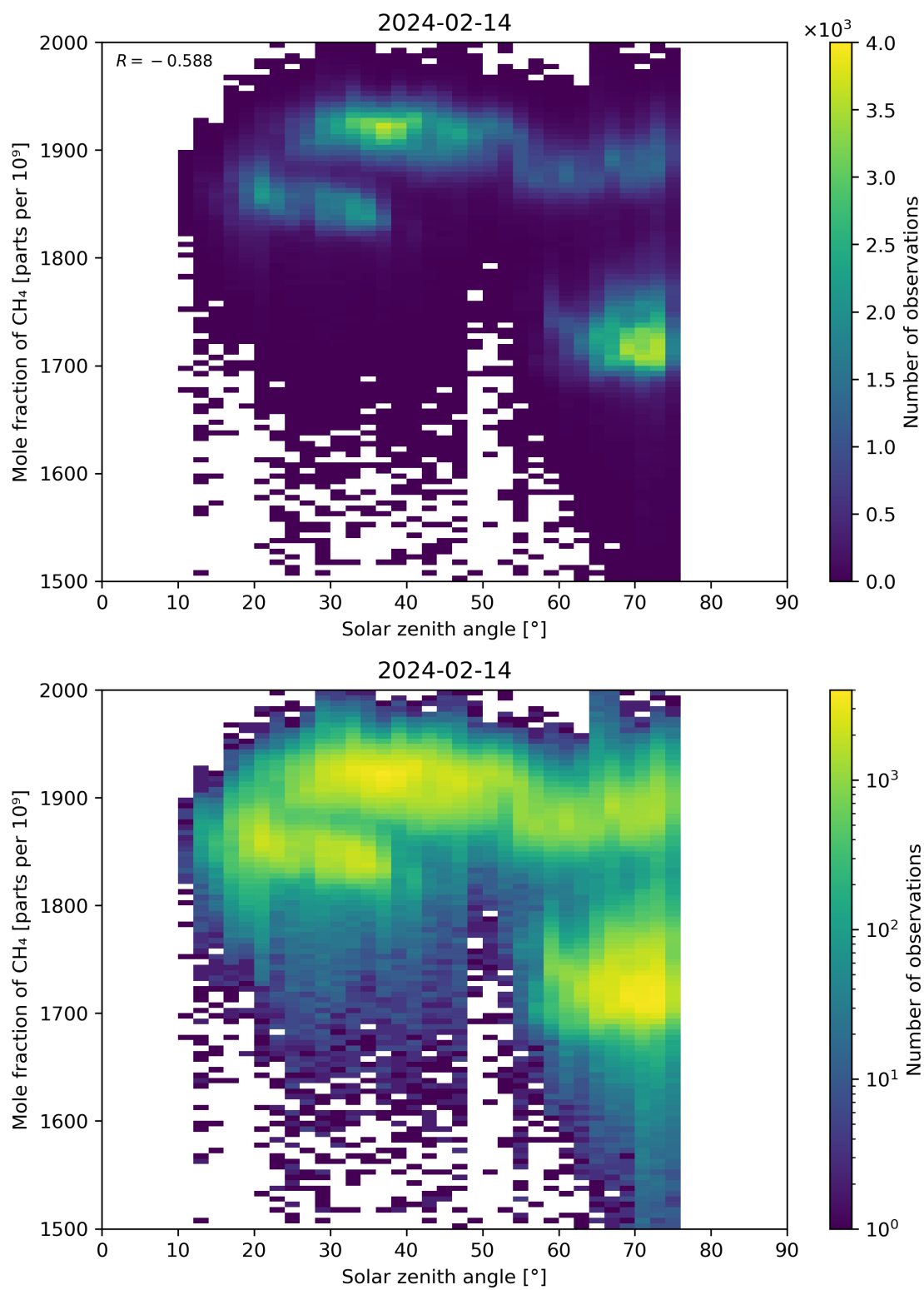
Figure 99: Scatter density plot of “Solar zenith angle” against “Mole fraction of CH 4 ” for 2024-02-13 to 2024-02-15.
