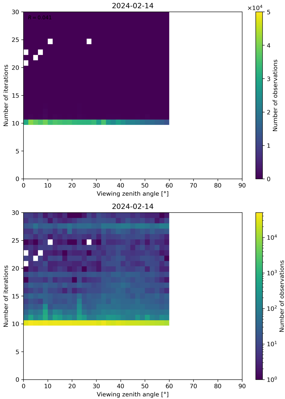
Figure 113: Scatter density plot of “Viewing zenith angle” against “Number of iterations” for 2024-02-13 to 2024-02-15.
