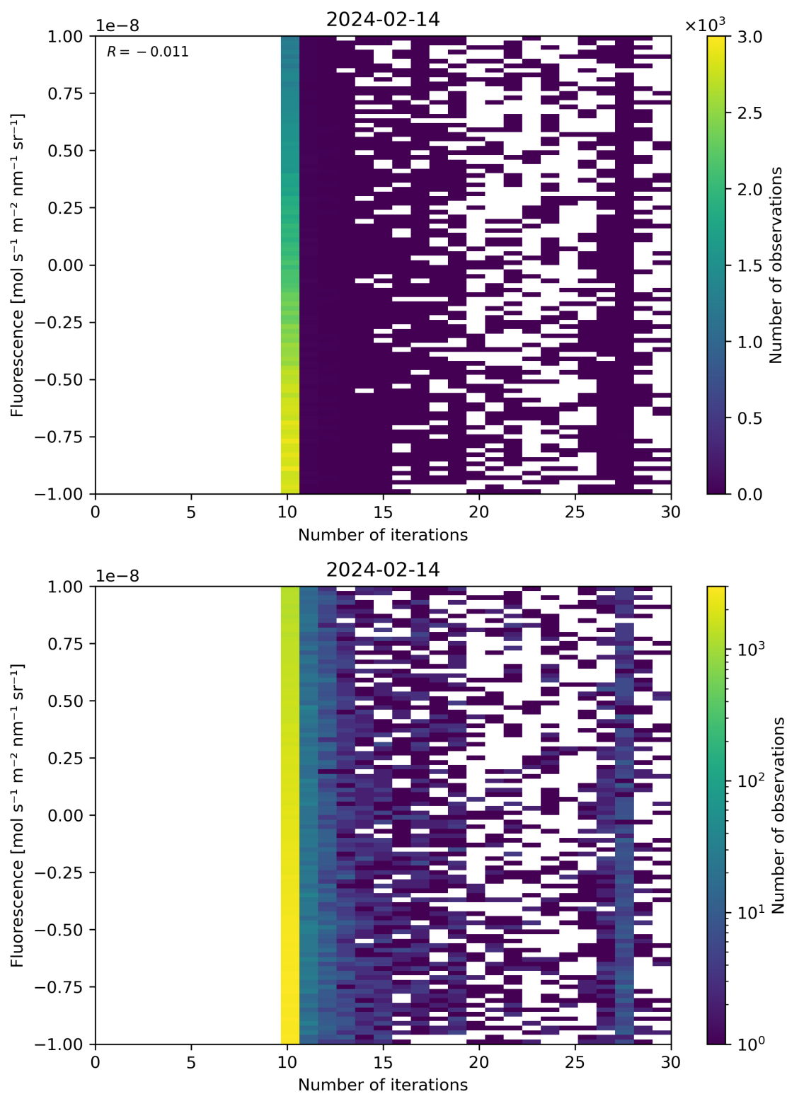
Figure 87: Scatter density plot of “Number of iterations” against “Fluorescence” for 2024-02-13 to 2024-02-15.
