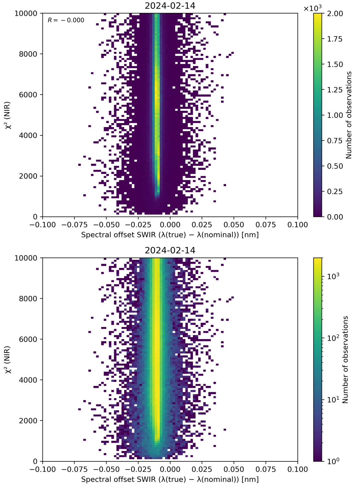
Figure 117: Scatter density plot of “Spectral offset SWIR ( \lambda(\text{true}) - \lambda(\text{nominal}) )” against “ \chi^2 (NIR)” for 2024-02-13 to 2024-02-15.
