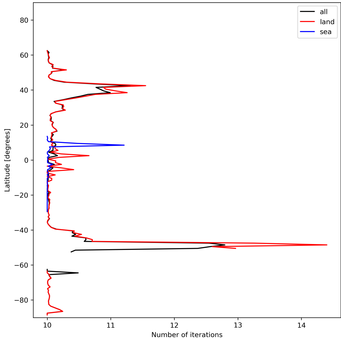
Figure 20: Zonal average of “Number of iterations” for 2024-02-13 to 2024-02-15.
