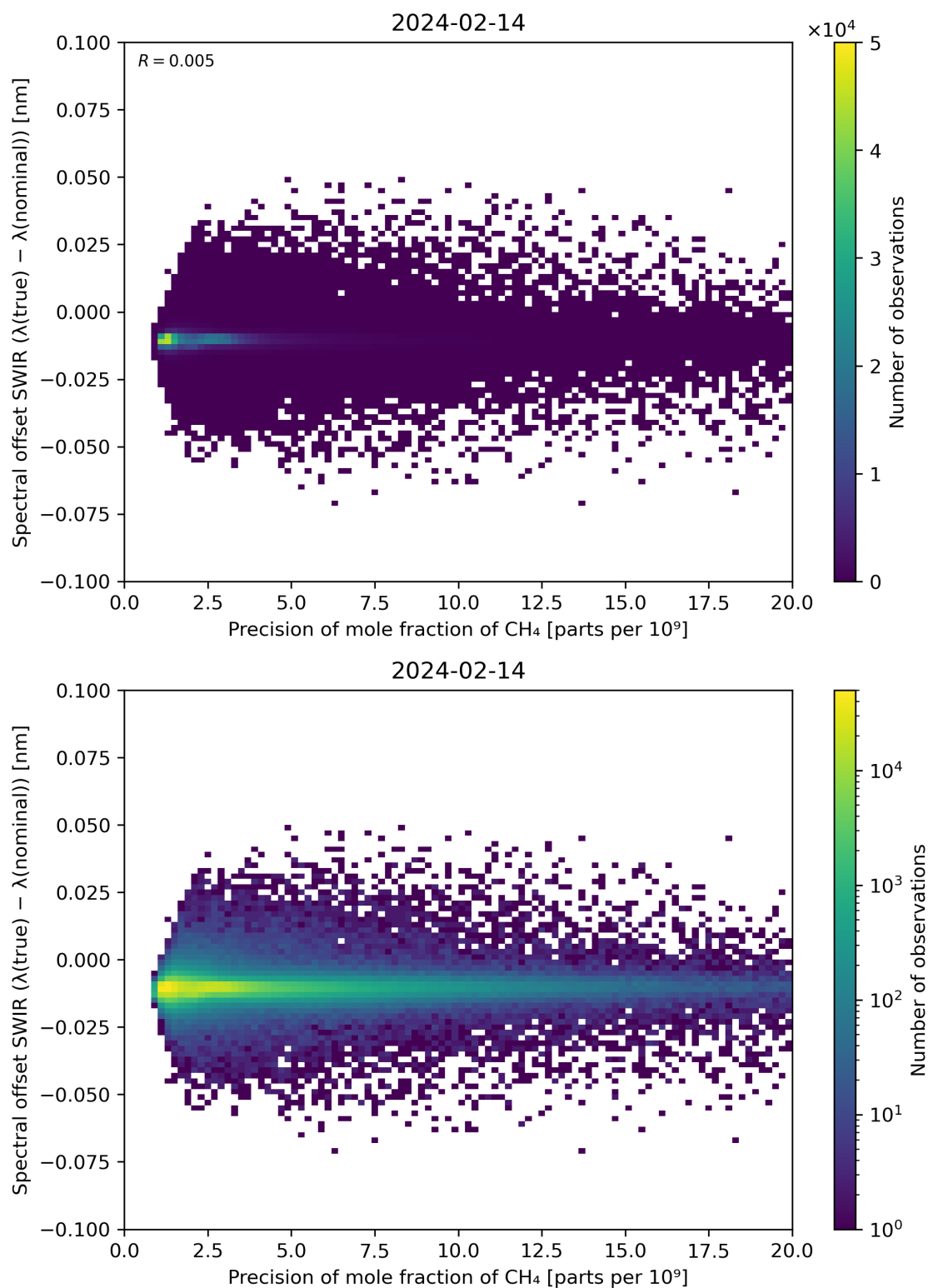
Figure 85: Scatter density plot of “Precision of mole fraction of CH 4 ” against “Spectral offset SWIR ( \lambda(\text{true}) - \lambda(\text{nominal}) )” for 2024-02-13 to 2024-02-15.
