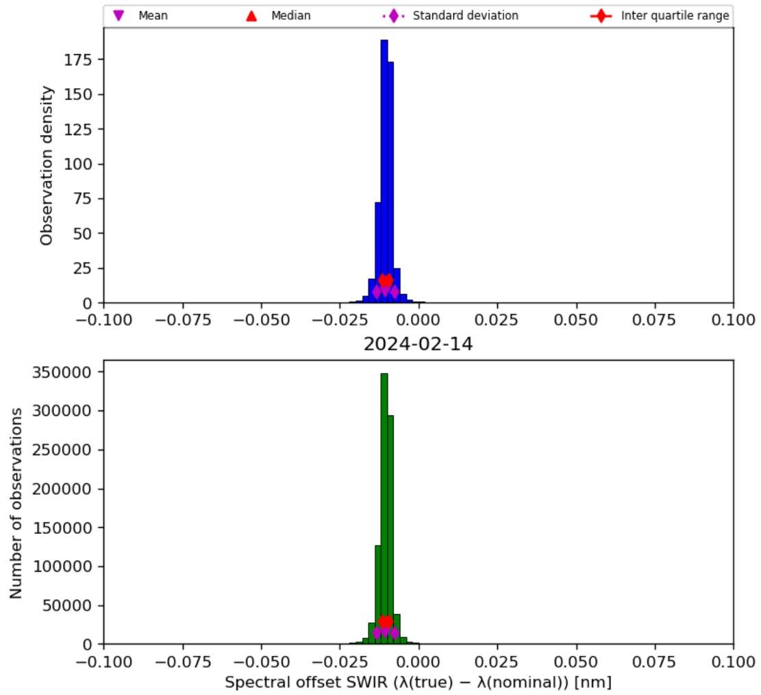
Figure 27: Histogram of “Spectral offset SWIR ( \lambda(\text{true}) - \lambda(\text{nominal}) )” for 2024-02-13 to 2024-02-15
