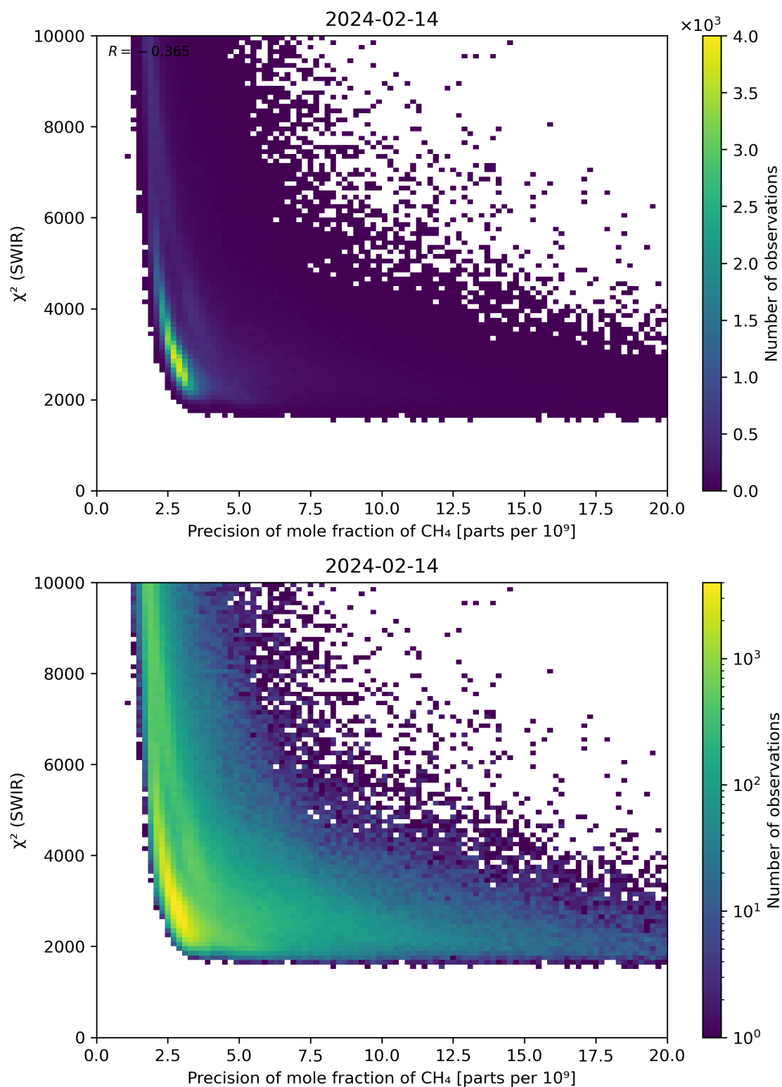
Figure 79: Scatter density plot of “Precision of mole fraction of \text{CH}_4 ” against “ \chi^2 (SWIR)” for 2024-02-13 to 2024-02-15.
