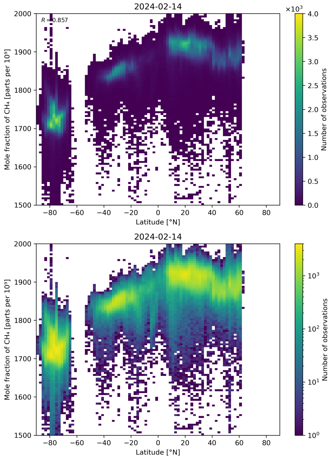
Figure 57: Scatter density plot of “Latitude” against “Mole fraction of CH 4 ” for 2024-02-13 to 2024-02-15.
