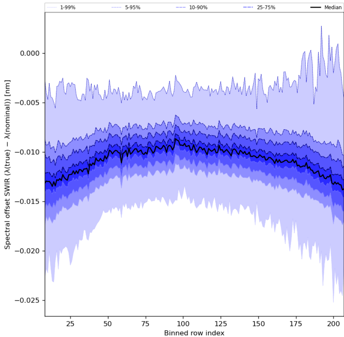
Figure 38: Along track statistics of “Spectral offset SWIR ( \lambda(\text{true}) - \lambda(\text{nominal}) )” for 2024-02-13 to 2024-02-15
