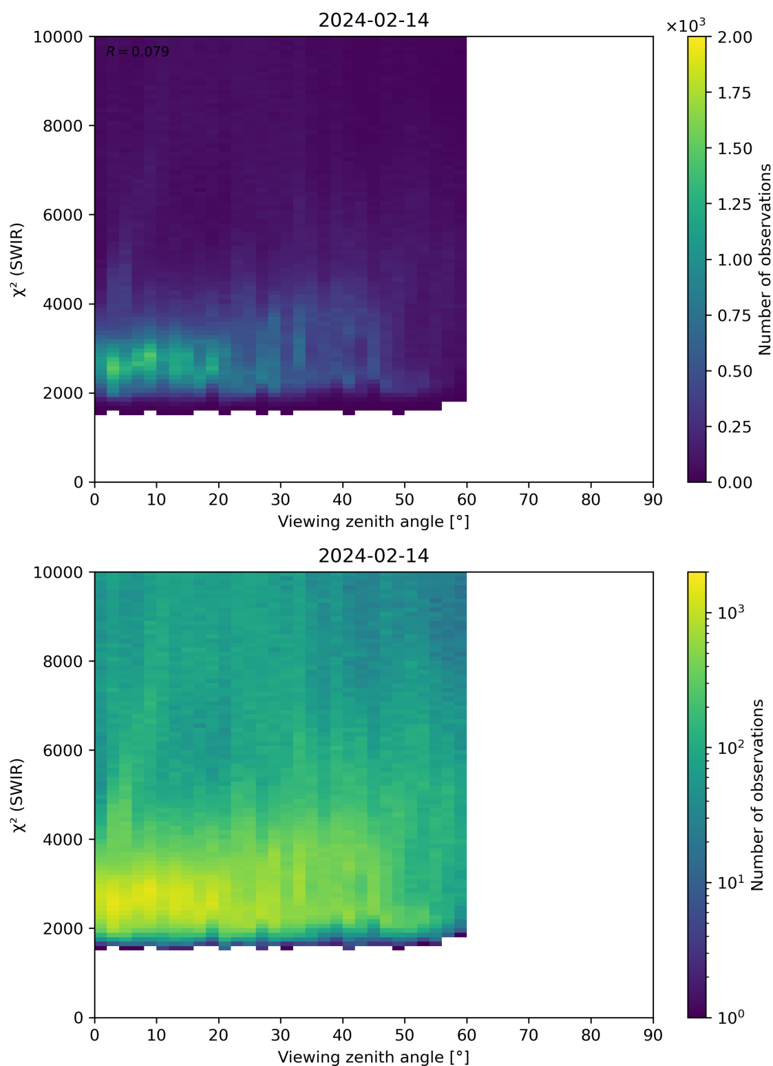
Figure 106: Scatter density plot of “Viewing zenith angle” against “ \chi^2 (SWIR)” for 2024-02-13 to 2024-02-15.
