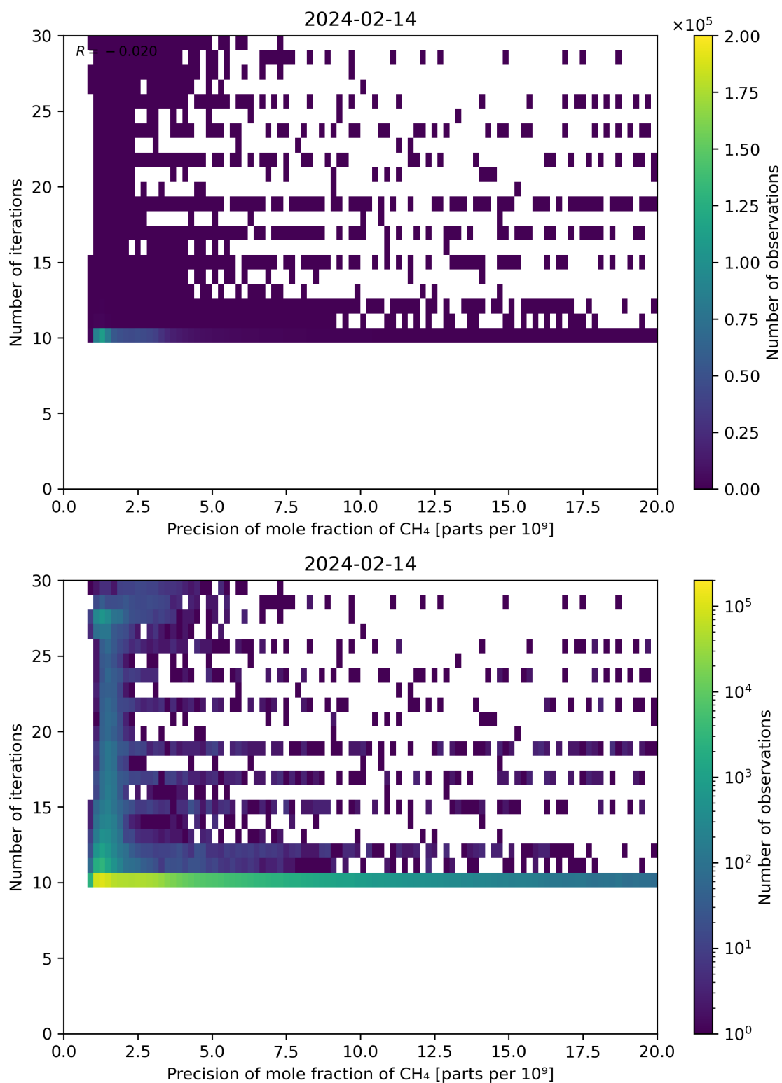
Figure 83: Scatter density plot of “Precision of mole fraction of CH 4 ” against “Number of iterations” for 2024-02-13 to 2024-02-15.
