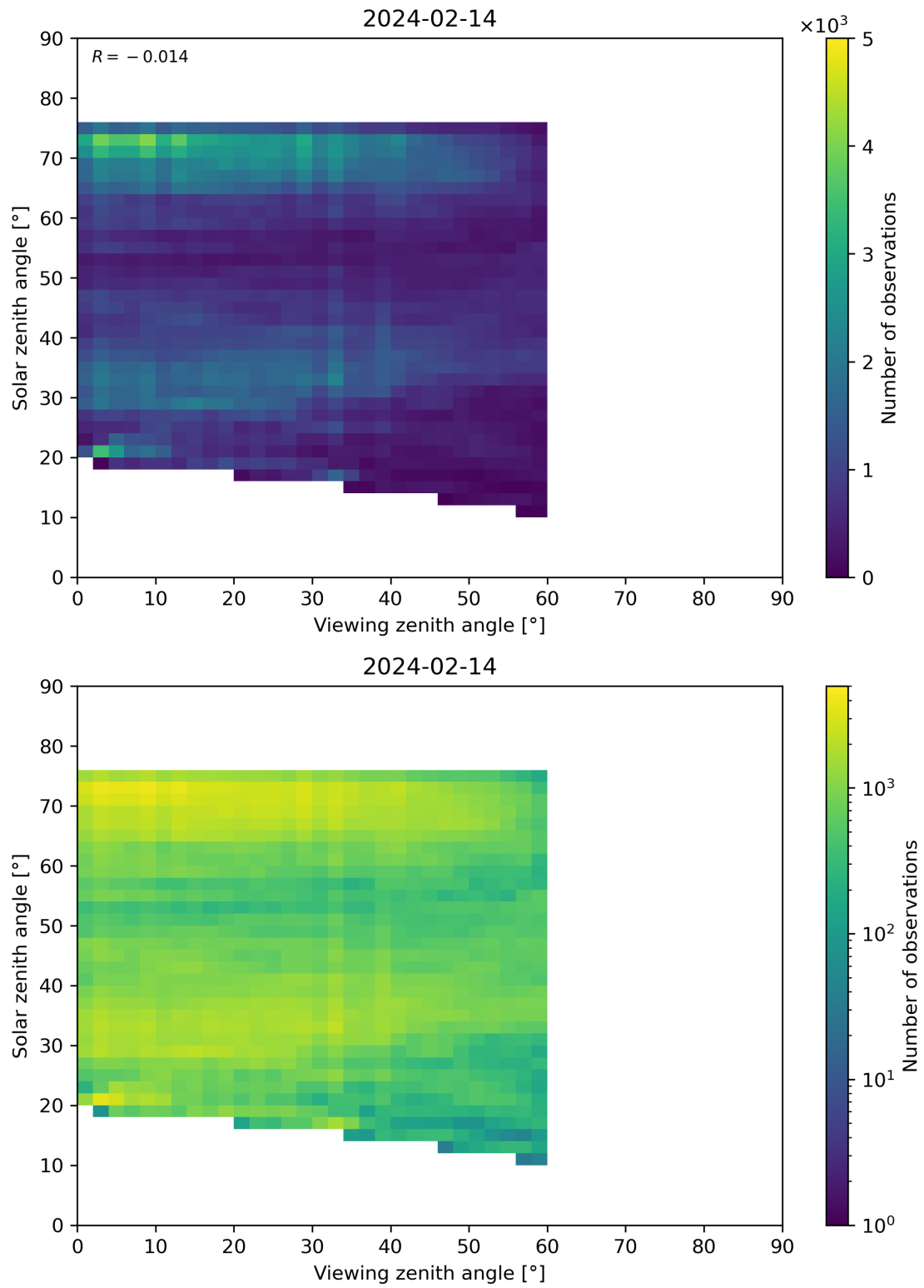
Figure 115: Scatter density plot of “Viewing zenith angle” against “Solar zenith angle” for 2024-02-13 to 2024-02-15.
