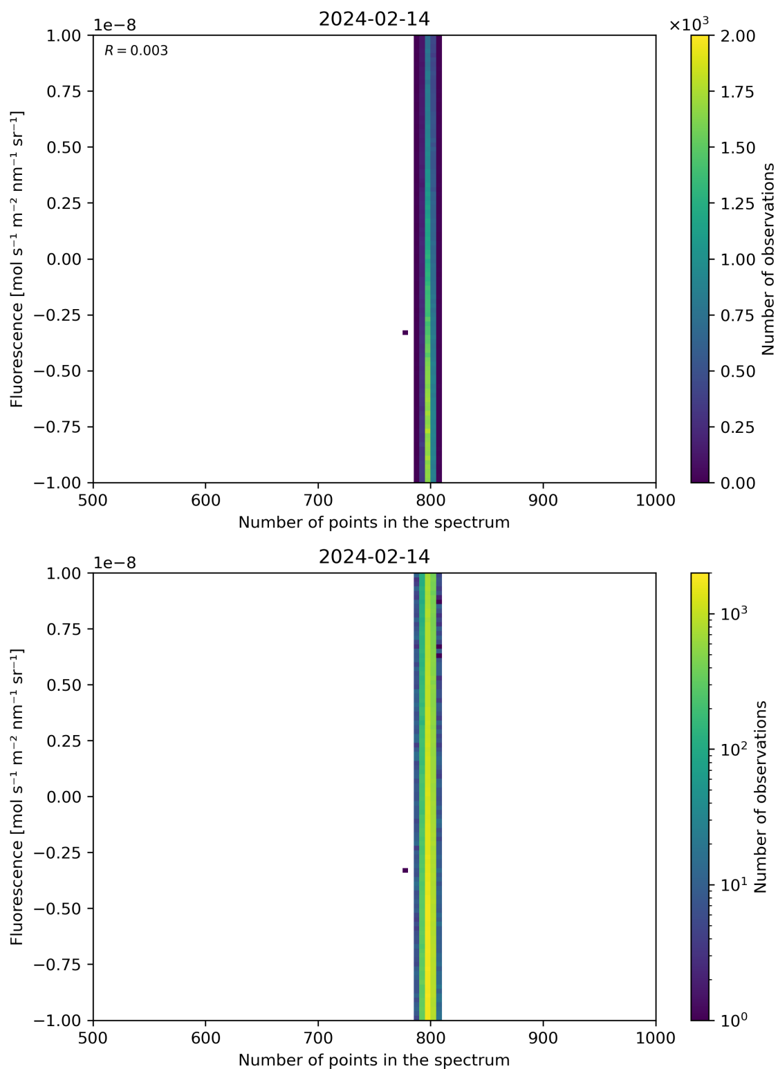
Figure 91: Scatter density plot of “Number of points in the spectrum” against “Fluorescence” for 2024-02-13 to 2024-02-15.
