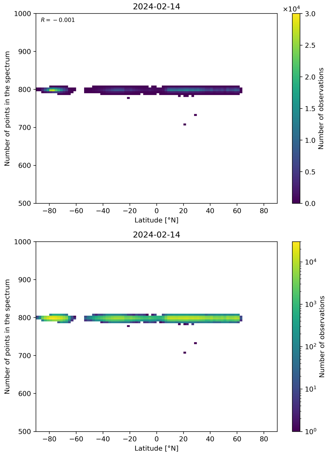
Figure 61: Scatter density plot of “Latitude” against “Number of points in the spectrum” for 2024-02-13 to 2024-02-15.
