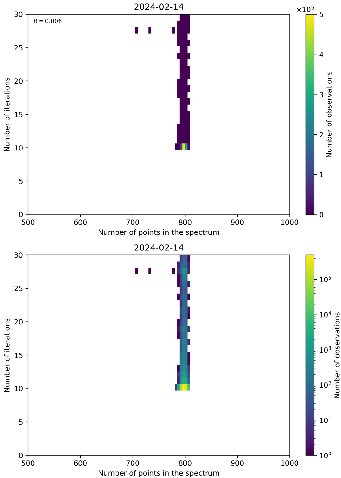
Figure 92: Scatter density plot of “Number of points in the spectrum” against “Number of iterations” for 2024-02-13 to 2024-02-15.
