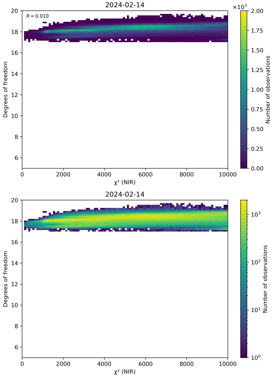
Figure 44: Scatter density plot of “ \chi^2 (NIR)” against “Degrees of freedom” for 2024-02-13 to 2024-02-15.
