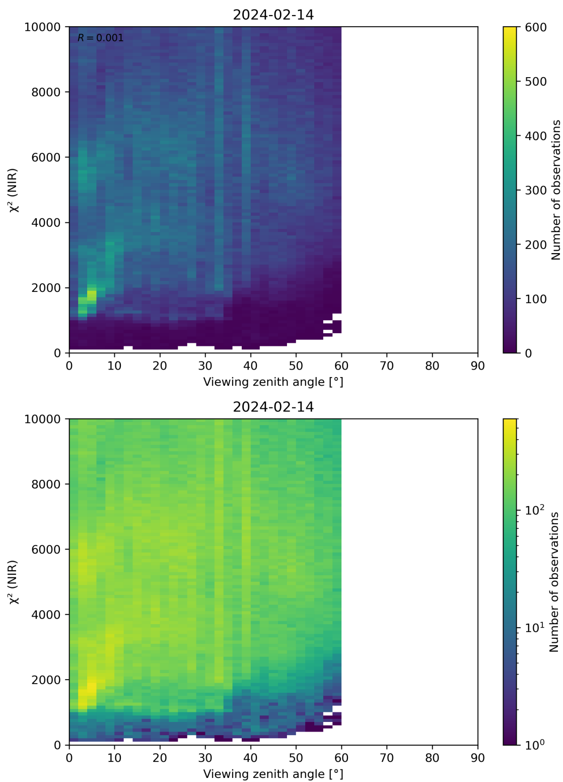
Figure 105: Scatter density plot of “Viewing zenith angle” against “ \chi^2 (NIR)” for 2024-02-13 to 2024-02-15.
