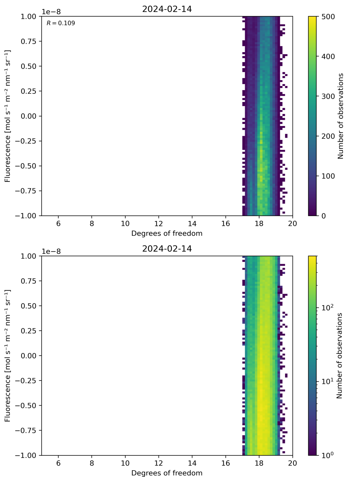
Figure 51: Scatter density plot of “Degrees of freedom” against “Fluorescence” for 2024-02-13 to 2024-02-15.
