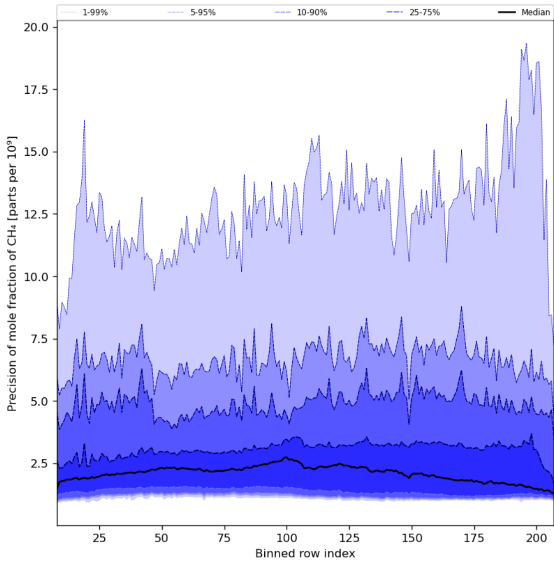
Figure 35: Along track statistics of “Precision of mole fraction of CH 4 ” for 2024-02-13 to 2024-02-15
