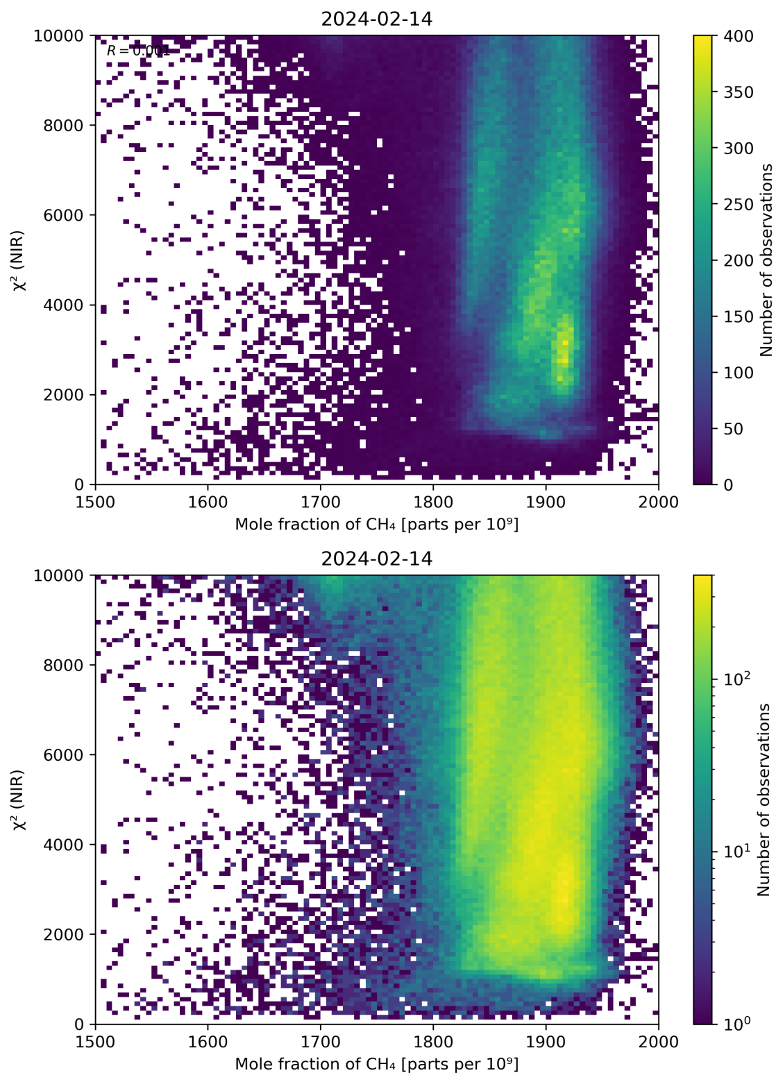
Figure 70: Scatter density plot of “Mole fraction of \text{CH}_4 ” against “ \chi^2 (NIR)” for 2024-02-13 to 2024-02-15.
