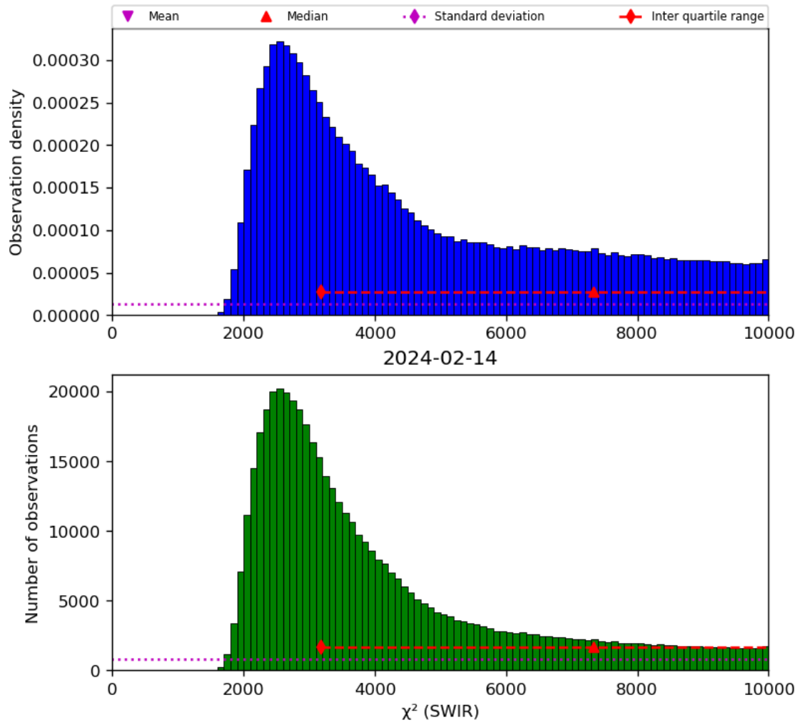
Figure 28: Histogram of “ \chi^2 (SWIR)” for 2024-02-13 to 2024-02-15
