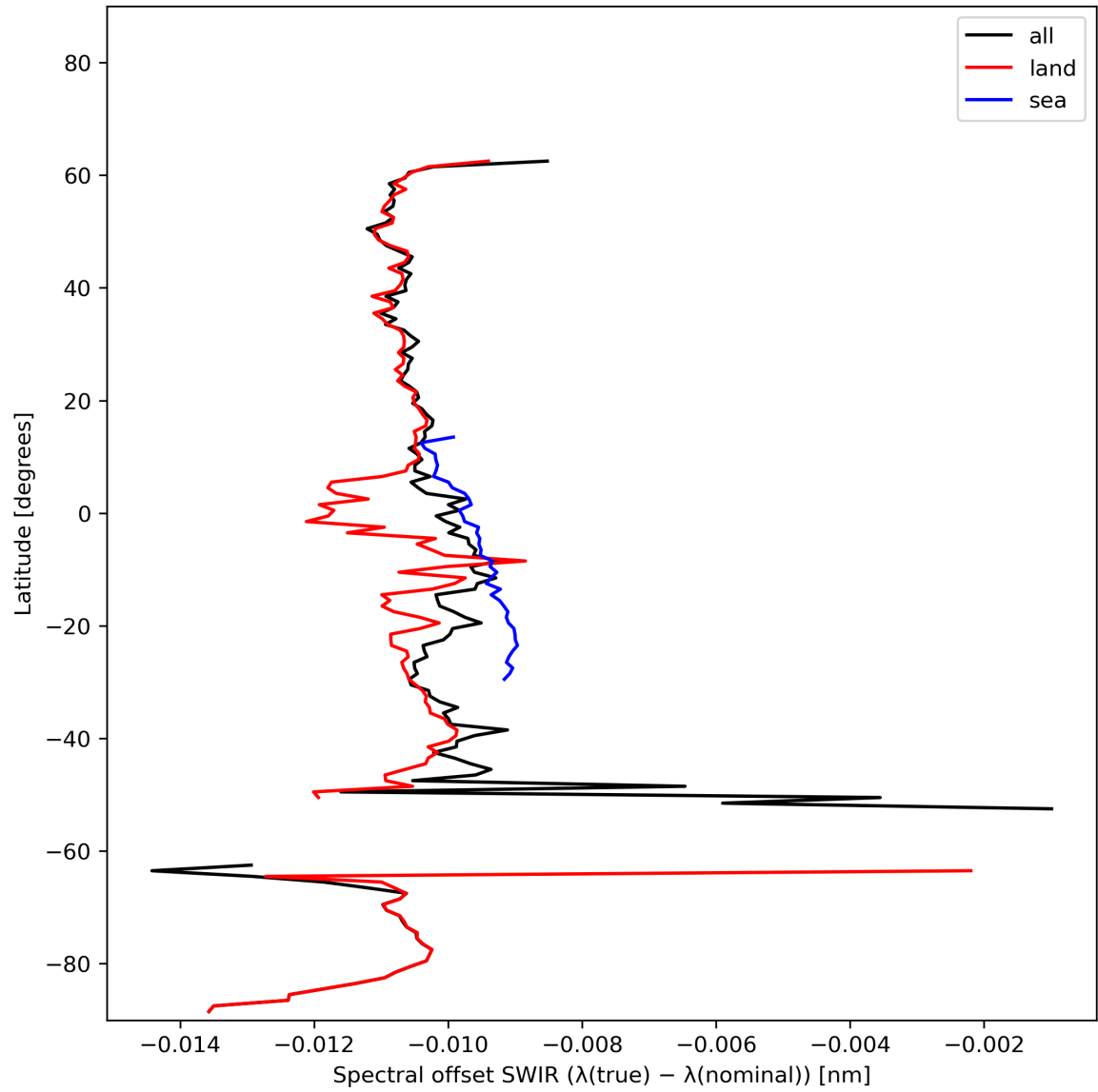
Figure 16: Zonal average of “Spectral offset SWIR ( \lambda(\text{true}) - \lambda(\text{nominal}) )” for 2024-02-13 to 2024-02-15.
