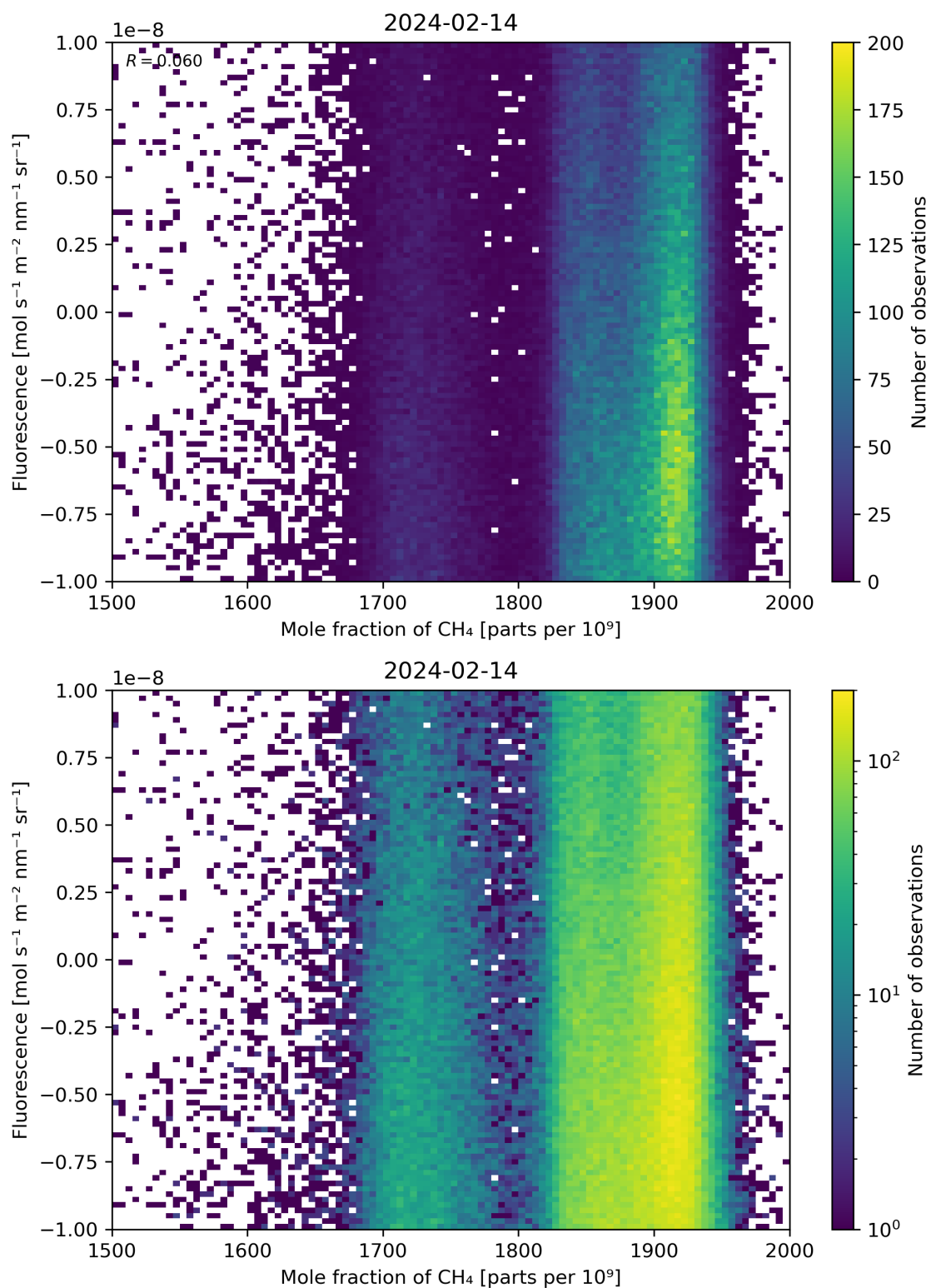
Figure 73: Scatter density plot of “Mole fraction of \text{CH}_4 ” against “Fluorescence” for 2024-02-13 to 2024-02-15.
