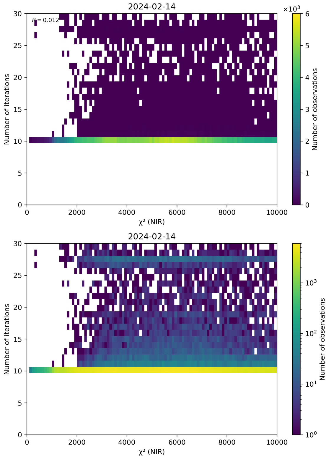
Figure 46: Scatter density plot of “ \chi^2 (NIR)” against “Number of iterations” for 2024-02-13 to 2024-02-15.
