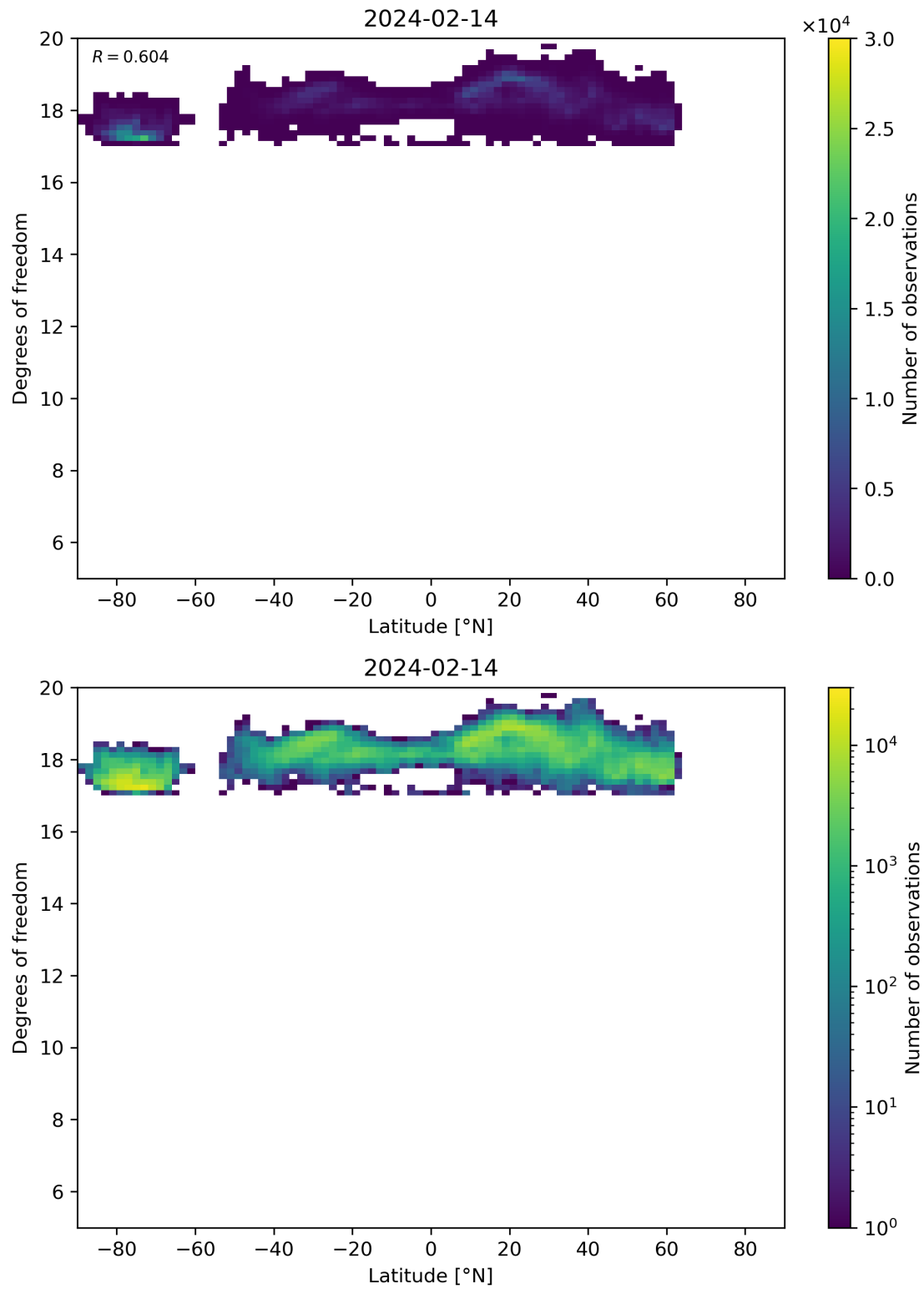
Figure 55: Scatter density plot of “Latitude” against “Degrees of freedom” for 2024-02-13 to 2024-02-15.
