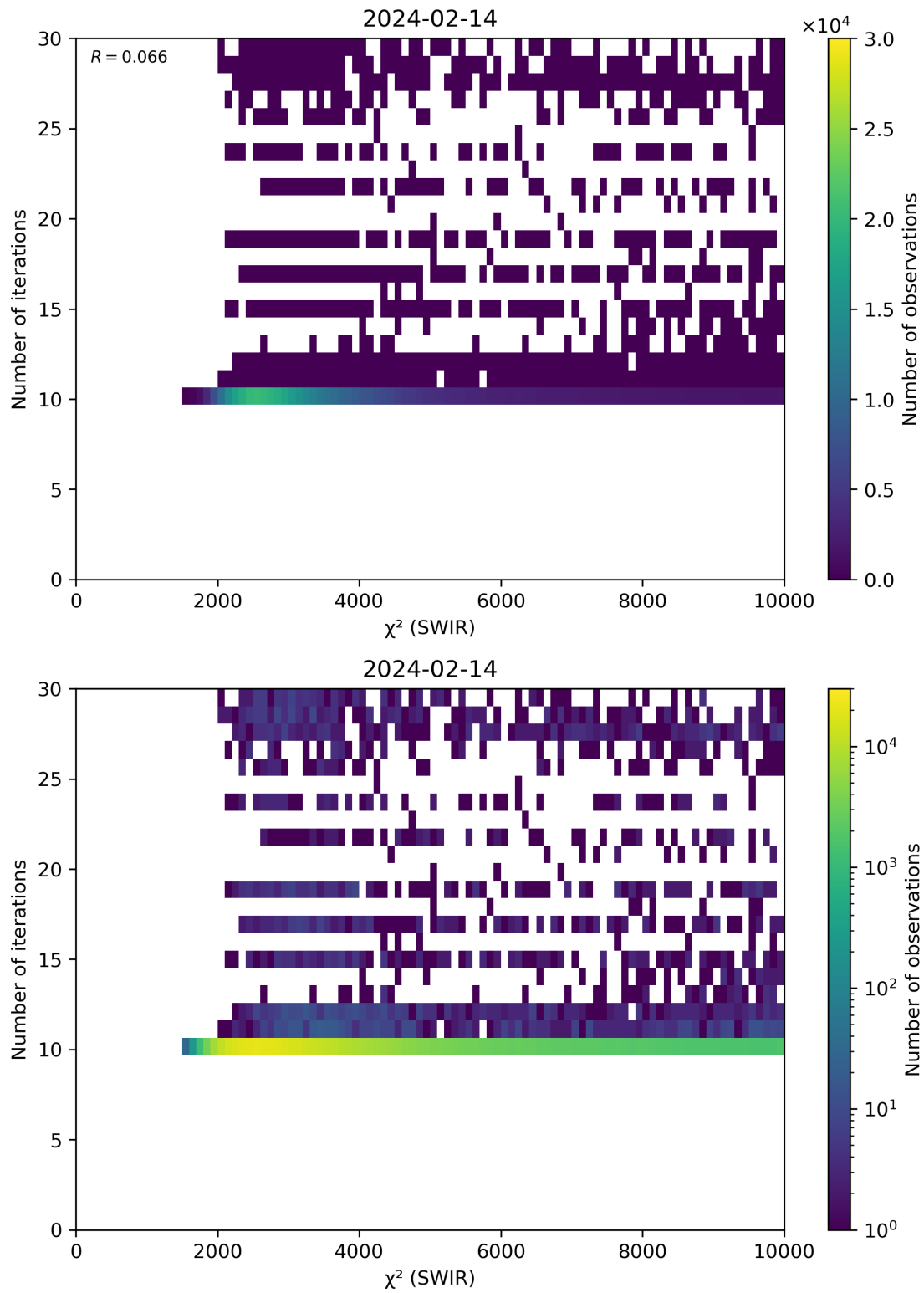
Figure 50: Scatter density plot of “ \chi^2 (SWIR)” against “Number of iterations” for 2024-02-13 to 2024-02-15.
