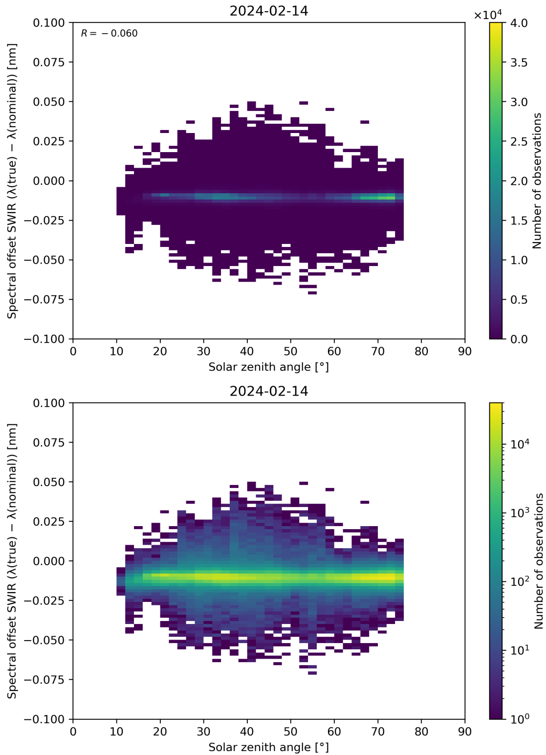
Figure 104: Scatter density plot of “Solar zenith angle” against “Spectral offset SWIR ( \lambda(\text{true}) - \lambda(\text{nominal}) )” for 2024-02-13 to 2024-02-15.
