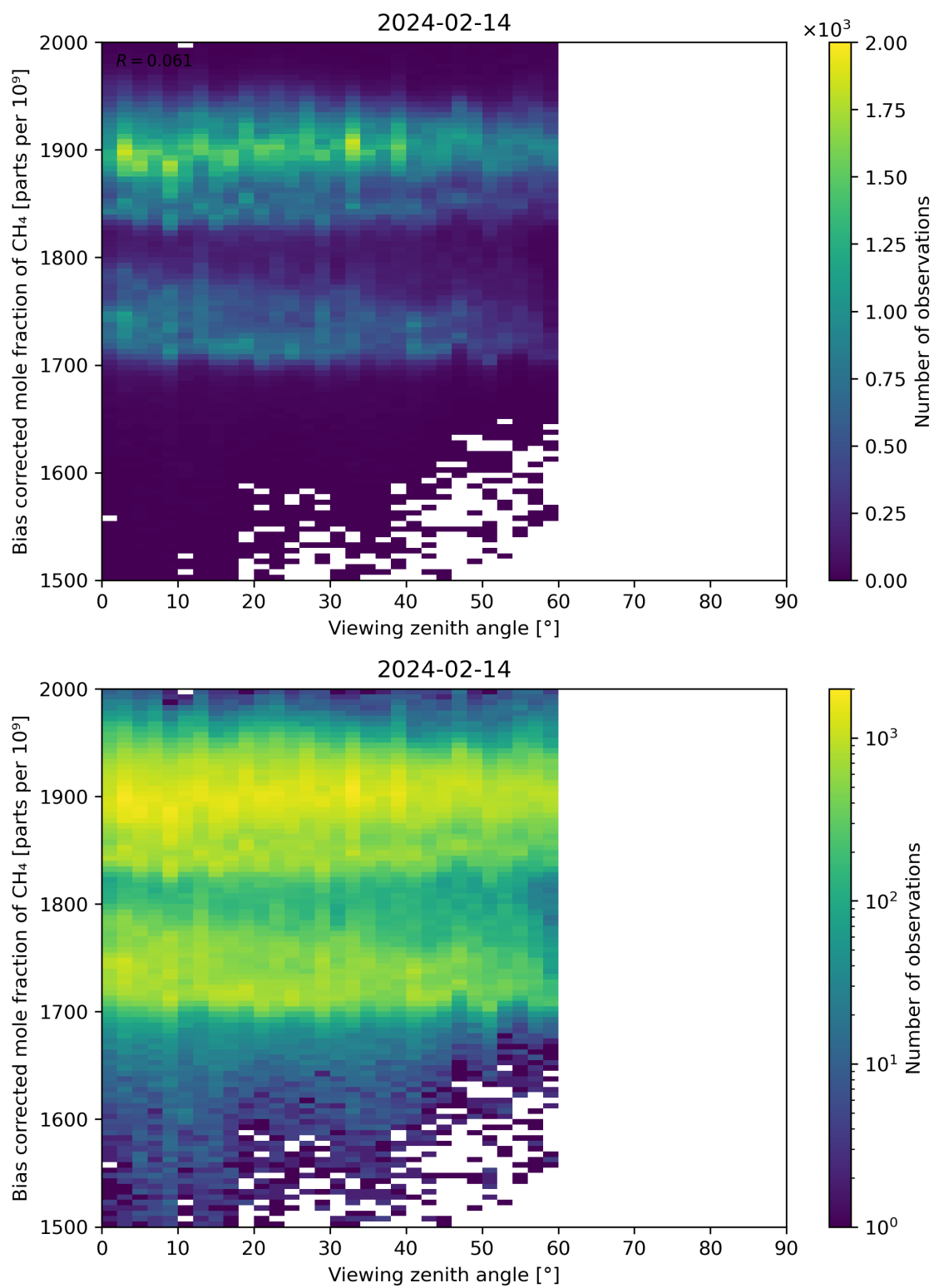
Figure 111: Scatter density plot of “Viewing zenith angle” against “Bias corrected mole fraction of \text{CH}_4 ” for 2024-02-13 to 2024-02-15.
