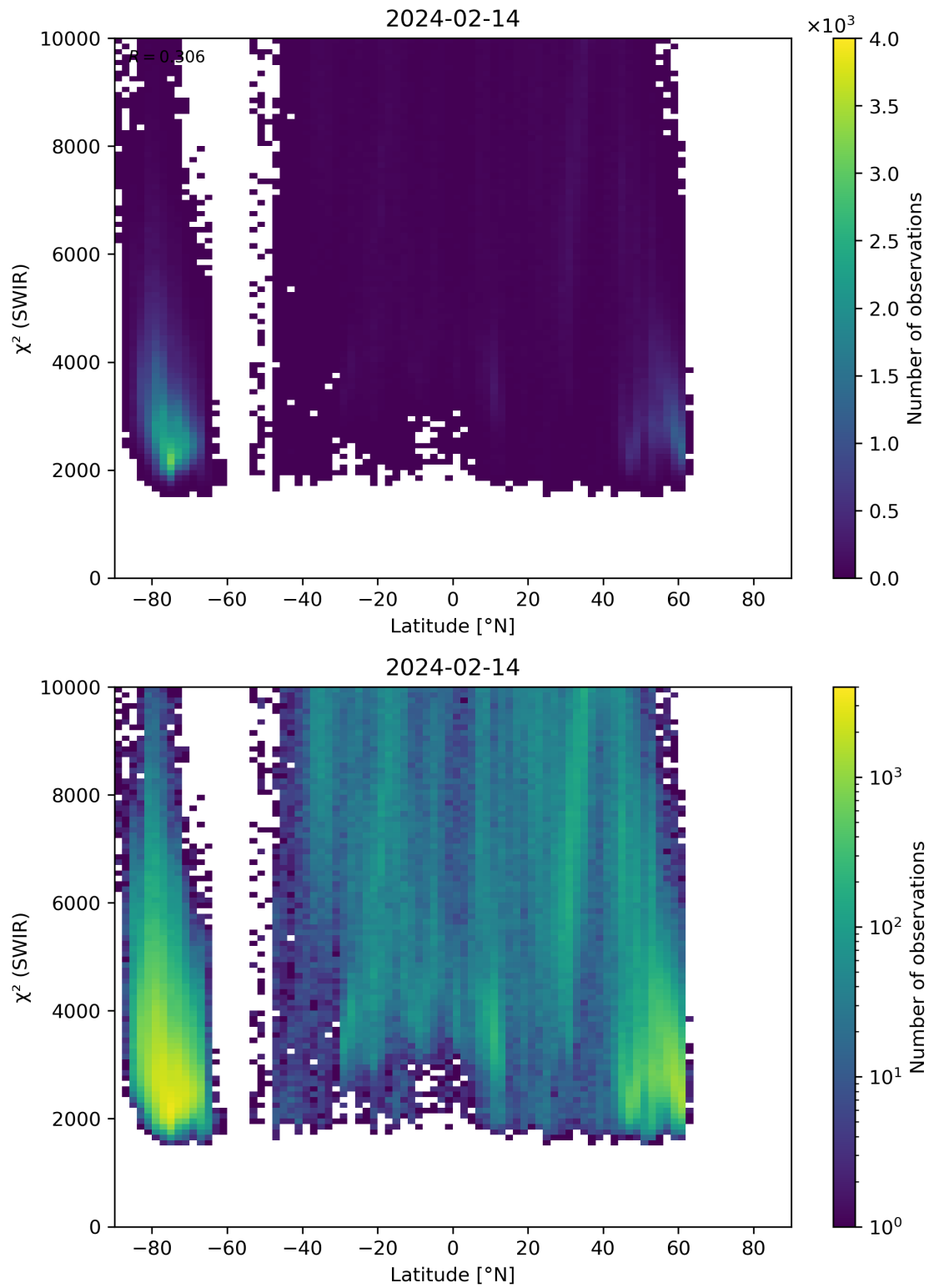
Figure 54: Scatter density plot of “Latitude” against “ \chi^2 (SWIR)” for 2024-02-13 to 2024-02-15.
