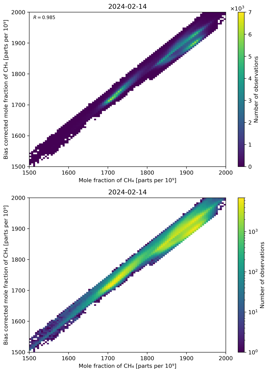
Figure 74: Scatter density plot of “Mole fraction of CH 4 ” against “Bias corrected mole fraction of CH 4 ” for 2024-02-13 to 2024-02-15.
