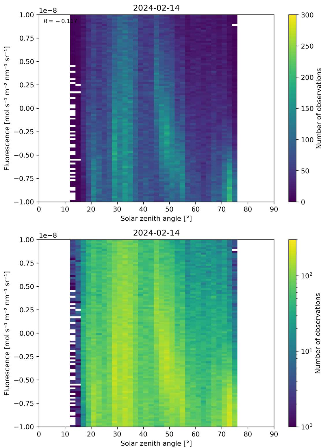
Figure 97: Scatter density plot of “Solar zenith angle” against “Fluorescence” for 2024-02-13 to 2024-02-15.
