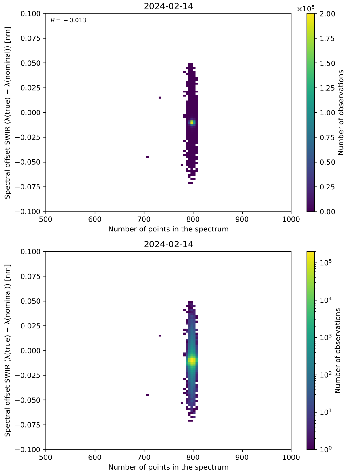
Figure 93: Scatter density plot of “Number of points in the spectrum” against “Spectral offset SWIR ( \lambda(\text{true}) - \lambda(\text{nominal}) )” for 2024-02-13 to 2024-02-15.
