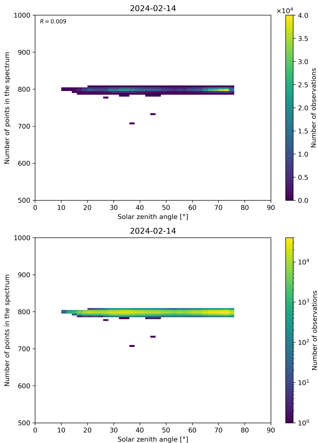
Figure 103: Scatter density plot of “Solar zenith angle” against “Number of points in the spectrum” for 2024-02-13 to 2024-02-15.
