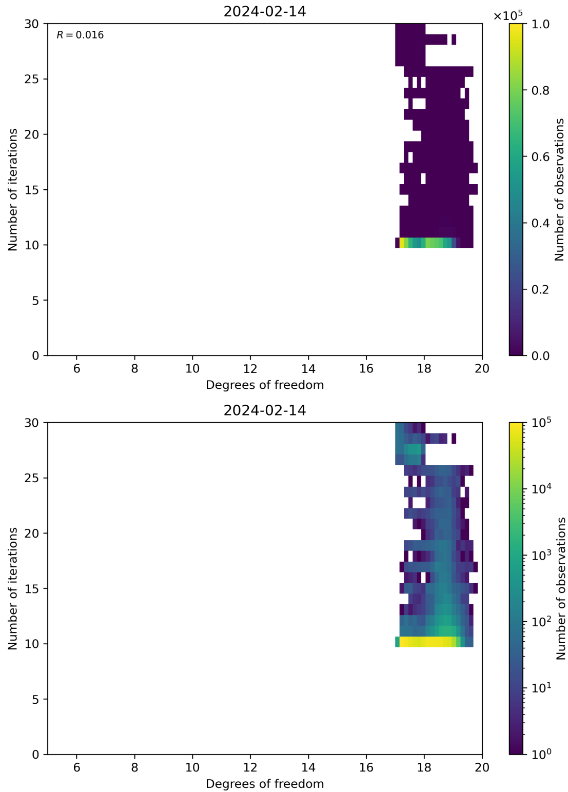
Figure 52: Scatter density plot of “Degrees of freedom” against “Number of iterations” for 2024-02-13 to 2024-02-15.
