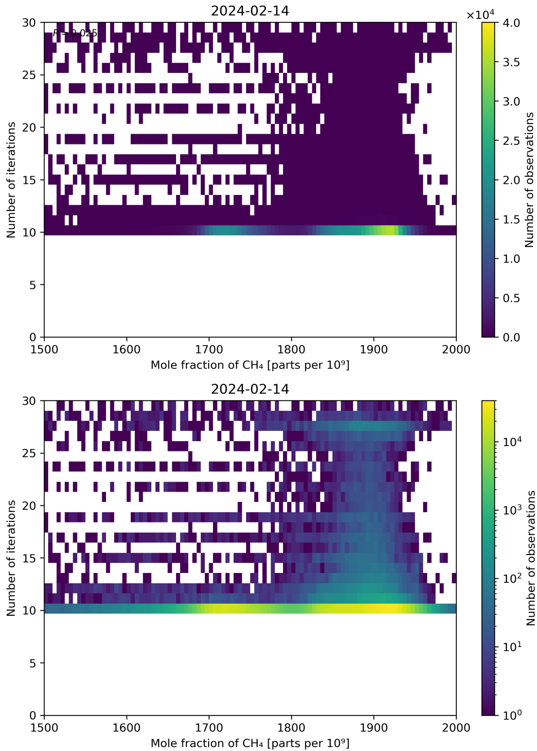
Figure 76: Scatter density plot of “Mole fraction of CH 4 ” against “Number of iterations” for 2024-02-13 to 2024-02-15.
