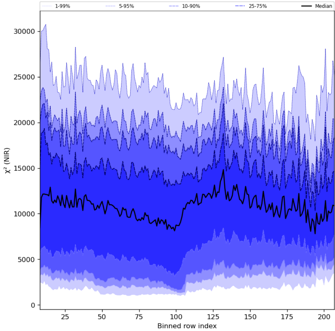
Figure 40: Along track statistics of “ \chi^2 (NIR)” for 2024-02-13 to 2024-02-15
