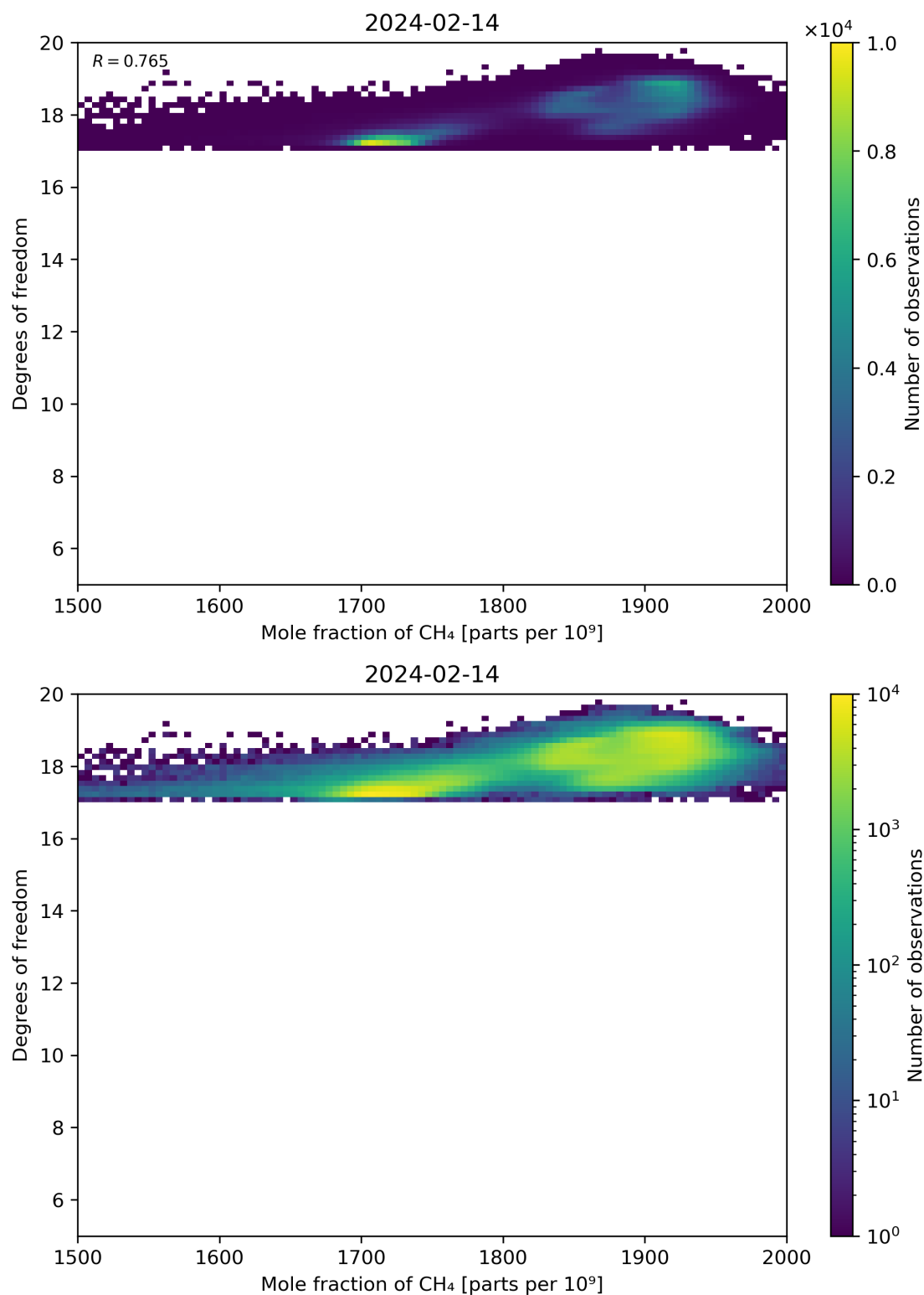
Figure 72: Scatter density plot of “Mole fraction of CH 4 ” against “Degrees of freedom” for 2024-02-13 to 2024-02-15.
