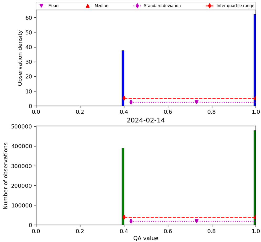
Figure 22: Histogram of “QA value” for 2024-02-13 to 2024-02-15
