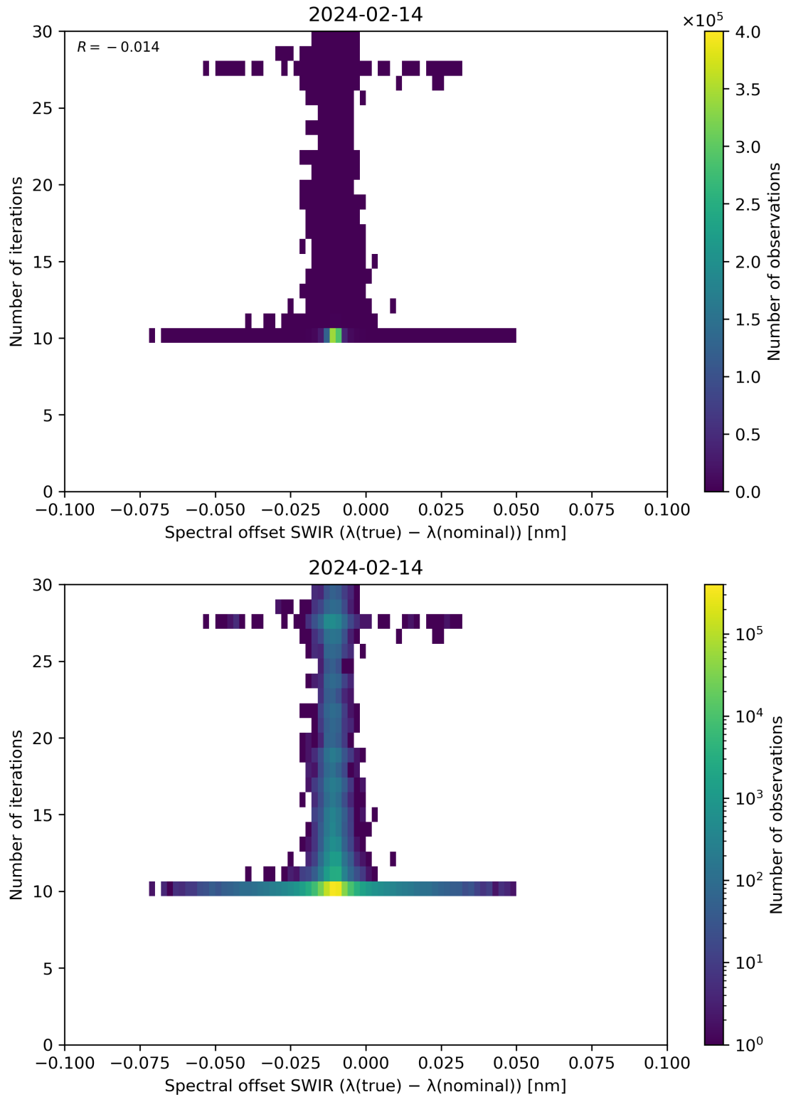
Figure 121: Scatter density plot of “Spectral offset SWIR ( \lambda(\text{true}) - \lambda(\text{nominal}) )” against “Number of iterations” for 2024-02-13 to 2024-02-15.
