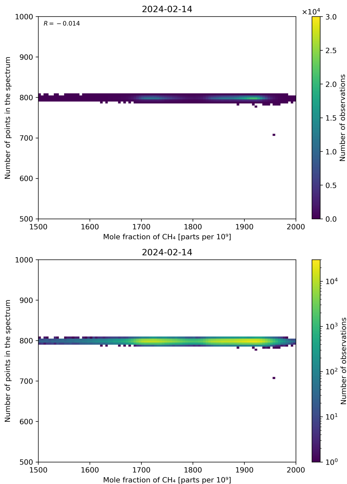
Figure 77: Scatter density plot of “Mole fraction of CH 4 ” against “Number of points in the spectrum” for 2024-02-13 to 2024-02-15.
