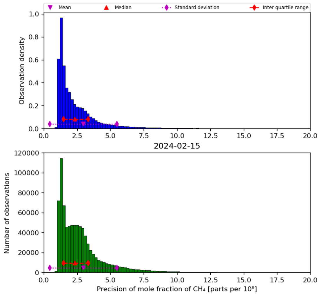
Figure 24: Histogram of “Precision of mole fraction of CH 4 ” for 2024-02-14 to 2024-02-16
