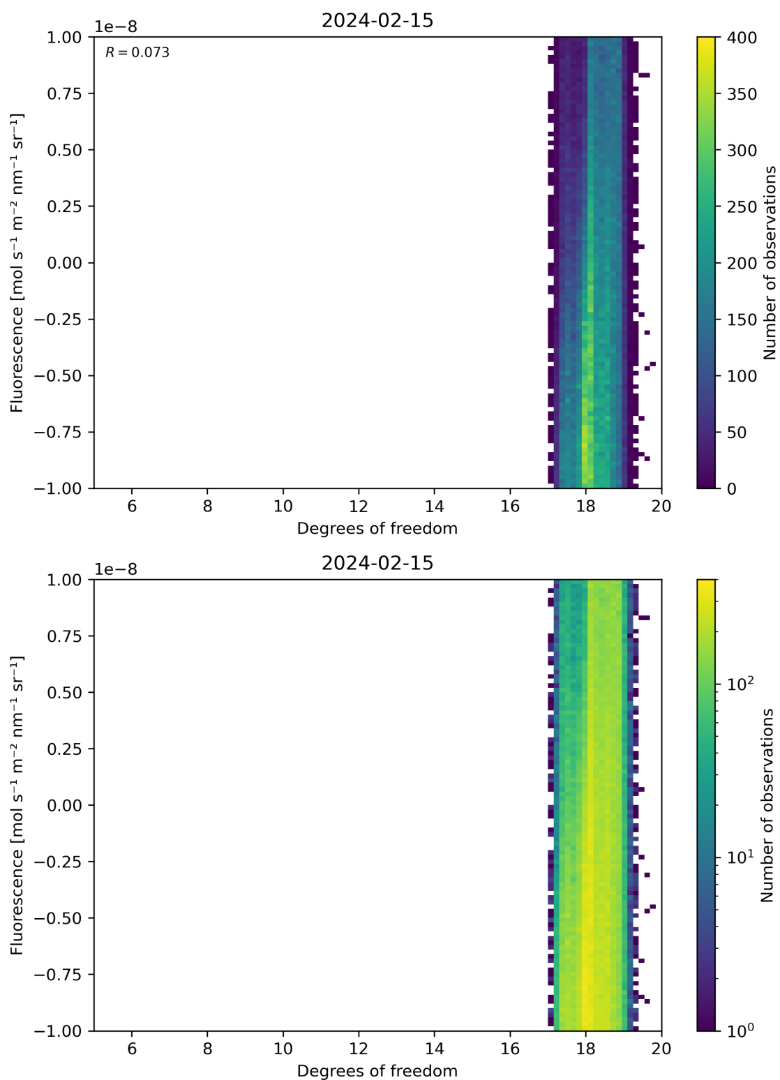
Figure 51: Scatter density plot of “Degrees of freedom” against “Fluorescence” for 2024-02-14 to 2024-02-16.
