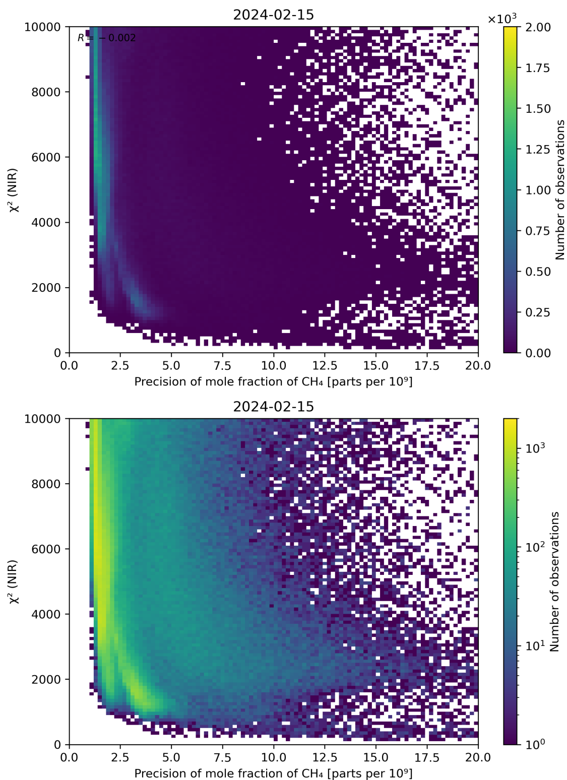
Figure 78: Scatter density plot of “Precision of mole fraction of CH 4 ” against “ \chi^2 (NIR)” for 2024-02-14 to 2024-02-16.
