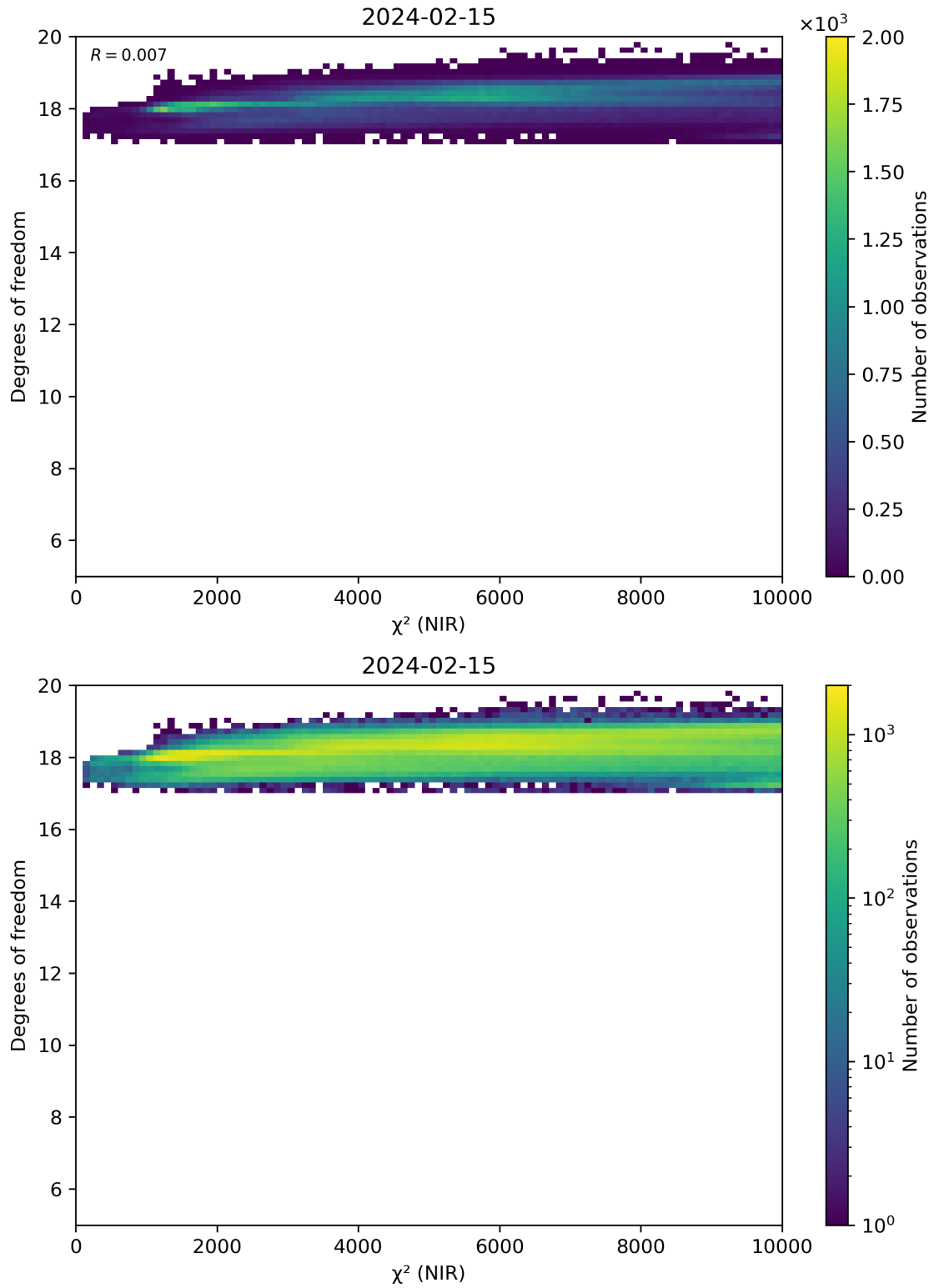
Figure 44: Scatter density plot of “ \chi^2 (NIR)” against “Degrees of freedom” for 2024-02-14 to 2024-02-16.
