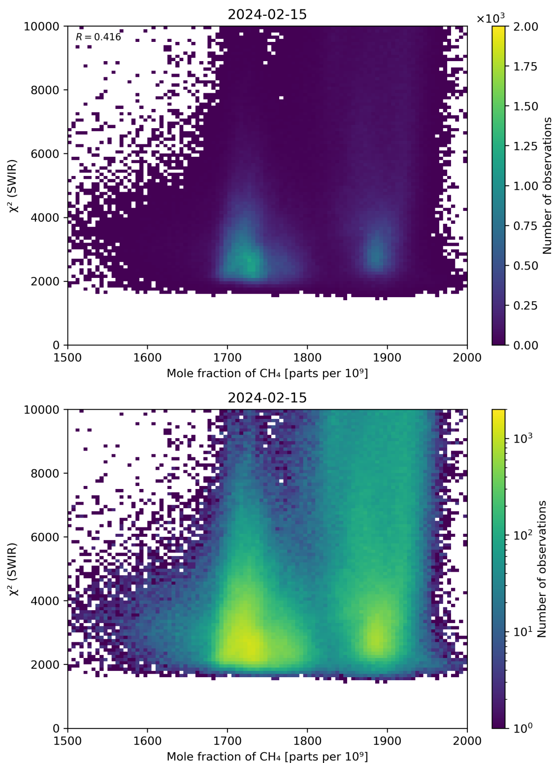
Figure 71: Scatter density plot of “Mole fraction of \text{CH}_4 ” against “ \chi^2 (SWIR)” for 2024-02-14 to 2024-02-16.
