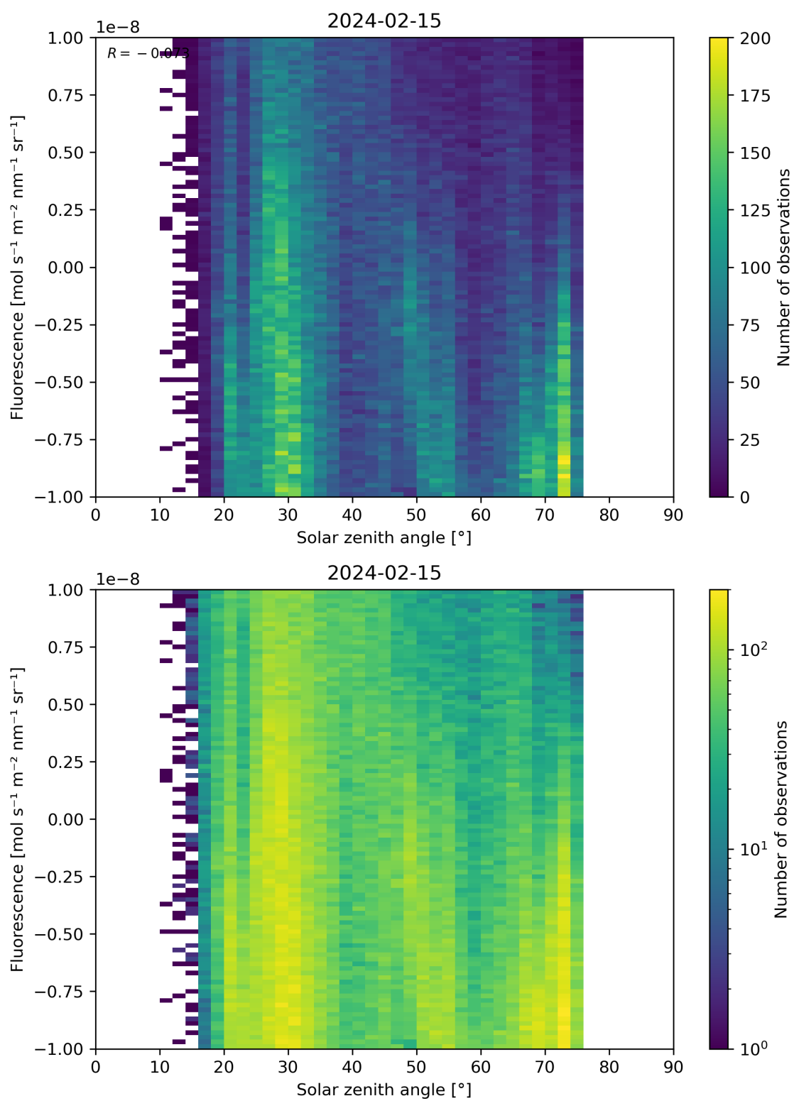
Figure 97: Scatter density plot of “Solar zenith angle” against “Fluorescence” for 2024-02-14 to 2024-02-16.
