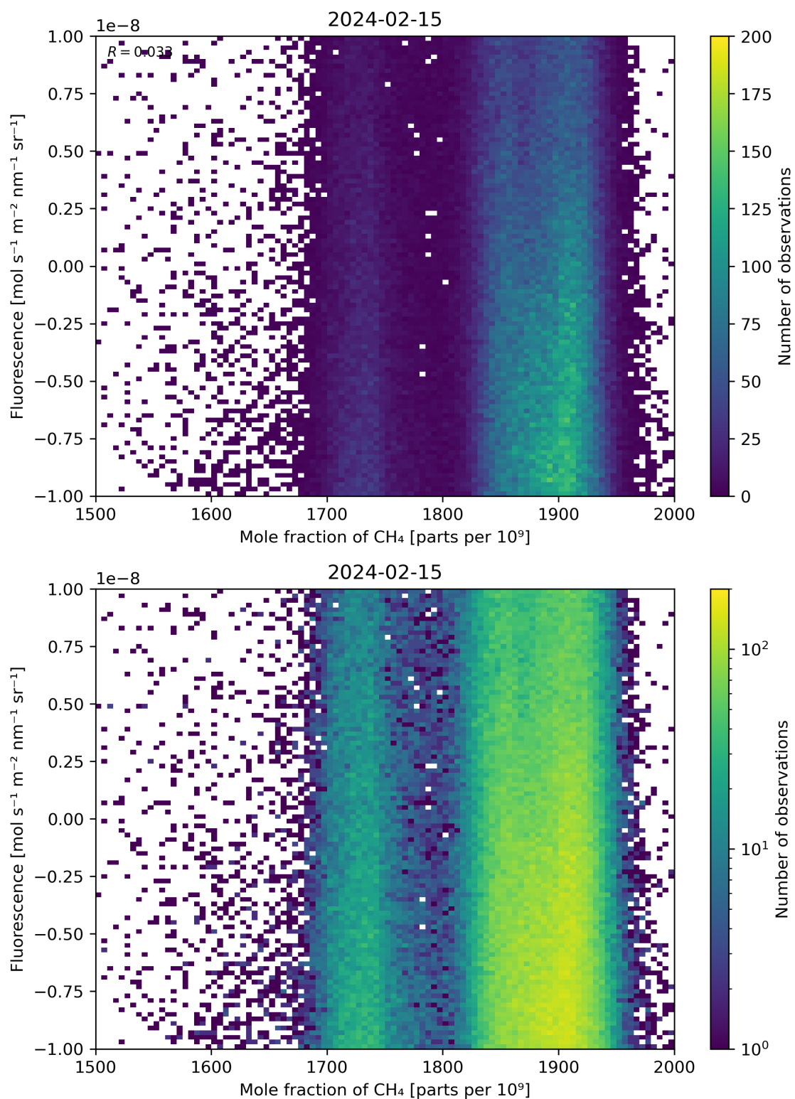
Figure 73: Scatter density plot of “Mole fraction of CH 4 ” against “Fluorescence” for 2024-02-14 to 2024-02-16.
