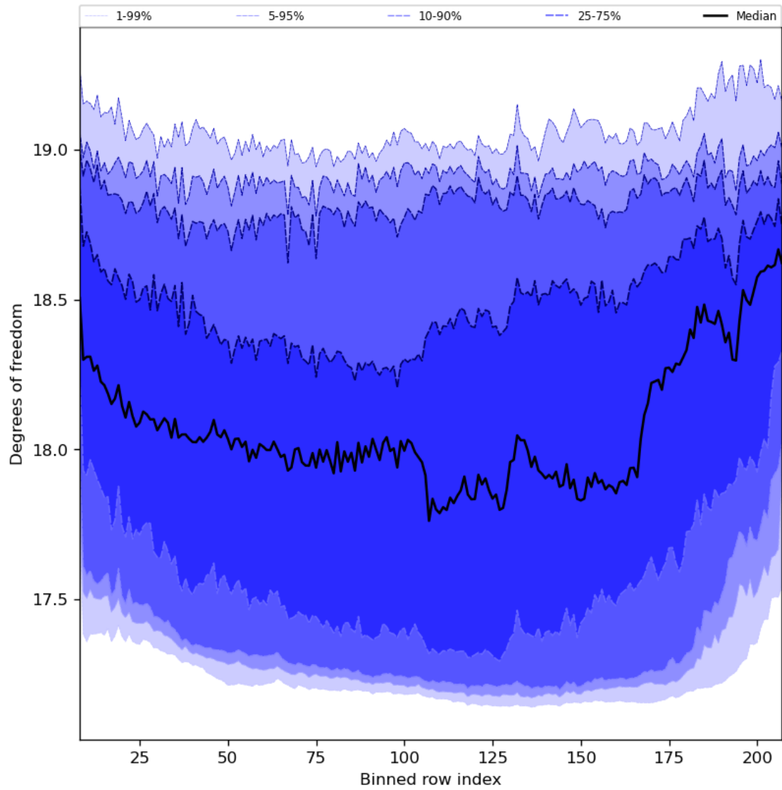
Figure 41: Along track statistics of “Degrees of freedom” for 2024-02-14 to 2024-02-16
