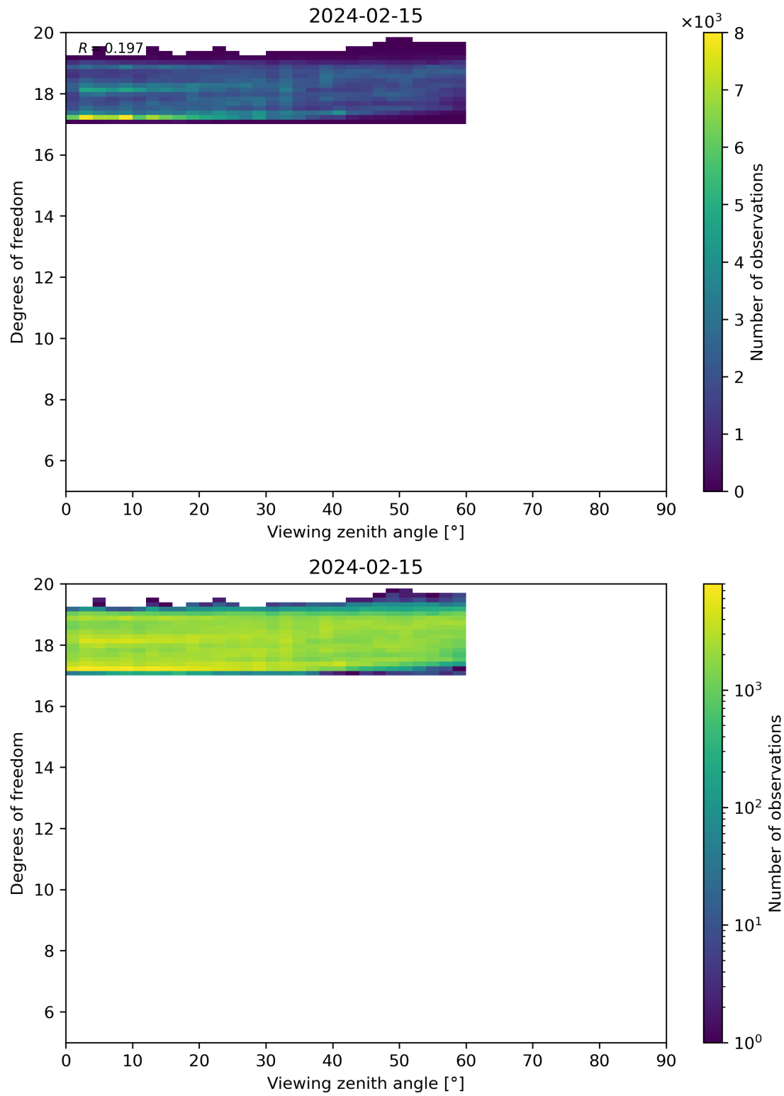
Figure 107: Scatter density plot of “Viewing zenith angle” against “Degrees of freedom” for 2024-02-14 to 2024-02-16.
