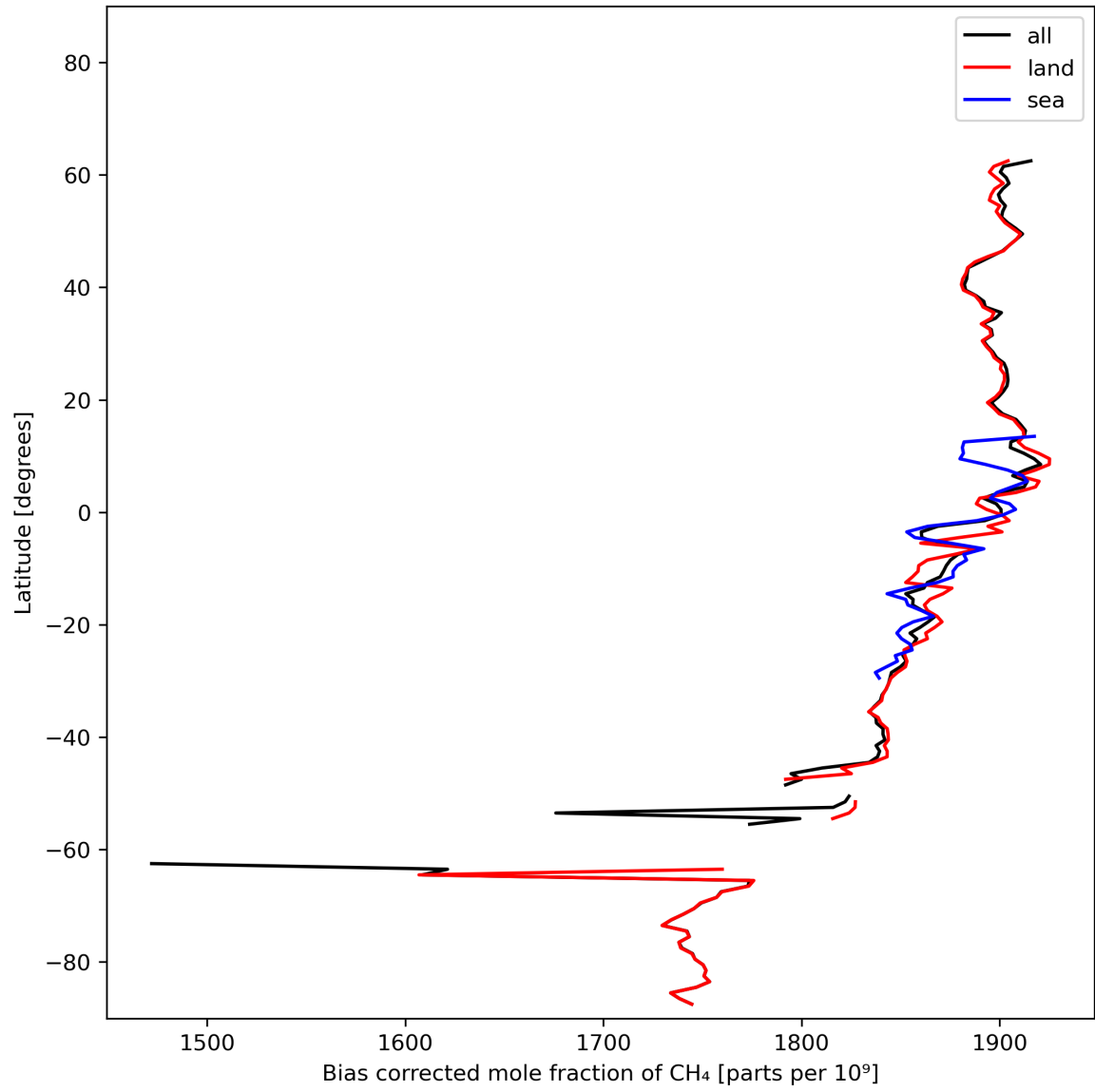
Figure 14: Zonal average of “Bias corrected mole fraction of CH 4 ” for 2024-02-14 to 2024-02-16.
