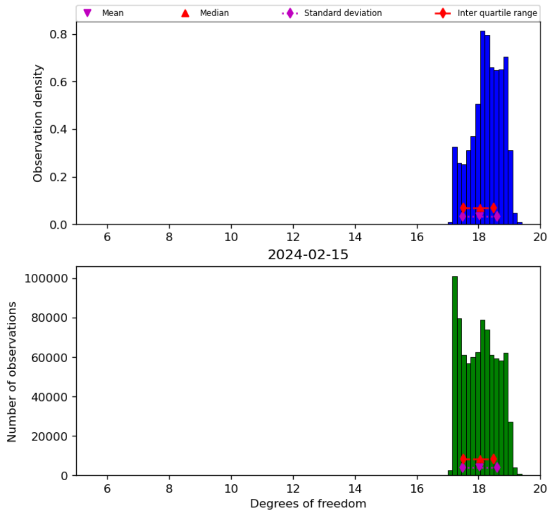
Figure 30: Histogram of “Degrees of freedom” for 2024-02-14 to 2024-02-16
