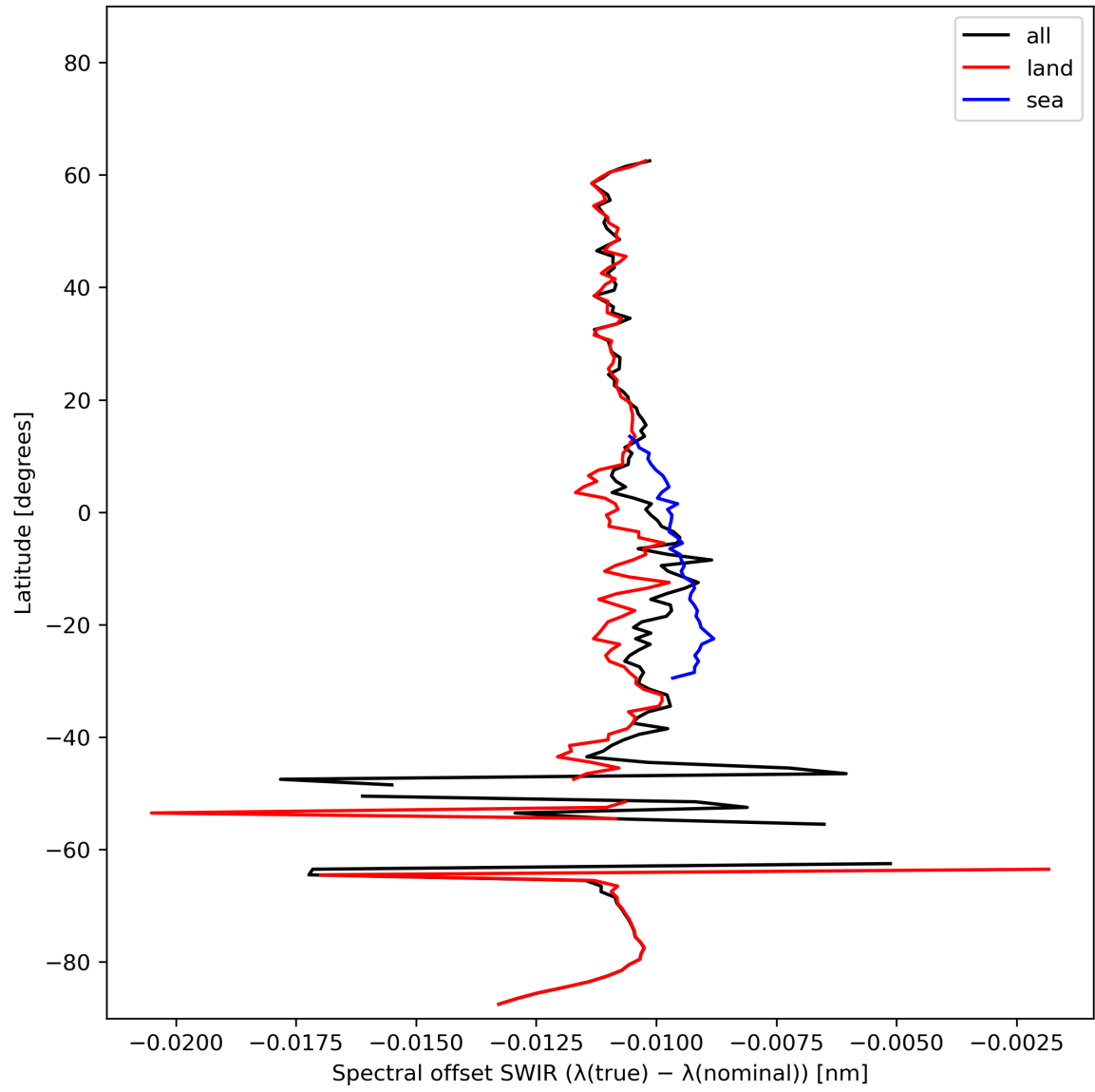
Figure 16: Zonal average of “Spectral offset SWIR ( \lambda(\text{true}) - \lambda(\text{nominal}) )” for 2024-02-14 to 2024-02-16.
