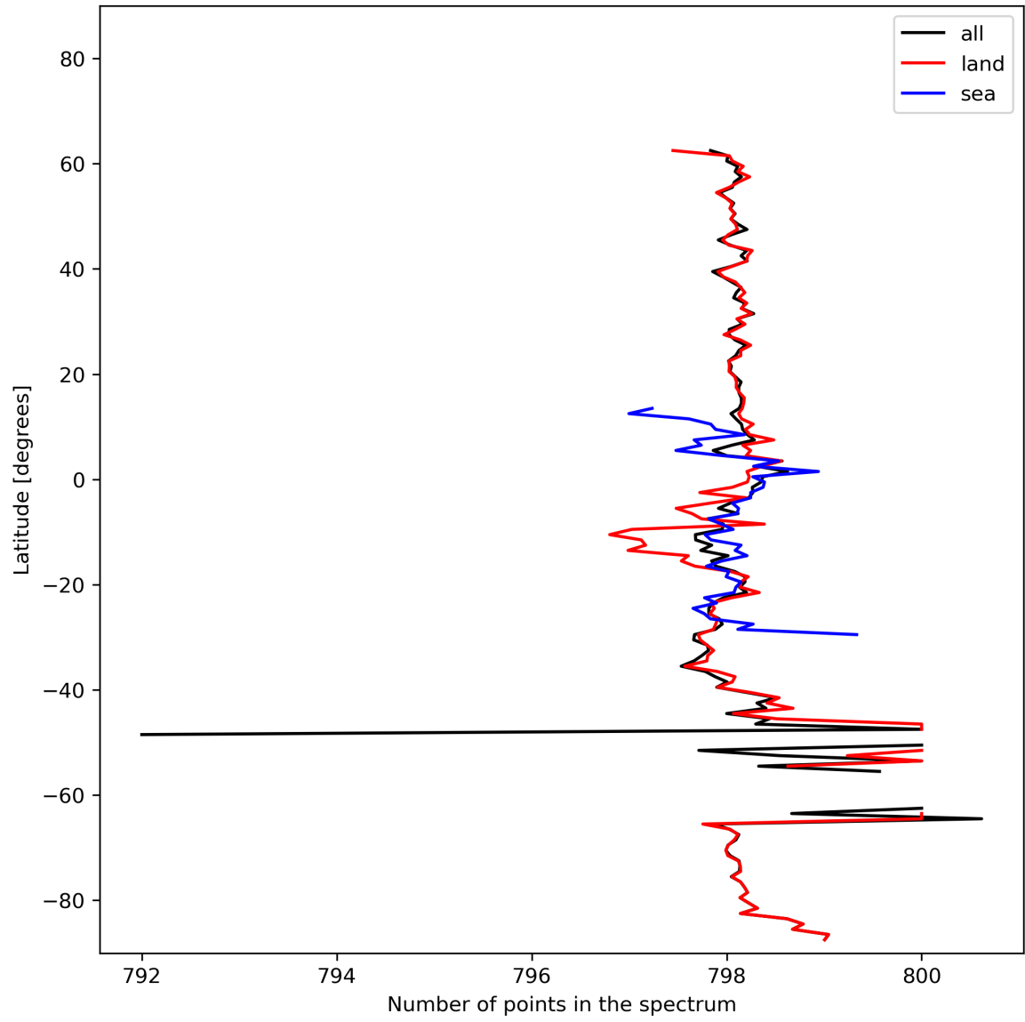
Figure 15: Zonal average of “Number of points in the spectrum” for 2024-02-14 to 2024-02-16.
