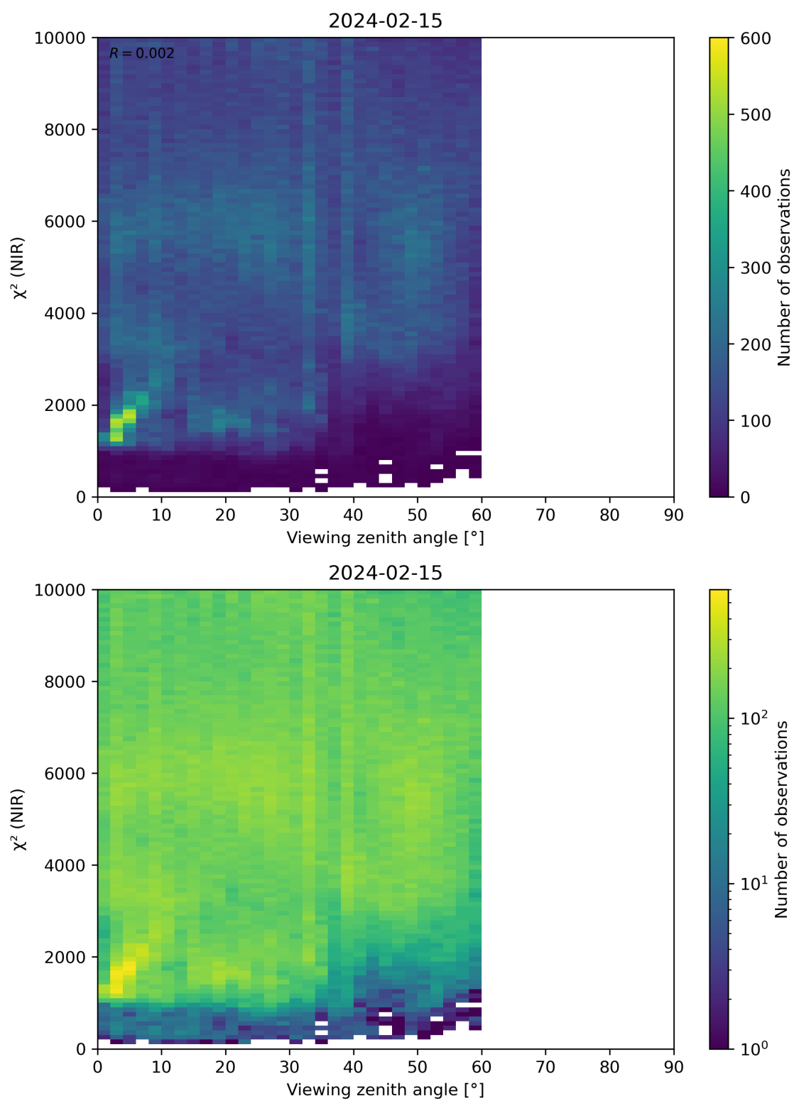
Figure 105: Scatter density plot of “Viewing zenith angle” against “ \chi^2 (NIR)” for 2024-02-14 to 2024-02-16.
