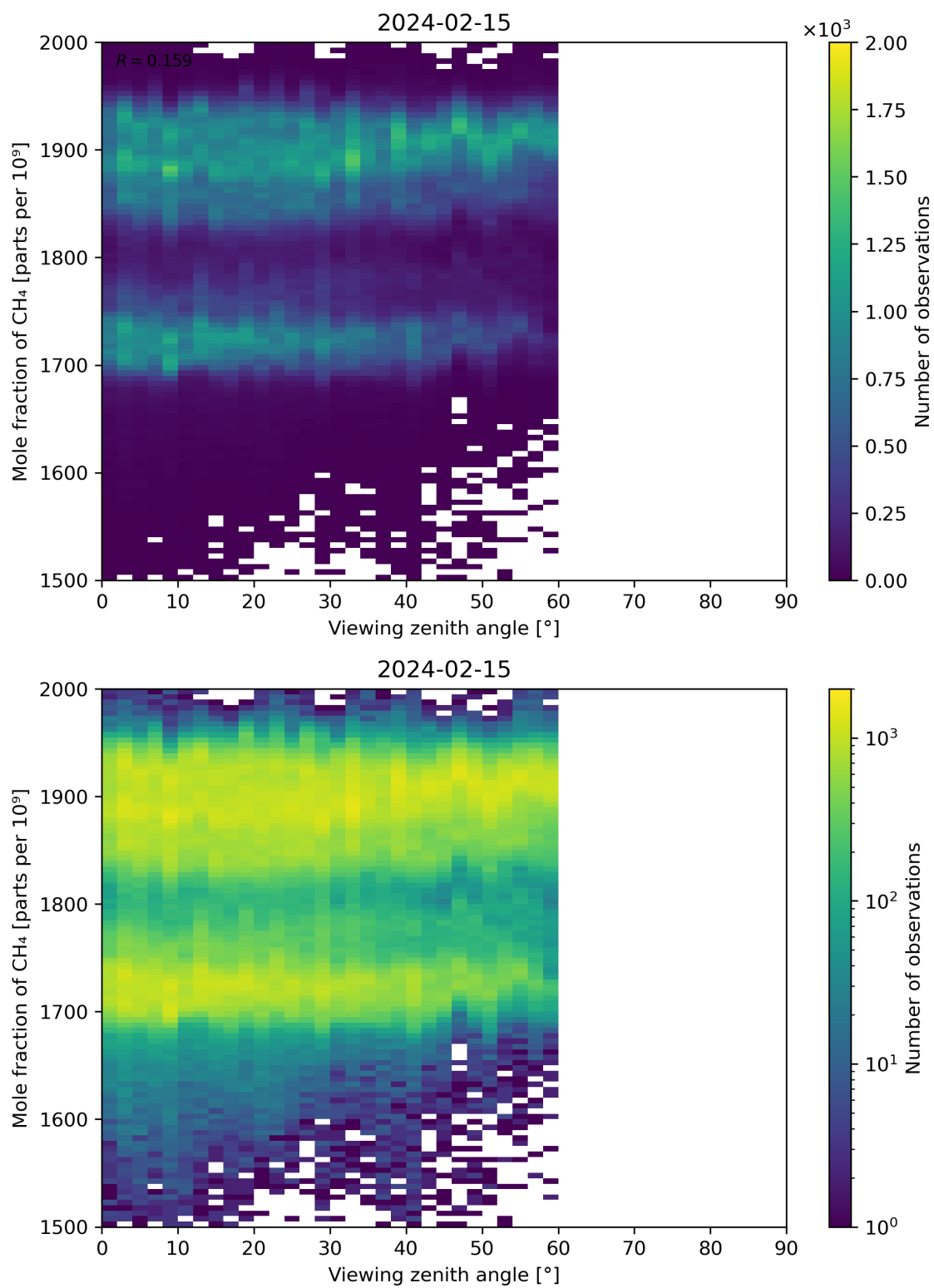
Figure 110: Scatter density plot of “Viewing zenith angle” against “Mole fraction of CH 4 ” for 2024-02-14 to 2024-02-16.
