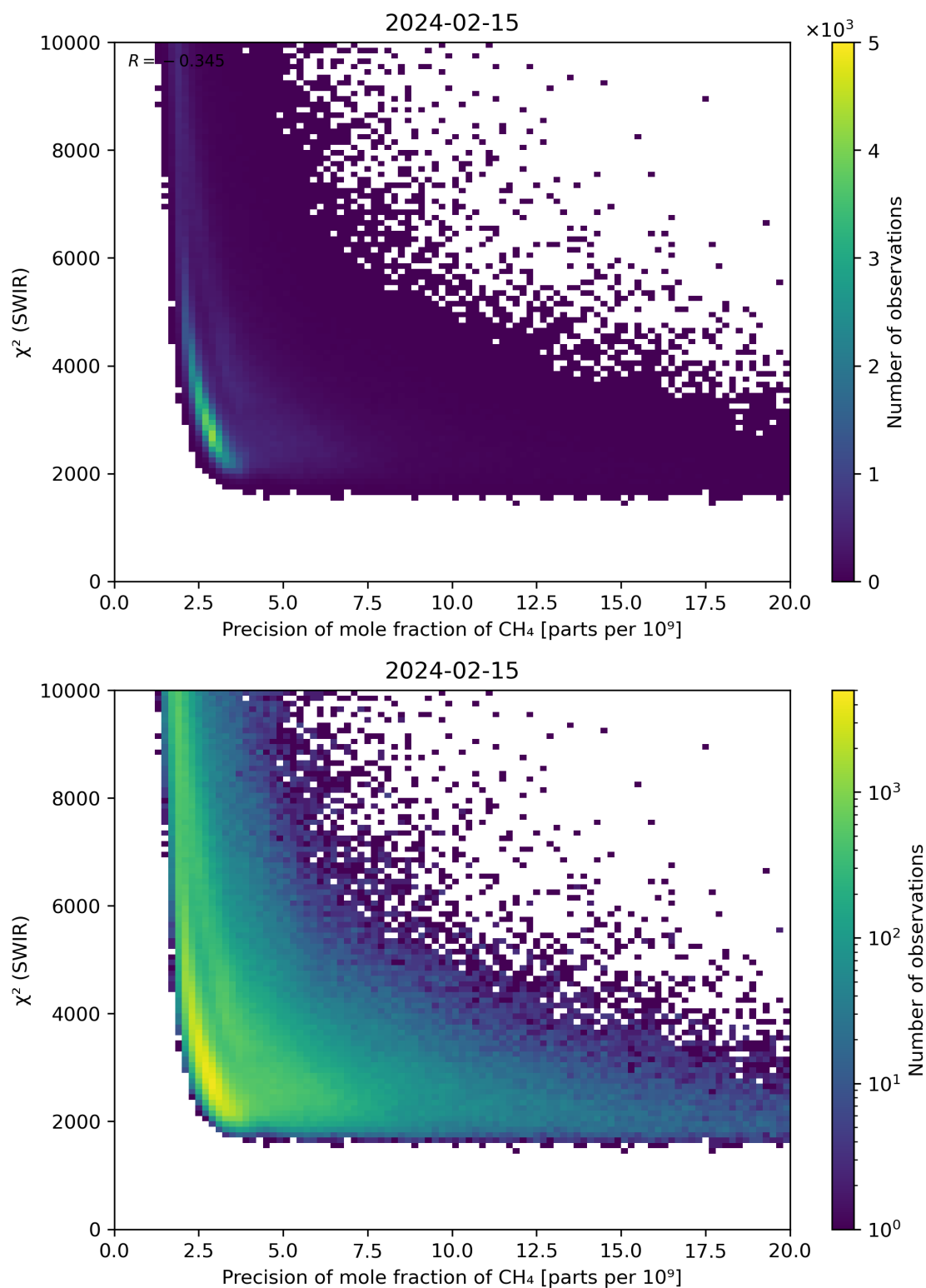
Figure 79: Scatter density plot of “Precision of mole fraction of \text{CH}_4 ” against “ \chi^2 (SWIR)” for 2024-02-14 to 2024-02-16.
