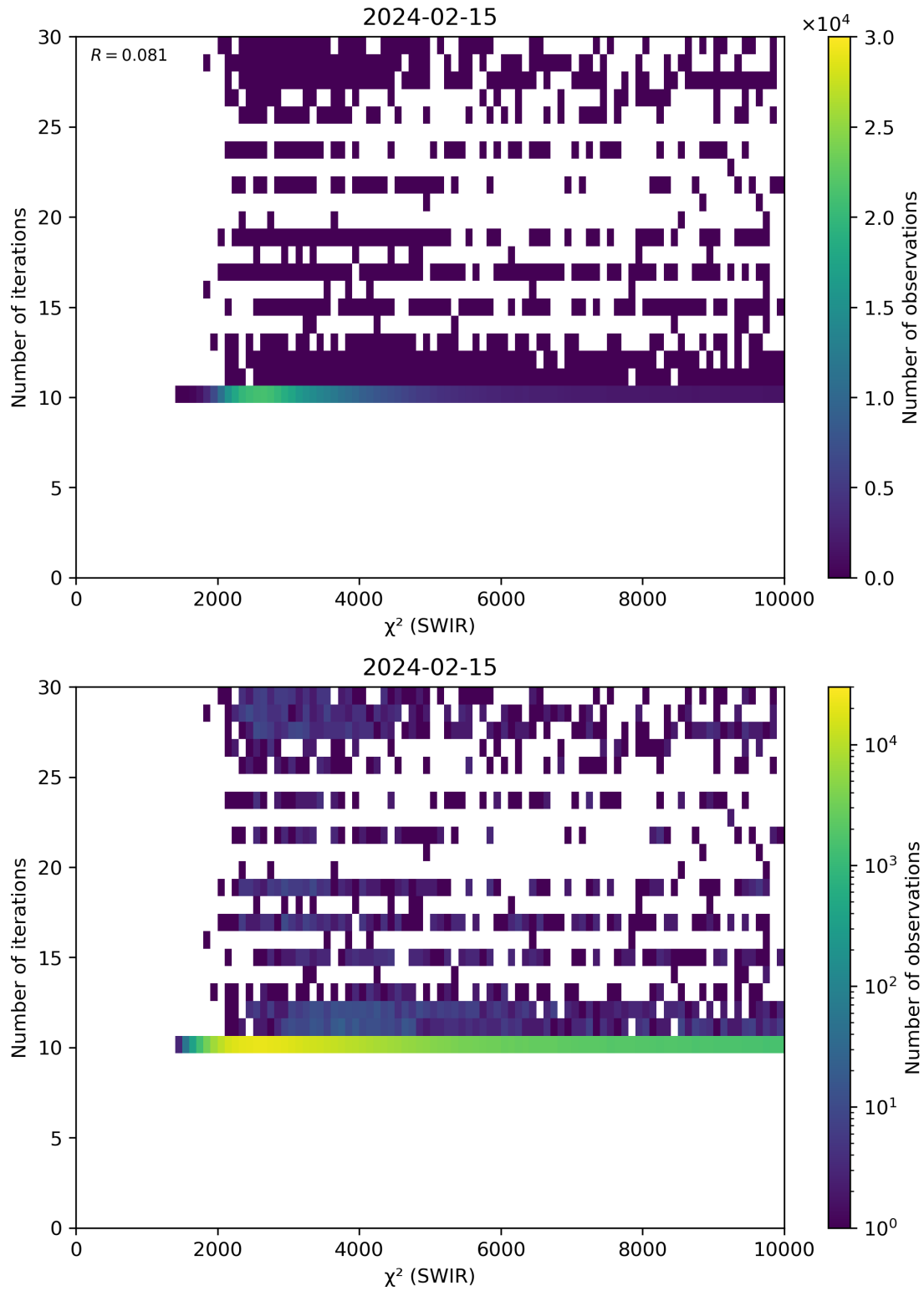
Figure 50: Scatter density plot of “ \chi^2 (SWIR)” against “Number of iterations” for 2024-02-14 to 2024-02-16.
