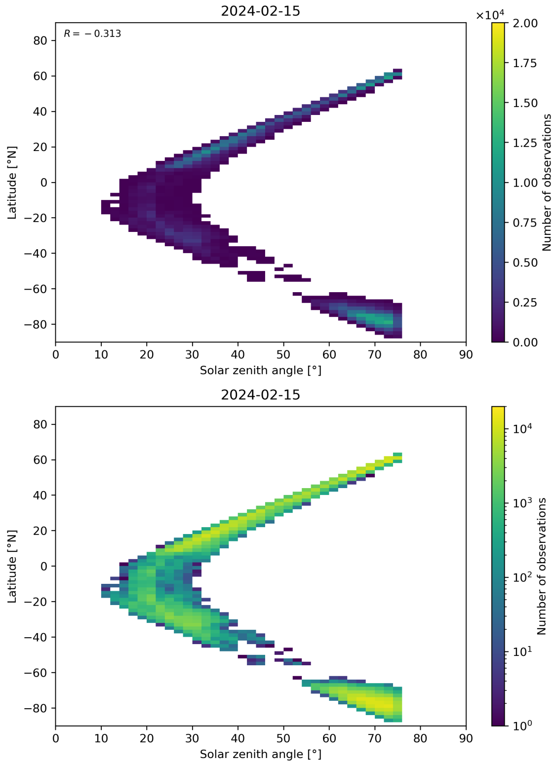
Figure 98: Scatter density plot of “Solar zenith angle” against “Latitude” for 2024-02-14 to 2024-02-16.
