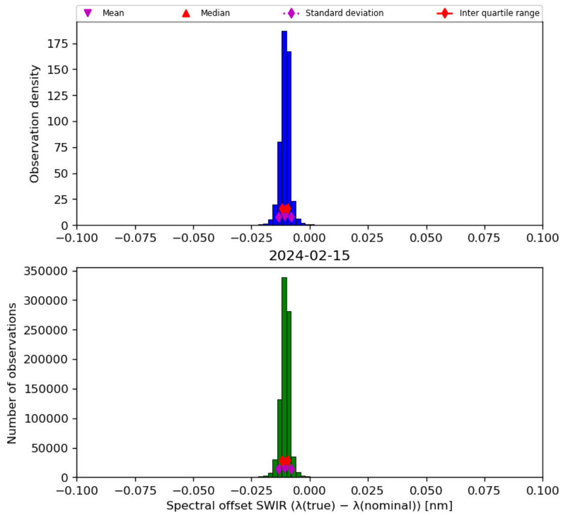
Figure 27: Histogram of “Spectral offset SWIR ( \lambda(\text{true}) - \lambda(\text{nominal}) )” for 2024-02-14 to 2024-02-16
