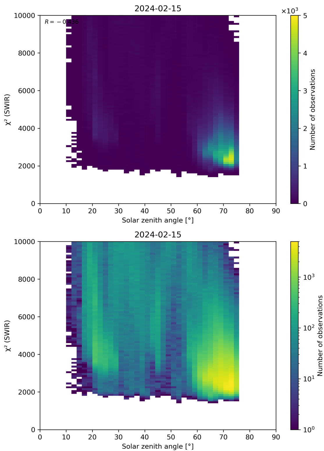
Figure 95: Scatter density plot of “Solar zenith angle” against “ \chi^2 (SWIR)” for 2024-02-14 to 2024-02-16.
