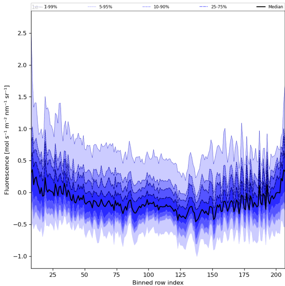
Figure 43: Along track statistics of “Fluorescence” for 2024-02-14 to 2024-02-16
