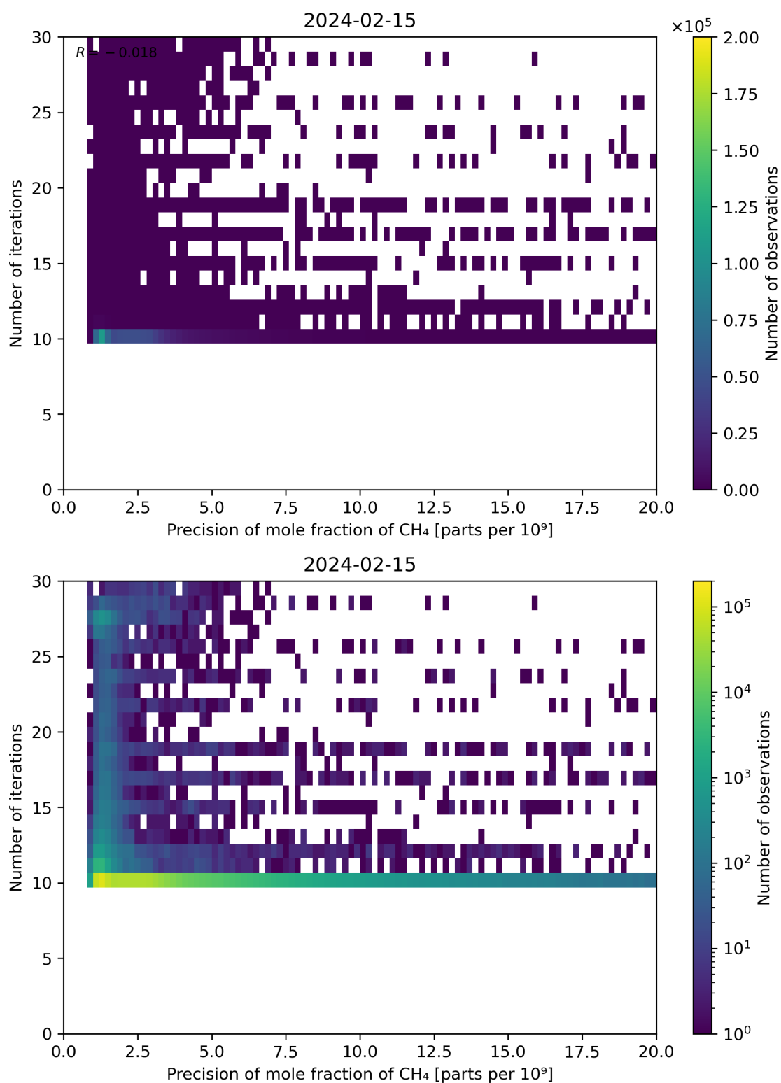
Figure 83: Scatter density plot of “Precision of mole fraction of CH 4 ” against “Number of iterations” for 2024-02-14 to 2024-02-16.
