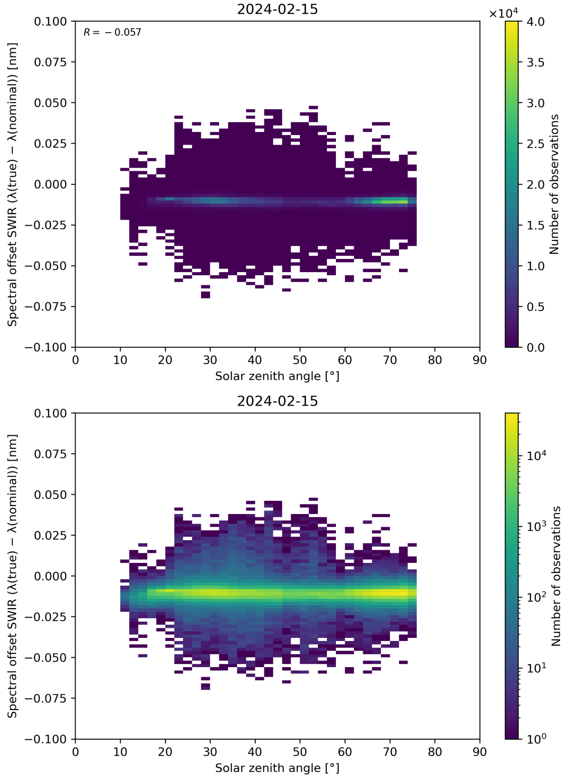
Figure 104: Scatter density plot of “Solar zenith angle” against “Spectral offset SWIR ( \lambda(\text{true}) - \lambda(\text{nominal}) )” for 2024-02-14 to 2024-02-16.
