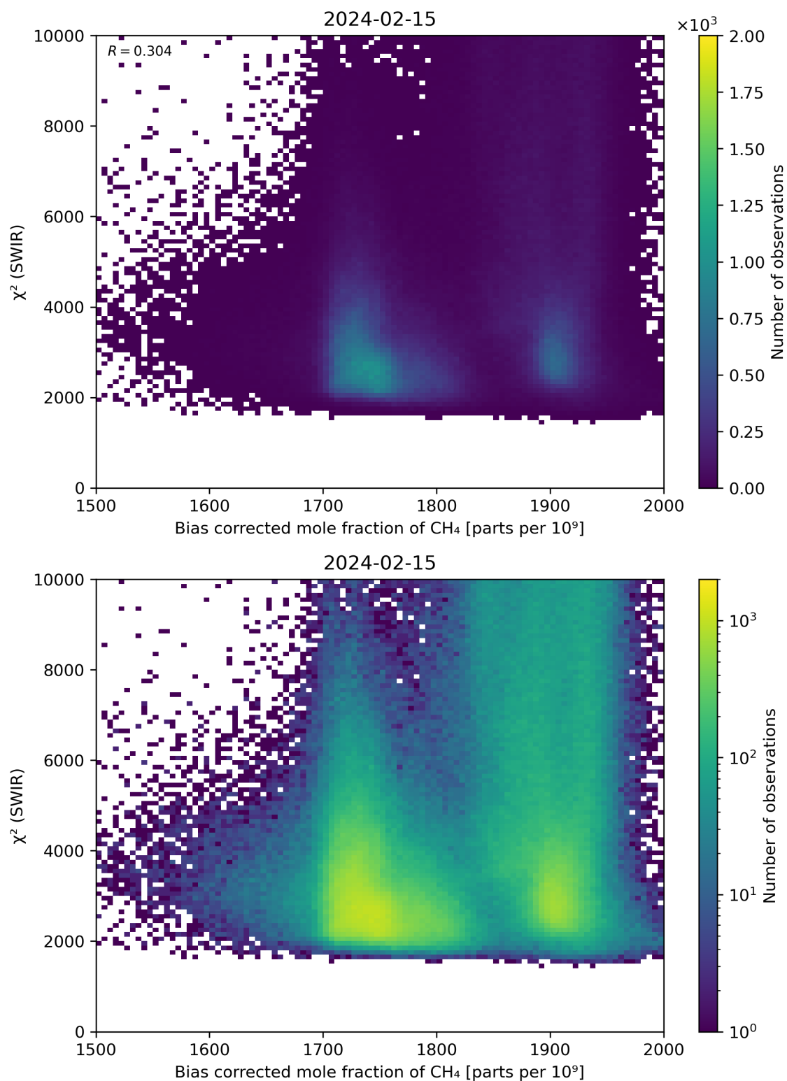
Figure 64: Scatter density plot of “Bias corrected mole fraction of \text{CH}_4 ” against “ \chi^2 (SWIR)” for 2024-02-14 to 2024-02-16.
