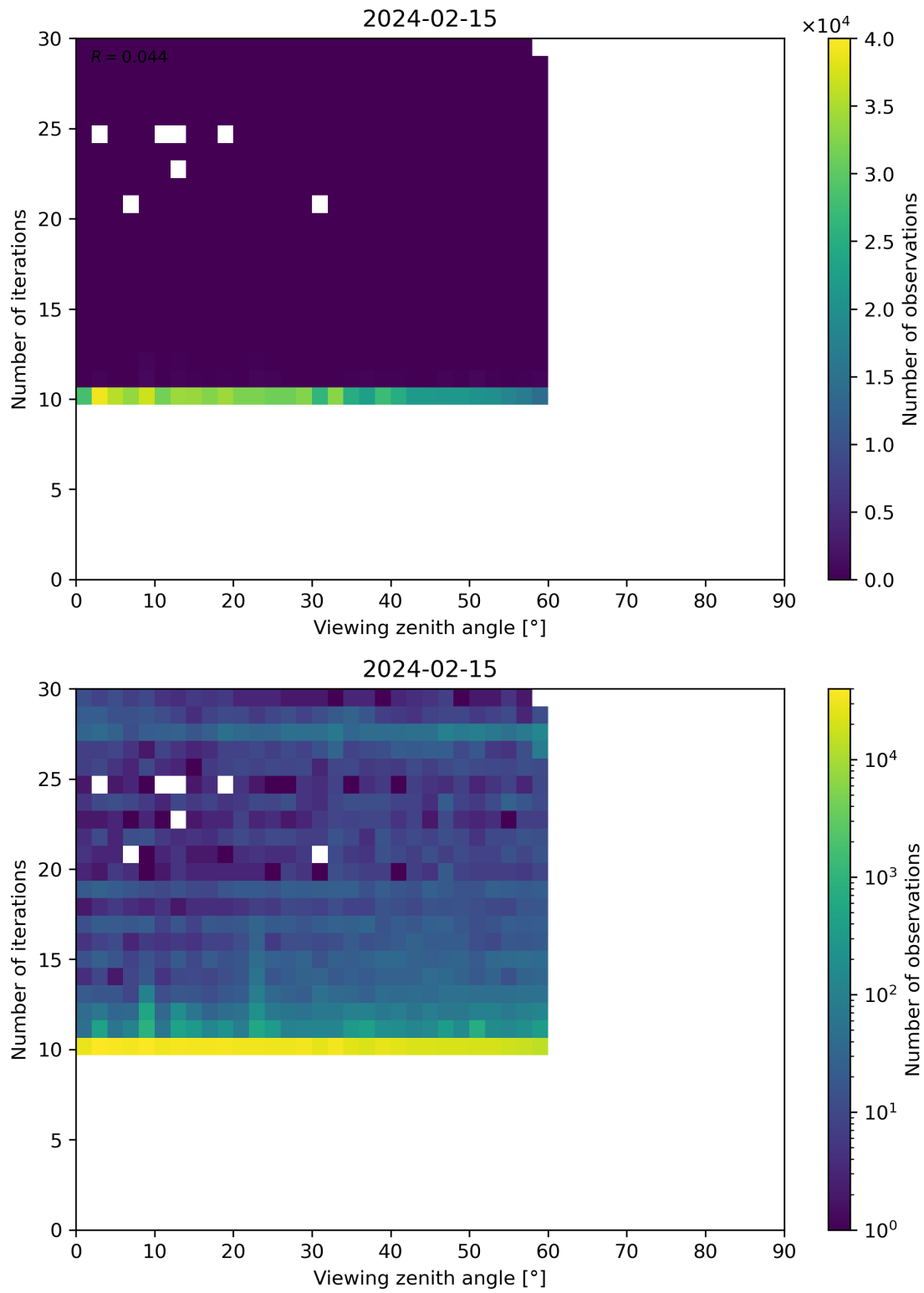
Figure 113: Scatter density plot of “Viewing zenith angle” against “Number of iterations” for 2024-02-14 to 2024-02-16.
