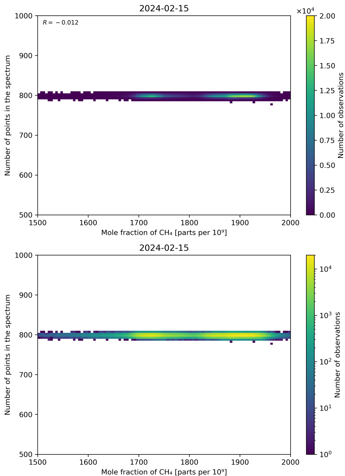
Figure 77: Scatter density plot of “Mole fraction of CH 4 ” against “Number of points in the spectrum” for 2024-02-14 to 2024-02-16.
