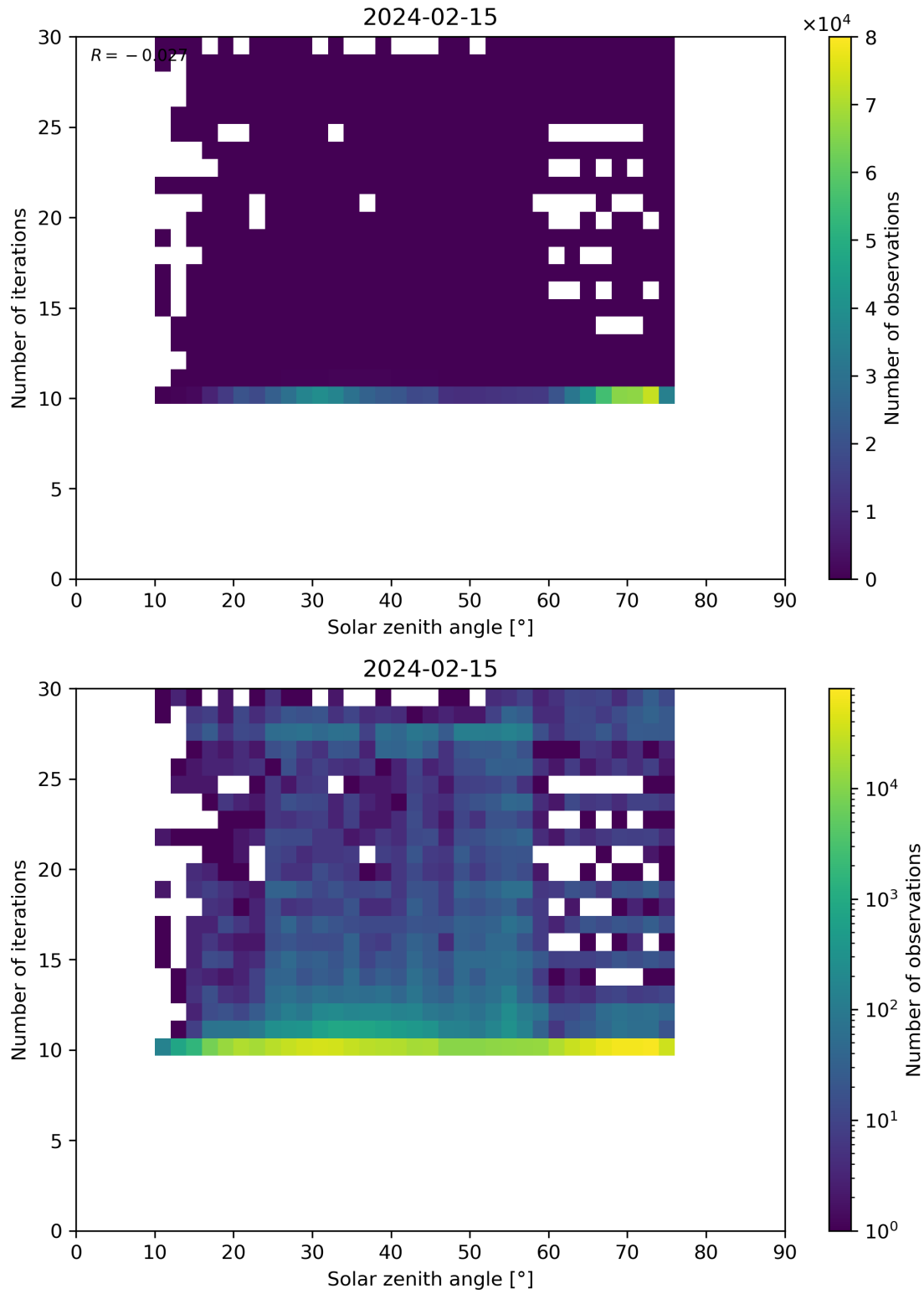
Figure 102: Scatter density plot of “Solar zenith angle” against “Number of iterations” for 2024-02-14 to 2024-02-16.
