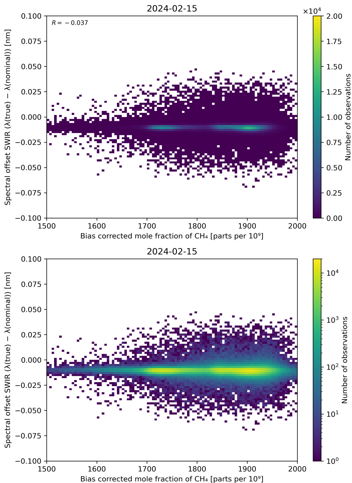
Figure 69: Scatter density plot of “Bias corrected mole fraction of \text{CH}_4 ” against “Spectral offset SWIR ( \lambda(\text{true}) - \lambda(\text{nominal}) )” for 2024-02-14 to 2024-02-16.
