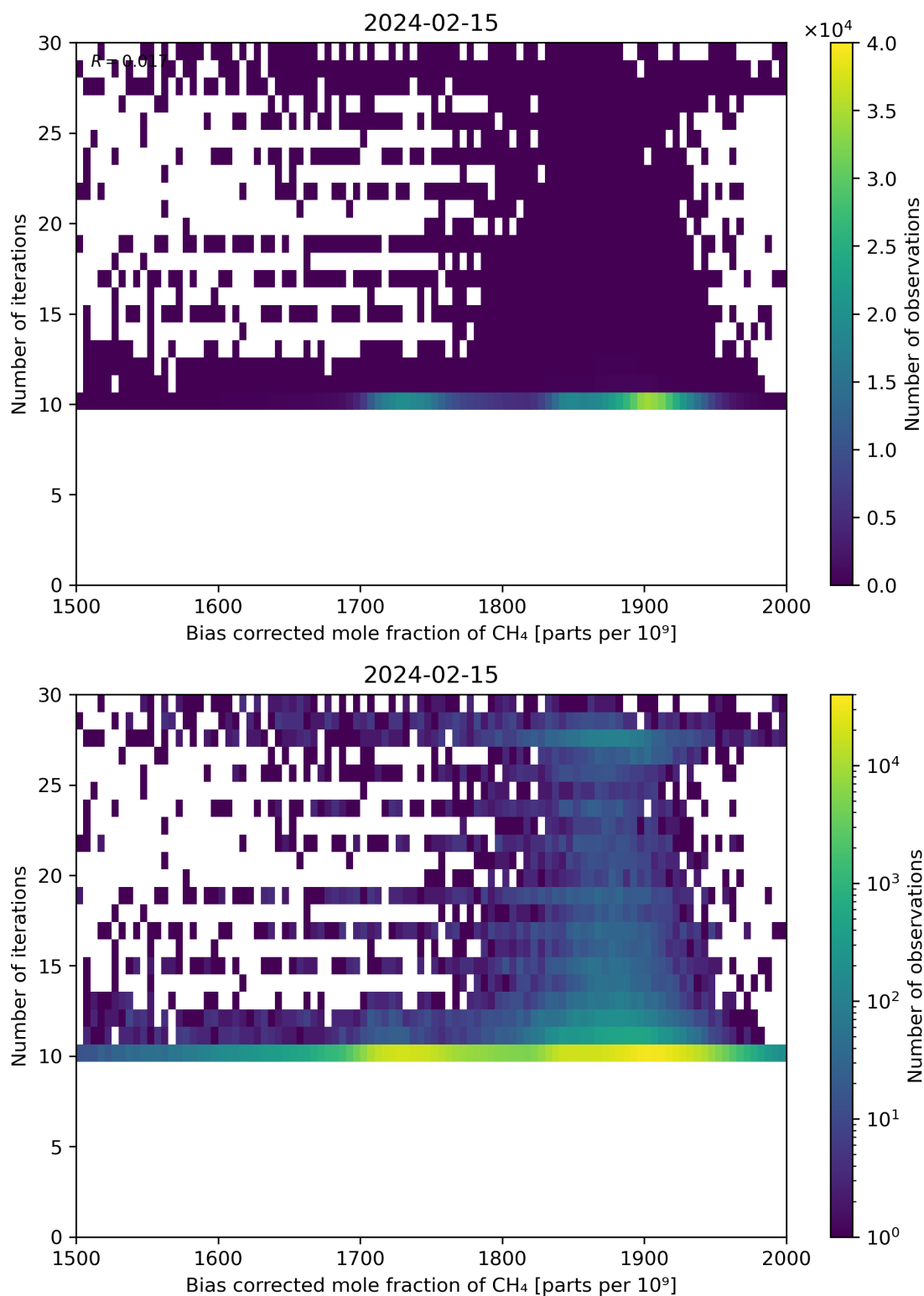
Figure 67: Scatter density plot of “Bias corrected mole fraction of \text{CH}_4 ” against “Number of iterations” for 2024-02-14 to 2024-02-16.
