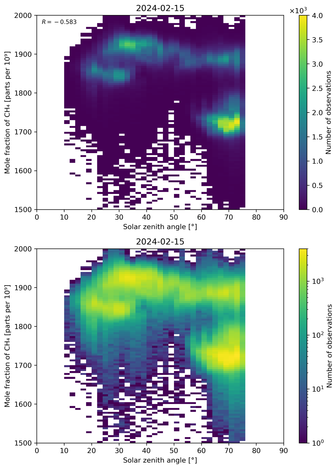
Figure 99: Scatter density plot of “Solar zenith angle” against “Mole fraction of CH 4 ” for 2024-02-14 to 2024-02-16.
