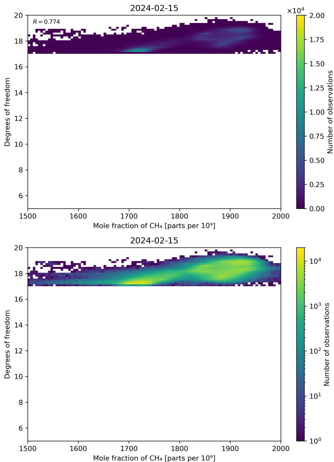
Figure 72: Scatter density plot of “Mole fraction of CH 4 ” against “Degrees of freedom” for 2024-02-14 to 2024-02-16.
