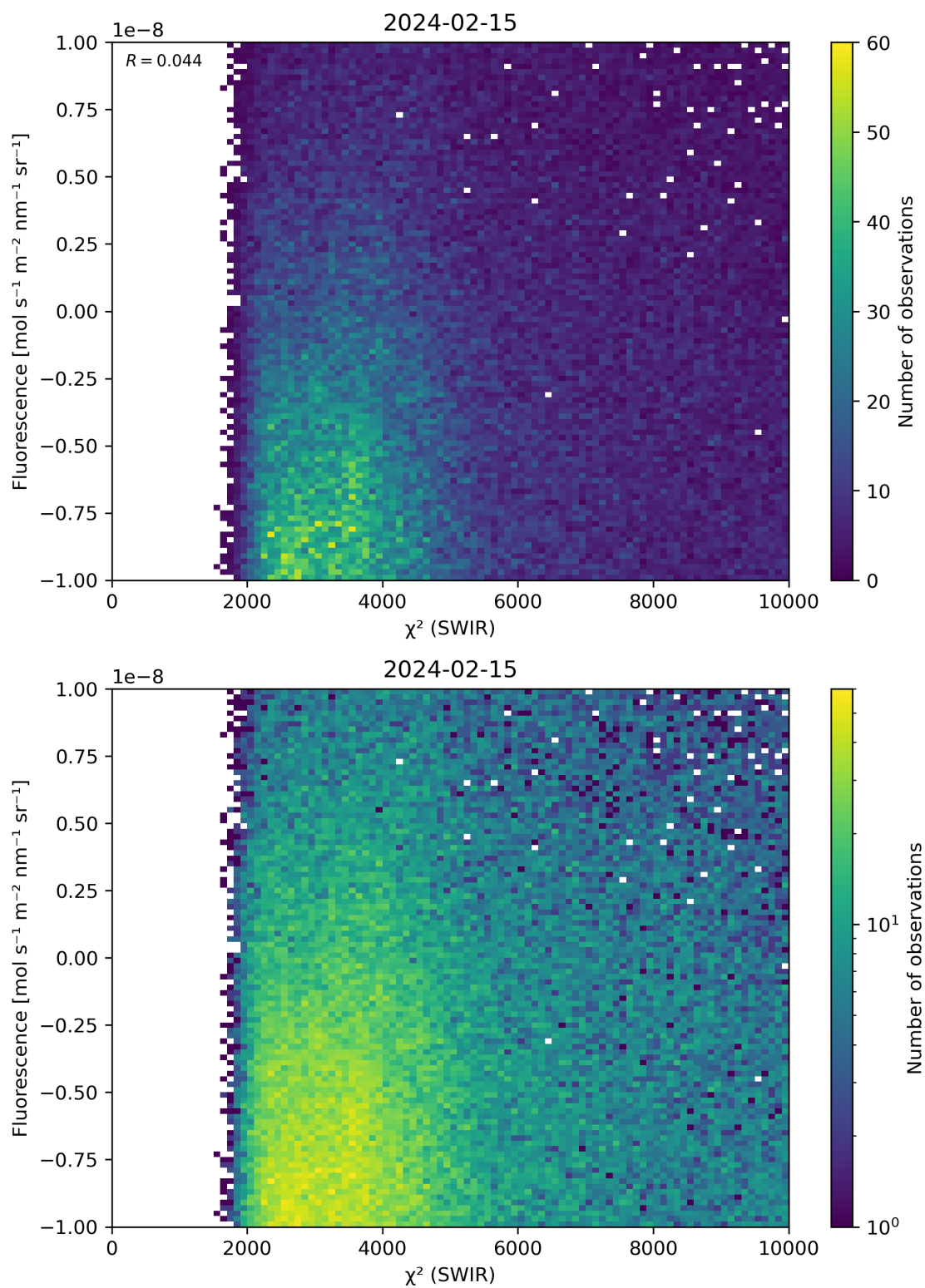
Figure 49: Scatter density plot of “ \chi^2 (SWIR)” against “Fluorescence” for 2024-02-14 to 2024-02-16.
