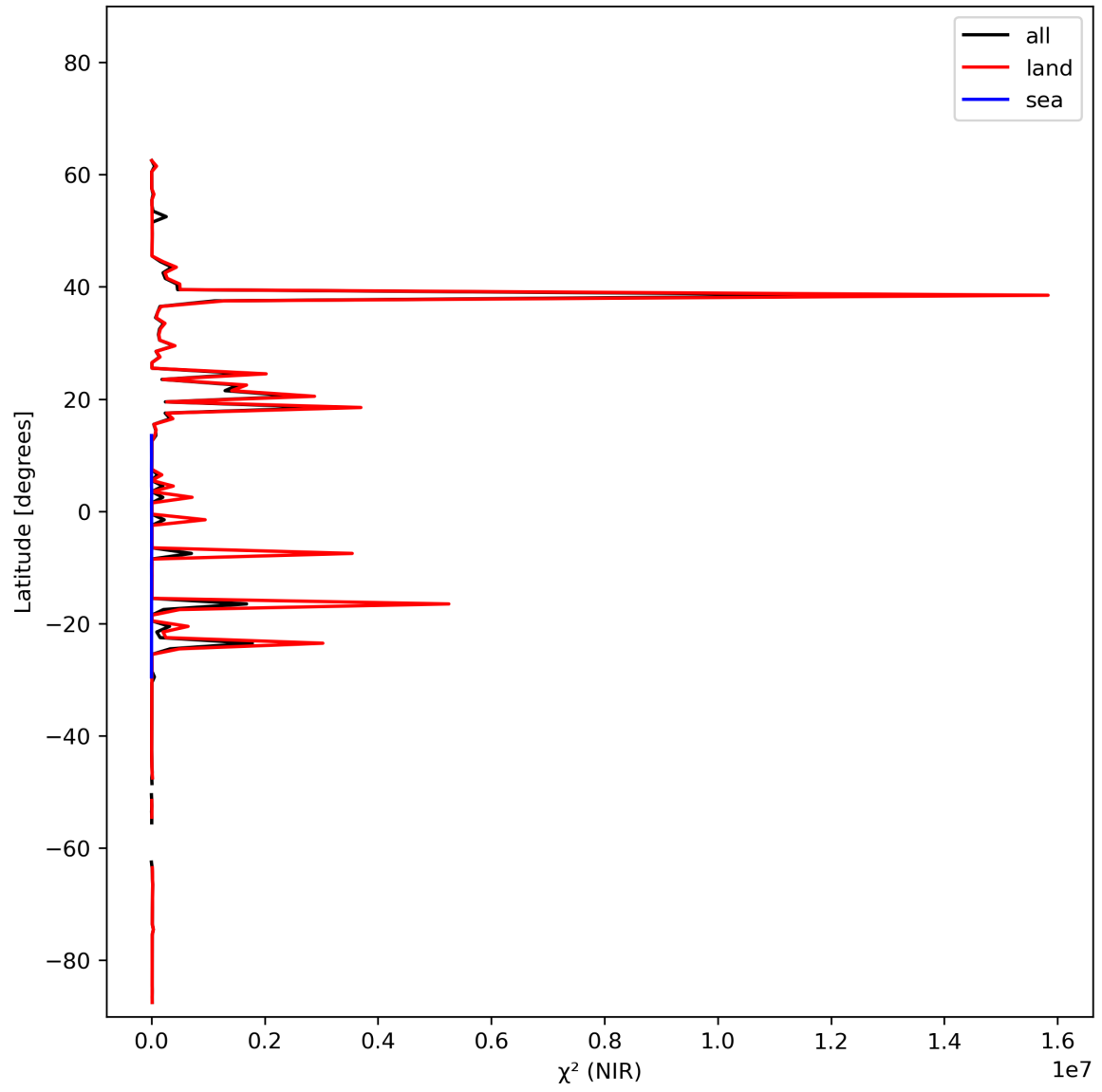
Figure 18: Zonal average of “ \chi^2 (NIR)” for 2024-02-14 to 2024-02-16.
