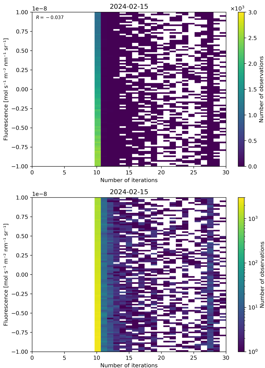
Figure 87: Scatter density plot of “Number of iterations” against “Fluorescence” for 2024-02-14 to 2024-02-16.
