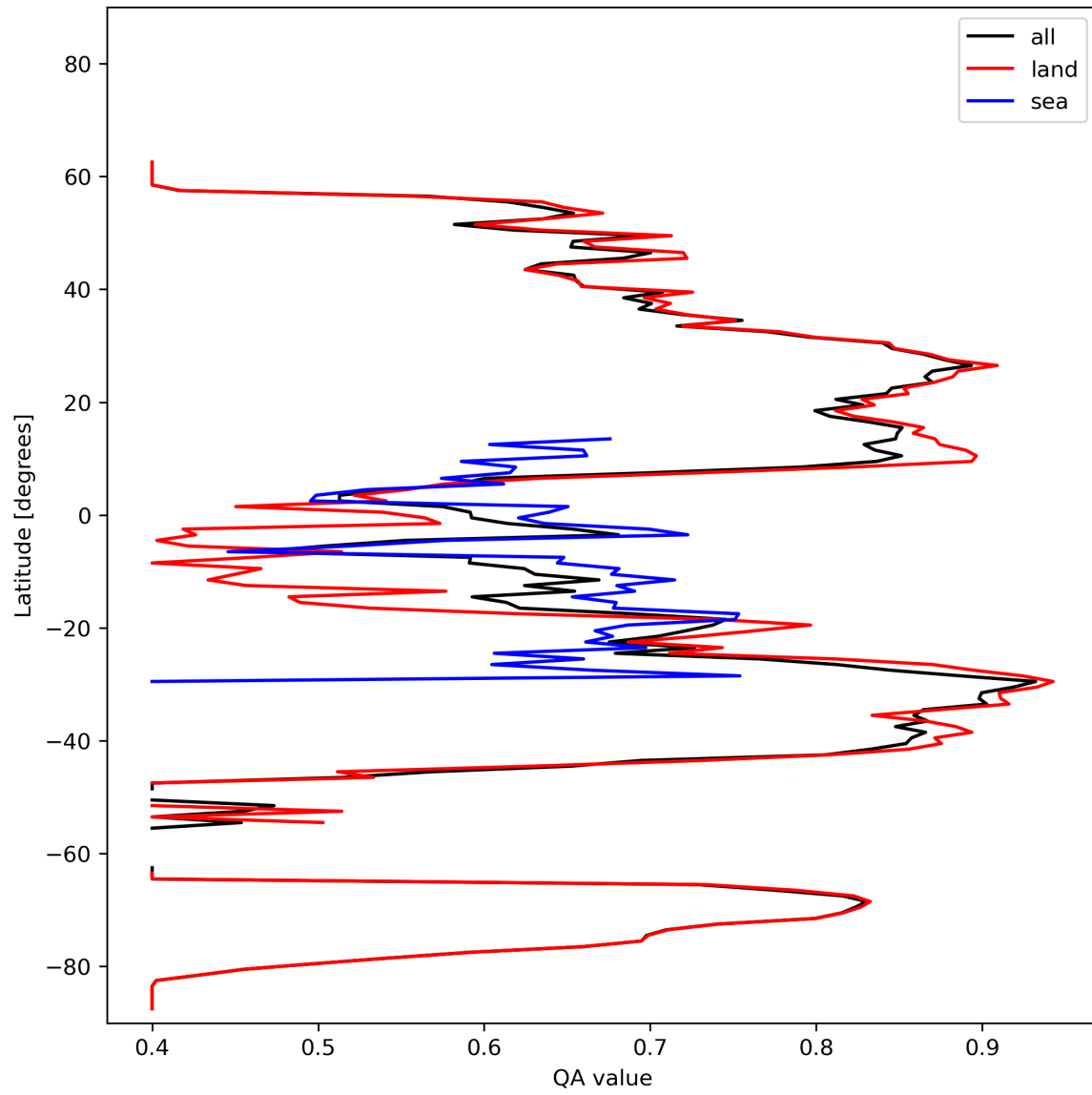
Figure 11: Zonal average of “QA value” for 2024-02-14 to 2024-02-16.
