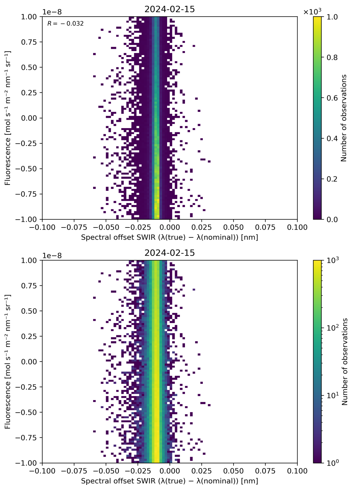
Figure 120: Scatter density plot of “Spectral offset SWIR ( \lambda(\text{true}) - \lambda(\text{nominal}) )” against “Fluorescence” for 2024-02-14 to 2024-02-16.
