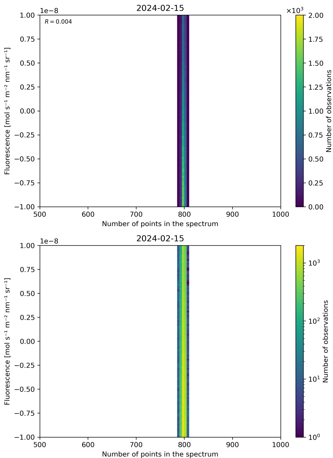
Figure 91: Scatter density plot of “Number of points in the spectrum” against “Fluorescence” for 2024-02-14 to 2024-02-16.
