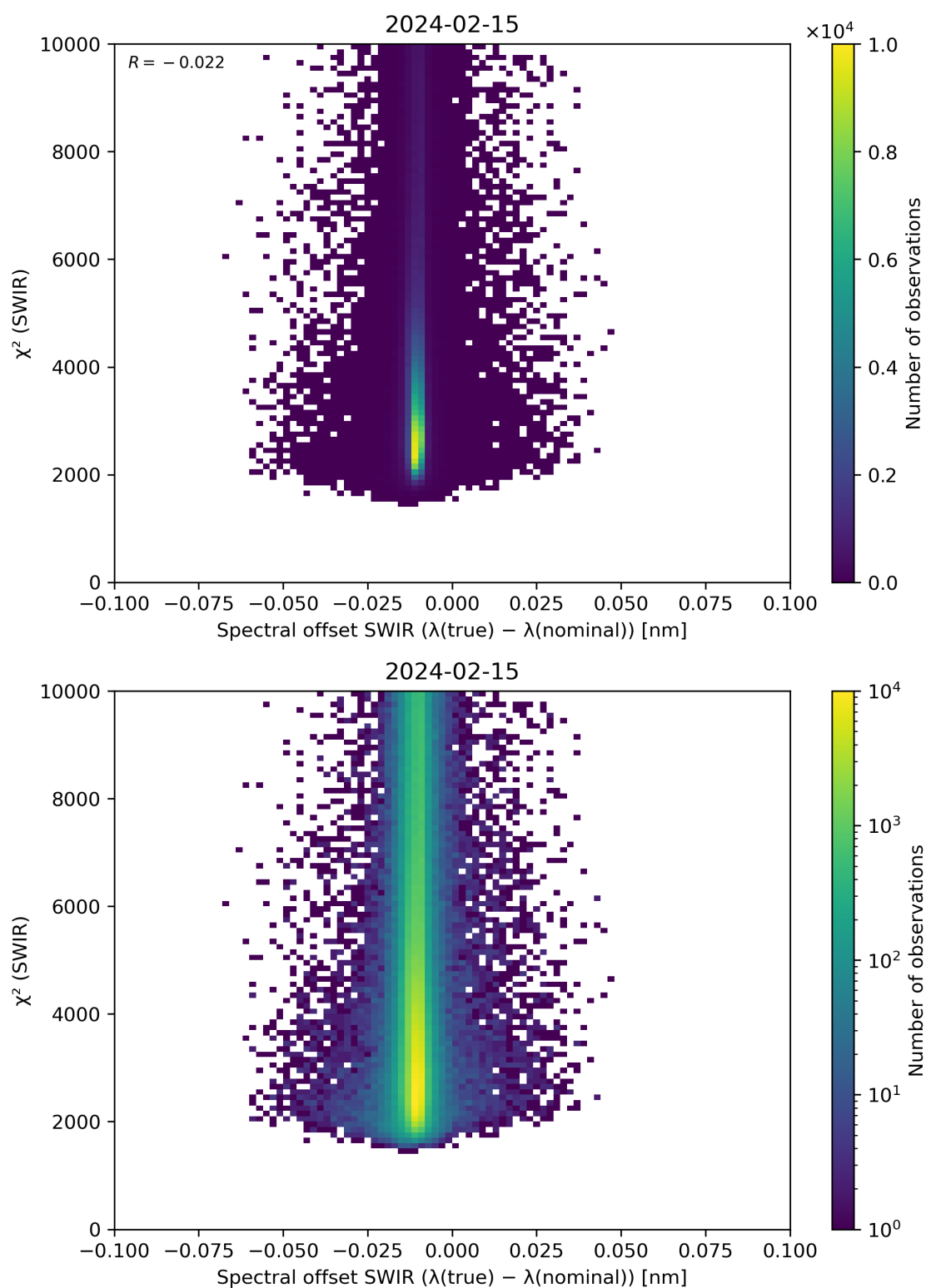
Figure 118: Scatter density plot of “Spectral offset SWIR ( \lambda(\text{true}) - \lambda(\text{nominal}) )” against “ \chi^2 (SWIR)” for 2024-02-14 to 2024-02-16.
