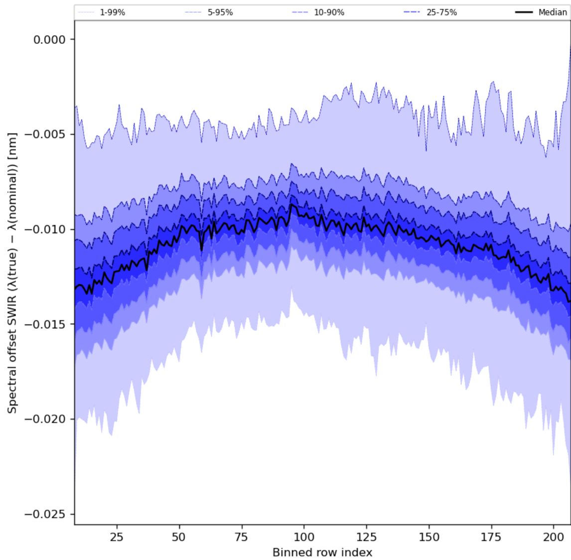
Figure 38: Along track statistics of “Spectral offset SWIR ( \lambda(\text{true}) - \lambda(\text{nominal}) )” for 2024-02-14 to 2024-02-16
