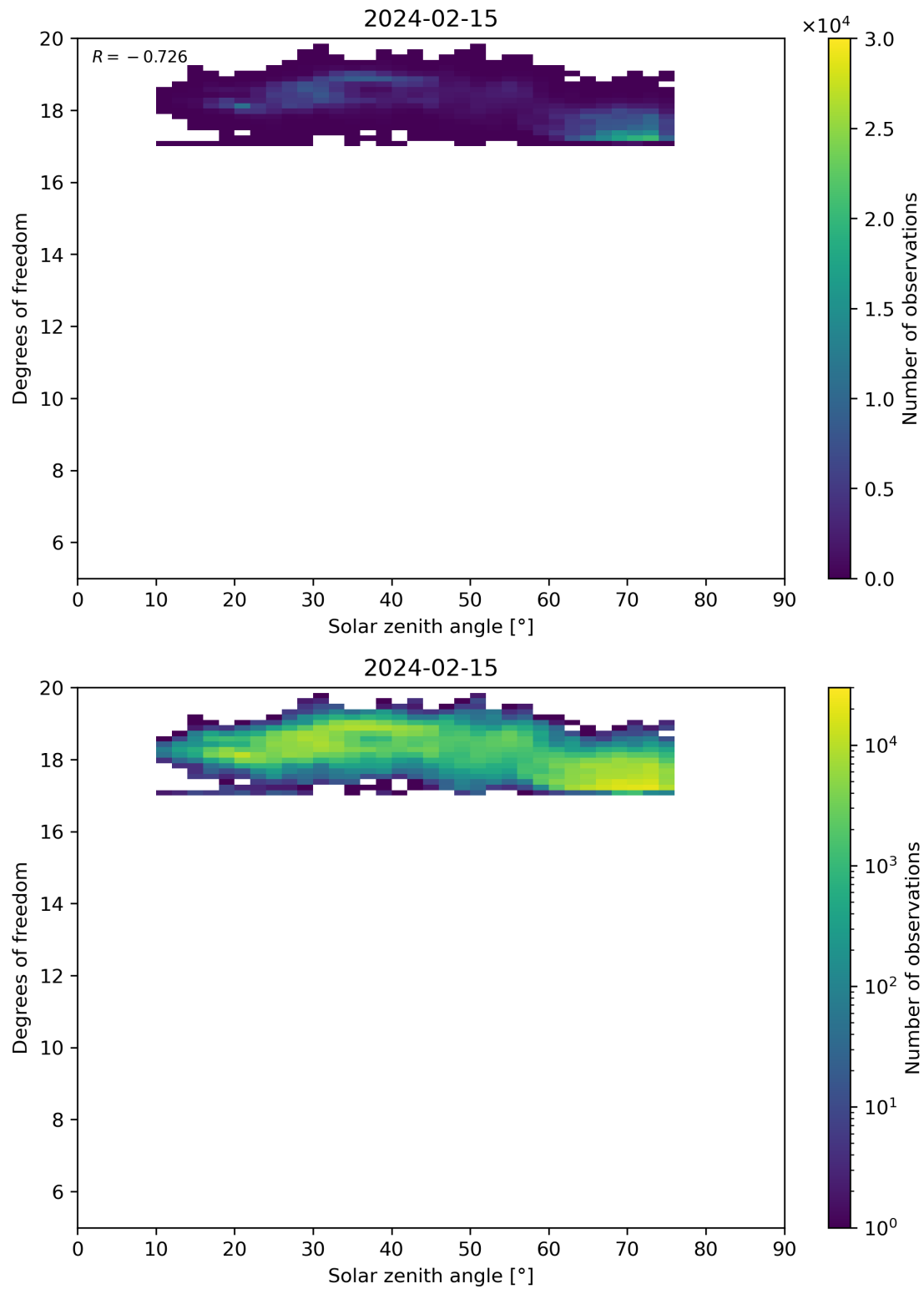
Figure 96: Scatter density plot of “Solar zenith angle” against “Degrees of freedom” for 2024-02-14 to 2024-02-16.
