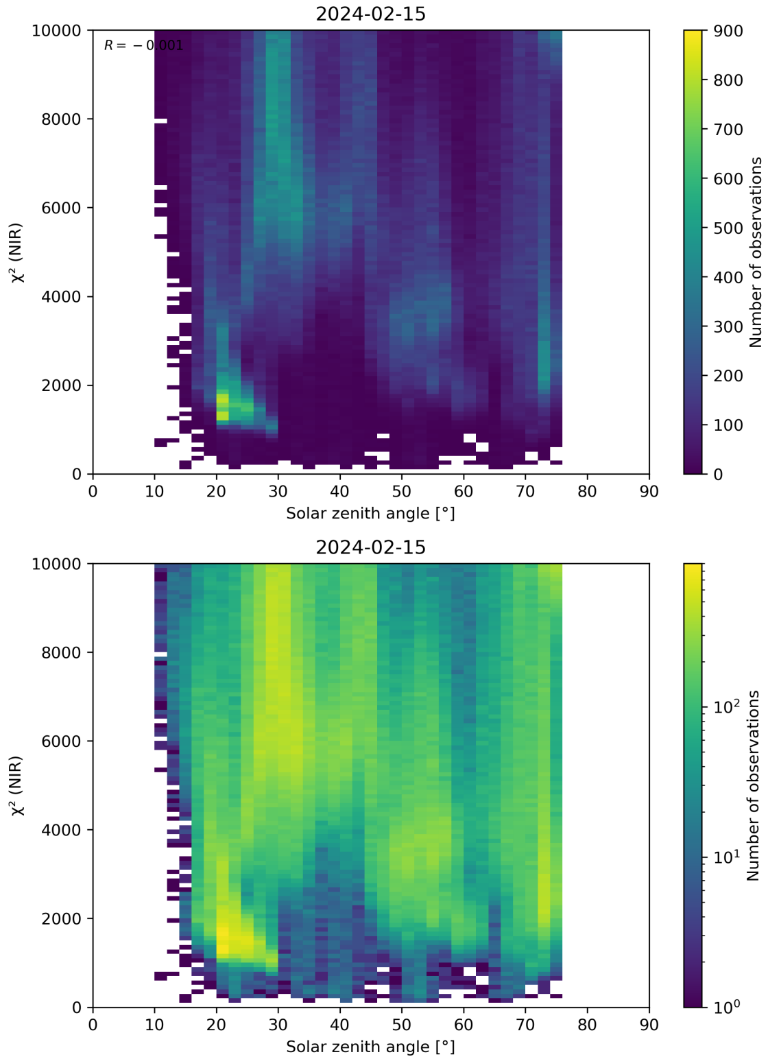
Figure 94: Scatter density plot of “Solar zenith angle” against “ \chi^2 (NIR)” for 2024-02-14 to 2024-02-16.
