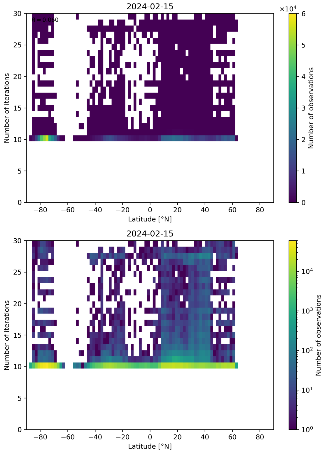
Figure 60: Scatter density plot of “Latitude” against “Number of iterations” for 2024-02-14 to 2024-02-16.
