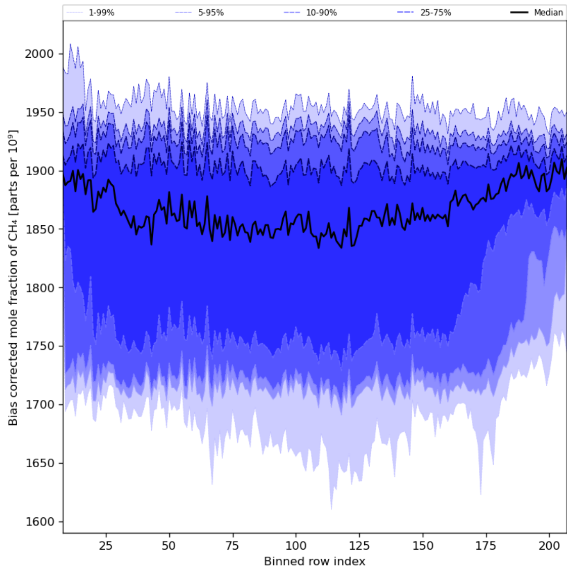
Figure 36: Along track statistics of “Bias corrected mole fraction of CH 4 ” for 2024-02-14 to 2024-02-16
