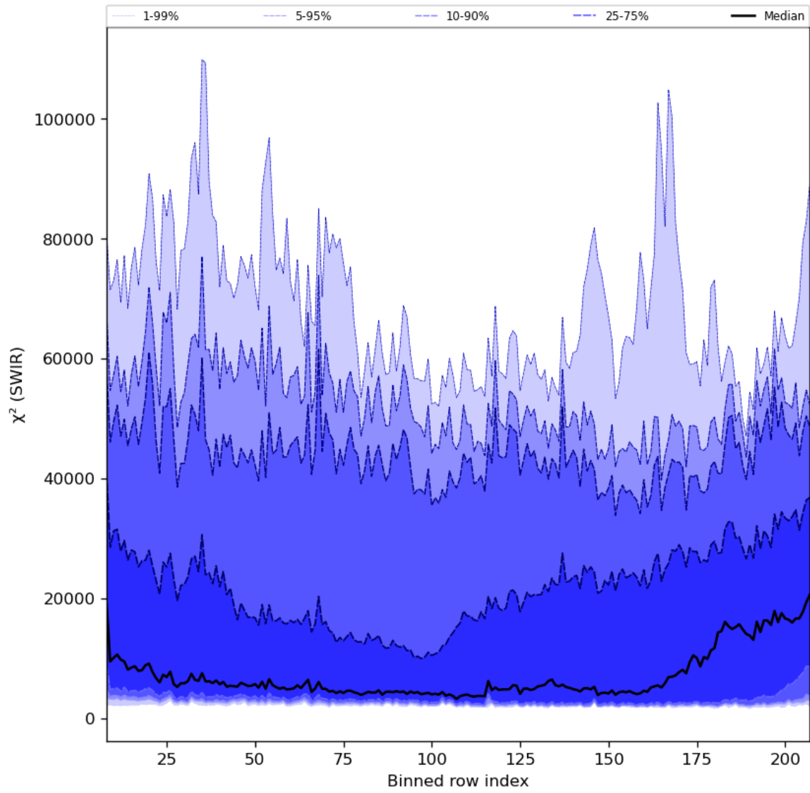
Figure 39: Along track statistics of “ \chi^2 (SWIR)” for 2024-02-14 to 2024-02-16
