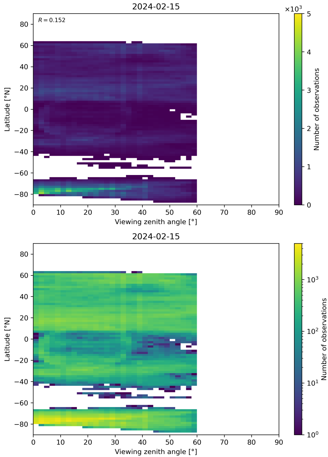
Figure 109: Scatter density plot of “Viewing zenith angle” against “Latitude” for 2024-02-14 to 2024-02-16.
