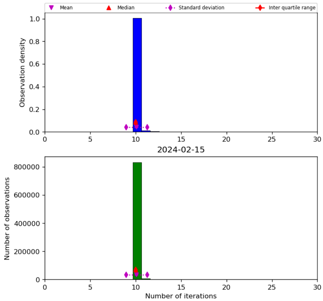
Figure 31: Histogram of “Number of iterations” for 2024-02-14 to 2024-02-16
