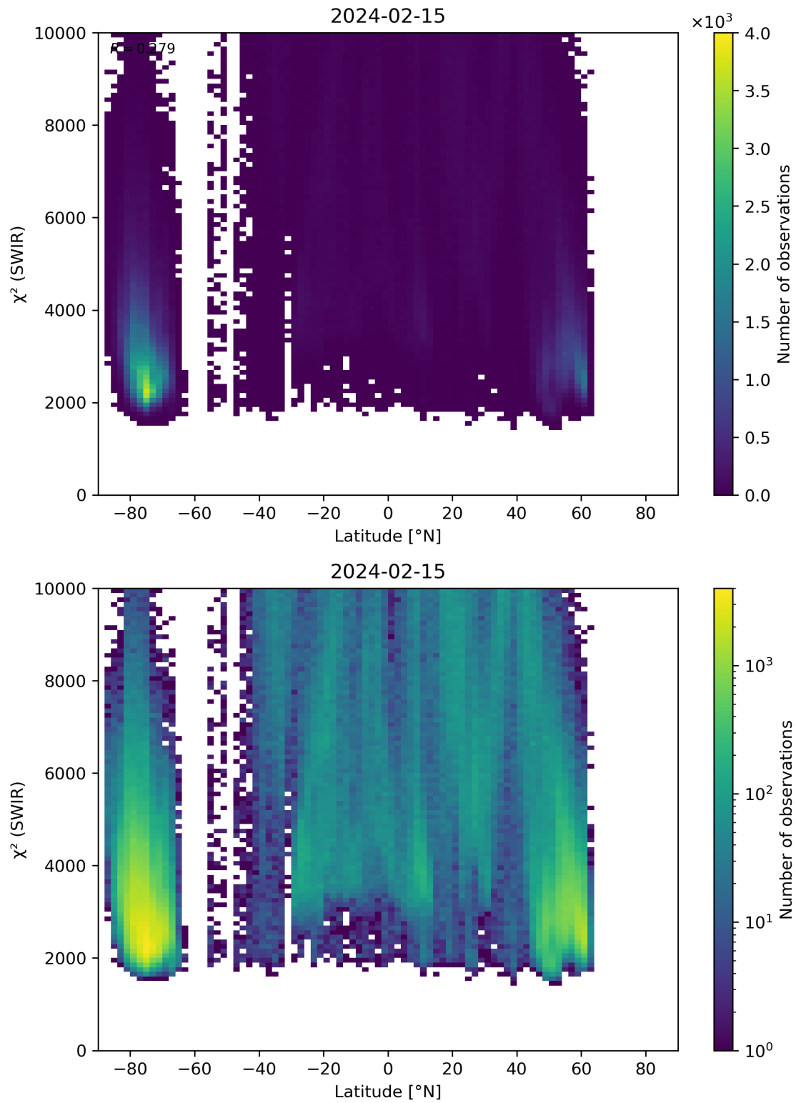
Figure 54: Scatter density plot of “Latitude” against “ \chi^2 (SWIR)” for 2024-02-14 to 2024-02-16.
