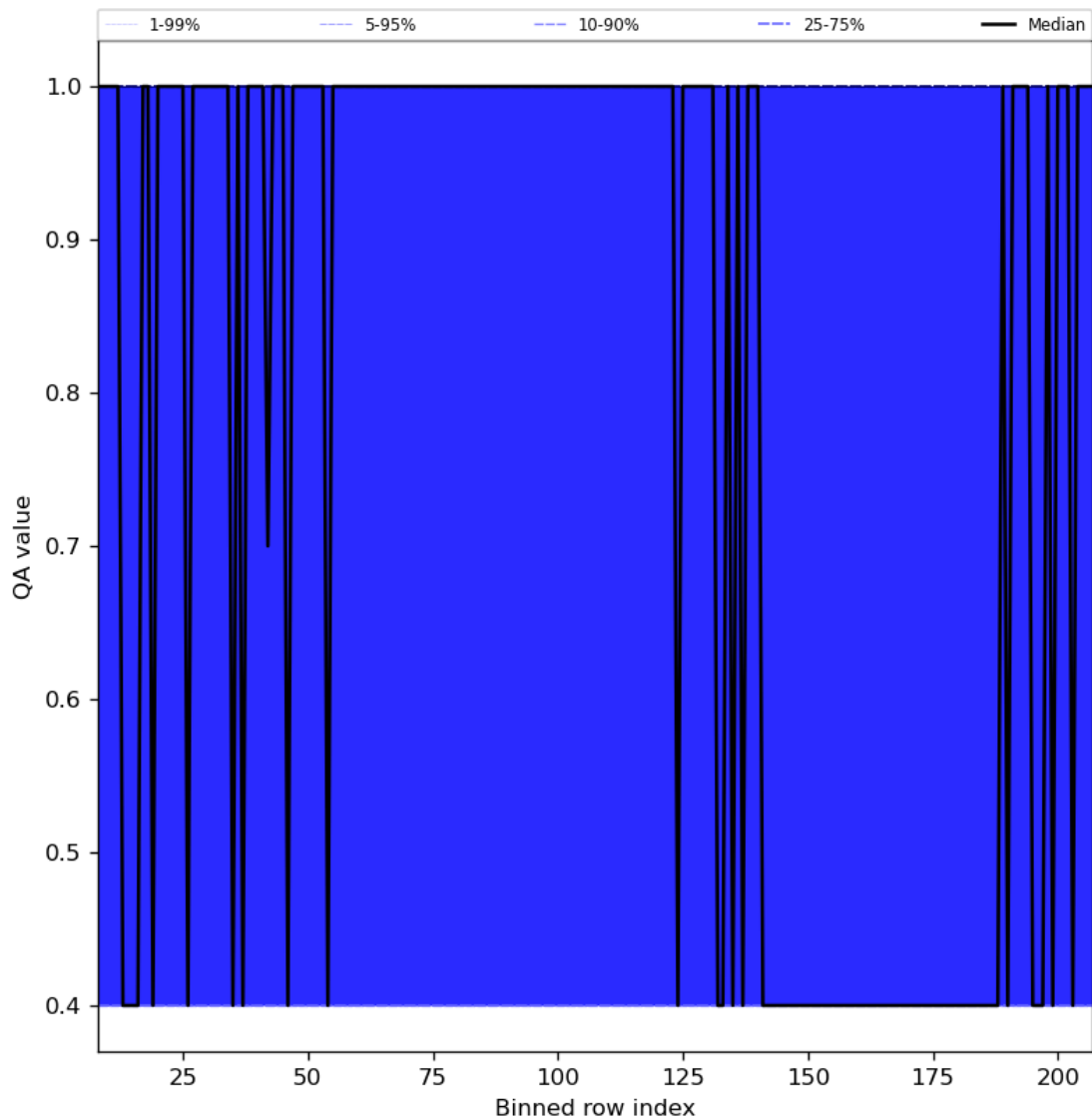
Figure 33: Along track statistics of “QA value” for 2024-02-14 to 2024-02-16
