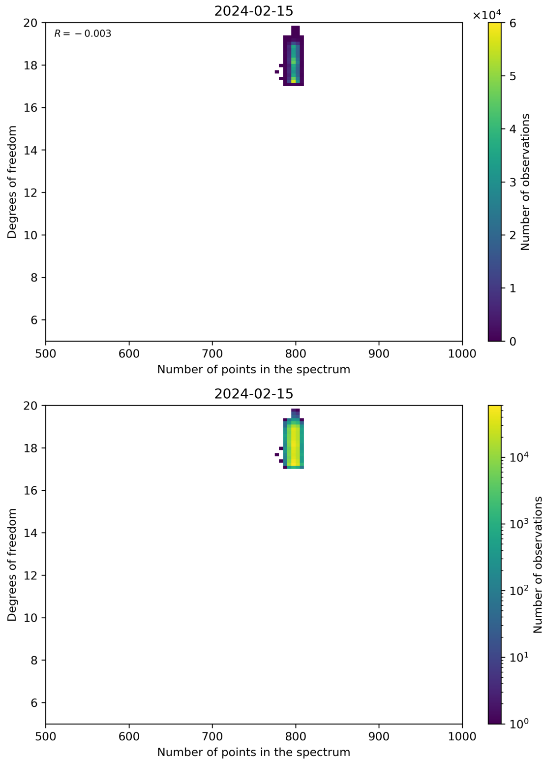
Figure 90: Scatter density plot of “Number of points in the spectrum” against “Degrees of freedom” for 2024-02-14 to 2024-02-16.
