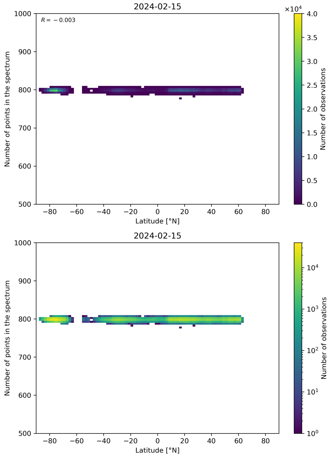
Figure 61: Scatter density plot of “Latitude” against “Number of points in the spectrum” for 2024-02-14 to 2024-02-16.
