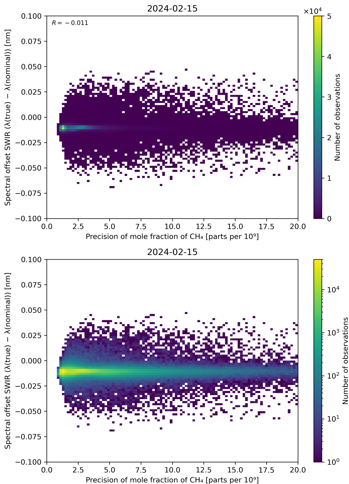
Figure 85: Scatter density plot of “Precision of mole fraction of CH 4 ” against “Spectral offset SWIR ( \lambda(\text{true}) - \lambda(\text{nominal}) )” for 2024-02-14 to 2024-02-16.
