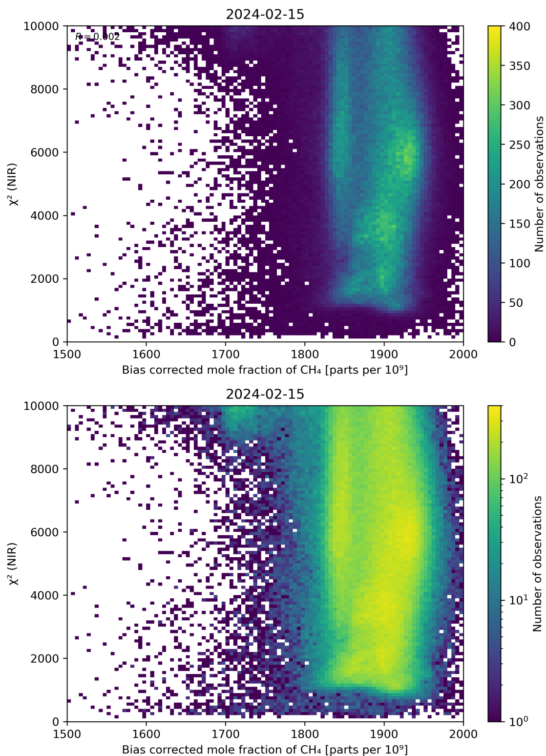
Figure 63: Scatter density plot of “Bias corrected mole fraction of CH 4 ” against “ \chi^2 (NIR)” for 2024-02-14 to 2024-02-16.
