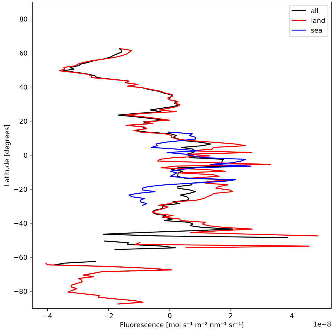
Figure 21: Zonal average of “Fluorescence” for 2024-02-14 to 2024-02-16.
