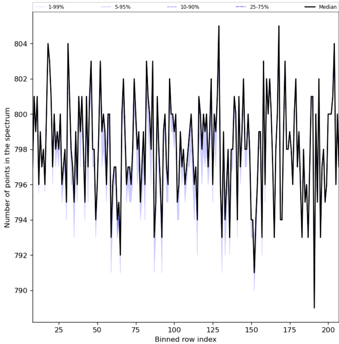
Figure 37: Along track statistics of “Number of points in the spectrum” for 2024-02-14 to 2024-02-16
