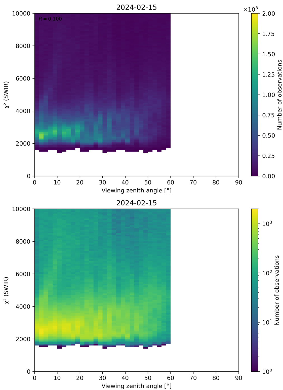
Figure 106: Scatter density plot of “Viewing zenith angle” against “ \chi^2 (SWIR)” for 2024-02-14 to 2024-02-16.
