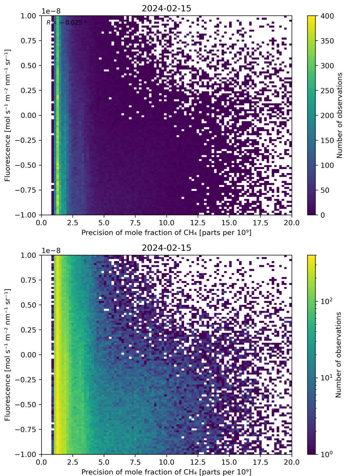
Figure 81: Scatter density plot of “Precision of mole fraction of \text{CH}_4 ” against “Fluorescence” for 2024-02-14 to 2024-02-16.
