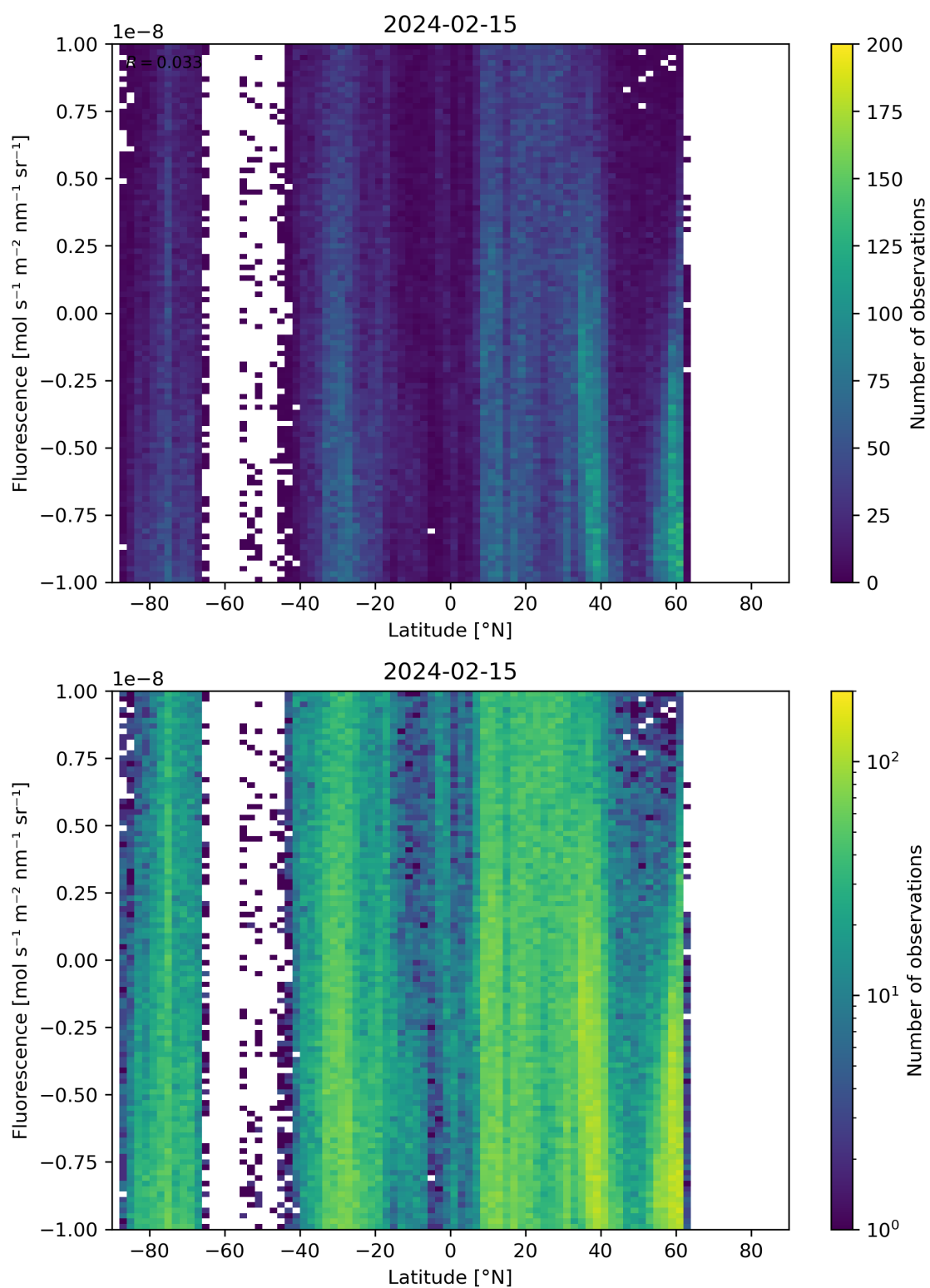
Figure 56: Scatter density plot of “Latitude” against “Fluorescence” for 2024-02-14 to 2024-02-16.
