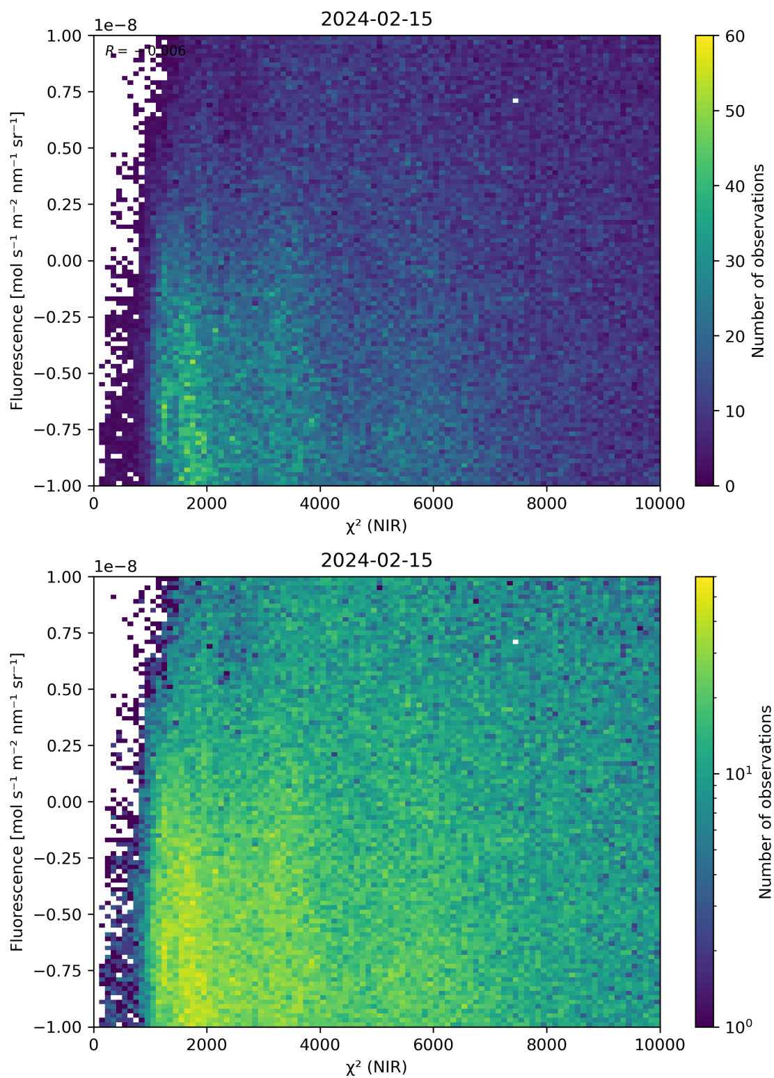
Figure 45: Scatter density plot of “ \chi^2 (NIR)” against “Fluorescence” for 2024-02-14 to 2024-02-16.
