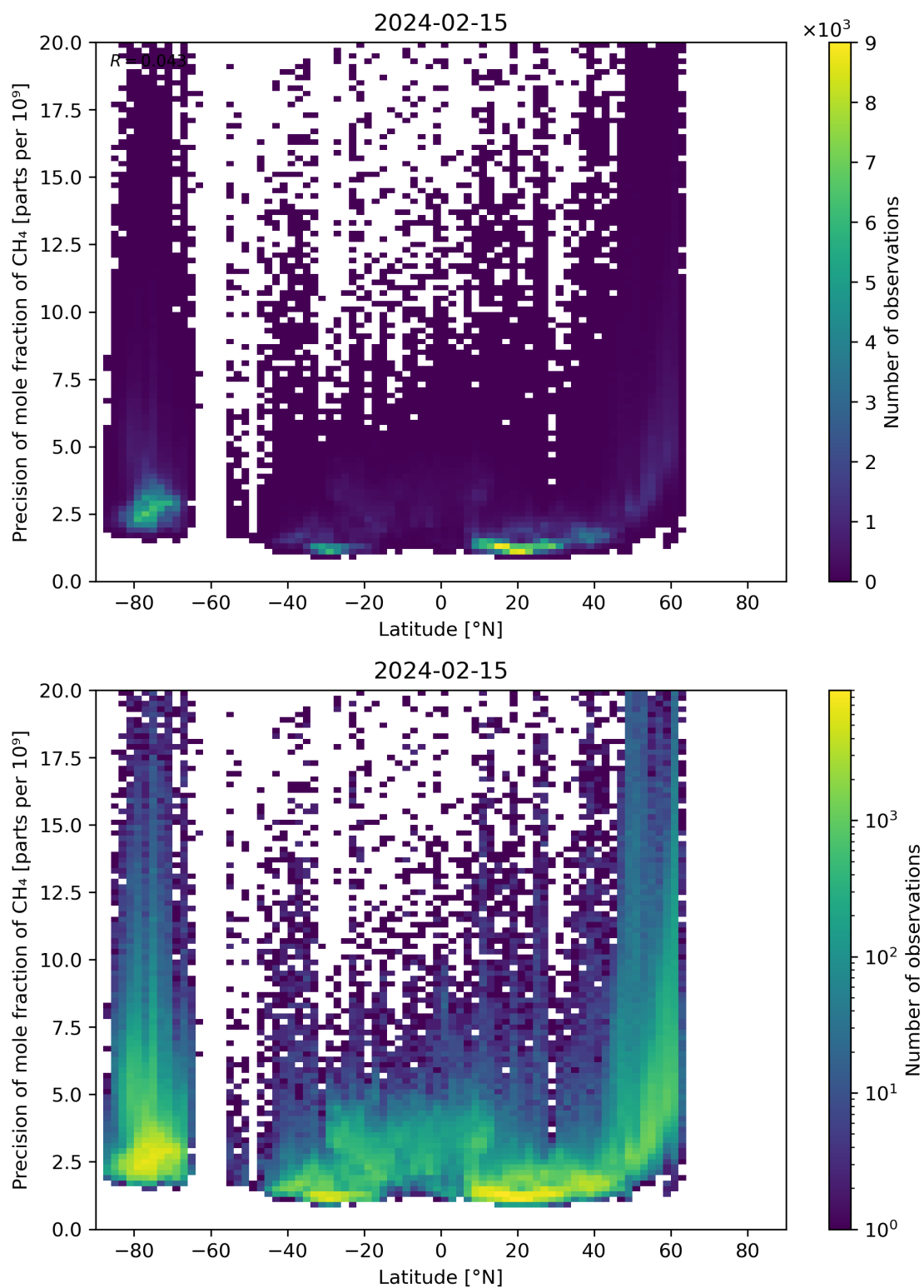
Figure 59: Scatter density plot of “Latitude” against “Precision of mole fraction of CH 4 ” for 2024-02-14 to 2024-02-16.
