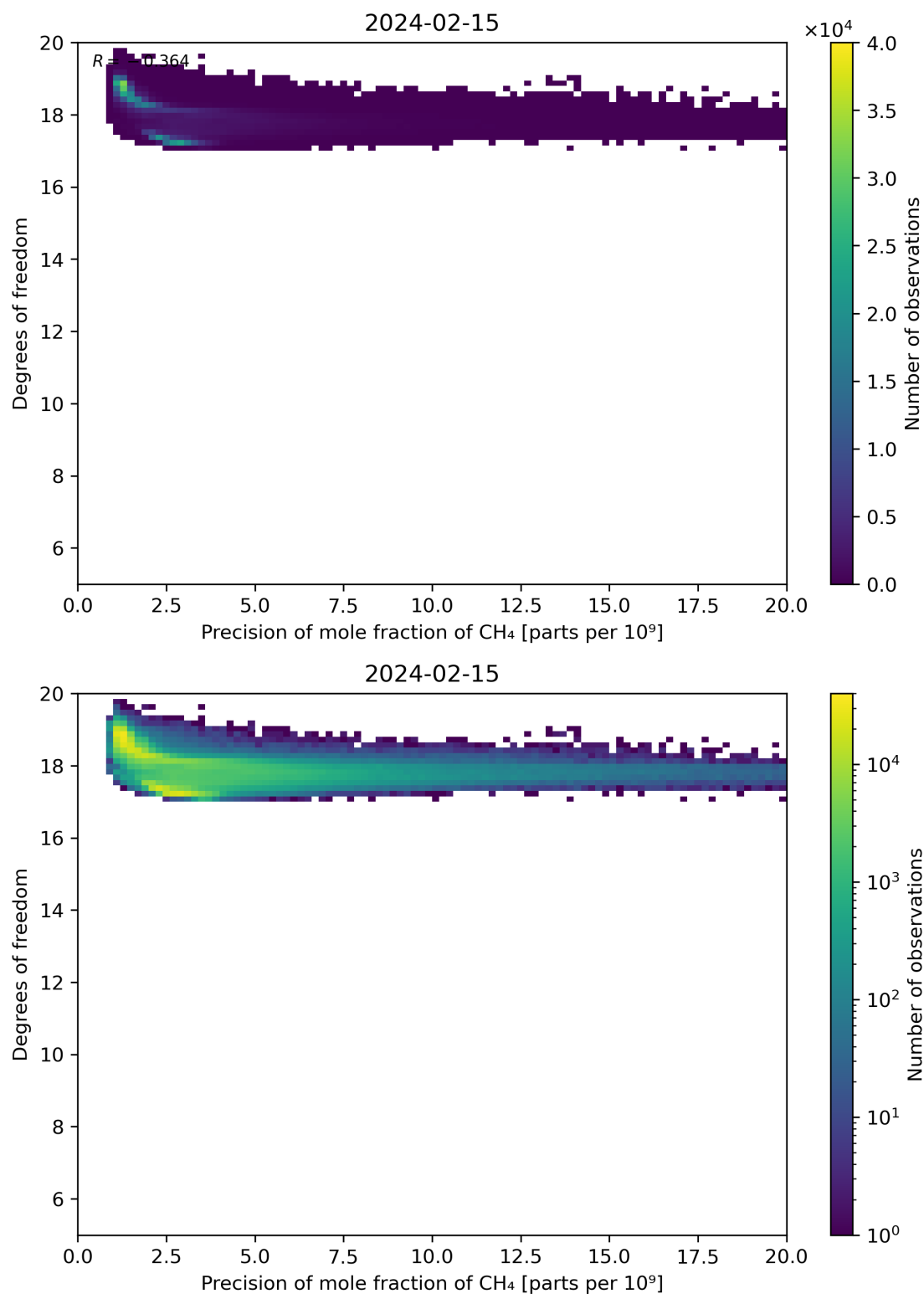
Figure 80: Scatter density plot of “Precision of mole fraction of CH 4 ” against “Degrees of freedom” for 2024-02-14 to 2024-02-16.
