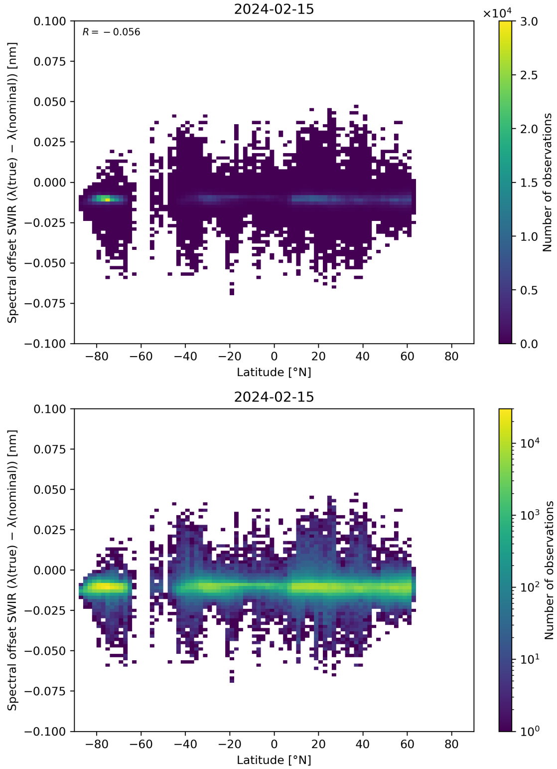
Figure 62: Scatter density plot of “Latitude” against “Spectral offset SWIR ( \lambda(\text{true}) - \lambda(\text{nominal}) )” for 2024-02-14 to 2024-02-16.
