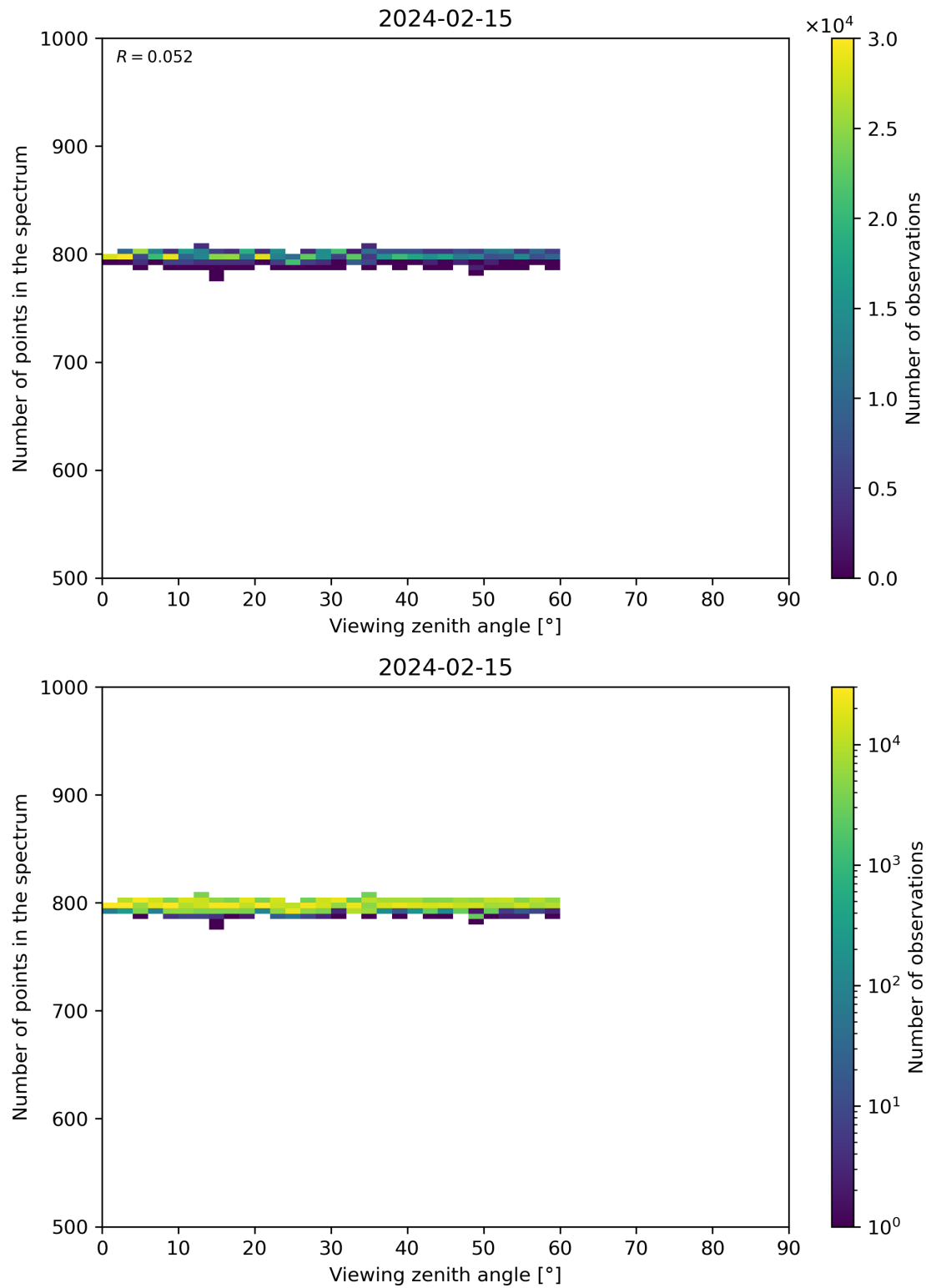
Figure 114: Scatter density plot of “Viewing zenith angle” against “Number of points in the spectrum” for 2024-02-14 to 2024-02-16.
