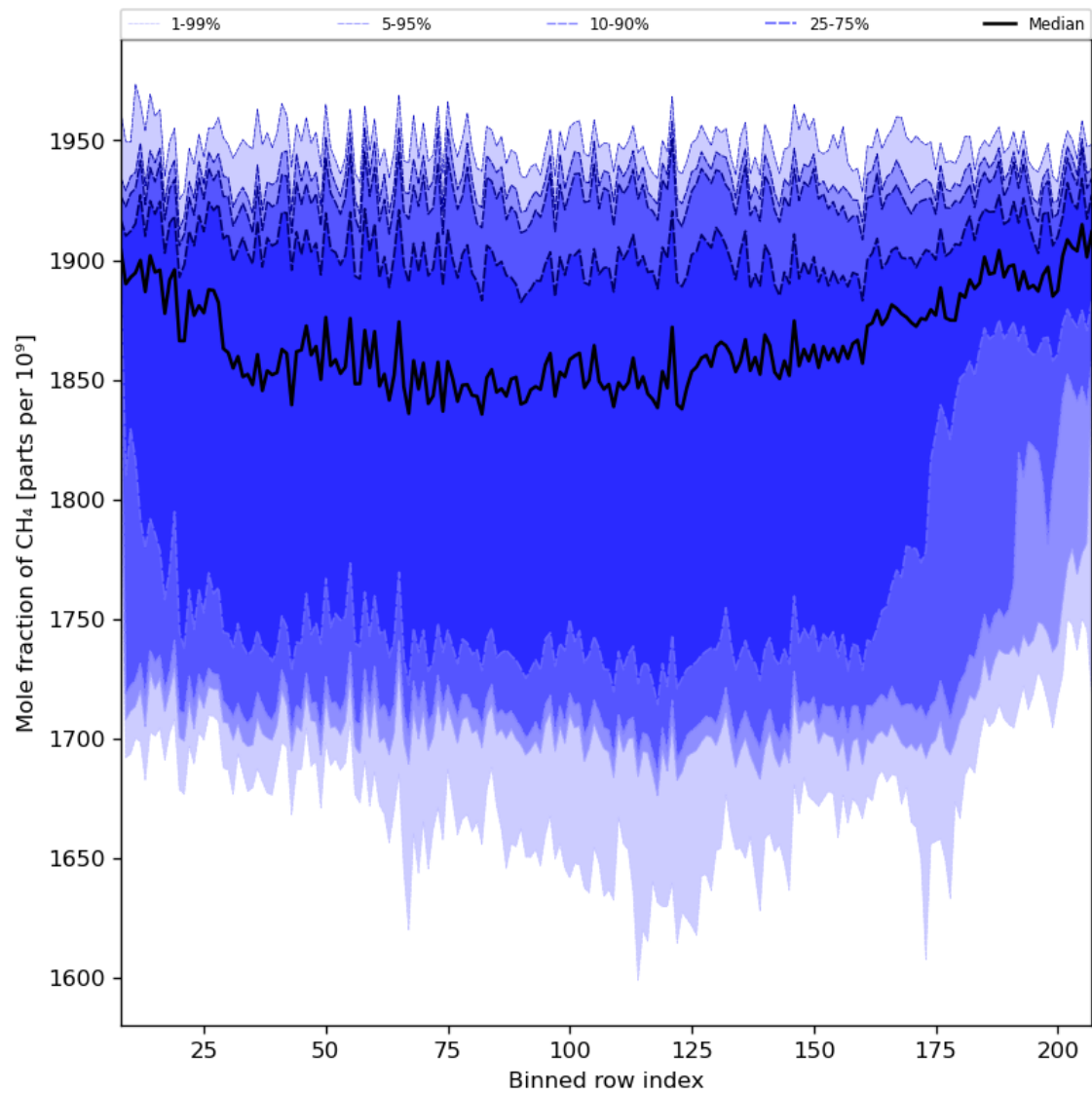
Figure 34: Along track statistics of “Mole fraction of CH 4 ” for 2024-02-14 to 2024-02-16
