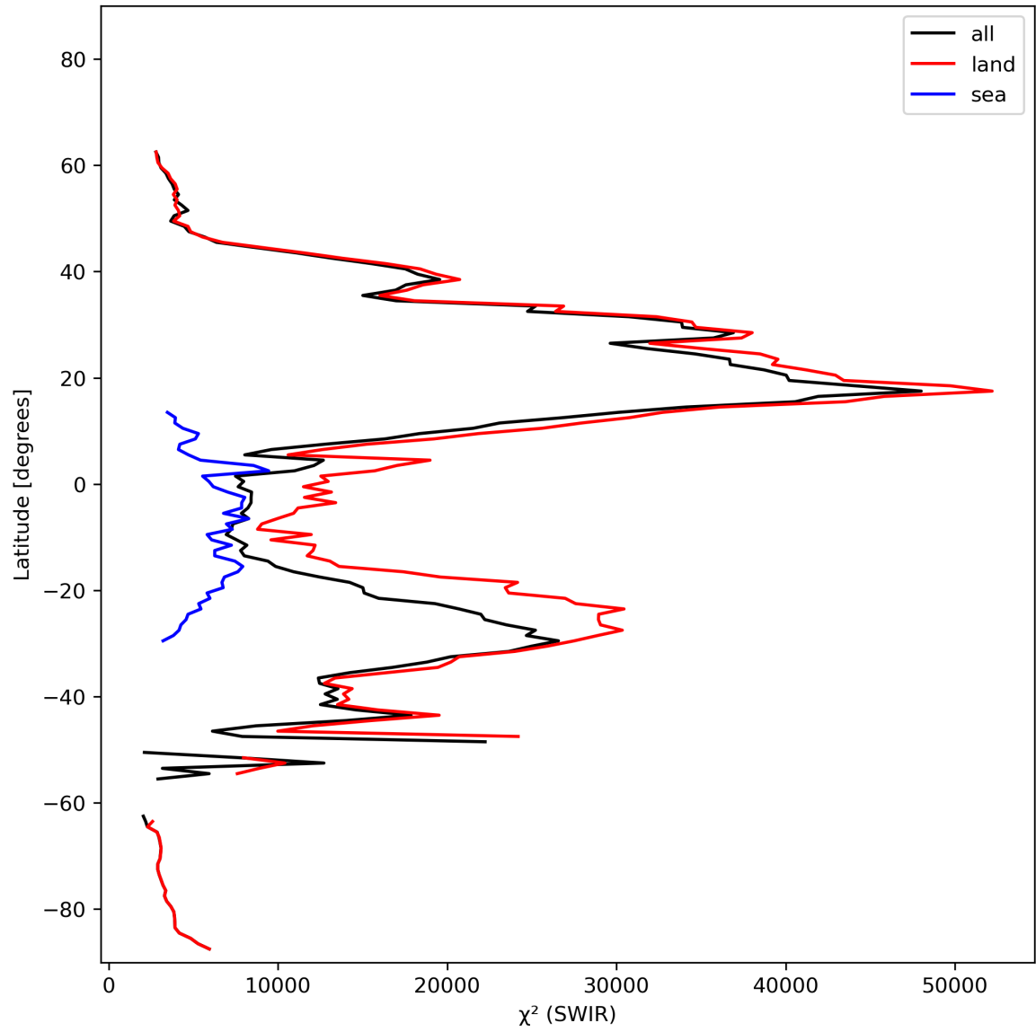
Figure 17: Zonal average of “ \chi^2 (SWIR)” for 2024-02-14 to 2024-02-16.
