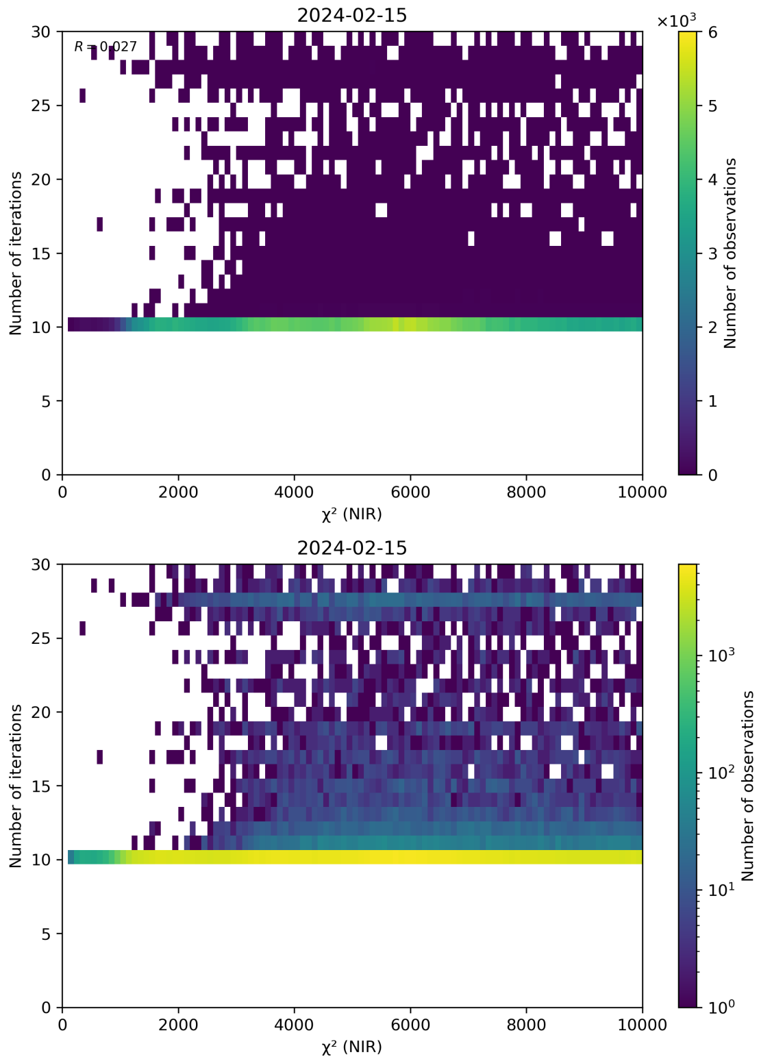
Figure 46: Scatter density plot of “ \chi^2 (NIR)” against “Number of iterations” for 2024-02-14 to 2024-02-16.
