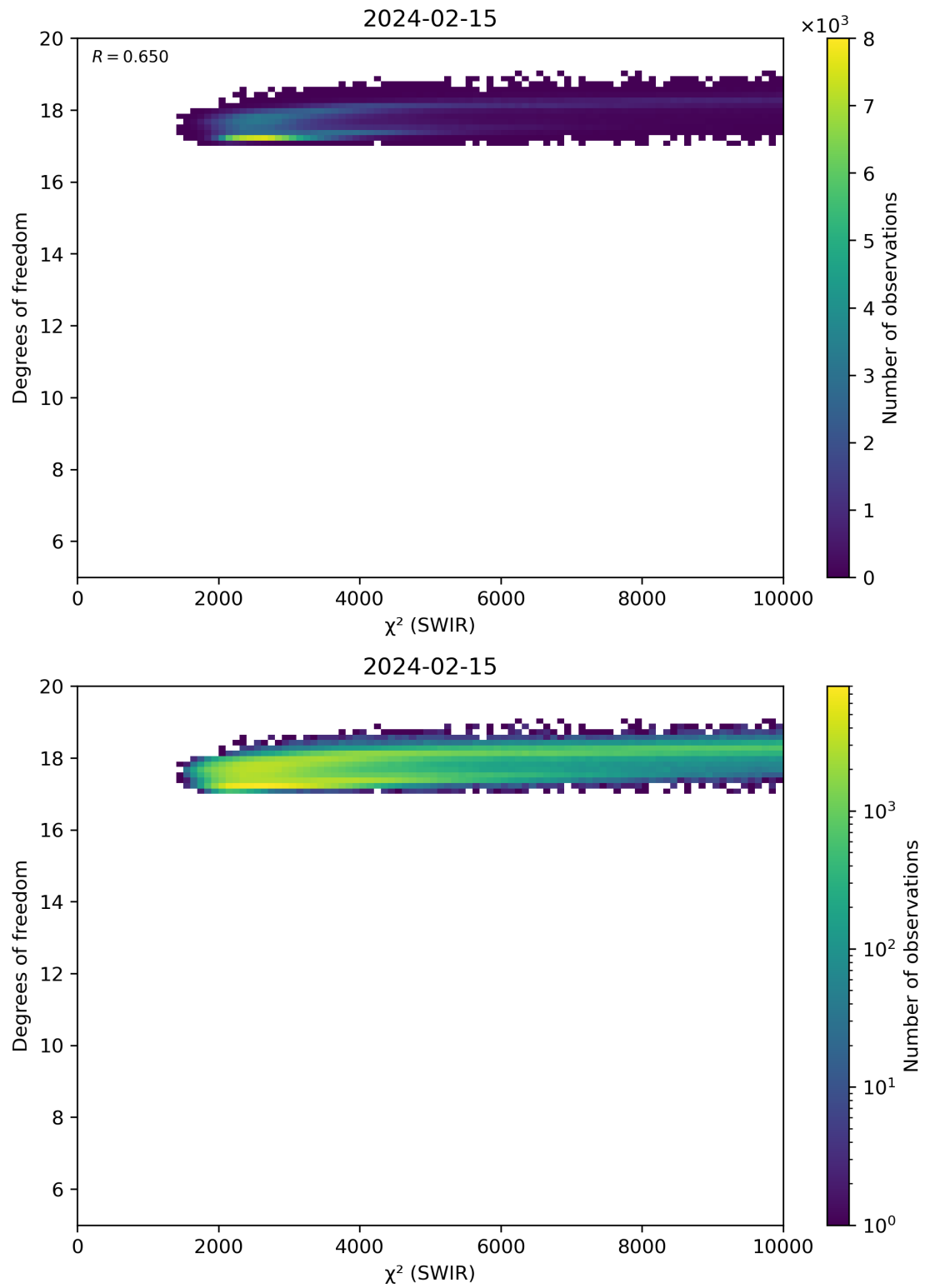
Figure 48: Scatter density plot of “ \chi^2 (SWIR)” against “Degrees of freedom” for 2024-02-14 to 2024-02-16.
