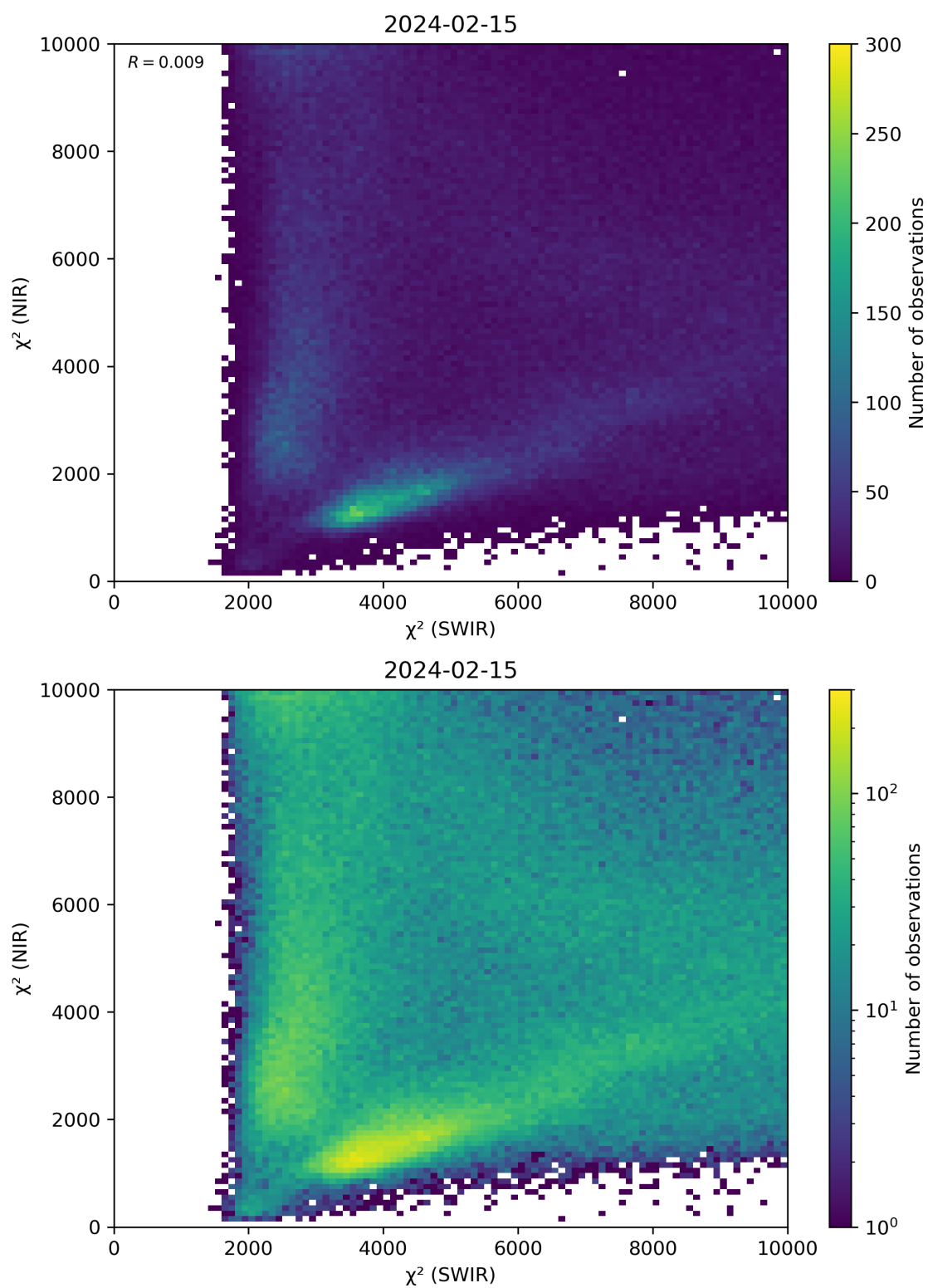
Figure 47: Scatter density plot of “ \chi^2 (SWIR)” against “ \chi^2 (NIR)” for 2024-02-14 to 2024-02-16.
