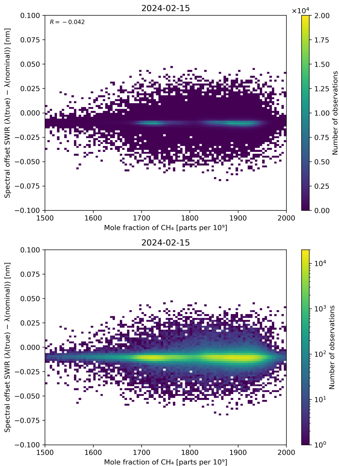
Figure 86: Scatter density plot of “Mole fraction of \text{CH}_4 ” against “Spectral offset SWIR ( \lambda(\text{true}) - \lambda(\text{nominal}) )” for 2024-02-14 to 2024-02-16.
