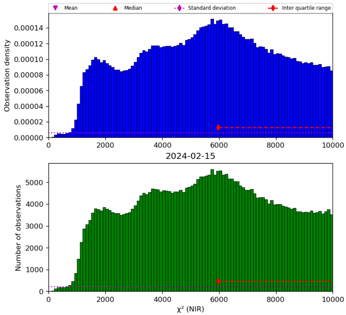
Figure 29: Histogram of “ \chi^2 (NIR)” for 2024-02-14 to 2024-02-16
