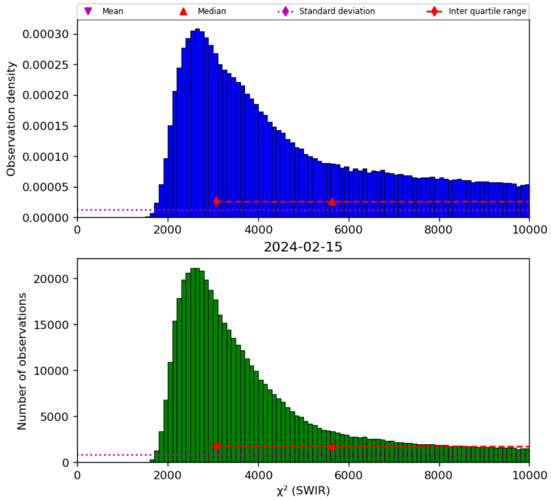
Figure 28: Histogram of “ \chi^2 (SWIR)” for 2024-02-14 to 2024-02-16
