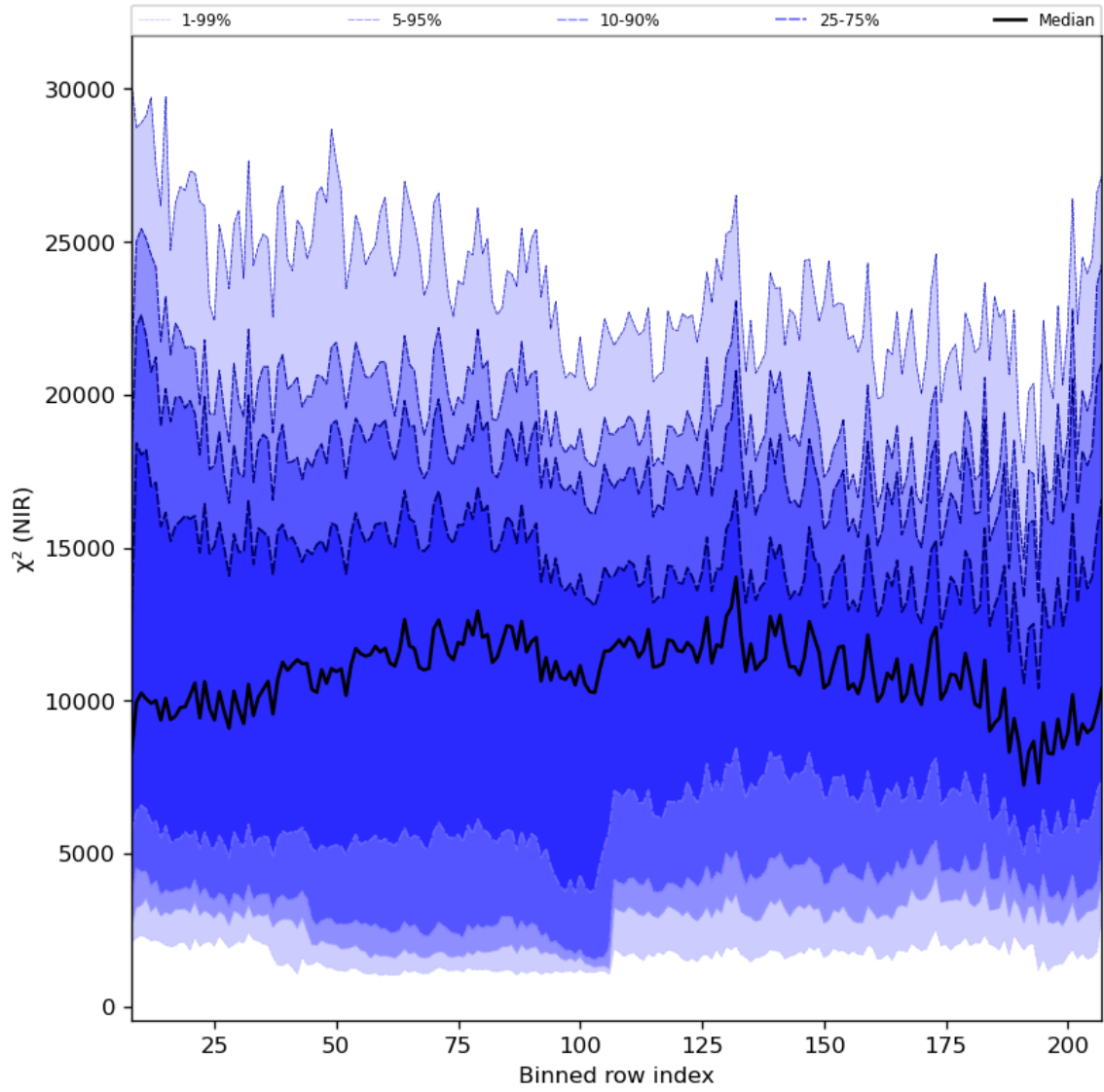
Figure 40: Along track statistics of “ \chi^2 (NIR)” for 2024-02-14 to 2024-02-16
