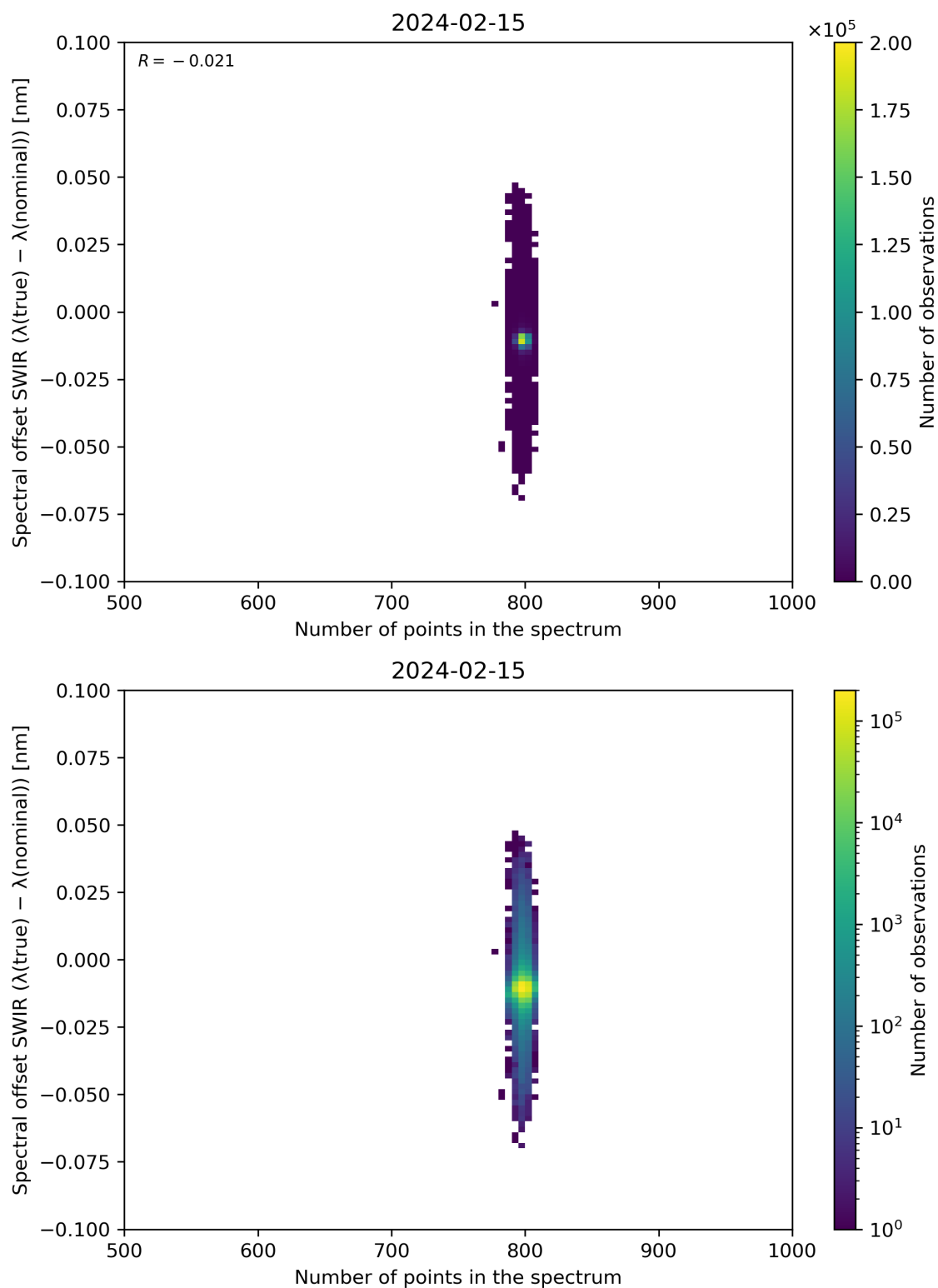
Figure 93: Scatter density plot of “Number of points in the spectrum” against “Spectral offset SWIR ( \lambda(\text{true}) - \lambda(\text{nominal}) )” for 2024-02-14 to 2024-02-16.
