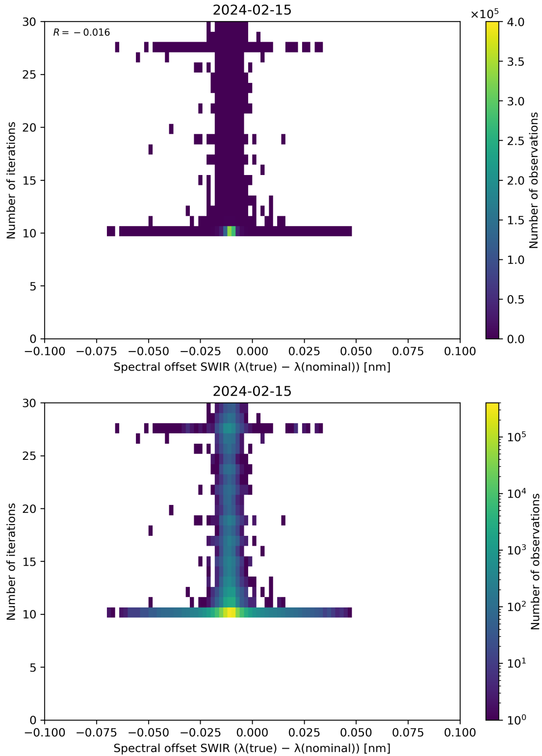
Figure 121: Scatter density plot of “Spectral offset SWIR ( \lambda(\text{true}) - \lambda(\text{nominal}) )” against “Number of iterations” for 2024-02-14 to 2024-02-16.
