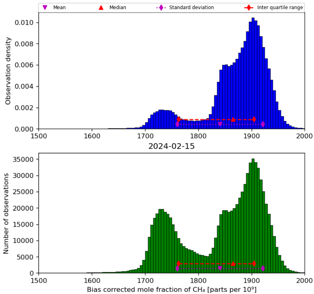
Figure 25: Histogram of “Bias corrected mole fraction of CH 4 ” for 2024-02-14 to 2024-02-16
