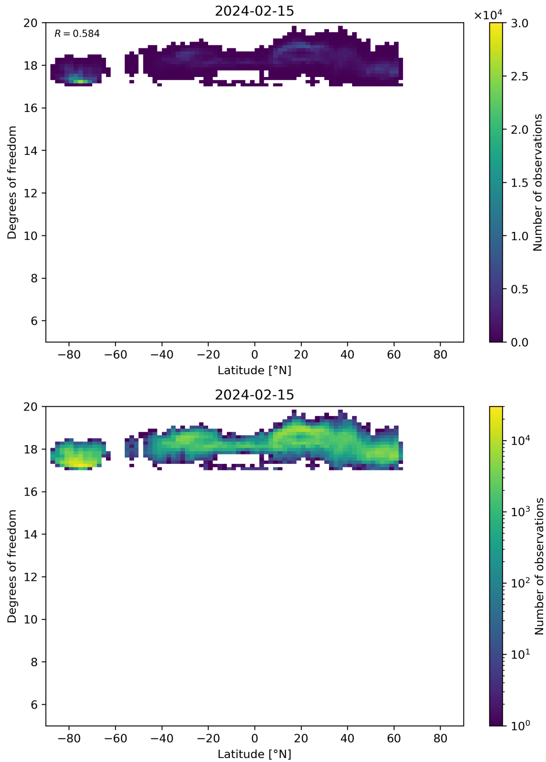
Figure 55: Scatter density plot of “Latitude” against “Degrees of freedom” for 2024-02-14 to 2024-02-16.
