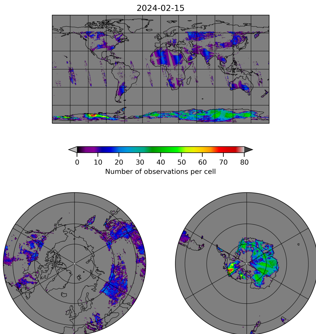
Figure 10: Map of the number of observations for 2024-02-14 to 2024-02-16
