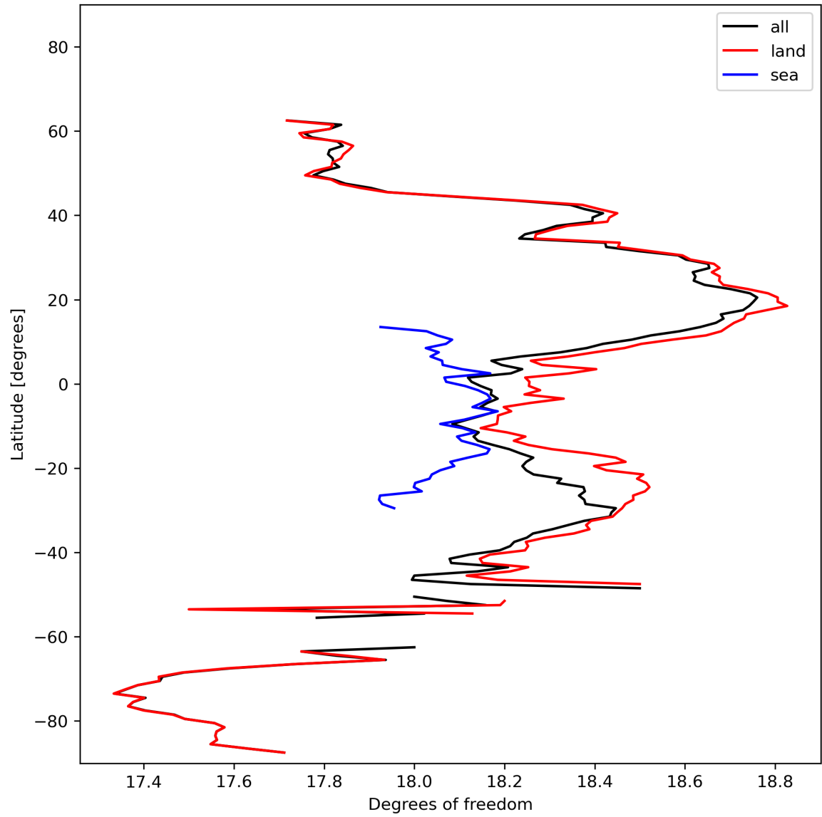
Figure 19: Zonal average of “Degrees of freedom” for 2024-02-14 to 2024-02-16.
