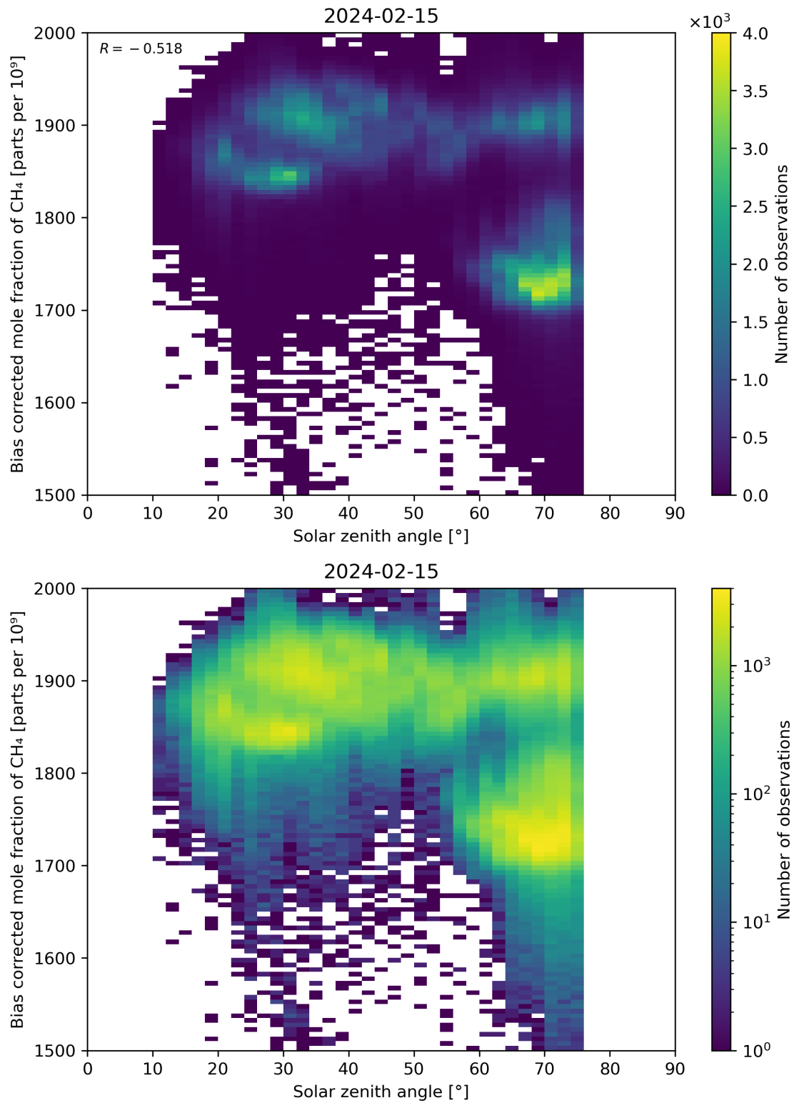
Figure 100: Scatter density plot of “Solar zenith angle” against “Bias corrected mole fraction of CH 4 ” for 2024-02-14 to 2024-02-16.
