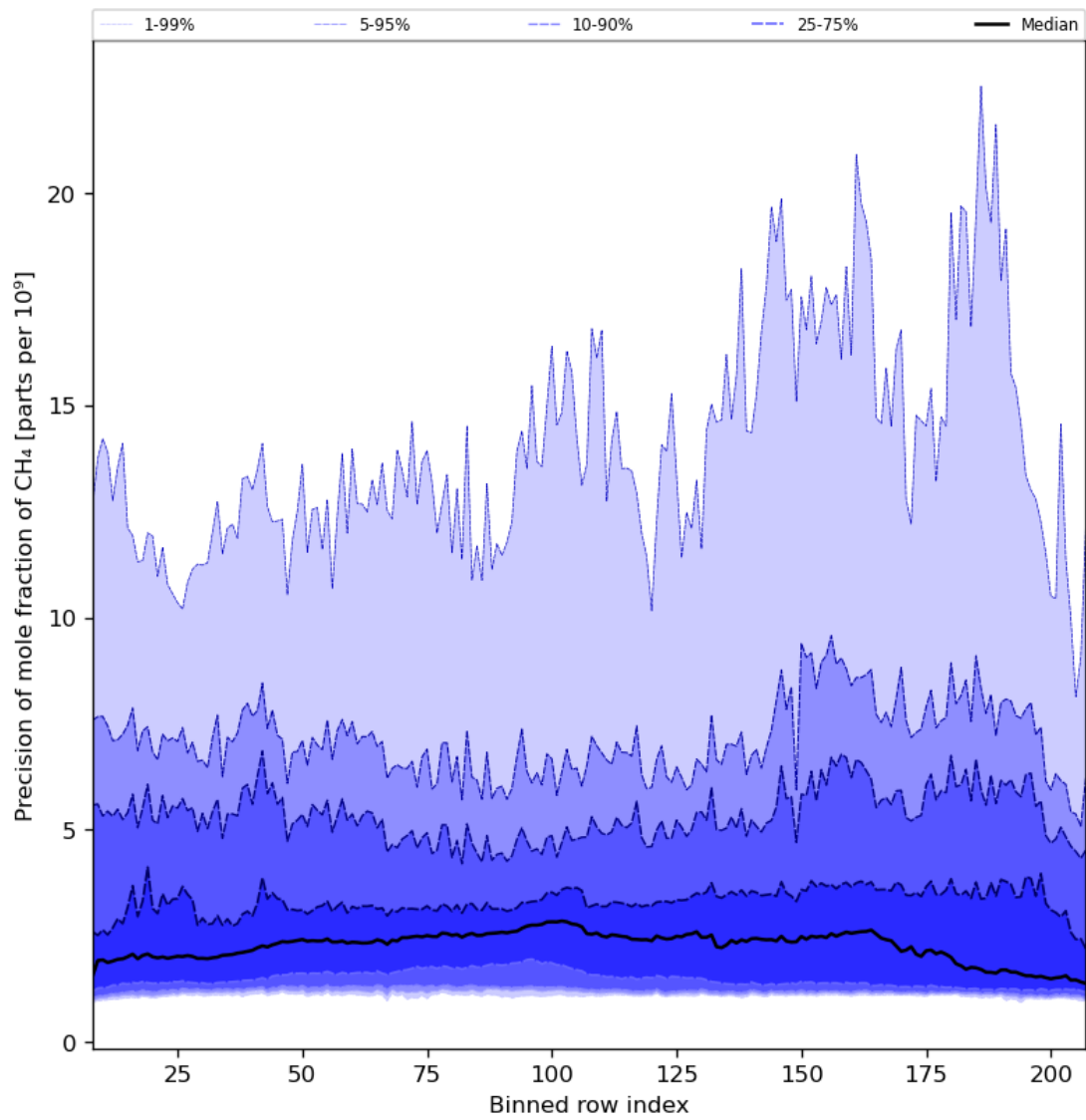
Figure 35: Along track statistics of “Precision of mole fraction of CH 4 ” for 2024-02-14 to 2024-02-16
