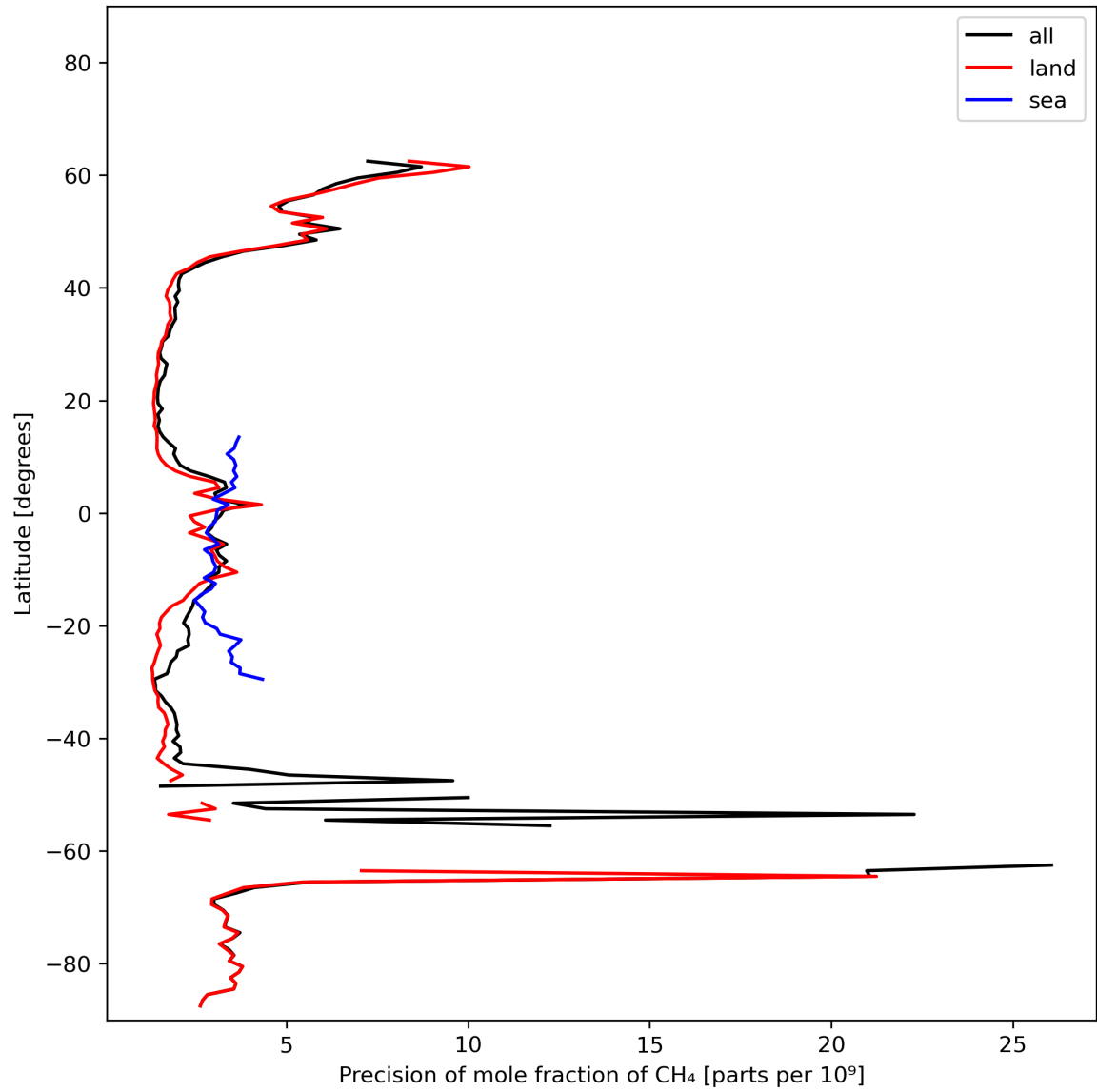
Figure 13: Zonal average of “Precision of mole fraction of CH 4 ” for 2024-02-14 to 2024-02-16.
