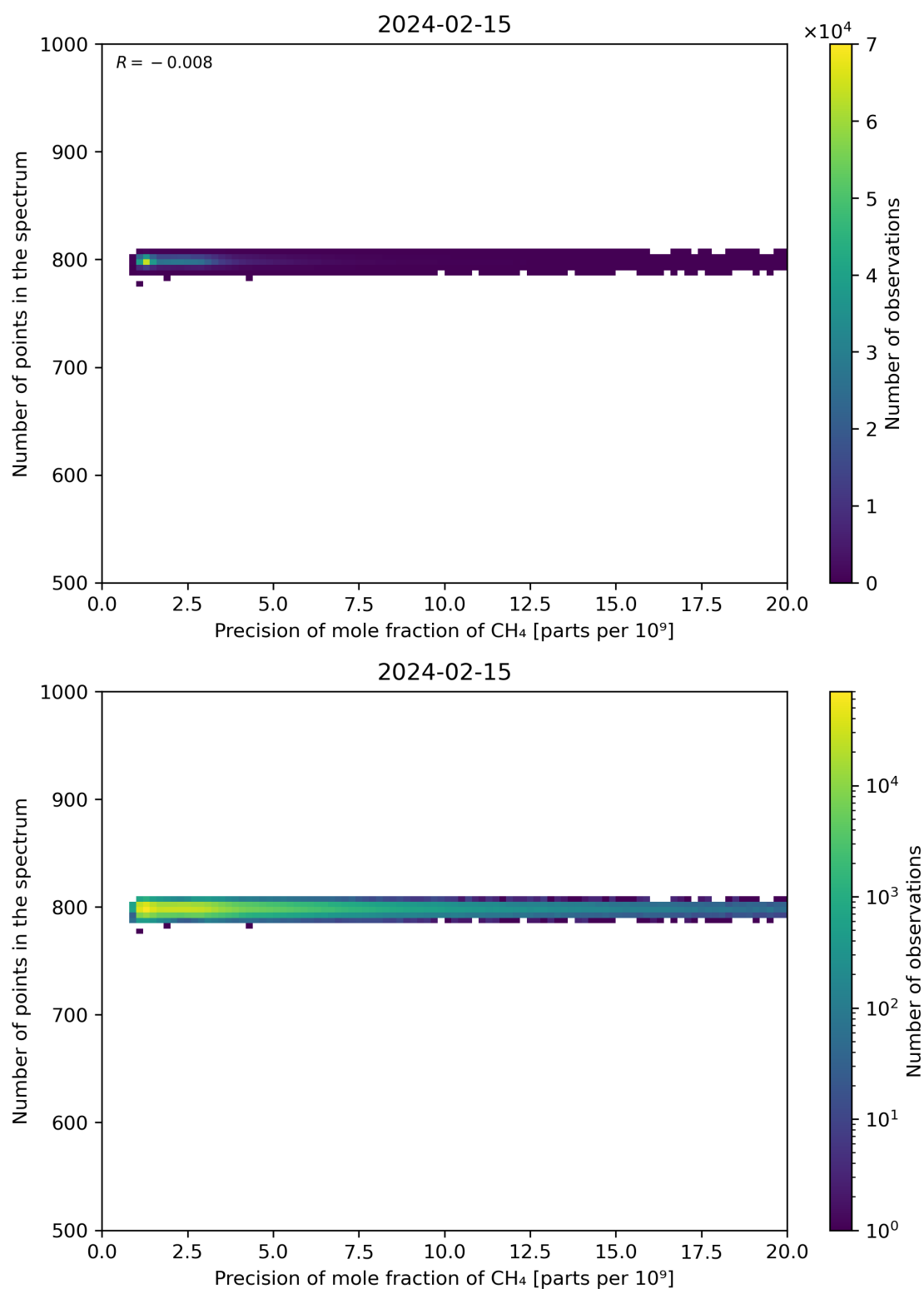
Figure 84: Scatter density plot of “Precision of mole fraction of CH 4 ” against “Number of points in the spectrum” for 2024-02-14 to 2024-02-16.
