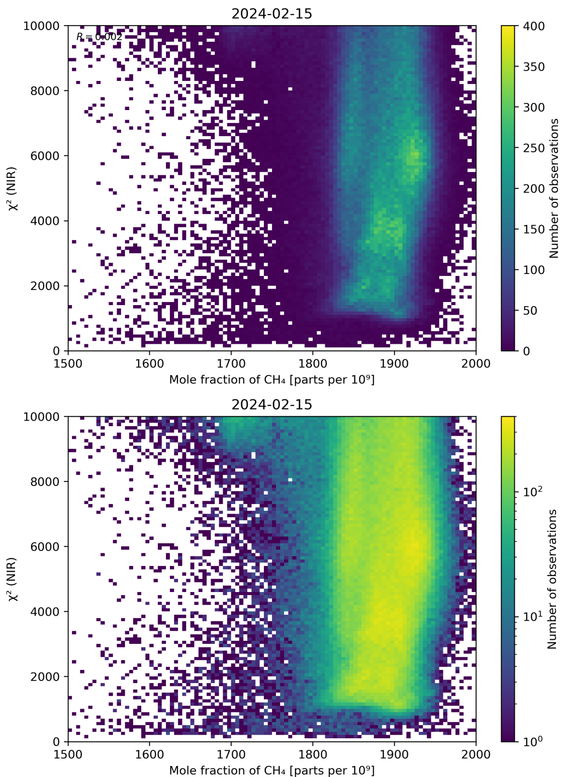
Figure 70: Scatter density plot of “Mole fraction of CH 4 ” against “ \chi^2 (NIR)” for 2024-02-14 to 2024-02-16.
