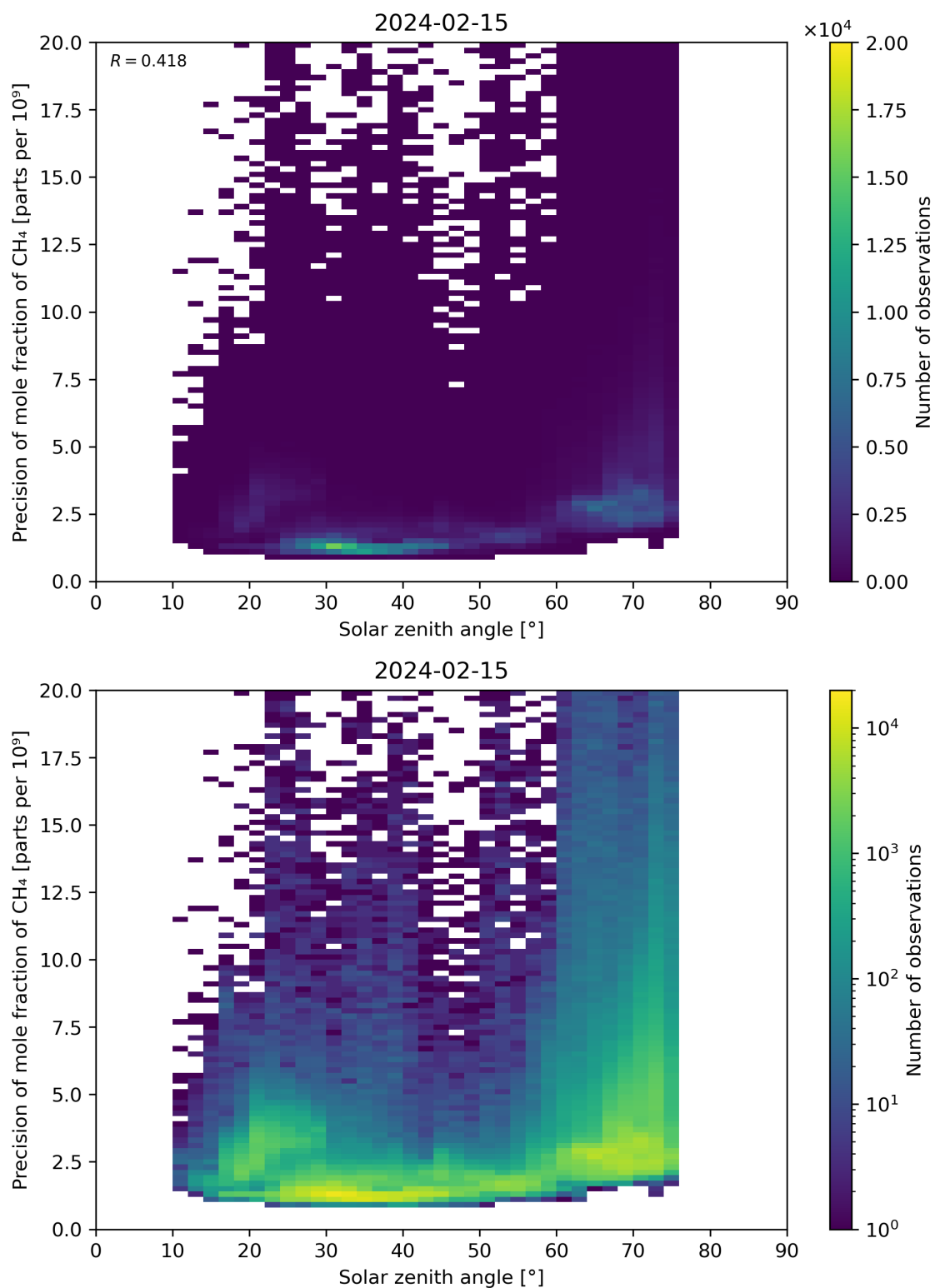
Figure 101: Scatter density plot of “Solar zenith angle” against “Precision of mole fraction of CH 4 ” for 2024-02-14 to 2024-02-16.
