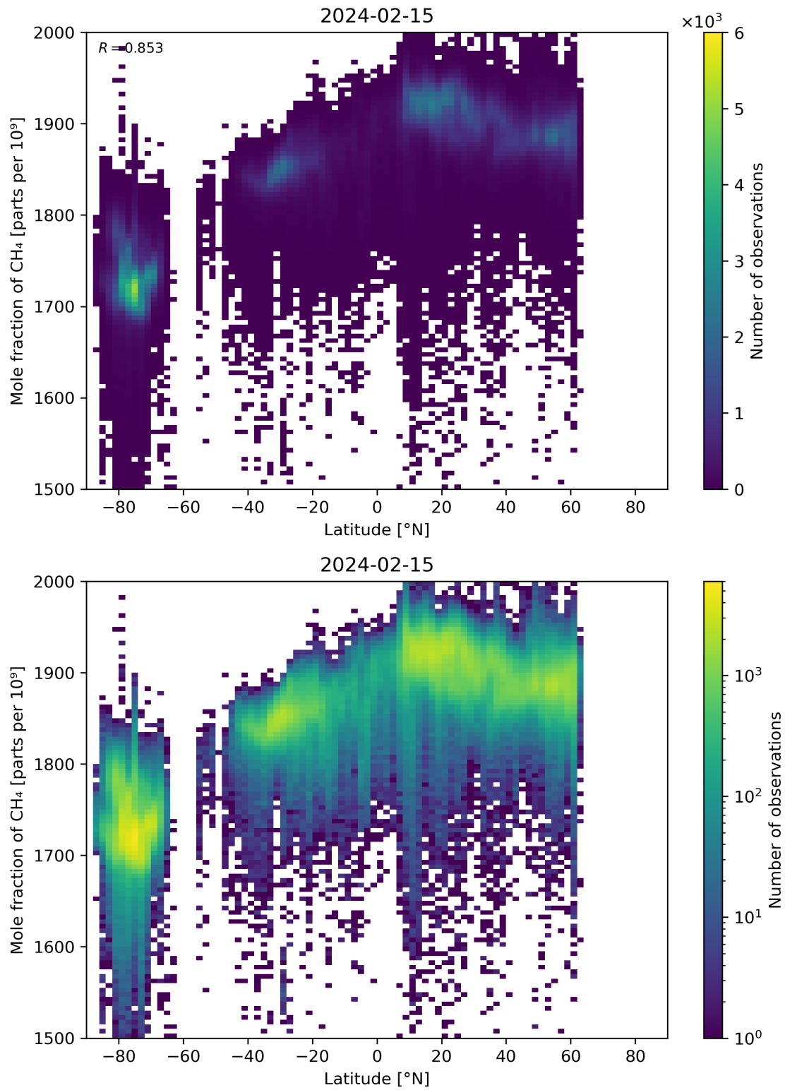
Figure 57: Scatter density plot of “Latitude” against “Mole fraction of CH 4 ” for 2024-02-14 to 2024-02-16.
