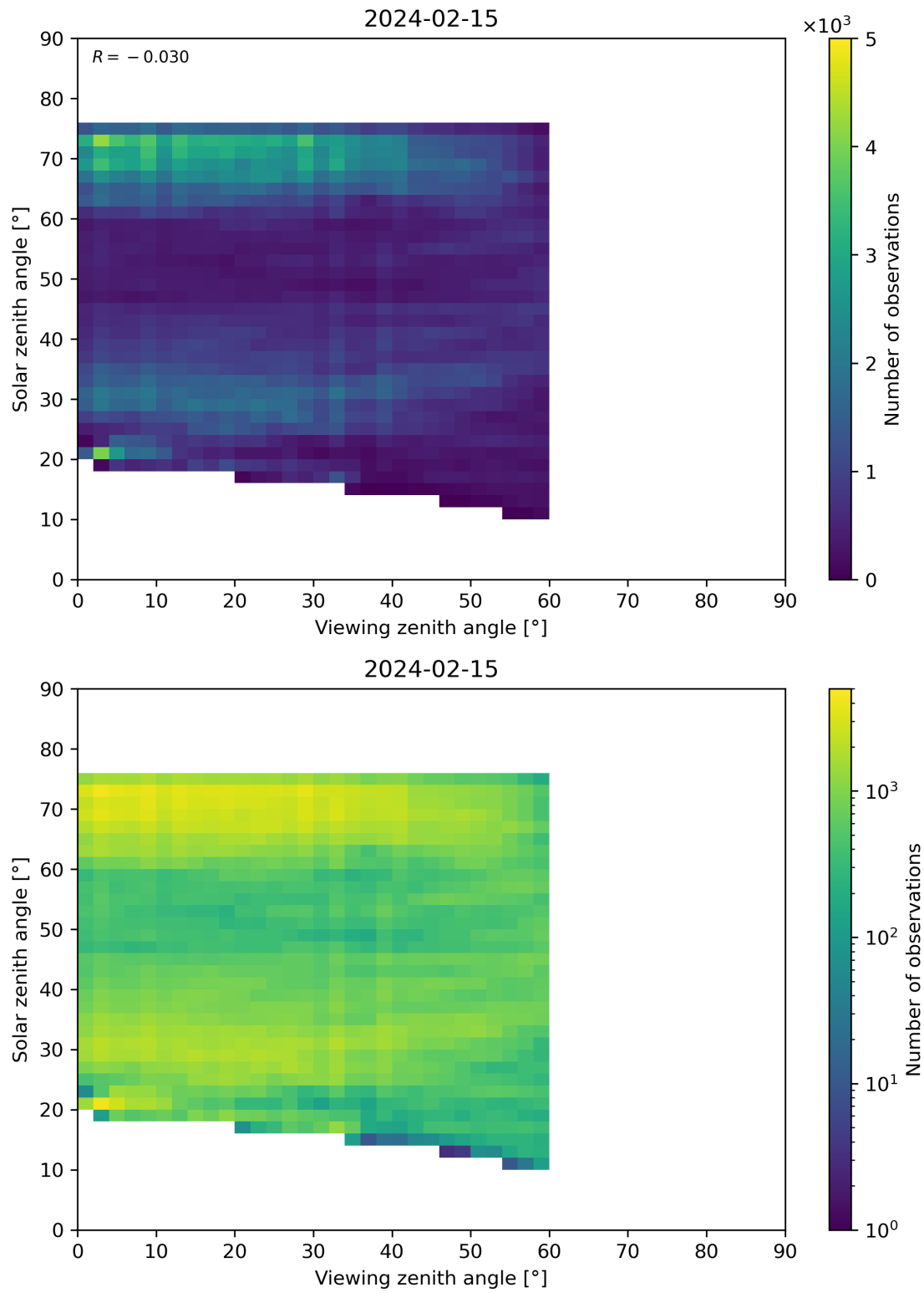
Figure 115: Scatter density plot of “Viewing zenith angle” against “Solar zenith angle” for 2024-02-14 to 2024-02-16.
