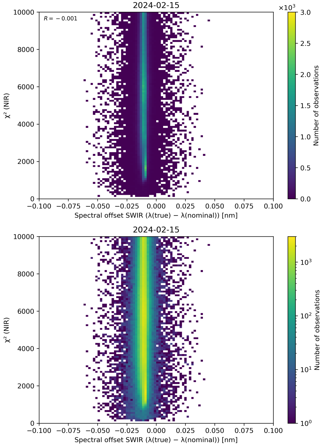
Figure 117: Scatter density plot of “Spectral offset SWIR ( \lambda(\text{true}) - \lambda(\text{nominal}) )” against “ \chi^2 (NIR)” for 2024-02-14 to 2024-02-16.
