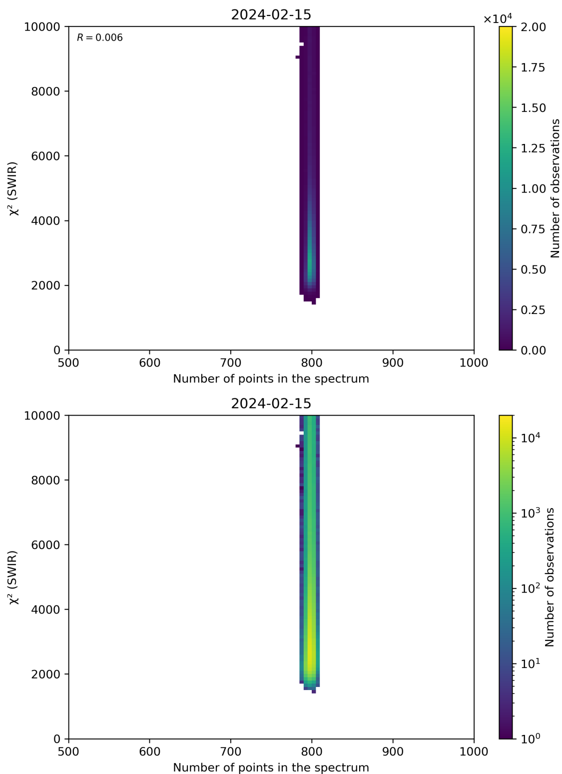
Figure 89: Scatter density plot of “Number of points in the spectrum” against “ \chi^2 (SWIR)” for 2024-02-14 to 2024-02-16.
