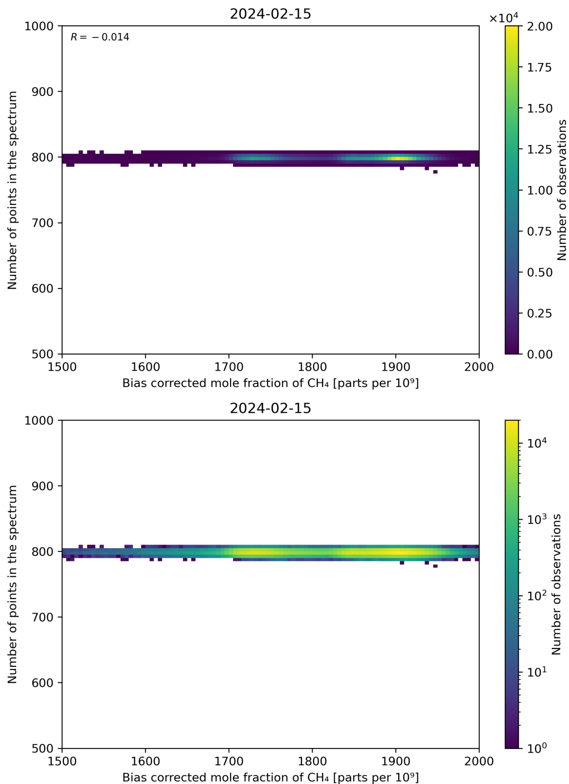
Figure 68: Scatter density plot of “Bias corrected mole fraction of CH 4 ” against “Number of points in the spectrum” for 2024-02-14 to 2024-02-16.
