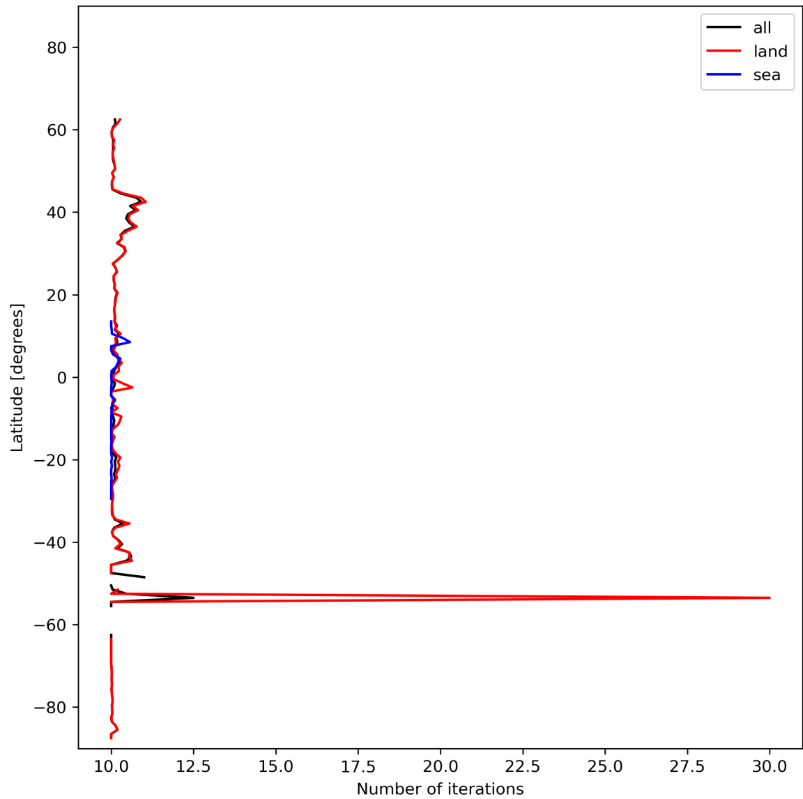
Figure 20: Zonal average of “Number of iterations” for 2024-02-14 to 2024-02-16.
