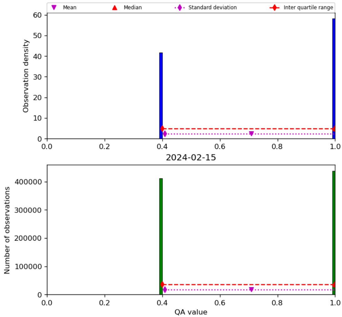
Figure 22: Histogram of “QA value” for 2024-02-14 to 2024-02-16
