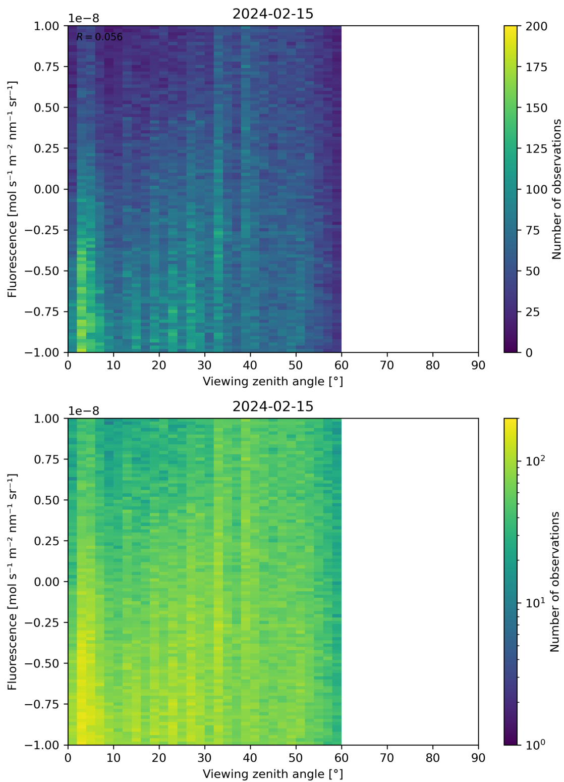
Figure 108: Scatter density plot of “Viewing zenith angle” against “Fluorescence” for 2024-02-14 to 2024-02-16.
