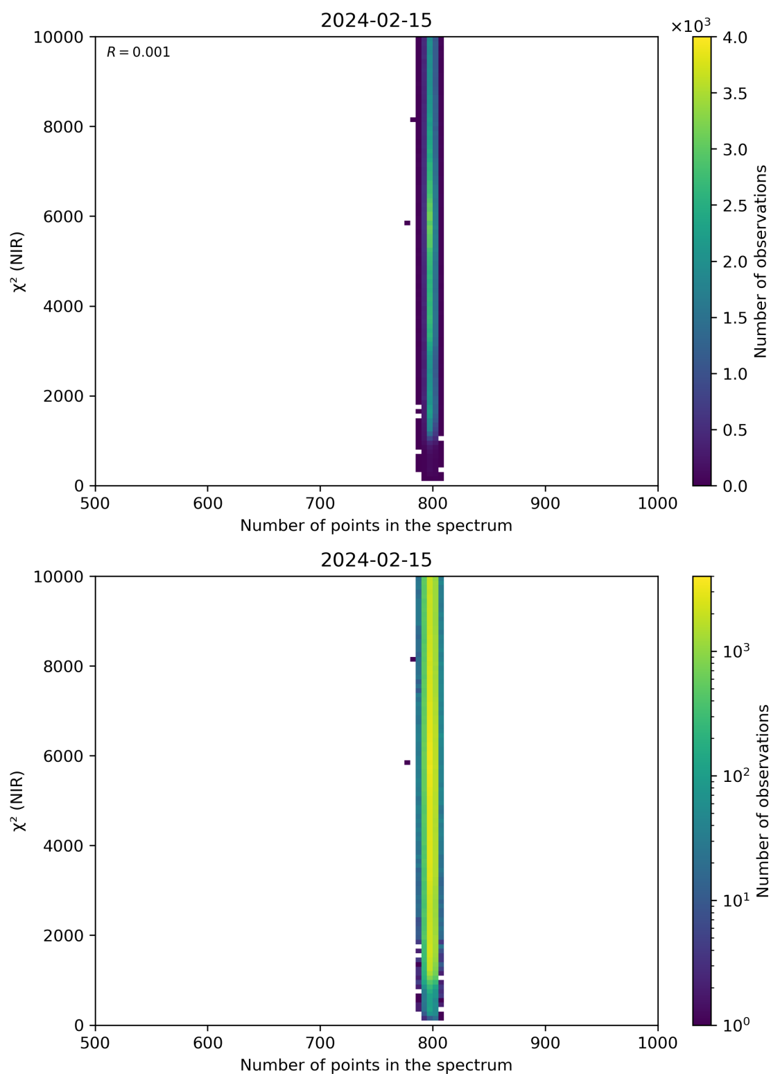
Figure 88: Scatter density plot of “Number of points in the spectrum” against “ \chi^2 (NIR)” for 2024-02-14 to 2024-02-16.
