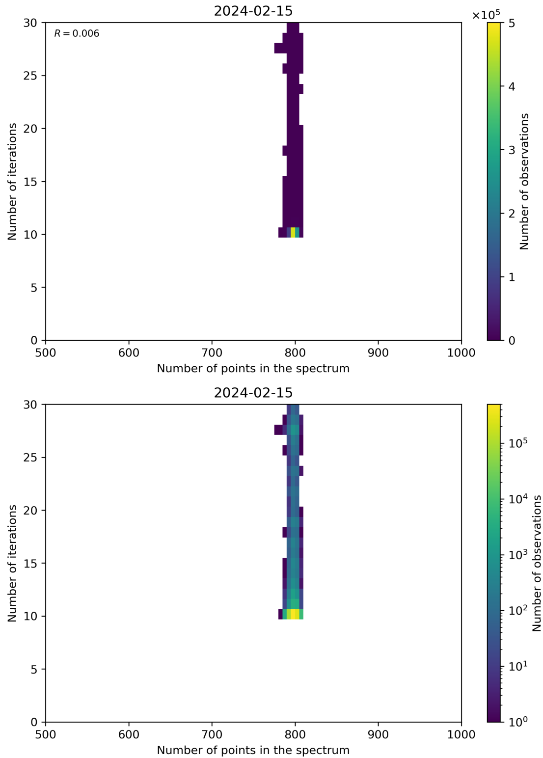
Figure 92: Scatter density plot of “Number of points in the spectrum” against “Number of iterations” for 2024-02-14 to 2024-02-16.
