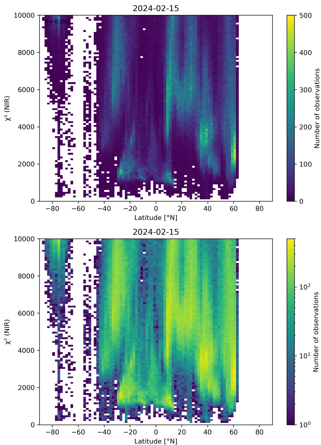
Figure 53: Scatter density plot of “Latitude” against “ \chi^2 (NIR)” for 2024-02-14 to 2024-02-16.
