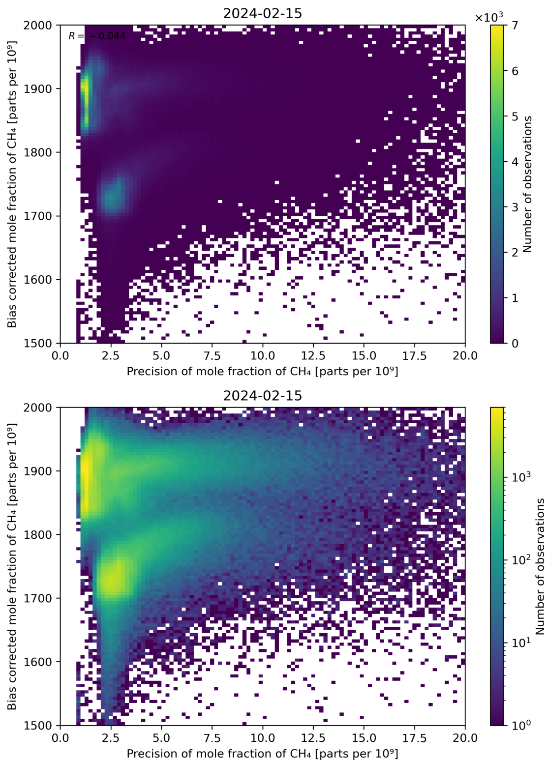
Figure 82: Scatter density plot of “Precision of mole fraction of CH 4 ” against “Bias corrected mole fraction of CH 4 ” for 2024-02-14 to 2024-02-16.
