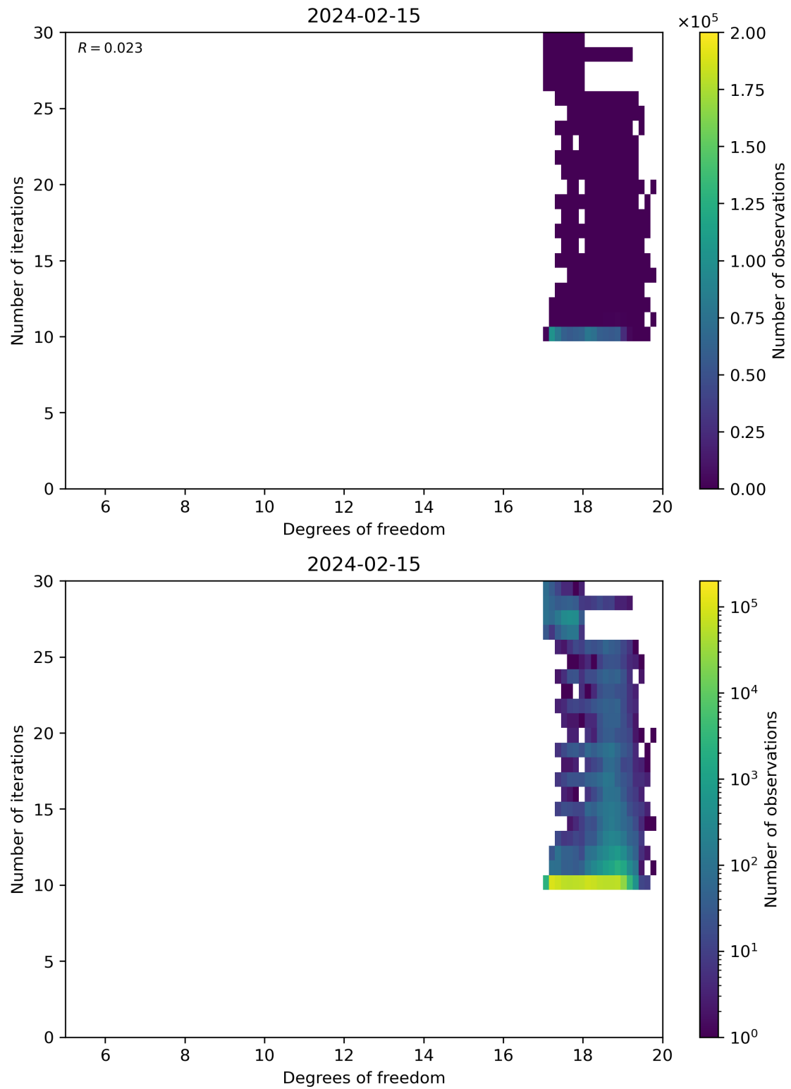
Figure 52: Scatter density plot of “Degrees of freedom” against “Number of iterations” for 2024-02-14 to 2024-02-16.
