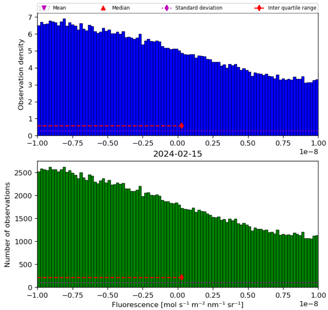
Figure 32: Histogram of “Fluorescence” for 2024-02-14 to 2024-02-16
