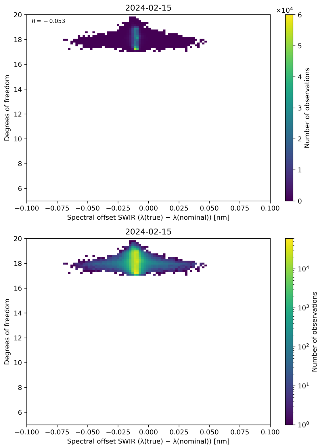
Figure 119: Scatter density plot of “Spectral offset SWIR ( \lambda(\text{true}) - \lambda(\text{nominal}) )” against “Degrees of freedom” for 2024-02-14 to 2024-02-16.
