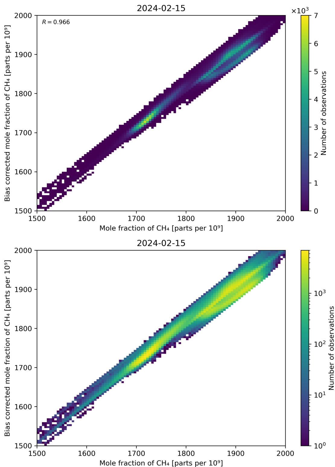
Figure 74: Scatter density plot of “Mole fraction of CH 4 ” against “Bias corrected mole fraction of CH 4 ” for 2024-02-14 to 2024-02-16.
