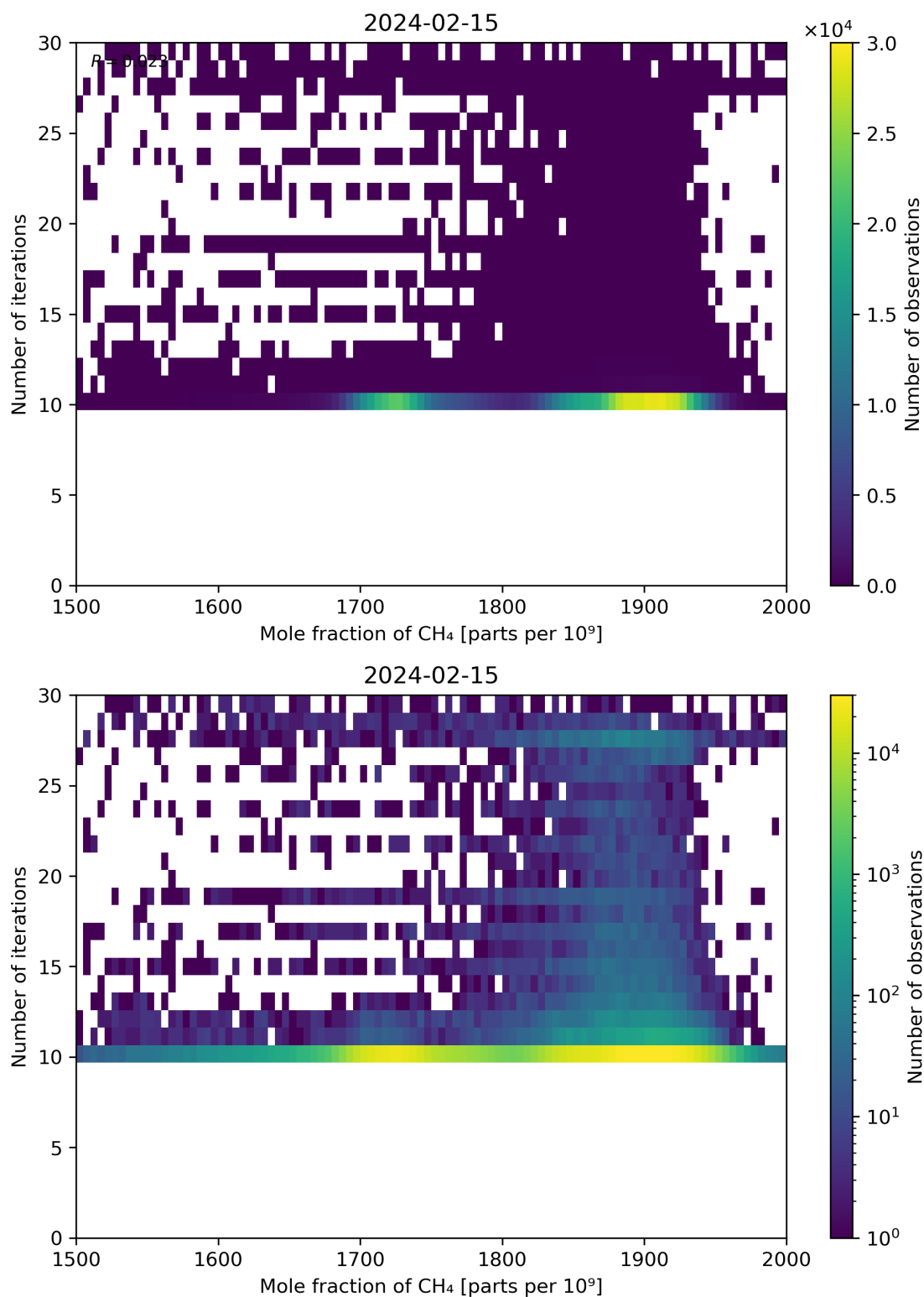
Figure 76: Scatter density plot of “Mole fraction of CH 4 ” against “Number of iterations” for 2024-02-14 to 2024-02-16.
