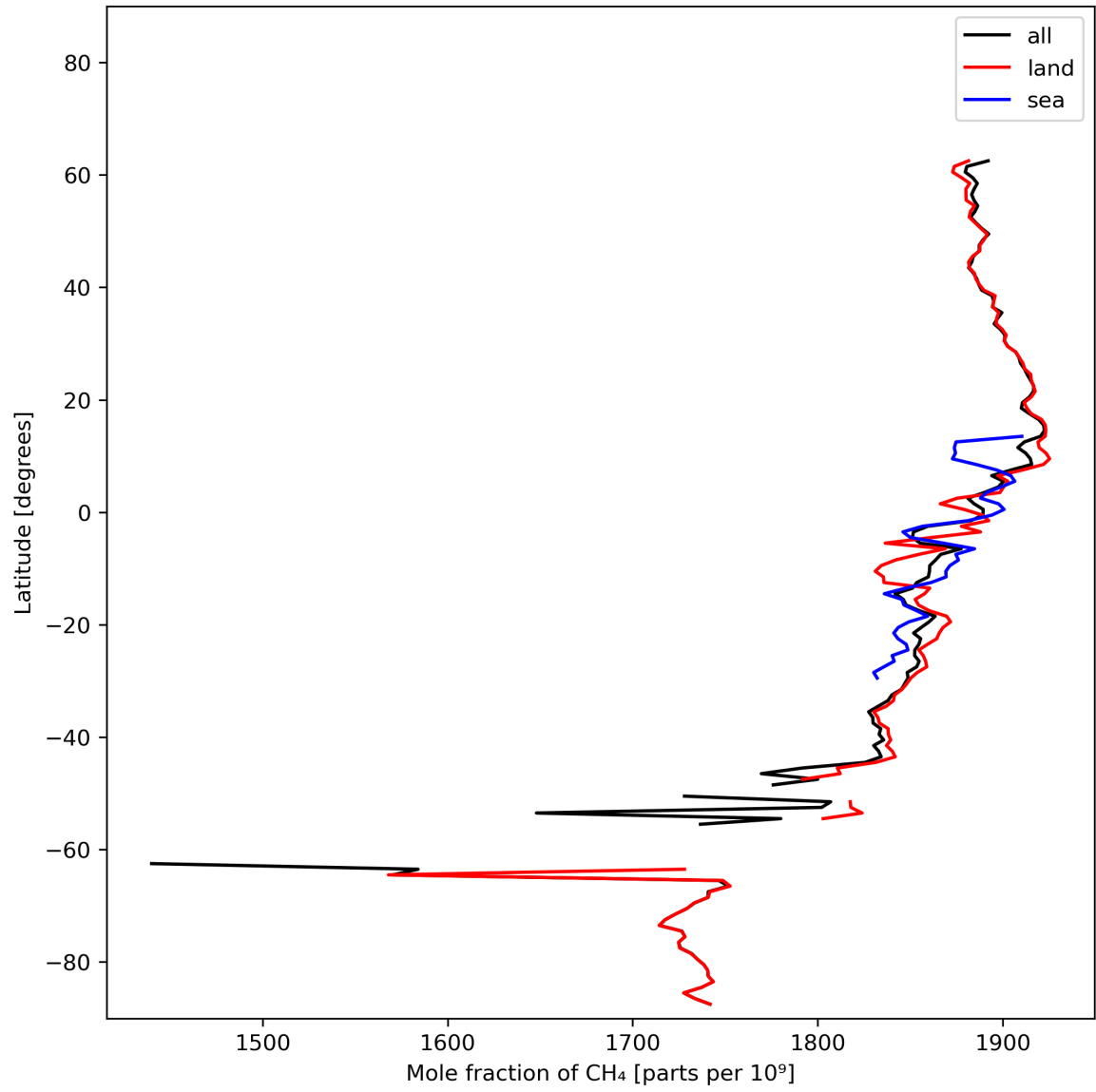
Figure 12: Zonal average of “Mole fraction of \text{CH}_4 ” for 2024-02-14 to 2024-02-16.
