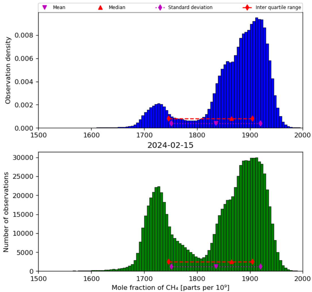
Figure 23: Histogram of “Mole fraction of CH 4 ” for 2024-02-14 to 2024-02-16
