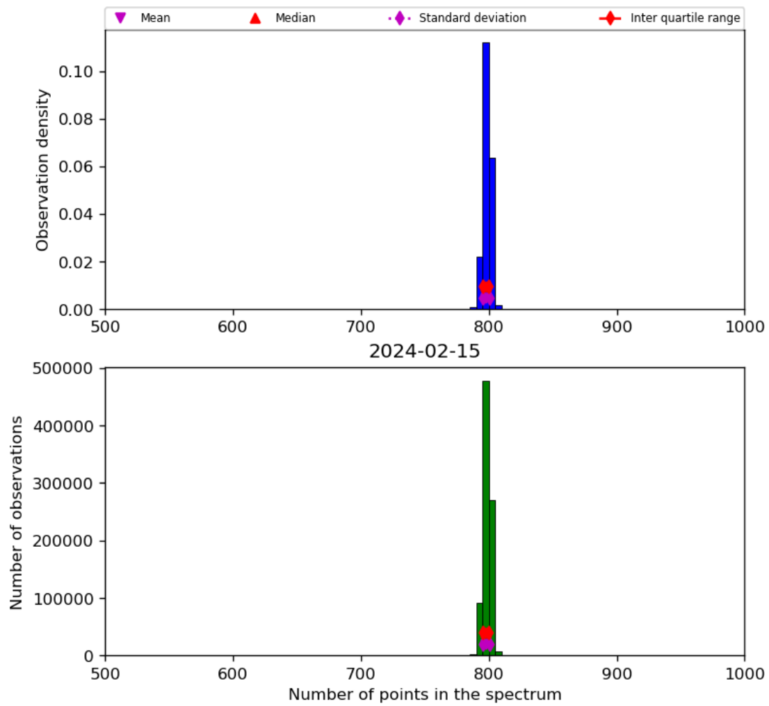
Figure 26: Histogram of “Number of points in the spectrum” for 2024-02-14 to 2024-02-16
