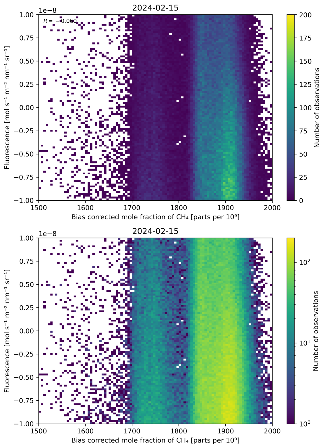
Figure 66: Scatter density plot of “Bias corrected mole fraction of \text{CH}_4 ” against “Fluorescence” for 2024-02-14 to 2024-02-16.
