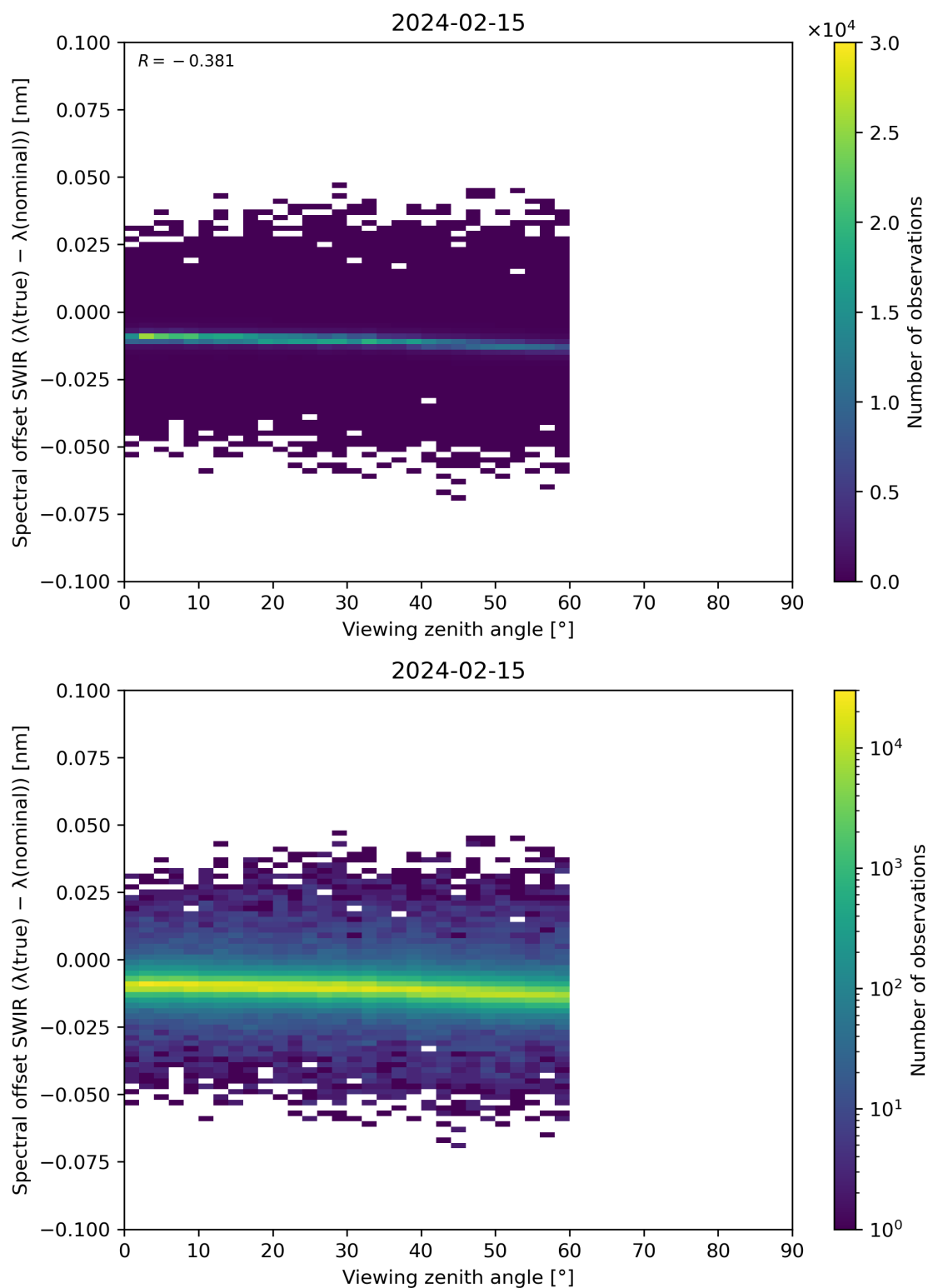
Figure 116: Scatter density plot of “Viewing zenith angle” against “Spectral offset SWIR ( \lambda(\text{true}) - \lambda(\text{nominal}) )” for 2024-02-14 to 2024-02-16.
