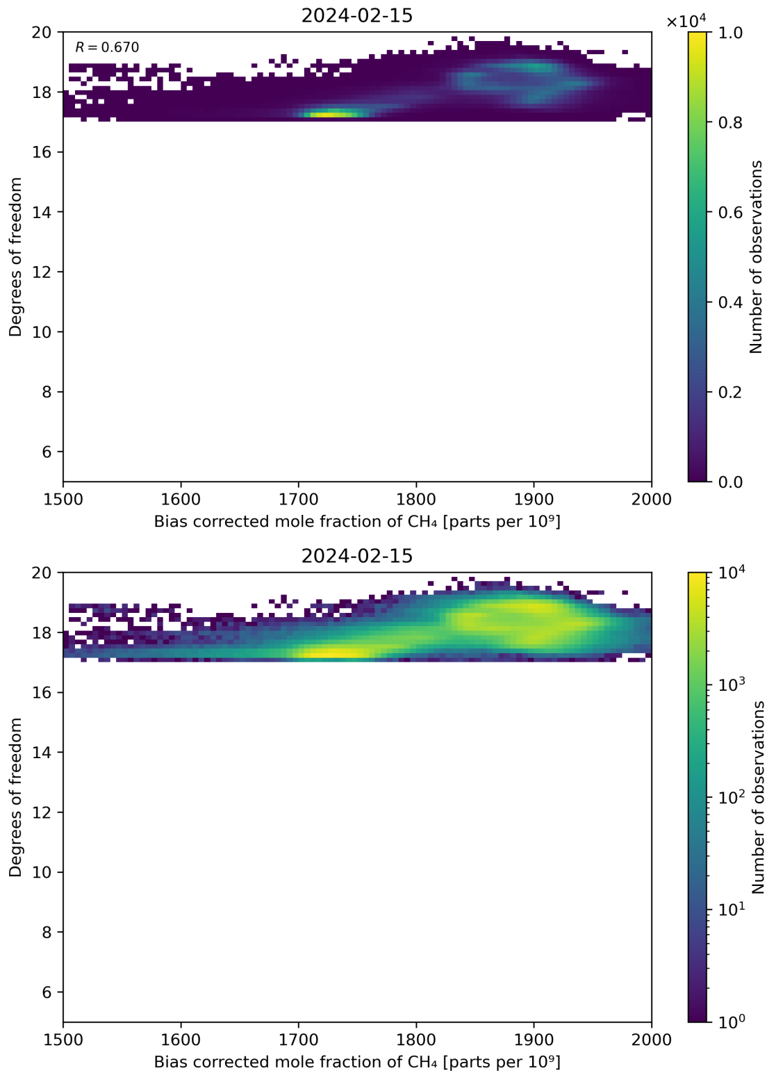
Figure 65: Scatter density plot of “Bias corrected mole fraction of \text{CH}_4 ” against “Degrees of freedom” for 2024-02-14 to 2024-02-16.
