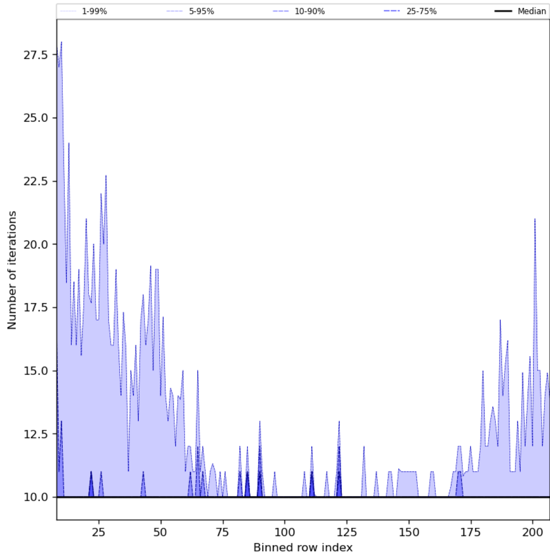
Figure 42: Along track statistics of “Number of iterations” for 2024-02-14 to 2024-02-16
