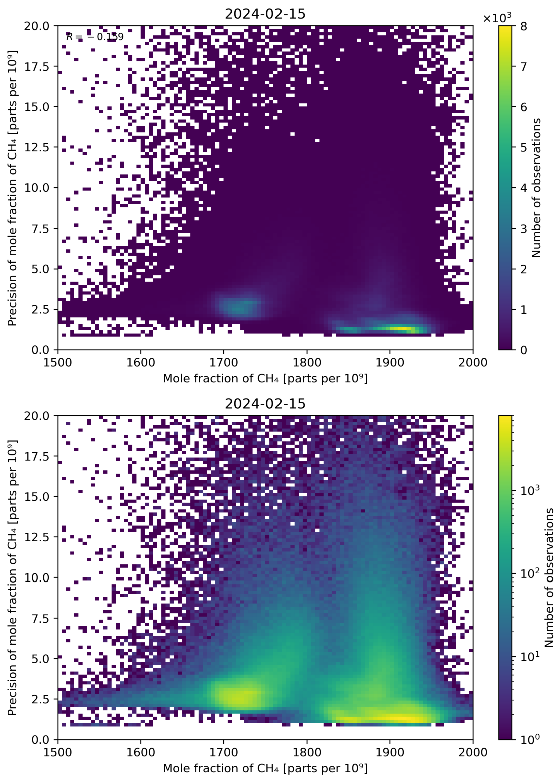
Figure 75: Scatter density plot of “Mole fraction of CH 4 ” against “Precision of mole fraction of CH 4 ” for 2024-02-14 to 2024-02-16.
