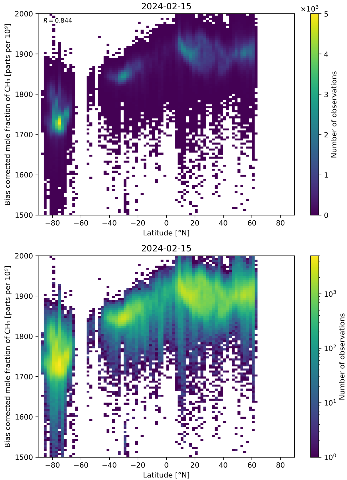
Figure 58: Scatter density plot of “Latitude” against “Bias corrected mole fraction of \text{CH}_4 ” for 2024-02-14 to 2024-02-16.
