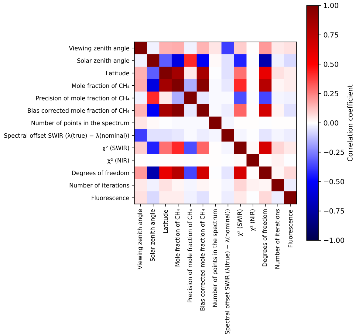
Figure 2: Map of correlation matrix for 2024-02-14 to 2024-02-16.
