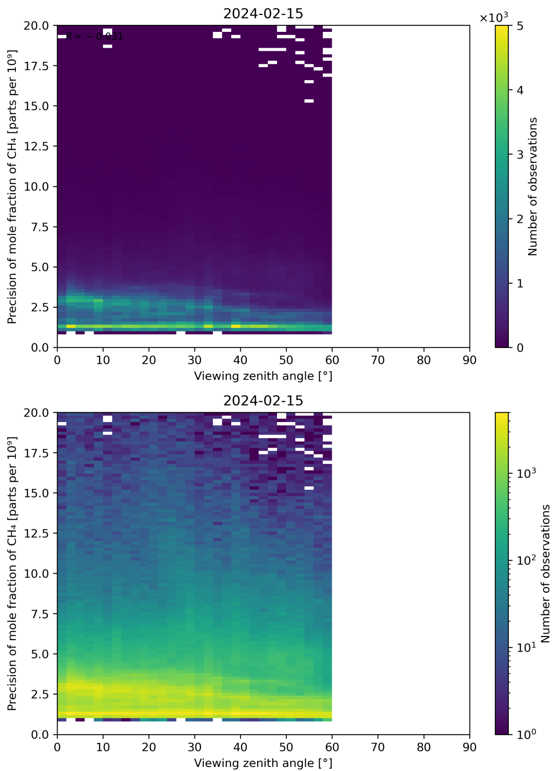
Figure 112: Scatter density plot of “Viewing zenith angle” against “Precision of mole fraction of CH 4 ” for 2024-02-14 to 2024-02-16.
