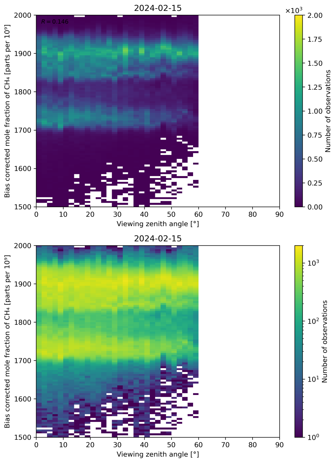
Figure 111: Scatter density plot of “Viewing zenith angle” against “Bias corrected mole fraction of CH 4 ” for 2024-02-14 to 2024-02-16.
