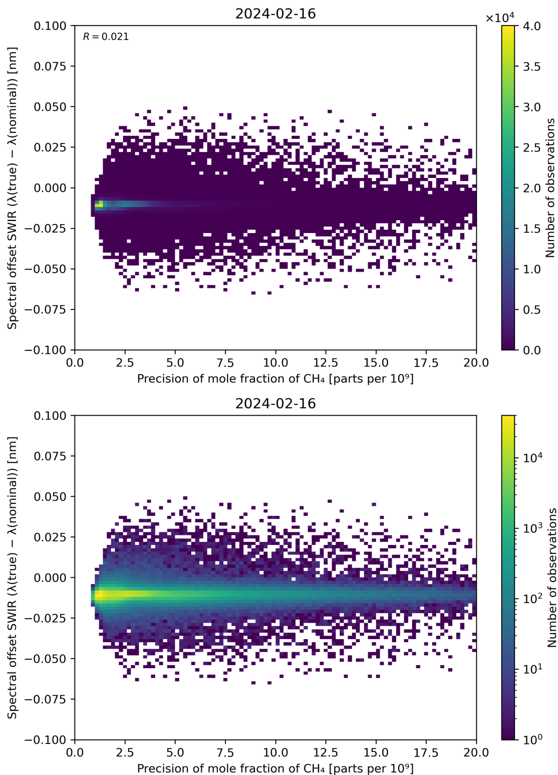
Figure 85: Scatter density plot of “Precision of mole fraction of \text{CH}_4 ” against “Spectral offset SWIR ( \lambda(\text{true}) - \lambda(\text{nominal}) )” for 2024-02-16 to 2024-02-17.
