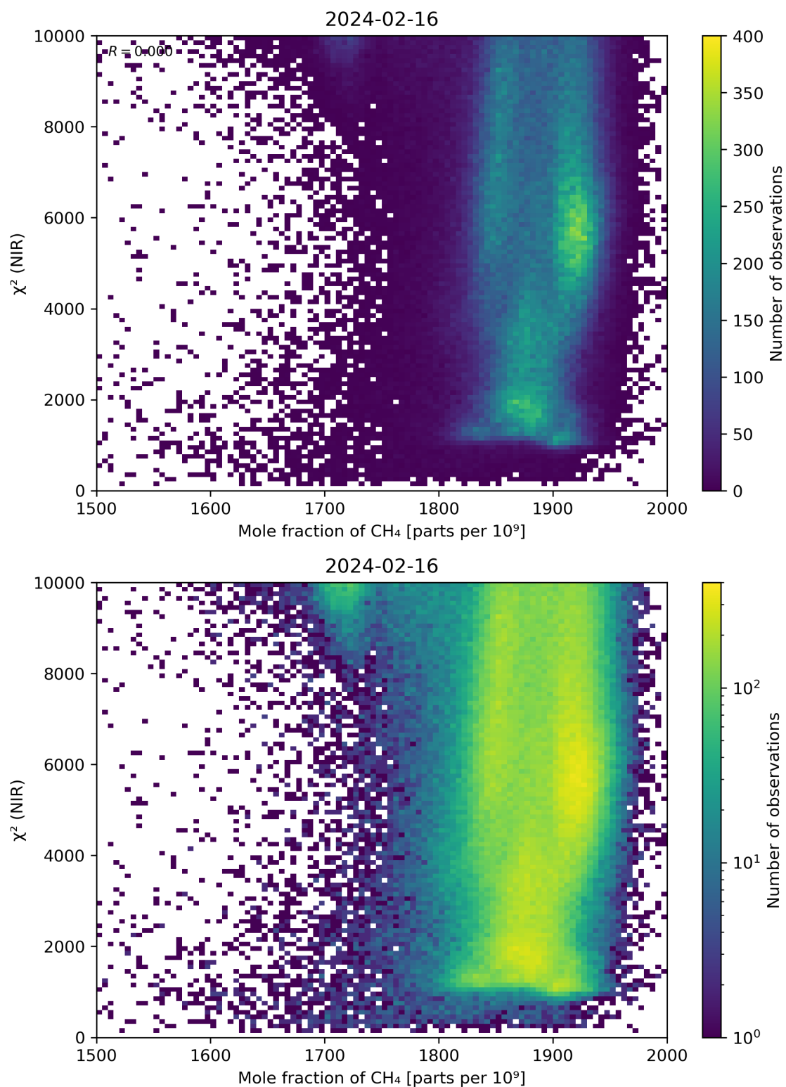
Figure 70: Scatter density plot of “Mole fraction of \text{CH}_4 ” against “ \chi^2 (NIR)” for 2024-02-16 to 2024-02-17.
