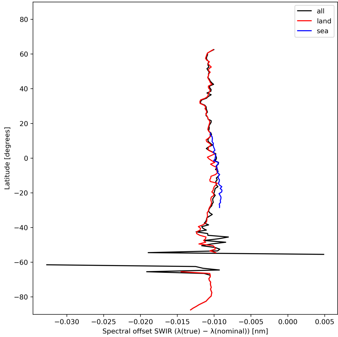
Figure 16: Zonal average of “Spectral offset SWIR ( \lambda(\text{true}) - \lambda(\text{nominal}) )” for 2024-02-16 to 2024-02-17.
