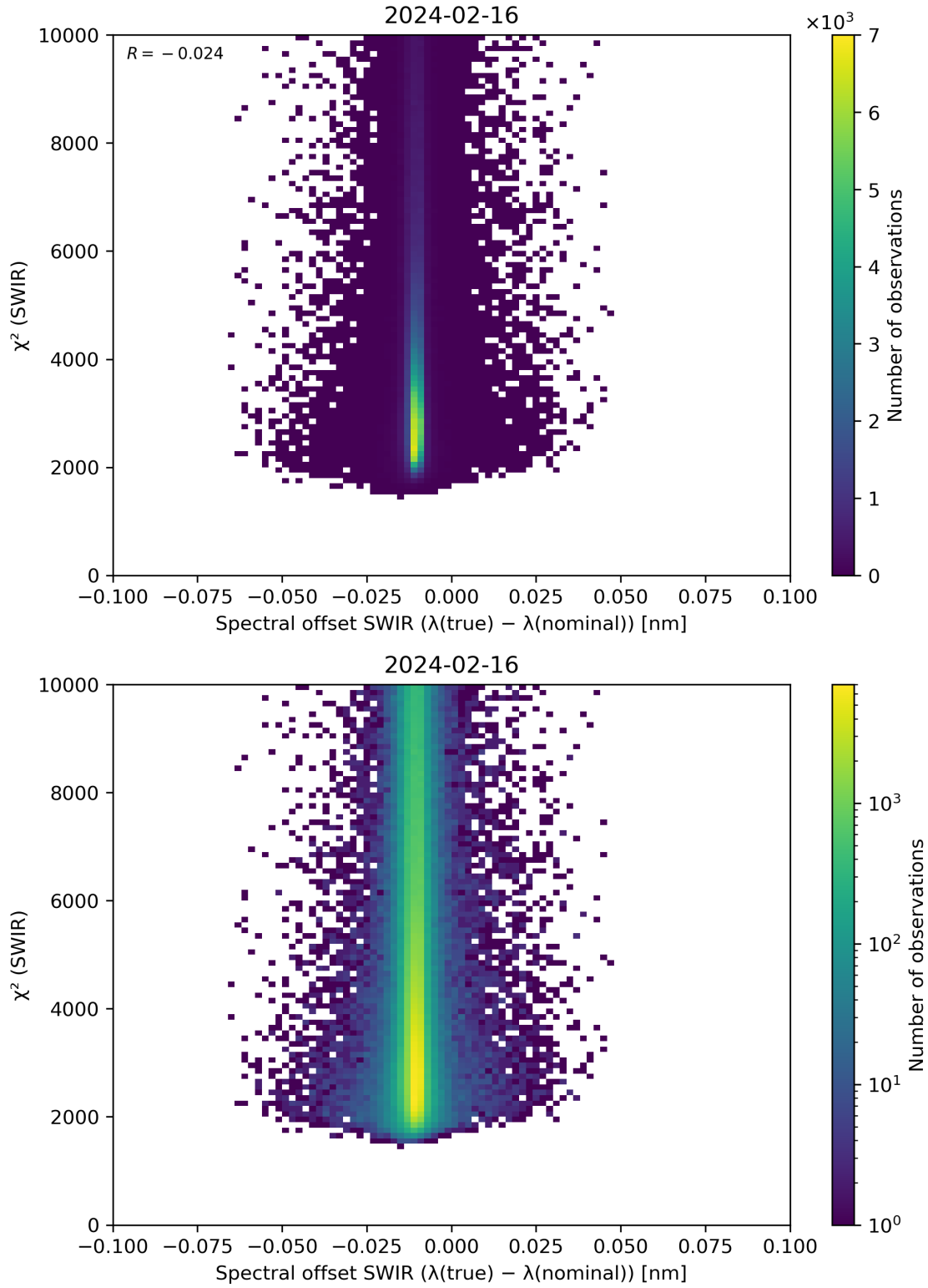
Figure 118: Scatter density plot of “Spectral offset SWIR ( \lambda(\text{true}) - \lambda(\text{nominal}) )” against “ \chi^2 (SWIR)” for 2024-02-16 to 2024-02-17.
