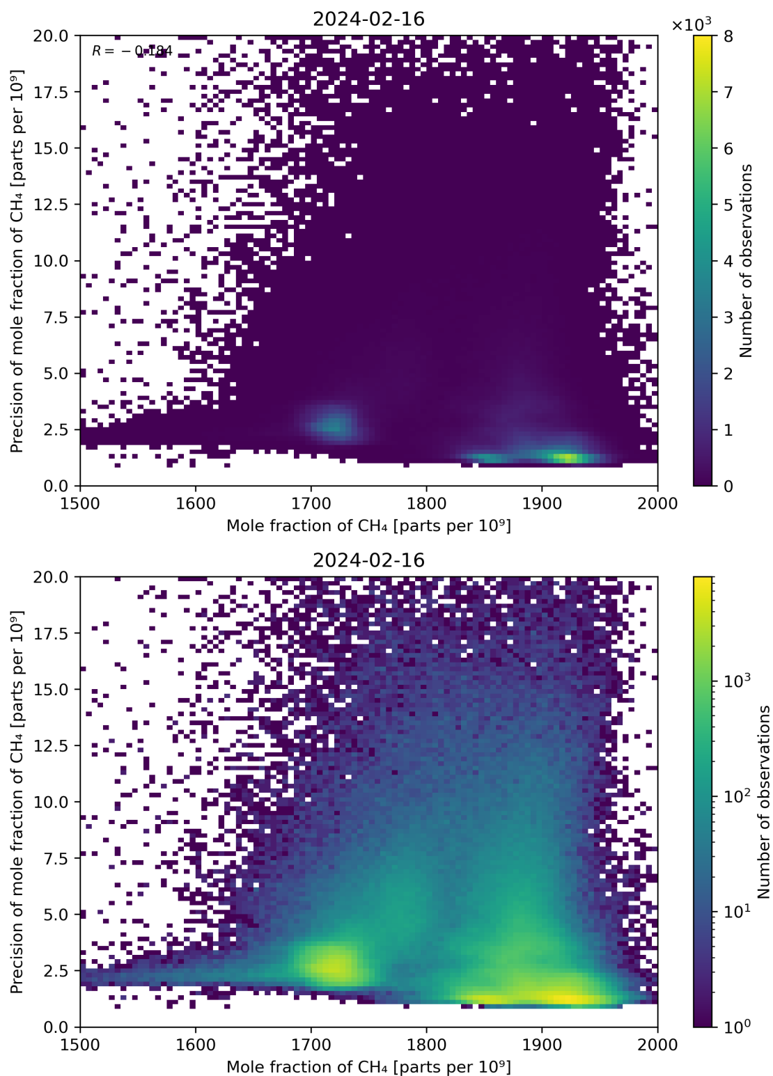
Figure 75: Scatter density plot of “Mole fraction of CH 4 ” against “Precision of mole fraction of CH 4 ” for 2024-02-16 to 2024-02-17.
