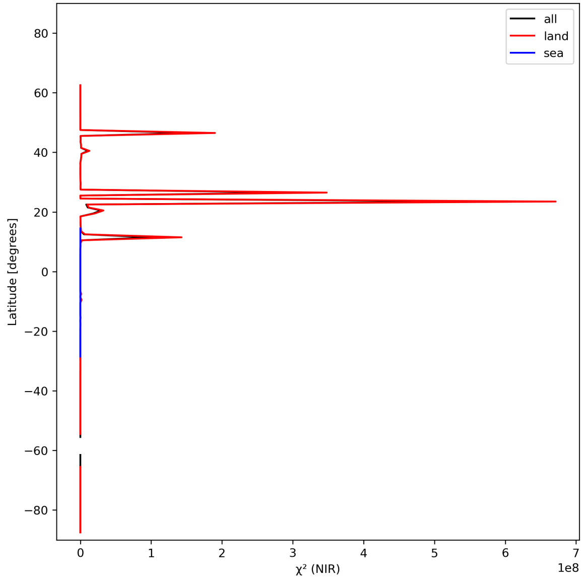
Figure 18: Zonal average of “ \chi^2 (NIR)” for 2024-02-16 to 2024-02-17.
