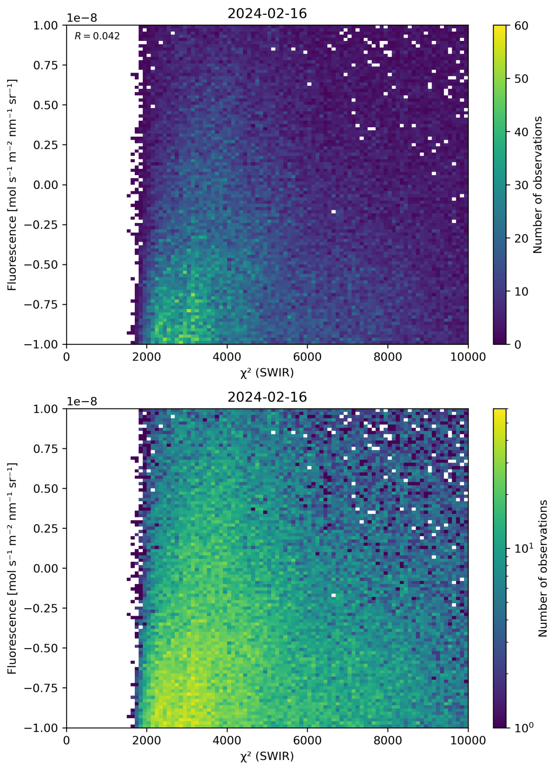
Figure 49: Scatter density plot of “ \chi^2 (SWIR)” against “Fluorescence” for 2024-02-16 to 2024-02-17.
