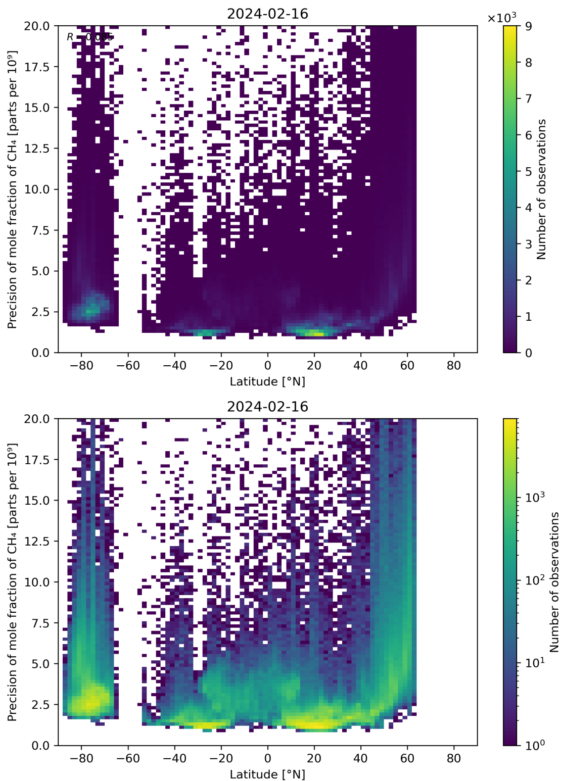
Figure 59: Scatter density plot of “Latitude” against “Precision of mole fraction of CH 4 ” for 2024-02-16 to 2024-02-17.
