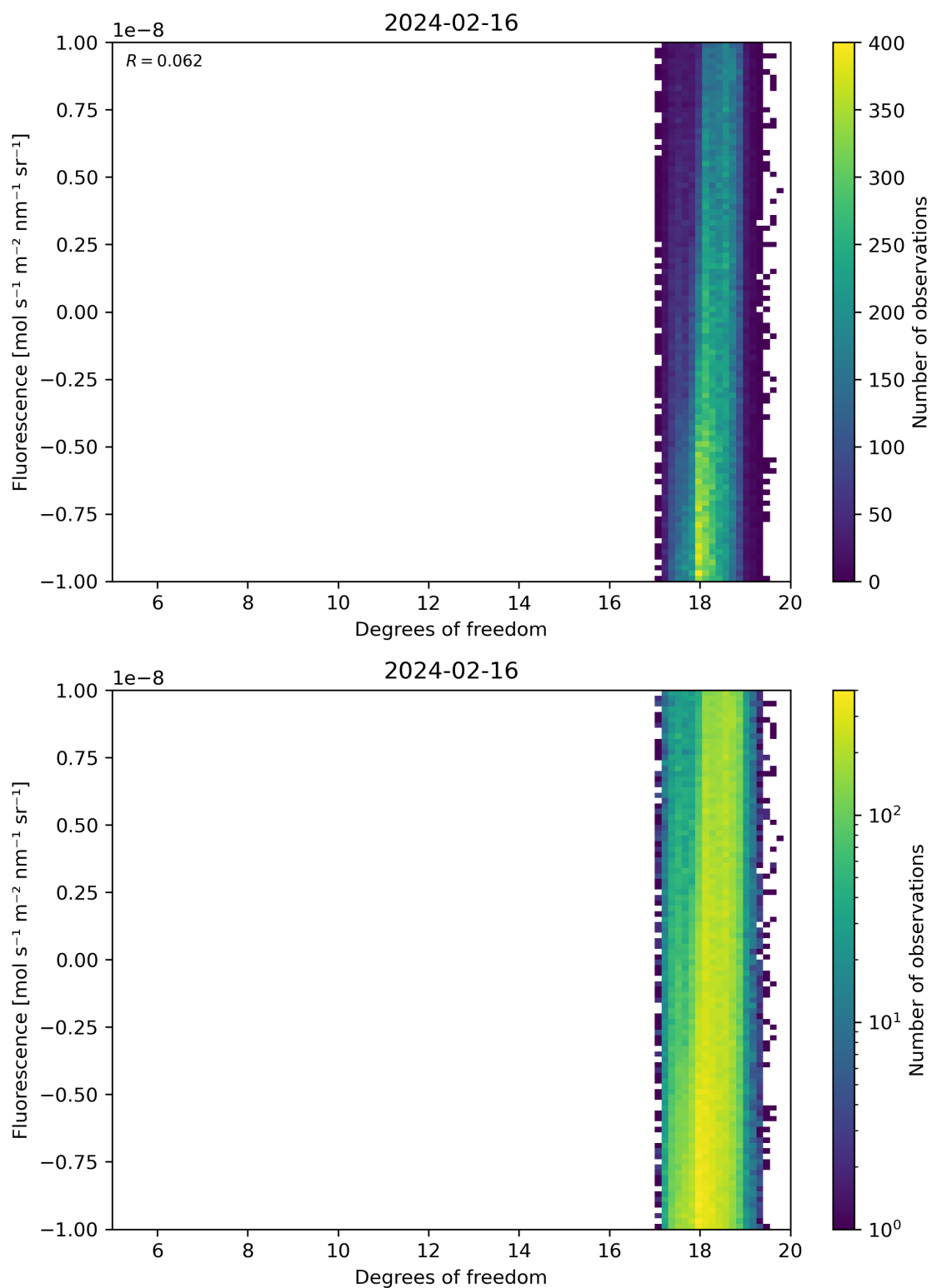
Figure 51: Scatter density plot of “Degrees of freedom” against “Fluorescence” for 2024-02-16 to 2024-02-17.
