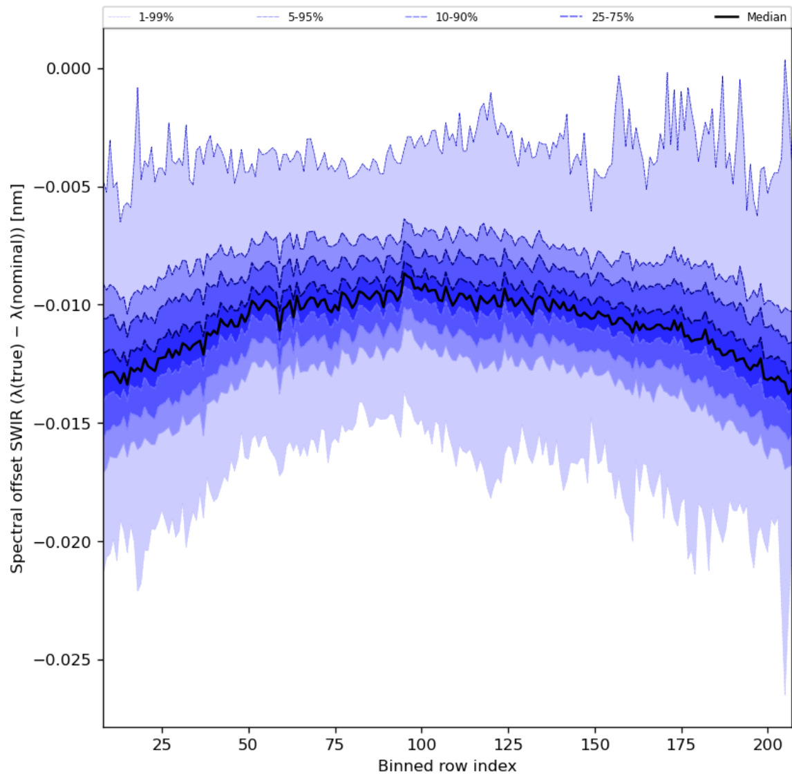
Figure 38: Along track statistics of “Spectral offset SWIR ( \lambda(\text{true}) - \lambda(\text{nominal}) )” for 2024-02-16 to 2024-02-17
