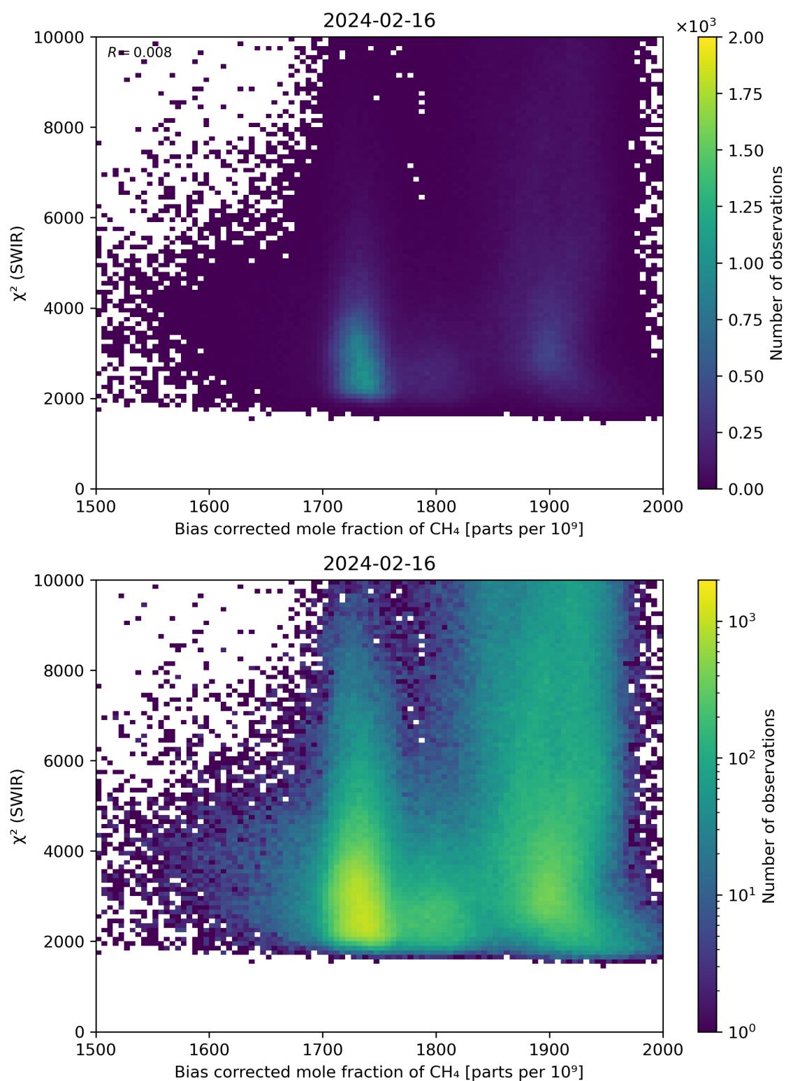
Figure 64: Scatter density plot of “Bias corrected mole fraction of CH 4 ” against “ \chi^2 (SWIR)” for 2024-02-16 to 2024-02-17.
