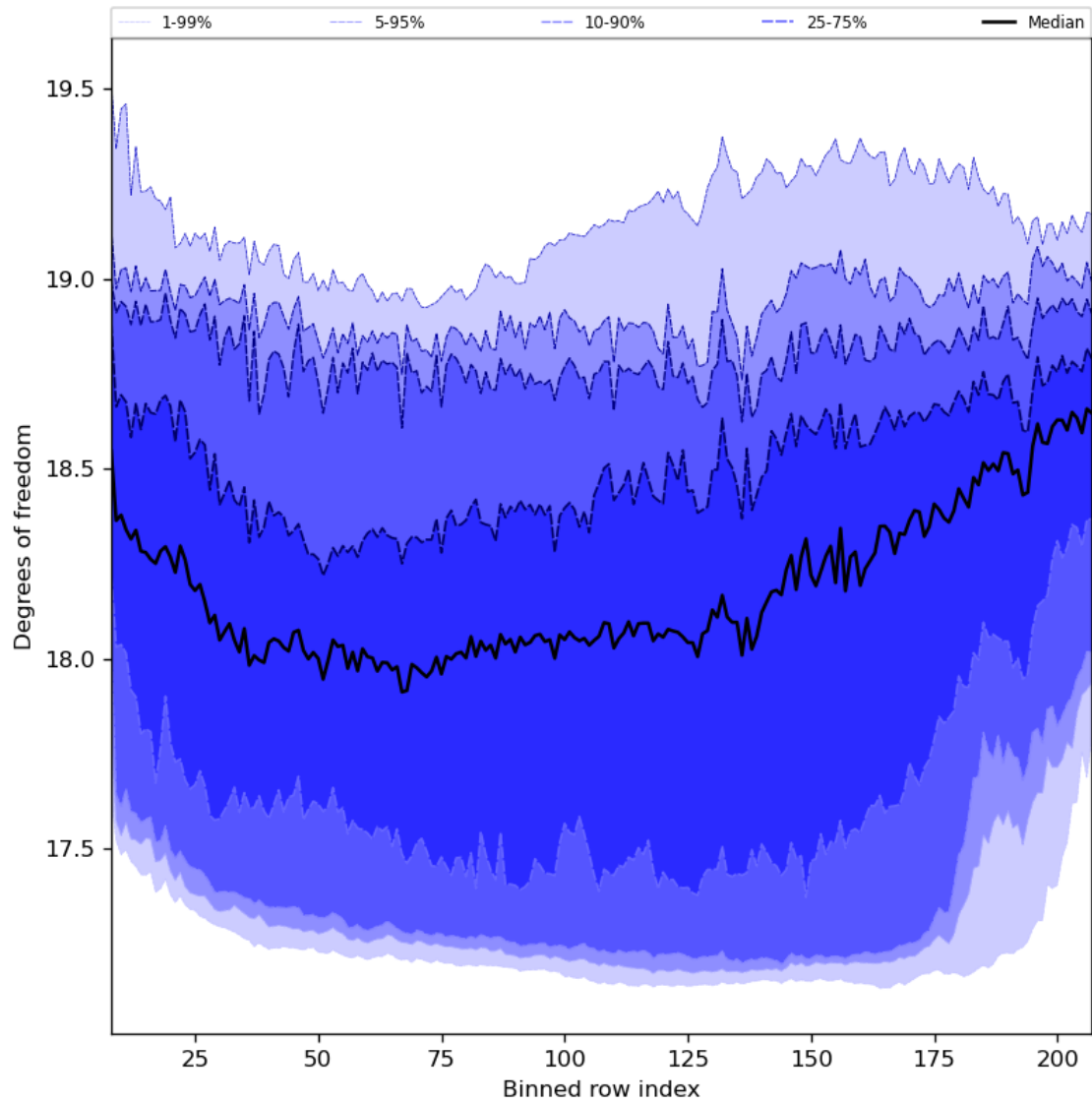
Figure 41: Along track statistics of “Degrees of freedom” for 2024-02-16 to 2024-02-17
