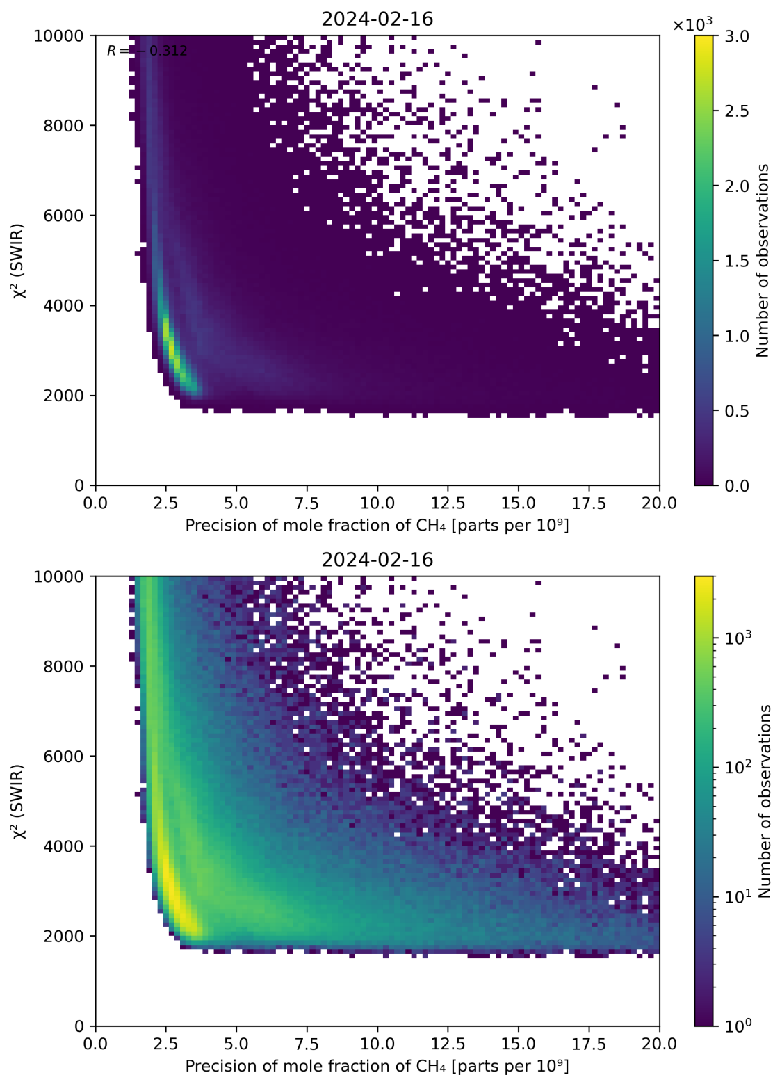
Figure 79: Scatter density plot of “Precision of mole fraction of CH 4 ” against “ \chi^2 (SWIR)” for 2024-02-16 to 2024-02-17.
