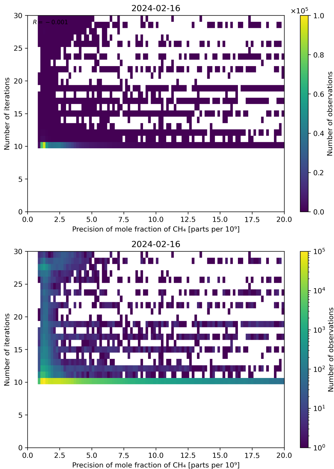
Figure 83: Scatter density plot of “Precision of mole fraction of CH 4 ” against “Number of iterations” for 2024-02-16 to 2024-02-17.
