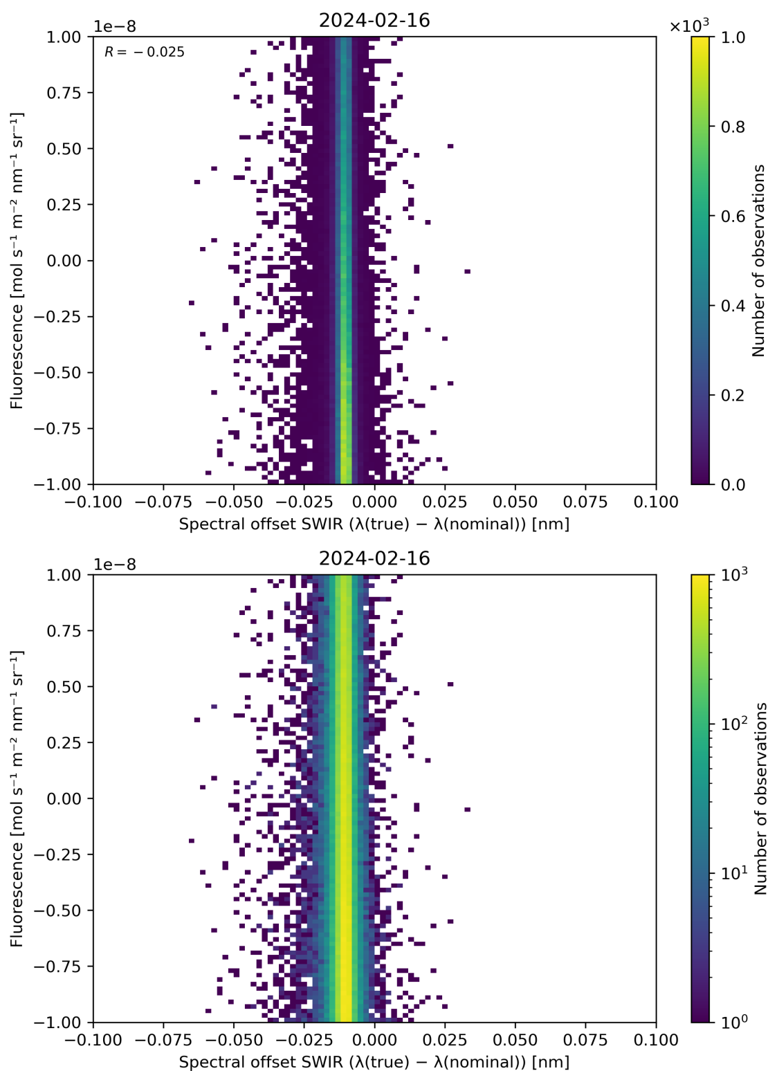
Figure 120: Scatter density plot of “Spectral offset SWIR ( \lambda(\text{true}) - \lambda(\text{nominal}) )” against “Fluorescence” for 2024-02-16 to 2024-02-17.
