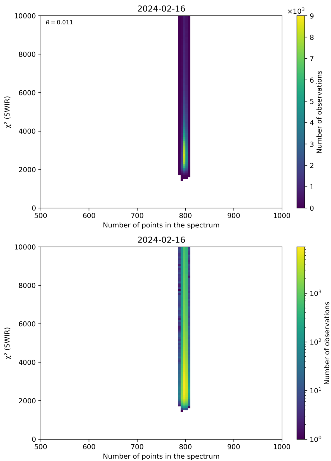
Figure 89: Scatter density plot of “Number of points in the spectrum” against “ \chi^2 (SWIR)” for 2024-02-16 to 2024-02-17.
