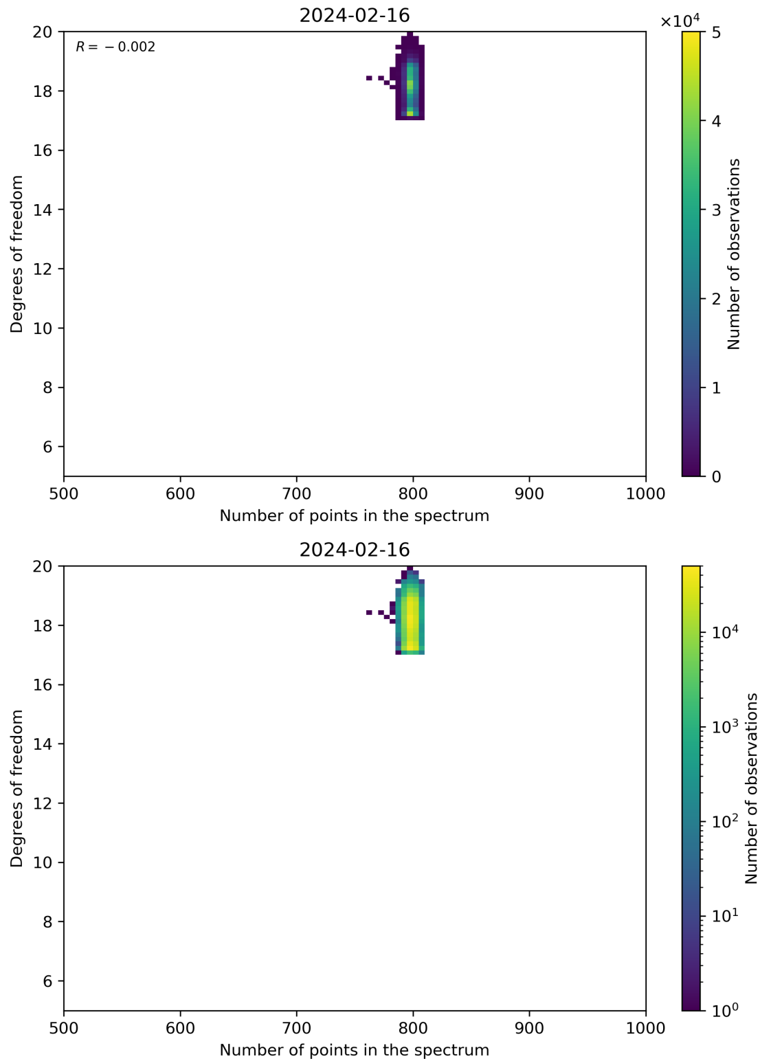
Figure 90: Scatter density plot of “Number of points in the spectrum” against “Degrees of freedom” for 2024-02-16 to 2024-02-17.
