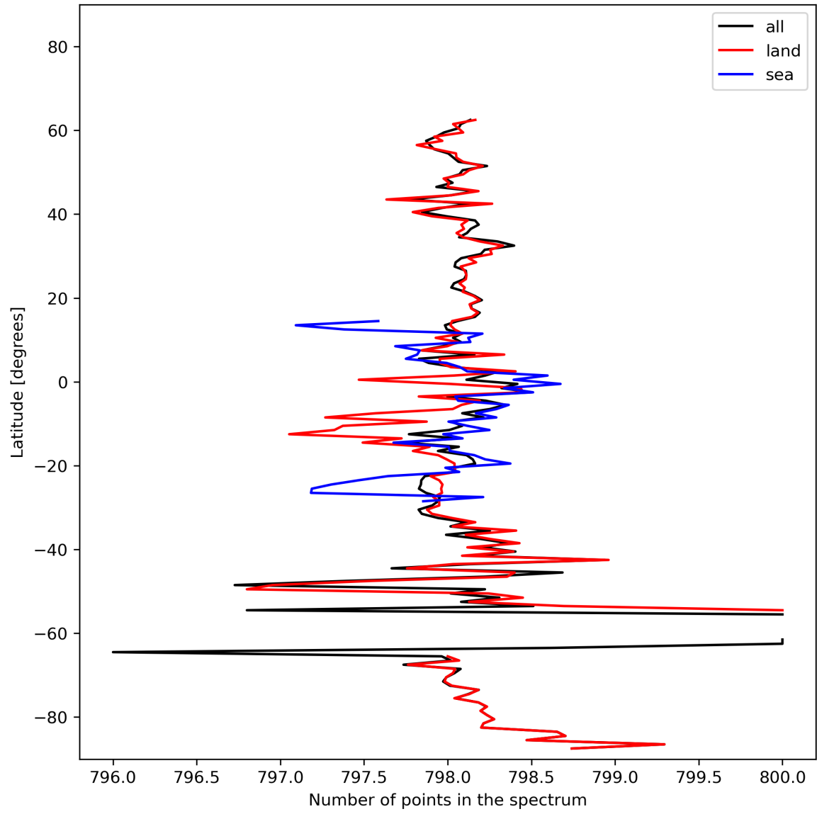
Figure 15: Zonal average of “Number of points in the spectrum” for 2024-02-16 to 2024-02-17.
