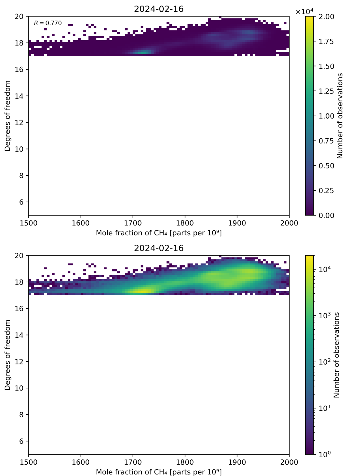
Figure 72: Scatter density plot of “Mole fraction of CH 4 ” against “Degrees of freedom” for 2024-02-16 to 2024-02-17.
