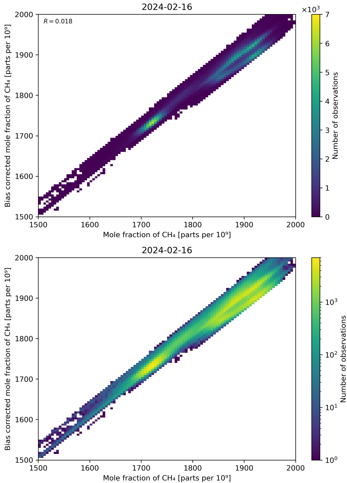
Figure 74: Scatter density plot of “Mole fraction of CH 4 ” against “Bias corrected mole fraction of CH 4 ” for 2024-02-16 to 2024-02-17.
