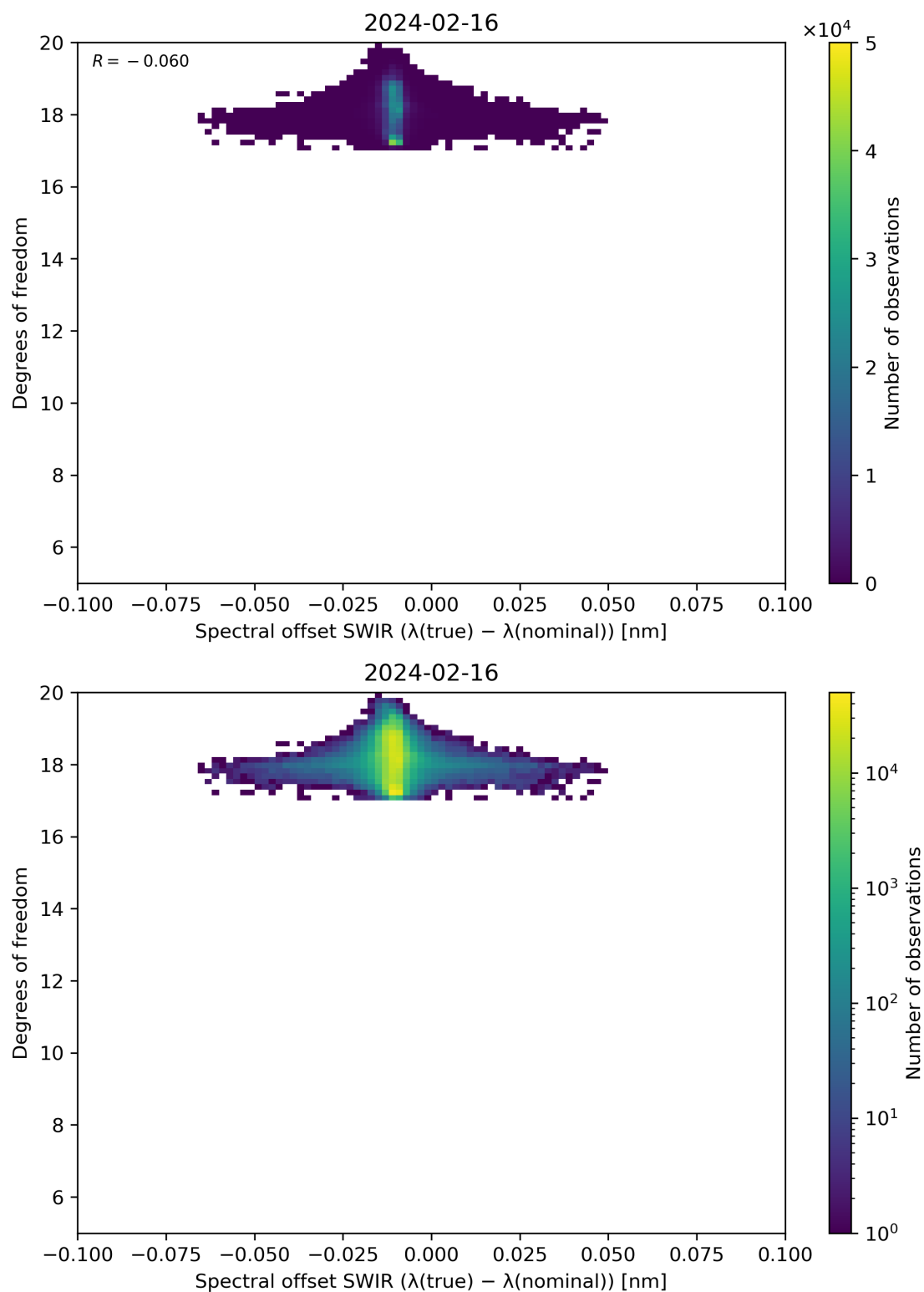
Figure 119: Scatter density plot of “Spectral offset SWIR ( \lambda(\text{true}) - \lambda(\text{nominal}) )” against “Degrees of freedom” for 2024-02-16 to 2024-02-17.
