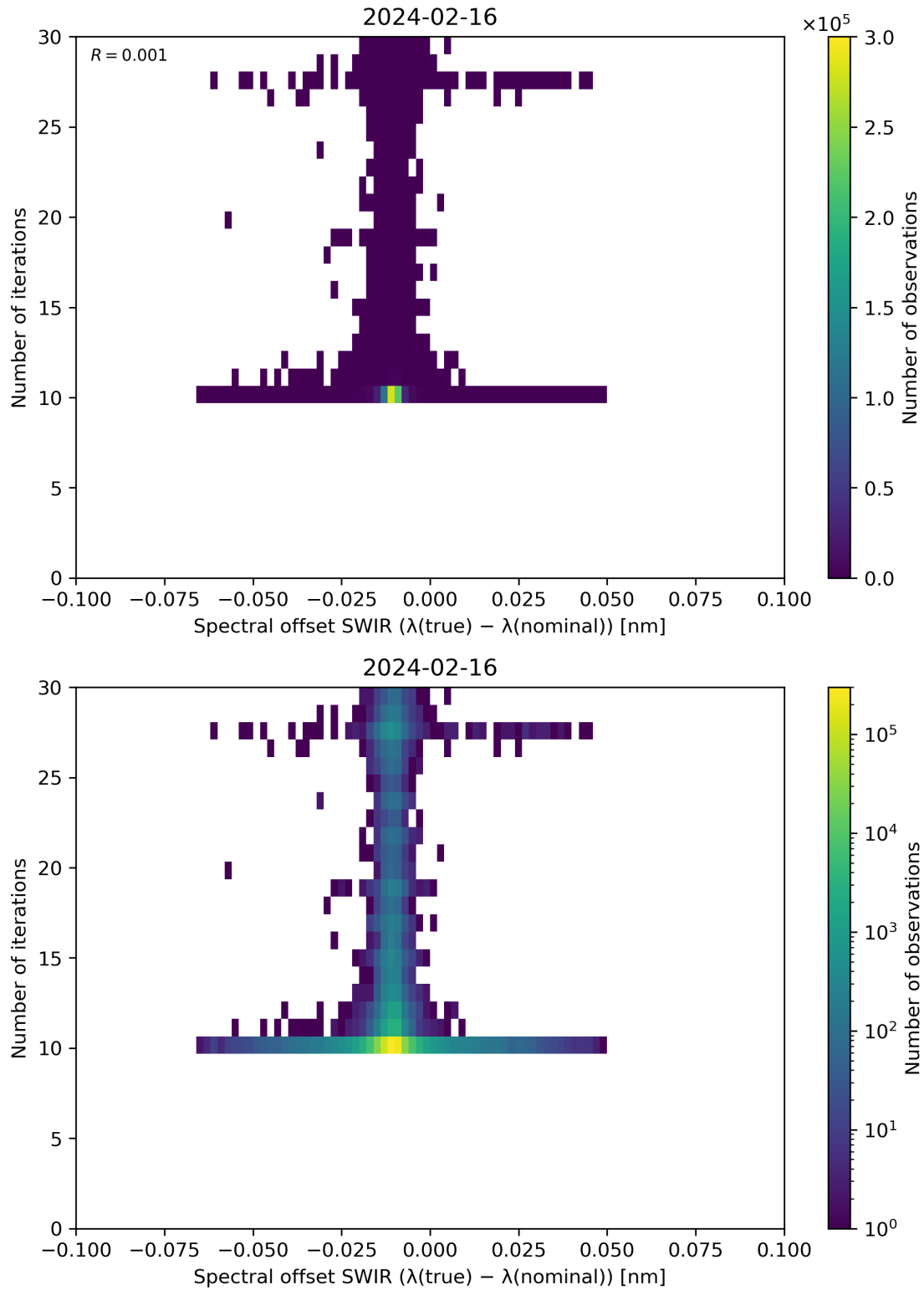
Figure 121: Scatter density plot of “Spectral offset SWIR ( \lambda(\text{true}) - \lambda(\text{nominal}) )” against “Number of iterations” for 2024-02-16 to 2024-02-17.
