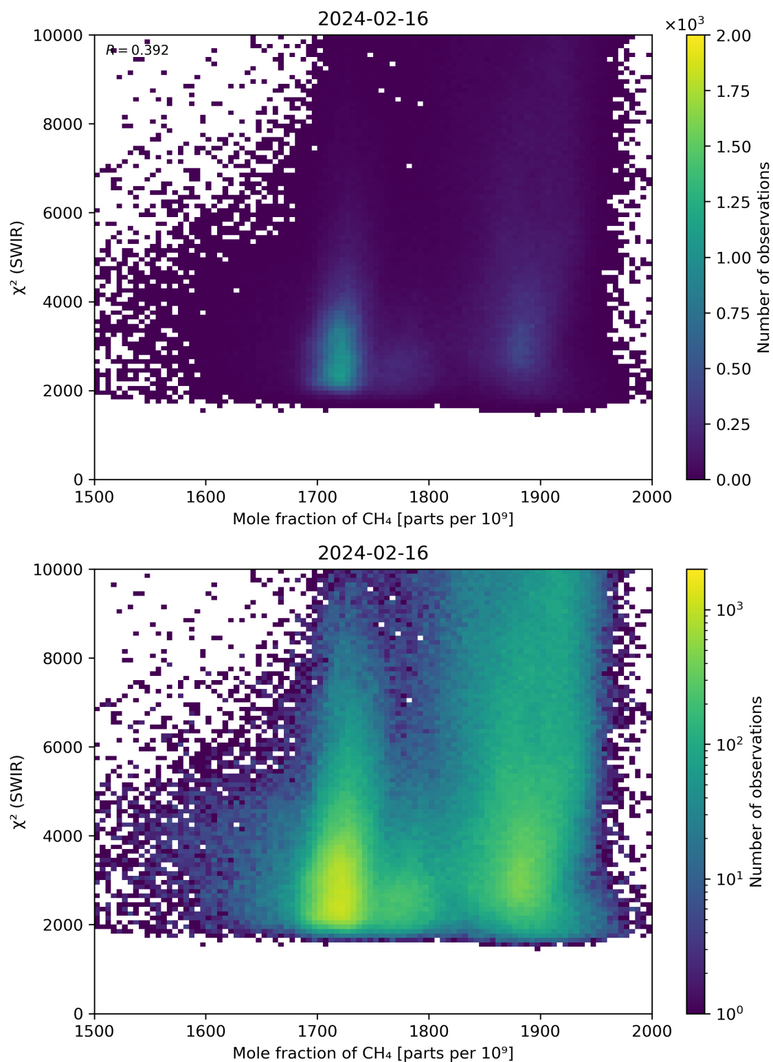
Figure 71: Scatter density plot of “Mole fraction of CH 4 ” against “ \chi^2 (SWIR)” for 2024-02-16 to 2024-02-17.
