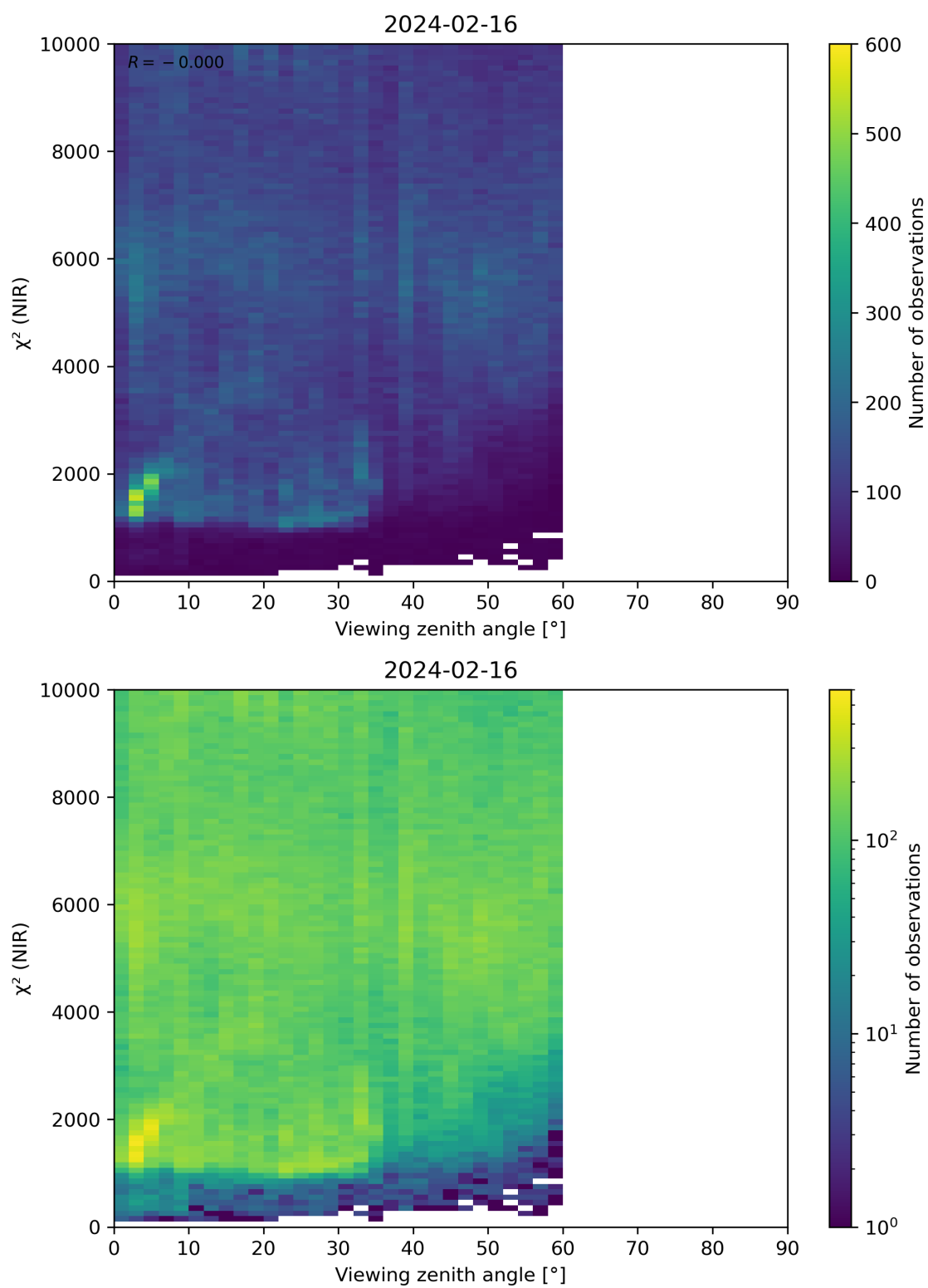
Figure 105: Scatter density plot of “Viewing zenith angle” against “ \chi^2 (NIR)” for 2024-02-16 to 2024-02-17.
