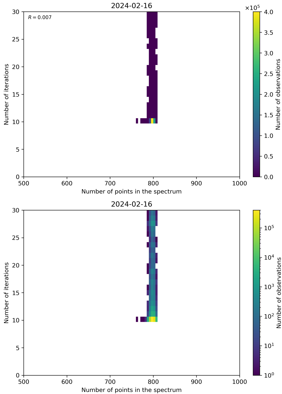
Figure 92: Scatter density plot of “Number of points in the spectrum” against “Number of iterations” for 2024-02-16 to 2024-02-17.
