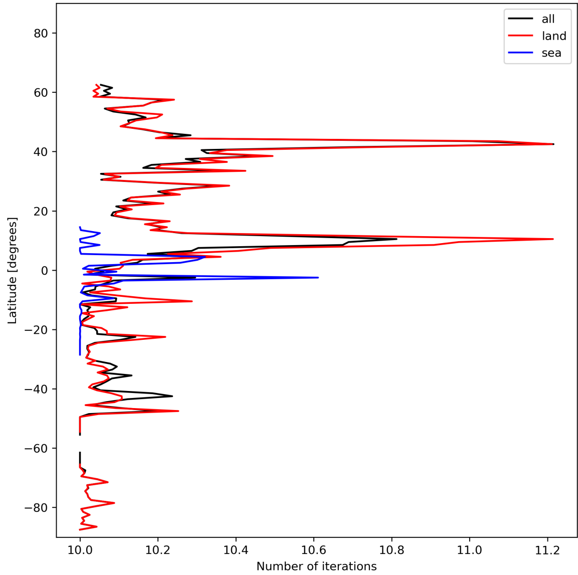
Figure 20: Zonal average of “Number of iterations” for 2024-02-16 to 2024-02-17.
