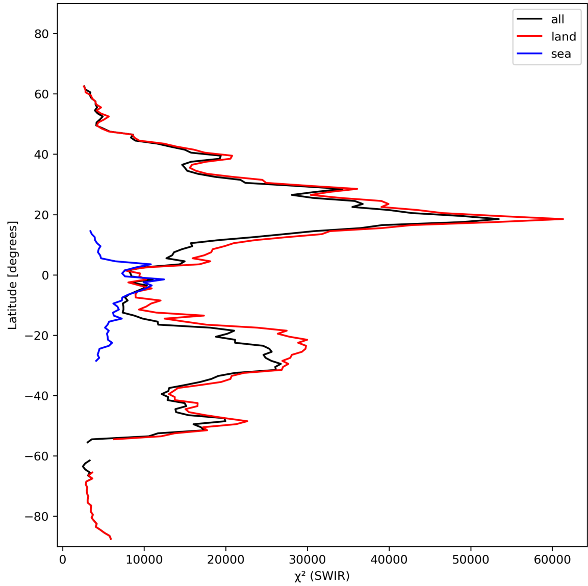
Figure 17: Zonal average of “ \chi^2 (SWIR)” for 2024-02-16 to 2024-02-17.
