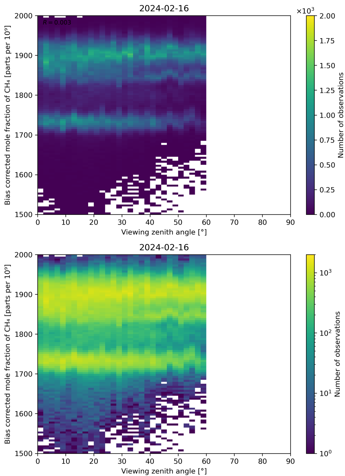
Figure 111: Scatter density plot of “Viewing zenith angle” against “Bias corrected mole fraction of CH 4 ” for 2024-02-16 to 2024-02-17.
