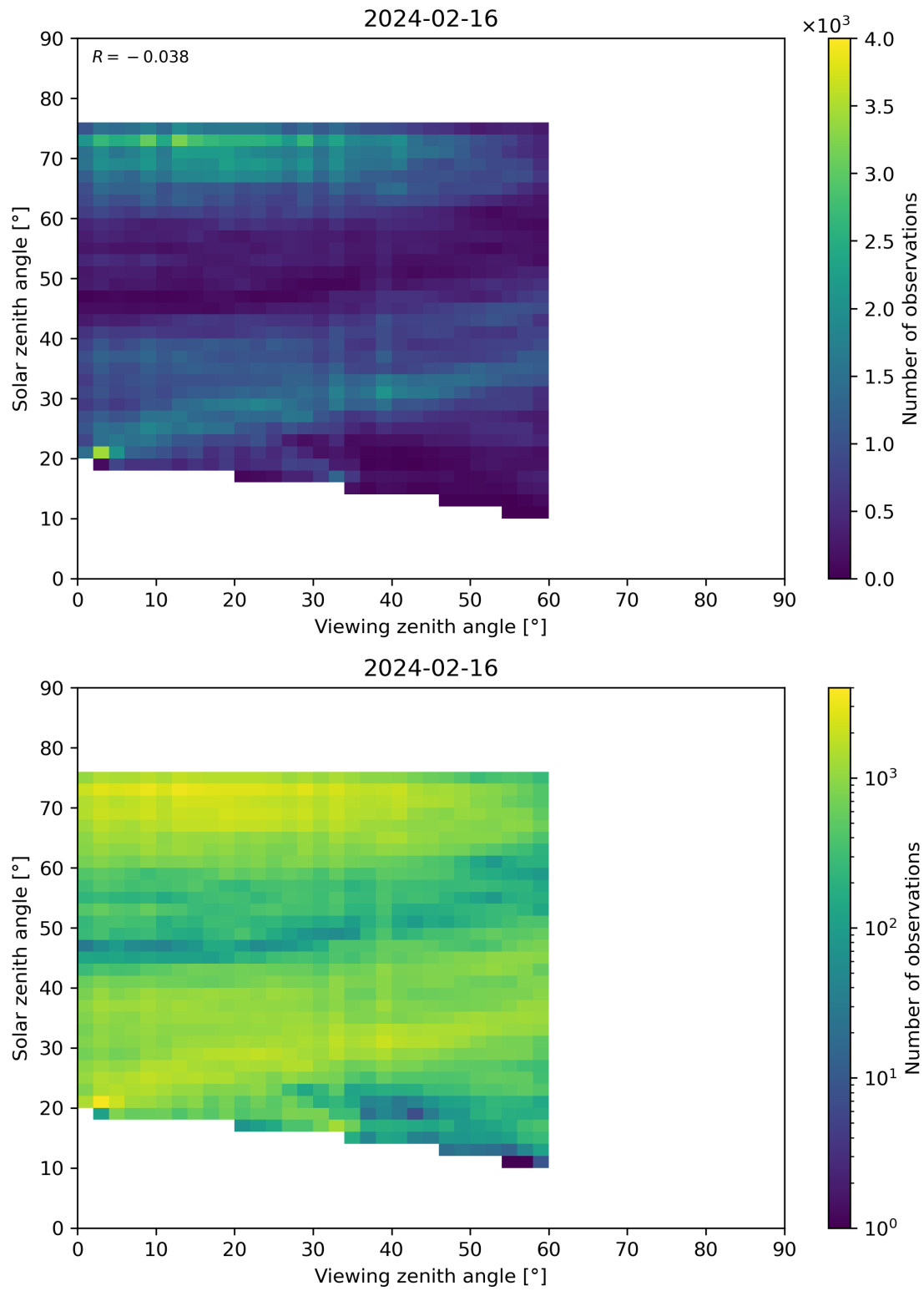
Figure 115: Scatter density plot of “Viewing zenith angle” against “Solar zenith angle” for 2024-02-16 to 2024-02-17.
