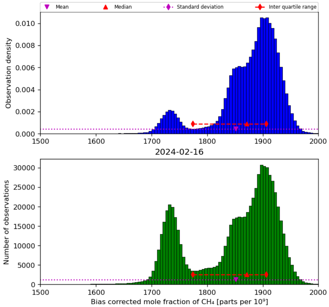
Figure 25: Histogram of “Bias corrected mole fraction of CH 4 ” for 2024-02-16 to 2024-02-17
