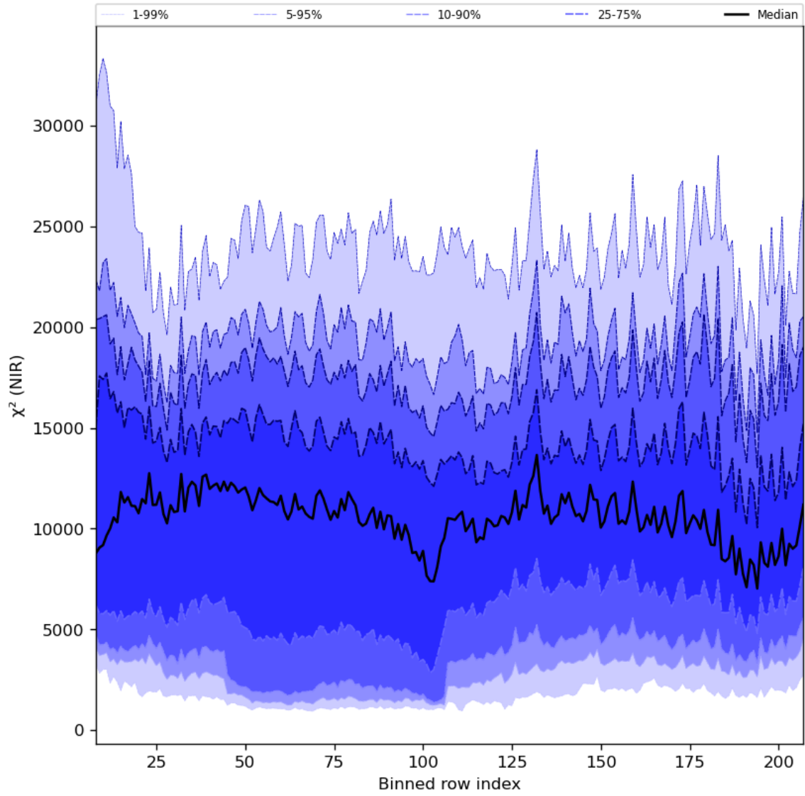
Figure 40: Along track statistics of " \chi^2 (NIR)" for 2024-02-16 to 2024-02-17
