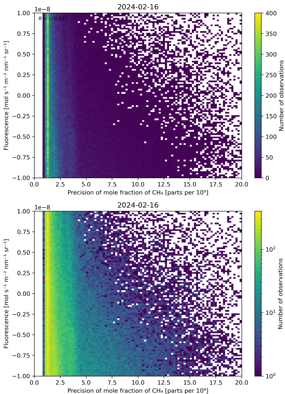
Figure 81: Scatter density plot of “Precision of mole fraction of \text{CH}_4 ” against “Fluorescence” for 2024-02-16 to 2024-02-17.
