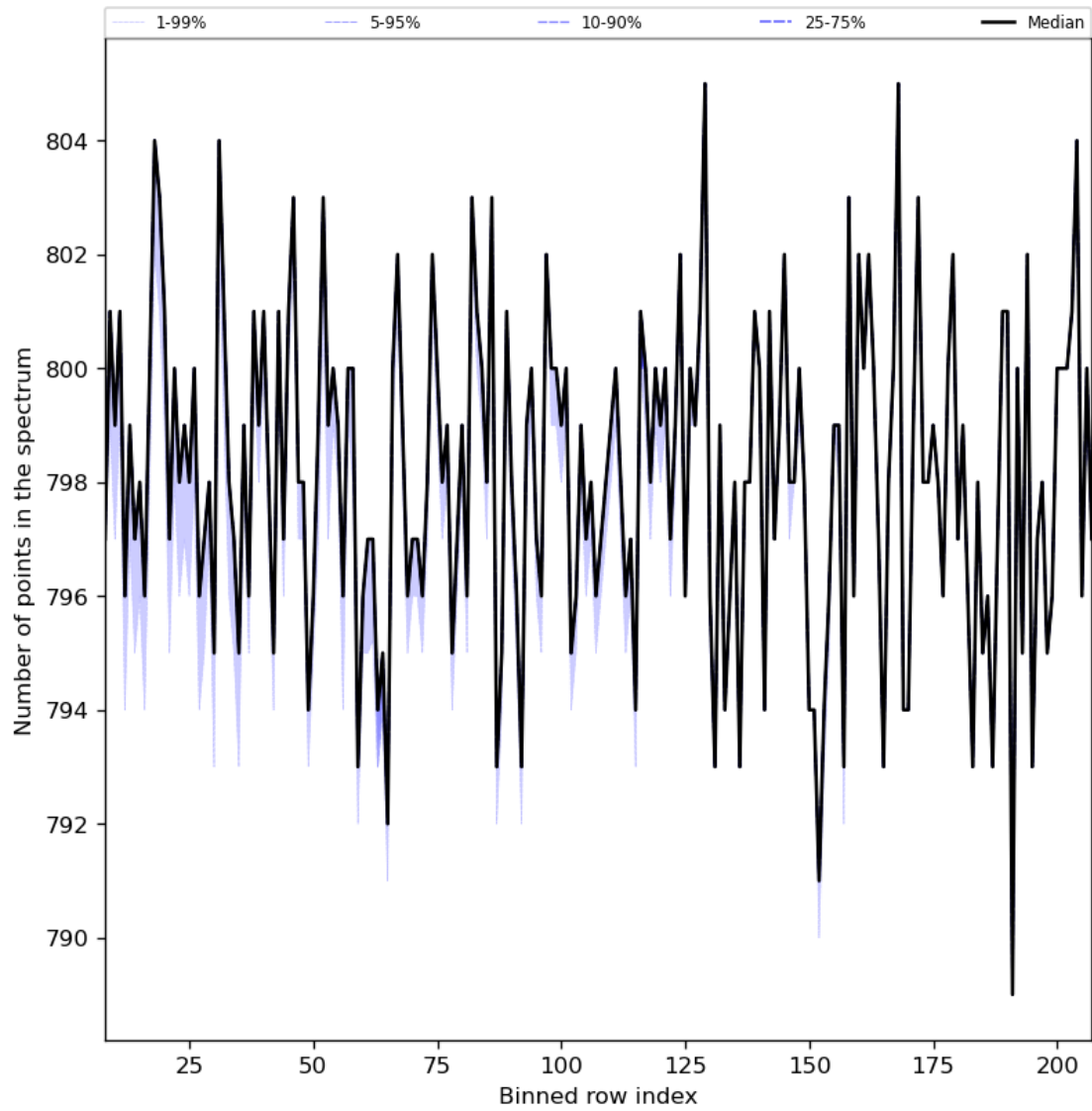
Figure 37: Along track statistics of “Number of points in the spectrum” for 2024-02-16 to 2024-02-17
