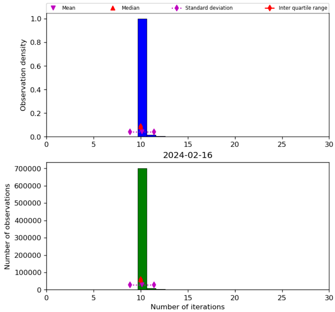
Figure 31: Histogram of “Number of iterations” for 2024-02-16 to 2024-02-17
