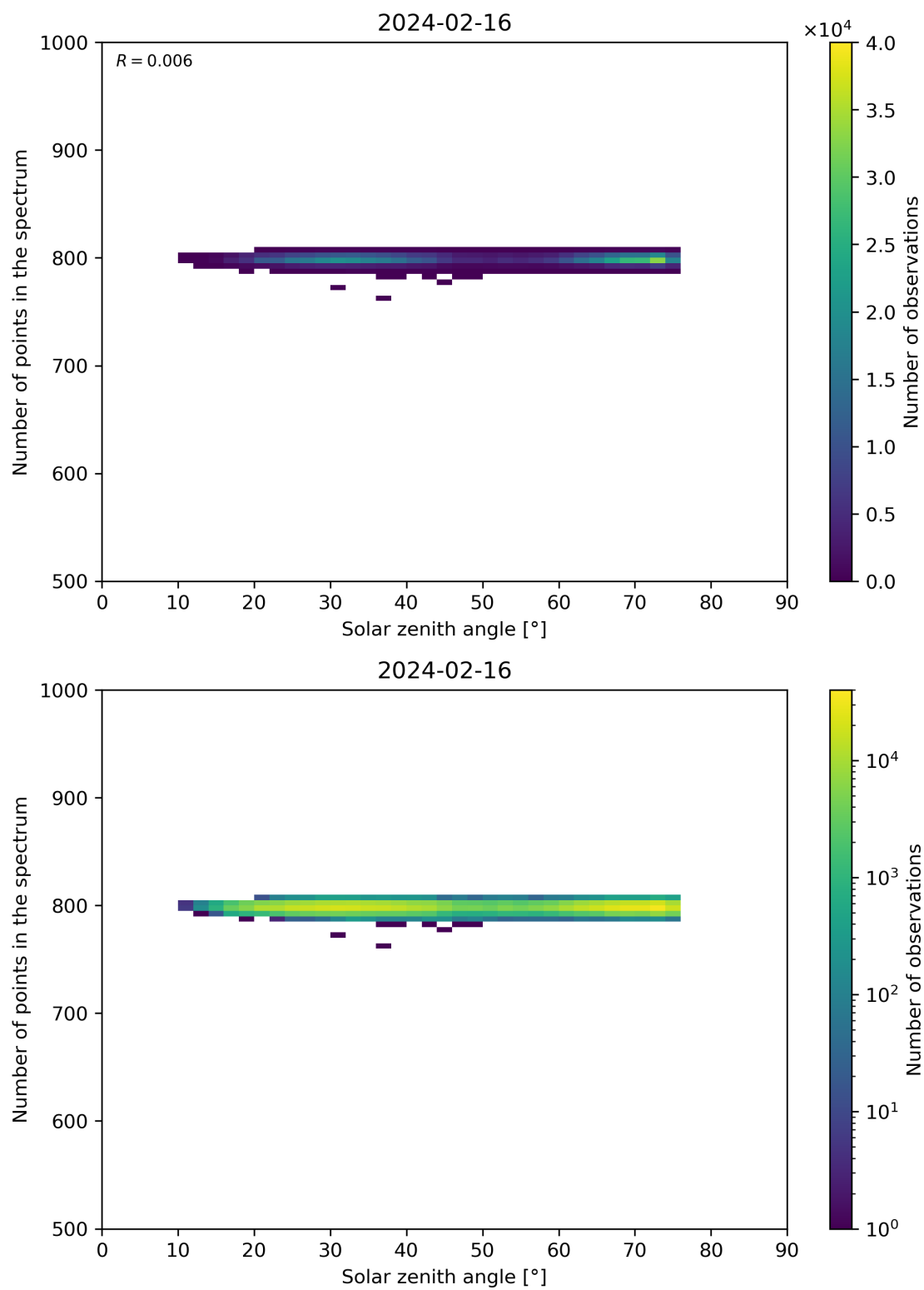
Figure 103: Scatter density plot of “Solar zenith angle” against “Number of points in the spectrum” for 2024-02-16 to 2024-02-17.
