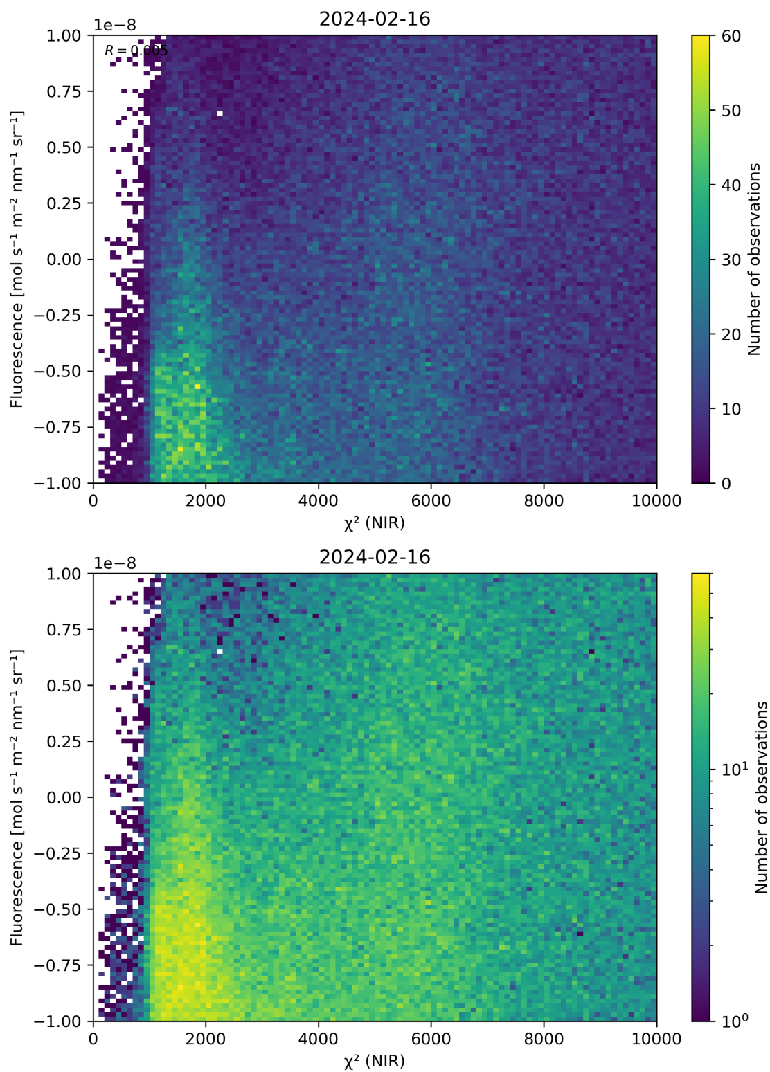
Figure 45: Scatter density plot of “ \chi^2 (NIR)” against “Fluorescence” for 2024-02-16 to 2024-02-17.
