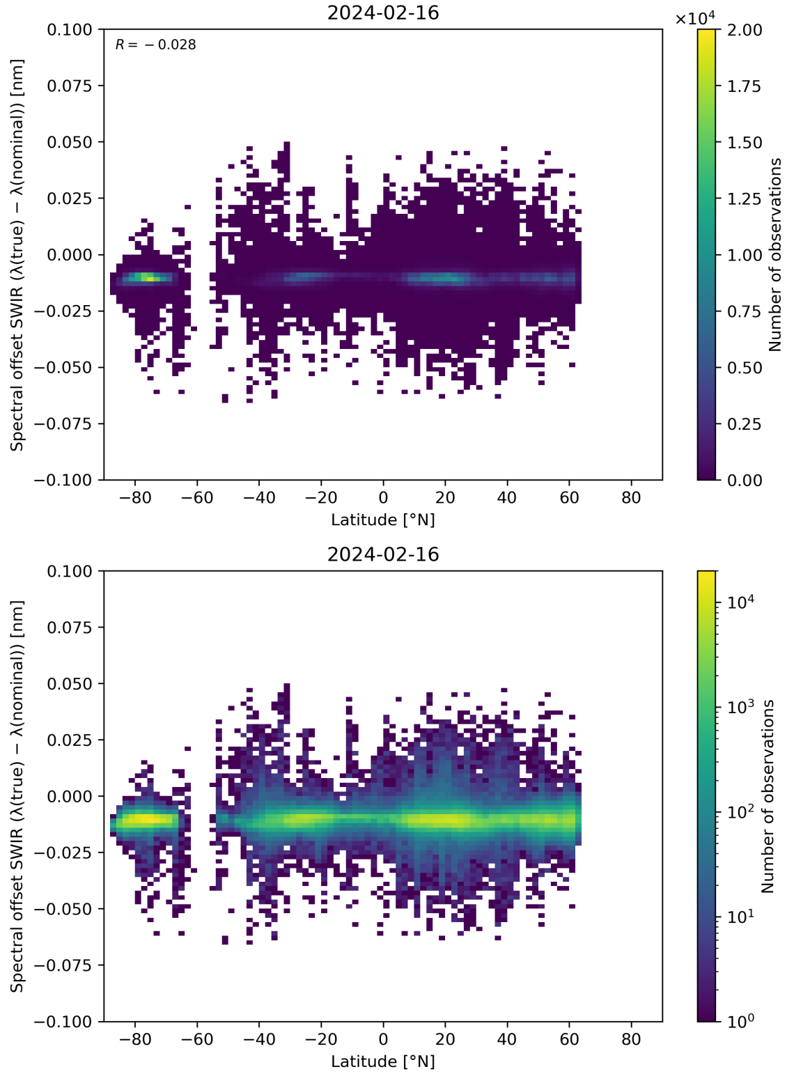
Figure 62: Scatter density plot of “Latitude” against “Spectral offset SWIR ( \lambda(\text{true}) - \lambda(\text{nominal}) )” for 2024-02-16 to 2024-02-17.
