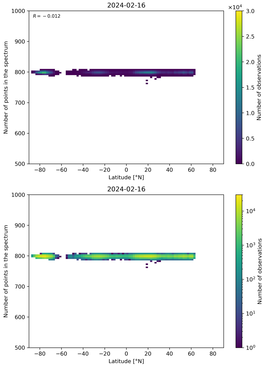
Figure 61: Scatter density plot of “Latitude” against “Number of points in the spectrum” for 2024-02-16 to 2024-02-17.
