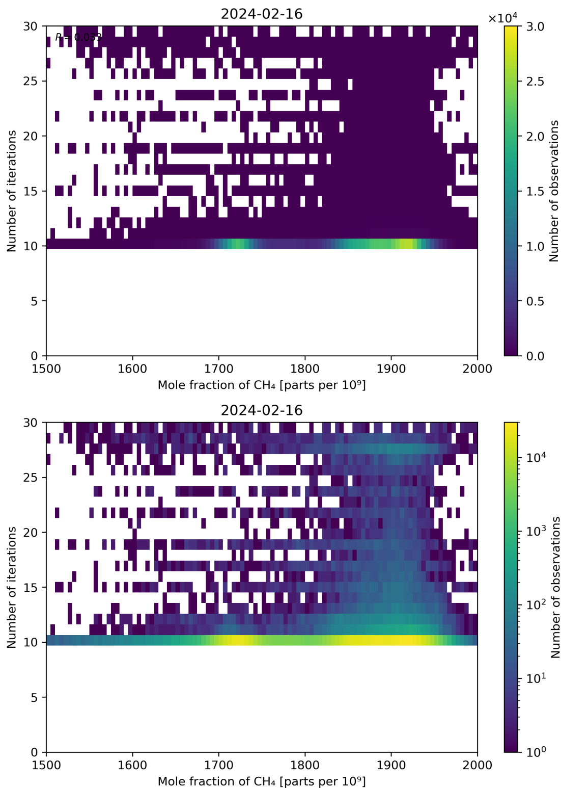
Figure 76: Scatter density plot of “Mole fraction of CH 4 ” against “Number of iterations” for 2024-02-16 to 2024-02-17.
