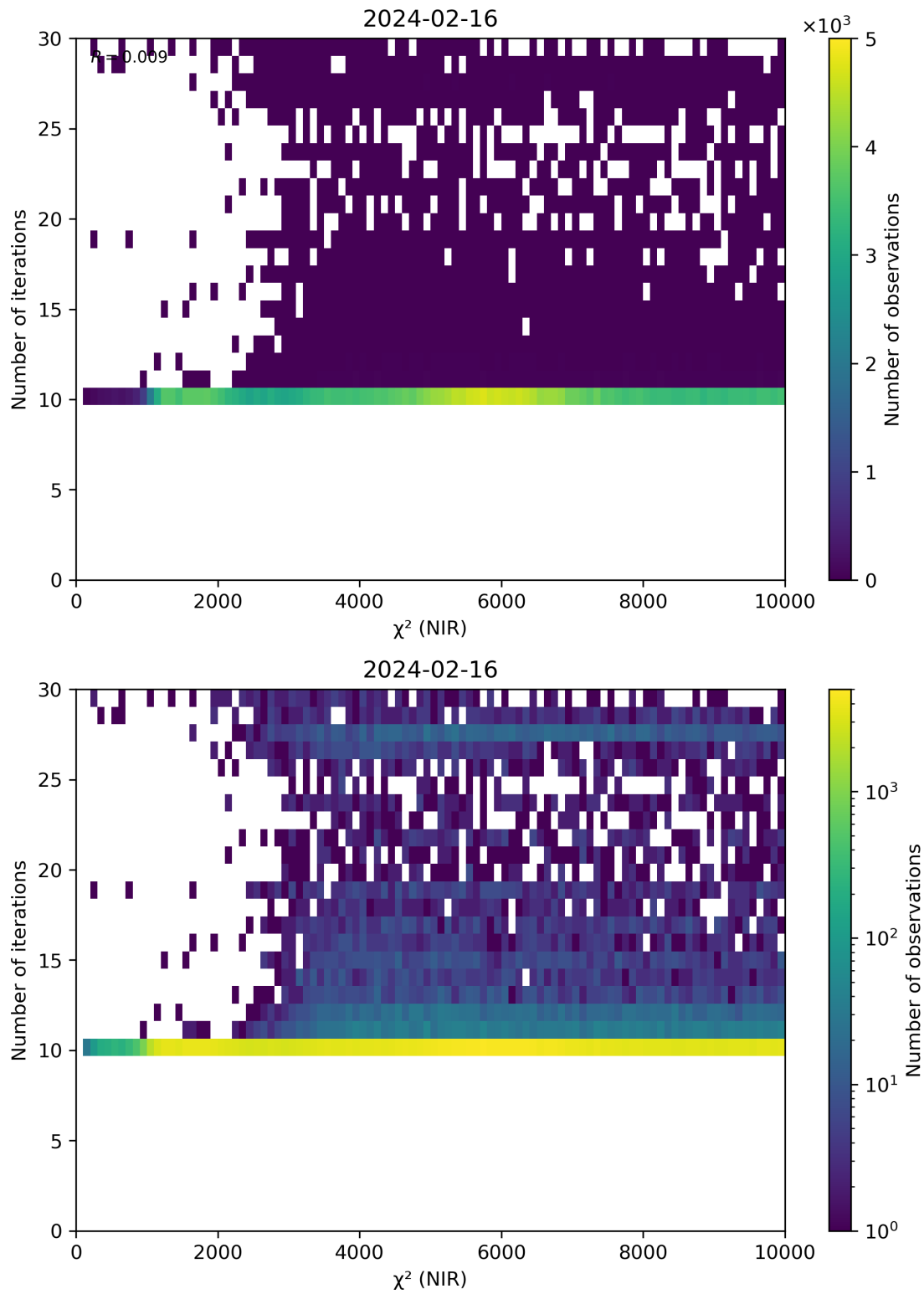
Figure 46: Scatter density plot of “ \chi^2 (NIR)” against “Number of iterations” for 2024-02-16 to 2024-02-17.
