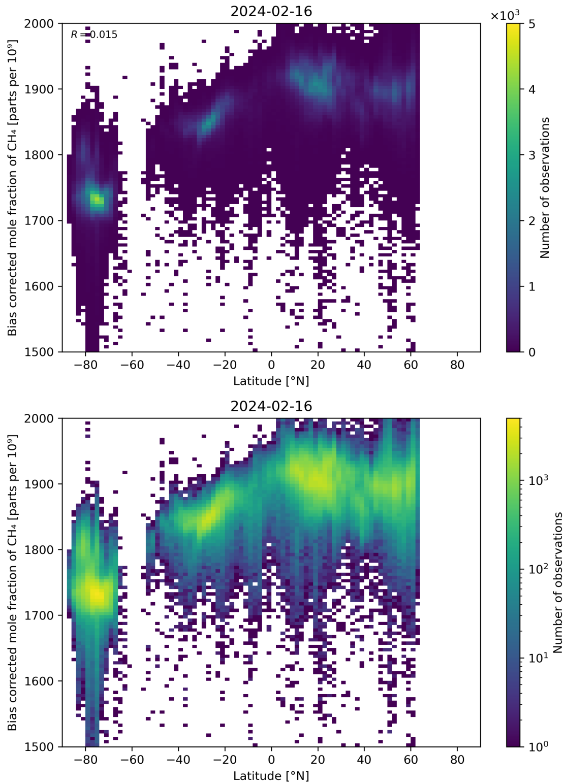
Figure 58: Scatter density plot of “Latitude” against “Bias corrected mole fraction of CH 4 ” for 2024-02-16 to 2024-02-17.
