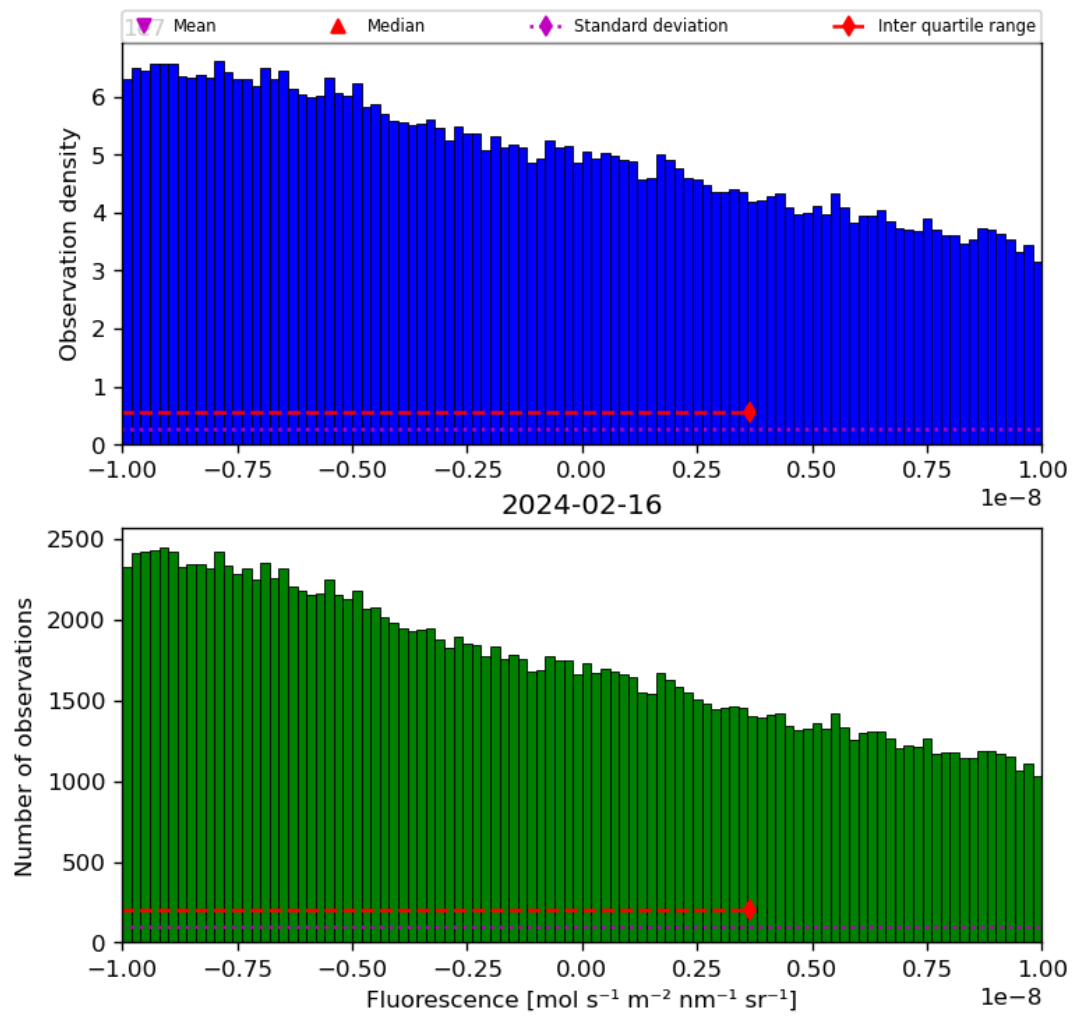
Figure 32: Histogram of “Fluorescence” for 2024-02-16 to 2024-02-17
