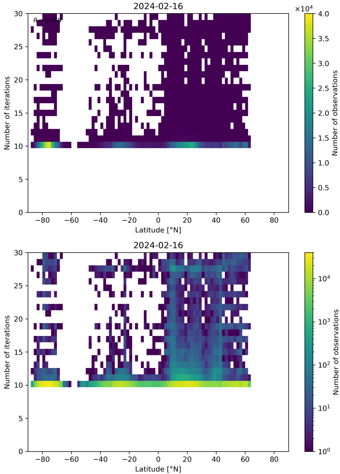
Figure 60: Scatter density plot of “Latitude” against “Number of iterations” for 2024-02-16 to 2024-02-17.
