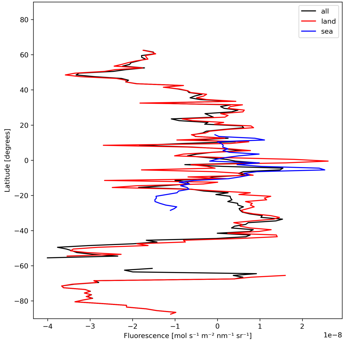
Figure 21: Zonal average of “Fluorescence” for 2024-02-16 to 2024-02-17.
