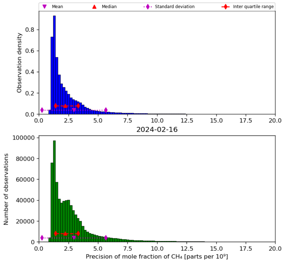
Figure 24: Histogram of “Precision of mole fraction of CH 4 ” for 2024-02-16 to 2024-02-17
