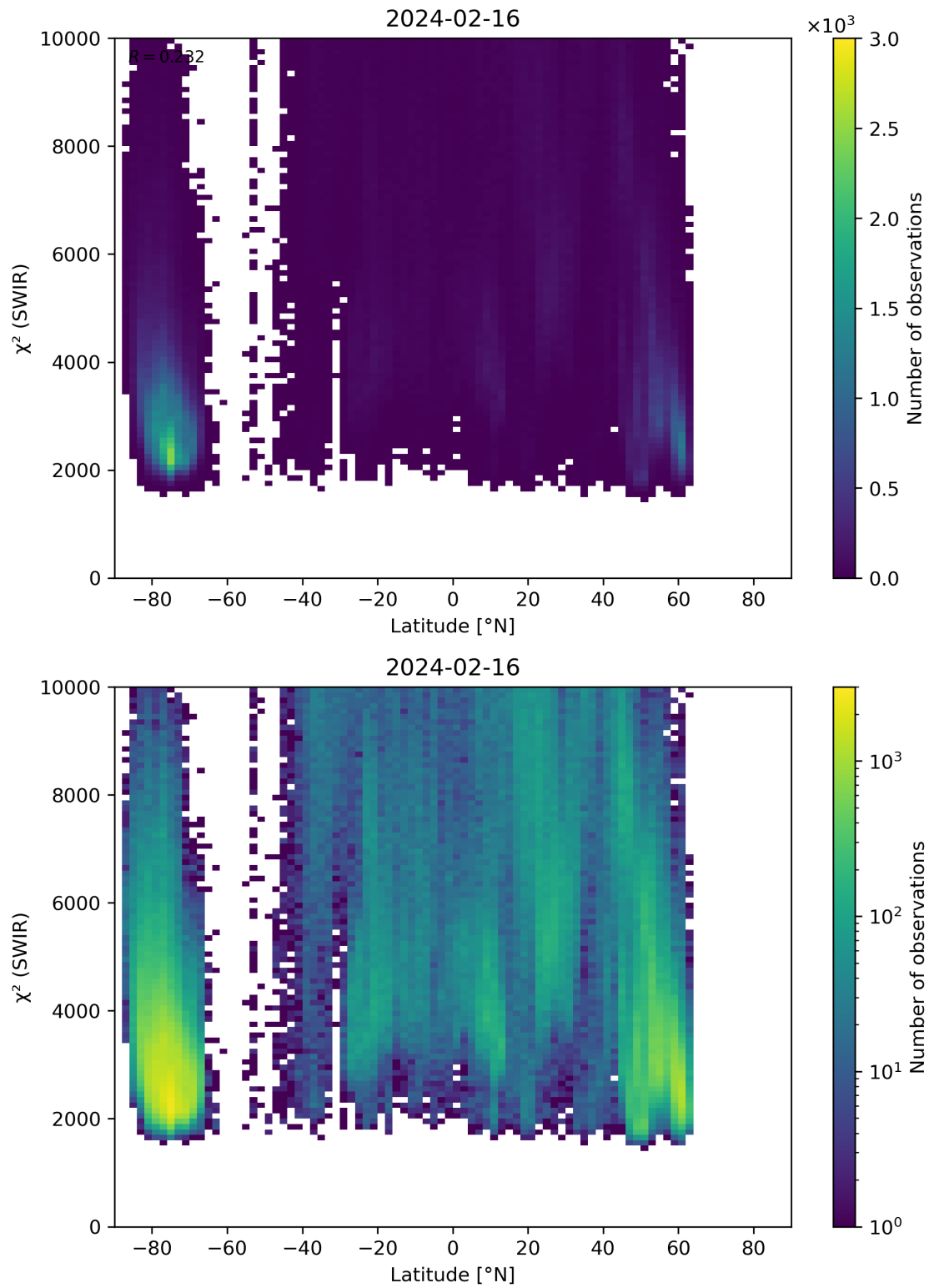
Figure 54: Scatter density plot of “Latitude” against “ \chi^2 (SWIR)” for 2024-02-16 to 2024-02-17.
