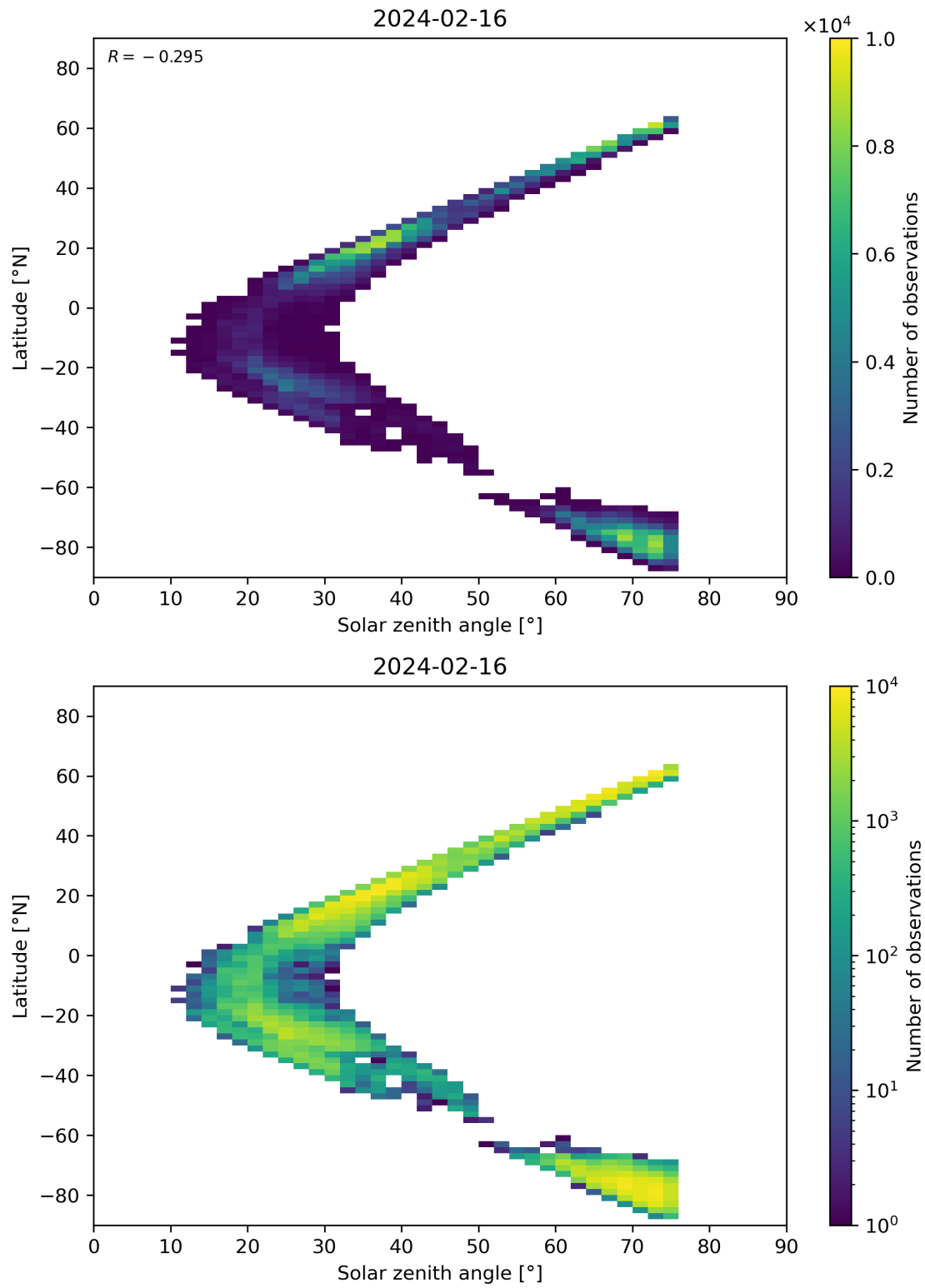
Figure 98: Scatter density plot of “Solar zenith angle” against “Latitude” for 2024-02-16 to 2024-02-17.
