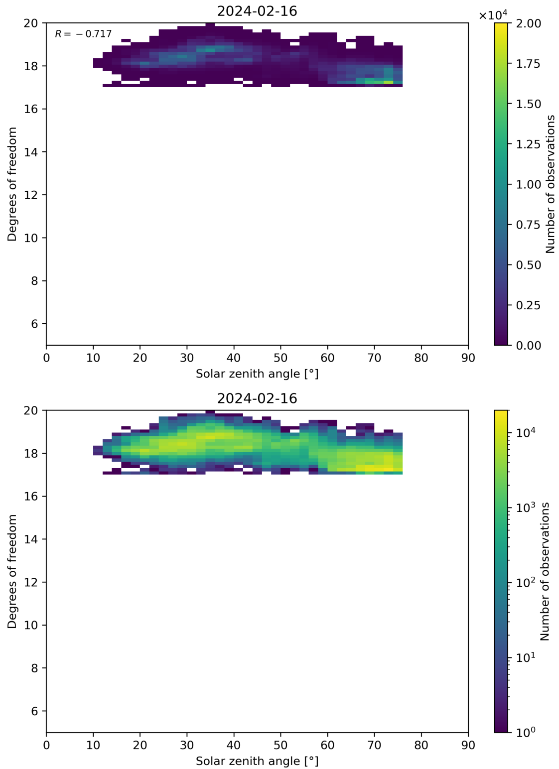
Figure 96: Scatter density plot of “Solar zenith angle” against “Degrees of freedom” for 2024-02-16 to 2024-02-17.
