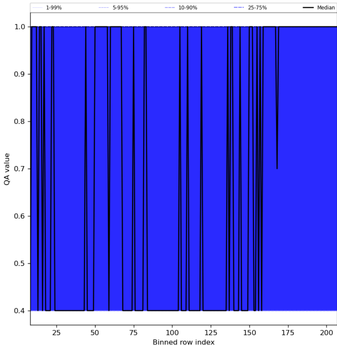
Figure 33: Along track statistics of “QA value” for 2024-02-16 to 2024-02-17
