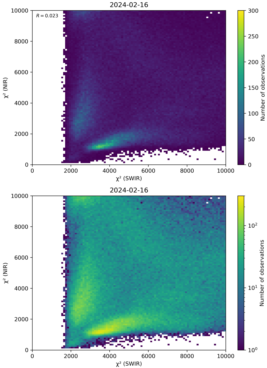
Figure 47: Scatter density plot of “ \chi^2 (SWIR)” against “ \chi^2 (NIR)” for 2024-02-16 to 2024-02-17.
