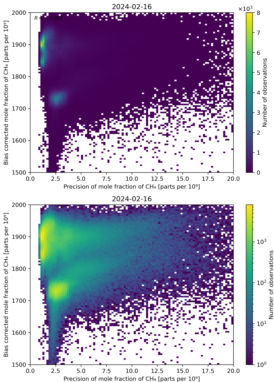
Figure 82: Scatter density plot of “Precision of mole fraction of CH 4 ” against “Bias corrected mole fraction of CH 4 ” for 2024-02-16 to 2024-02-17.
