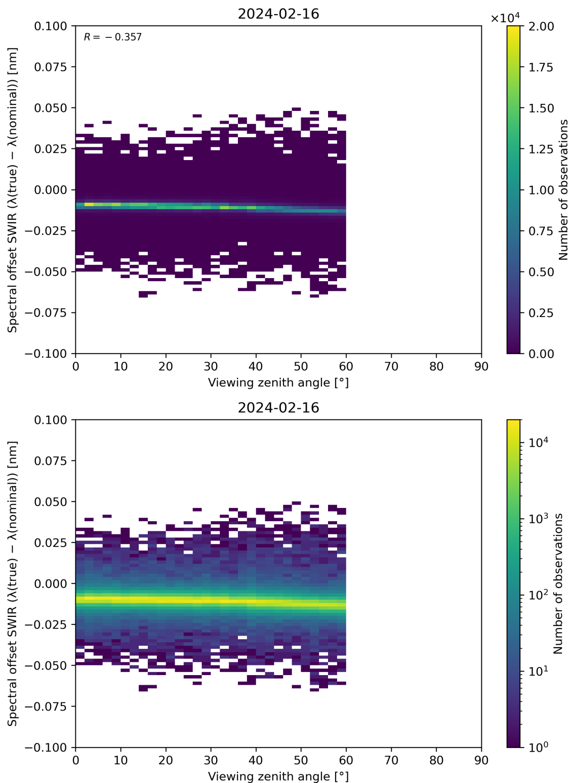
Figure 116: Scatter density plot of “Viewing zenith angle” against “Spectral offset SWIR ( \lambda(\text{true}) - \lambda(\text{nominal}) )” for 2024-02-16 to 2024-02-17.
