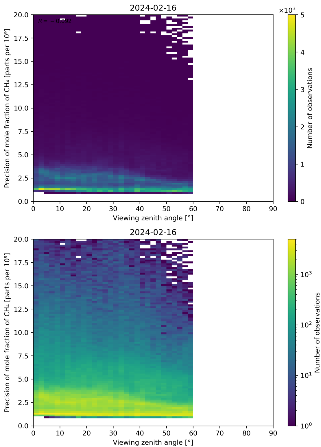
Figure 112: Scatter density plot of “Viewing zenith angle” against “Precision of mole fraction of CH 4 ” for 2024-02-16 to 2024-02-17.
