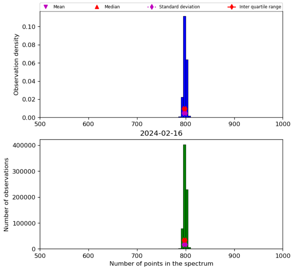
Figure 26: Histogram of “Number of points in the spectrum” for 2024-02-16 to 2024-02-17
