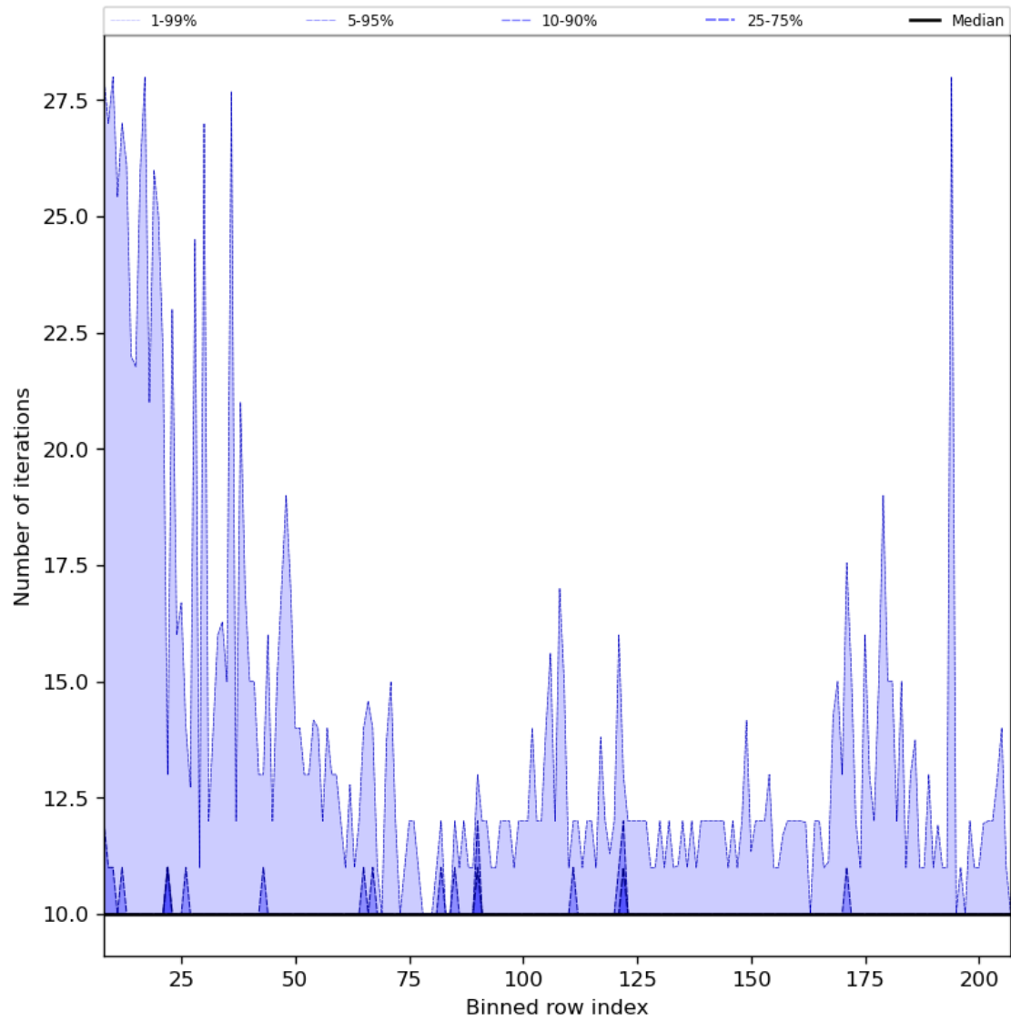
Figure 42: Along track statistics of “Number of iterations” for 2024-02-16 to 2024-02-17
