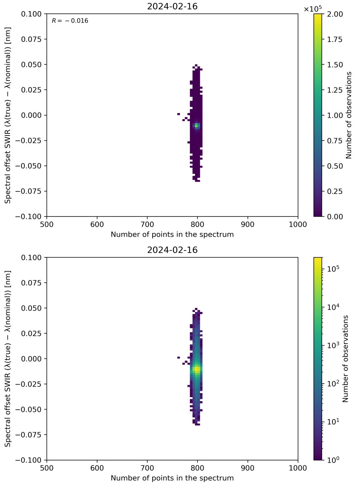
Figure 93: Scatter density plot of “Number of points in the spectrum” against “Spectral offset SWIR ( \lambda(\text{true}) - \lambda(\text{nominal}) )” for 2024-02-16 to 2024-02-17.
