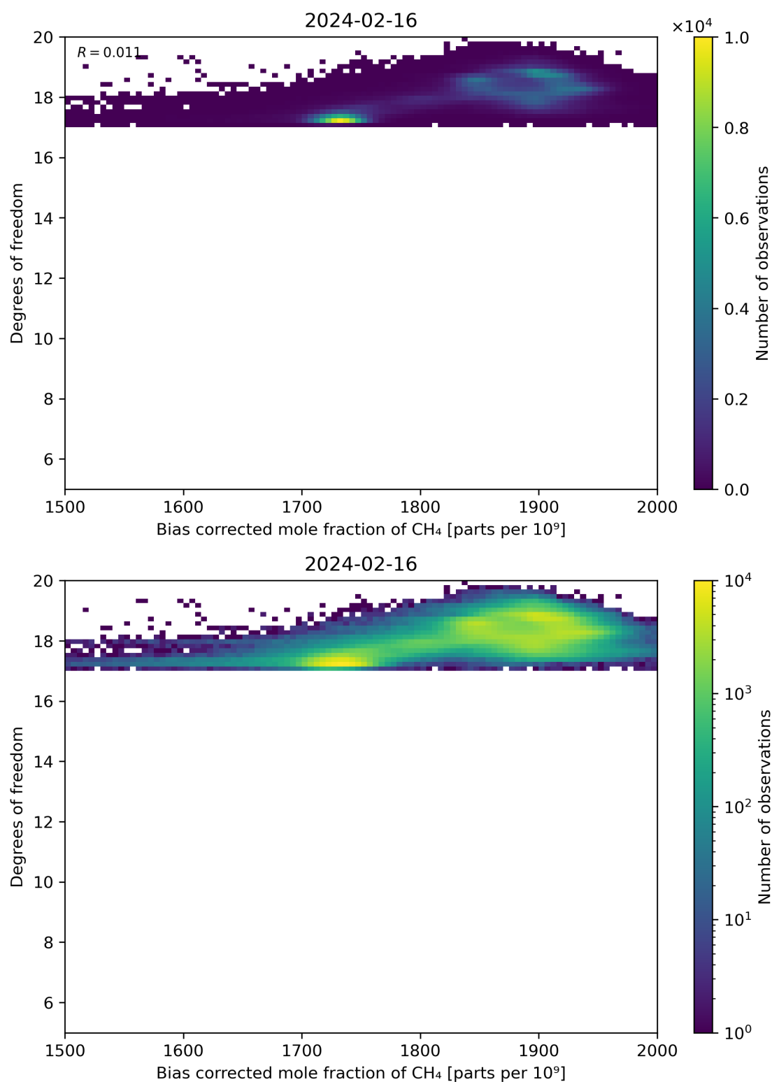
Figure 65: Scatter density plot of “Bias corrected mole fraction of CH 4 ” against “Degrees of freedom” for 2024-02-16 to 2024-02-17.
