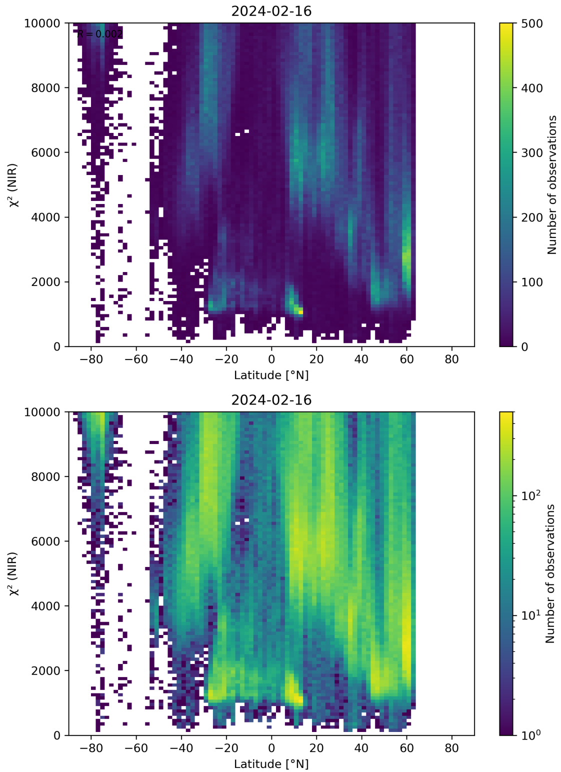
Figure 53: Scatter density plot of “Latitude” against “ \chi^2 (NIR)” for 2024-02-16 to 2024-02-17.
