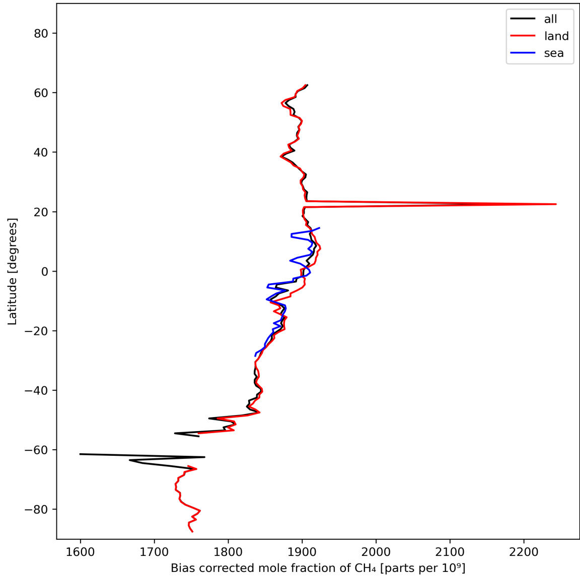
Figure 14: Zonal average of “Bias corrected mole fraction of CH 4 ” for 2024-02-16 to 2024-02-17.
