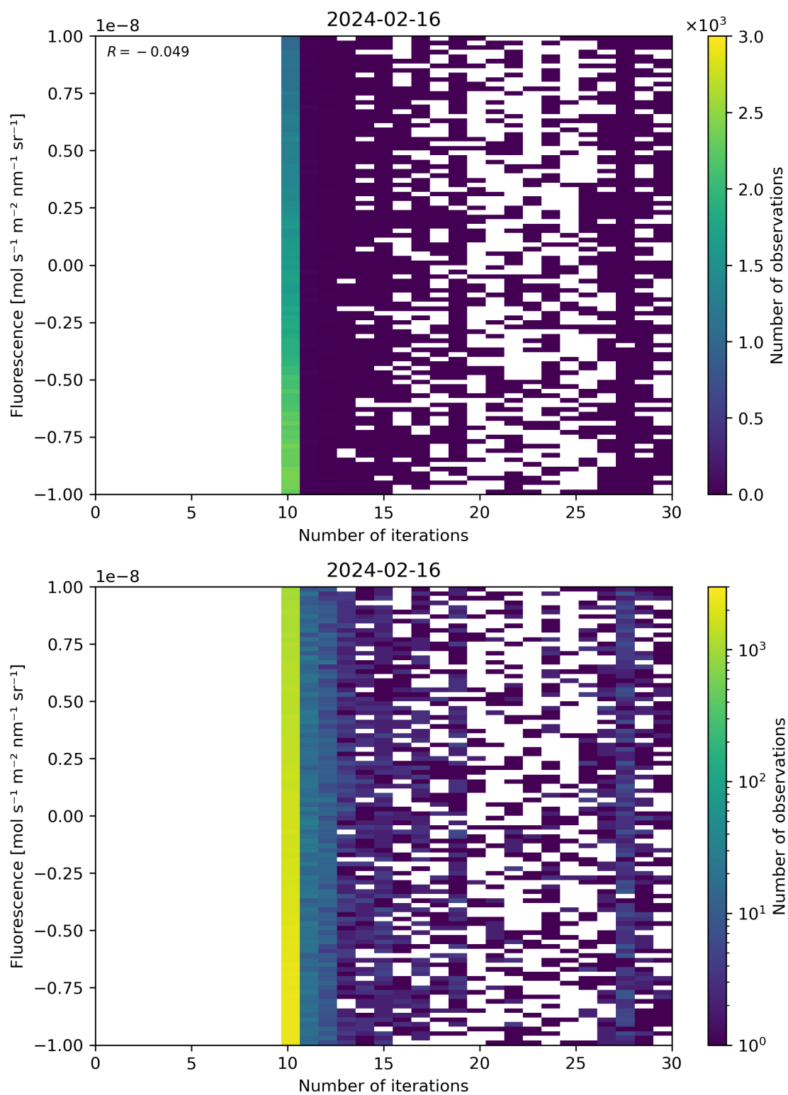
Figure 87: Scatter density plot of “Number of iterations” against “Fluorescence” for 2024-02-16 to 2024-02-17.
