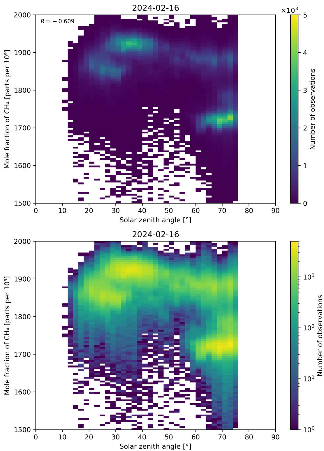
Figure 99: Scatter density plot of “Solar zenith angle” against “Mole fraction of CH 4 ” for 2024-02-16 to 2024-02-17.
