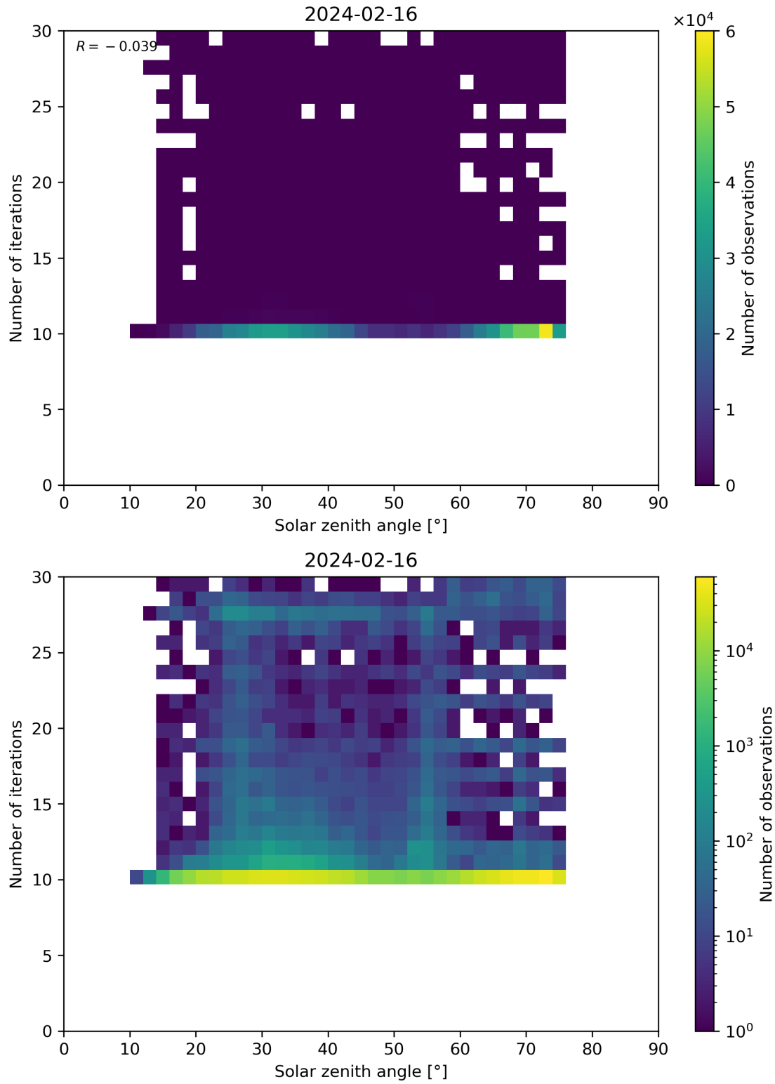
Figure 102: Scatter density plot of “Solar zenith angle” against “Number of iterations” for 2024-02-16 to 2024-02-17.
