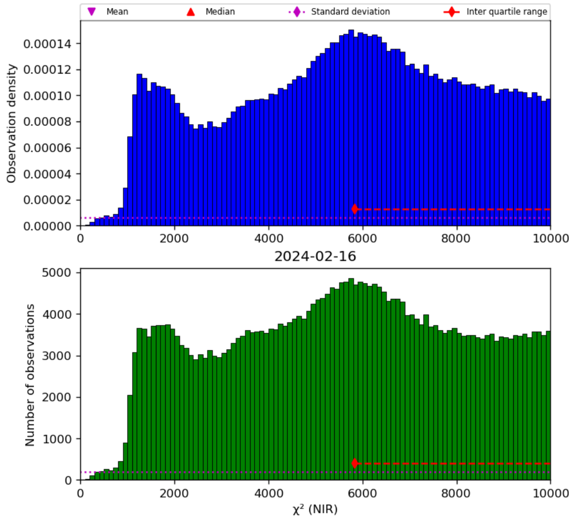
Figure 29: Histogram of " \chi^2 (NIR)" for 2024-02-16 to 2024-02-17
