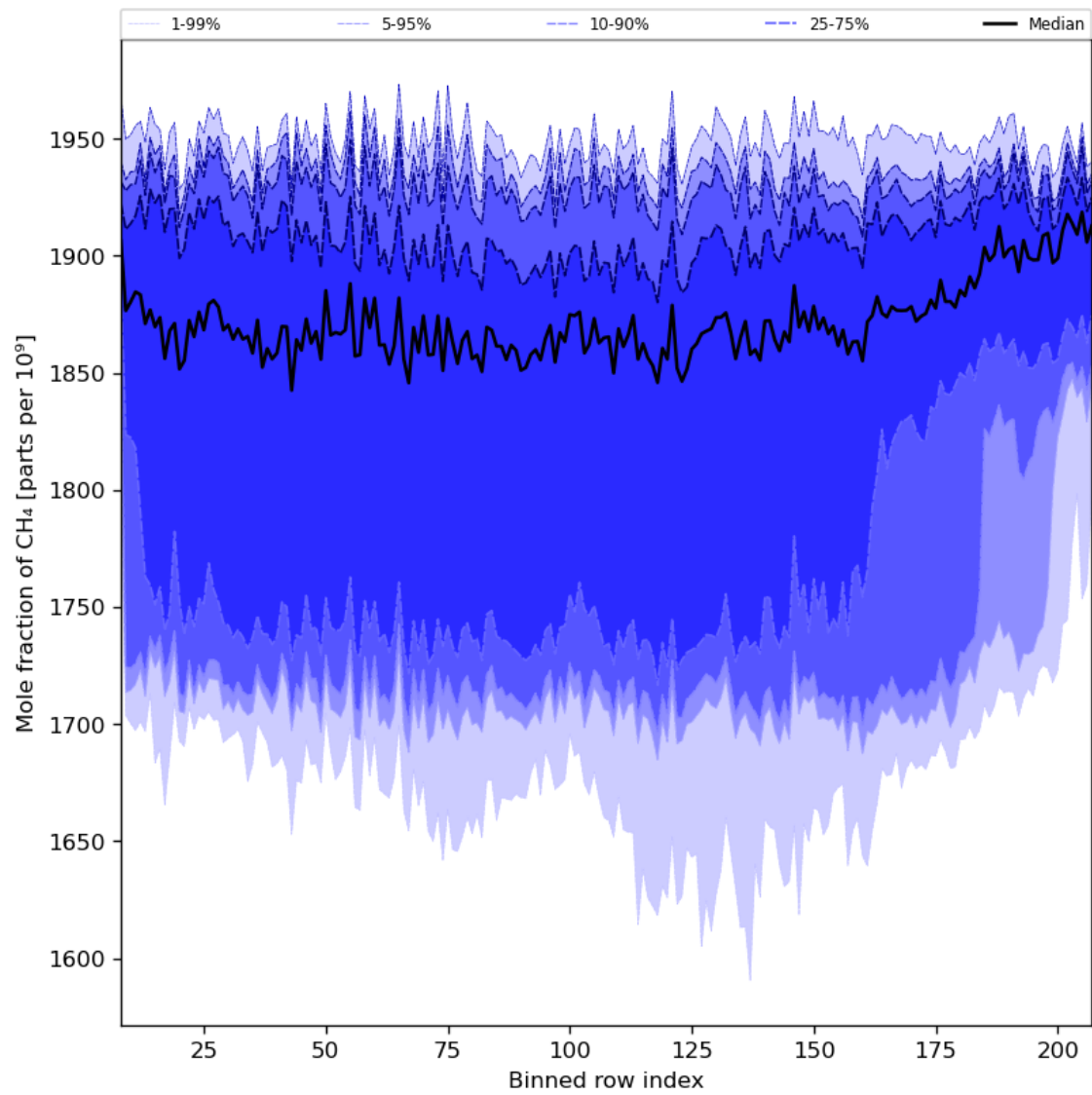
Figure 34: Along track statistics of “Mole fraction of CH 4 ” for 2024-02-16 to 2024-02-17
