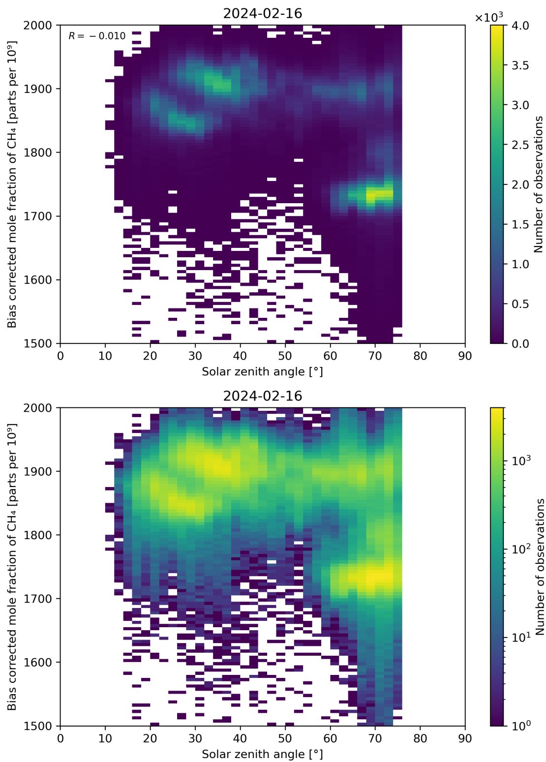
Figure 100: Scatter density plot of “Solar zenith angle” against “Bias corrected mole fraction of \text{CH}_4 ” for 2024-02-16 to 2024-02-17.
