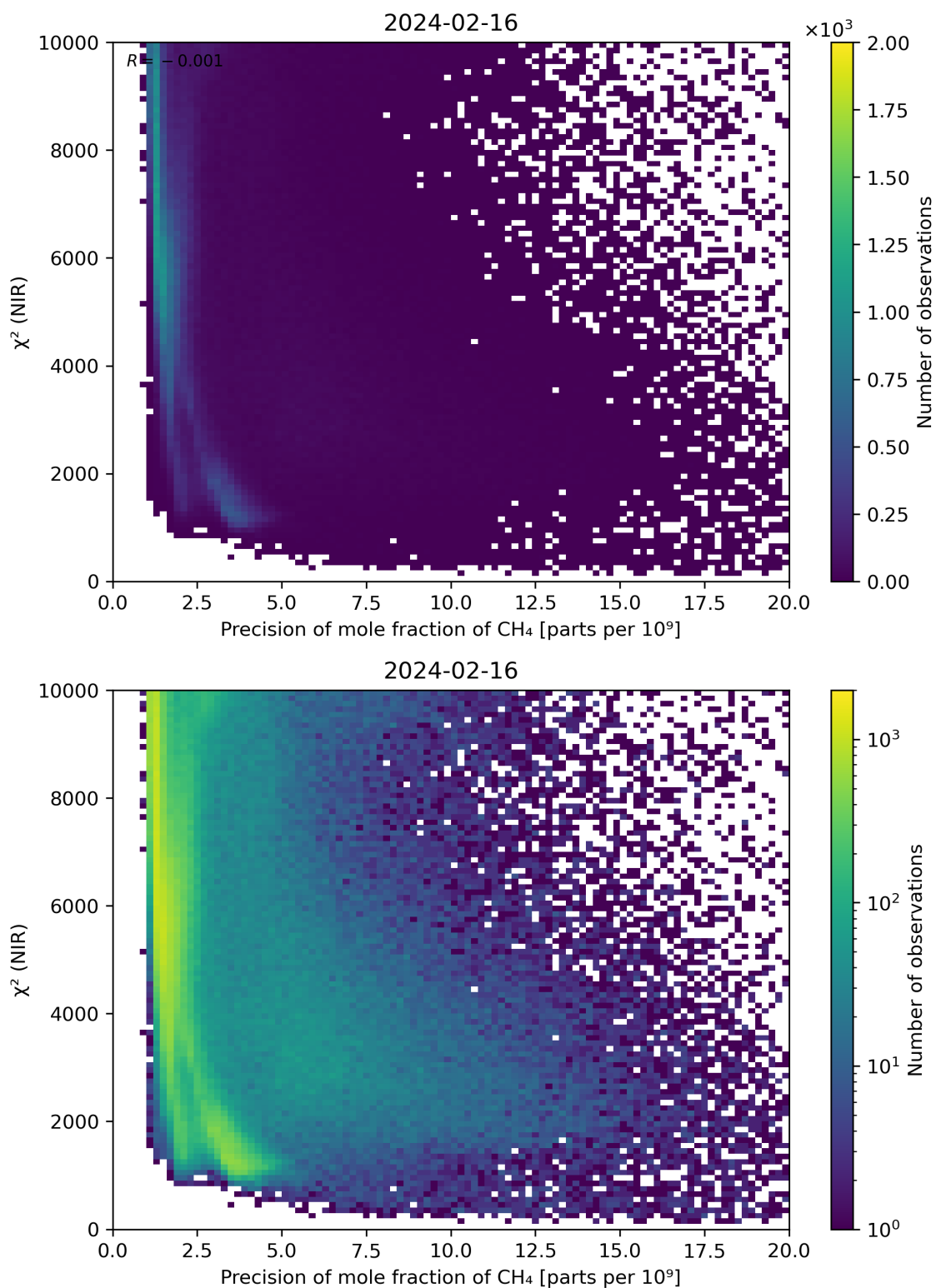
Figure 78: Scatter density plot of “Precision of mole fraction of CH 4 ” against “ \chi^2 (NIR)” for 2024-02-16 to 2024-02-17.
