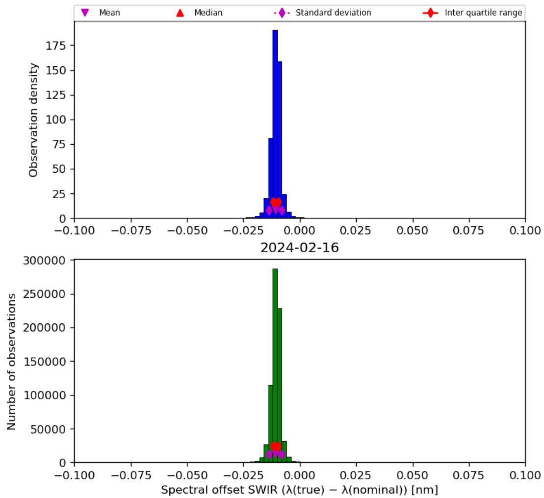
Figure 27: Histogram of “Spectral offset SWIR ( \lambda(\text{true}) - \lambda(\text{nominal}) )” for 2024-02-16 to 2024-02-17
