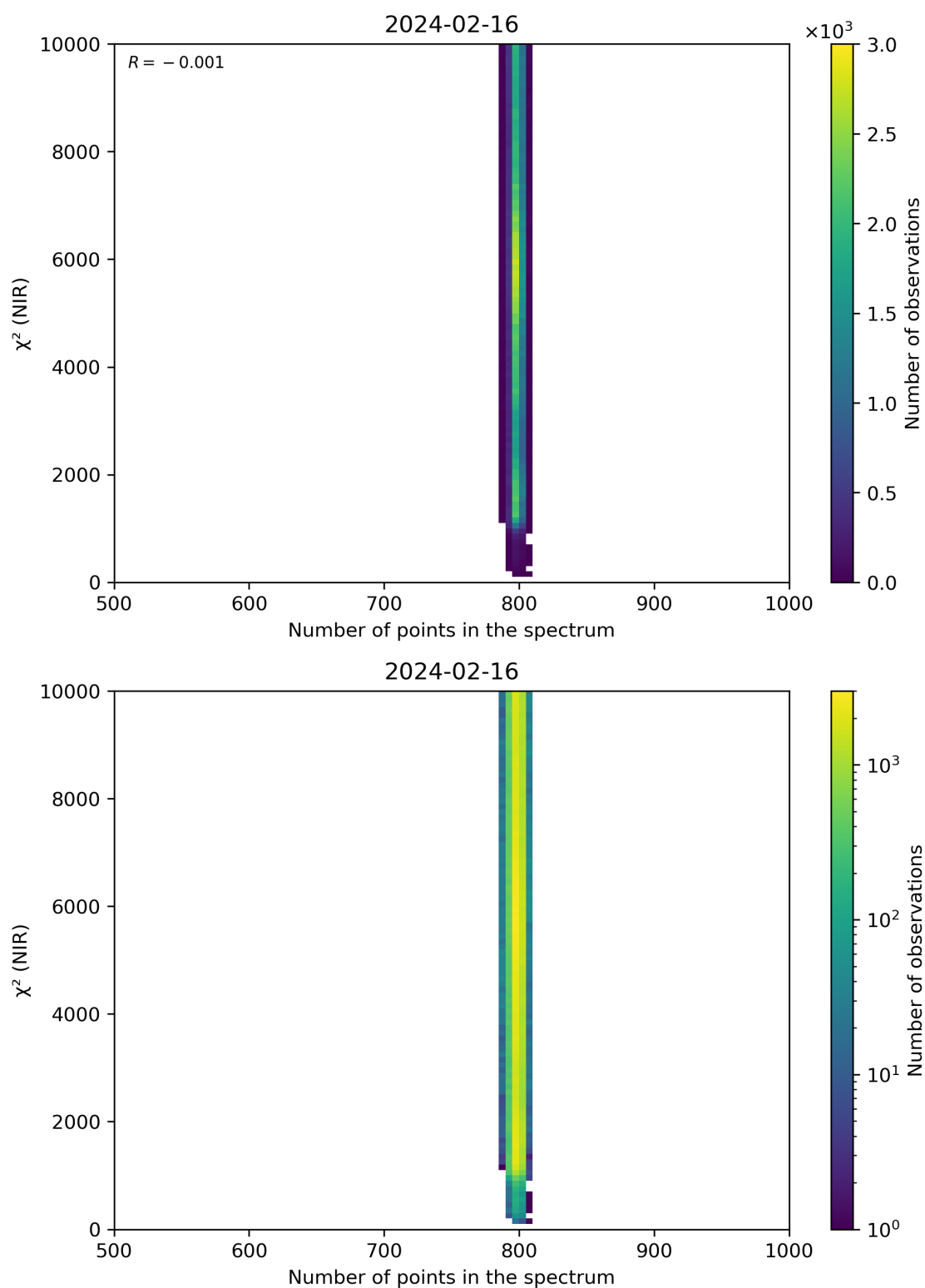
Figure 88: Scatter density plot of “Number of points in the spectrum” against “ \chi^2 (NIR)” for 2024-02-16 to 2024-02-17.
