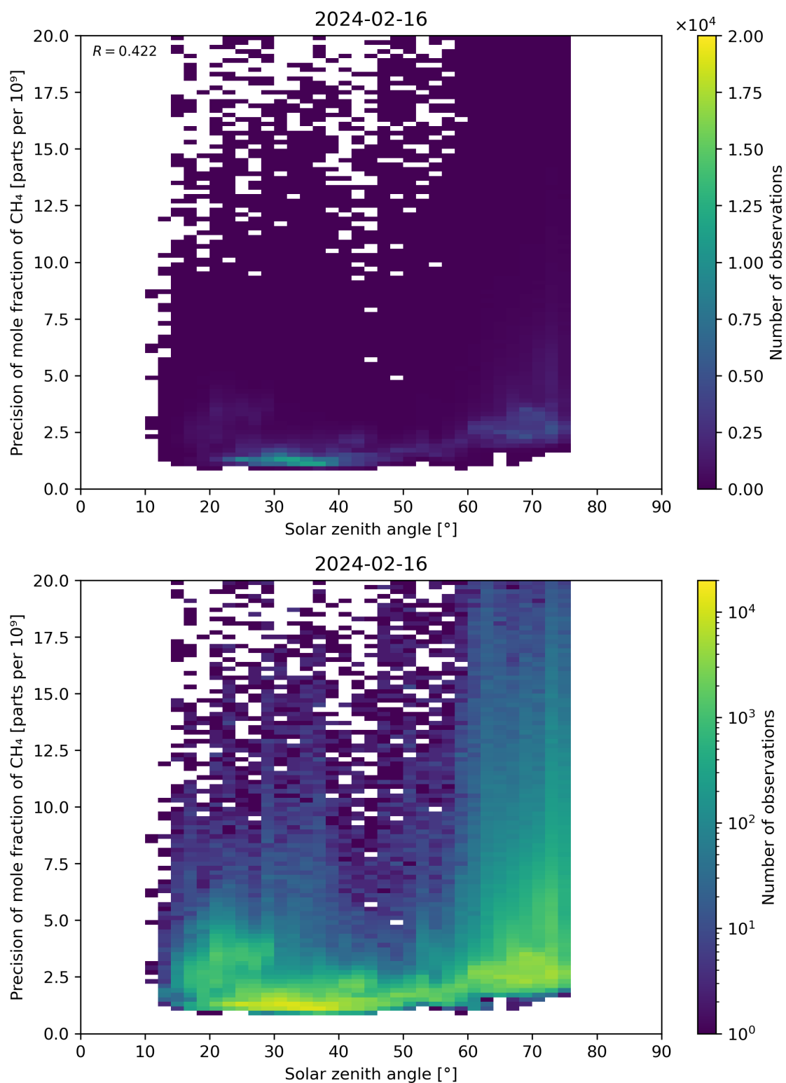
Figure 101: Scatter density plot of “Solar zenith angle” against “Precision of mole fraction of CH 4 ” for 2024-02-16 to 2024-02-17.
