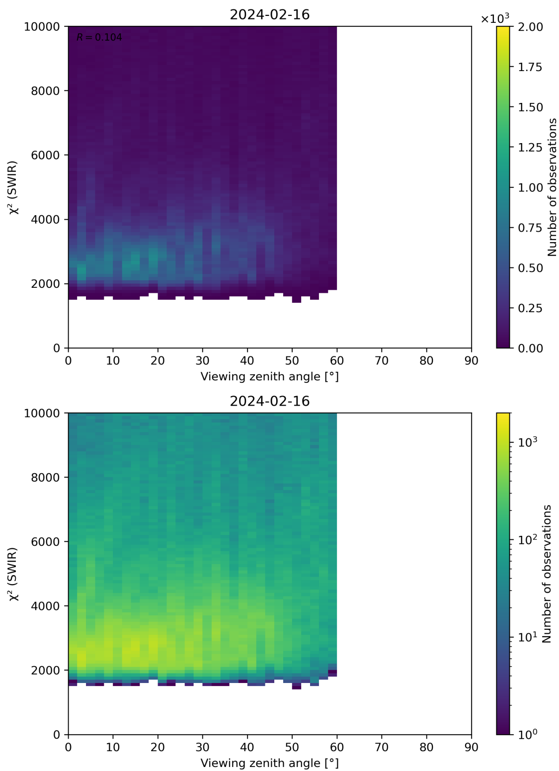
Figure 106: Scatter density plot of “Viewing zenith angle” against “ \chi^2 (SWIR)” for 2024-02-16 to 2024-02-17.
