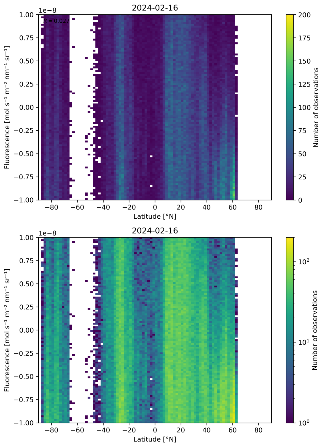
Figure 56: Scatter density plot of “Latitude” against “Fluorescence” for 2024-02-16 to 2024-02-17.
