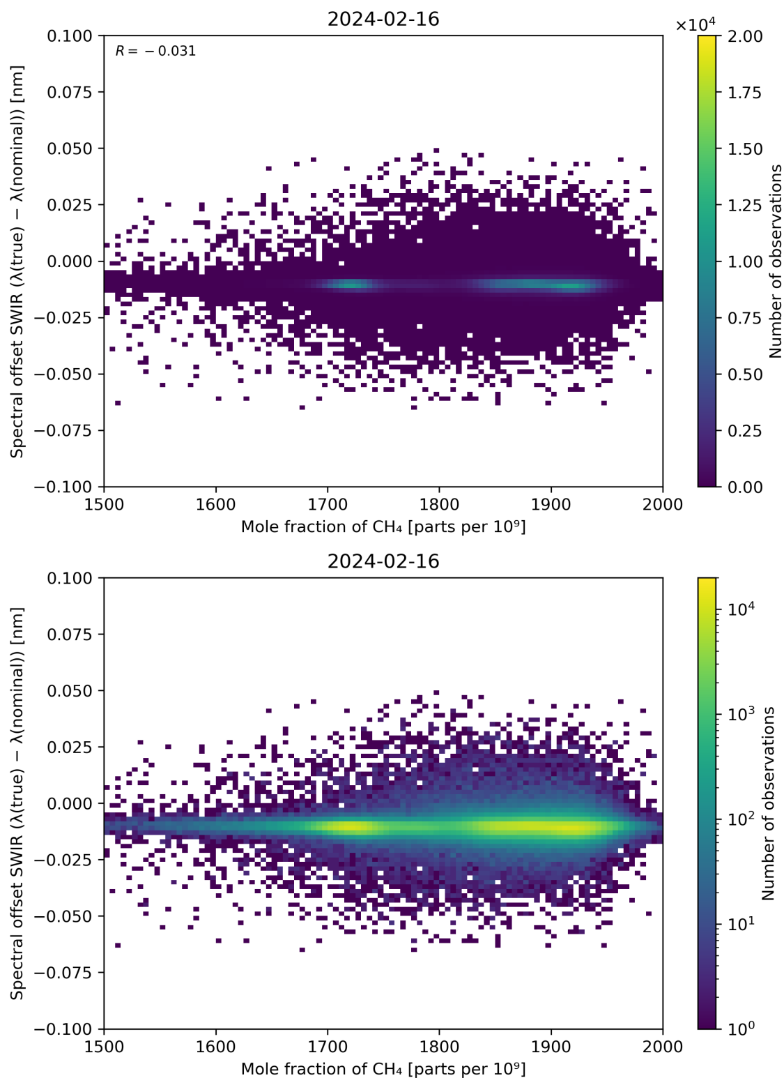
Figure 86: Scatter density plot of “Mole fraction of CH 4 ” against “Spectral offset SWIR ( \lambda(\text{true}) - \lambda(\text{nominal}) )” for 2024-02-16 to 2024-02-17.
