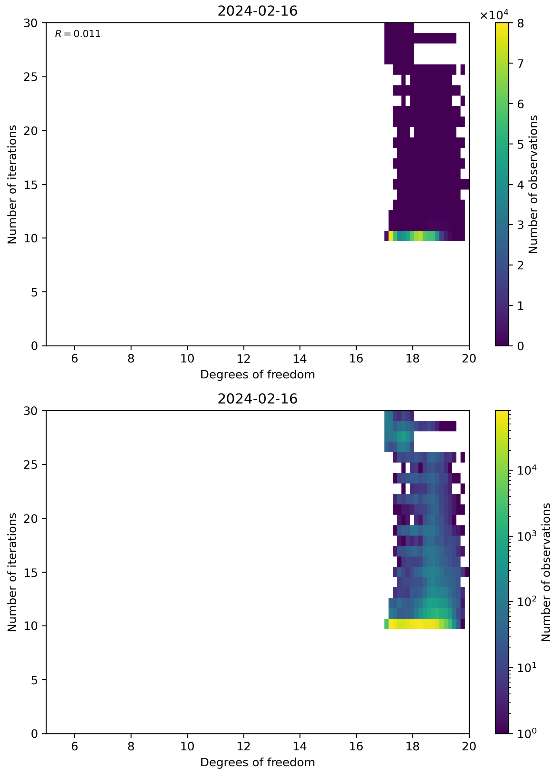
Figure 52: Scatter density plot of “Degrees of freedom” against “Number of iterations” for 2024-02-16 to 2024-02-17.
