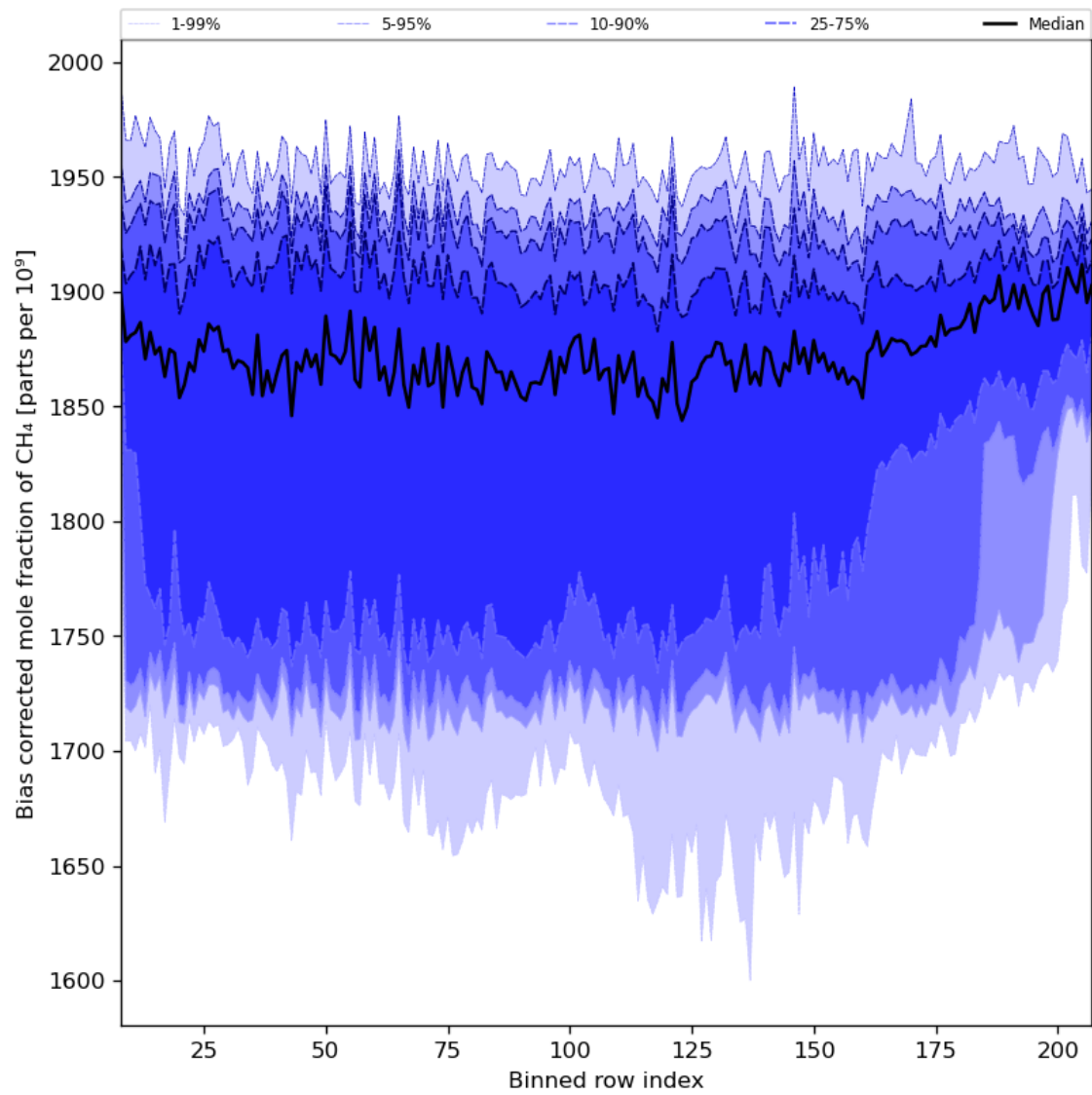
Figure 36: Along track statistics of “Bias corrected mole fraction of CH 4 ” for 2024-02-16 to 2024-02-17
