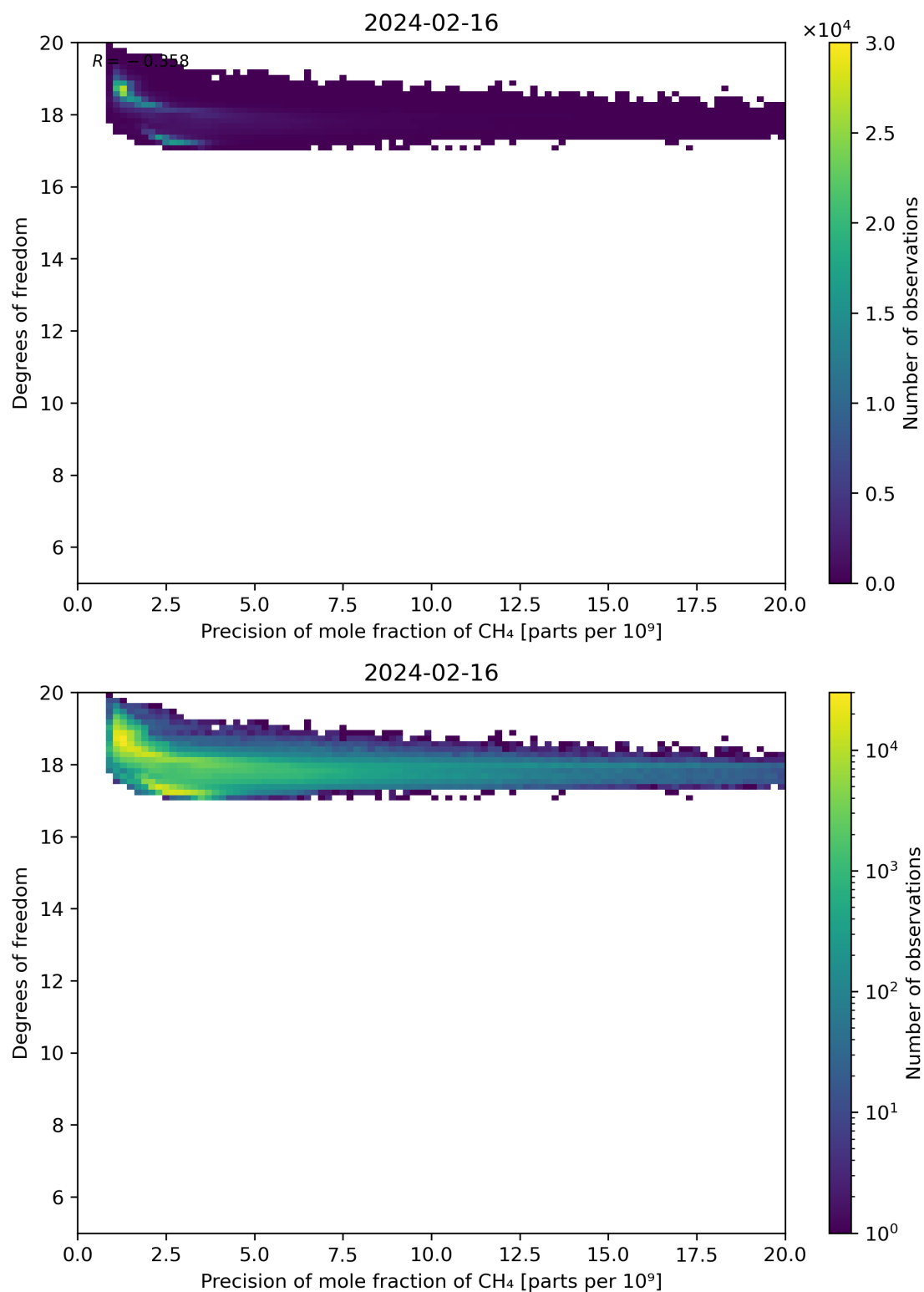
Figure 80: Scatter density plot of “Precision of mole fraction of CH 4 ” against “Degrees of freedom” for 2024-02-16 to 2024-02-17.
