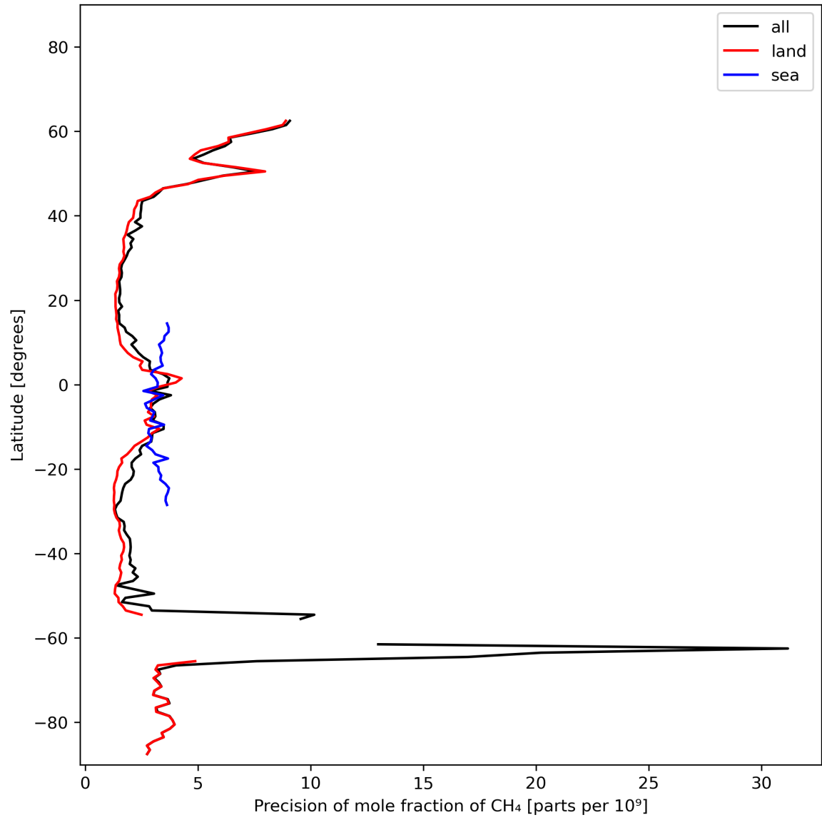
Figure 13: Zonal average of “Precision of mole fraction of CH 4 ” for 2024-02-16 to 2024-02-17.
