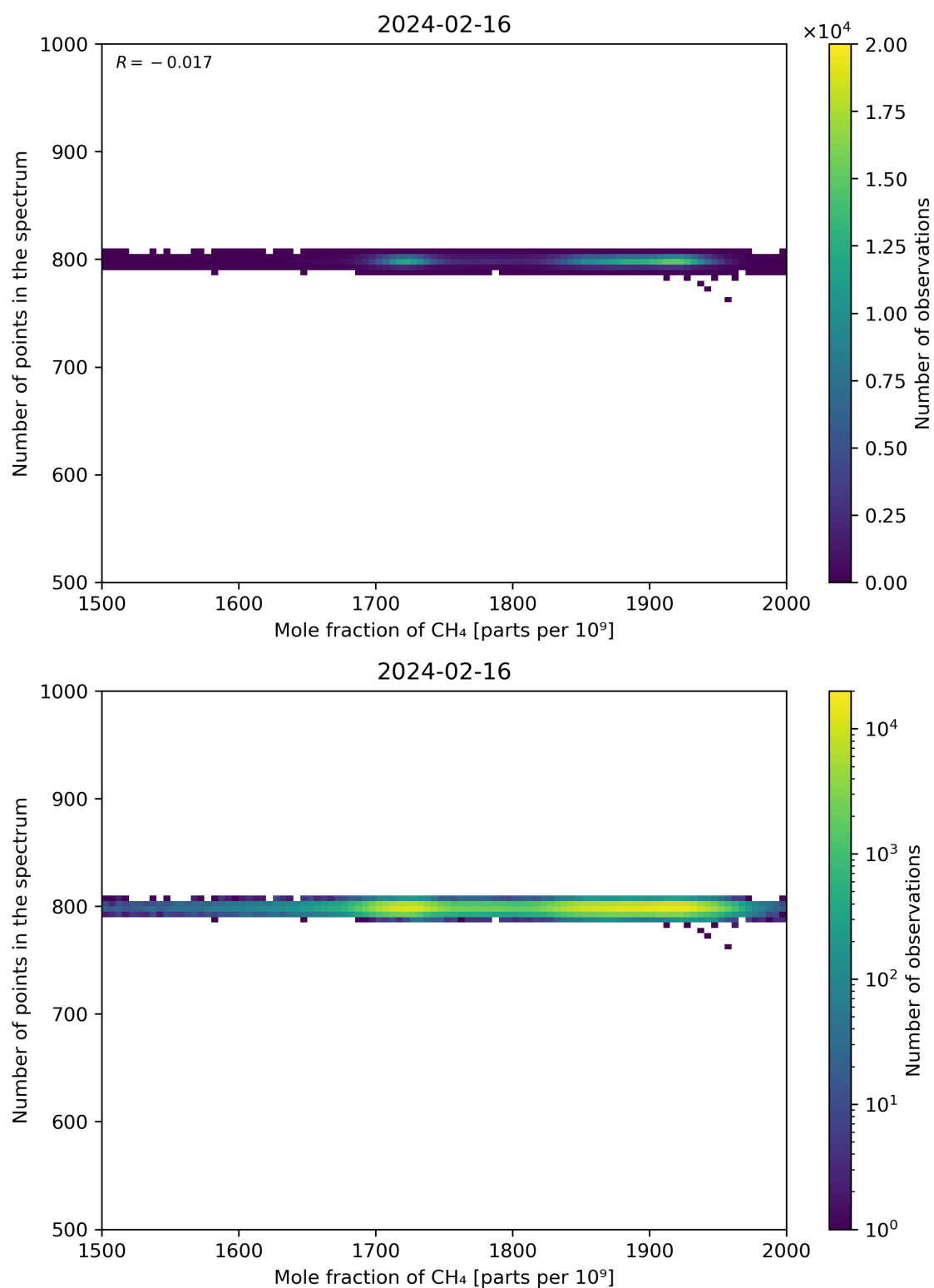
Figure 77: Scatter density plot of “Mole fraction of CH 4 ” against “Number of points in the spectrum” for 2024-02-16 to 2024-02-17.
