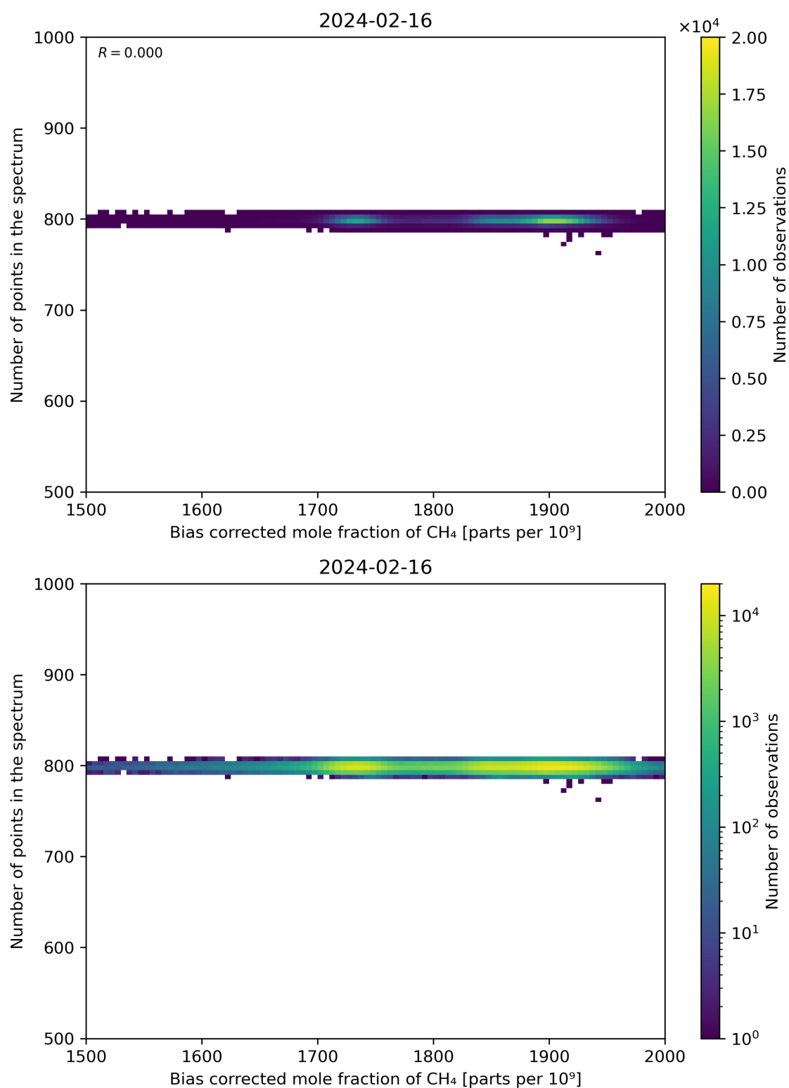
Figure 68: Scatter density plot of “Bias corrected mole fraction of CH 4 ” against “Number of points in the spectrum” for 2024-02-16 to 2024-02-17.
