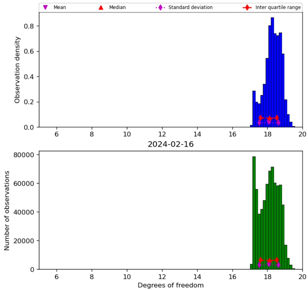
Figure 30: Histogram of “Degrees of freedom” for 2024-02-16 to 2024-02-17
