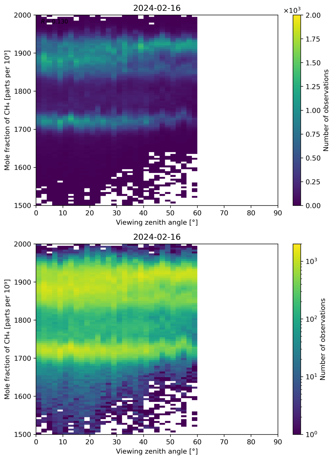
Figure 110: Scatter density plot of “Viewing zenith angle” against “Mole fraction of CH 4 ” for 2024-02-16 to 2024-02-17.
