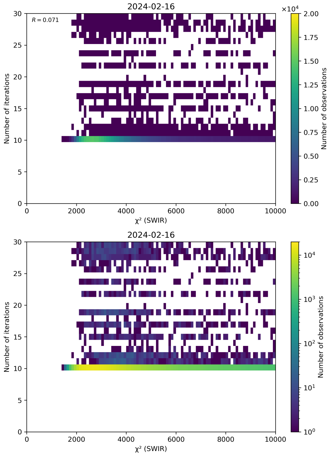
Figure 50: Scatter density plot of “ \chi^2 (SWIR)” against “Number of iterations” for 2024-02-16 to 2024-02-17.
