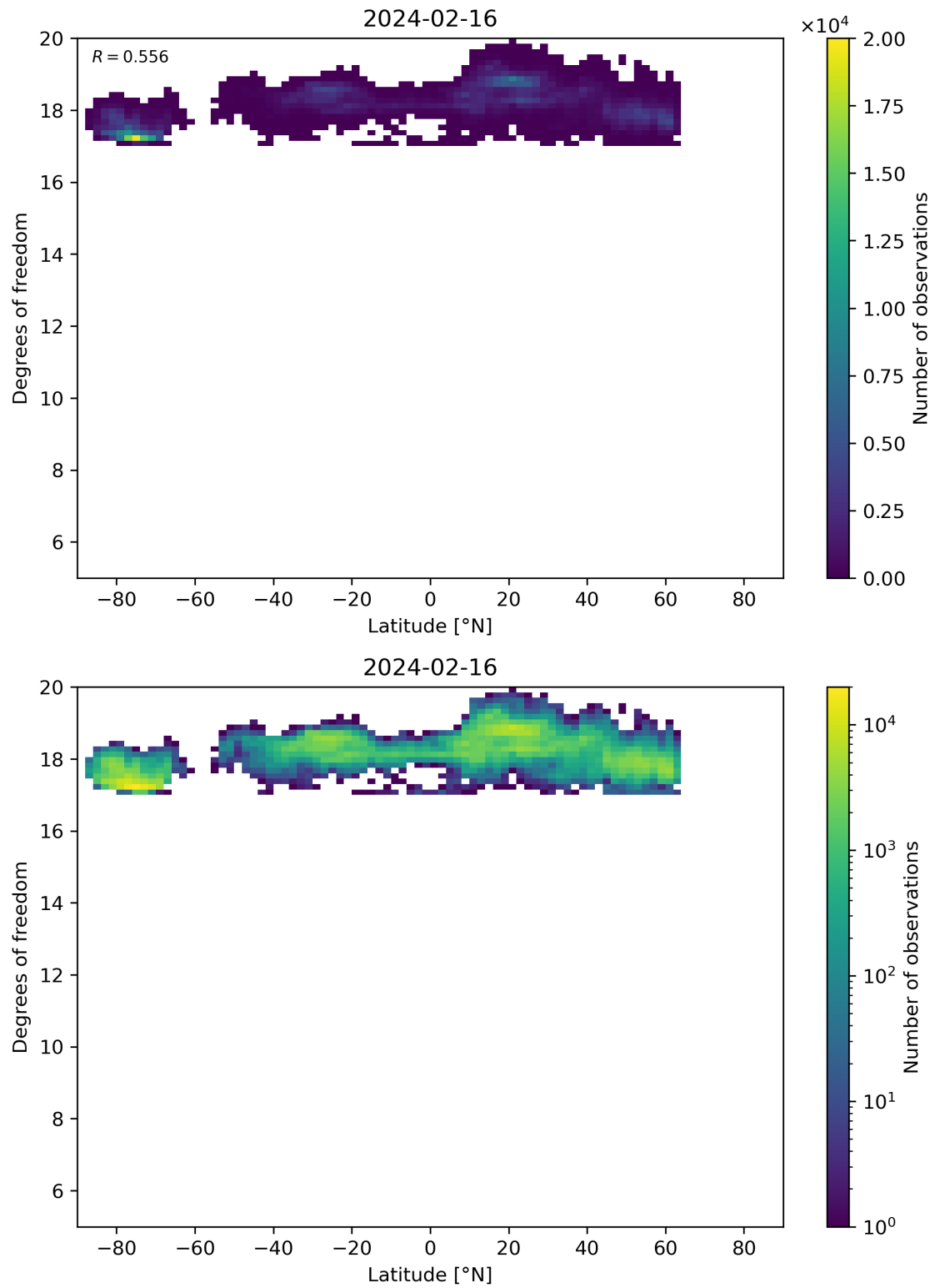
Figure 55: Scatter density plot of “Latitude” against “Degrees of freedom” for 2024-02-16 to 2024-02-17.
