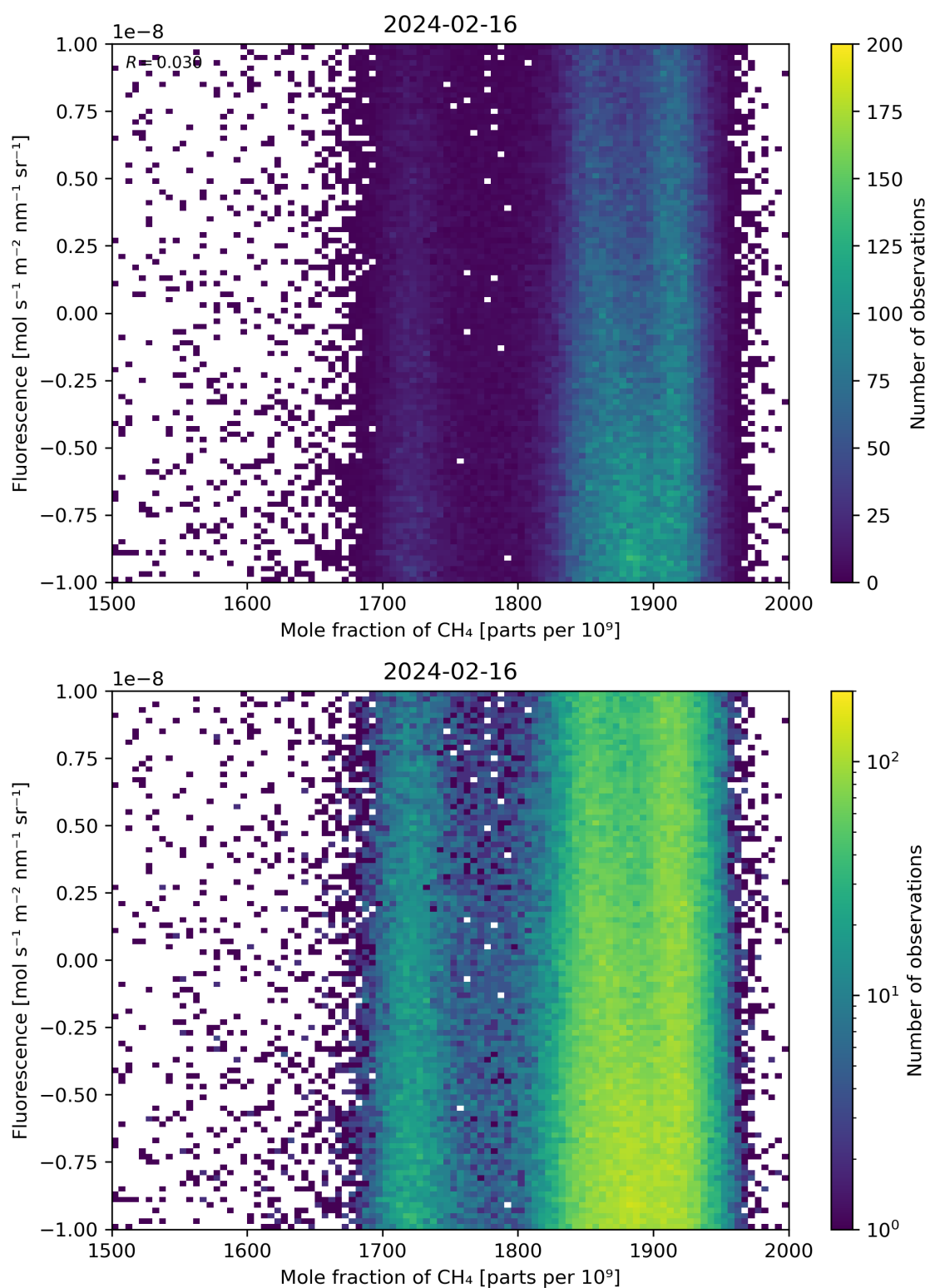
Figure 73: Scatter density plot of “Mole fraction of \text{CH}_4 ” against “Fluorescence” for 2024-02-16 to 2024-02-17.
