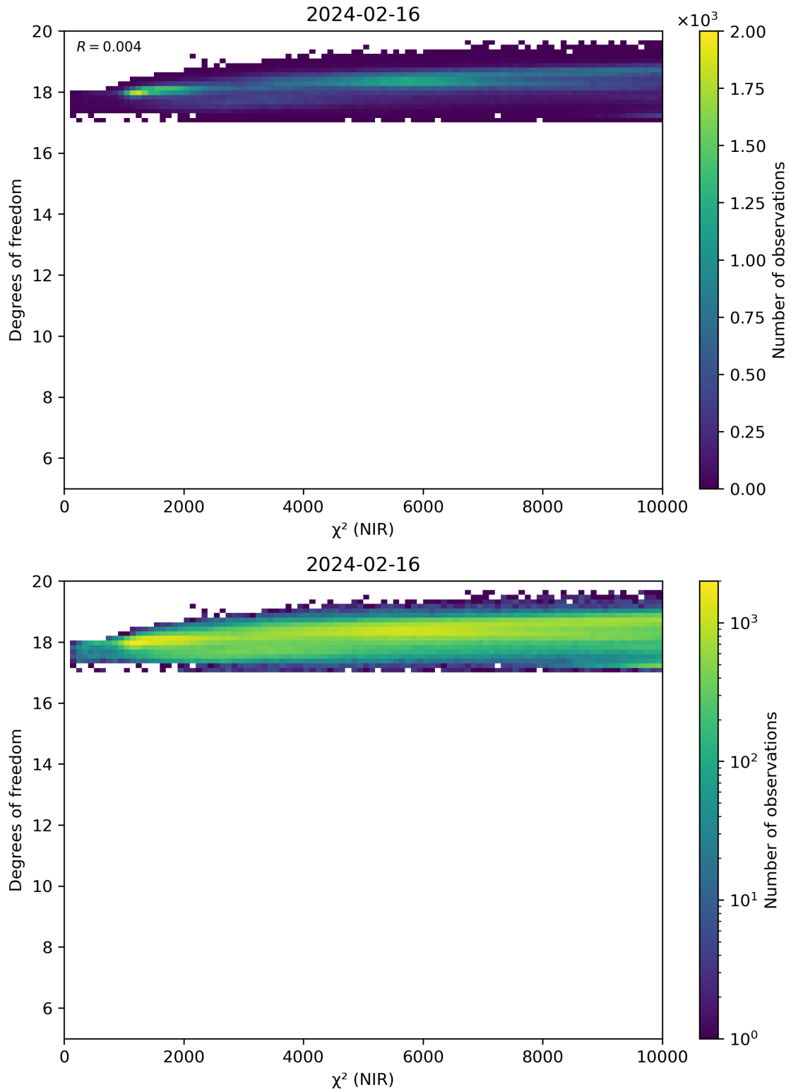
Figure 44: Scatter density plot of “ \chi^2 (NIR)” against “Degrees of freedom” for 2024-02-16 to 2024-02-17.
