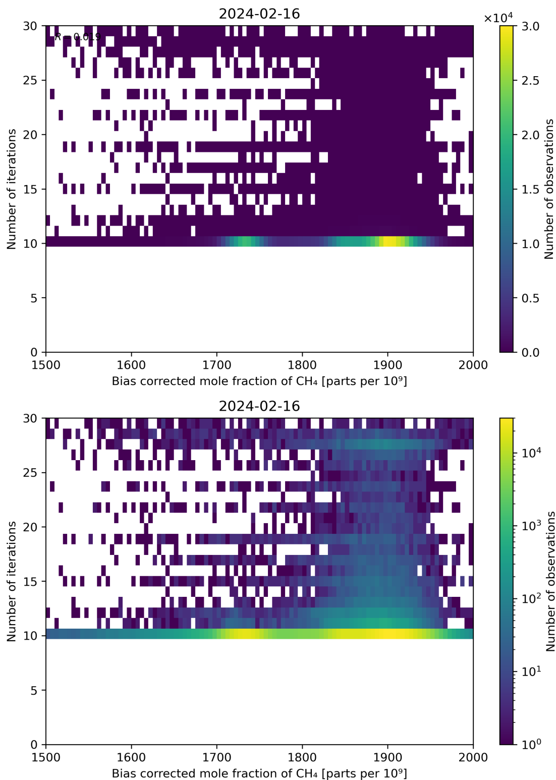
Figure 67: Scatter density plot of “Bias corrected mole fraction of \text{CH}_4 ” against “Number of iterations” for 2024-02-16 to 2024-02-17.
