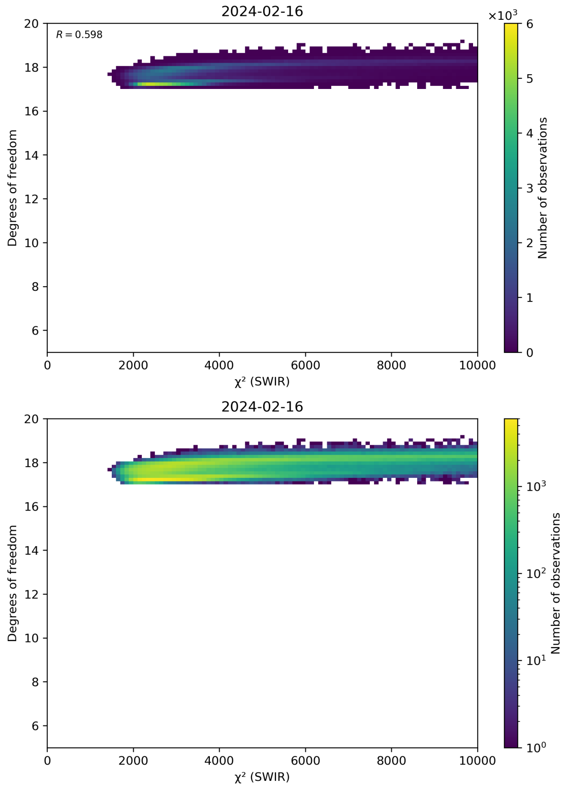
Figure 48: Scatter density plot of “ \chi^2 (SWIR)” against “Degrees of freedom” for 2024-02-16 to 2024-02-17.
