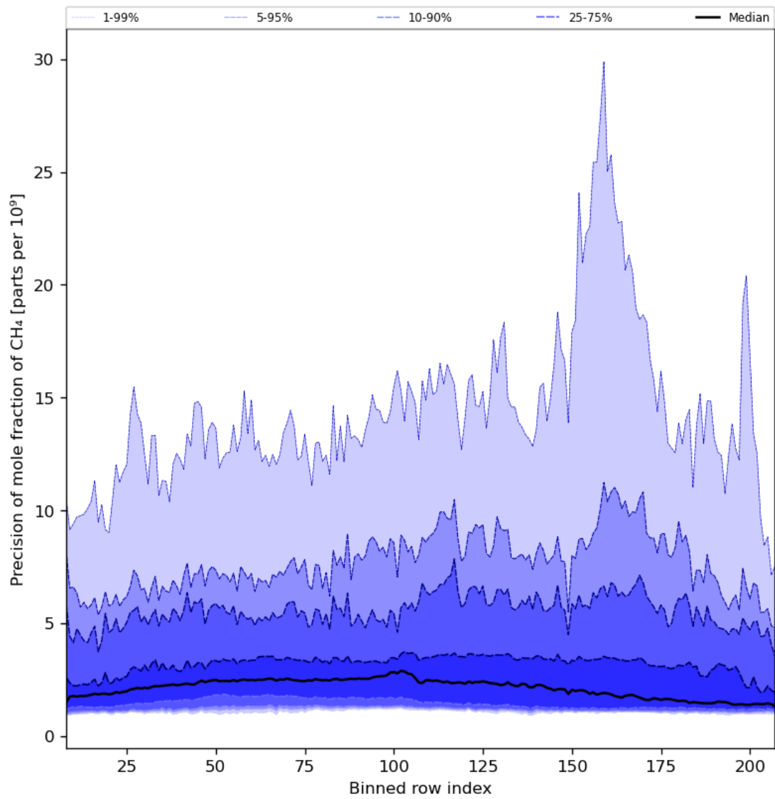
Figure 35: Along track statistics of “Precision of mole fraction of CH 4 ” for 2024-02-16 to 2024-02-17
