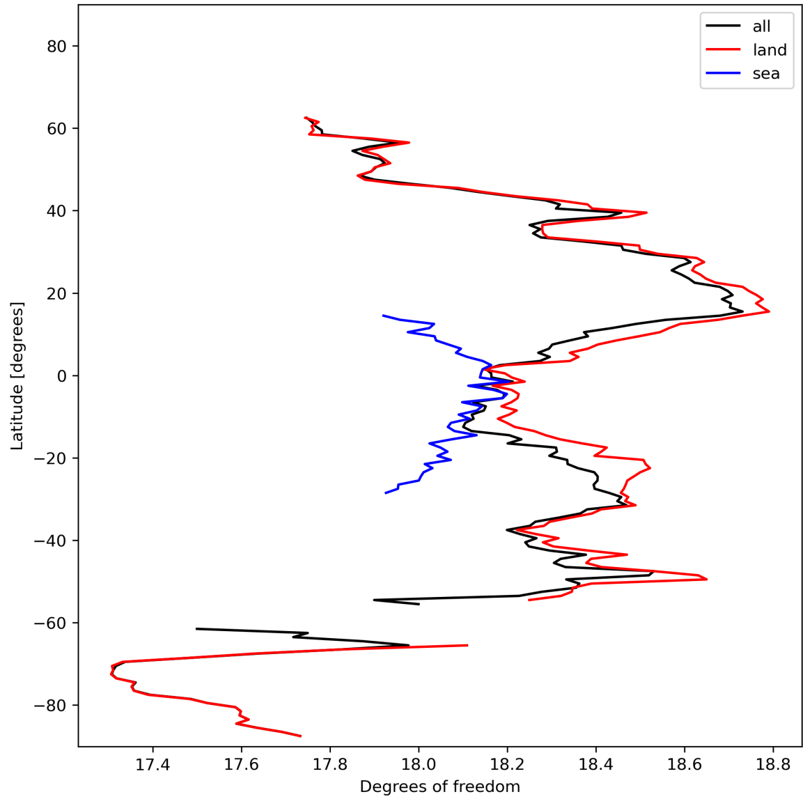
Figure 19: Zonal average of “Degrees of freedom” for 2024-02-16 to 2024-02-17.
