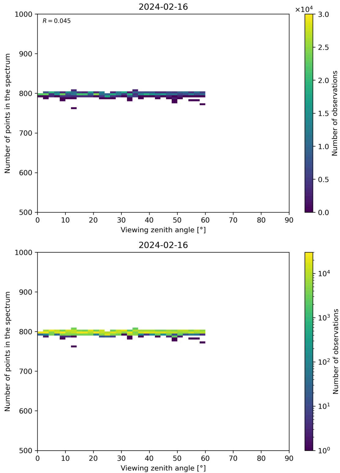
Figure 114: Scatter density plot of “Viewing zenith angle” against “Number of points in the spectrum” for 2024-02-16 to 2024-02-17.
