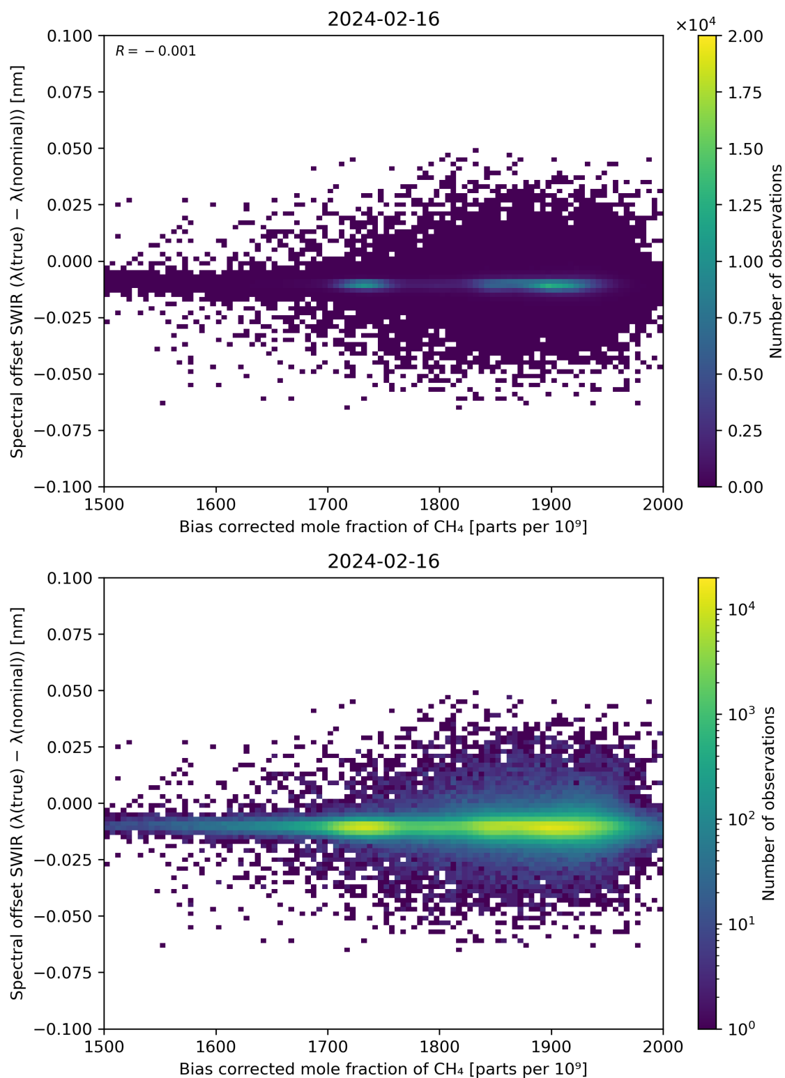
Figure 69: Scatter density plot of “Bias corrected mole fraction of \text{CH}_4 ” against “Spectral offset SWIR ( \lambda(\text{true}) - \lambda(\text{nominal}) )” for 2024-02-16 to 2024-02-17.
