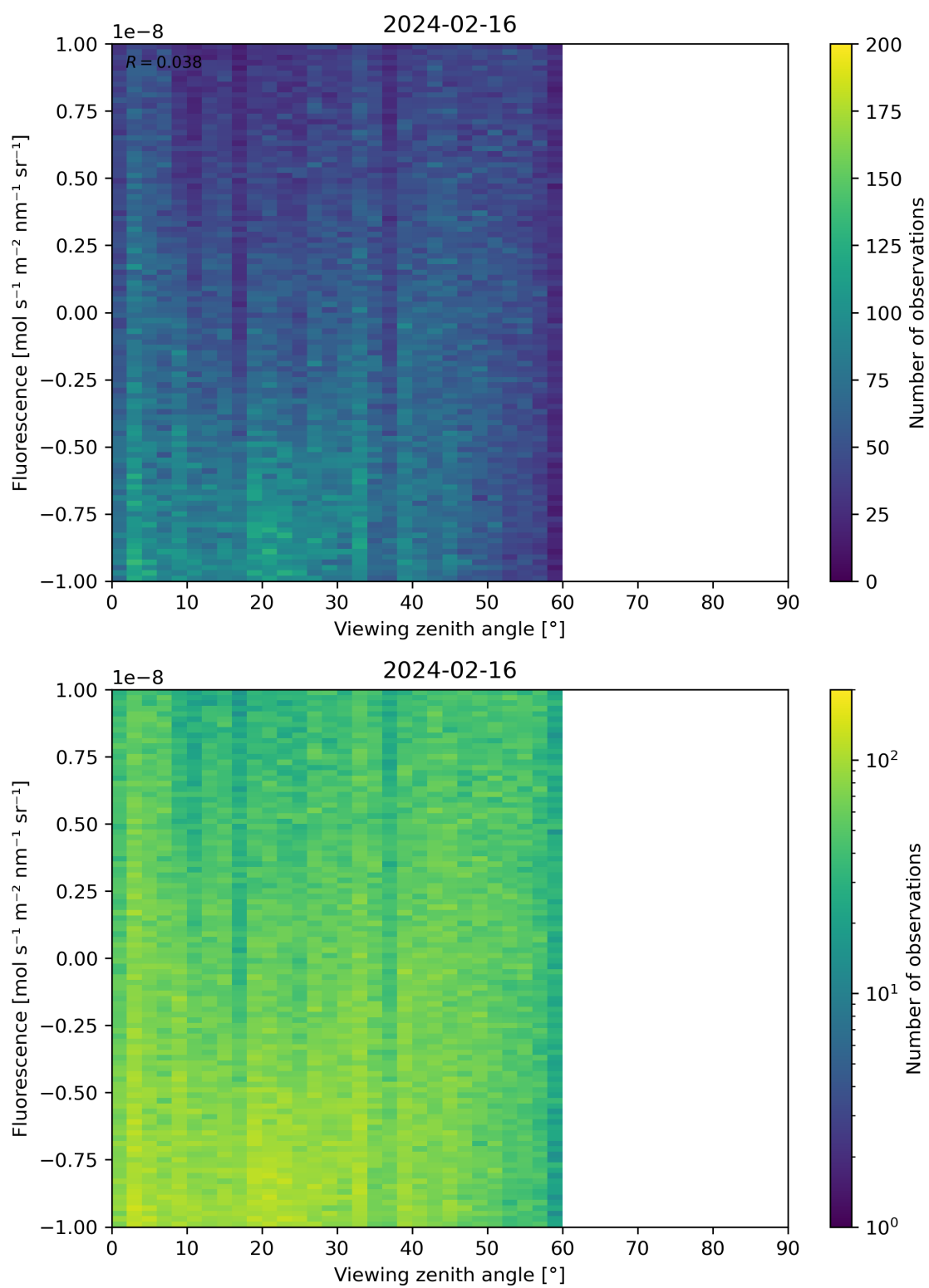
Figure 108: Scatter density plot of “Viewing zenith angle” against “Fluorescence” for 2024-02-16 to 2024-02-17.
