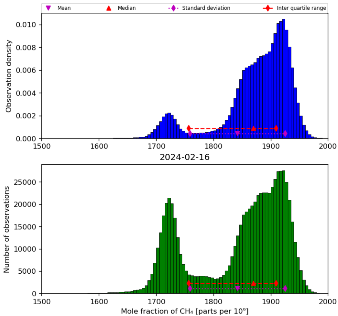
Figure 23: Histogram of “Mole fraction of CH 4 ” for 2024-02-16 to 2024-02-17
