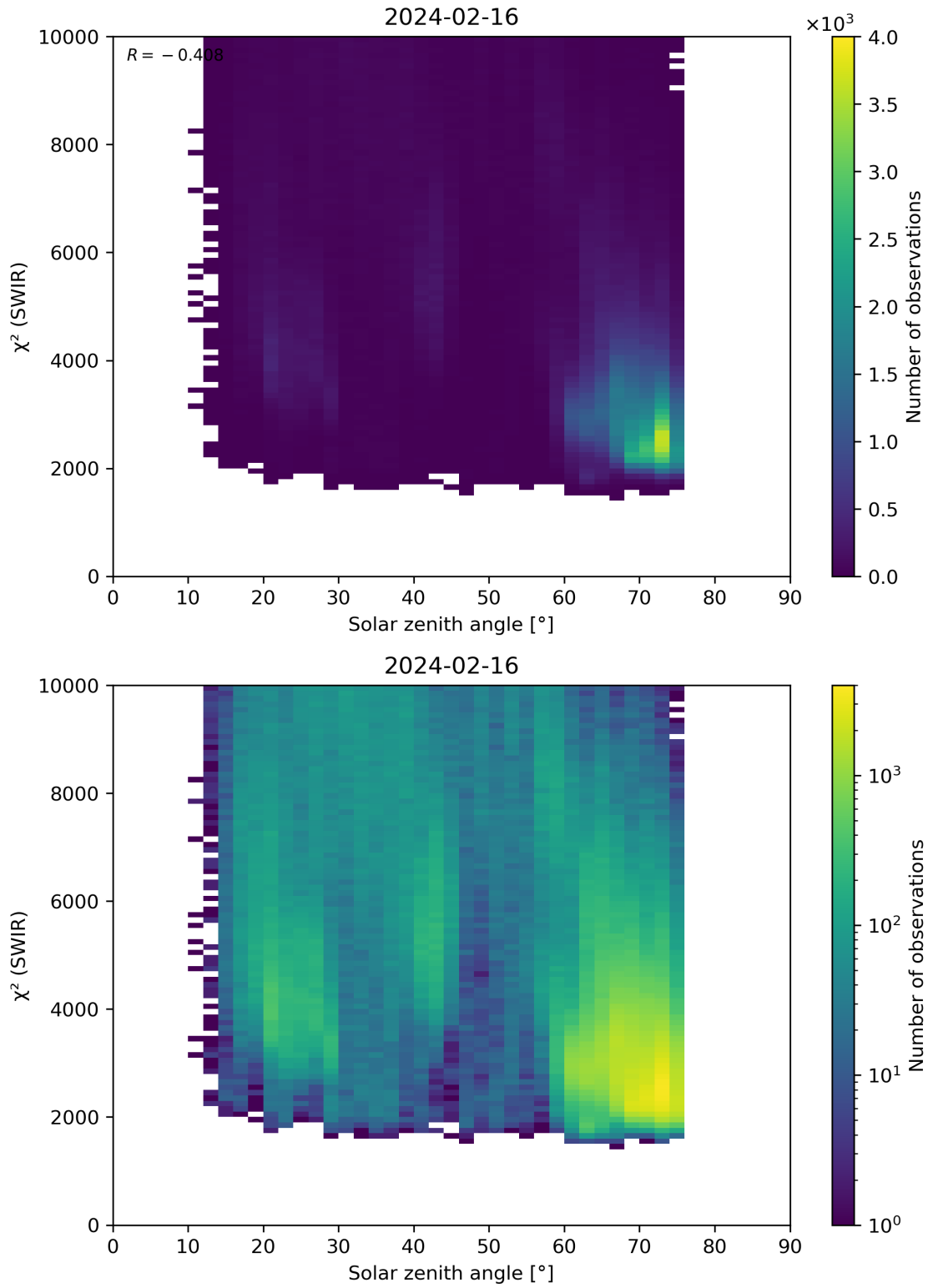
Figure 95: Scatter density plot of “Solar zenith angle” against “ \chi^2 (SWIR)” for 2024-02-16 to 2024-02-17.
