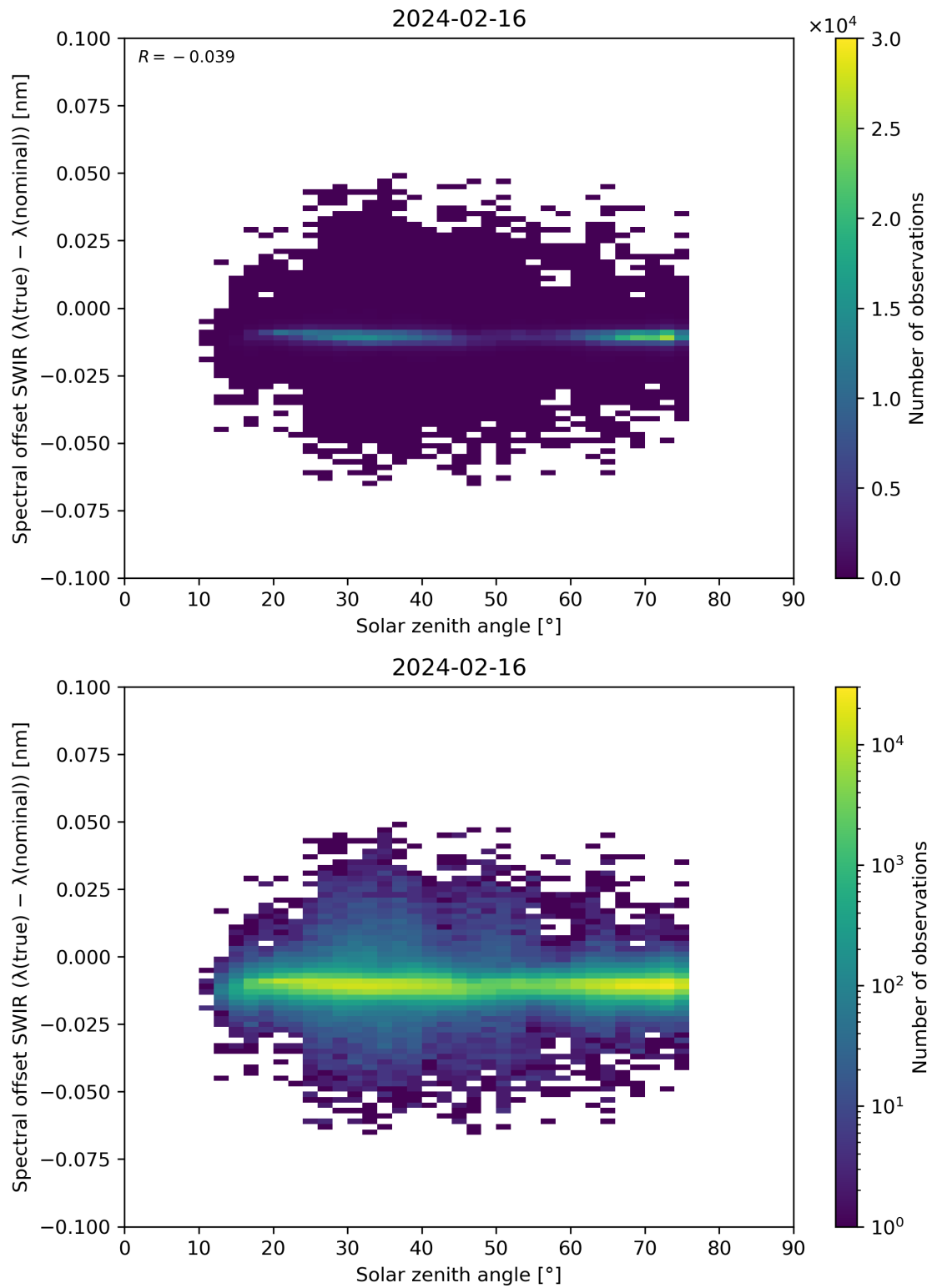
Figure 104: Scatter density plot of “Solar zenith angle” against “Spectral offset SWIR ( \lambda(\text{true}) - \lambda(\text{nominal}) )” for 2024-02-16 to 2024-02-17.
