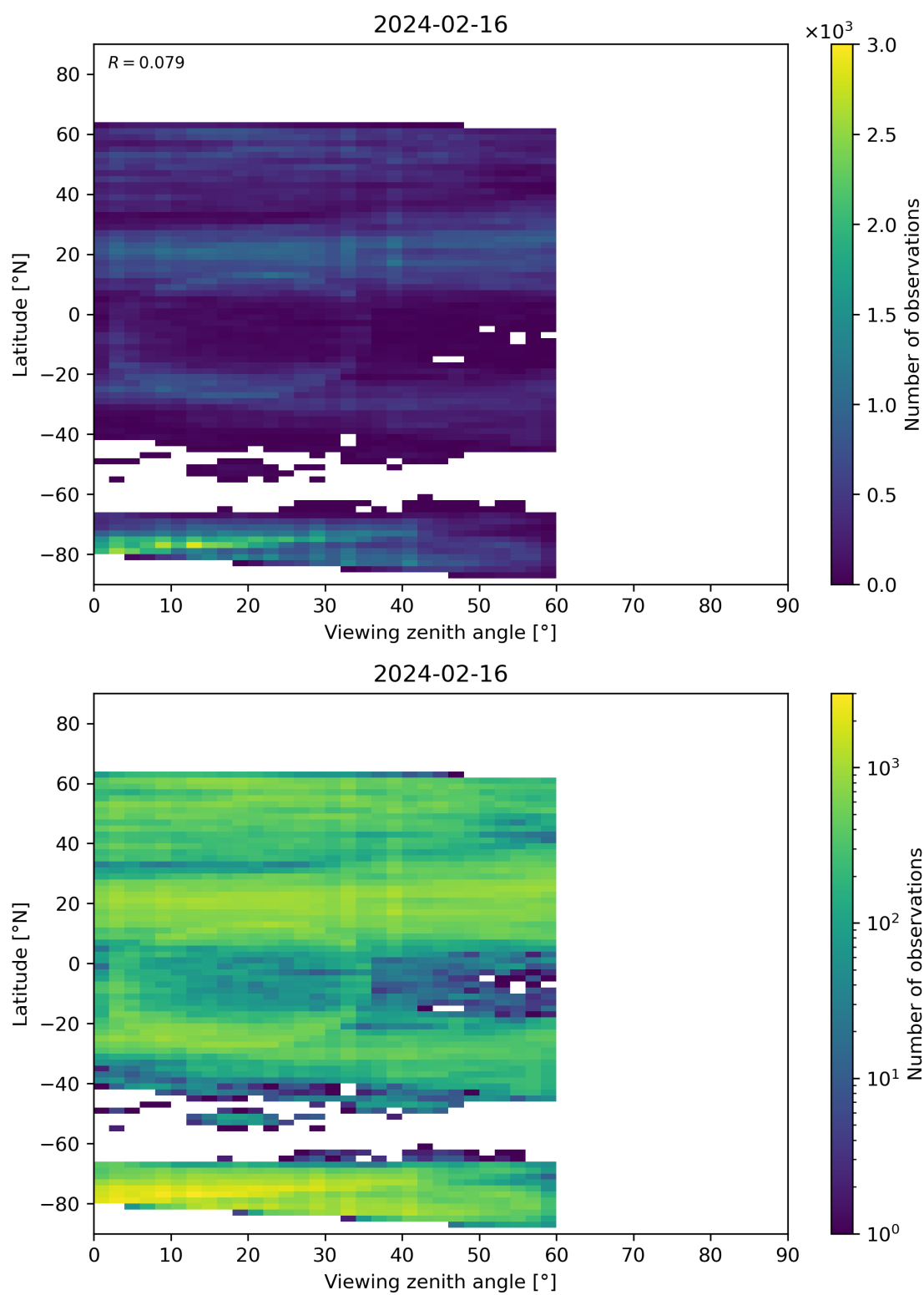
Figure 109: Scatter density plot of “Viewing zenith angle” against “Latitude” for 2024-02-16 to 2024-02-17.
