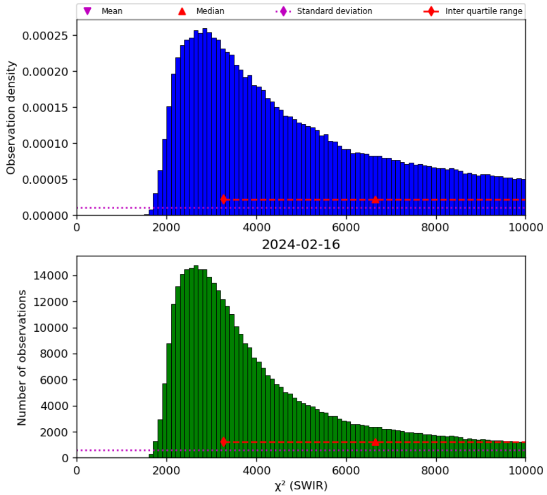
Figure 28: Histogram of “ \chi^2 (SWIR)” for 2024-02-16 to 2024-02-17
