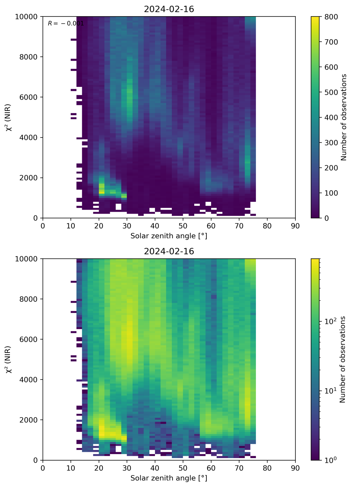
Figure 94: Scatter density plot of “Solar zenith angle” against “ \chi^2 (NIR)” for 2024-02-16 to 2024-02-17.
