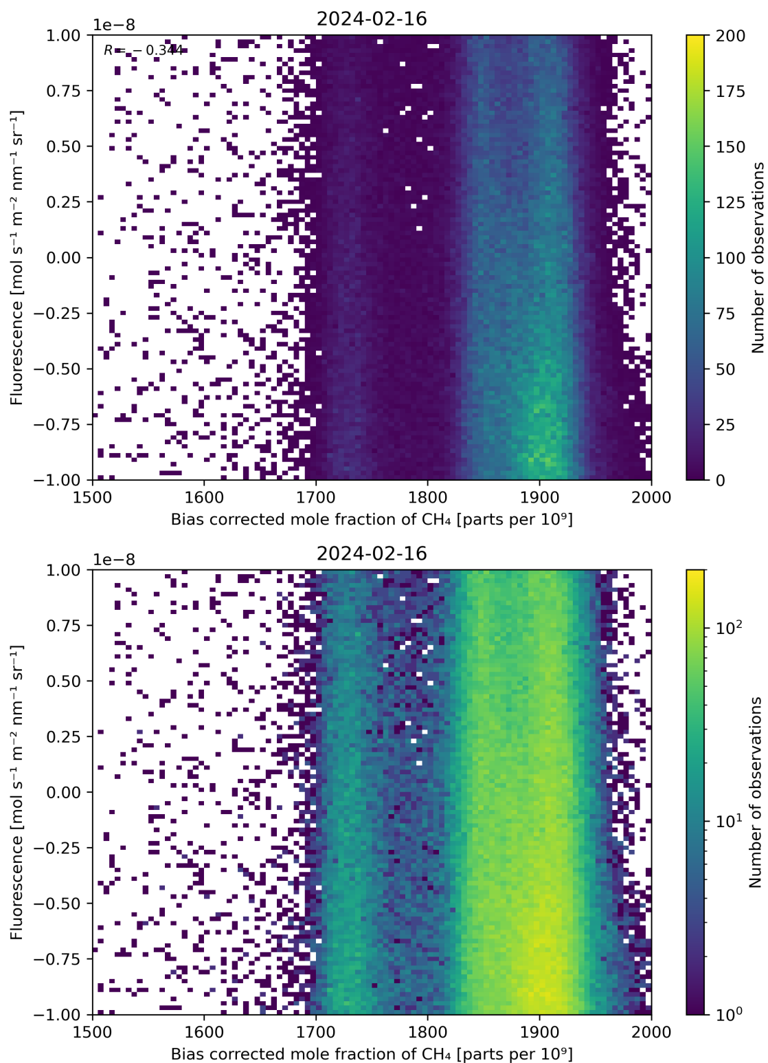
Figure 66: Scatter density plot of “Bias corrected mole fraction of CH 4 ” against “Fluorescence” for 2024-02-16 to 2024-02-17.
