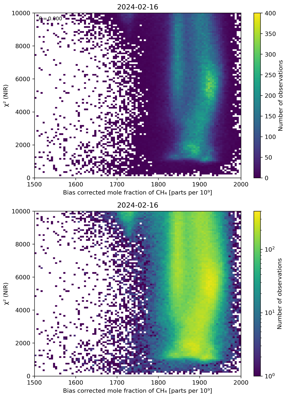
Figure 63: Scatter density plot of “Bias corrected mole fraction of CH 4 ” against “ \chi^2 (NIR)” for 2024-02-16 to 2024-02-17.
