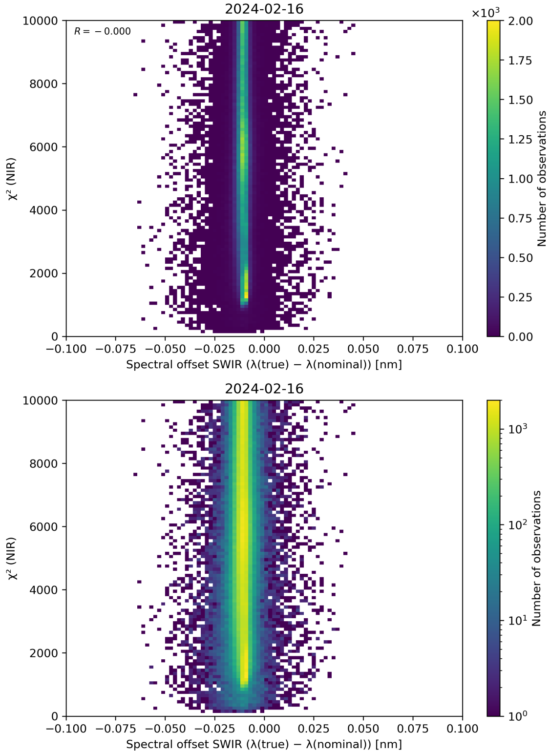
Figure 117: Scatter density plot of “Spectral offset SWIR ( \lambda(\text{true}) - \lambda(\text{nominal}) )” against “ \chi^2 (NIR)” for 2024-02-16 to 2024-02-17.
