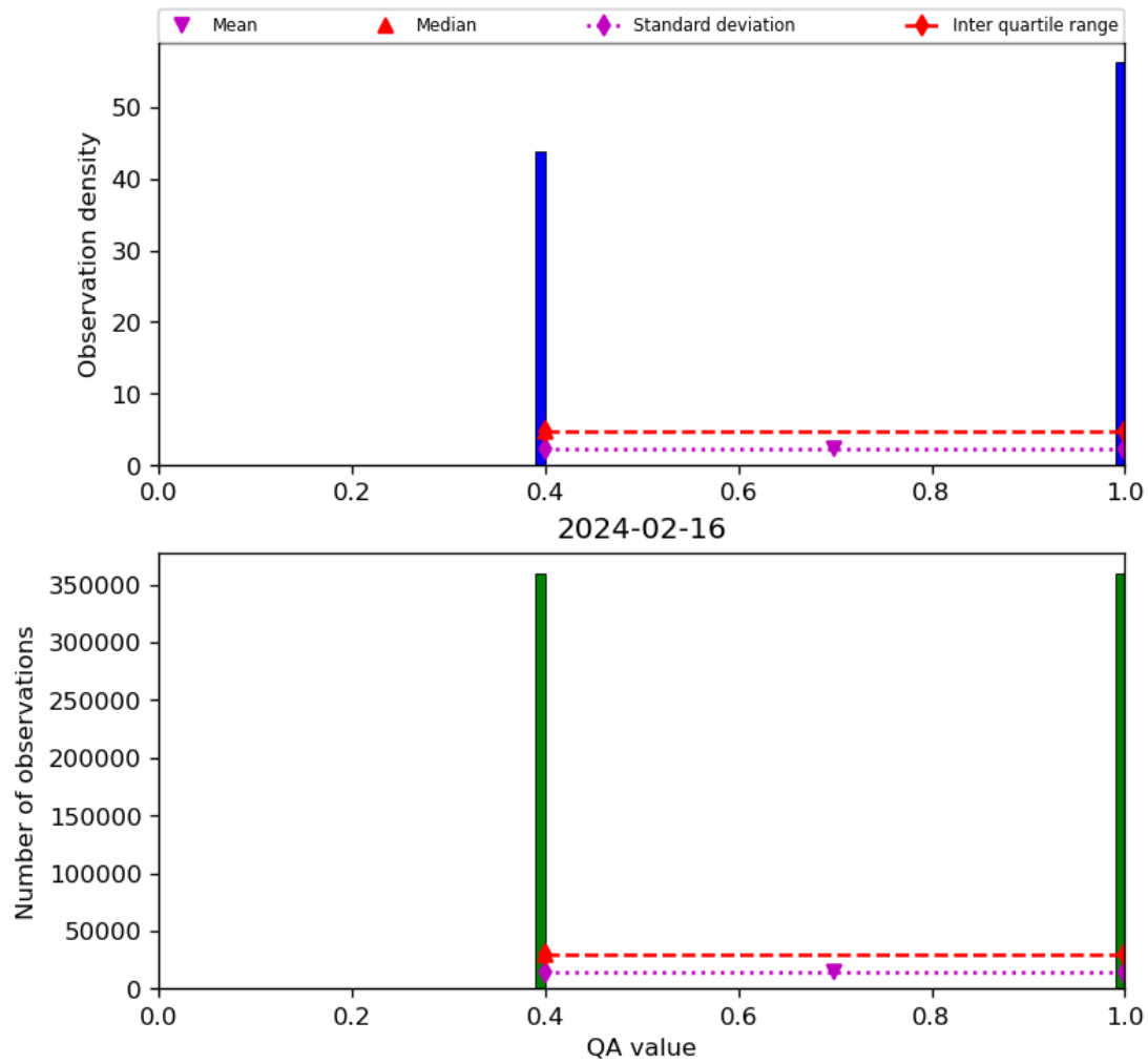
Figure 22: Histogram of “QA value” for 2024-02-16 to 2024-02-17
