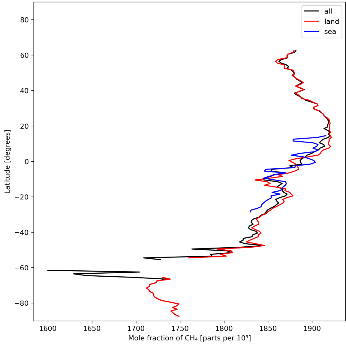
Figure 12: Zonal average of “Mole fraction of CH 4 ” for 2024-02-16 to 2024-02-17.
