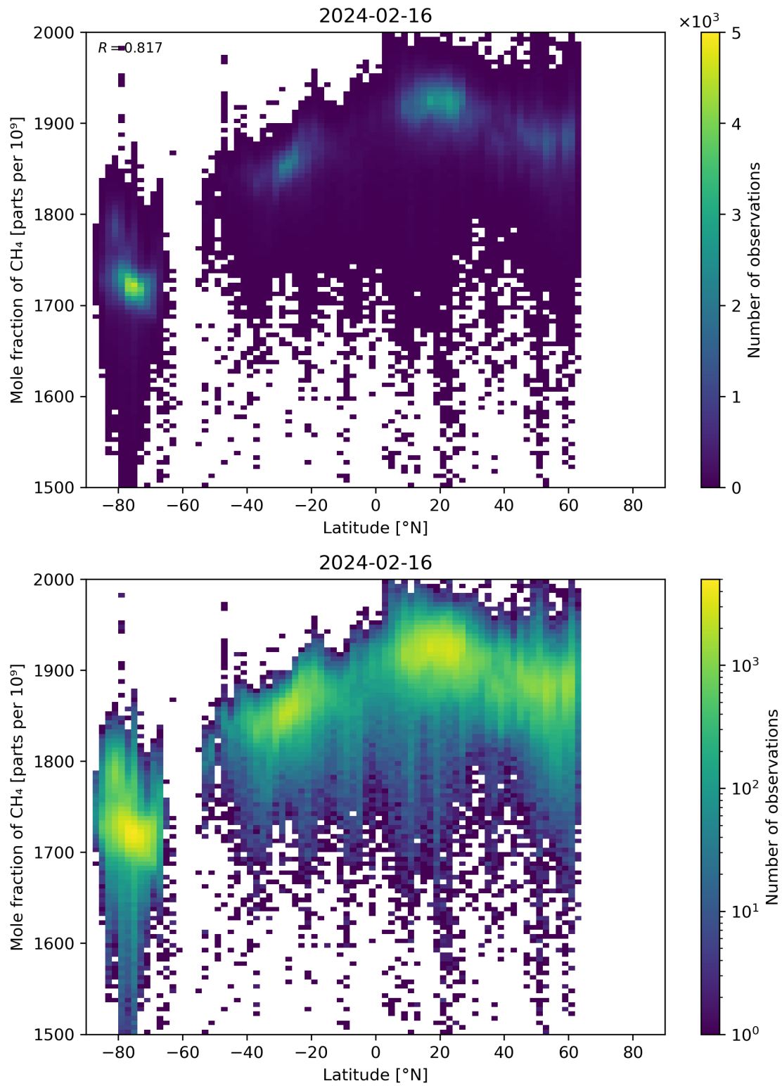
Figure 57: Scatter density plot of “Latitude” against “Mole fraction of \text{CH}_4 ” for 2024-02-16 to 2024-02-17.
