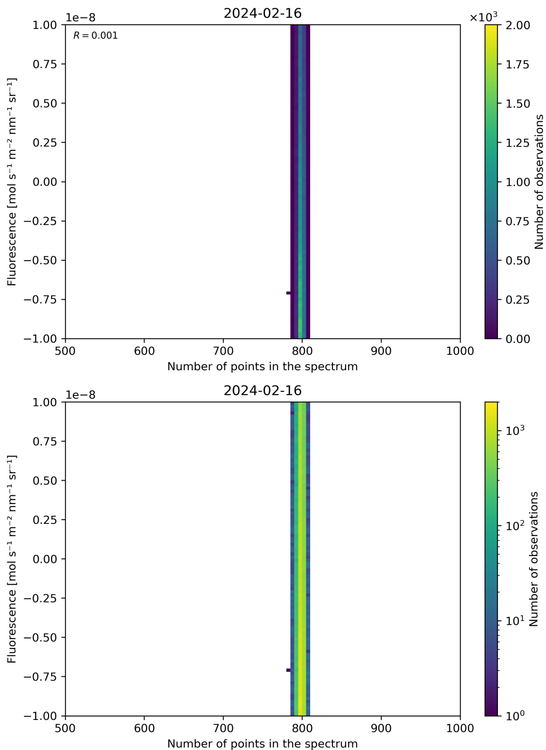
Figure 91: Scatter density plot of “Number of points in the spectrum” against “Fluorescence” for 2024-02-16 to 2024-02-17.
