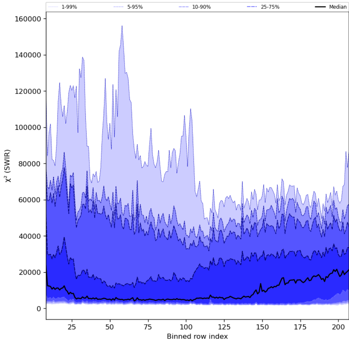
Figure 39: Along track statistics of “ \chi^2 (SWIR)” for 2024-02-16 to 2024-02-17
