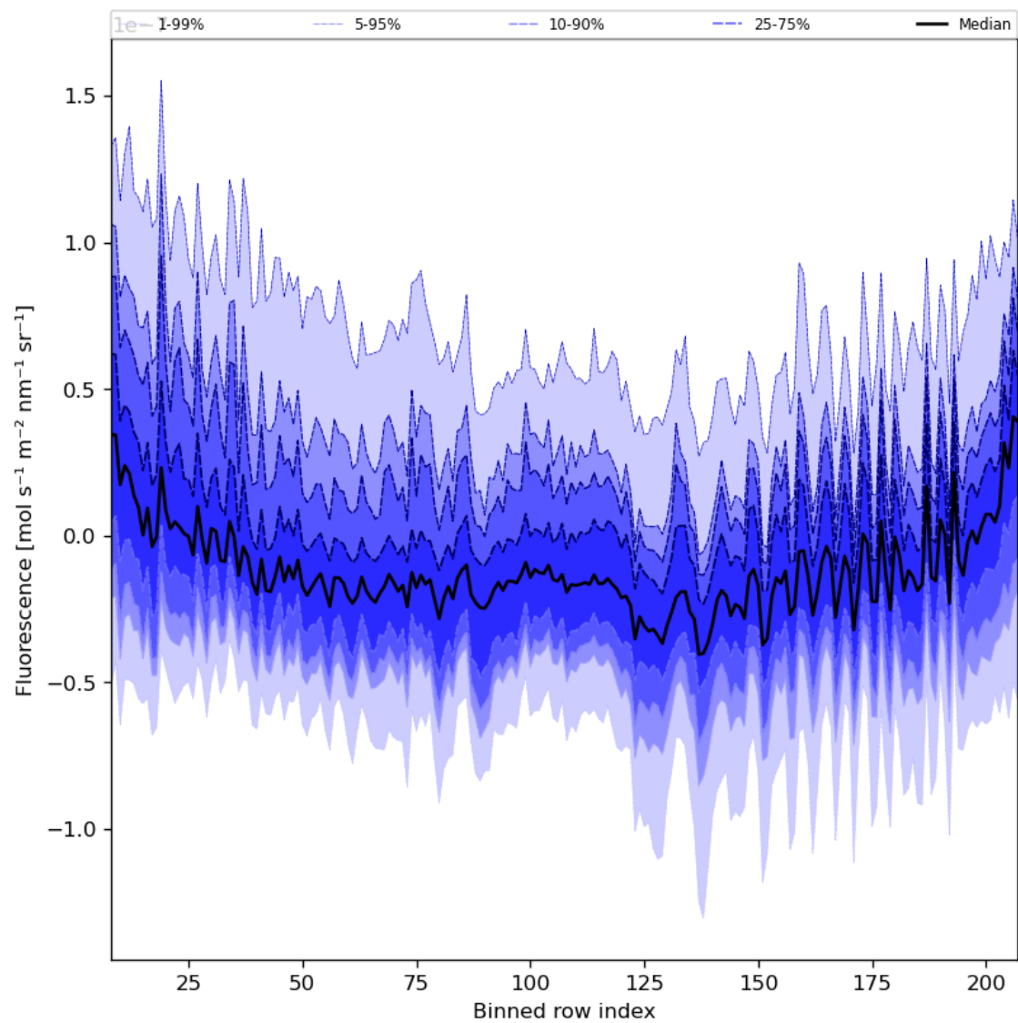
Figure 43: Along track statistics of “Fluorescence” for 2024-02-16 to 2024-02-17
