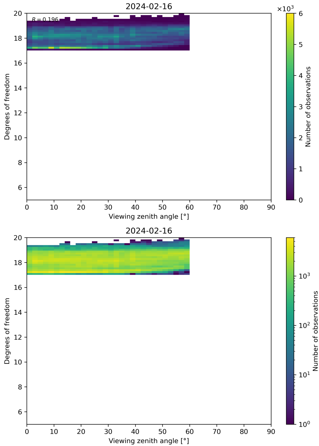
Figure 107: Scatter density plot of “Viewing zenith angle” against “Degrees of freedom” for 2024-02-16 to 2024-02-17.
