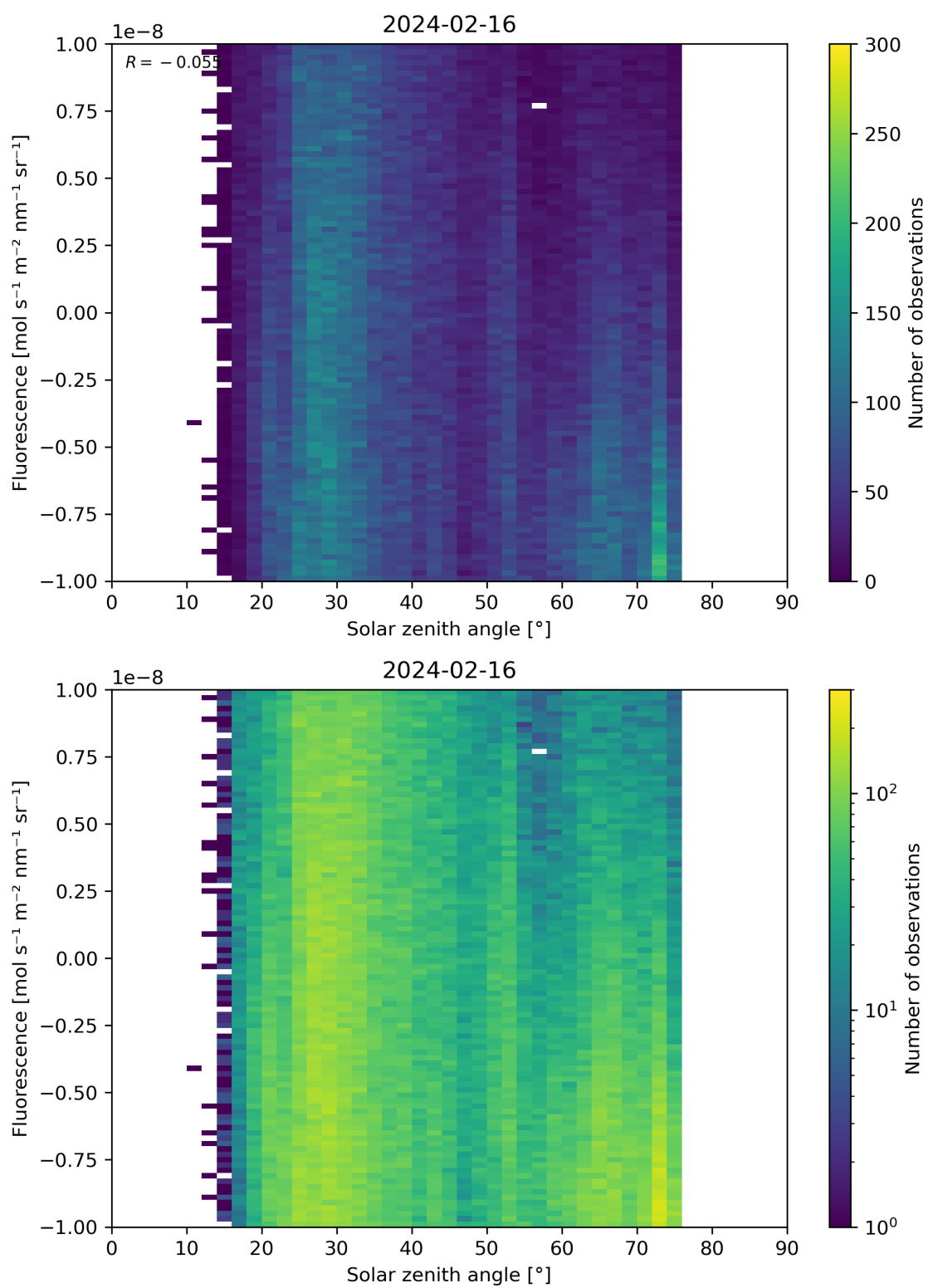
Figure 97: Scatter density plot of “Solar zenith angle” against “Fluorescence” for 2024-02-16 to 2024-02-17.
