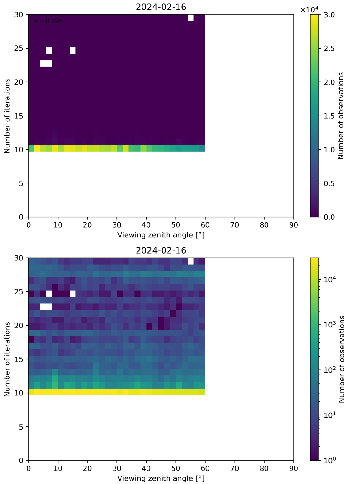
Figure 113: Scatter density plot of “Viewing zenith angle” against “Number of iterations” for 2024-02-16 to 2024-02-17.
