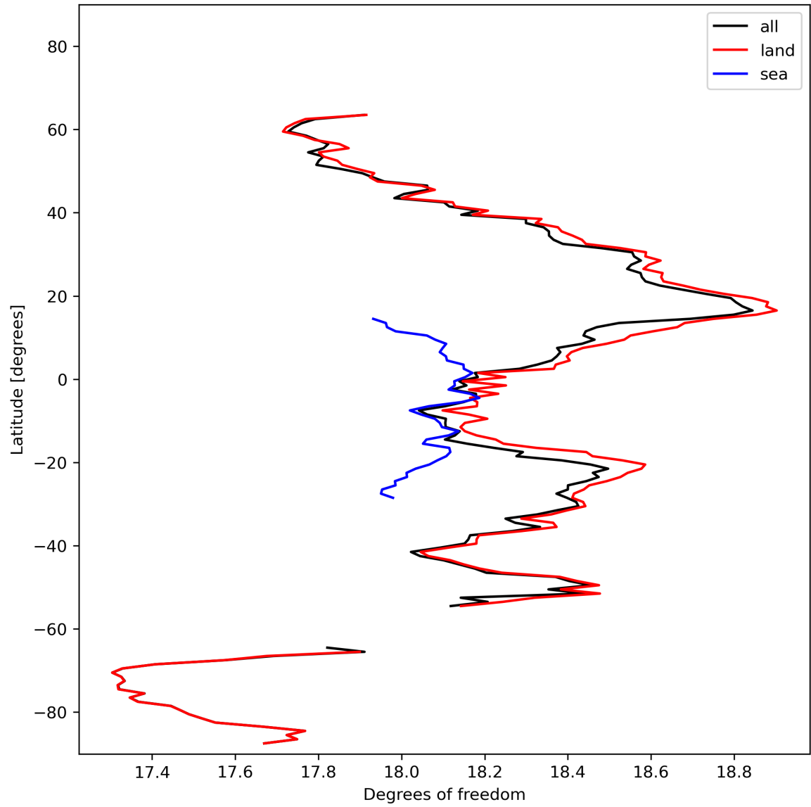
Figure 19: Zonal average of “Degrees of freedom” for 2024-02-17 to 2024-02-18.
