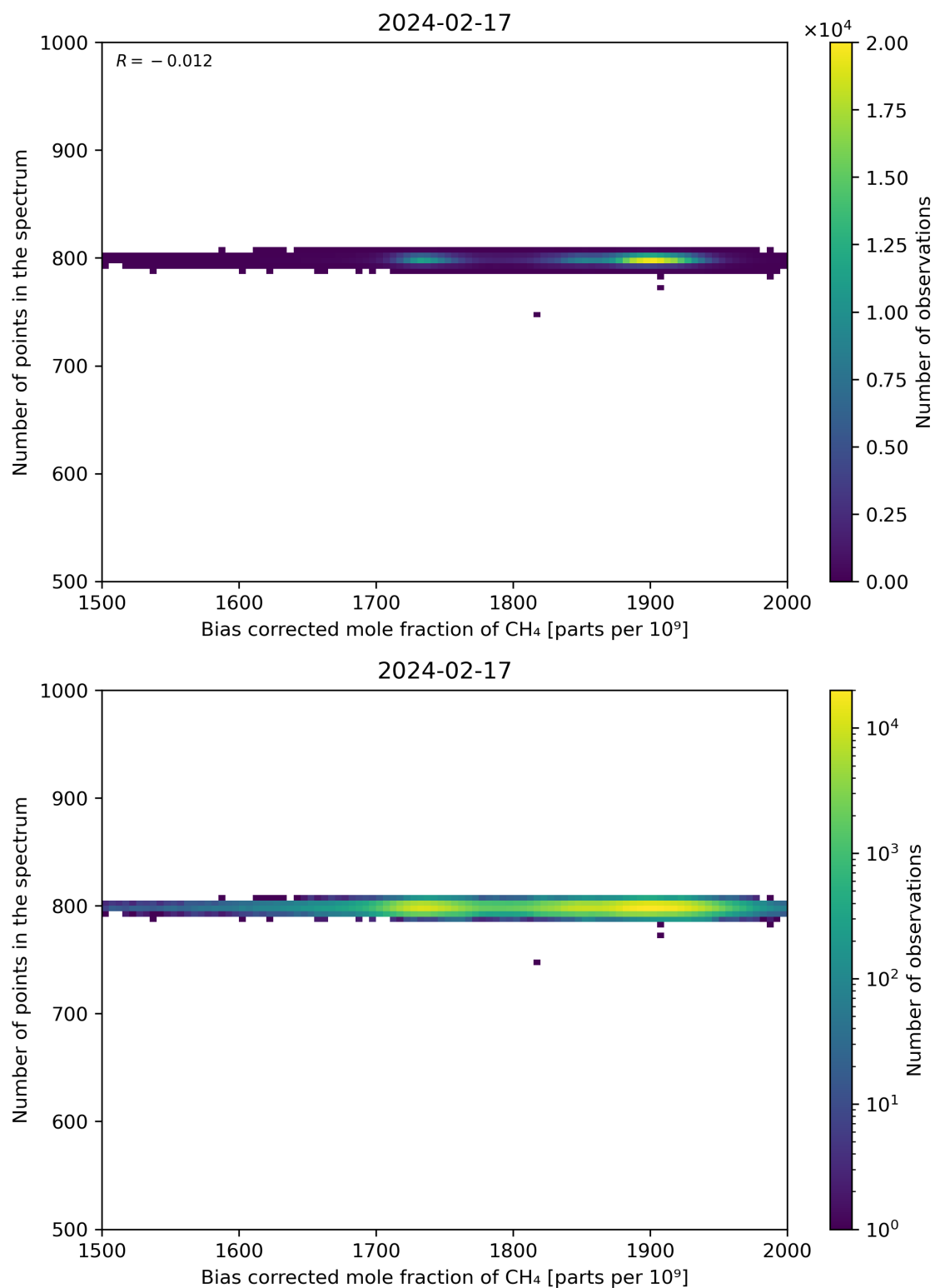
Figure 68: Scatter density plot of “Bias corrected mole fraction of CH 4 ” against “Number of points in the spectrum” for 2024-02-17 to 2024-02-18.
