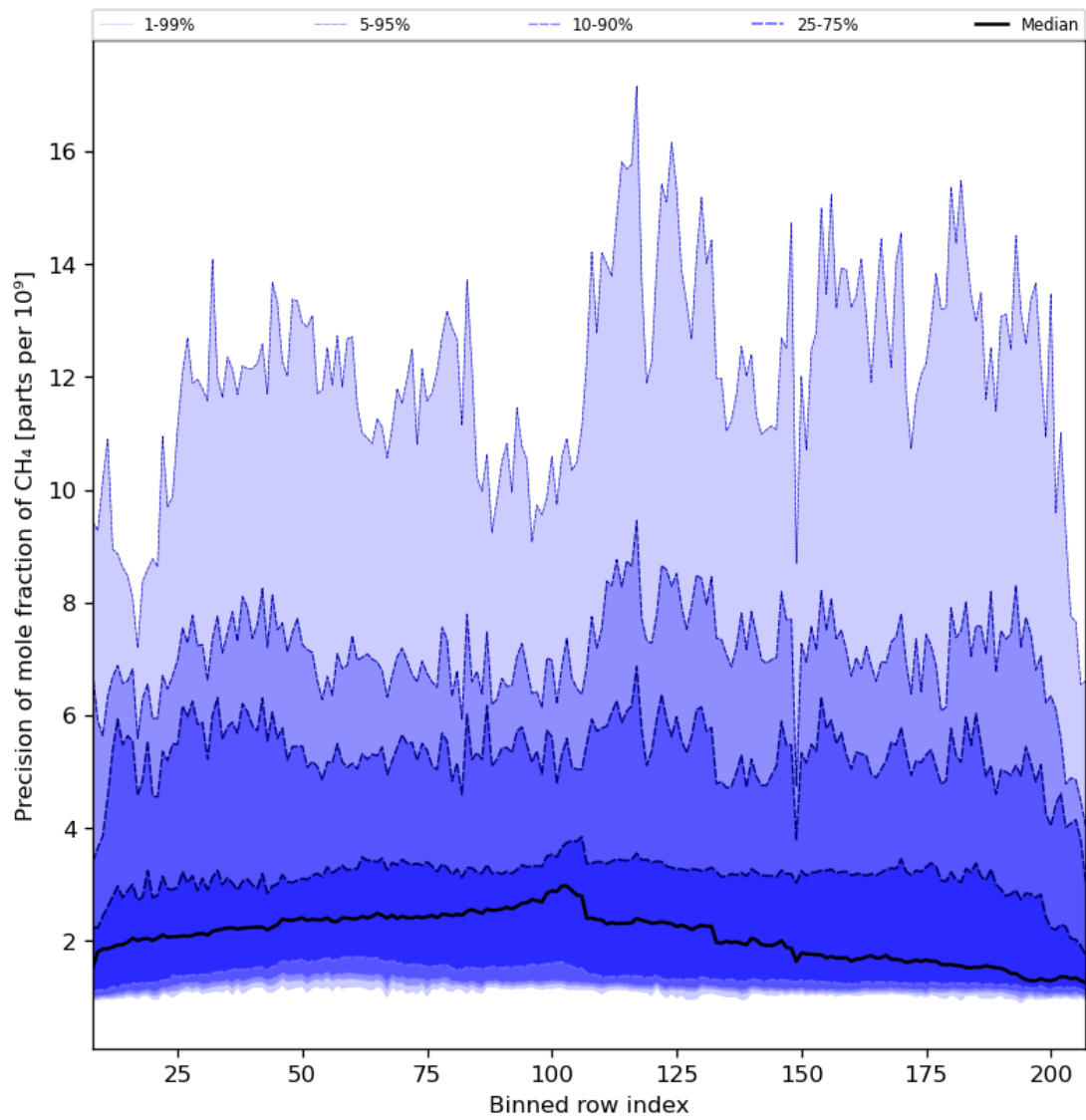
Figure 35: Along track statistics of “Precision of mole fraction of CH 4 ” for 2024-02-17 to 2024-02-18
