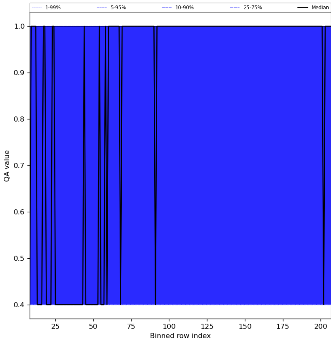
Figure 33: Along track statistics of “QA value” for 2024-02-17 to 2024-02-18
