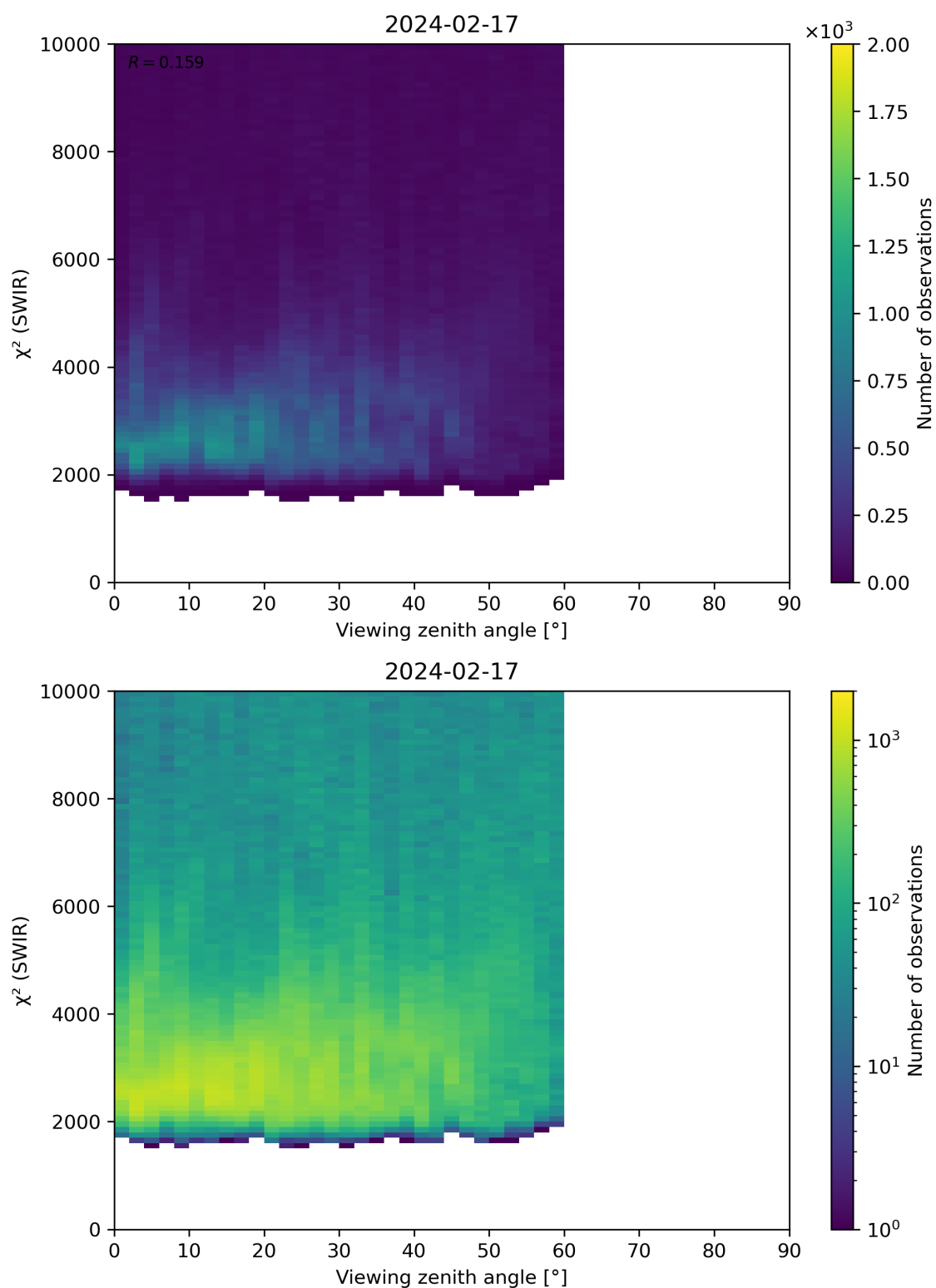
Figure 106: Scatter density plot of “Viewing zenith angle” against “ \chi^2 (SWIR)” for 2024-02-17 to 2024-02-18.
