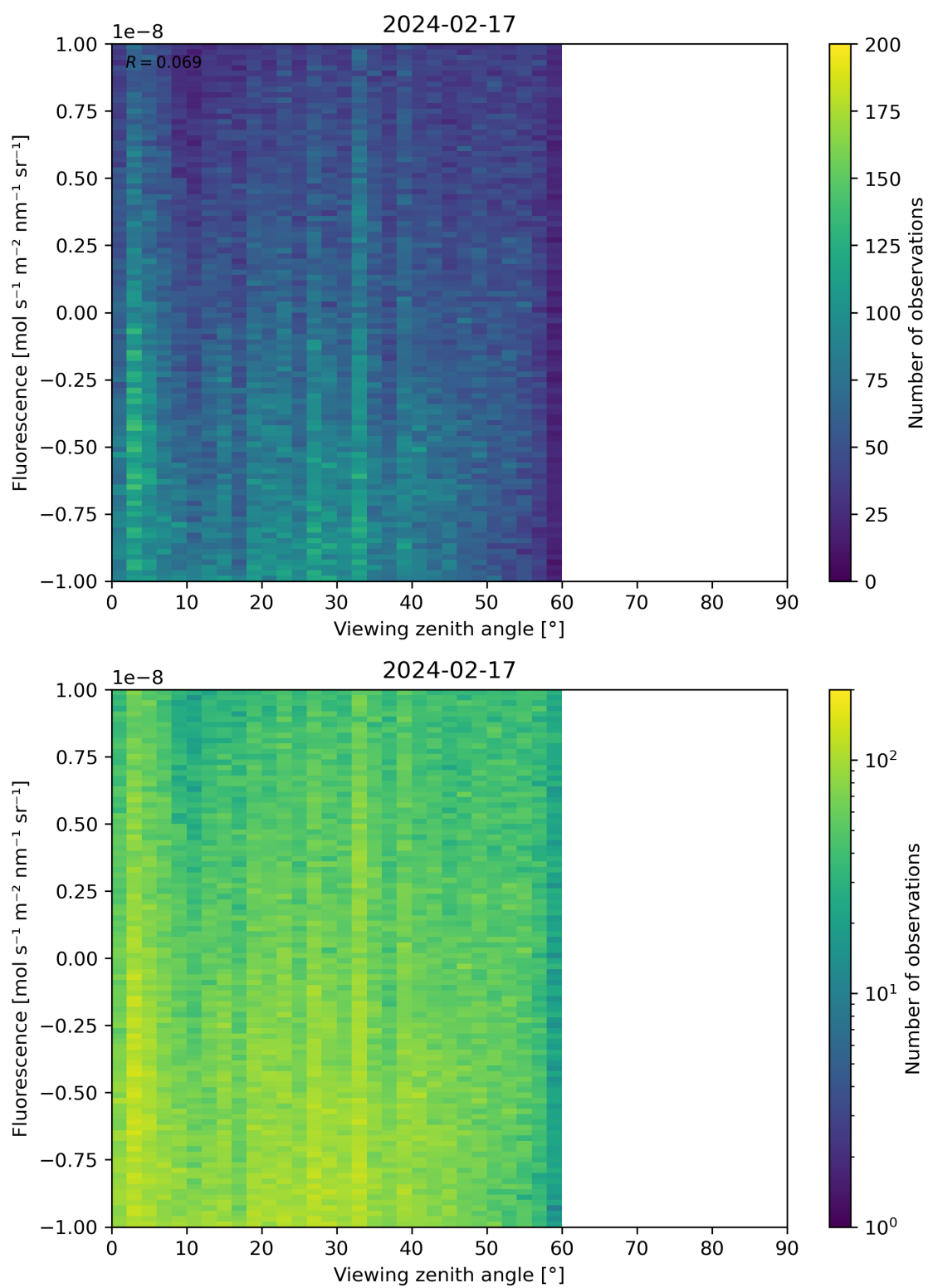
Figure 108: Scatter density plot of “Viewing zenith angle” against “Fluorescence” for 2024-02-17 to 2024-02-18.
