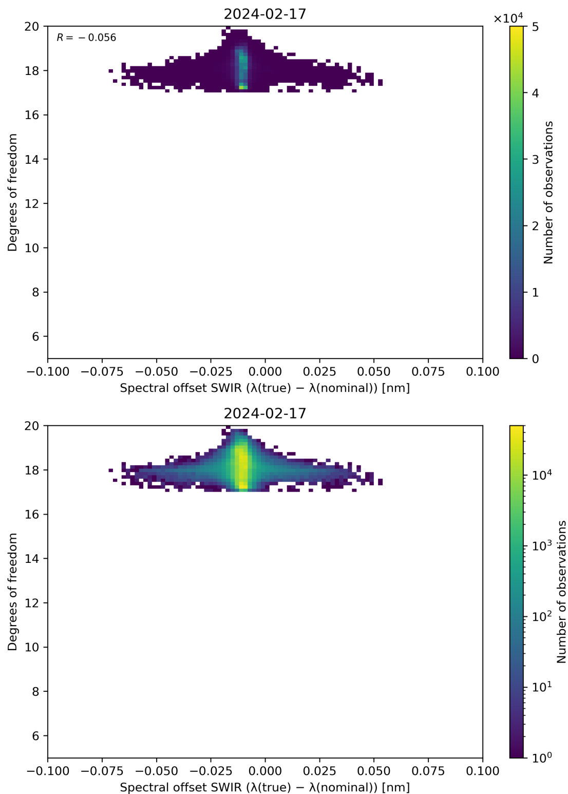
Figure 119: Scatter density plot of “Spectral offset SWIR ( \lambda(\text{true}) - \lambda(\text{nominal}) )” against “Degrees of freedom” for 2024-02-17 to 2024-02-18.
