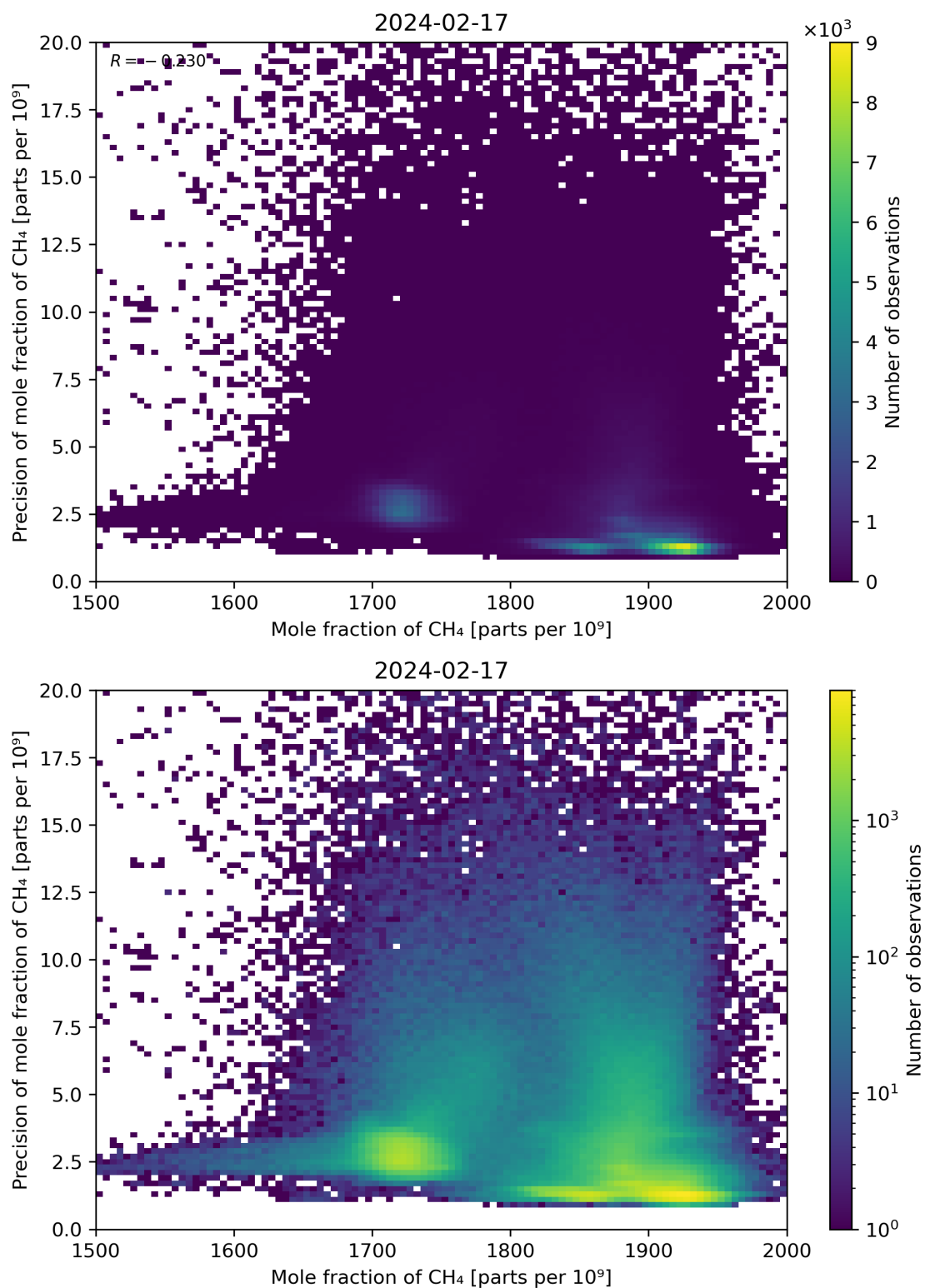
Figure 75: Scatter density plot of “Mole fraction of CH 4 ” against “Precision of mole fraction of CH 4 ” for 2024-02-17 to 2024-02-18.
