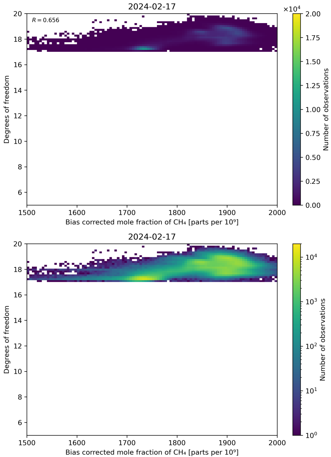
Figure 65: Scatter density plot of “Bias corrected mole fraction of CH 4 ” against “Degrees of freedom” for 2024-02-17 to 2024-02-18.
