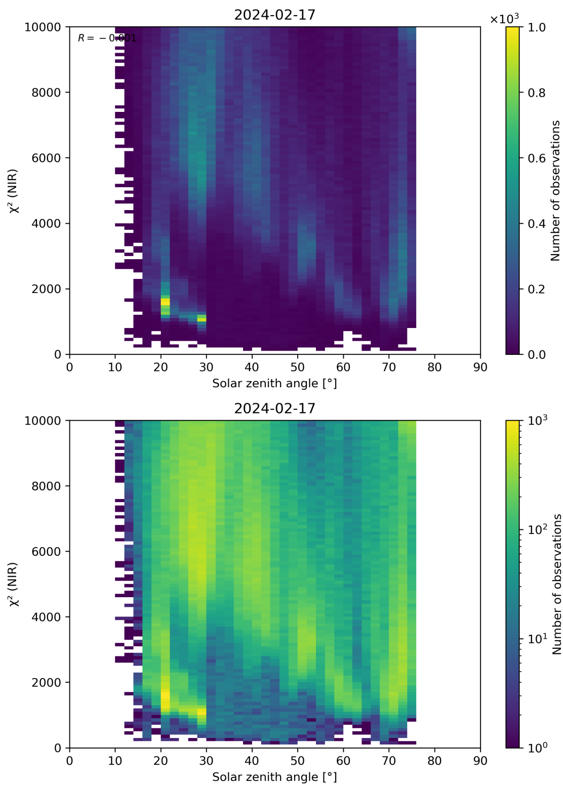
Figure 94: Scatter density plot of “Solar zenith angle” against “ \chi^2 (NIR)” for 2024-02-17 to 2024-02-18.
