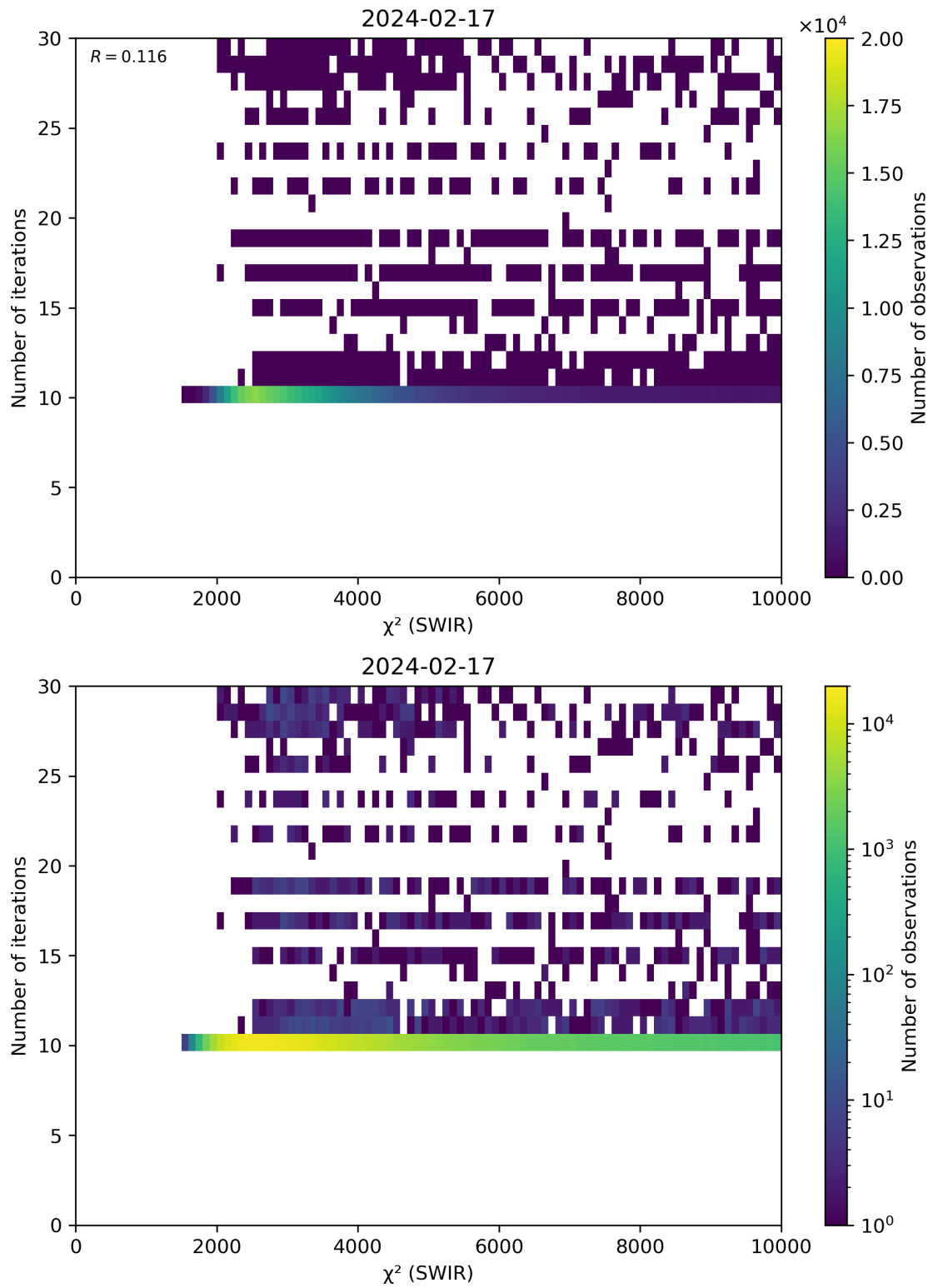
Figure 50: Scatter density plot of “ \chi^2 (SWIR)” against “Number of iterations” for 2024-02-17 to 2024-02-18.
