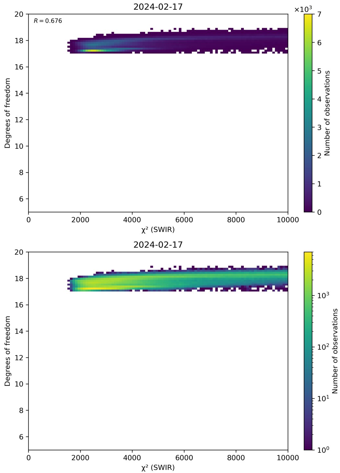
Figure 48: Scatter density plot of “ \chi^2 (SWIR)” against “Degrees of freedom” for 2024-02-17 to 2024-02-18.
