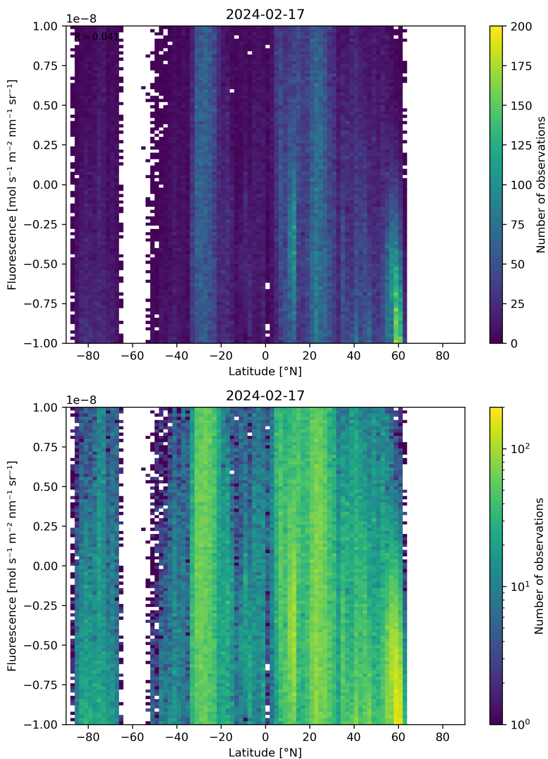
Figure 56: Scatter density plot of “Latitude” against “Fluorescence” for 2024-02-17 to 2024-02-18.
