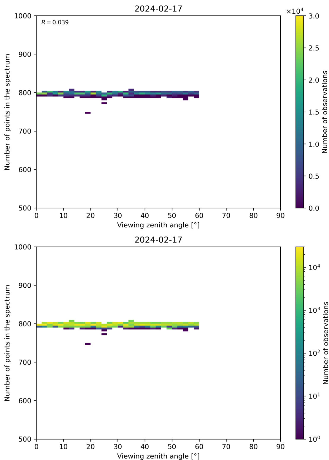
Figure 114: Scatter density plot of “Viewing zenith angle” against “Number of points in the spectrum” for 2024-02-17 to 2024-02-18.
