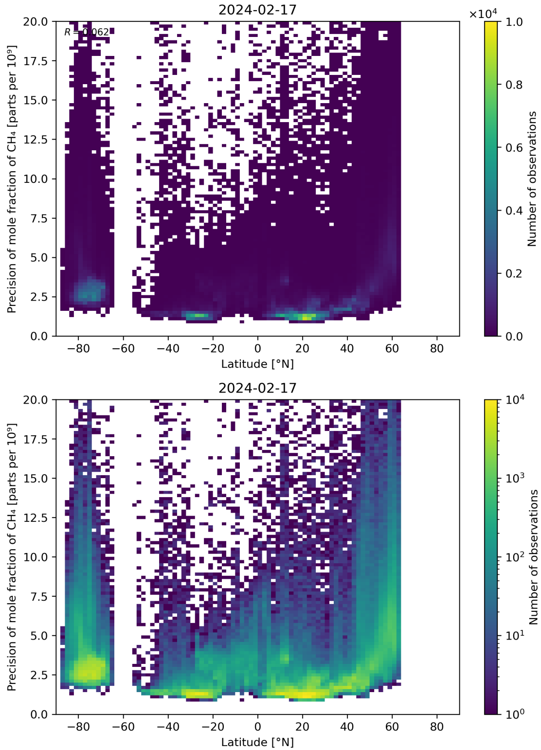
Figure 59: Scatter density plot of “Latitude” against “Precision of mole fraction of CH 4 ” for 2024-02-17 to 2024-02-18.
