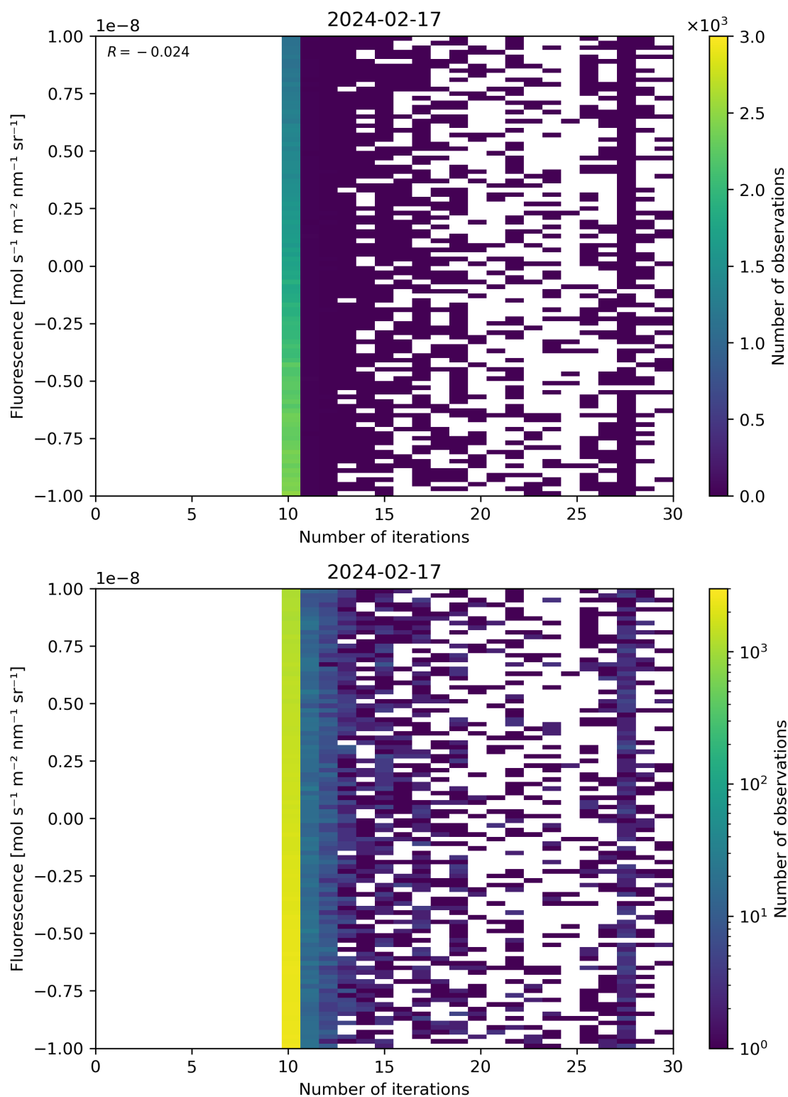
Figure 87: Scatter density plot of “Number of iterations” against “Fluorescence” for 2024-02-17 to 2024-02-18.
