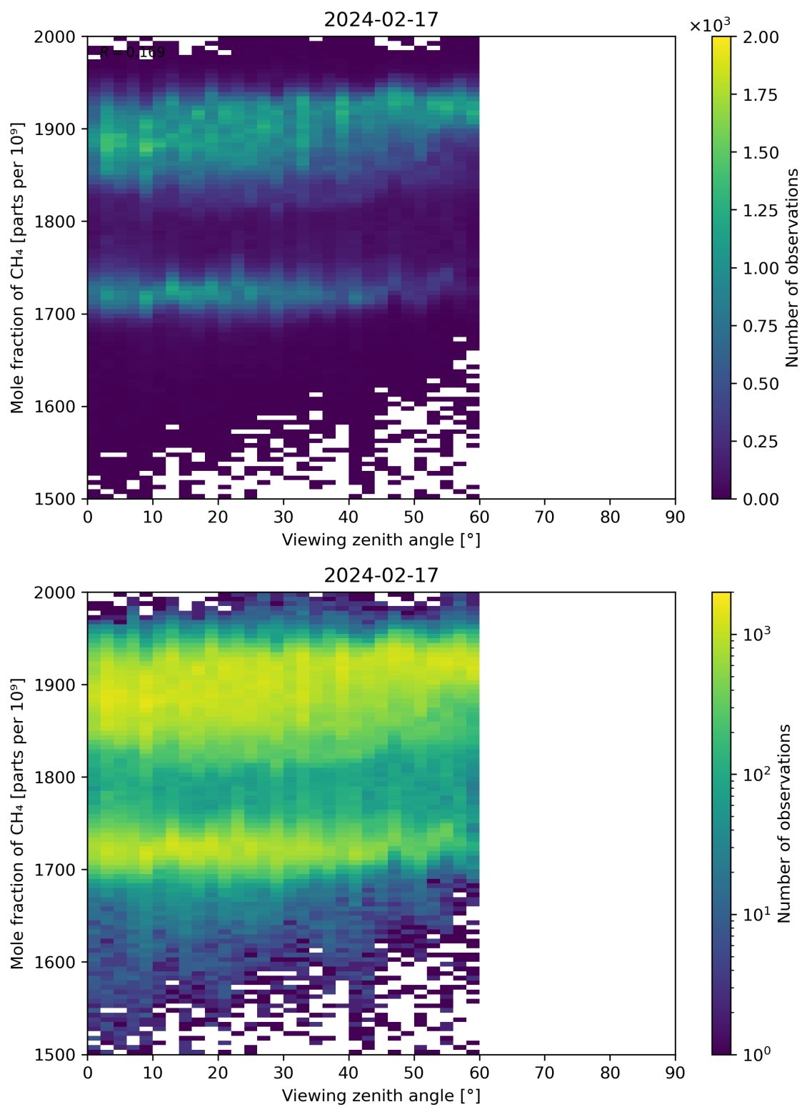
Figure 110: Scatter density plot of “Viewing zenith angle” against “Mole fraction of CH 4 ” for 2024-02-17 to 2024-02-18.
