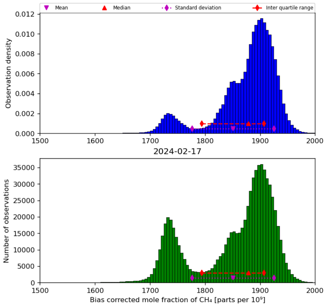
Figure 25: Histogram of “Bias corrected mole fraction of CH 4 ” for 2024-02-17 to 2024-02-18
