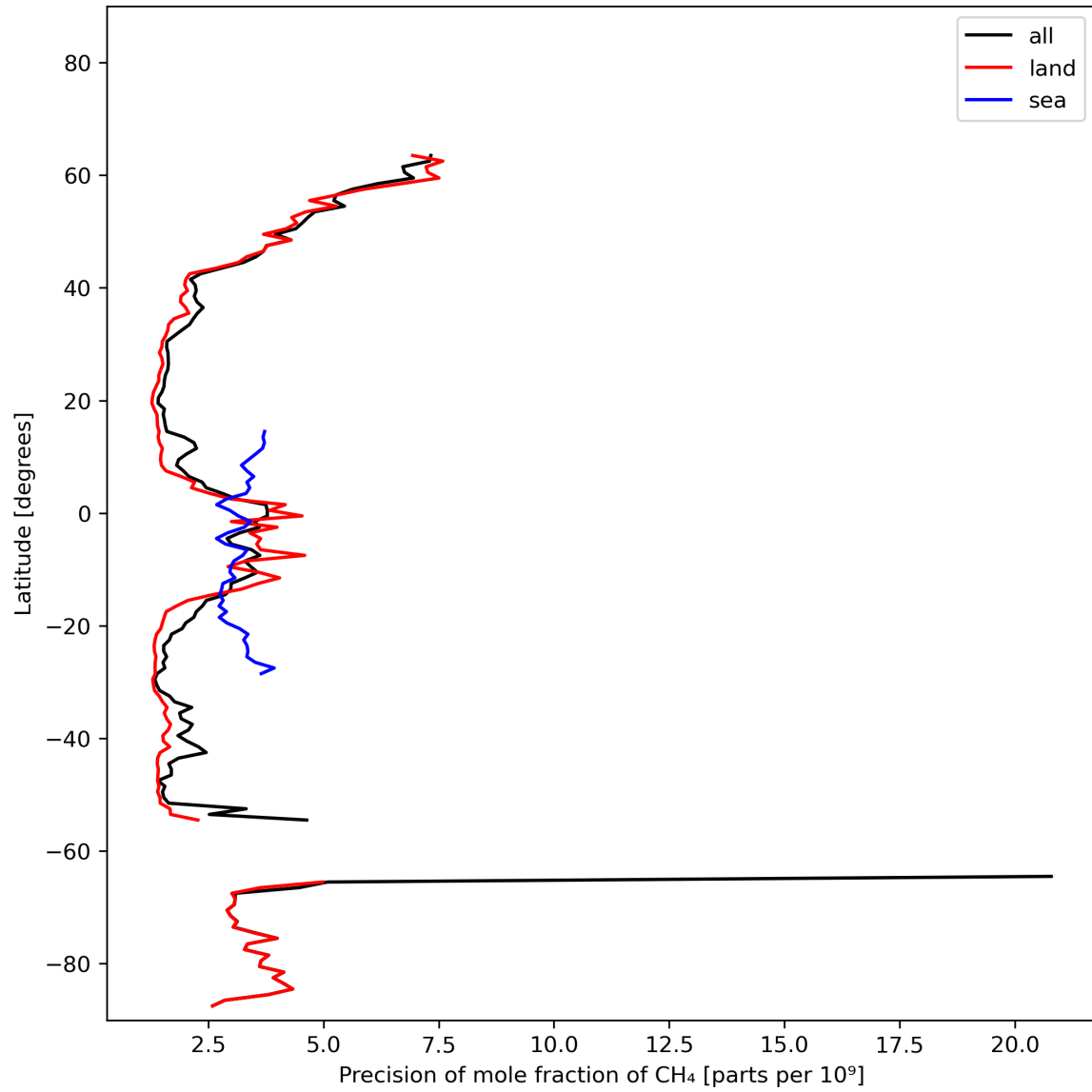
Figure 13: Zonal average of “Precision of mole fraction of \text{CH}_4 ” for 2024-02-17 to 2024-02-18.
