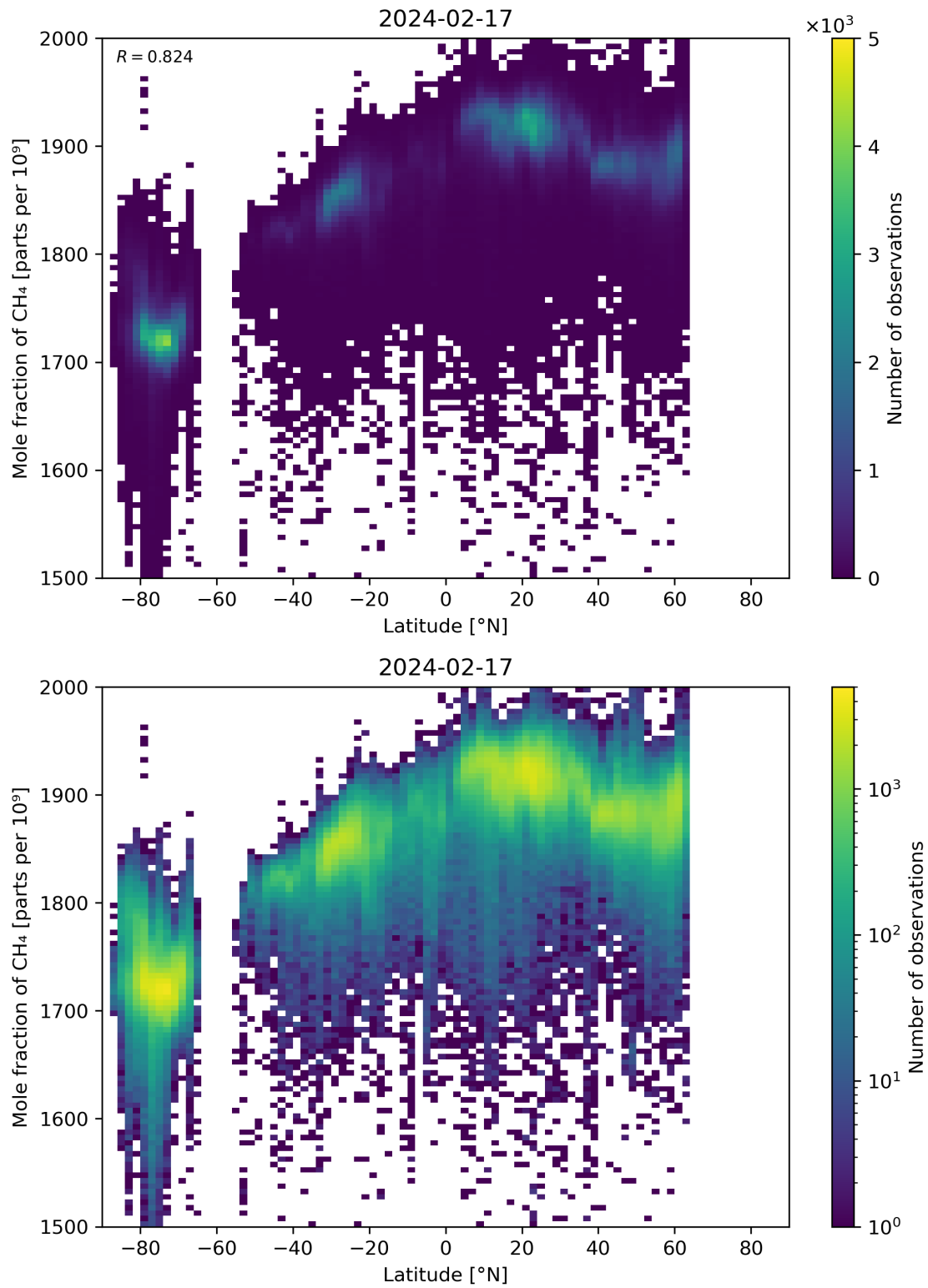
Figure 57: Scatter density plot of “Latitude” against “Mole fraction of \text{CH}_4 ” for 2024-02-17 to 2024-02-18.
