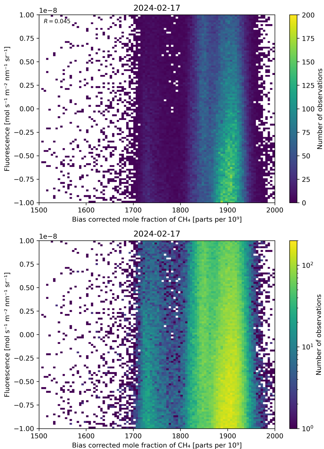
Figure 66: Scatter density plot of “Bias corrected mole fraction of \text{CH}_4 ” against “Fluorescence” for 2024-02-17 to 2024-02-18.
