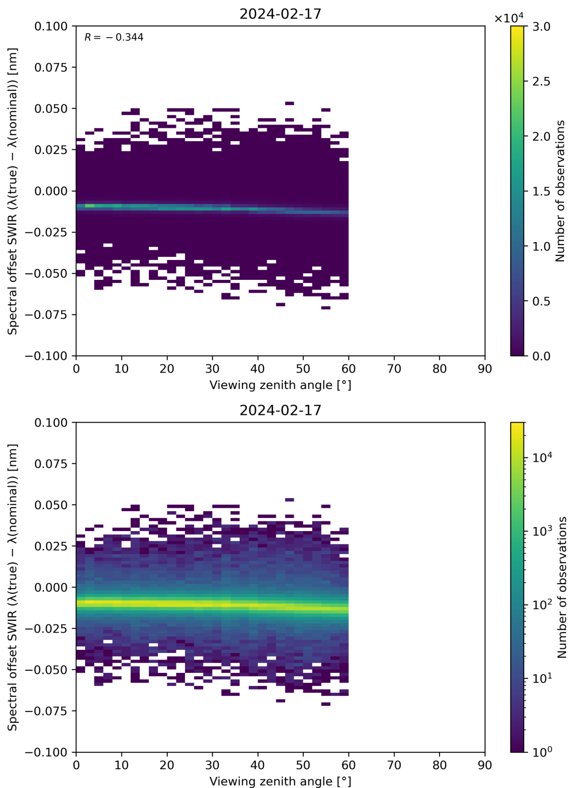
Figure 116: Scatter density plot of “Viewing zenith angle” against “Spectral offset SWIR ( \lambda(\text{true}) - \lambda(\text{nominal}) )” for 2024-02-17 to 2024-02-18.
