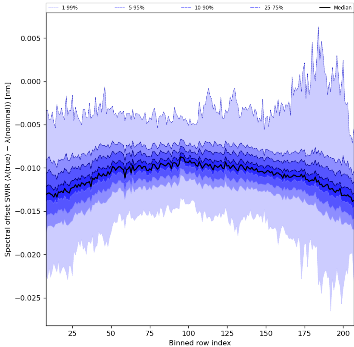
Figure 38: Along track statistics of “Spectral offset SWIR ( \lambda(\text{true}) - \lambda(\text{nominal}) )” for 2024-02-17 to 2024-02-18
