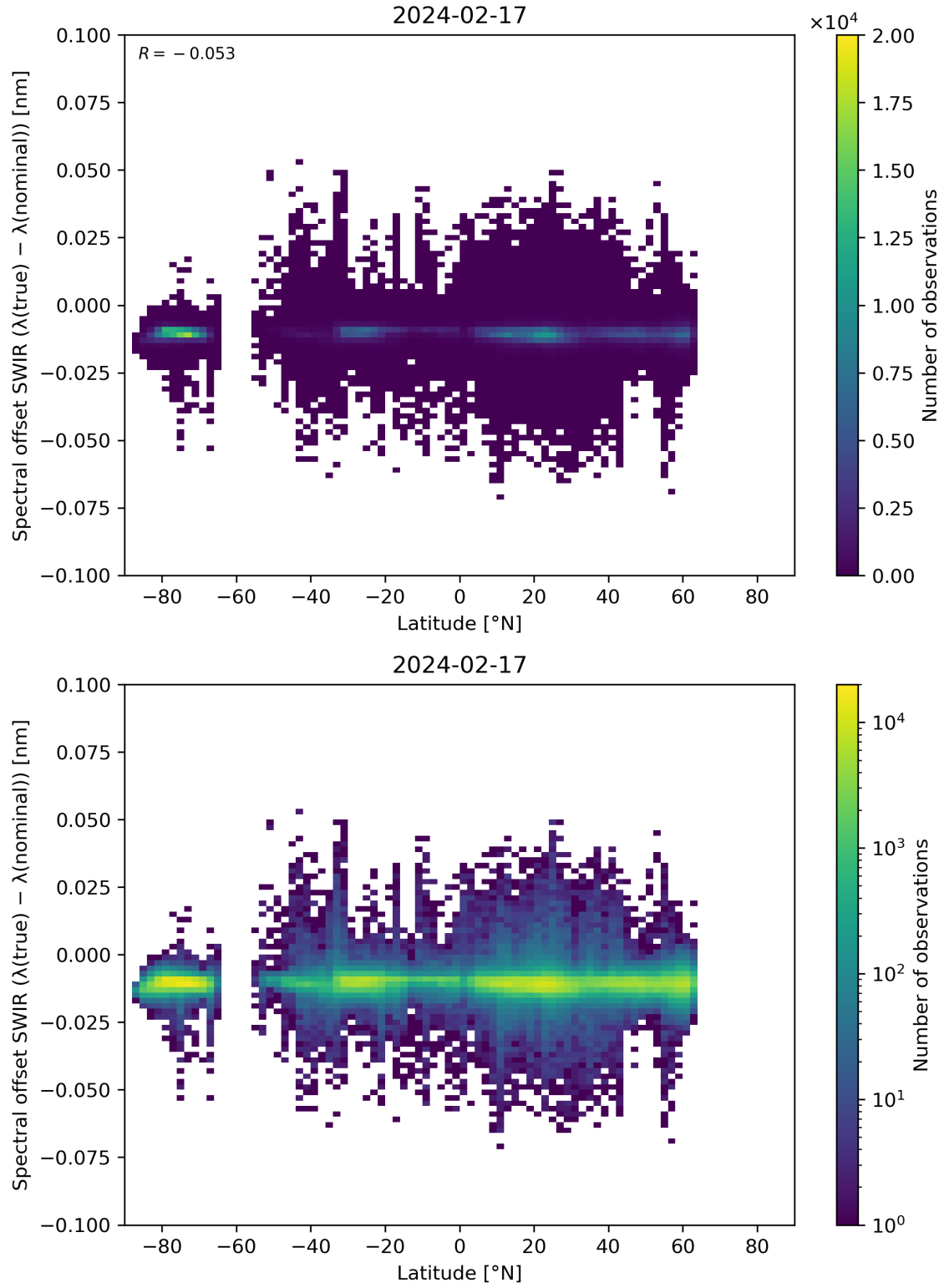
Figure 62: Scatter density plot of “Latitude” against “Spectral offset SWIR ( \lambda(\text{true}) - \lambda(\text{nominal}) )” for 2024-02-17 to 2024-02-18.
