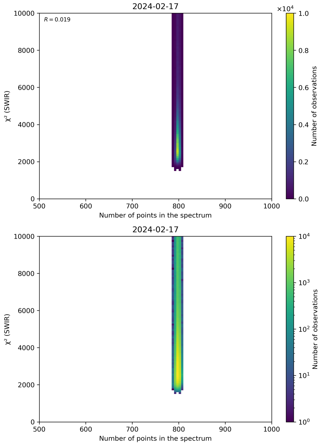
Figure 89: Scatter density plot of “Number of points in the spectrum” against “ \chi^2 (SWIR)” for 2024-02-17 to 2024-02-18.
