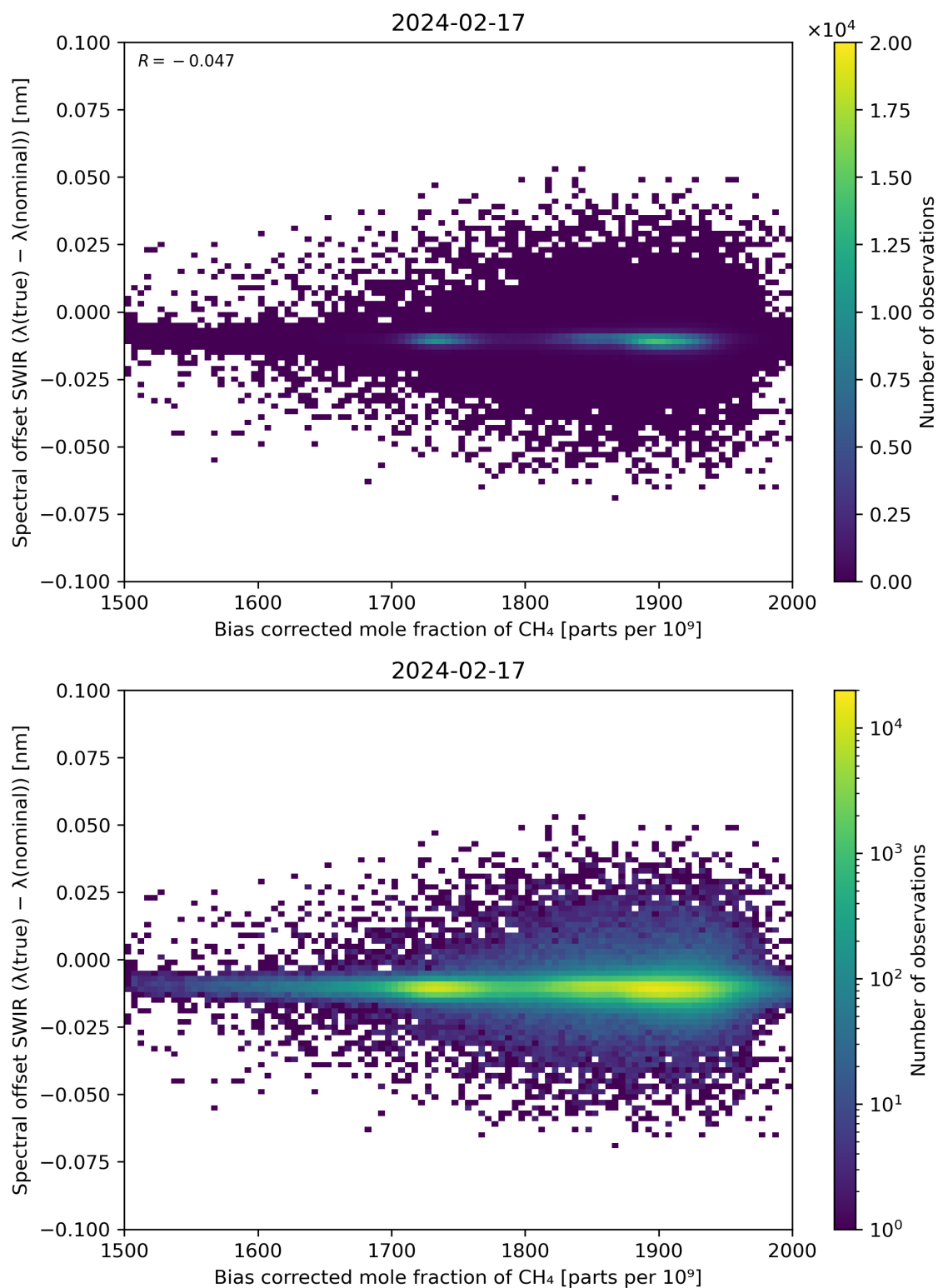
Figure 69: Scatter density plot of “Bias corrected mole fraction of \text{CH}_4 ” against “Spectral offset SWIR ( \lambda(\text{true}) - \lambda(\text{nominal}) )” for 2024-02-17 to 2024-02-18.
