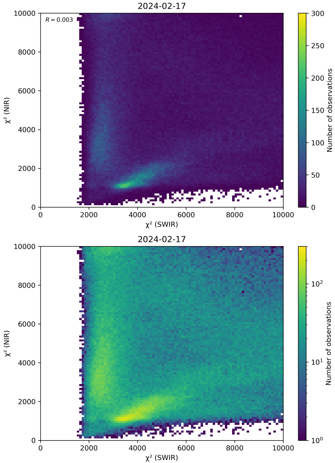
Figure 47: Scatter density plot of “ \chi^2 (SWIR)” against “ \chi^2 (NIR)” for 2024-02-17 to 2024-02-18.
