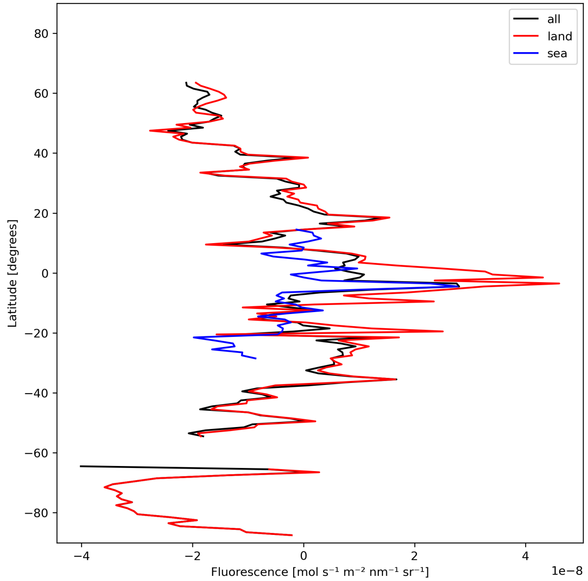
Figure 21: Zonal average of “Fluorescence” for 2024-02-17 to 2024-02-18.
