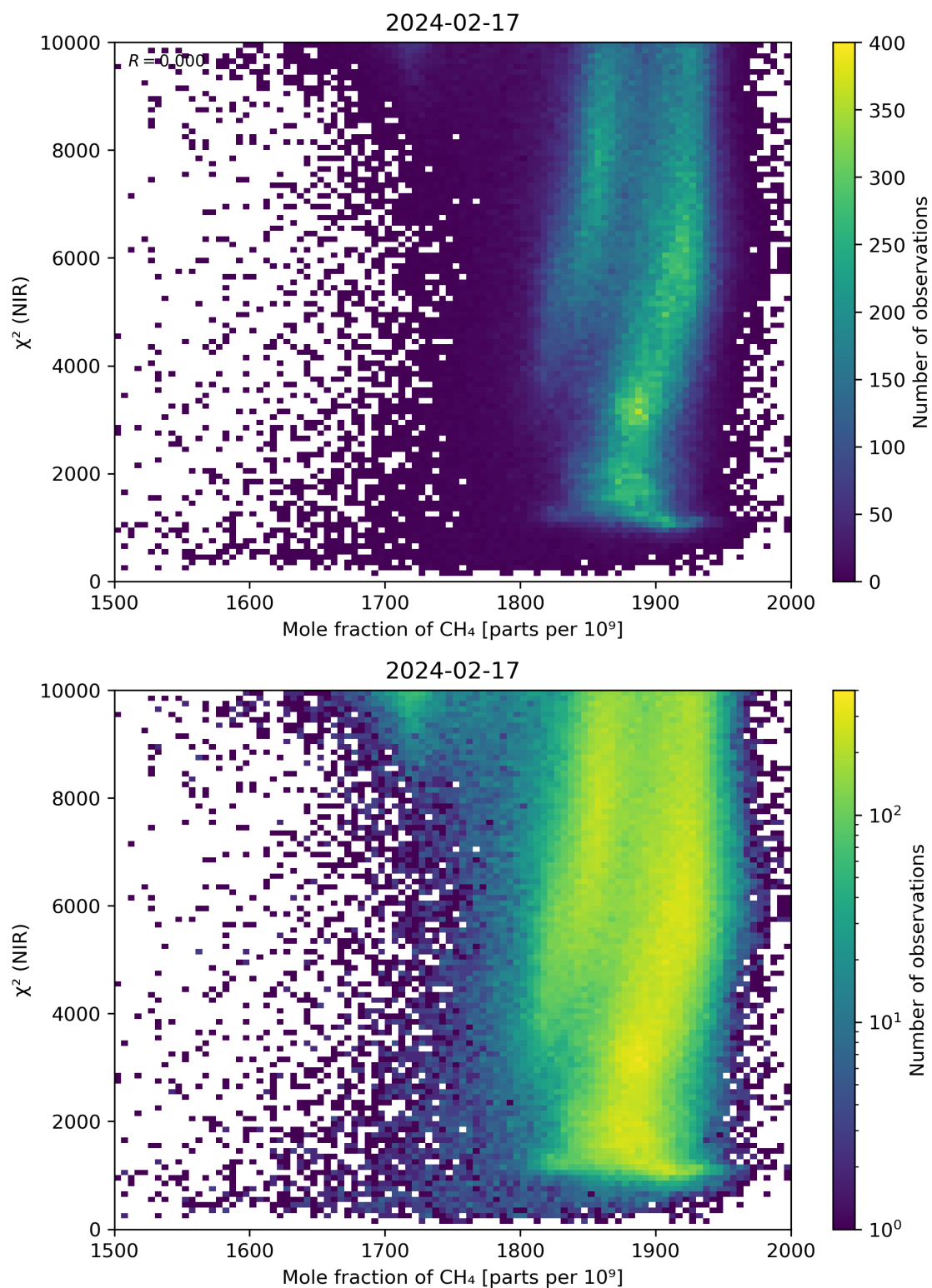
Figure 70: Scatter density plot of “Mole fraction of \text{CH}_4 ” against “ \chi^2 (NIR)” for 2024-02-17 to 2024-02-18.
