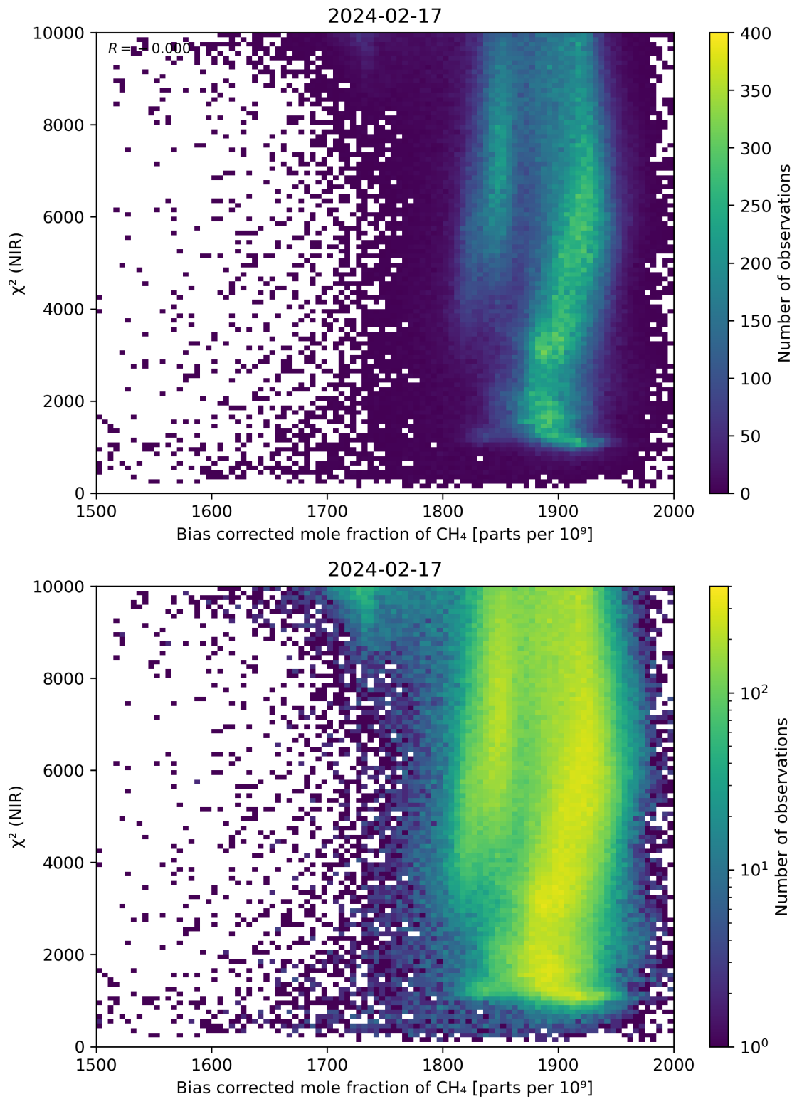
Figure 63: Scatter density plot of “Bias corrected mole fraction of \text{CH}_4 ” against “ \chi^2 (NIR)” for 2024-02-17 to 2024-02-18.
