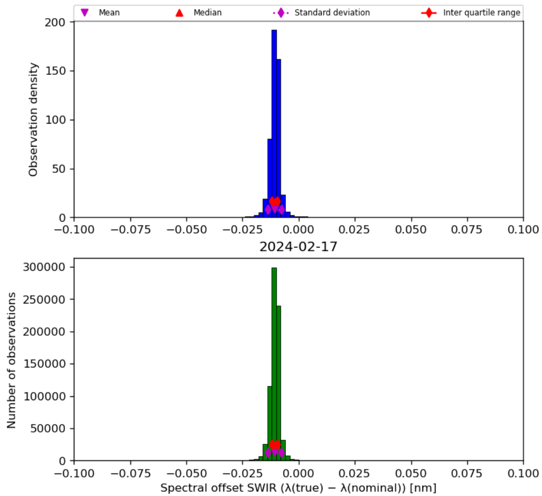
Figure 27: Histogram of “Spectral offset SWIR ( \lambda(\text{true}) - \lambda(\text{nominal}) )” for 2024-02-17 to 2024-02-18
