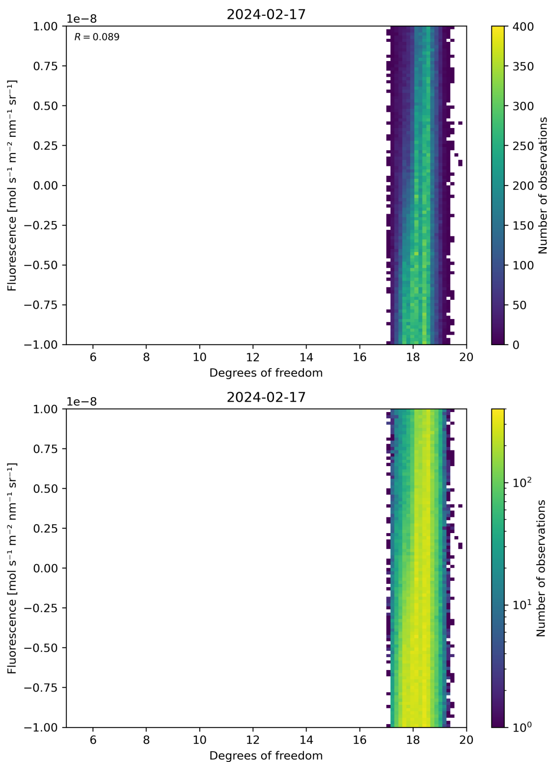
Figure 51: Scatter density plot of “Degrees of freedom” against “Fluorescence” for 2024-02-17 to 2024-02-18.
