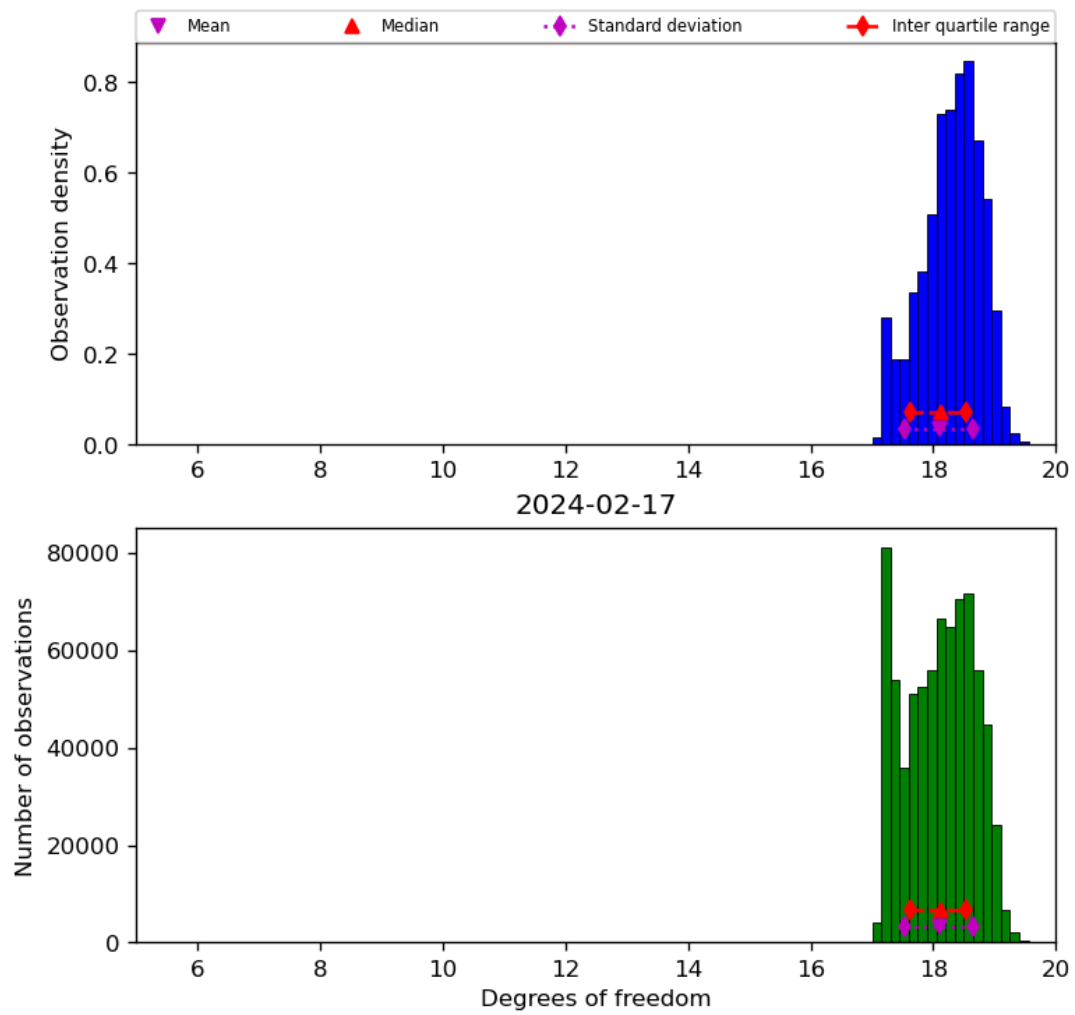
Figure 30: Histogram of “Degrees of freedom” for 2024-02-17 to 2024-02-18
