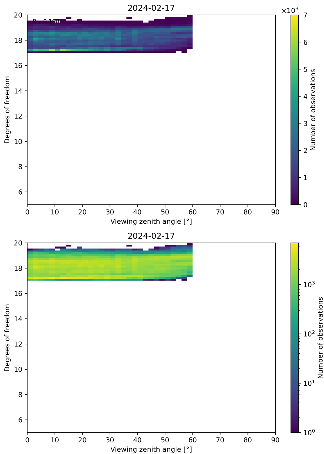
Figure 107: Scatter density plot of “Viewing zenith angle” against “Degrees of freedom” for 2024-02-17 to 2024-02-18.
