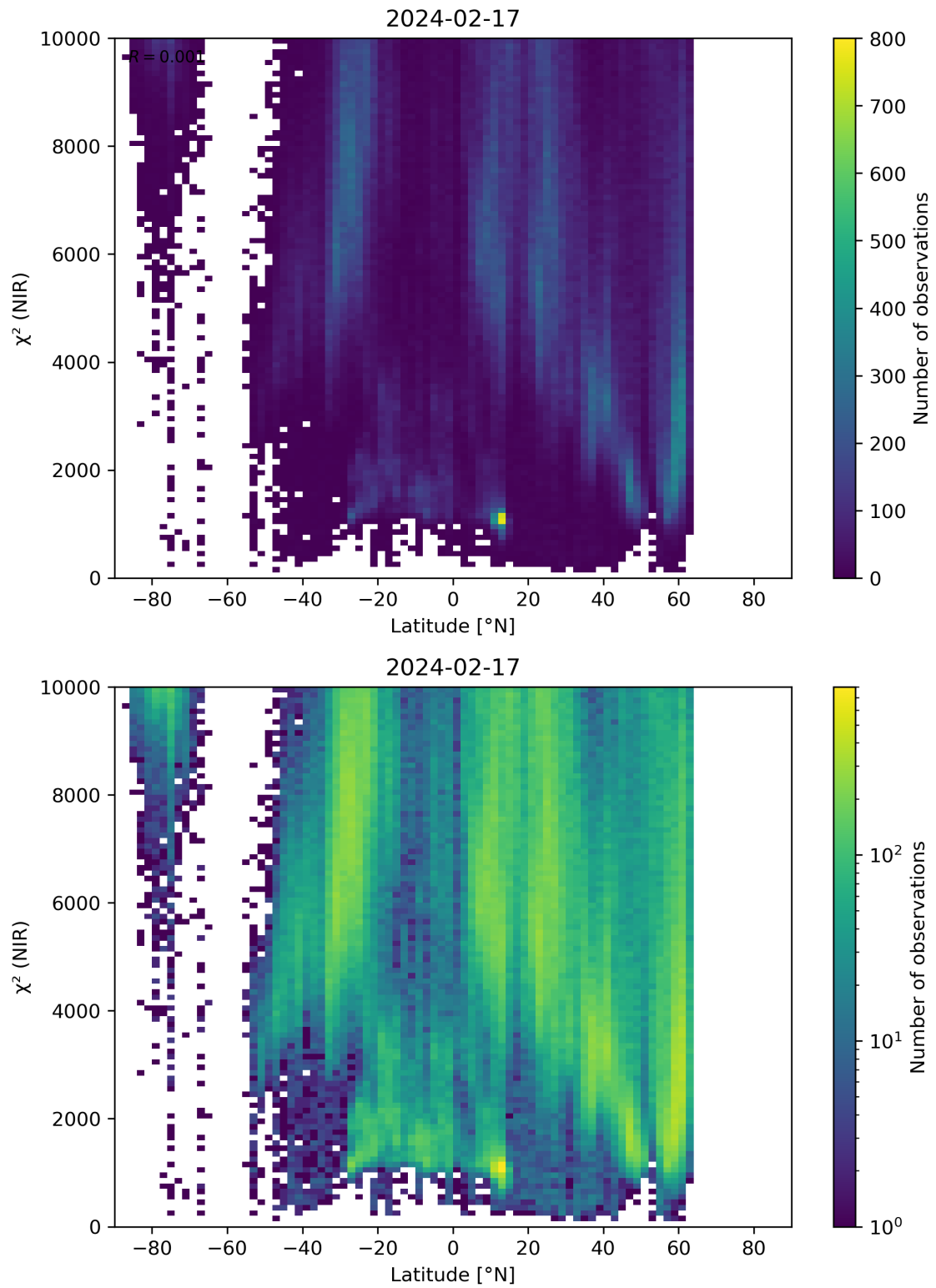
Figure 53: Scatter density plot of “Latitude” against “ \chi^2 (NIR)” for 2024-02-17 to 2024-02-18.
