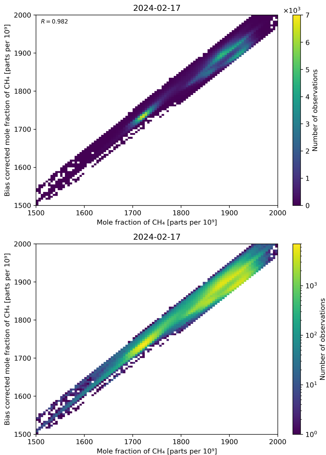
Figure 74: Scatter density plot of “Mole fraction of CH 4 ” against “Bias corrected mole fraction of CH 4 ” for 2024-02-17 to 2024-02-18.
