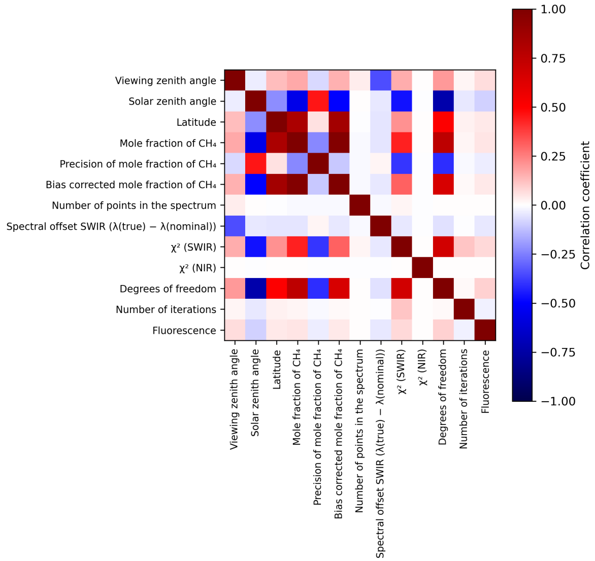
Figure 2: Map of correlation matrix for 2024-02-17 to 2024-02-18.
