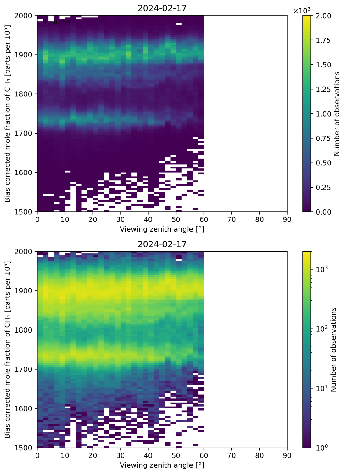
Figure 111: Scatter density plot of “Viewing zenith angle” against “Bias corrected mole fraction of CH 4 ” for 2024-02-17 to 2024-02-18.
