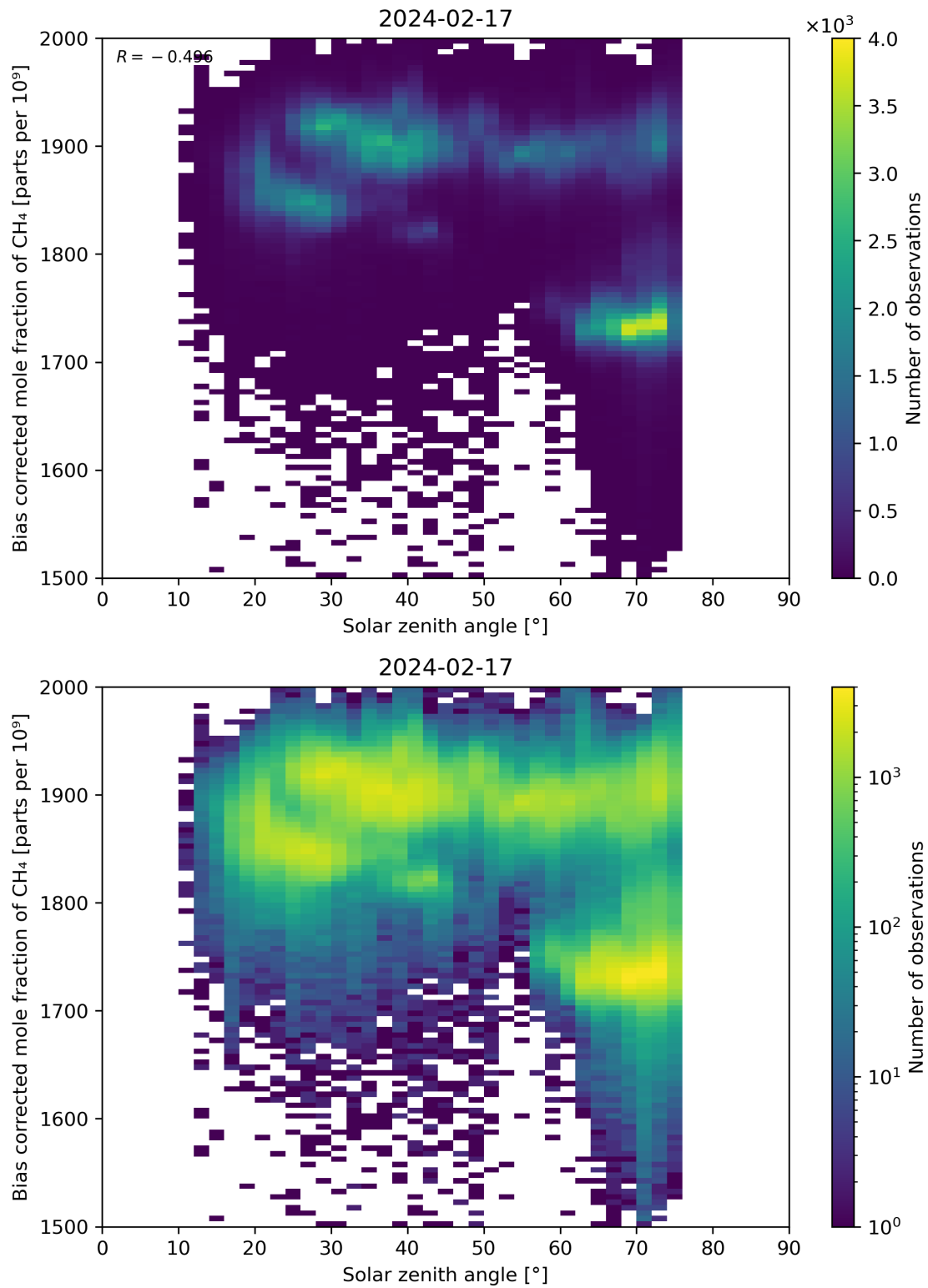
Figure 100: Scatter density plot of “Solar zenith angle” against “Bias corrected mole fraction of CH 4 ” for 2024-02-17 to 2024-02-18.
