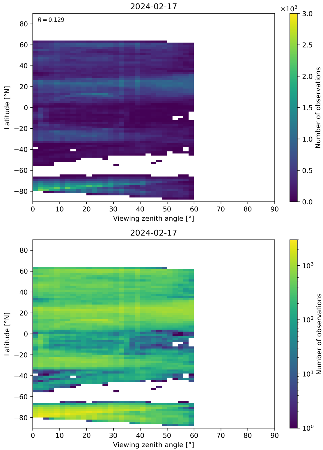
Figure 109: Scatter density plot of “Viewing zenith angle” against “Latitude” for 2024-02-17 to 2024-02-18.
