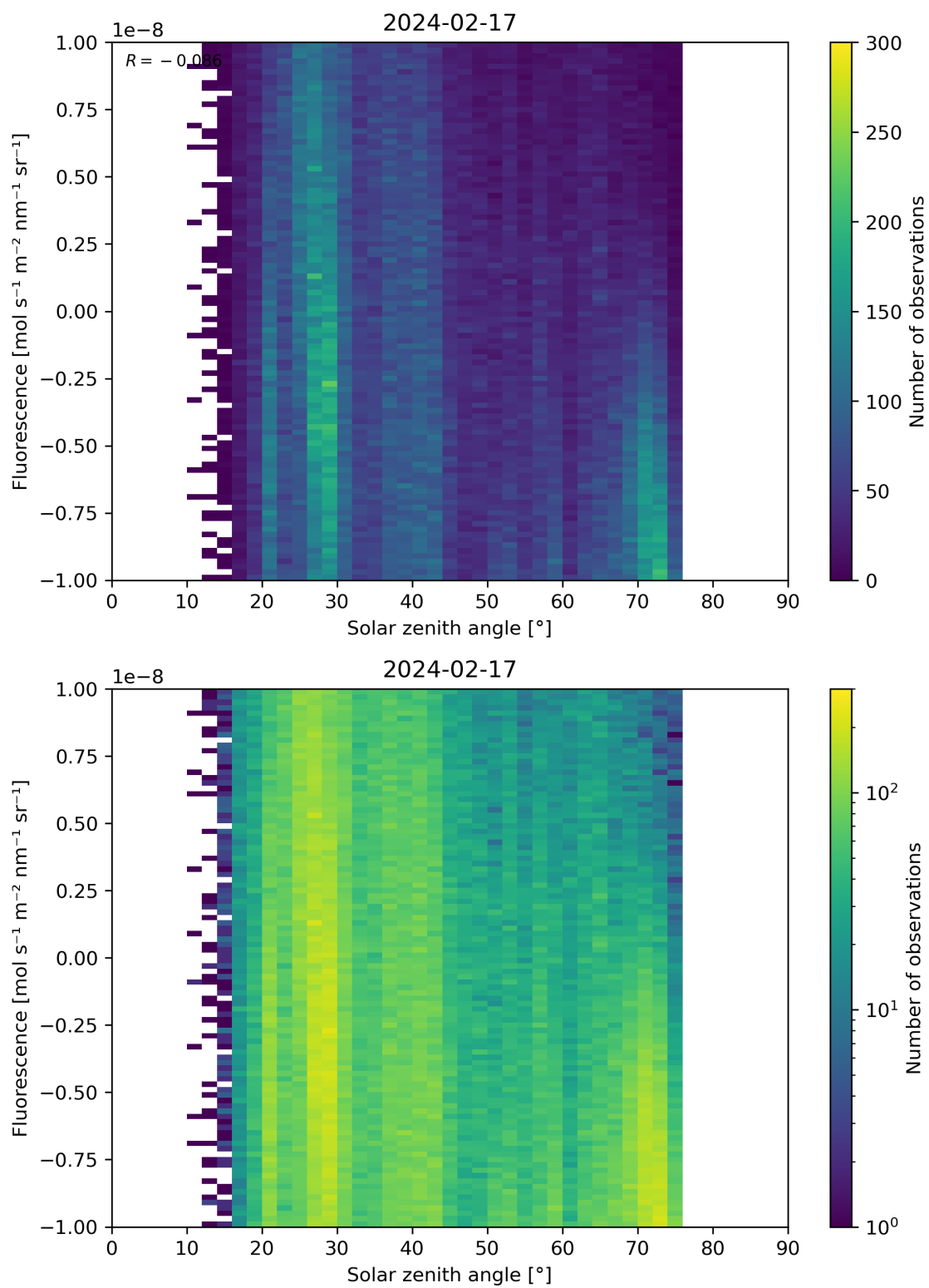
Figure 97: Scatter density plot of “Solar zenith angle” against “Fluorescence” for 2024-02-17 to 2024-02-18.
