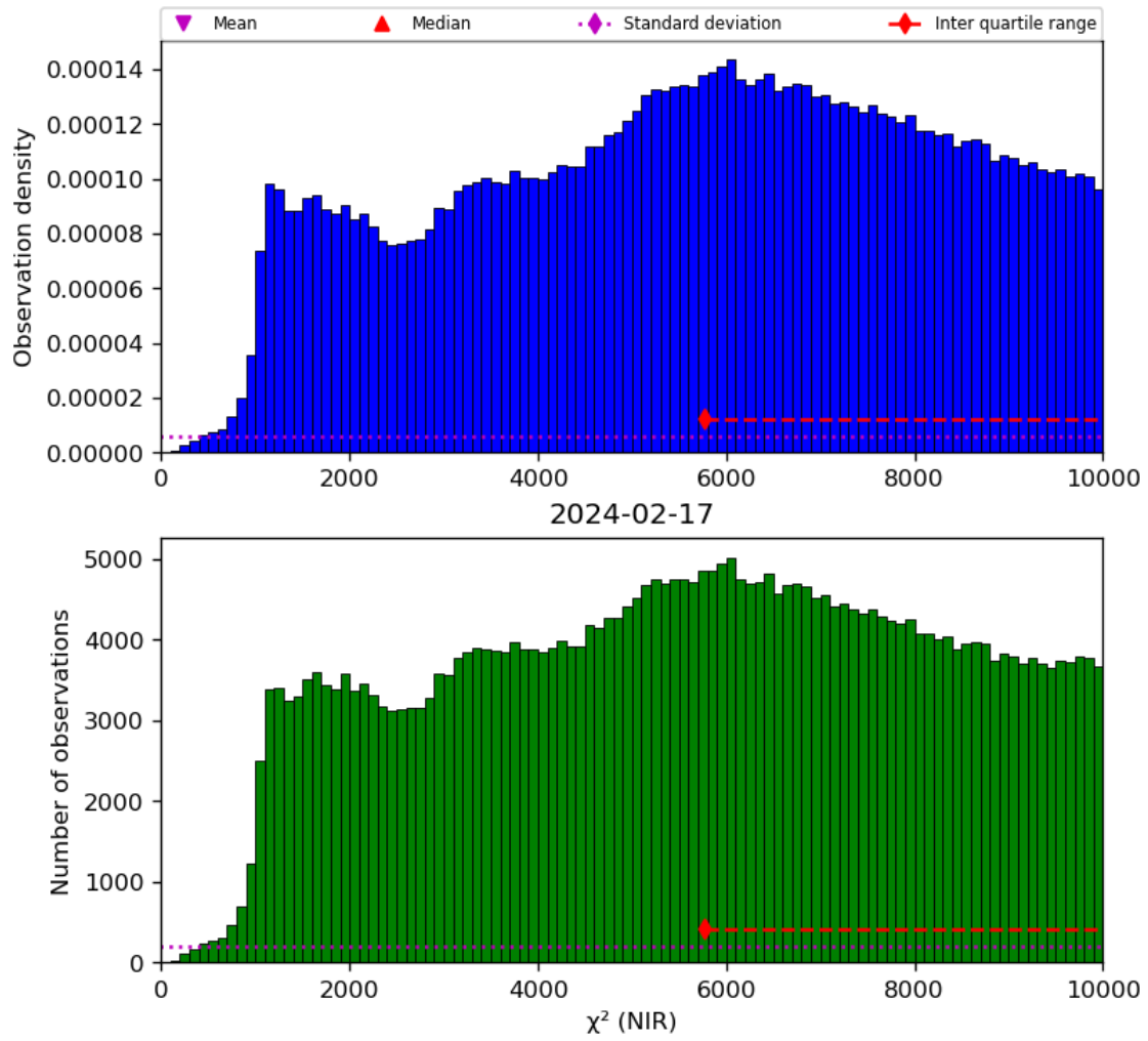
Figure 29: Histogram of “ \chi^2 (NIR)” for 2024-02-17 to 2024-02-18
