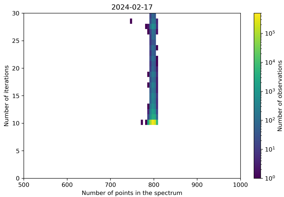
Figure 92: Scatter density plot of “Number of points in the spectrum” against “Number of iterations” for 2024-02-17 to 2024-02-18.
