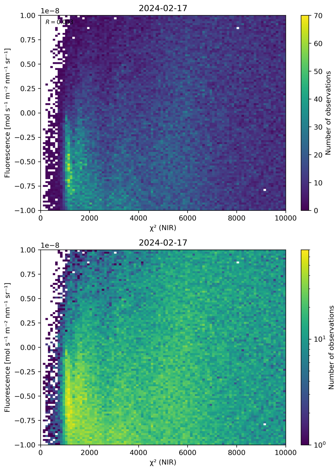
Figure 45: Scatter density plot of “ \chi^2 (NIR)” against “Fluorescence” for 2024-02-17 to 2024-02-18.
