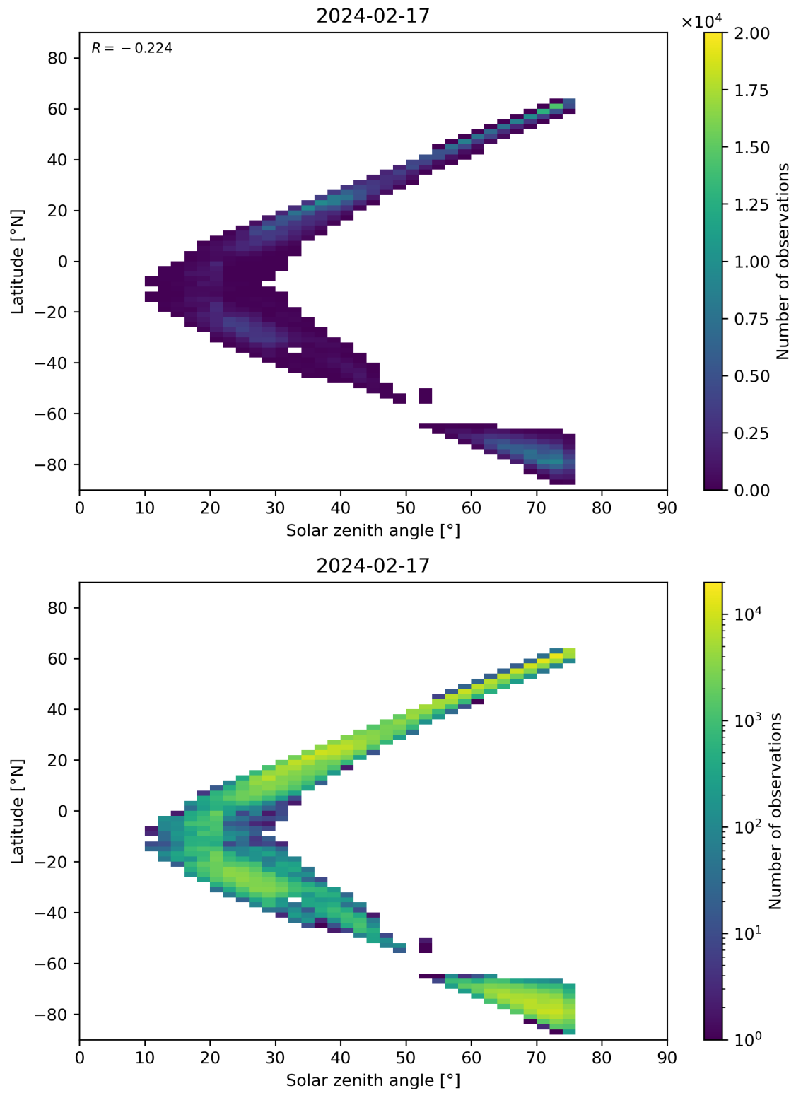
Figure 98: Scatter density plot of “Solar zenith angle” against “Latitude” for 2024-02-17 to 2024-02-18.
