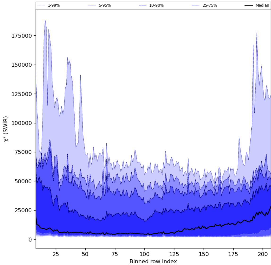
Figure 39: Along track statistics of " \chi^2 (SWIR)" for 2024-02-17 to 2024-02-18
