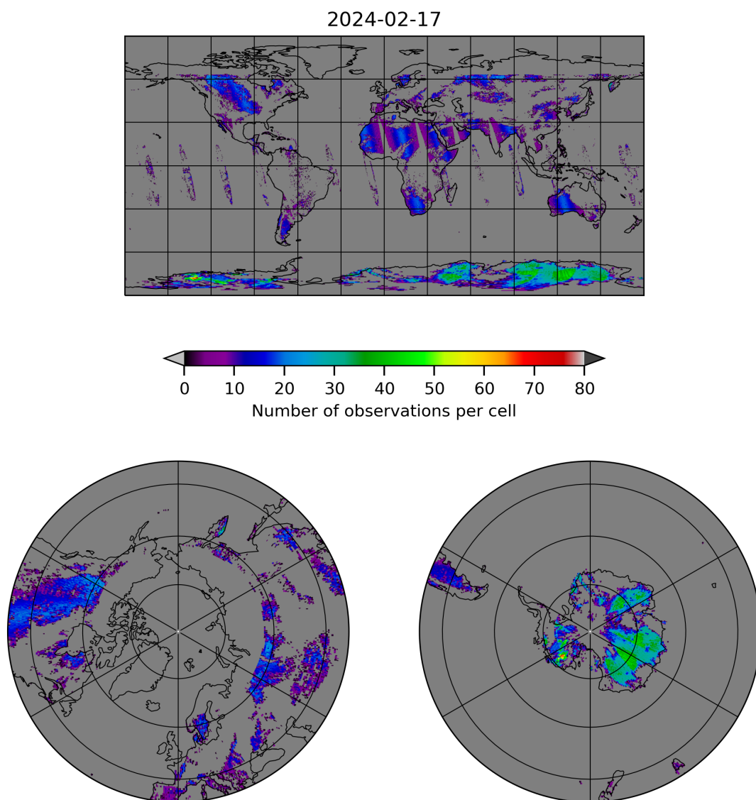
Figure 10: Map of the number of observations for 2024-02-17 to 2024-02-18
