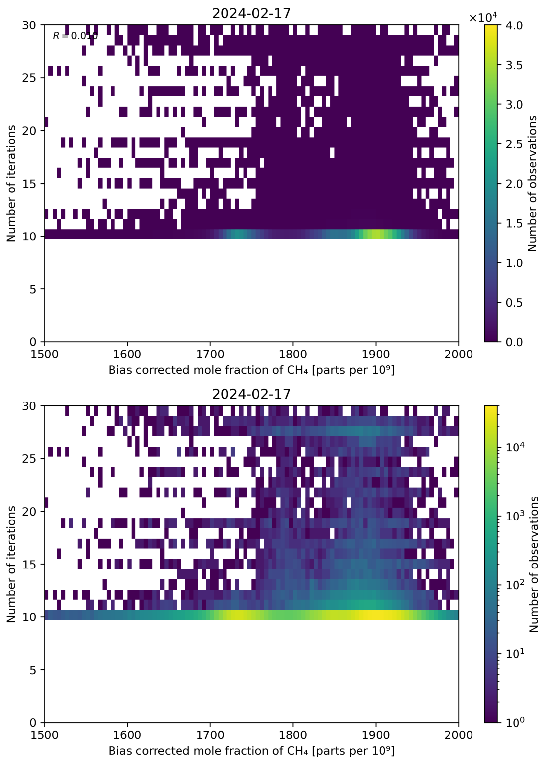
Figure 67: Scatter density plot of “Bias corrected mole fraction of CH 4 ” against “Number of iterations” for 2024-02-17 to 2024-02-18.
