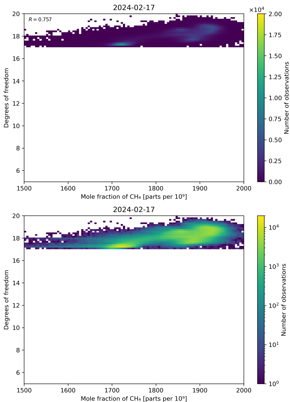
Figure 72: Scatter density plot of “Mole fraction of CH 4 ” against “Degrees of freedom” for 2024-02-17 to 2024-02-18.
