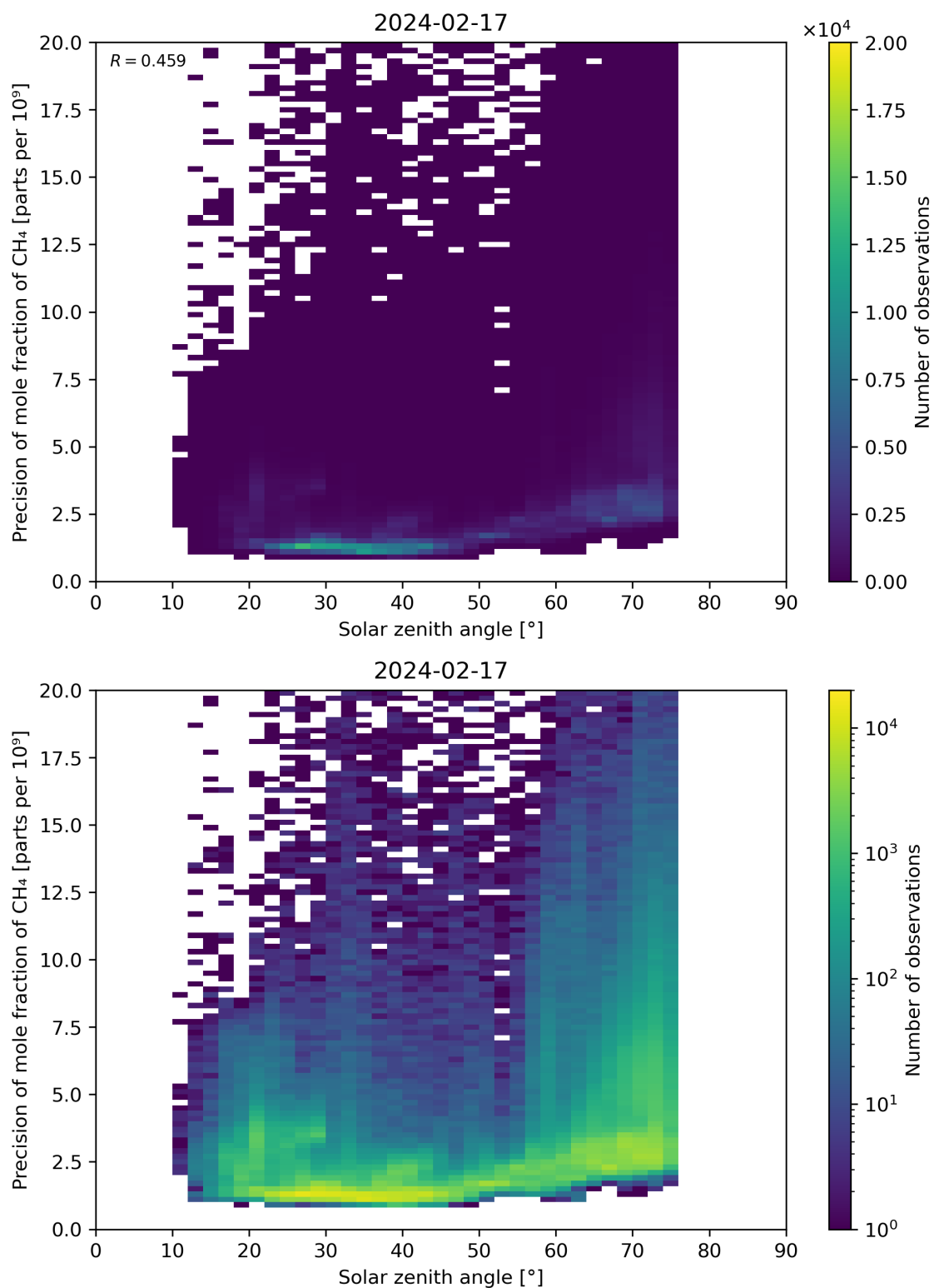
Figure 101: Scatter density plot of “Solar zenith angle” against “Precision of mole fraction of CH 4 ” for 2024-02-17 to 2024-02-18.
