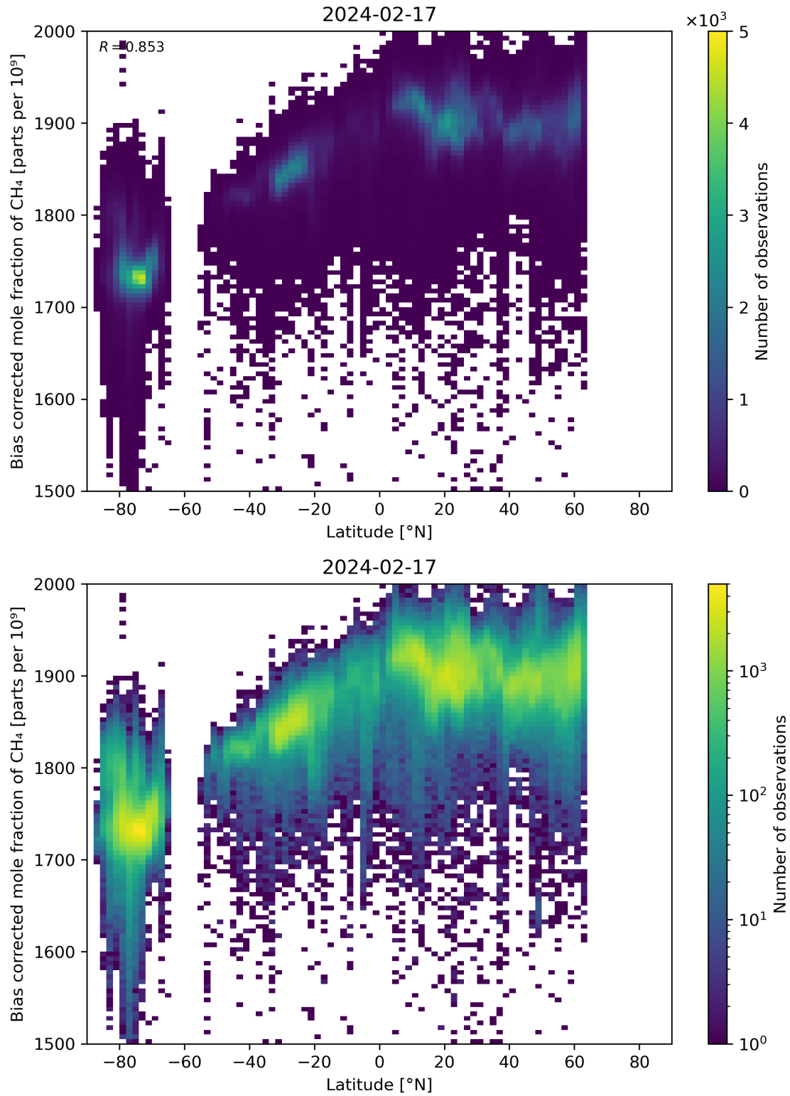
Figure 58: Scatter density plot of “Latitude” against “Bias corrected mole fraction of CH 4 ” for 2024-02-17 to 2024-02-18.
