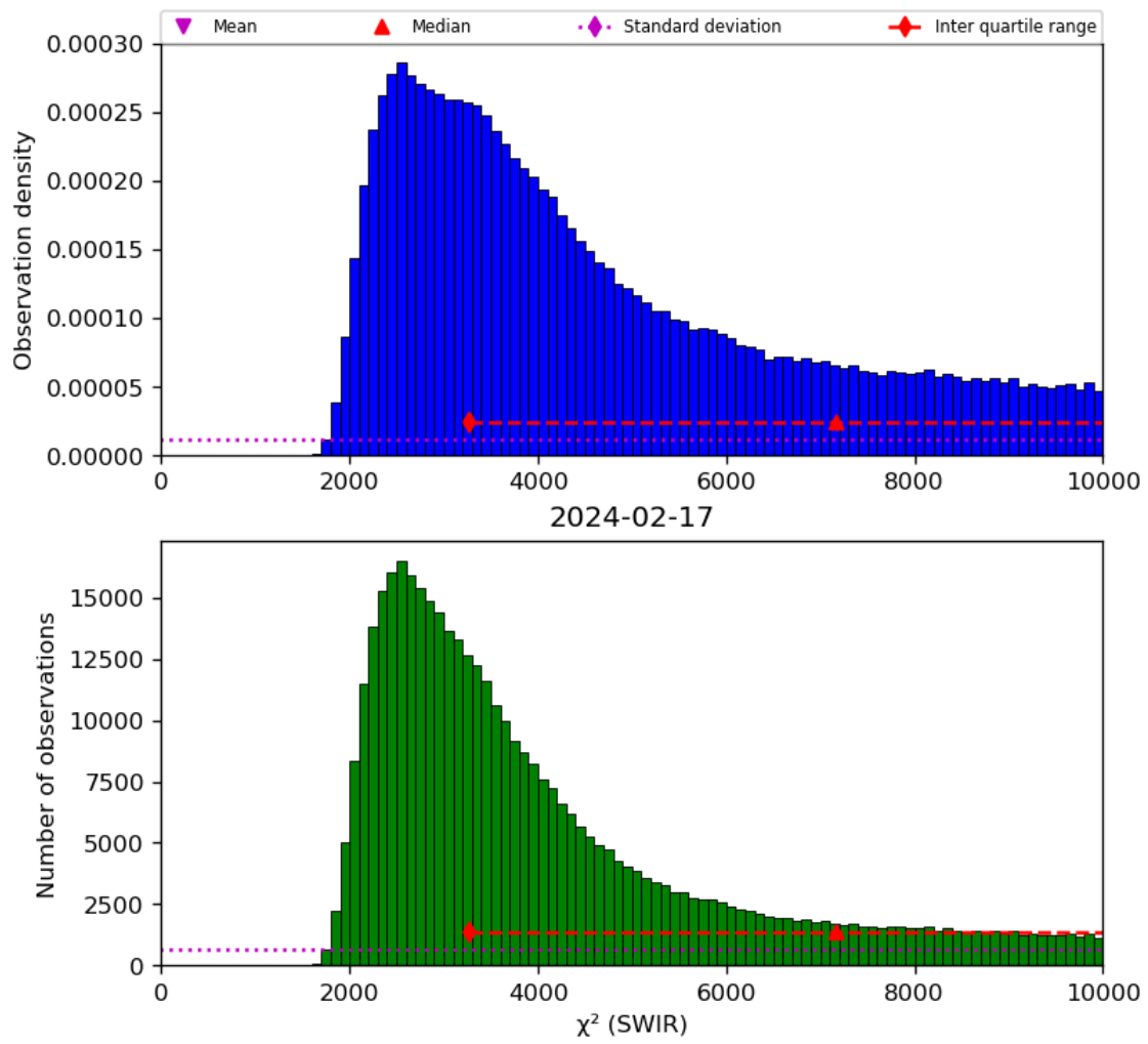
Figure 28: Histogram of “ \chi^2 (SWIR)” for 2024-02-17 to 2024-02-18
