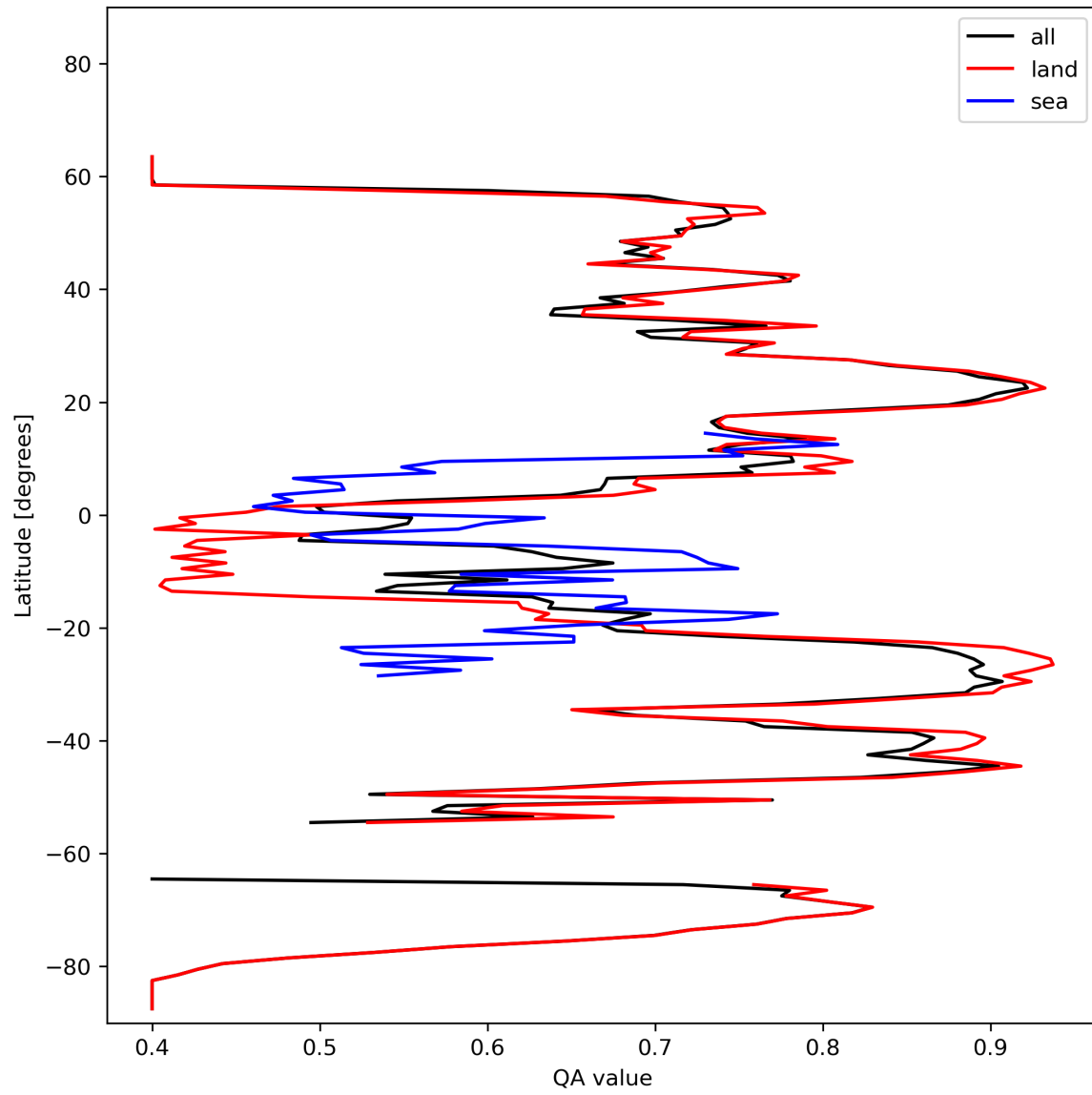
Figure 11: Zonal average of “QA value” for 2024-02-17 to 2024-02-18.
