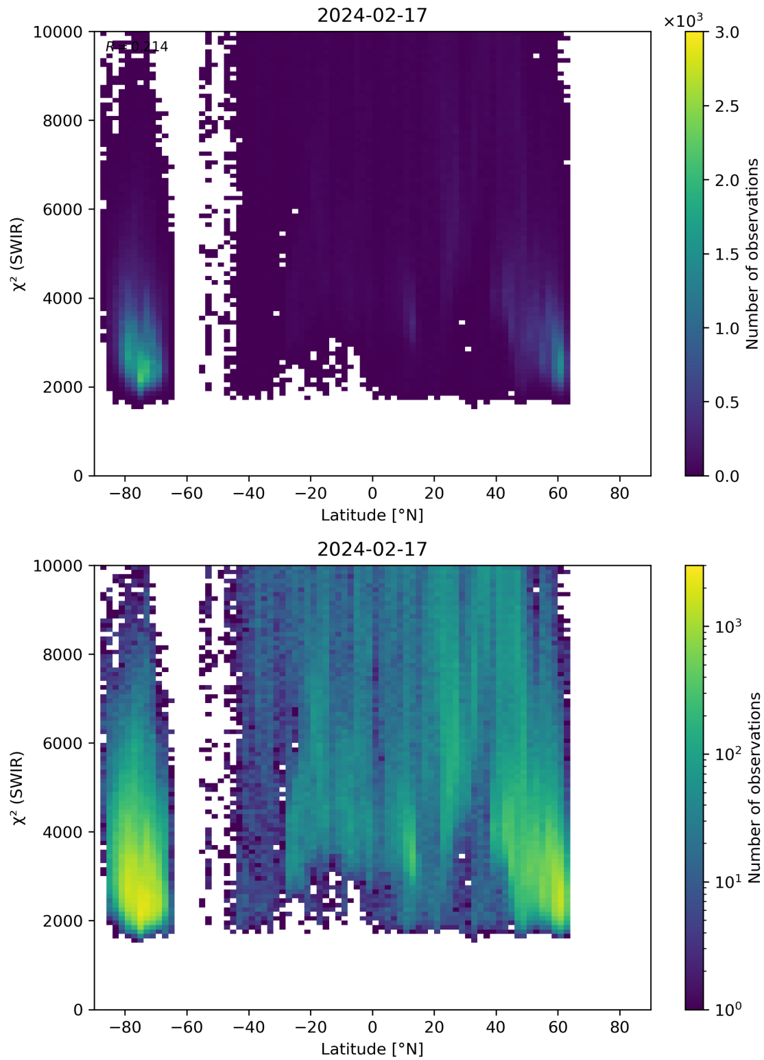
Figure 54: Scatter density plot of “Latitude” against “ \chi^2 (SWIR)” for 2024-02-17 to 2024-02-18.
