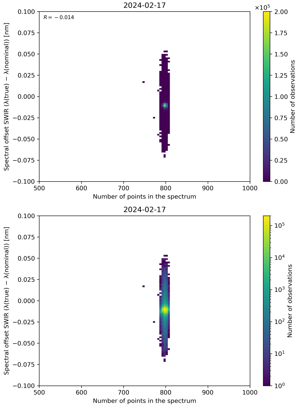
Figure 93: Scatter density plot of “Number of points in the spectrum” against “Spectral offset SWIR ( \lambda(\text{true}) - \lambda(\text{nominal}) )” for 2024-02-17 to 2024-02-18.
