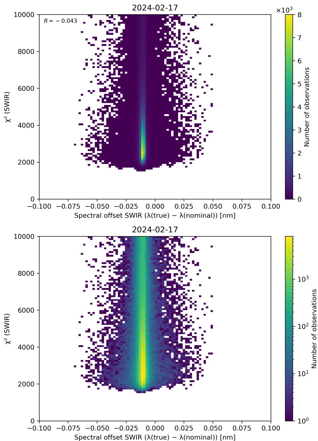
Figure 118: Scatter density plot of “Spectral offset SWIR ( \lambda(\text{true}) - \lambda(\text{nominal}) )” against “ \chi^2 (SWIR)” for 2024-02-17 to 2024-02-18.
