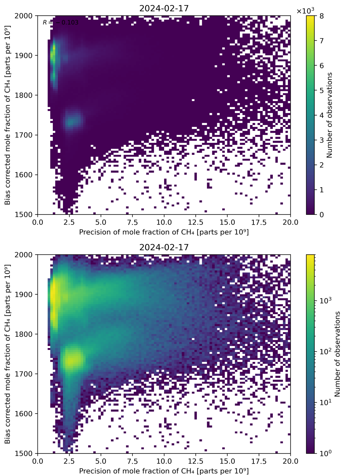
Figure 82: Scatter density plot of “Precision of mole fraction of CH 4 ” against “Bias corrected mole fraction of CH 4 ” for 2024-02-17 to 2024-02-18.
