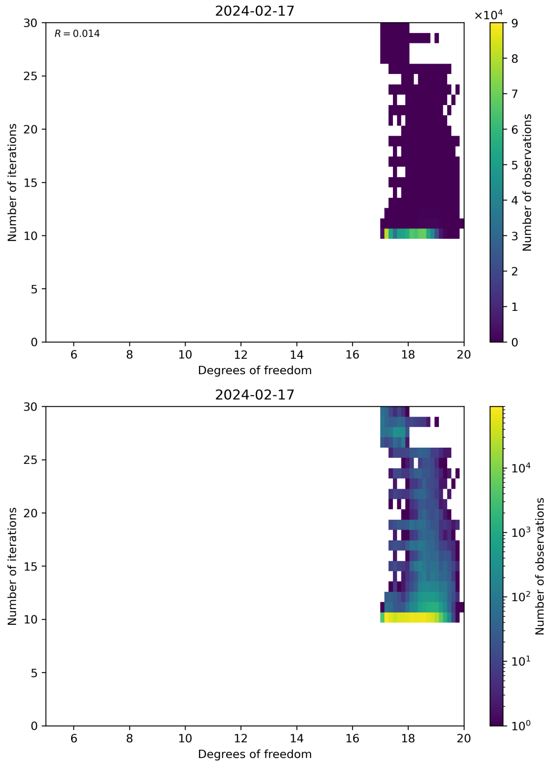
Figure 52: Scatter density plot of “Degrees of freedom” against “Number of iterations” for 2024-02-17 to 2024-02-18.
