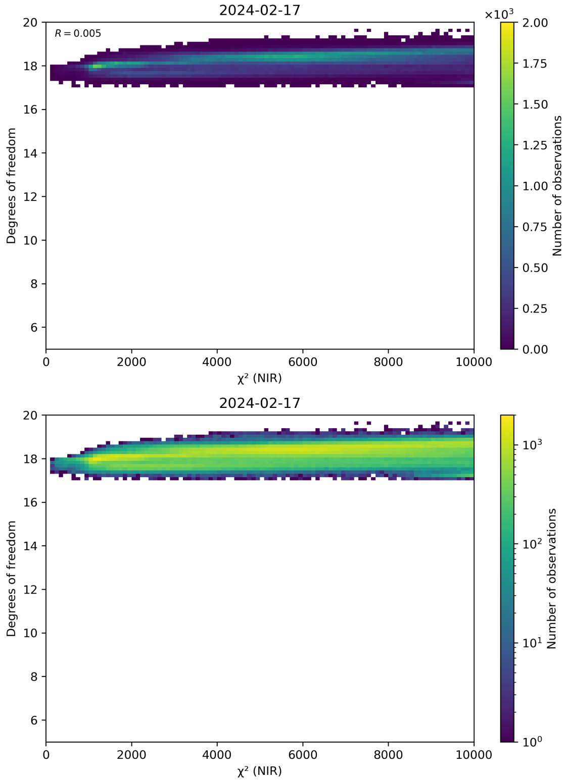
Figure 44: Scatter density plot of “ \chi^2 (NIR)” against “Degrees of freedom” for 2024-02-17 to 2024-02-18.
