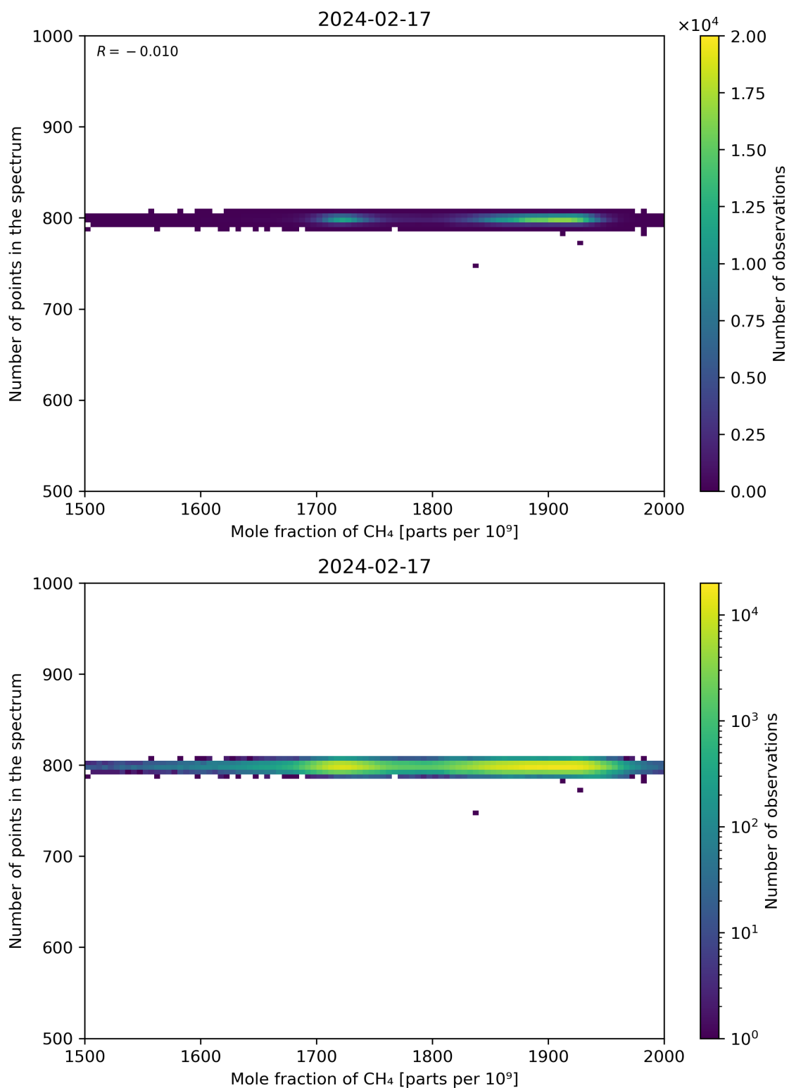
Figure 77: Scatter density plot of “Mole fraction of CH 4 ” against “Number of points in the spectrum” for 2024-02-17 to 2024-02-18.
