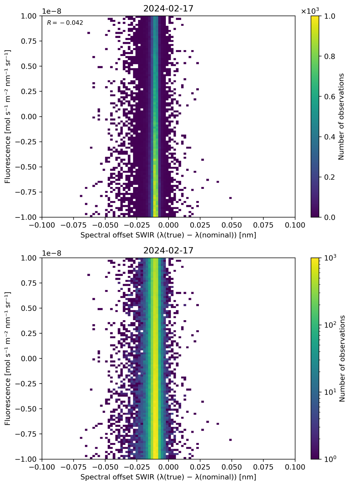
Figure 120: Scatter density plot of “Spectral offset SWIR ( \lambda(\text{true}) - \lambda(\text{nominal}) )” against “Fluorescence” for 2024-02-17 to 2024-02-18.
