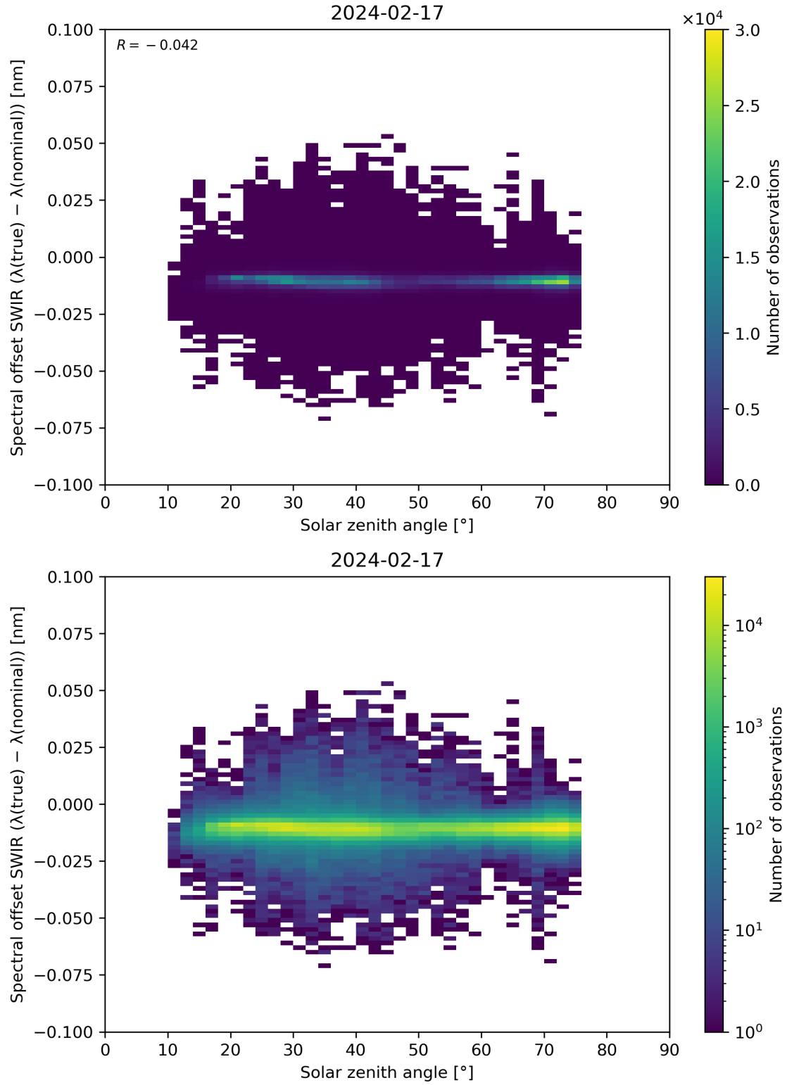
Figure 104: Scatter density plot of “Solar zenith angle” against “Spectral offset SWIR ( \lambda(\text{true}) - \lambda(\text{nominal}) )” for 2024-02-17 to 2024-02-18.
