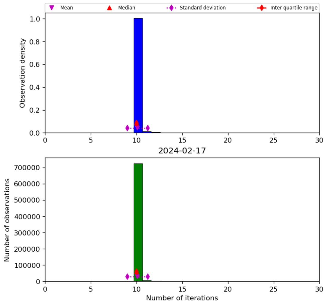
Figure 31: Histogram of “Number of iterations” for 2024-02-17 to 2024-02-18
