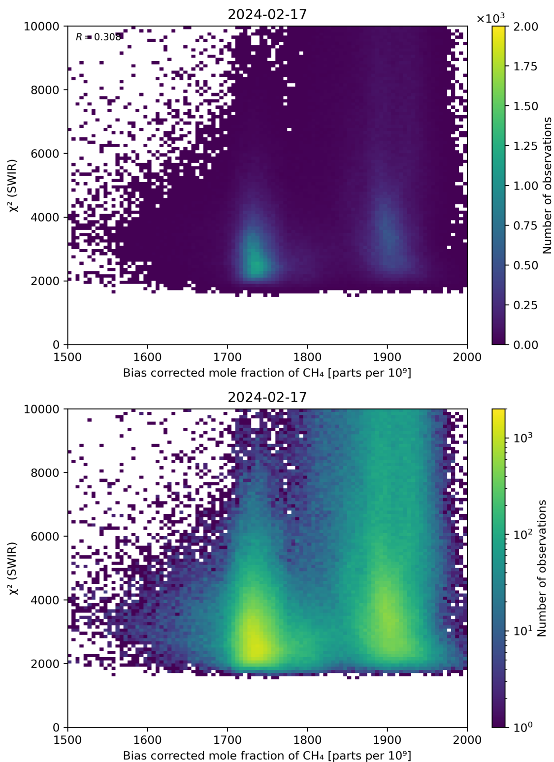
Figure 64: Scatter density plot of “Bias corrected mole fraction of CH 4 ” against “ \chi^2 (SWIR)” for 2024-02-17 to 2024-02-18.
