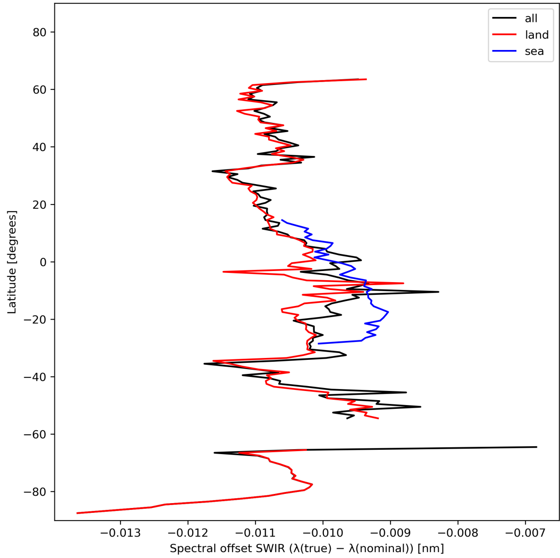
Figure 16: Zonal average of “Spectral offset SWIR ( \lambda(\text{true}) - \lambda(\text{nominal}) )” for 2024-02-17 to 2024-02-18.
