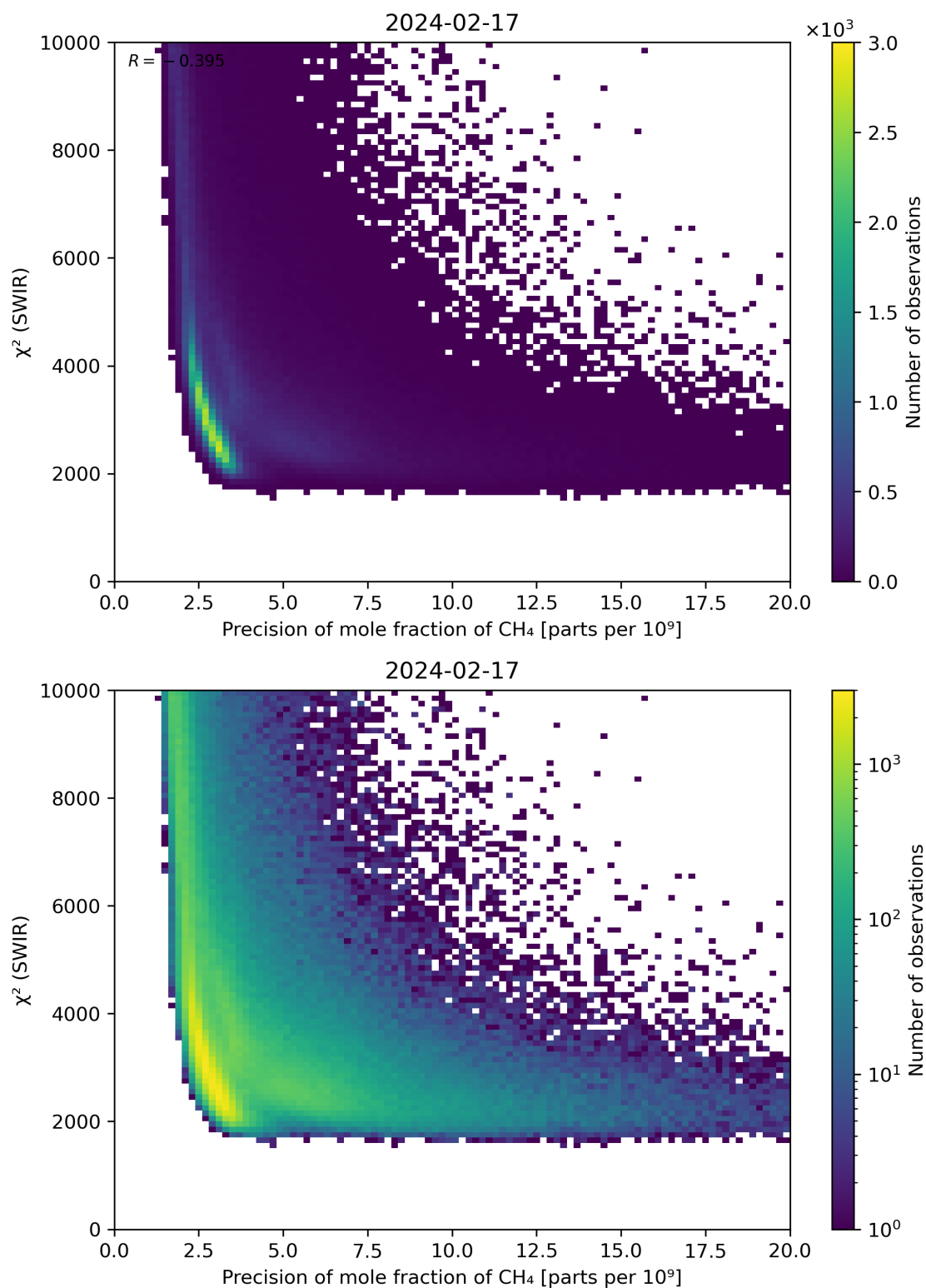
Figure 79: Scatter density plot of “Precision of mole fraction of CH 4 ” against “ \chi^2 (SWIR)” for 2024-02-17 to 2024-02-18.
