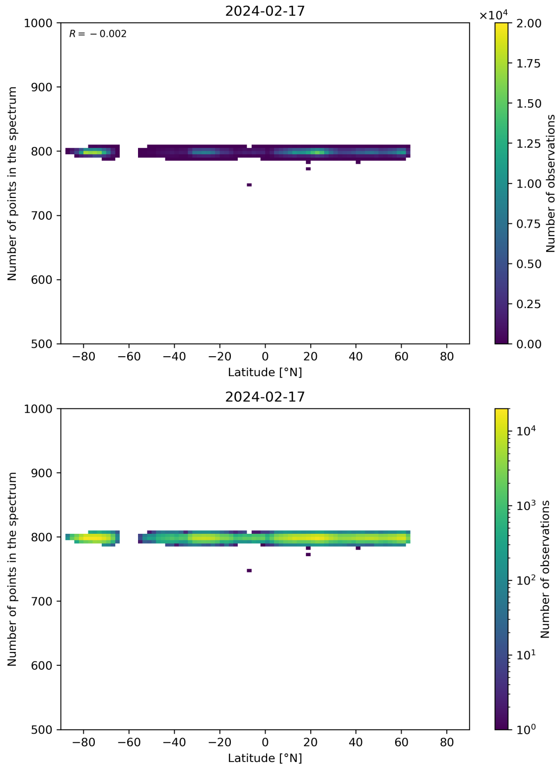
Figure 61: Scatter density plot of “Latitude” against “Number of points in the spectrum” for 2024-02-17 to 2024-02-18.
