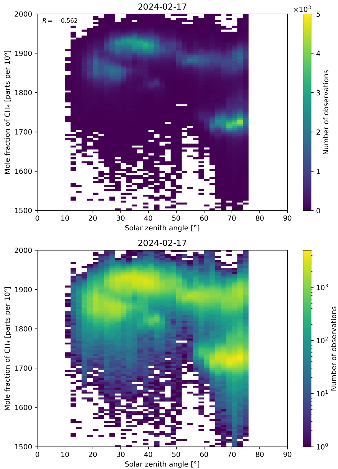
Figure 99: Scatter density plot of “Solar zenith angle” against “Mole fraction of CH 4 ” for 2024-02-17 to 2024-02-18.
