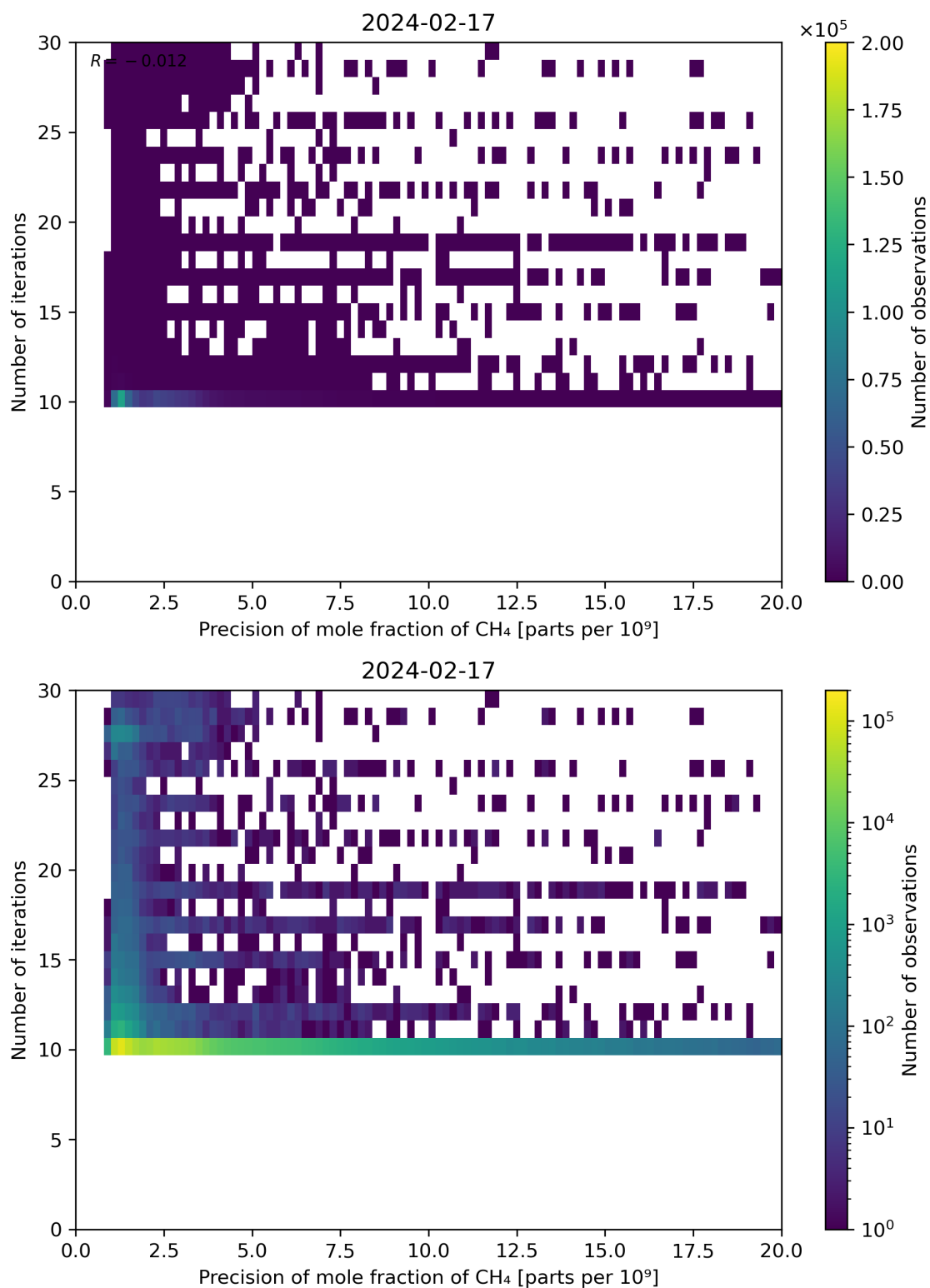
Figure 83: Scatter density plot of “Precision of mole fraction of CH 4 ” against “Number of iterations” for 2024-02-17 to 2024-02-18.
