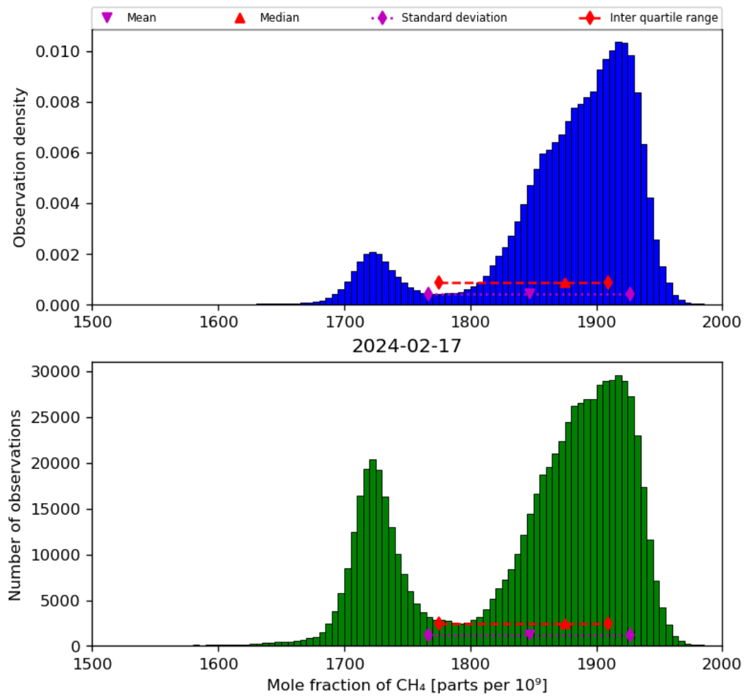
Figure 23: Histogram of “Mole fraction of CH 4 ” for 2024-02-17 to 2024-02-18
