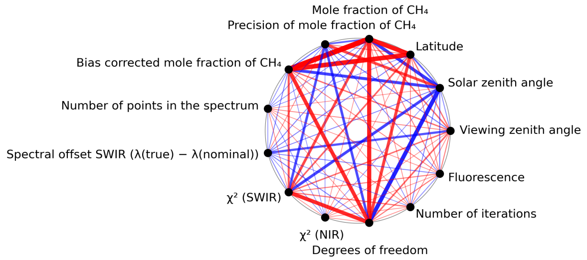
Figure 1: Map of correlation graph for 2024-02-17 to 2024-02-18.
