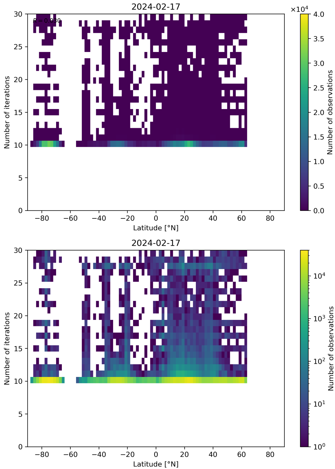
Figure 60: Scatter density plot of “Latitude” against “Number of iterations” for 2024-02-17 to 2024-02-18.
