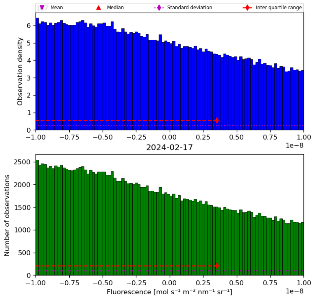
Figure 32: Histogram of “Fluorescence” for 2024-02-17 to 2024-02-18
