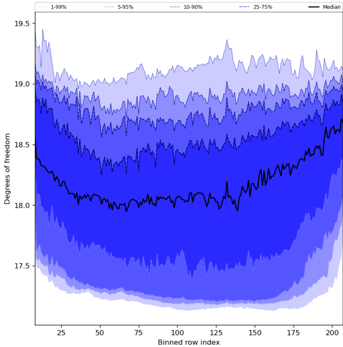
Figure 41: Along track statistics of “Degrees of freedom” for 2024-02-17 to 2024-02-18
