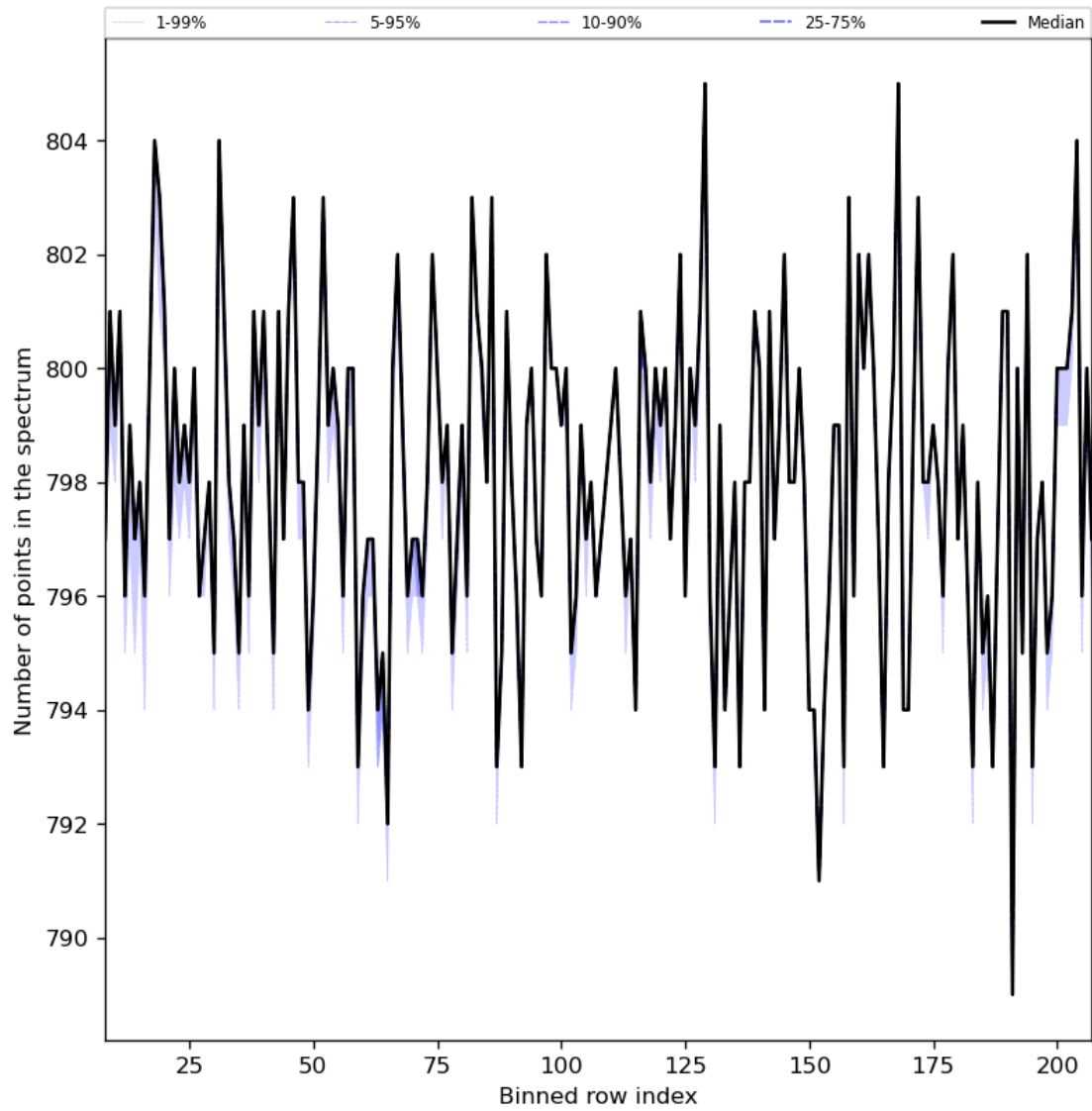
Figure 37: Along track statistics of “Number of points in the spectrum” for 2024-02-17 to 2024-02-18
