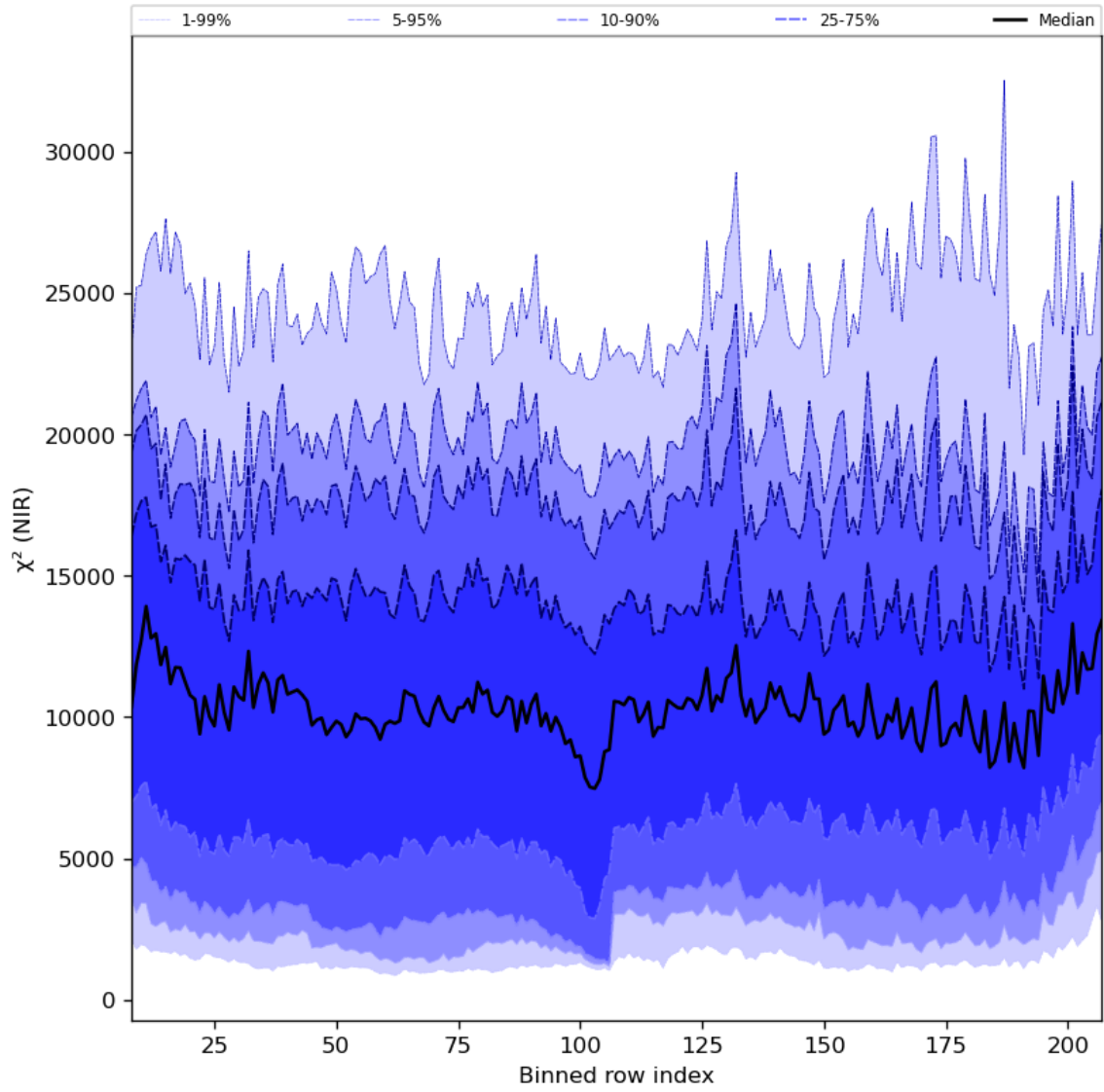
Figure 40: Along track statistics of " \chi^2 (NIR)" for 2024-02-17 to 2024-02-18
