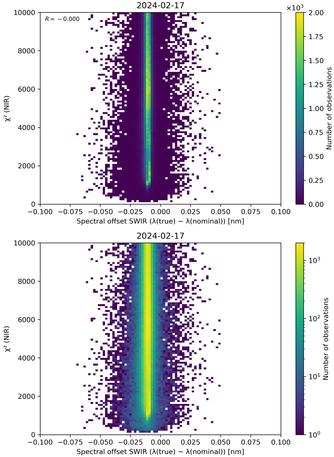
Figure 117: Scatter density plot of “Spectral offset SWIR ( \lambda(\text{true}) - \lambda(\text{nominal}) )” against “ \chi^2 (NIR)” for 2024-02-17 to 2024-02-18.
