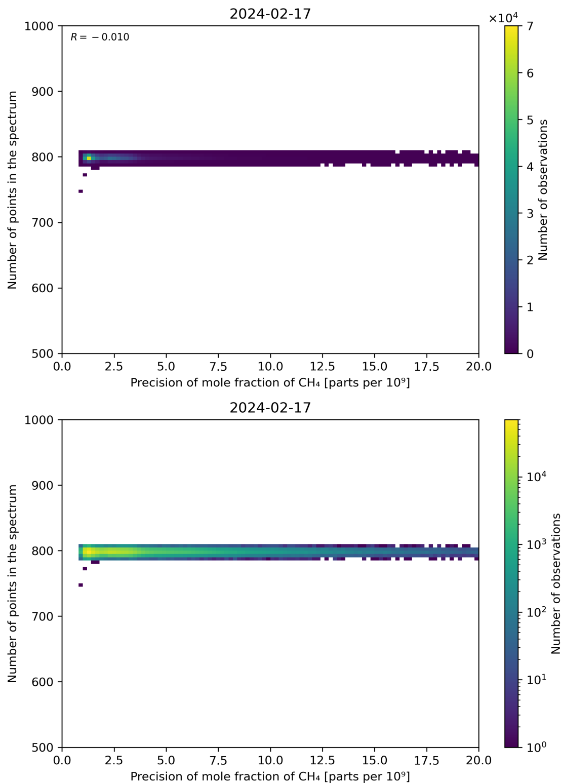
Figure 84: Scatter density plot of “Precision of mole fraction of CH 4 ” against “Number of points in the spectrum” for 2024-02-17 to 2024-02-18.
