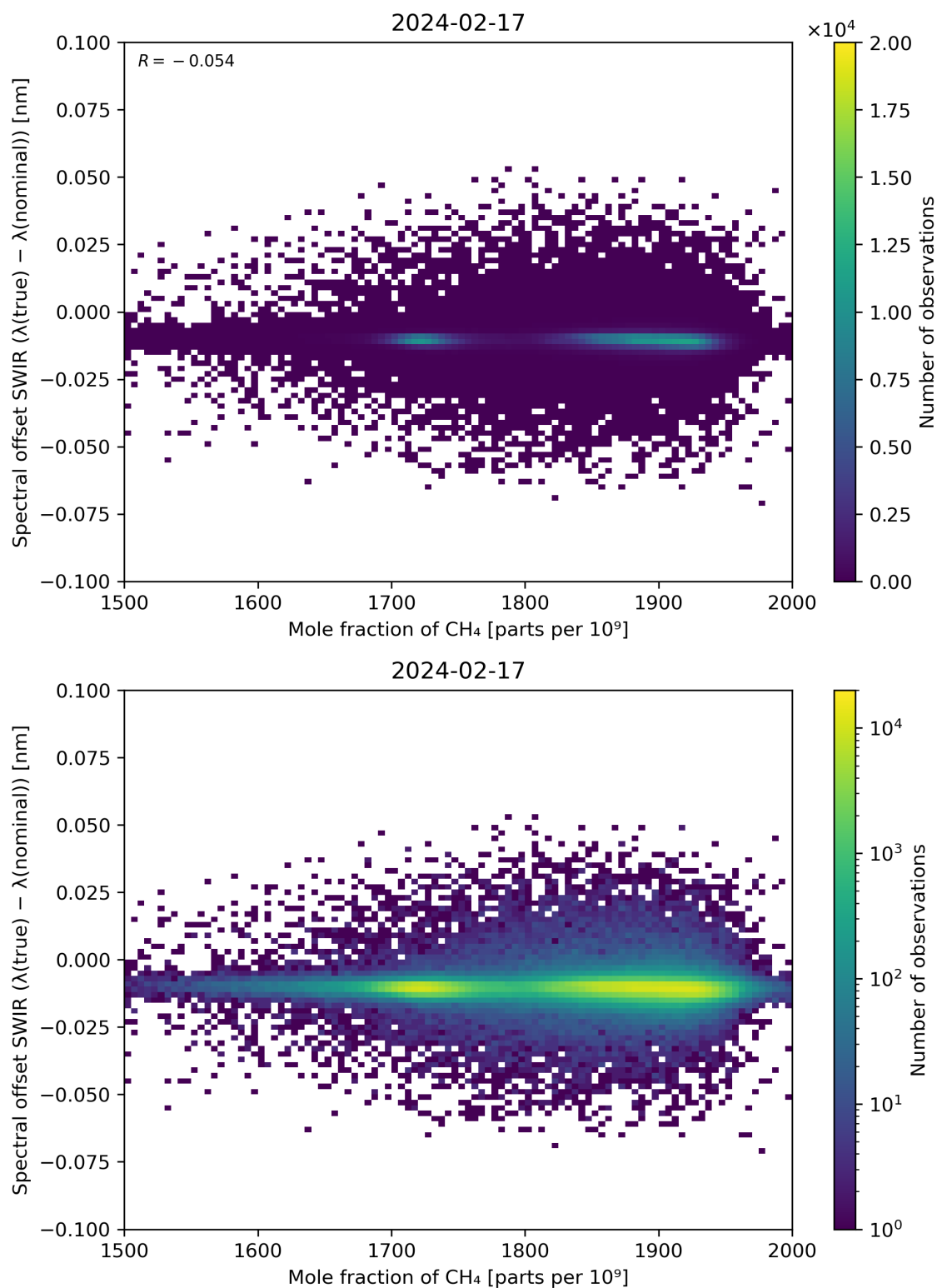
Figure 86: Scatter density plot of “Mole fraction of CH 4 ” against “Spectral offset SWIR ( \lambda(\text{true}) - \lambda(\text{nominal}) )” for 2024-02-17 to 2024-02-18.
