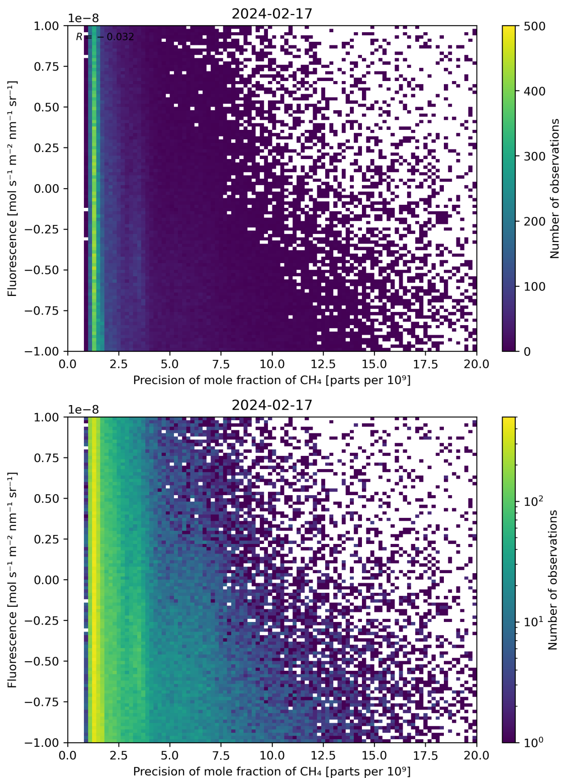
Figure 81: Scatter density plot of “Precision of mole fraction of CH 4 ” against “Fluorescence” for 2024-02-17 to 2024-02-18.
