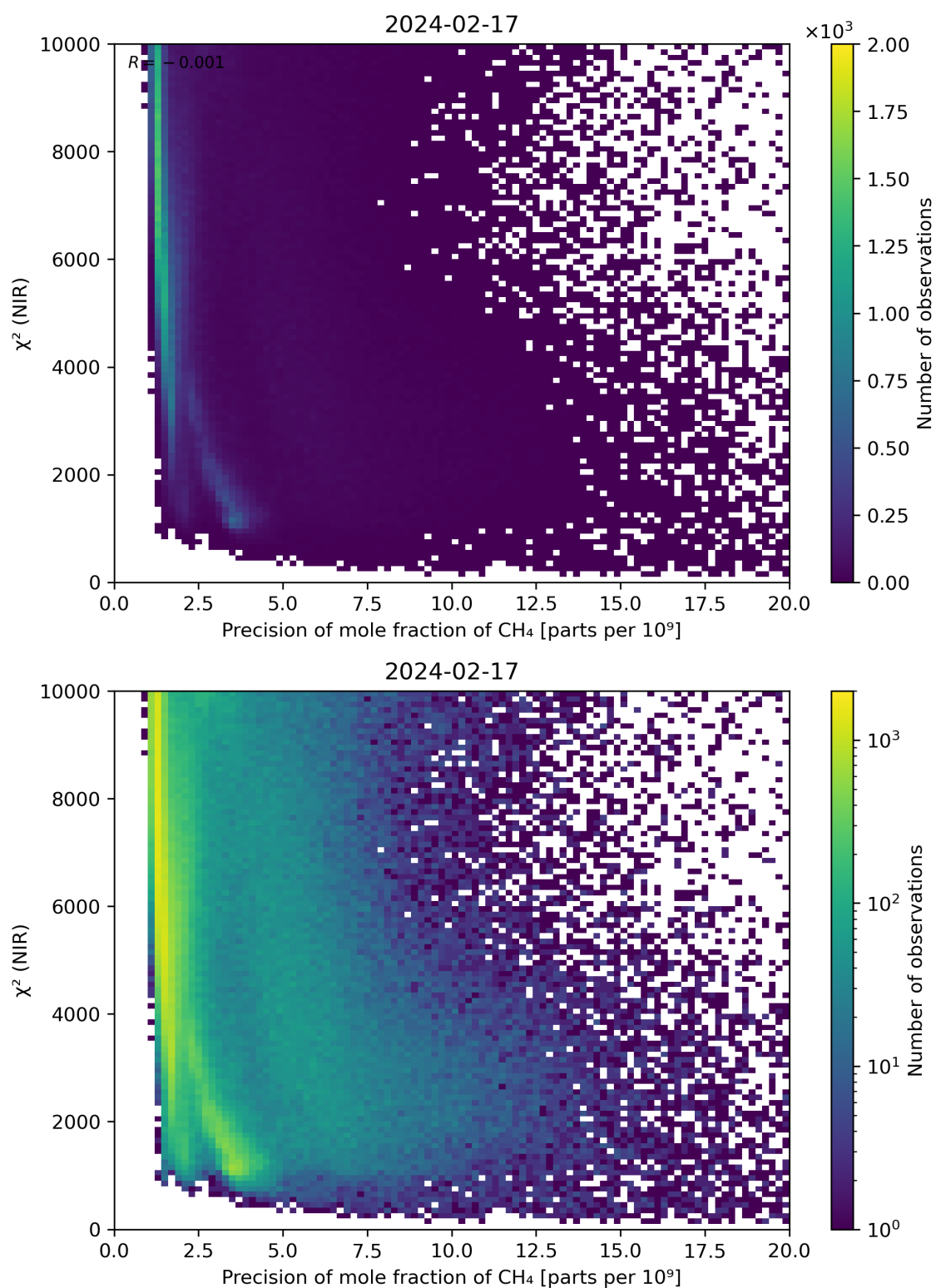
Figure 78: Scatter density plot of “Precision of mole fraction of \text{CH}_4 ” against “ \chi^2 (NIR)” for 2024-02-17 to 2024-02-18.
