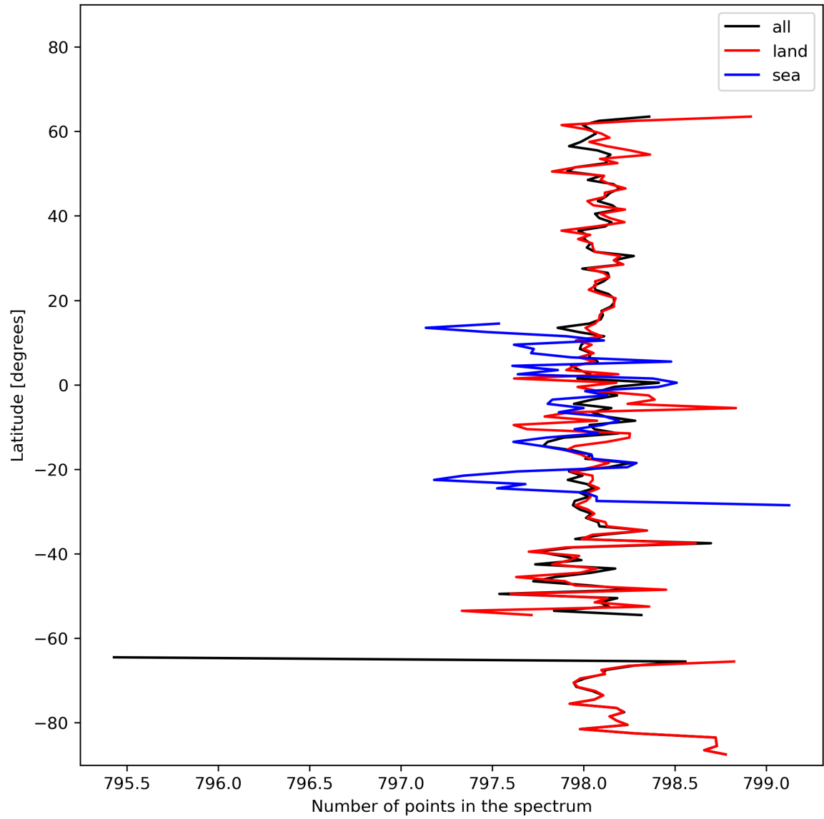
Figure 15: Zonal average of “Number of points in the spectrum” for 2024-02-17 to 2024-02-18.
