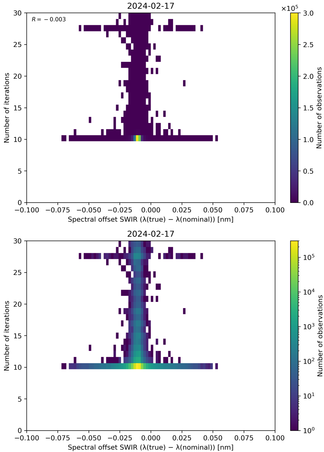
Figure 121: Scatter density plot of “Spectral offset SWIR ( \lambda(\text{true}) - \lambda(\text{nominal}) )” against “Number of iterations” for 2024-02-17 to 2024-02-18.
