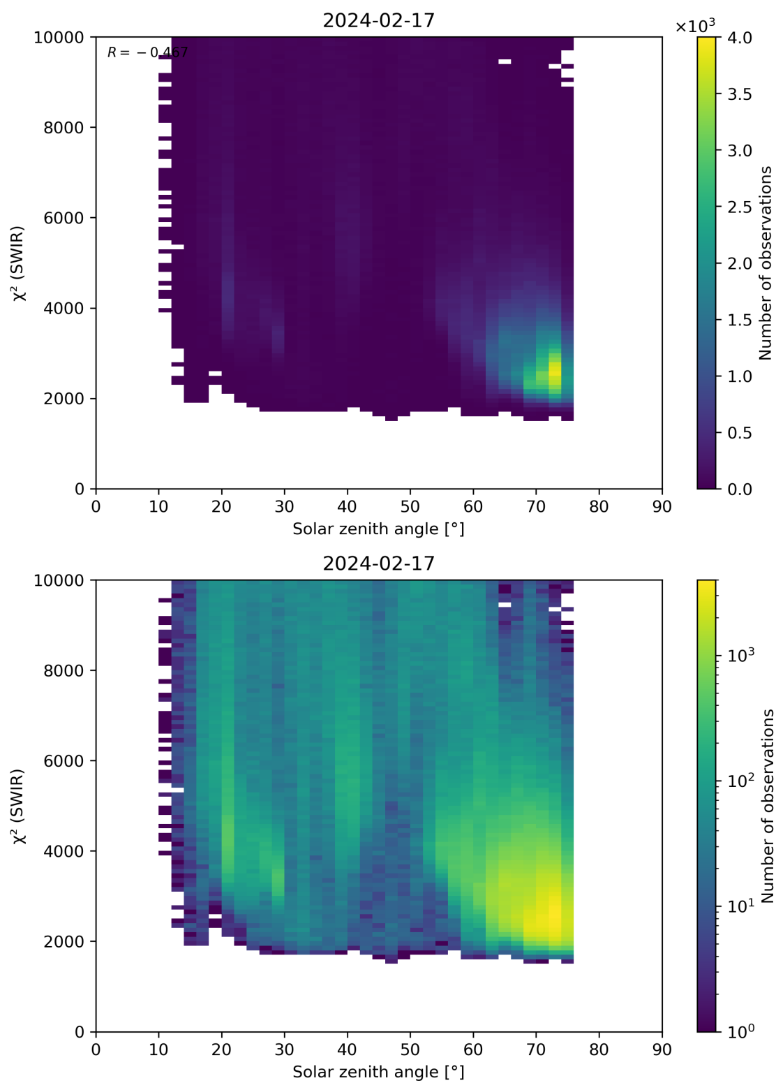
Figure 95: Scatter density plot of “Solar zenith angle” against “ \chi^2 (SWIR)” for 2024-02-17 to 2024-02-18.
