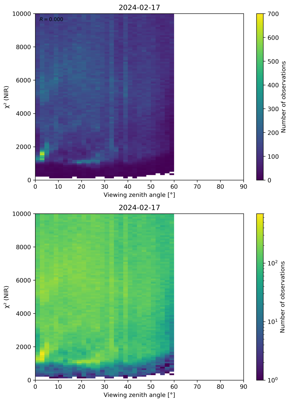
Figure 105: Scatter density plot of “Viewing zenith angle” against “ \chi^2 (NIR)” for 2024-02-17 to 2024-02-18.
