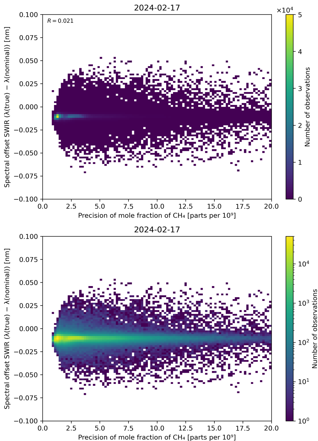
Figure 85: Scatter density plot of “Precision of mole fraction of \text{CH}_4 ” against “Spectral offset SWIR ( \lambda(\text{true}) - \lambda(\text{nominal}) )” for 2024-02-17 to 2024-02-18.
