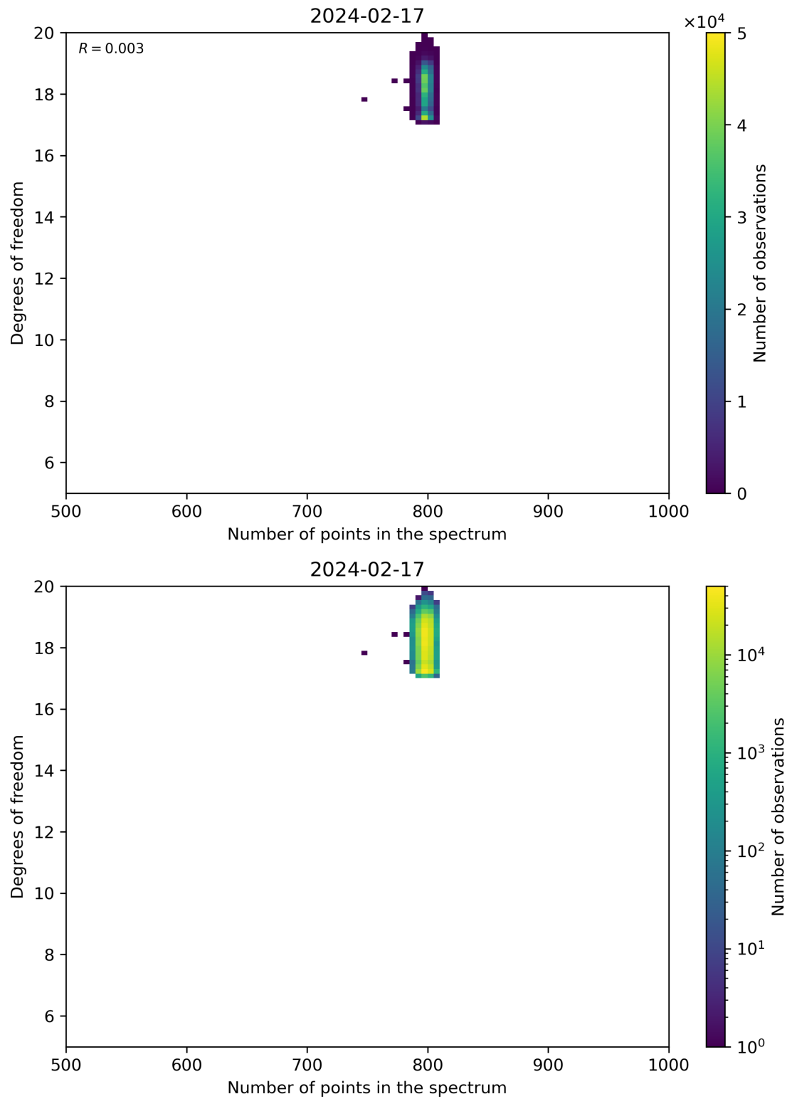
Figure 90: Scatter density plot of “Number of points in the spectrum” against “Degrees of freedom” for 2024-02-17 to 2024-02-18.
