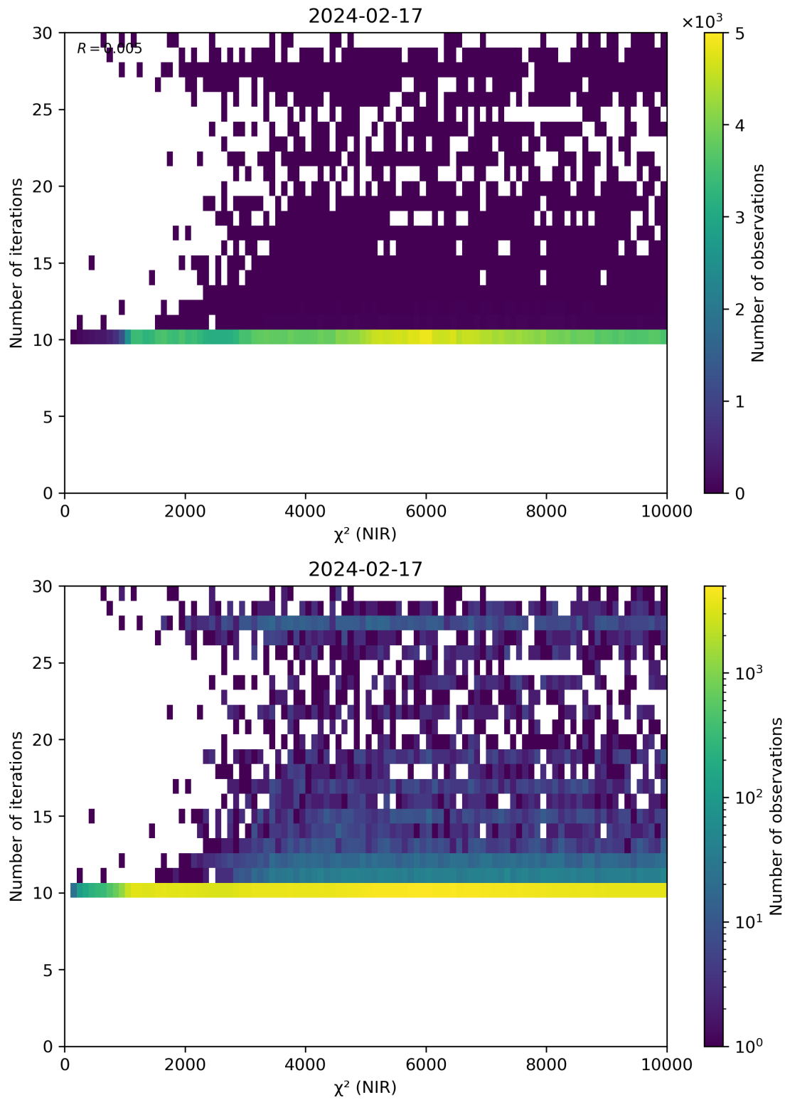
Figure 46: Scatter density plot of “ \chi^2 (NIR)” against “Number of iterations” for 2024-02-17 to 2024-02-18.
