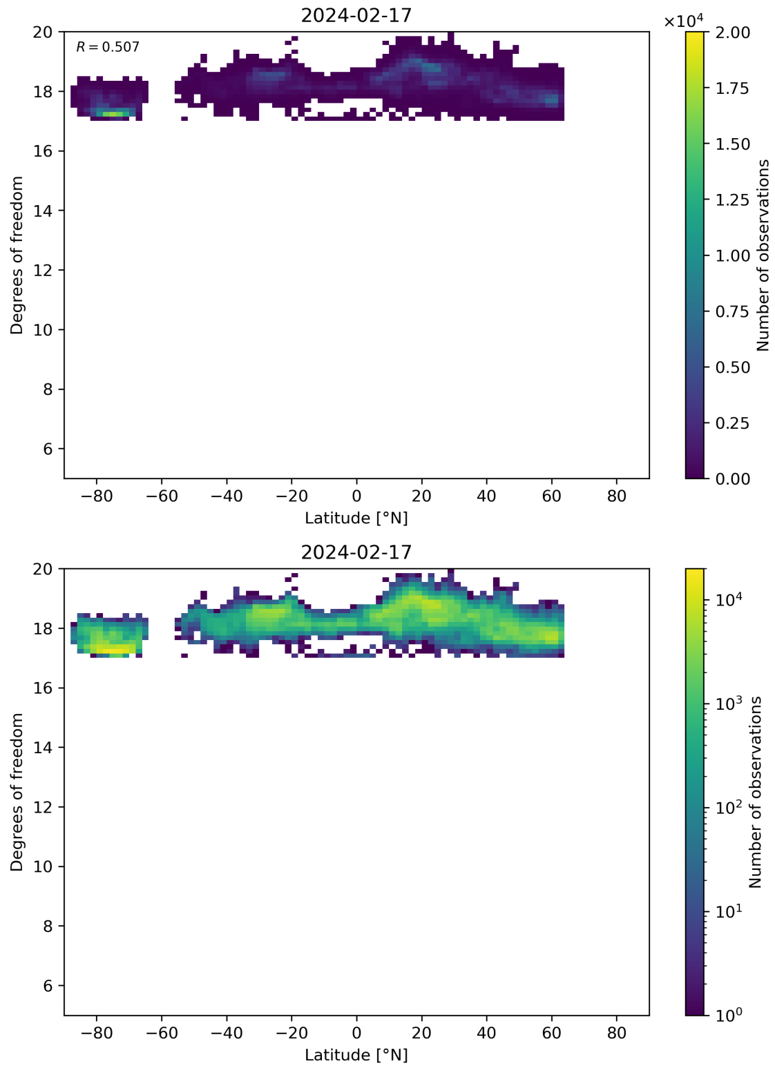
Figure 55: Scatter density plot of “Latitude” against “Degrees of freedom” for 2024-02-17 to 2024-02-18.
