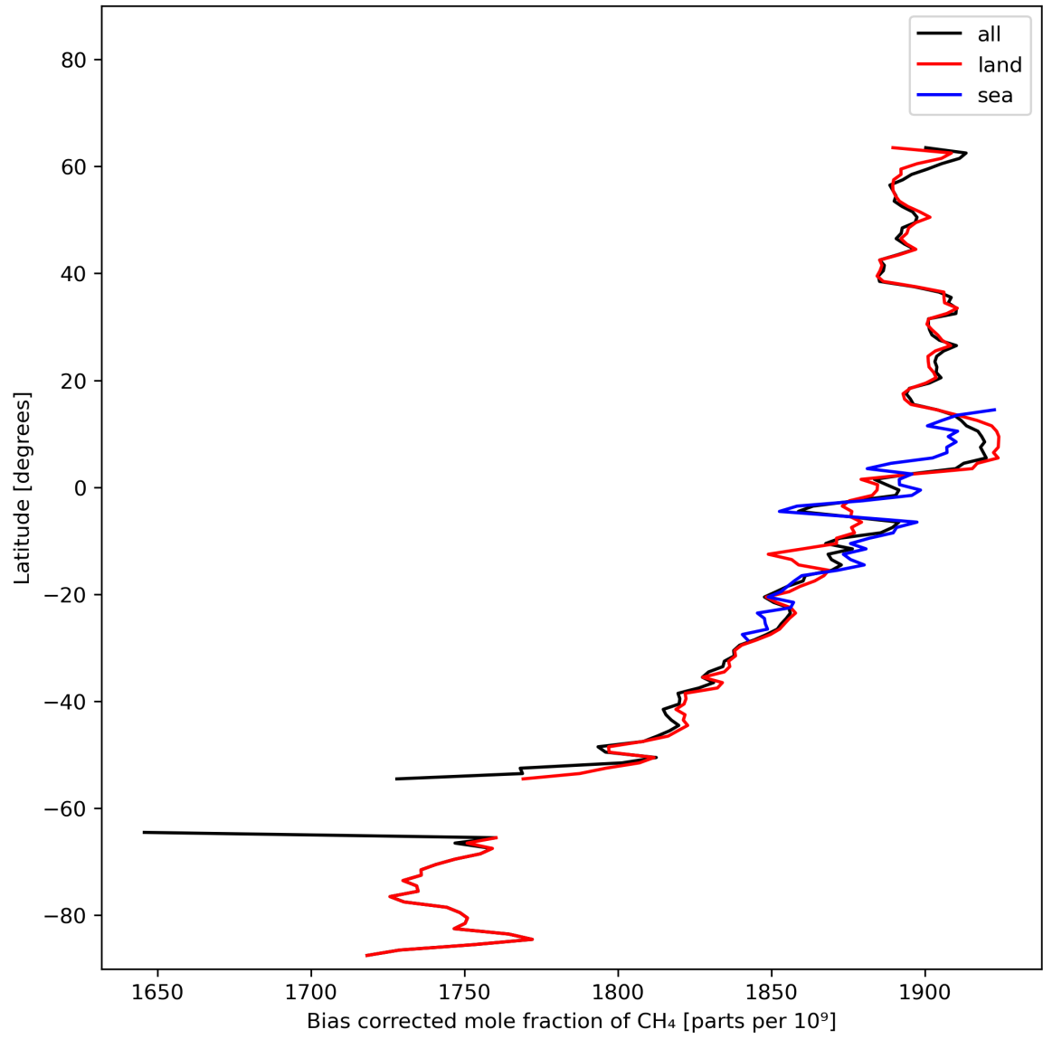
Figure 14: Zonal average of “Bias corrected mole fraction of CH 4 ” for 2024-02-17 to 2024-02-18.
