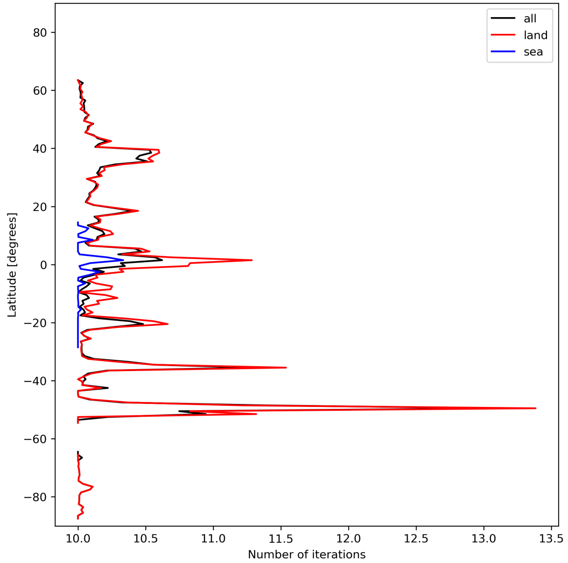
Figure 20: Zonal average of “Number of iterations” for 2024-02-17 to 2024-02-18.
