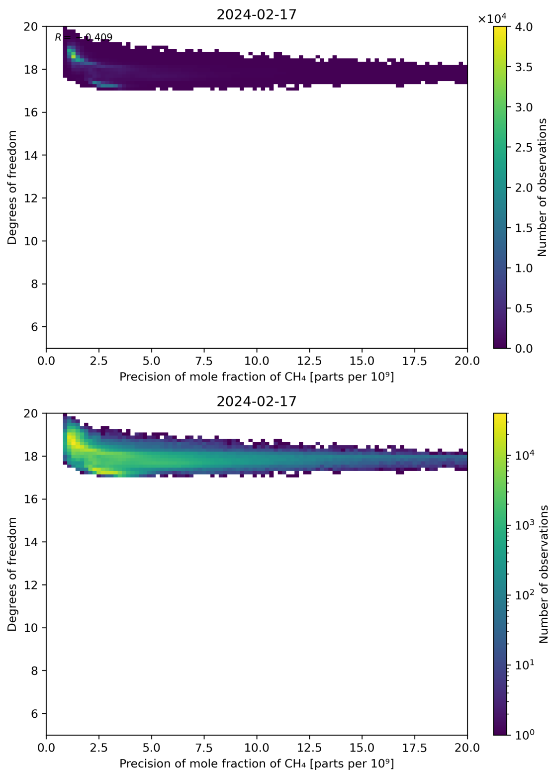
Figure 80: Scatter density plot of “Precision of mole fraction of CH 4 ” against “Degrees of freedom” for 2024-02-17 to 2024-02-18.
