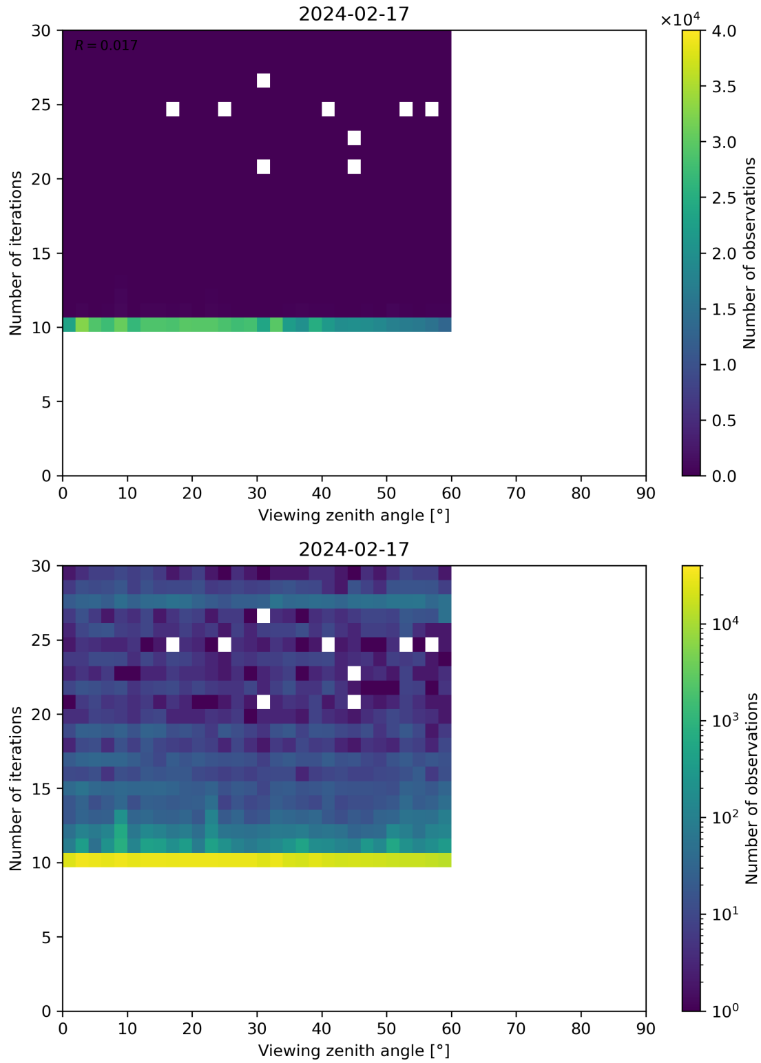
Figure 113: Scatter density plot of “Viewing zenith angle” against “Number of iterations” for 2024-02-17 to 2024-02-18.
