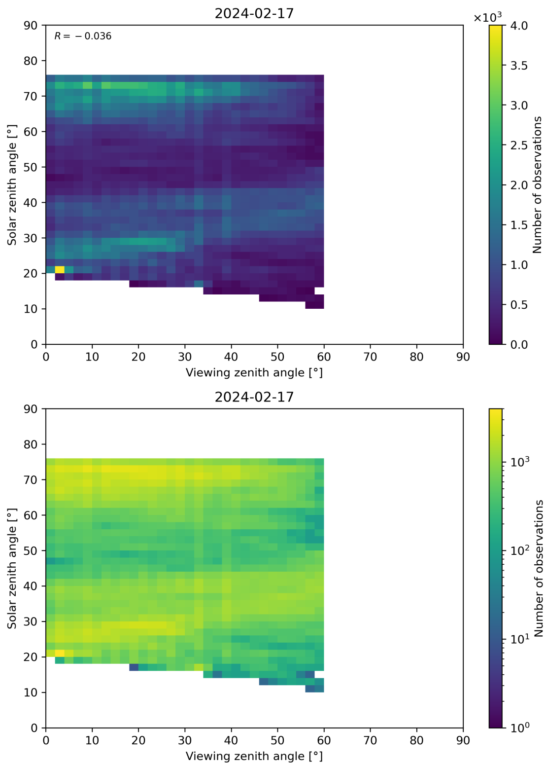
Figure 115: Scatter density plot of “Viewing zenith angle” against “Solar zenith angle” for 2024-02-17 to 2024-02-18.
