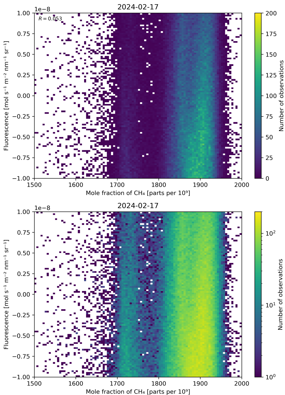
Figure 73: Scatter density plot of “Mole fraction of \text{CH}_4 ” against “Fluorescence” for 2024-02-17 to 2024-02-18.
