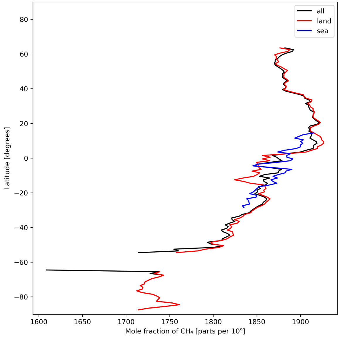
Figure 12: Zonal average of “Mole fraction of \text{CH}_4 ” for 2024-02-17 to 2024-02-18.
