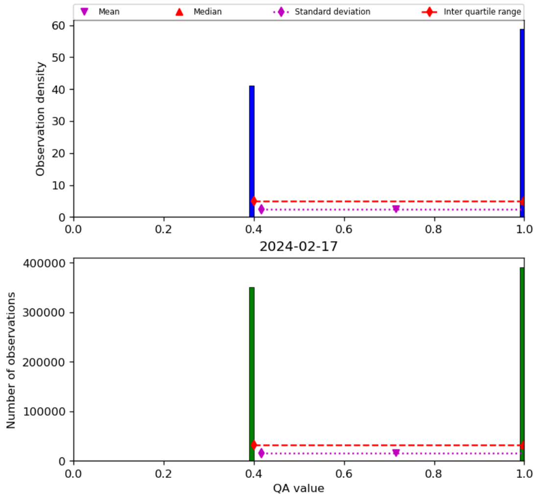
Figure 22: Histogram of “QA value” for 2024-02-17 to 2024-02-18
