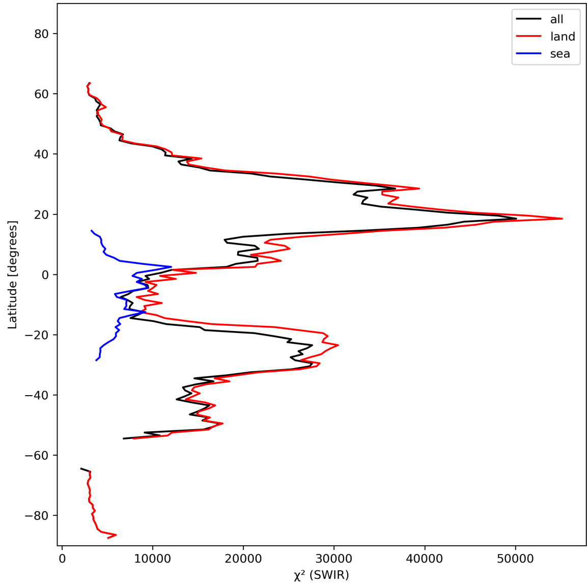
Figure 17: Zonal average of “ \chi^2 (SWIR)” for 2024-02-17 to 2024-02-18.
