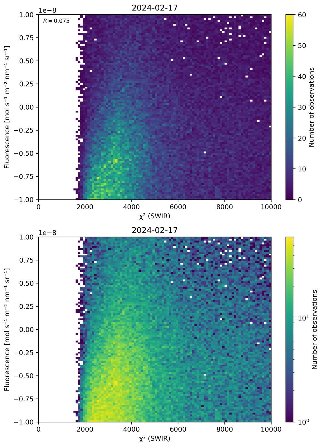
Figure 49: Scatter density plot of “ \chi^2 (SWIR)” against “Fluorescence” for 2024-02-17 to 2024-02-18.
