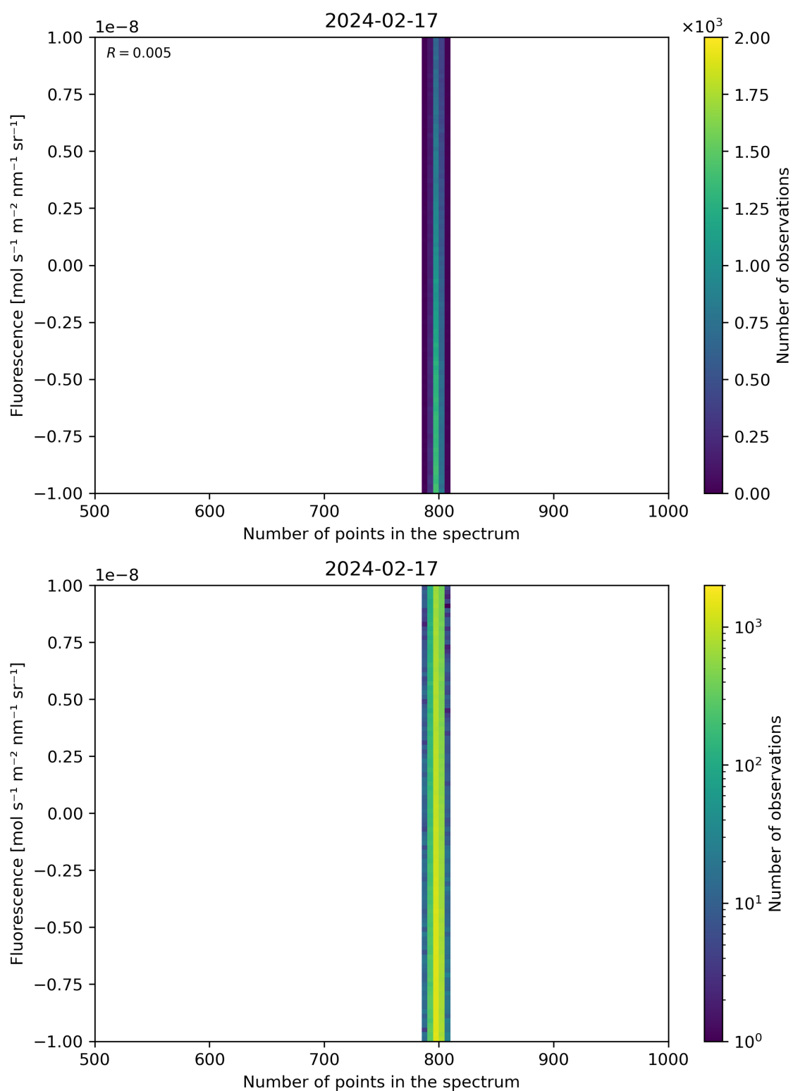
Figure 91: Scatter density plot of “Number of points in the spectrum” against “Fluorescence” for 2024-02-17 to 2024-02-18.
