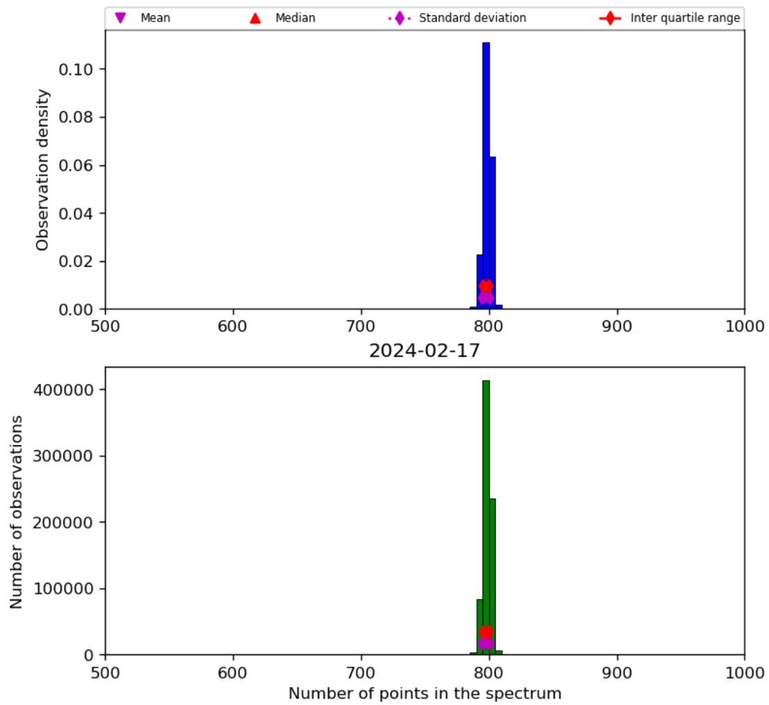
Figure 26: Histogram of “Number of points in the spectrum” for 2024-02-17 to 2024-02-18
