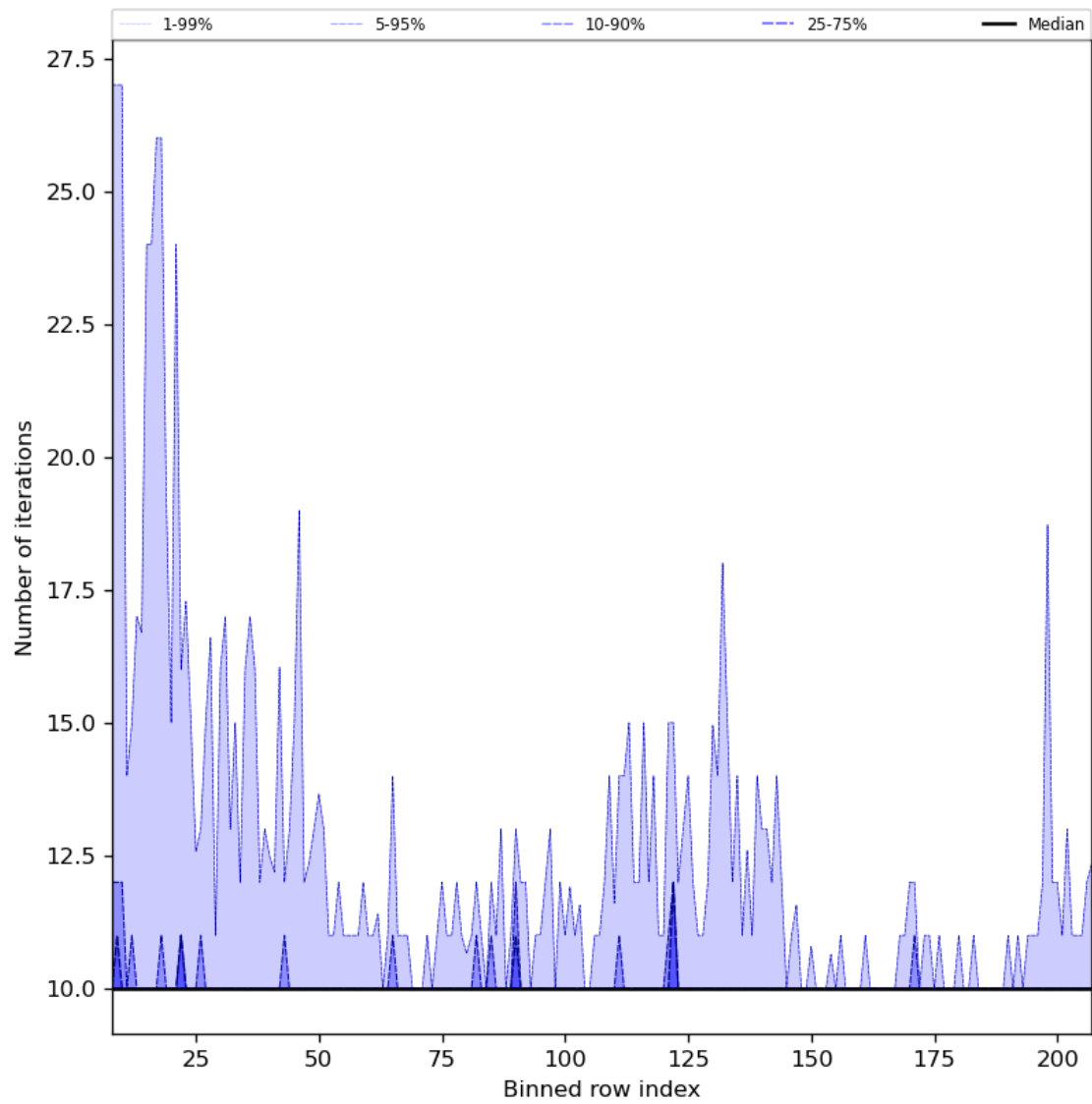
Figure 42: Along track statistics of “Number of iterations” for 2024-02-17 to 2024-02-18
