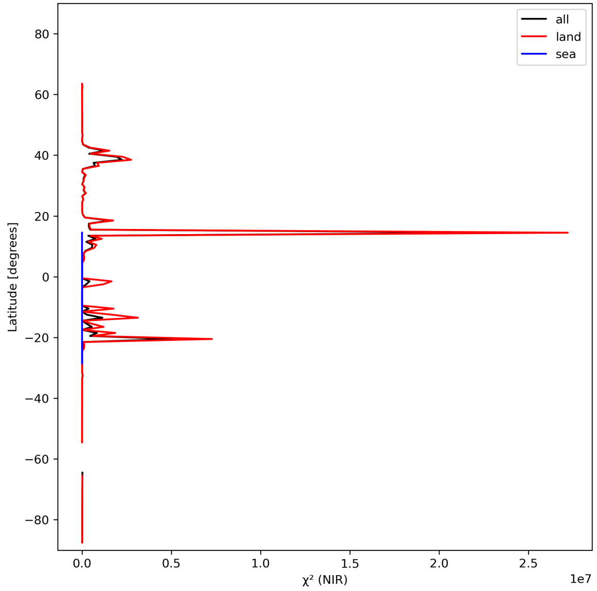
Figure 18: Zonal average of “ \chi^2 (NIR)” for 2024-02-17 to 2024-02-18.
