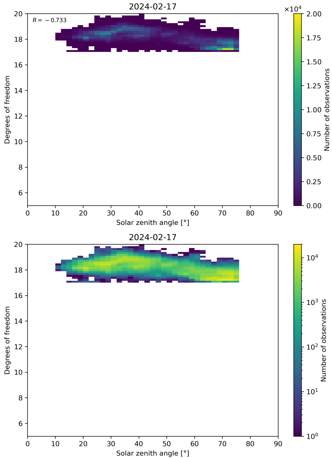
Figure 96: Scatter density plot of “Solar zenith angle” against “Degrees of freedom” for 2024-02-17 to 2024-02-18.
