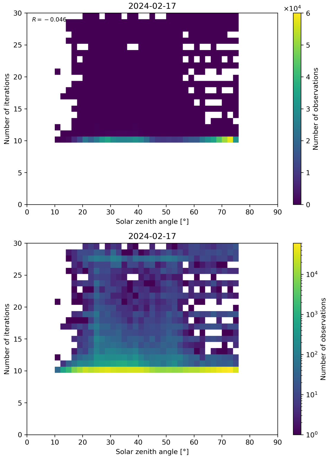
Figure 102: Scatter density plot of “Solar zenith angle” against “Number of iterations” for 2024-02-17 to 2024-02-18.
