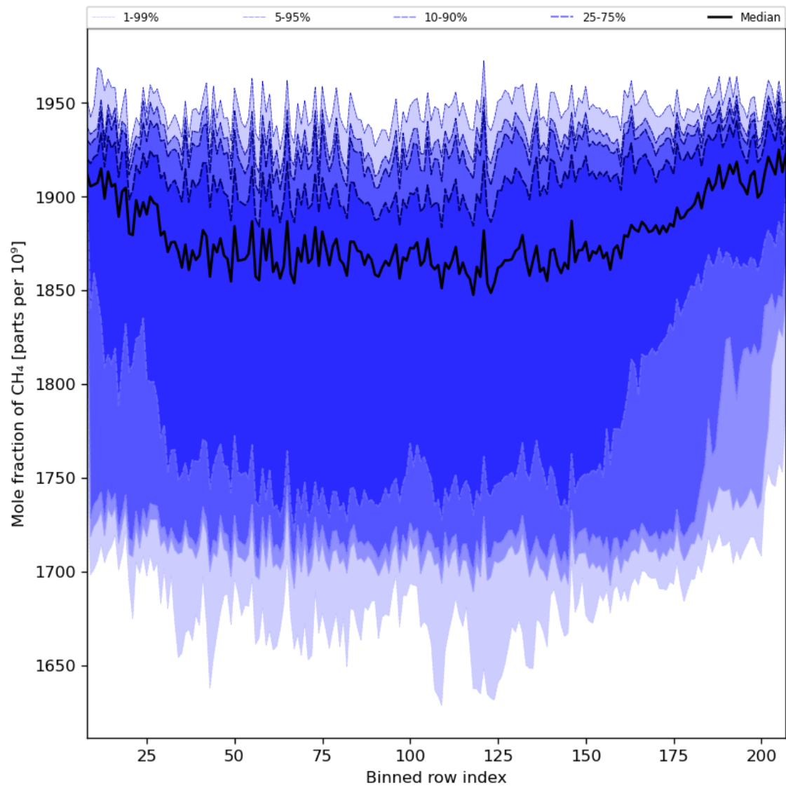
Figure 34: Along track statistics of “Mole fraction of CH 4 ” for 2024-02-17 to 2024-02-18
