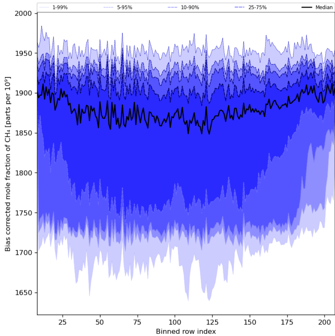
Figure 36: Along track statistics of “Bias corrected mole fraction of CH 4 ” for 2024-02-17 to 2024-02-18
