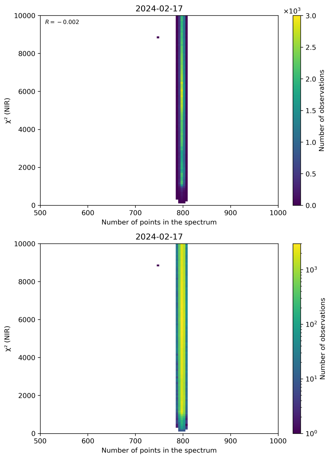
Figure 88: Scatter density plot of “Number of points in the spectrum” against “ \chi^2 (NIR)” for 2024-02-17 to 2024-02-18.
