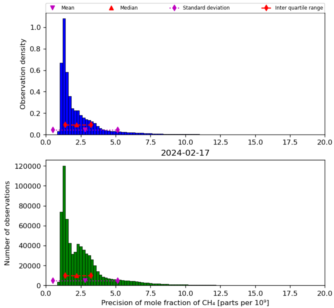
Figure 24: Histogram of “Precision of mole fraction of CH 4 ” for 2024-02-17 to 2024-02-18
