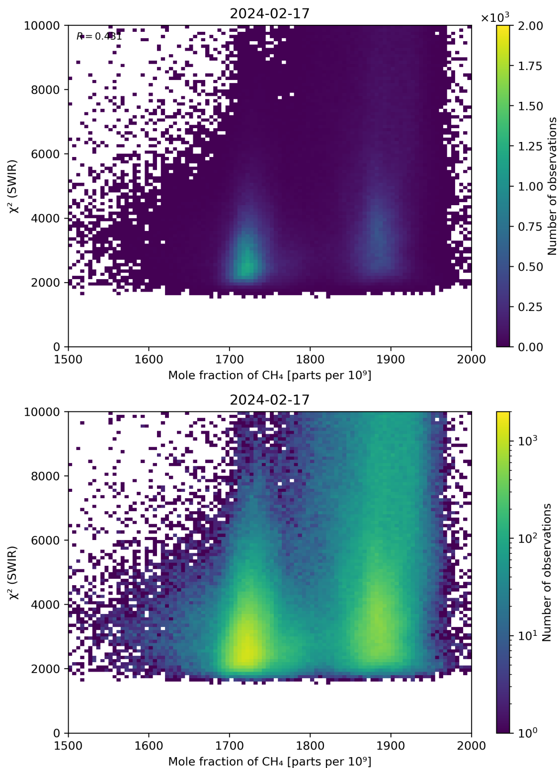
Figure 71: Scatter density plot of “Mole fraction of \text{CH}_4 ” against “ \chi^2 (SWIR)” for 2024-02-17 to 2024-02-18.
