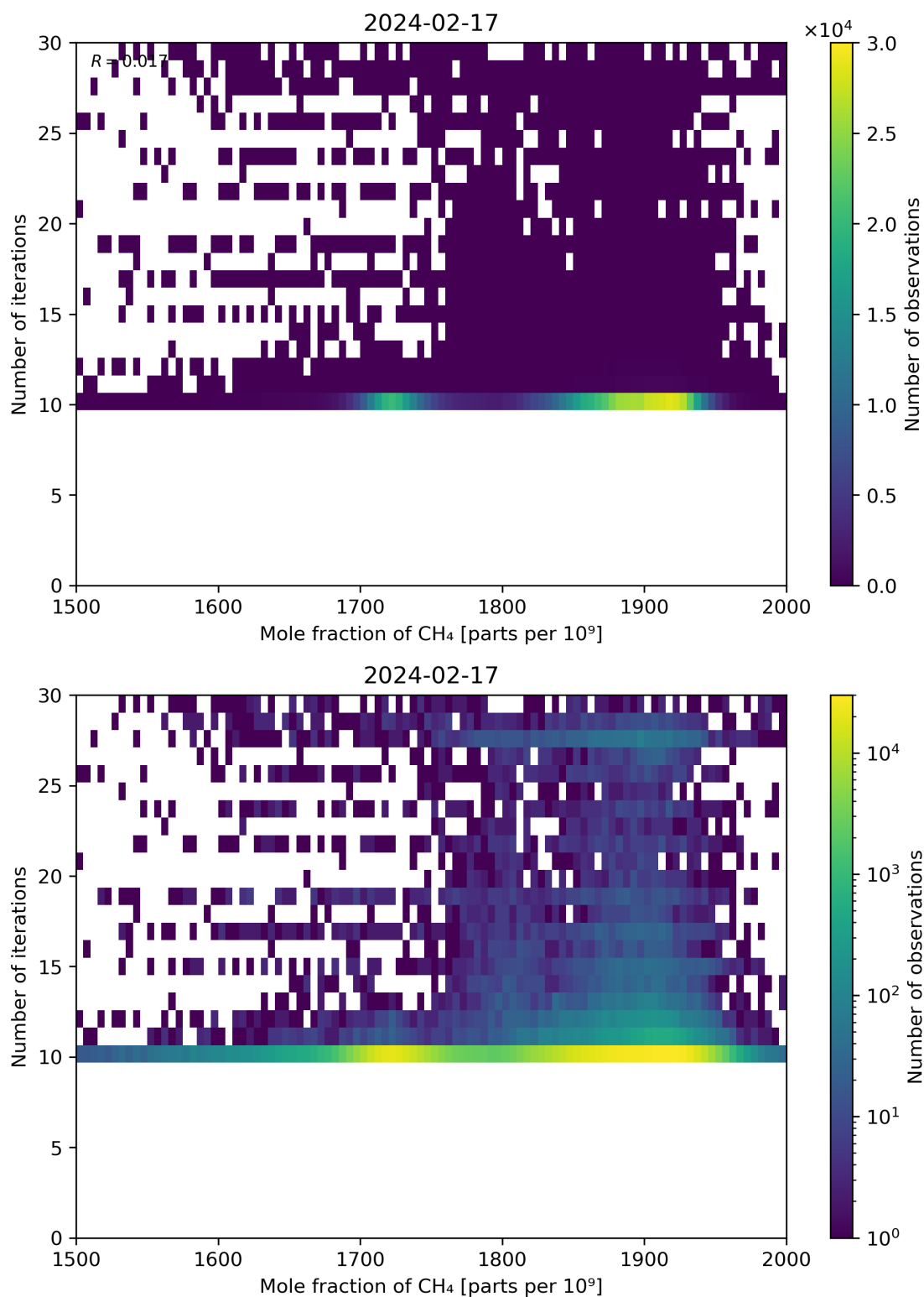
Figure 76: Scatter density plot of “Mole fraction of CH 4 ” against “Number of iterations” for 2024-02-17 to 2024-02-18.
