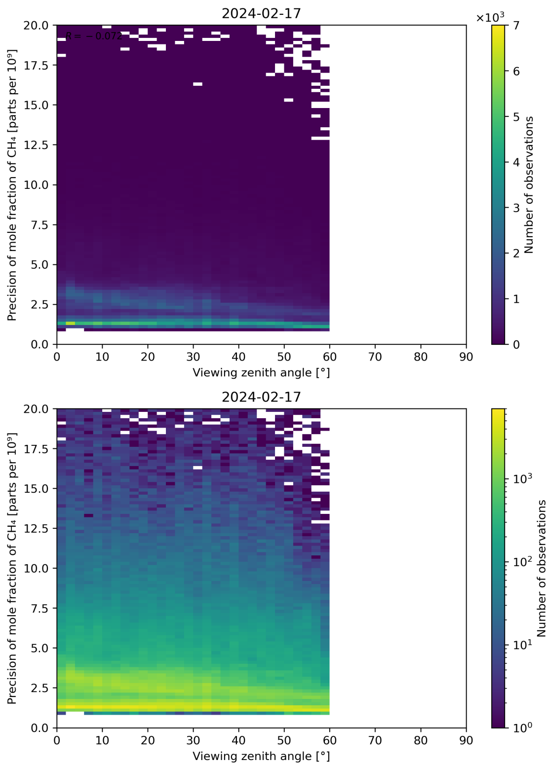
Figure 112: Scatter density plot of “Viewing zenith angle” against “Precision of mole fraction of CH 4 ” for 2024-02-17 to 2024-02-18.
