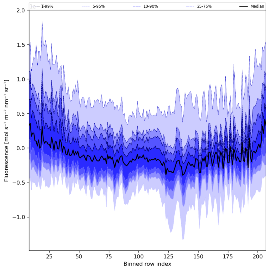
Figure 43: Along track statistics of “Fluorescence” for 2024-02-17 to 2024-02-18
