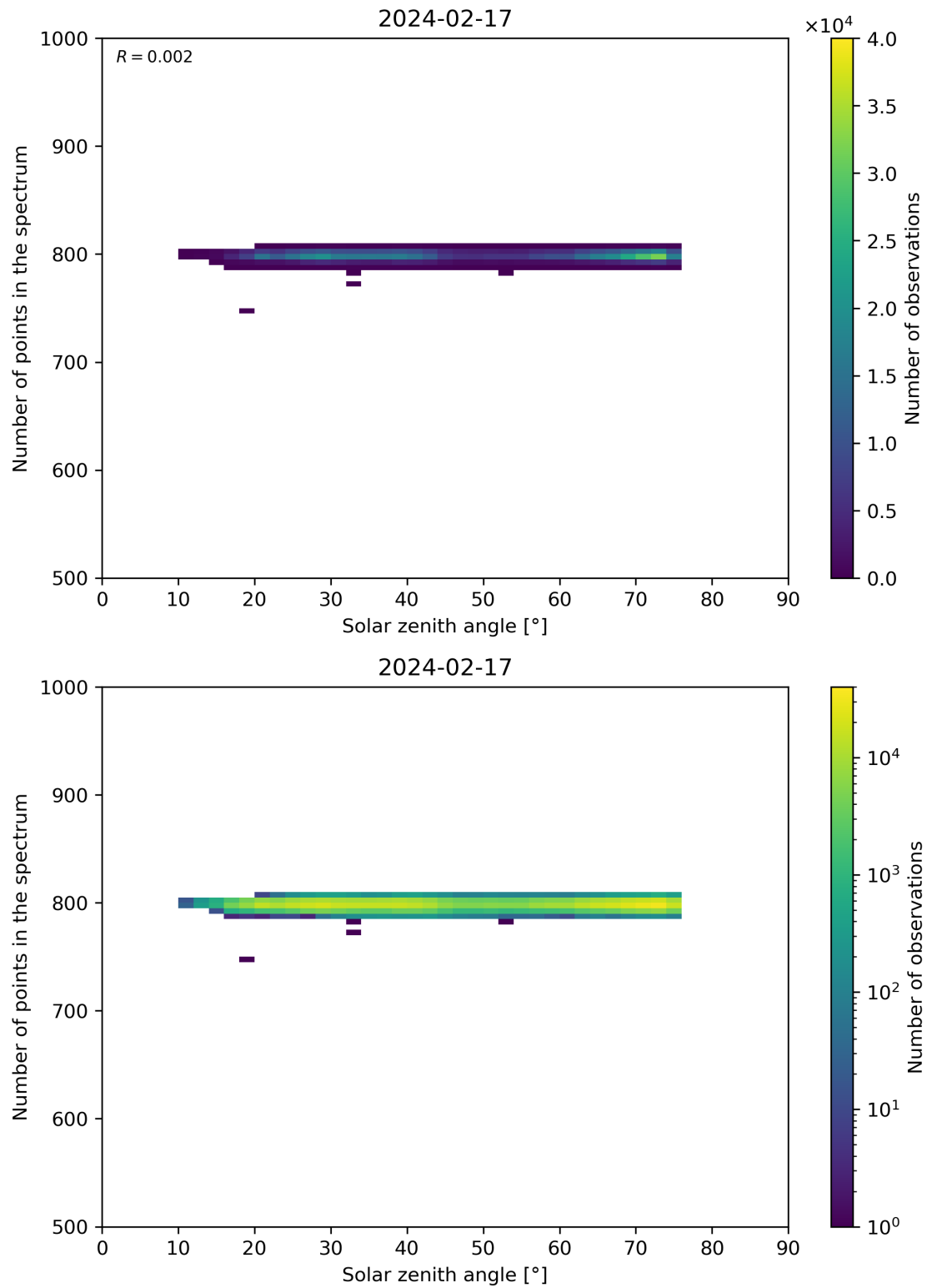
Figure 103: Scatter density plot of “Solar zenith angle” against “Number of points in the spectrum” for 2024-02-17 to 2024-02-18.
