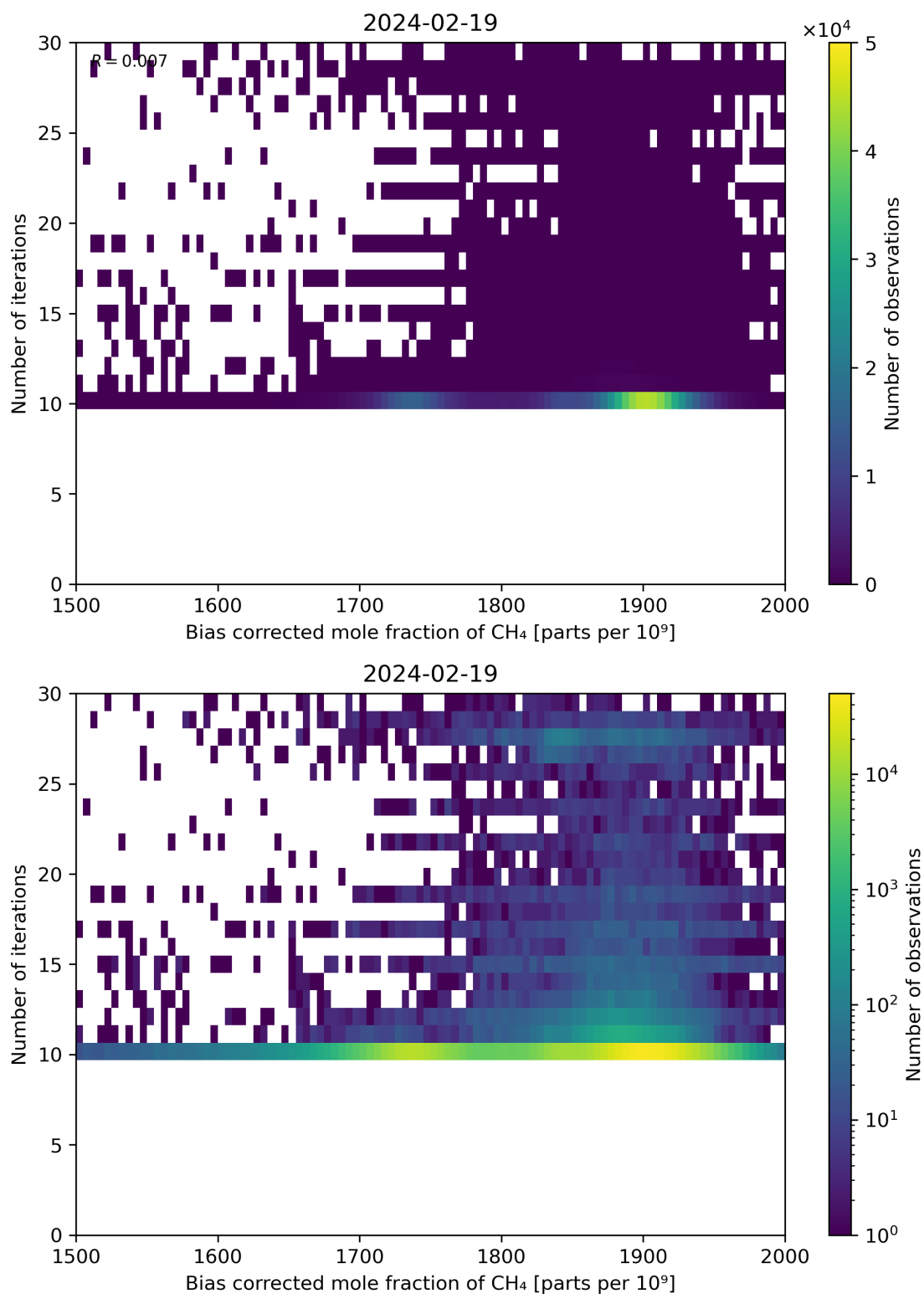
Figure 67: Scatter density plot of “Bias corrected mole fraction of \text{CH}_4 ” against “Number of iterations” for 2024-02-18 to 2024-02-20.
