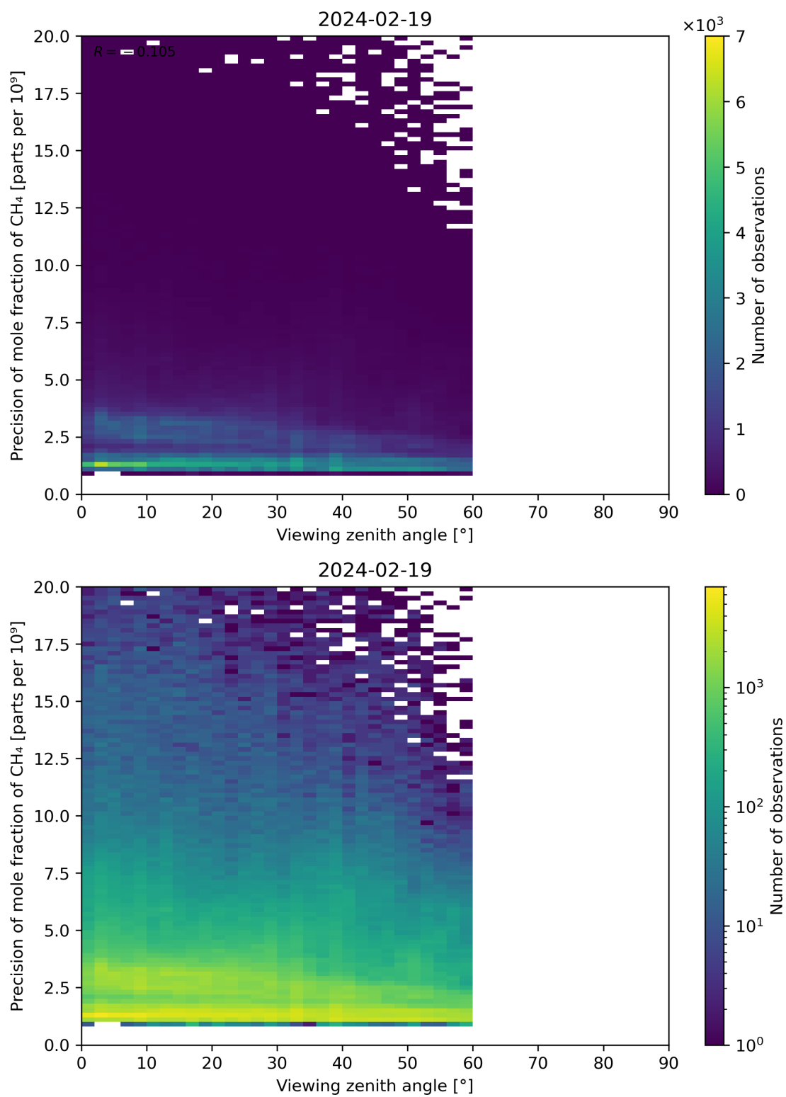
Figure 112: Scatter density plot of “Viewing zenith angle” against “Precision of mole fraction of CH 4 ” for 2024-02-18 to 2024-02-20.
