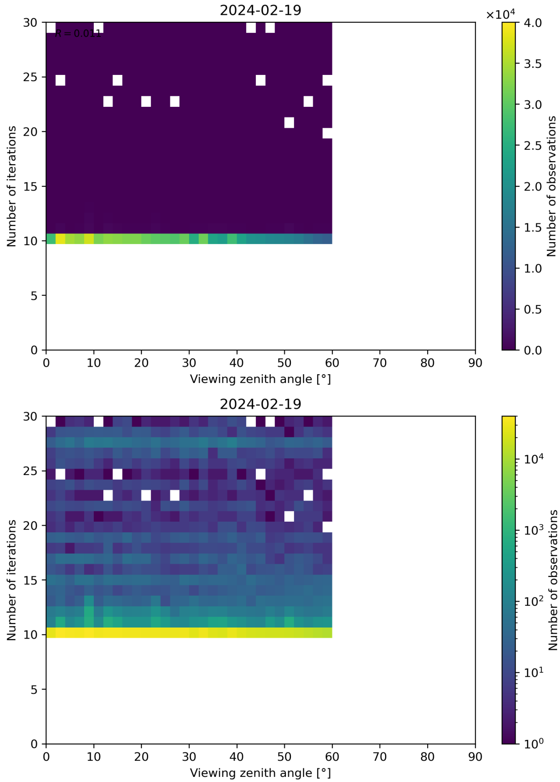
Figure 113: Scatter density plot of “Viewing zenith angle” against “Number of iterations” for 2024-02-18 to 2024-02-20.
