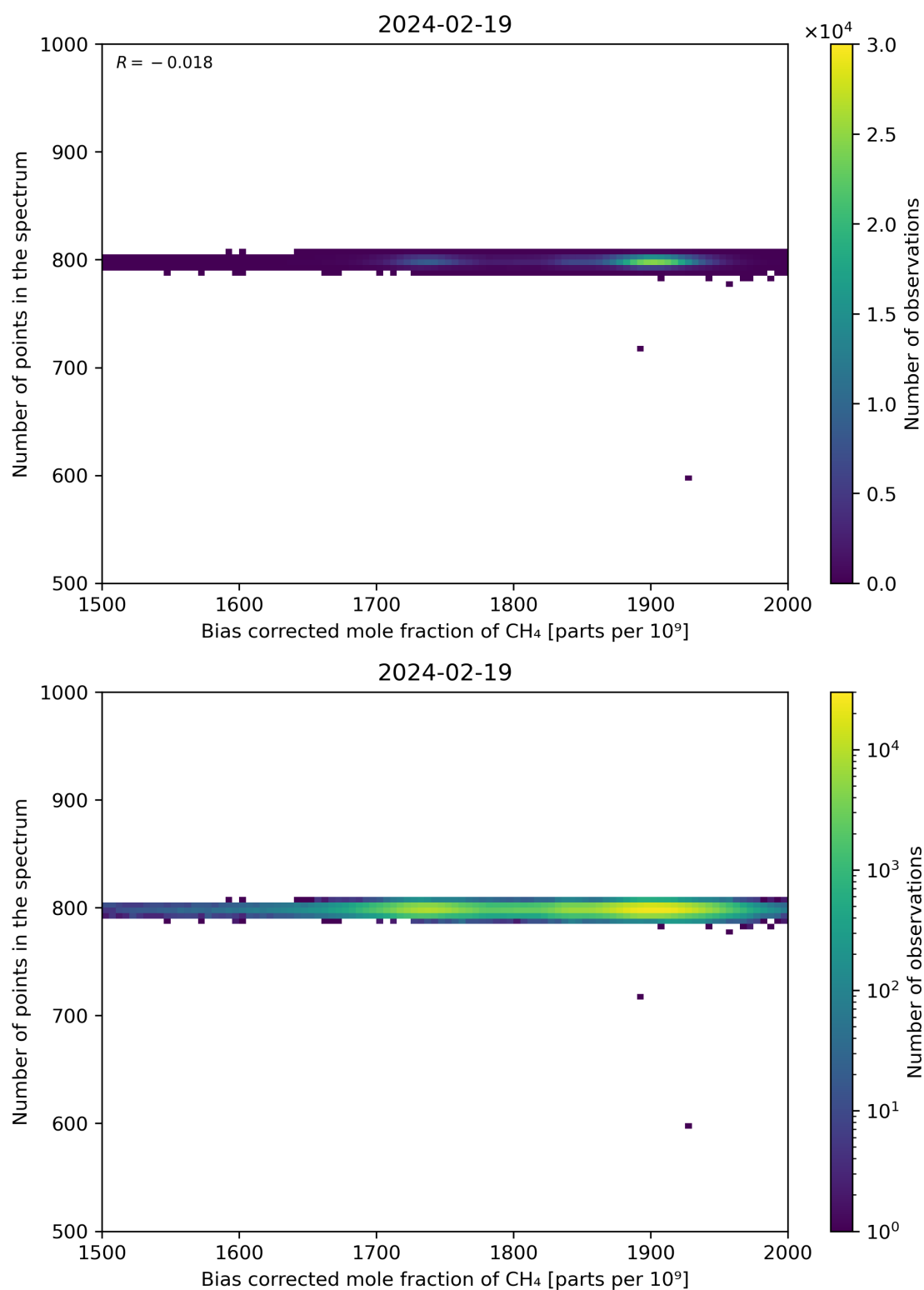
Figure 68: Scatter density plot of “Bias corrected mole fraction of CH 4 ” against “Number of points in the spectrum” for 2024-02-18 to 2024-02-20.
