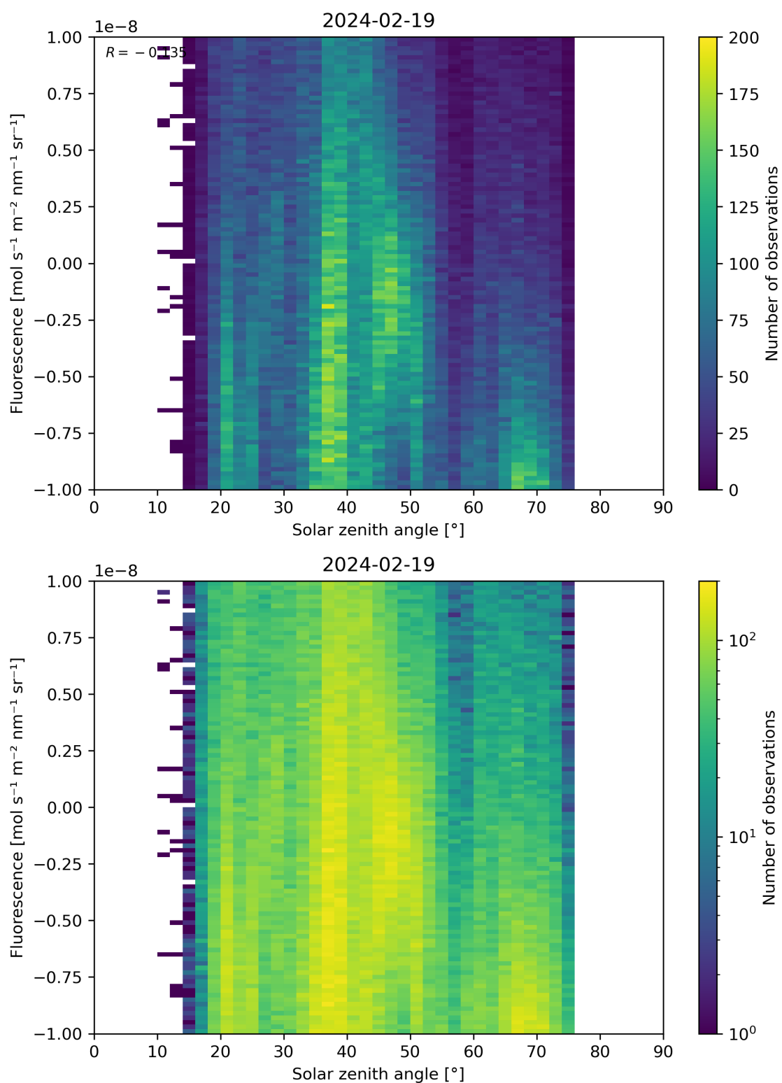
Figure 97: Scatter density plot of “Solar zenith angle” against “Fluorescence” for 2024-02-18 to 2024-02-20.
