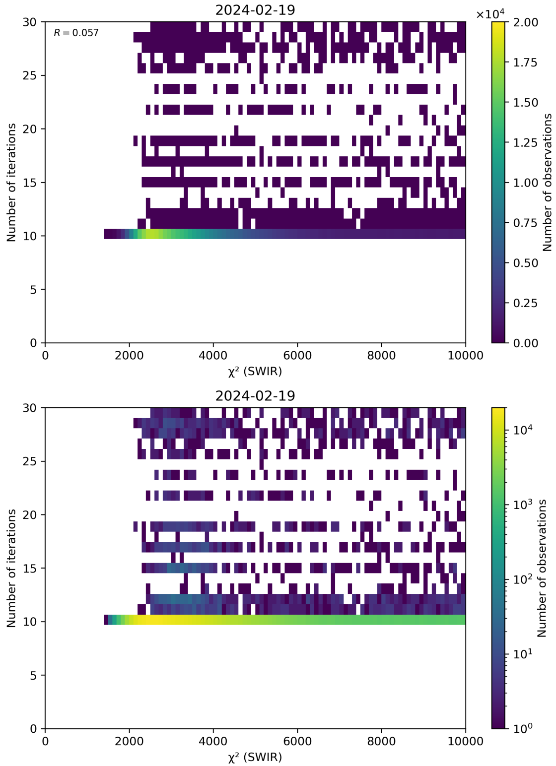
Figure 50: Scatter density plot of “ \chi^2 (SWIR)” against “Number of iterations” for 2024-02-18 to 2024-02-20.
