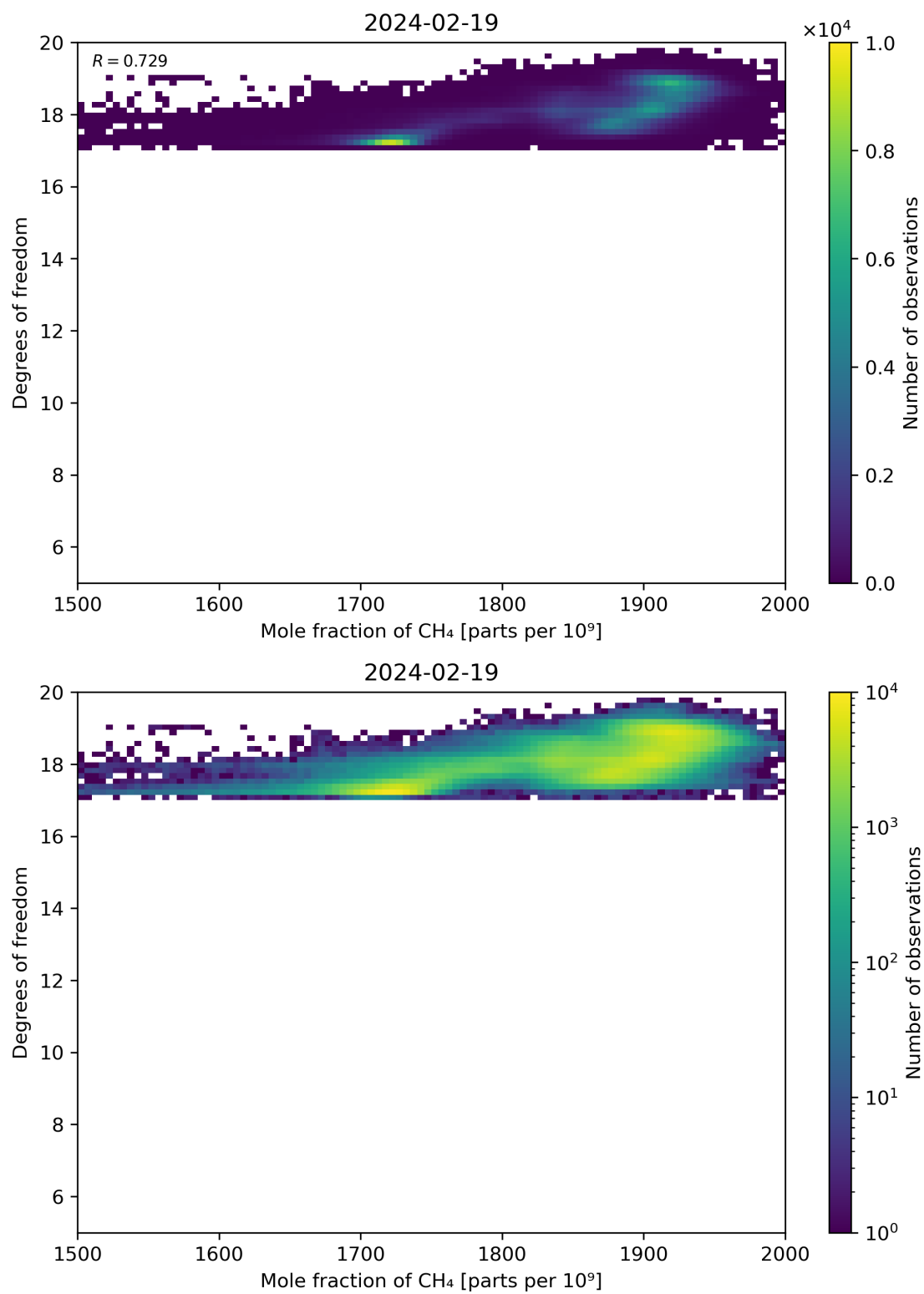
Figure 72: Scatter density plot of “Mole fraction of CH 4 ” against “Degrees of freedom” for 2024-02-18 to 2024-02-20.
