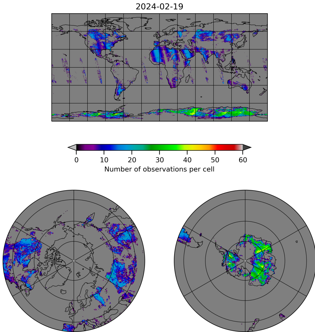
Figure 10: Map of the number of observations for 2024-02-18 to 2024-02-20
