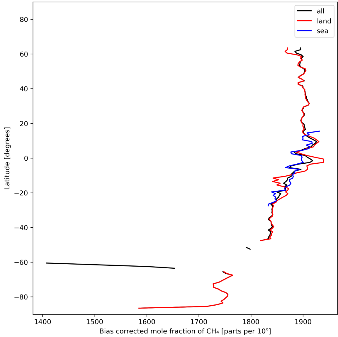
Figure 14: Zonal average of “Bias corrected mole fraction of CH 4 ” for 2024-02-18 to 2024-02-20.
