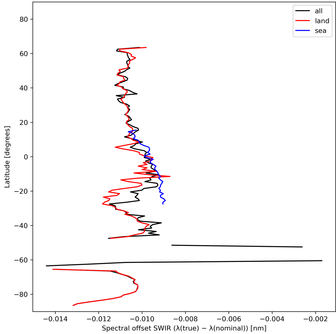
Figure 16: Zonal average of “Spectral offset SWIR ( \lambda(\text{true}) - \lambda(\text{nominal}) )” for 2024-02-18 to 2024-02-20.
