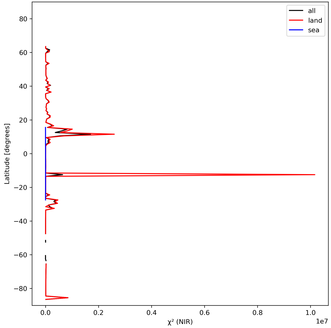
Figure 18: Zonal average of “ \chi^2 (NIR)” for 2024-02-18 to 2024-02-20.
