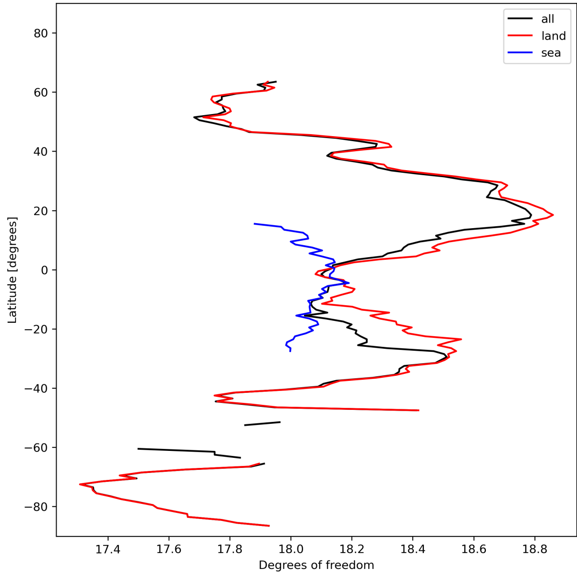
Figure 19: Zonal average of “Degrees of freedom” for 2024-02-18 to 2024-02-20.
