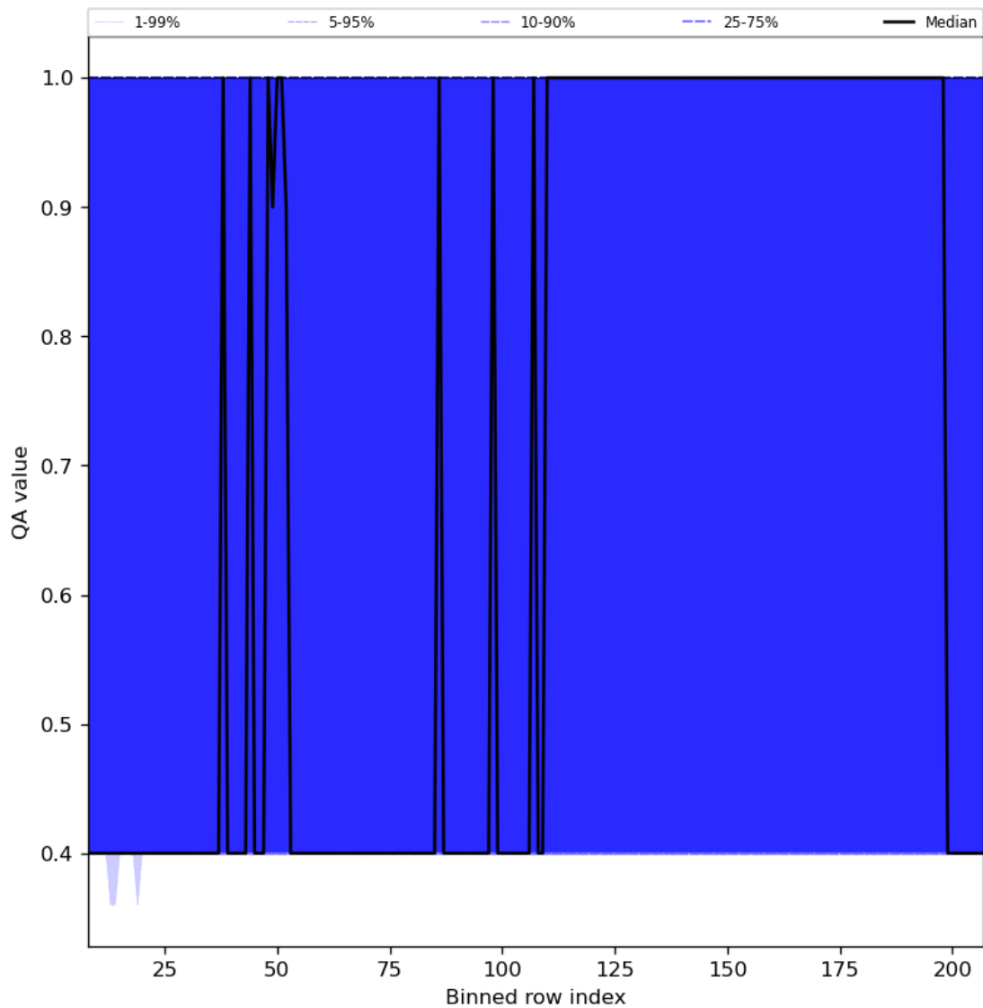
Figure 33: Along track statistics of “QA value” for 2024-02-18 to 2024-02-20
