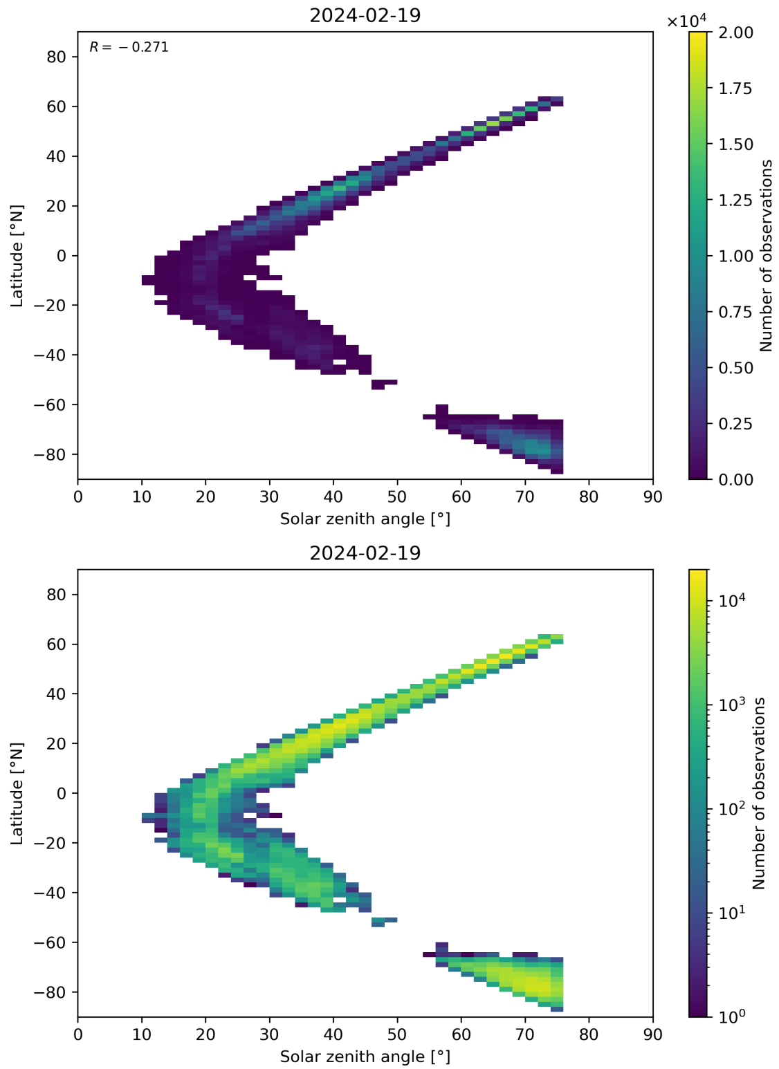
Figure 98: Scatter density plot of “Solar zenith angle” against “Latitude” for 2024-02-18 to 2024-02-20.
