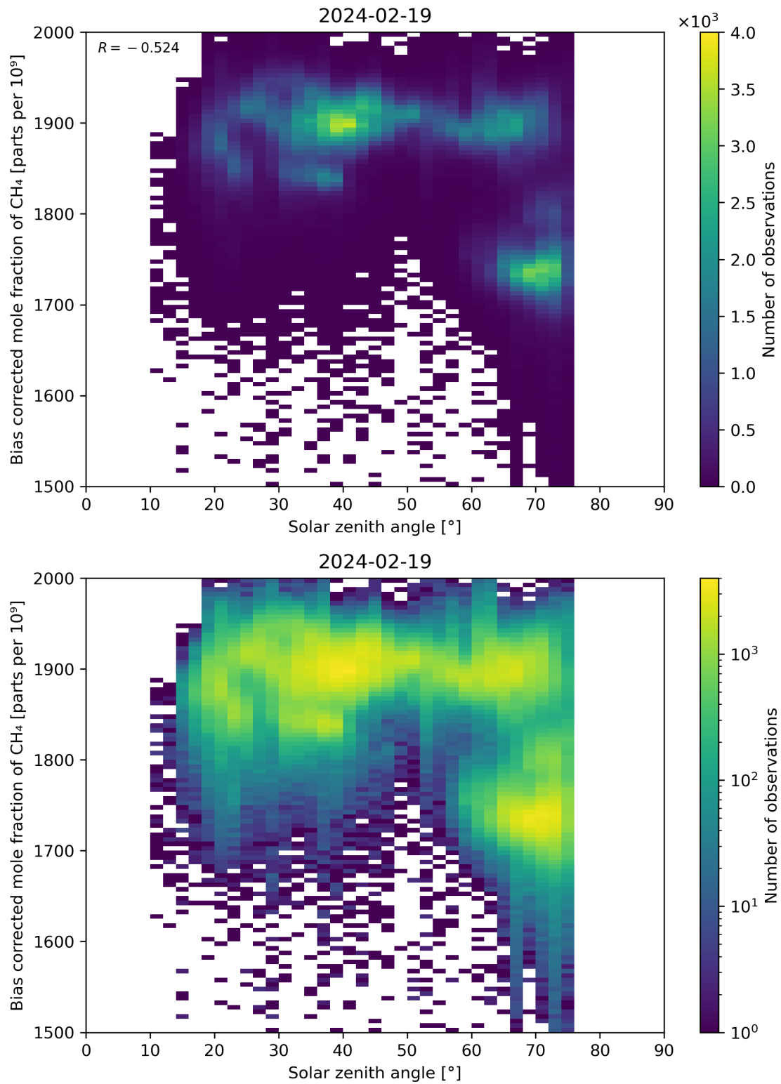
Figure 100: Scatter density plot of “Solar zenith angle” against “Bias corrected mole fraction of \text{CH}_4 ” for 2024-02-18 to 2024-02-20.
