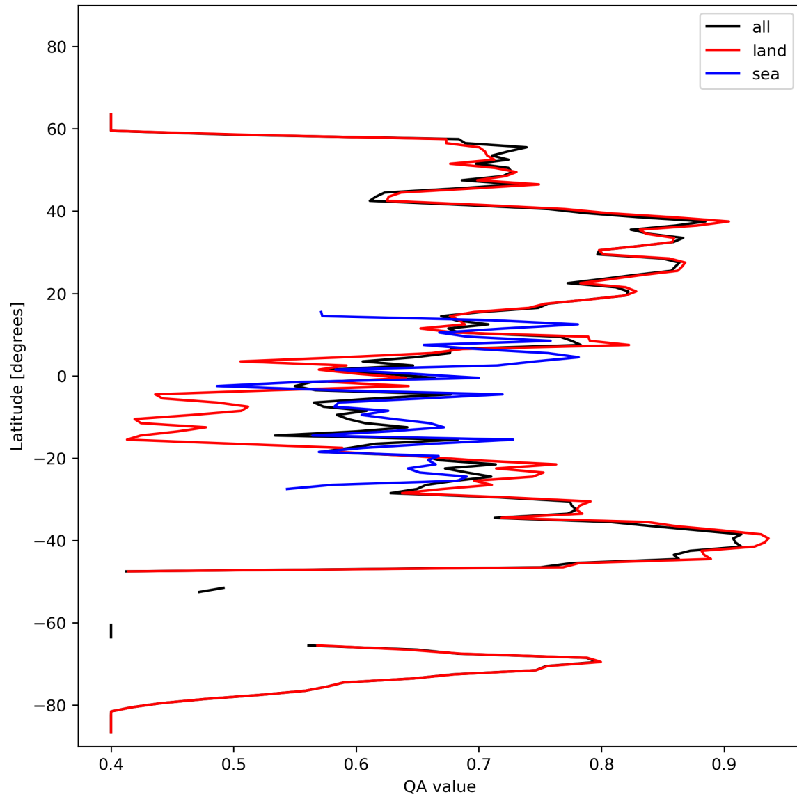
Figure 11: Zonal average of “QA value” for 2024-02-18 to 2024-02-20.
