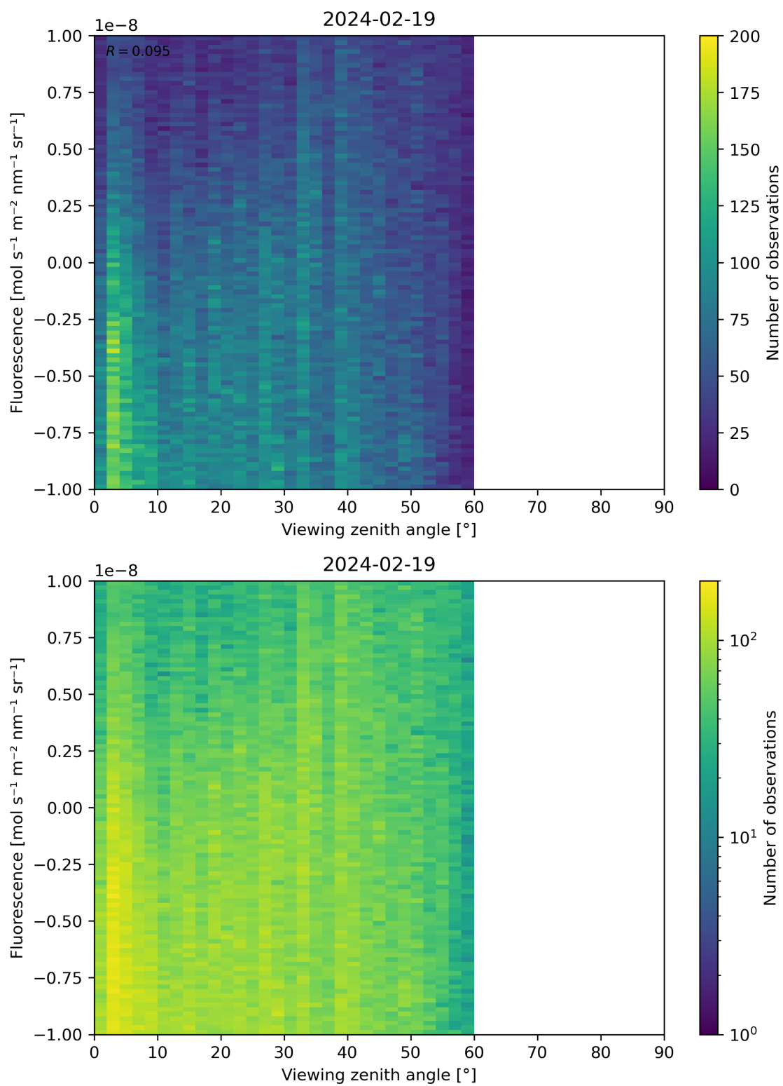
Figure 108: Scatter density plot of “Viewing zenith angle” against “Fluorescence” for 2024-02-18 to 2024-02-20.
