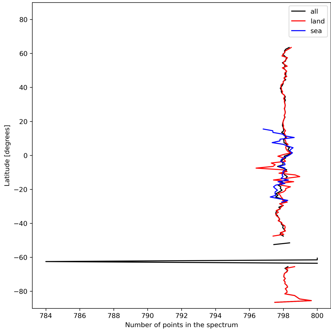
Figure 15: Zonal average of “Number of points in the spectrum” for 2024-02-18 to 2024-02-20.
