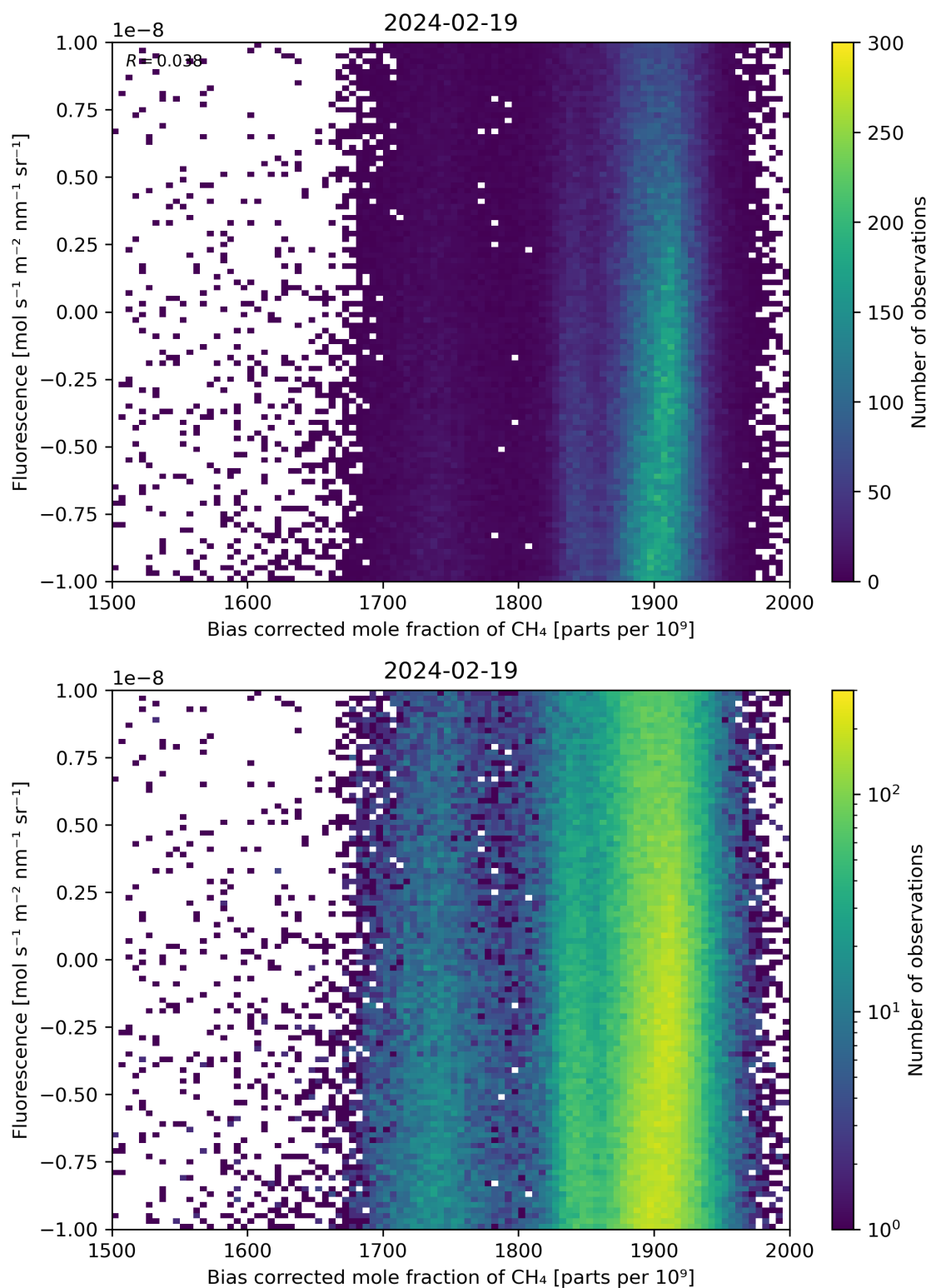
Figure 66: Scatter density plot of “Bias corrected mole fraction of \text{CH}_4 ” against “Fluorescence” for 2024-02-18 to 2024-02-20.
