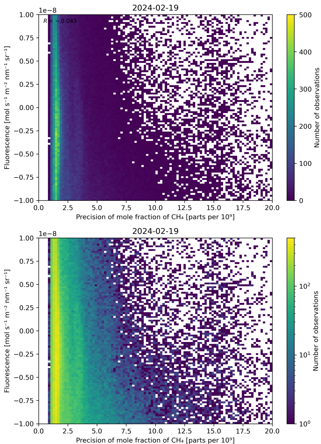
Figure 81: Scatter density plot of “Precision of mole fraction of \text{CH}_4 ” against “Fluorescence” for 2024-02-18 to 2024-02-20.
