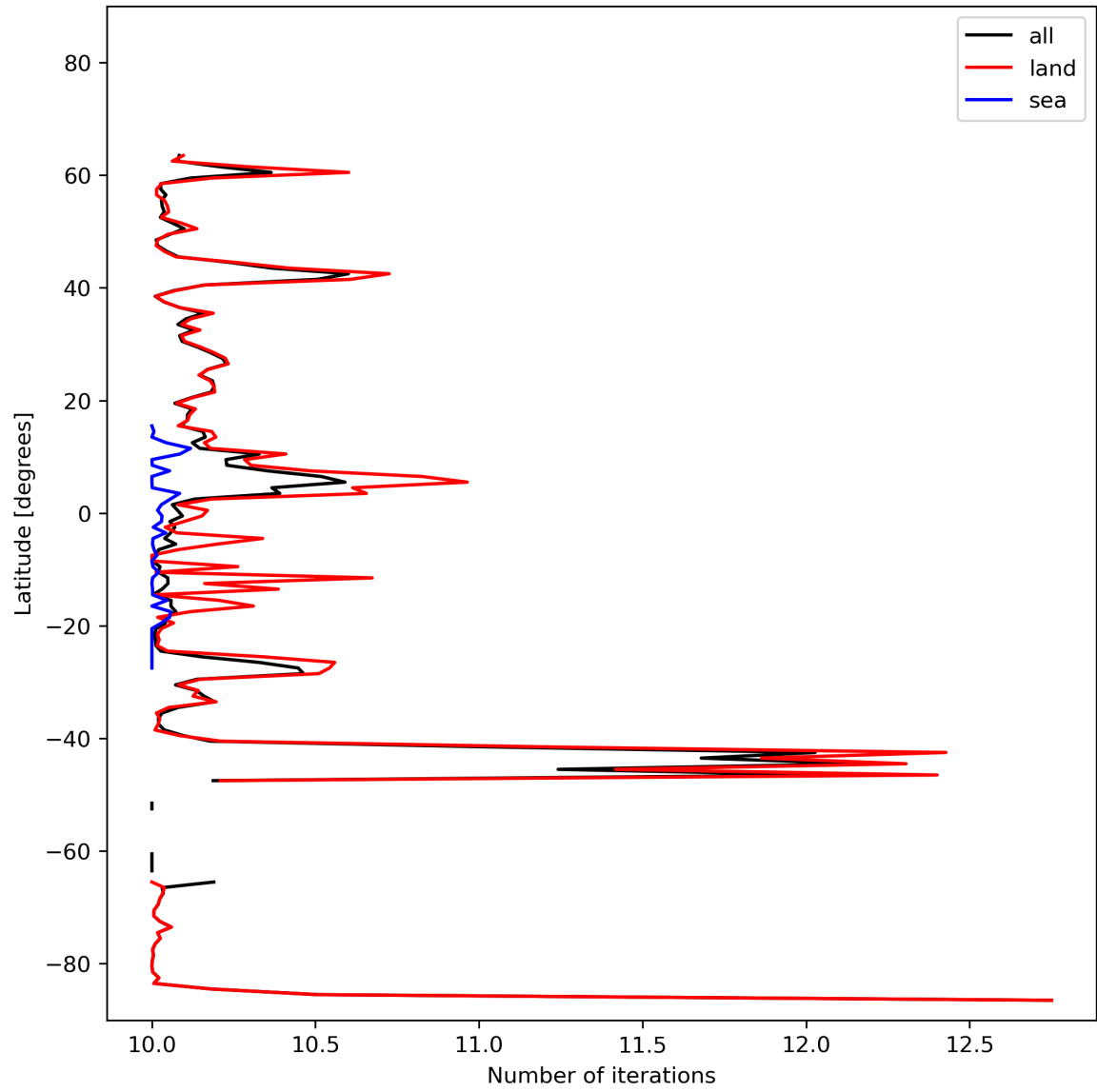
Figure 20: Zonal average of “Number of iterations” for 2024-02-18 to 2024-02-20.
