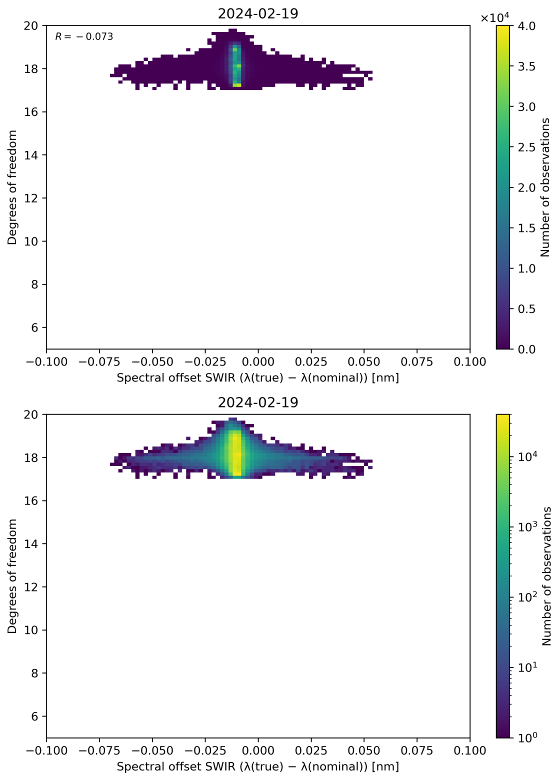
Figure 119: Scatter density plot of “Spectral offset SWIR ( \lambda(\text{true}) - \lambda(\text{nominal}) )” against “Degrees of freedom” for 2024-02-18 to 2024-02-20.
