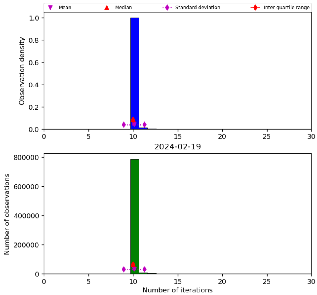
Figure 31: Histogram of "Number of iterations" for 2024-02-18 to 2024-02-20
