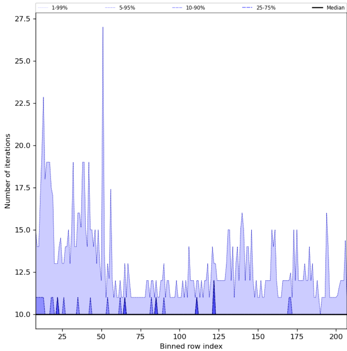
Figure 42: Along track statistics of “Number of iterations” for 2024-02-18 to 2024-02-20
