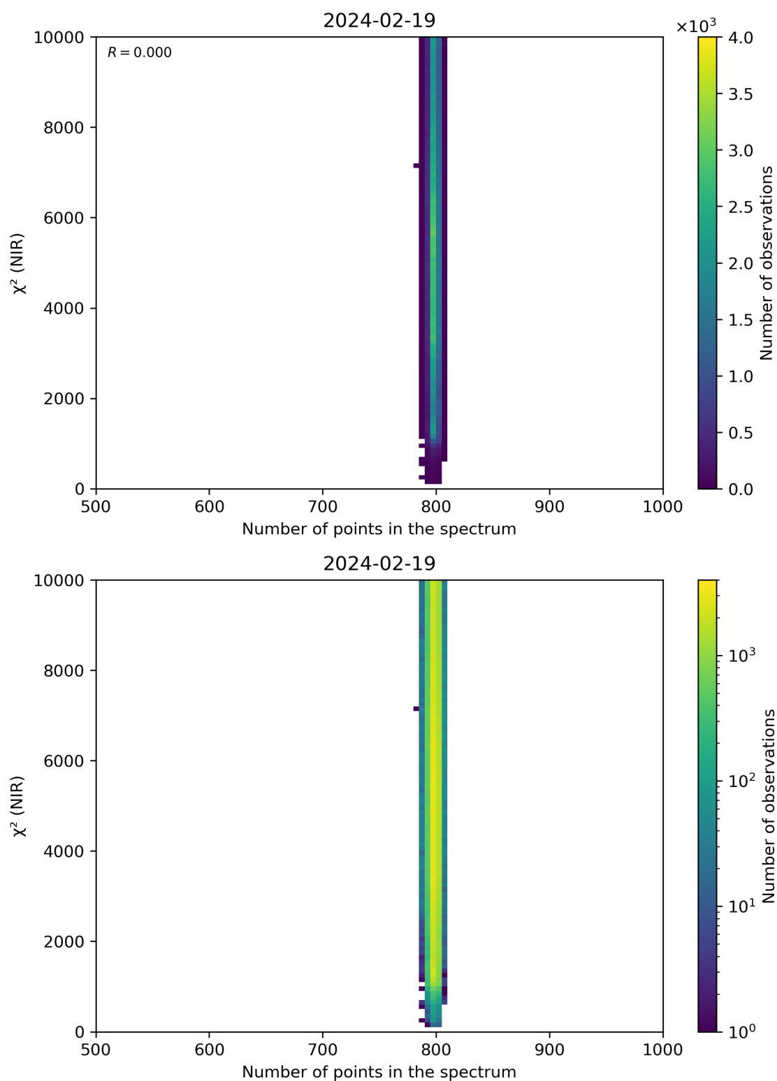
Figure 88: Scatter density plot of “Number of points in the spectrum” against “ \chi^2 (NIR)” for 2024-02-18 to 2024-02-20.
