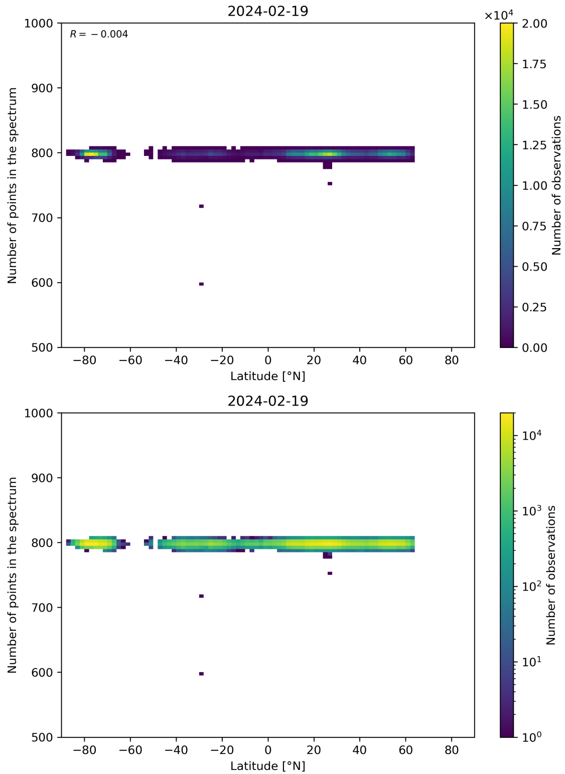
Figure 61: Scatter density plot of “Latitude” against “Number of points in the spectrum” for 2024-02-18 to 2024-02-20.
