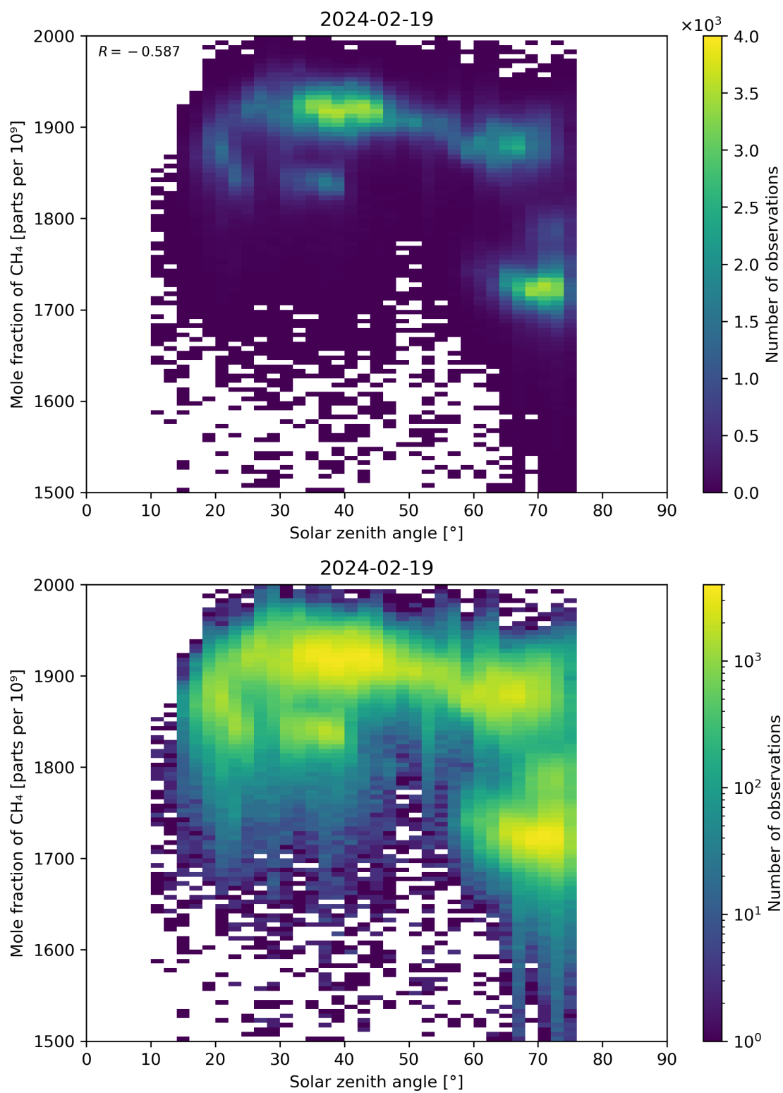
Figure 99: Scatter density plot of “Solar zenith angle” against “Mole fraction of CH 4 ” for 2024-02-18 to 2024-02-20.
