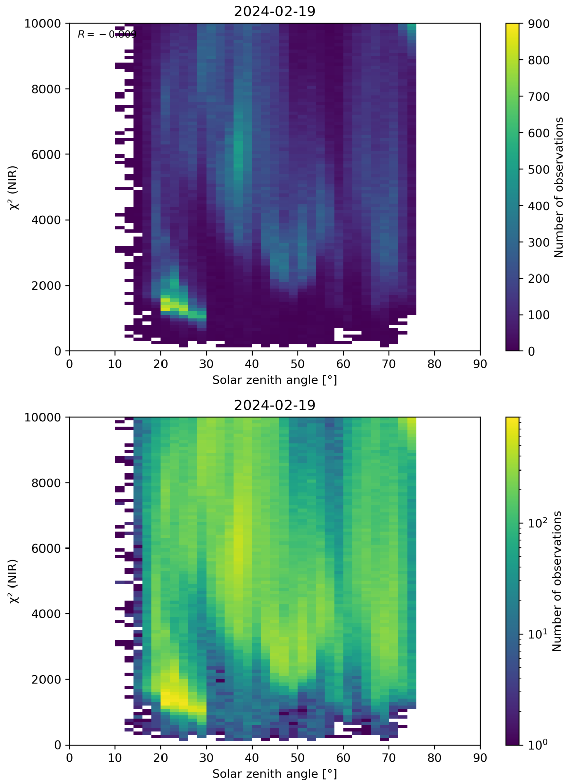
Figure 94: Scatter density plot of “Solar zenith angle” against “ \chi^2 (NIR)” for 2024-02-18 to 2024-02-20.
