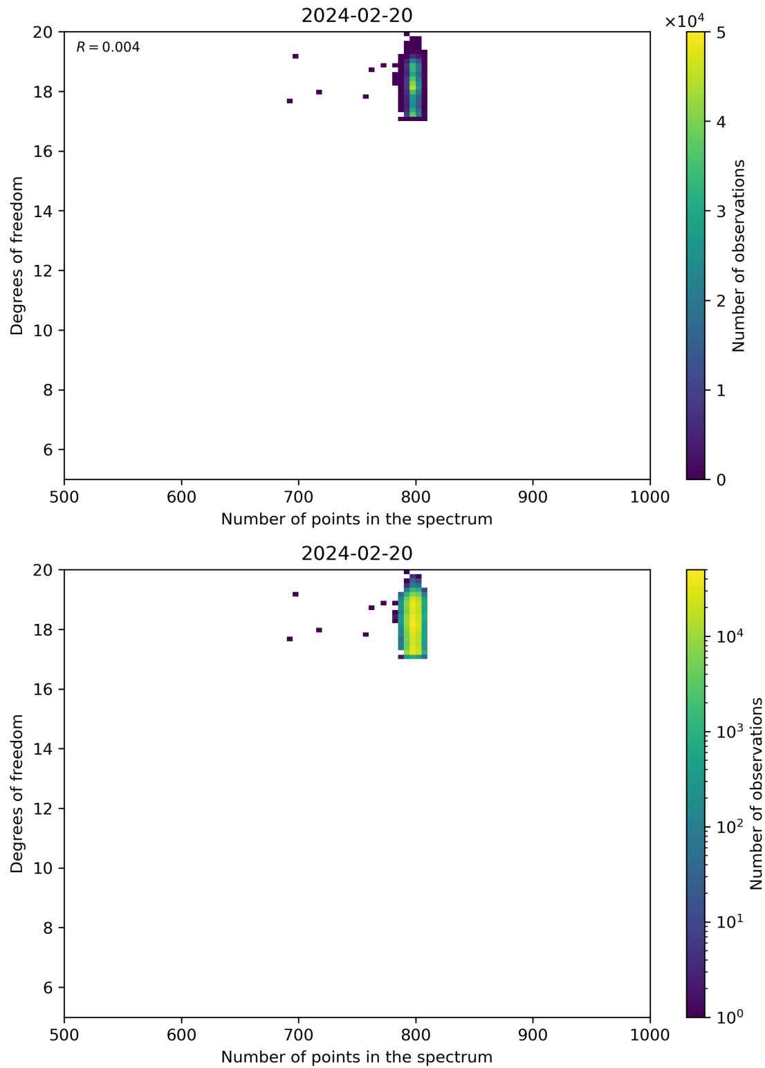
Figure 90: Scatter density plot of “Number of points in the spectrum” against “Degrees of freedom” for 2024-02-19 to 2024-02-21.
