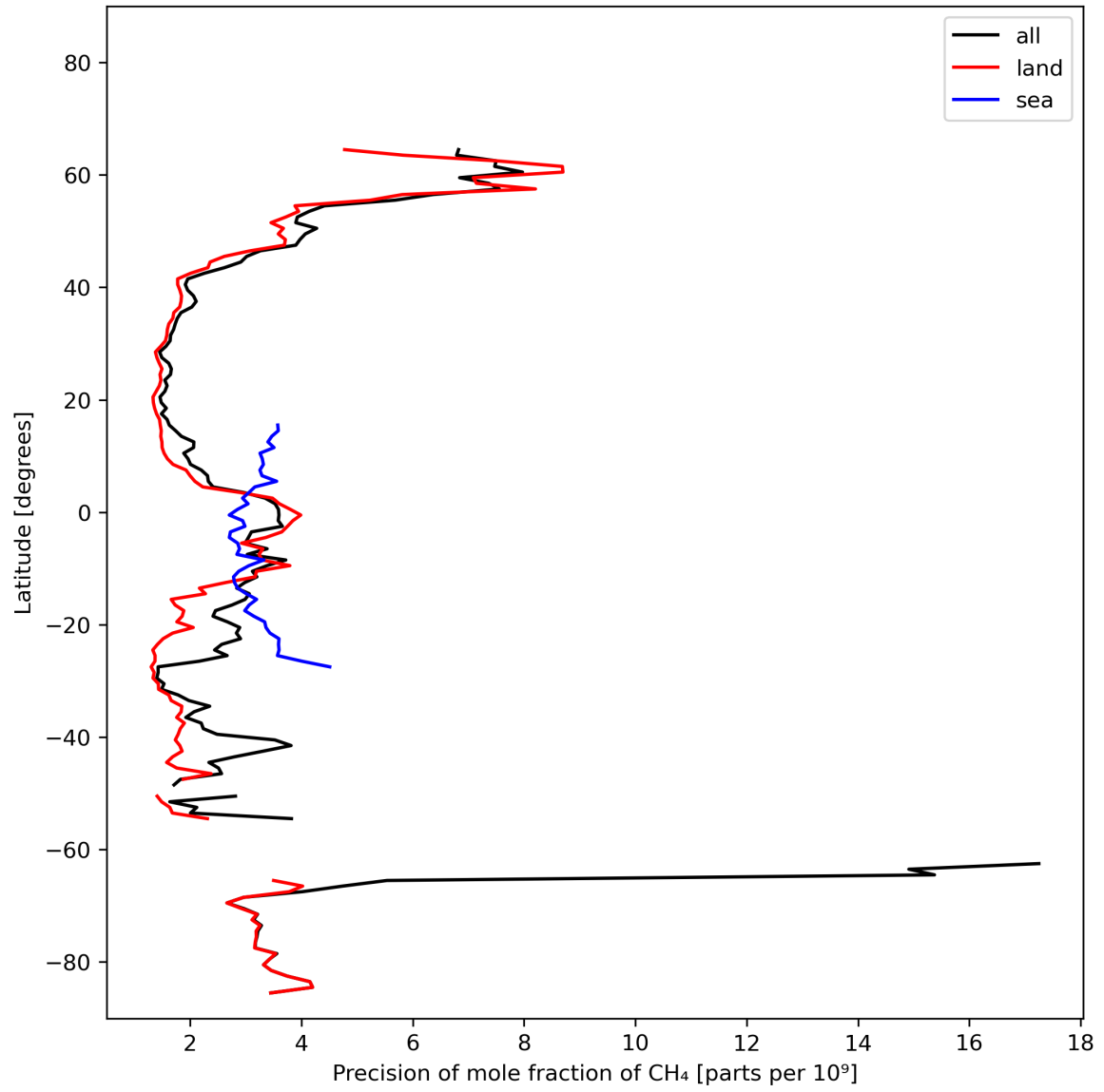
Figure 13: Zonal average of “Precision of mole fraction of CH 4 ” for 2024-02-19 to 2024-02-21.
