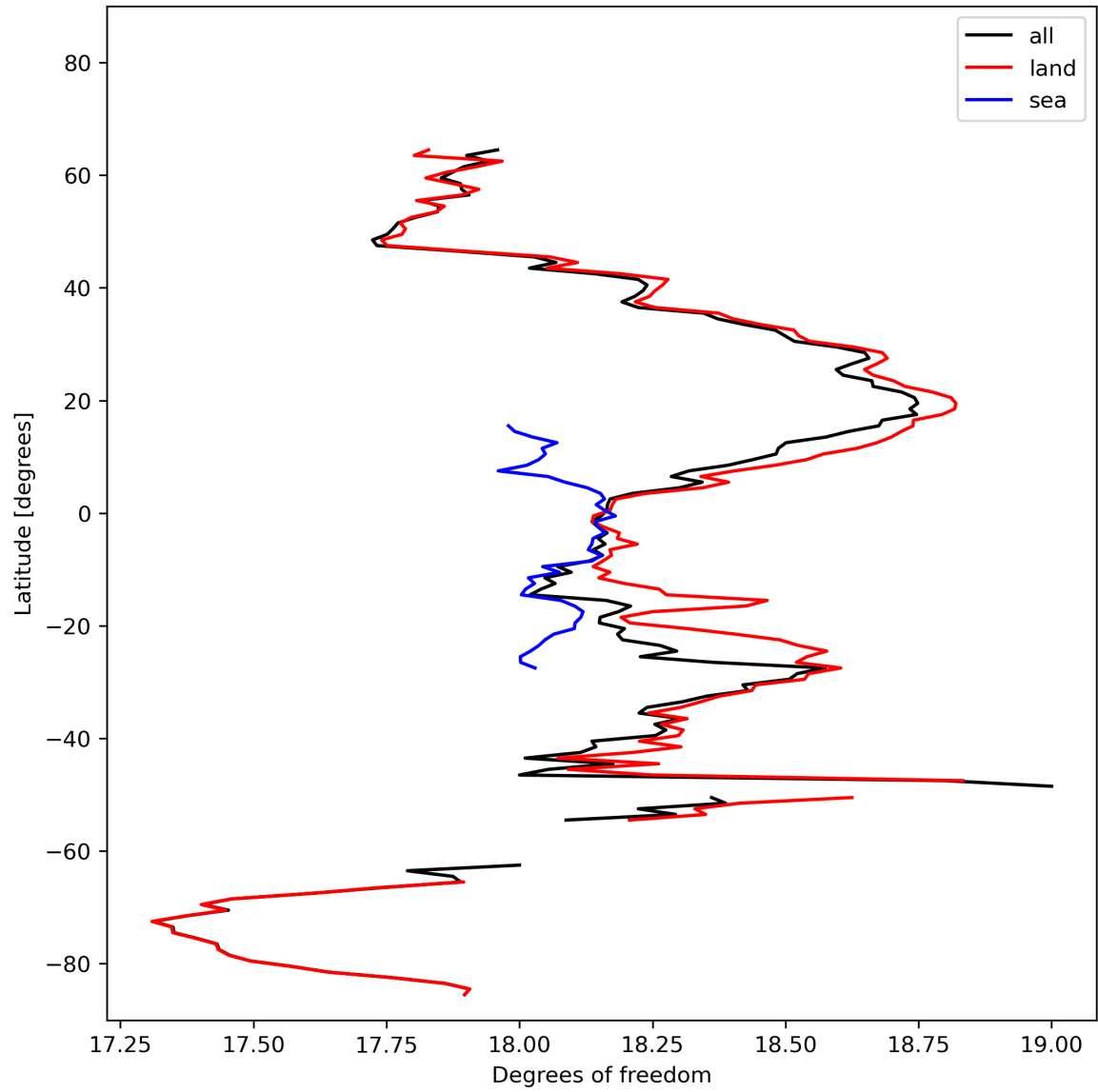
Figure 19: Zonal average of “Degrees of freedom” for 2024-02-19 to 2024-02-21.
