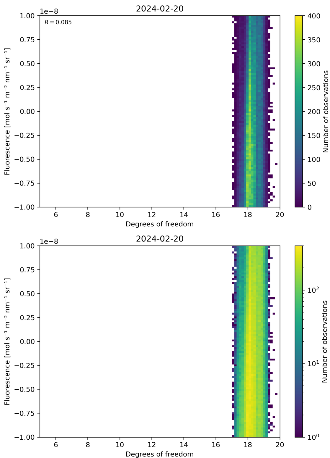
Figure 51: Scatter density plot of “Degrees of freedom” against “Fluorescence” for 2024-02-19 to 2024-02-21.
