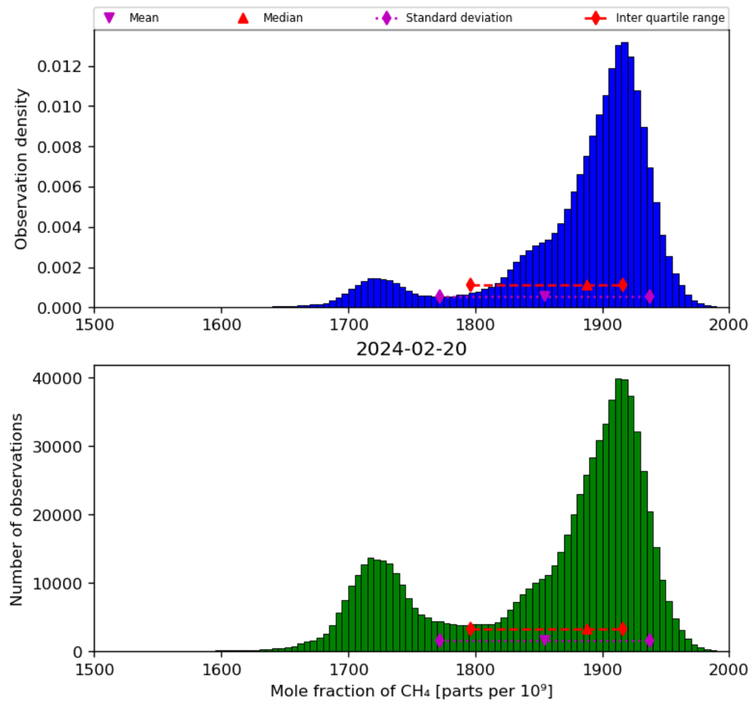
Figure 23: Histogram of “Mole fraction of CH 4 ” for 2024-02-19 to 2024-02-21
