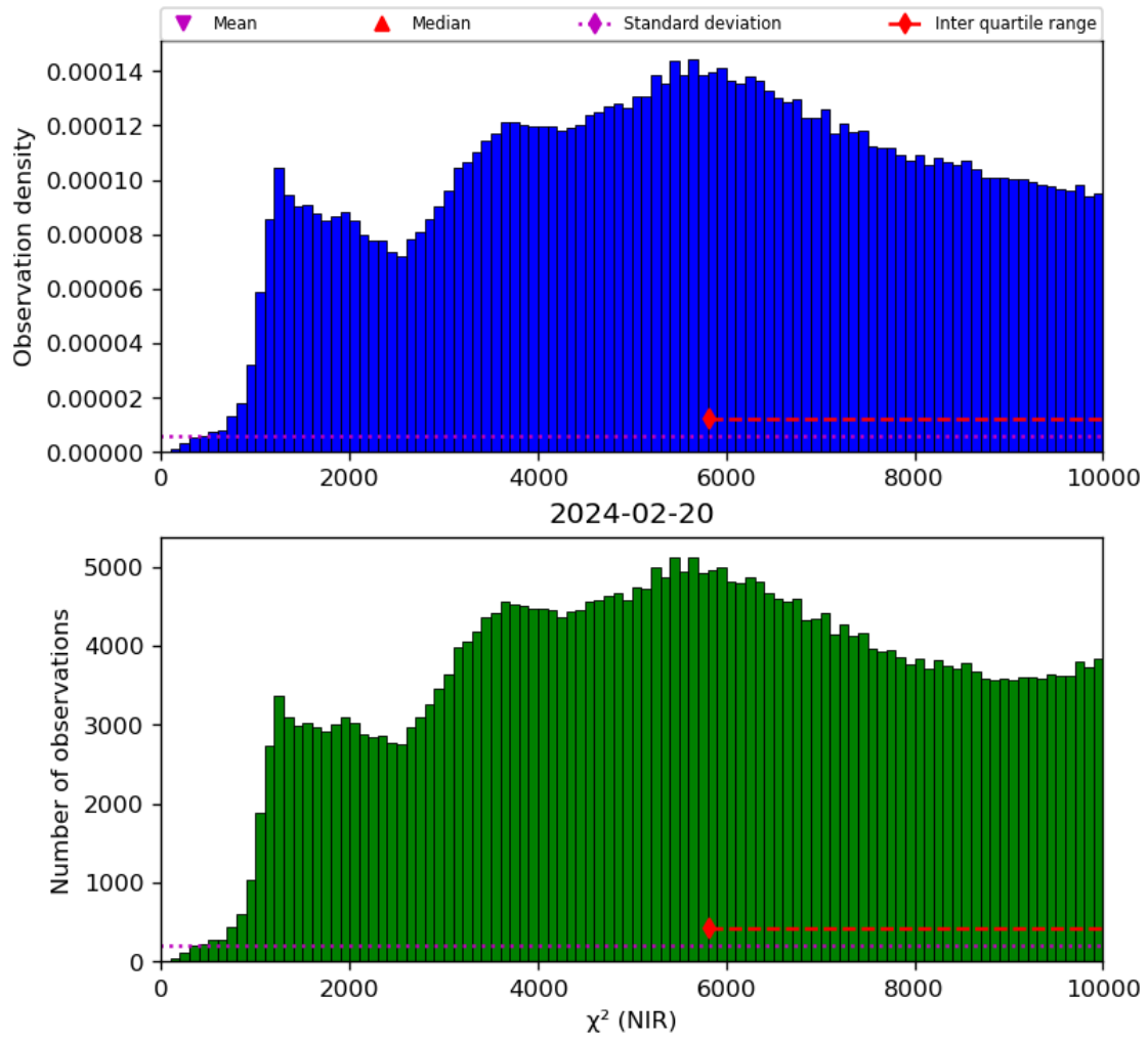
Figure 29: Histogram of “ \chi^2 (NIR)” for 2024-02-19 to 2024-02-21
