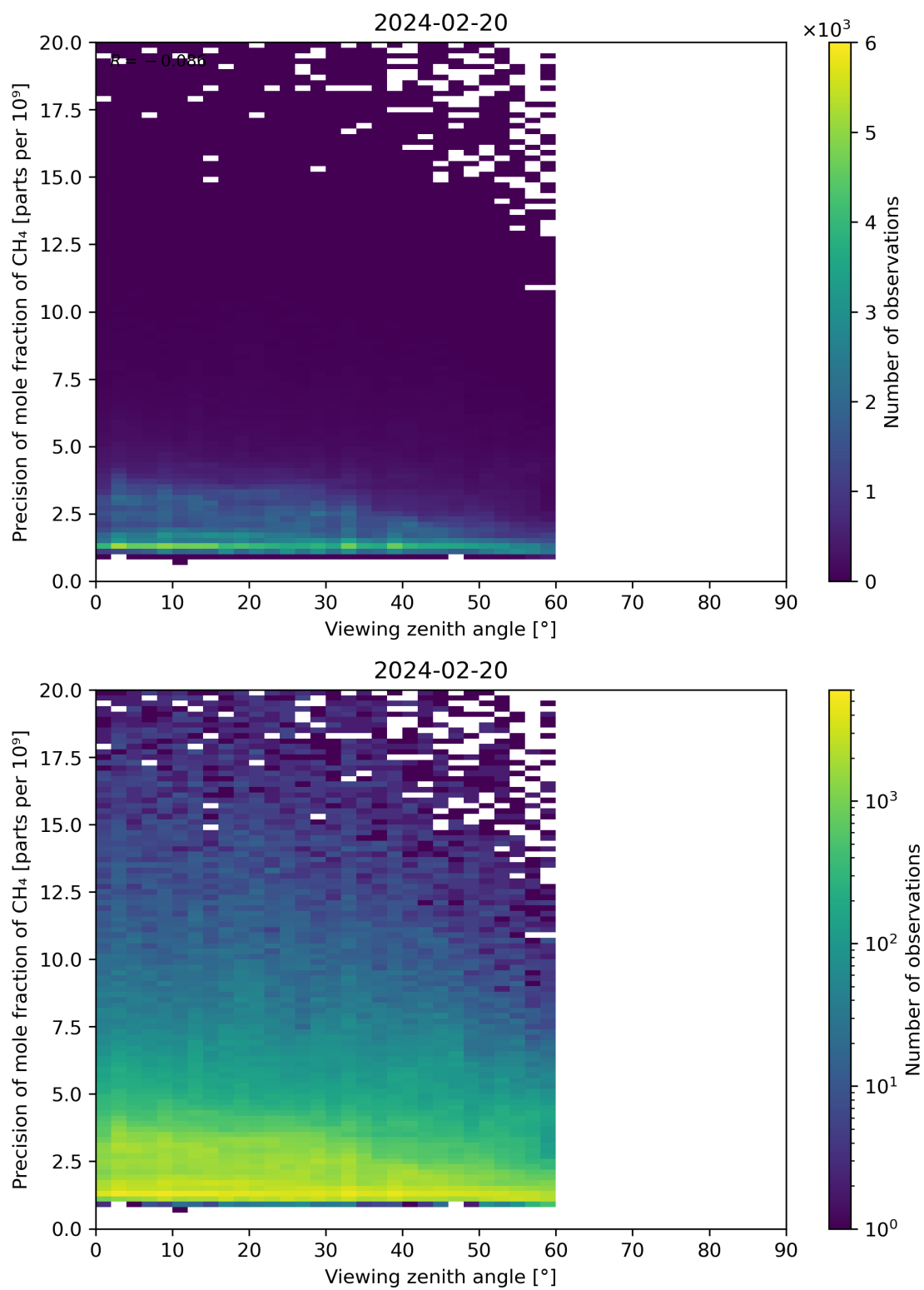
Figure 112: Scatter density plot of “Viewing zenith angle” against “Precision of mole fraction of CH 4 ” for 2024-02-19 to 2024-02-21.
