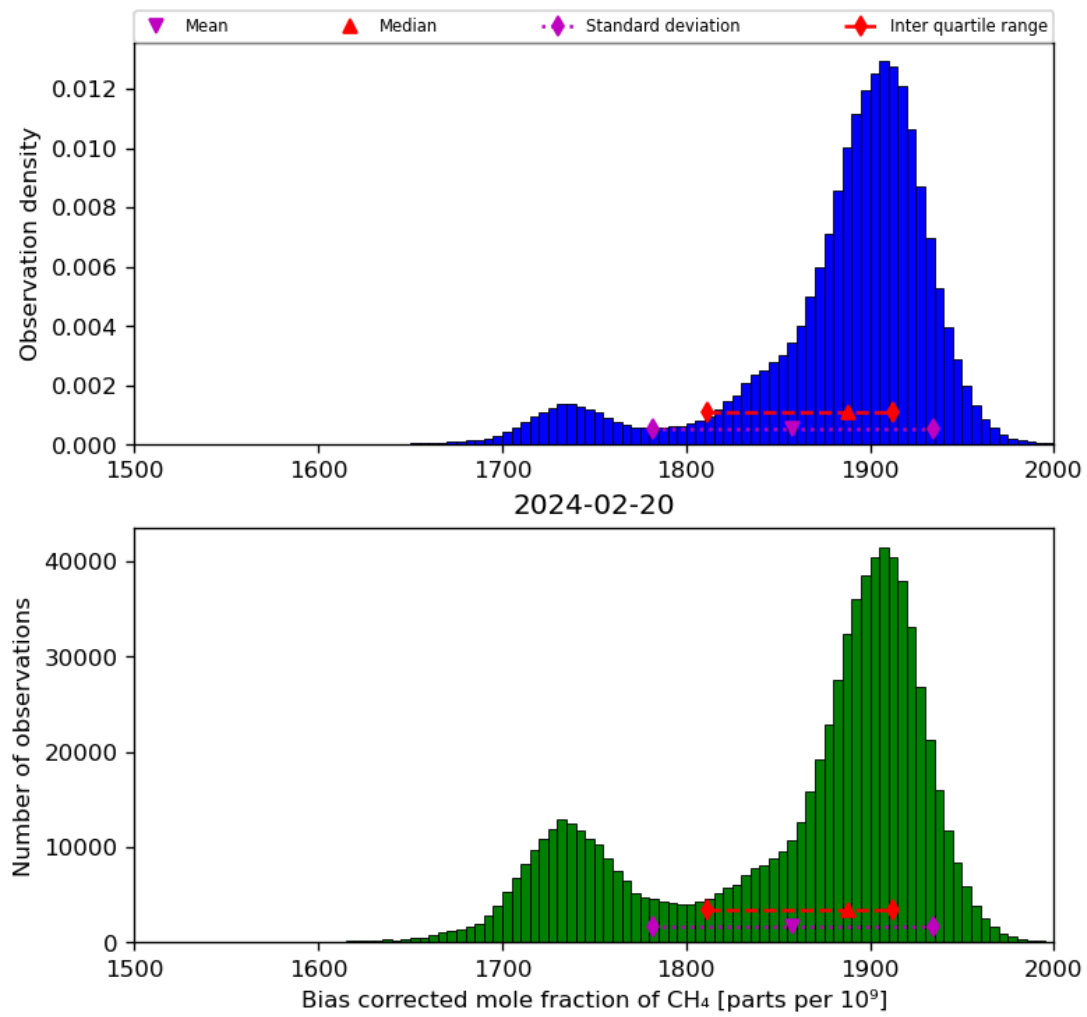
Figure 25: Histogram of “Bias corrected mole fraction of CH 4 ” for 2024-02-19 to 2024-02-21
