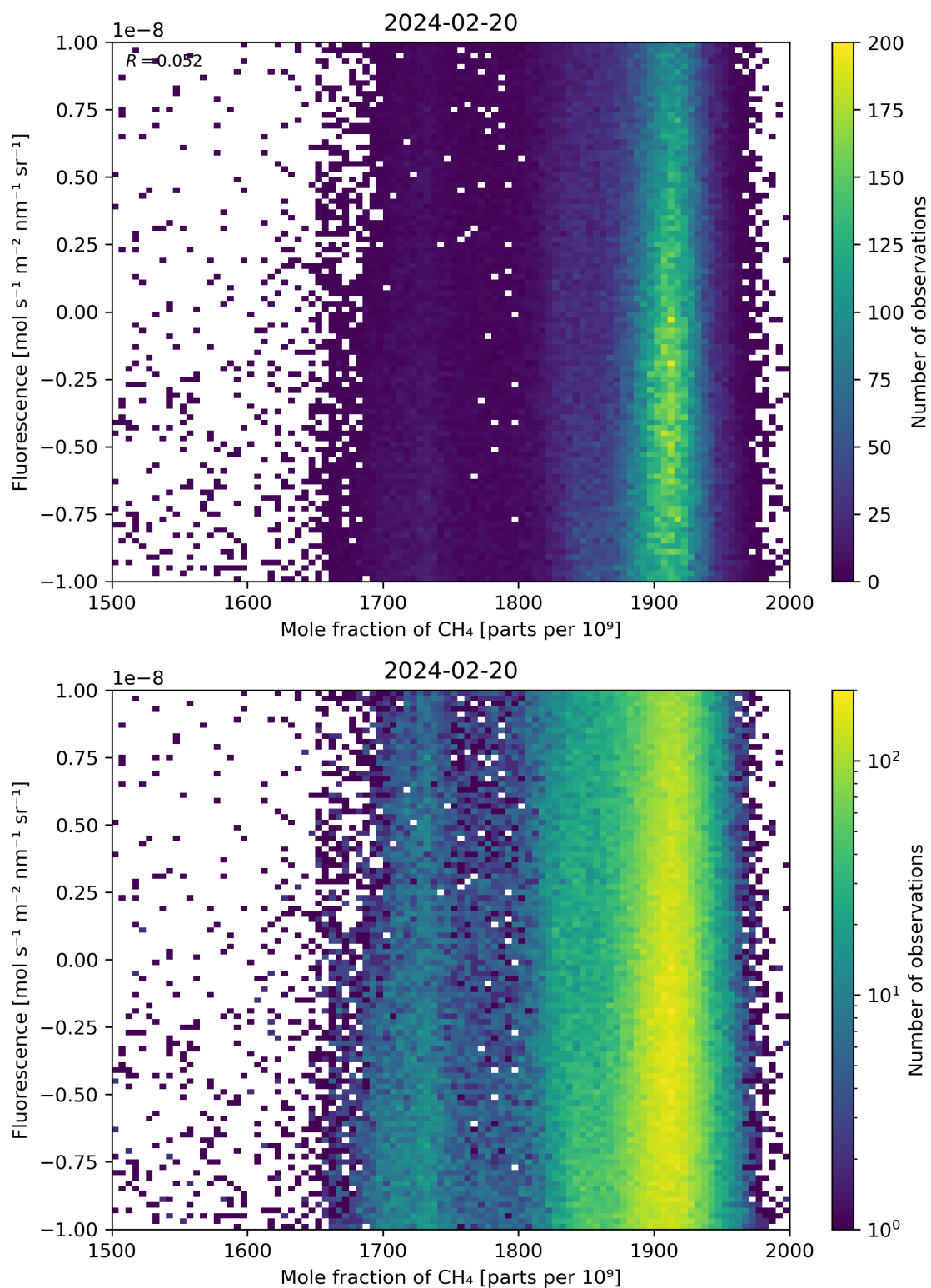
Figure 73: Scatter density plot of “Mole fraction of \text{CH}_4 ” against “Fluorescence” for 2024-02-19 to 2024-02-21.
