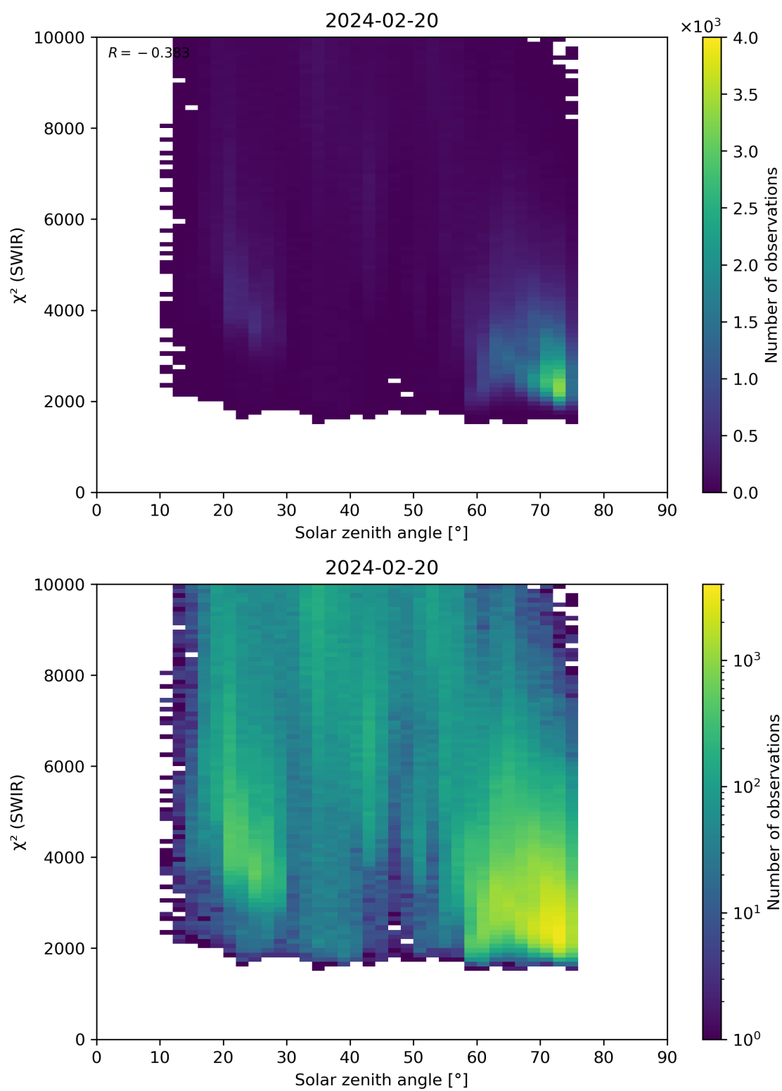
Figure 95: Scatter density plot of “Solar zenith angle” against “ \chi^2 (SWIR)” for 2024-02-19 to 2024-02-21.
