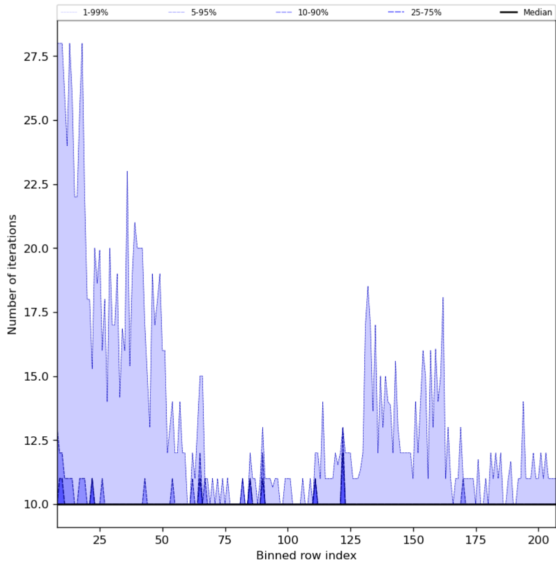
Figure 42: Along track statistics of “Number of iterations” for 2024-02-19 to 2024-02-21
