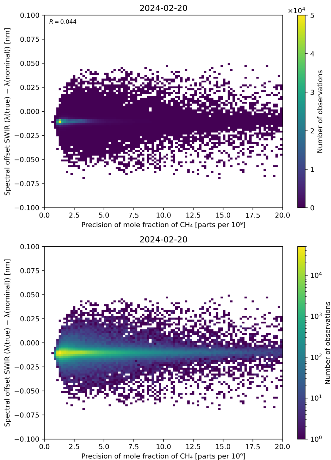
Figure 85: Scatter density plot of “Precision of mole fraction of \text{CH}_4 ” against “Spectral offset SWIR ( \lambda(\text{true}) - \lambda(\text{nominal}) )” for 2024-02-19 to 2024-02-21.
