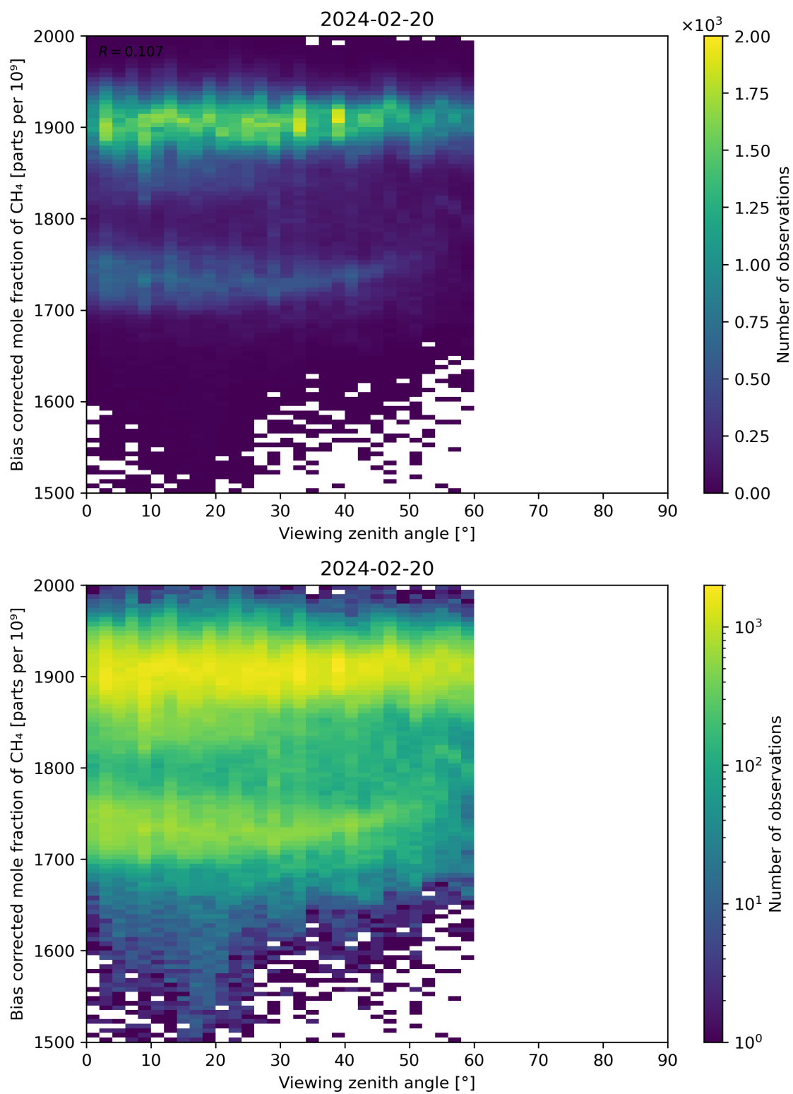
Figure 111: Scatter density plot of “Viewing zenith angle” against “Bias corrected mole fraction of CH 4 ” for 2024-02-19 to 2024-02-21.
