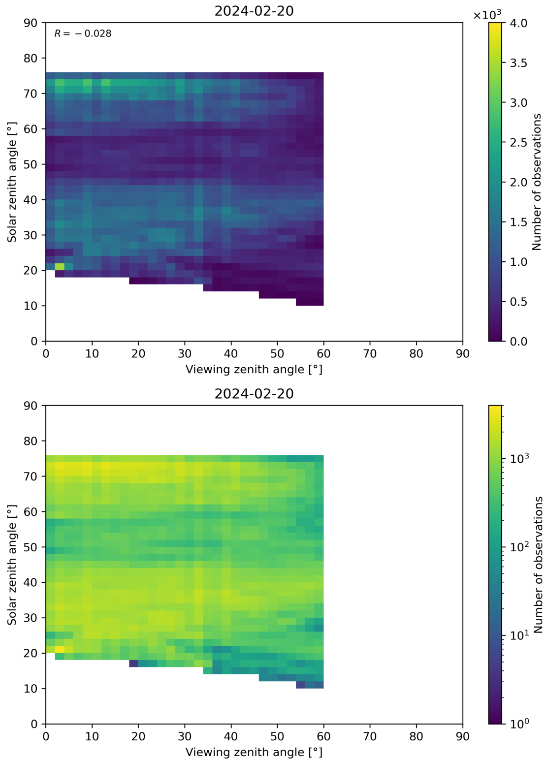
Figure 115: Scatter density plot of “Viewing zenith angle” against “Solar zenith angle” for 2024-02-19 to 2024-02-21.
