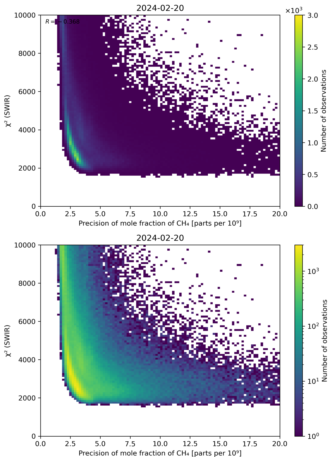
Figure 79: Scatter density plot of “Precision of mole fraction of CH 4 ” against “ \chi^2 (SWIR)” for 2024-02-19 to 2024-02-21.
