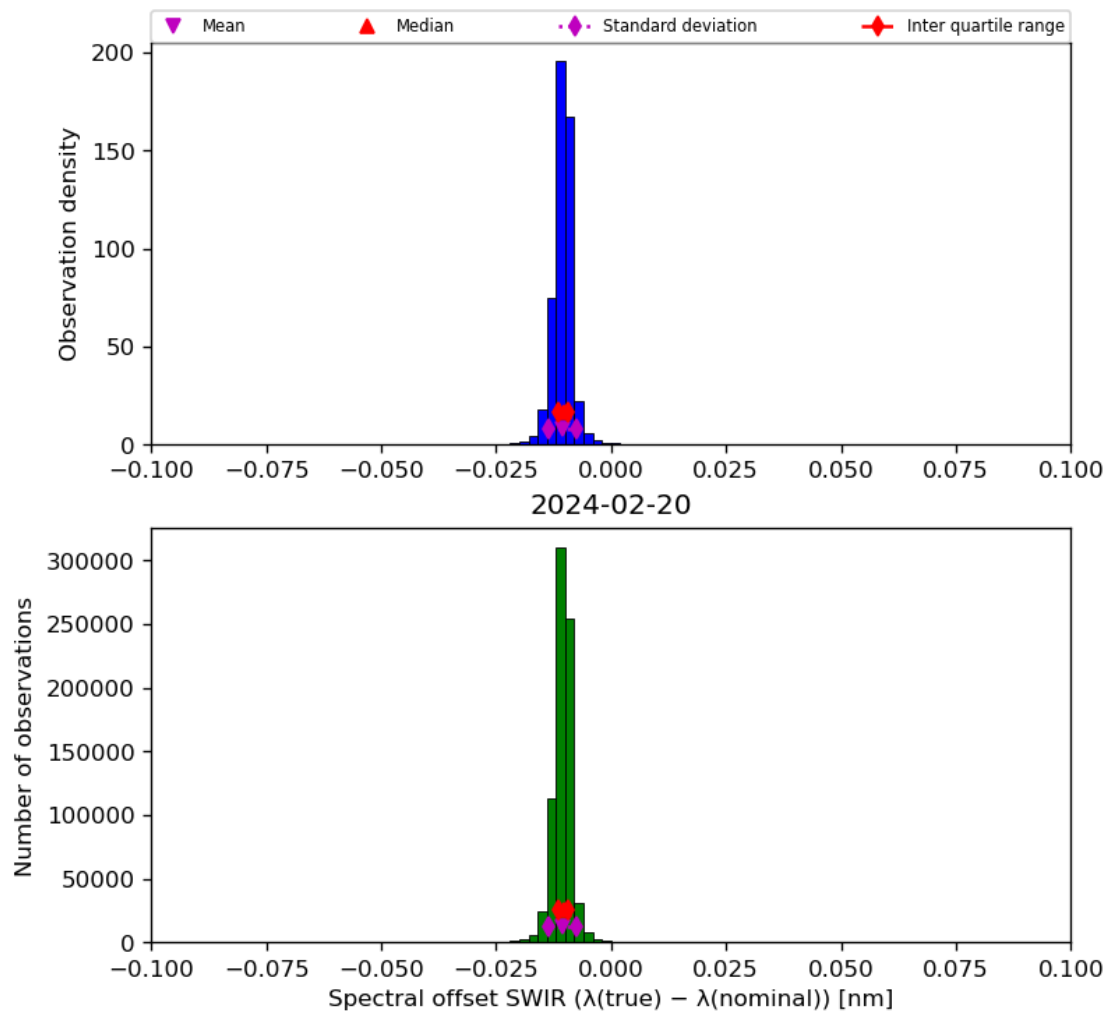
Figure 27: Histogram of “Spectral offset SWIR ( \lambda(\text{true}) - \lambda(\text{nominal}) )” for 2024-02-19 to 2024-02-21
