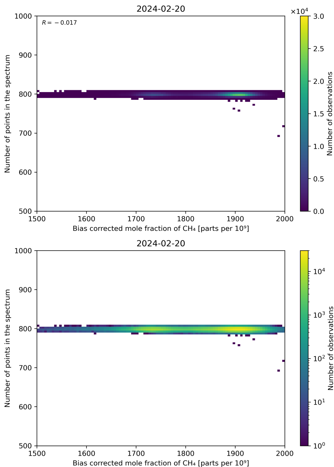
Figure 68: Scatter density plot of “Bias corrected mole fraction of CH 4 ” against “Number of points in the spectrum” for 2024-02-19 to 2024-02-21.
