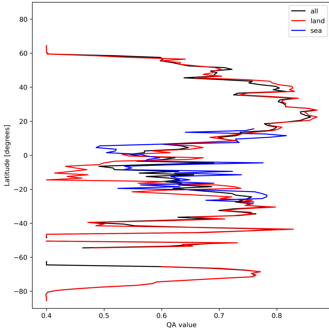
Figure 11: Zonal average of “QA value” for 2024-02-19 to 2024-02-21.
