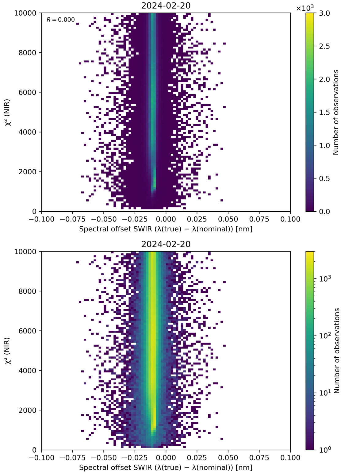
Figure 117: Scatter density plot of “Spectral offset SWIR ( \lambda(\text{true}) - \lambda(\text{nominal}) )” against “ \chi^2 (NIR)” for 2024-02-19 to 2024-02-21.
