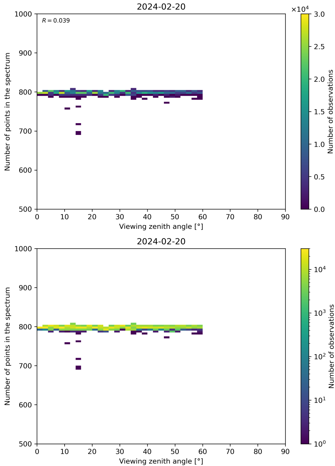
Figure 114: Scatter density plot of “Viewing zenith angle” against “Number of points in the spectrum” for 2024-02-19 to 2024-02-21.
