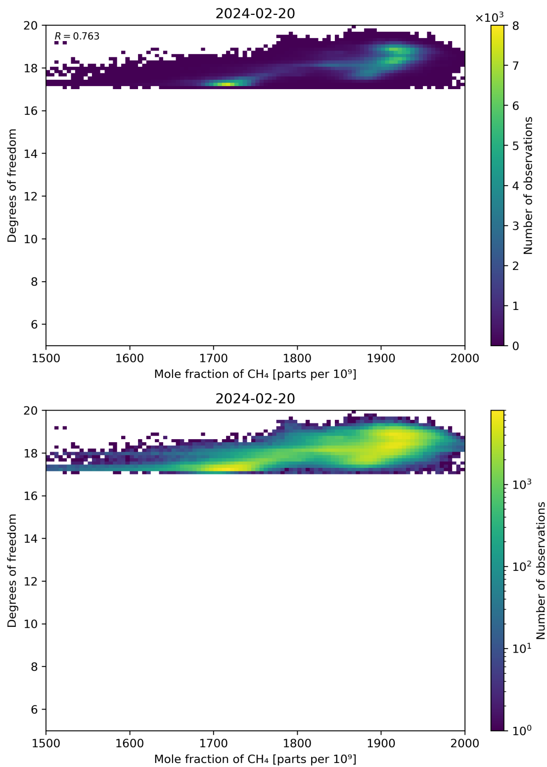
Figure 72: Scatter density plot of “Mole fraction of CH 4 ” against “Degrees of freedom” for 2024-02-19 to 2024-02-21.
