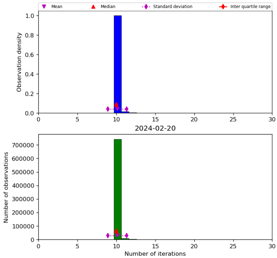
Figure 31: Histogram of “Number of iterations” for 2024-02-19 to 2024-02-21
