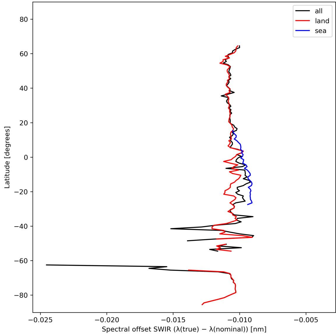
Figure 16: Zonal average of “Spectral offset SWIR ( \lambda(\text{true}) - \lambda(\text{nominal}) )” for 2024-02-19 to 2024-02-21.
