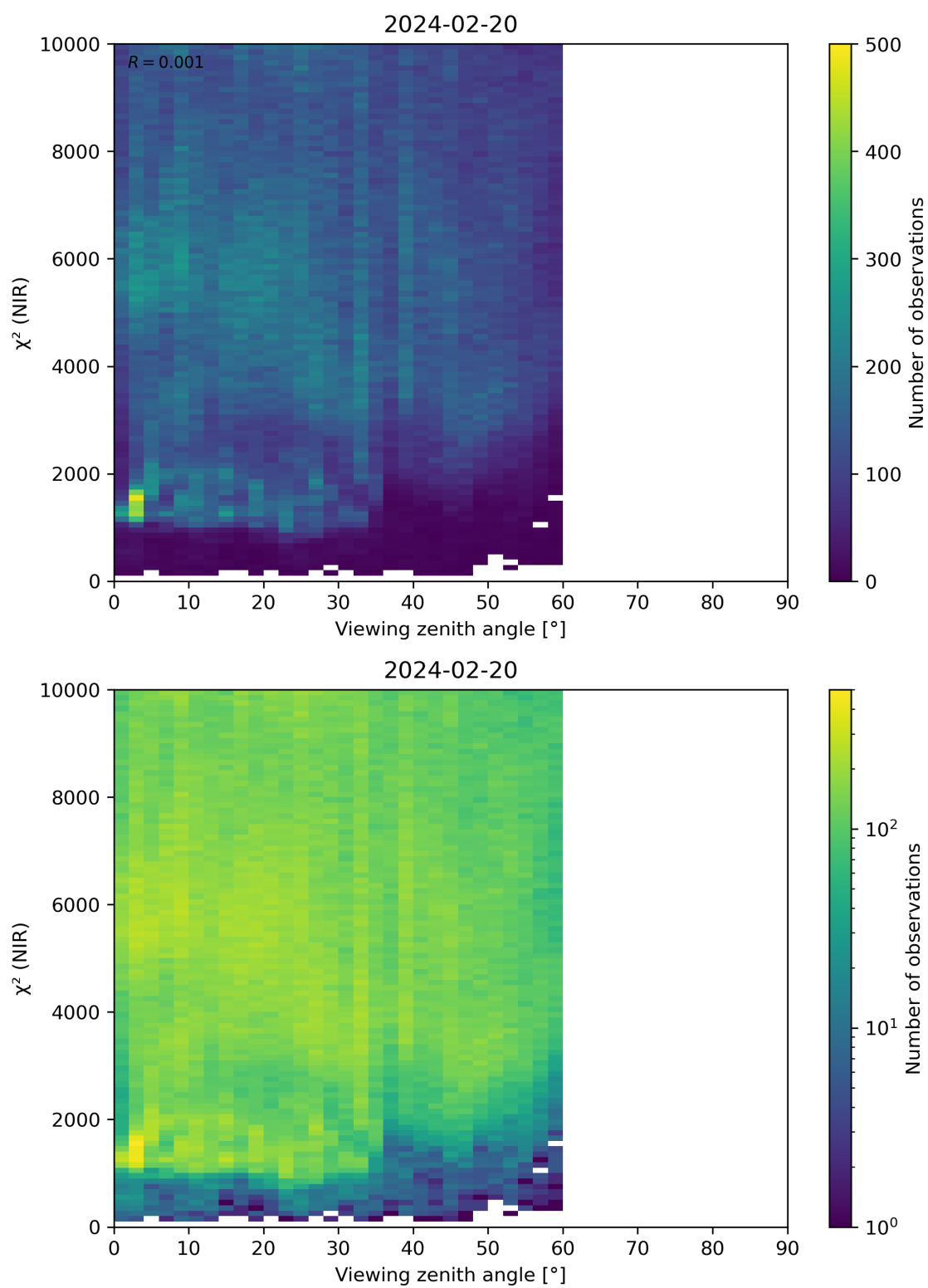
Figure 105: Scatter density plot of “Viewing zenith angle” against “ \chi^2 (NIR)” for 2024-02-19 to 2024-02-21.
