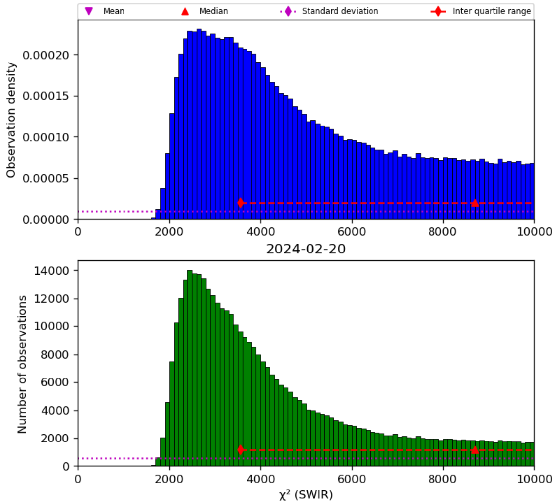
Figure 28: Histogram of “ \chi^2 (SWIR)” for 2024-02-19 to 2024-02-21
