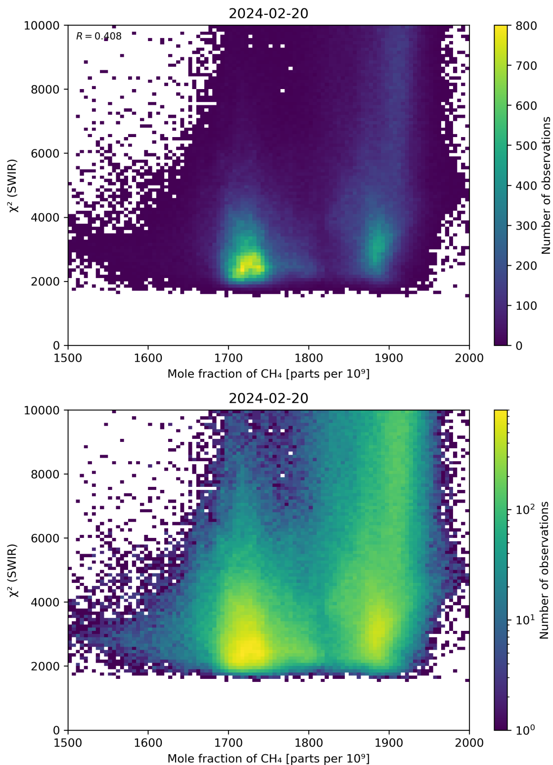
Figure 71: Scatter density plot of “Mole fraction of \text{CH}_4 ” against “ \chi^2 (SWIR)” for 2024-02-19 to 2024-02-21.
