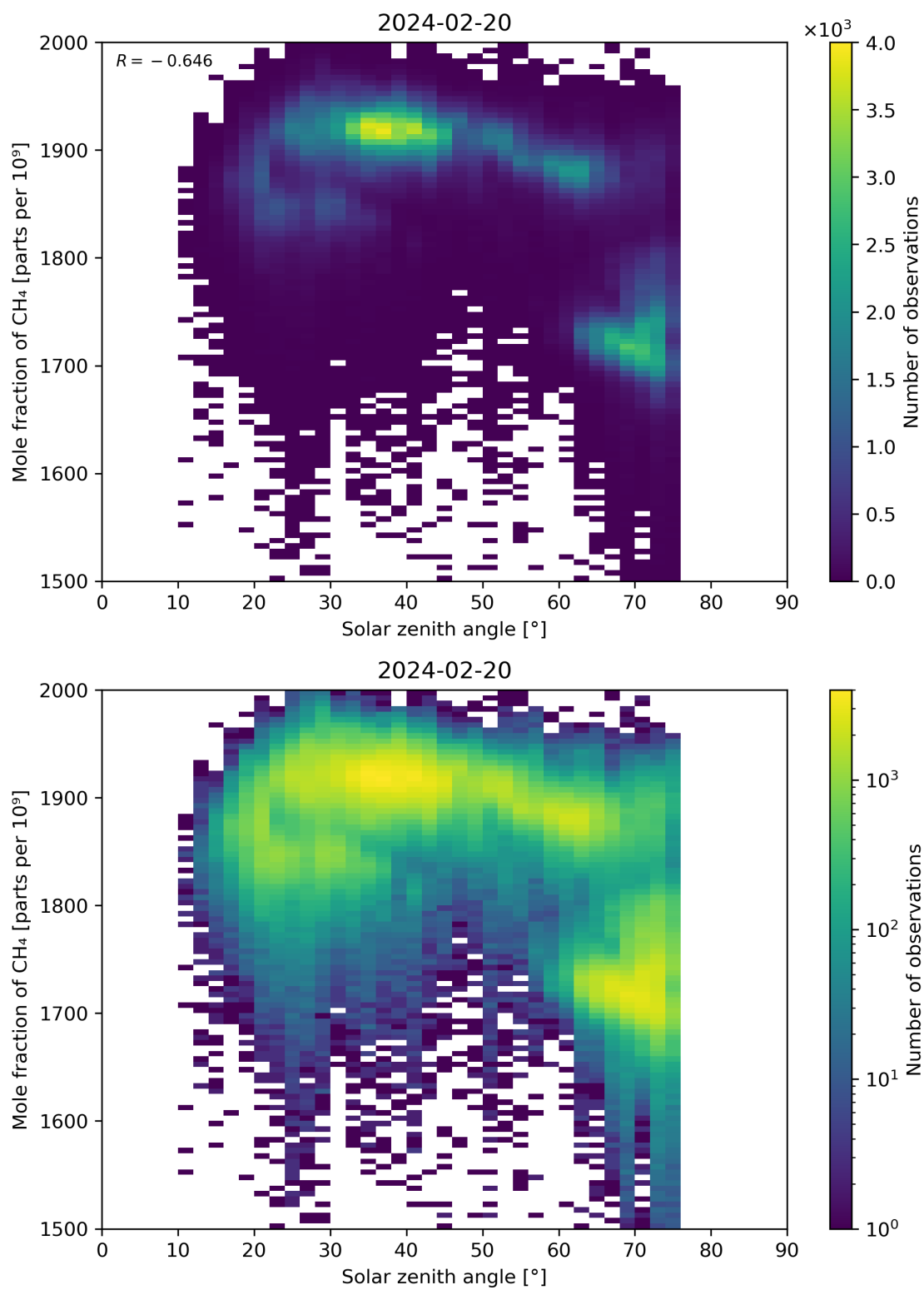
Figure 99: Scatter density plot of “Solar zenith angle” against “Mole fraction of CH 4 ” for 2024-02-19 to 2024-02-21.
