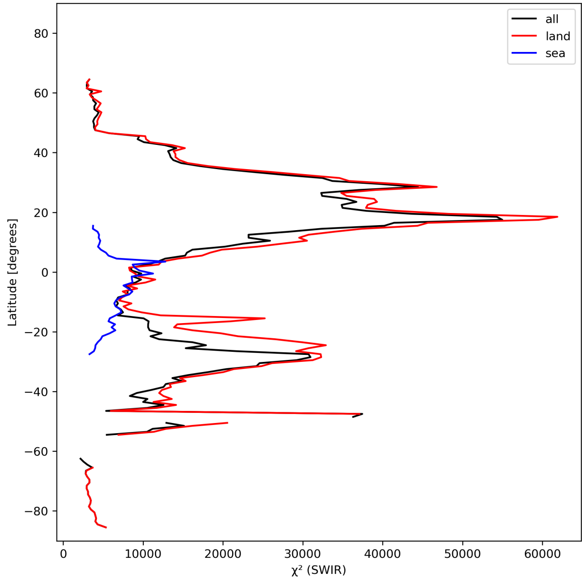
Figure 17: Zonal average of “ \chi^2 (SWIR)” for 2024-02-19 to 2024-02-21.
