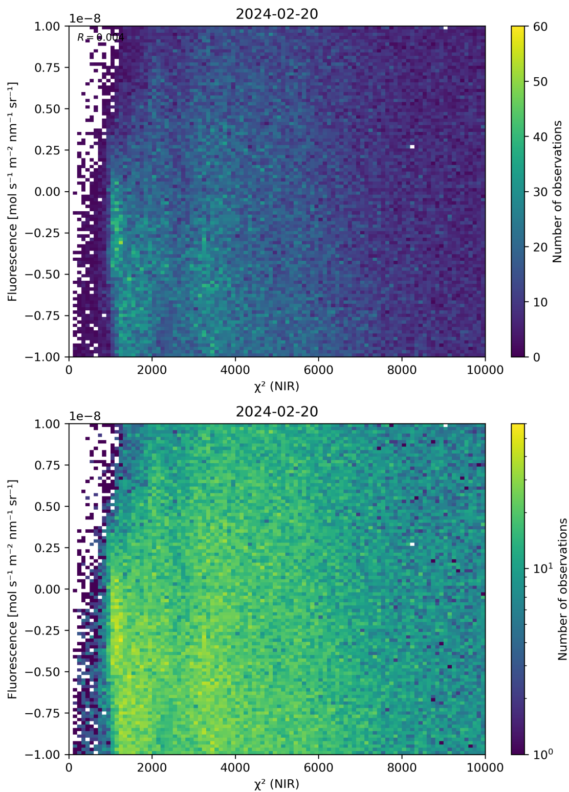
Figure 45: Scatter density plot of “ \chi^2 (NIR)” against “Fluorescence” for 2024-02-19 to 2024-02-21.
