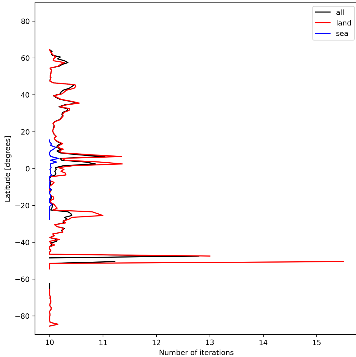
Figure 20: Zonal average of “Number of iterations” for 2024-02-19 to 2024-02-21.
