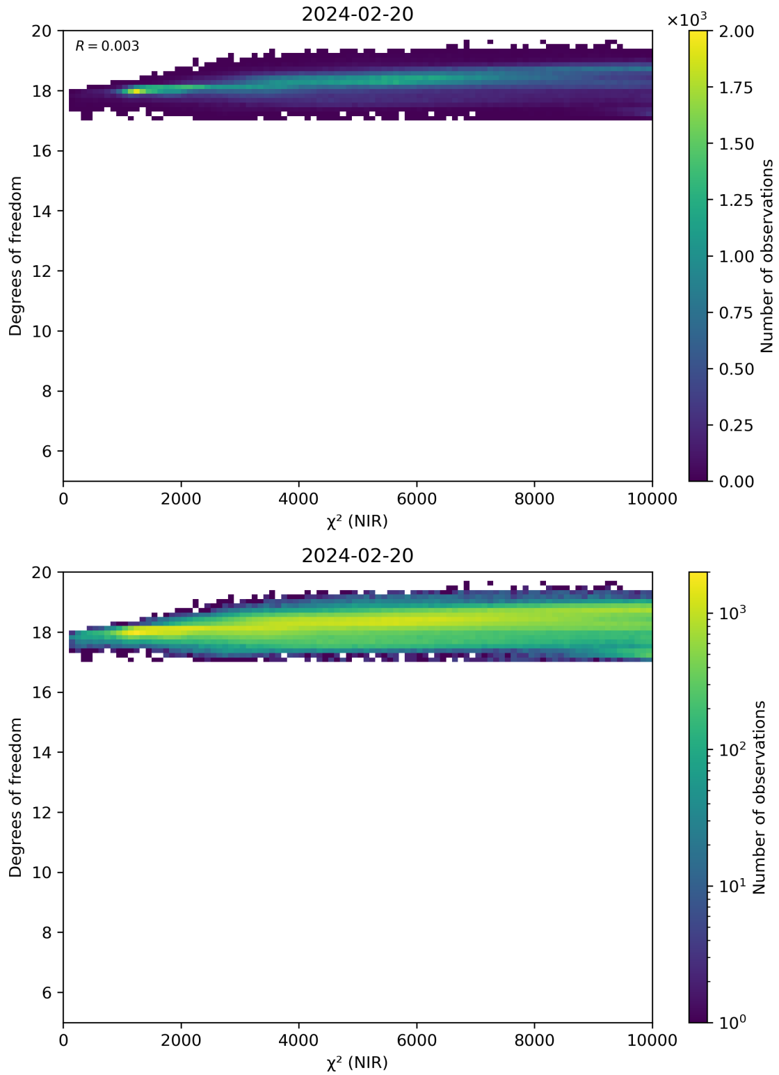
Figure 44: Scatter density plot of “ \chi^2 (NIR)” against “Degrees of freedom” for 2024-02-19 to 2024-02-21.
