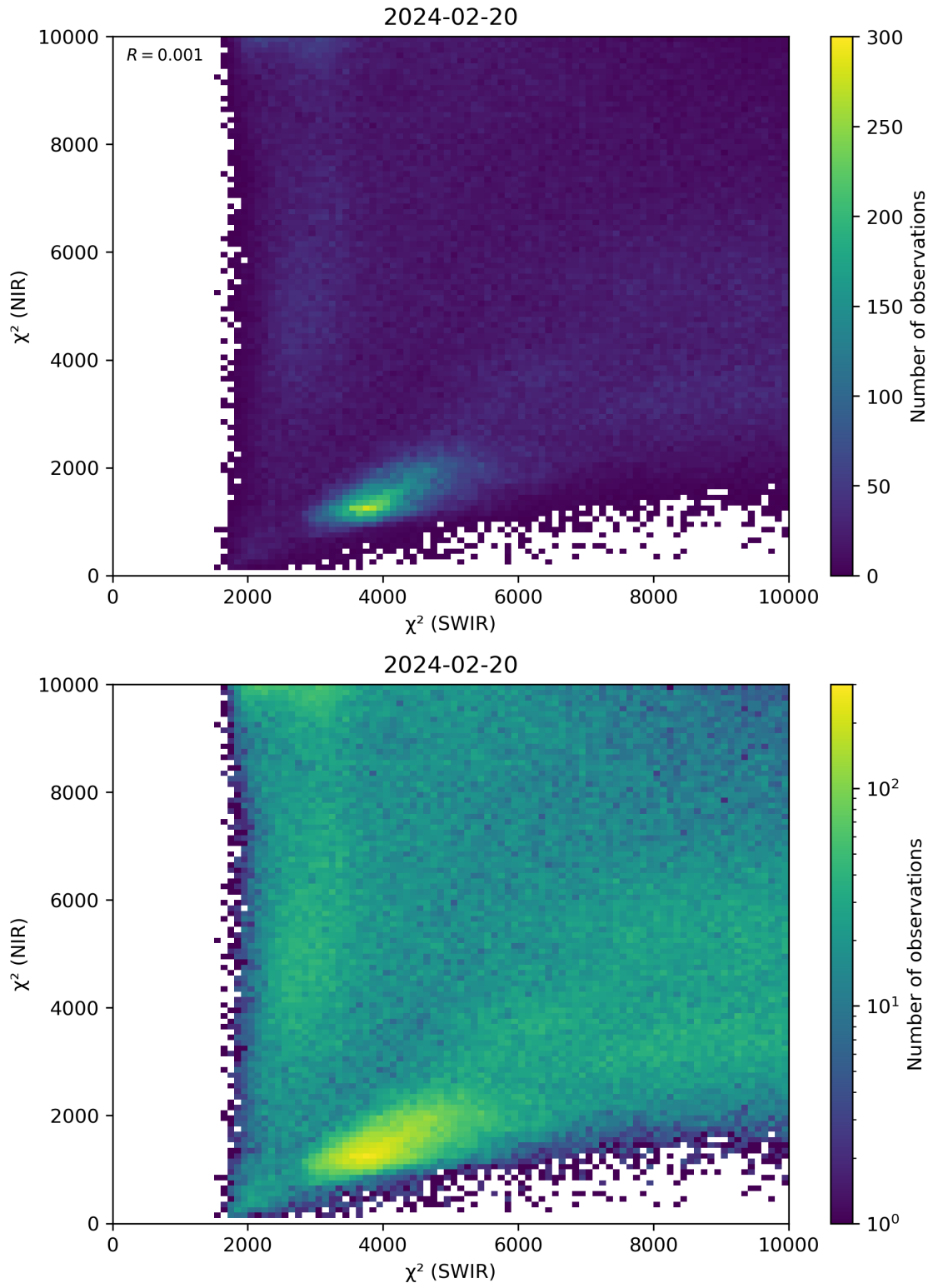
Figure 47: Scatter density plot of “ \chi^2 (SWIR)” against “ \chi^2 (NIR)” for 2024-02-19 to 2024-02-21.
