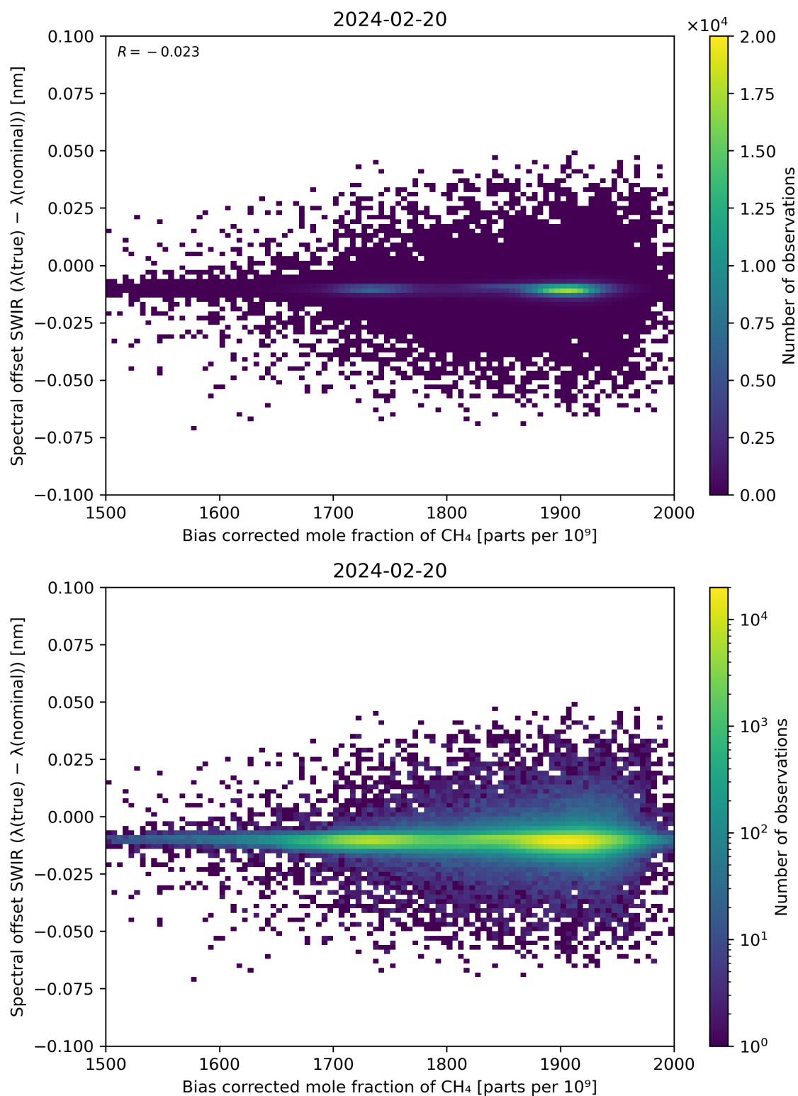
Figure 69: Scatter density plot of “Bias corrected mole fraction of \text{CH}_4 ” against “Spectral offset SWIR ( \lambda(\text{true}) - \lambda(\text{nominal}) )” for 2024-02-19 to 2024-02-21.
