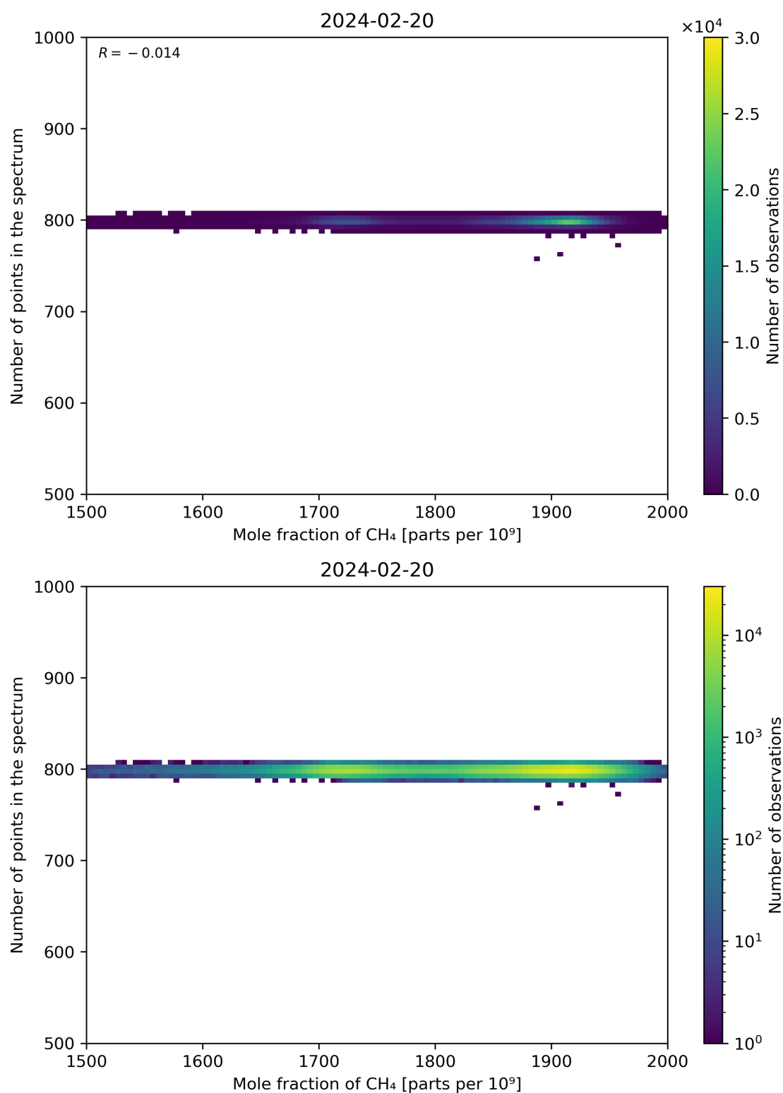
Figure 77: Scatter density plot of “Mole fraction of CH 4 ” against “Number of points in the spectrum” for 2024-02-19 to 2024-02-21.
