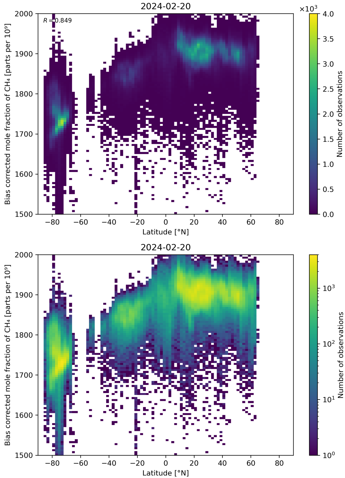
Figure 58: Scatter density plot of “Latitude” against “Bias corrected mole fraction of CH 4 ” for 2024-02-19 to 2024-02-21.
