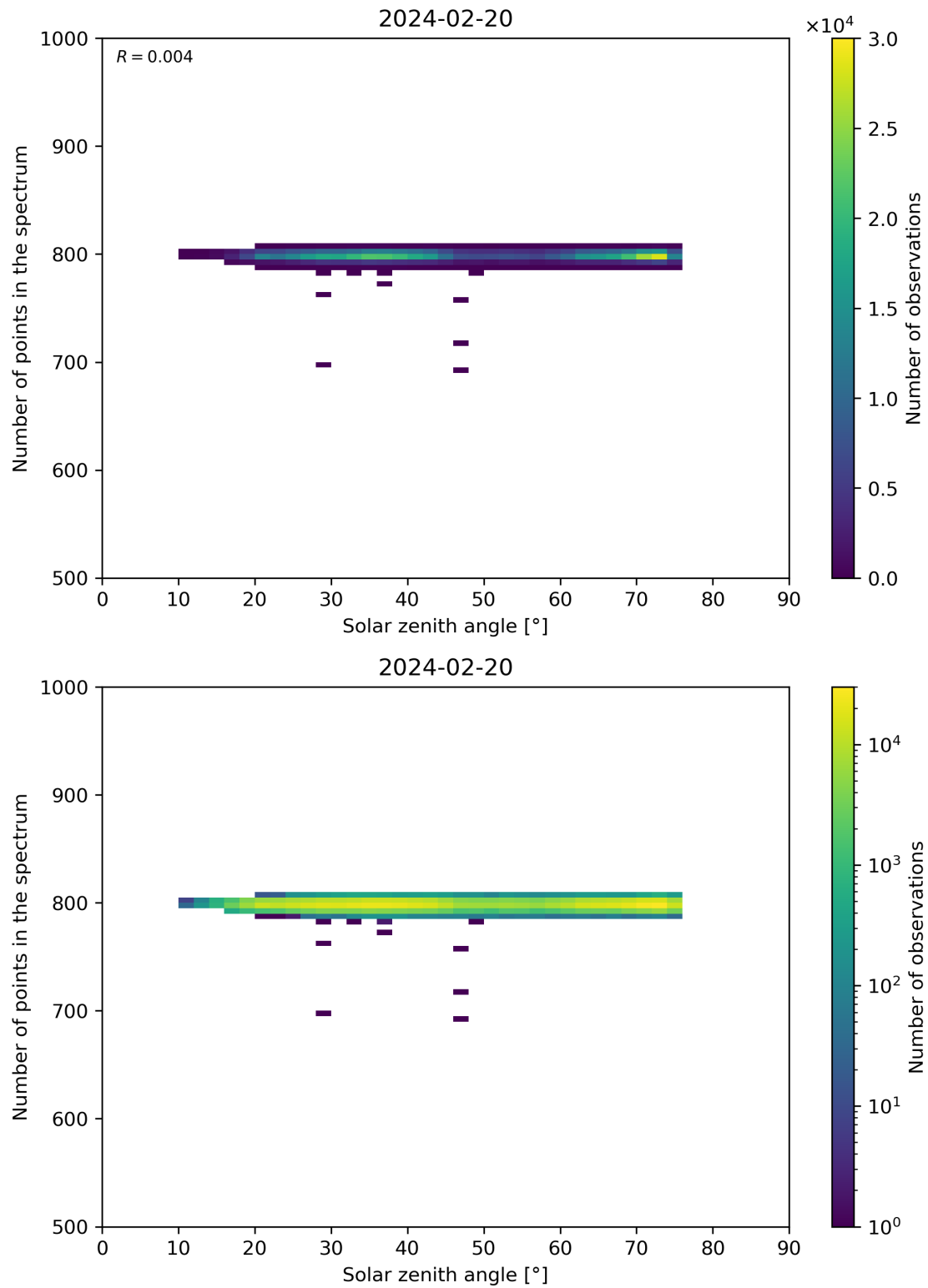
Figure 103: Scatter density plot of “Solar zenith angle” against “Number of points in the spectrum” for 2024-02-19 to 2024-02-21.
