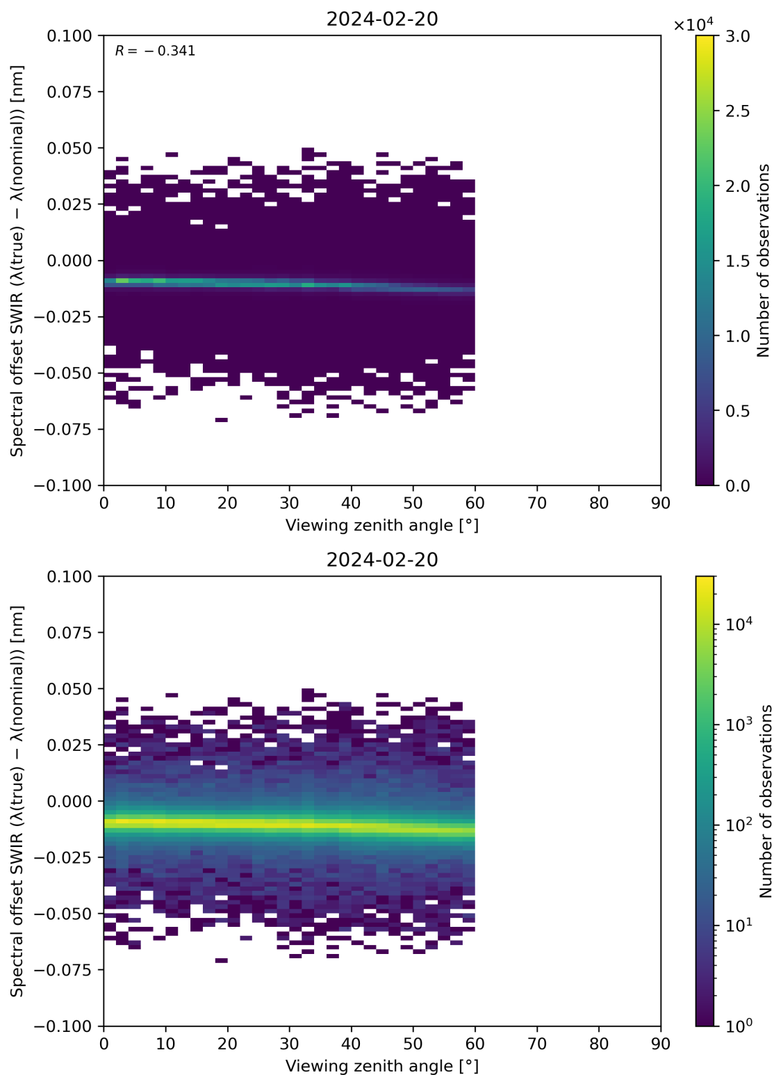
Figure 116: Scatter density plot of “Viewing zenith angle” against “Spectral offset SWIR ( \lambda(\text{true}) - \lambda(\text{nominal}) )” for 2024-02-19 to 2024-02-21.
