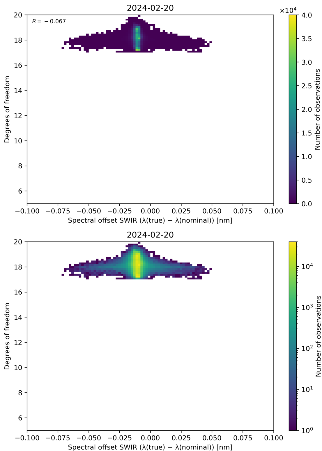
Figure 119: Scatter density plot of “Spectral offset SWIR ( \lambda(\text{true}) - \lambda(\text{nominal}) )” against “Degrees of freedom” for 2024-02-19 to 2024-02-21.
