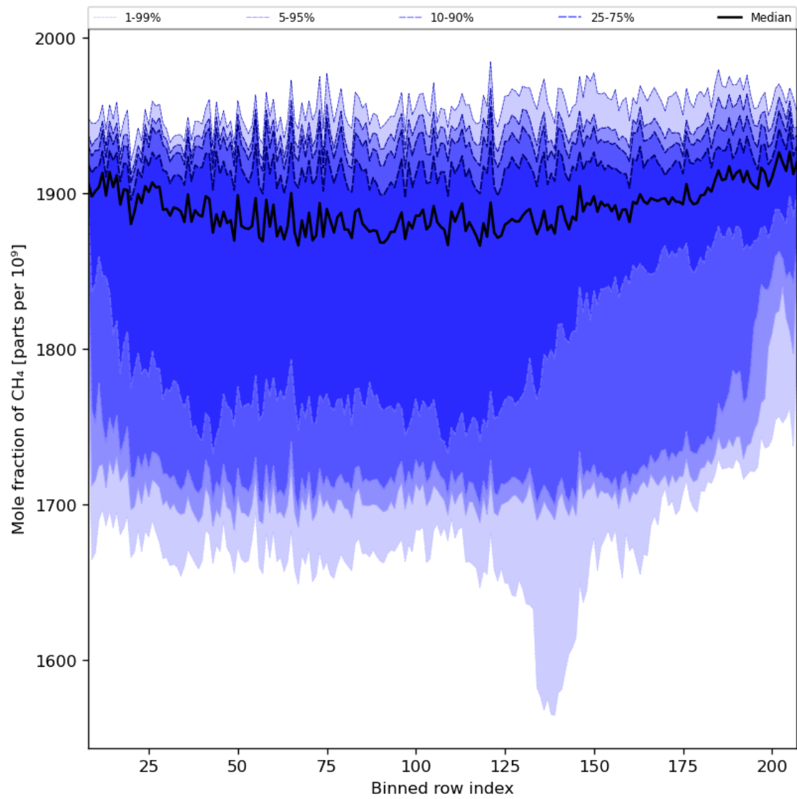
Figure 34: Along track statistics of “Mole fraction of CH 4 ” for 2024-02-19 to 2024-02-21
