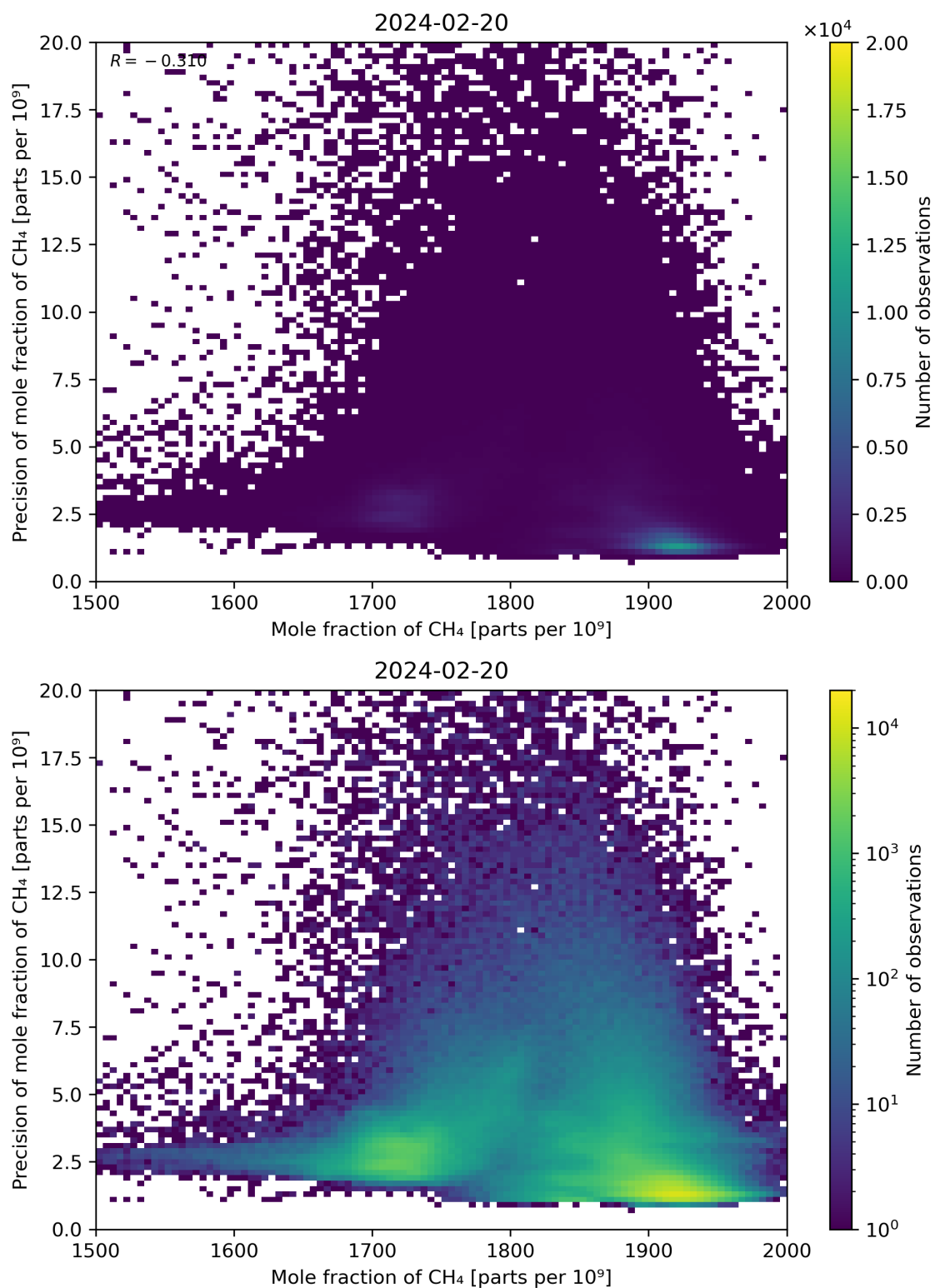
Figure 75: Scatter density plot of “Mole fraction of CH 4 ” against “Precision of mole fraction of CH 4 ” for 2024-02-19 to 2024-02-21.
