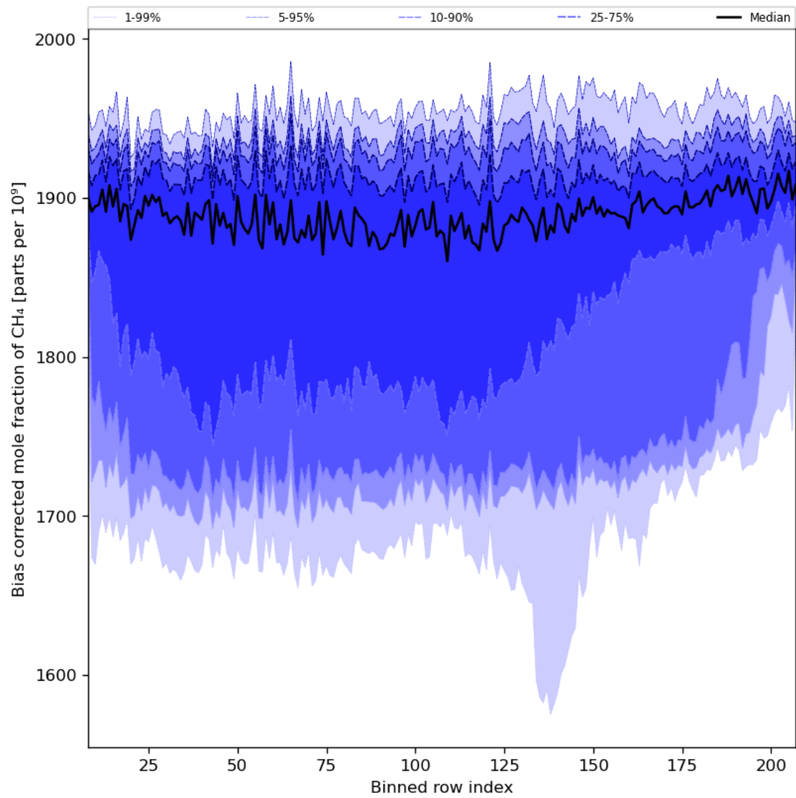
Figure 36: Along track statistics of “Bias corrected mole fraction of \text{CH}_4 ” for 2024-02-19 to 2024-02-21
