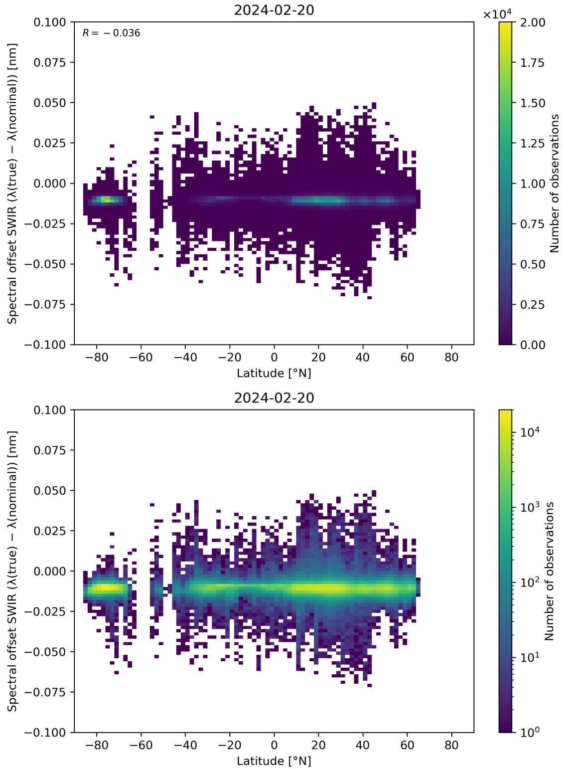
Figure 62: Scatter density plot of “Latitude” against “Spectral offset SWIR ( \lambda(\text{true}) - \lambda(\text{nominal}) )” for 2024-02-19 to 2024-02-21.
