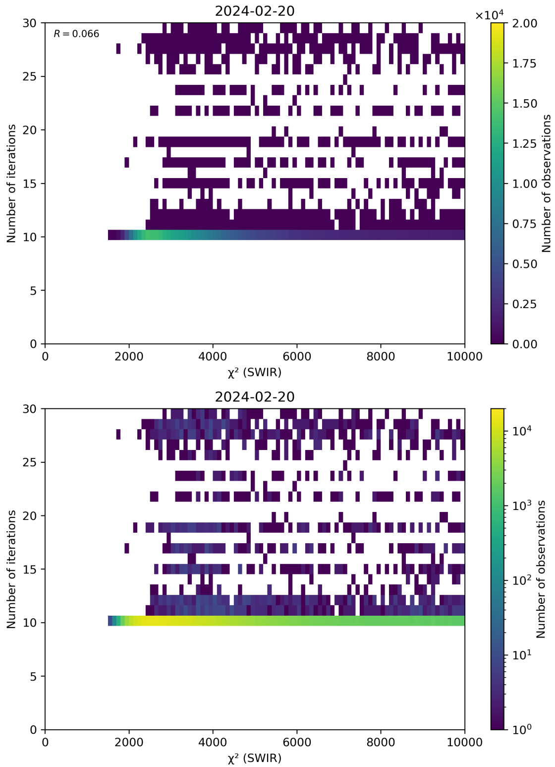
Figure 50: Scatter density plot of “ \chi^2 (SWIR)” against “Number of iterations” for 2024-02-19 to 2024-02-21.
