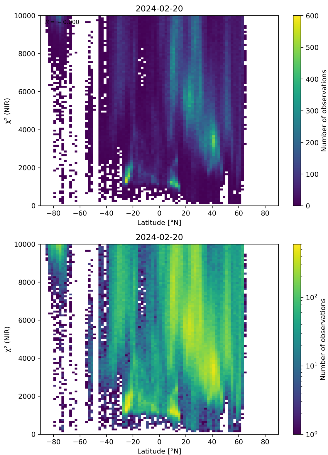
Figure 53: Scatter density plot of “Latitude” against “ \chi^2 (NIR)” for 2024-02-19 to 2024-02-21.
