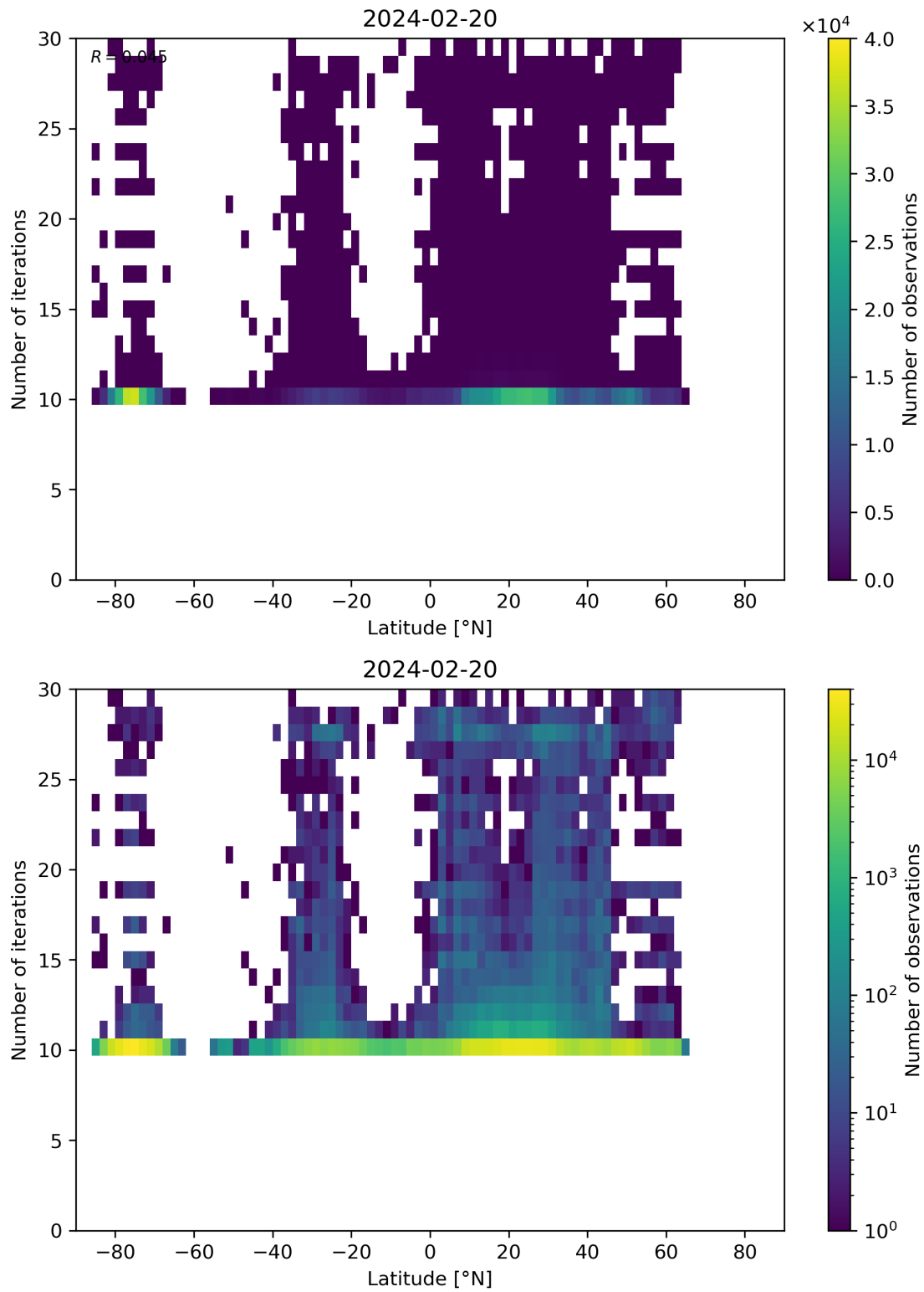
Figure 60: Scatter density plot of “Latitude” against “Number of iterations” for 2024-02-19 to 2024-02-21.
