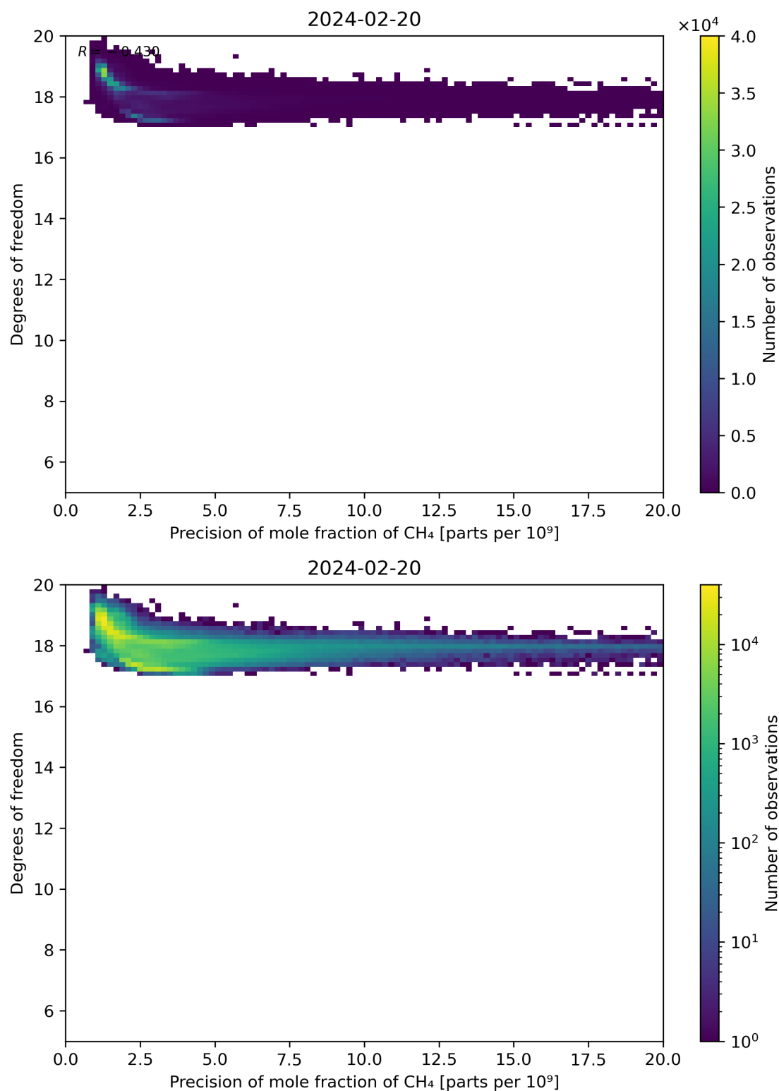
Figure 80: Scatter density plot of “Precision of mole fraction of CH 4 ” against “Degrees of freedom” for 2024-02-19 to 2024-02-21.
