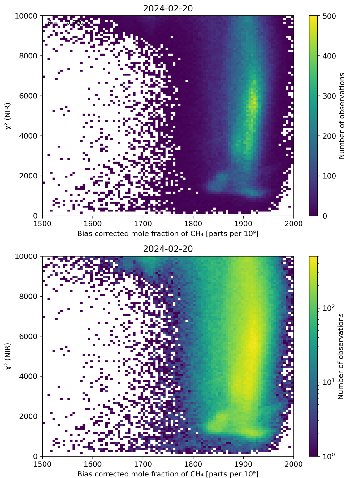
Figure 63: Scatter density plot of “Bias corrected mole fraction of \text{CH}_4 ” against “ \chi^2 (NIR)” for 2024-02-19 to 2024-02-21.
