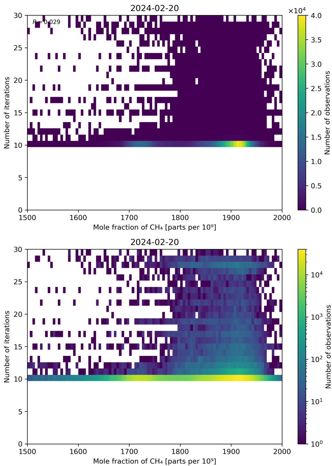
Figure 76: Scatter density plot of “Mole fraction of CH 4 ” against “Number of iterations” for 2024-02-19 to 2024-02-21.
