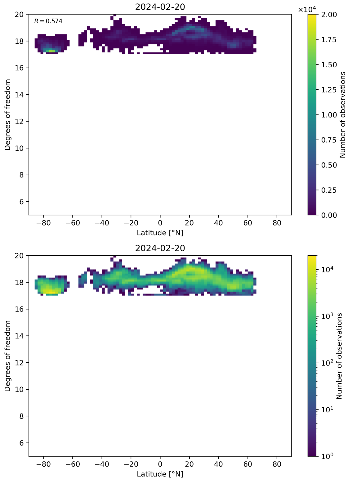
Figure 55: Scatter density plot of “Latitude” against “Degrees of freedom” for 2024-02-19 to 2024-02-21.
