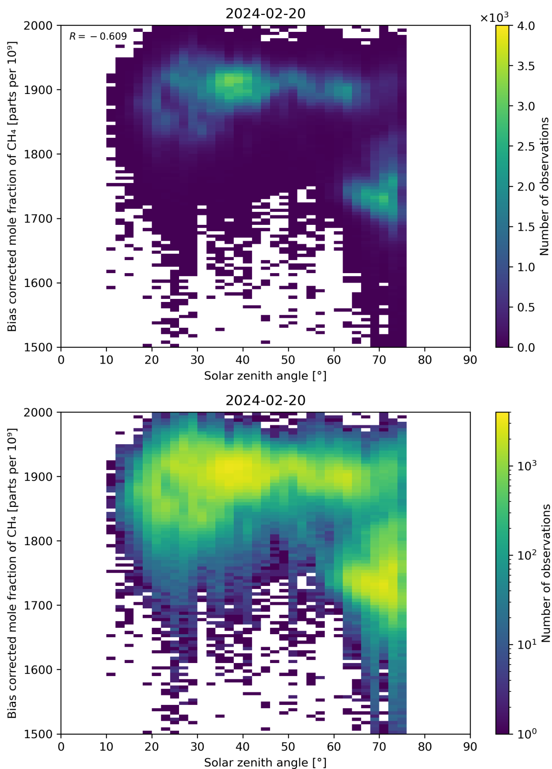
Figure 100: Scatter density plot of “Solar zenith angle” against “Bias corrected mole fraction of \text{CH}_4 ” for 2024-02-19 to 2024-02-21.
