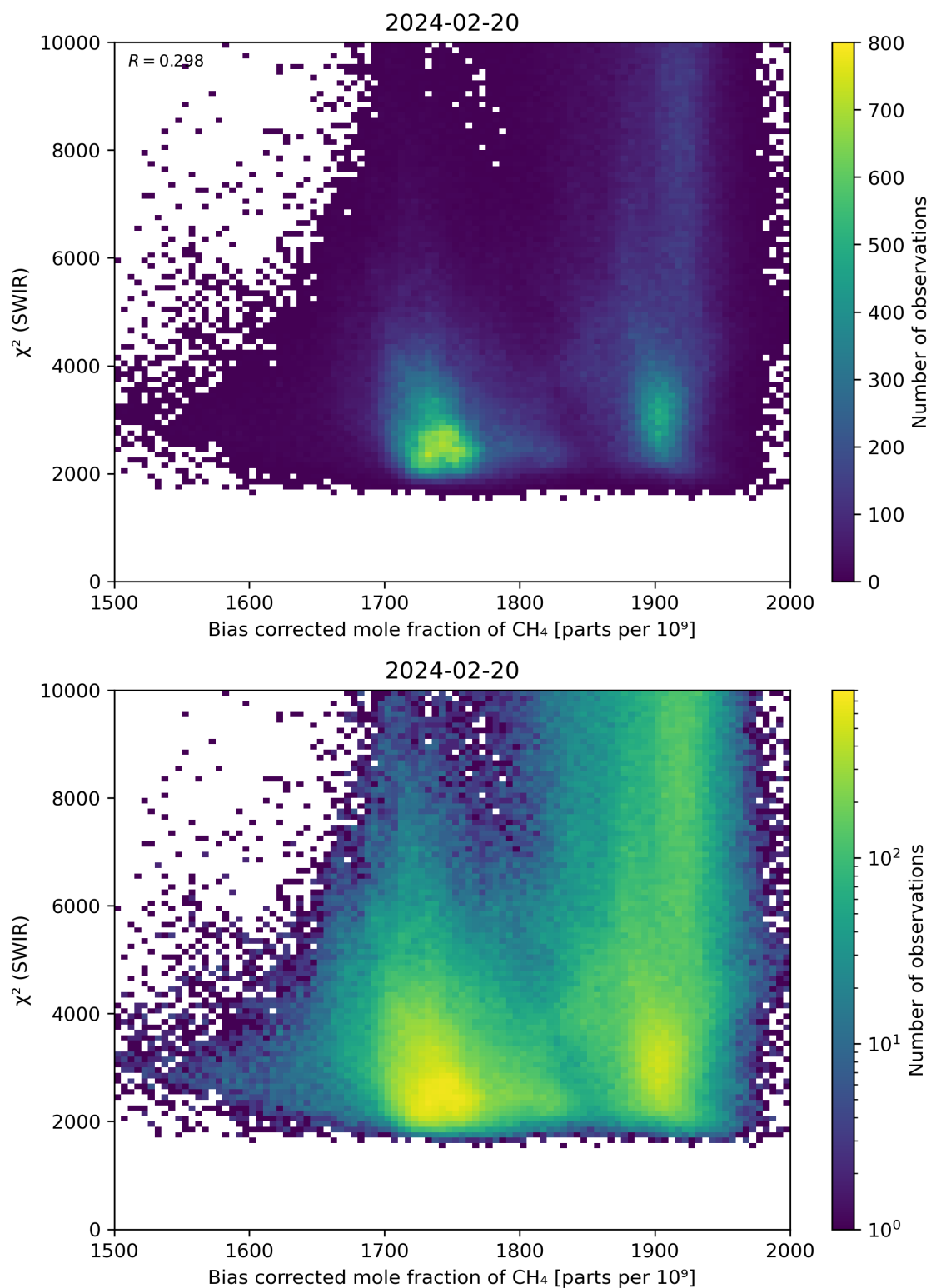
Figure 64: Scatter density plot of “Bias corrected mole fraction of CH 4 ” against “ \chi^2 (SWIR)” for 2024-02-19 to 2024-02-21.
