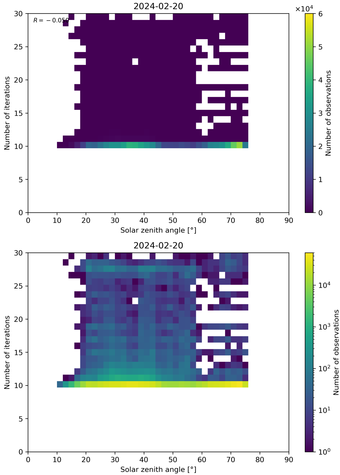
Figure 102: Scatter density plot of “Solar zenith angle” against “Number of iterations” for 2024-02-19 to 2024-02-21.
