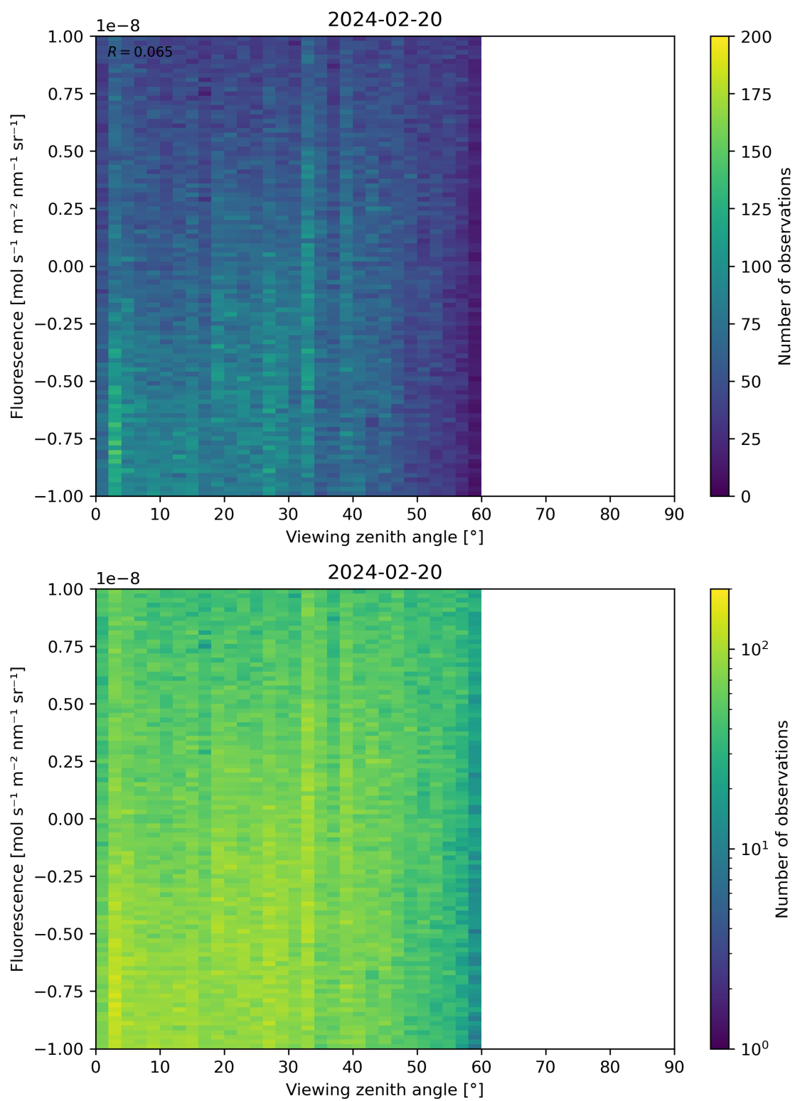
Figure 108: Scatter density plot of “Viewing zenith angle” against “Fluorescence” for 2024-02-19 to 2024-02-21.
