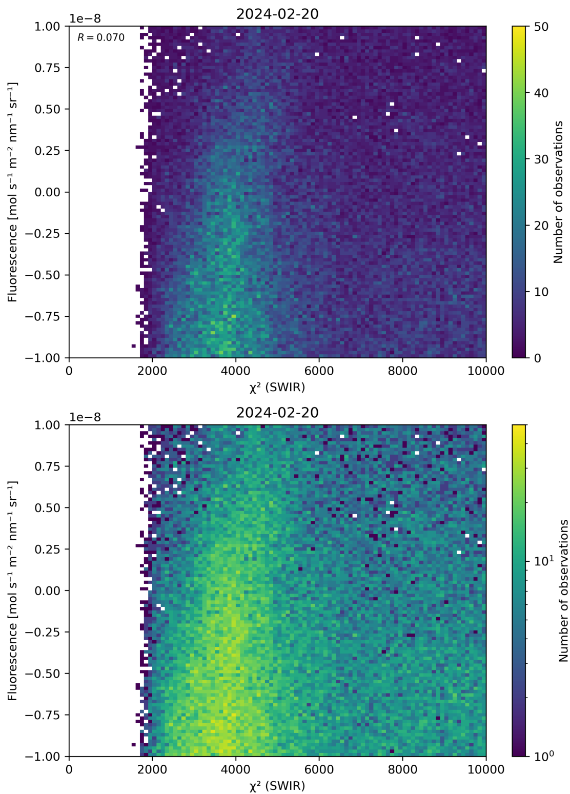
Figure 49: Scatter density plot of “ \chi^2 (SWIR)” against “Fluorescence” for 2024-02-19 to 2024-02-21.
