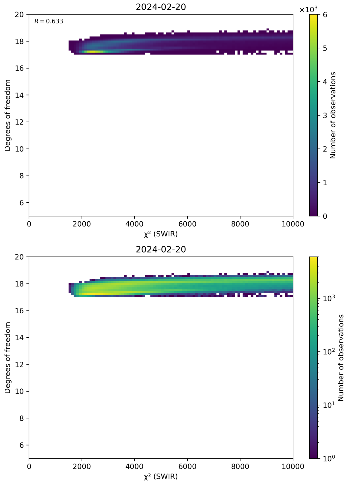
Figure 48: Scatter density plot of “ \chi^2 (SWIR)” against “Degrees of freedom” for 2024-02-19 to 2024-02-21.
