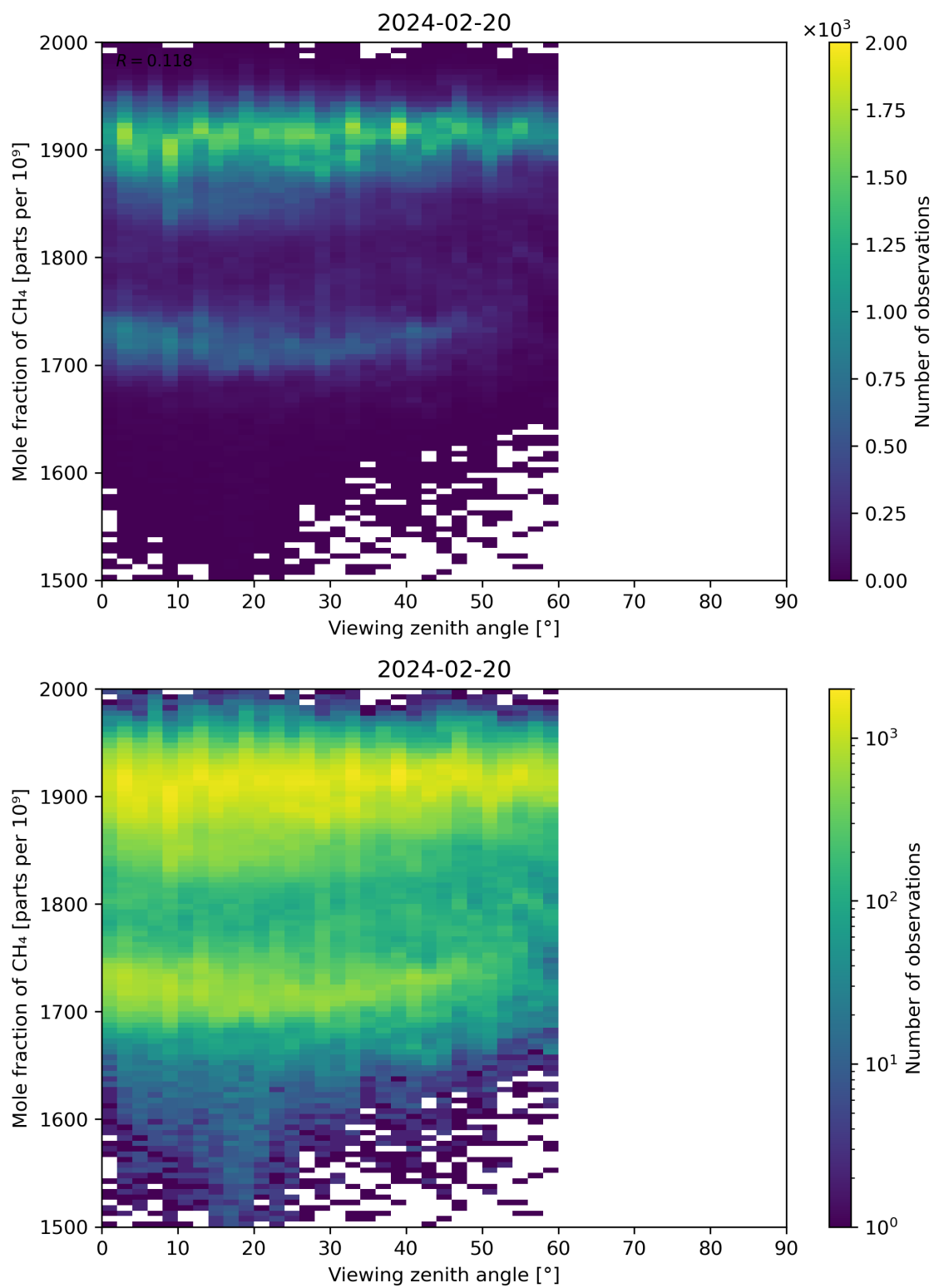
Figure 110: Scatter density plot of “Viewing zenith angle” against “Mole fraction of CH 4 ” for 2024-02-19 to 2024-02-21.
