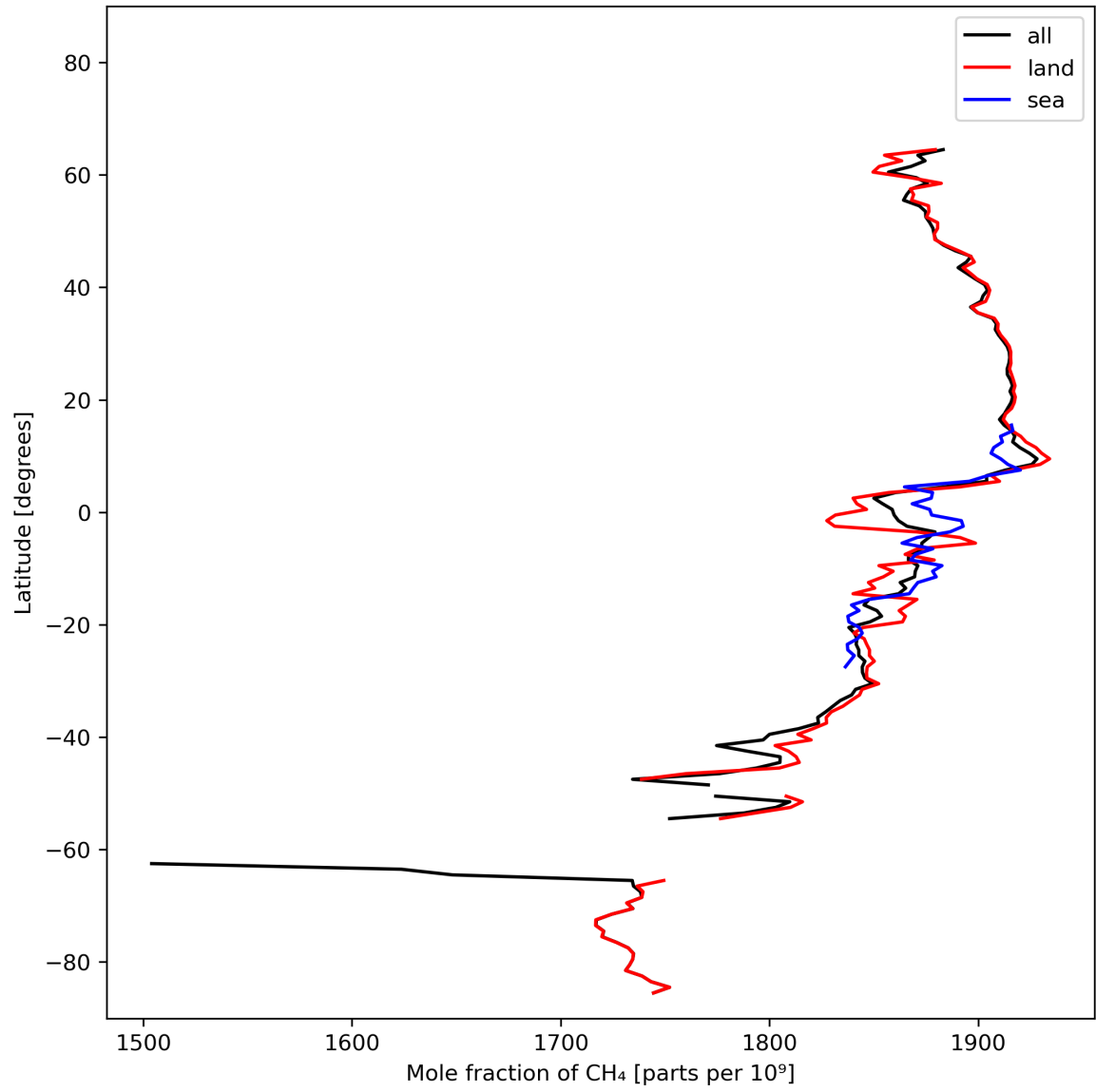
Figure 12: Zonal average of “Mole fraction of \text{CH}_4 ” for 2024-02-19 to 2024-02-21.
