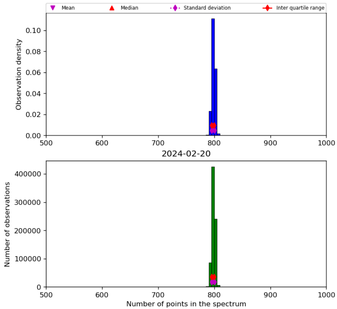
Figure 26: Histogram of “Number of points in the spectrum” for 2024-02-19 to 2024-02-21
