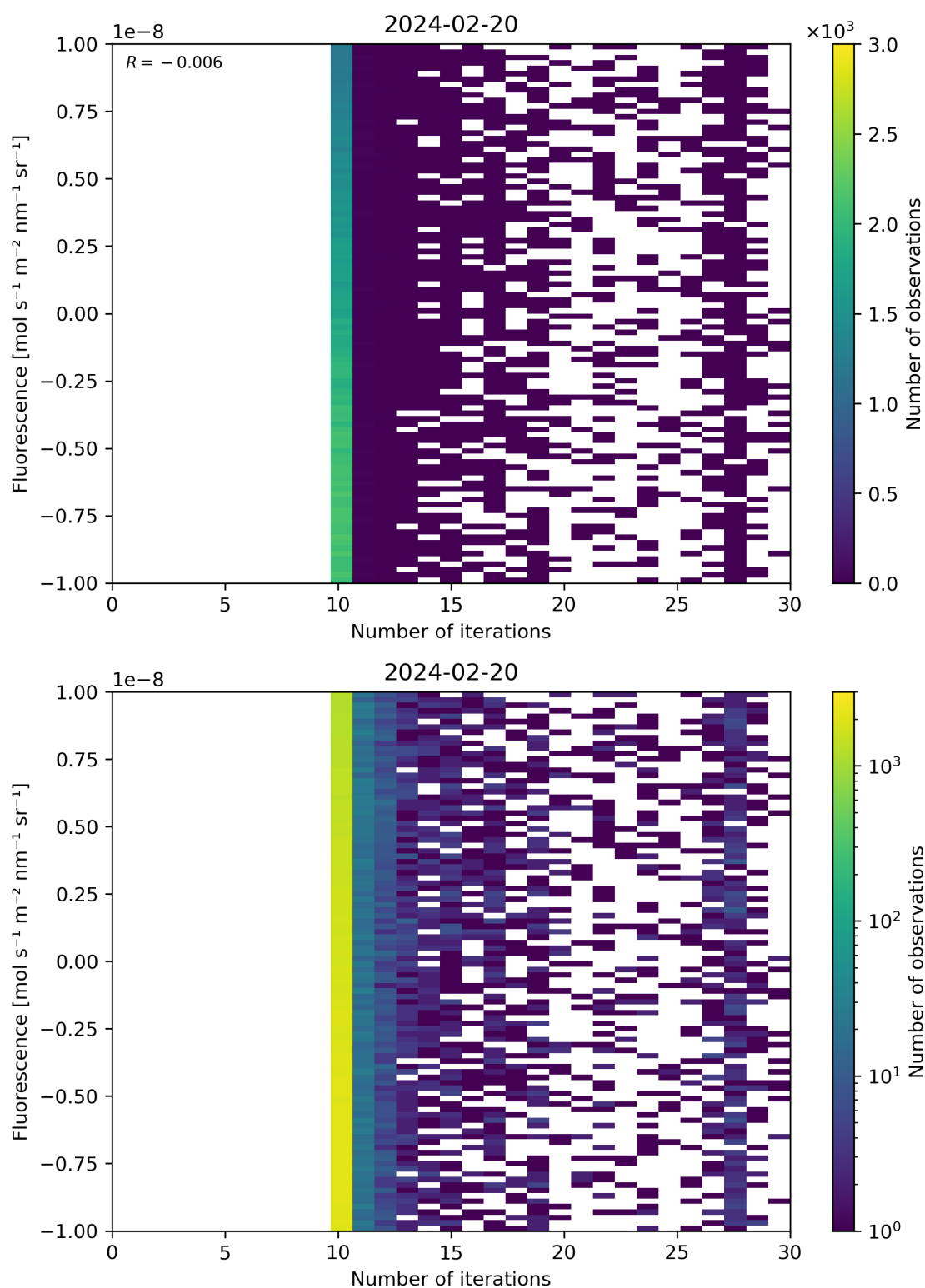
Figure 87: Scatter density plot of “Number of iterations” against “Fluorescence” for 2024-02-19 to 2024-02-21.
