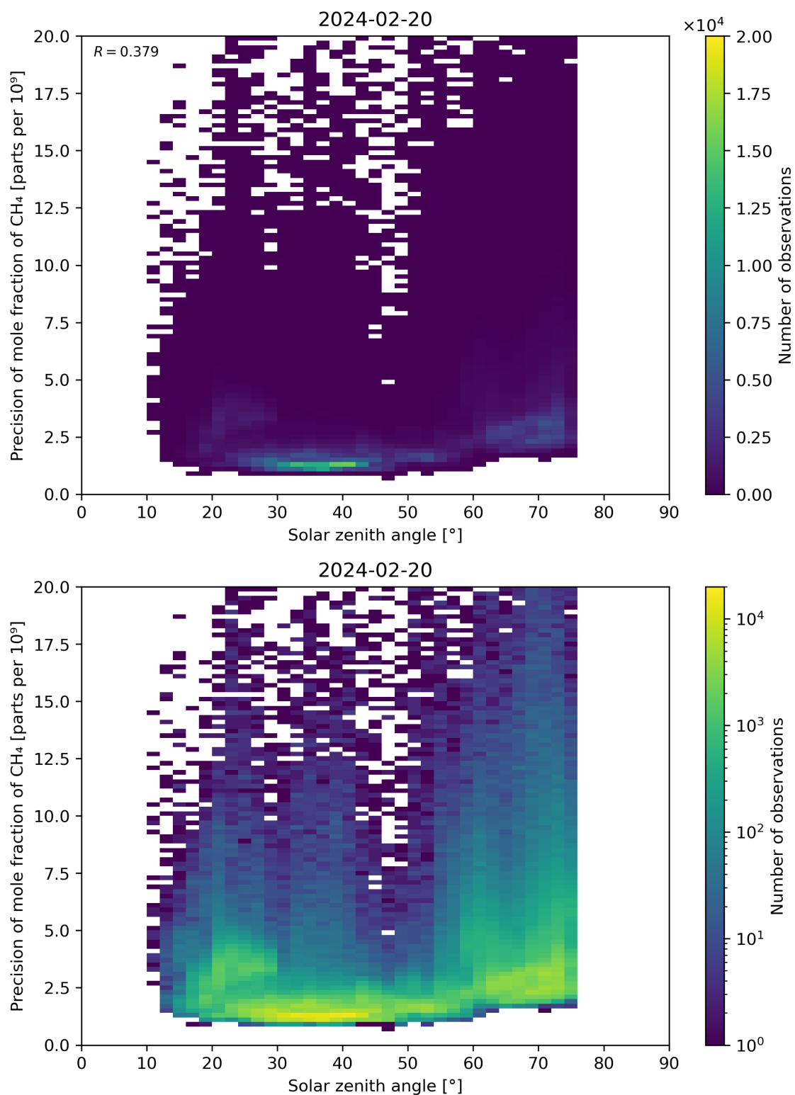
Figure 101: Scatter density plot of “Solar zenith angle” against “Precision of mole fraction of CH 4 ” for 2024-02-19 to 2024-02-21.
