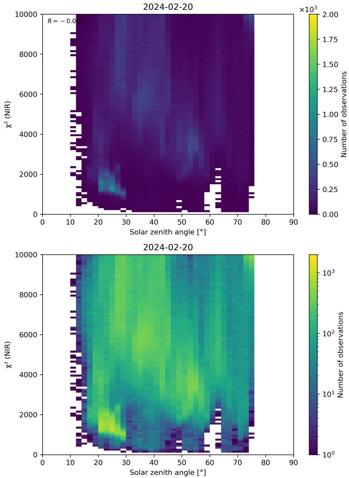
Figure 94: Scatter density plot of “Solar zenith angle” against “ \chi^2 (NIR)” for 2024-02-19 to 2024-02-21.
