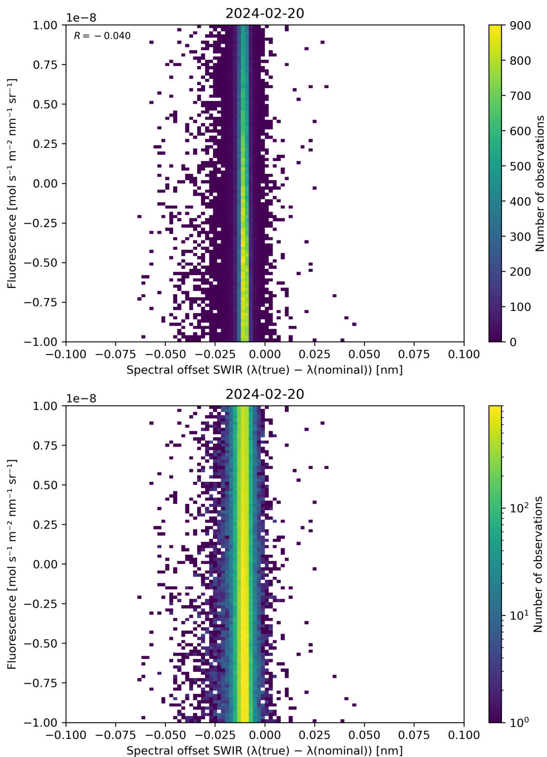
Figure 120: Scatter density plot of “Spectral offset SWIR ( \lambda(\text{true}) - \lambda(\text{nominal}) )” against “Fluorescence” for 2024-02-19 to 2024-02-21.
