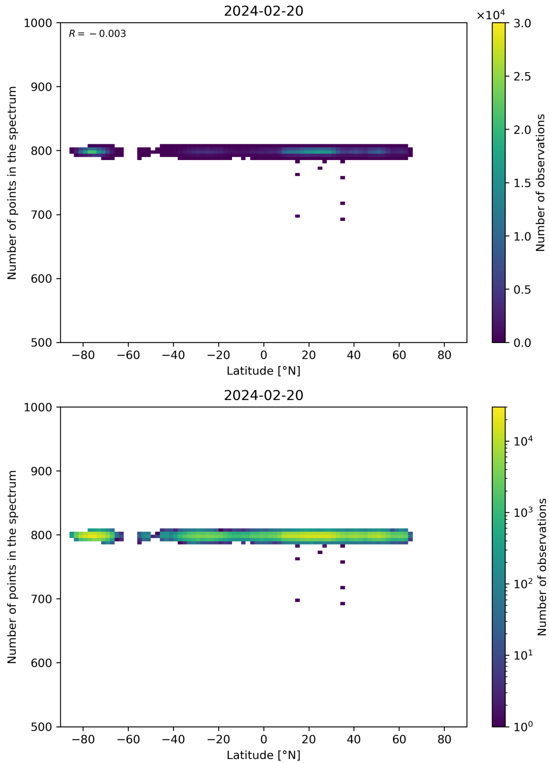
Figure 61: Scatter density plot of “Latitude” against “Number of points in the spectrum” for 2024-02-19 to 2024-02-21.
