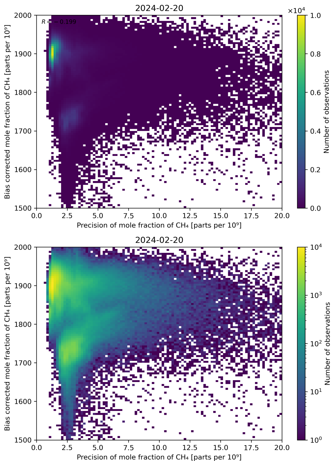
Figure 82: Scatter density plot of “Precision of mole fraction of \text{CH}_4 ” against “Bias corrected mole fraction of \text{CH}_4 ” for 2024-02-19 to 2024-02-21.
