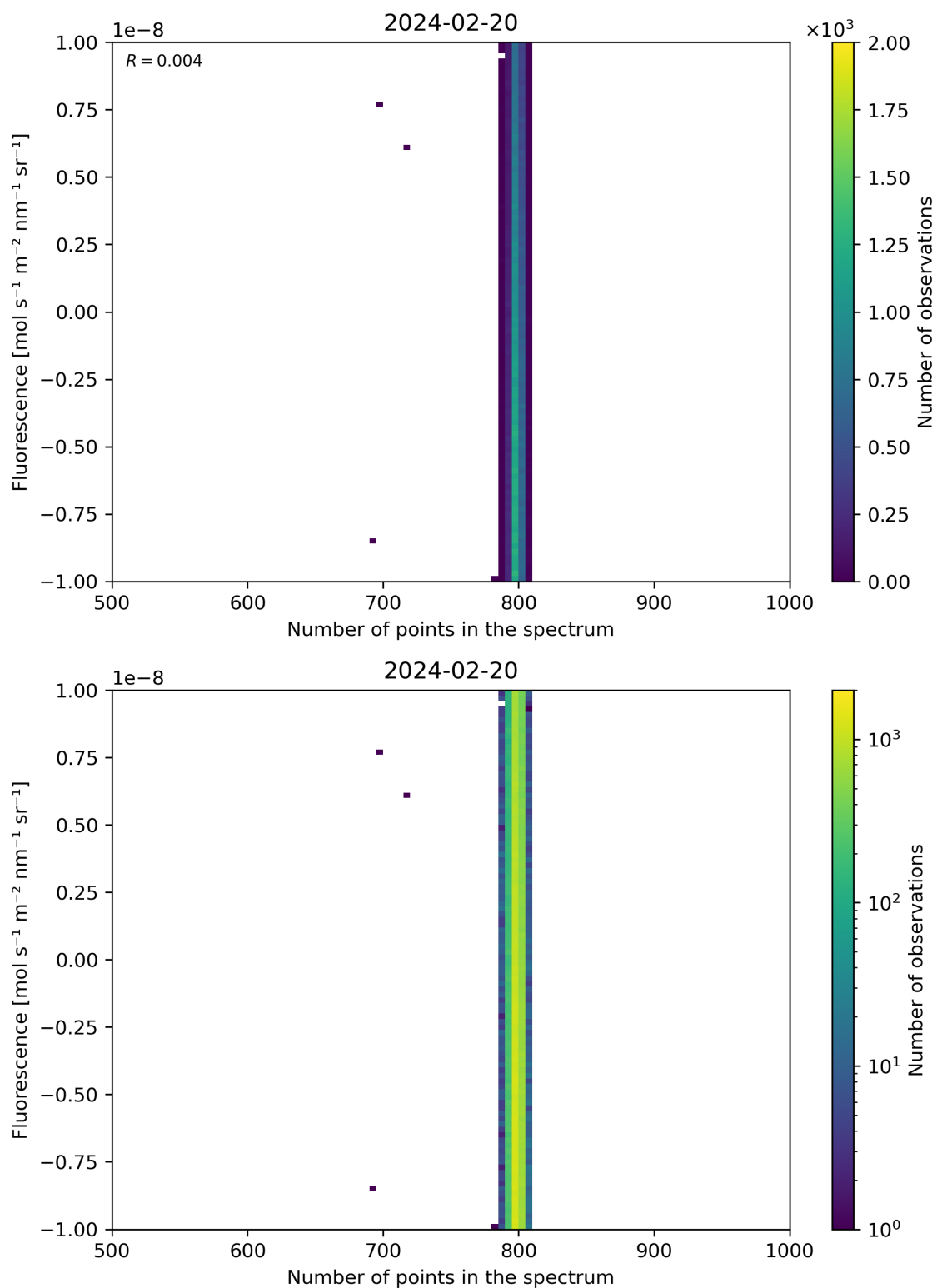
Figure 91: Scatter density plot of “Number of points in the spectrum” against “Fluorescence” for 2024-02-19 to 2024-02-21.
