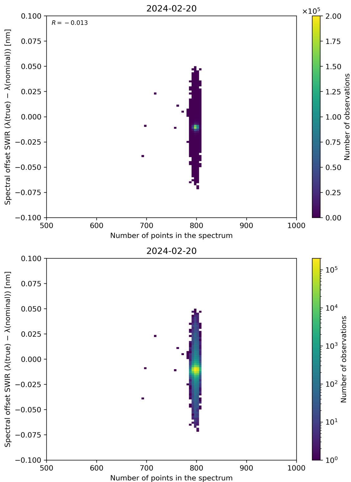
Figure 93: Scatter density plot of “Number of points in the spectrum” against “Spectral offset SWIR ( \lambda(\text{true}) - \lambda(\text{nominal}) )” for 2024-02-19 to 2024-02-21.
