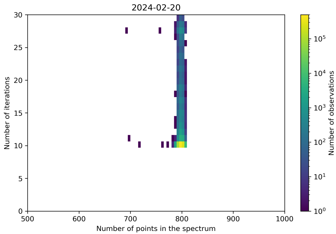
Figure 92: Scatter density plot of “Number of points in the spectrum” against “Number of iterations” for 2024-02-19 to 2024-02-21.
