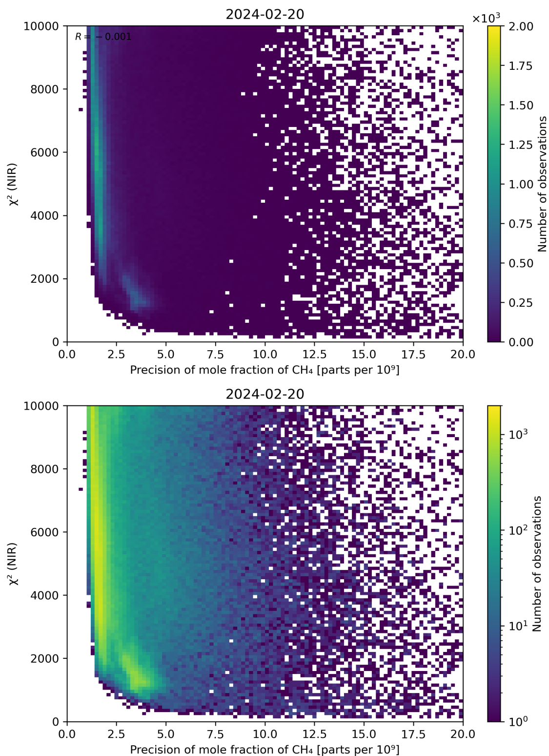
Figure 78: Scatter density plot of “Precision of mole fraction of CH 4 ” against “ \chi^2 (NIR)” for 2024-02-19 to 2024-02-21.
