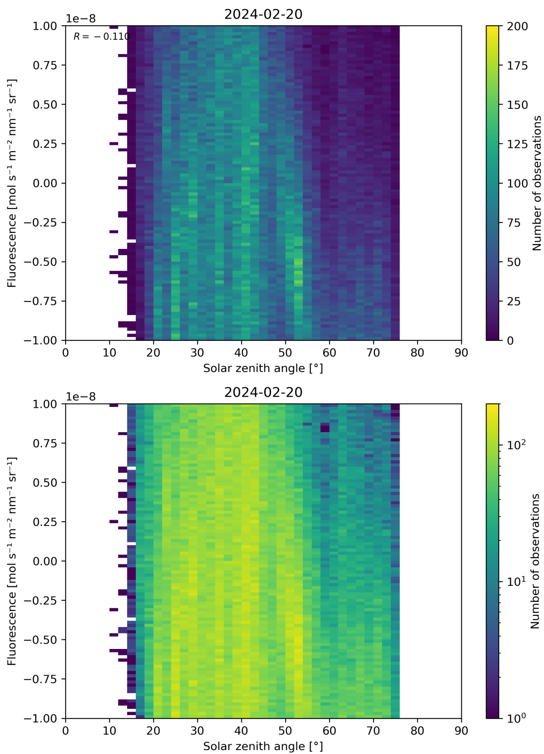
Figure 97: Scatter density plot of “Solar zenith angle” against “Fluorescence” for 2024-02-19 to 2024-02-21.
