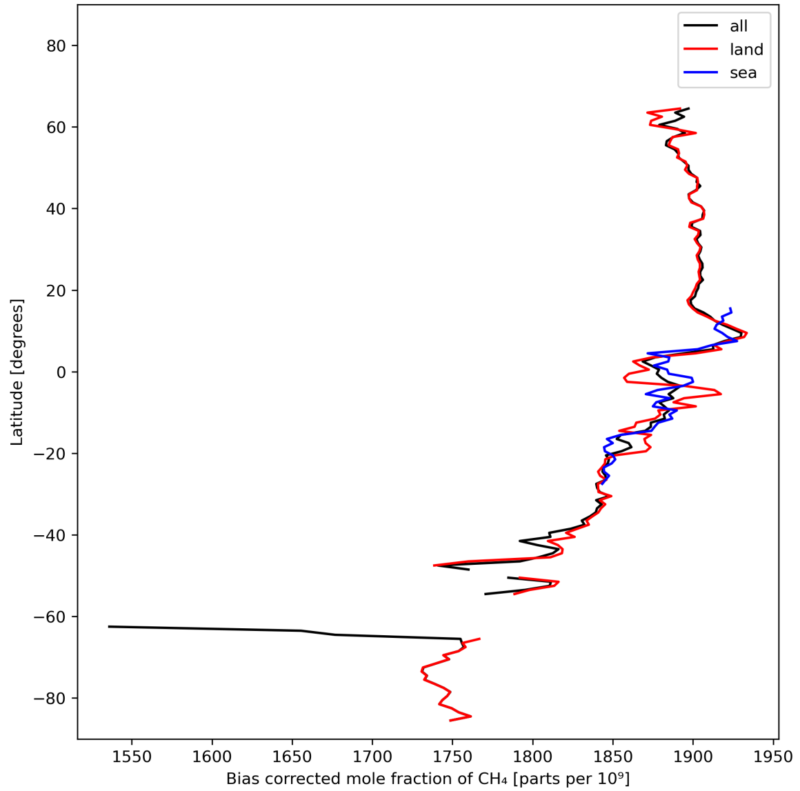
Figure 14: Zonal average of “Bias corrected mole fraction of CH 4 ” for 2024-02-19 to 2024-02-21.
