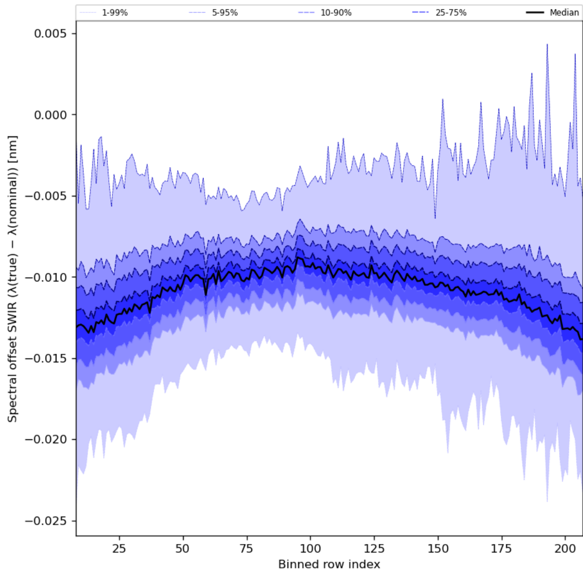
Figure 38: Along track statistics of “Spectral offset SWIR ( \lambda(\text{true}) - \lambda(\text{nominal}) )” for 2024-02-19 to 2024-02-21
