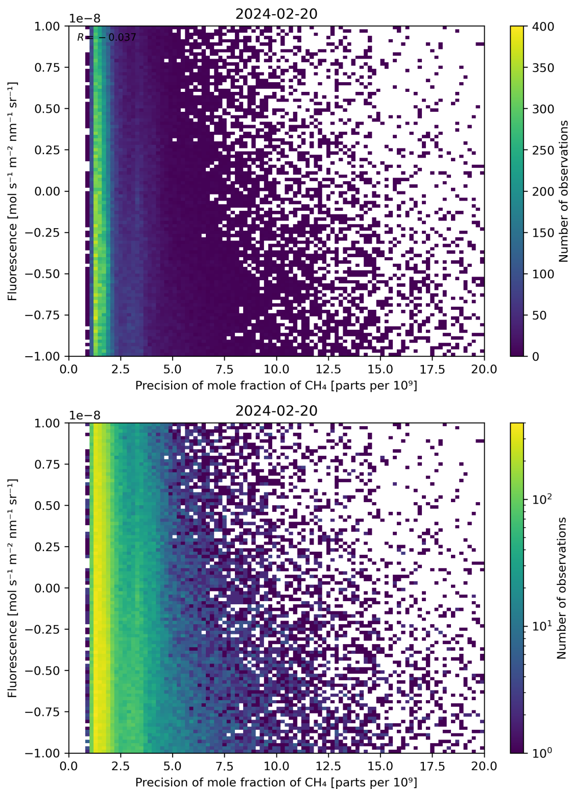
Figure 81: Scatter density plot of “Precision of mole fraction of \text{CH}_4 ” against “Fluorescence” for 2024-02-19 to 2024-02-21.
