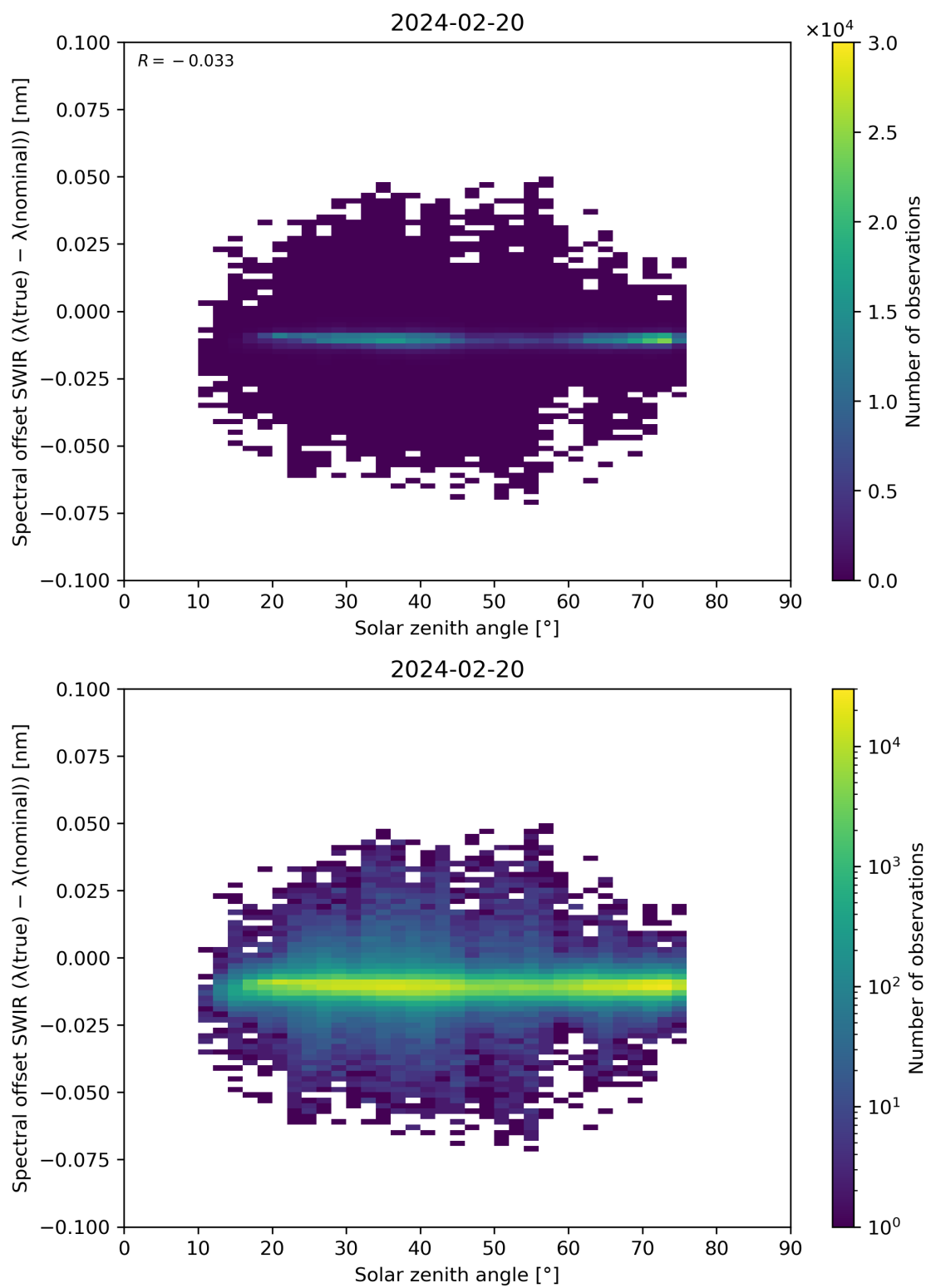
Figure 104: Scatter density plot of “Solar zenith angle” against “Spectral offset SWIR ( \lambda(\text{true}) - \lambda(\text{nominal}) )” for 2024-02-19 to 2024-02-21.
