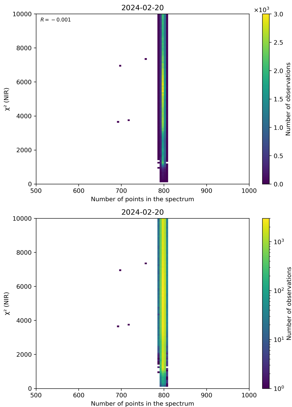
Figure 88: Scatter density plot of “Number of points in the spectrum” against “ \chi^2 (NIR)” for 2024-02-19 to 2024-02-21.
