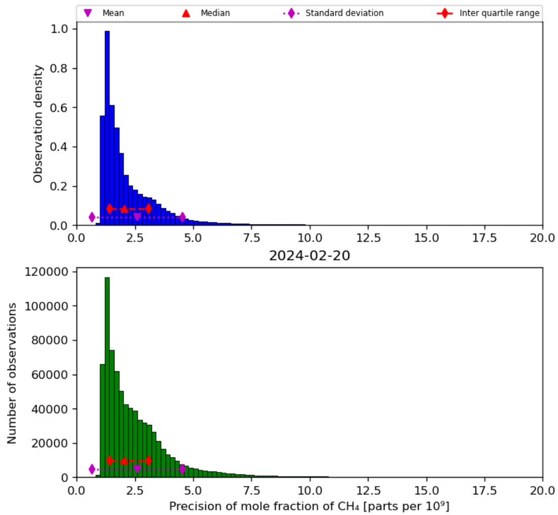
Figure 24: Histogram of “Precision of mole fraction of CH 4 ” for 2024-02-19 to 2024-02-21
