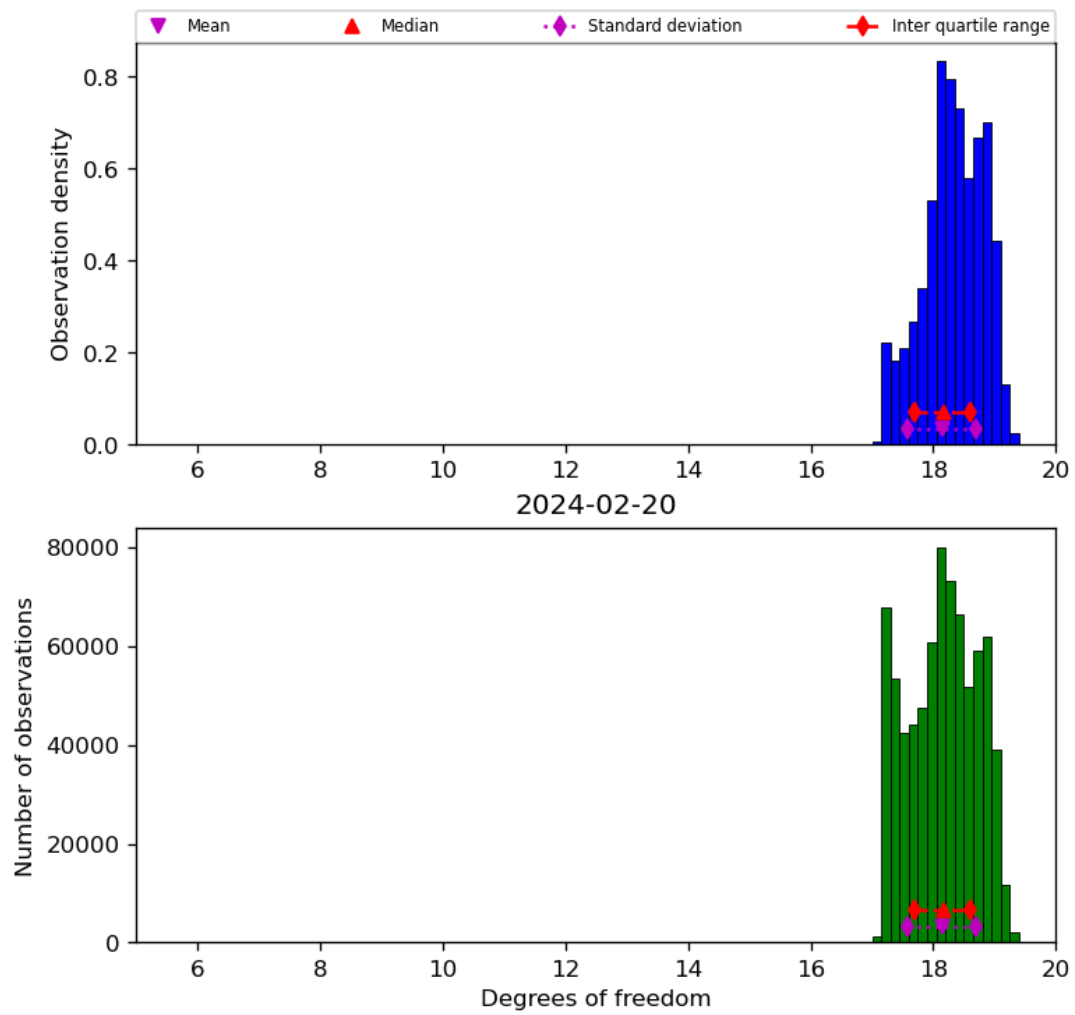
Figure 30: Histogram of “Degrees of freedom” for 2024-02-19 to 2024-02-21
