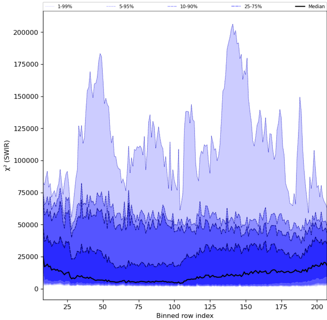
Figure 39: Along track statistics of “ \chi^2 (SWIR)” for 2024-02-19 to 2024-02-21
