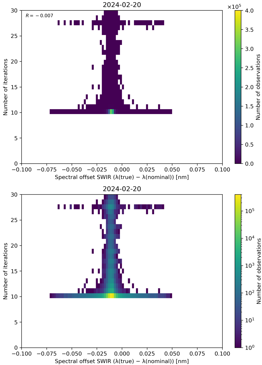
Figure 121: Scatter density plot of “Spectral offset SWIR ( \lambda(\text{true}) - \lambda(\text{nominal}) )” against “Number of iterations” for 2024-02-19 to 2024-02-21.
