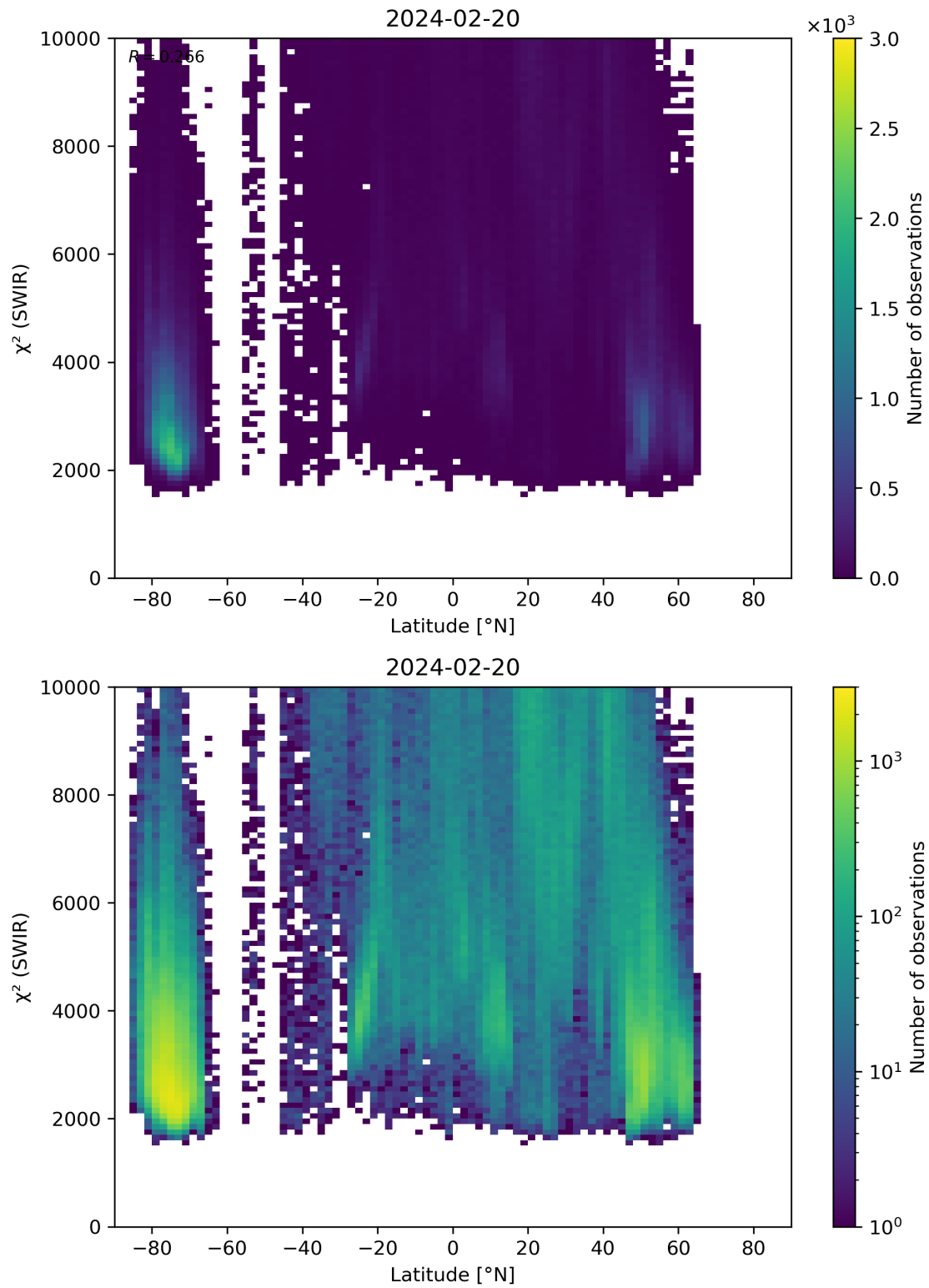
Figure 54: Scatter density plot of “Latitude” against “ \chi^2 (SWIR)” for 2024-02-19 to 2024-02-21.
