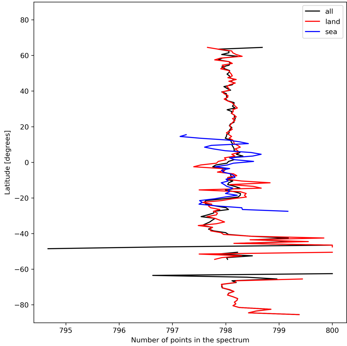
Figure 15: Zonal average of “Number of points in the spectrum” for 2024-02-19 to 2024-02-21.
