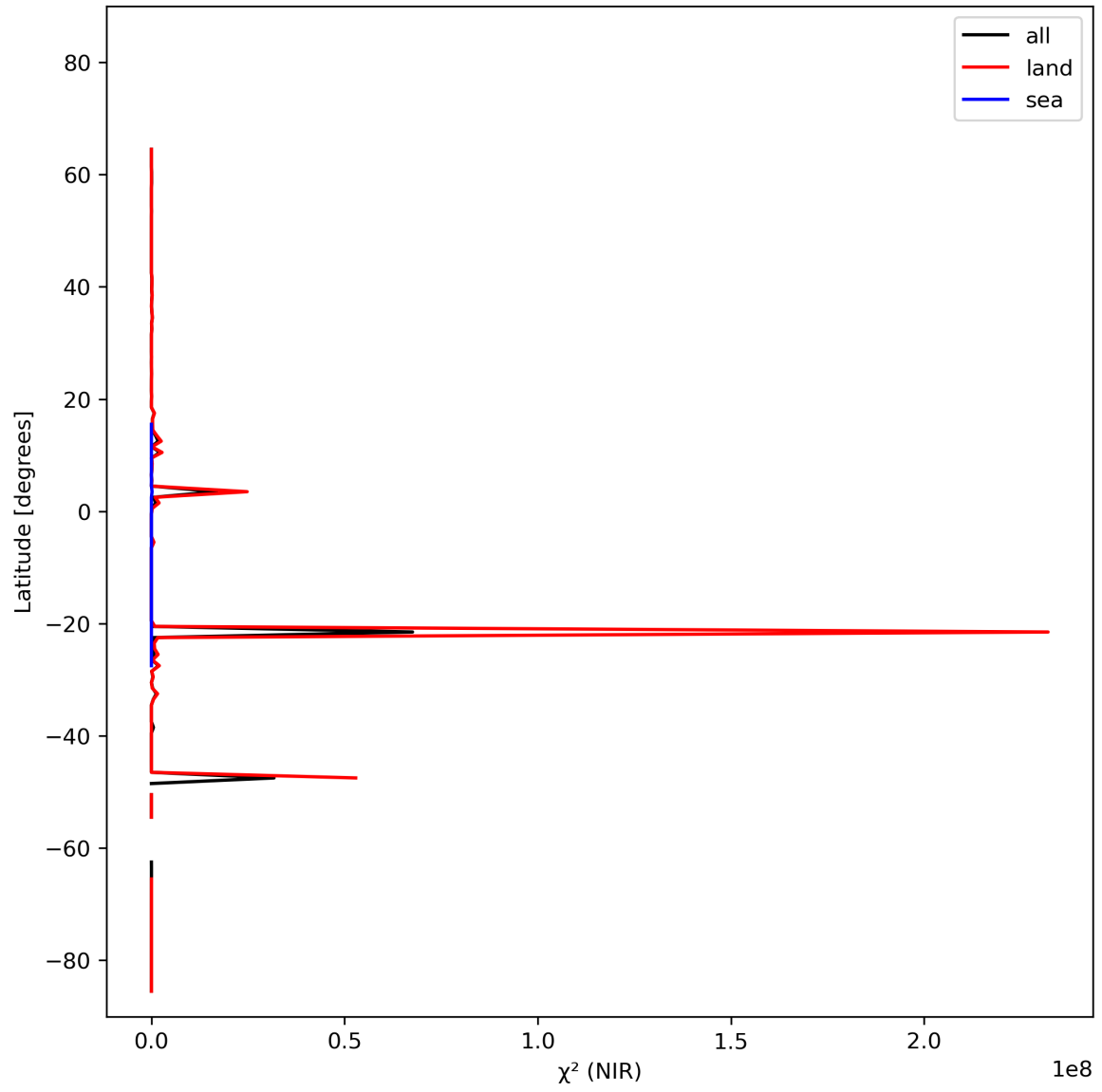
Figure 18: Zonal average of “ \chi^2 (NIR)” for 2024-02-19 to 2024-02-21.
