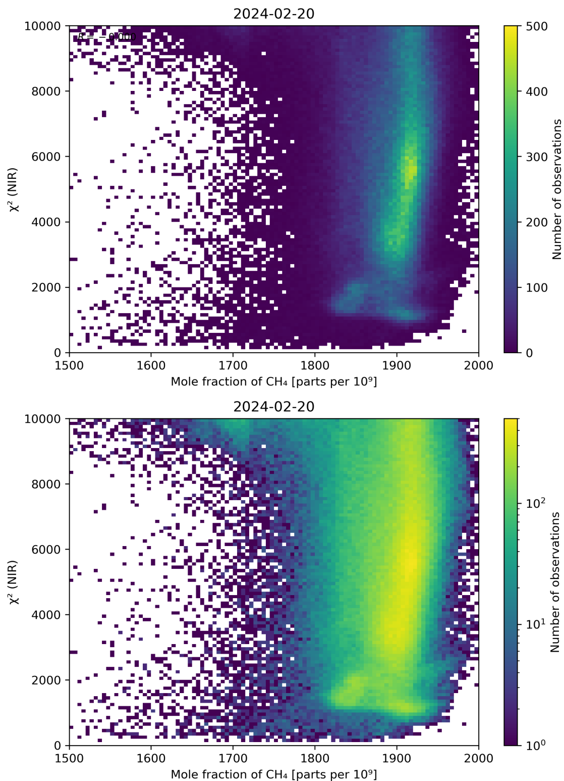
Figure 70: Scatter density plot of “Mole fraction of \text{CH}_4 ” against “ \chi^2 (NIR)” for 2024-02-19 to 2024-02-21.
