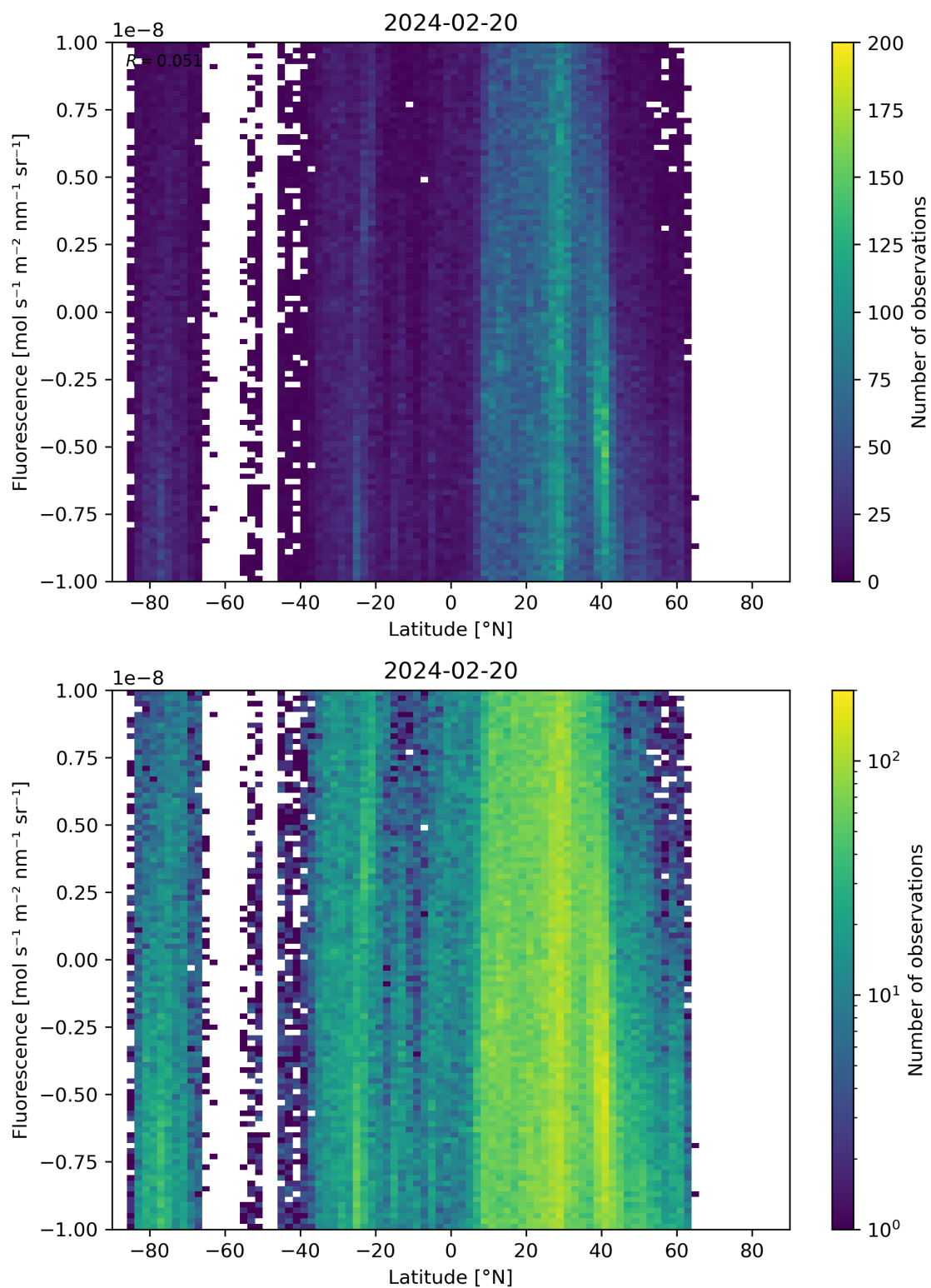
Figure 56: Scatter density plot of “Latitude” against “Fluorescence” for 2024-02-19 to 2024-02-21.
