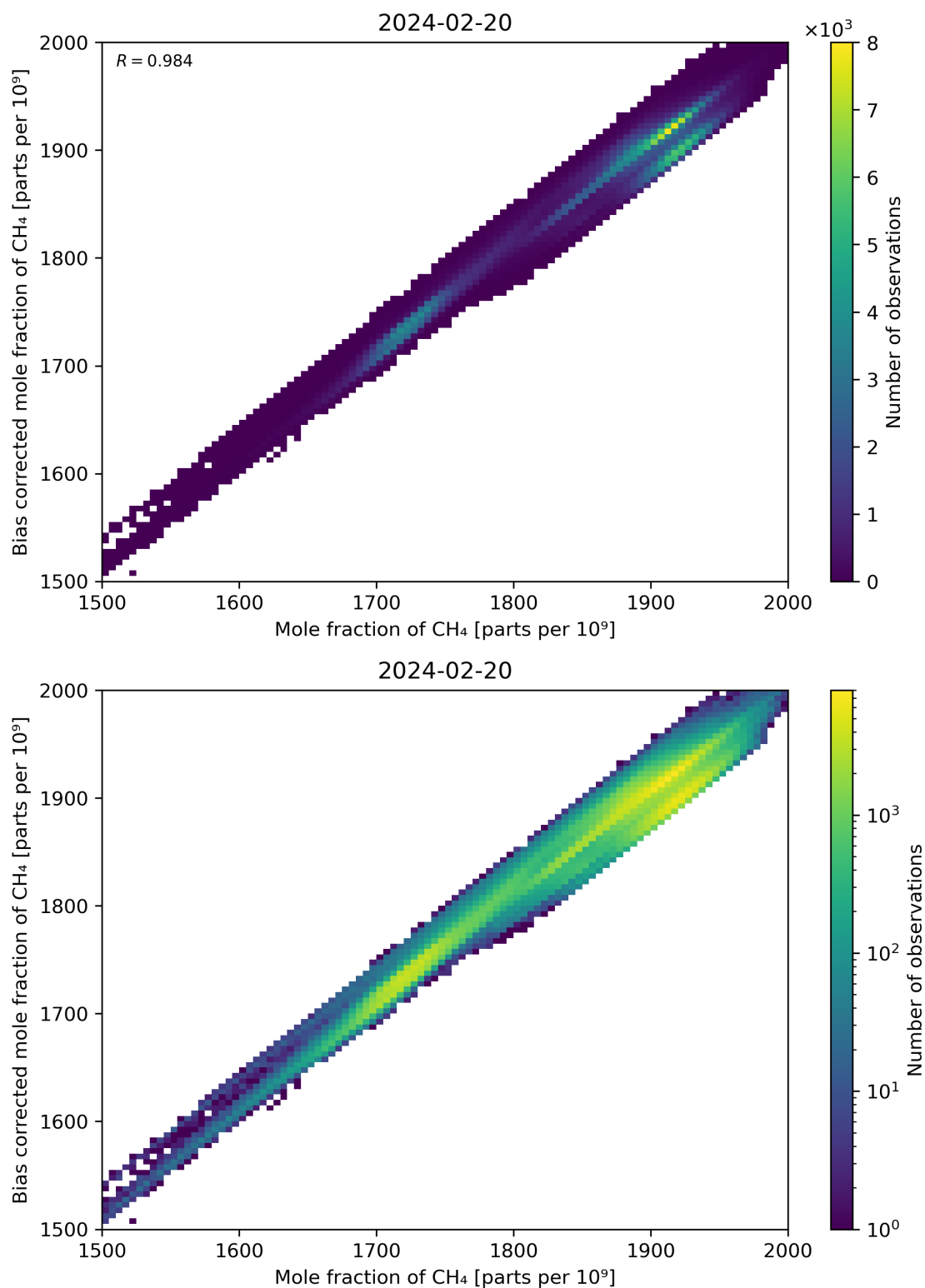
Figure 74: Scatter density plot of “Mole fraction of CH 4 ” against “Bias corrected mole fraction of CH 4 ” for 2024-02-19 to 2024-02-21.
