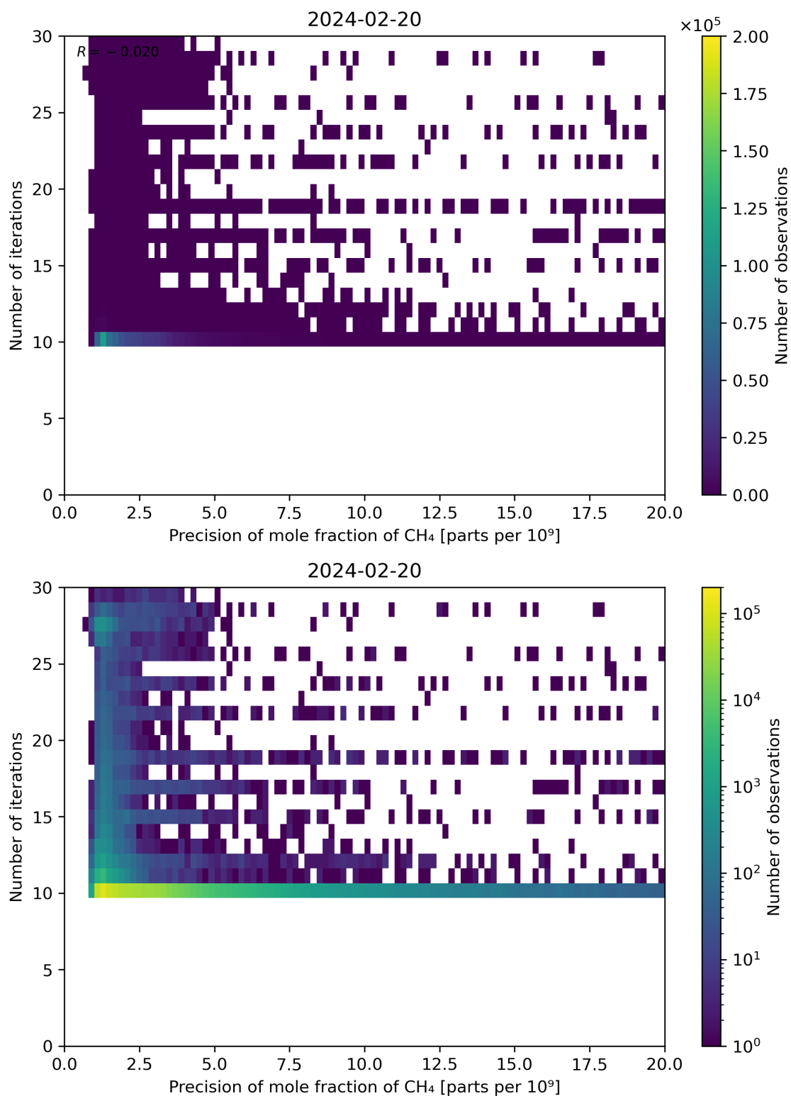
Figure 83: Scatter density plot of “Precision of mole fraction of CH 4 ” against “Number of iterations” for 2024-02-19 to 2024-02-21.
