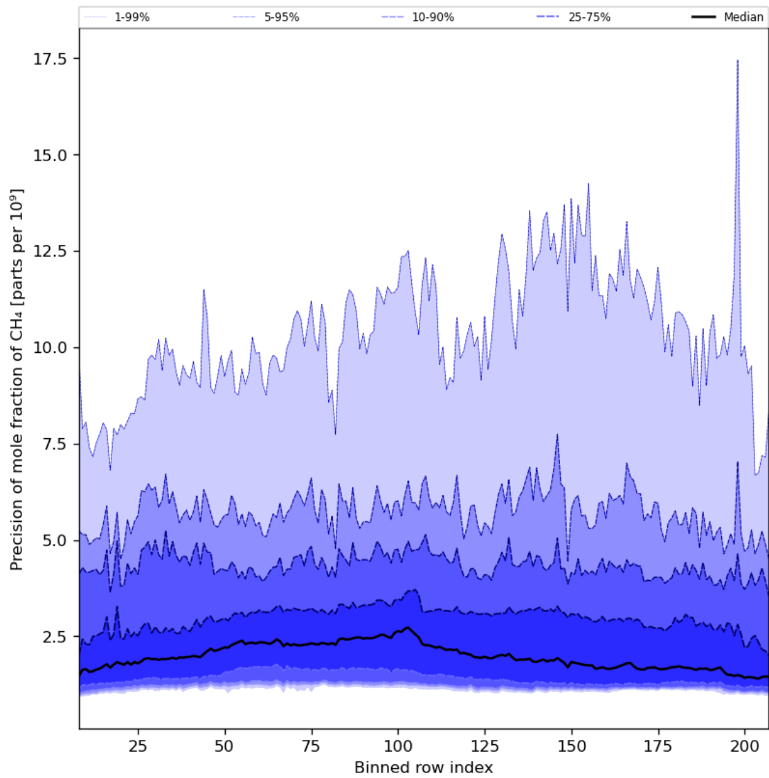
Figure 35: Along track statistics of “Precision of mole fraction of CH 4 ” for 2024-02-19 to 2024-02-21
