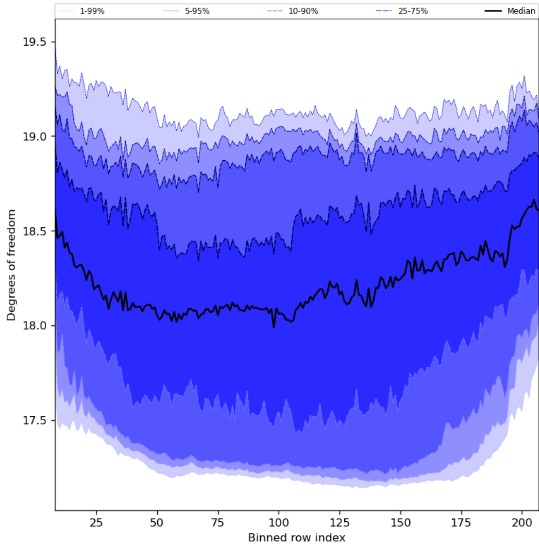
Figure 41: Along track statistics of “Degrees of freedom” for 2024-02-19 to 2024-02-21
