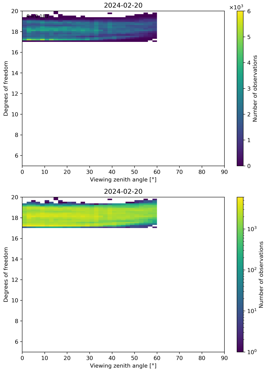
Figure 107: Scatter density plot of “Viewing zenith angle” against “Degrees of freedom” for 2024-02-19 to 2024-02-21.
