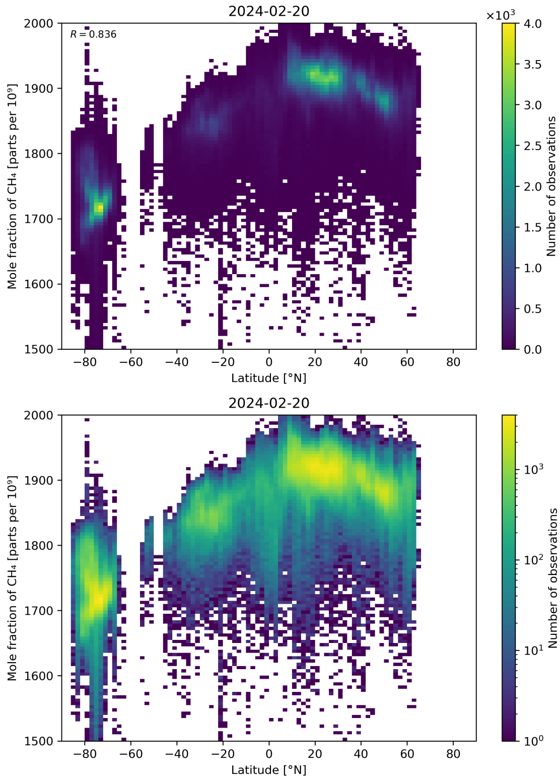
Figure 57: Scatter density plot of “Latitude” against “Mole fraction of CH 4 ” for 2024-02-19 to 2024-02-21.
