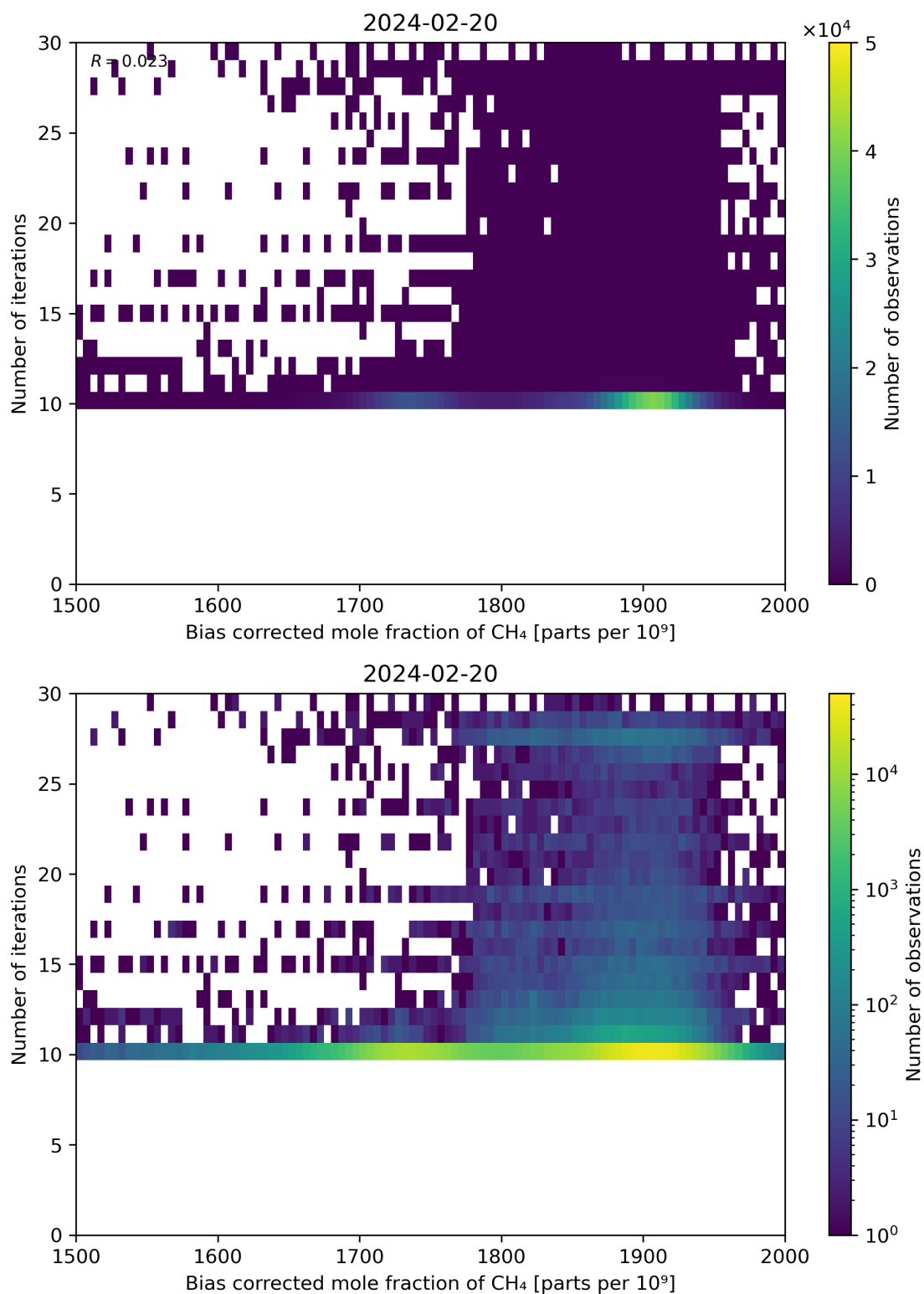
Figure 67: Scatter density plot of “Bias corrected mole fraction of \text{CH}_4 ” against “Number of iterations” for 2024-02-19 to 2024-02-21.
