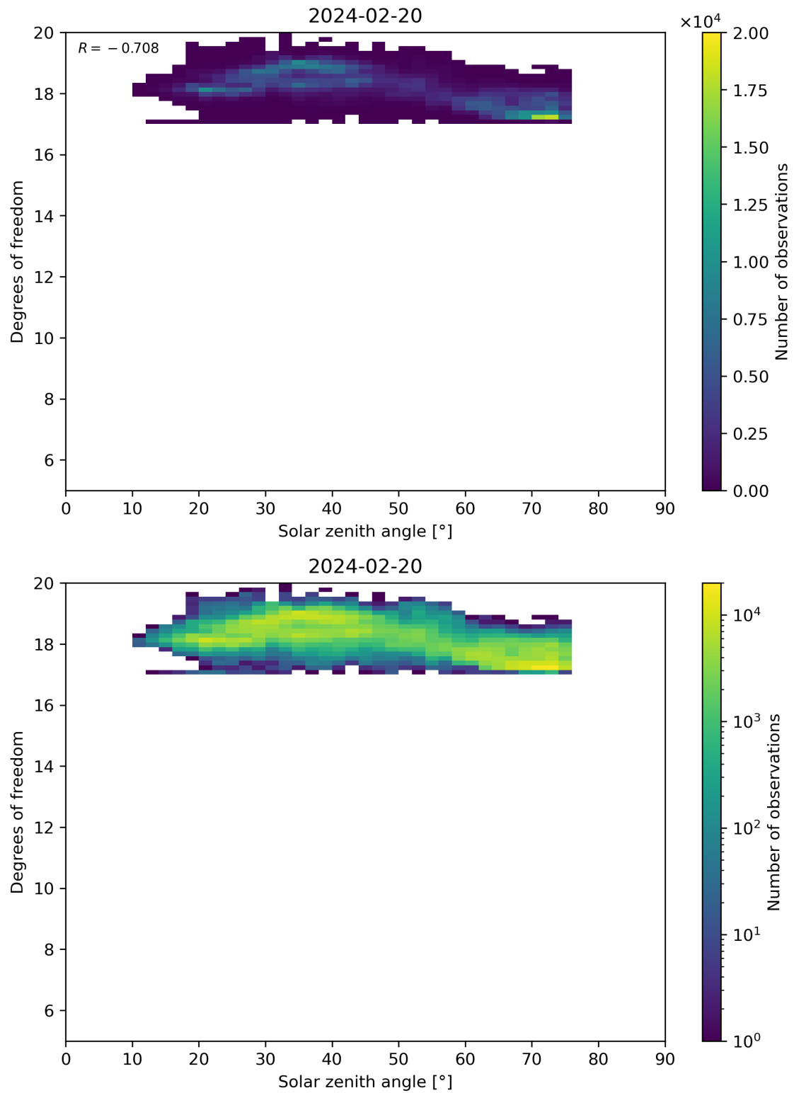
Figure 96: Scatter density plot of “Solar zenith angle” against “Degrees of freedom” for 2024-02-19 to 2024-02-21.
