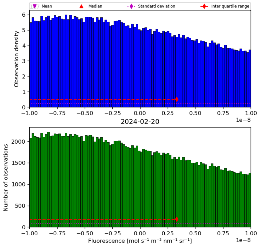
Figure 32: Histogram of “Fluorescence” for 2024-02-19 to 2024-02-21
