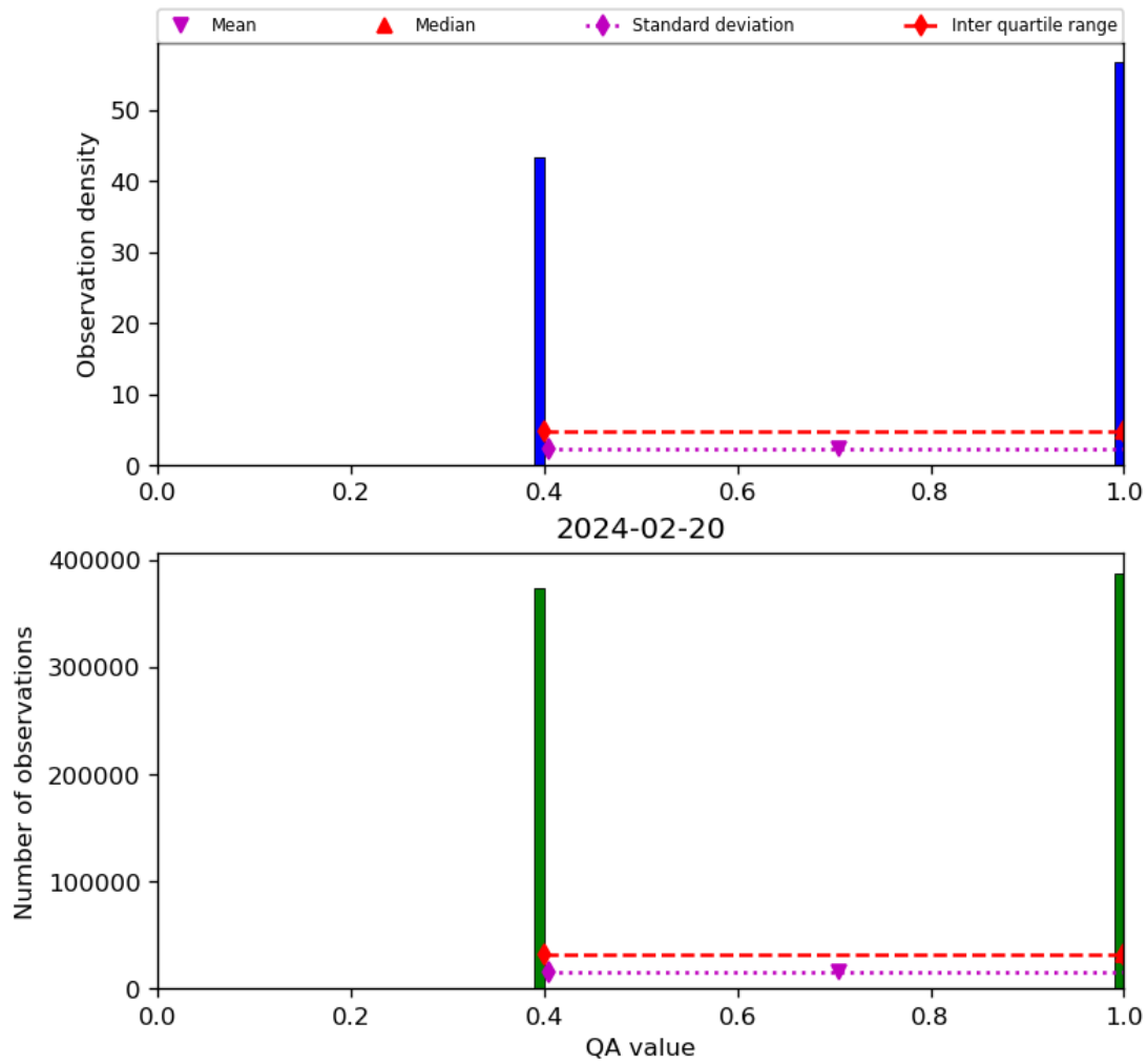
Figure 22: Histogram of “QA value” for 2024-02-19 to 2024-02-21
