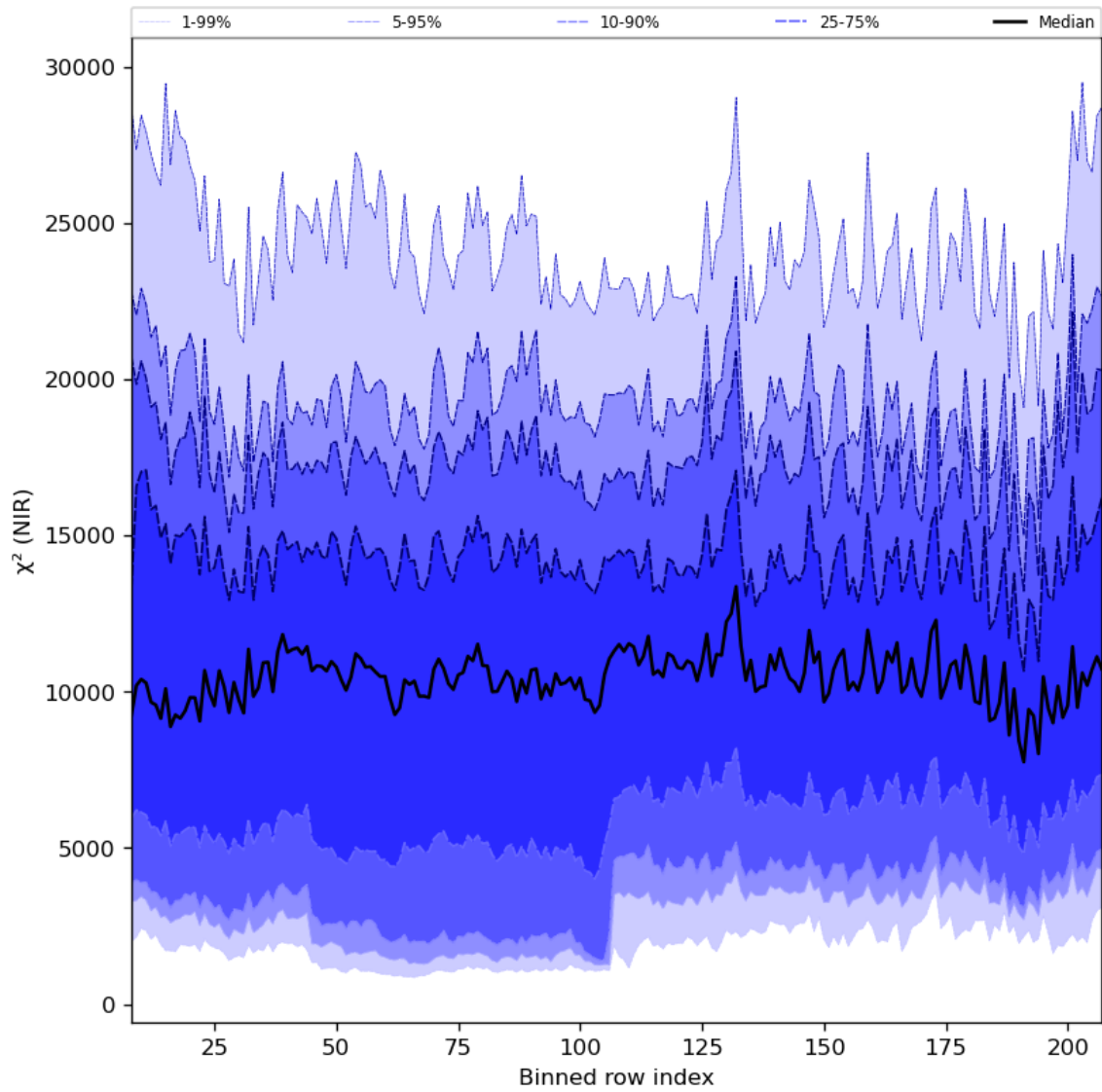
Figure 40: Along track statistics of “ \chi^2 (NIR)” for 2024-02-19 to 2024-02-21
