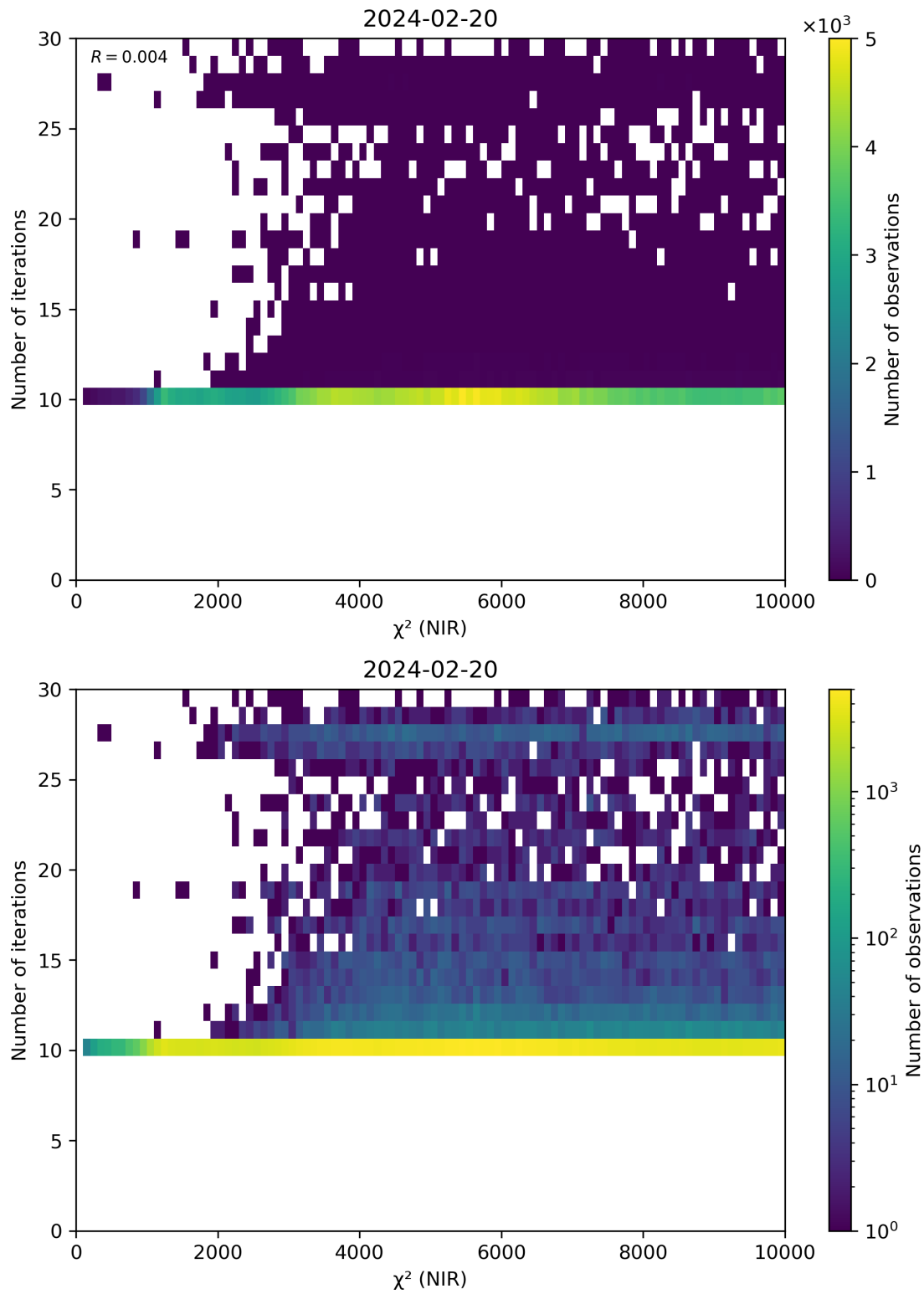
Figure 46: Scatter density plot of “ \chi^2 (NIR)” against “Number of iterations” for 2024-02-19 to 2024-02-21.
