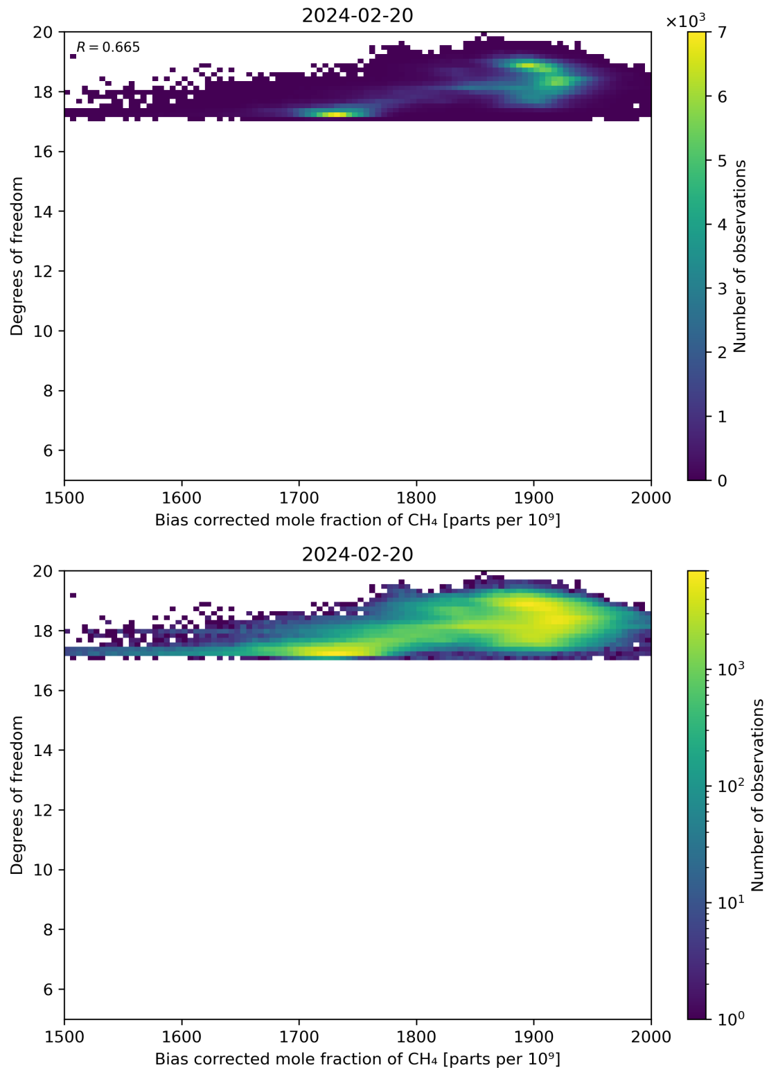
Figure 65: Scatter density plot of “Bias corrected mole fraction of CH 4 ” against “Degrees of freedom” for 2024-02-19 to 2024-02-21.
