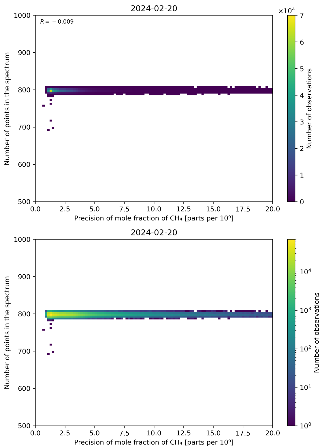
Figure 84: Scatter density plot of “Precision of mole fraction of CH 4 ” against “Number of points in the spectrum” for 2024-02-19 to 2024-02-21.
