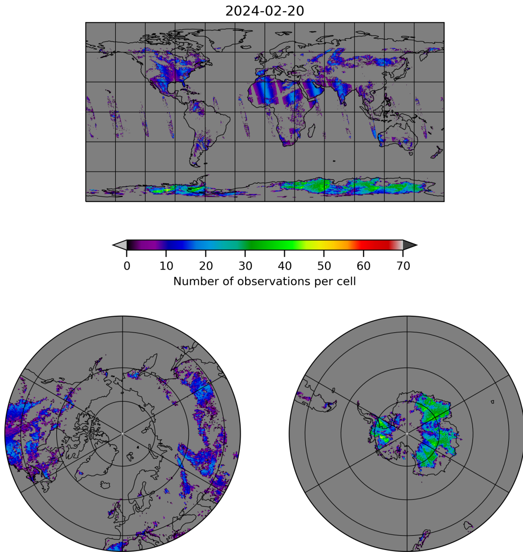
Figure 10: Map of the number of observations for 2024-02-19 to 2024-02-21
