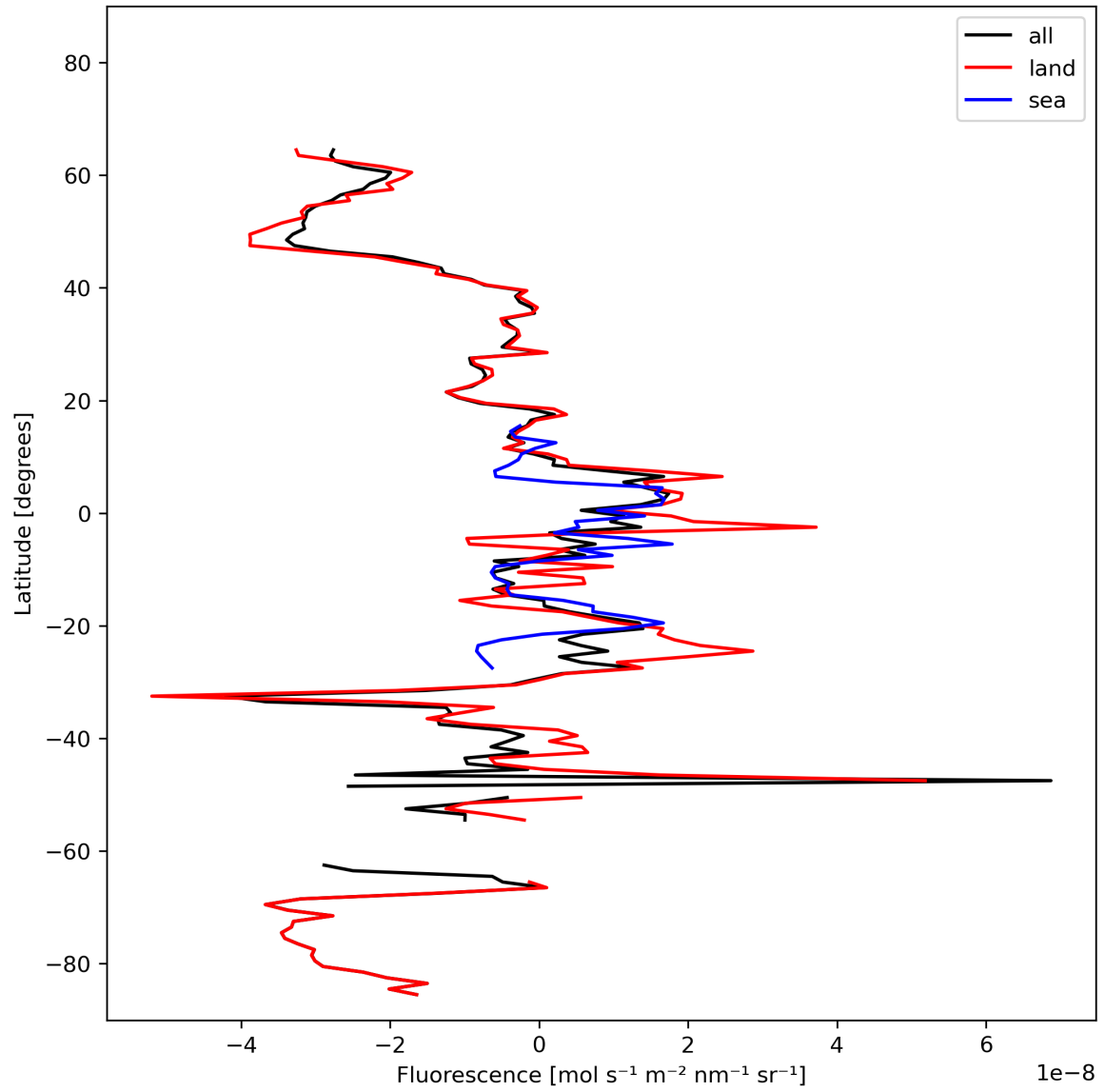
Figure 21: Zonal average of “Fluorescence” for 2024-02-19 to 2024-02-21.
