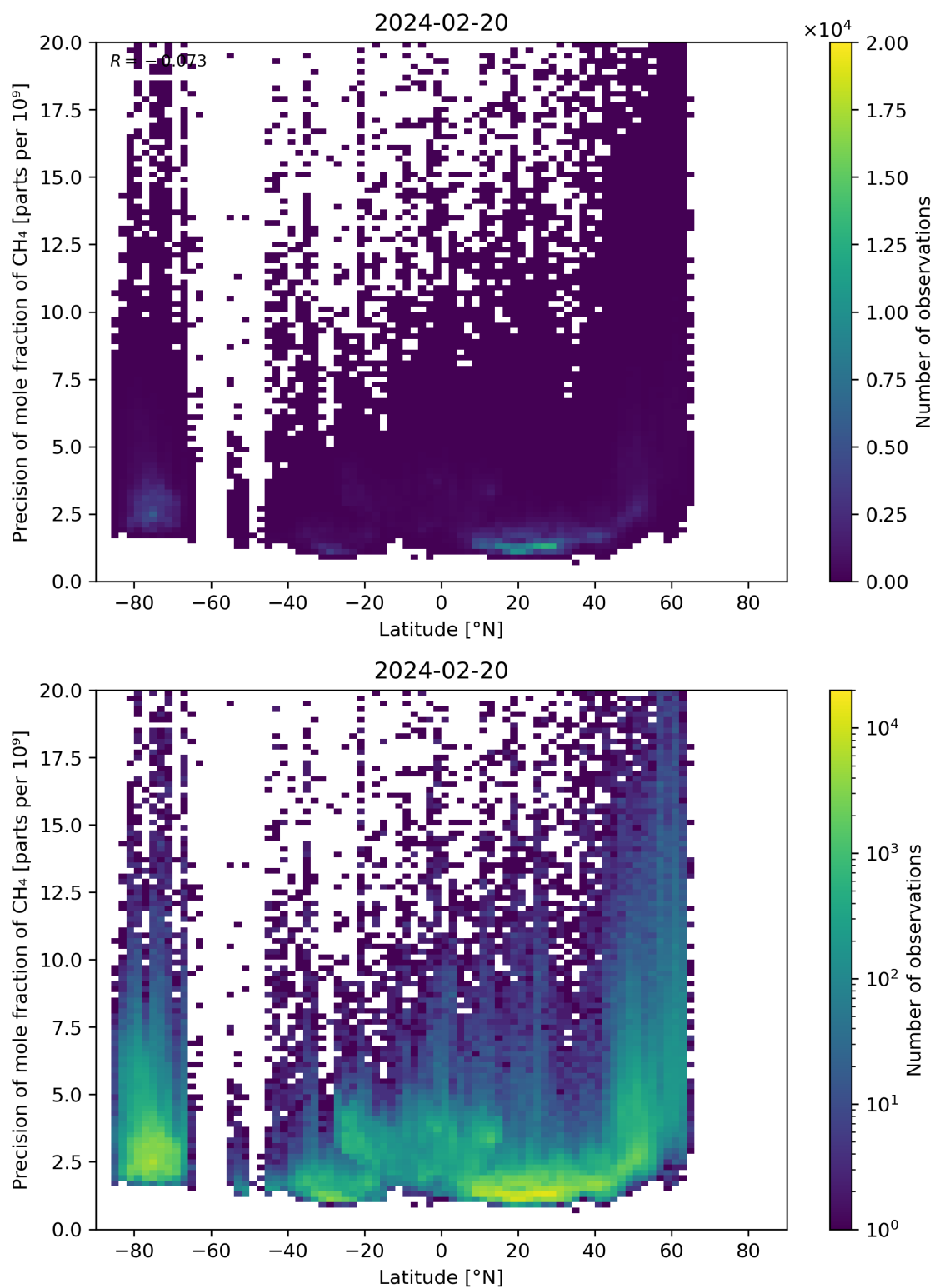
Figure 59: Scatter density plot of “Latitude” against “Precision of mole fraction of CH 4 ” for 2024-02-19 to 2024-02-21.
