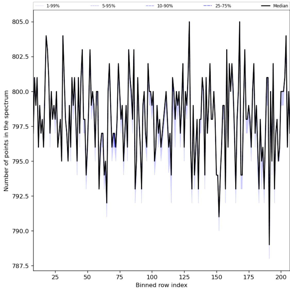
Figure 37: Along track statistics of “Number of points in the spectrum” for 2024-02-19 to 2024-02-21
