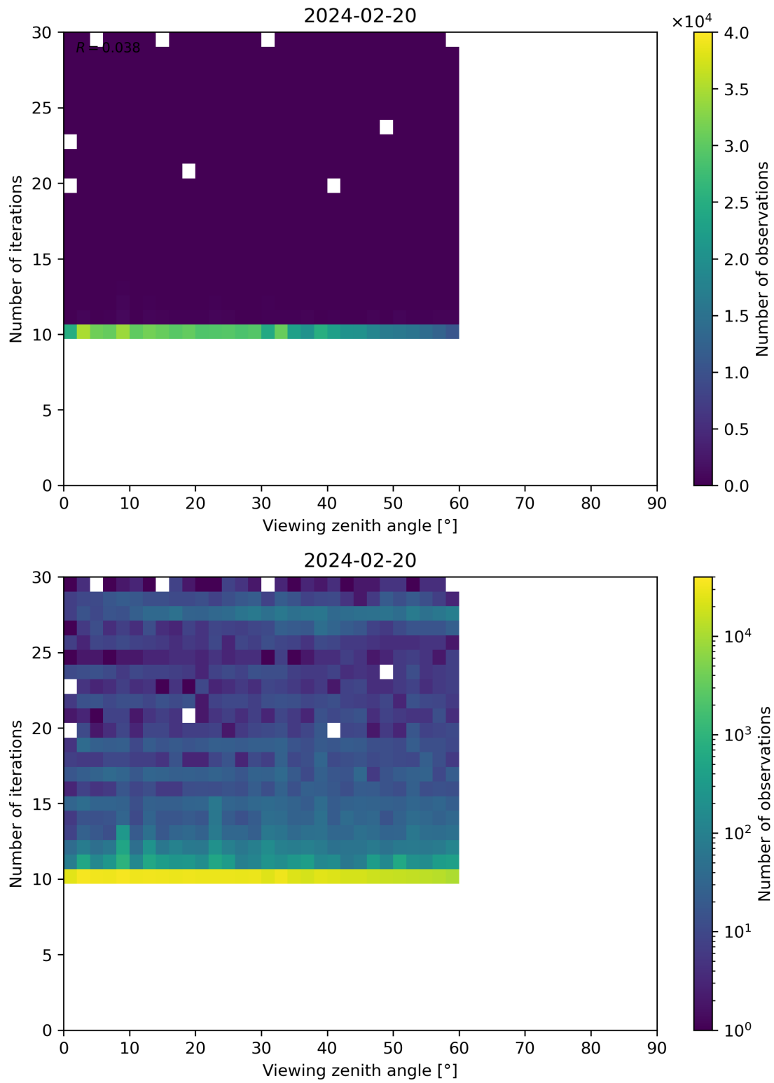
Figure 113: Scatter density plot of “Viewing zenith angle” against “Number of iterations” for 2024-02-19 to 2024-02-21.
