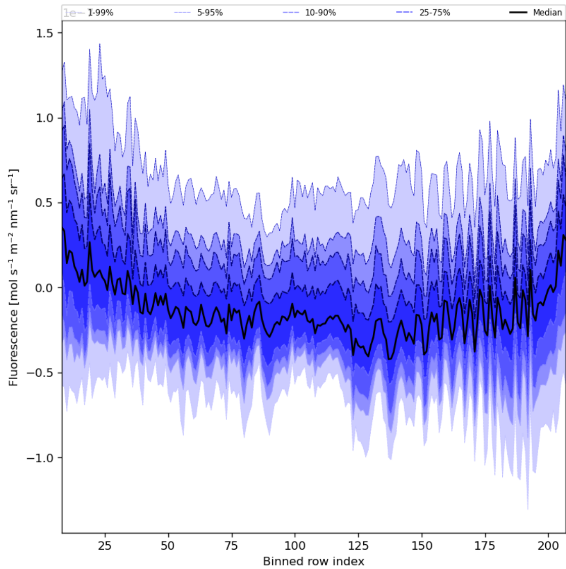
Figure 43: Along track statistics of "Fluorescence" for 2024-02-19 to 2024-02-21
