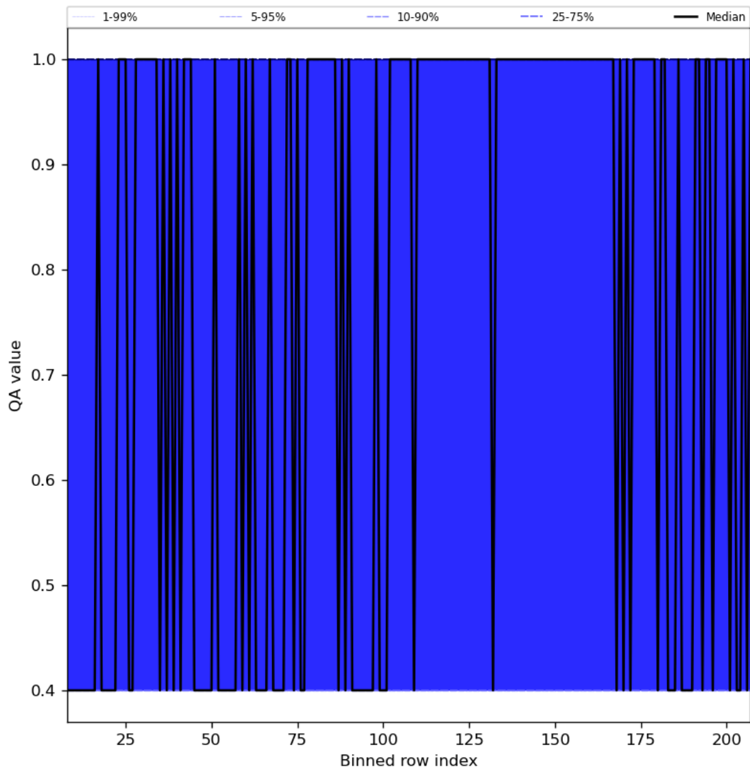
Figure 33: Along track statistics of “QA value” for 2024-02-19 to 2024-02-21
