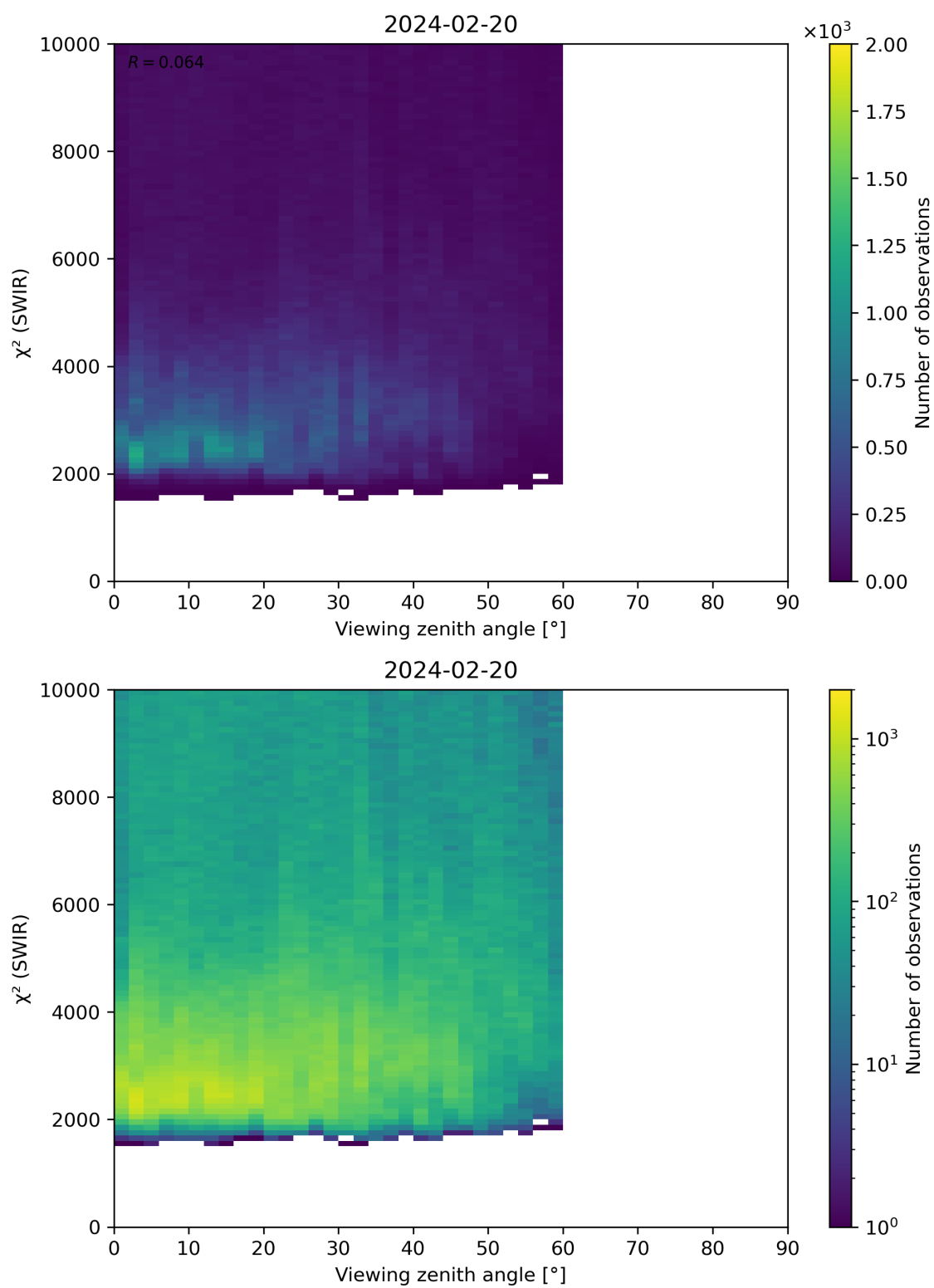
Figure 106: Scatter density plot of “Viewing zenith angle” against “ \chi^2 (SWIR)” for 2024-02-19 to 2024-02-21.
