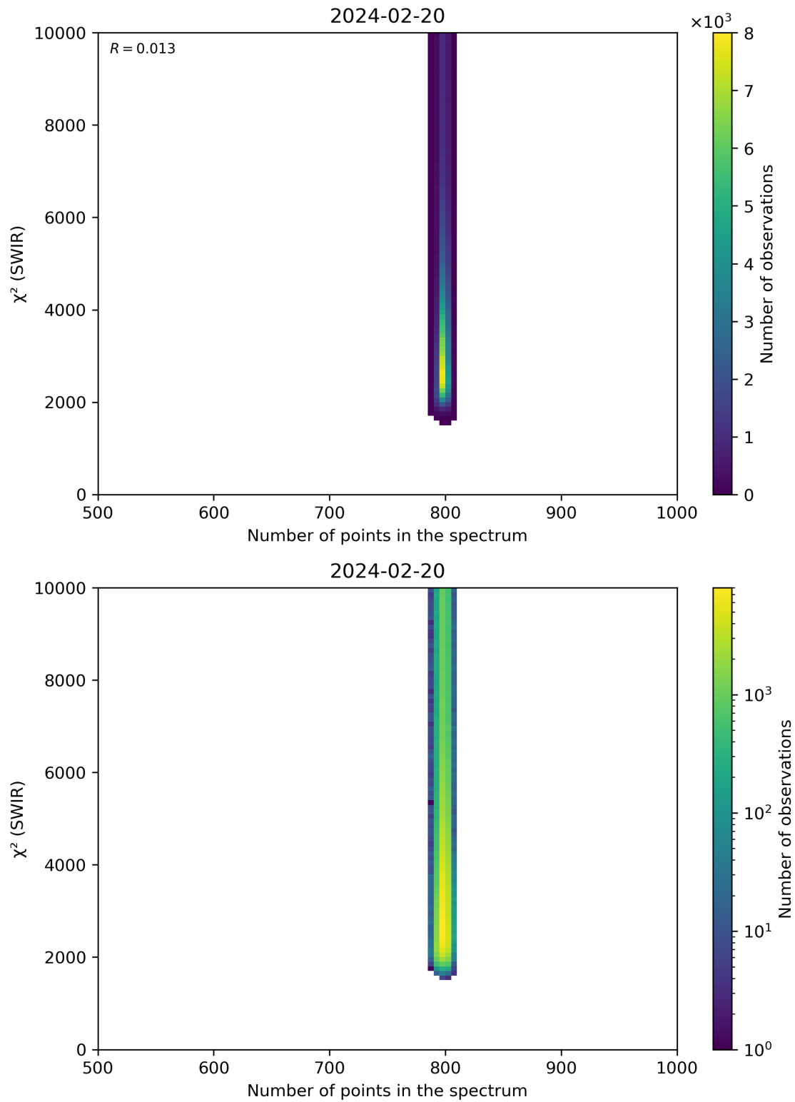
Figure 89: Scatter density plot of “Number of points in the spectrum” against “ \chi^2 (SWIR)” for 2024-02-19 to 2024-02-21.
