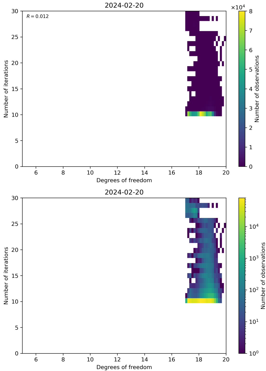
Figure 52: Scatter density plot of “Degrees of freedom” against “Number of iterations” for 2024-02-19 to 2024-02-21.
