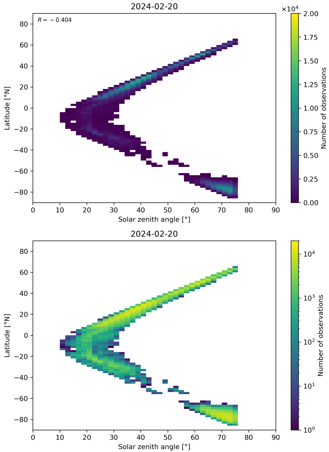
Figure 98: Scatter density plot of “Solar zenith angle” against “Latitude” for 2024-02-19 to 2024-02-21.
