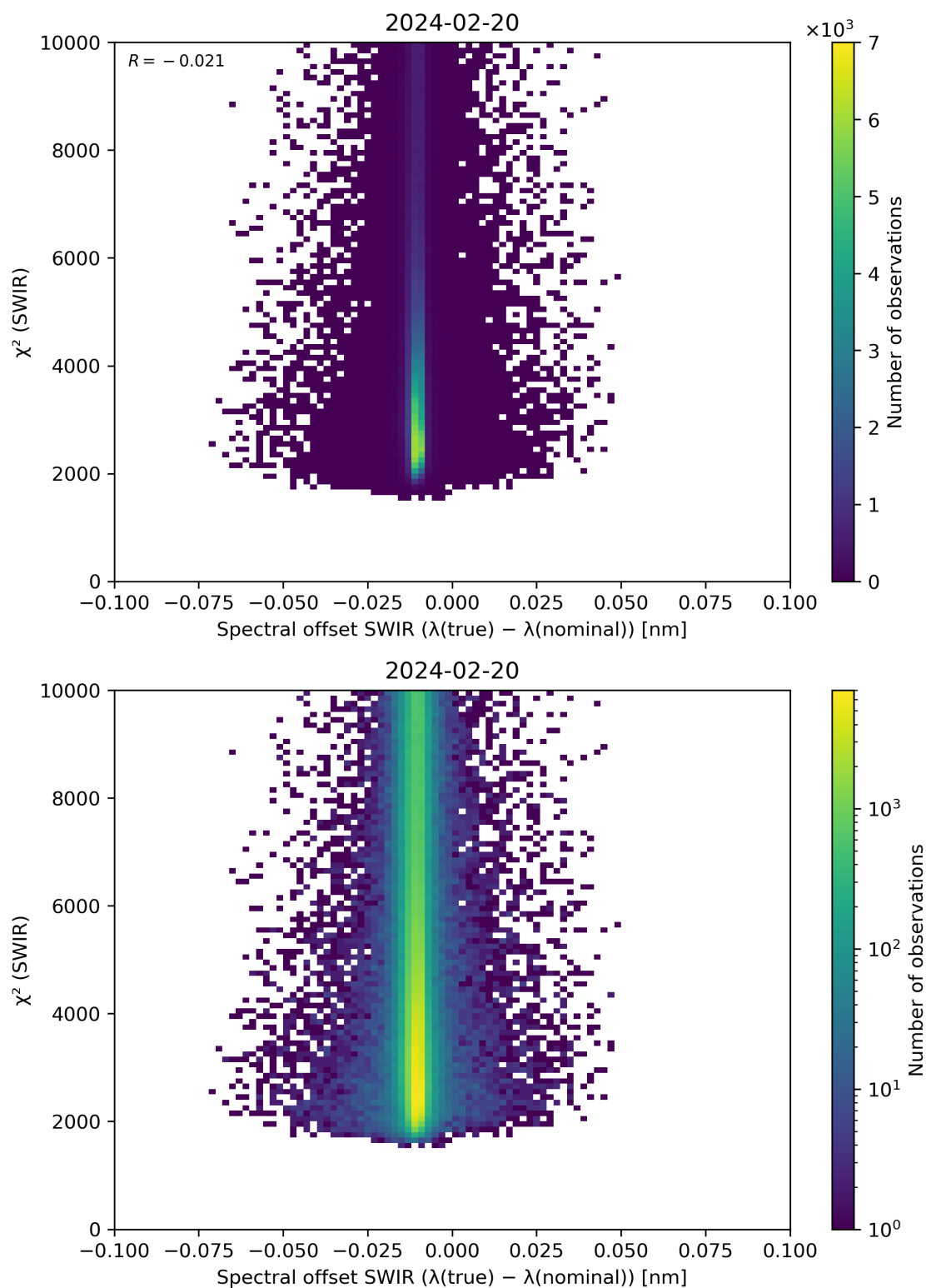
Figure 118: Scatter density plot of “Spectral offset SWIR ( \lambda(\text{true}) - \lambda(\text{nominal}) )” against “ \chi^2 (SWIR)” for 2024-02-19 to 2024-02-21.
