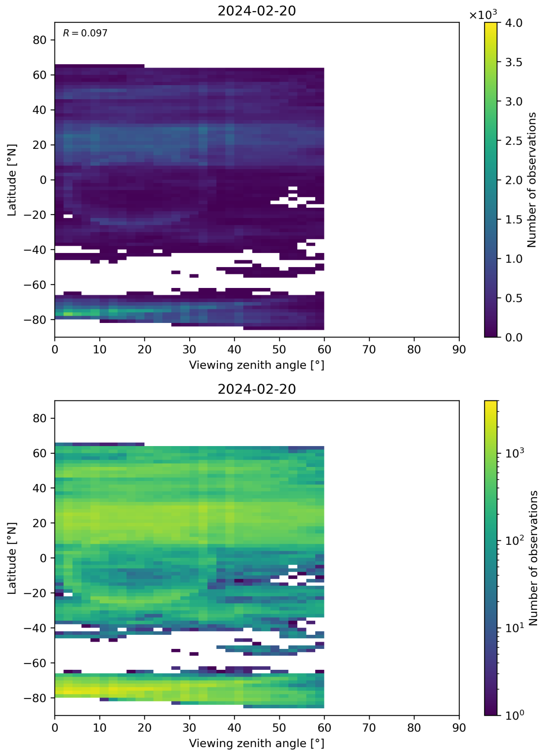
Figure 109: Scatter density plot of “Viewing zenith angle” against “Latitude” for 2024-02-19 to 2024-02-21.
