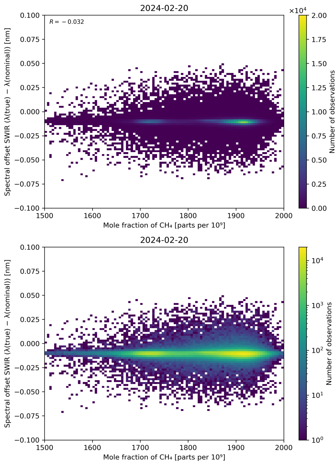
Figure 86: Scatter density plot of “Mole fraction of CH 4 ” against “Spectral offset SWIR ( \lambda(\text{true}) - \lambda(\text{nominal}) )” for 2024-02-19 to 2024-02-21.
