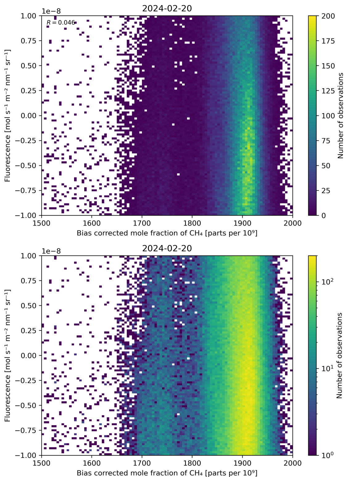
Figure 66: Scatter density plot of “Bias corrected mole fraction of \text{CH}_4 ” against “Fluorescence” for 2024-02-19 to 2024-02-21.
