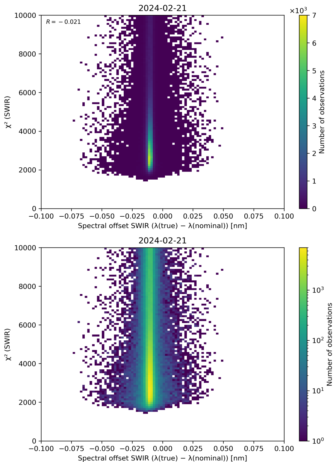
Figure 118: Scatter density plot of “Spectral offset SWIR ( \lambda(\text{true}) - \lambda(\text{nominal}) )” against “ \chi^2 (SWIR)” for 2024-02-20 to 2024-02-22.
