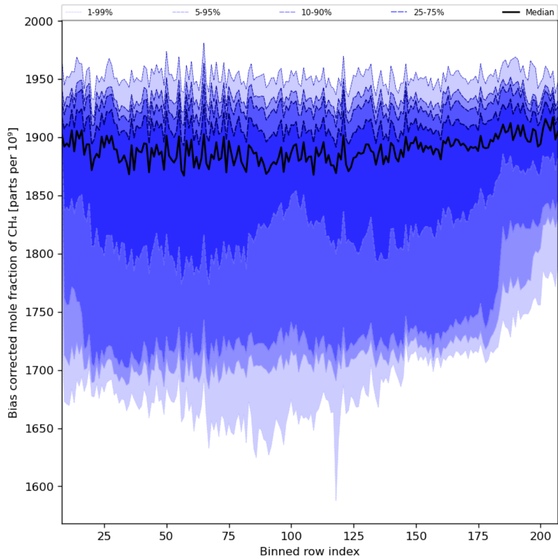
Figure 36: Along track statistics of “Bias corrected mole fraction of CH 4 ” for 2024-02-20 to 2024-02-22
