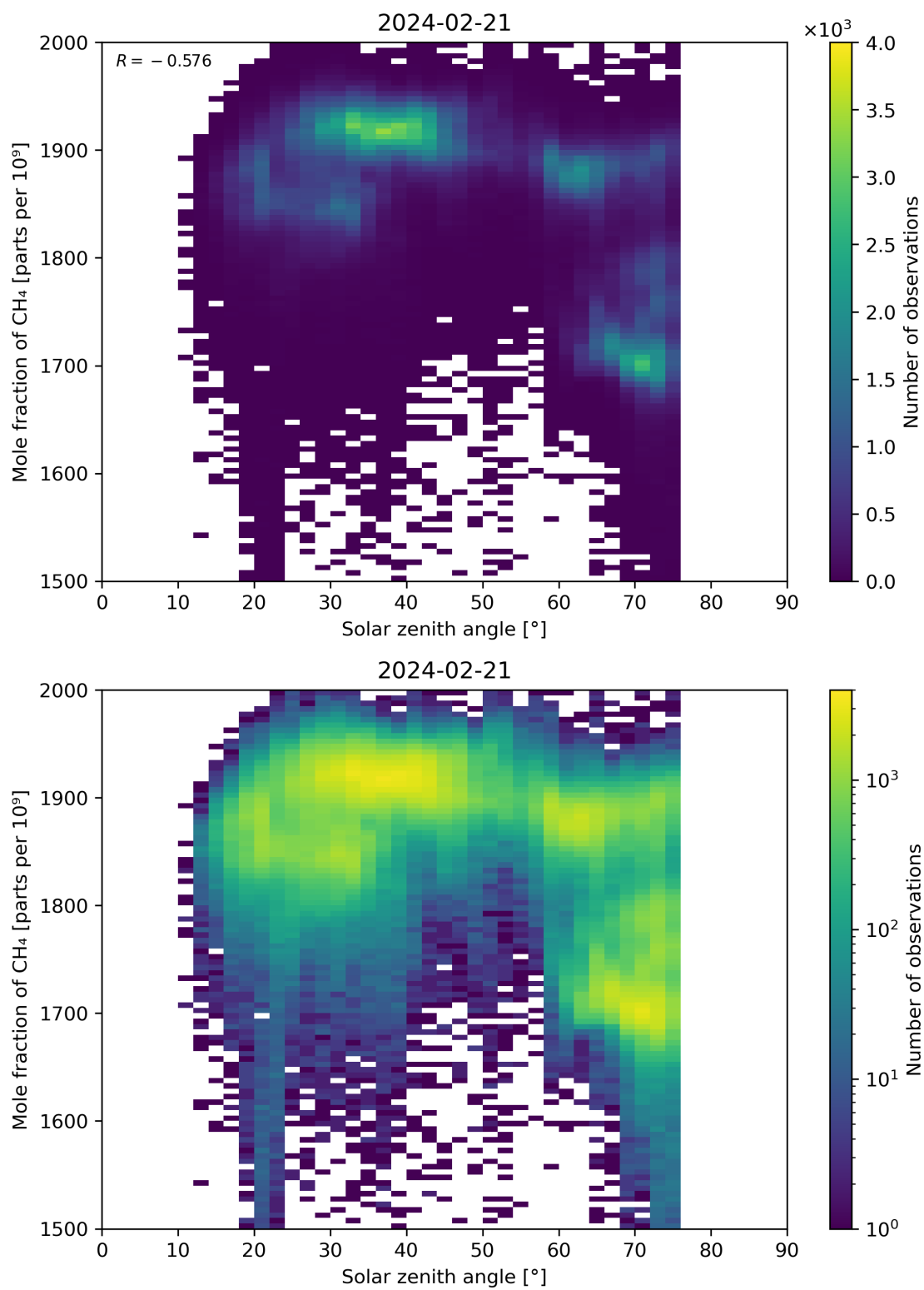
Figure 99: Scatter density plot of “Solar zenith angle” against “Mole fraction of \text{CH}_4 ” for 2024-02-20 to 2024-02-22.
