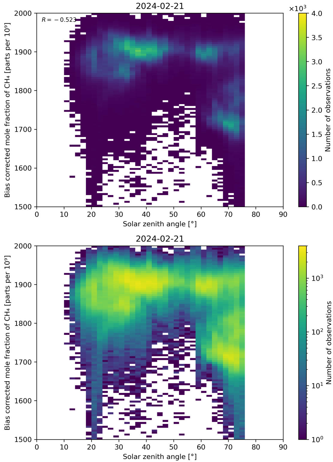
Figure 100: Scatter density plot of “Solar zenith angle” against “Bias corrected mole fraction of CH 4 ” for 2024-02-20 to 2024-02-22.
