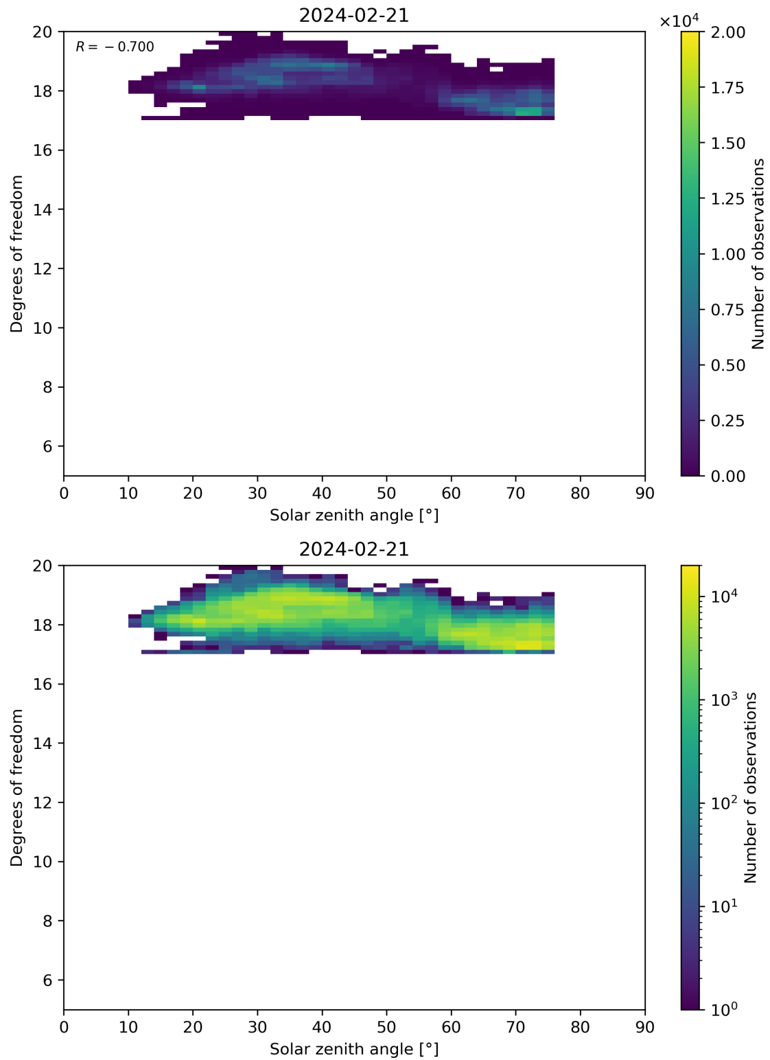
Figure 96: Scatter density plot of “Solar zenith angle” against “Degrees of freedom” for 2024-02-20 to 2024-02-22.
