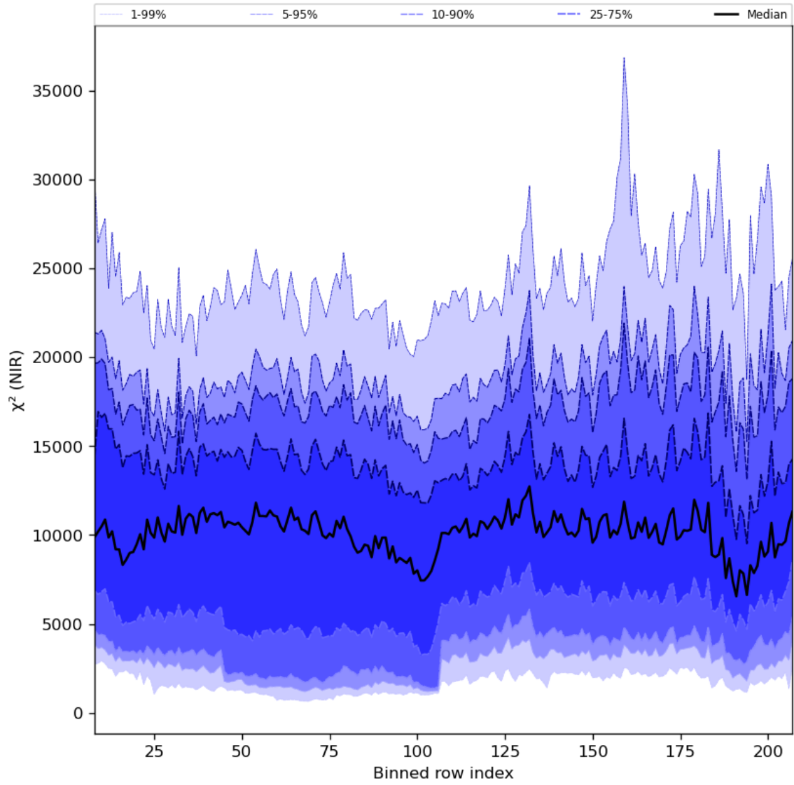
Figure 40: Along track statistics of “ \chi^2 (NIR)” for 2024-02-20 to 2024-02-22
