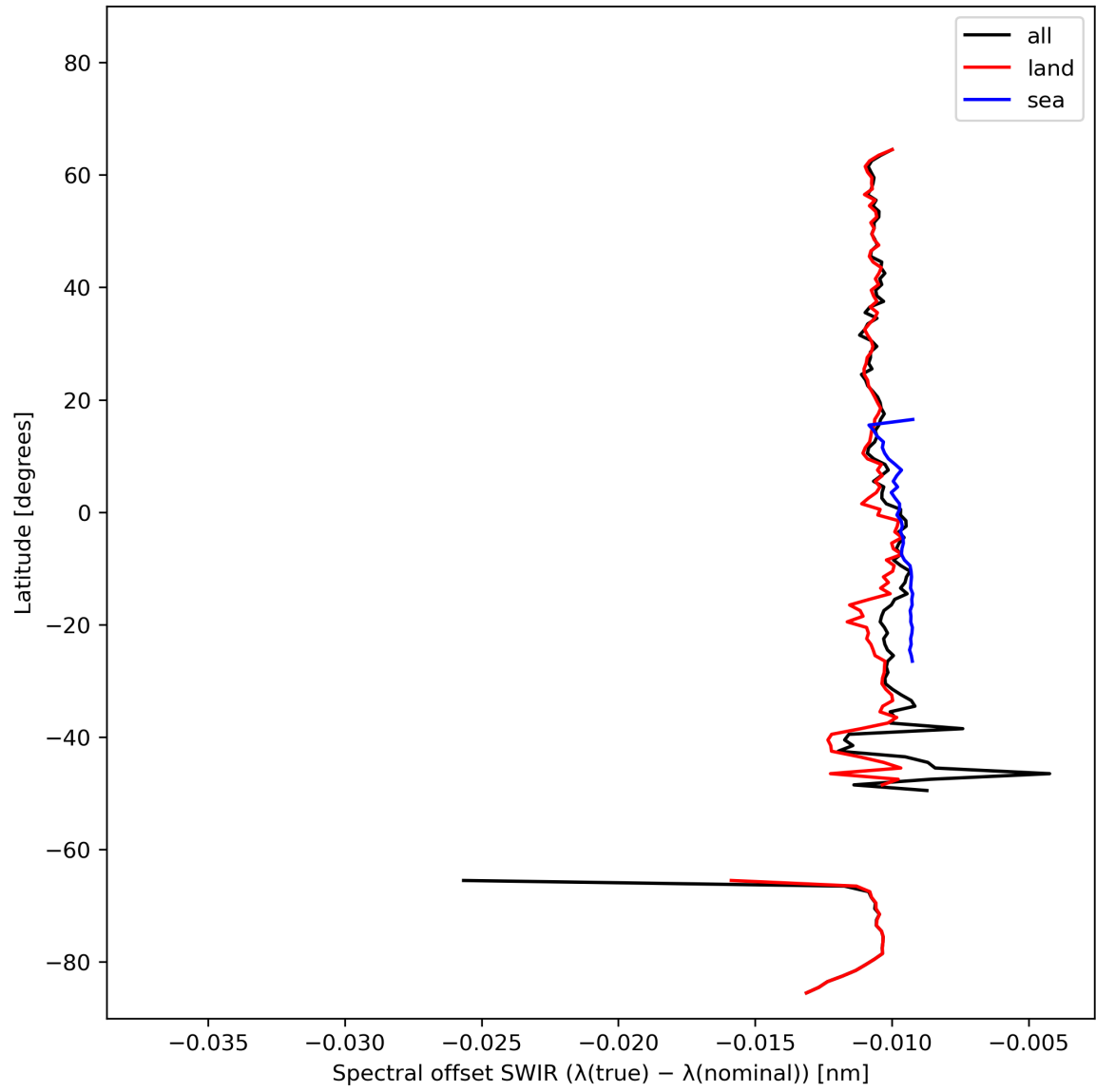
Figure 16: Zonal average of “Spectral offset SWIR ( \lambda(\text{true}) - \lambda(\text{nominal}) )” for 2024-02-20 to 2024-02-22.
