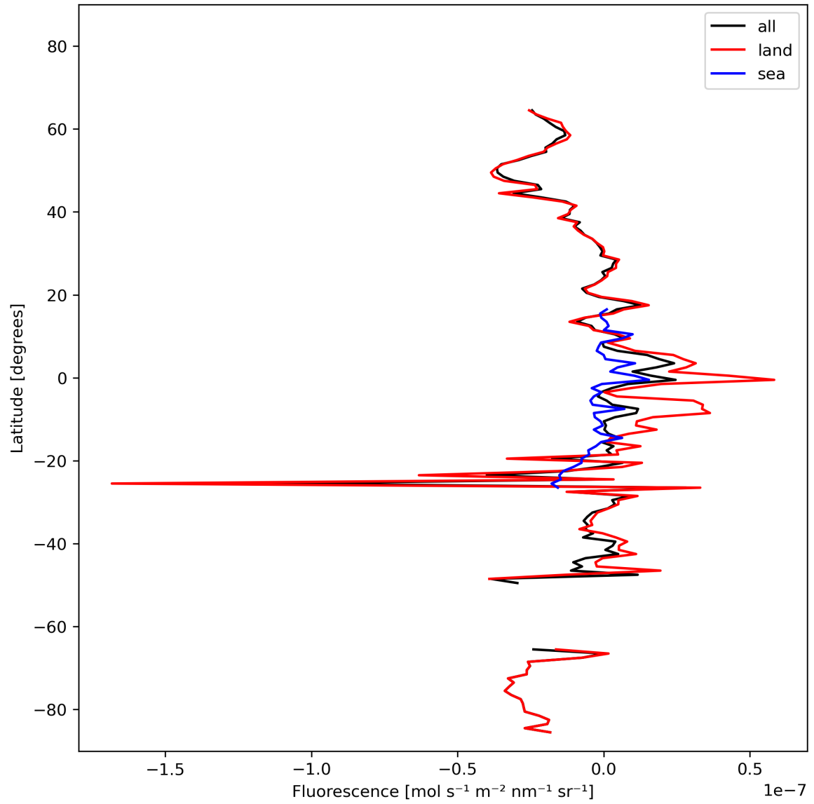
Figure 21: Zonal average of “Fluorescence” for 2024-02-20 to 2024-02-22.
