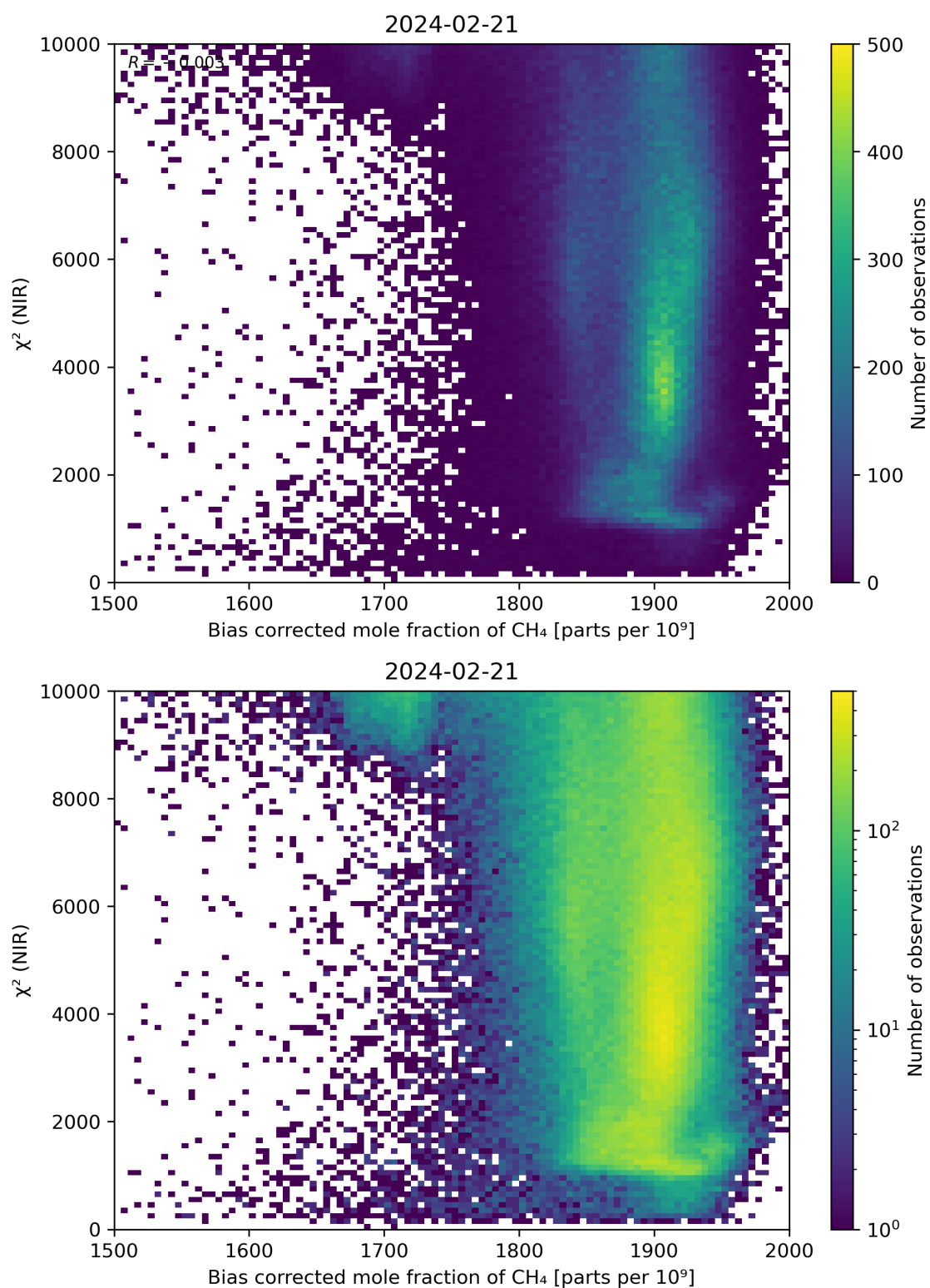
Figure 63: Scatter density plot of “Bias corrected mole fraction of CH 4 ” against “ \chi^2 (NIR)” for 2024-02-20 to 2024-02-22.
