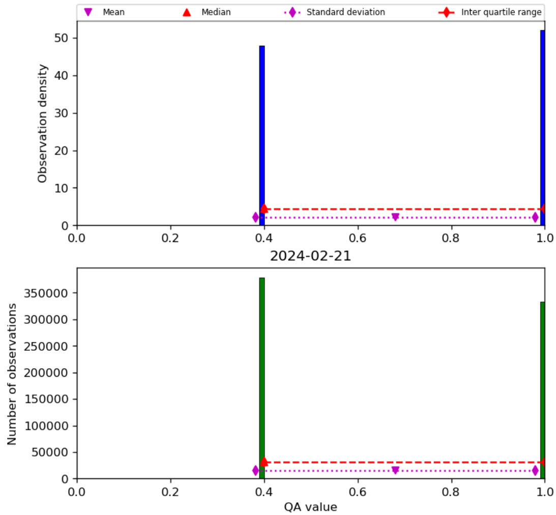
Figure 22: Histogram of “QA value” for 2024-02-20 to 2024-02-22
