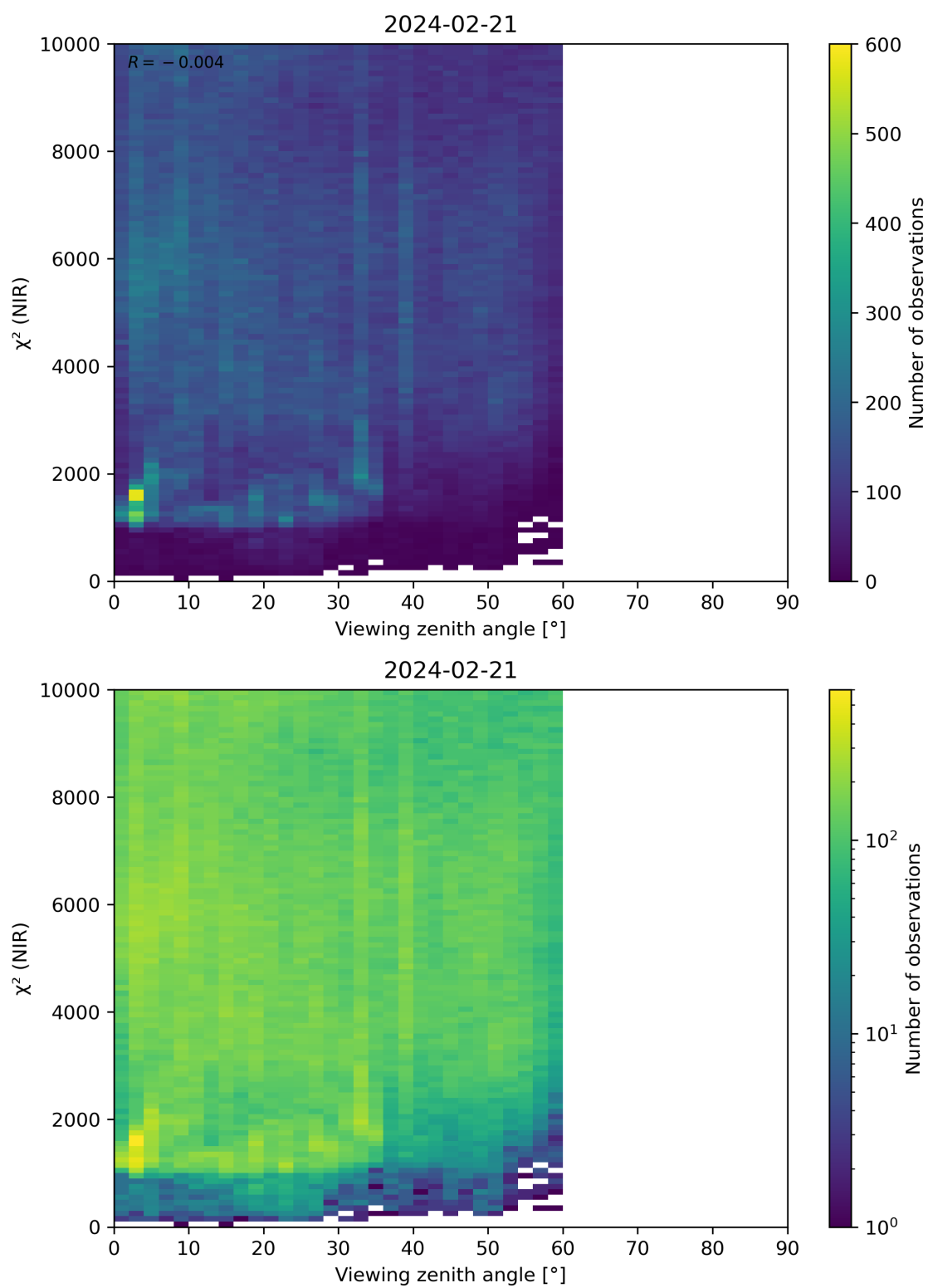
Figure 105: Scatter density plot of “Viewing zenith angle” against “ \chi^2 (NIR)” for 2024-02-20 to 2024-02-22.
