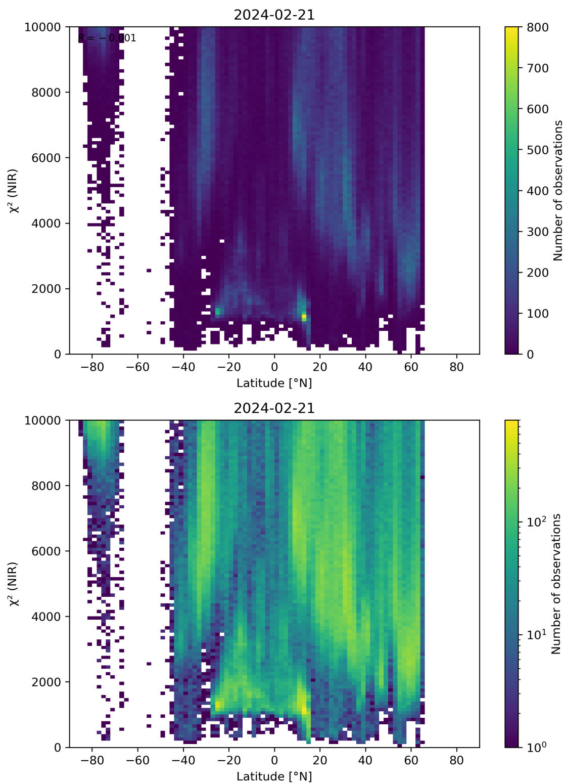
Figure 53: Scatter density plot of “Latitude” against “ \chi^2 (NIR)” for 2024-02-20 to 2024-02-22.
