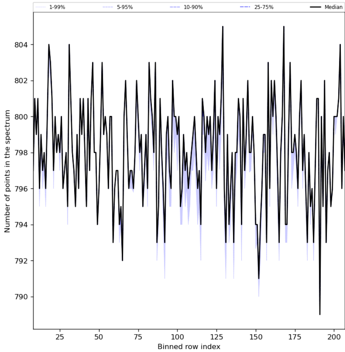
Figure 37: Along track statistics of “Number of points in the spectrum” for 2024-02-20 to 2024-02-22
