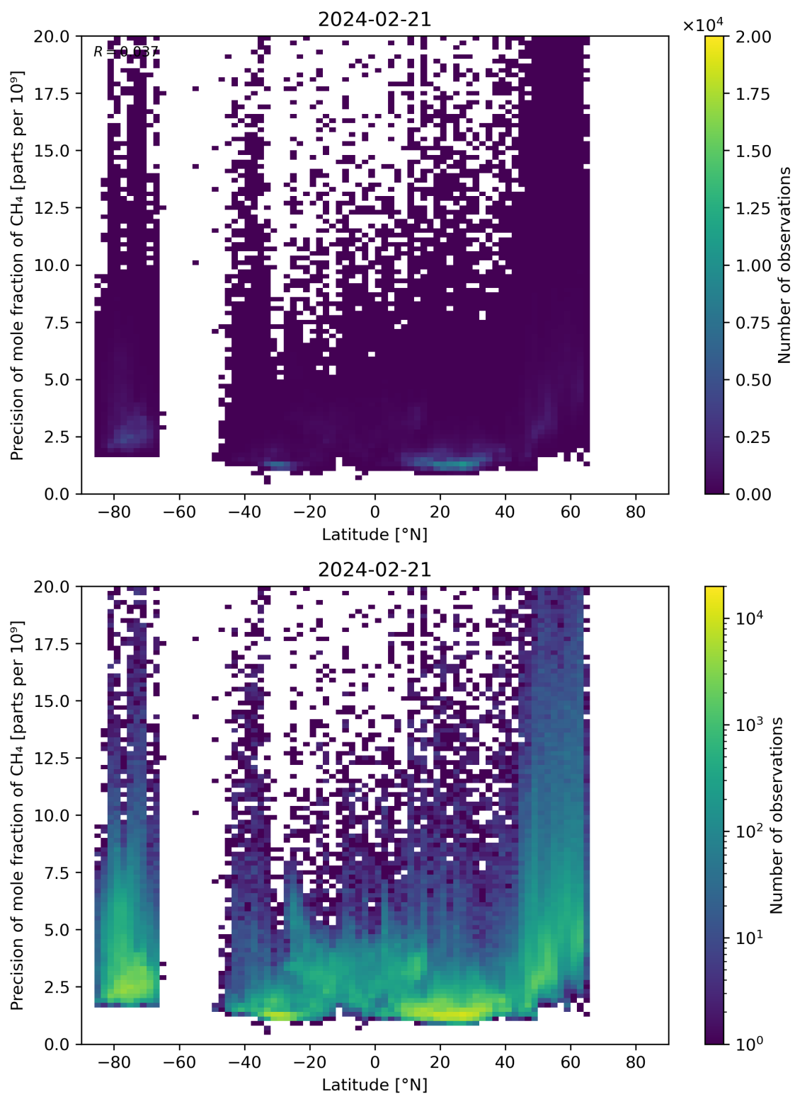
Figure 59: Scatter density plot of “Latitude” against “Precision of mole fraction of CH 4 ” for 2024-02-20 to 2024-02-22.
