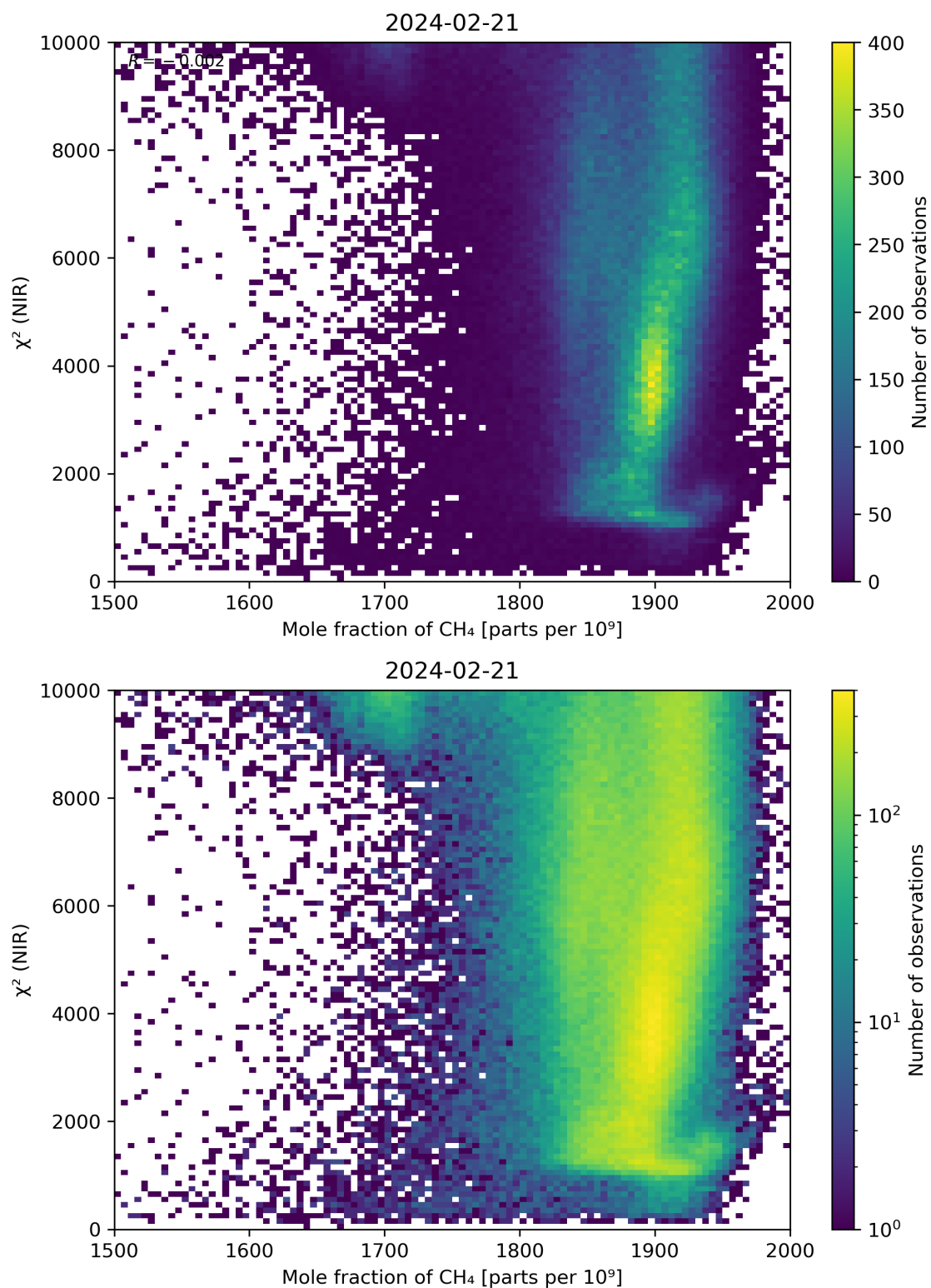
Figure 70: Scatter density plot of “Mole fraction of CH 4 ” against “ \chi^2 (NIR)” for 2024-02-20 to 2024-02-22.
