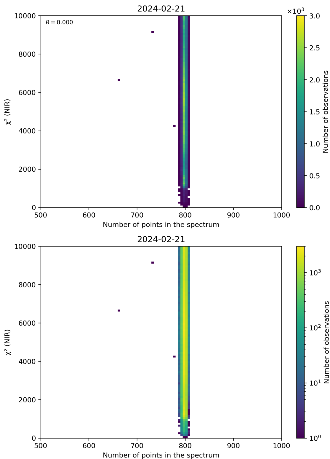
Figure 88: Scatter density plot of “Number of points in the spectrum” against “ \chi^2 (NIR)” for 2024-02-20 to 2024-02-22.
