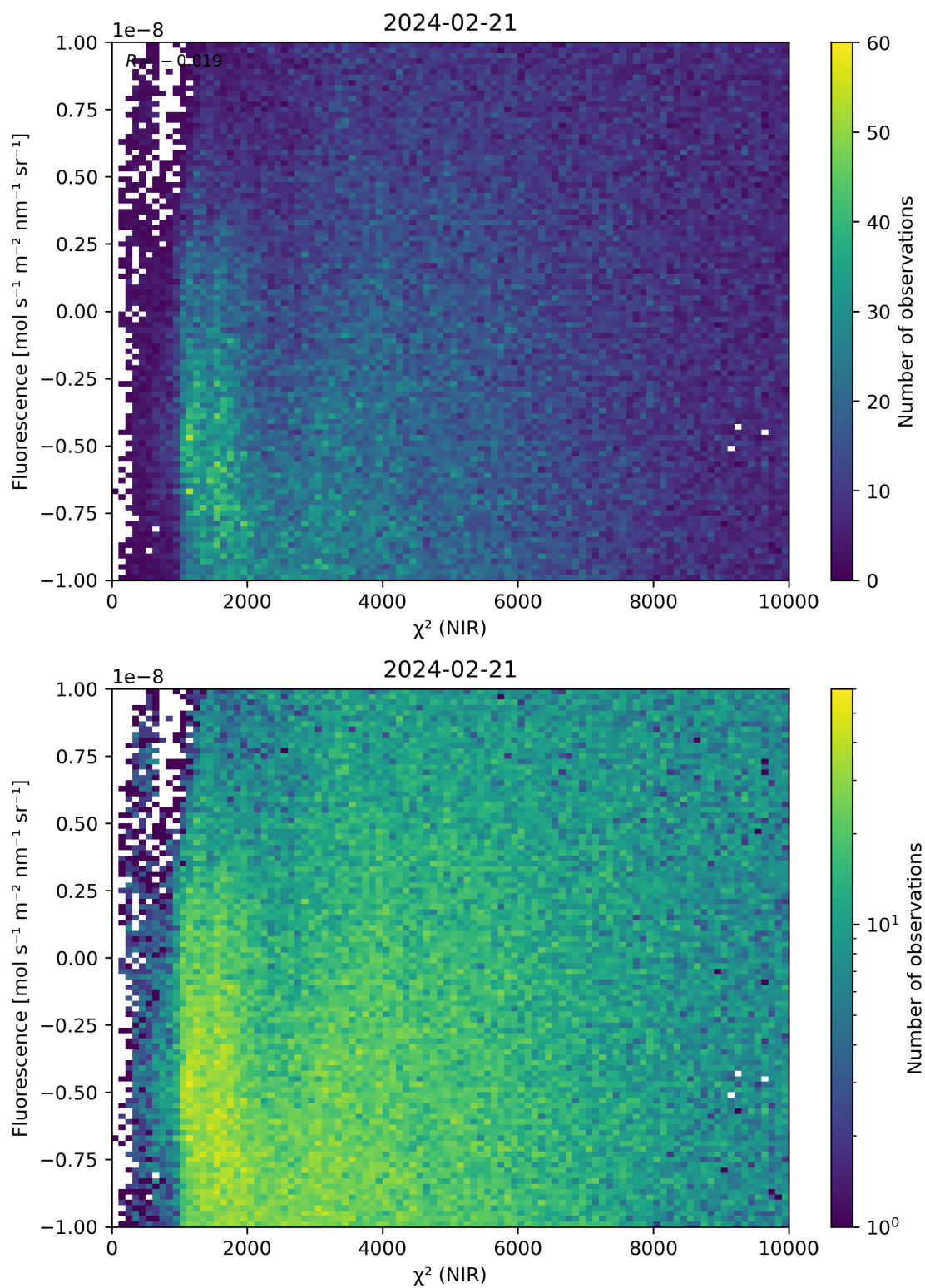
Figure 45: Scatter density plot of “ \chi^2 (NIR)” against “Fluorescence” for 2024-02-20 to 2024-02-22.
