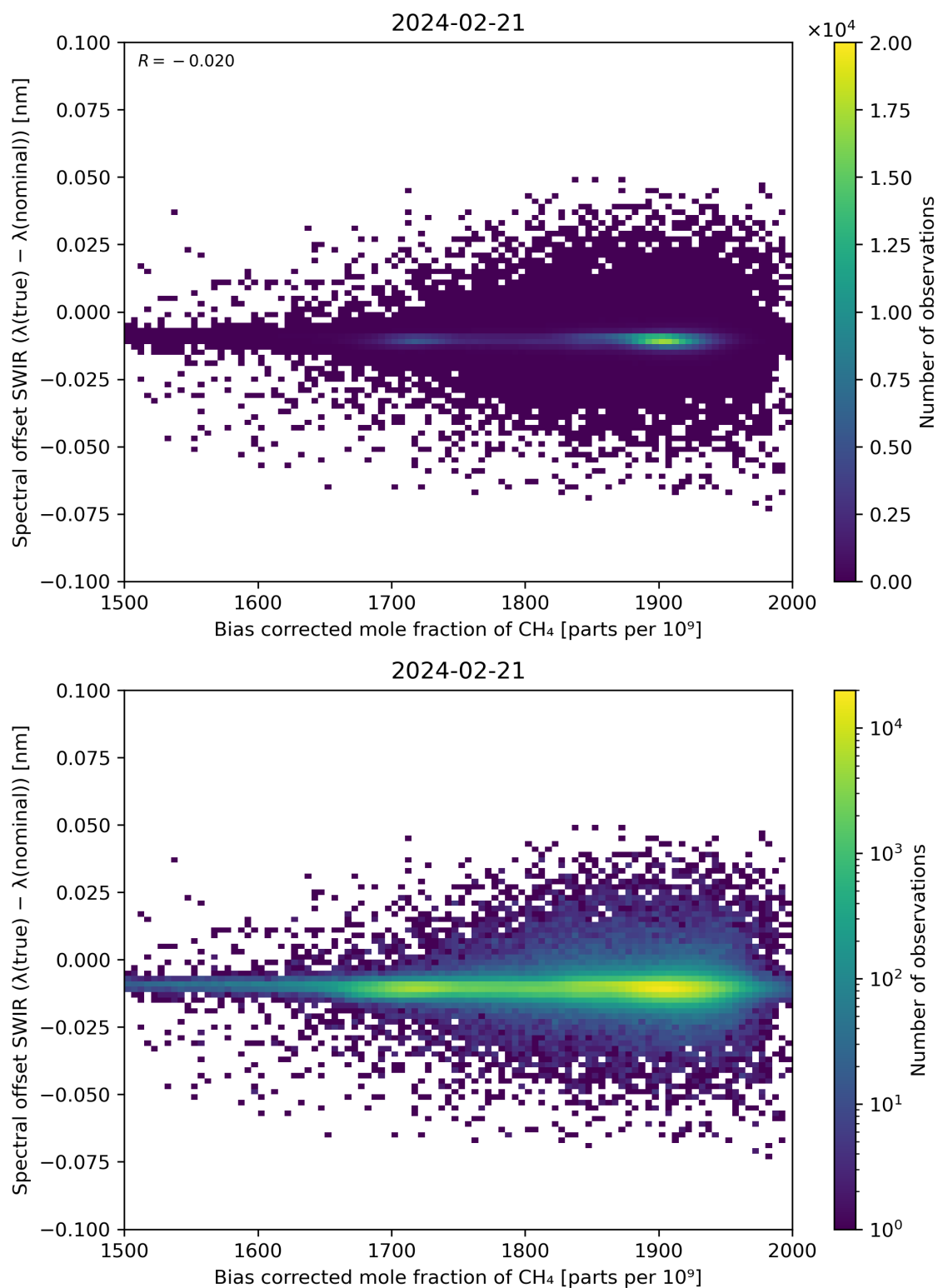
Figure 69: Scatter density plot of “Bias corrected mole fraction of \text{CH}_4 ” against “Spectral offset SWIR ( \lambda(\text{true}) - \lambda(\text{nominal}) )” for 2024-02-20 to 2024-02-22.
