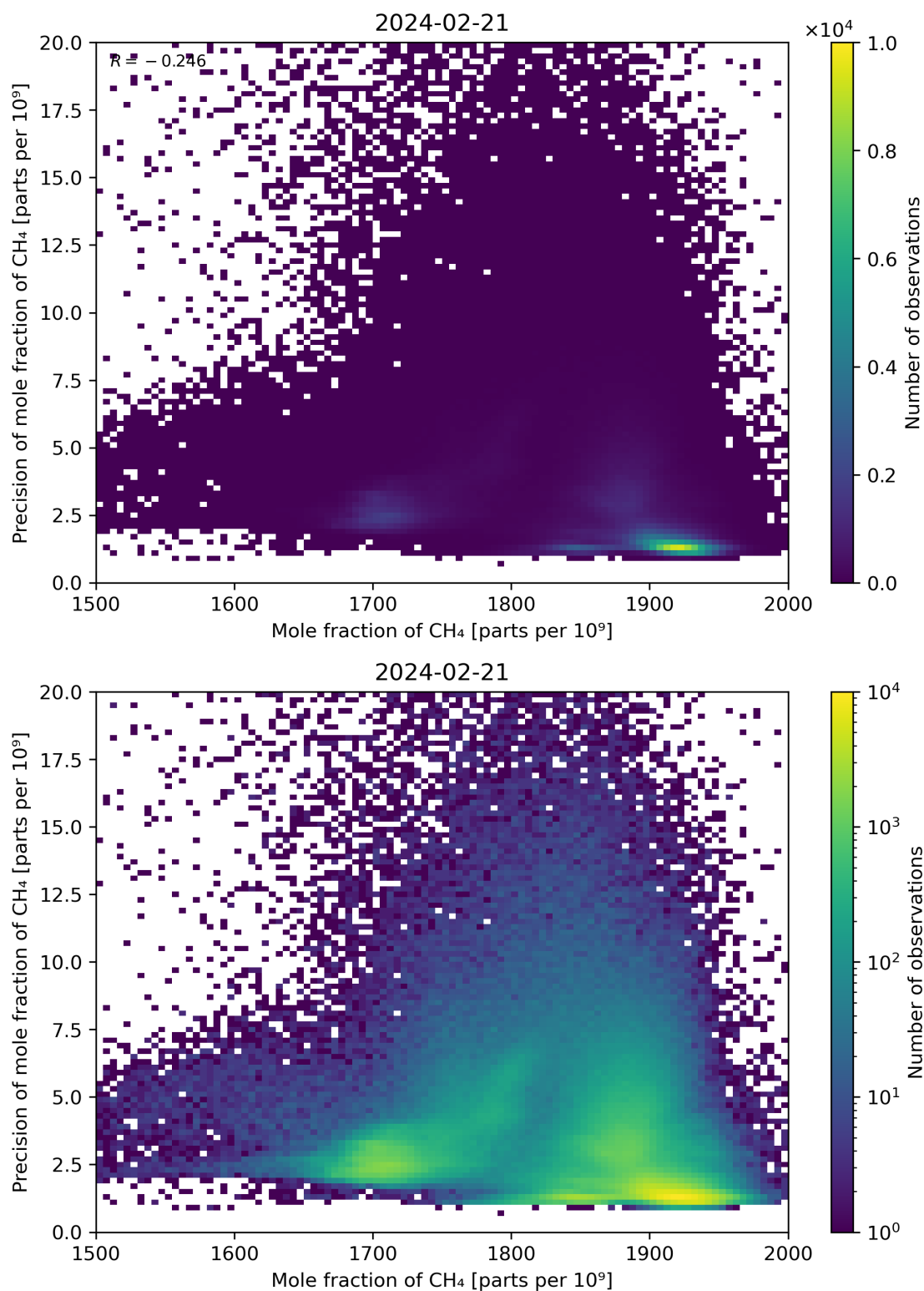
Figure 75: Scatter density plot of “Mole fraction of CH 4 ” against “Precision of mole fraction of CH 4 ” for 2024-02-20 to 2024-02-22.
