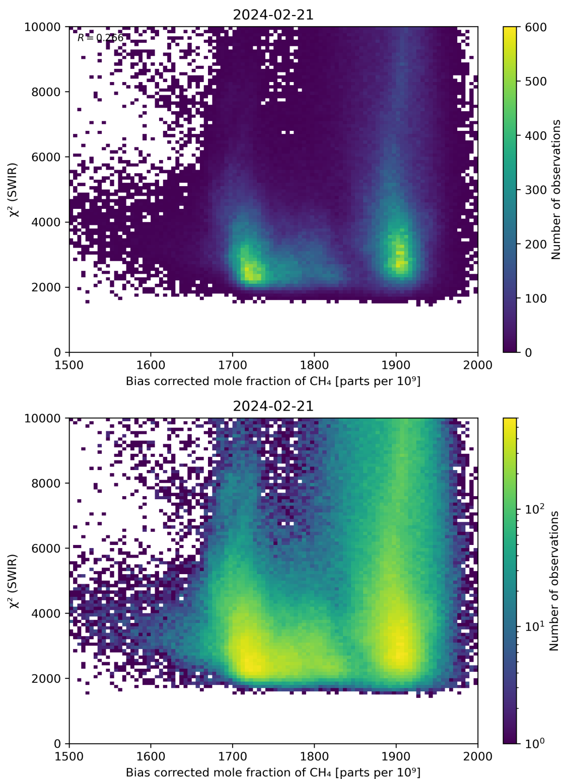
Figure 64: Scatter density plot of “Bias corrected mole fraction of CH 4 ” against “ \chi^2 (SWIR)” for 2024-02-20 to 2024-02-22.
