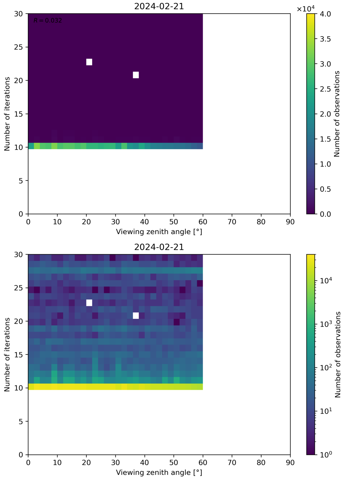
Figure 113: Scatter density plot of “Viewing zenith angle” against “Number of iterations” for 2024-02-20 to 2024-02-22.
