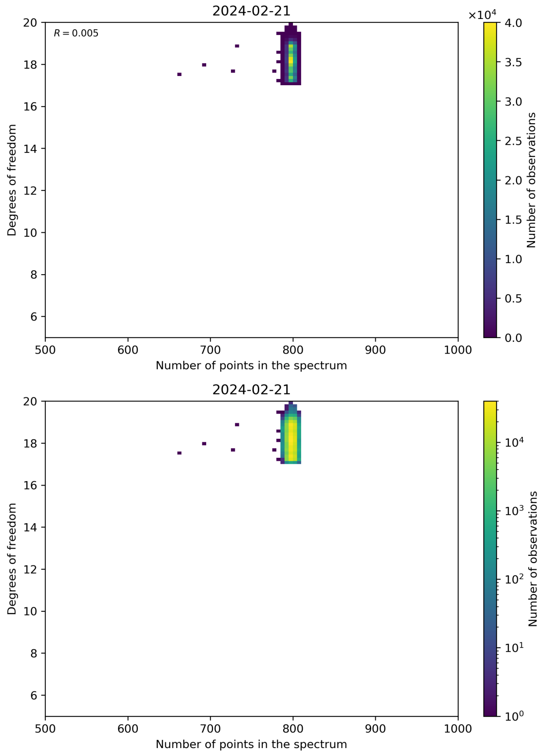
Figure 90: Scatter density plot of “Number of points in the spectrum” against “Degrees of freedom” for 2024-02-20 to 2024-02-22.
