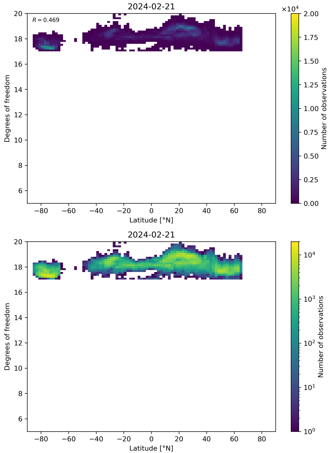
Figure 55: Scatter density plot of “Latitude” against “Degrees of freedom” for 2024-02-20 to 2024-02-22.
