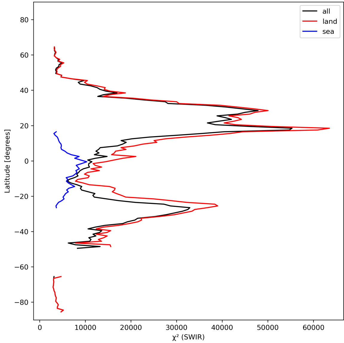
Figure 17: Zonal average of “ \chi^2 (SWIR)” for 2024-02-20 to 2024-02-22.
