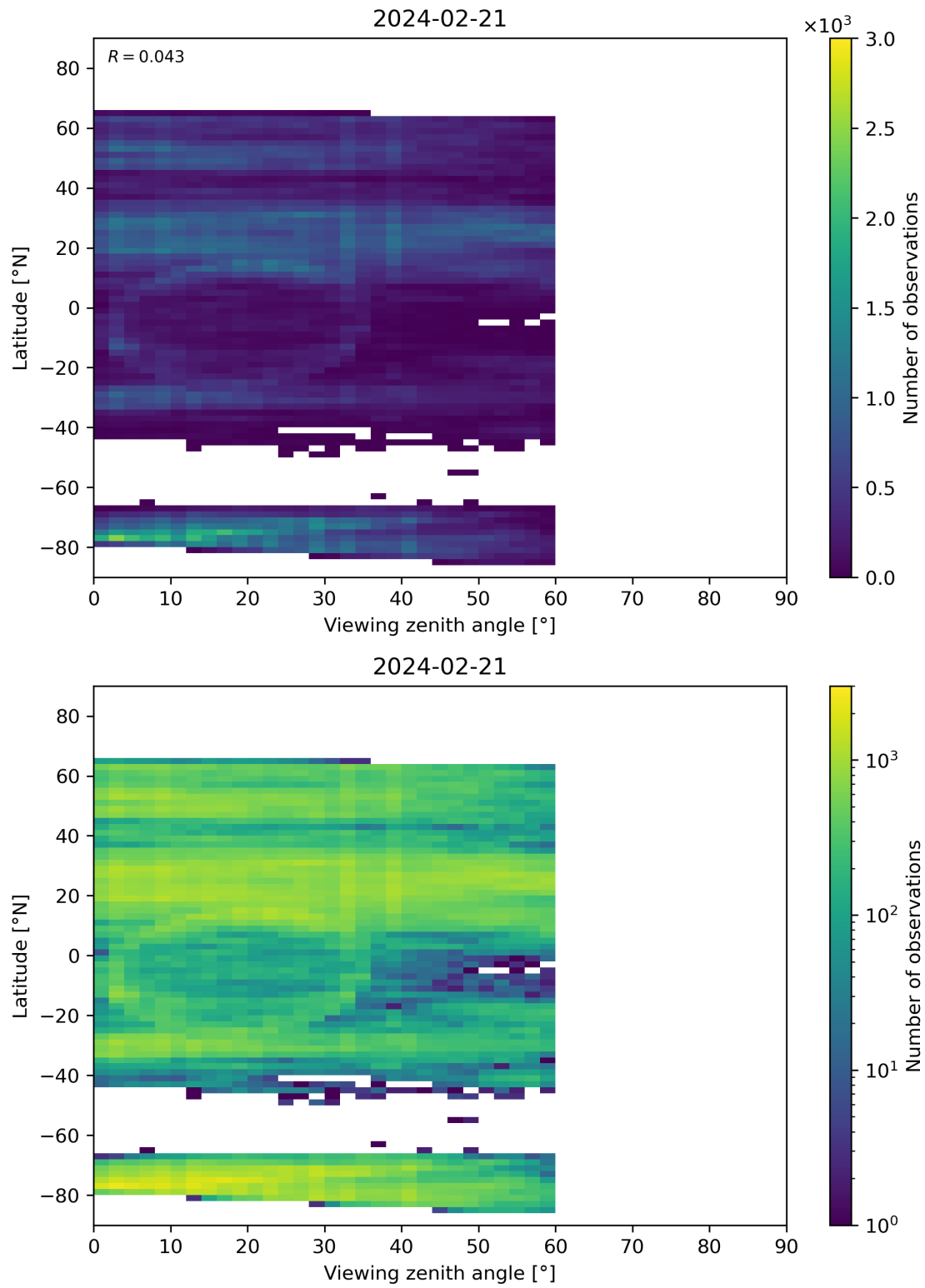
Figure 109: Scatter density plot of “Viewing zenith angle” against “Latitude” for 2024-02-20 to 2024-02-22.
