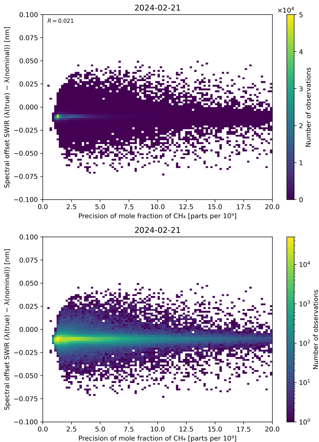
Figure 85: Scatter density plot of “Precision of mole fraction of \text{CH}_4 ” against “Spectral offset SWIR ( \lambda(\text{true}) - \lambda(\text{nominal}) )” for 2024-02-20 to 2024-02-22.
