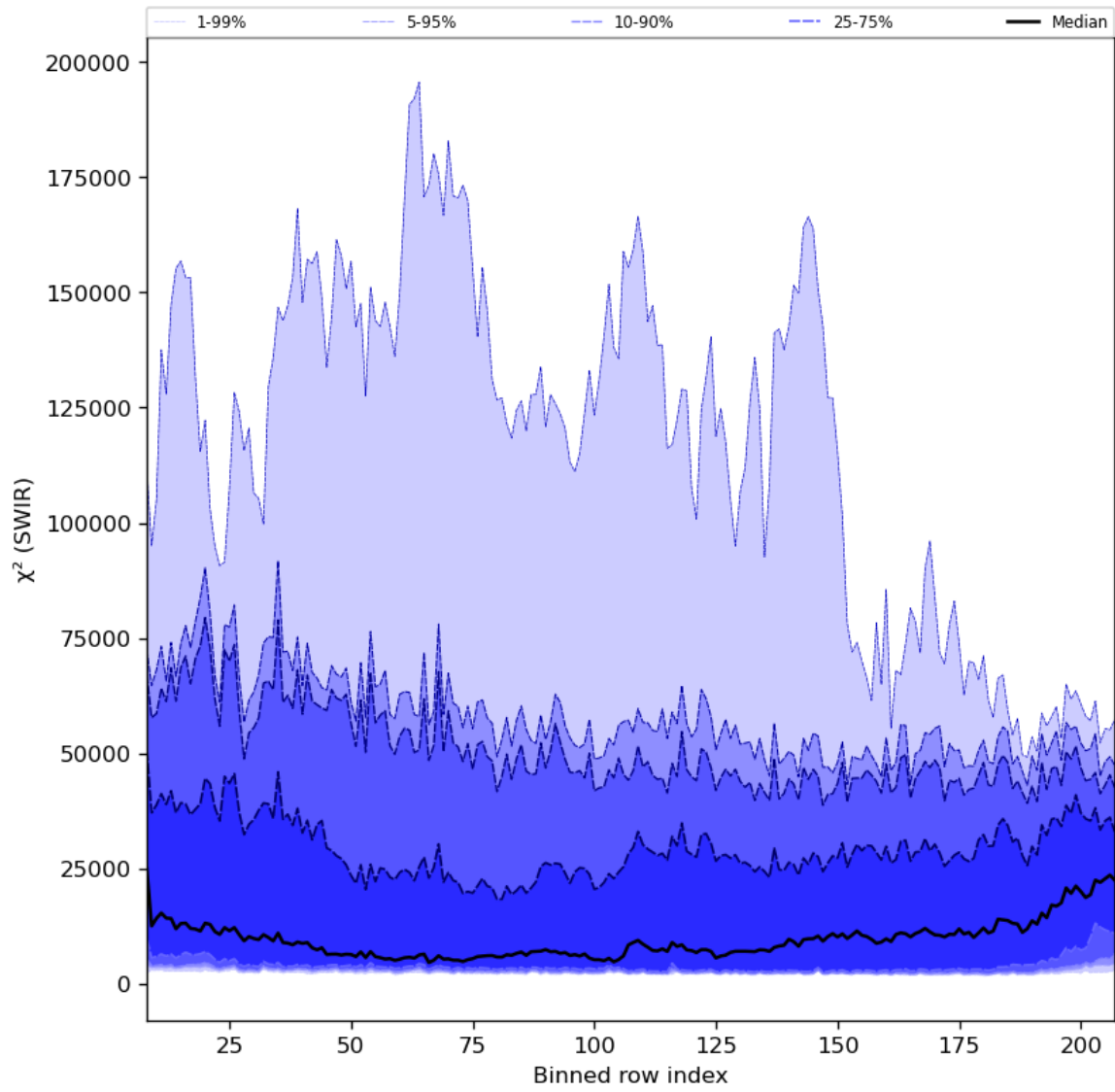
Figure 39: Along track statistics of " \chi^2 (SWIR)" for 2024-02-20 to 2024-02-22
