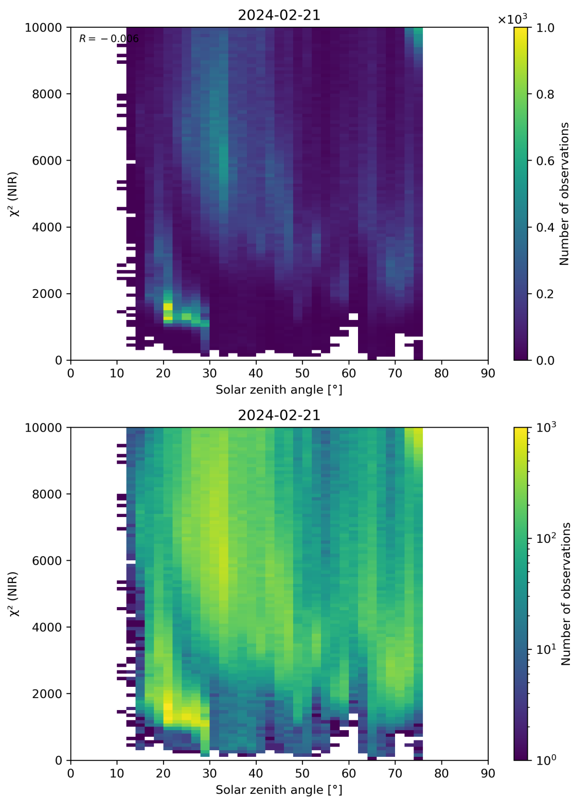
Figure 94: Scatter density plot of “Solar zenith angle” against “ \chi^2 (NIR)” for 2024-02-20 to 2024-02-22.
