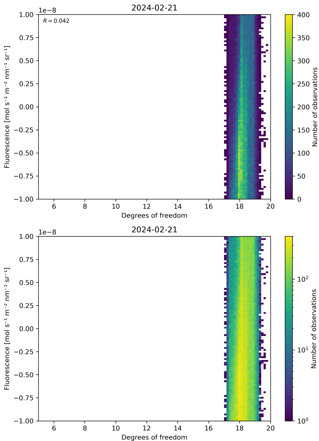
Figure 51: Scatter density plot of “Degrees of freedom” against “Fluorescence” for 2024-02-20 to 2024-02-22.
