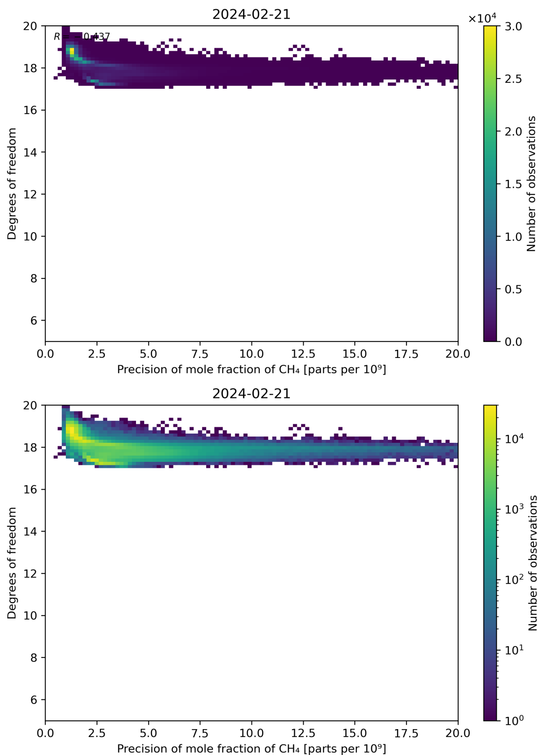
Figure 80: Scatter density plot of “Precision of mole fraction of CH 4 ” against “Degrees of freedom” for 2024-02-20 to 2024-02-22.
