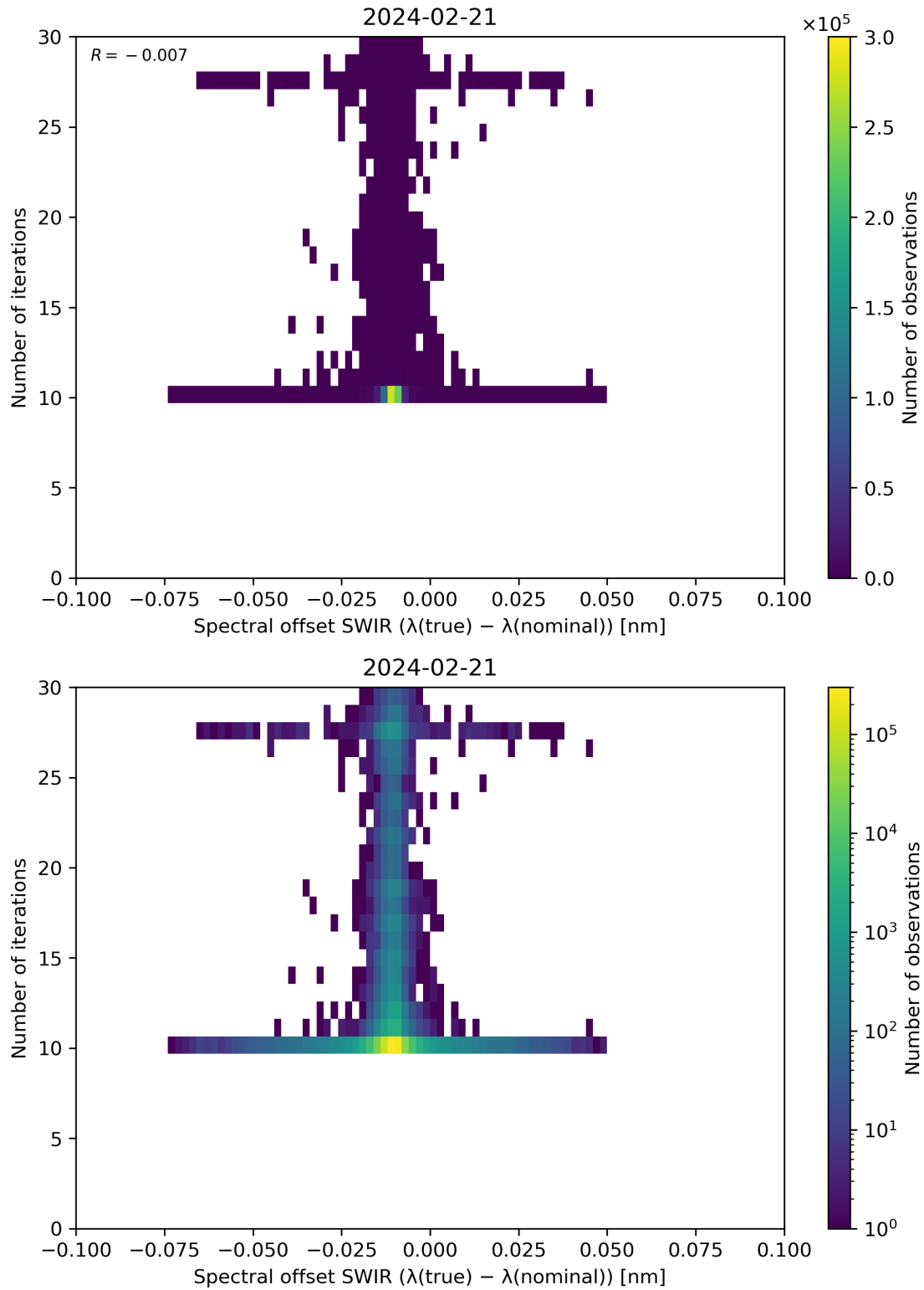
Figure 121: Scatter density plot of “Spectral offset SWIR ( \lambda(\text{true}) - \lambda(\text{nominal}) )” against “Number of iterations” for 2024-02-20 to 2024-02-22.
