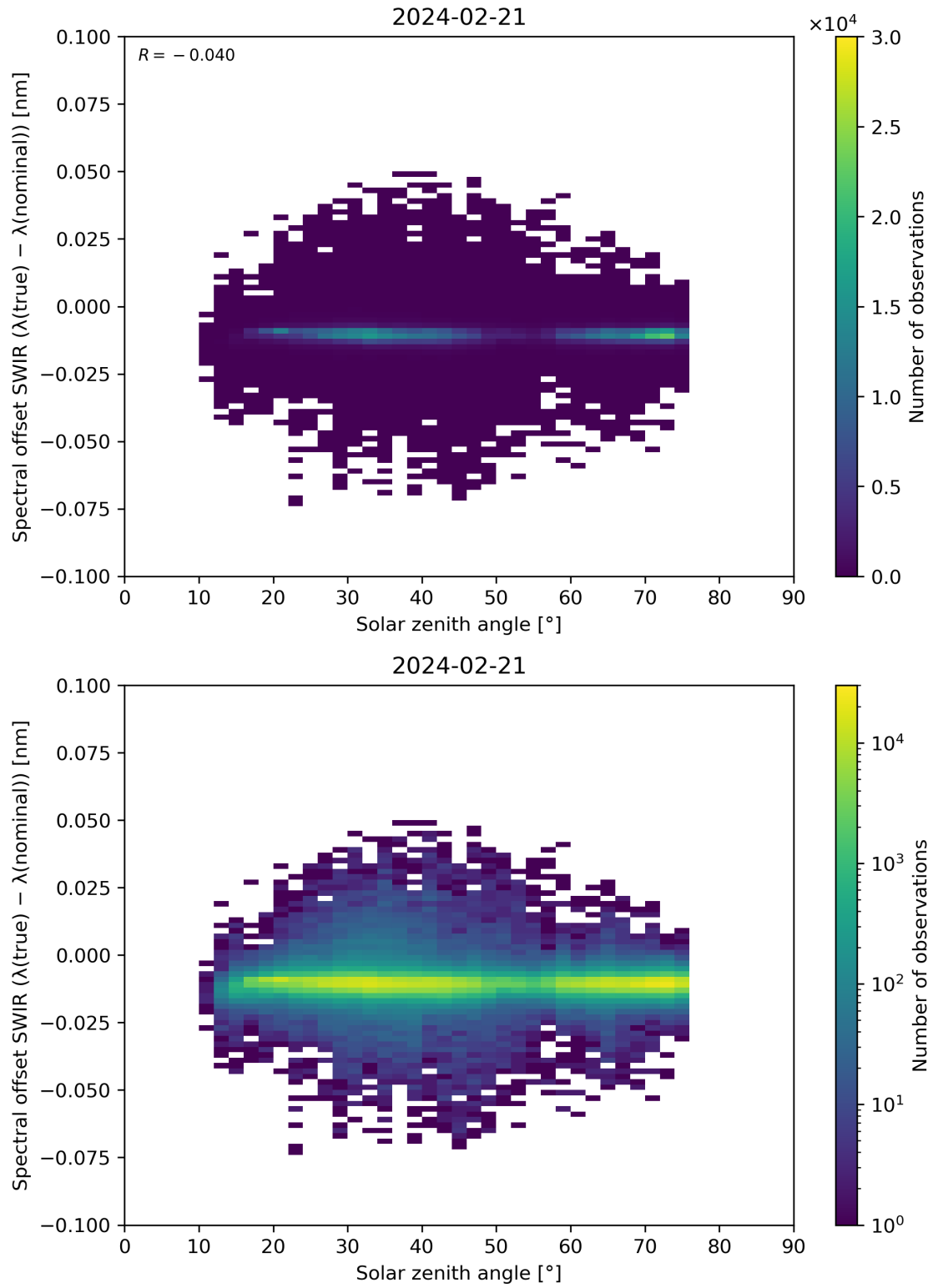
Figure 104: Scatter density plot of “Solar zenith angle” against “Spectral offset SWIR ( \lambda(\text{true}) - \lambda(\text{nominal}) )” for 2024-02-20 to 2024-02-22.
