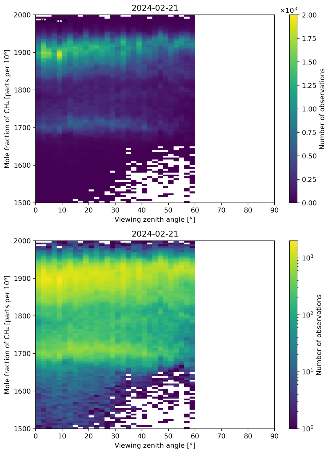
Figure 110: Scatter density plot of “Viewing zenith angle” against “Mole fraction of CH 4 ” for 2024-02-20 to 2024-02-22.
