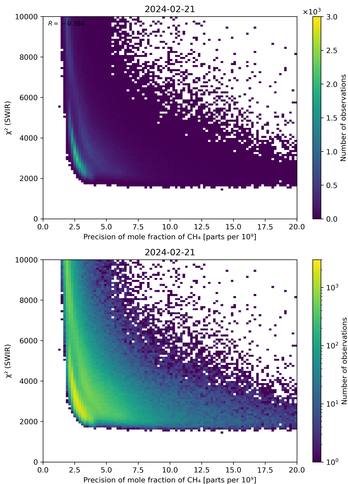
Figure 79: Scatter density plot of “Precision of mole fraction of \text{CH}_4 ” against “ \chi^2 (SWIR)” for 2024-02-20 to 2024-02-22.
