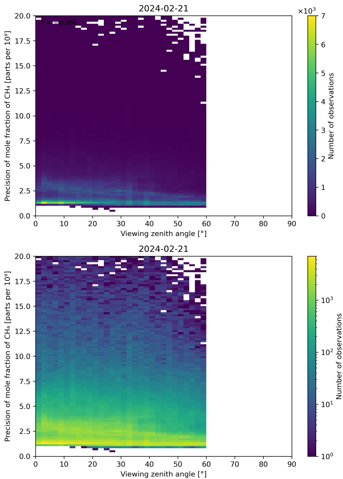
Figure 112: Scatter density plot of “Viewing zenith angle” against “Precision of mole fraction of CH 4 ” for 2024-02-20 to 2024-02-22.
