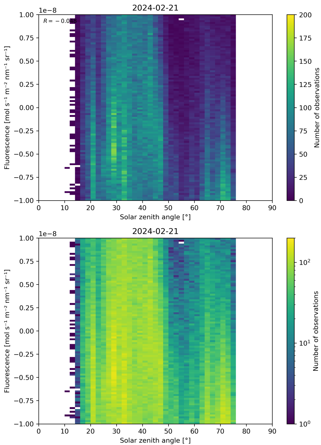
Figure 97: Scatter density plot of “Solar zenith angle” against “Fluorescence” for 2024-02-20 to 2024-02-22.
