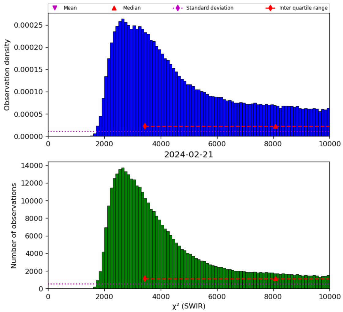
Figure 28: Histogram of “ \chi^2 (SWIR)” for 2024-02-20 to 2024-02-22
