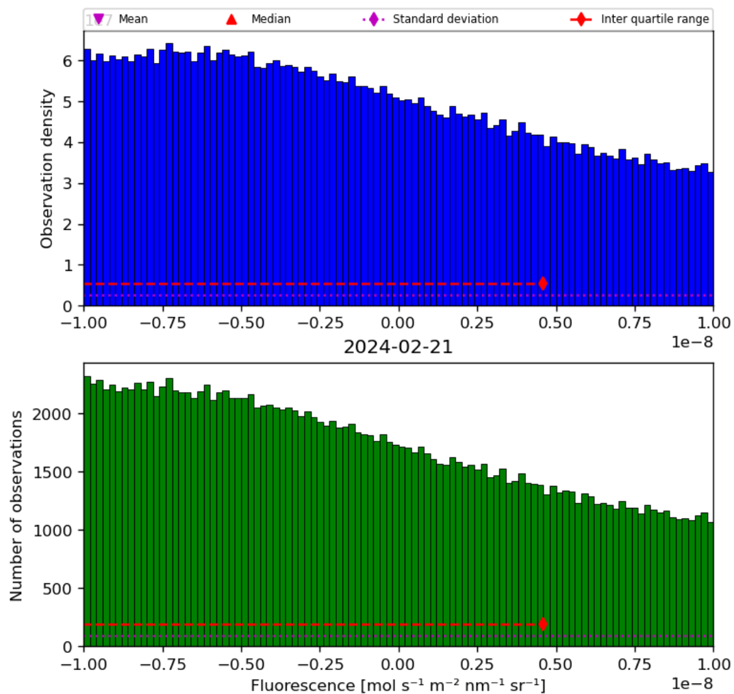
Figure 32: Histogram of “Fluorescence” for 2024-02-20 to 2024-02-22
