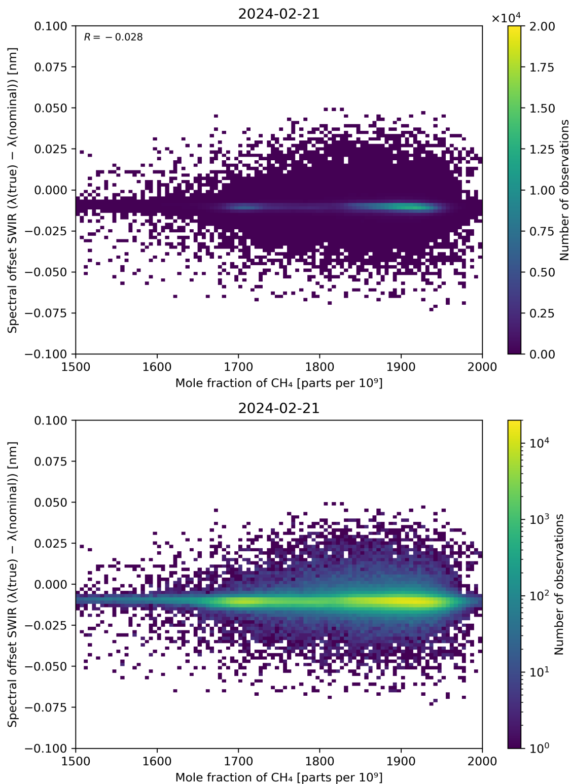
Figure 86: Scatter density plot of “Mole fraction of CH 4 ” against “Spectral offset SWIR ( \lambda(\text{true}) - \lambda(\text{nominal}) )” for 2024-02-20 to 2024-02-22.
