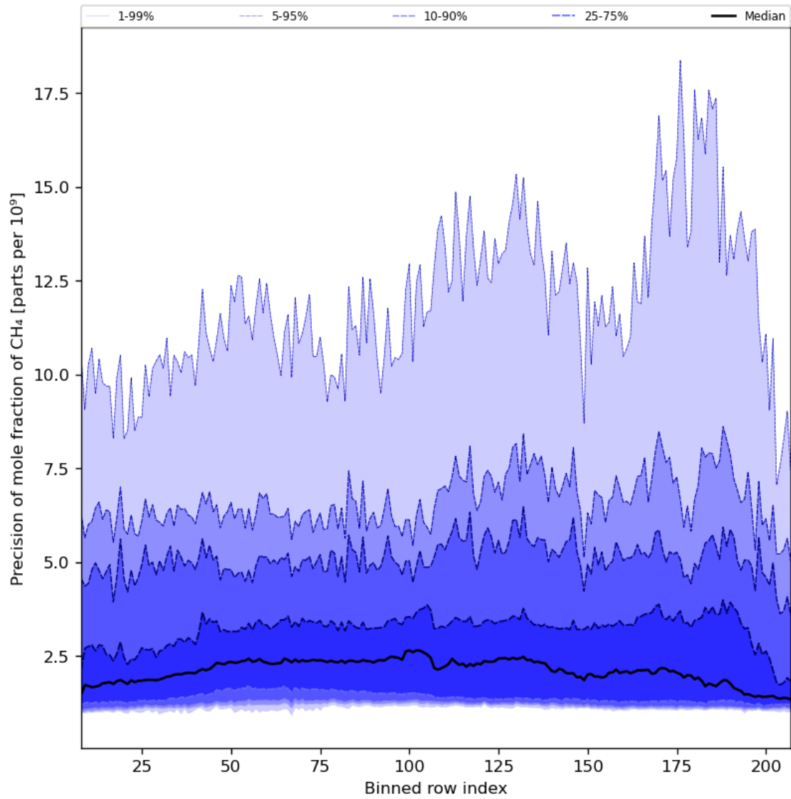
Figure 35: Along track statistics of “Precision of mole fraction of CH 4 ” for 2024-02-20 to 2024-02-22
