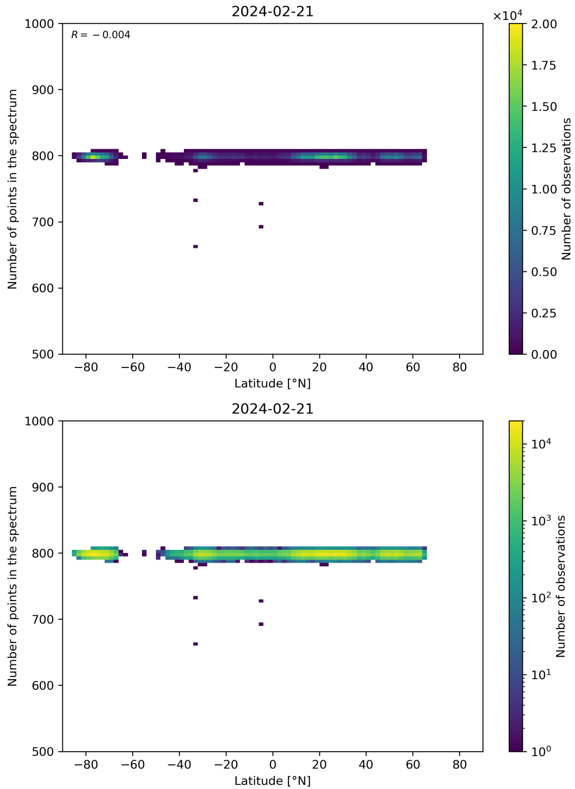
Figure 61: Scatter density plot of “Latitude” against “Number of points in the spectrum” for 2024-02-20 to 2024-02-22.
