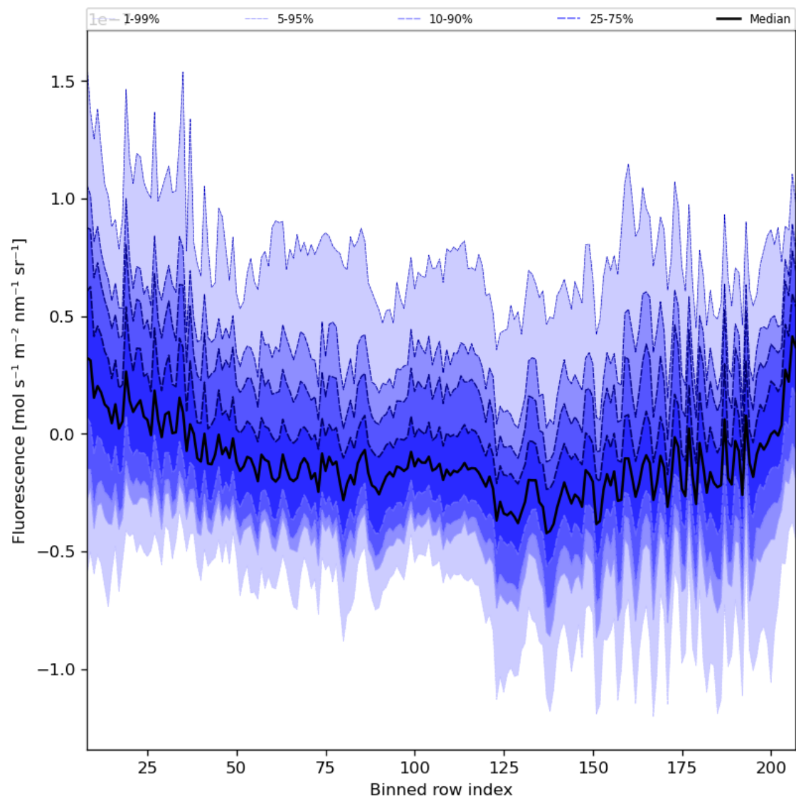
Figure 43: Along track statistics of “Fluorescence” for 2024-02-20 to 2024-02-22
