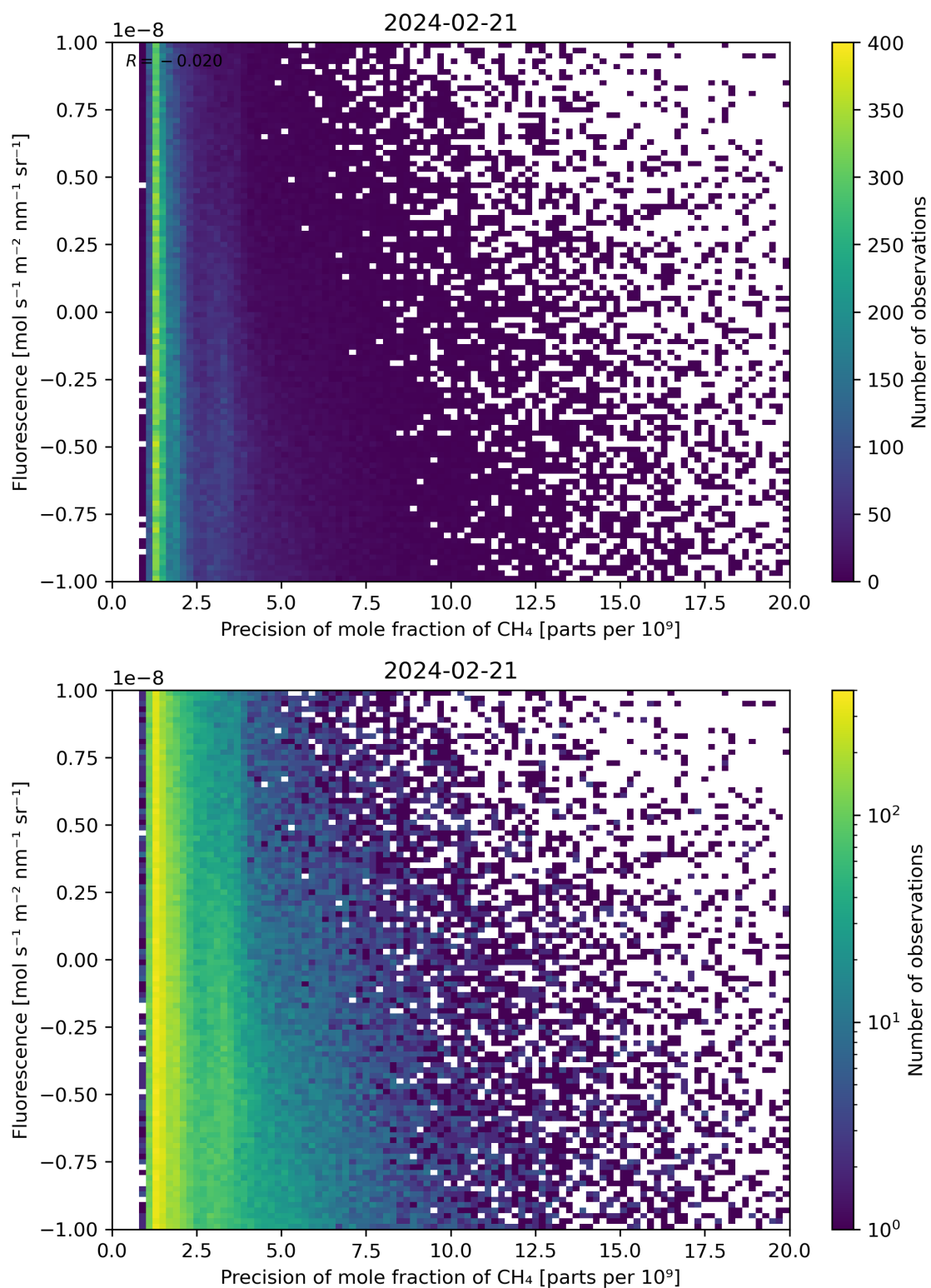
Figure 81: Scatter density plot of “Precision of mole fraction of \text{CH}_4 ” against “Fluorescence” for 2024-02-20 to 2024-02-22.
