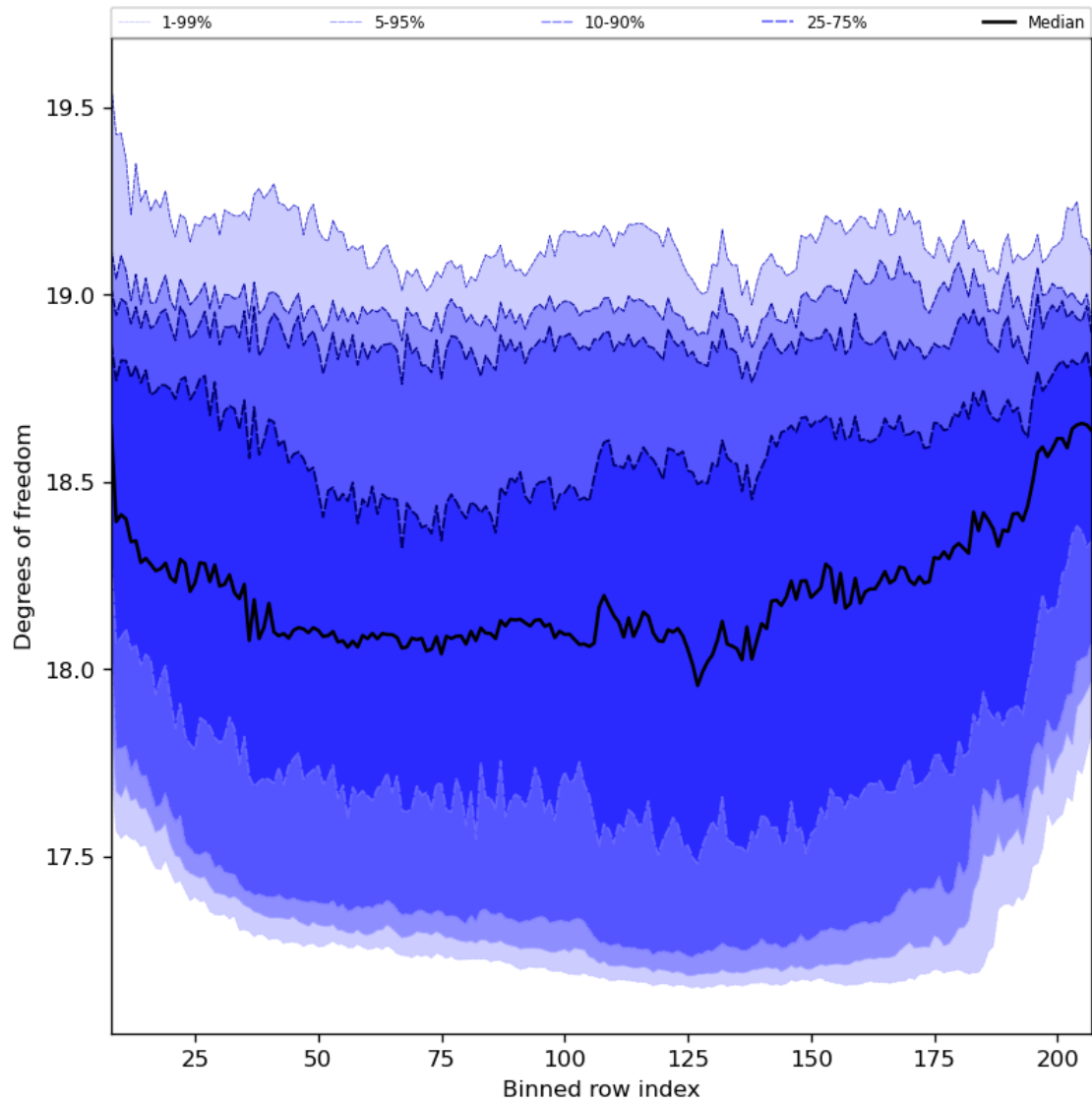
Figure 41: Along track statistics of “Degrees of freedom” for 2024-02-20 to 2024-02-22
