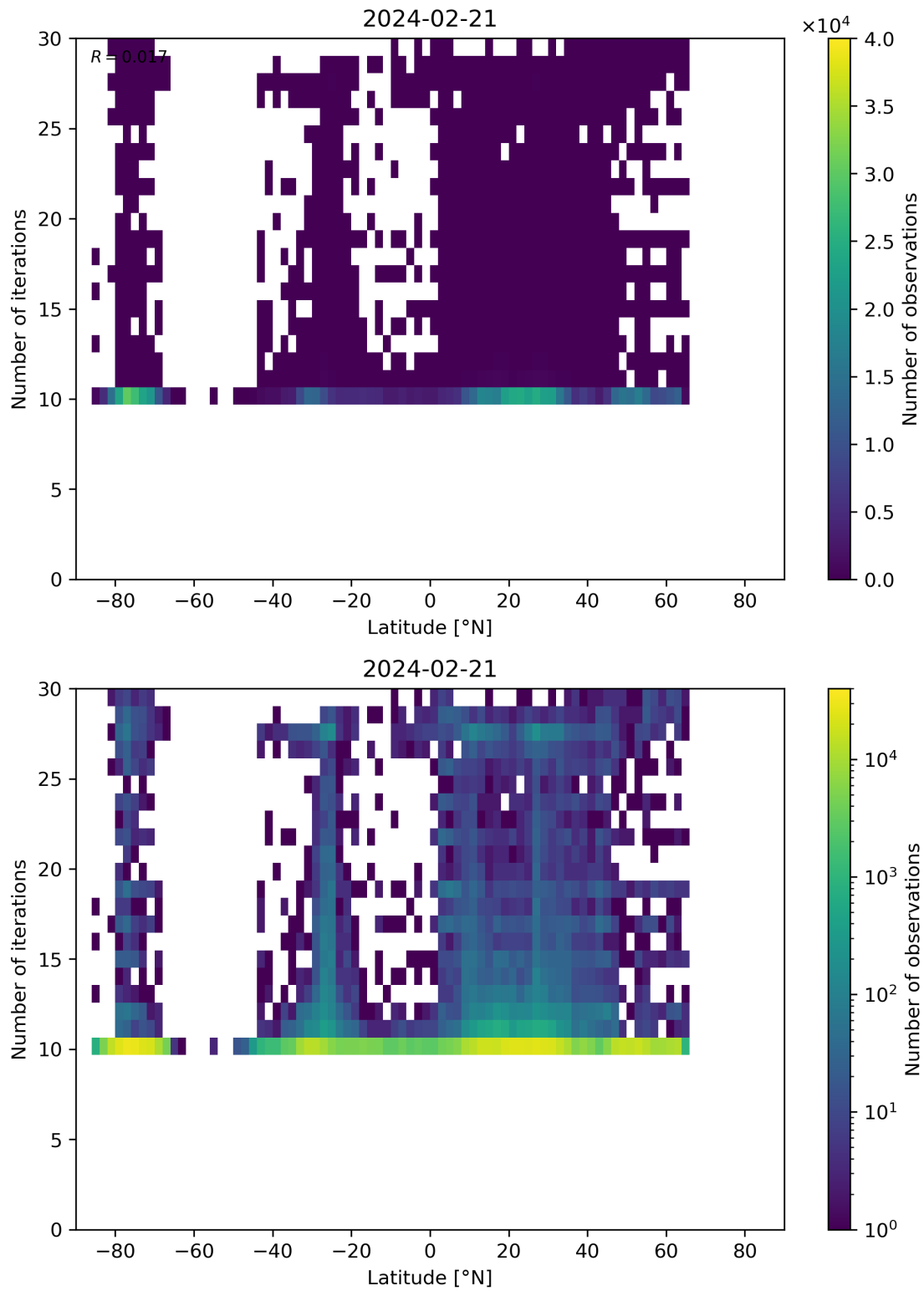
Figure 60: Scatter density plot of “Latitude” against “Number of iterations” for 2024-02-20 to 2024-02-22.
