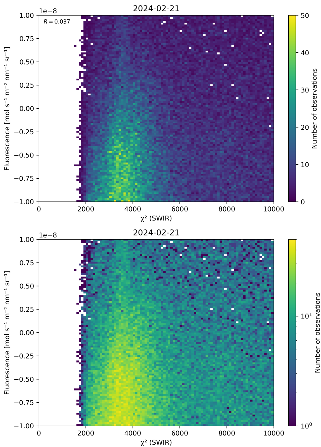
Figure 49: Scatter density plot of “ \chi^2 (SWIR)” against “Fluorescence” for 2024-02-20 to 2024-02-22.
