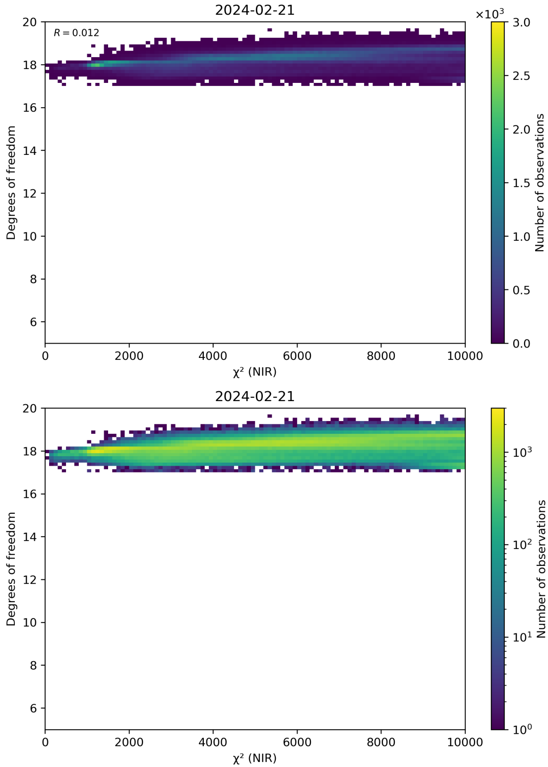
Figure 44: Scatter density plot of “ \chi^2 (NIR)” against “Degrees of freedom” for 2024-02-20 to 2024-02-22.
