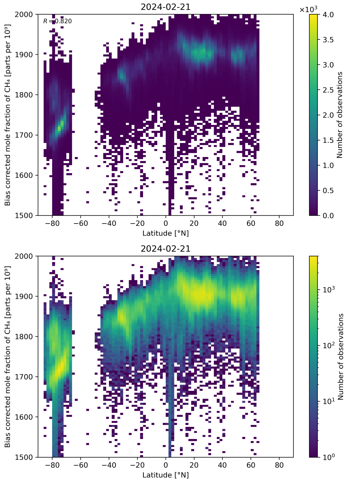
Figure 58: Scatter density plot of “Latitude” against “Bias corrected mole fraction of CH 4 ” for 2024-02-20 to 2024-02-22.
