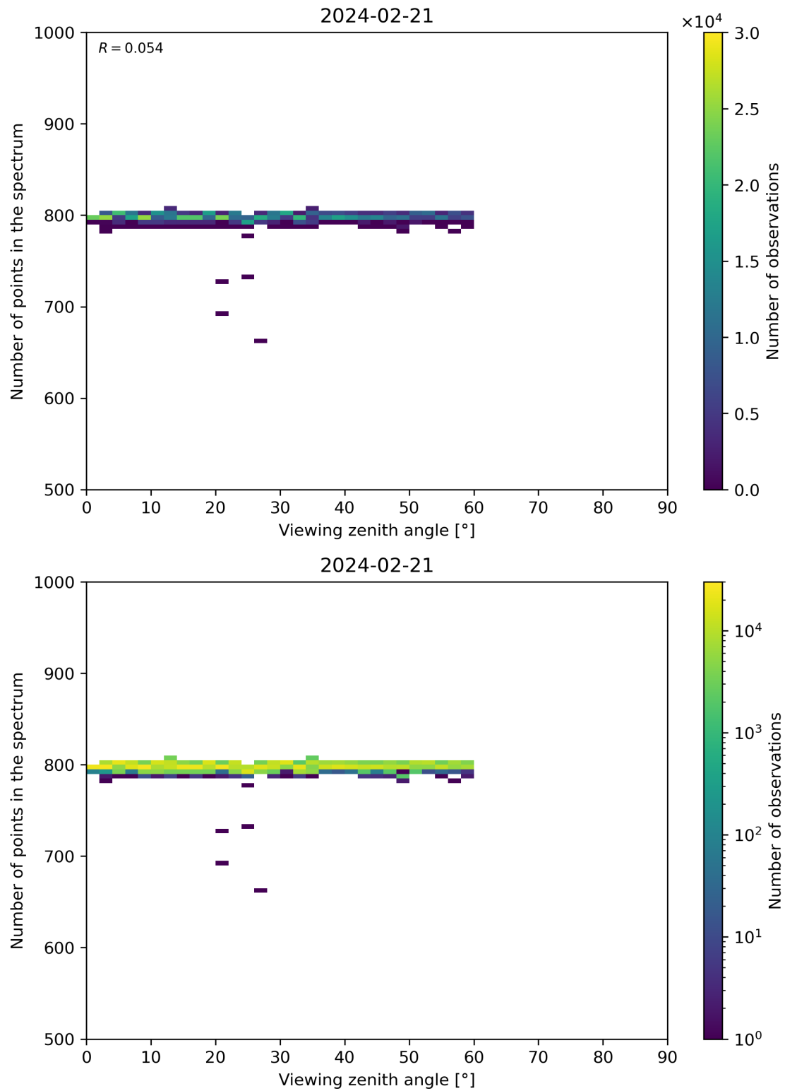
Figure 114: Scatter density plot of “Viewing zenith angle” against “Number of points in the spectrum” for 2024-02-20 to 2024-02-22.
