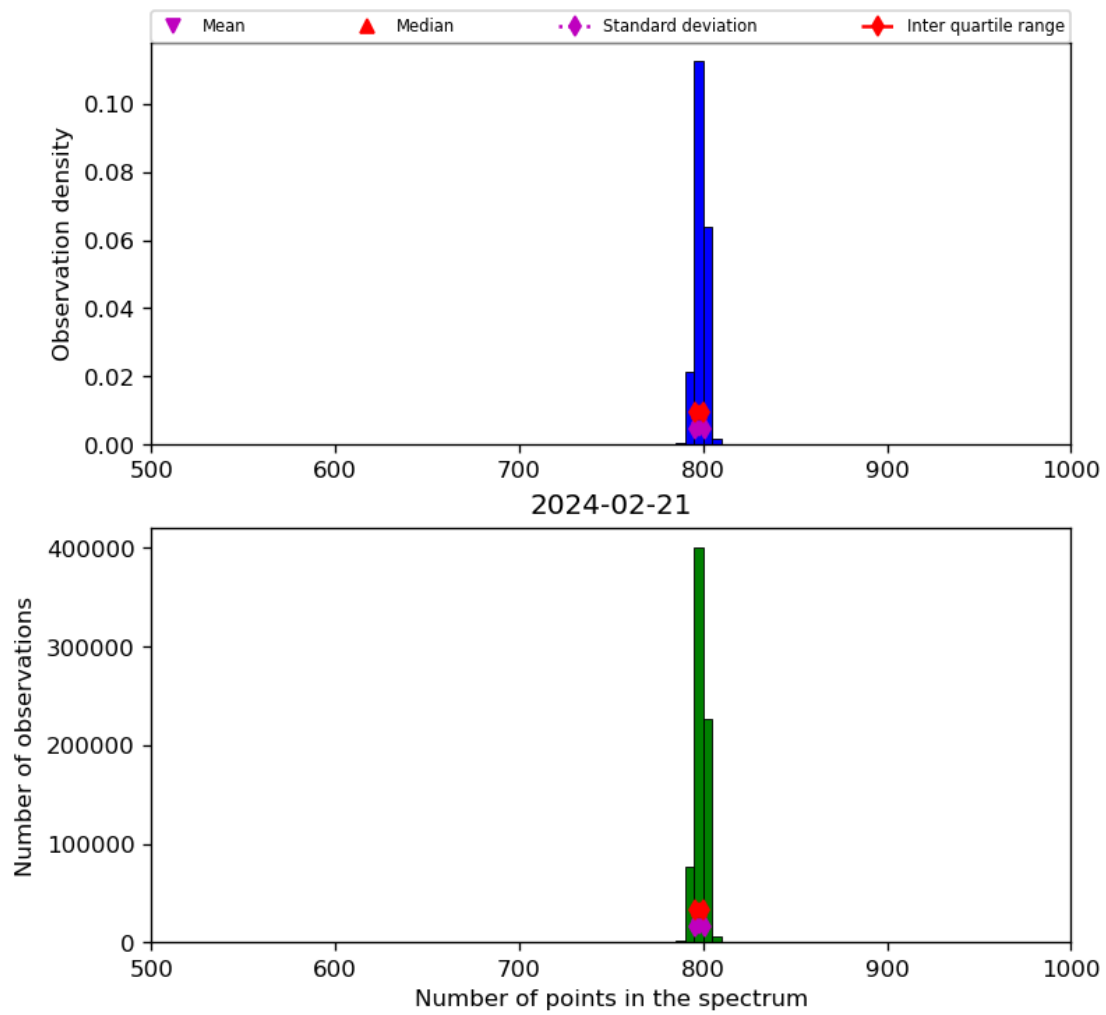
Figure 26: Histogram of “Number of points in the spectrum” for 2024-02-20 to 2024-02-22
