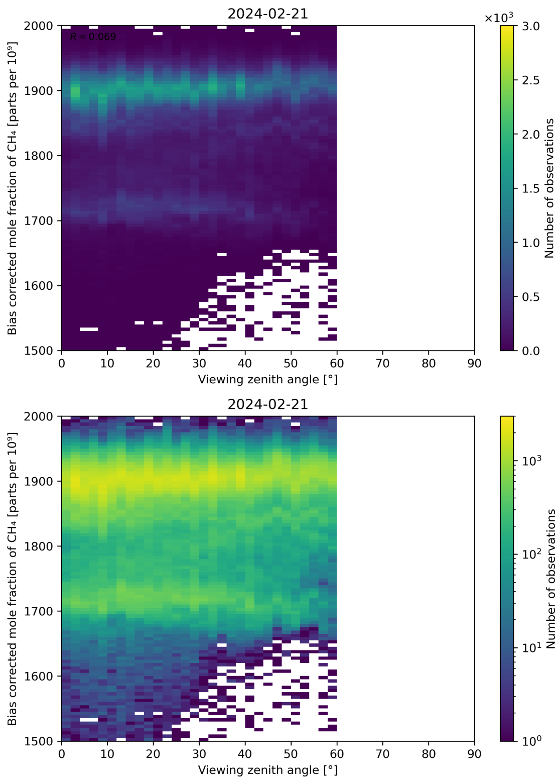
Figure 111: Scatter density plot of “Viewing zenith angle” against “Bias corrected mole fraction of CH 4 ” for 2024-02-20 to 2024-02-22.
