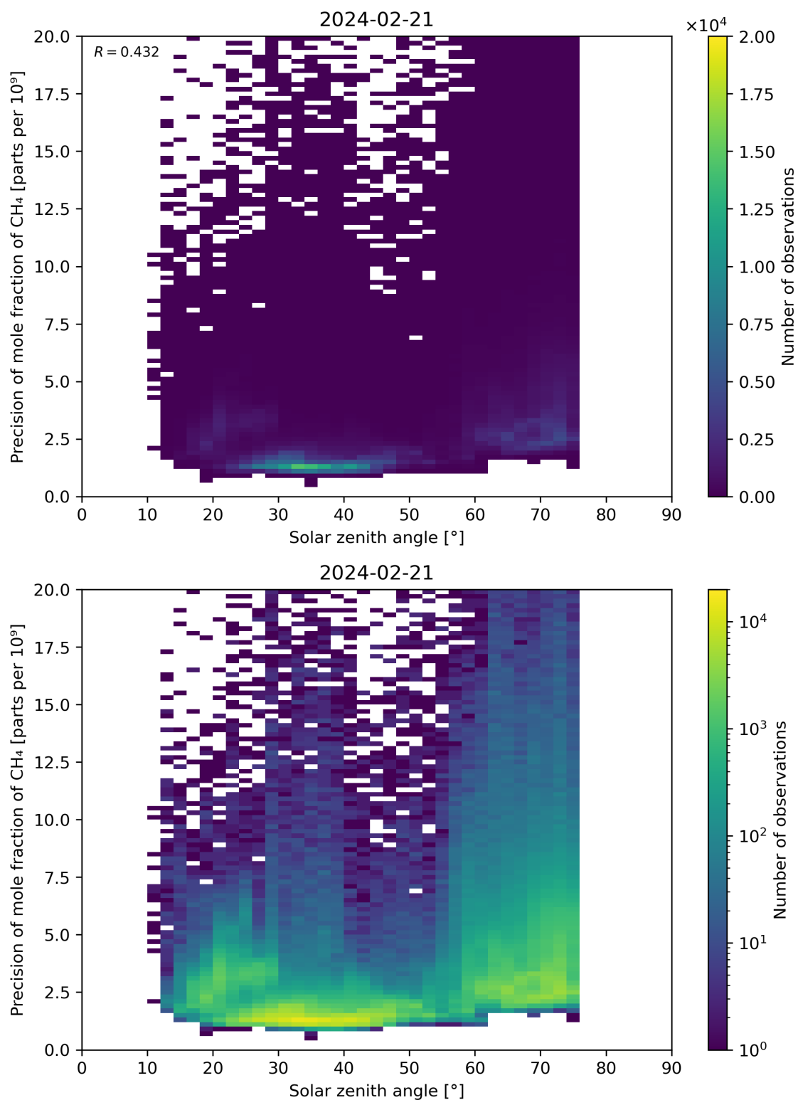
Figure 101: Scatter density plot of “Solar zenith angle” against “Precision of mole fraction of CH 4 ” for 2024-02-20 to 2024-02-22.
