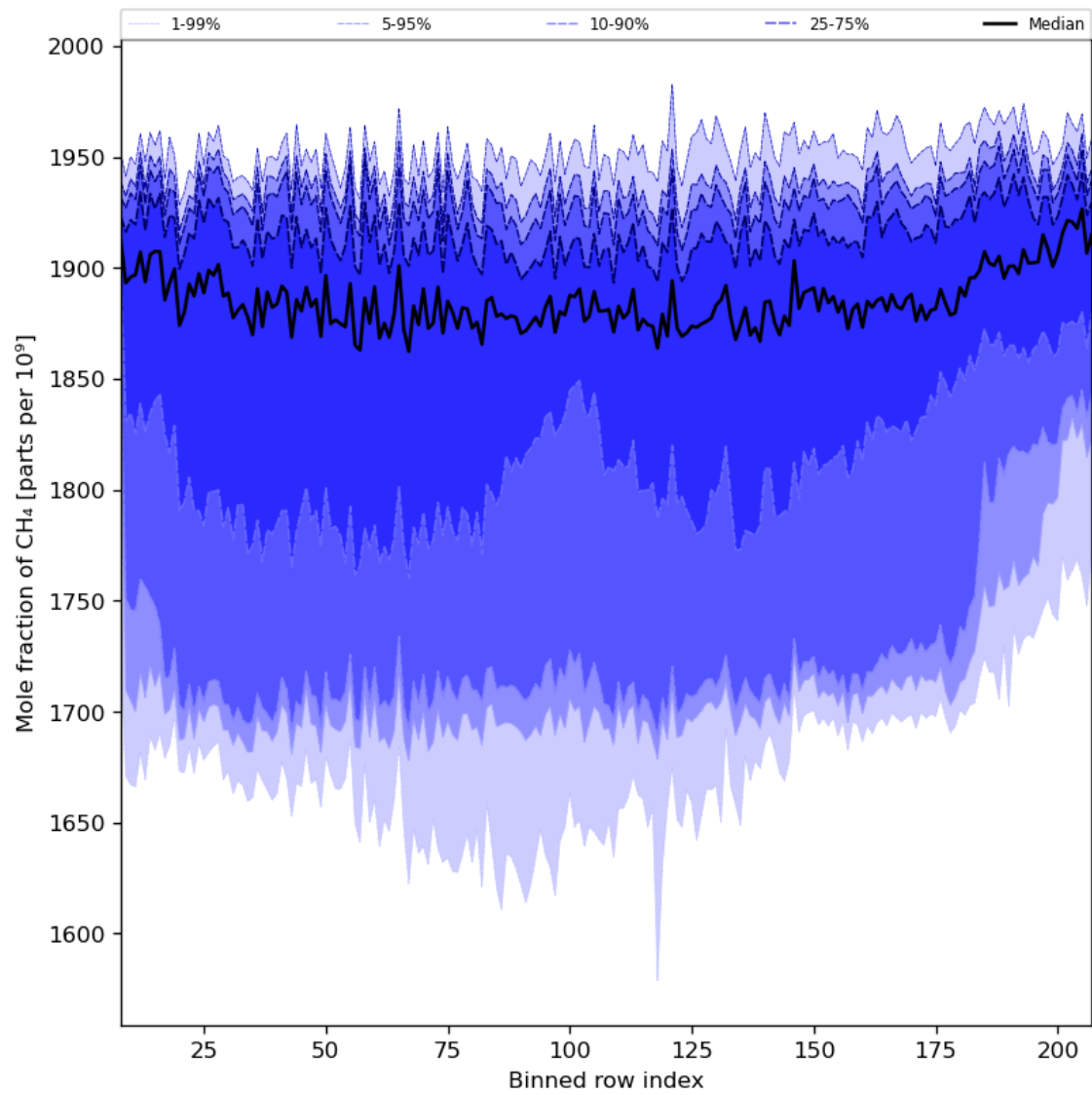
Figure 34: Along track statistics of “Mole fraction of CH 4 ” for 2024-02-20 to 2024-02-22
