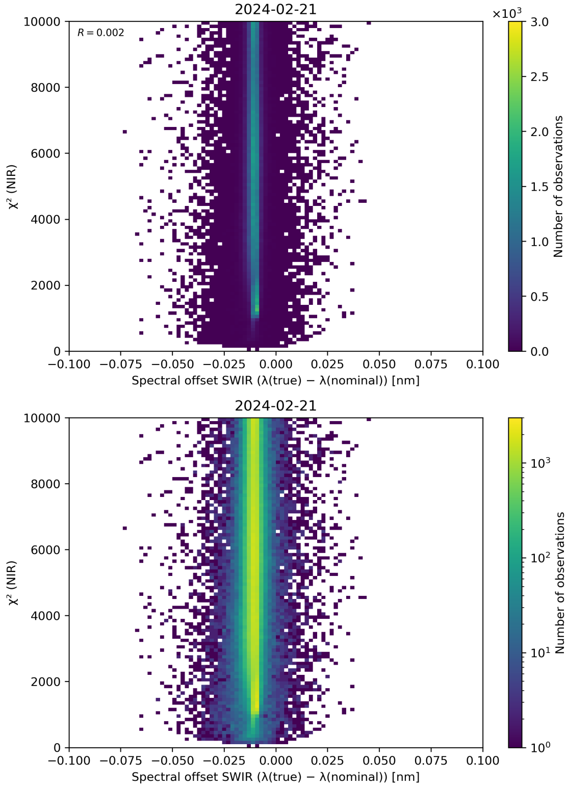
Figure 117: Scatter density plot of “Spectral offset SWIR ( \lambda(\text{true}) - \lambda(\text{nominal}) )” against “ \chi^2 (NIR)” for 2024-02-20 to 2024-02-22.
