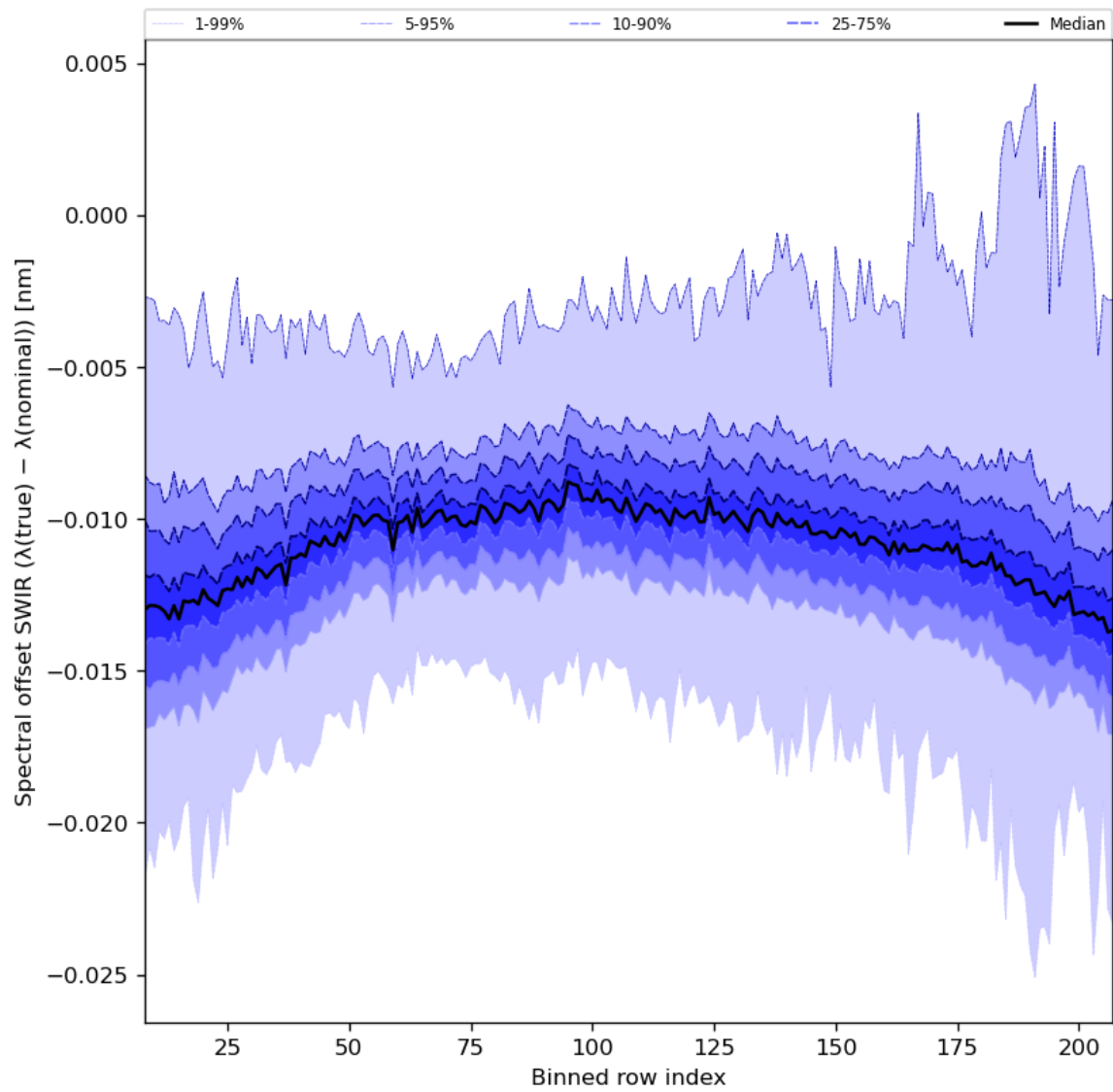
Figure 38: Along track statistics of “Spectral offset SWIR ( \lambda(\text{true}) - \lambda(\text{nominal}) )” for 2024-02-20 to 2024-02-22
