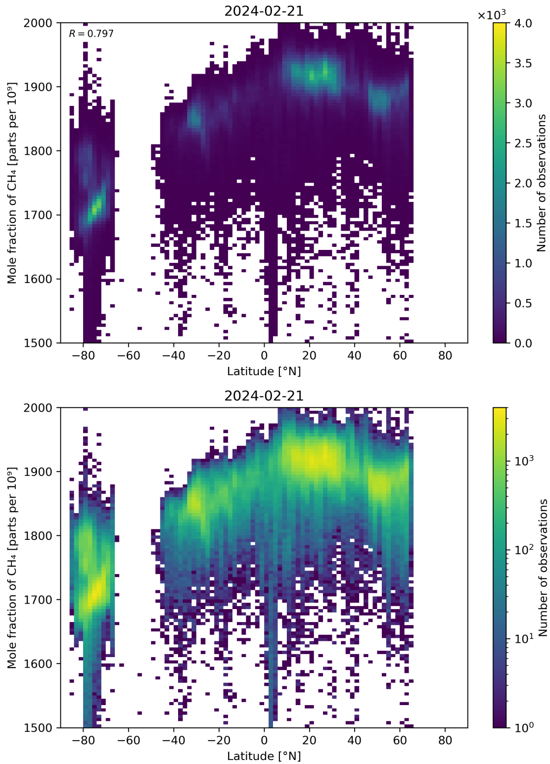
Figure 57: Scatter density plot of “Latitude” against “Mole fraction of CH 4 ” for 2024-02-20 to 2024-02-22.
