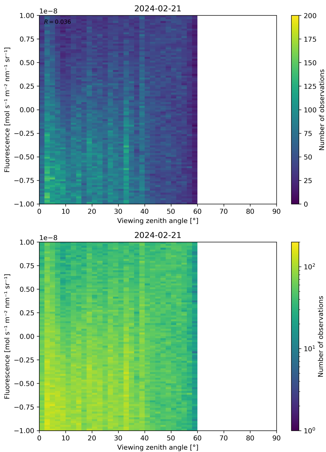
Figure 108: Scatter density plot of “Viewing zenith angle” against “Fluorescence” for 2024-02-20 to 2024-02-22.
