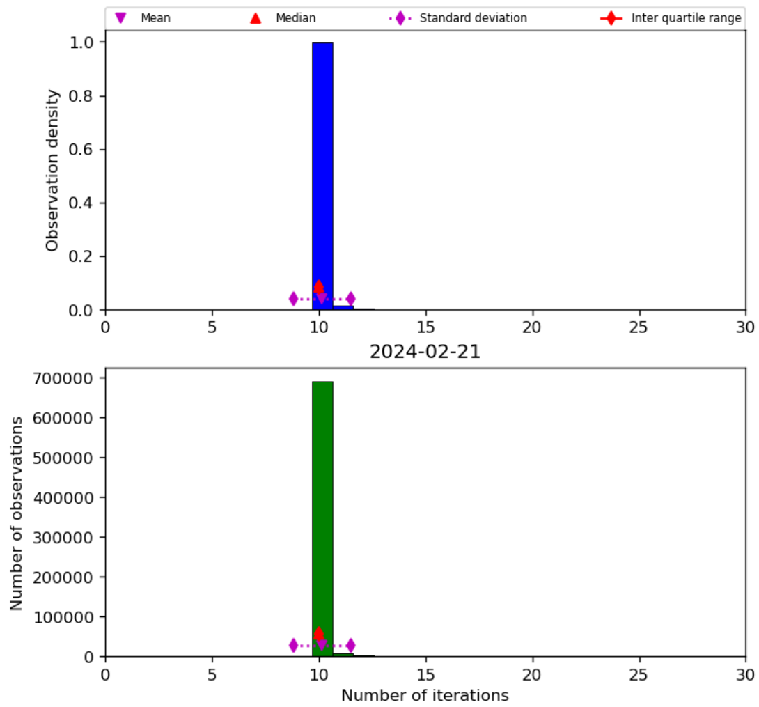
Figure 31: Histogram of “Number of iterations” for 2024-02-20 to 2024-02-22
