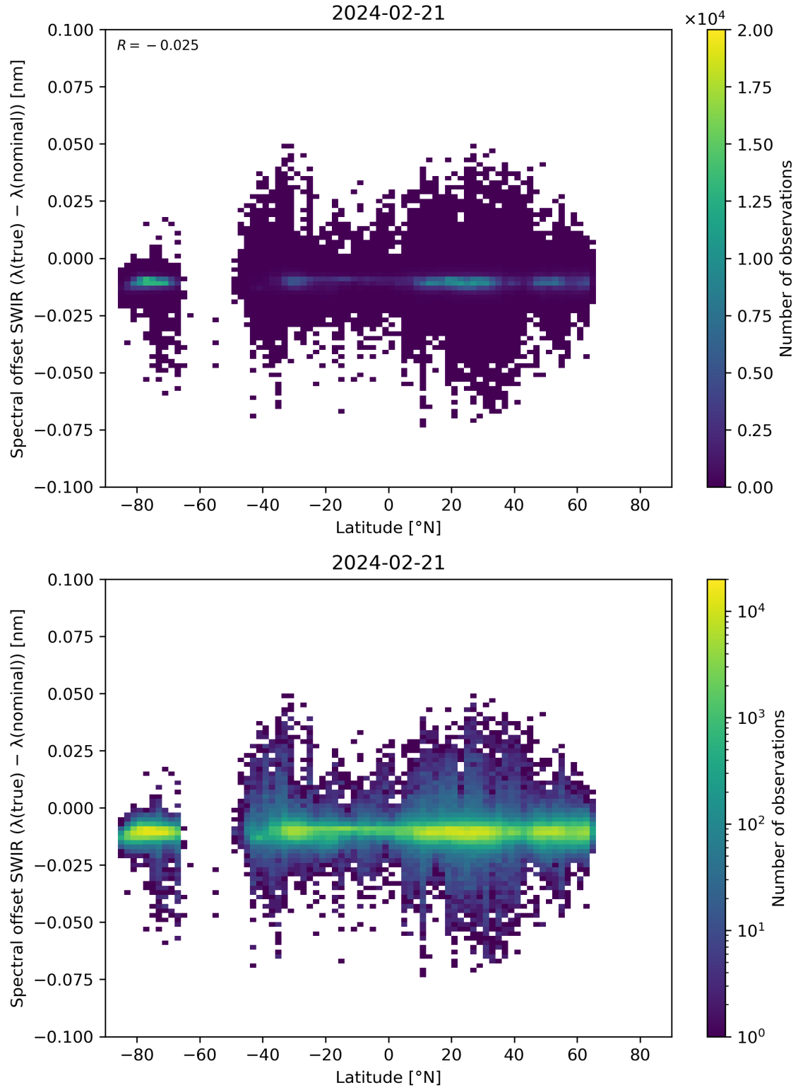
Figure 62: Scatter density plot of “Latitude” against “Spectral offset SWIR ( \lambda(\text{true}) - \lambda(\text{nominal}) )” for 2024-02-20 to 2024-02-22.
