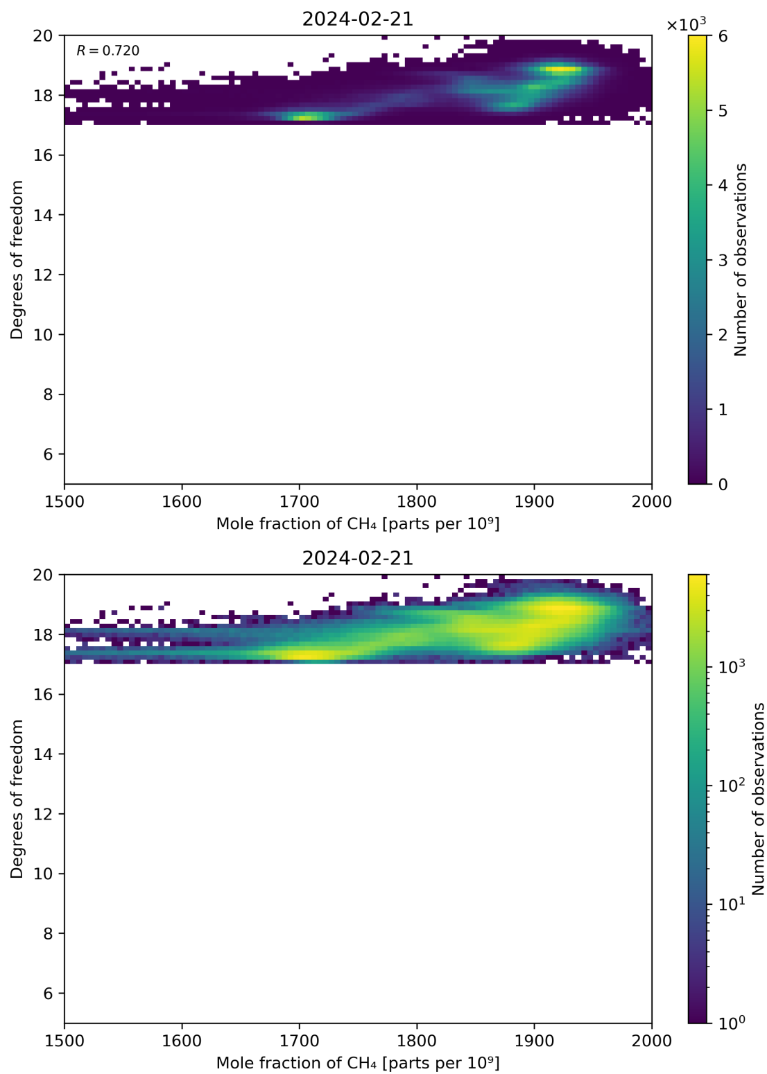
Figure 72: Scatter density plot of “Mole fraction of CH 4 ” against “Degrees of freedom” for 2024-02-20 to 2024-02-22.
