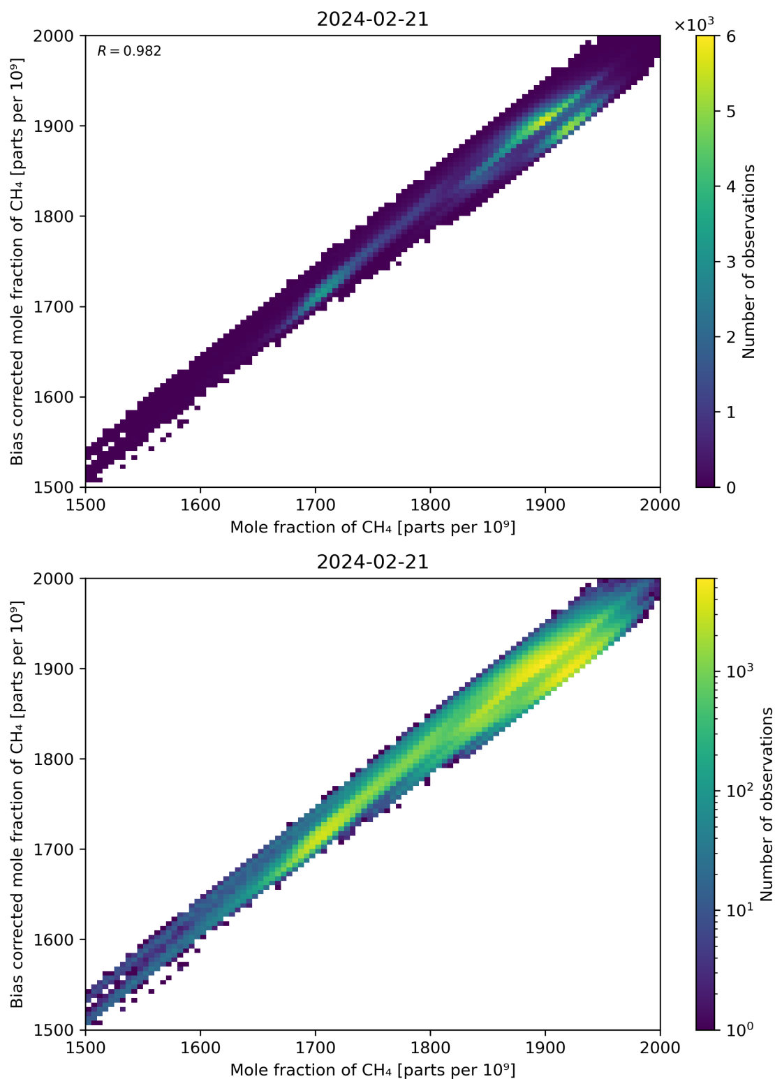
Figure 74: Scatter density plot of “Mole fraction of CH 4 ” against “Bias corrected mole fraction of CH 4 ” for 2024-02-20 to 2024-02-22.
