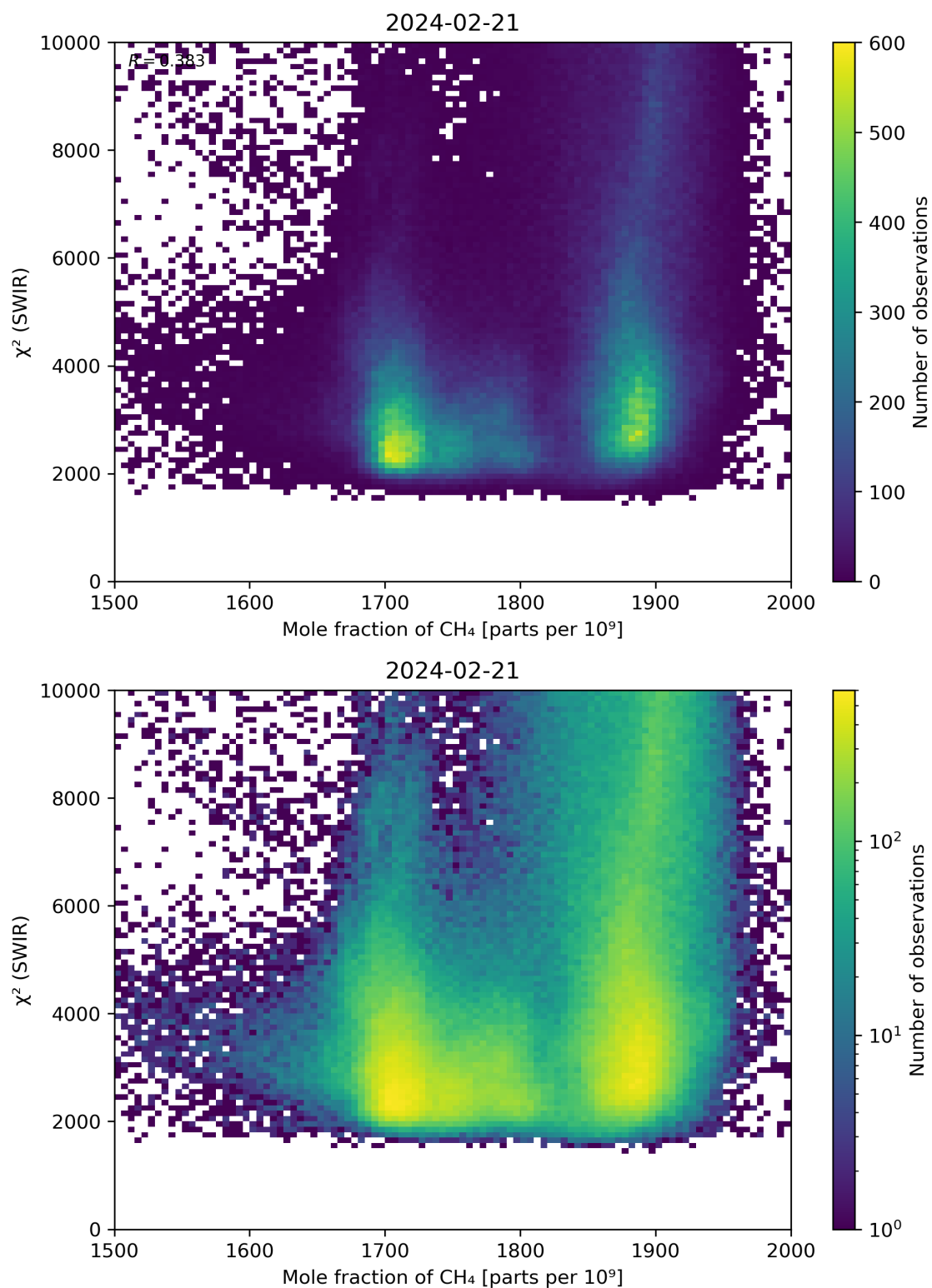
Figure 71: Scatter density plot of “Mole fraction of CH 4 ” against “ \chi^2 (SWIR)” for 2024-02-20 to 2024-02-22.
