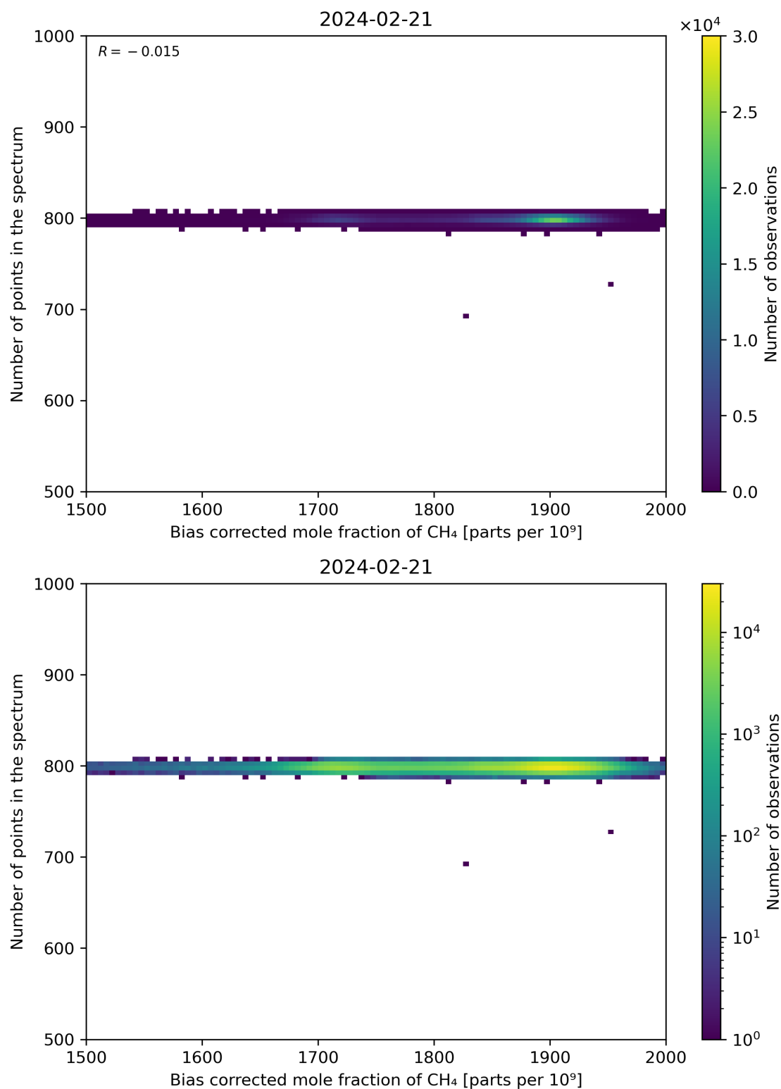
Figure 68: Scatter density plot of “Bias corrected mole fraction of CH 4 ” against “Number of points in the spectrum” for 2024-02-20 to 2024-02-22.
