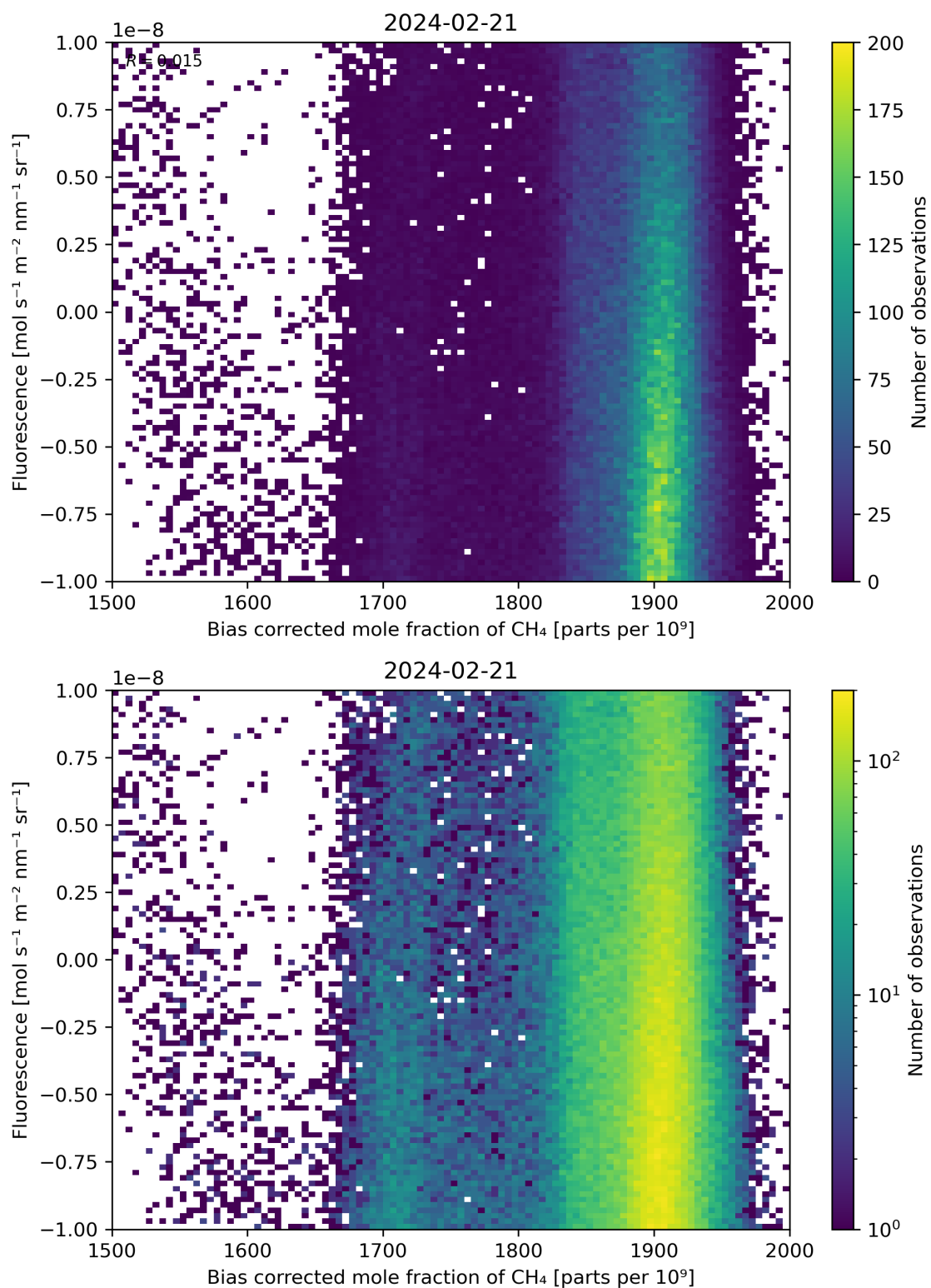
Figure 66: Scatter density plot of “Bias corrected mole fraction of CH 4 ” against “Fluorescence” for 2024-02-20 to 2024-02-22.
