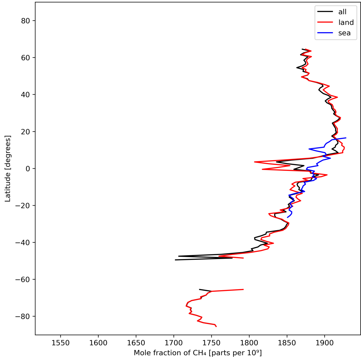
Figure 12: Zonal average of “Mole fraction of CH 4 ” for 2024-02-20 to 2024-02-22.
