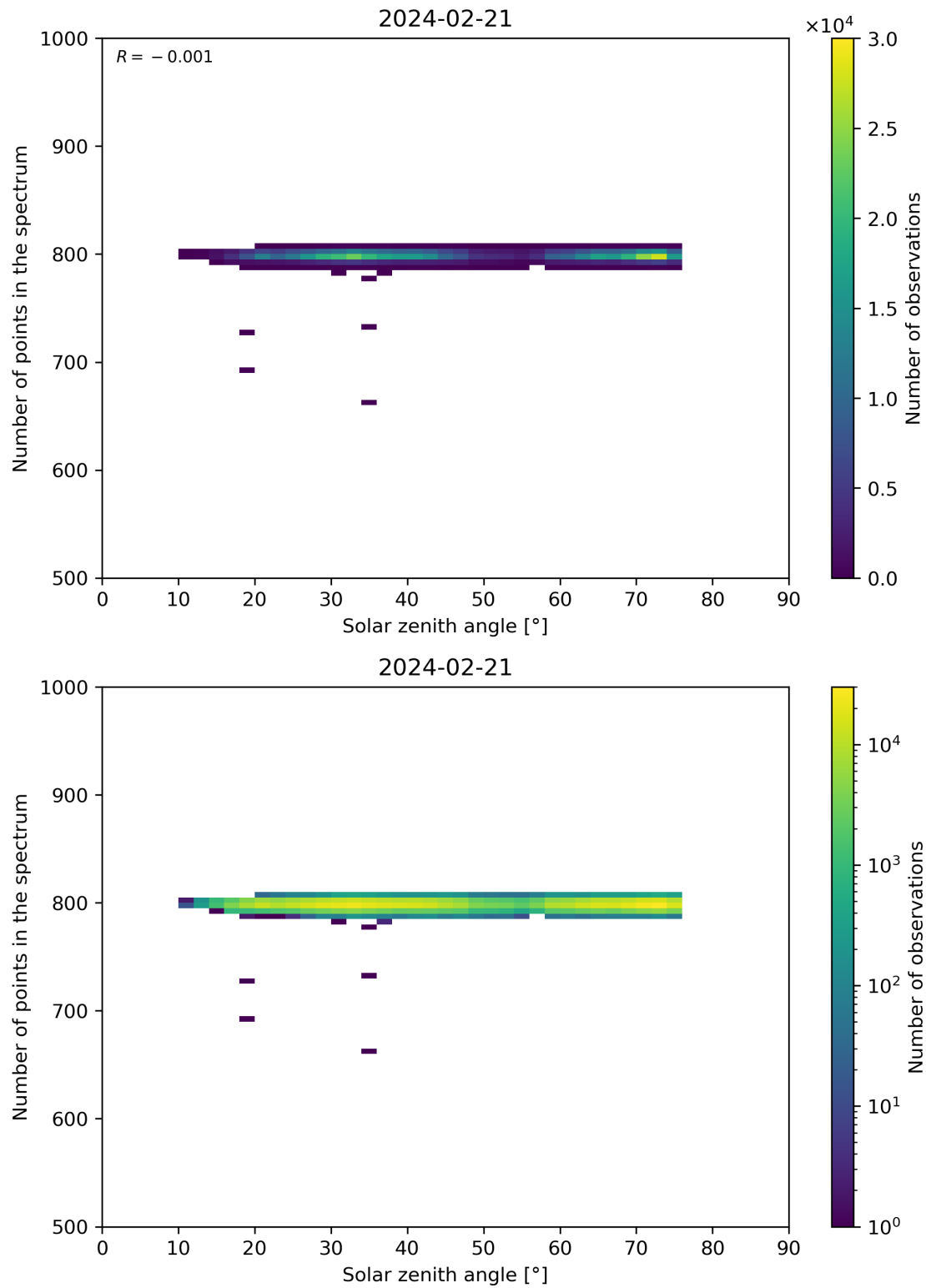
Figure 103: Scatter density plot of “Solar zenith angle” against “Number of points in the spectrum” for 2024-02-20 to 2024-02-22.
