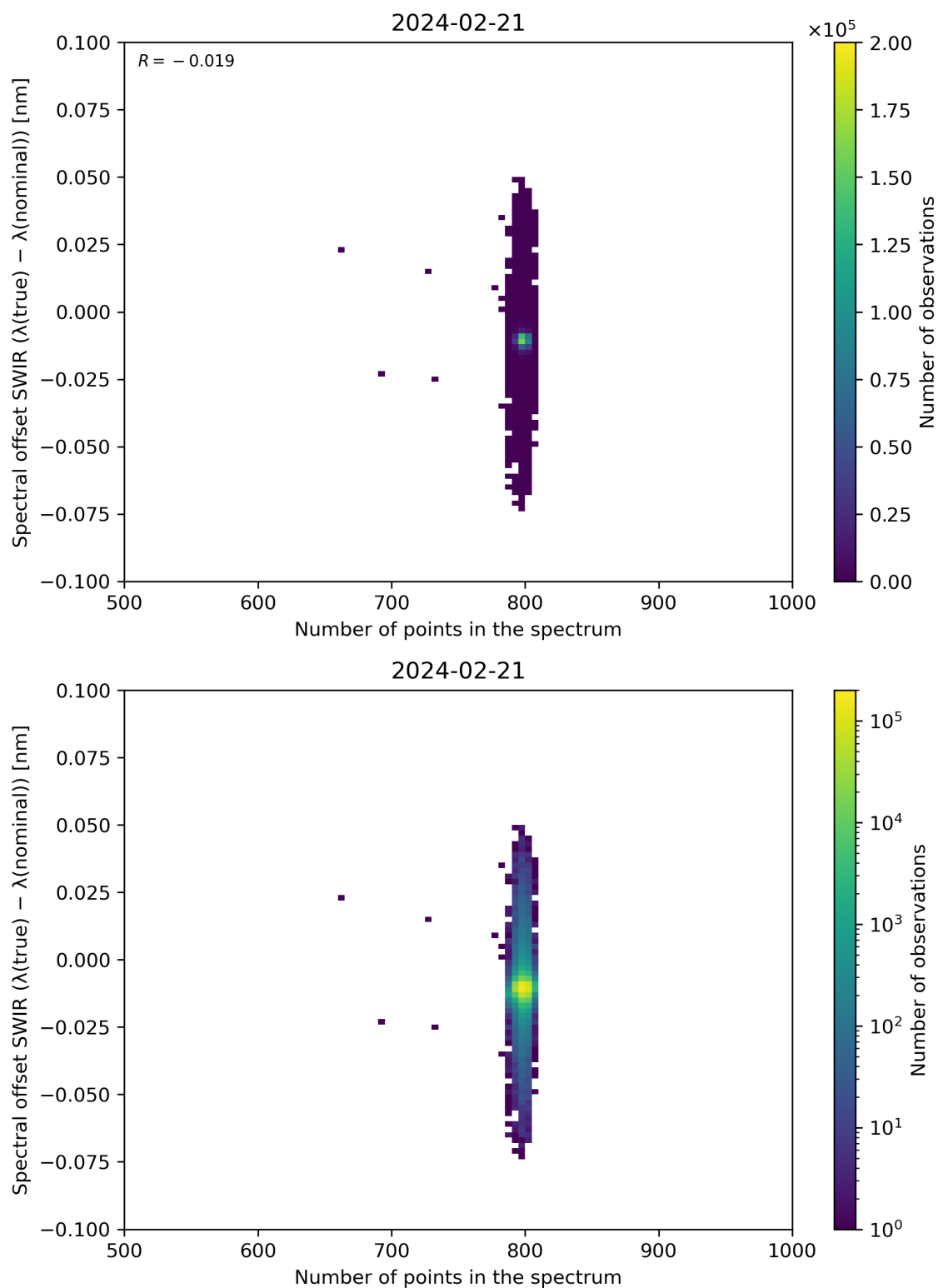
Figure 93: Scatter density plot of “Number of points in the spectrum” against “Spectral offset SWIR ( \lambda(\text{true}) - \lambda(\text{nominal}) )” for 2024-02-20 to 2024-02-22.
