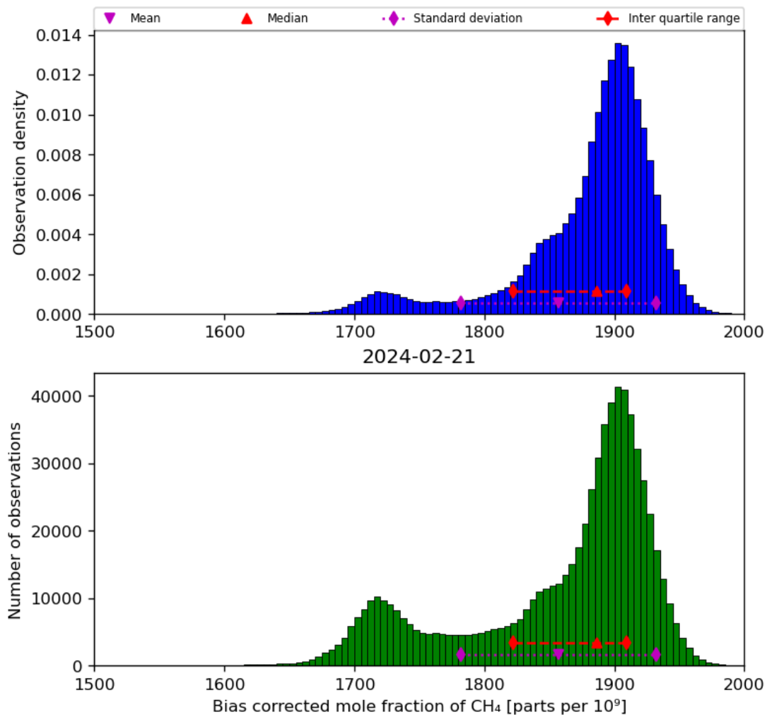
Figure 25: Histogram of “Bias corrected mole fraction of CH 4 ” for 2024-02-20 to 2024-02-22
