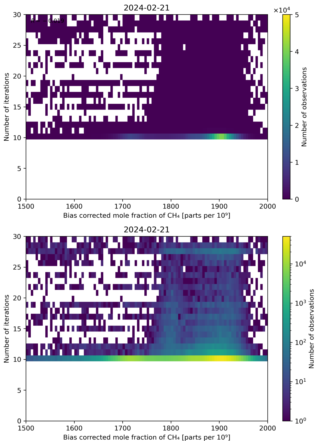
Figure 67: Scatter density plot of “Bias corrected mole fraction of \text{CH}_4 ” against “Number of iterations” for 2024-02-20 to 2024-02-22.
