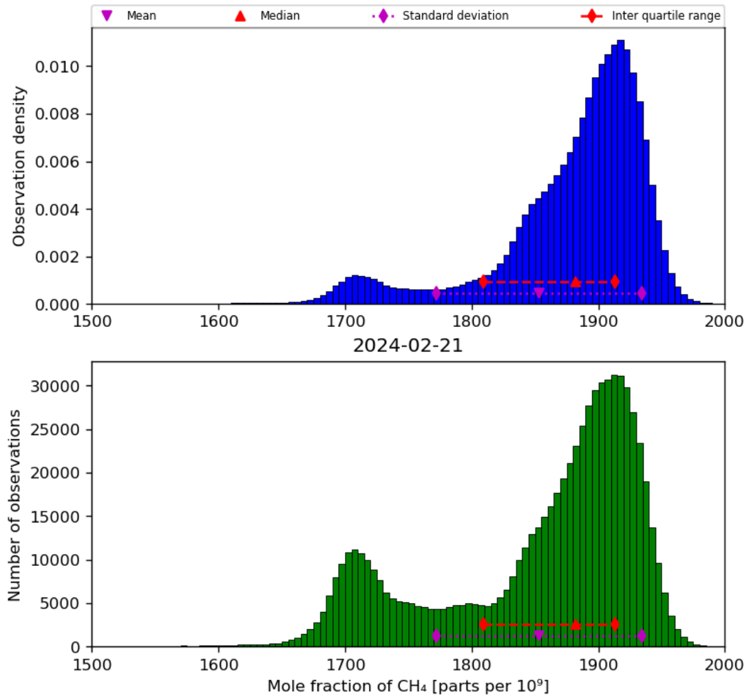
Figure 23: Histogram of “Mole fraction of CH 4 ” for 2024-02-20 to 2024-02-22
