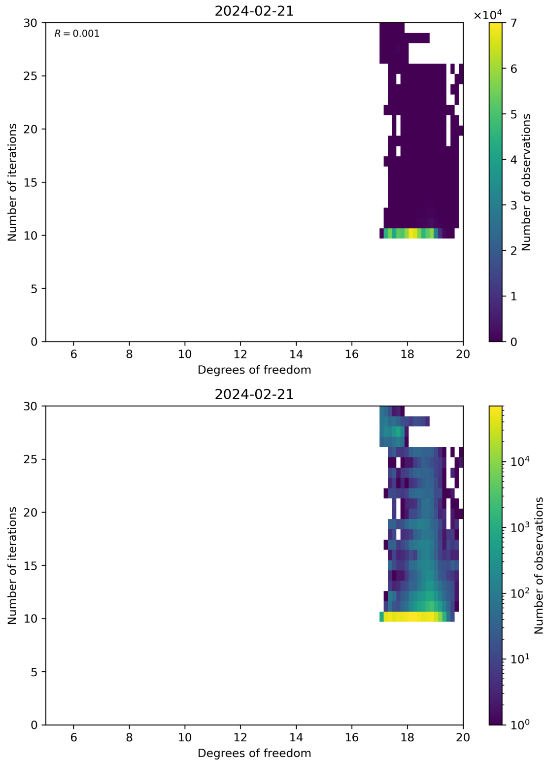
Figure 52: Scatter density plot of “Degrees of freedom” against “Number of iterations” for 2024-02-20 to 2024-02-22.
