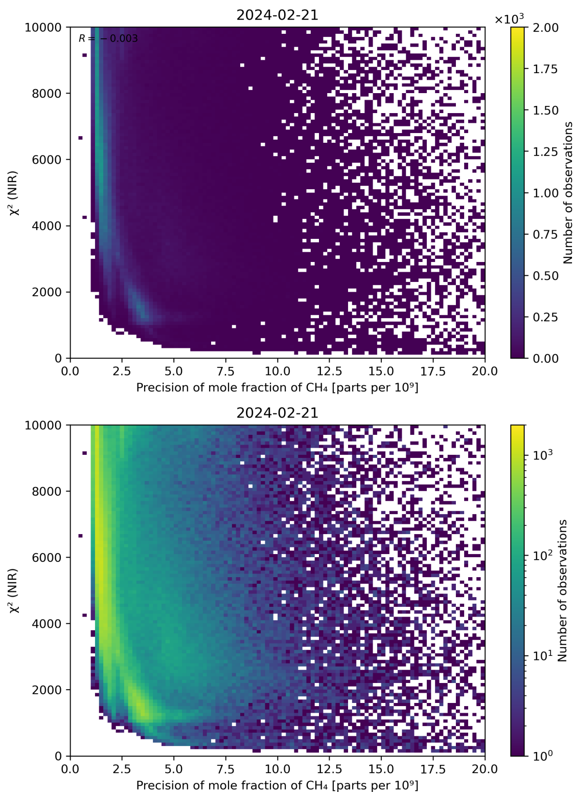
Figure 78: Scatter density plot of “Precision of mole fraction of CH 4 ” against “ \chi^2 (NIR)” for 2024-02-20 to 2024-02-22.
