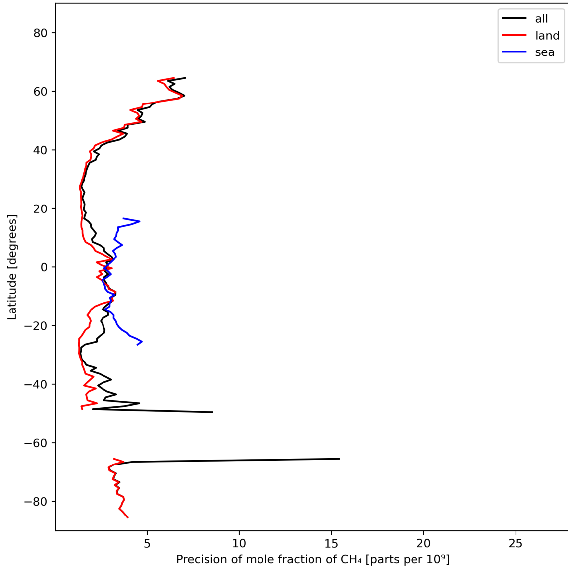
Figure 13: Zonal average of “Precision of mole fraction of CH 4 ” for 2024-02-20 to 2024-02-22.
