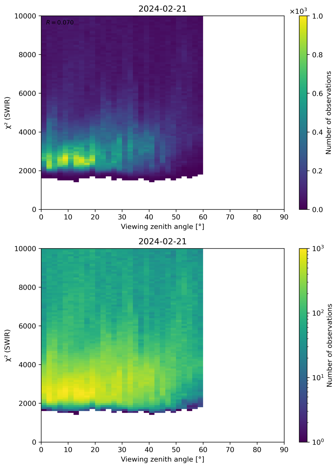
Figure 106: Scatter density plot of “Viewing zenith angle” against “ \chi^2 (SWIR)” for 2024-02-20 to 2024-02-22.
