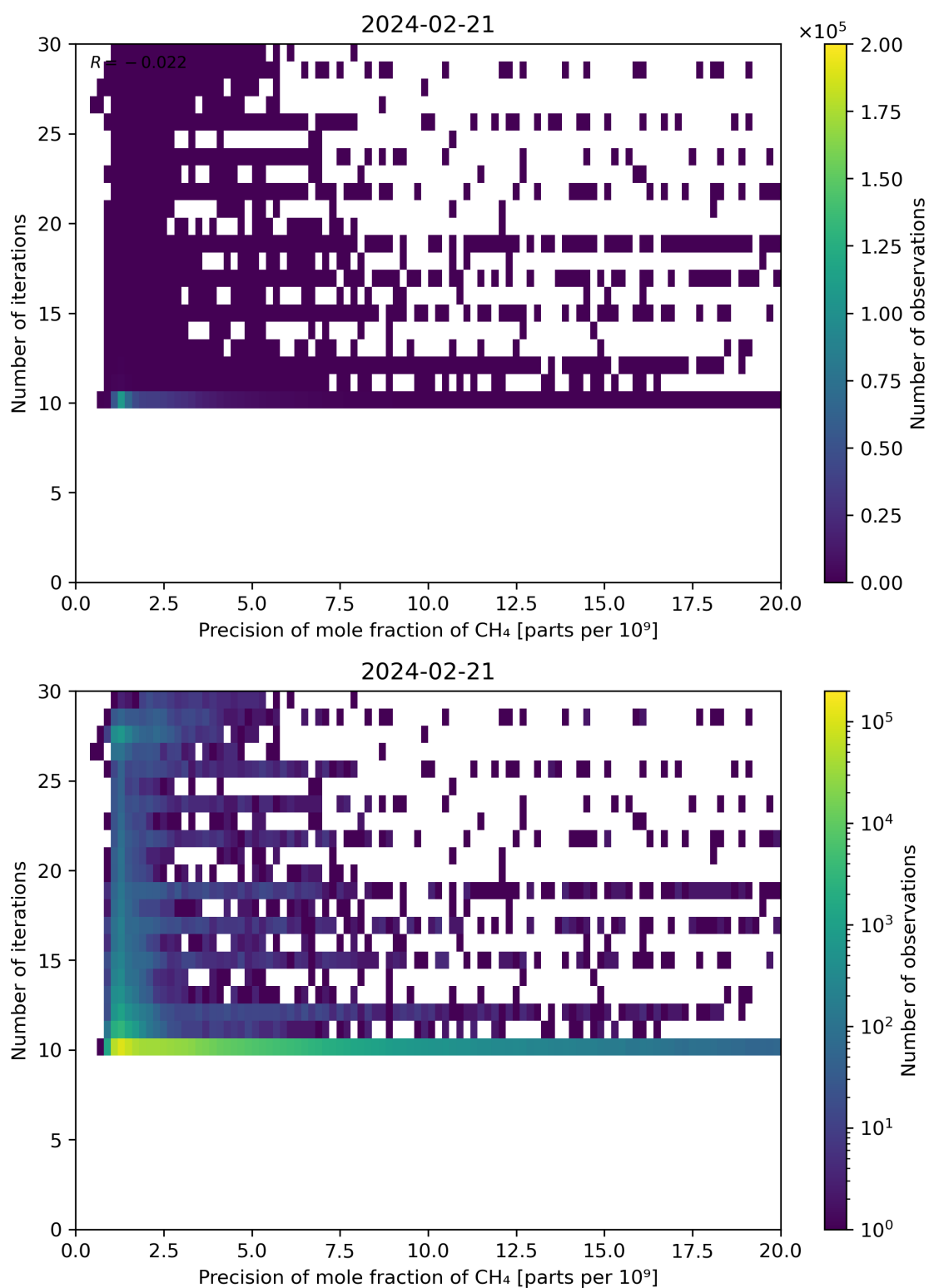
Figure 83: Scatter density plot of “Precision of mole fraction of CH 4 ” against “Number of iterations” for 2024-02-20 to 2024-02-22.
