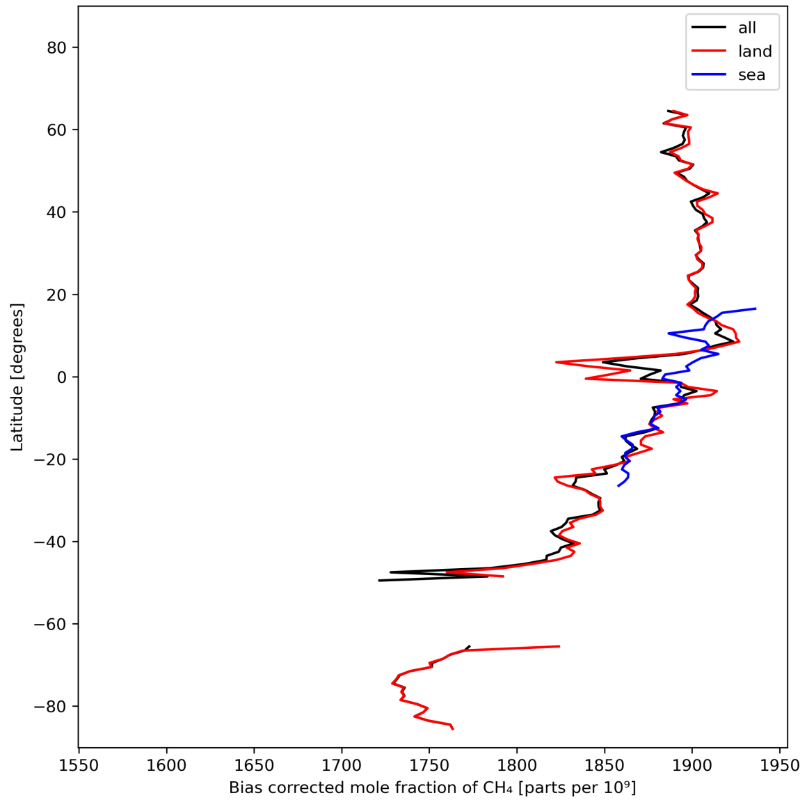
Figure 14: Zonal average of “Bias corrected mole fraction of CH 4 ” for 2024-02-20 to 2024-02-22.
