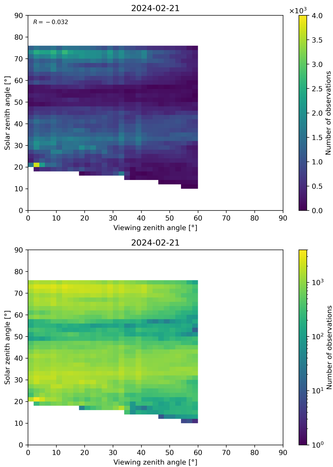
Figure 115: Scatter density plot of “Viewing zenith angle” against “Solar zenith angle” for 2024-02-20 to 2024-02-22.
