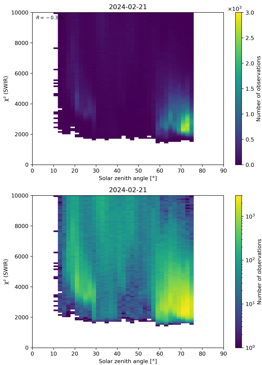
Figure 95: Scatter density plot of “Solar zenith angle” against “ \chi^2 (SWIR)” for 2024-02-20 to 2024-02-22.
