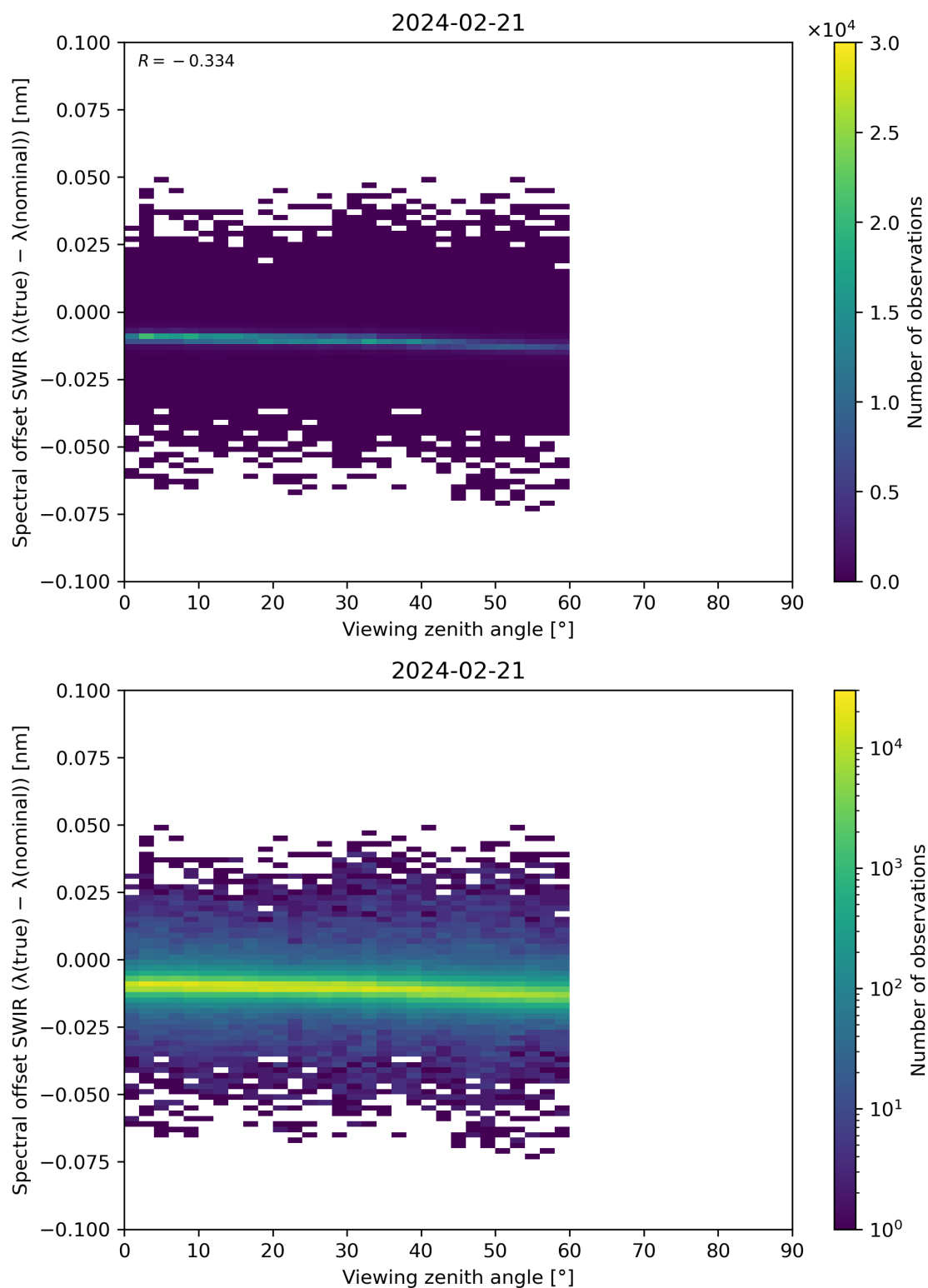
Figure 116: Scatter density plot of “Viewing zenith angle” against “Spectral offset SWIR ( \lambda(\text{true}) - \lambda(\text{nominal}) )” for 2024-02-20 to 2024-02-22.
