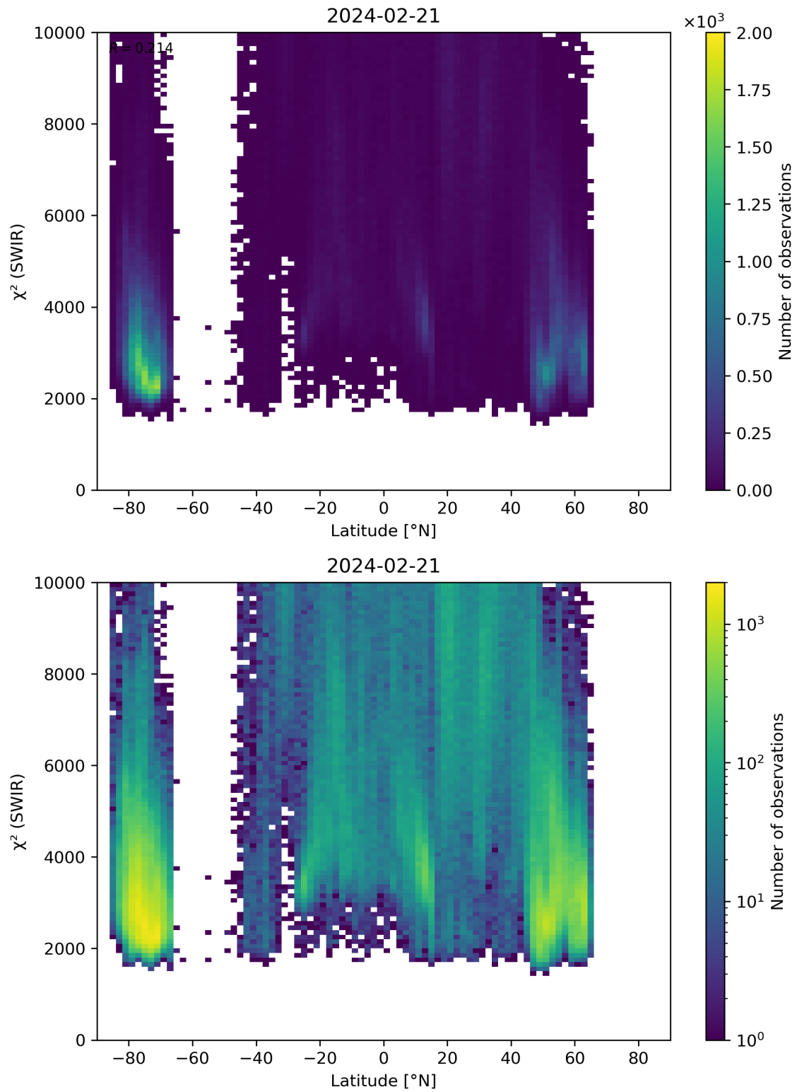
Figure 54: Scatter density plot of “Latitude” against “ \chi^2 (SWIR)” for 2024-02-20 to 2024-02-22.
