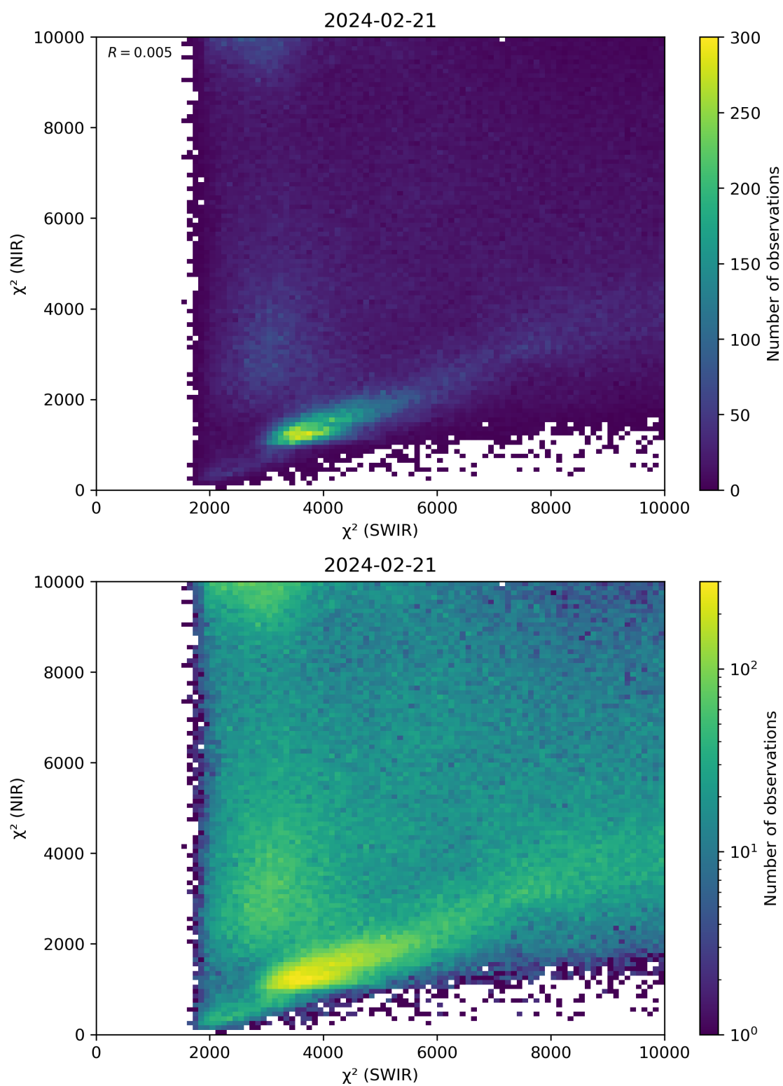
Figure 47: Scatter density plot of “ \chi^2 (SWIR)” against “ \chi^2 (NIR)” for 2024-02-20 to 2024-02-22.
