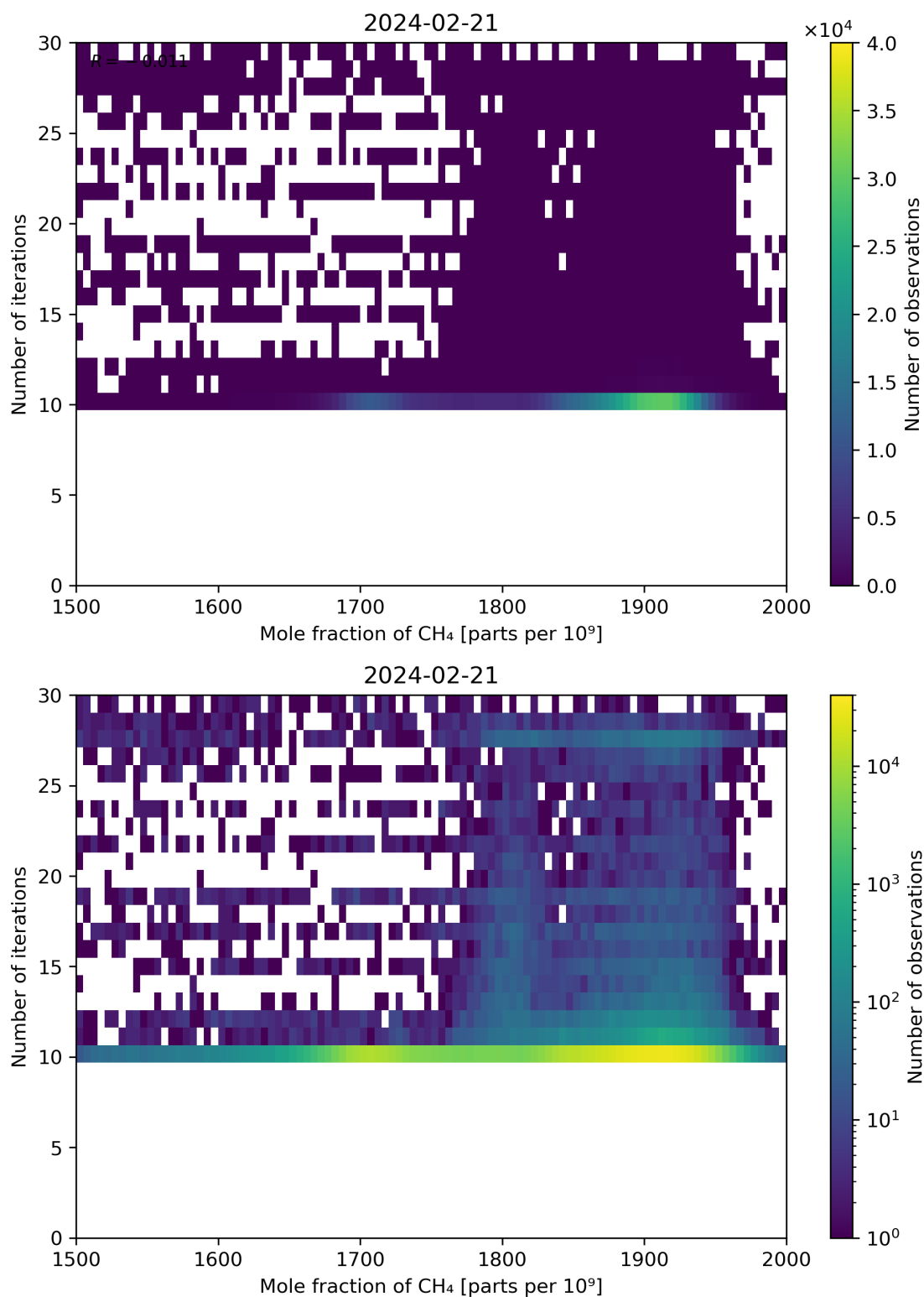
Figure 76: Scatter density plot of “Mole fraction of CH 4 ” against “Number of iterations” for 2024-02-20 to 2024-02-22.
