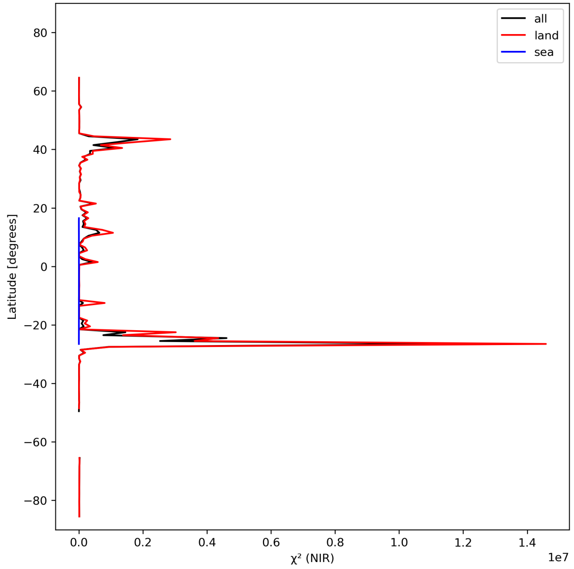
Figure 18: Zonal average of “ \chi^2 (NIR)” for 2024-02-20 to 2024-02-22.
