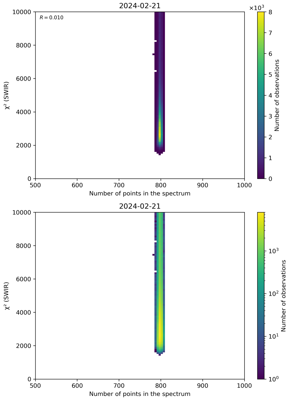
Figure 89: Scatter density plot of “Number of points in the spectrum” against “ \chi^2 (SWIR)” for 2024-02-20 to 2024-02-22.
