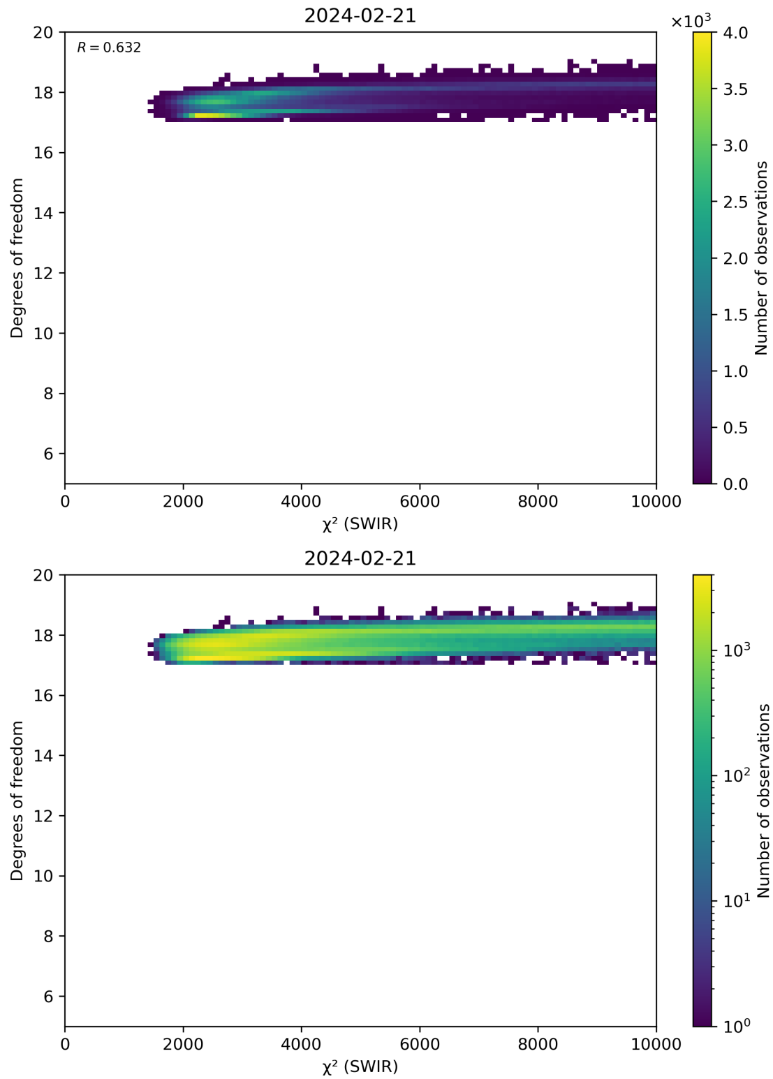
Figure 48: Scatter density plot of “ \chi^2 (SWIR)” against “Degrees of freedom” for 2024-02-20 to 2024-02-22.
