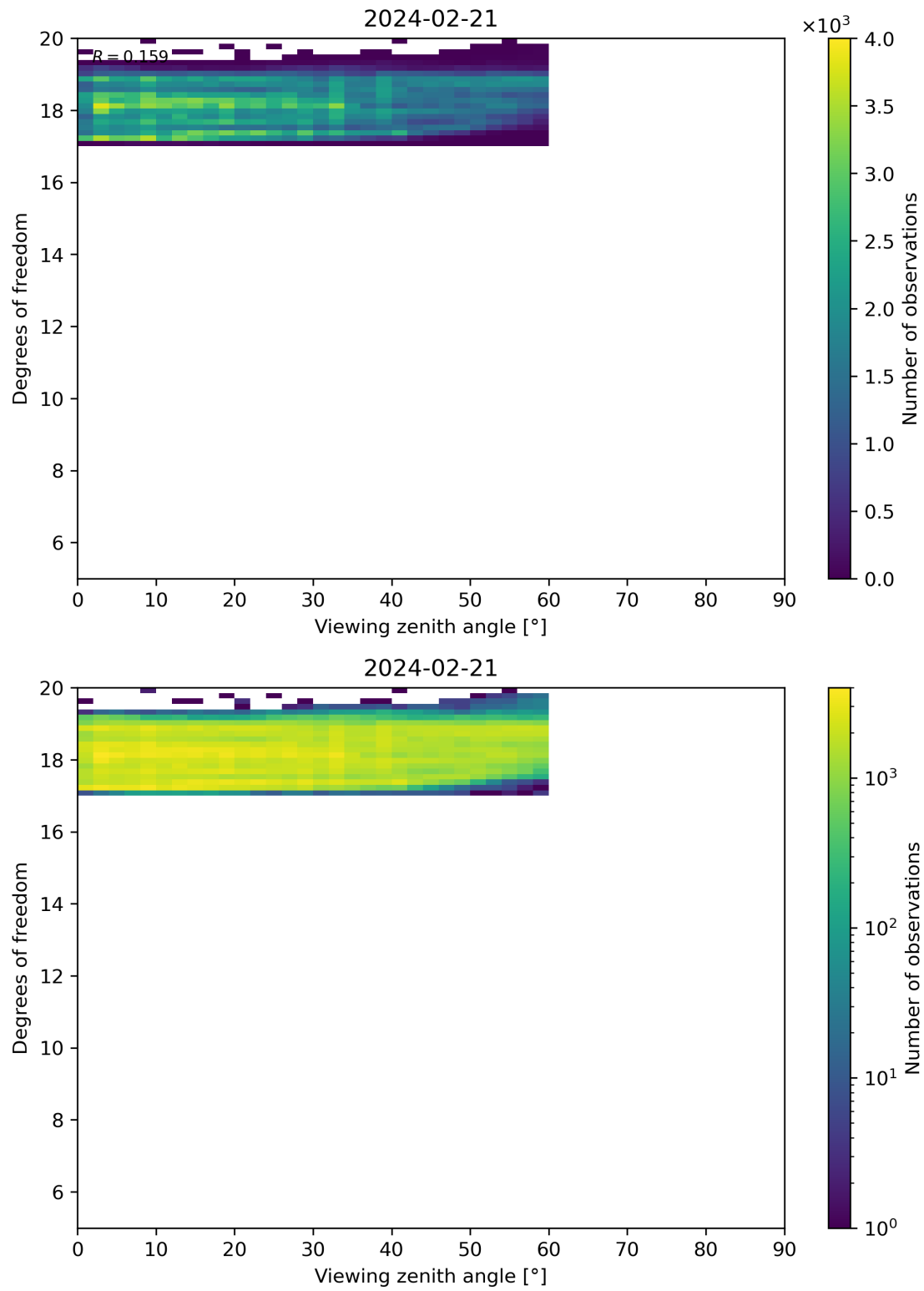
Figure 107: Scatter density plot of “Viewing zenith angle” against “Degrees of freedom” for 2024-02-20 to 2024-02-22.
