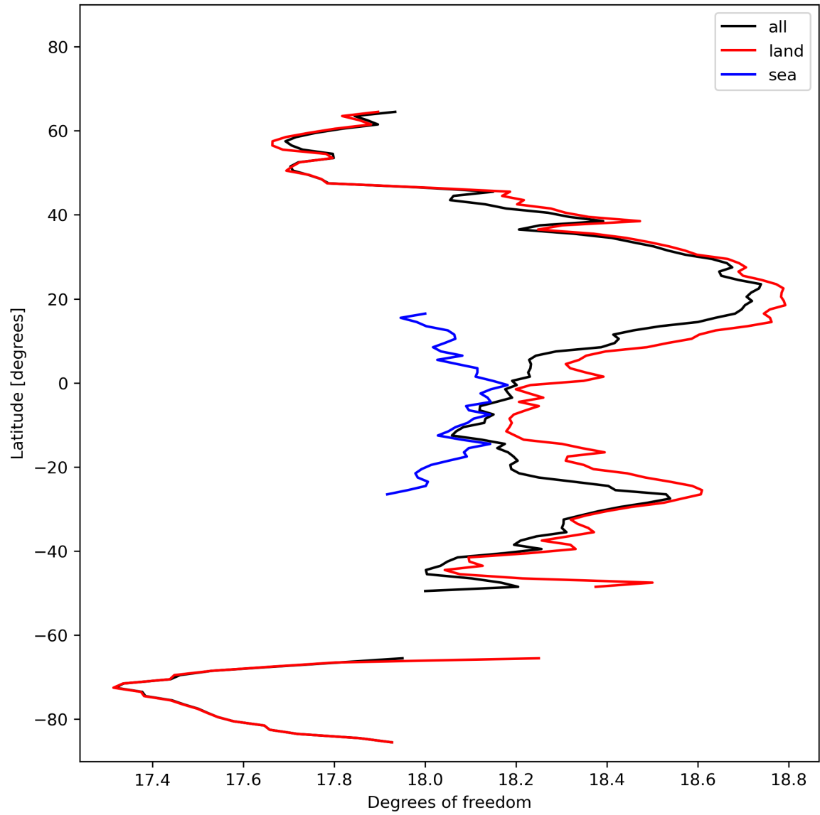
Figure 19: Zonal average of “Degrees of freedom” for 2024-02-20 to 2024-02-22.
