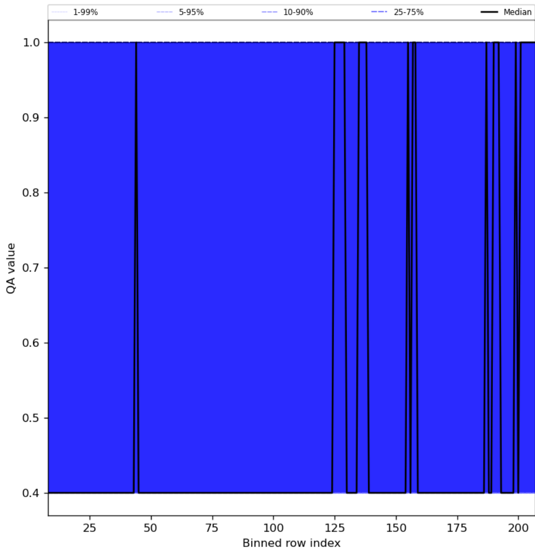
Figure 33: Along track statistics of “QA value” for 2024-02-20 to 2024-02-22
