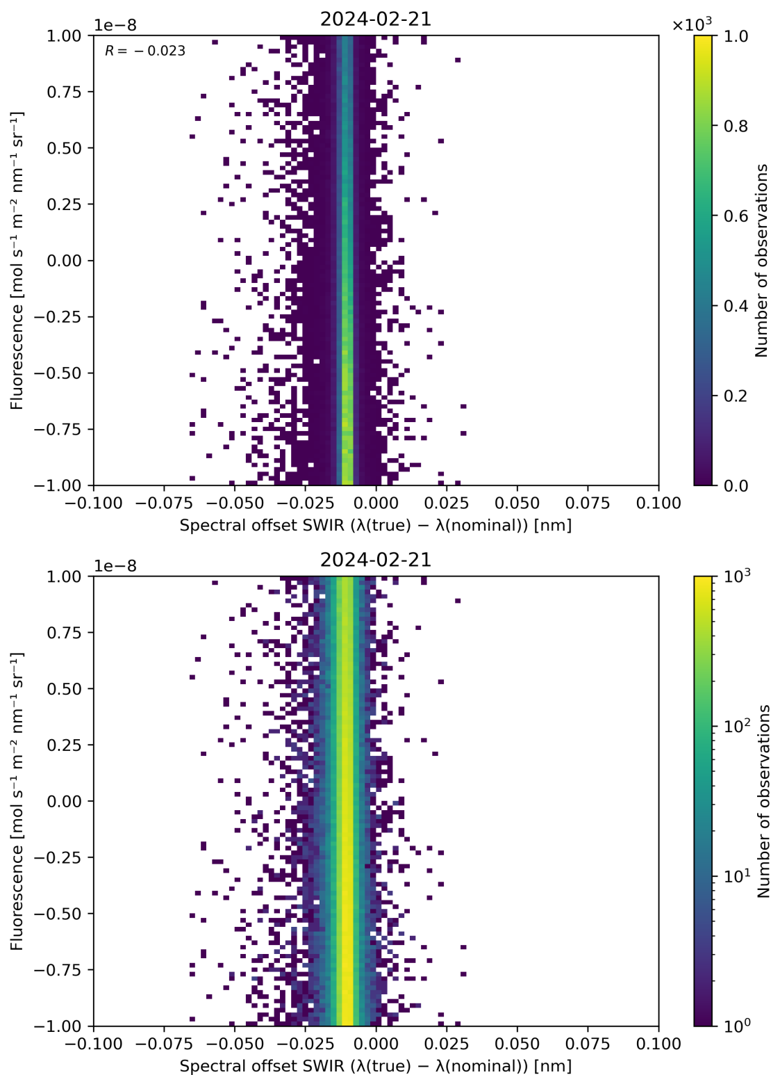
Figure 120: Scatter density plot of “Spectral offset SWIR ( \lambda(\text{true}) - \lambda(\text{nominal}) )” against “Fluorescence” for 2024-02-20 to 2024-02-22.
