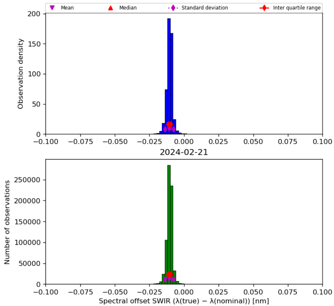
Figure 27: Histogram of “Spectral offset SWIR ( \lambda(\text{true}) - \lambda(\text{nominal}) )” for 2024-02-20 to 2024-02-22
