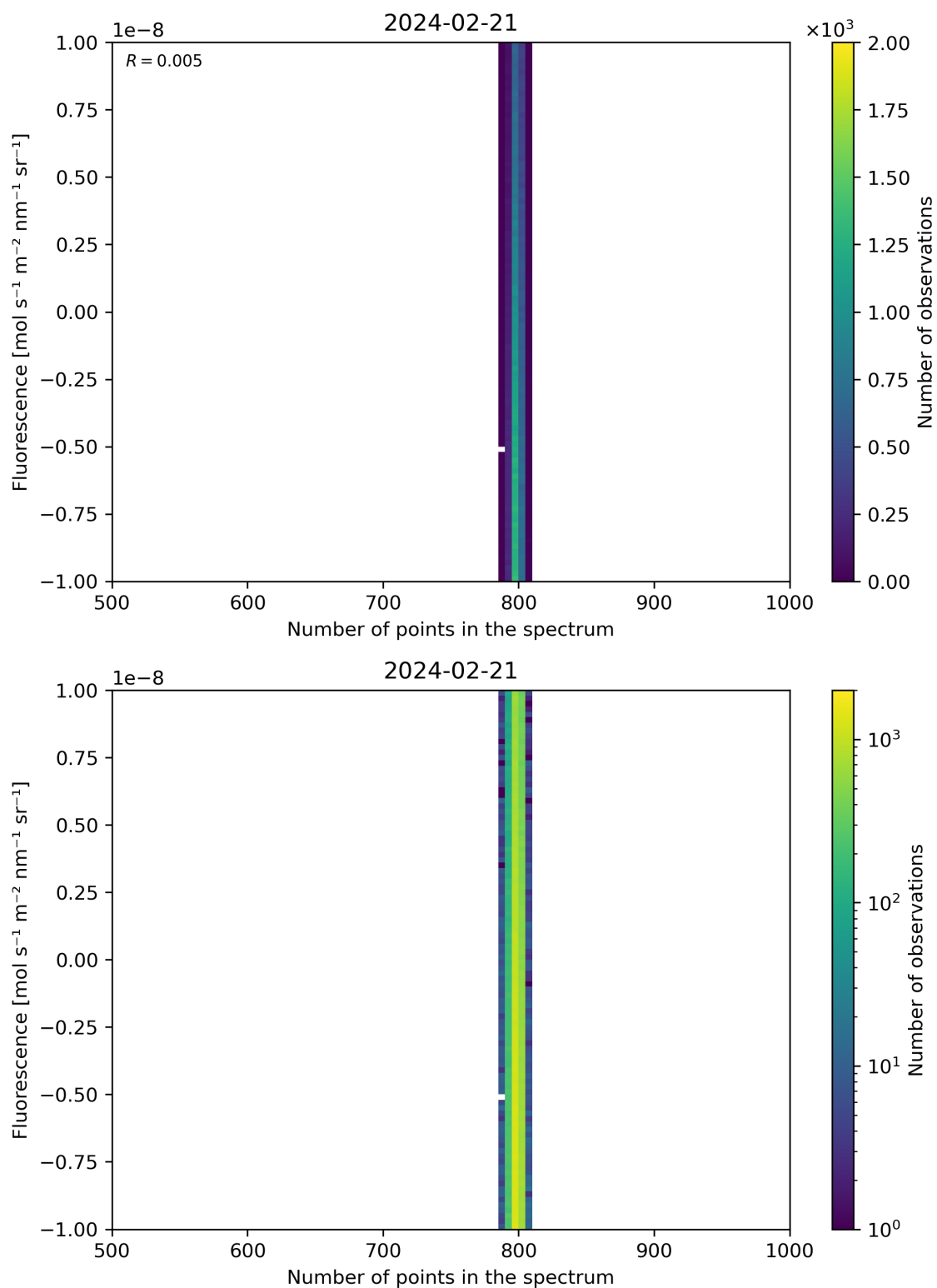
Figure 91: Scatter density plot of “Number of points in the spectrum” against “Fluorescence” for 2024-02-20 to 2024-02-22.
