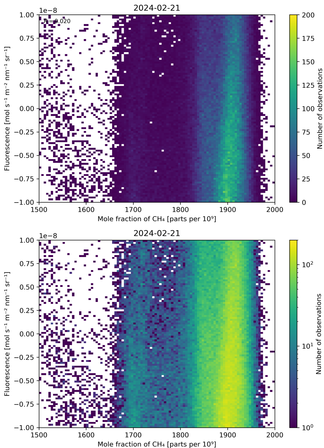
Figure 73: Scatter density plot of “Mole fraction of \text{CH}_4 ” against “Fluorescence” for 2024-02-20 to 2024-02-22.
