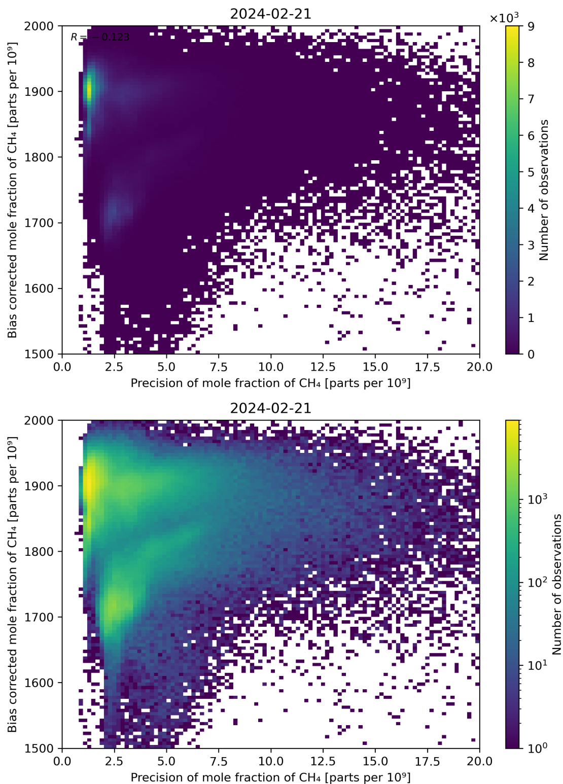
Figure 82: Scatter density plot of “Precision of mole fraction of CH 4 ” against “Bias corrected mole fraction of CH 4 ” for 2024-02-20 to 2024-02-22.
