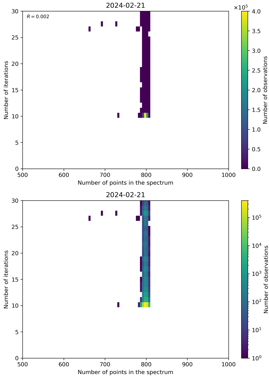
Figure 92: Scatter density plot of “Number of points in the spectrum” against “Number of iterations” for 2024-02-20 to 2024-02-22.
