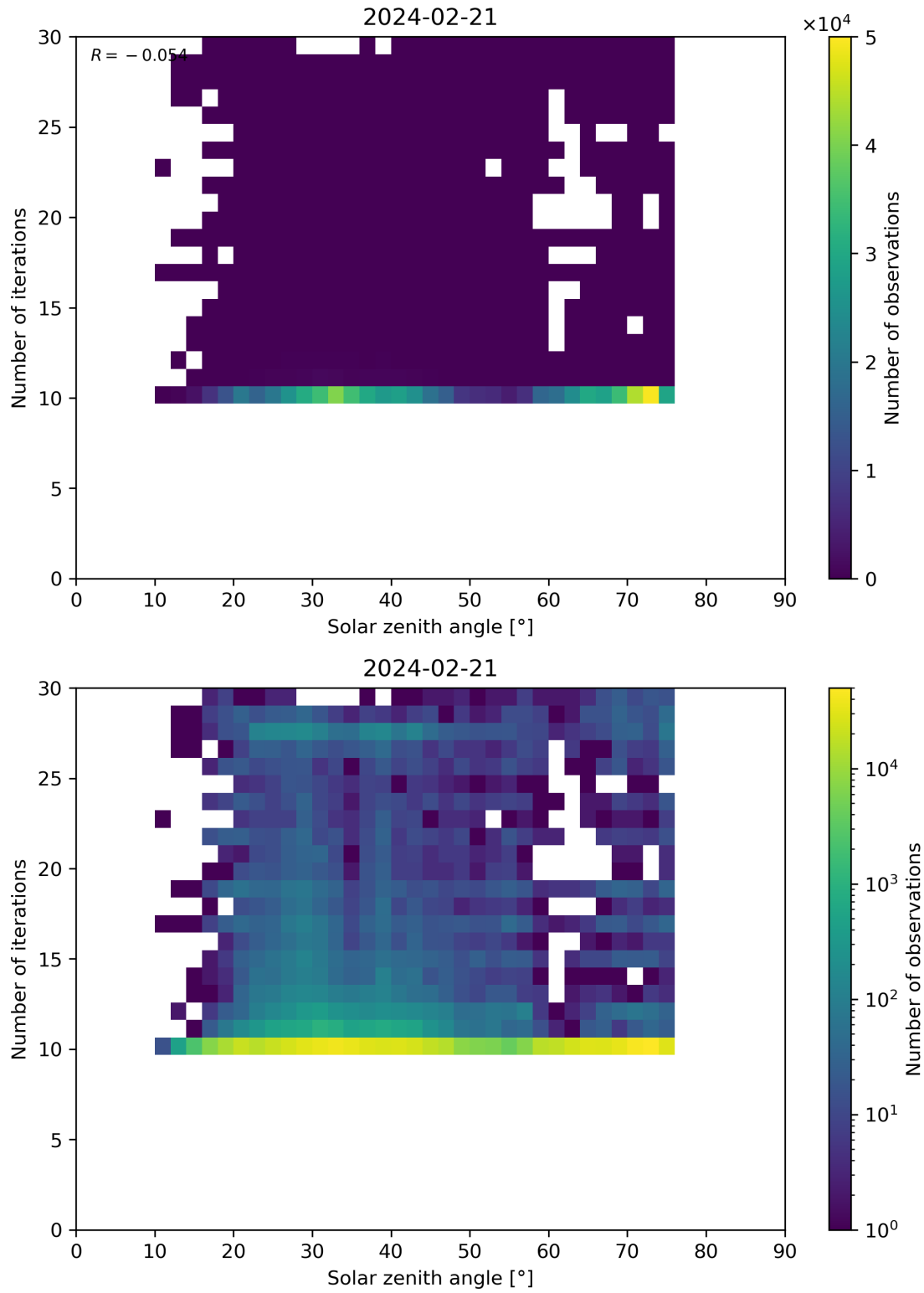
Figure 102: Scatter density plot of “Solar zenith angle” against “Number of iterations” for 2024-02-20 to 2024-02-22.
