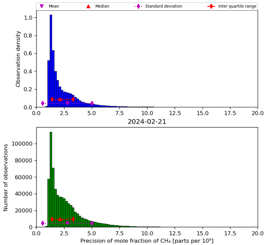
Figure 24: Histogram of “Precision of mole fraction of CH 4 ” for 2024-02-20 to 2024-02-22
