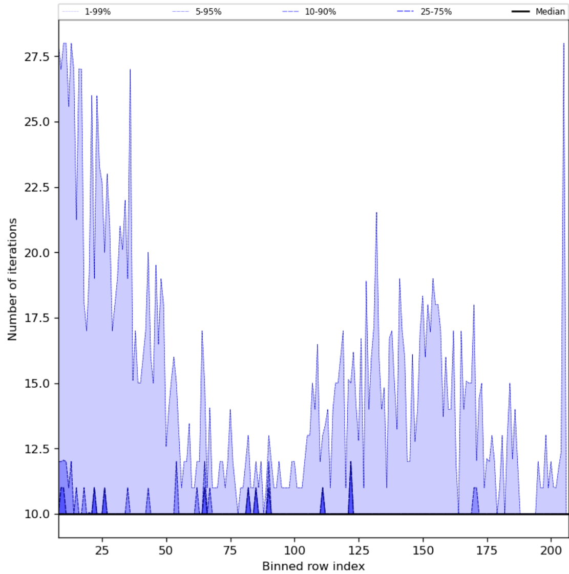
Figure 42: Along track statistics of “Number of iterations” for 2024-02-20 to 2024-02-22
