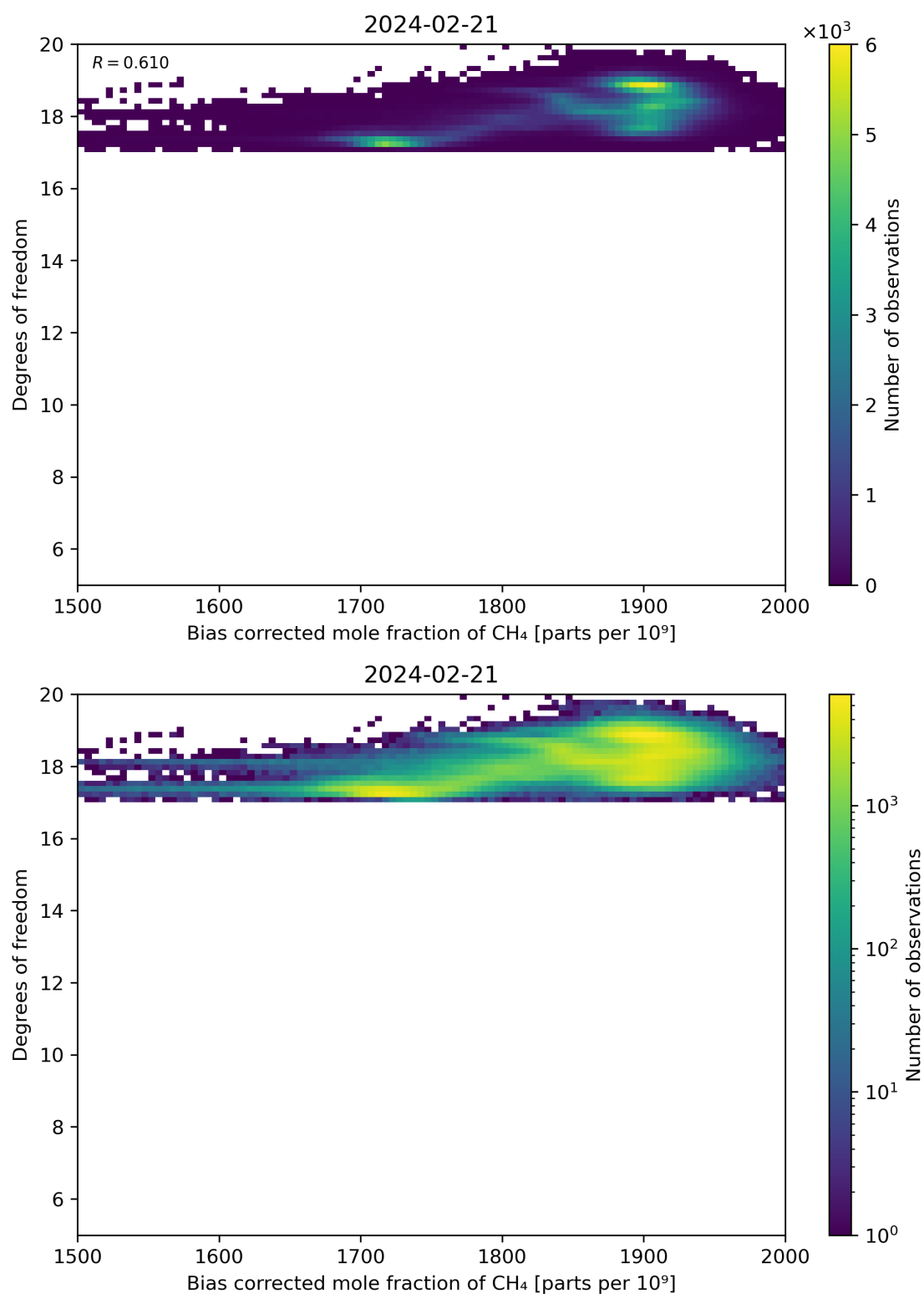
Figure 65: Scatter density plot of “Bias corrected mole fraction of CH 4 ” against “Degrees of freedom” for 2024-02-20 to 2024-02-22.
