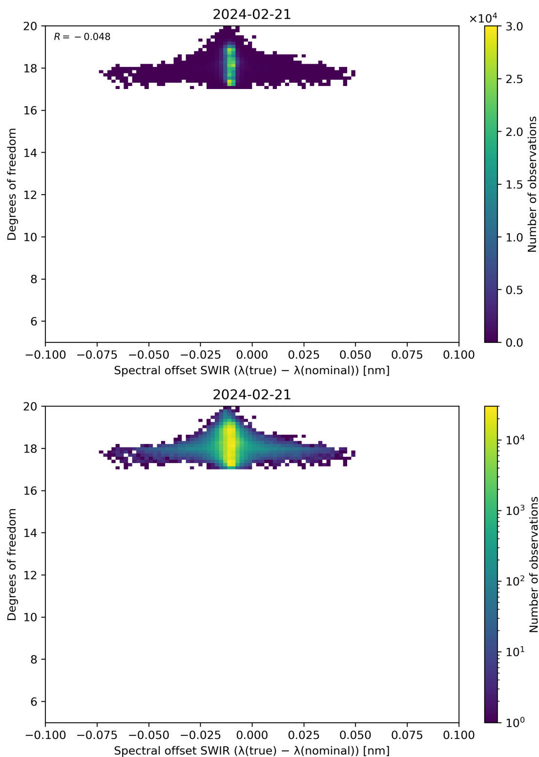
Figure 119: Scatter density plot of “Spectral offset SWIR ( \lambda(\text{true}) - \lambda(\text{nominal}) )” against “Degrees of freedom” for 2024-02-20 to 2024-02-22.
