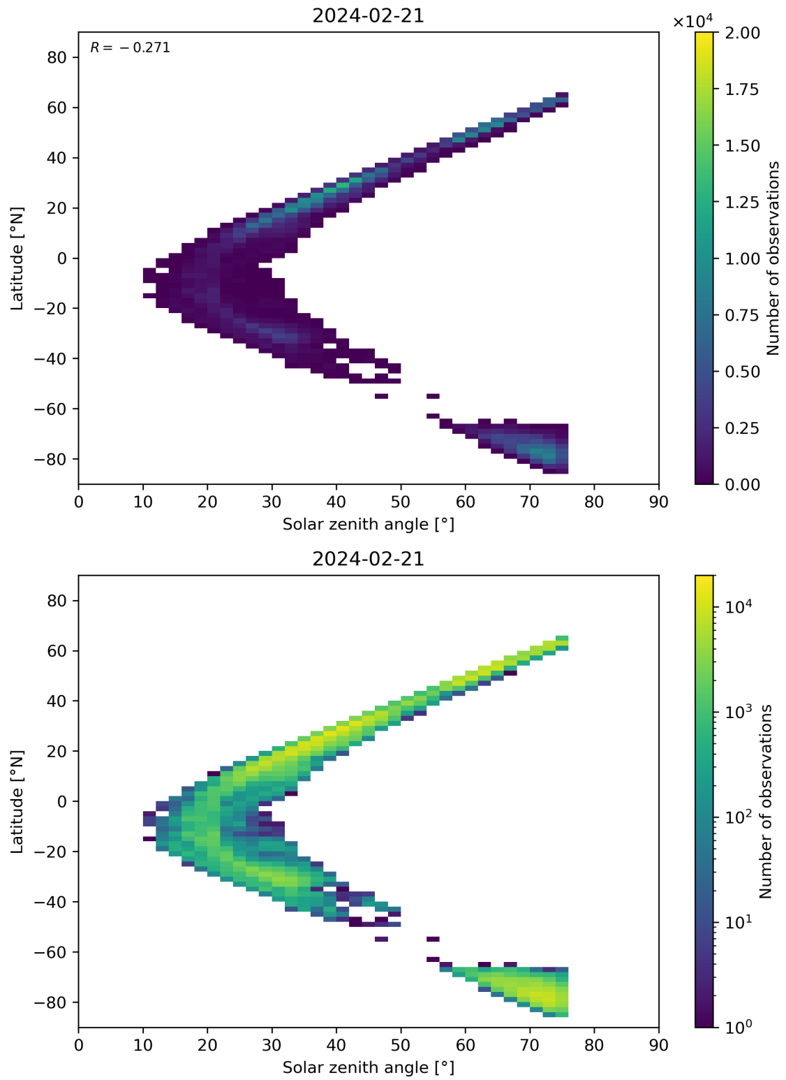
Figure 98: Scatter density plot of “Solar zenith angle” against “Latitude” for 2024-02-20 to 2024-02-22.
