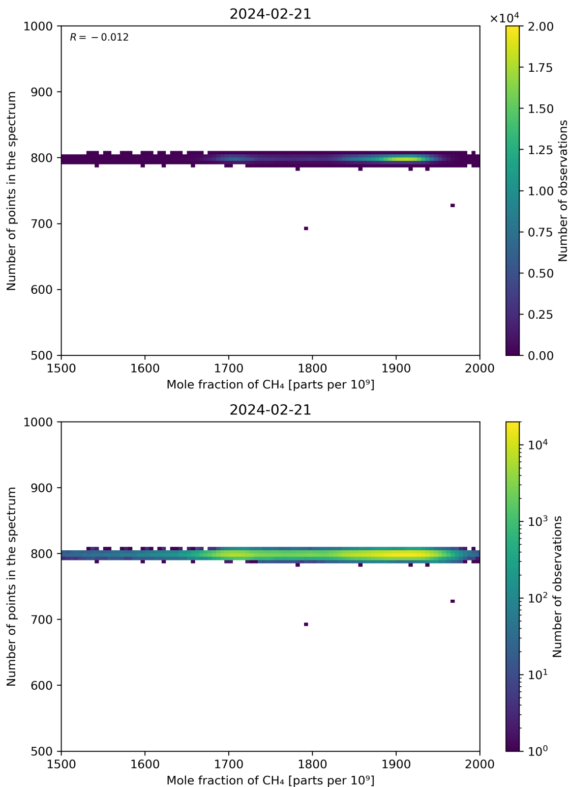
Figure 77: Scatter density plot of “Mole fraction of CH 4 ” against “Number of points in the spectrum” for 2024-02-20 to 2024-02-22.
