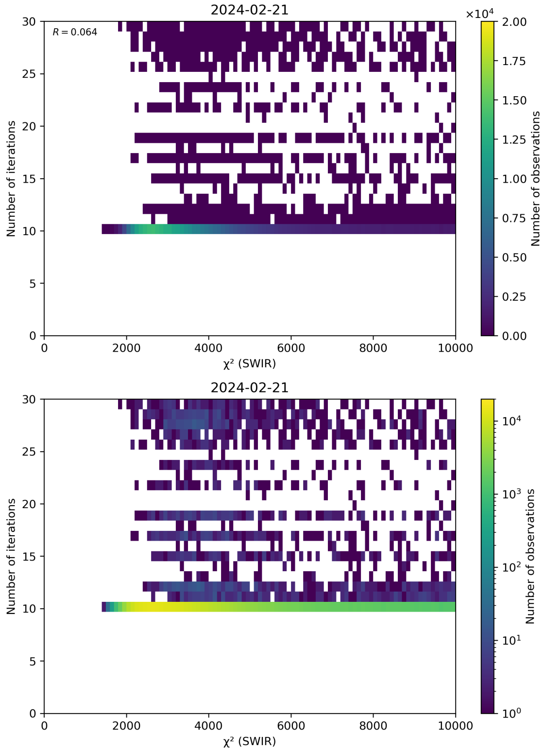
Figure 50: Scatter density plot of “ \chi^2 (SWIR)” against “Number of iterations” for 2024-02-20 to 2024-02-22.
