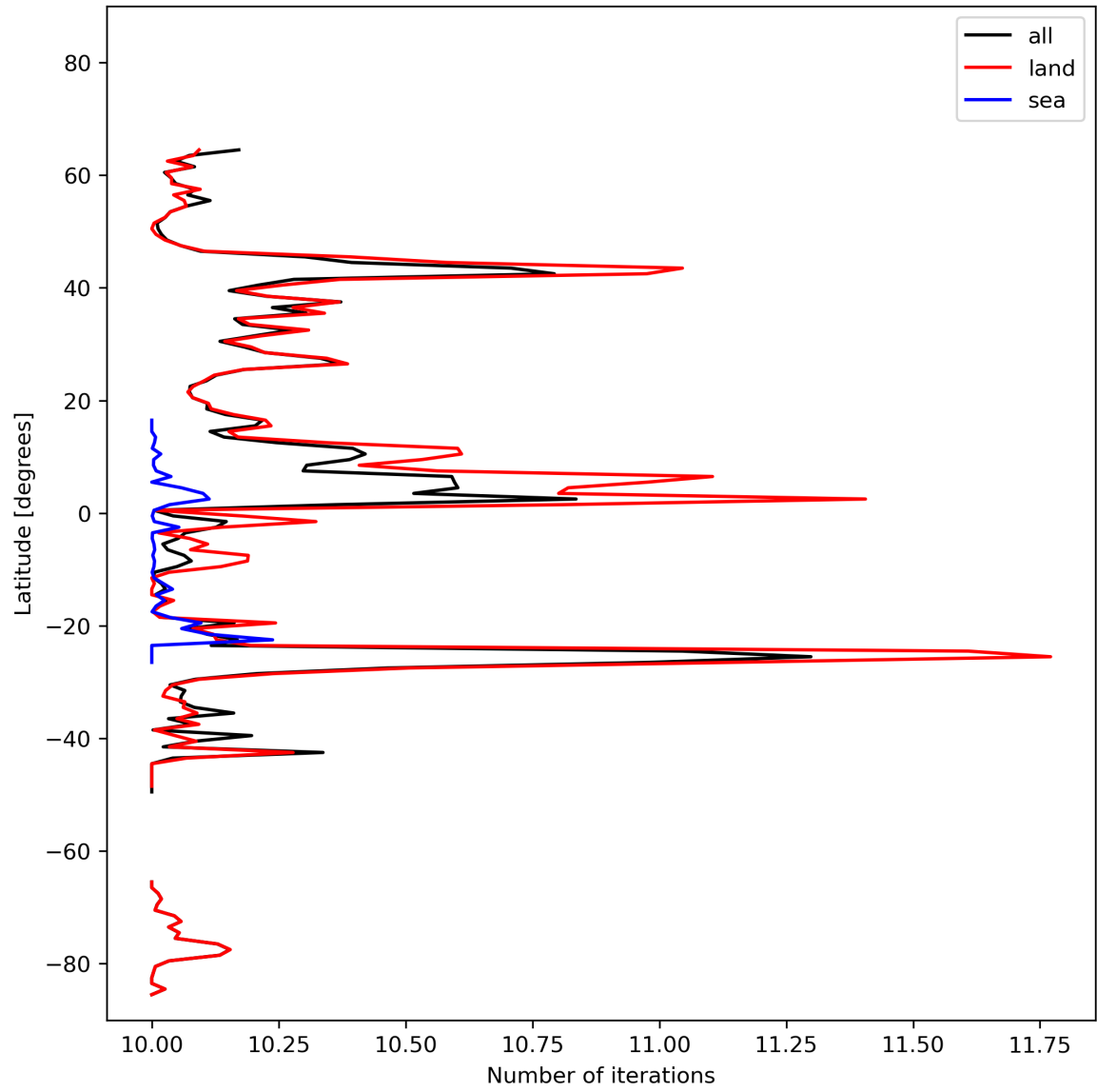
Figure 20: Zonal average of “Number of iterations” for 2024-02-20 to 2024-02-22.
