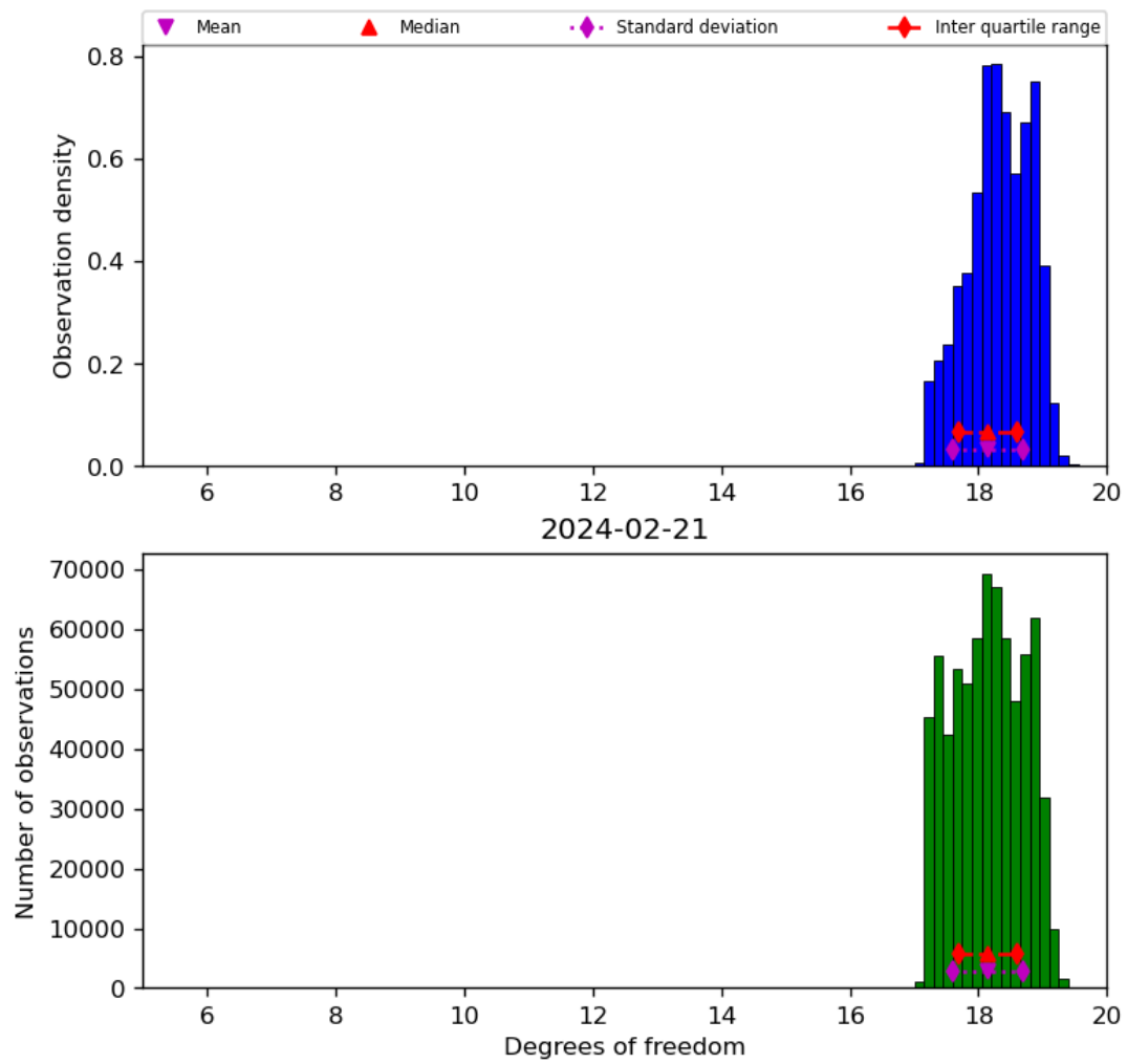
Figure 30: Histogram of “Degrees of freedom” for 2024-02-20 to 2024-02-22
