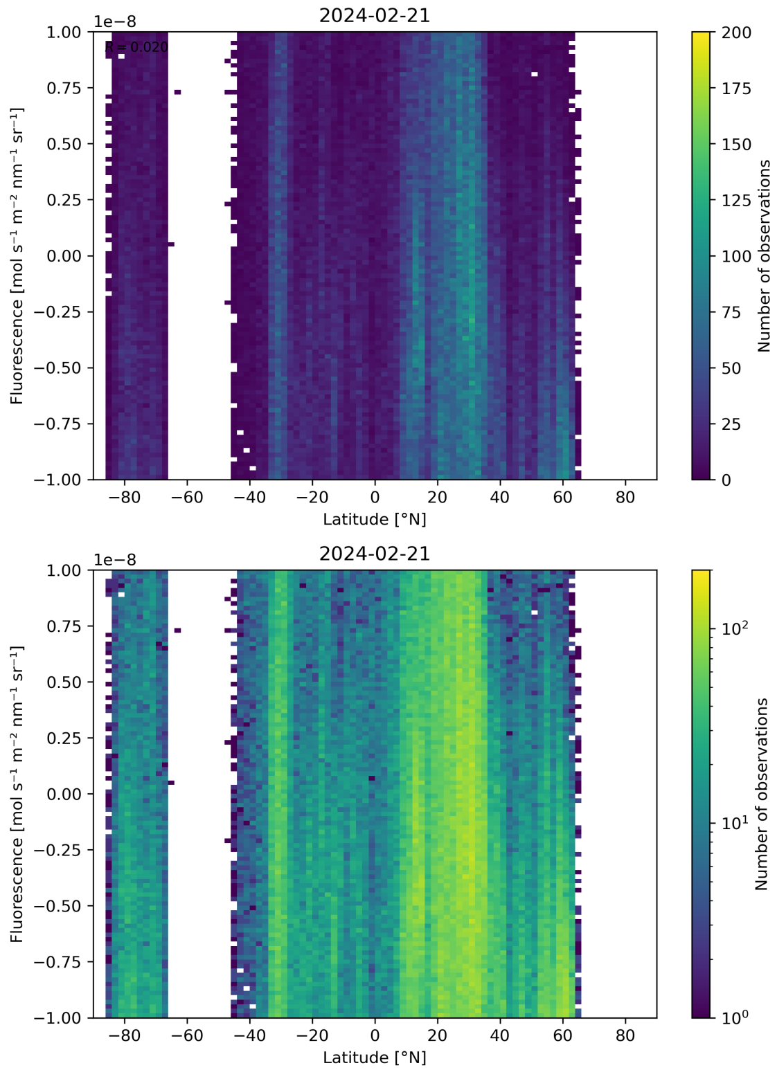
Figure 56: Scatter density plot of “Latitude” against “Fluorescence” for 2024-02-20 to 2024-02-22.
