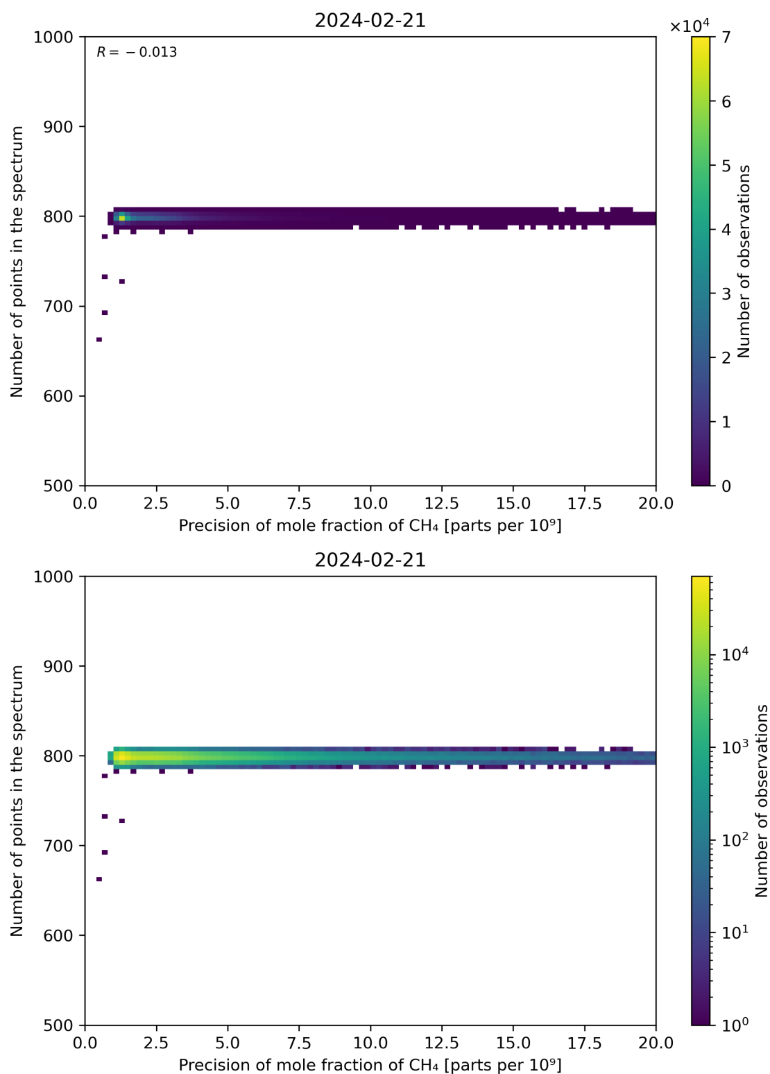
Figure 84: Scatter density plot of “Precision of mole fraction of CH 4 ” against “Number of points in the spectrum” for 2024-02-20 to 2024-02-22.
