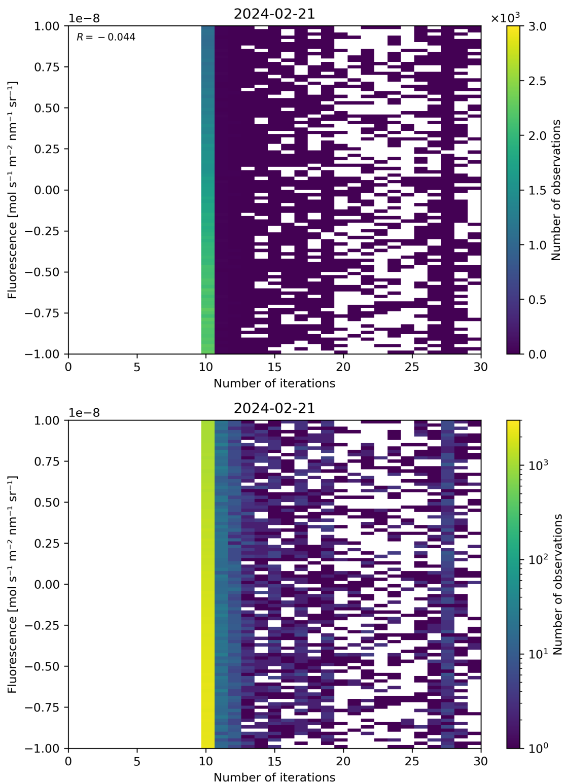
Figure 87: Scatter density plot of “Number of iterations” against “Fluorescence” for 2024-02-20 to 2024-02-22.
