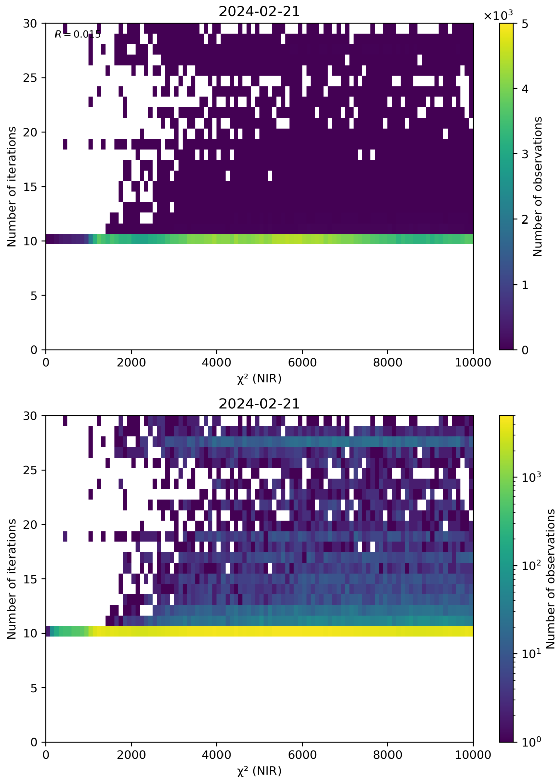
Figure 46: Scatter density plot of “ \chi^2 (NIR)” against “Number of iterations” for 2024-02-20 to 2024-02-22.
