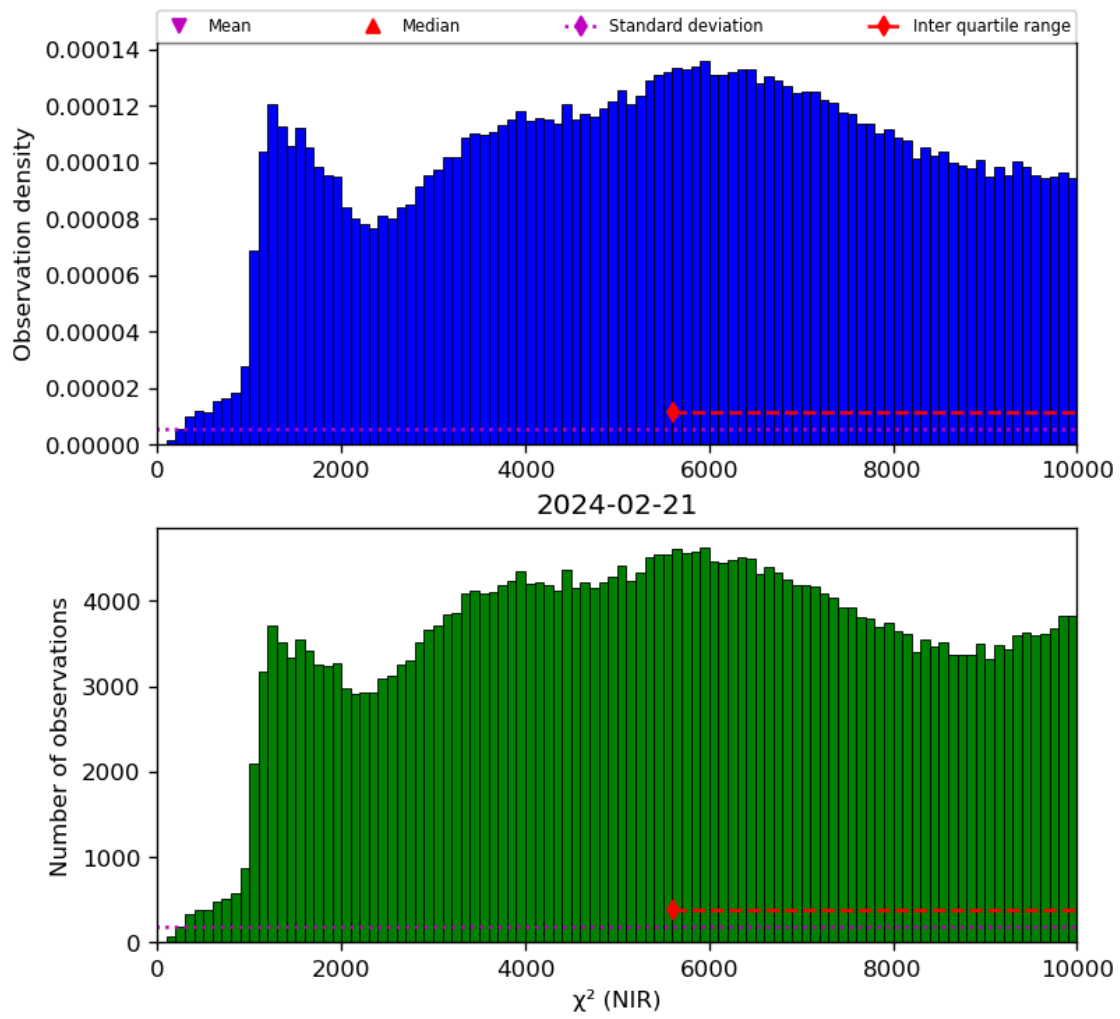
Figure 29: Histogram of " \chi^2 (NIR)" for 2024-02-20 to 2024-02-22
