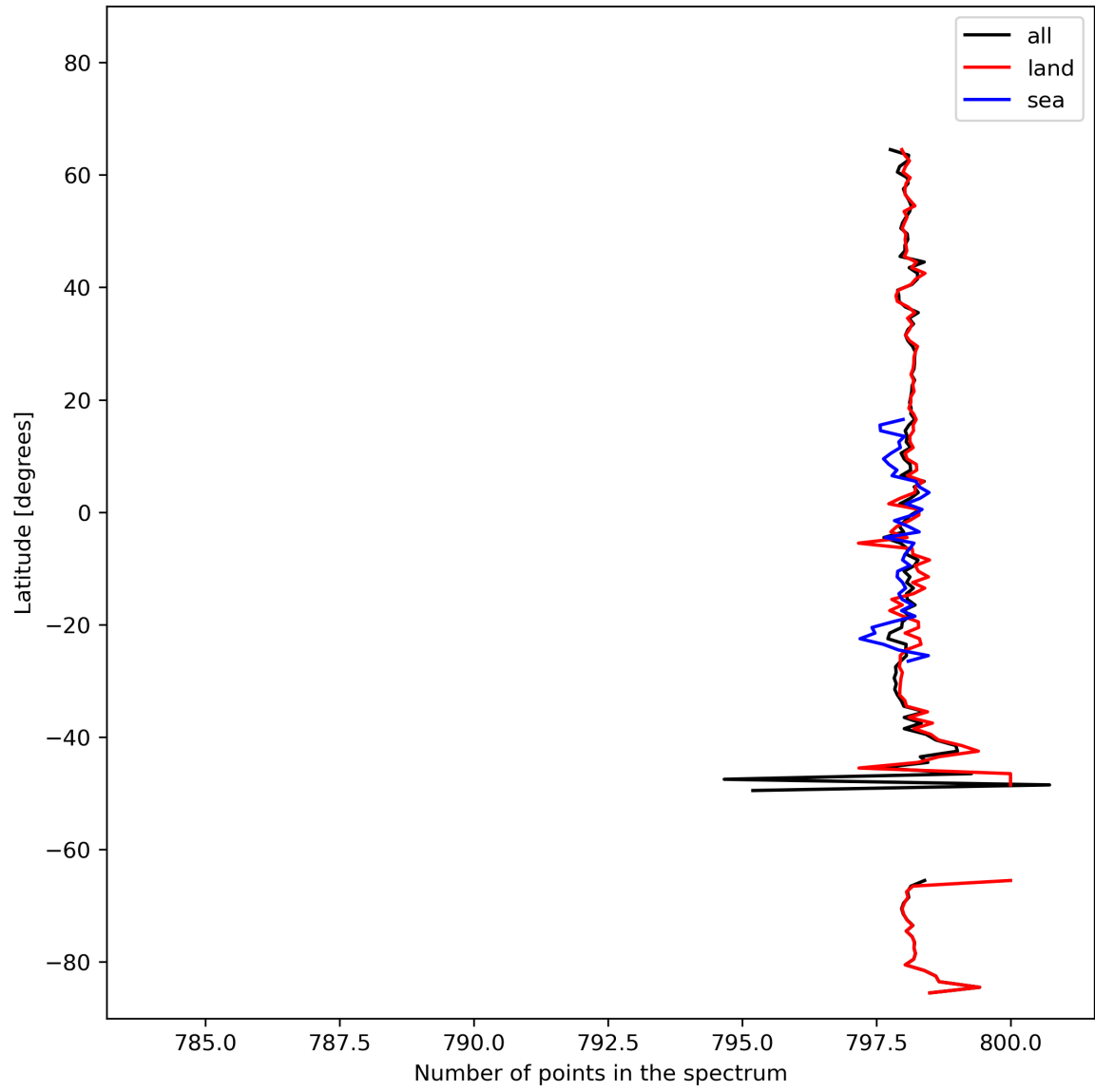
Figure 15: Zonal average of “Number of points in the spectrum” for 2024-02-20 to 2024-02-22.
