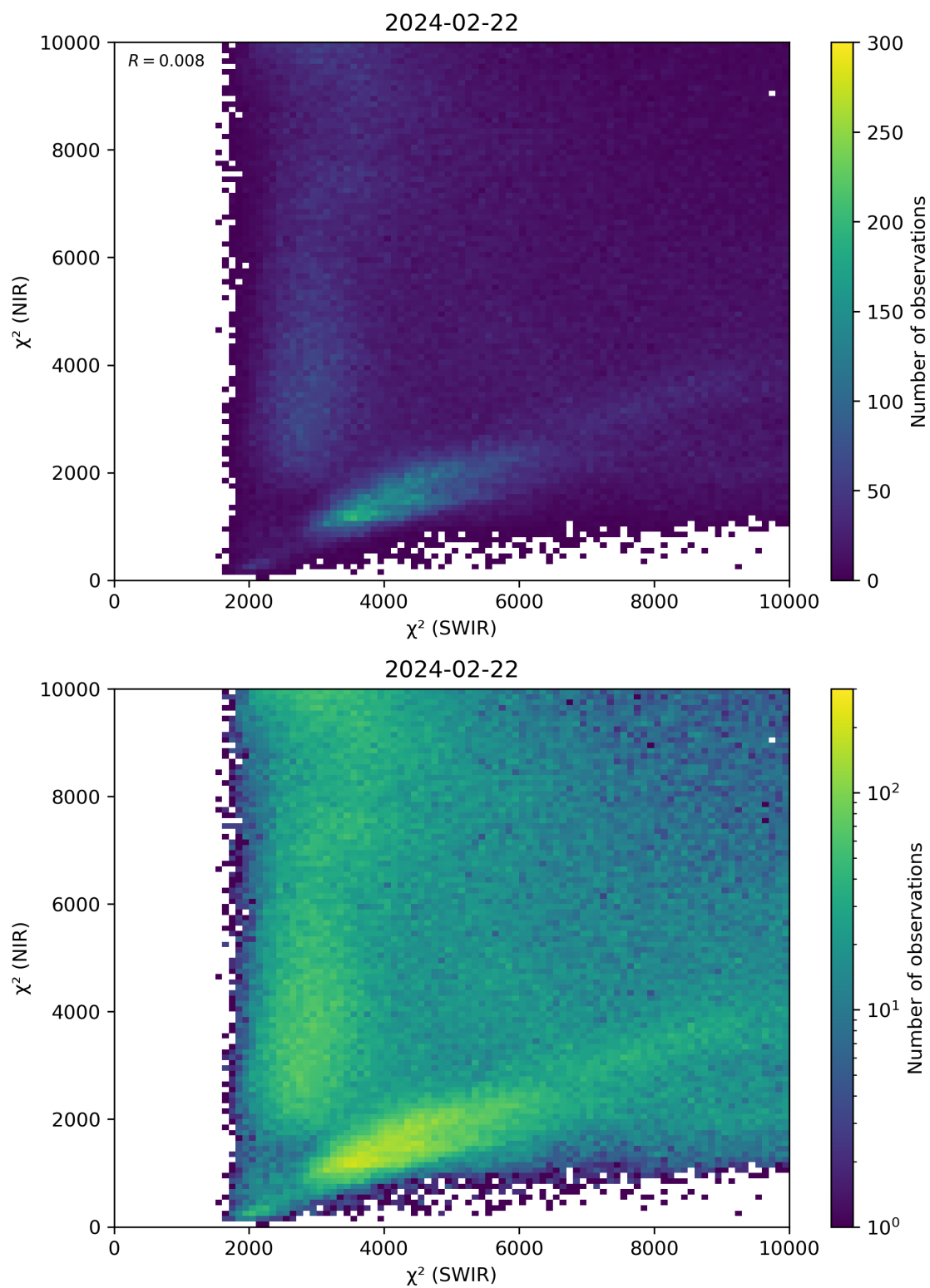
Figure 47: Scatter density plot of “ \chi^2 (SWIR)” against “ \chi^2 (NIR)” for 2024-02-22 to 2024-02-23.
