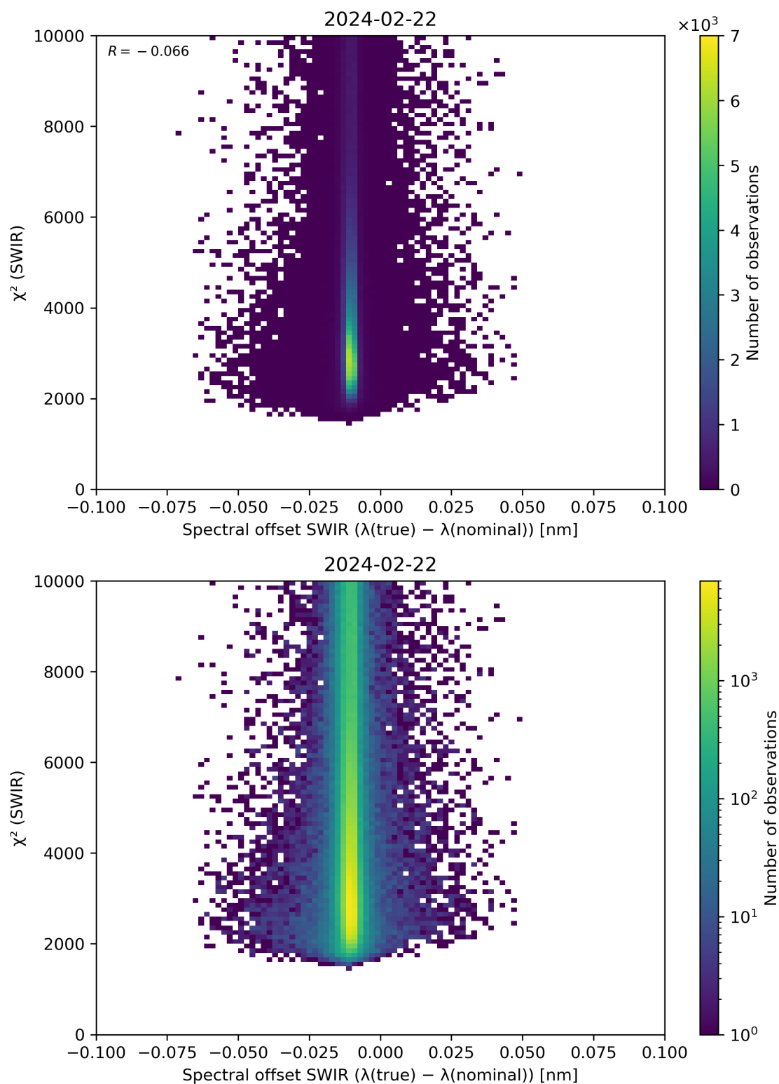
Figure 118: Scatter density plot of “Spectral offset SWIR ( \lambda(\text{true}) - \lambda(\text{nominal}) )” against “ \chi^2 (SWIR)” for 2024-02-22 to 2024-02-23.
