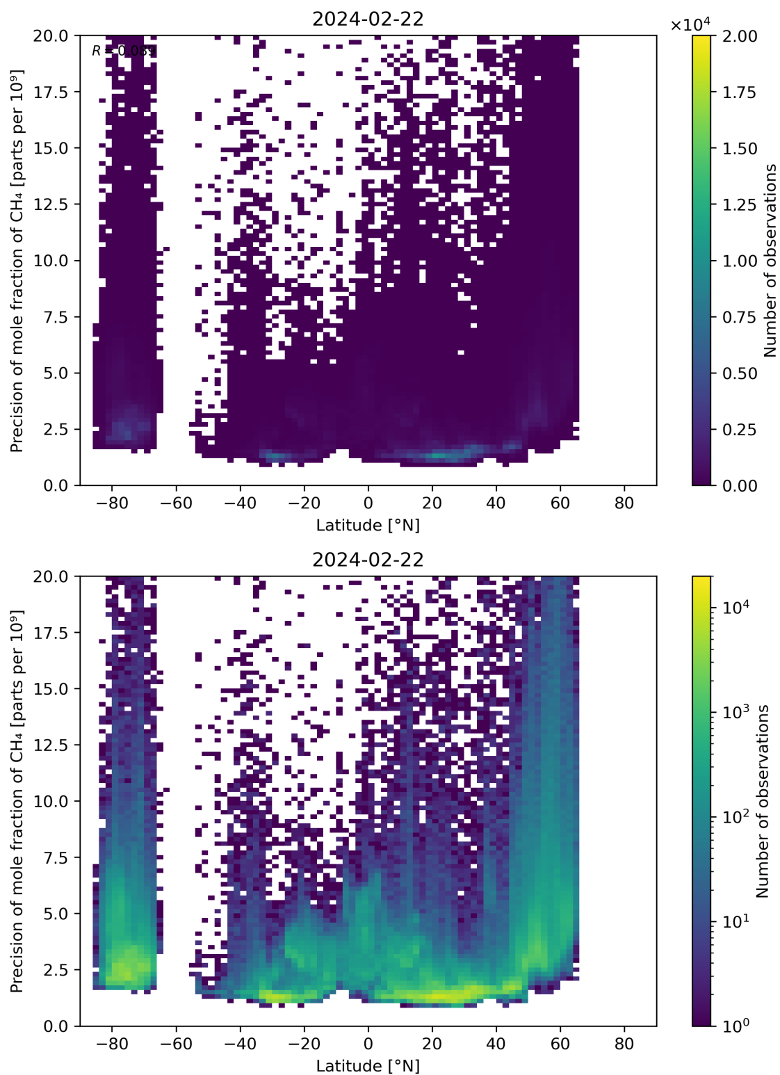
Figure 59: Scatter density plot of “Latitude” against “Precision of mole fraction of CH 4 ” for 2024-02-22 to 2024-02-23.
