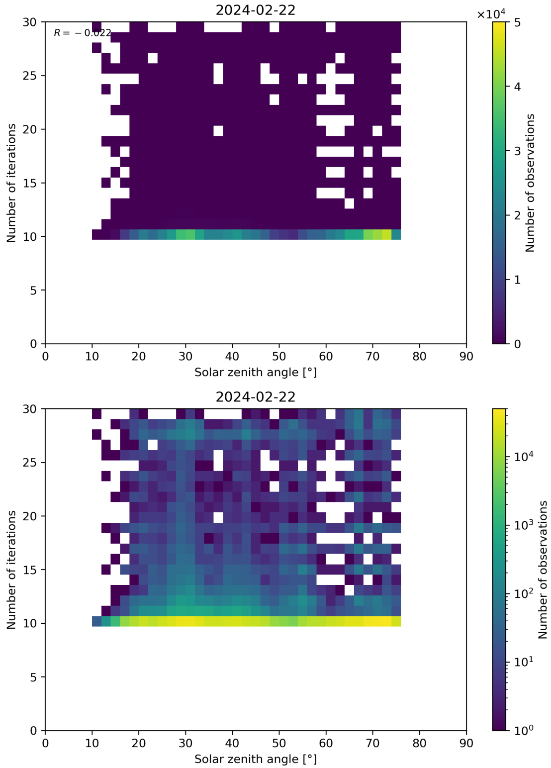
Figure 102: Scatter density plot of “Solar zenith angle” against “Number of iterations” for 2024-02-22 to 2024-02-23.
