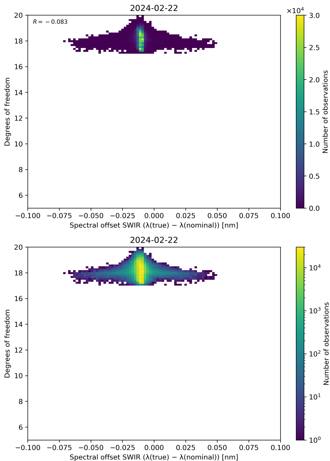
Figure 119: Scatter density plot of “Spectral offset SWIR ( \lambda(\text{true}) - \lambda(\text{nominal}) )” against “Degrees of freedom” for 2024-02-22 to 2024-02-23.
