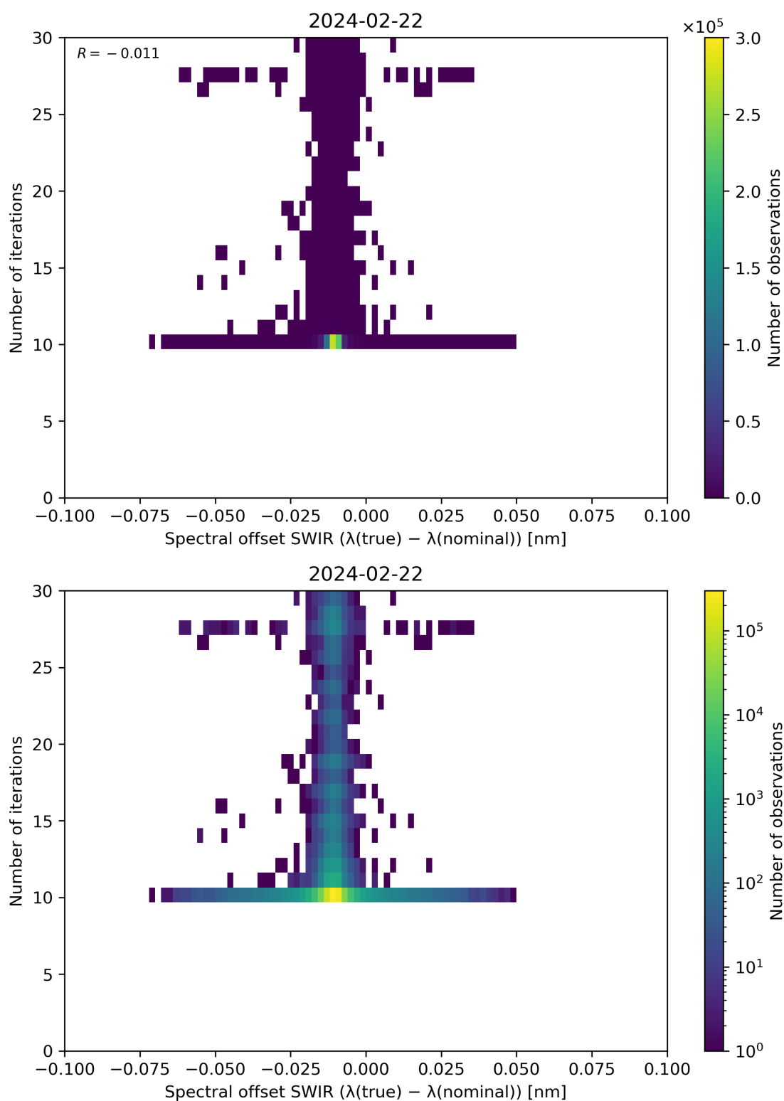
Figure 121: Scatter density plot of “Spectral offset SWIR ( \lambda(\text{true}) - \lambda(\text{nominal}) )” against “Number of iterations” for 2024-02-22 to 2024-02-23.
