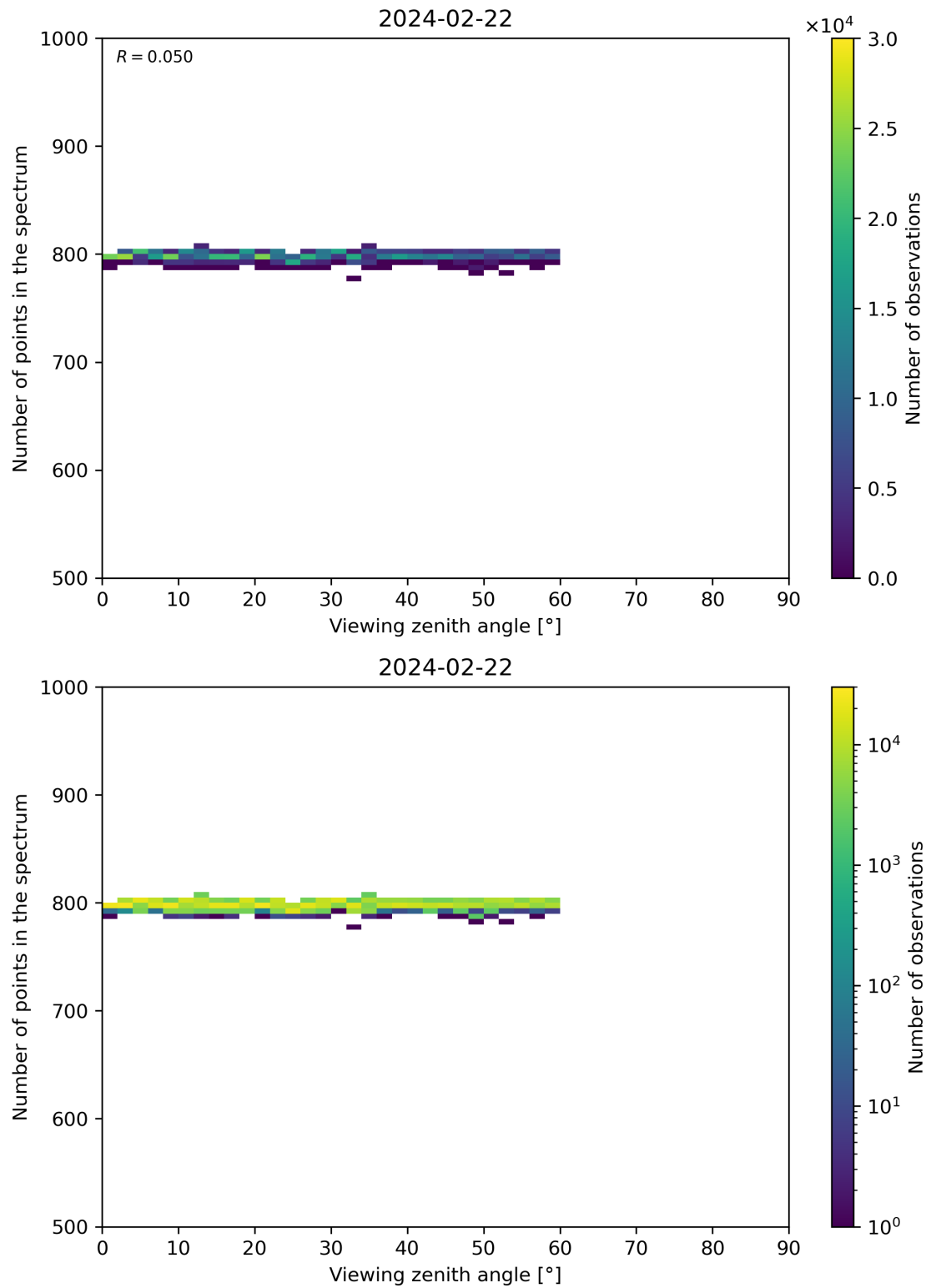
Figure 114: Scatter density plot of “Viewing zenith angle” against “Number of points in the spectrum” for 2024-02-22 to 2024-02-23.
