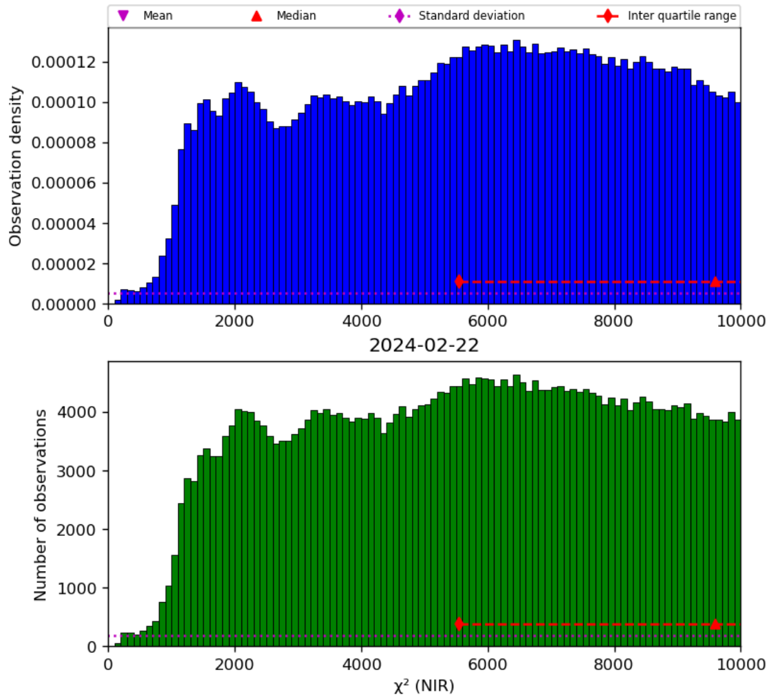
Figure 29: Histogram of " \chi^2 (NIR)" for 2024-02-22 to 2024-02-23
