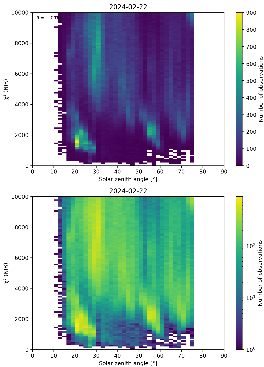
Figure 94: Scatter density plot of “Solar zenith angle” against “ \chi^2 (NIR)” for 2024-02-22 to 2024-02-23.
