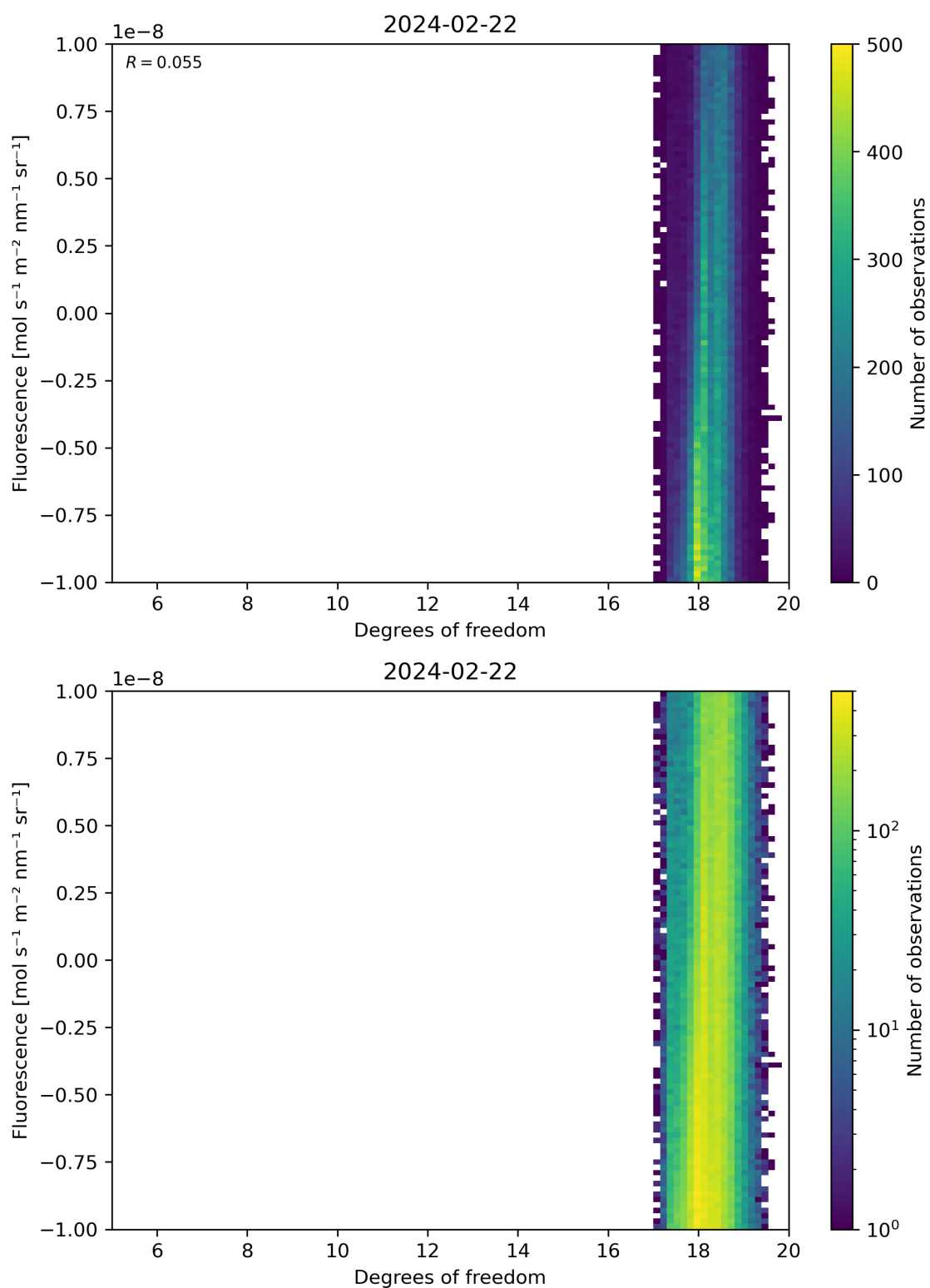
Figure 51: Scatter density plot of “Degrees of freedom” against “Fluorescence” for 2024-02-22 to 2024-02-23.
