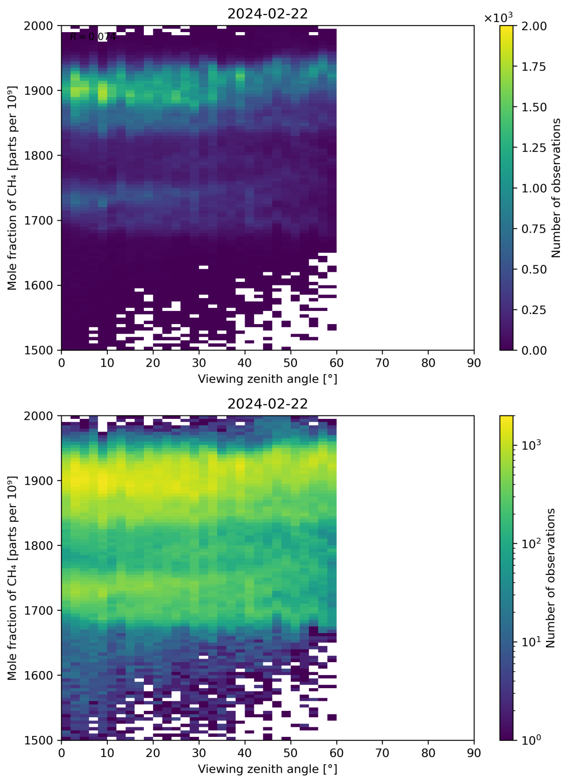
Figure 110: Scatter density plot of “Viewing zenith angle” against “Mole fraction of CH 4 ” for 2024-02-22 to 2024-02-23.
