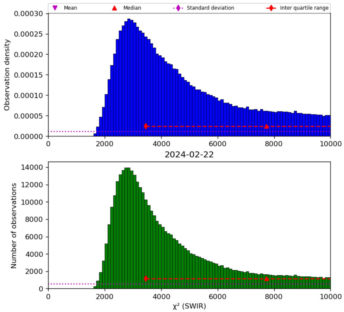
Figure 28: Histogram of “ \chi^2 (SWIR)” for 2024-02-22 to 2024-02-23
