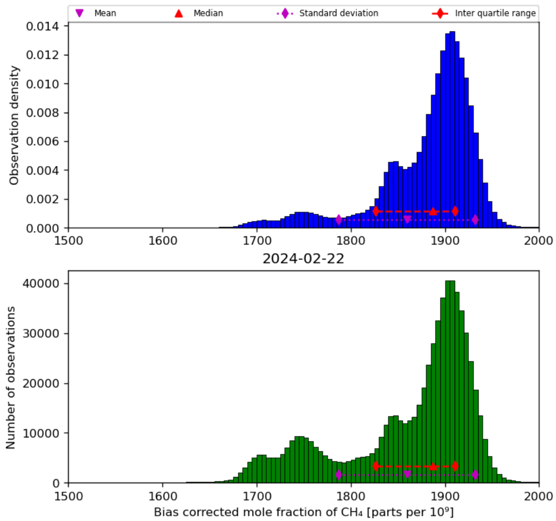
Figure 25: Histogram of “Bias corrected mole fraction of CH 4 ” for 2024-02-22 to 2024-02-23
