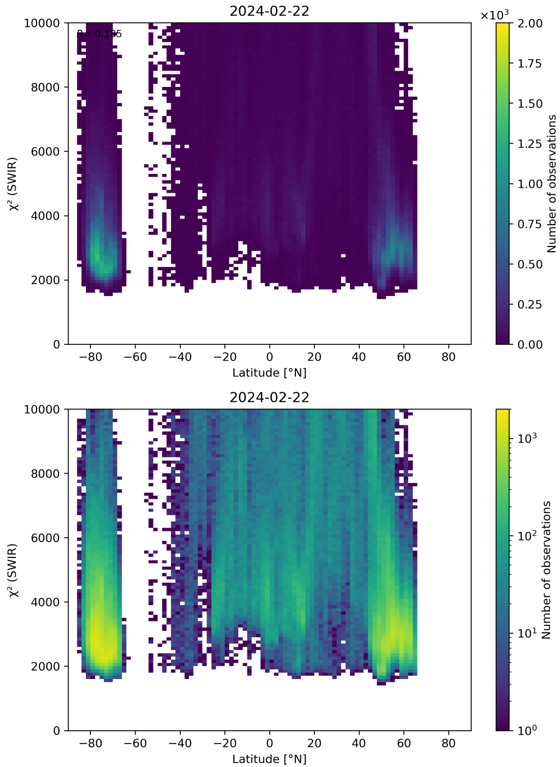
Figure 54: Scatter density plot of “Latitude” against “ \chi^2 (SWIR)” for 2024-02-22 to 2024-02-23.
