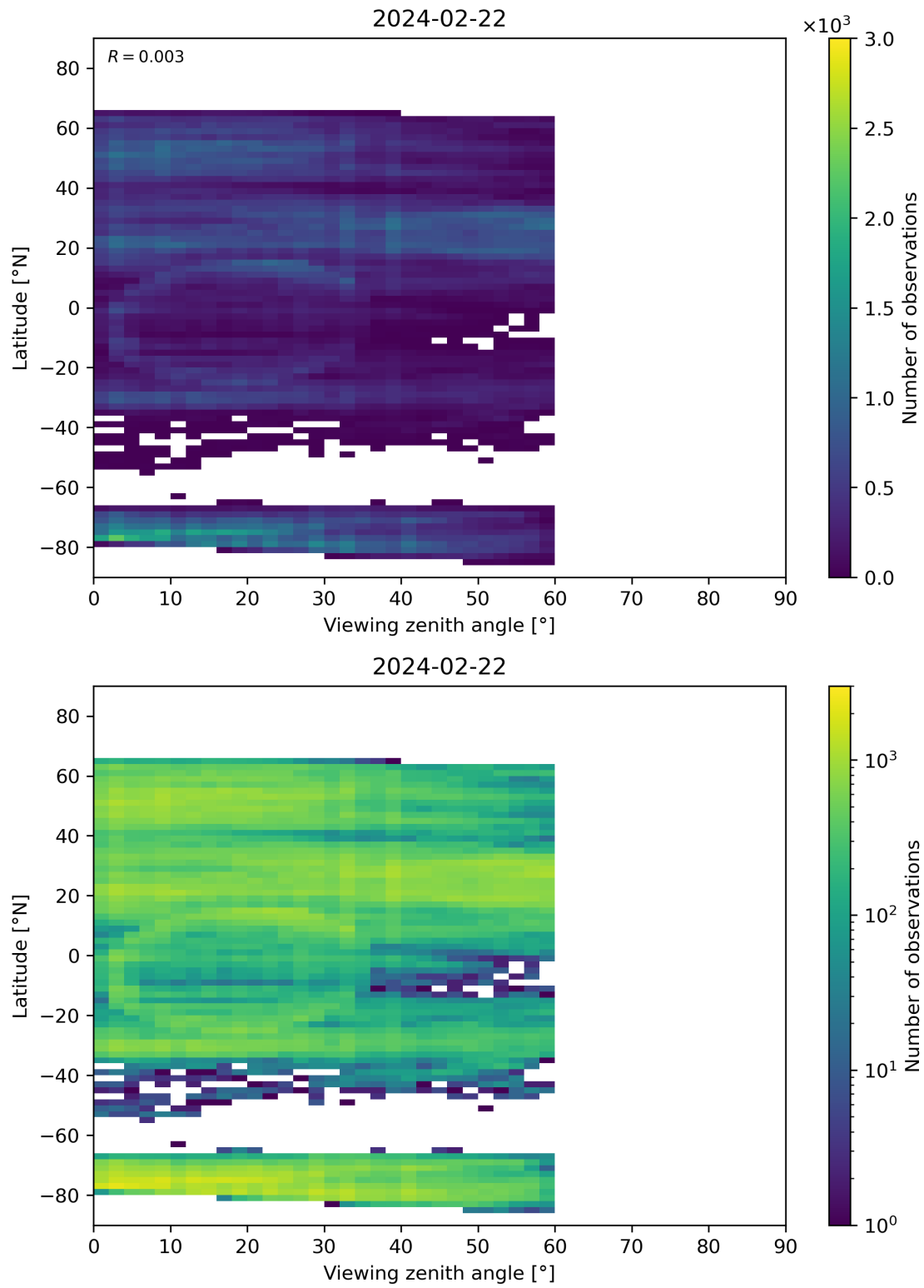
Figure 109: Scatter density plot of “Viewing zenith angle” against “Latitude” for 2024-02-22 to 2024-02-23.
