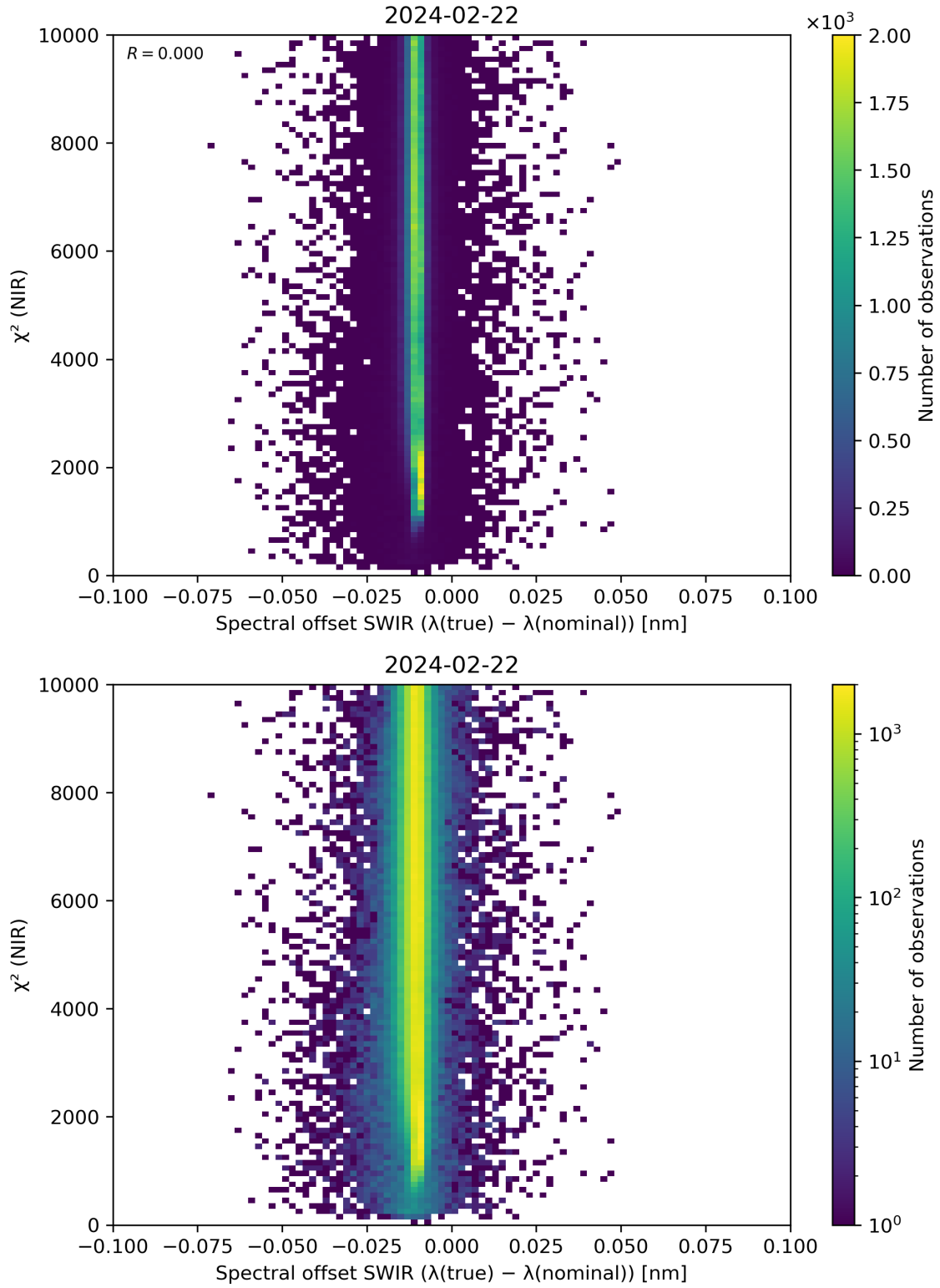
Figure 117: Scatter density plot of “Spectral offset SWIR ( \lambda(\text{true}) - \lambda(\text{nominal}) )” against “ \chi^2 (NIR)” for 2024-02-22 to 2024-02-23.
