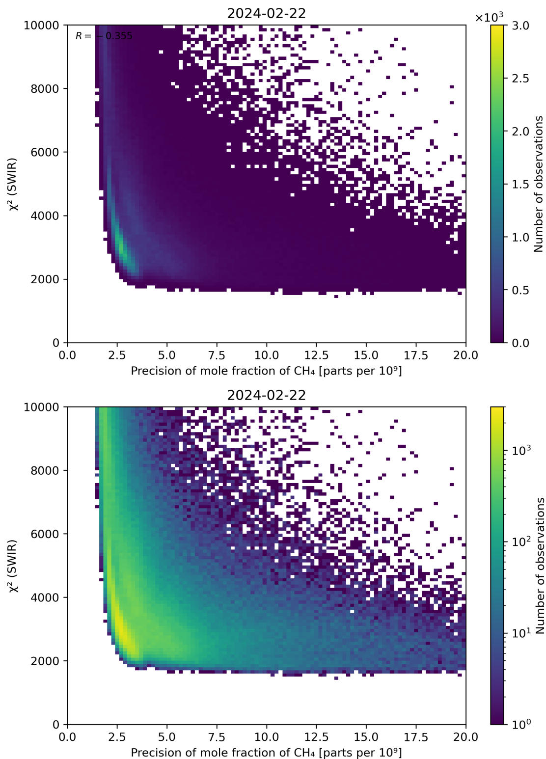
Figure 79: Scatter density plot of “Precision of mole fraction of CH 4 ” against “ \chi^2 (SWIR)” for 2024-02-22 to 2024-02-23.
