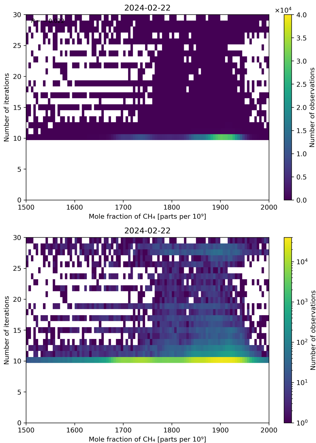
Figure 76: Scatter density plot of “Mole fraction of CH 4 ” against “Number of iterations” for 2024-02-22 to 2024-02-23.
