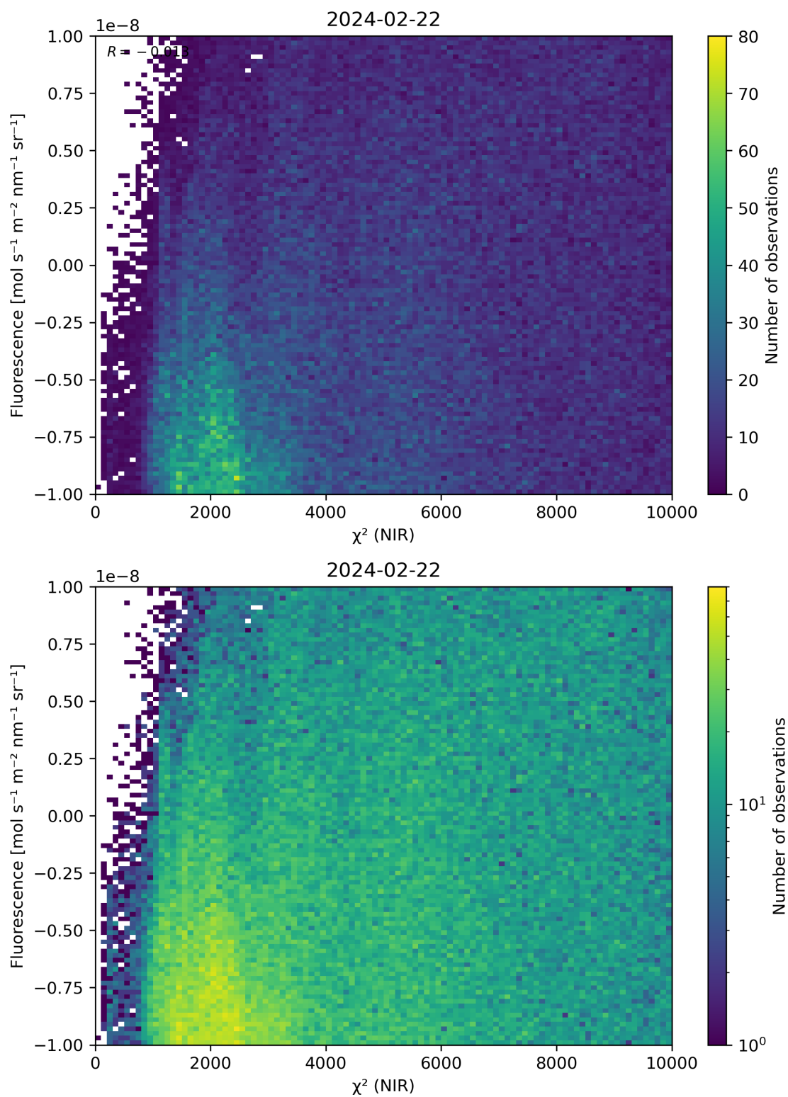
Figure 45: Scatter density plot of “ \chi^2 (NIR)” against “Fluorescence” for 2024-02-22 to 2024-02-23.
