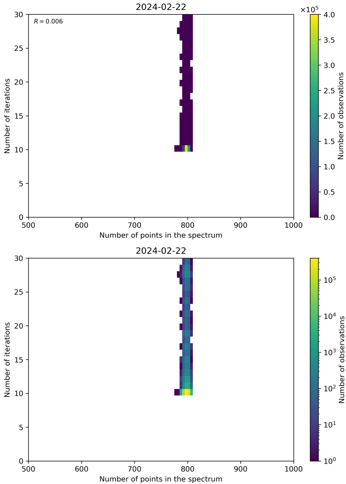
Figure 92: Scatter density plot of “Number of points in the spectrum” against “Number of iterations” for 2024-02-22 to 2024-02-23.
