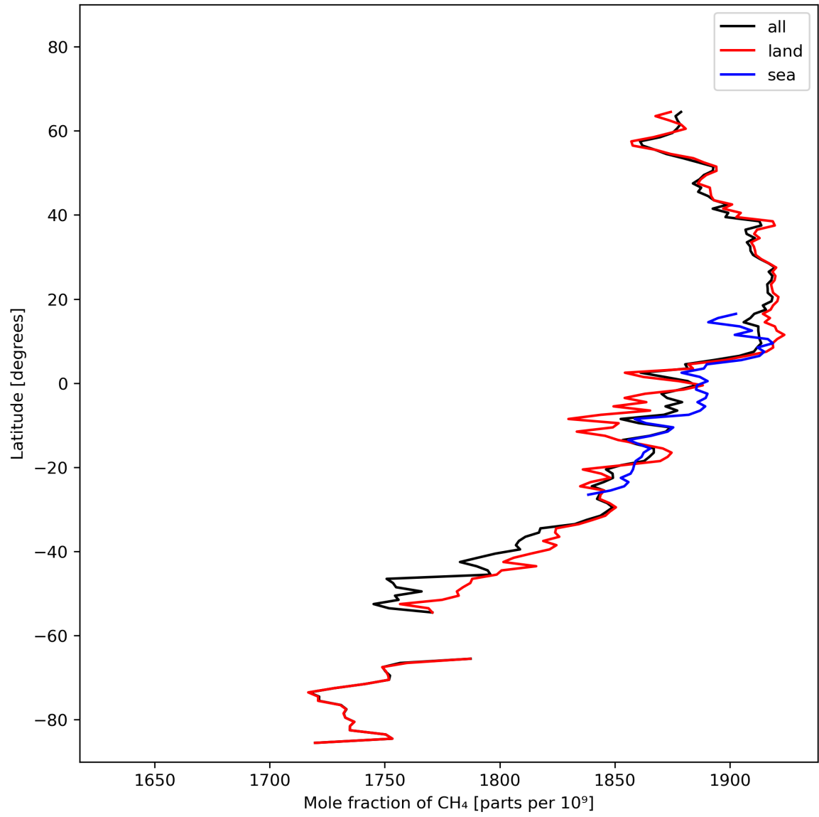
Figure 12: Zonal average of “Mole fraction of \text{CH}_4 ” for 2024-02-22 to 2024-02-23.
