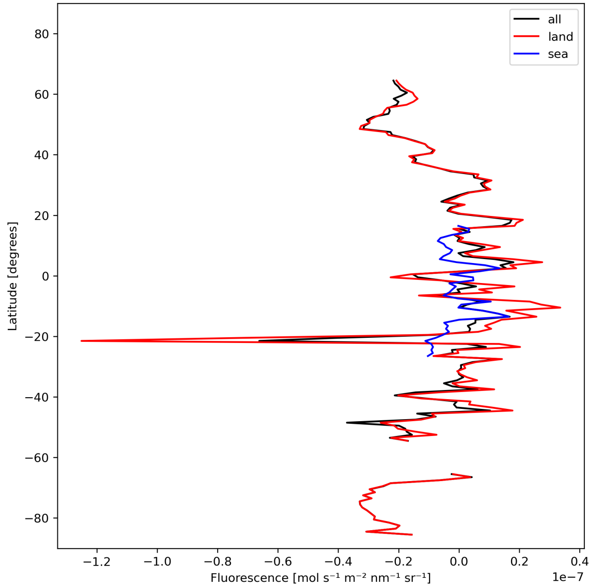
Figure 21: Zonal average of “Fluorescence” for 2024-02-22 to 2024-02-23.
