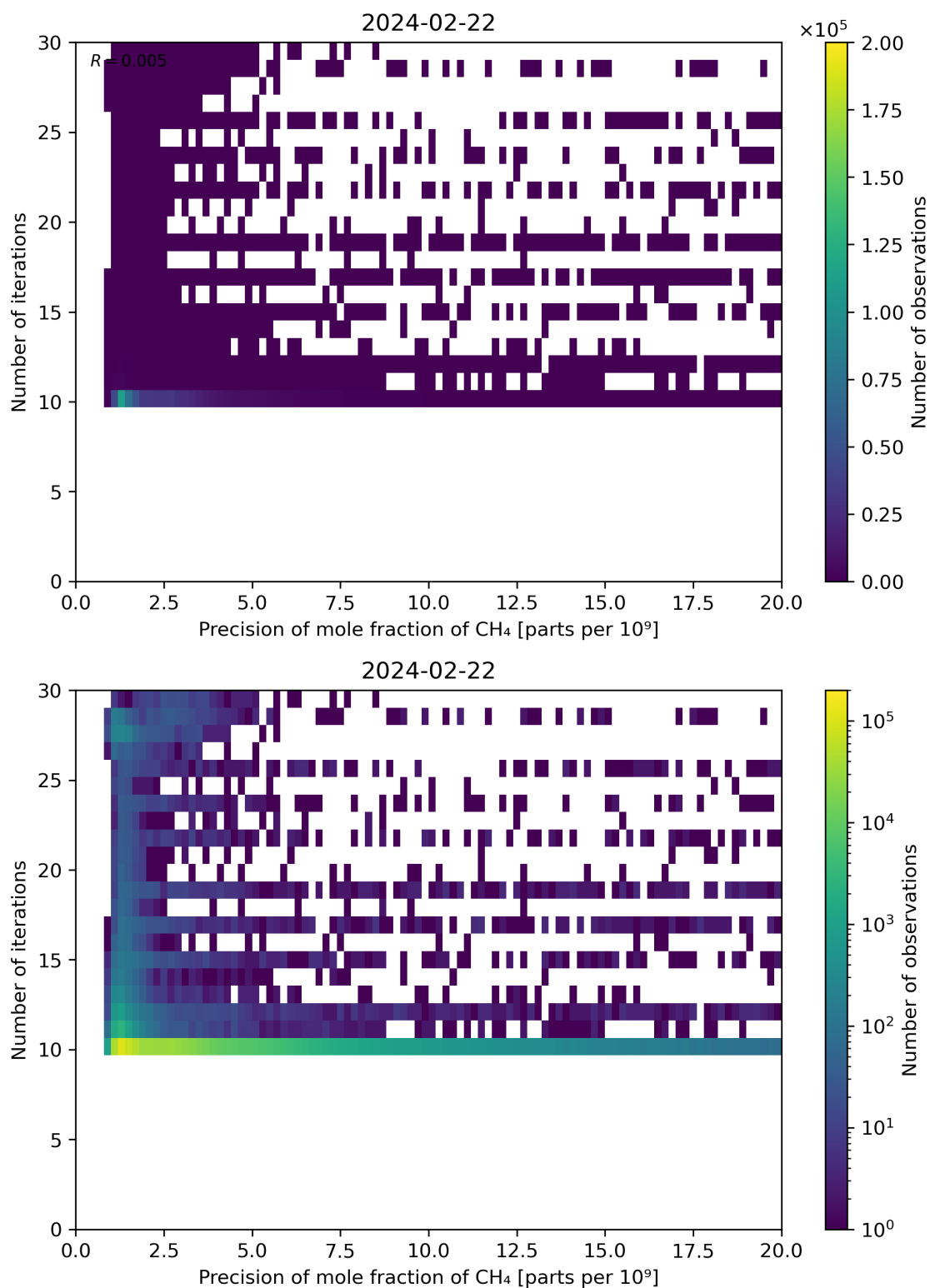
Figure 83: Scatter density plot of “Precision of mole fraction of CH 4 ” against “Number of iterations” for 2024-02-22 to 2024-02-23.
