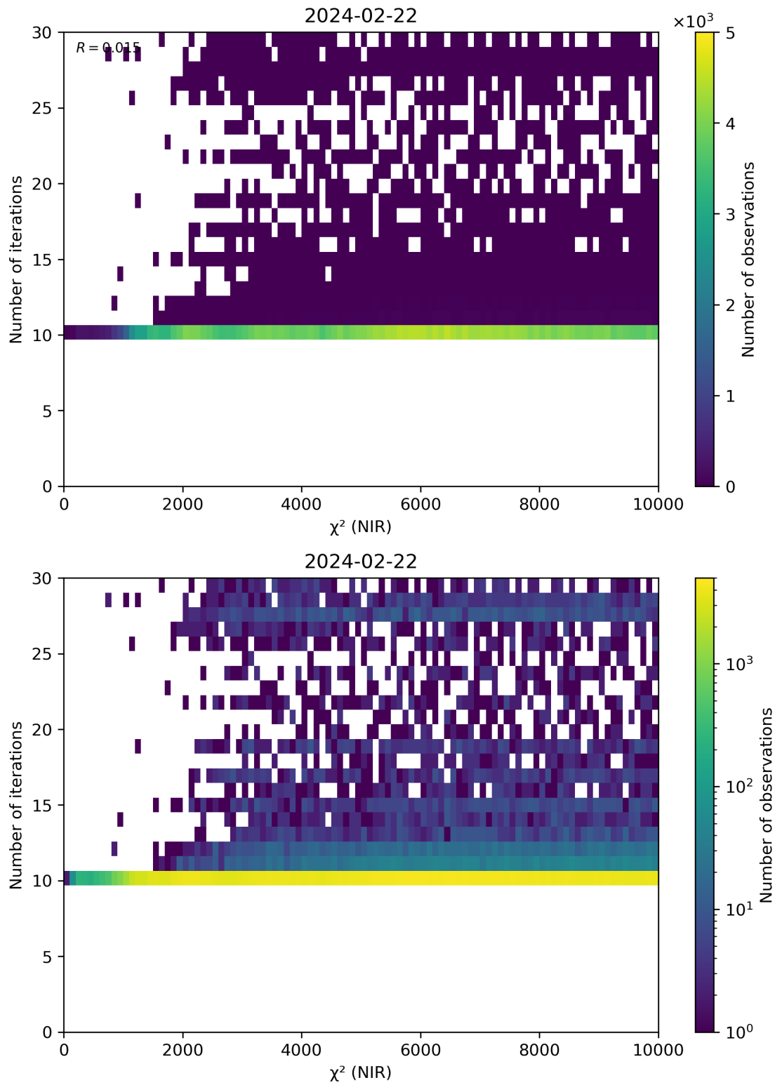
Figure 46: Scatter density plot of “ \chi^2 (NIR)” against “Number of iterations” for 2024-02-22 to 2024-02-23.
