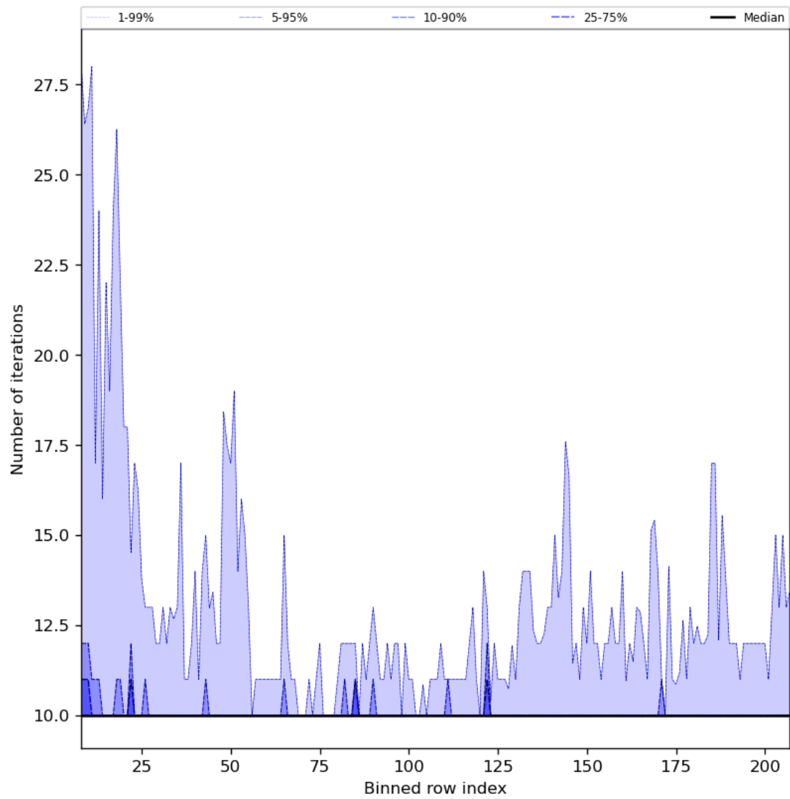
Figure 42: Along track statistics of “Number of iterations” for 2024-02-22 to 2024-02-23
