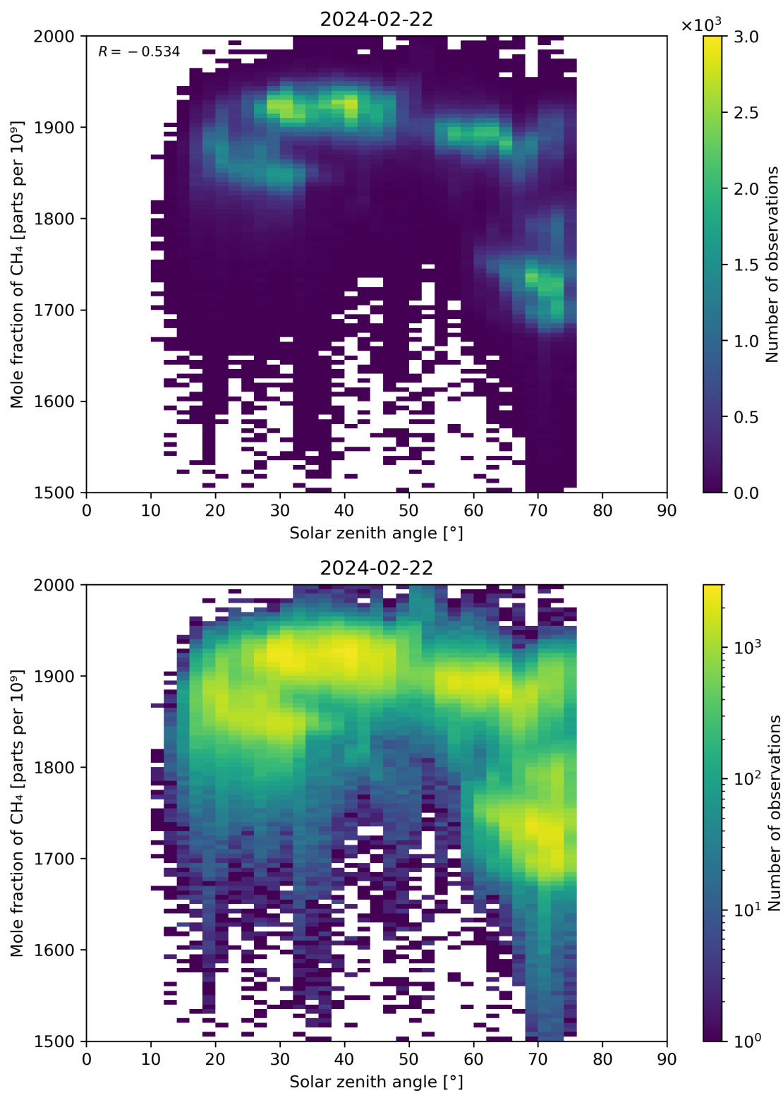
Figure 99: Scatter density plot of “Solar zenith angle” against “Mole fraction of CH 4 ” for 2024-02-22 to 2024-02-23.
