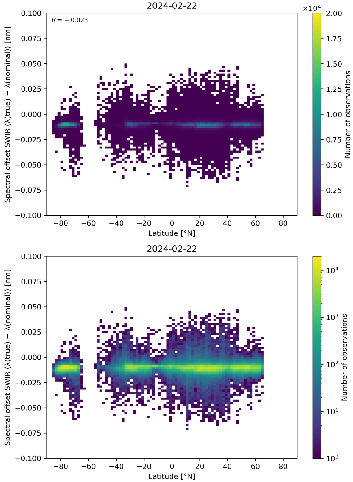
Figure 62: Scatter density plot of “Latitude” against “Spectral offset SWIR ( \lambda(\text{true}) - \lambda(\text{nominal}) )” for 2024-02-22 to 2024-02-23.
