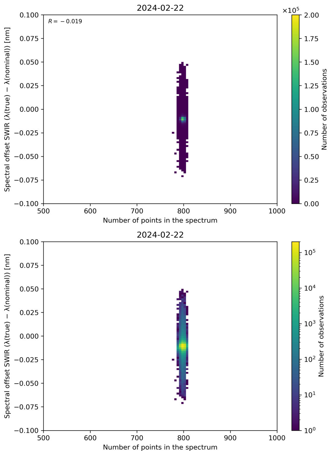
Figure 93: Scatter density plot of “Number of points in the spectrum” against “Spectral offset SWIR ( \lambda(\text{true}) - \lambda(\text{nominal}) )” for 2024-02-22 to 2024-02-23.
