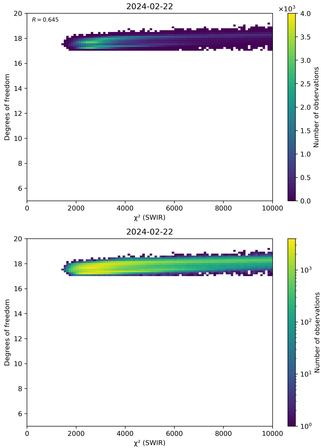
Figure 48: Scatter density plot of “ \chi^2 (SWIR)” against “Degrees of freedom” for 2024-02-22 to 2024-02-23.
