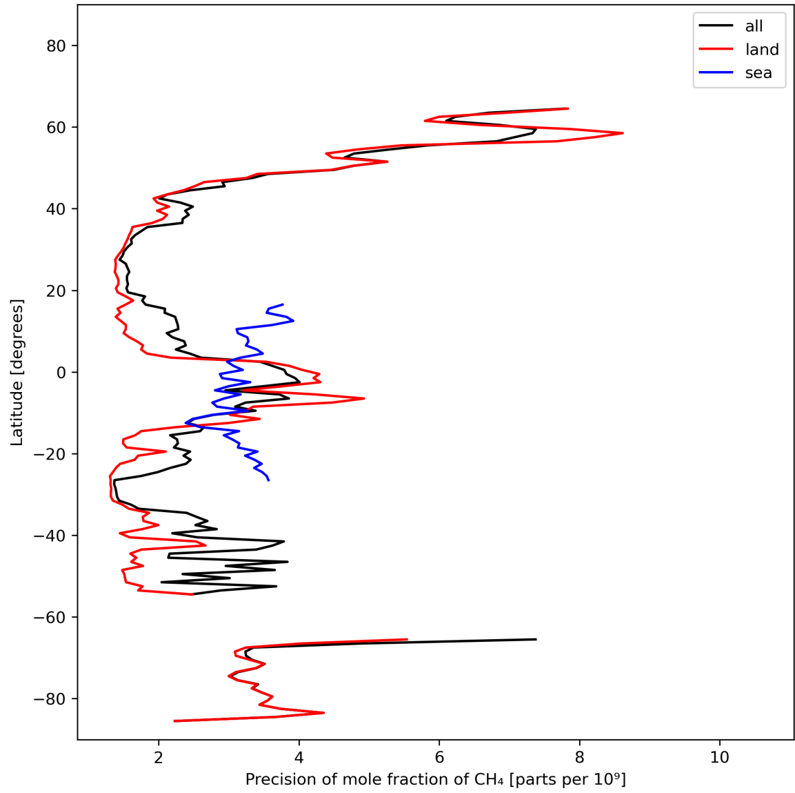
Figure 13: Zonal average of “Precision of mole fraction of CH 4 ” for 2024-02-22 to 2024-02-23.
