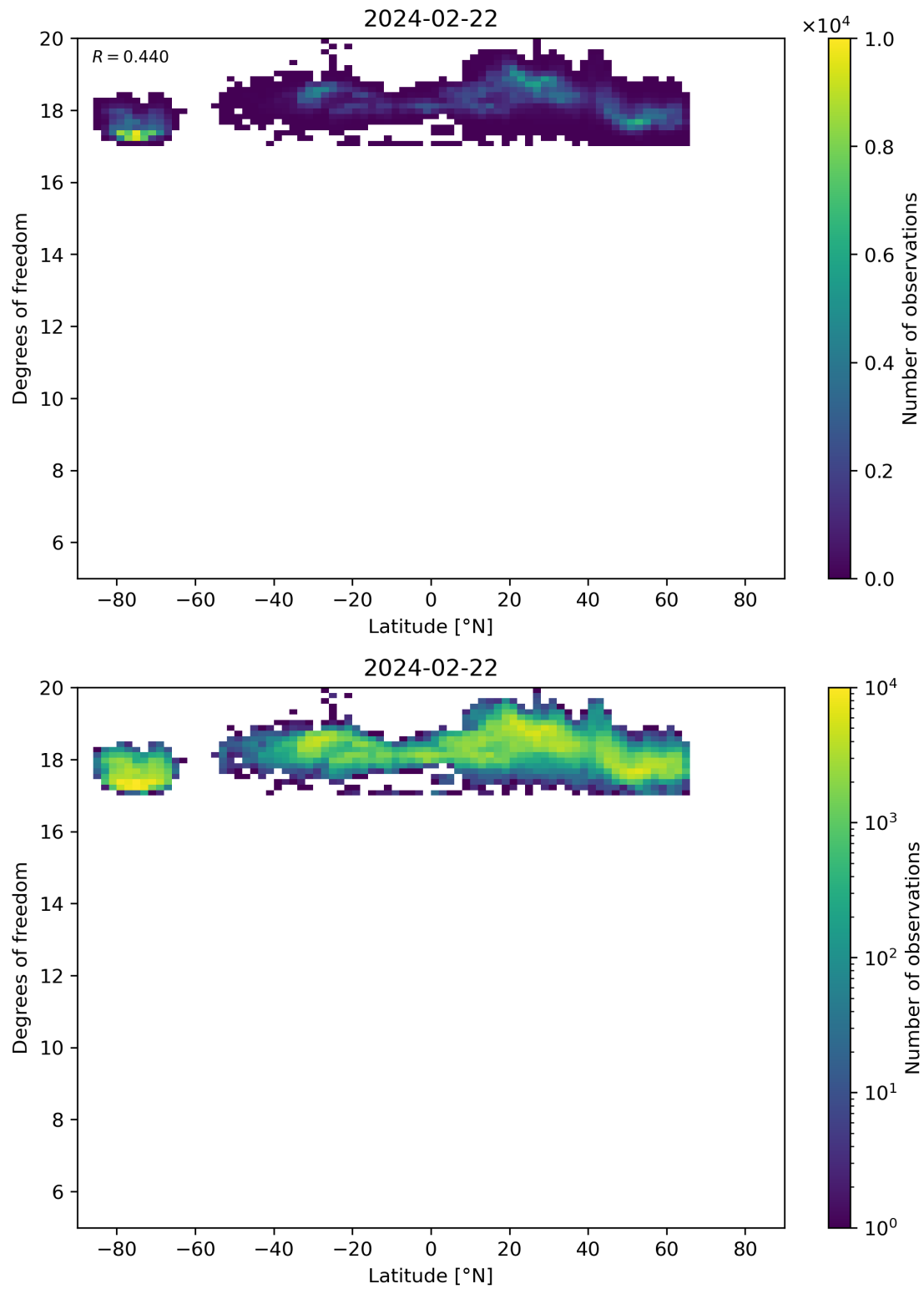
Figure 55: Scatter density plot of “Latitude” against “Degrees of freedom” for 2024-02-22 to 2024-02-23.
