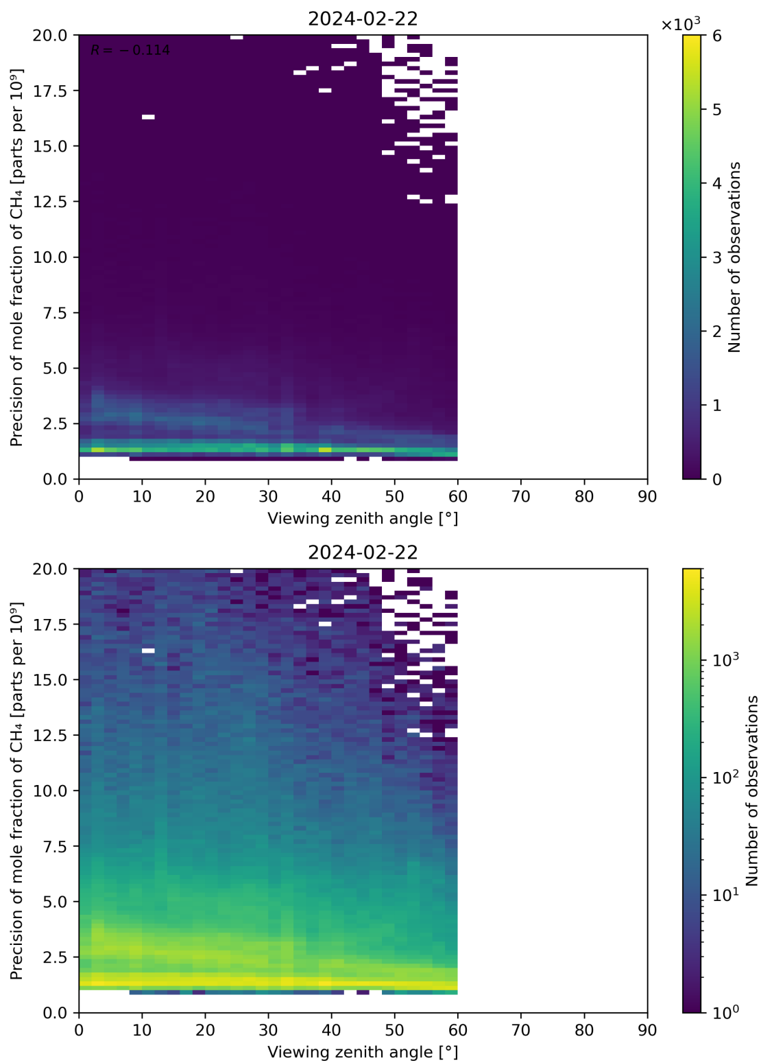
Figure 112: Scatter density plot of “Viewing zenith angle” against “Precision of mole fraction of CH 4 ” for 2024-02-22 to 2024-02-23.
