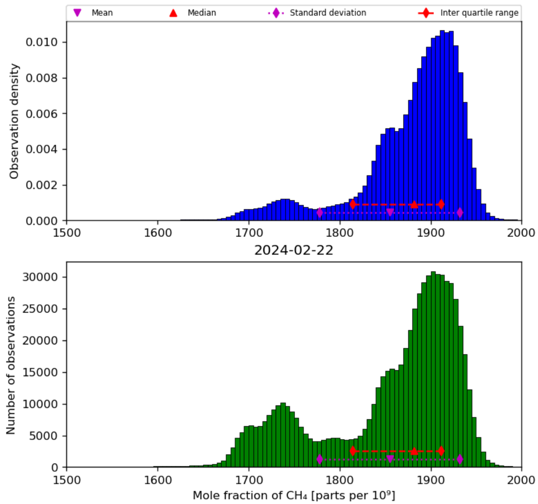
Figure 23: Histogram of “Mole fraction of CH 4 ” for 2024-02-22 to 2024-02-23
