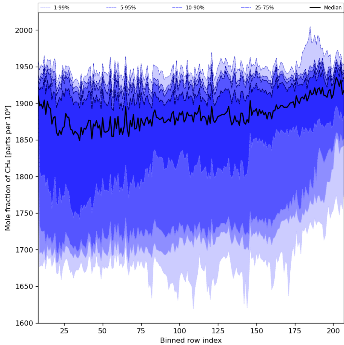
Figure 34: Along track statistics of “Mole fraction of CH 4 ” for 2024-02-22 to 2024-02-23
