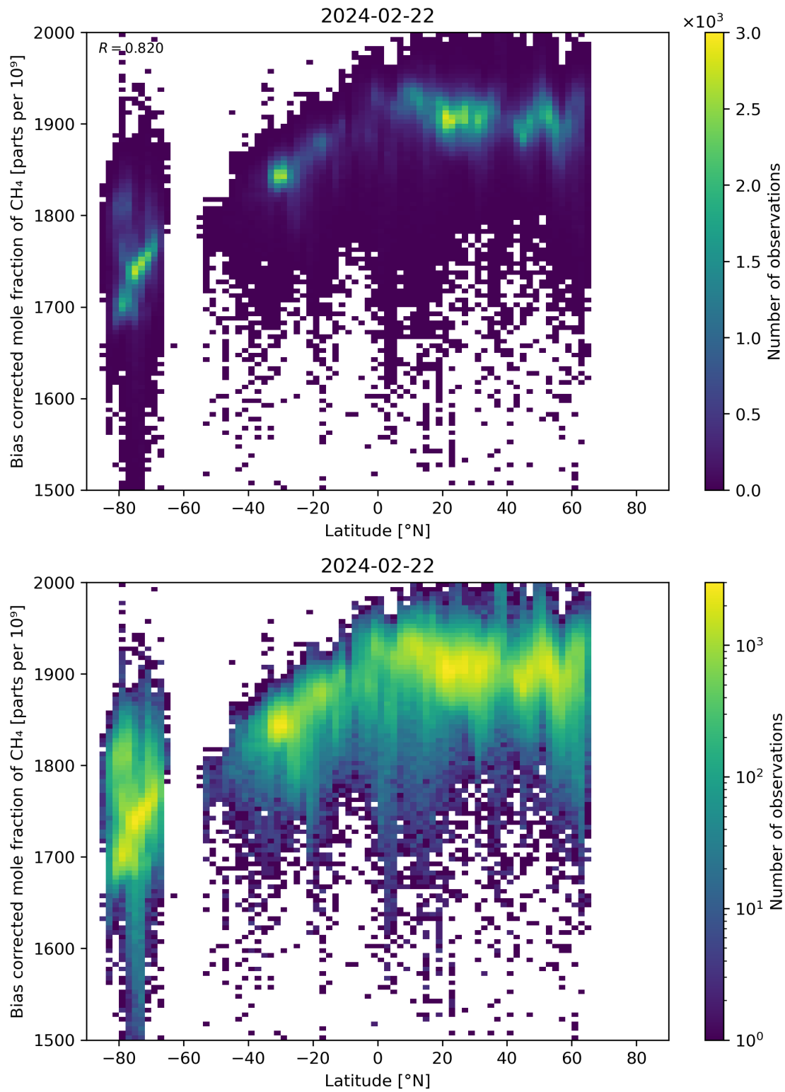
Figure 58: Scatter density plot of “Latitude” against “Bias corrected mole fraction of CH 4 ” for 2024-02-22 to 2024-02-23.
