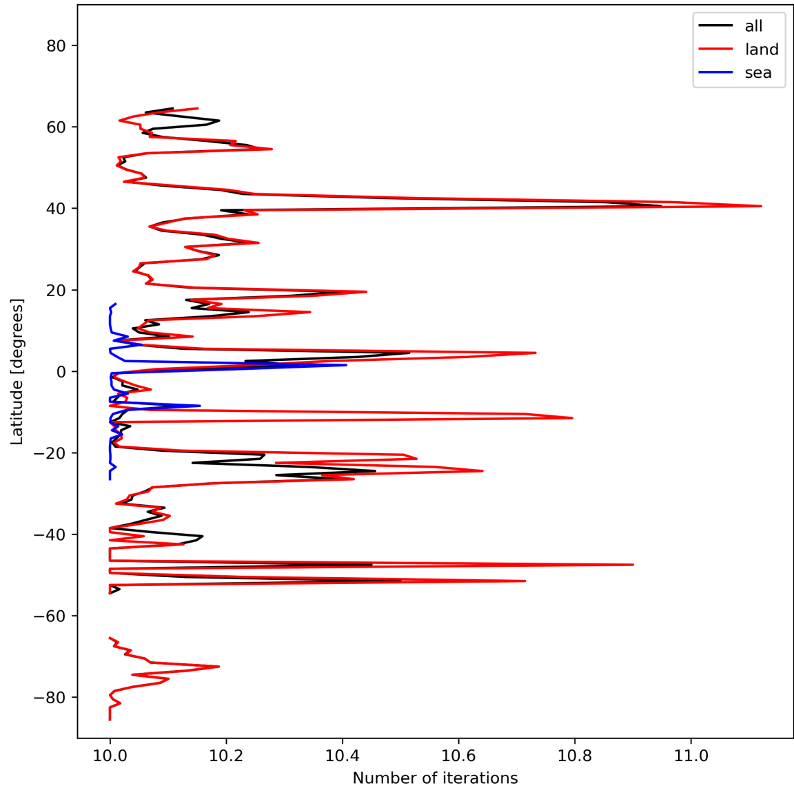
Figure 20: Zonal average of “Number of iterations” for 2024-02-22 to 2024-02-23.
