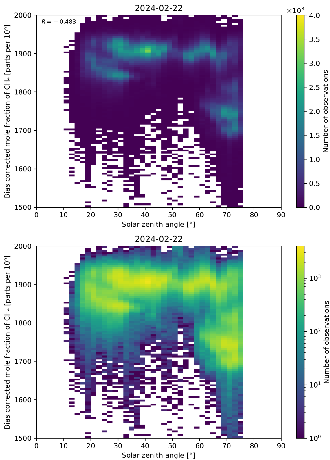
Figure 100: Scatter density plot of “Solar zenith angle” against “Bias corrected mole fraction of \text{CH}_4 ” for 2024-02-22 to 2024-02-23.
