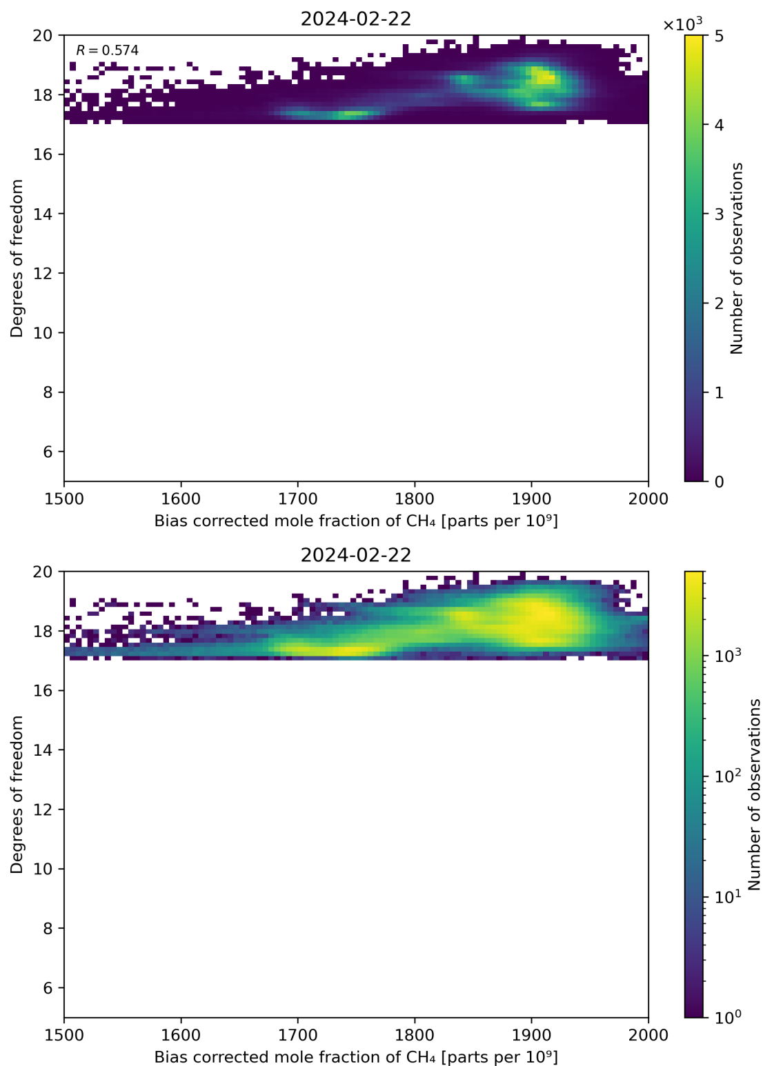
Figure 65: Scatter density plot of “Bias corrected mole fraction of CH 4 ” against “Degrees of freedom” for 2024-02-22 to 2024-02-23.
