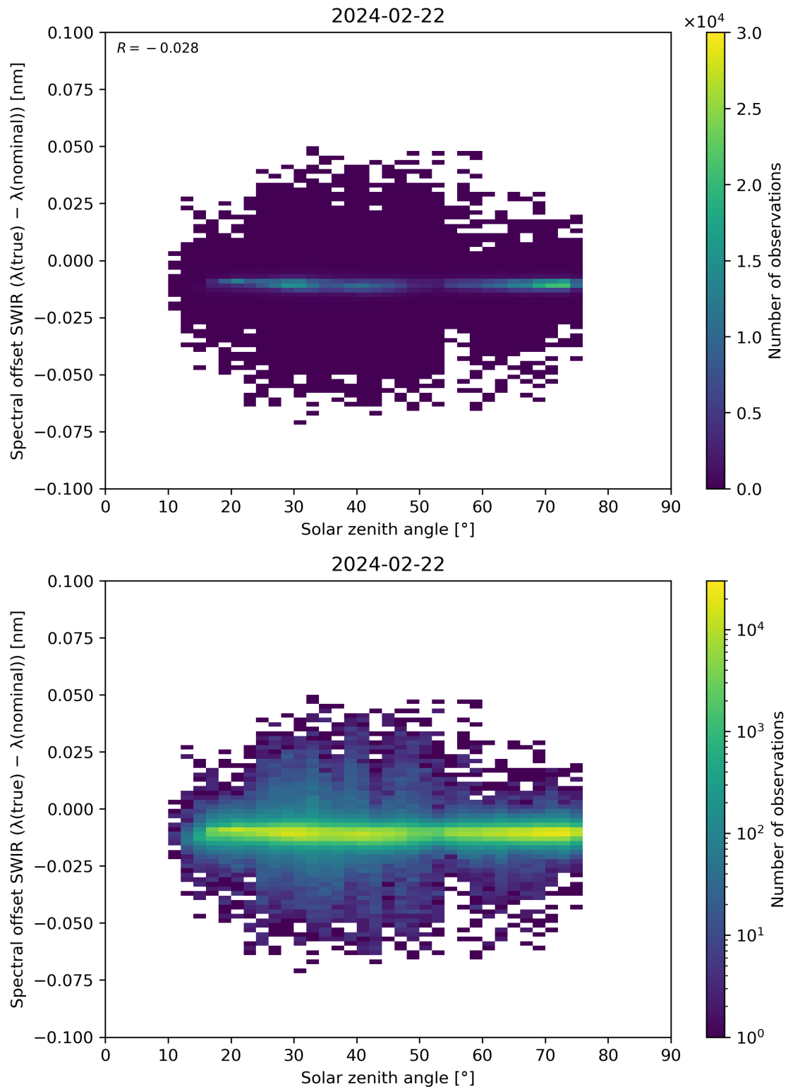
Figure 104: Scatter density plot of “Solar zenith angle” against “Spectral offset SWIR ( \lambda(\text{true}) - \lambda(\text{nominal}) )” for 2024-02-22 to 2024-02-23.
