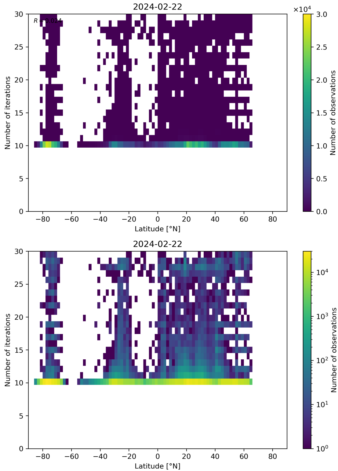
Figure 60: Scatter density plot of “Latitude” against “Number of iterations” for 2024-02-22 to 2024-02-23.
