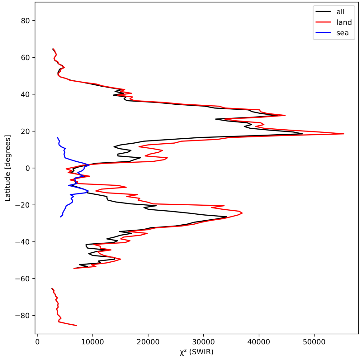
Figure 17: Zonal average of “ \chi^2 (SWIR)” for 2024-02-22 to 2024-02-23.
