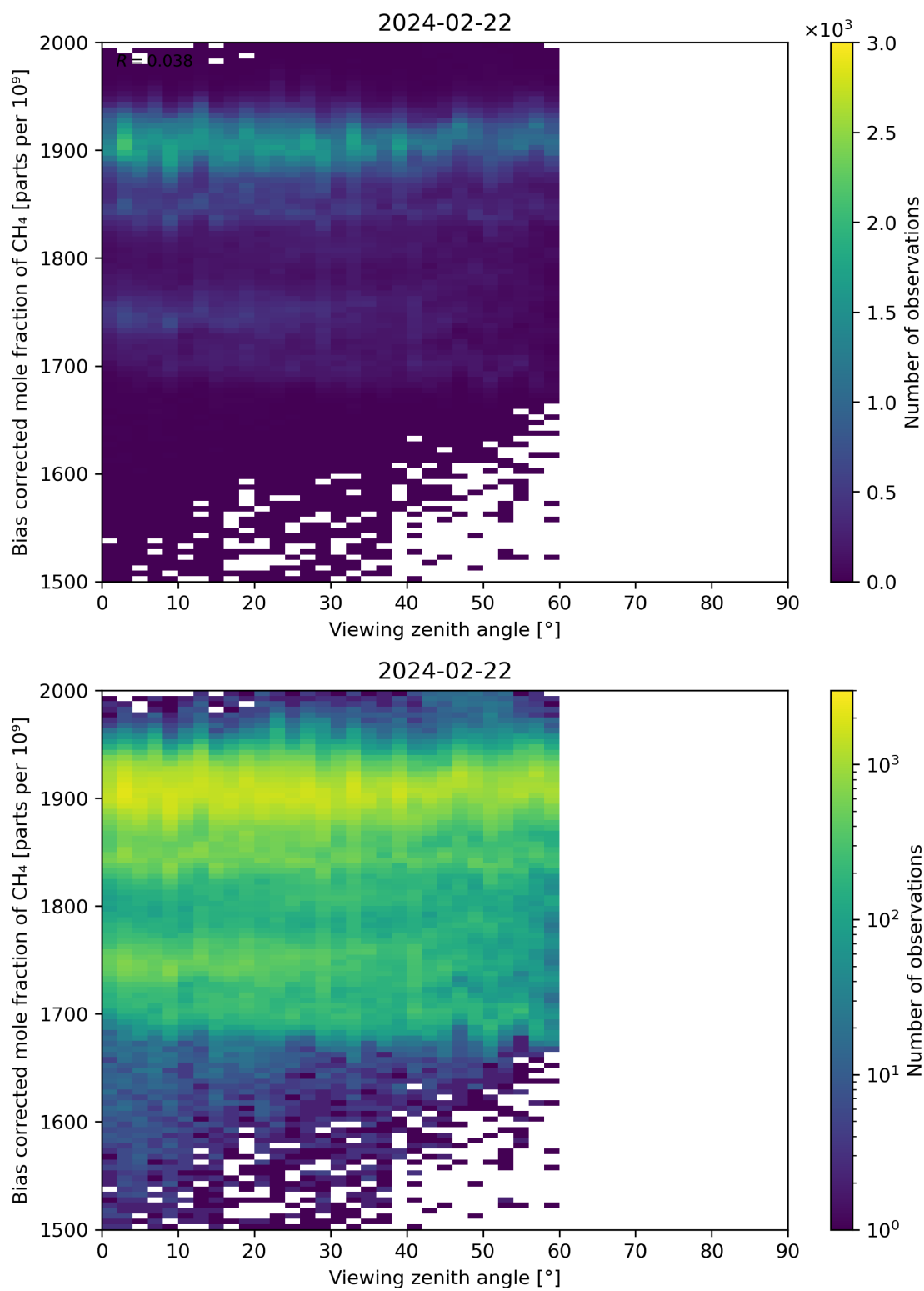
Figure 111: Scatter density plot of “Viewing zenith angle” against “Bias corrected mole fraction of CH 4 ” for 2024-02-22 to 2024-02-23.
