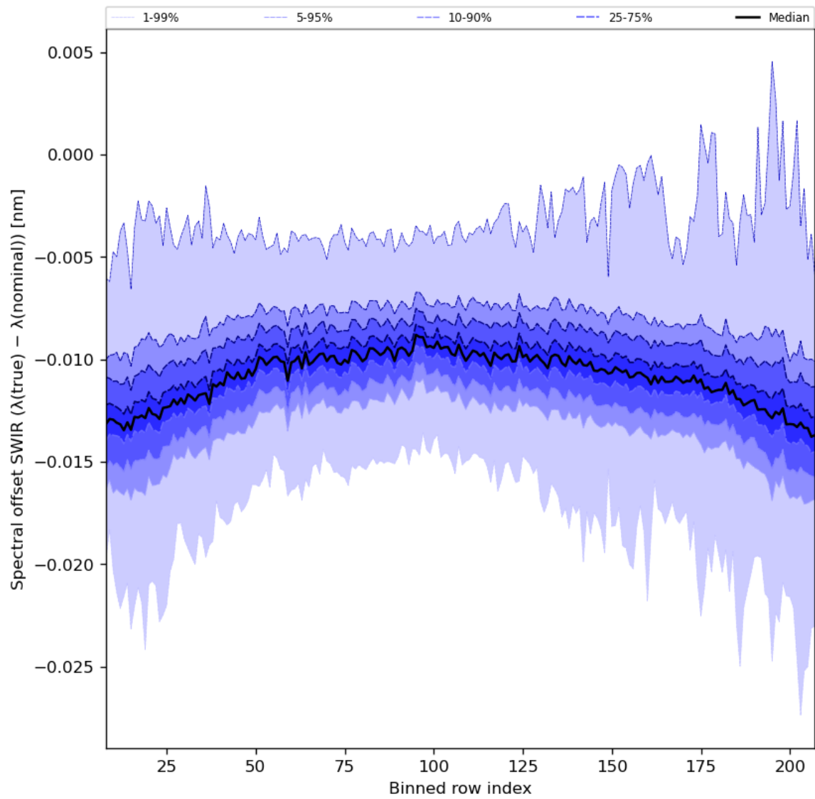
Figure 38: Along track statistics of “Spectral offset SWIR ( \lambda(\text{true}) - \lambda(\text{nominal}) )” for 2024-02-22 to 2024-02-23
