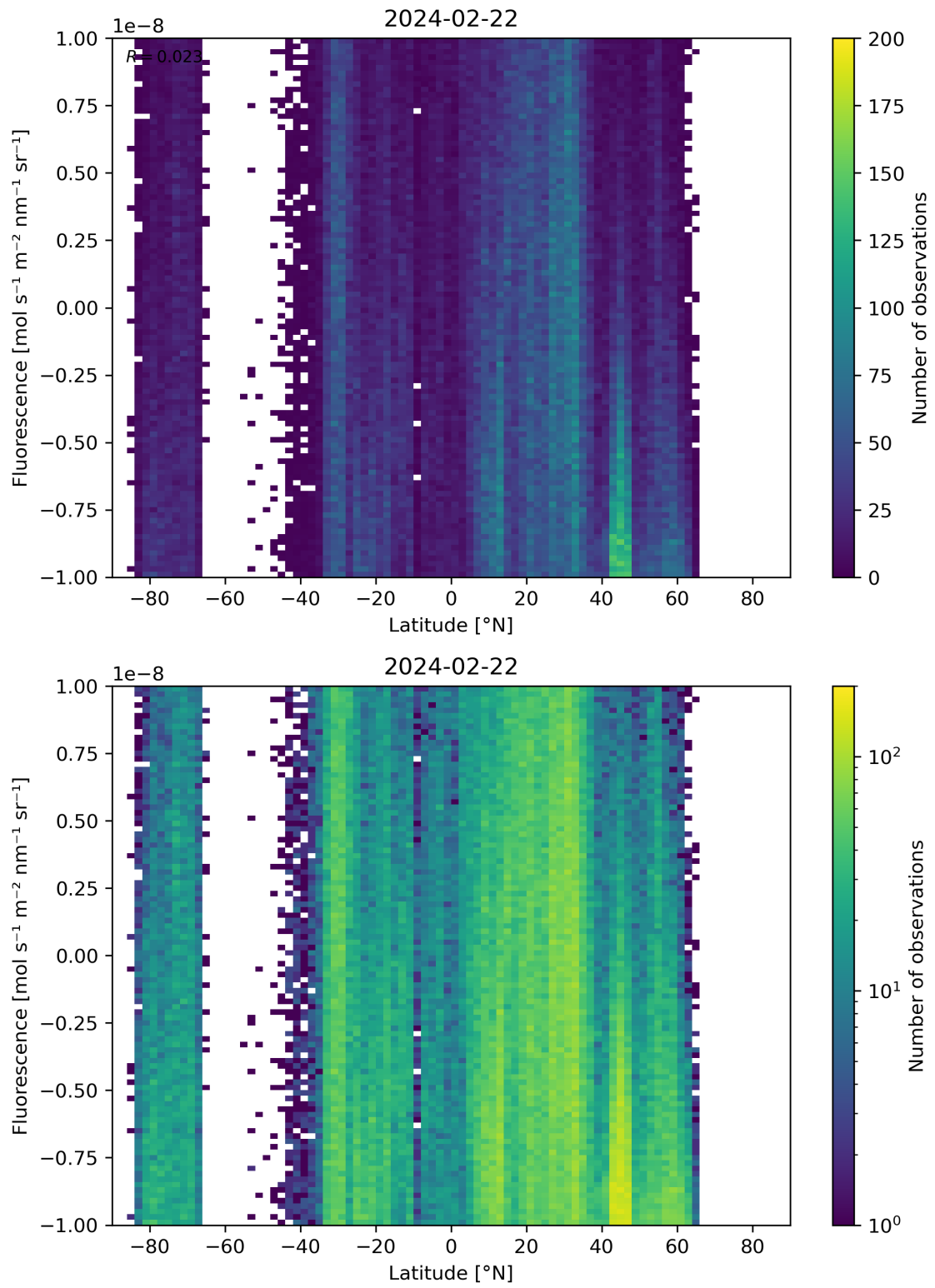
Figure 56: Scatter density plot of “Latitude” against “Fluorescence” for 2024-02-22 to 2024-02-23.
