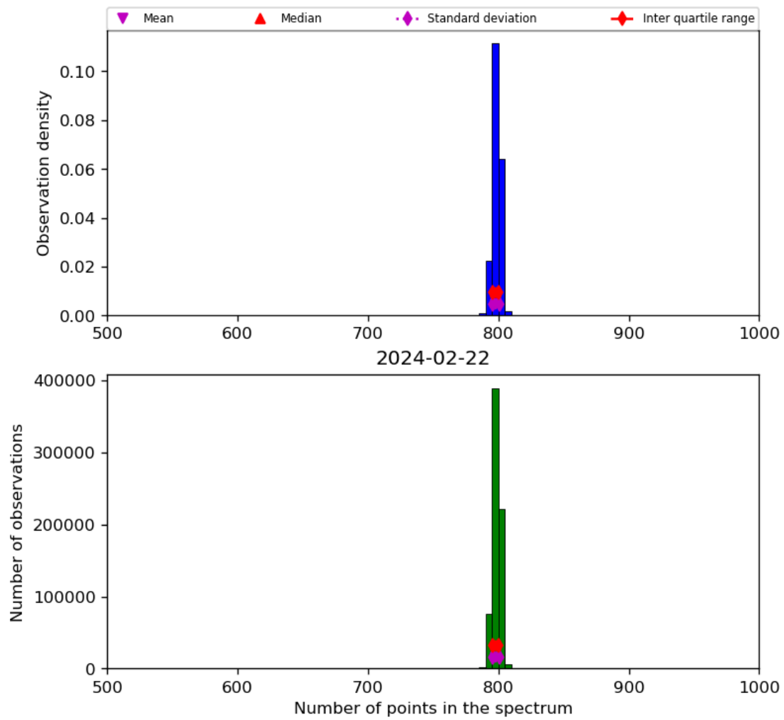
Figure 26: Histogram of “Number of points in the spectrum” for 2024-02-22 to 2024-02-23
