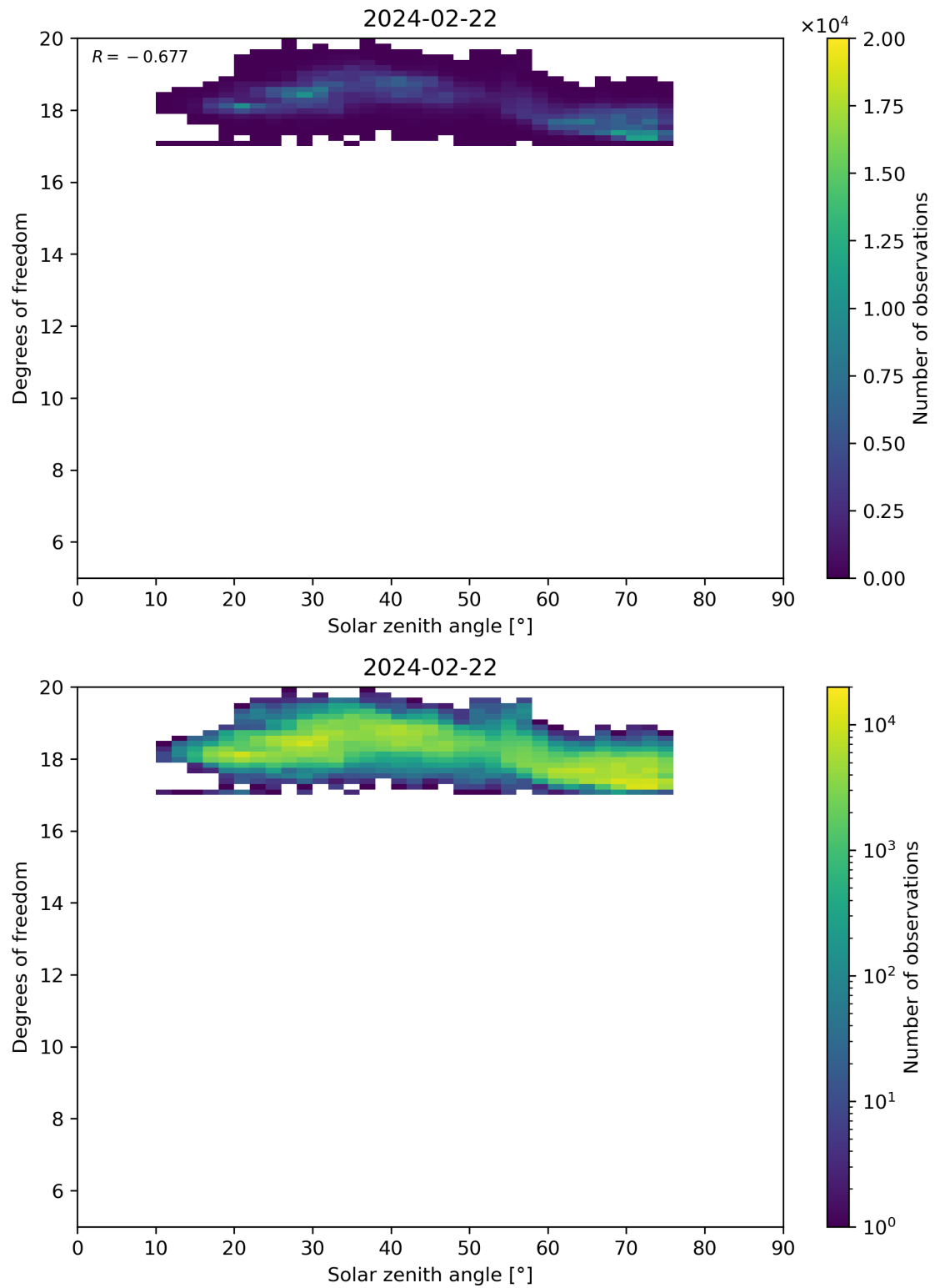
Figure 96: Scatter density plot of “Solar zenith angle” against “Degrees of freedom” for 2024-02-22 to 2024-02-23.
