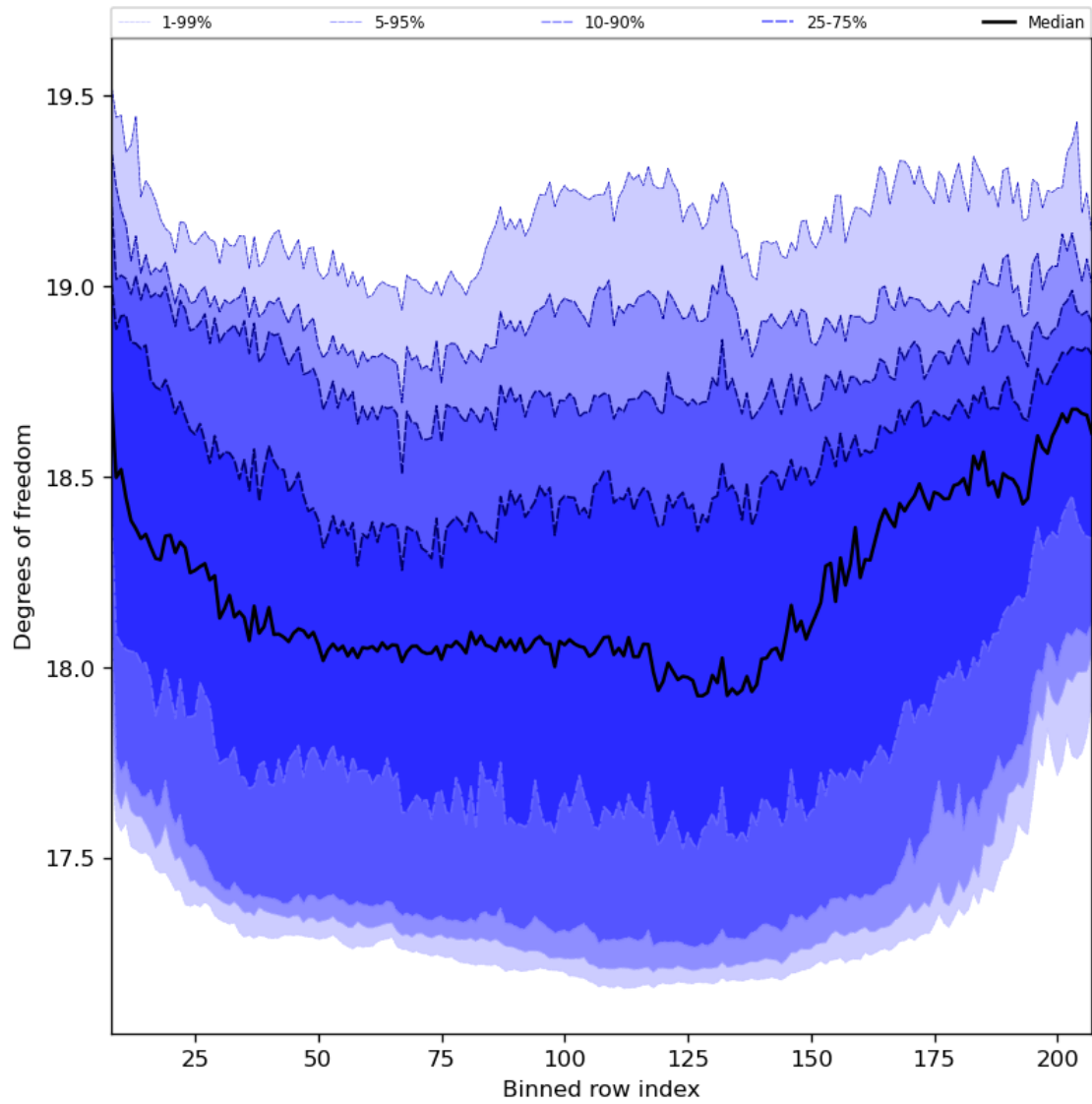
Figure 41: Along track statistics of “Degrees of freedom” for 2024-02-22 to 2024-02-23
