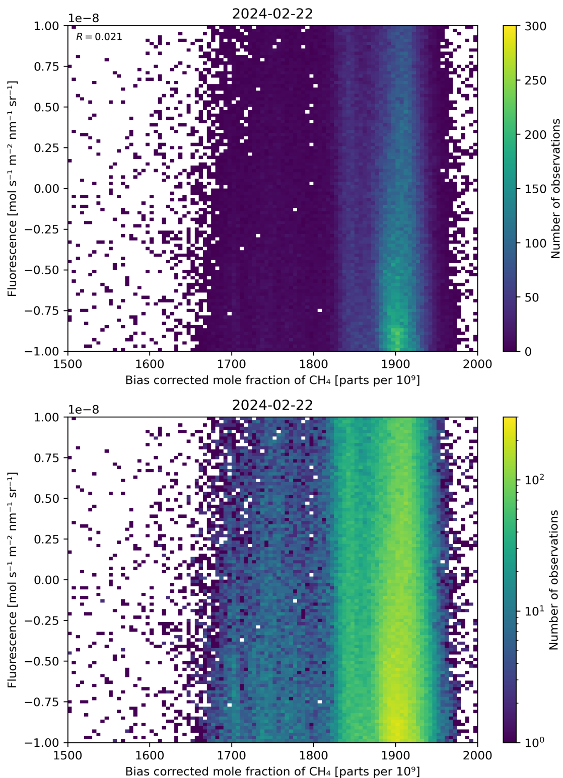
Figure 66: Scatter density plot of “Bias corrected mole fraction of \text{CH}_4 ” against “Fluorescence” for 2024-02-22 to 2024-02-23.
