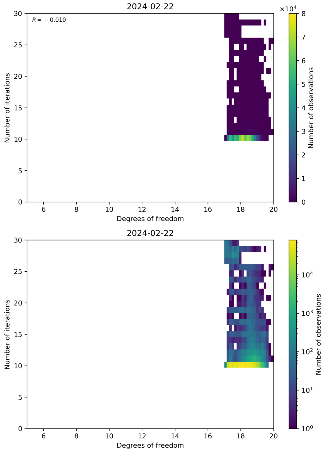
Figure 52: Scatter density plot of “Degrees of freedom” against “Number of iterations” for 2024-02-22 to 2024-02-23.
