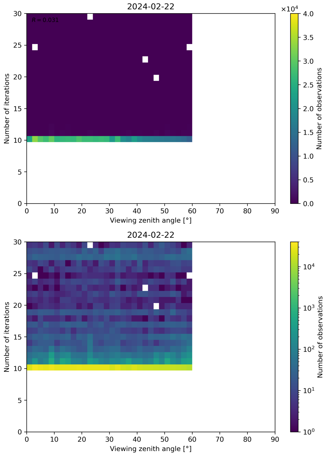
Figure 113: Scatter density plot of “Viewing zenith angle” against “Number of iterations” for 2024-02-22 to 2024-02-23.
