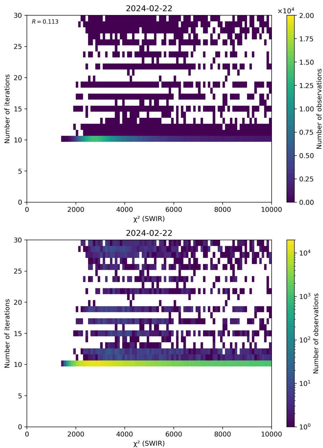
Figure 50: Scatter density plot of “ \chi^2 (SWIR)” against “Number of iterations” for 2024-02-22 to 2024-02-23.
