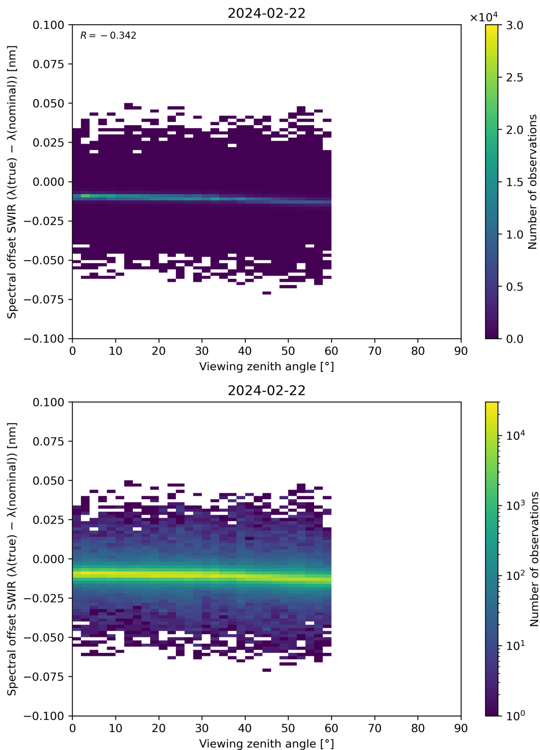
Figure 116: Scatter density plot of “Viewing zenith angle” against “Spectral offset SWIR ( \lambda(\text{true}) - \lambda(\text{nominal}) )” for 2024-02-22 to 2024-02-23.
