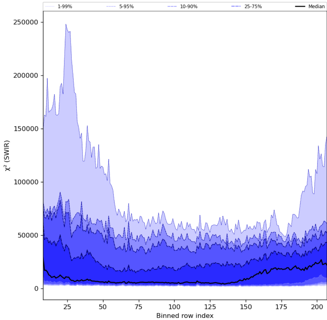
Figure 39: Along track statistics of " \chi^2 (SWIR)" for 2024-02-22 to 2024-02-23
