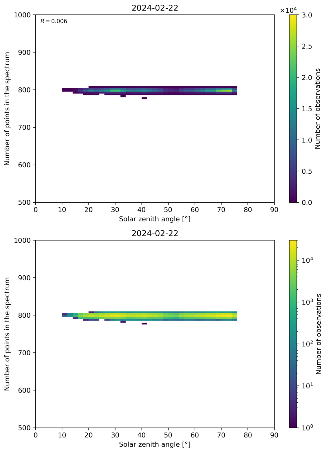
Figure 103: Scatter density plot of “Solar zenith angle” against “Number of points in the spectrum” for 2024-02-22 to 2024-02-23.
