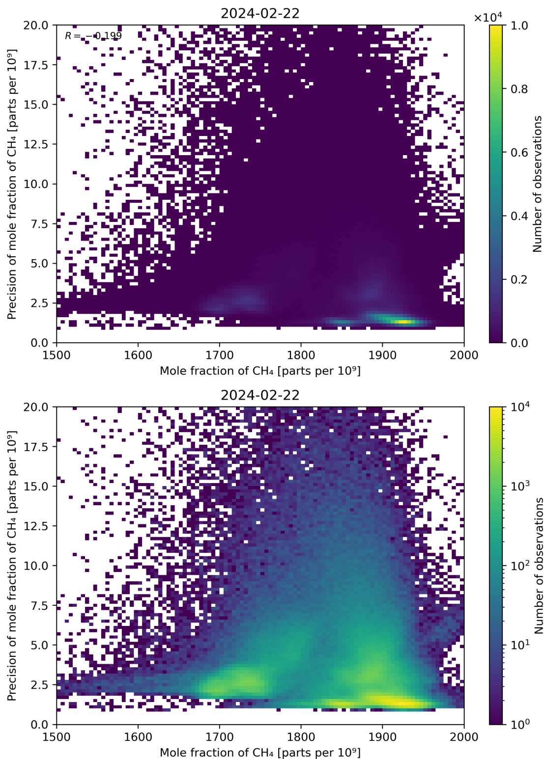
Figure 75: Scatter density plot of “Mole fraction of CH 4 ” against “Precision of mole fraction of CH 4 ” for 2024-02-22 to 2024-02-23.
