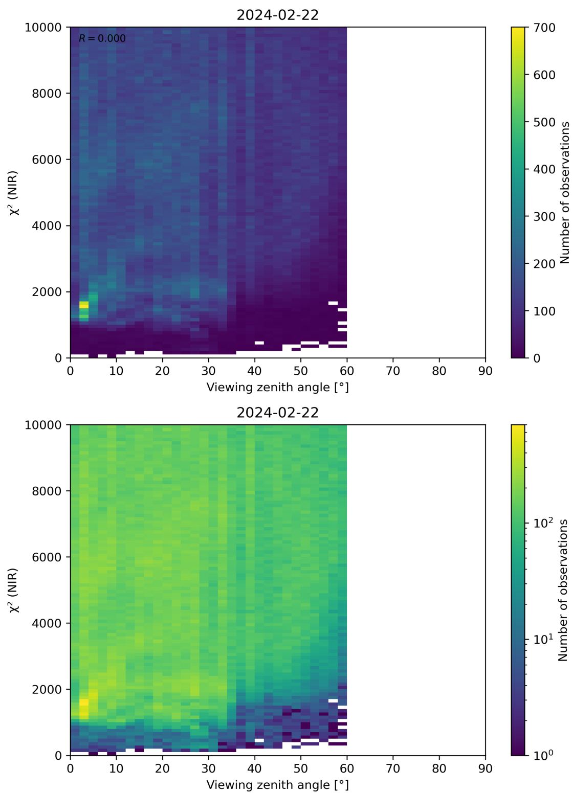
Figure 105: Scatter density plot of “Viewing zenith angle” against “ \chi^2 (NIR)” for 2024-02-22 to 2024-02-23.
