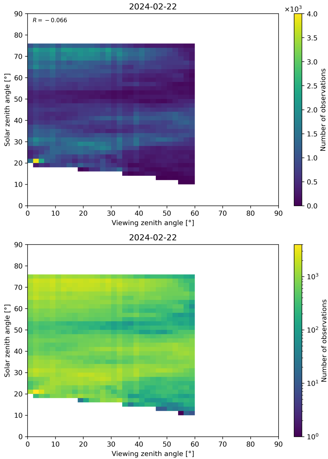
Figure 115: Scatter density plot of “Viewing zenith angle” against “Solar zenith angle” for 2024-02-22 to 2024-02-23.
