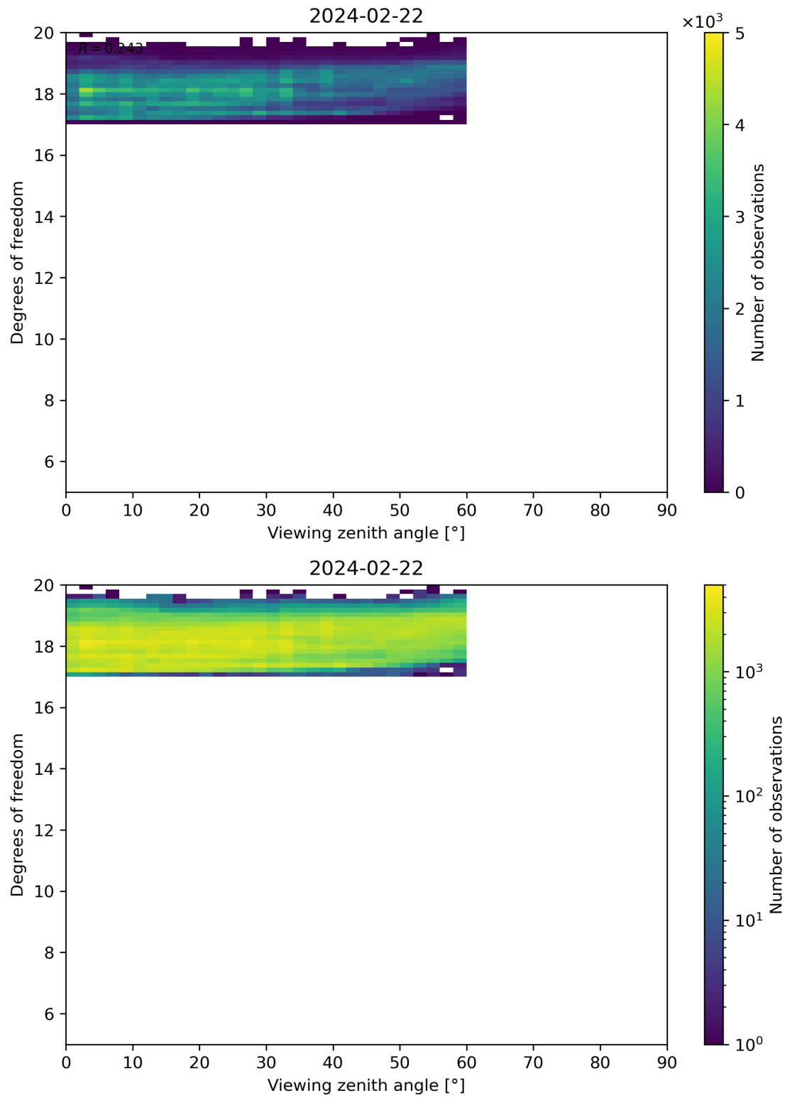
Figure 107: Scatter density plot of “Viewing zenith angle” against “Degrees of freedom” for 2024-02-22 to 2024-02-23.
