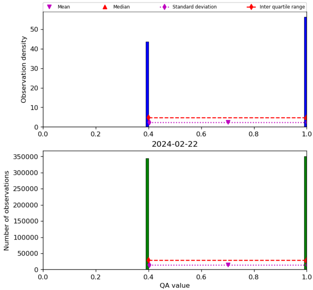
Figure 22: Histogram of “QA value” for 2024-02-22 to 2024-02-23
