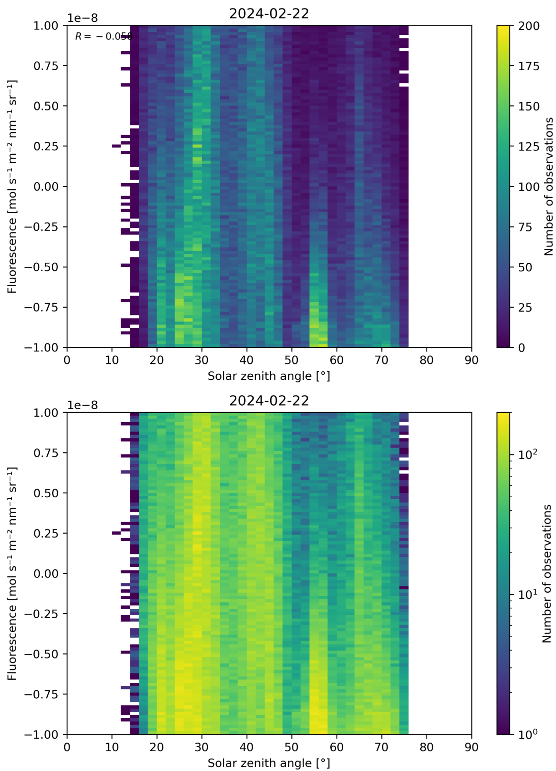
Figure 97: Scatter density plot of “Solar zenith angle” against “Fluorescence” for 2024-02-22 to 2024-02-23.
