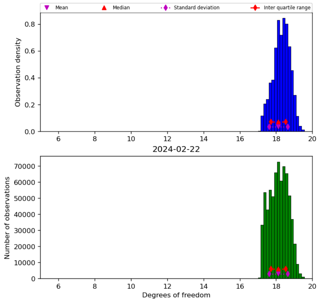
Figure 30: Histogram of “Degrees of freedom” for 2024-02-22 to 2024-02-23
