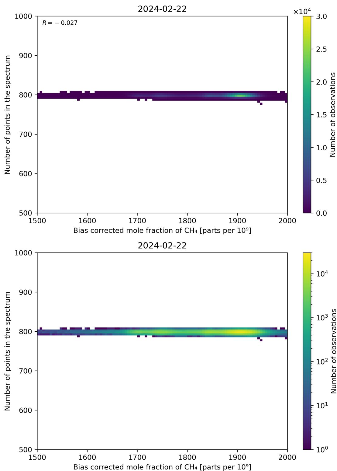
Figure 68: Scatter density plot of “Bias corrected mole fraction of CH 4 ” against “Number of points in the spectrum” for 2024-02-22 to 2024-02-23.
