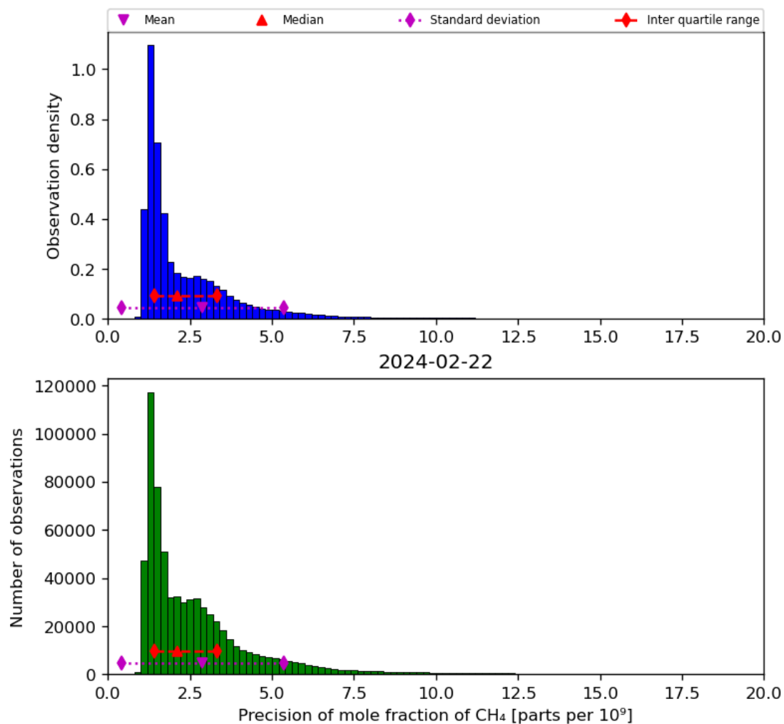
Figure 24: Histogram of “Precision of mole fraction of CH 4 ” for 2024-02-22 to 2024-02-23
