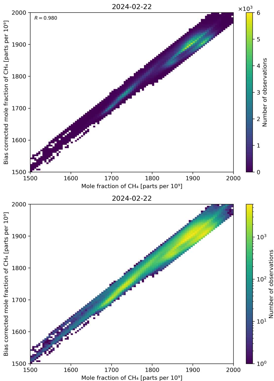
Figure 74: Scatter density plot of “Mole fraction of CH 4 ” against “Bias corrected mole fraction of CH 4 ” for 2024-02-22 to 2024-02-23.
