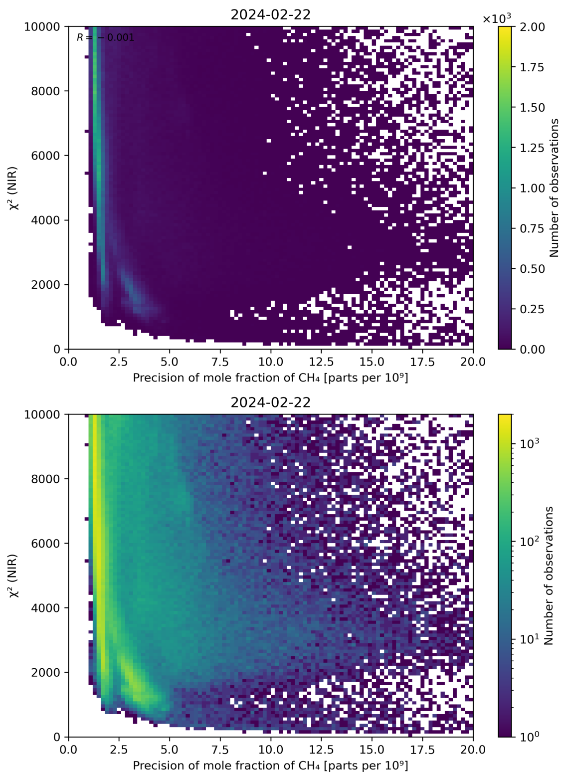
Figure 78: Scatter density plot of “Precision of mole fraction of CH 4 ” against “ \chi^2 (NIR)” for 2024-02-22 to 2024-02-23.
