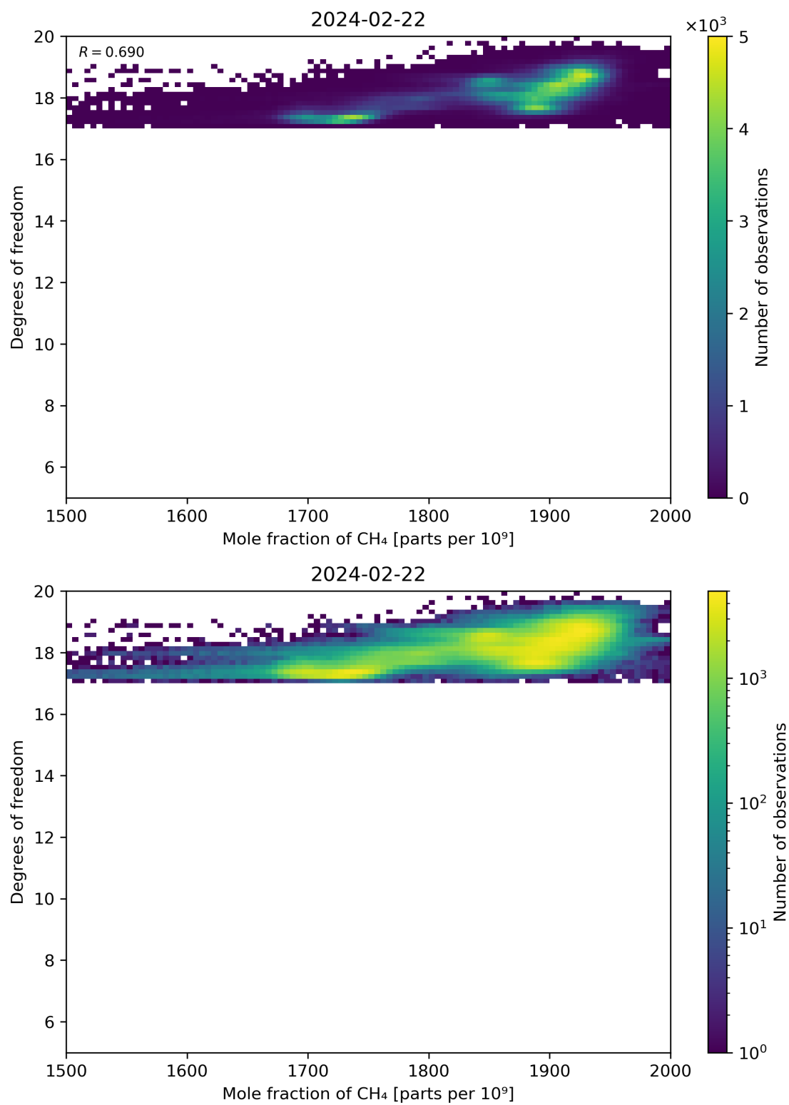
Figure 72: Scatter density plot of “Mole fraction of CH 4 ” against “Degrees of freedom” for 2024-02-22 to 2024-02-23.
