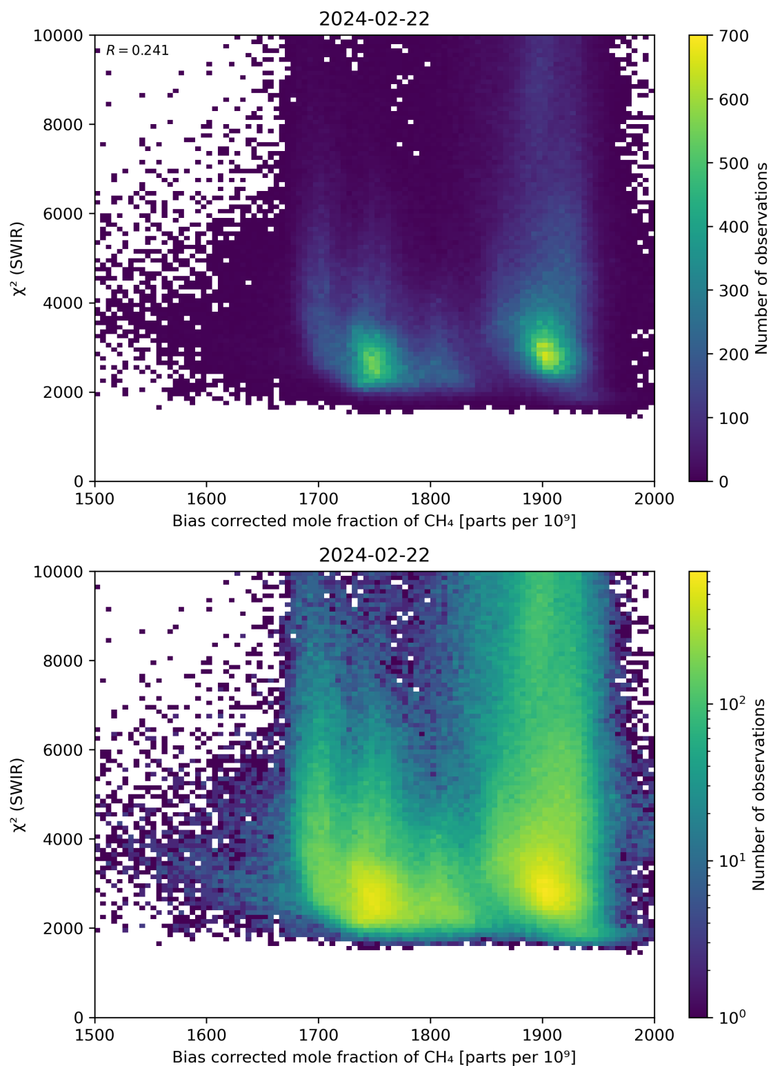
Figure 64: Scatter density plot of “Bias corrected mole fraction of CH 4 ” against “ \chi^2 (SWIR)” for 2024-02-22 to 2024-02-23.
