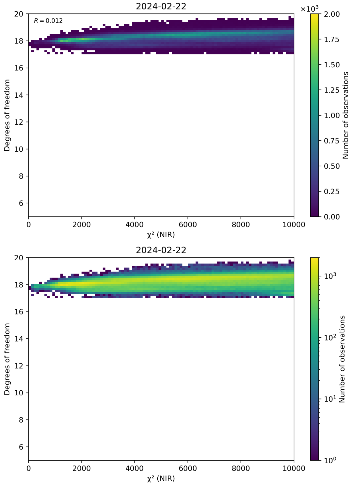
Figure 44: Scatter density plot of “ \chi^2 (NIR)” against “Degrees of freedom” for 2024-02-22 to 2024-02-23.
