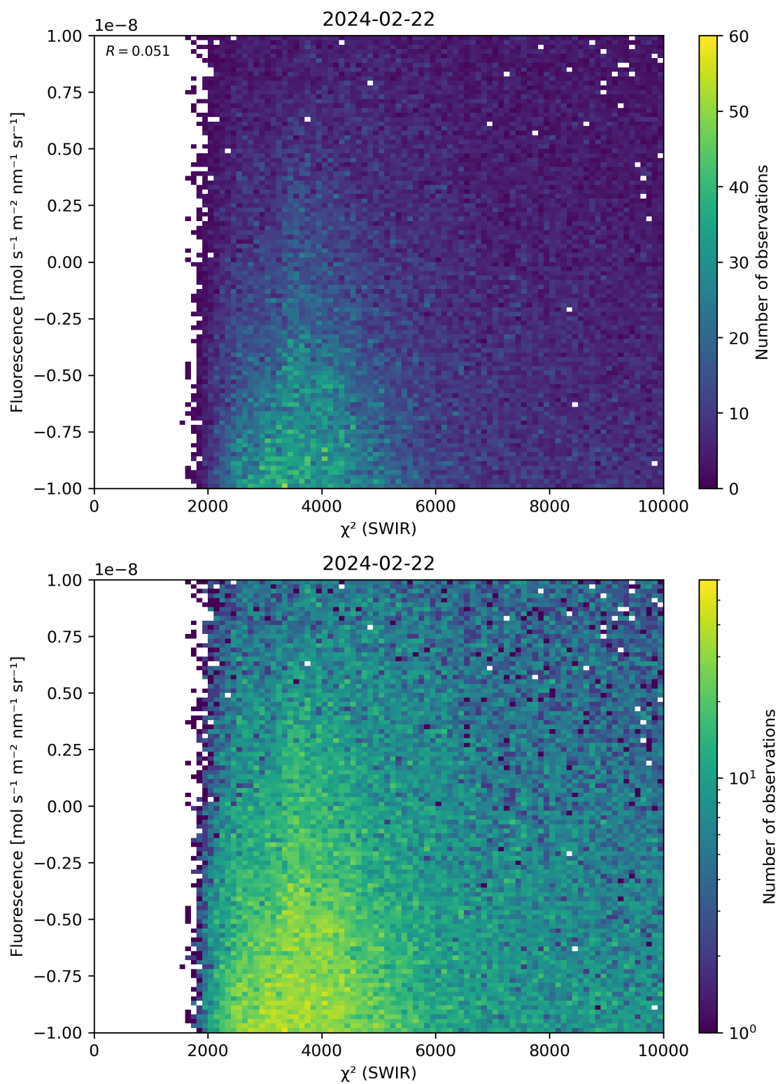
Figure 49: Scatter density plot of “ \chi^2 (SWIR)” against “Fluorescence” for 2024-02-22 to 2024-02-23.
