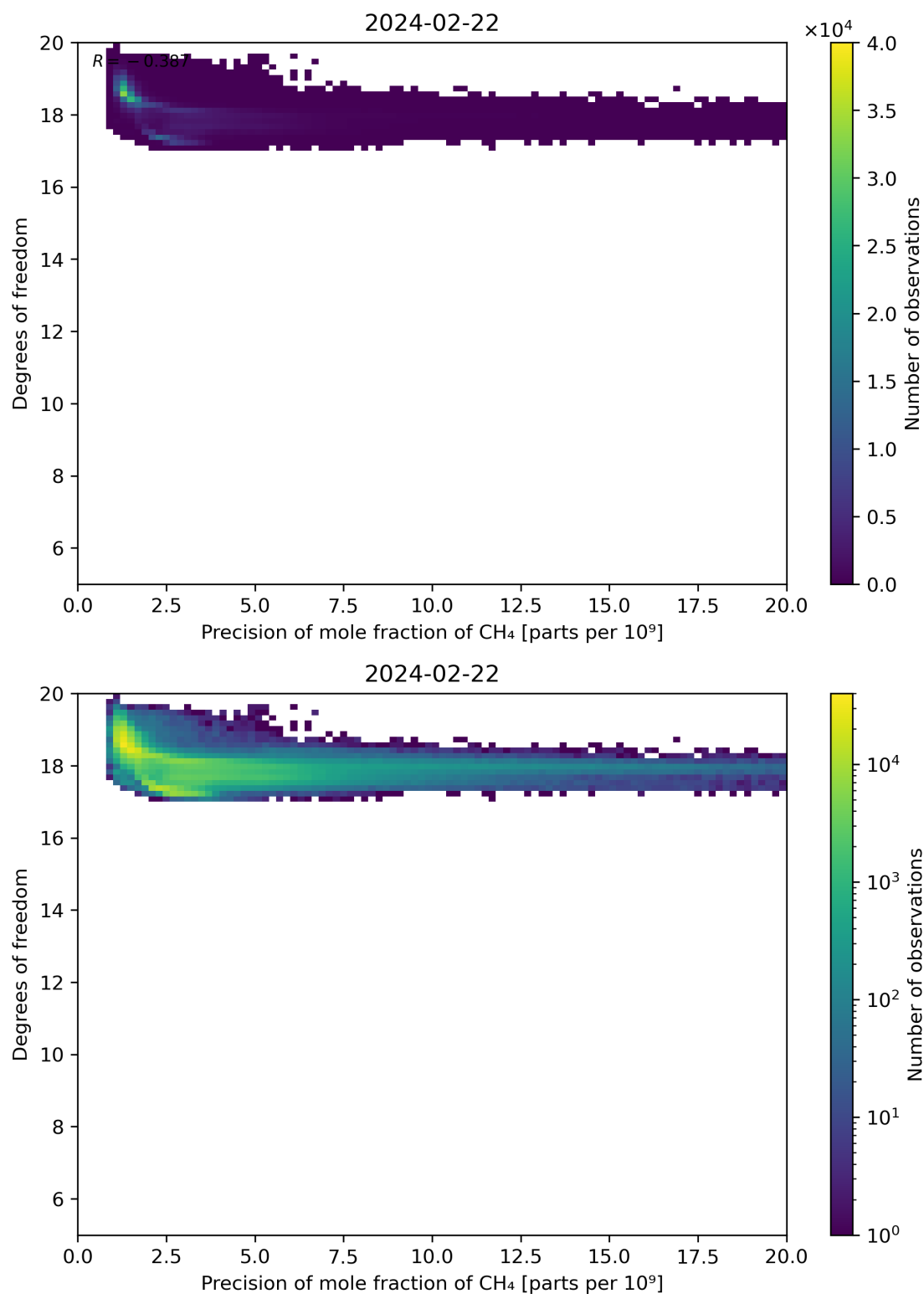
Figure 80: Scatter density plot of “Precision of mole fraction of CH 4 ” against “Degrees of freedom” for 2024-02-22 to 2024-02-23.
