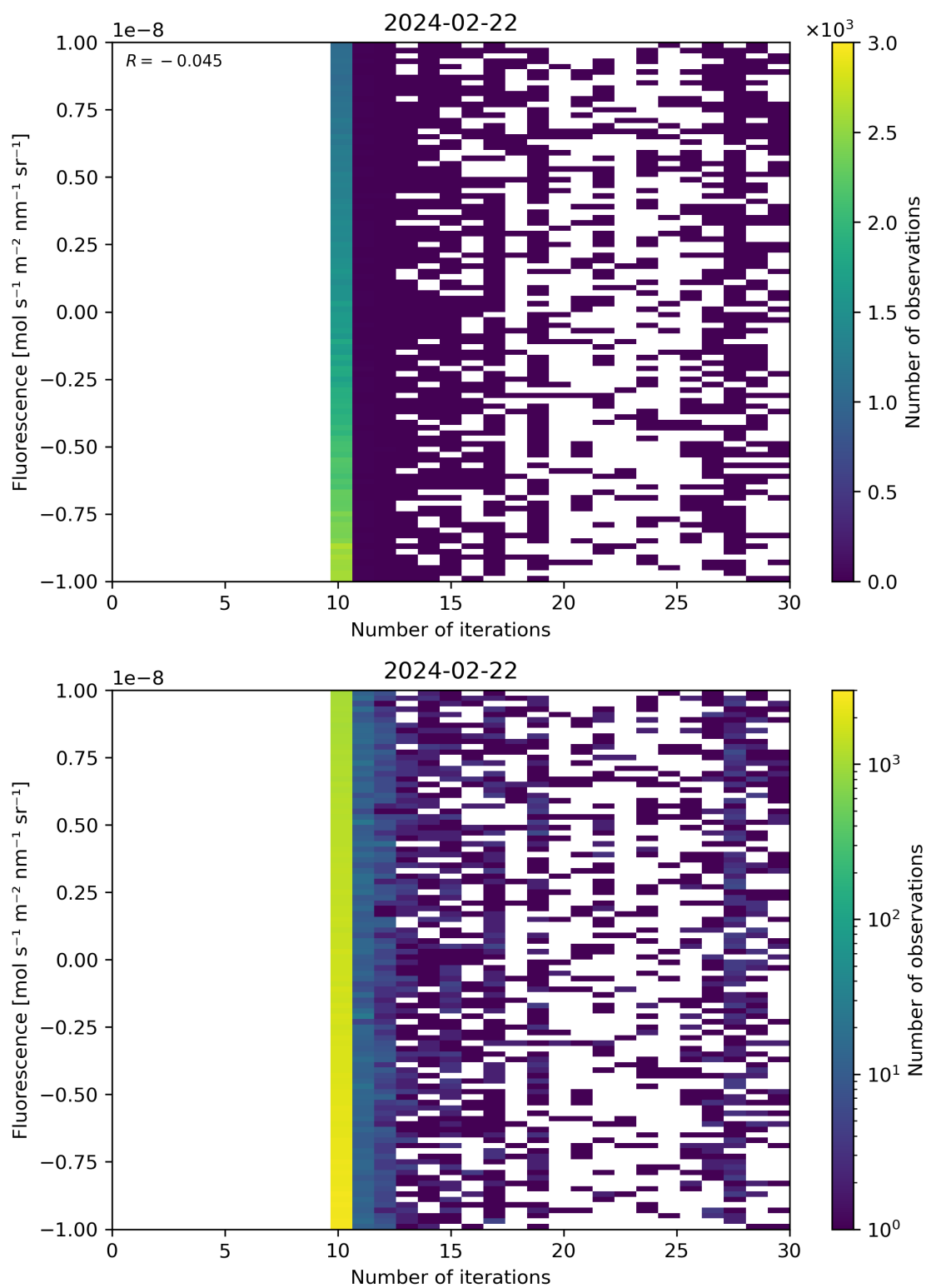
Figure 87: Scatter density plot of “Number of iterations” against “Fluorescence” for 2024-02-22 to 2024-02-23.
