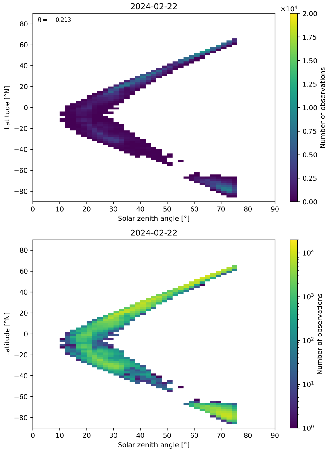
Figure 98: Scatter density plot of “Solar zenith angle” against “Latitude” for 2024-02-22 to 2024-02-23.
