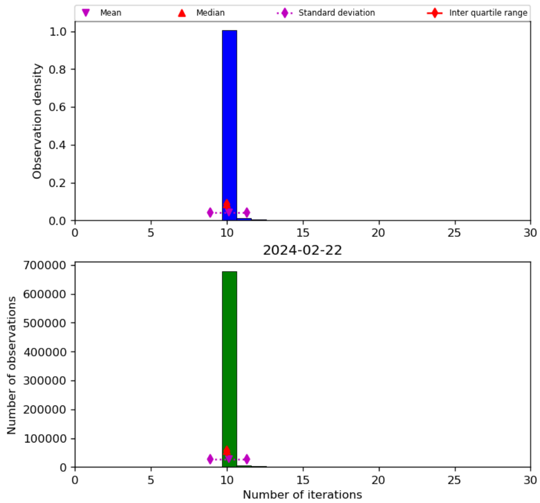
Figure 31: Histogram of “Number of iterations” for 2024-02-22 to 2024-02-23
