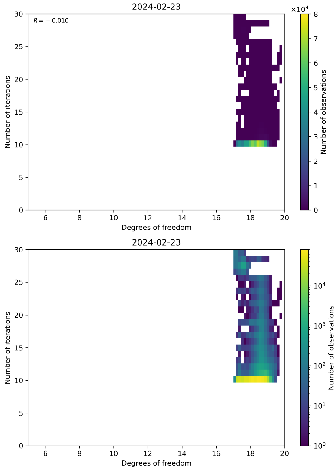
Figure 52: Scatter density plot of “Degrees of freedom” against “Number of iterations” for 2024-02-22 to 2024-02-24.
