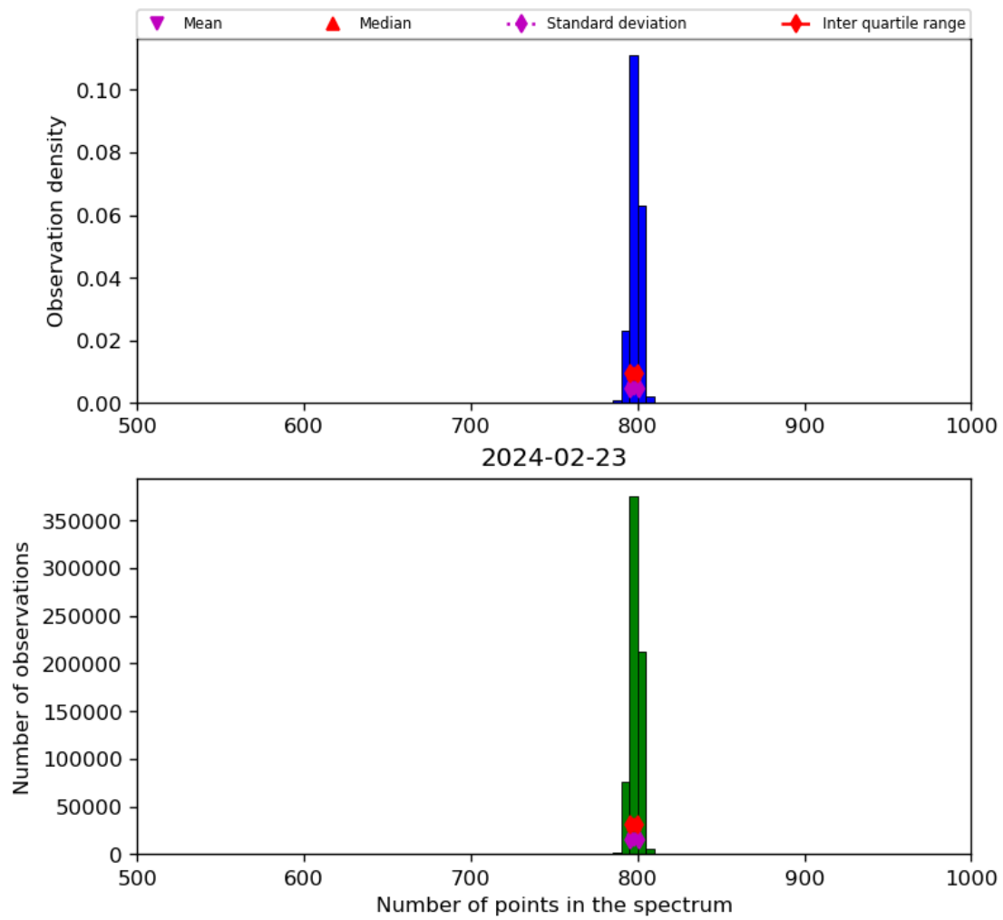
Figure 26: Histogram of “Number of points in the spectrum” for 2024-02-22 to 2024-02-24
