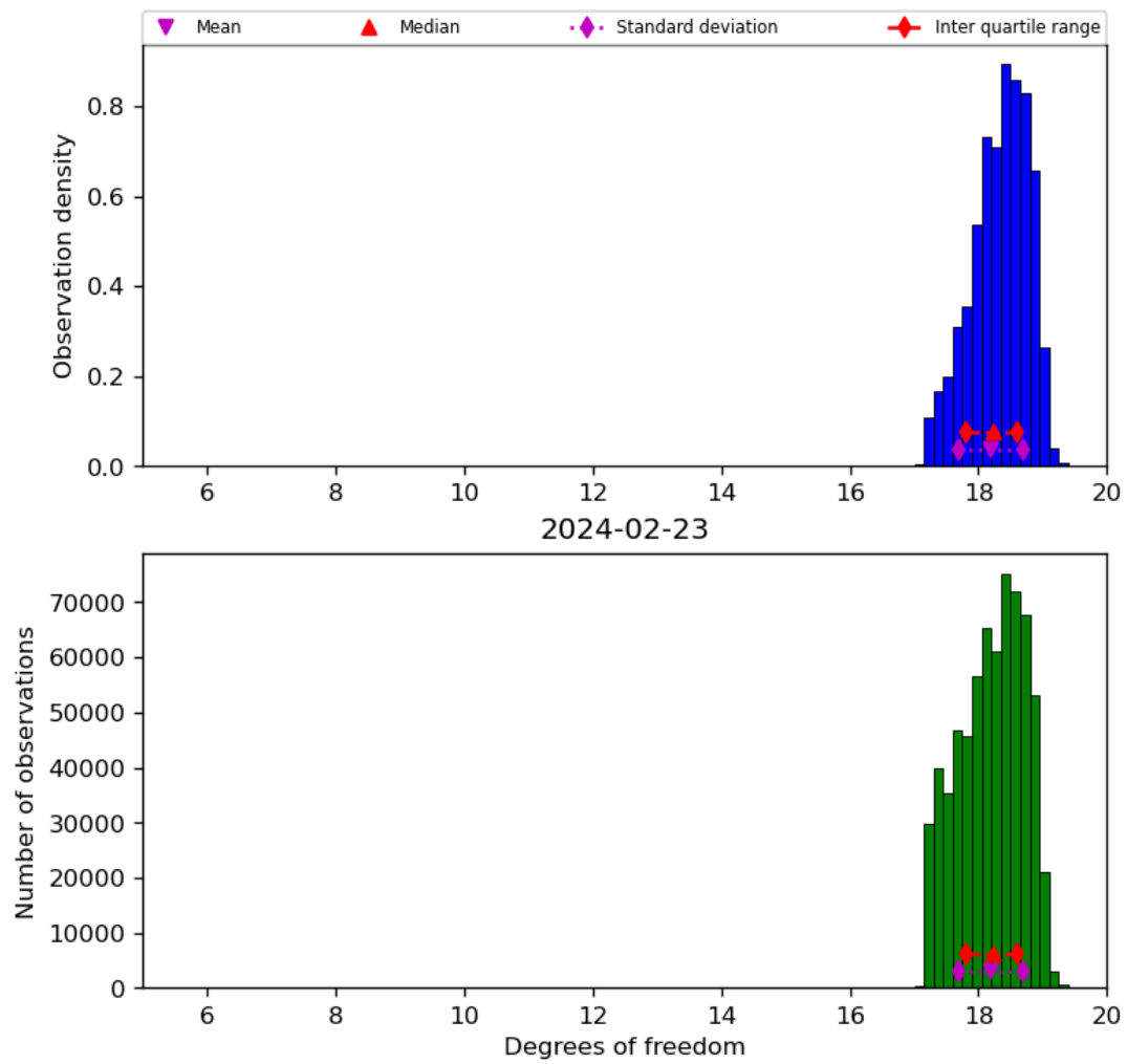
Figure 30: Histogram of “Degrees of freedom” for 2024-02-22 to 2024-02-24
