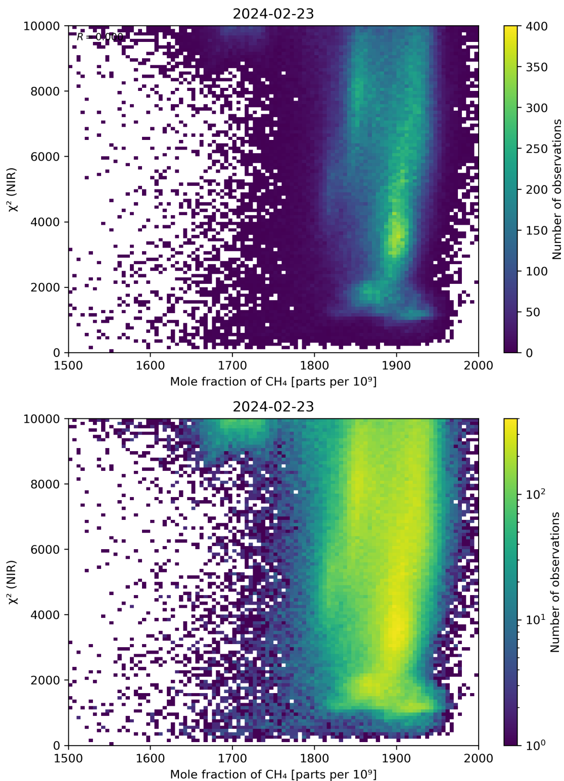
Figure 70: Scatter density plot of “Mole fraction of CH 4 ” against “ \chi^2 (NIR)” for 2024-02-22 to 2024-02-24.
