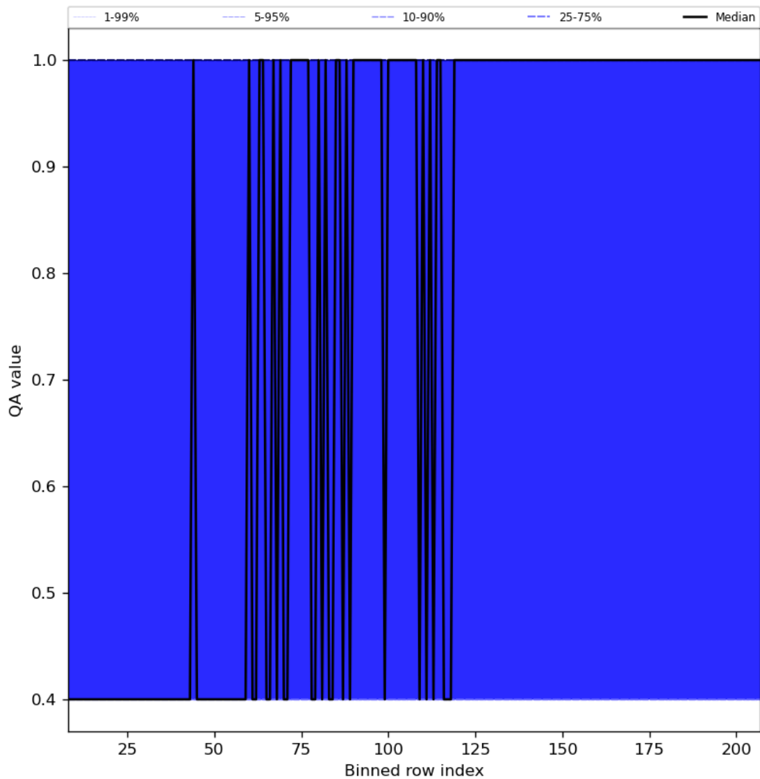
Figure 33: Along track statistics of “QA value” for 2024-02-22 to 2024-02-24
