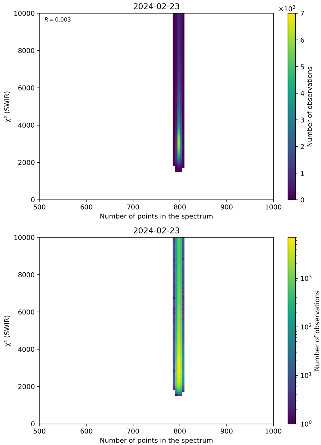
Figure 89: Scatter density plot of “Number of points in the spectrum” against “ \chi^2 (SWIR)” for 2024-02-22 to 2024-02-24.
