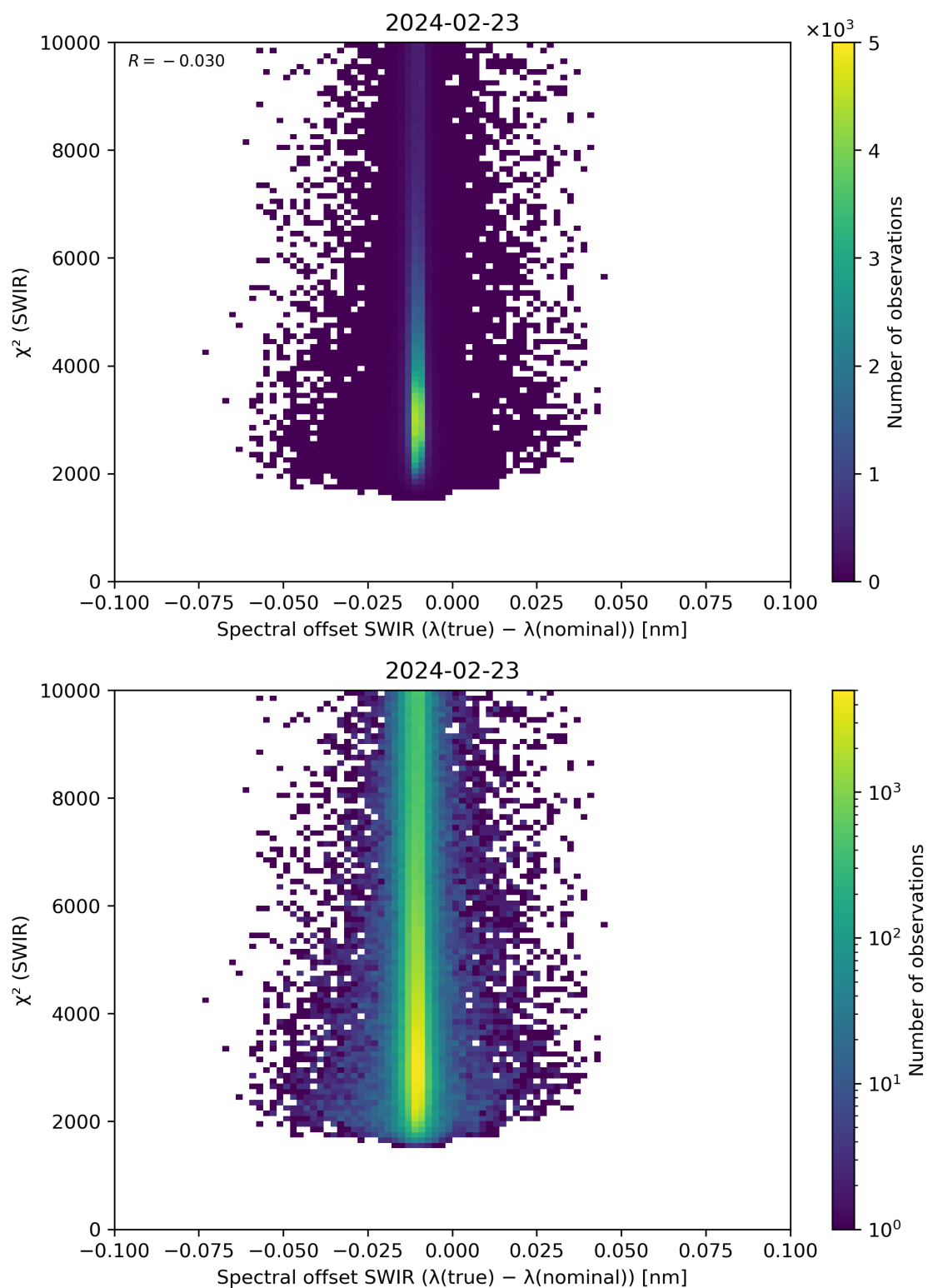
Figure 118: Scatter density plot of “Spectral offset SWIR ( \lambda(\text{true}) - \lambda(\text{nominal}) )” against “ \chi^2 (SWIR)” for 2024-02-22 to 2024-02-24.
