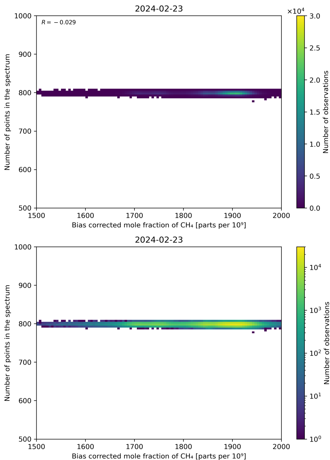
Figure 68: Scatter density plot of “Bias corrected mole fraction of CH 4 ” against “Number of points in the spectrum” for 2024-02-22 to 2024-02-24.
