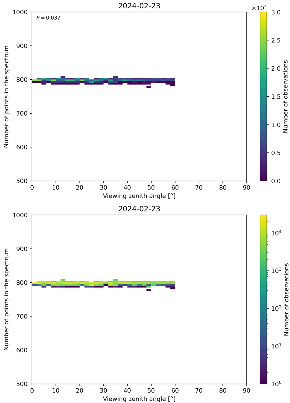
Figure 114: Scatter density plot of “Viewing zenith angle” against “Number of points in the spectrum” for 2024-02-22 to 2024-02-24.
