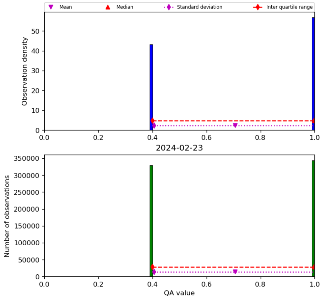
Figure 22: Histogram of “QA value” for 2024-02-22 to 2024-02-24
