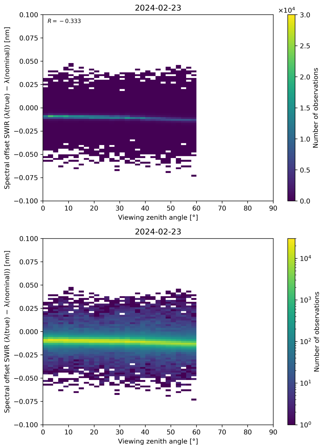
Figure 116: Scatter density plot of “Viewing zenith angle” against “Spectral offset SWIR ( \lambda(\text{true}) - \lambda(\text{nominal}) )” for 2024-02-22 to 2024-02-24.
