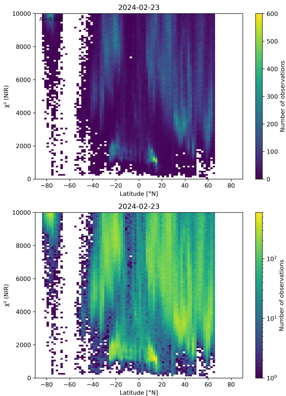
Figure 53: Scatter density plot of “Latitude” against “ \chi^2 (NIR)” for 2024-02-22 to 2024-02-24.
