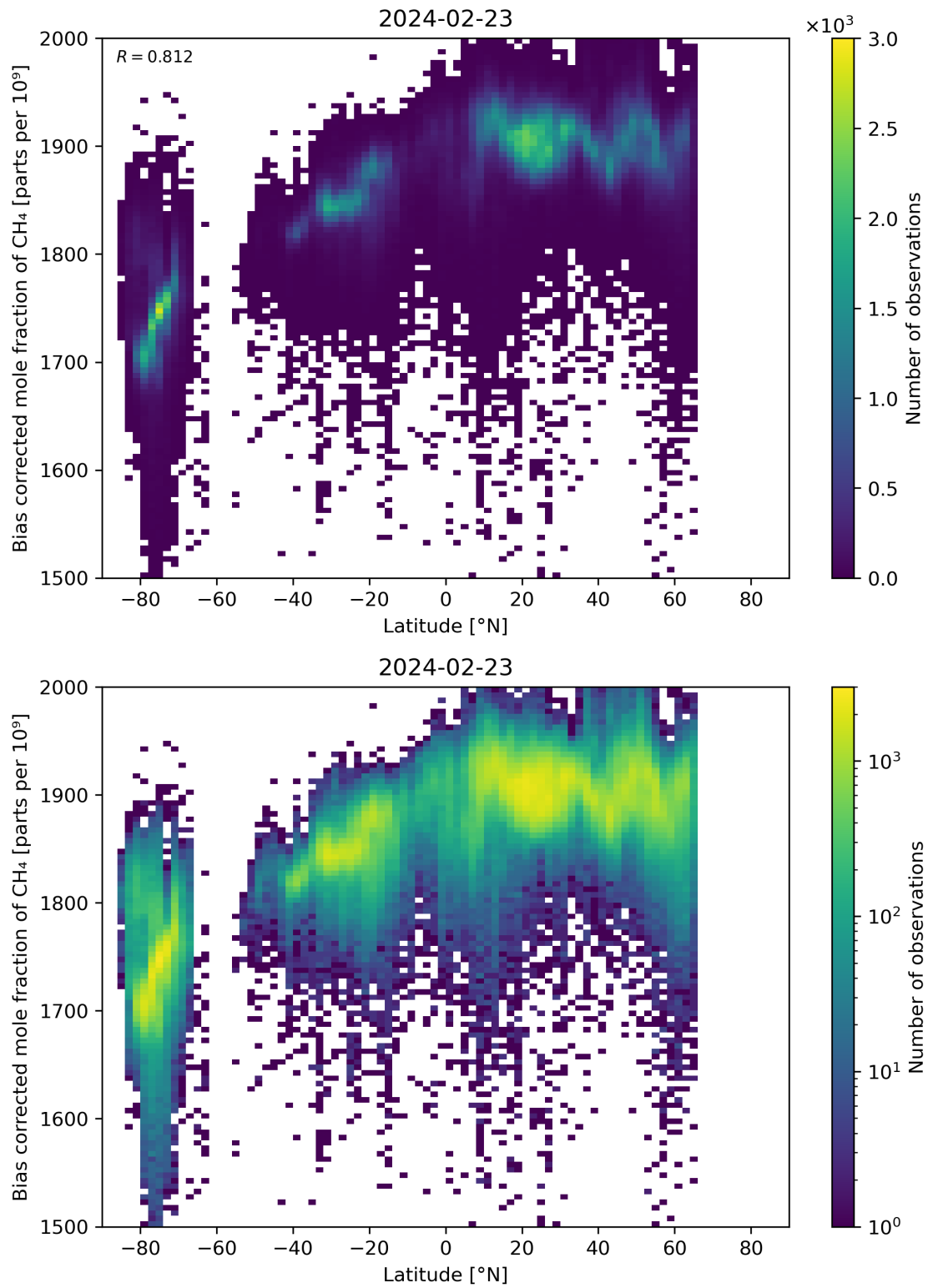
Figure 58: Scatter density plot of “Latitude” against “Bias corrected mole fraction of \text{CH}_4 ” for 2024-02-22 to 2024-02-24.
