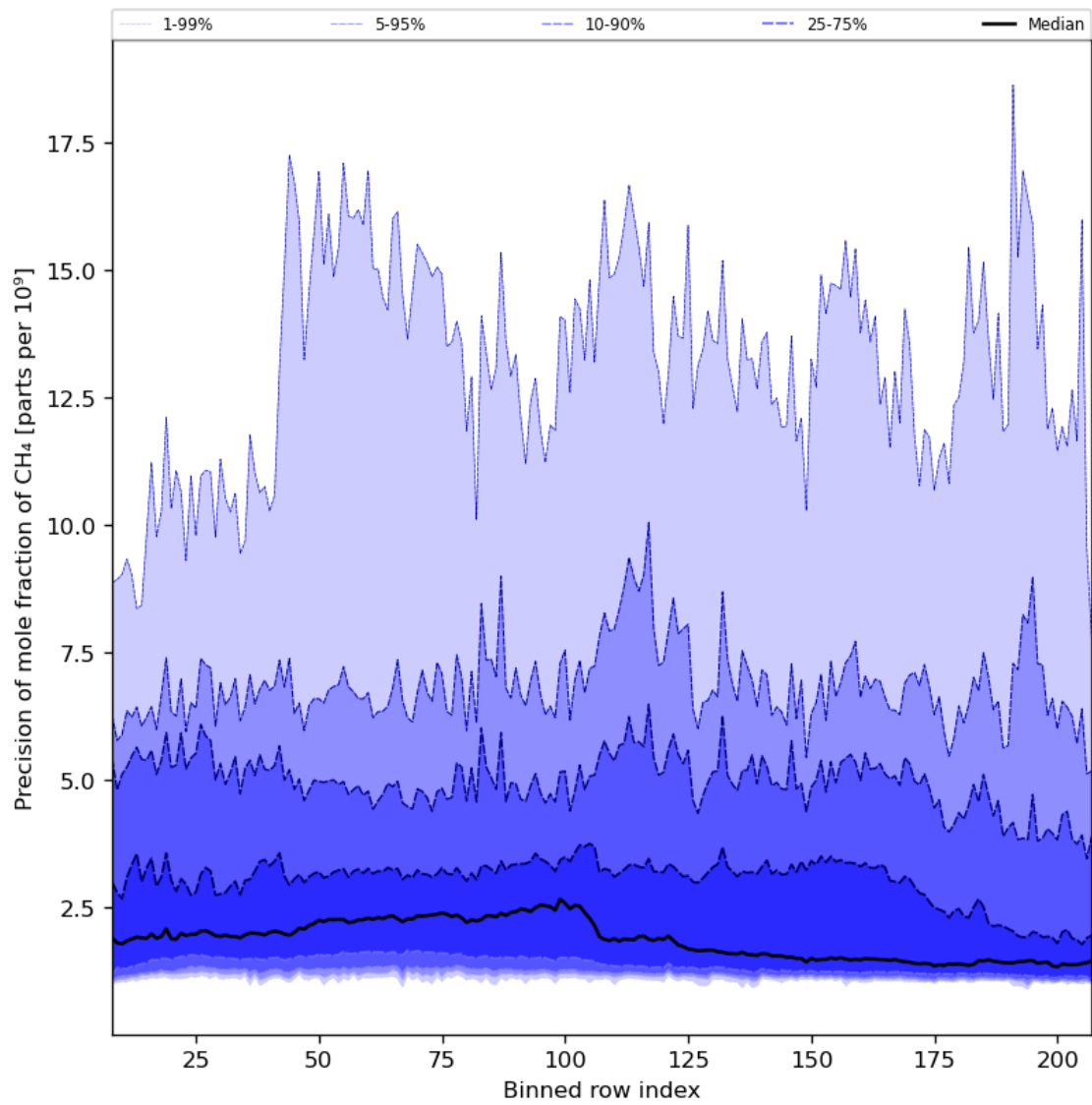
Figure 35: Along track statistics of “Precision of mole fraction of CH 4 ” for 2024-02-22 to 2024-02-24
