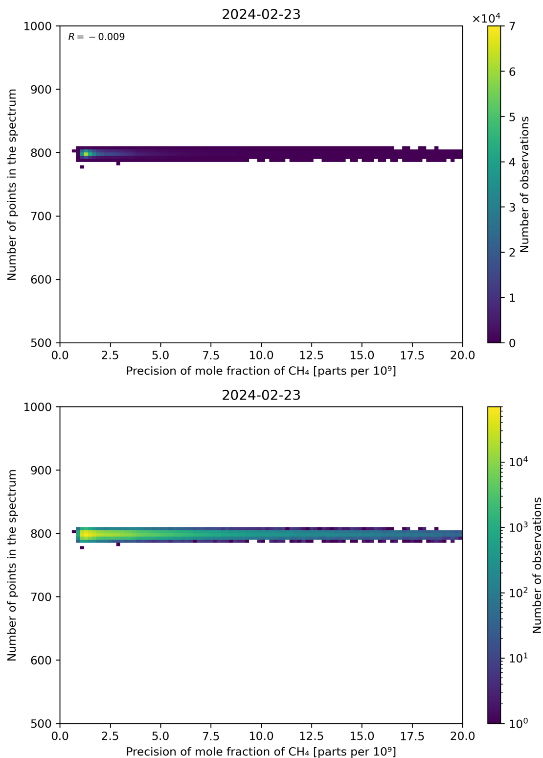
Figure 84: Scatter density plot of “Precision of mole fraction of CH 4 ” against “Number of points in the spectrum” for 2024-02-22 to 2024-02-24.
