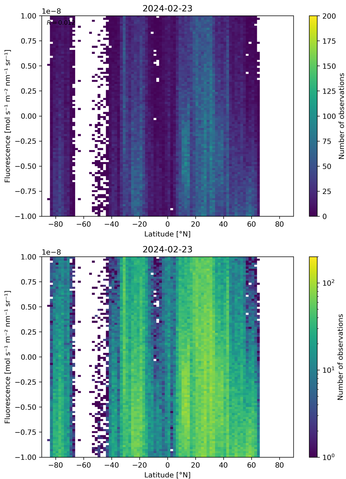
Figure 56: Scatter density plot of “Latitude” against “Fluorescence” for 2024-02-22 to 2024-02-24.
