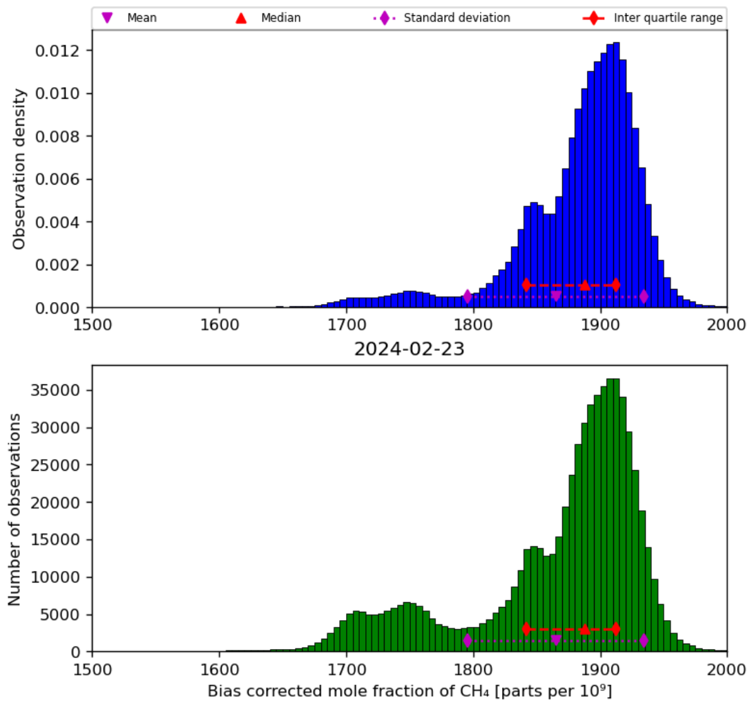
Figure 25: Histogram of “Bias corrected mole fraction of CH 4 ” for 2024-02-22 to 2024-02-24
