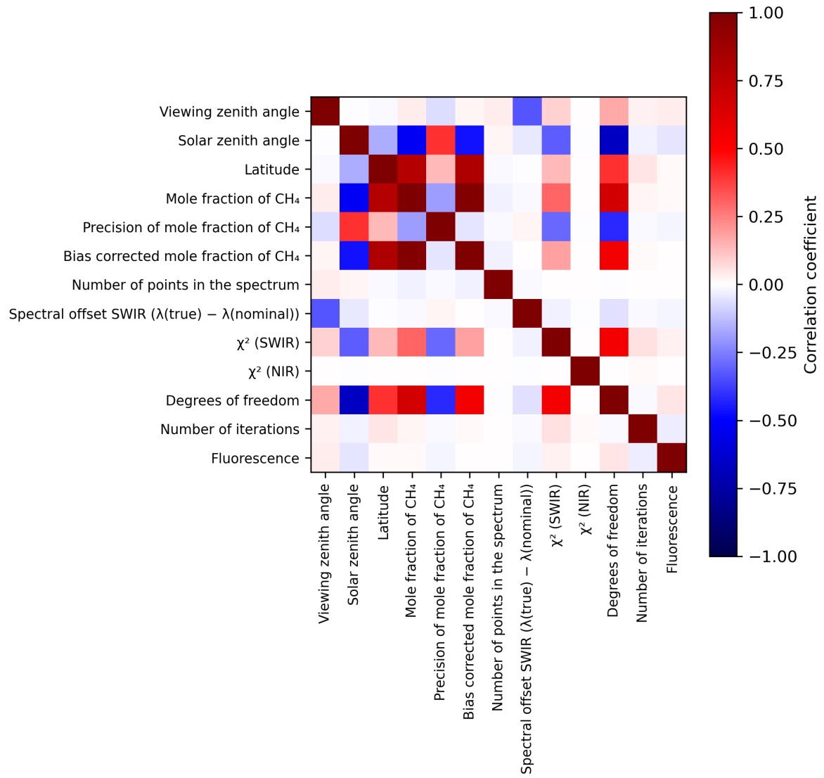
Figure 2: Map of correlation matrix for 2024-02-22 to 2024-02-24.
