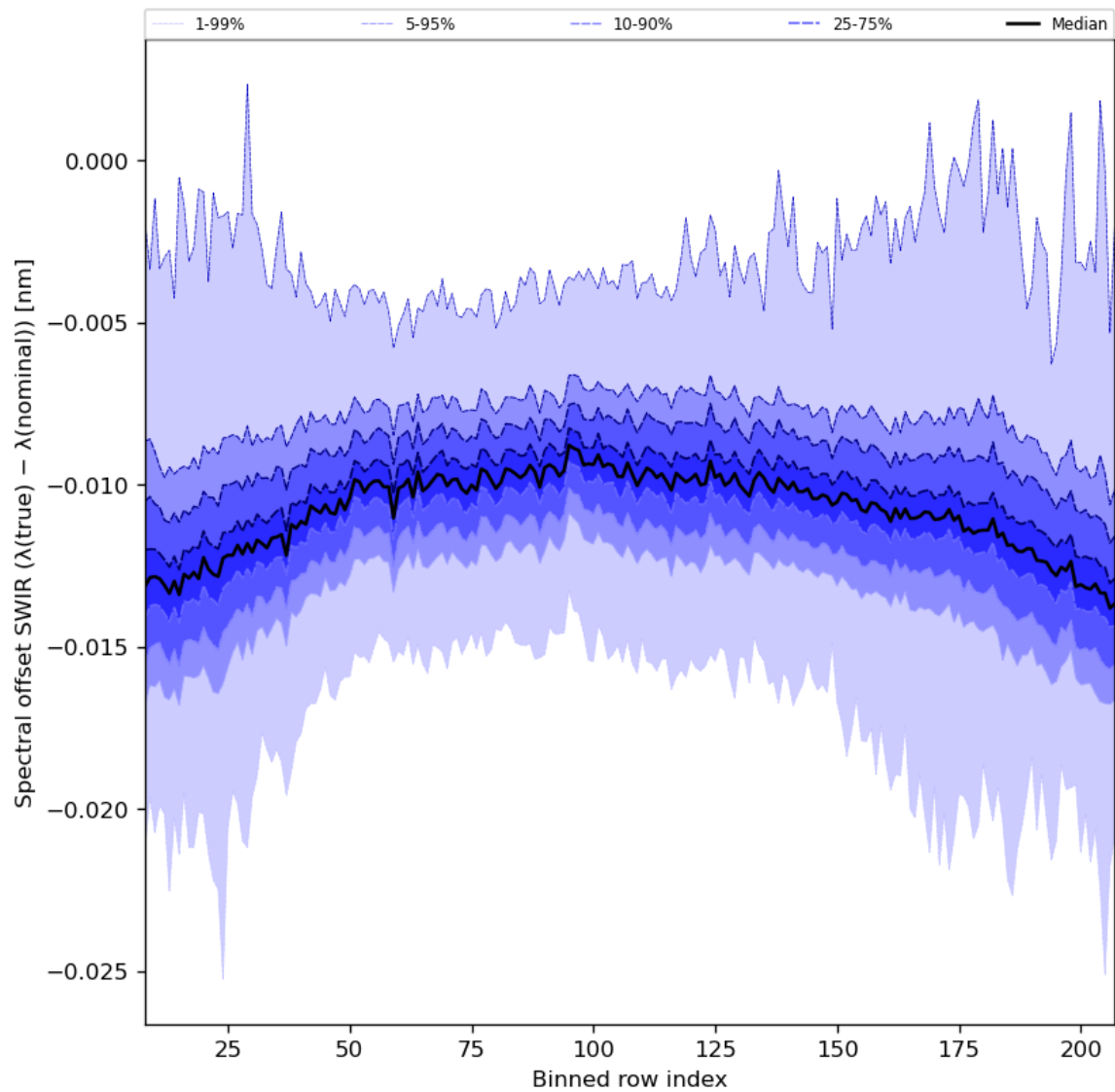
Figure 38: Along track statistics of “Spectral offset SWIR ( \lambda(\text{true}) - \lambda(\text{nominal}) )” for 2024-02-22 to 2024-02-24
