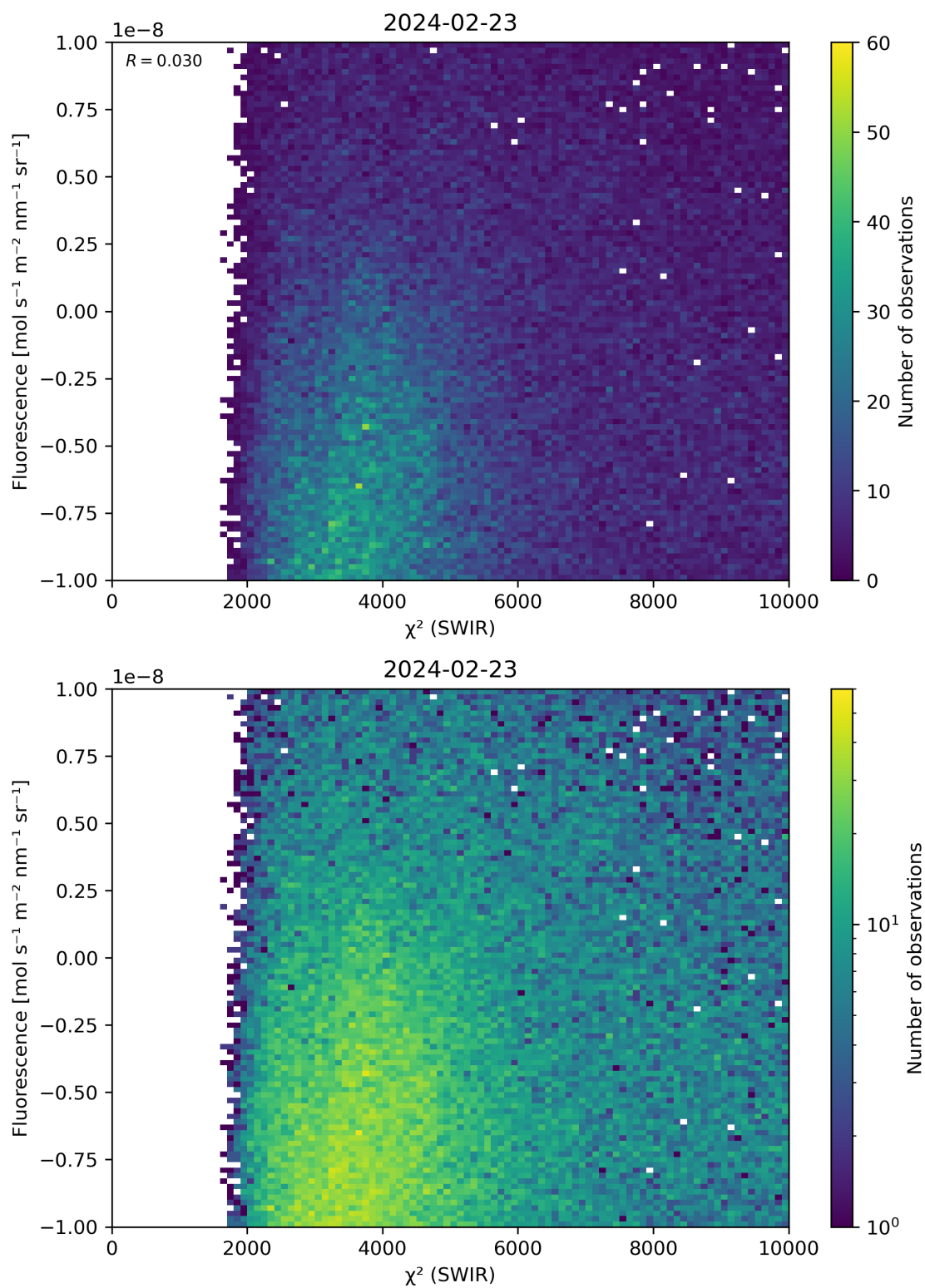
Figure 49: Scatter density plot of “ \chi^2 (SWIR)” against “Fluorescence” for 2024-02-22 to 2024-02-24.
