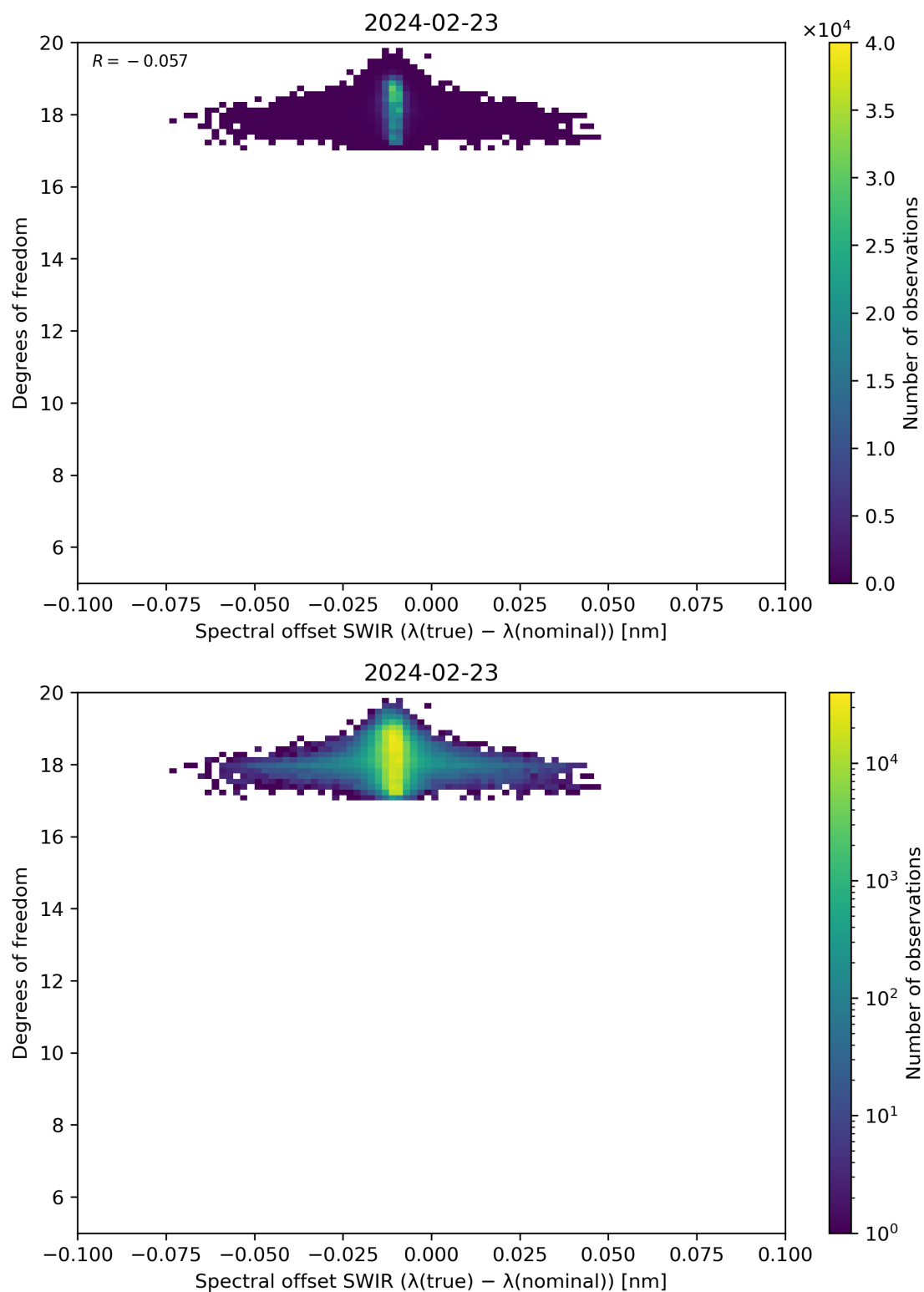
Figure 119: Scatter density plot of “Spectral offset SWIR ( \lambda(\text{true}) - \lambda(\text{nominal}) )” against “Degrees of freedom” for 2024-02-22 to 2024-02-24.
