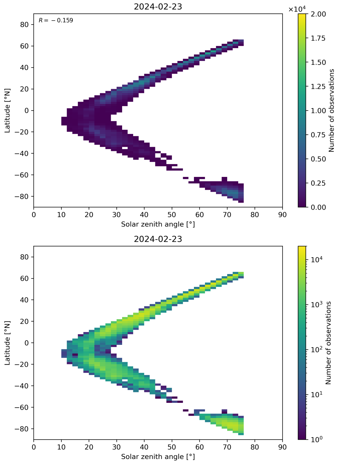
Figure 98: Scatter density plot of “Solar zenith angle” against “Latitude” for 2024-02-22 to 2024-02-24.
