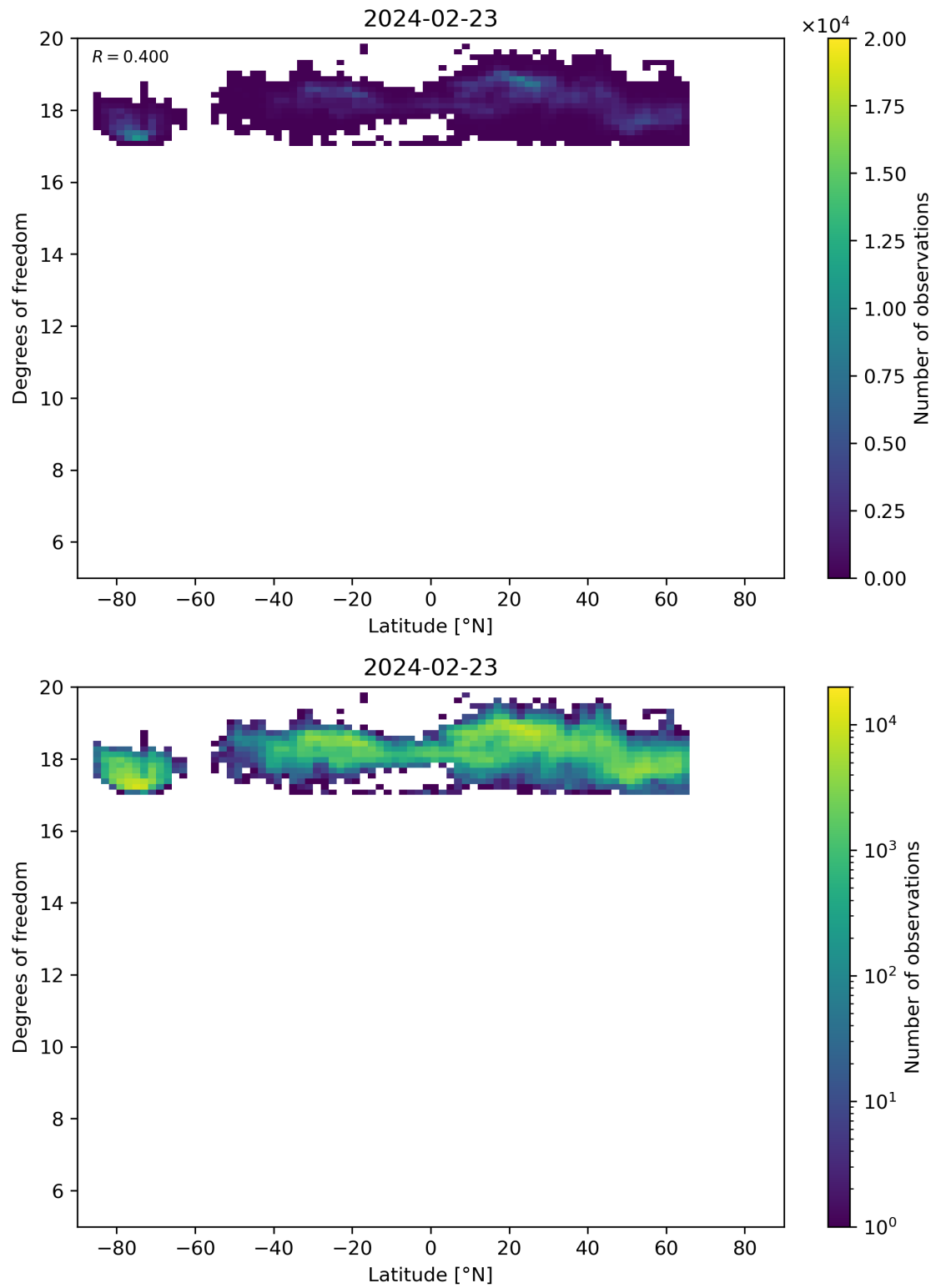
Figure 55: Scatter density plot of “Latitude” against “Degrees of freedom” for 2024-02-22 to 2024-02-24.
