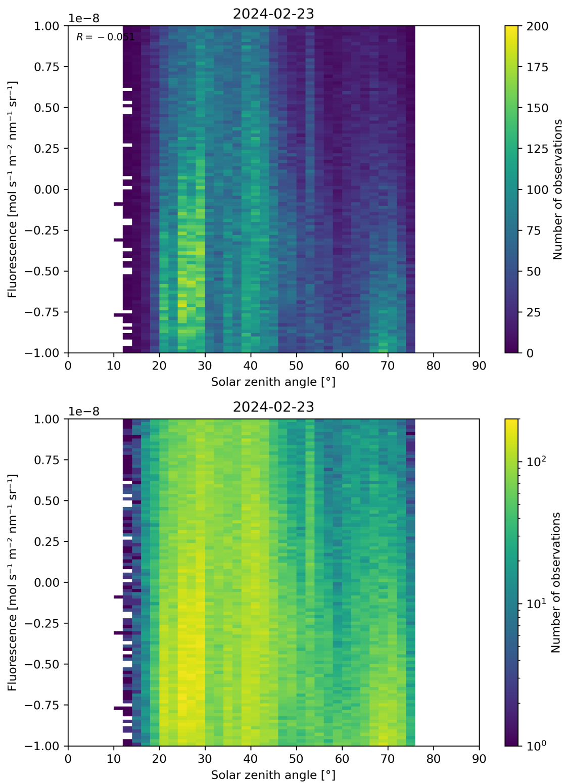
Figure 97: Scatter density plot of “Solar zenith angle” against “Fluorescence” for 2024-02-22 to 2024-02-24.
