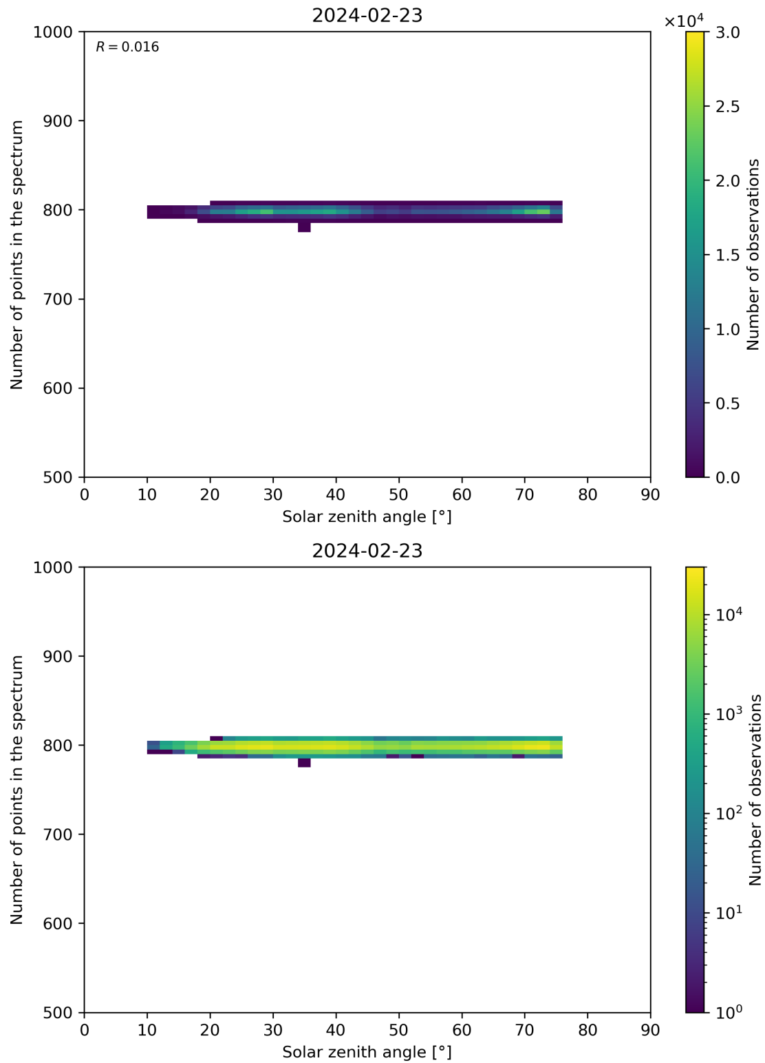
Figure 103: Scatter density plot of “Solar zenith angle” against “Number of points in the spectrum” for 2024-02-22 to 2024-02-24.
