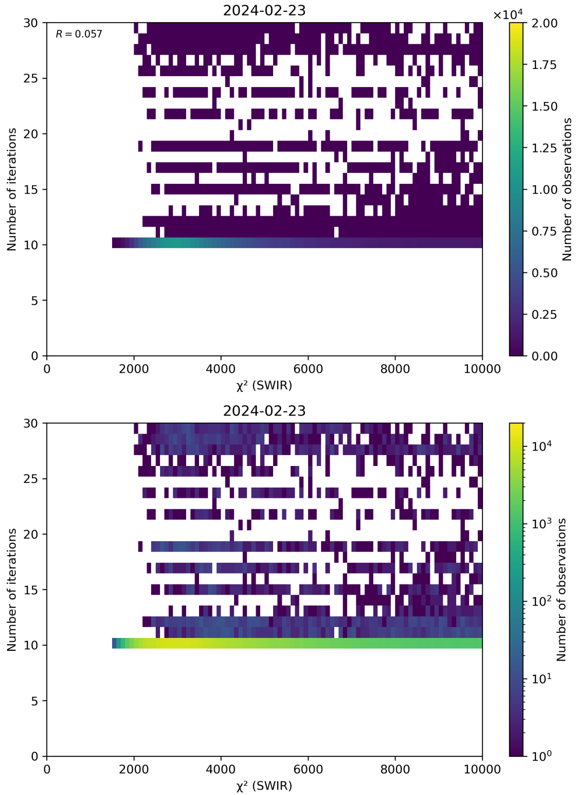
Figure 50: Scatter density plot of “ \chi^2 (SWIR)” against “Number of iterations” for 2024-02-22 to 2024-02-24.
