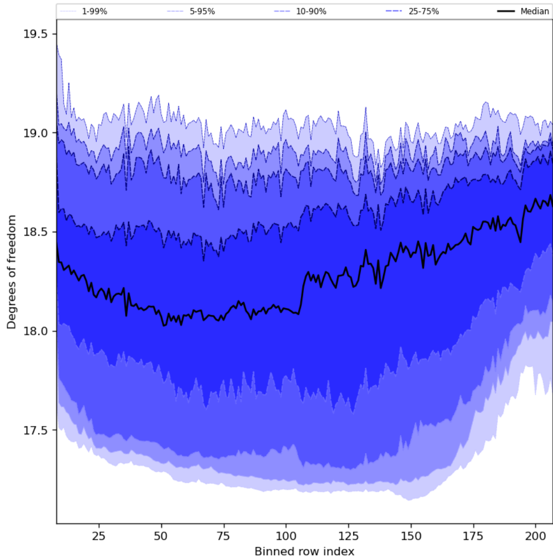
Figure 41: Along track statistics of “Degrees of freedom” for 2024-02-22 to 2024-02-24
