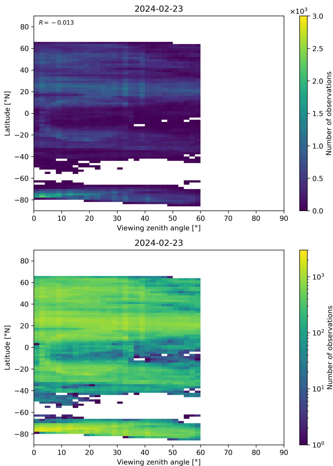
Figure 109: Scatter density plot of “Viewing zenith angle” against “Latitude” for 2024-02-22 to 2024-02-24.
