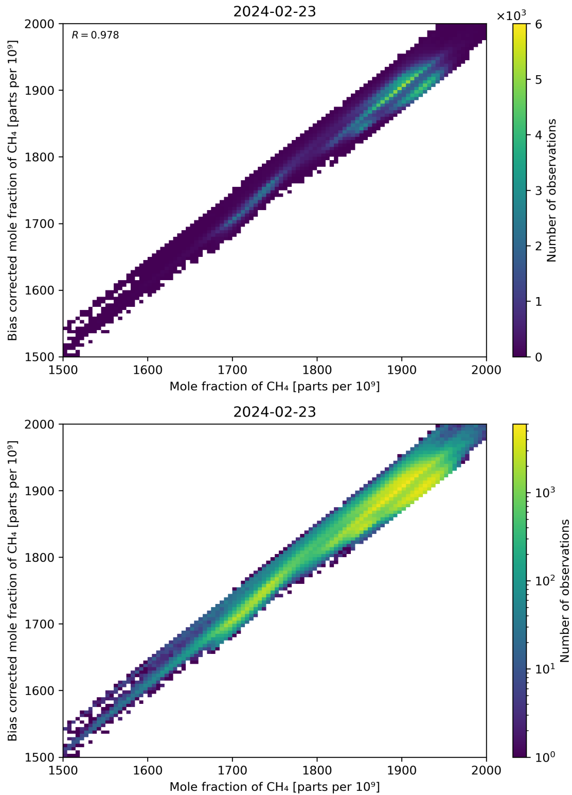
Figure 74: Scatter density plot of “Mole fraction of CH 4 ” against “Bias corrected mole fraction of CH 4 ” for 2024-02-22 to 2024-02-24.
