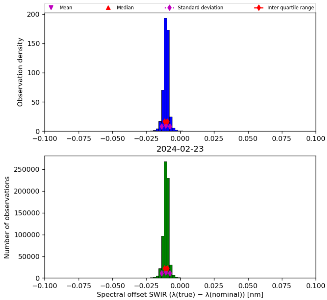
Figure 27: Histogram of “Spectral offset SWIR ( \lambda(\text{true}) - \lambda(\text{nominal}) )” for 2024-02-22 to 2024-02-24
