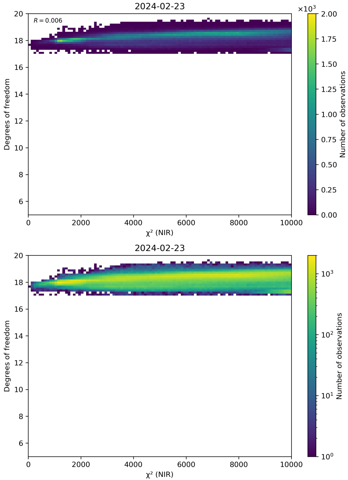
Figure 44: Scatter density plot of “ \chi^2 (NIR)” against “Degrees of freedom” for 2024-02-22 to 2024-02-24.
