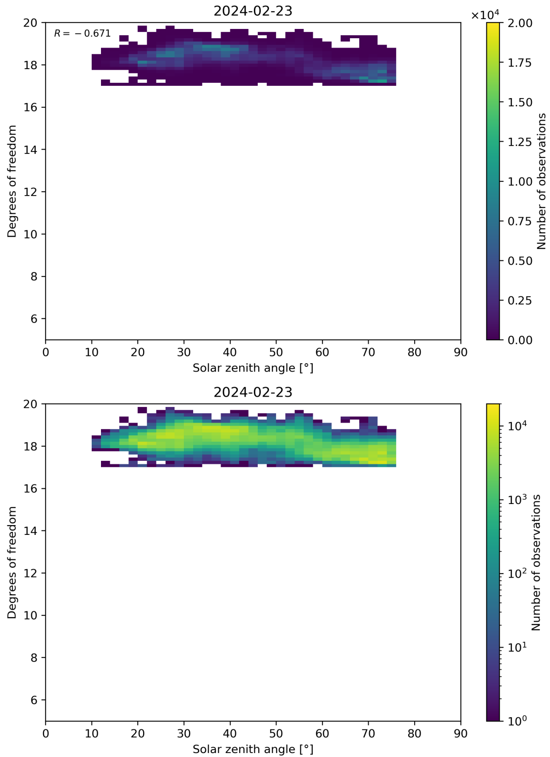
Figure 96: Scatter density plot of “Solar zenith angle” against “Degrees of freedom” for 2024-02-22 to 2024-02-24.
