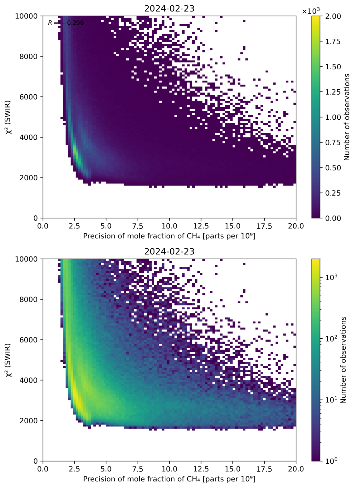
Figure 79: Scatter density plot of “Precision of mole fraction of \text{CH}_4 ” against “ \chi^2 (SWIR)” for 2024-02-22 to 2024-02-24.
