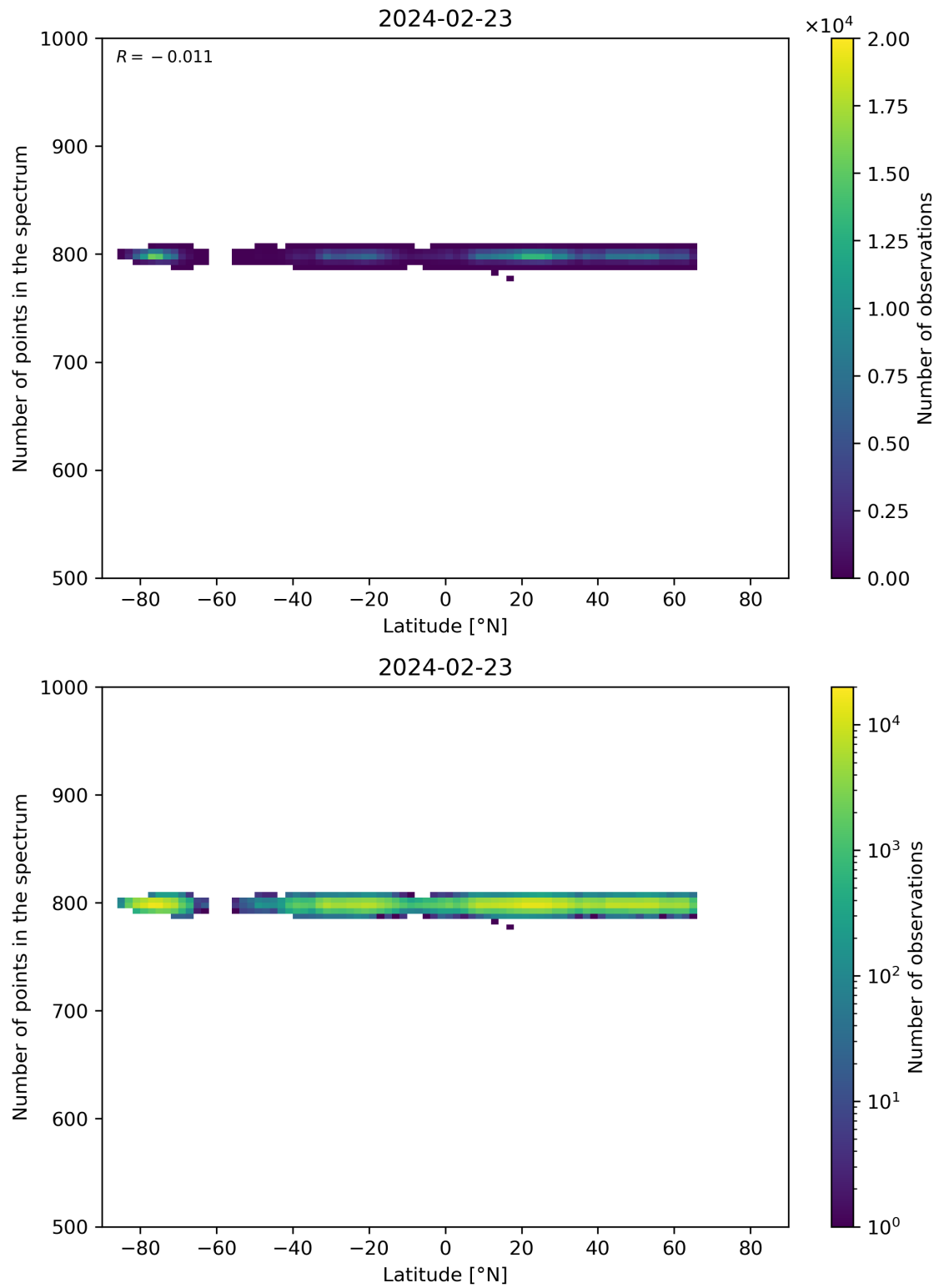
Figure 61: Scatter density plot of “Latitude” against “Number of points in the spectrum” for 2024-02-22 to 2024-02-24.
