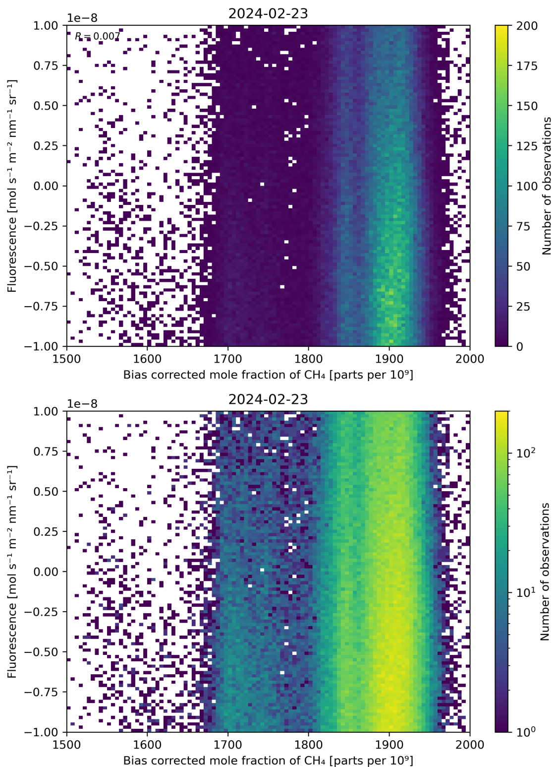
Figure 66: Scatter density plot of “Bias corrected mole fraction of \text{CH}_4 ” against “Fluorescence” for 2024-02-22 to 2024-02-24.
