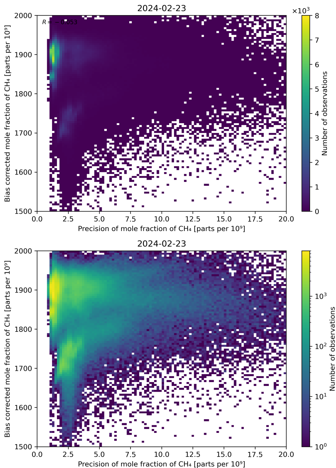
Figure 82: Scatter density plot of “Precision of mole fraction of \text{CH}_4 ” against “Bias corrected mole fraction of \text{CH}_4 ” for 2024-02-22 to 2024-02-24.
