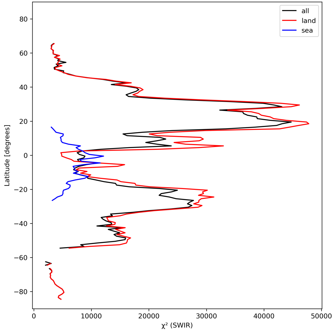
Figure 17: Zonal average of “ \chi^2 (SWIR)” for 2024-02-22 to 2024-02-24.
