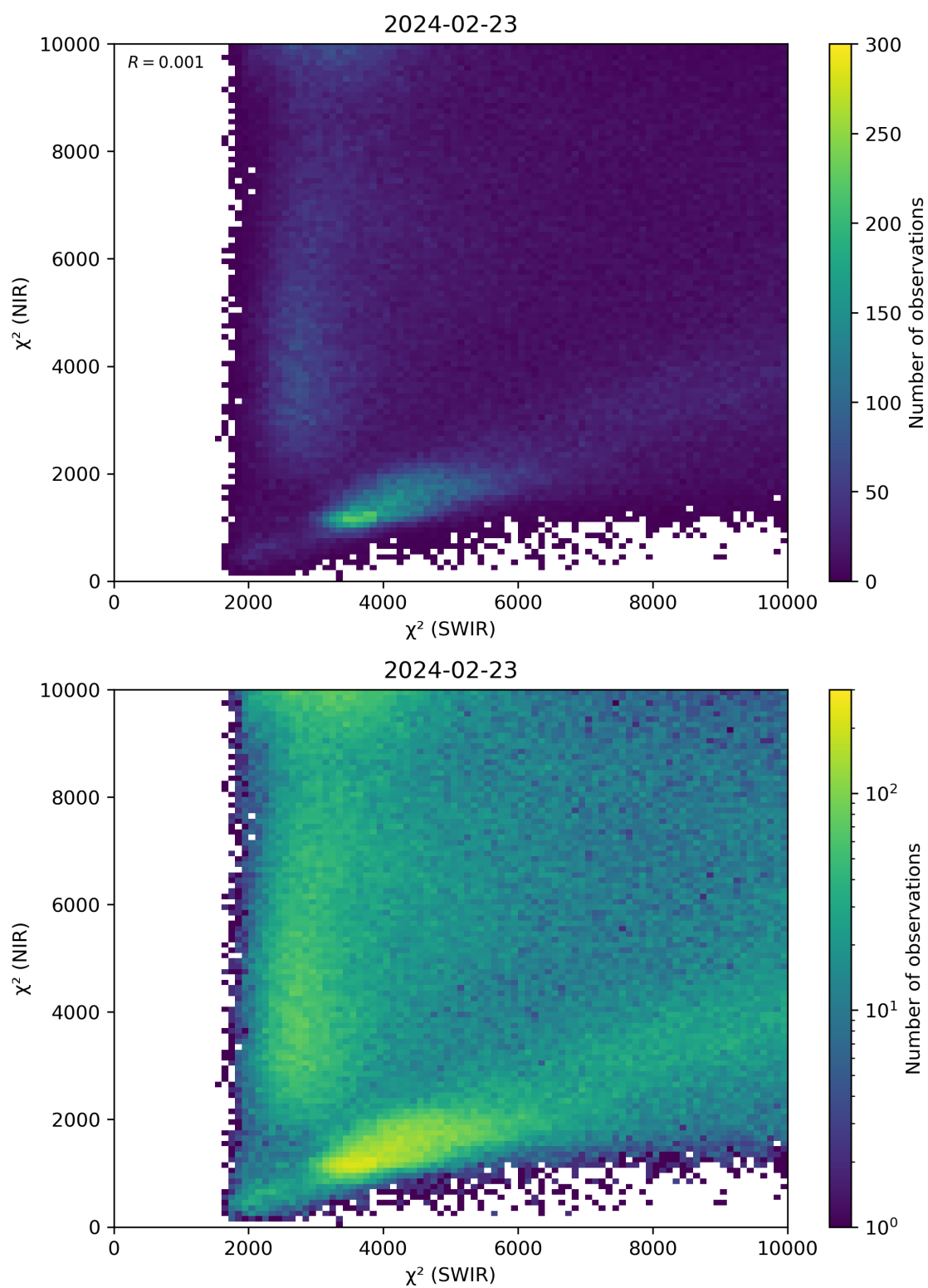
Figure 47: Scatter density plot of “ \chi^2 (SWIR)” against “ \chi^2 (NIR)” for 2024-02-22 to 2024-02-24.
