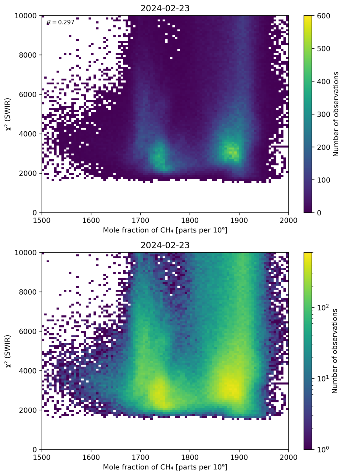
Figure 71: Scatter density plot of “Mole fraction of \text{CH}_4 ” against “ \chi^2 (SWIR)” for 2024-02-22 to 2024-02-24.
