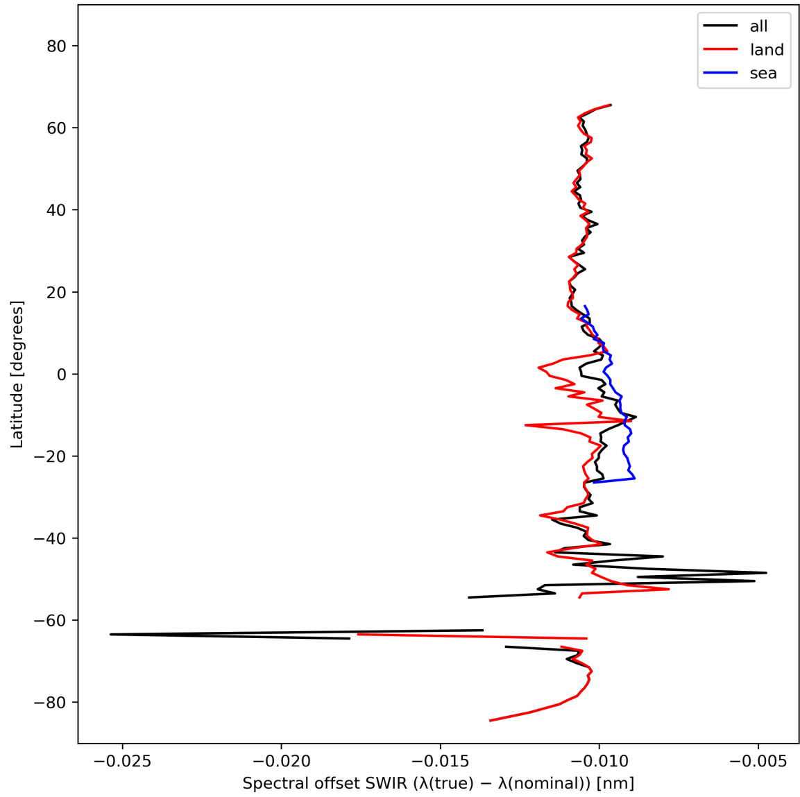
Figure 16: Zonal average of “Spectral offset SWIR ( \lambda(\text{true}) - \lambda(\text{nominal}) )” for 2024-02-22 to 2024-02-24.
