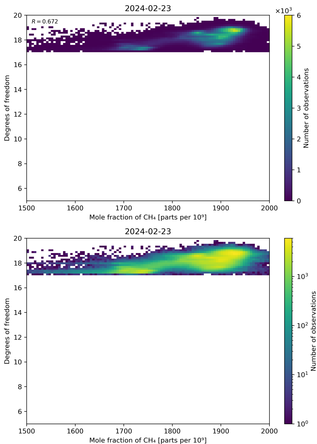
Figure 72: Scatter density plot of “Mole fraction of CH 4 ” against “Degrees of freedom” for 2024-02-22 to 2024-02-24.
