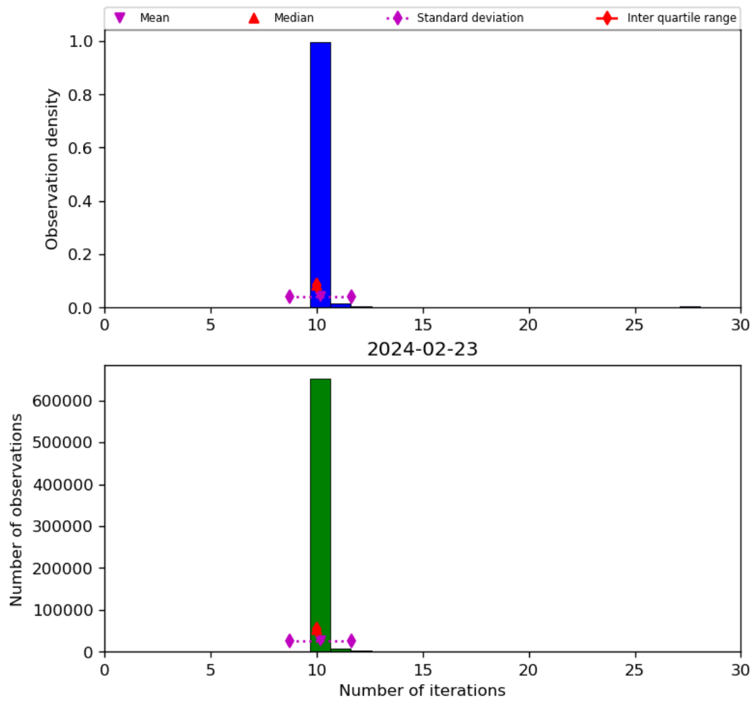
Figure 31: Histogram of “Number of iterations” for 2024-02-22 to 2024-02-24
