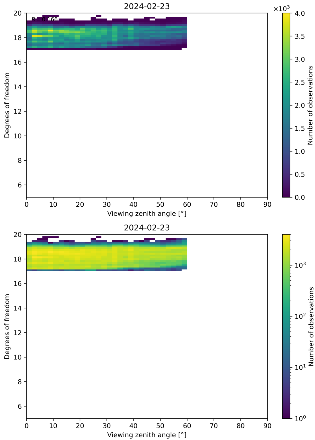
Figure 107: Scatter density plot of “Viewing zenith angle” against “Degrees of freedom” for 2024-02-22 to 2024-02-24.
