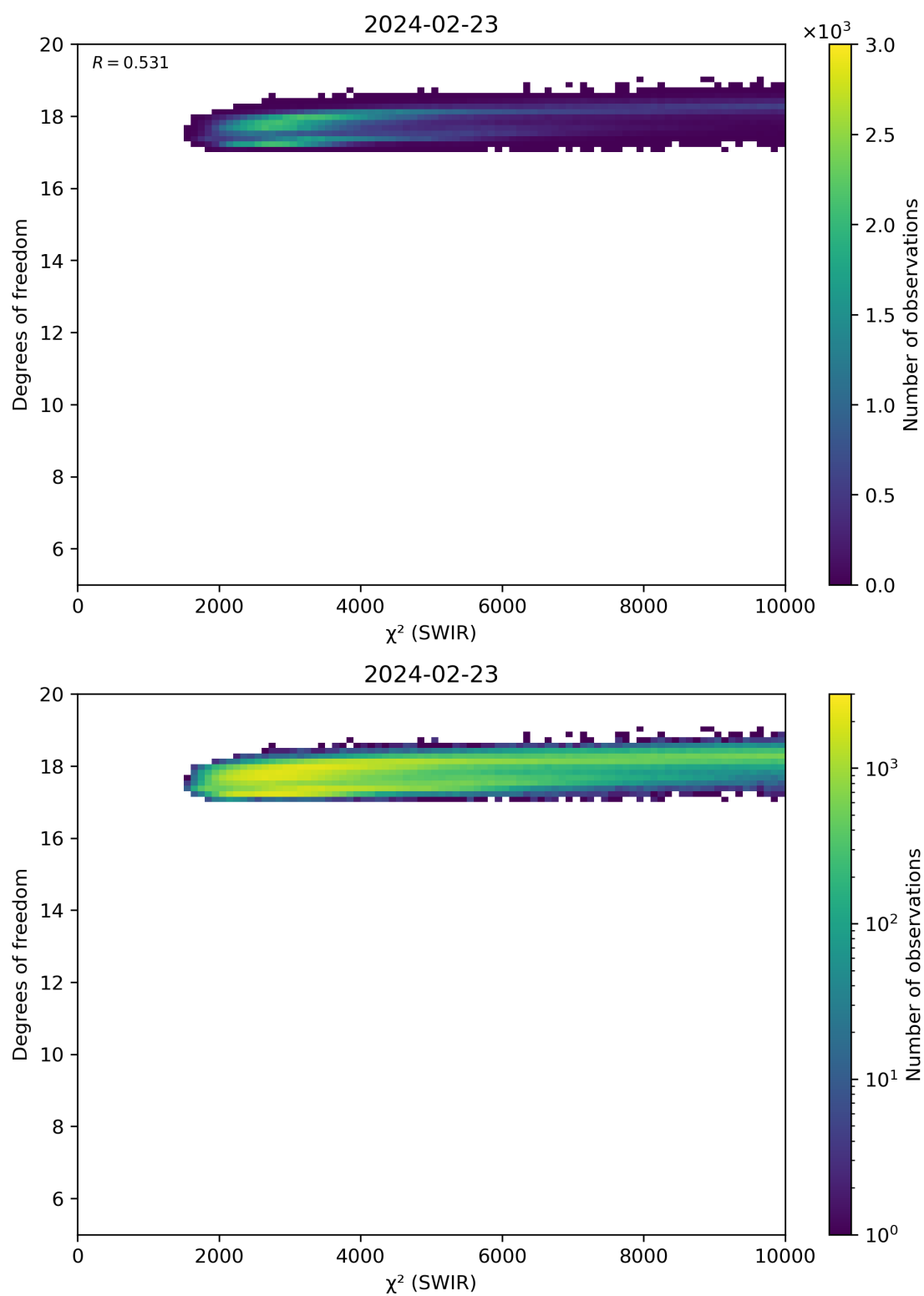
Figure 48: Scatter density plot of “ \chi^2 (SWIR)” against “Degrees of freedom” for 2024-02-22 to 2024-02-24.
