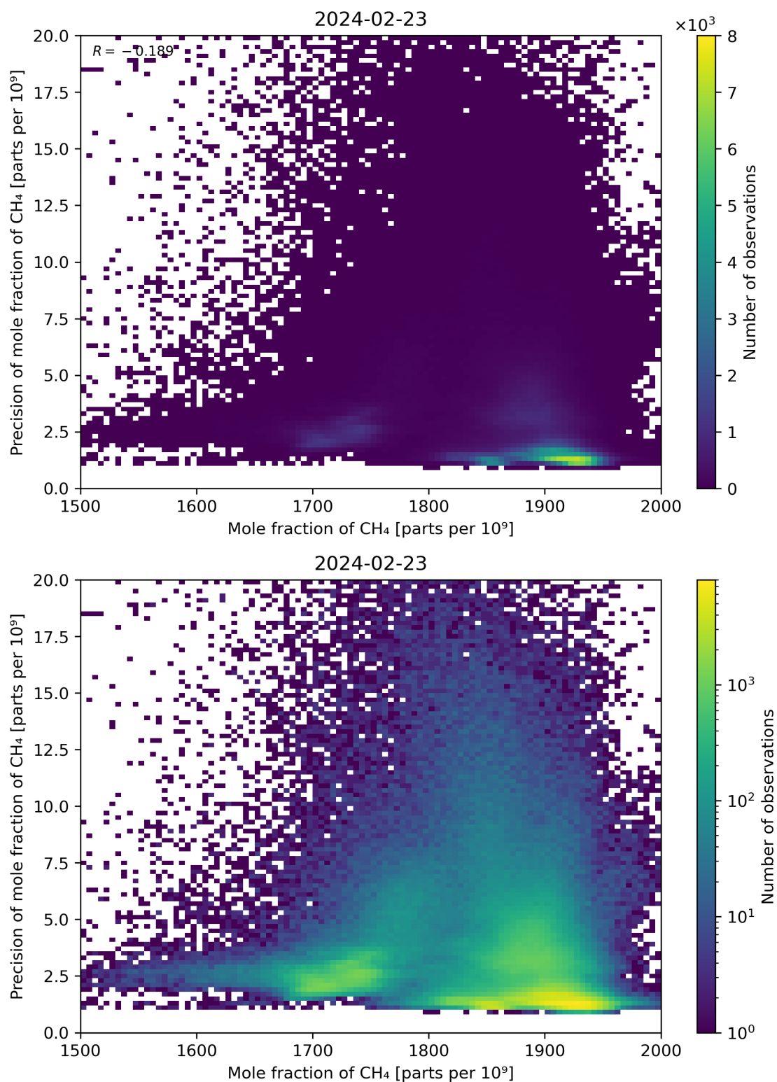
Figure 75: Scatter density plot of “Mole fraction of CH 4 ” against “Precision of mole fraction of CH 4 ” for 2024-02-22 to 2024-02-24.
