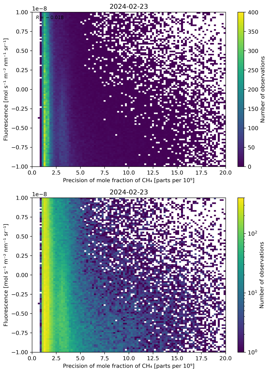
Figure 81: Scatter density plot of “Precision of mole fraction of \text{CH}_4 ” against “Fluorescence” for 2024-02-22 to 2024-02-24.
