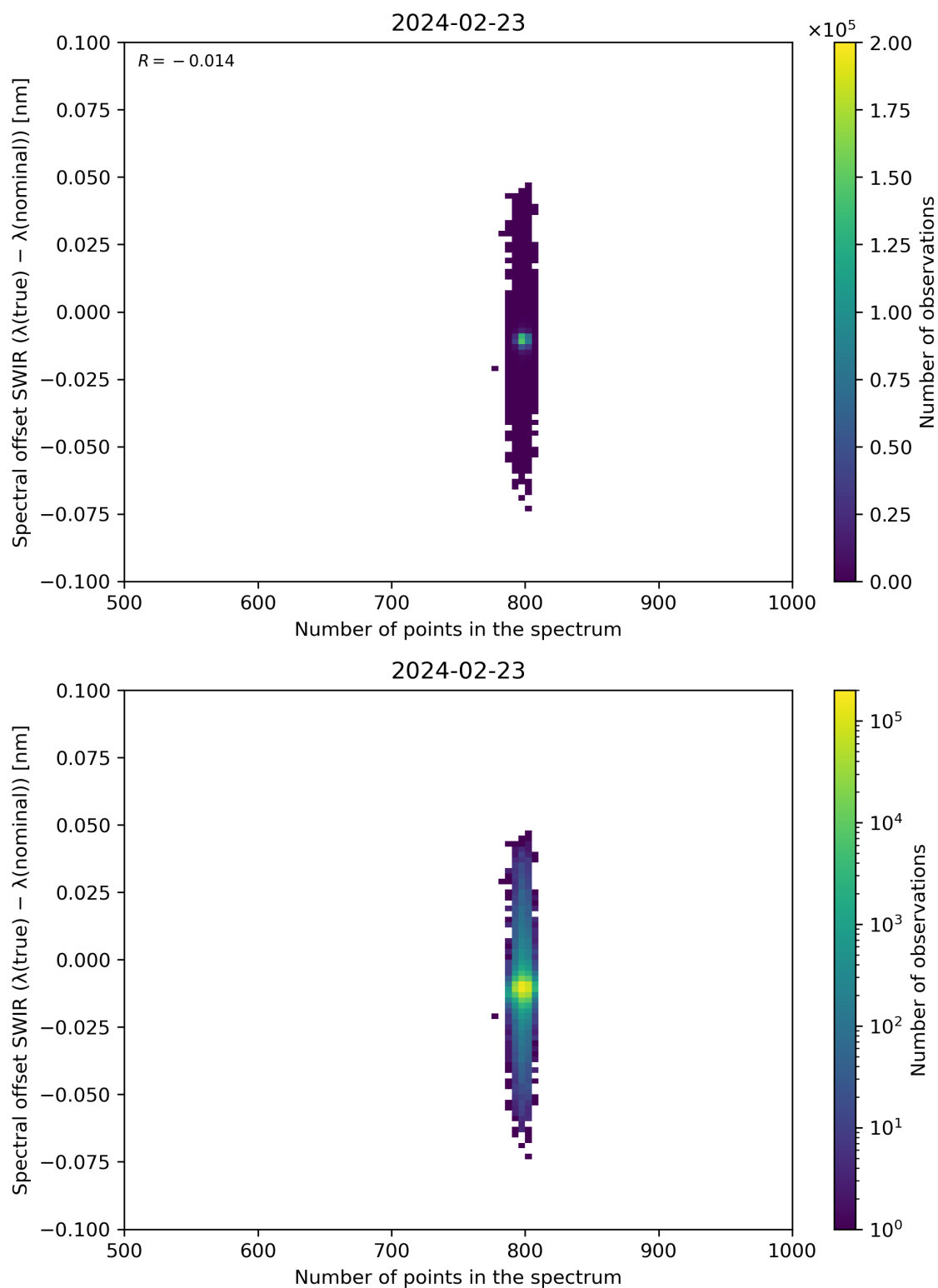
Figure 93: Scatter density plot of “Number of points in the spectrum” against “Spectral offset SWIR ( \lambda(\text{true}) - \lambda(\text{nominal}) )” for 2024-02-22 to 2024-02-24.
