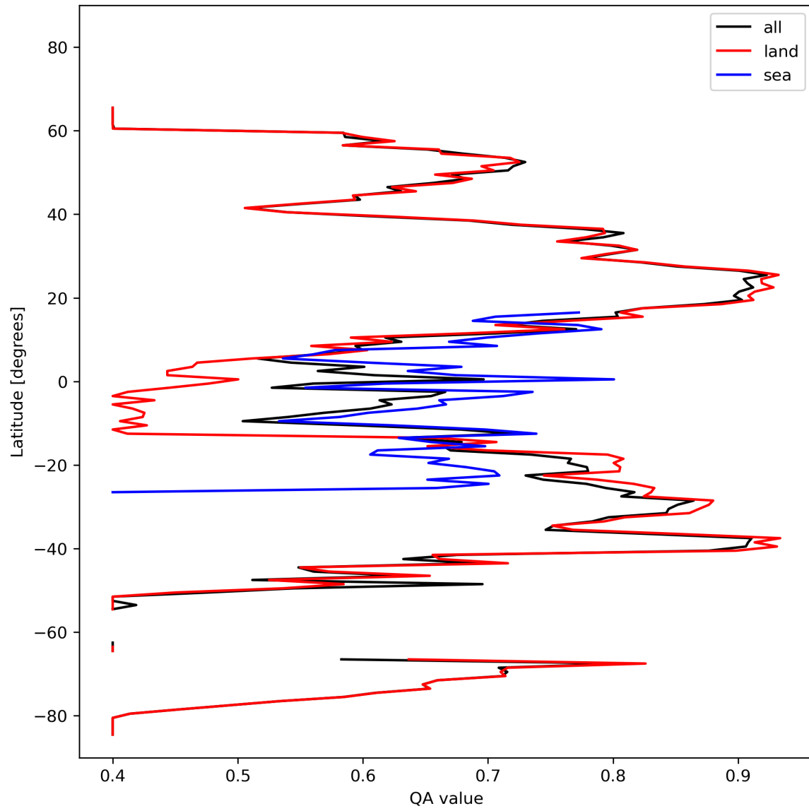
Figure 11: Zonal average of “QA value” for 2024-02-22 to 2024-02-24.
