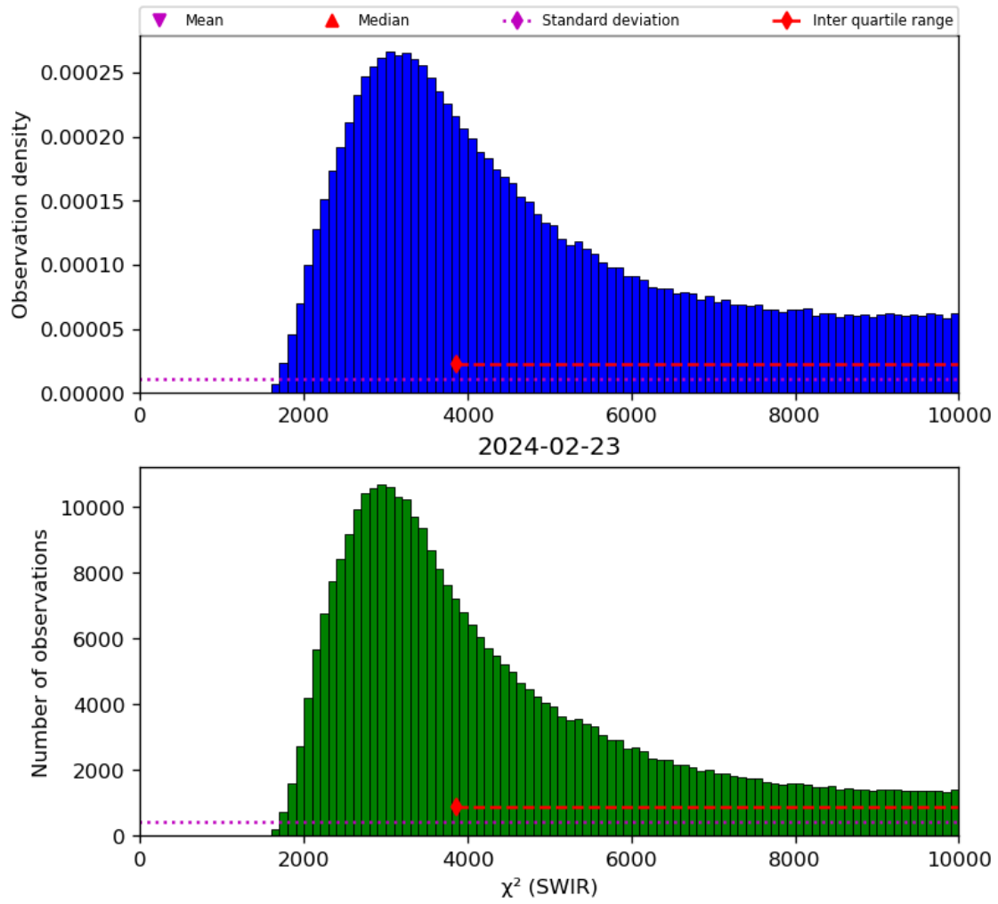
Figure 28: Histogram of “ \chi^2 (SWIR)” for 2024-02-22 to 2024-02-24
