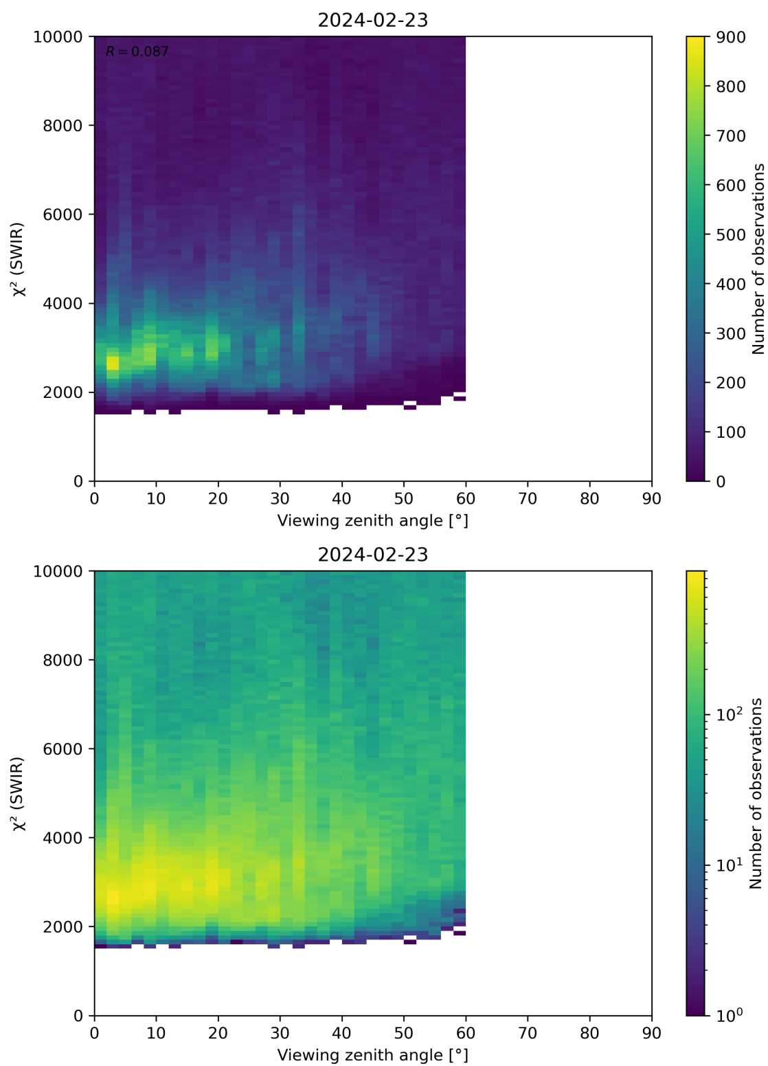
Figure 106: Scatter density plot of “Viewing zenith angle” against “ \chi^2 (SWIR)” for 2024-02-22 to 2024-02-24.
