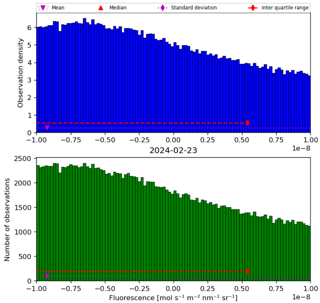
Figure 32: Histogram of “Fluorescence” for 2024-02-22 to 2024-02-24
