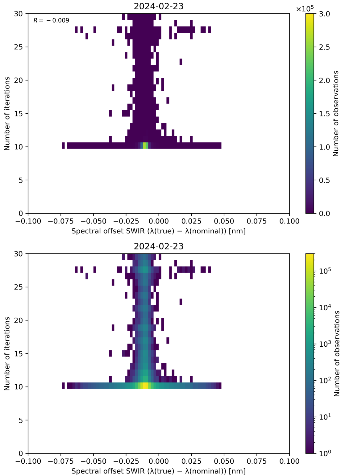
Figure 121: Scatter density plot of “Spectral offset SWIR ( \lambda(\text{true}) - \lambda(\text{nominal}) )” against “Number of iterations” for 2024-02-22 to 2024-02-24.
