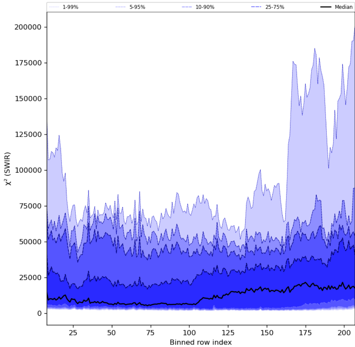
Figure 39: Along track statistics of “ \chi^2 (SWIR)” for 2024-02-22 to 2024-02-24
