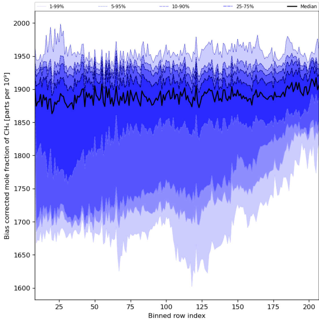
Figure 36: Along track statistics of “Bias corrected mole fraction of CH 4 ” for 2024-02-22 to 2024-02-24
