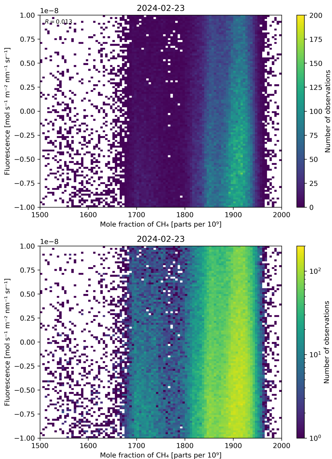
Figure 73: Scatter density plot of “Mole fraction of \text{CH}_4 ” against “Fluorescence” for 2024-02-22 to 2024-02-24.
