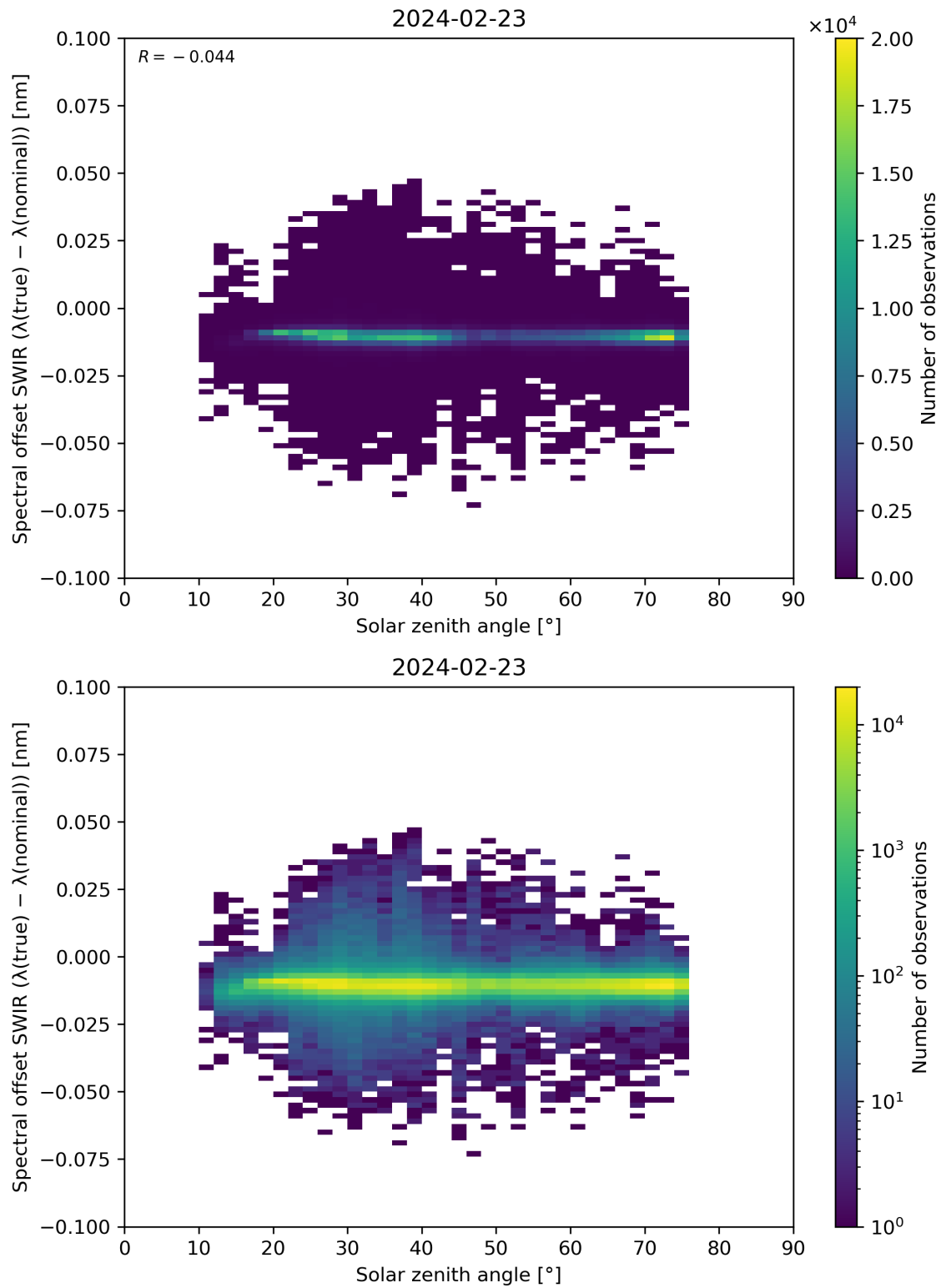
Figure 104: Scatter density plot of “Solar zenith angle” against “Spectral offset SWIR ( \lambda(\text{true}) - \lambda(\text{nominal}) )” for 2024-02-22 to 2024-02-24.
