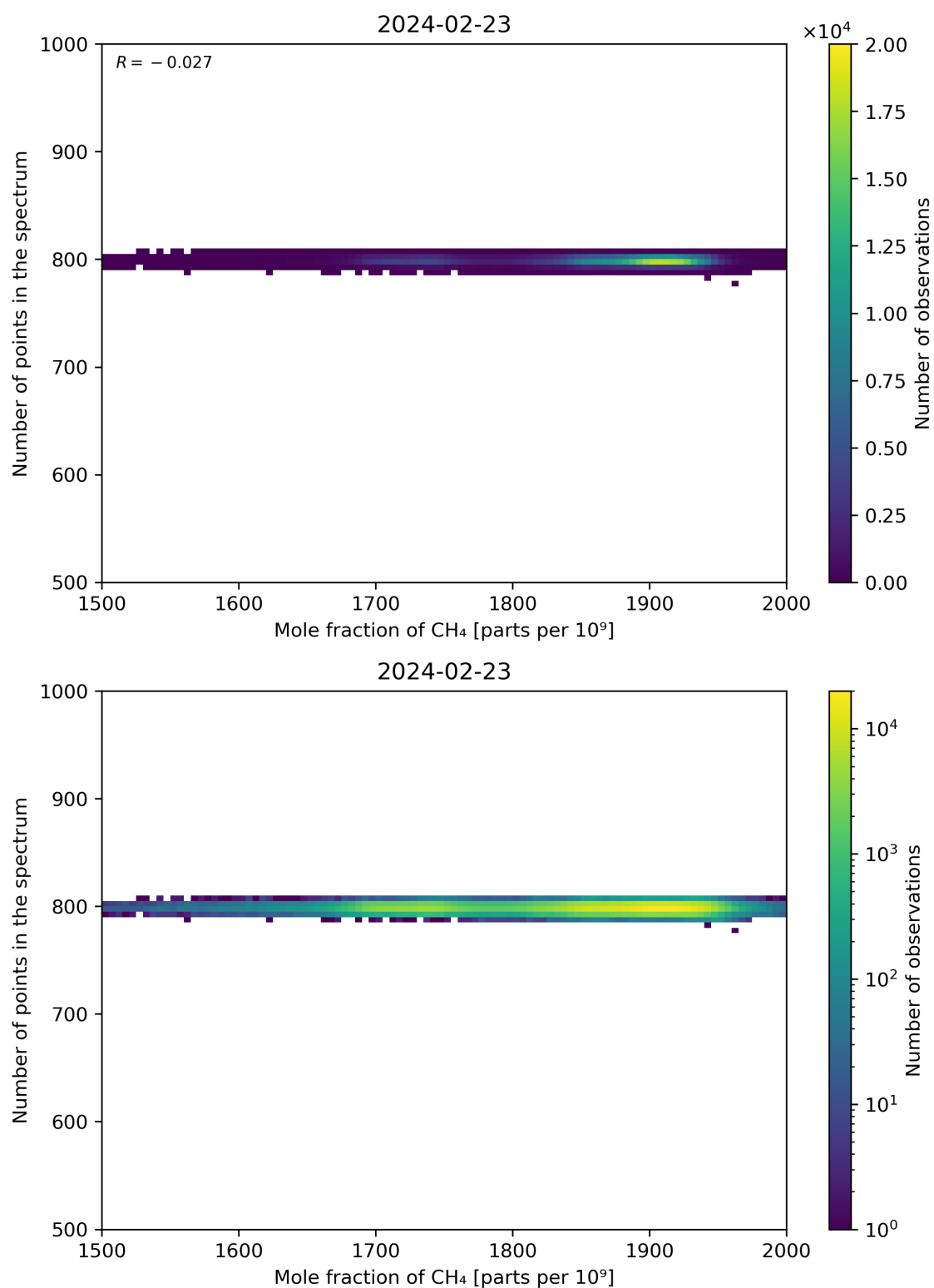
Figure 77: Scatter density plot of “Mole fraction of CH 4 ” against “Number of points in the spectrum” for 2024-02-22 to 2024-02-24.
