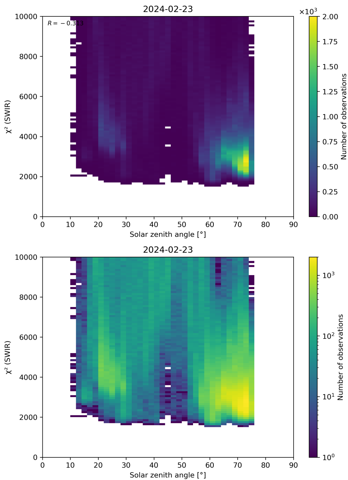
Figure 95: Scatter density plot of “Solar zenith angle” against “ \chi^2 (SWIR)” for 2024-02-22 to 2024-02-24.
