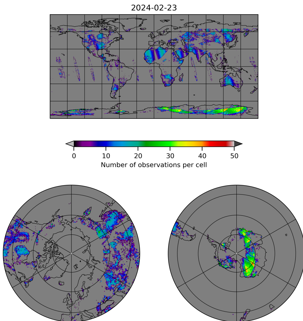
Figure 10: Map of the number of observations for 2024-02-22 to 2024-02-24
