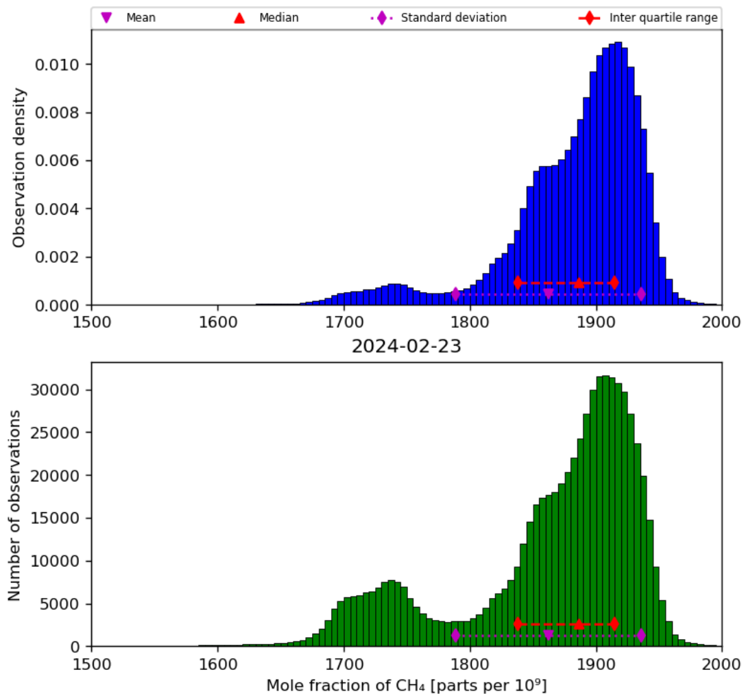
Figure 23: Histogram of “Mole fraction of CH 4 ” for 2024-02-22 to 2024-02-24
