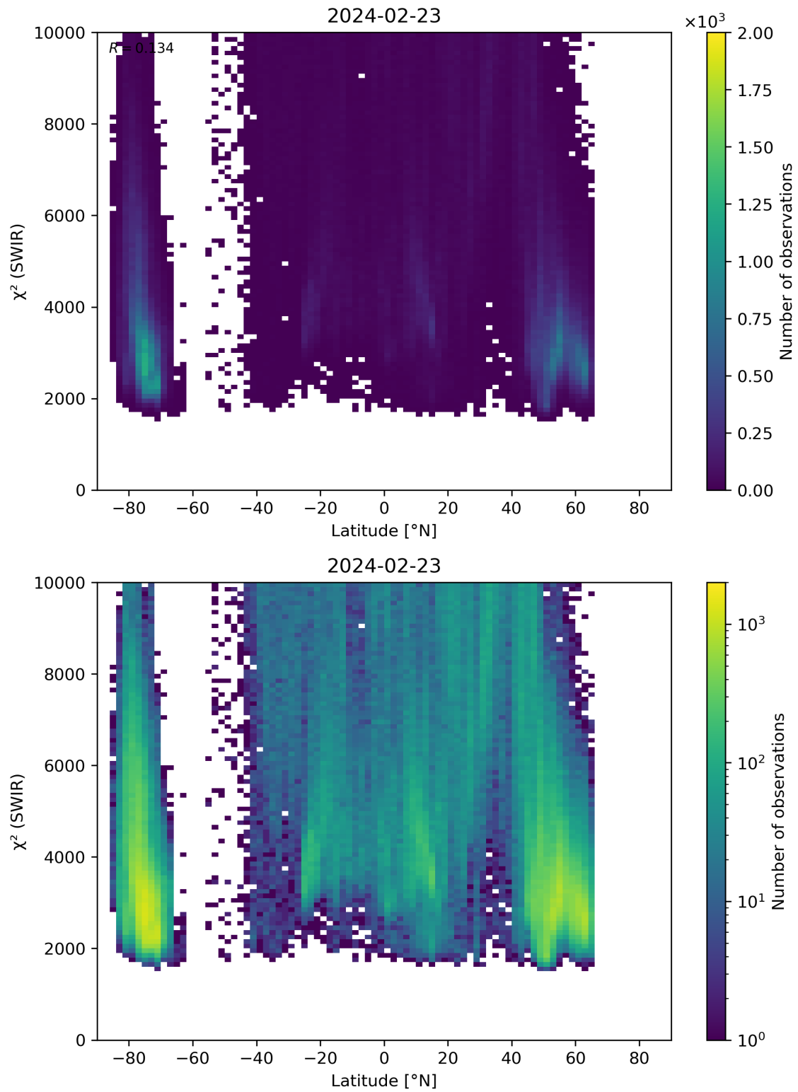
Figure 54: Scatter density plot of “Latitude” against “ \chi^2 (SWIR)” for 2024-02-22 to 2024-02-24.
