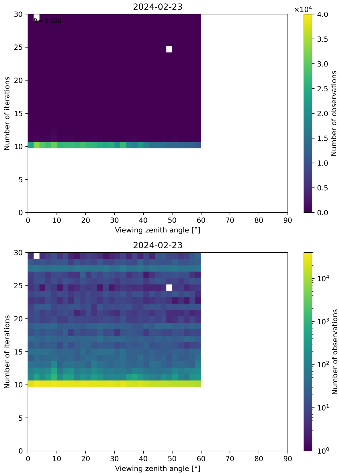
Figure 113: Scatter density plot of “Viewing zenith angle” against “Number of iterations” for 2024-02-22 to 2024-02-24.
