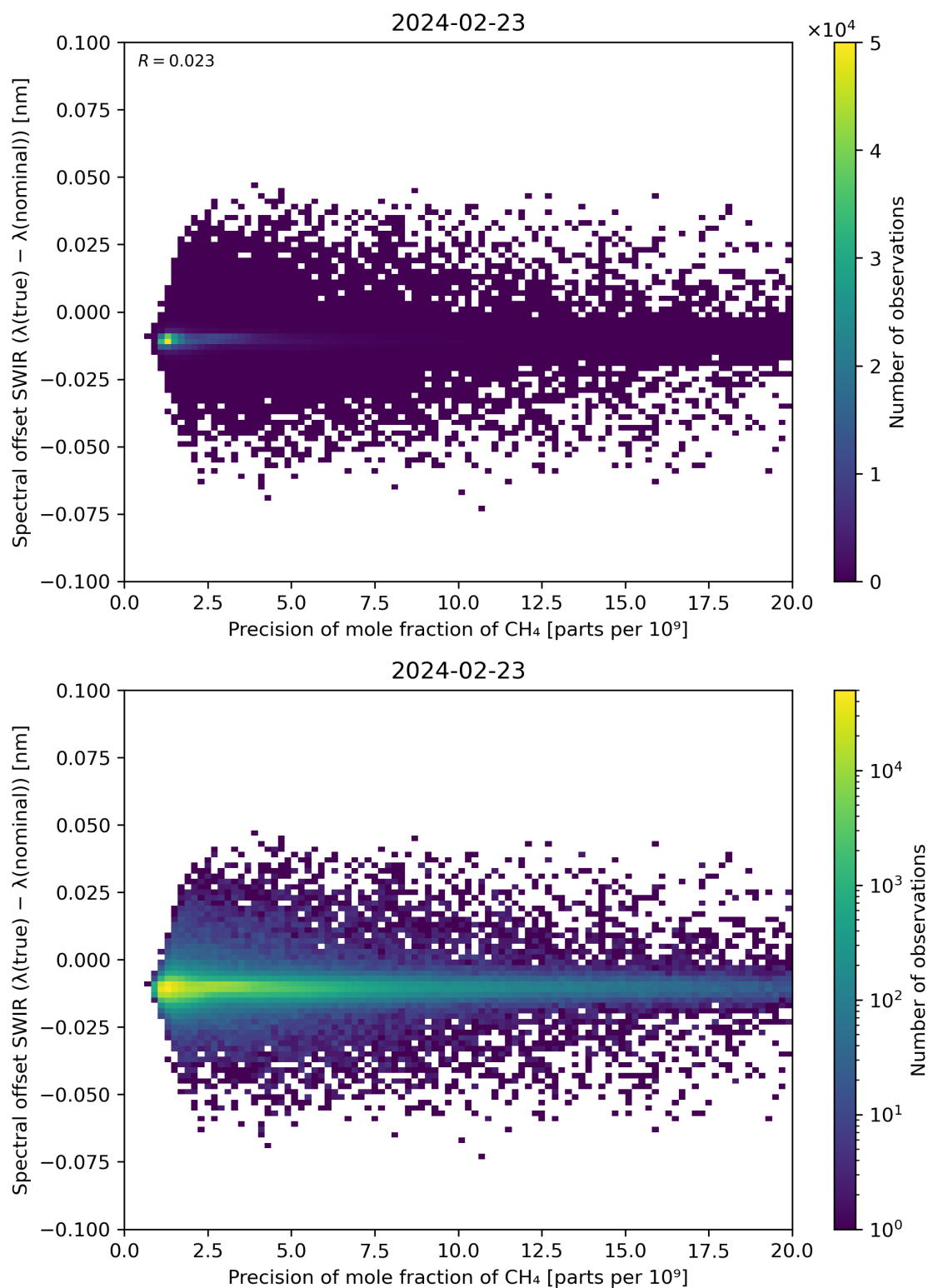
Figure 85: Scatter density plot of “Precision of mole fraction of \text{CH}_4 ” against “Spectral offset SWIR ( \lambda(\text{true}) - \lambda(\text{nominal}) )” for 2024-02-22 to 2024-02-24.
