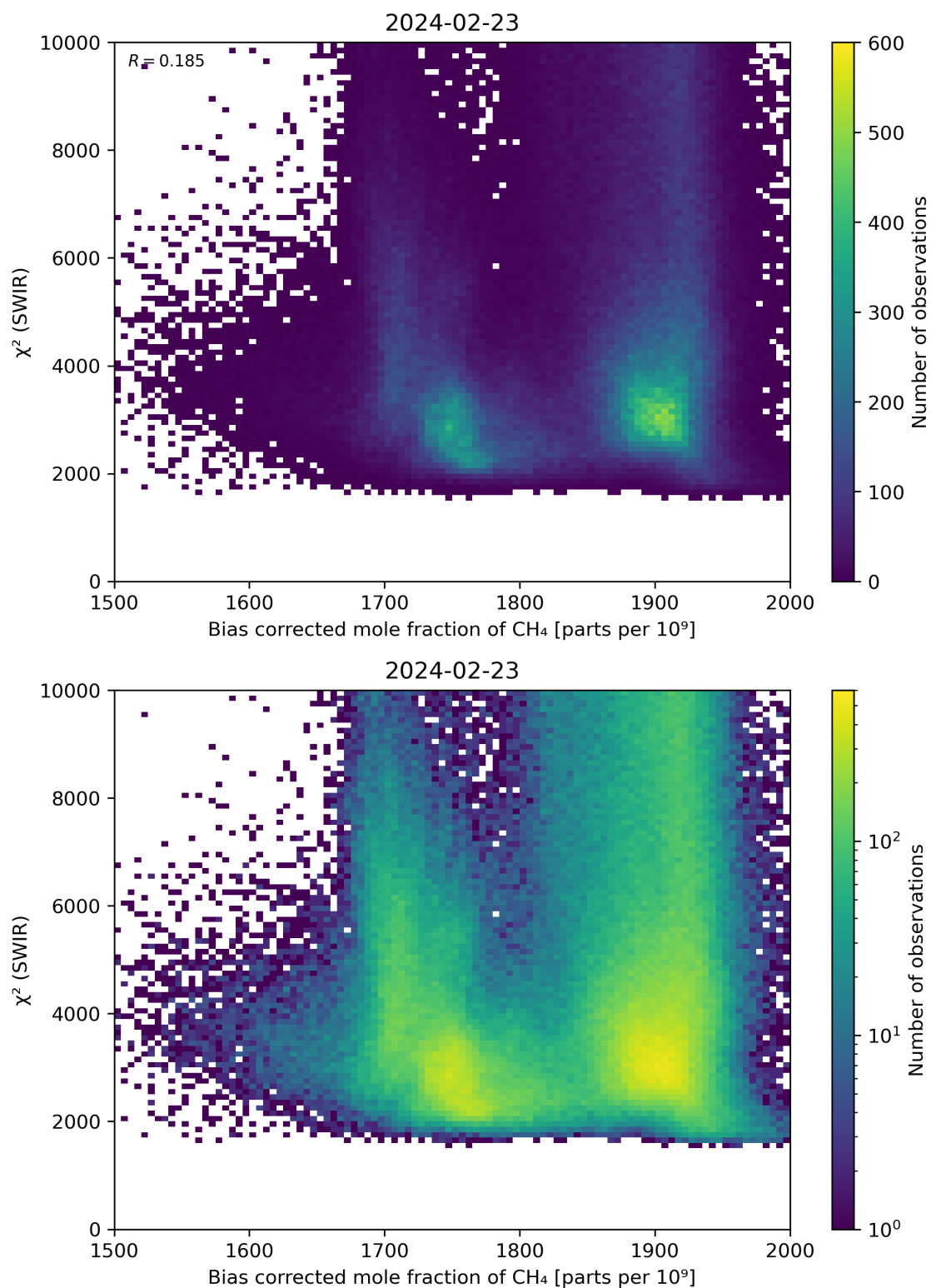
Figure 64: Scatter density plot of “Bias corrected mole fraction of CH 4 ” against “ \chi^2 (SWIR)” for 2024-02-22 to 2024-02-24.
