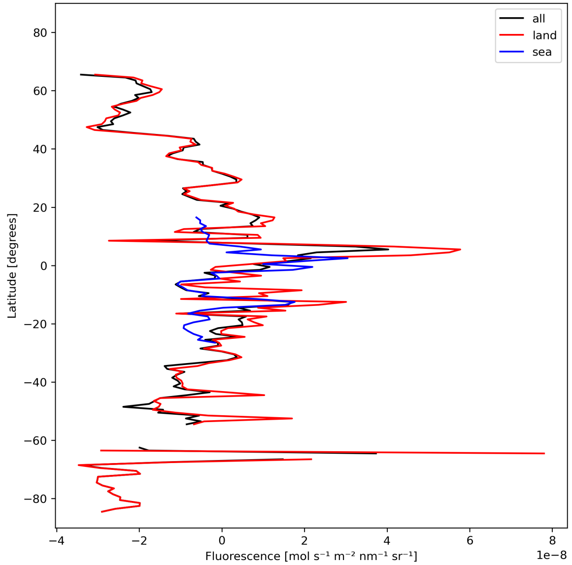
Figure 21: Zonal average of “Fluorescence” for 2024-02-22 to 2024-02-24.
