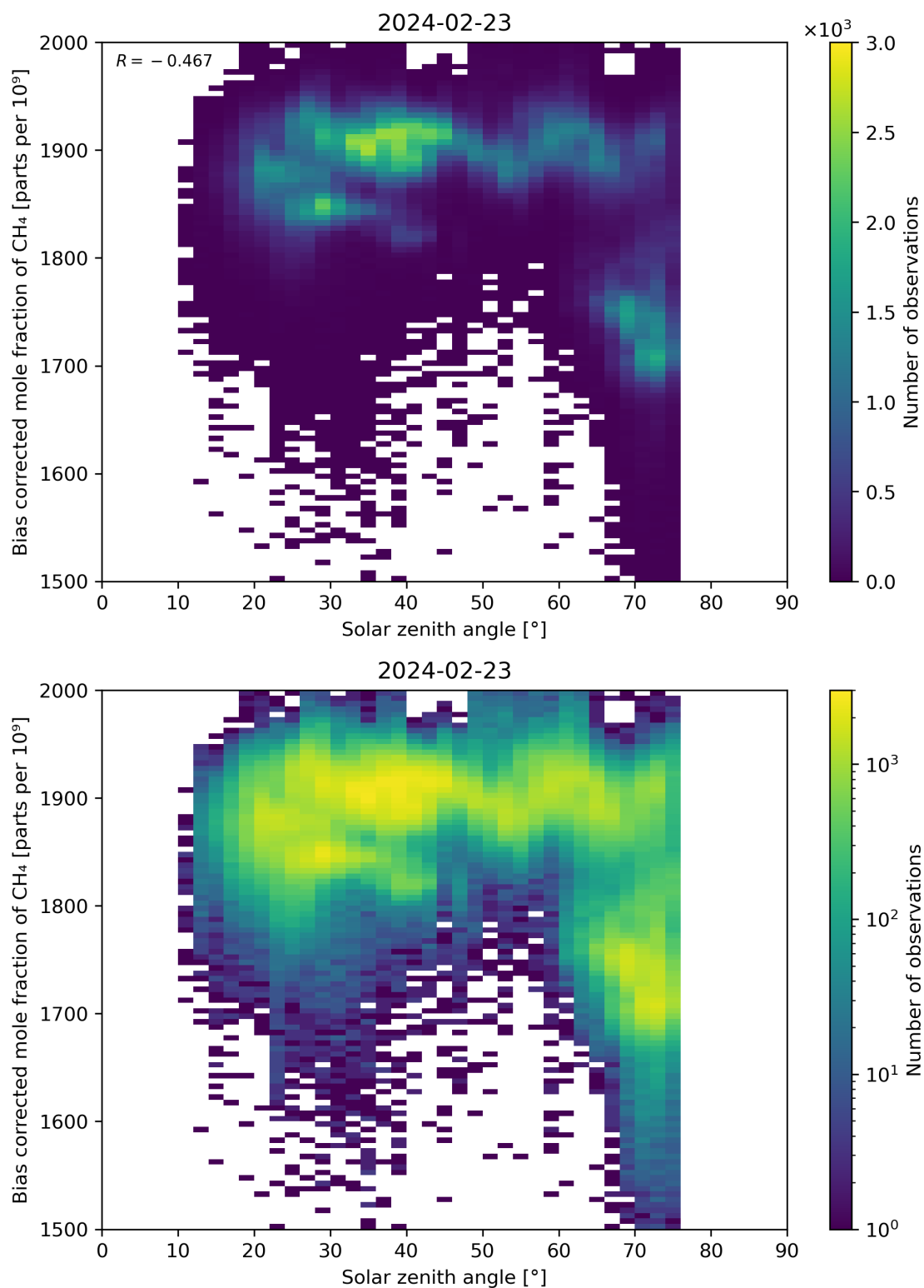
Figure 100: Scatter density plot of “Solar zenith angle” against “Bias corrected mole fraction of \text{CH}_4 ” for 2024-02-22 to 2024-02-24.
