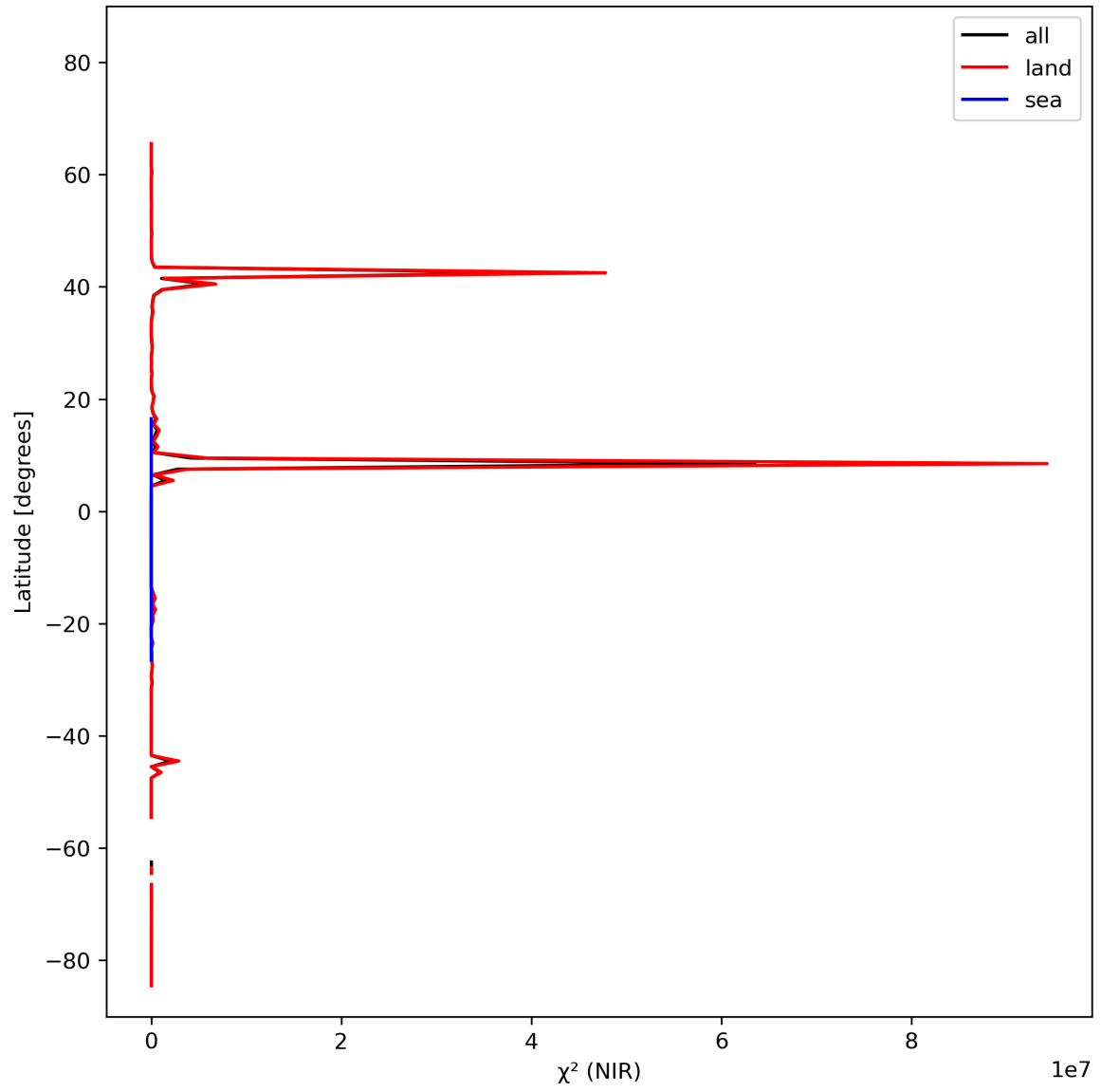
Figure 18: Zonal average of “ \chi^2 (NIR)” for 2024-02-22 to 2024-02-24.
