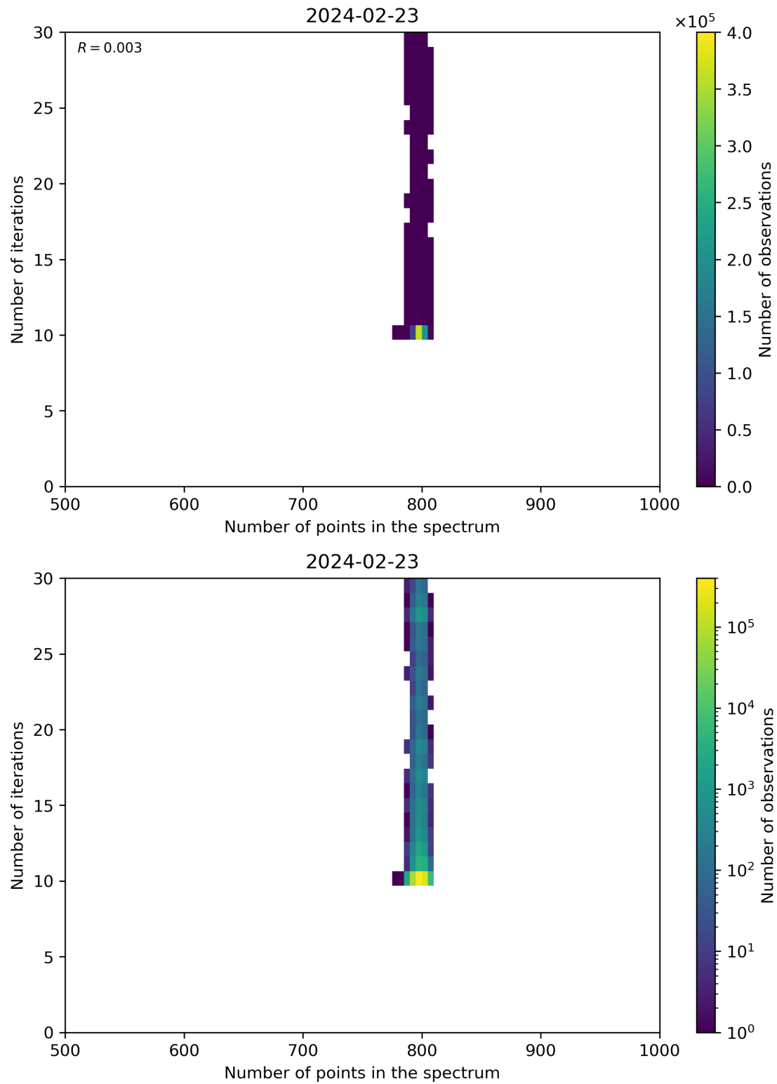
Figure 92: Scatter density plot of “Number of points in the spectrum” against “Number of iterations” for 2024-02-22 to 2024-02-24.
