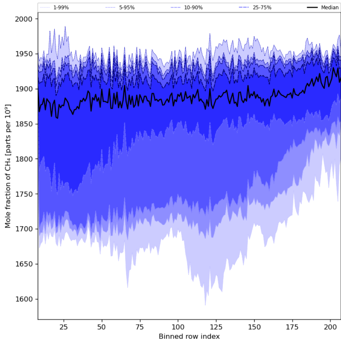
Figure 34: Along track statistics of “Mole fraction of CH 4 ” for 2024-02-22 to 2024-02-24
