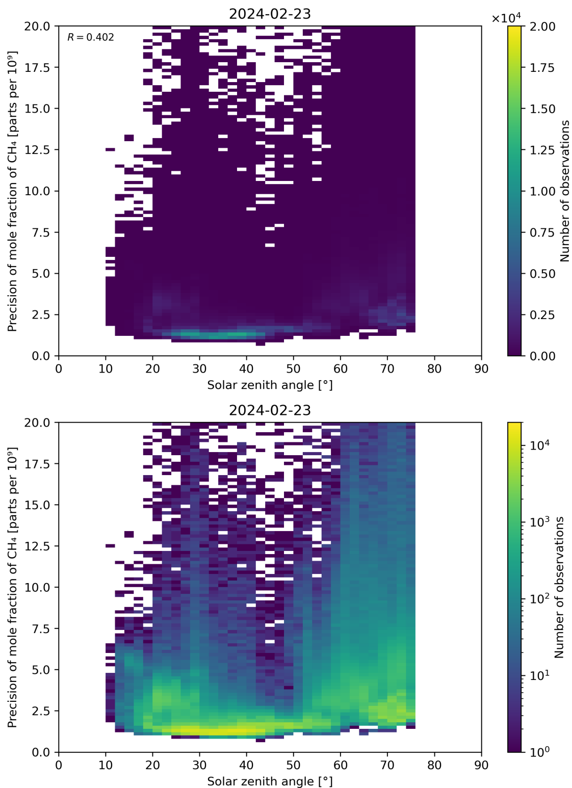
Figure 101: Scatter density plot of “Solar zenith angle” against “Precision of mole fraction of CH 4 ” for 2024-02-22 to 2024-02-24.
