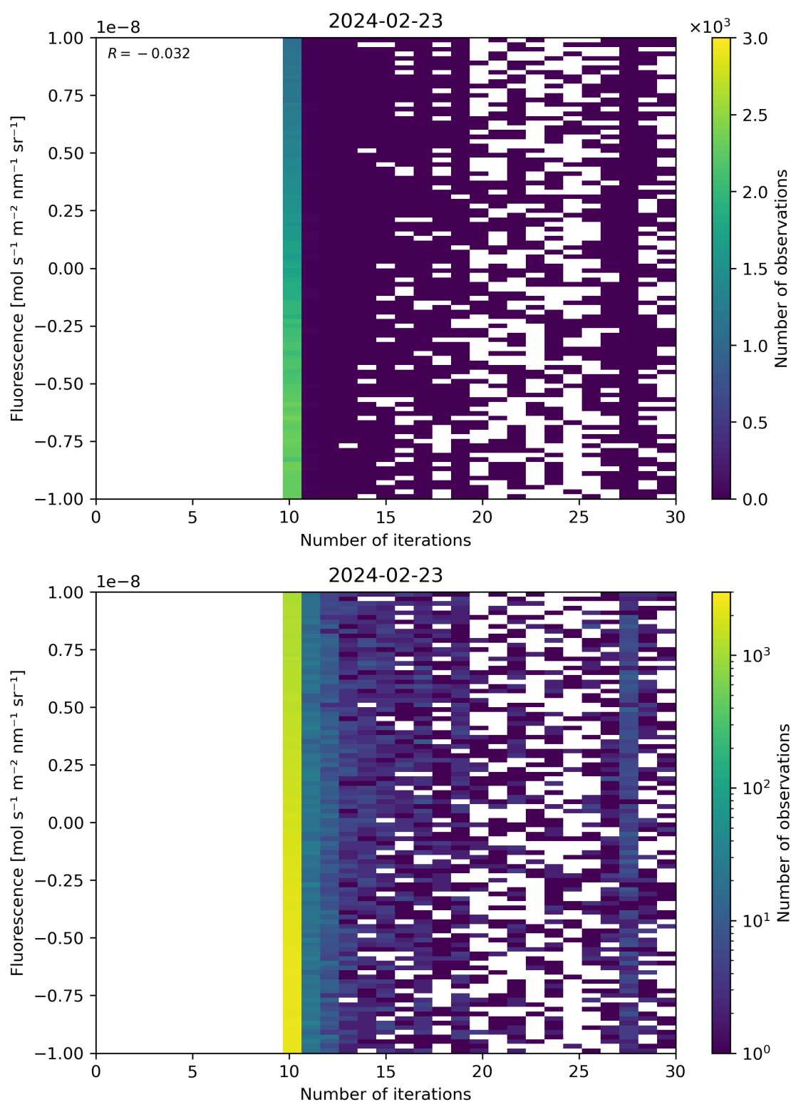
Figure 87: Scatter density plot of “Number of iterations” against “Fluorescence” for 2024-02-22 to 2024-02-24.
