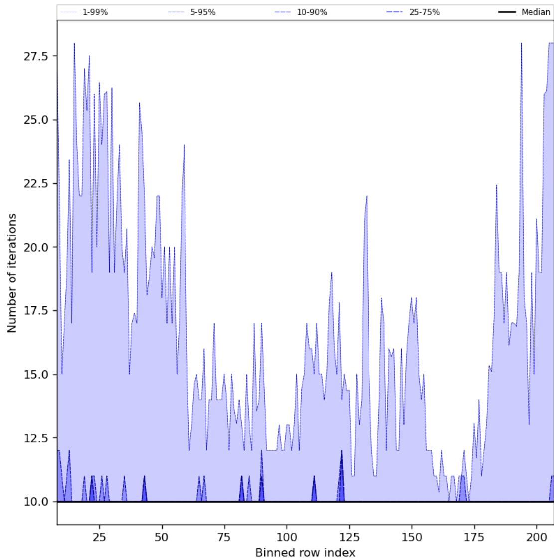
Figure 42: Along track statistics of “Number of iterations” for 2024-02-22 to 2024-02-24
