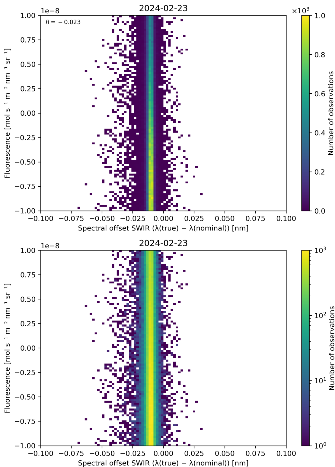
Figure 120: Scatter density plot of “Spectral offset SWIR ( \lambda(\text{true}) - \lambda(\text{nominal}) )” against “Fluorescence” for 2024-02-22 to 2024-02-24.
