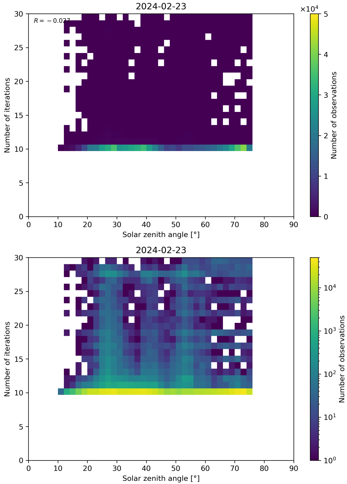
Figure 102: Scatter density plot of “Solar zenith angle” against “Number of iterations” for 2024-02-22 to 2024-02-24.
