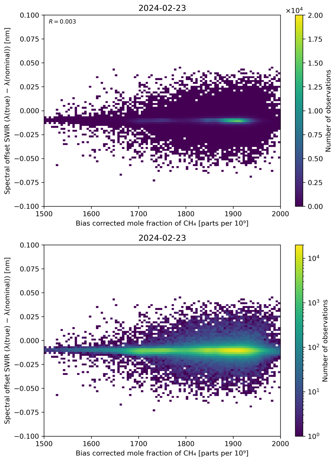
Figure 69: Scatter density plot of “Bias corrected mole fraction of \text{CH}_4 ” against “Spectral offset SWIR ( \lambda(\text{true}) - \lambda(\text{nominal}) )” for 2024-02-22 to 2024-02-24.
