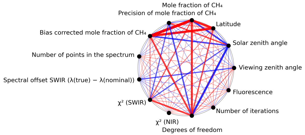
Figure 1: Map of correlation graph for 2024-02-22 to 2024-02-24.
