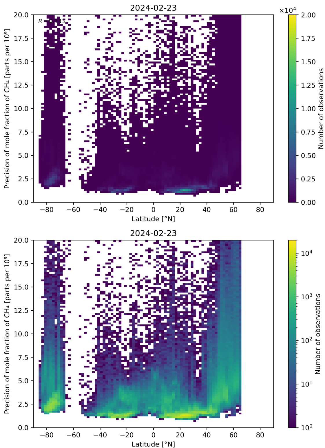
Figure 59: Scatter density plot of “Latitude” against “Precision of mole fraction of CH 4 ” for 2024-02-22 to 2024-02-24.
