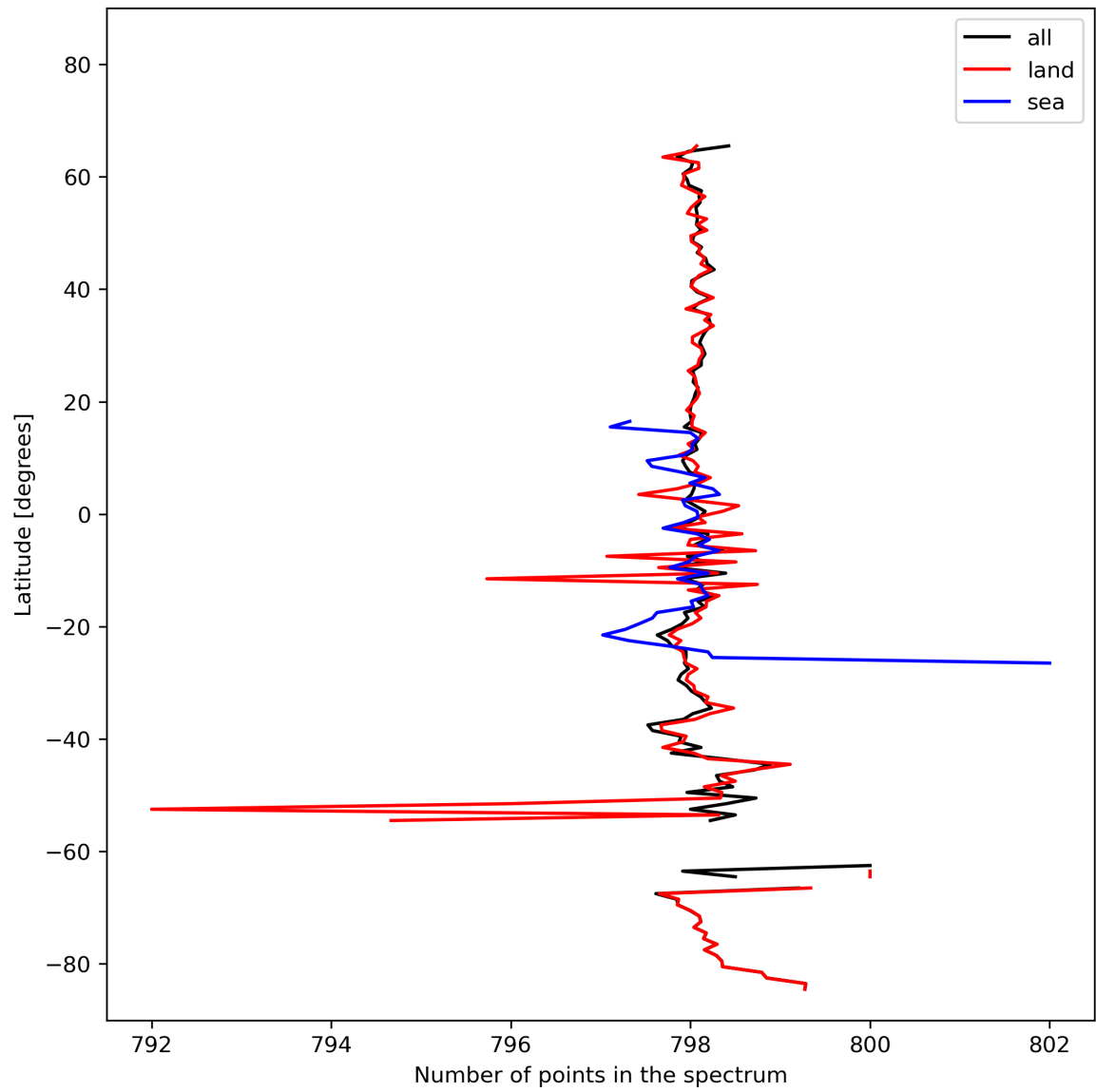
Figure 15: Zonal average of “Number of points in the spectrum” for 2024-02-22 to 2024-02-24.
