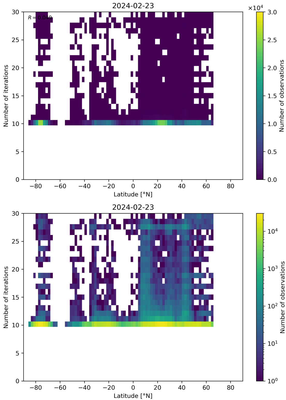
Figure 60: Scatter density plot of “Latitude” against “Number of iterations” for 2024-02-22 to 2024-02-24.
