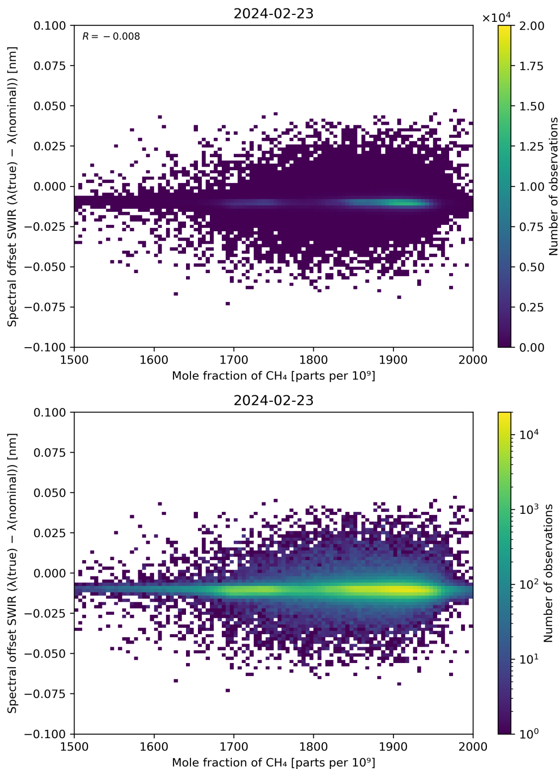
Figure 86: Scatter density plot of “Mole fraction of \text{CH}_4 ” against “Spectral offset SWIR ( \lambda(\text{true}) - \lambda(\text{nominal}) )” for 2024-02-22 to 2024-02-24.
