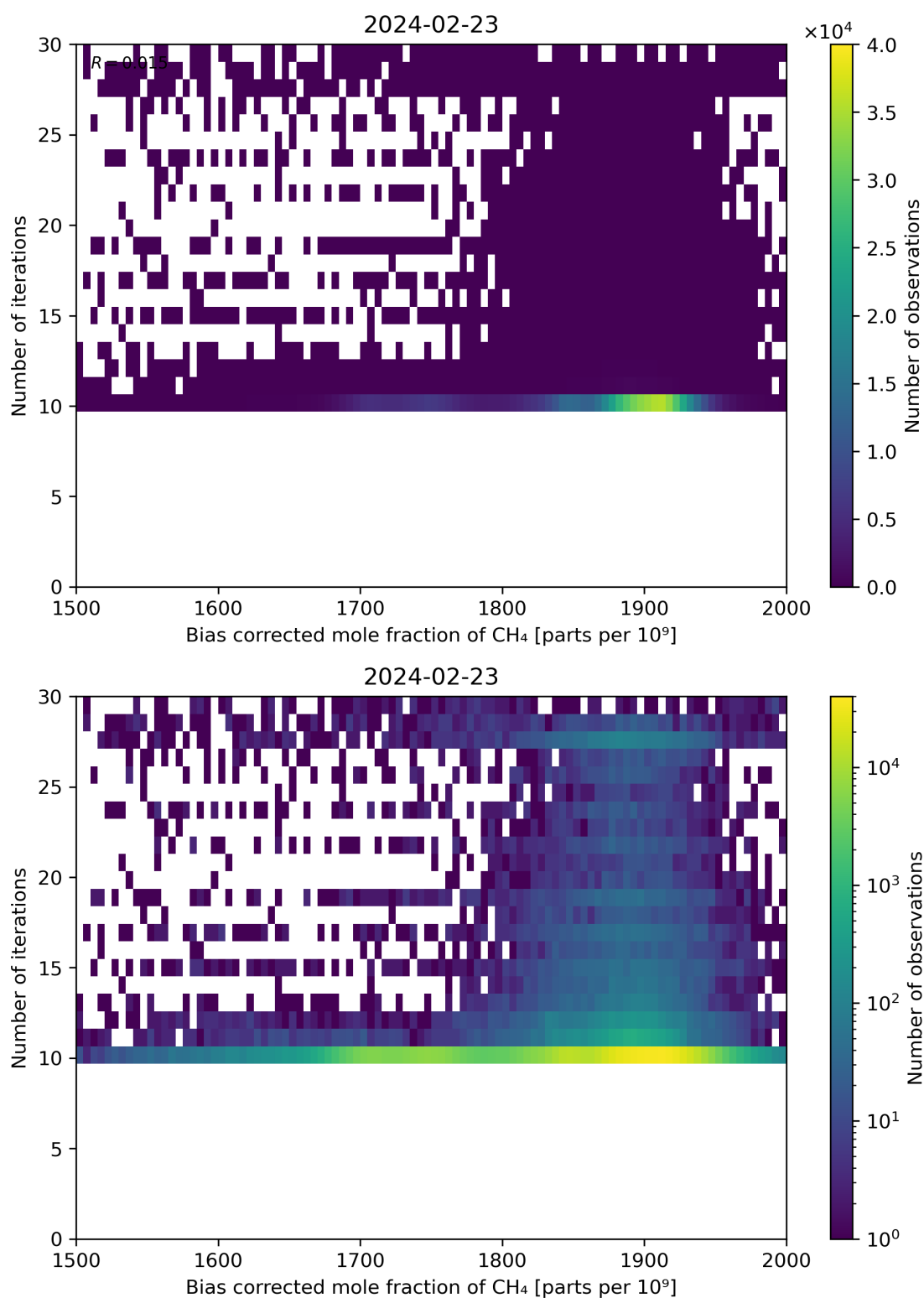
Figure 67: Scatter density plot of “Bias corrected mole fraction of \text{CH}_4 ” against “Number of iterations” for 2024-02-22 to 2024-02-24.
