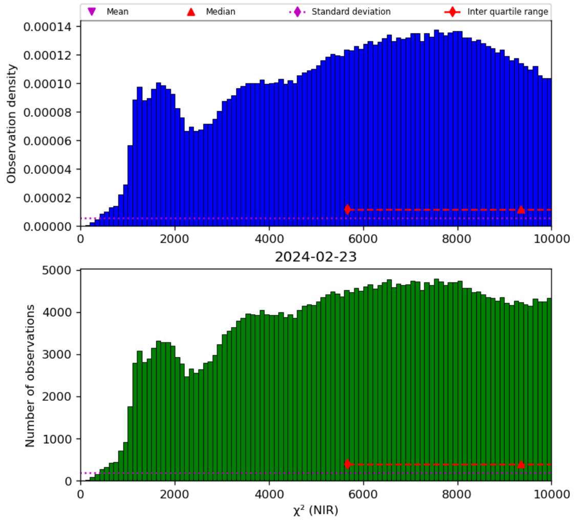
Figure 29: Histogram of " \chi^2 (NIR)" for 2024-02-22 to 2024-02-24
