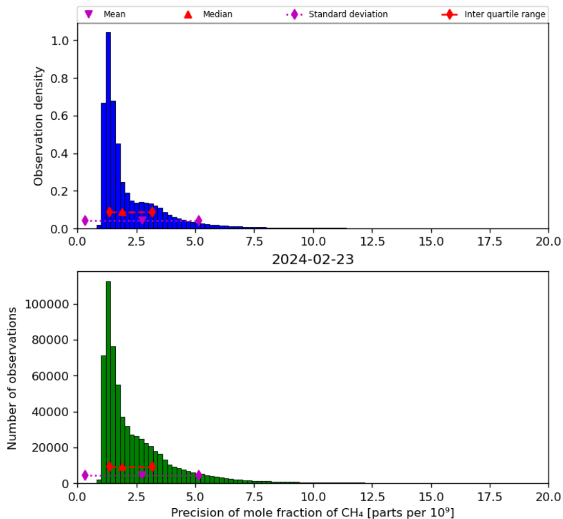
Figure 24: Histogram of “Precision of mole fraction of CH 4 ” for 2024-02-22 to 2024-02-24
