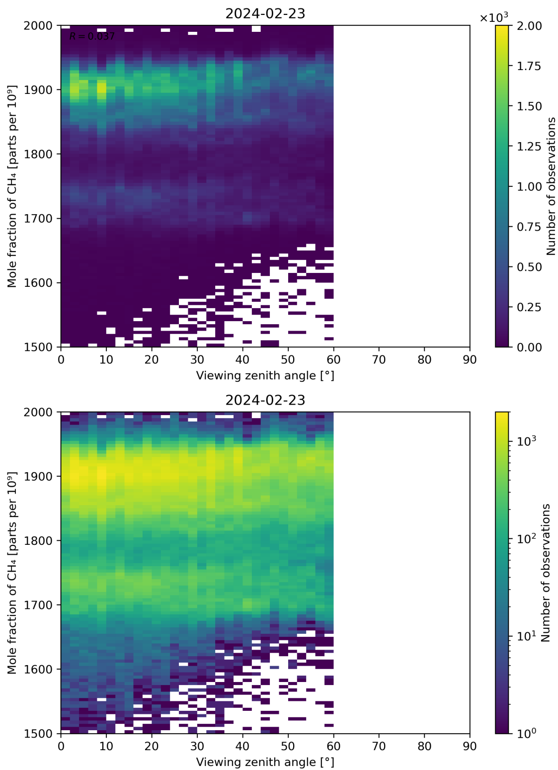
Figure 110: Scatter density plot of “Viewing zenith angle” against “Mole fraction of CH 4 ” for 2024-02-22 to 2024-02-24.
