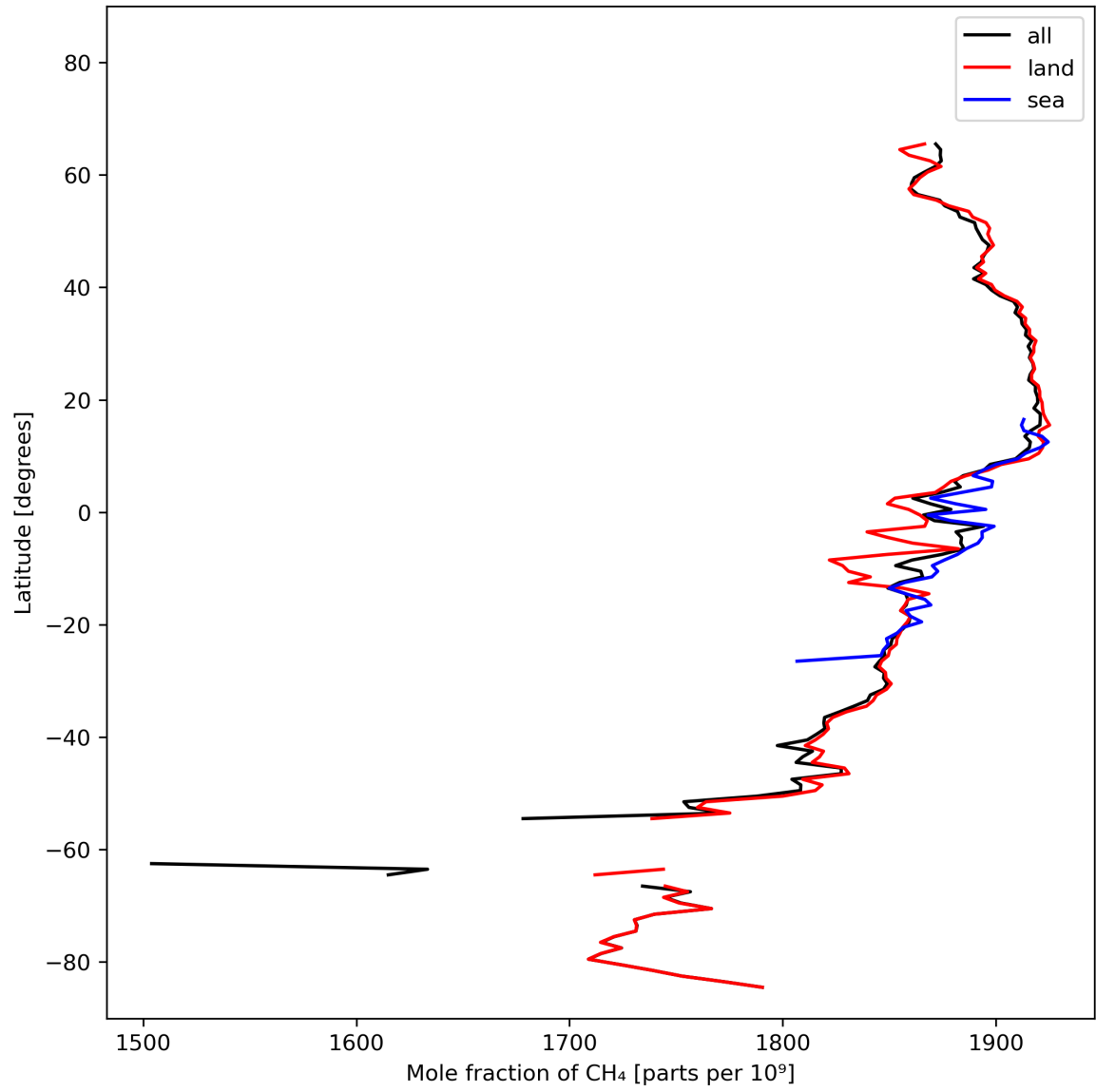
Figure 12: Zonal average of “Mole fraction of CH 4 ” for 2024-02-22 to 2024-02-24.
