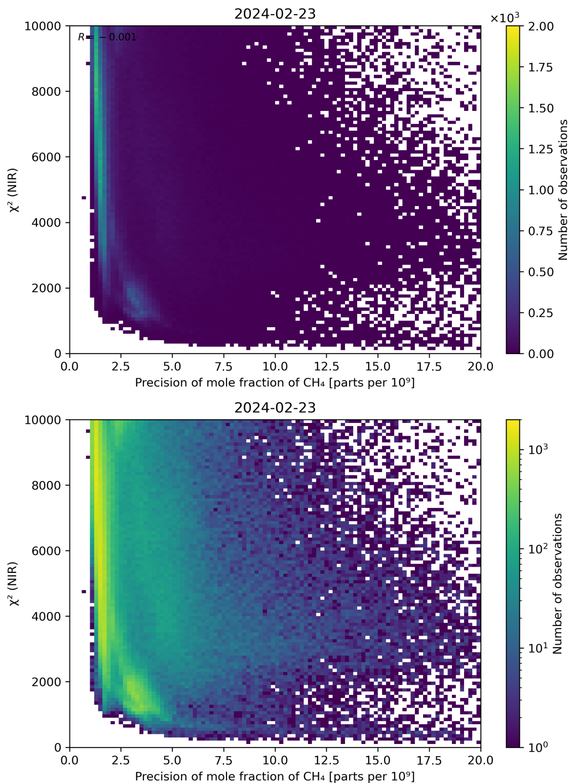
Figure 78: Scatter density plot of “Precision of mole fraction of CH 4 ” against “ \chi^2 (NIR)” for 2024-02-22 to 2024-02-24.
