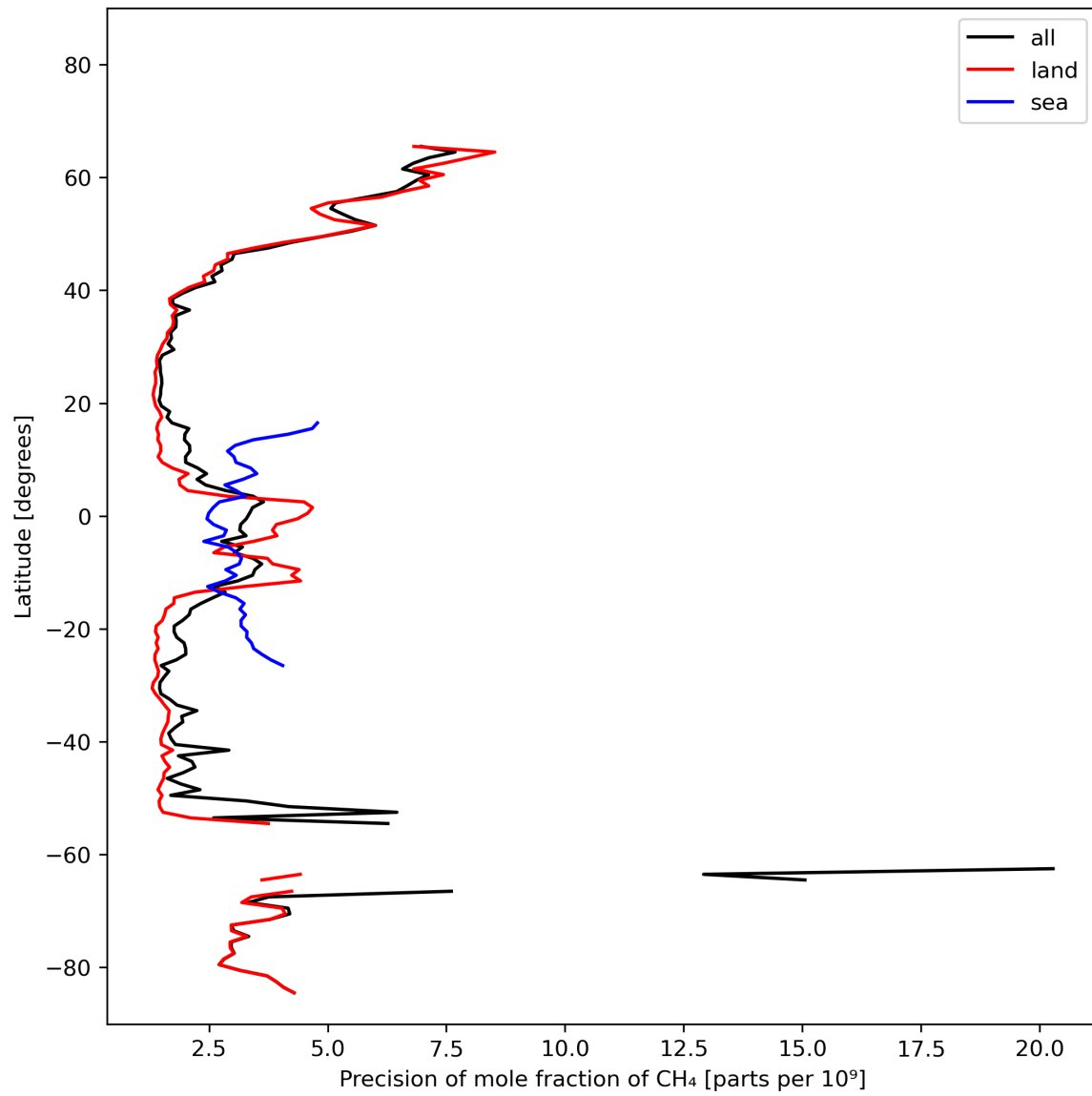
Figure 13: Zonal average of “Precision of mole fraction of CH 4 ” for 2024-02-22 to 2024-02-24.
