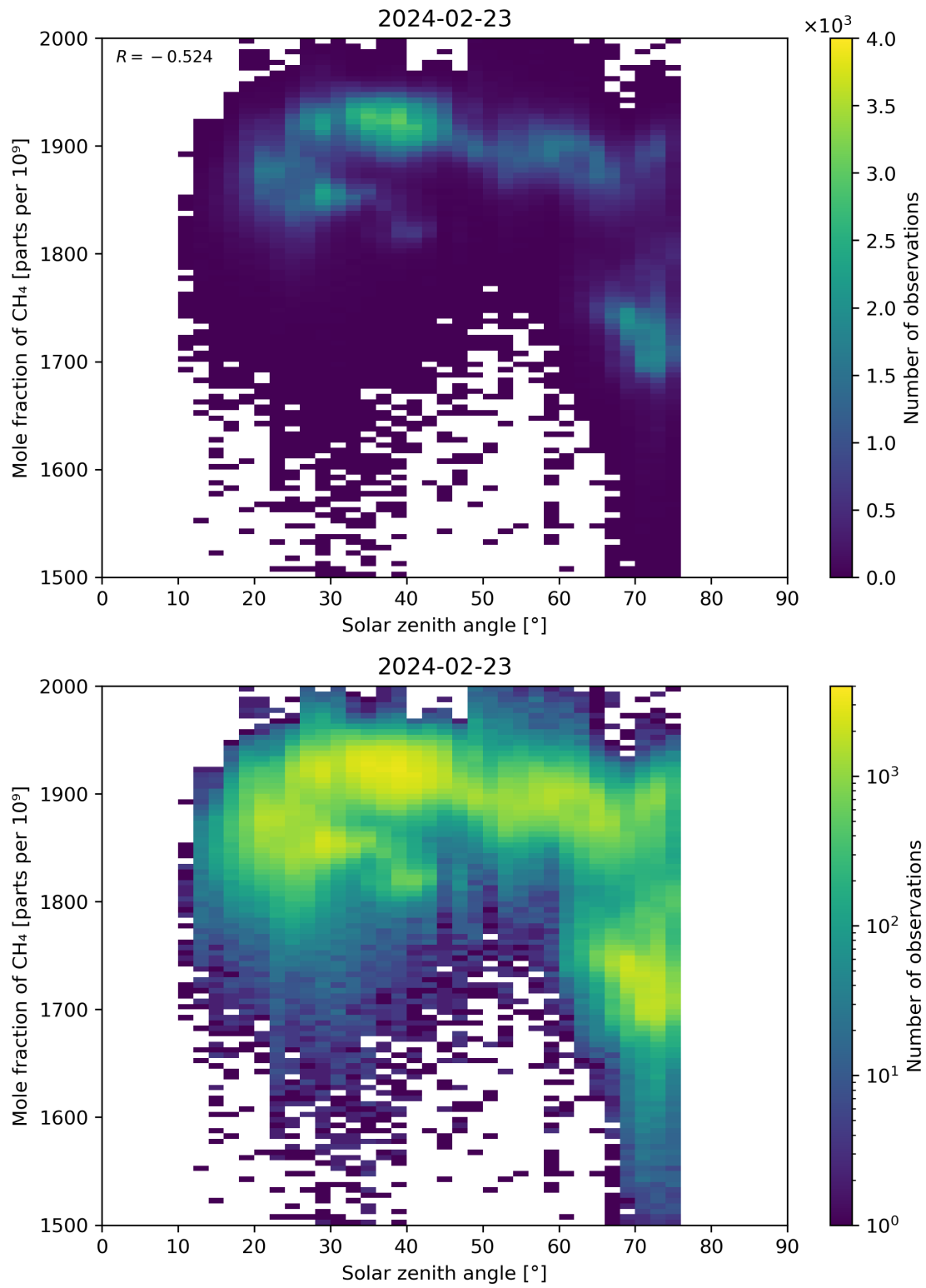
Figure 99: Scatter density plot of “Solar zenith angle” against “Mole fraction of \text{CH}_4 ” for 2024-02-22 to 2024-02-24.
