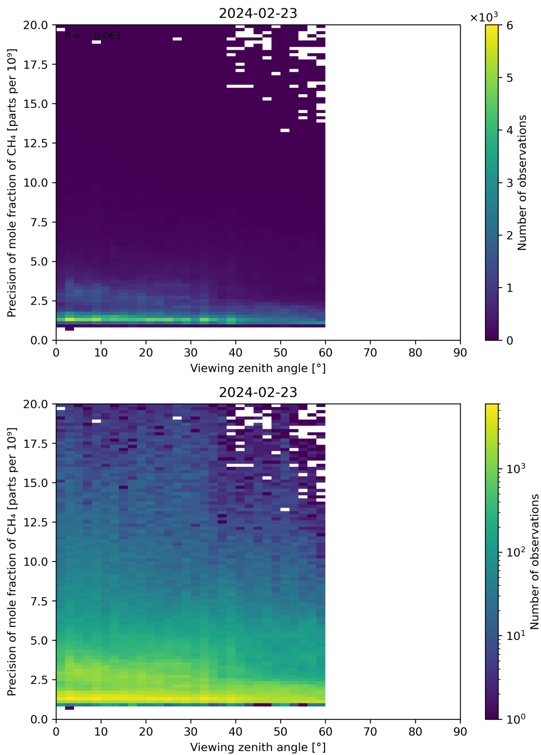
Figure 112: Scatter density plot of “Viewing zenith angle” against “Precision of mole fraction of CH 4 ” for 2024-02-22 to 2024-02-24.
