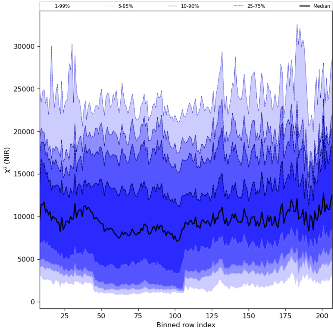
Figure 40: Along track statistics of “ \chi^2 (NIR)” for 2024-02-22 to 2024-02-24
