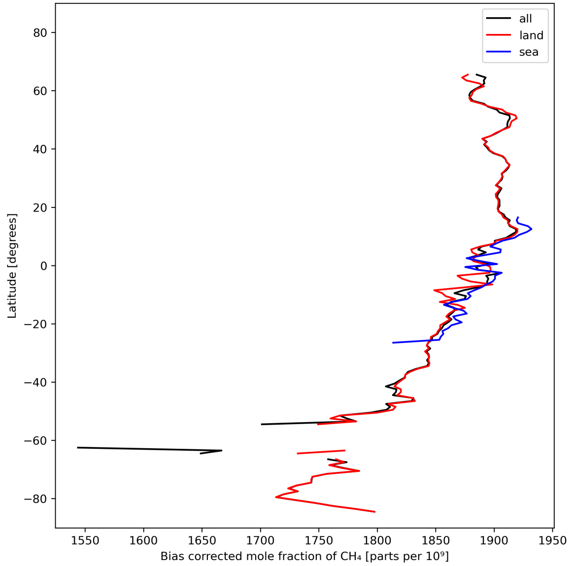
Figure 14: Zonal average of “Bias corrected mole fraction of CH 4 ” for 2024-02-22 to 2024-02-24.
