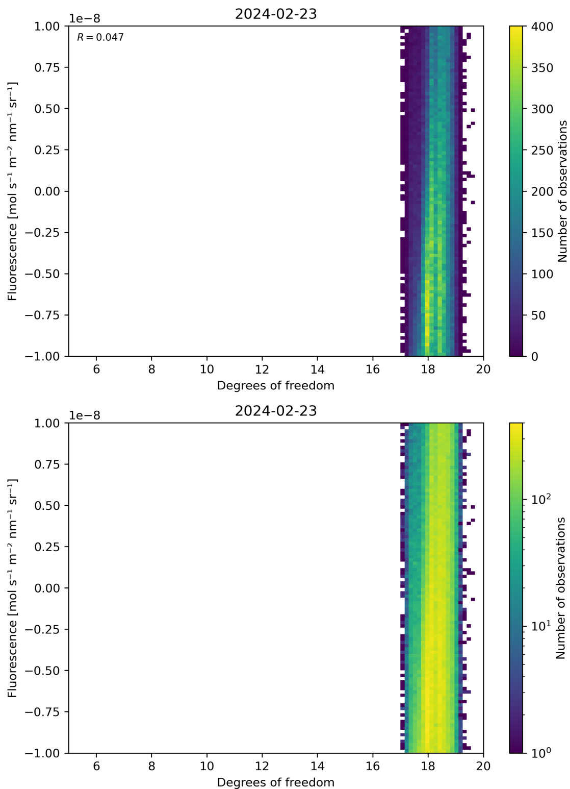
Figure 51: Scatter density plot of “Degrees of freedom” against “Fluorescence” for 2024-02-22 to 2024-02-24.
