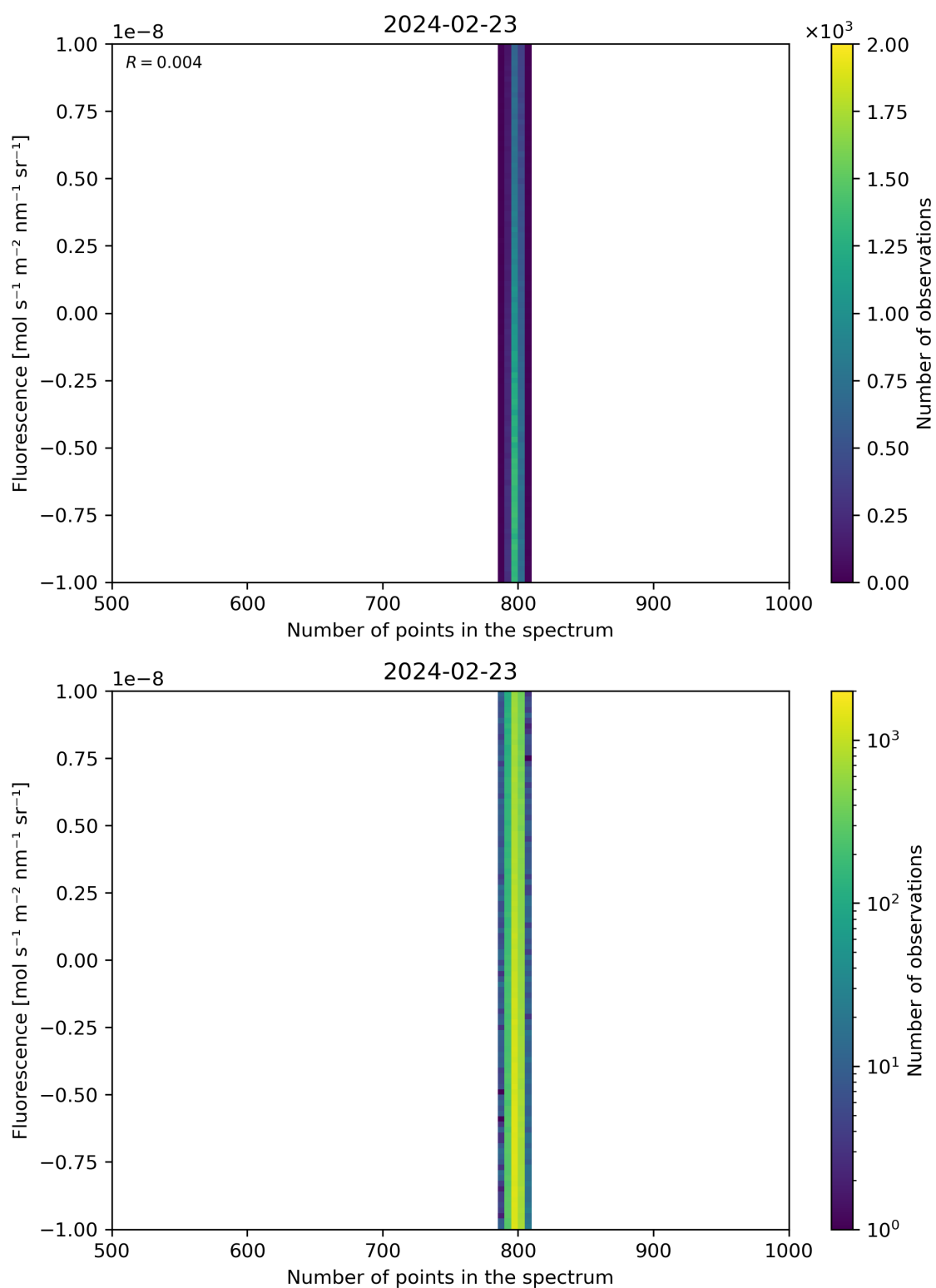
Figure 91: Scatter density plot of “Number of points in the spectrum” against “Fluorescence” for 2024-02-22 to 2024-02-24.
