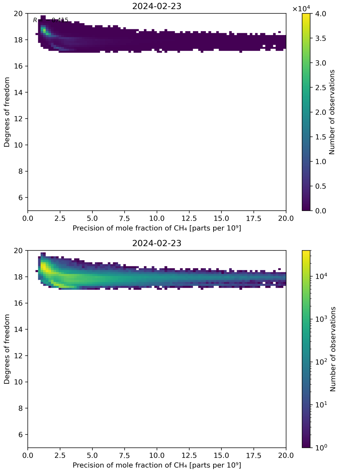
Figure 80: Scatter density plot of “Precision of mole fraction of CH 4 ” against “Degrees of freedom” for 2024-02-22 to 2024-02-24.
