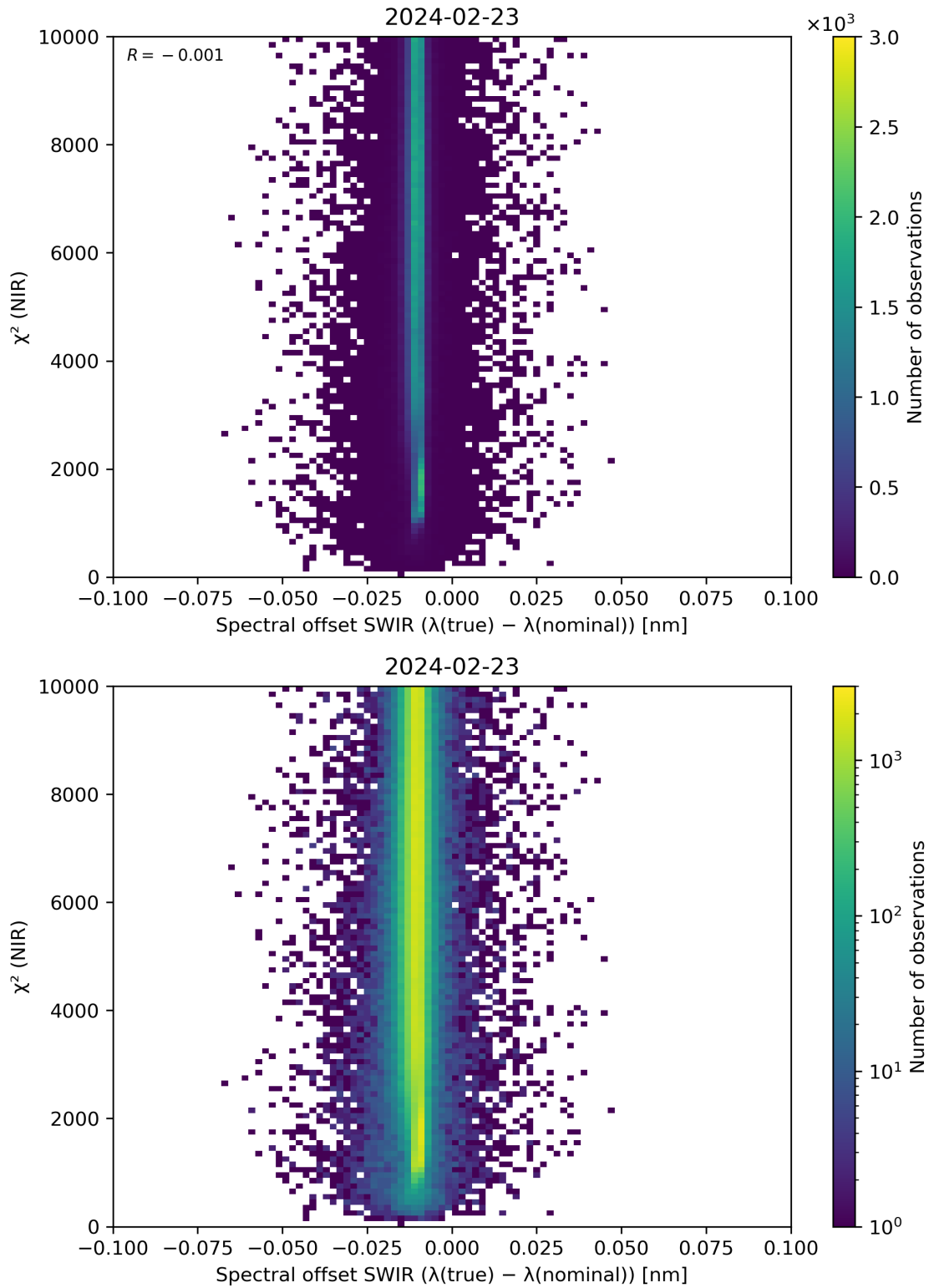
Figure 117: Scatter density plot of “Spectral offset SWIR ( \lambda(\text{true}) - \lambda(\text{nominal}) )” against “ \chi^2 (NIR)” for 2024-02-22 to 2024-02-24.
