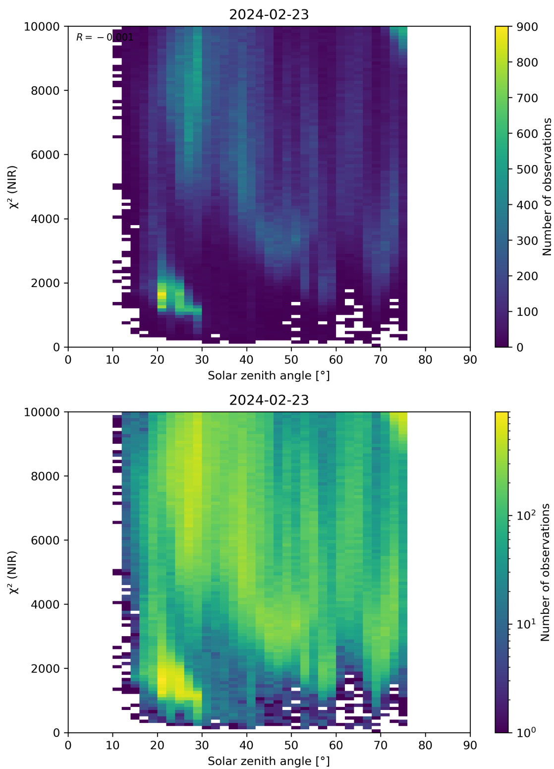
Figure 94: Scatter density plot of “Solar zenith angle” against “ \chi^2 (NIR)” for 2024-02-22 to 2024-02-24.
