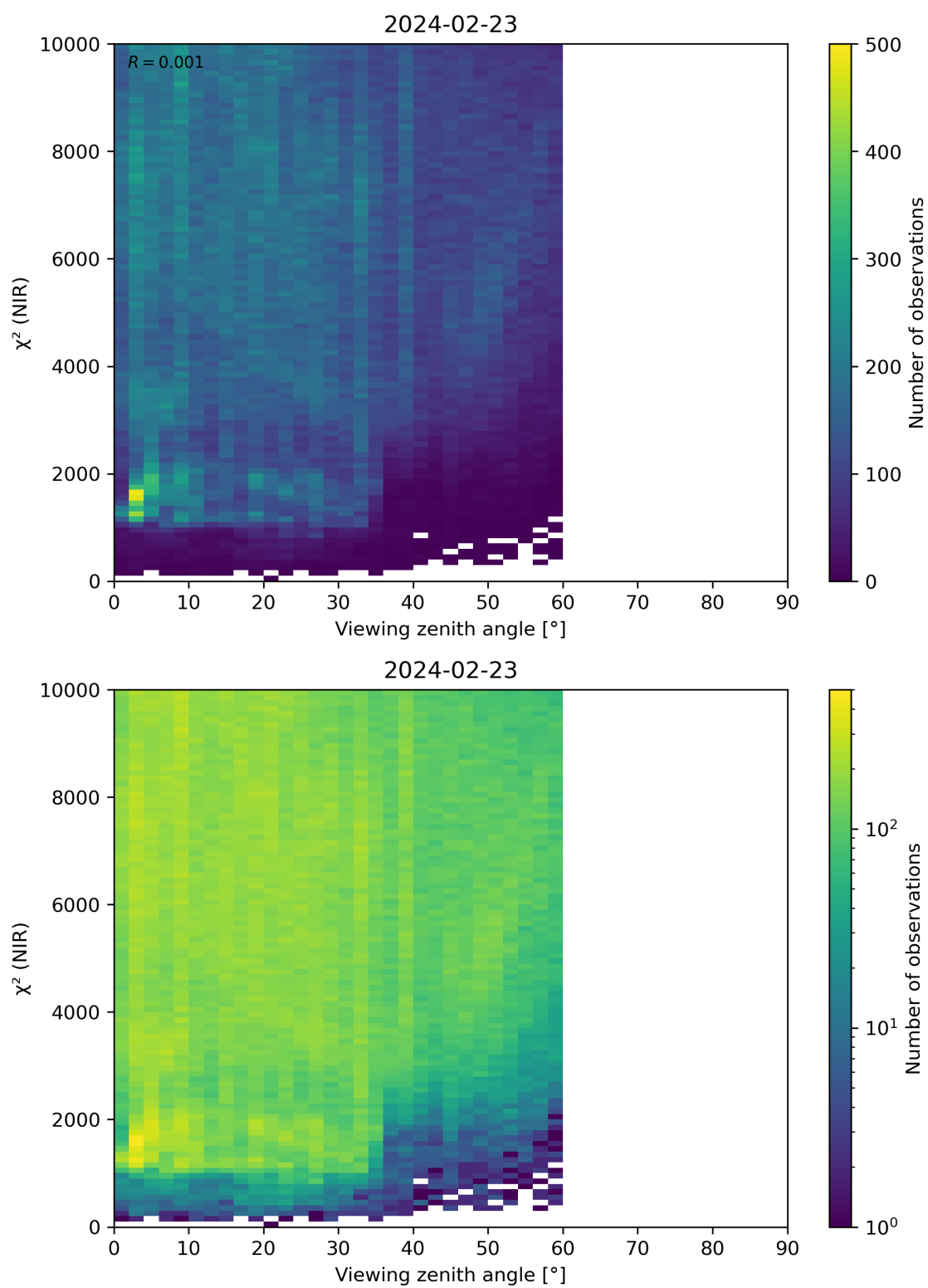
Figure 105: Scatter density plot of “Viewing zenith angle” against “ \chi^2 (NIR)” for 2024-02-22 to 2024-02-24.
