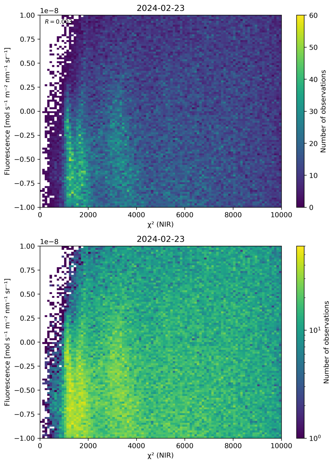
Figure 45: Scatter density plot of “ \chi^2 (NIR)” against “Fluorescence” for 2024-02-22 to 2024-02-24.
