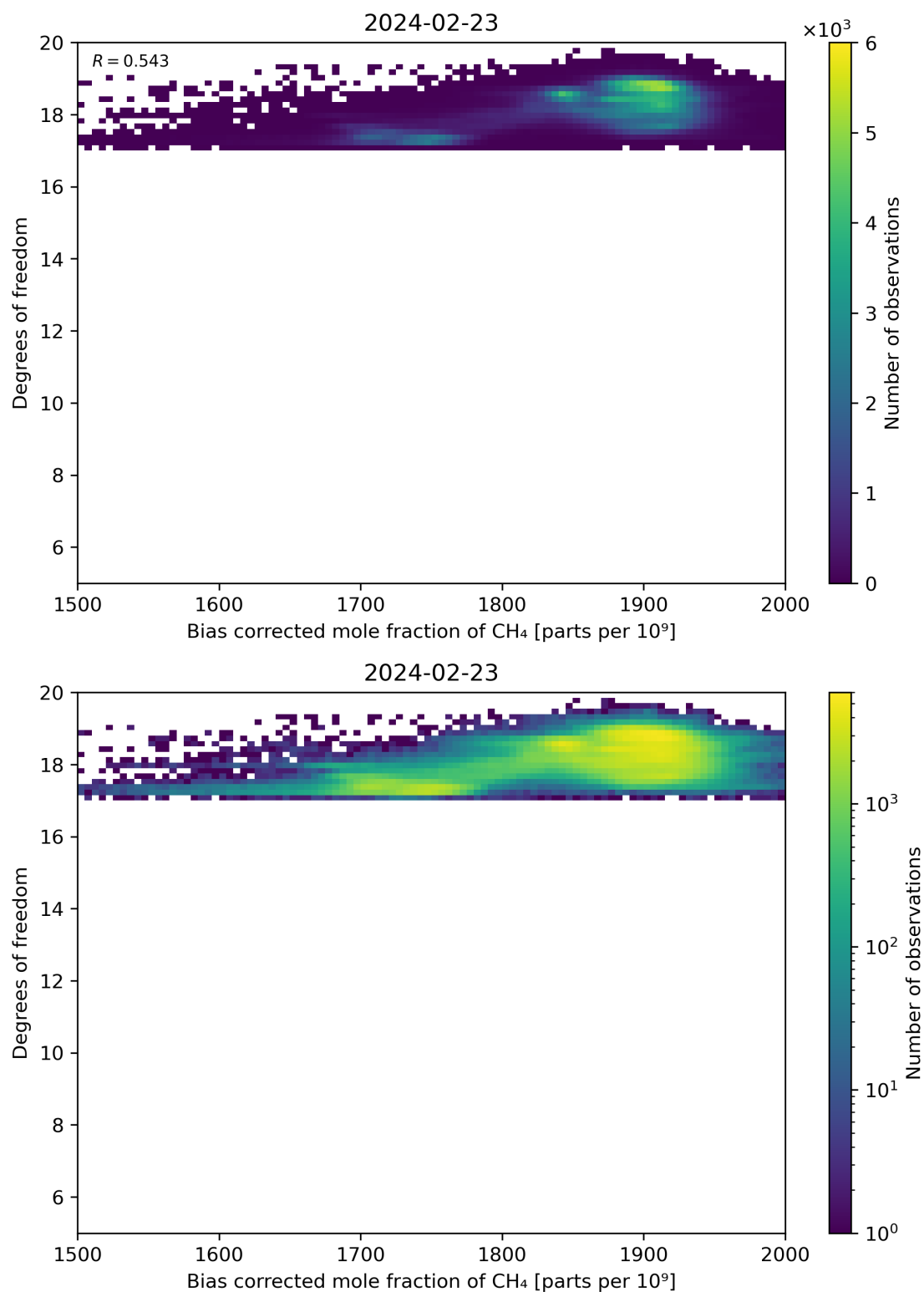
Figure 65: Scatter density plot of “Bias corrected mole fraction of CH 4 ” against “Degrees of freedom” for 2024-02-22 to 2024-02-24.
