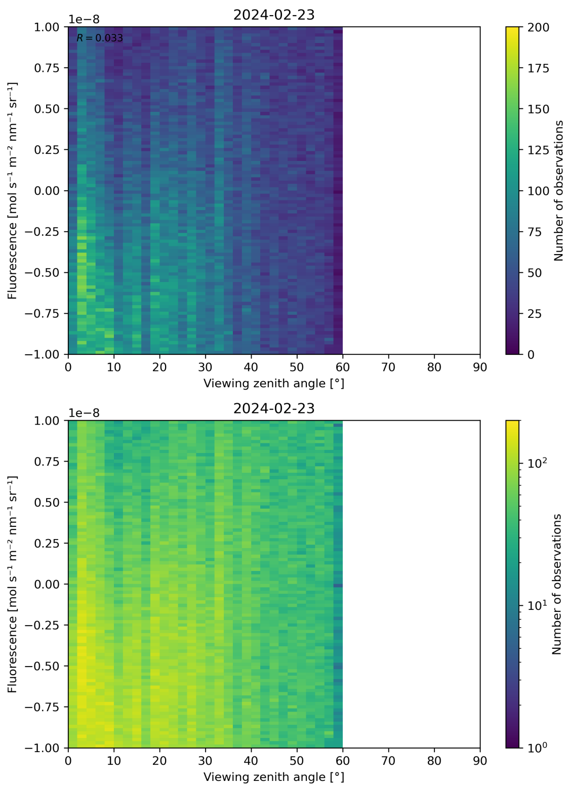
Figure 108: Scatter density plot of “Viewing zenith angle” against “Fluorescence” for 2024-02-22 to 2024-02-24.
