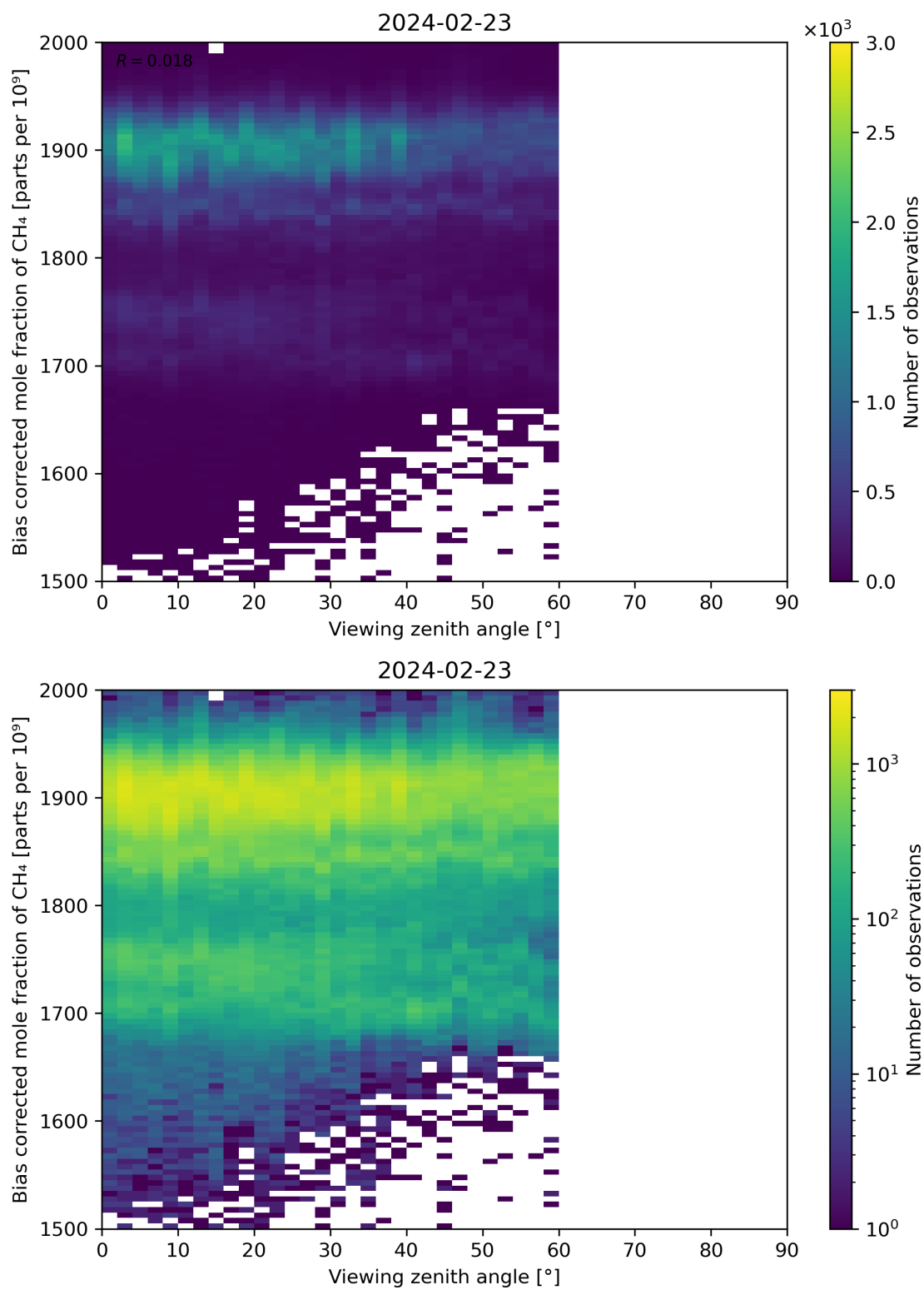
Figure 111: Scatter density plot of “Viewing zenith angle” against “Bias corrected mole fraction of CH 4 ” for 2024-02-22 to 2024-02-24.
