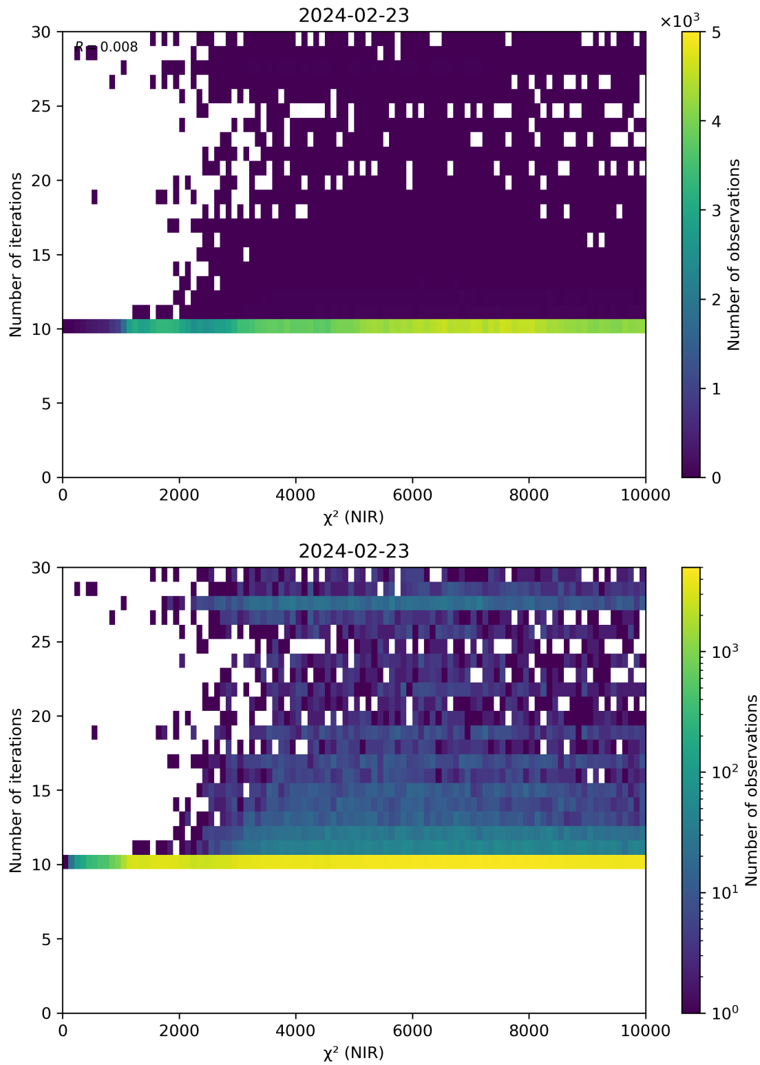
Figure 46: Scatter density plot of “ \chi^2 (NIR)” against “Number of iterations” for 2024-02-22 to 2024-02-24.
