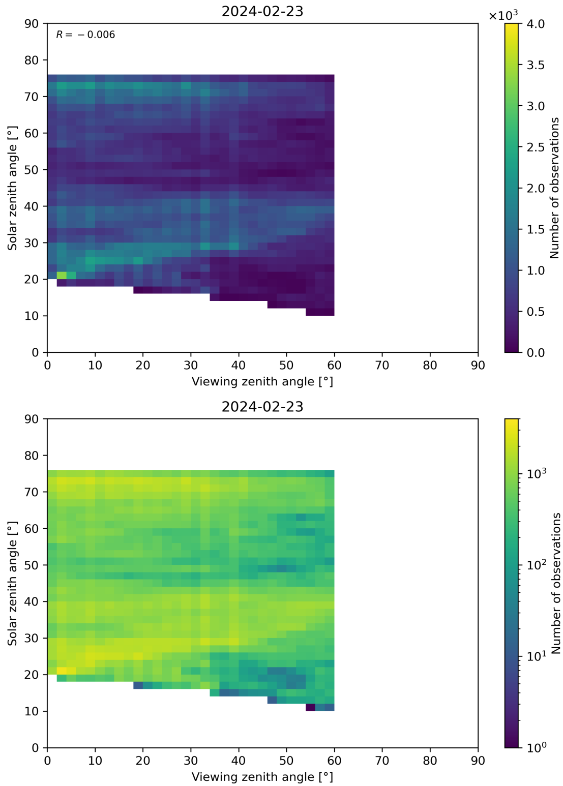
Figure 115: Scatter density plot of “Viewing zenith angle” against “Solar zenith angle” for 2024-02-22 to 2024-02-24.
