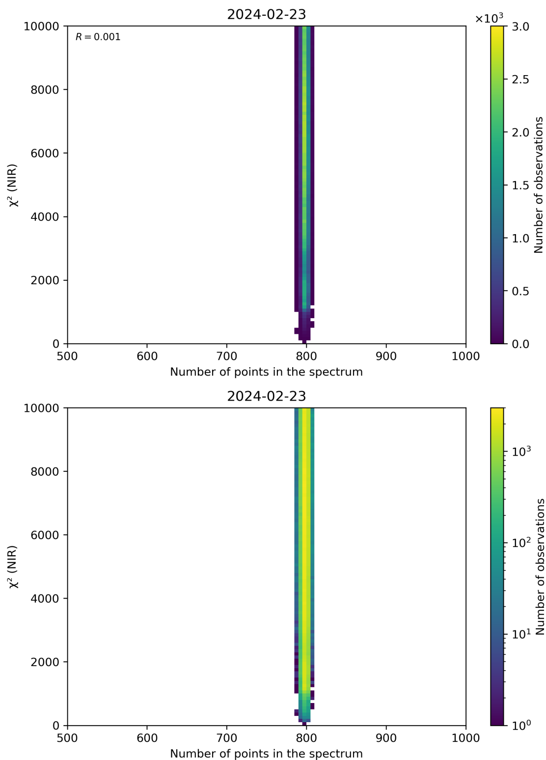
Figure 88: Scatter density plot of “Number of points in the spectrum” against “ \chi^2 (NIR)” for 2024-02-22 to 2024-02-24.
