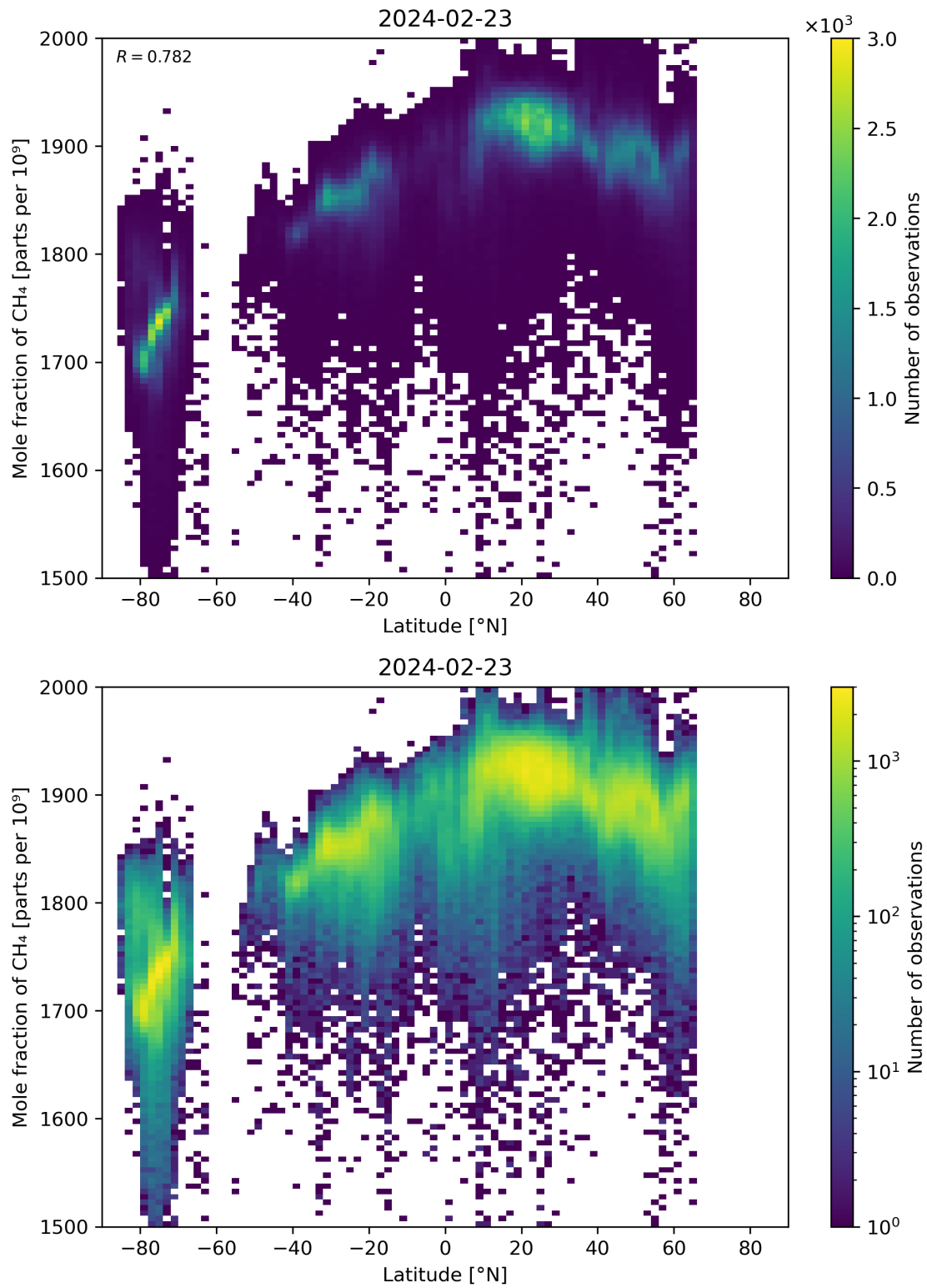
Figure 57: Scatter density plot of “Latitude” against “Mole fraction of \text{CH}_4 ” for 2024-02-22 to 2024-02-24.
