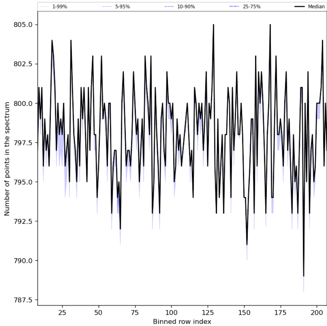
Figure 37: Along track statistics of “Number of points in the spectrum” for 2024-02-22 to 2024-02-24
