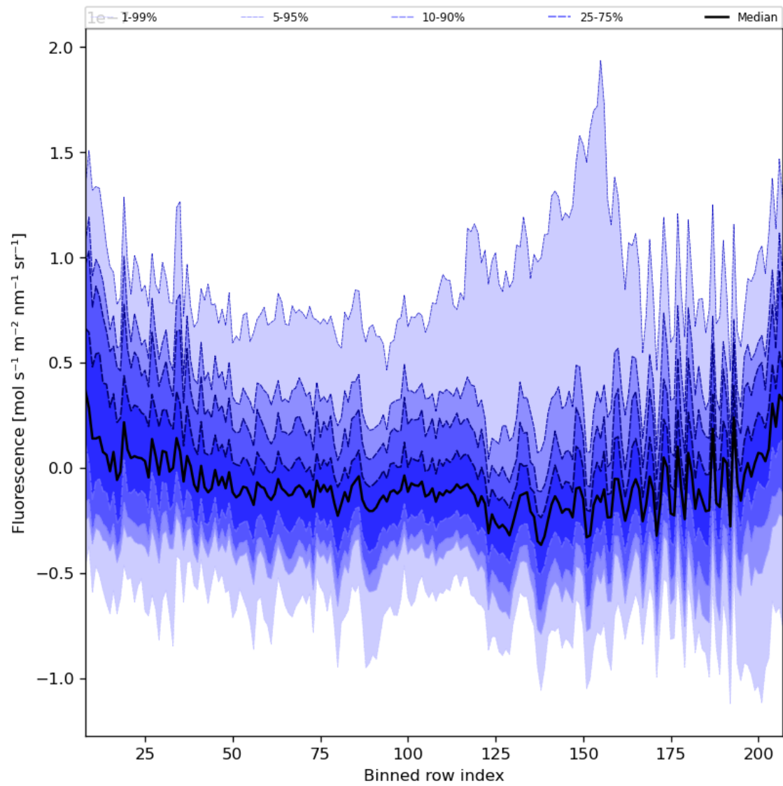
Figure 43: Along track statistics of “Fluorescence” for 2024-02-22 to 2024-02-24
