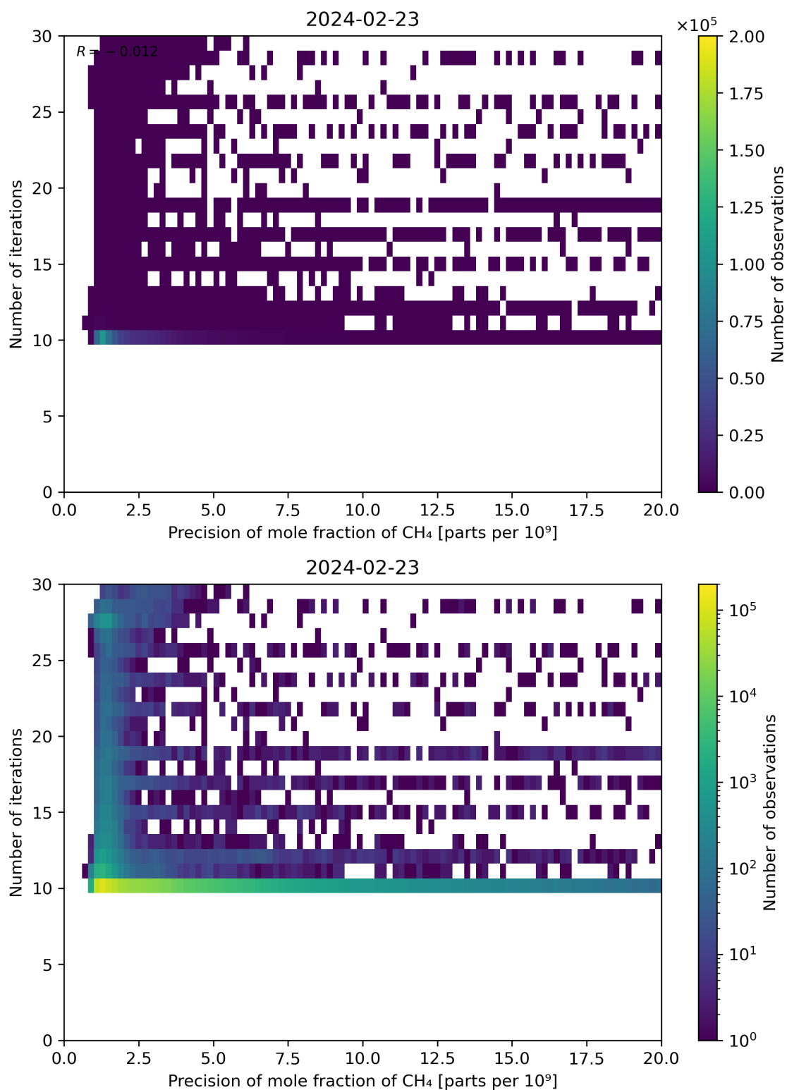
Figure 83: Scatter density plot of “Precision of mole fraction of CH 4 ” against “Number of iterations” for 2024-02-22 to 2024-02-24.
