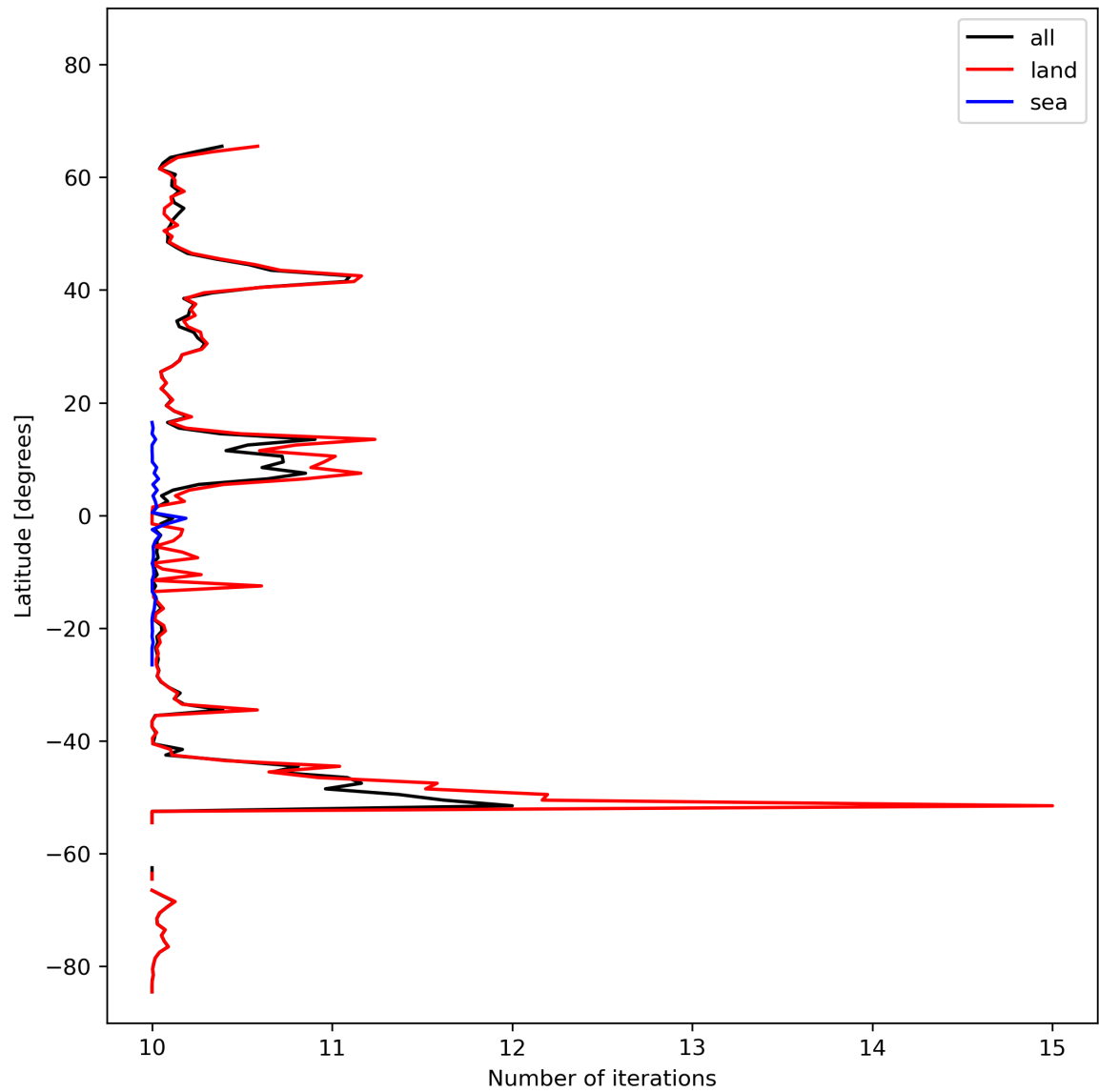
Figure 20: Zonal average of “Number of iterations” for 2024-02-22 to 2024-02-24.
