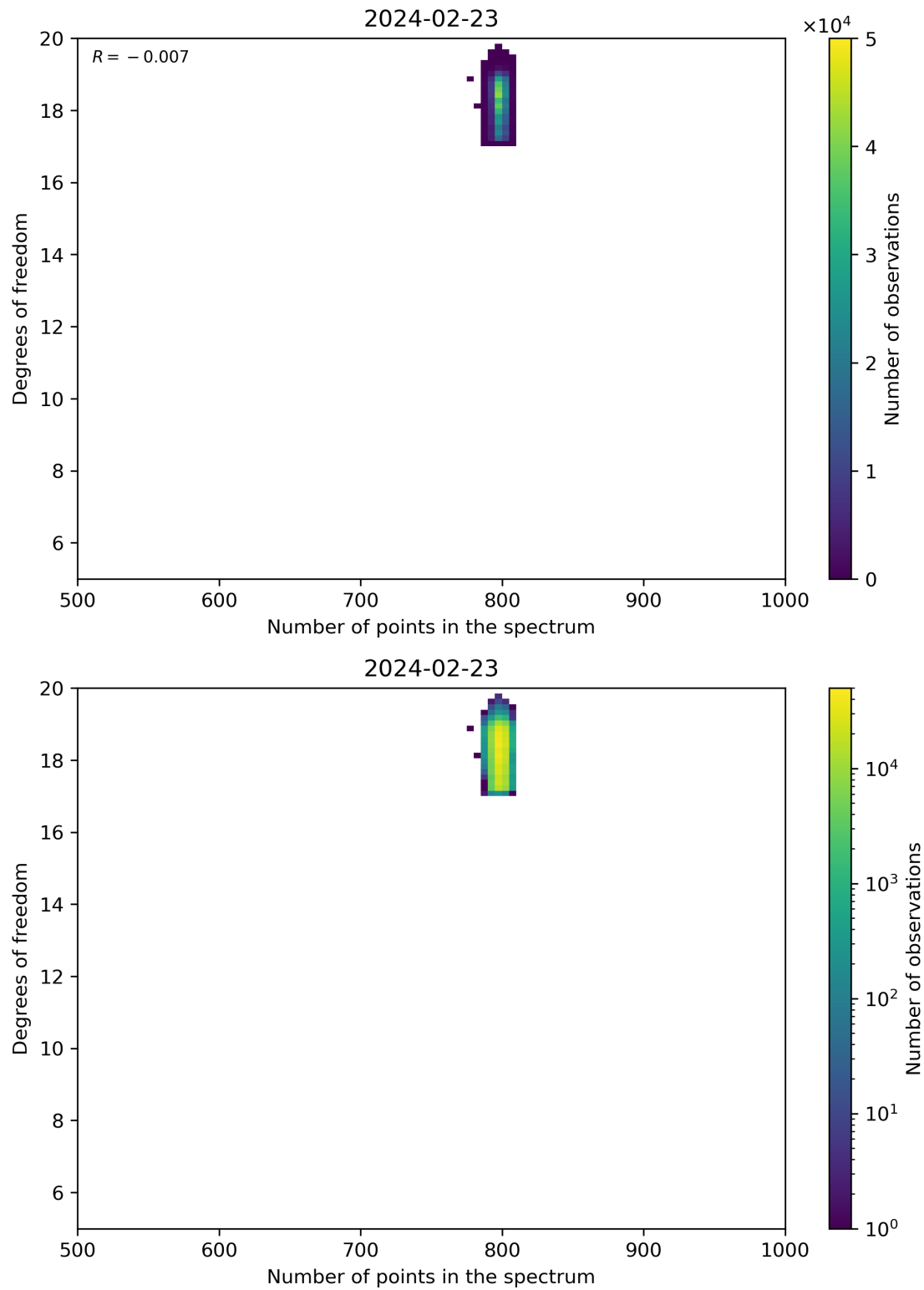
Figure 90: Scatter density plot of “Number of points in the spectrum” against “Degrees of freedom” for 2024-02-22 to 2024-02-24.
