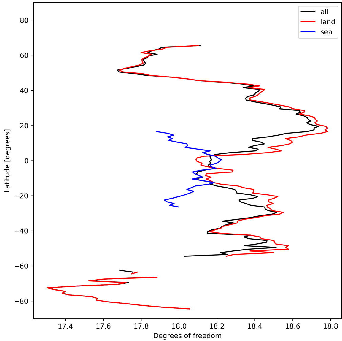
Figure 19: Zonal average of “Degrees of freedom” for 2024-02-22 to 2024-02-24.
