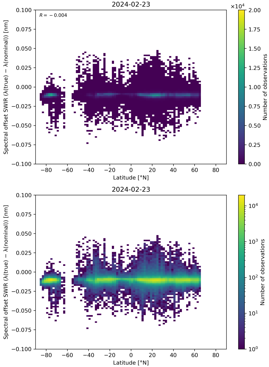
Figure 62: Scatter density plot of “Latitude” against “Spectral offset SWIR ( \lambda(\text{true}) - \lambda(\text{nominal}) )” for 2024-02-22 to 2024-02-24.
