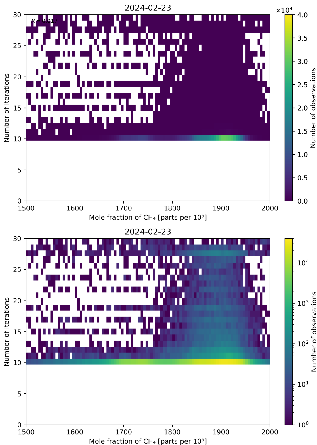
Figure 76: Scatter density plot of “Mole fraction of CH 4 ” against “Number of iterations” for 2024-02-22 to 2024-02-24.
