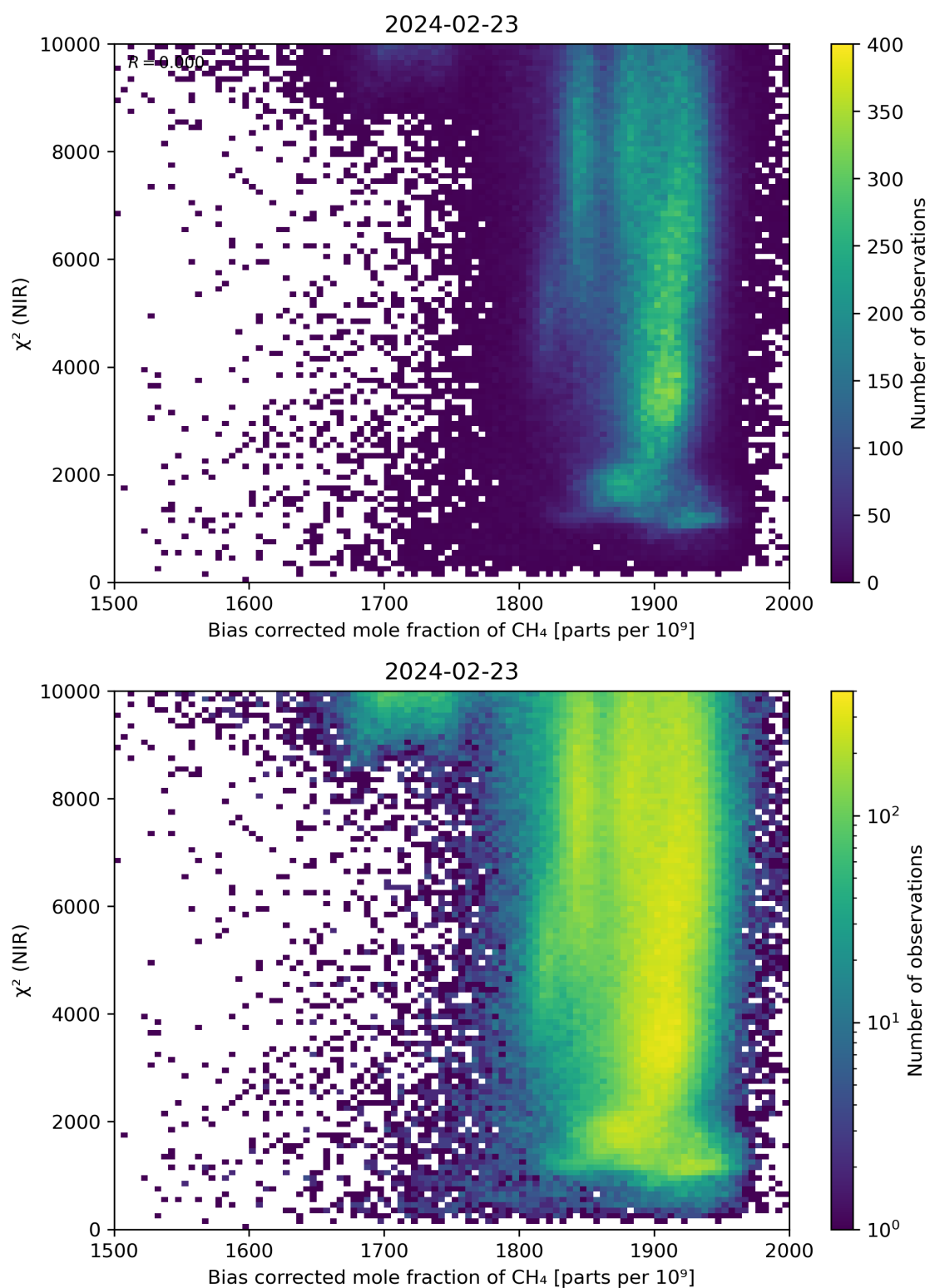
Figure 63: Scatter density plot of “Bias corrected mole fraction of \text{CH}_4 ” against “ \chi^2 (NIR)” for 2024-02-22 to 2024-02-24.
