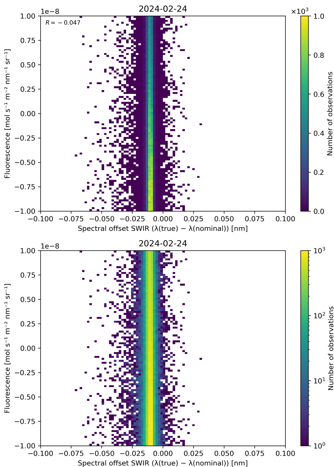
Figure 120: Scatter density plot of “Spectral offset SWIR ( \lambda(\text{true}) - \lambda(\text{nominal}) )” against “Fluorescence” for 2024-02-23 to 2024-02-25.
