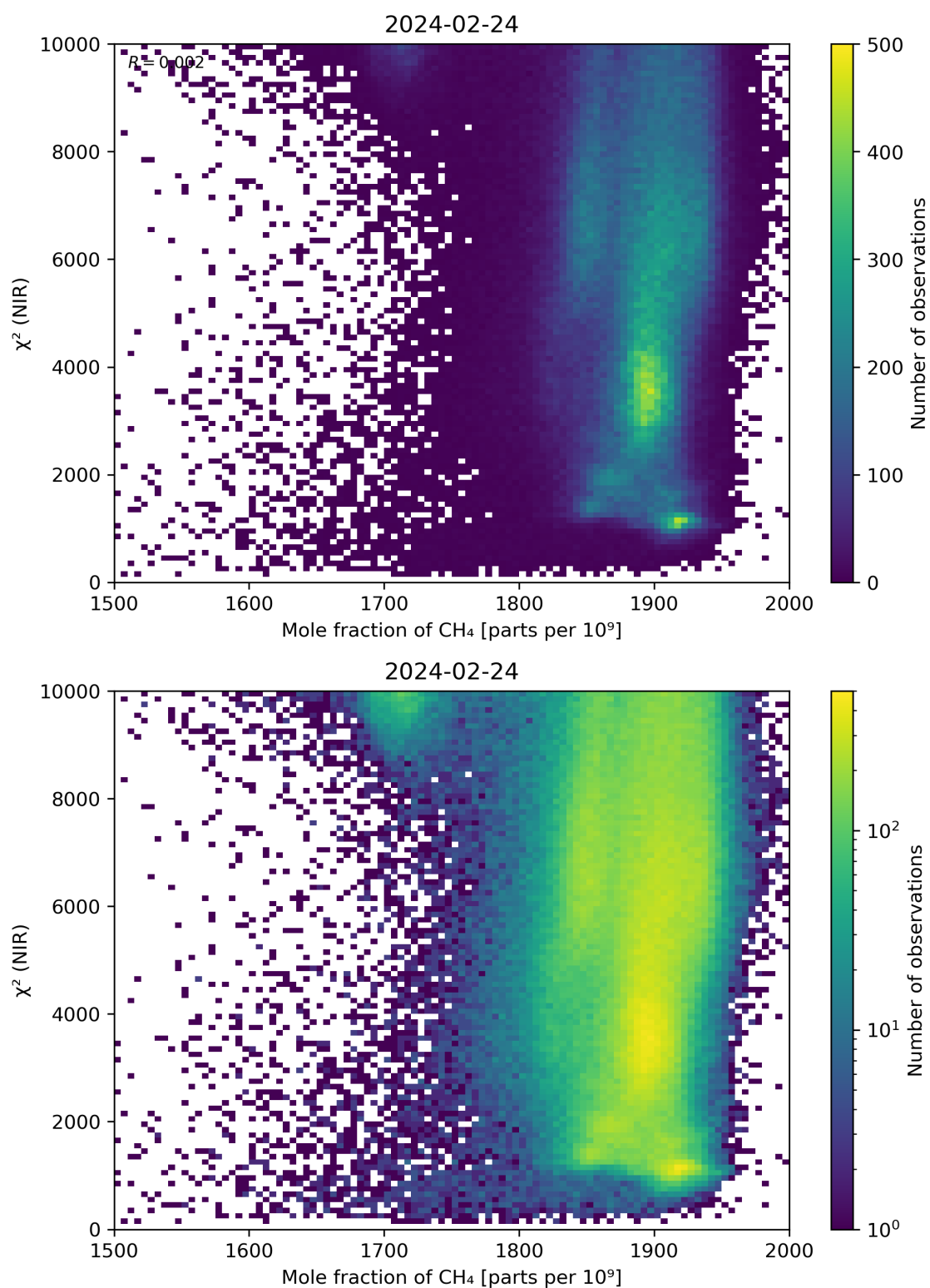
Figure 70: Scatter density plot of “Mole fraction of CH 4 ” against “ \chi^2 (NIR)” for 2024-02-23 to 2024-02-25.
