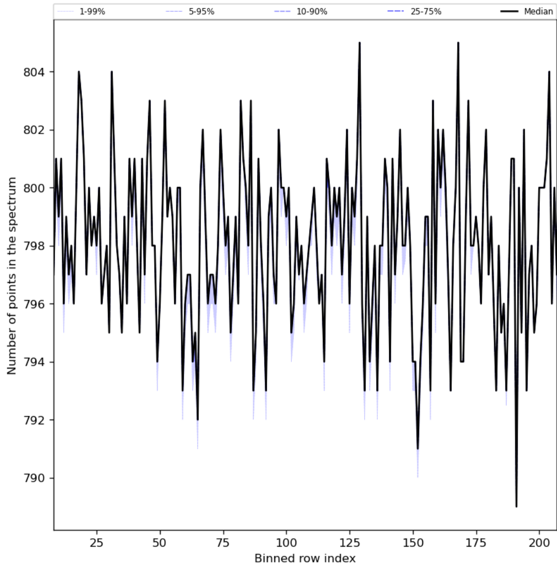
Figure 37: Along track statistics of “Number of points in the spectrum” for 2024-02-23 to 2024-02-25
