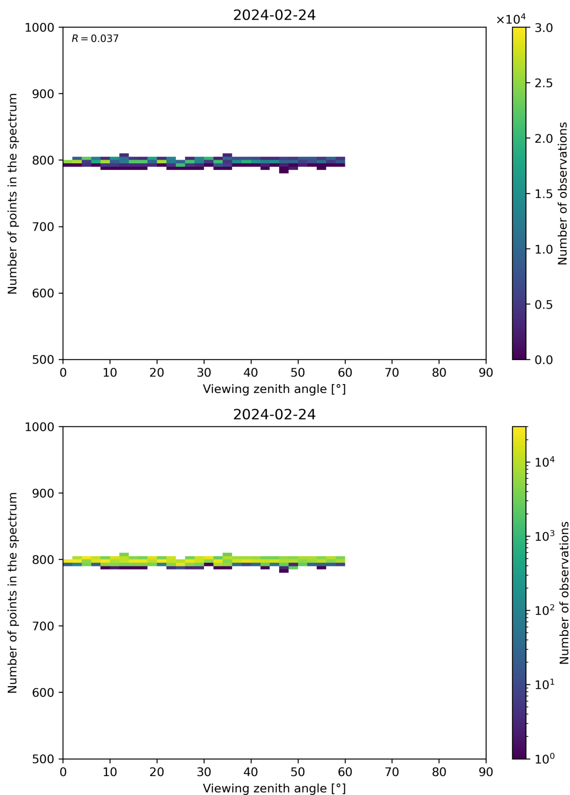
Figure 114: Scatter density plot of “Viewing zenith angle” against “Number of points in the spectrum” for 2024-02-23 to 2024-02-25.
