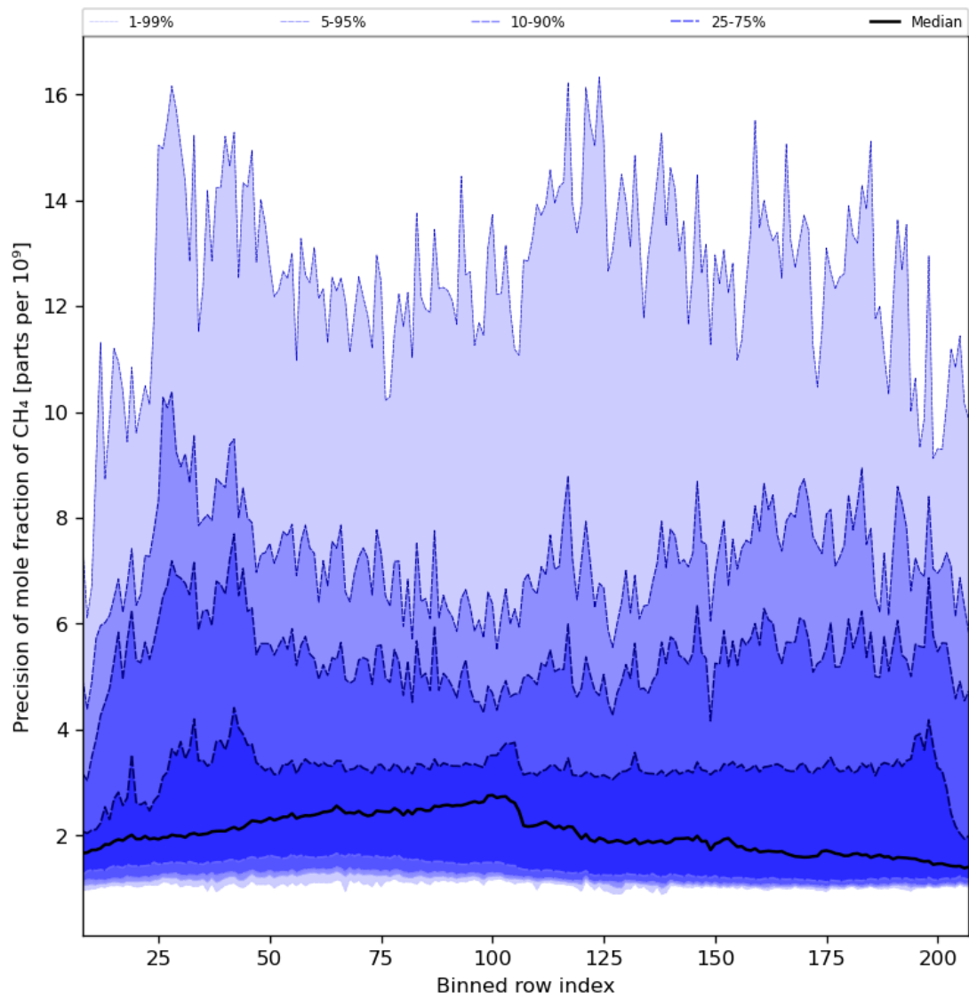
Figure 35: Along track statistics of “Precision of mole fraction of CH 4 ” for 2024-02-23 to 2024-02-25
