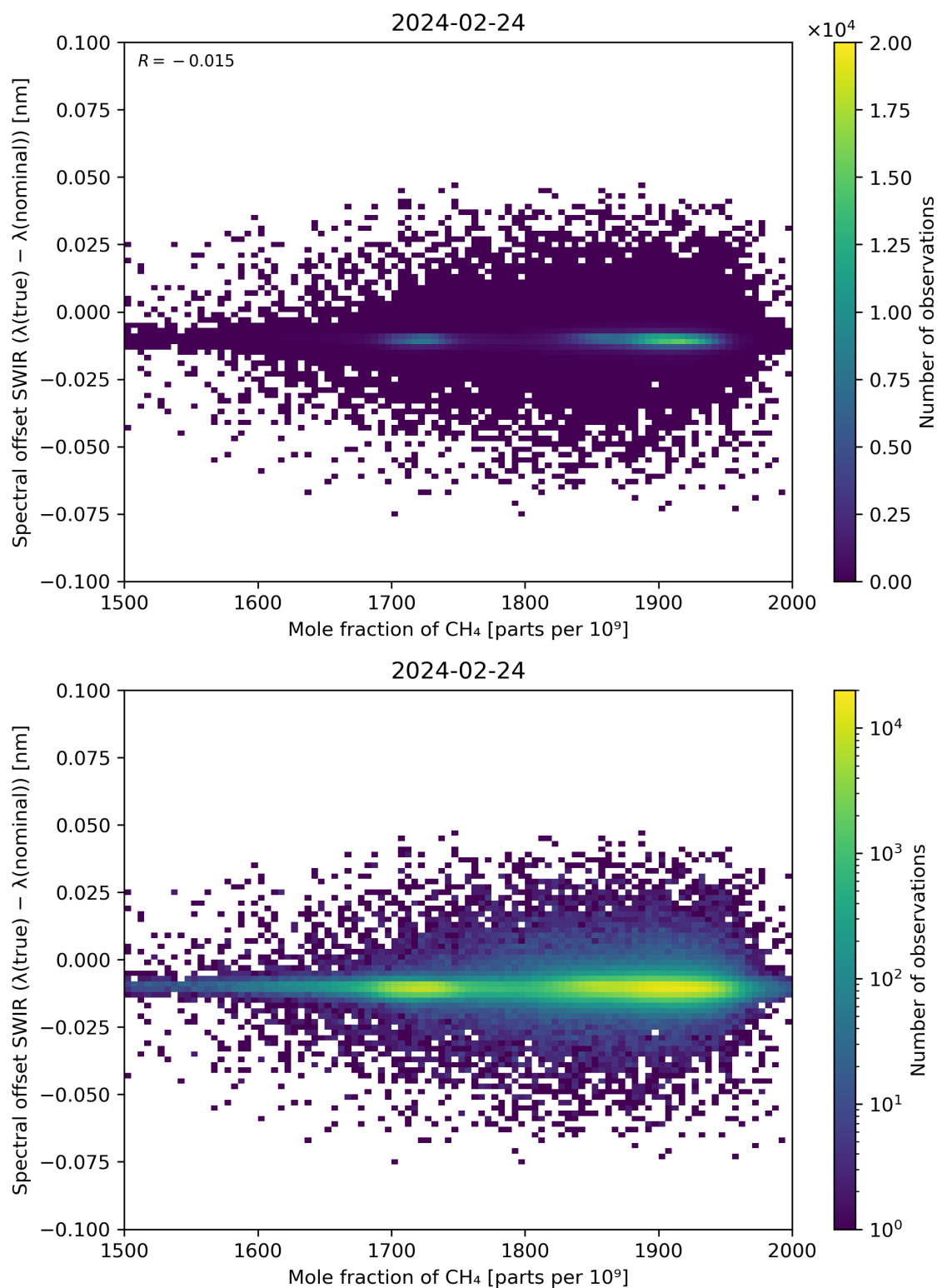
Figure 86: Scatter density plot of “Mole fraction of CH 4 ” against “Spectral offset SWIR ( \lambda(\text{true}) - \lambda(\text{nominal}) )” for 2024-02-23 to 2024-02-25.
