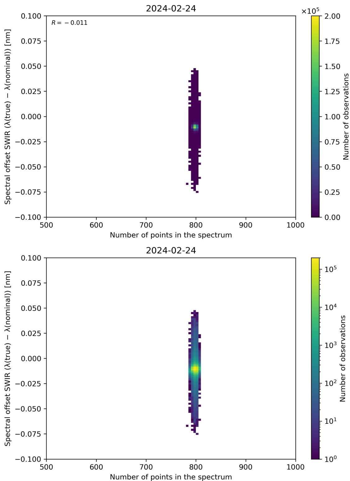
Figure 93: Scatter density plot of “Number of points in the spectrum” against “Spectral offset SWIR ( \lambda(\text{true}) - \lambda(\text{nominal}) )” for 2024-02-23 to 2024-02-25.
