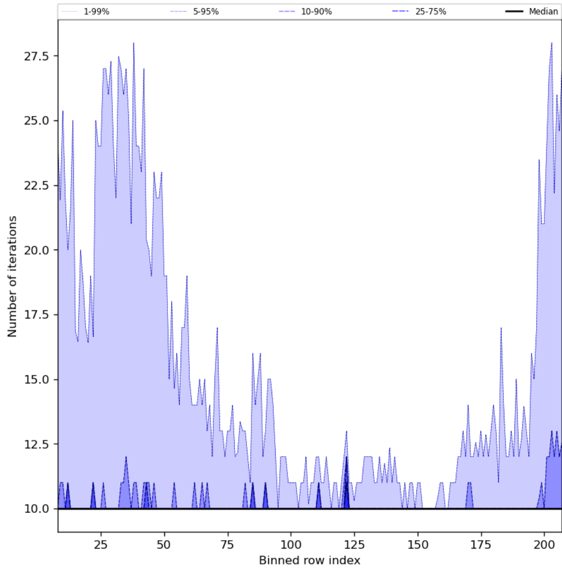
Figure 42: Along track statistics of “Number of iterations” for 2024-02-23 to 2024-02-25
