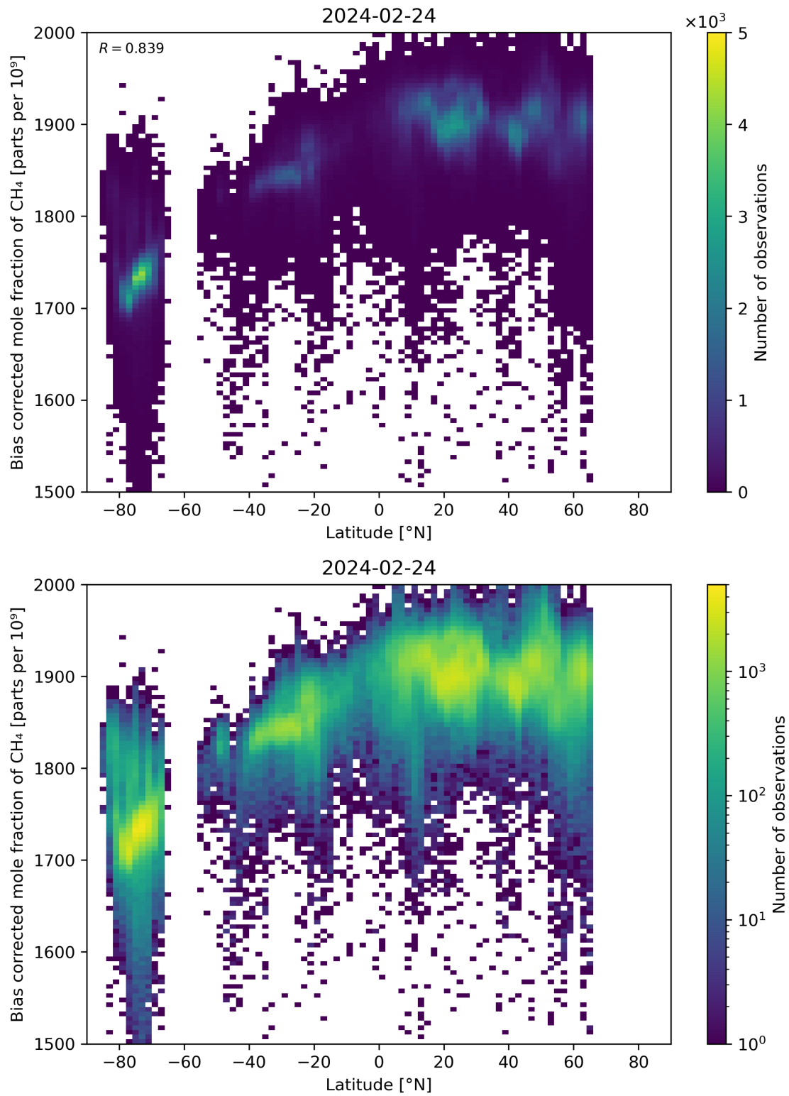
Figure 58: Scatter density plot of “Latitude” against “Bias corrected mole fraction of CH 4 ” for 2024-02-23 to 2024-02-25.
