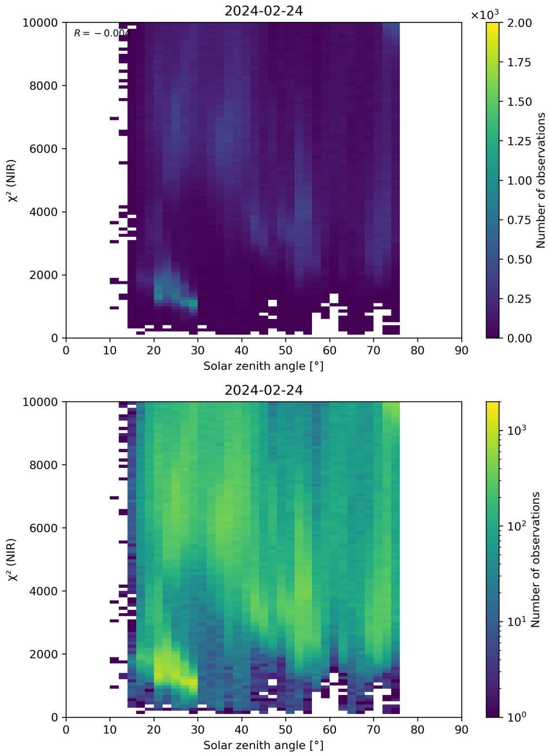
Figure 94: Scatter density plot of “Solar zenith angle” against “ \chi^2 (NIR)” for 2024-02-23 to 2024-02-25.
