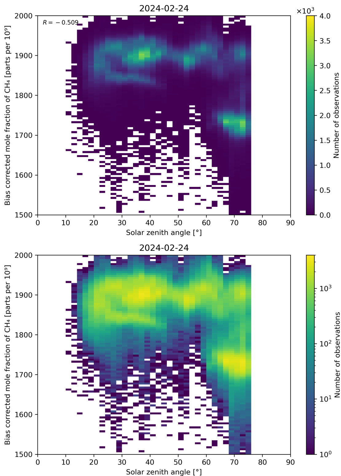
Figure 100: Scatter density plot of “Solar zenith angle” against “Bias corrected mole fraction of CH 4 ” for 2024-02-23 to 2024-02-25.
