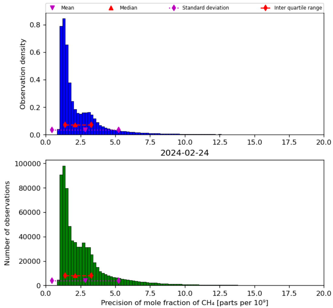
Figure 24: Histogram of “Precision of mole fraction of CH 4 ” for 2024-02-23 to 2024-02-25
