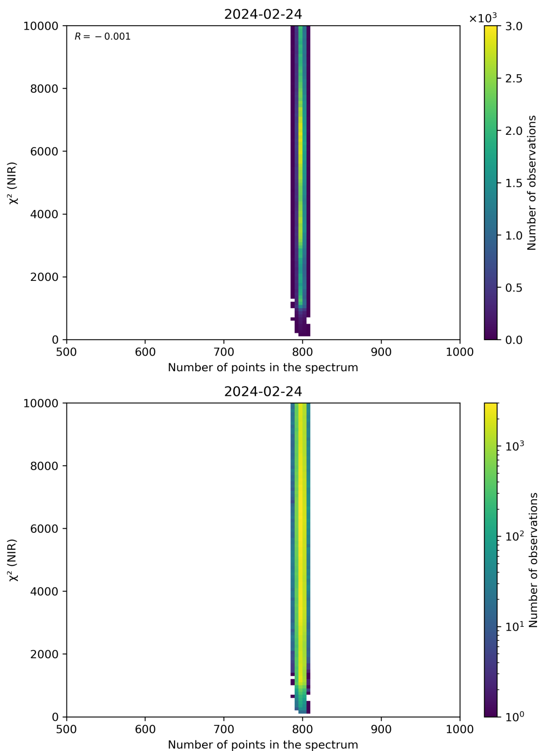
Figure 88: Scatter density plot of “Number of points in the spectrum” against “ \chi^2 (NIR)” for 2024-02-23 to 2024-02-25.
