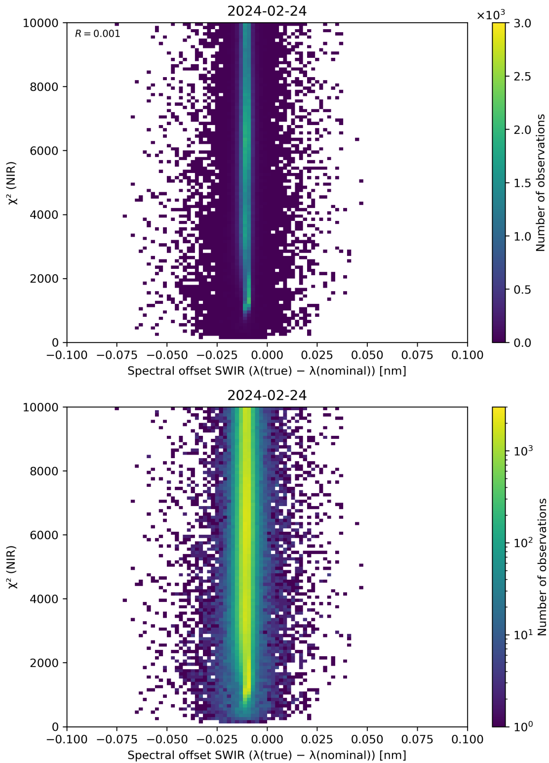
Figure 117: Scatter density plot of “Spectral offset SWIR ( \lambda(\text{true}) - \lambda(\text{nominal}) )” against “ \chi^2 (NIR)” for 2024-02-23 to 2024-02-25.
