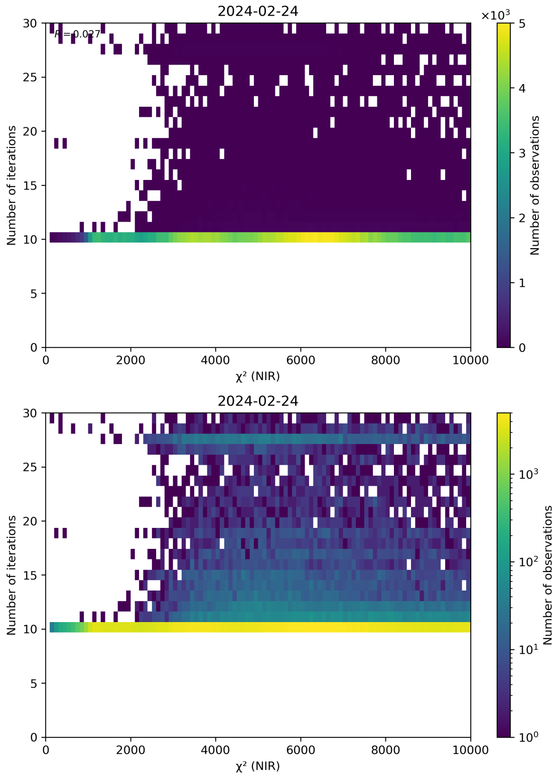
Figure 46: Scatter density plot of “ \chi^2 (NIR)” against “Number of iterations” for 2024-02-23 to 2024-02-25.
