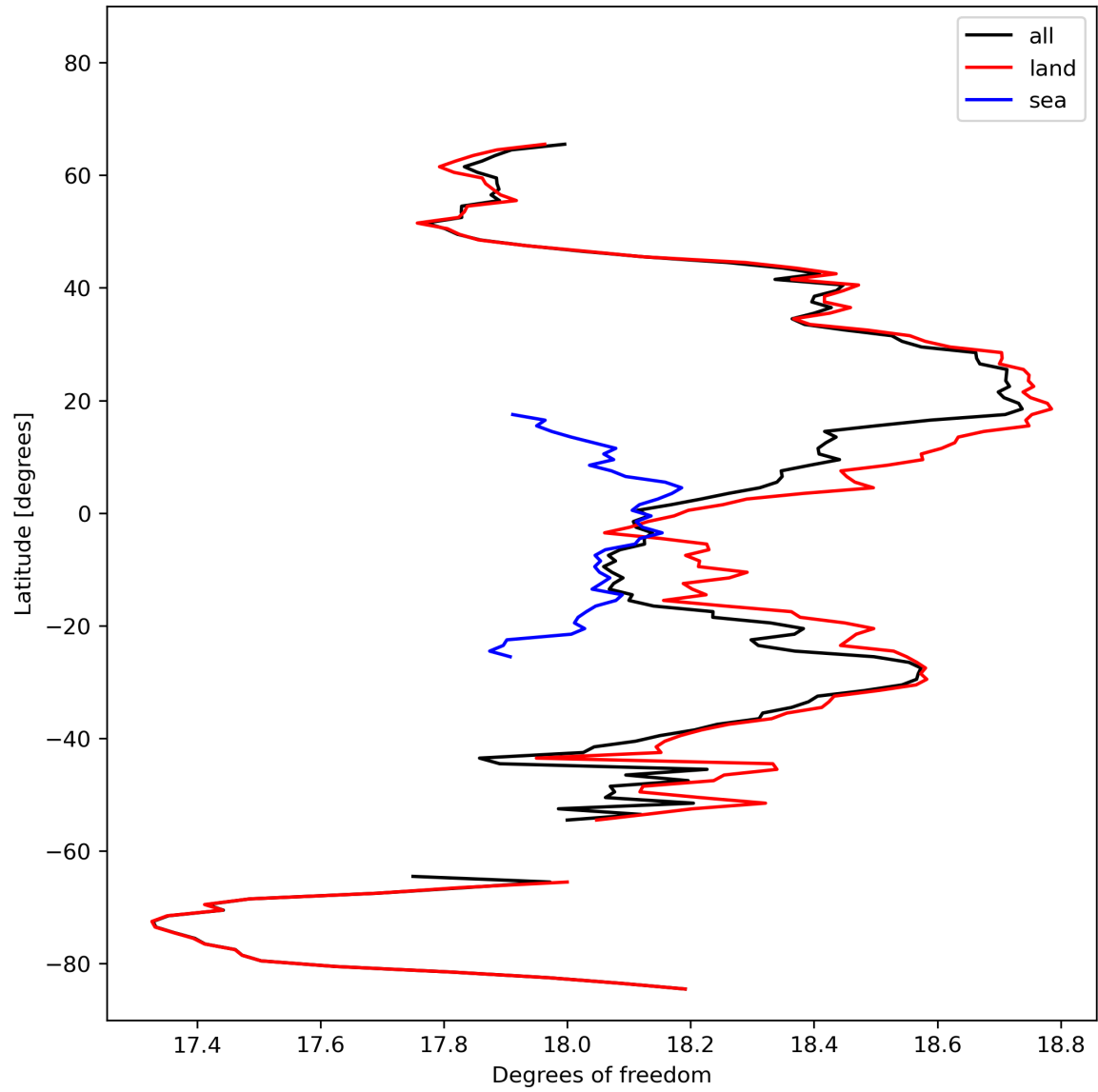
Figure 19: Zonal average of “Degrees of freedom” for 2024-02-23 to 2024-02-25.
