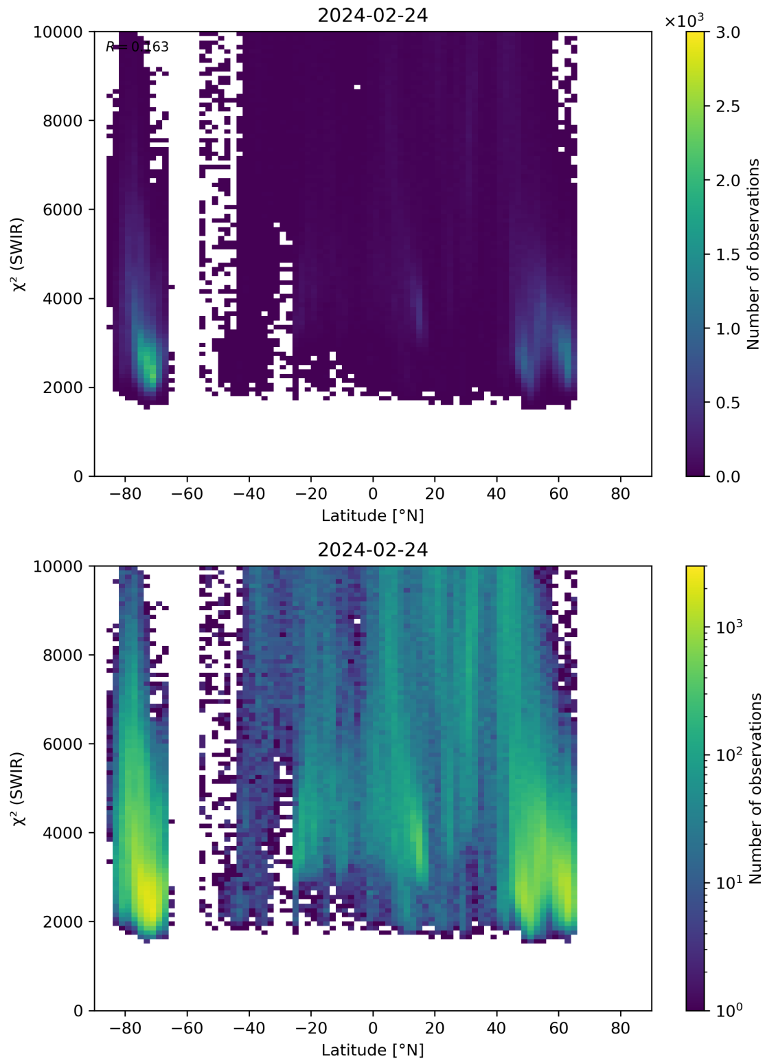
Figure 54: Scatter density plot of “Latitude” against “ \chi^2 (SWIR)” for 2024-02-23 to 2024-02-25.
