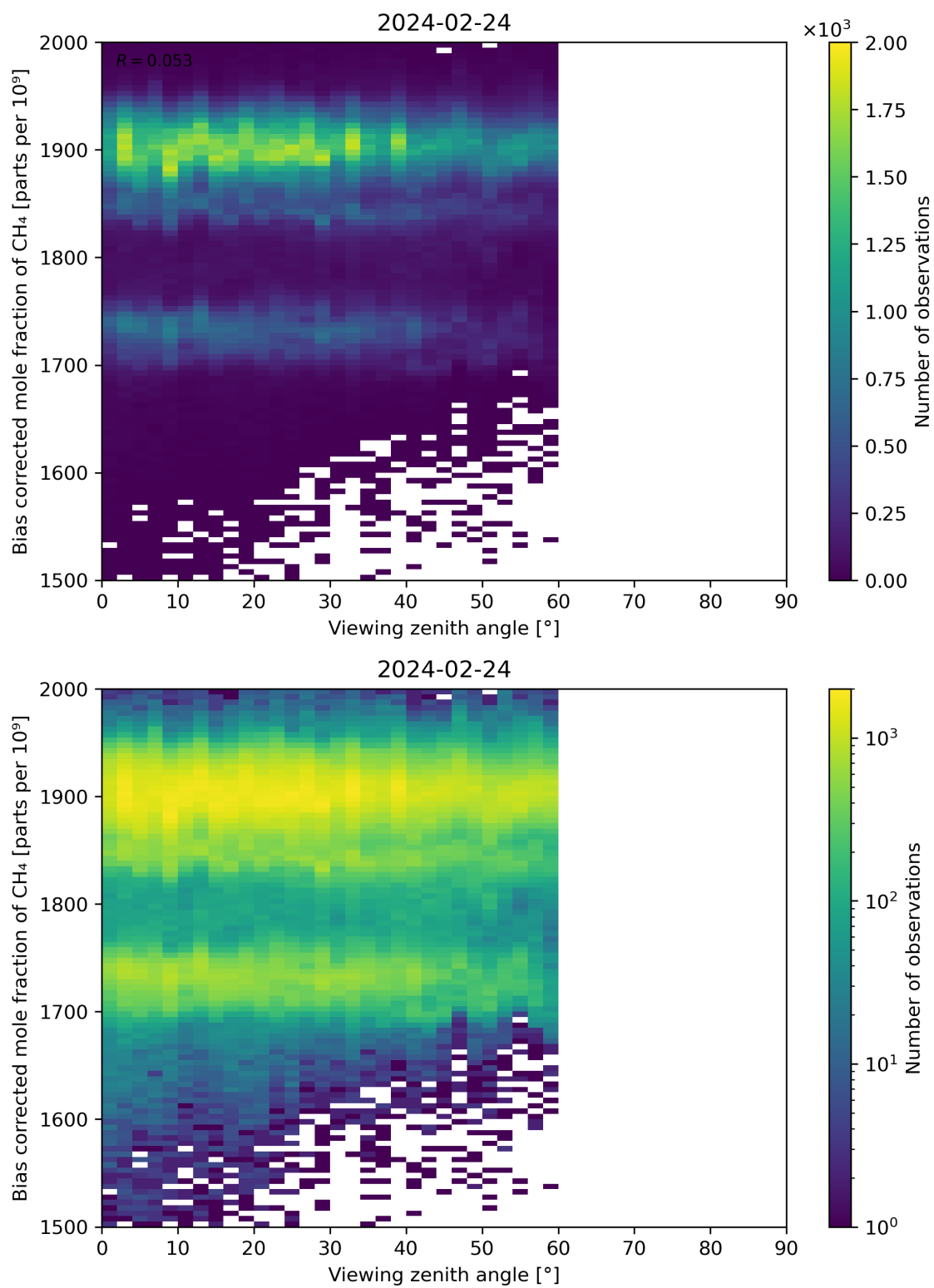
Figure 111: Scatter density plot of “Viewing zenith angle” against “Bias corrected mole fraction of CH 4 ” for 2024-02-23 to 2024-02-25.
