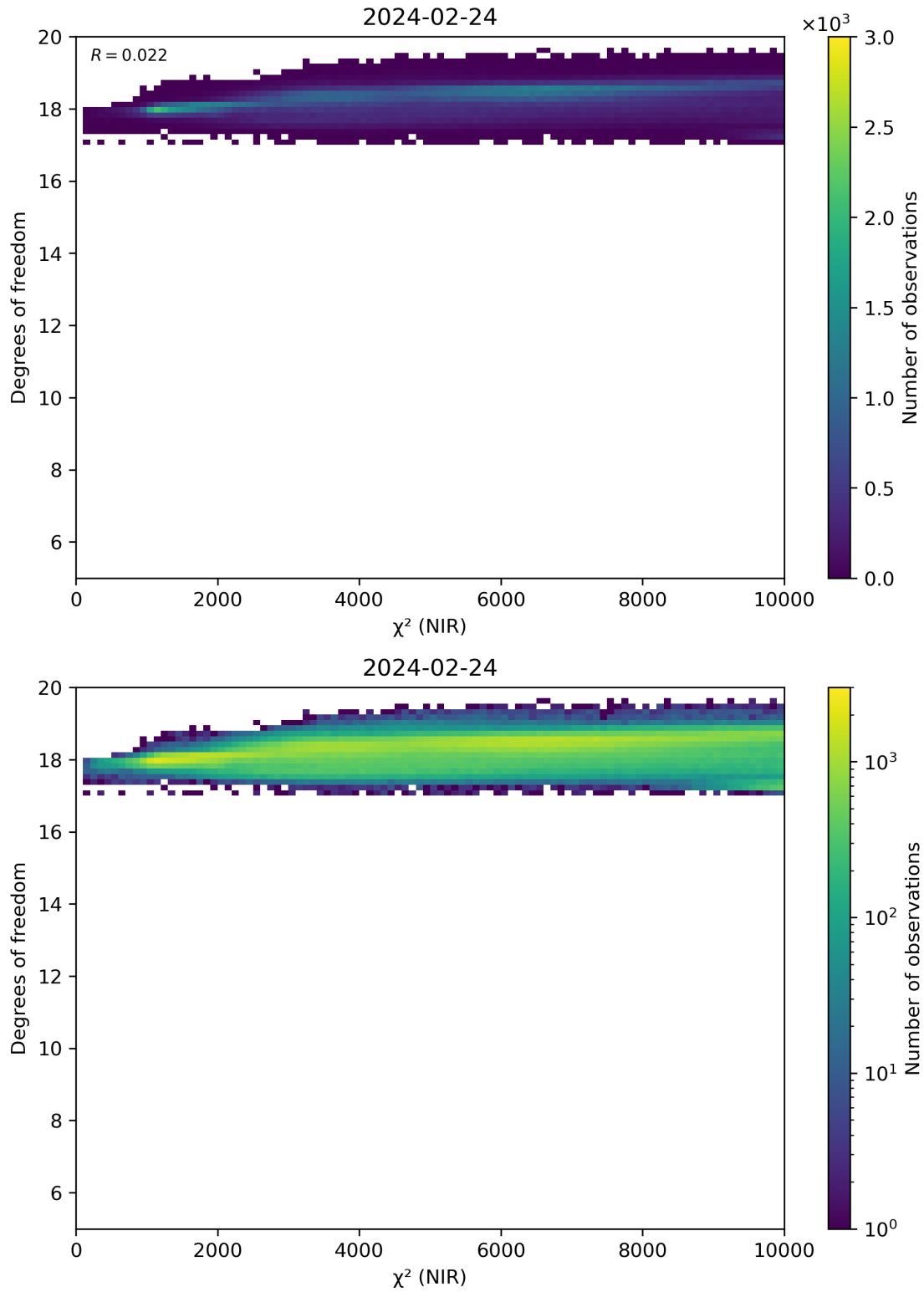
Figure 44: Scatter density plot of “ \chi^2 (NIR)” against “Degrees of freedom” for 2024-02-23 to 2024-02-25.
