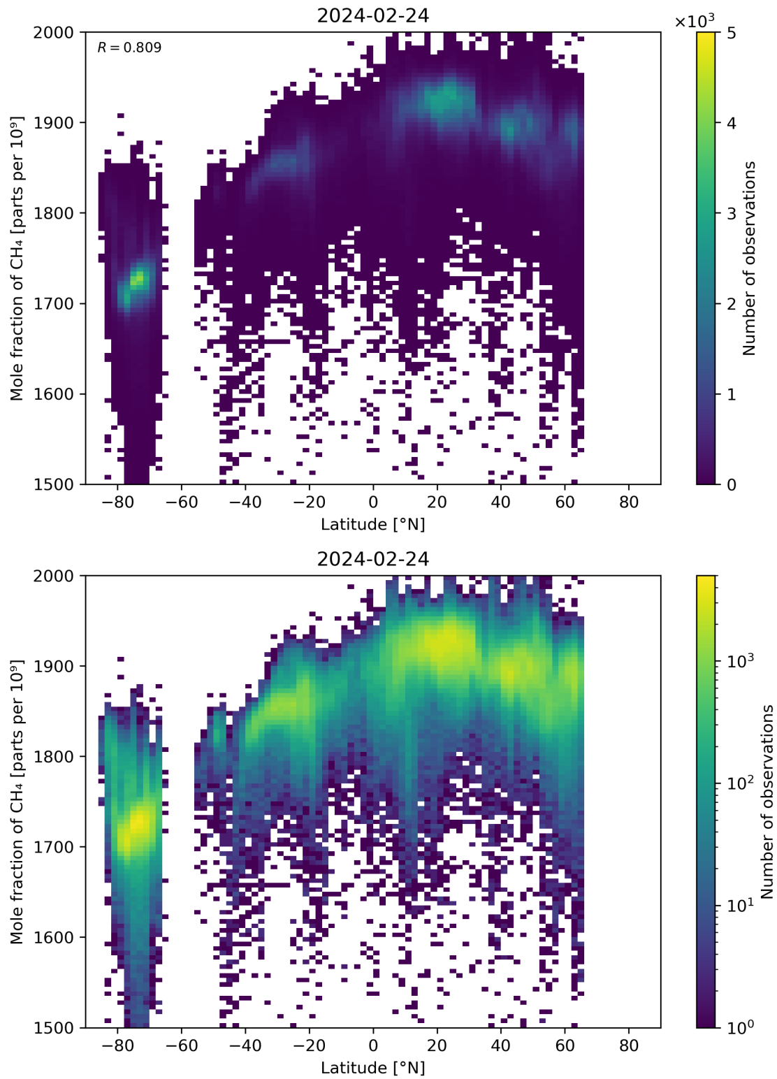
Figure 57: Scatter density plot of “Latitude” against “Mole fraction of CH 4 ” for 2024-02-23 to 2024-02-25.
