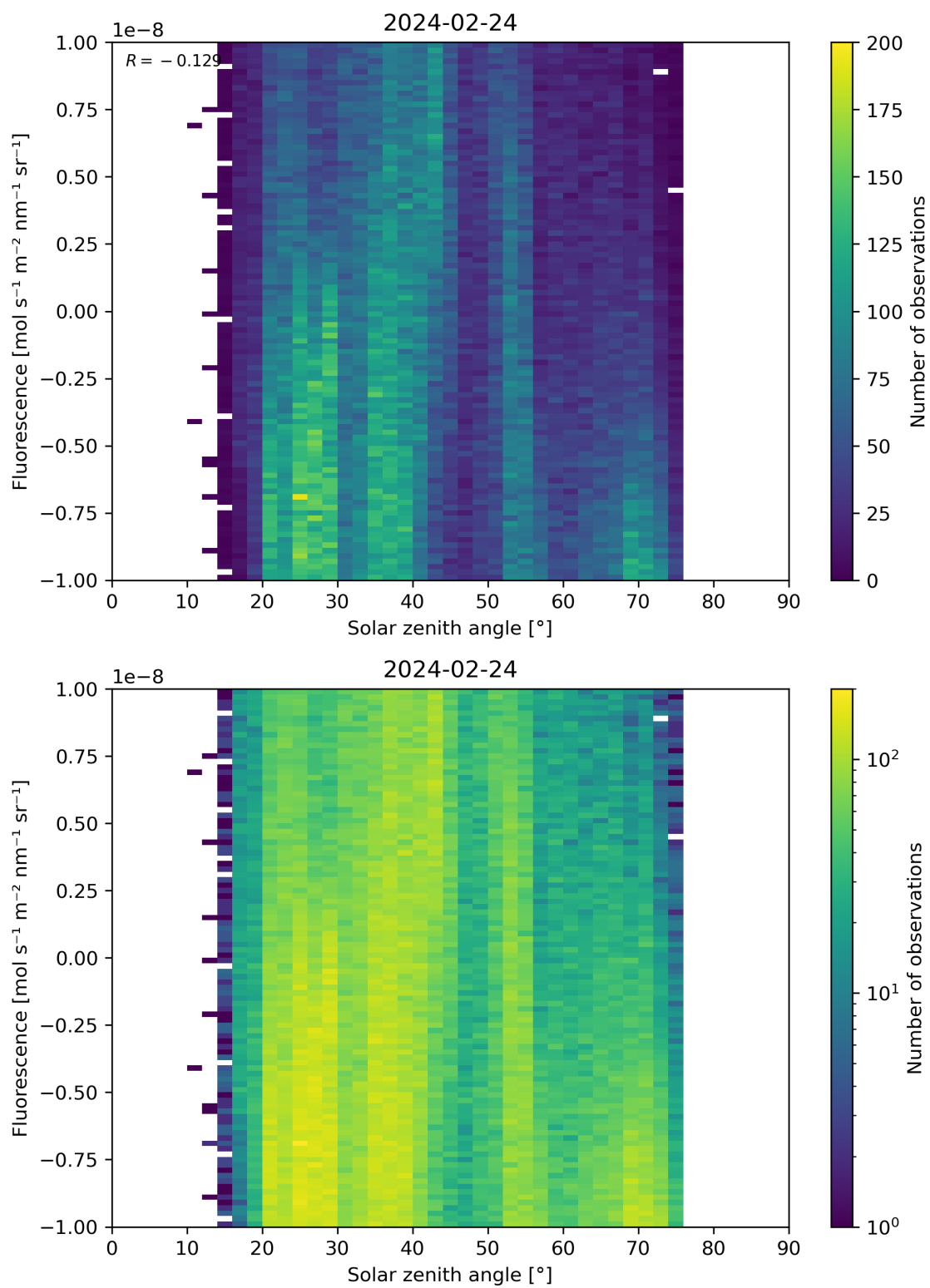
Figure 97: Scatter density plot of “Solar zenith angle” against “Fluorescence” for 2024-02-23 to 2024-02-25.
