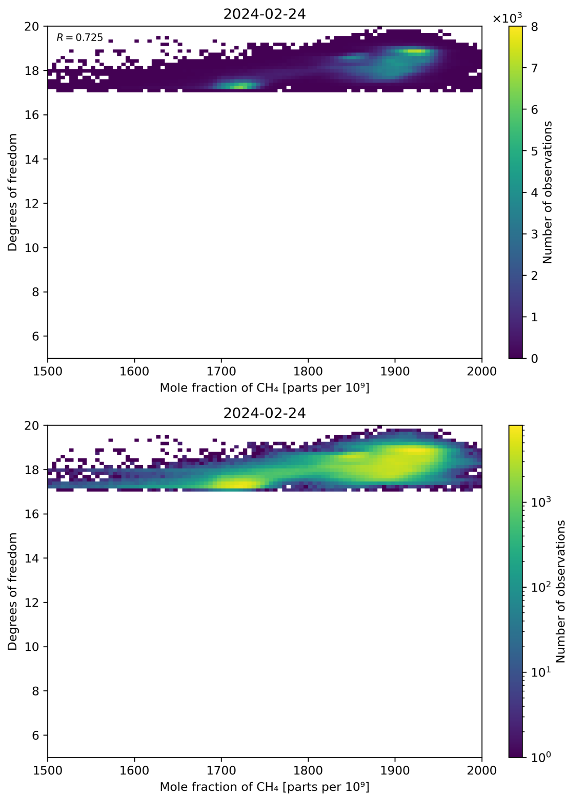
Figure 72: Scatter density plot of “Mole fraction of CH 4 ” against “Degrees of freedom” for 2024-02-23 to 2024-02-25.
