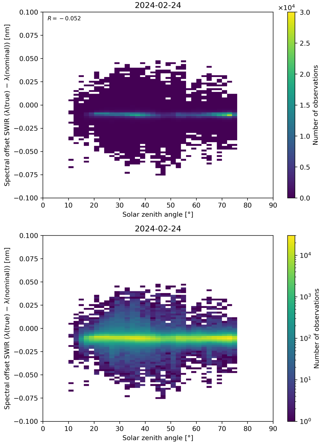
Figure 104: Scatter density plot of “Solar zenith angle” against “Spectral offset SWIR ( \lambda(\text{true}) - \lambda(\text{nominal}) )” for 2024-02-23 to 2024-02-25.
