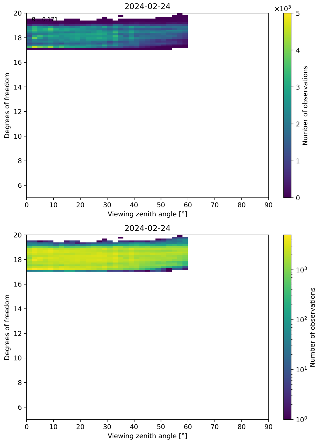
Figure 107: Scatter density plot of “Viewing zenith angle” against “Degrees of freedom” for 2024-02-23 to 2024-02-25.
