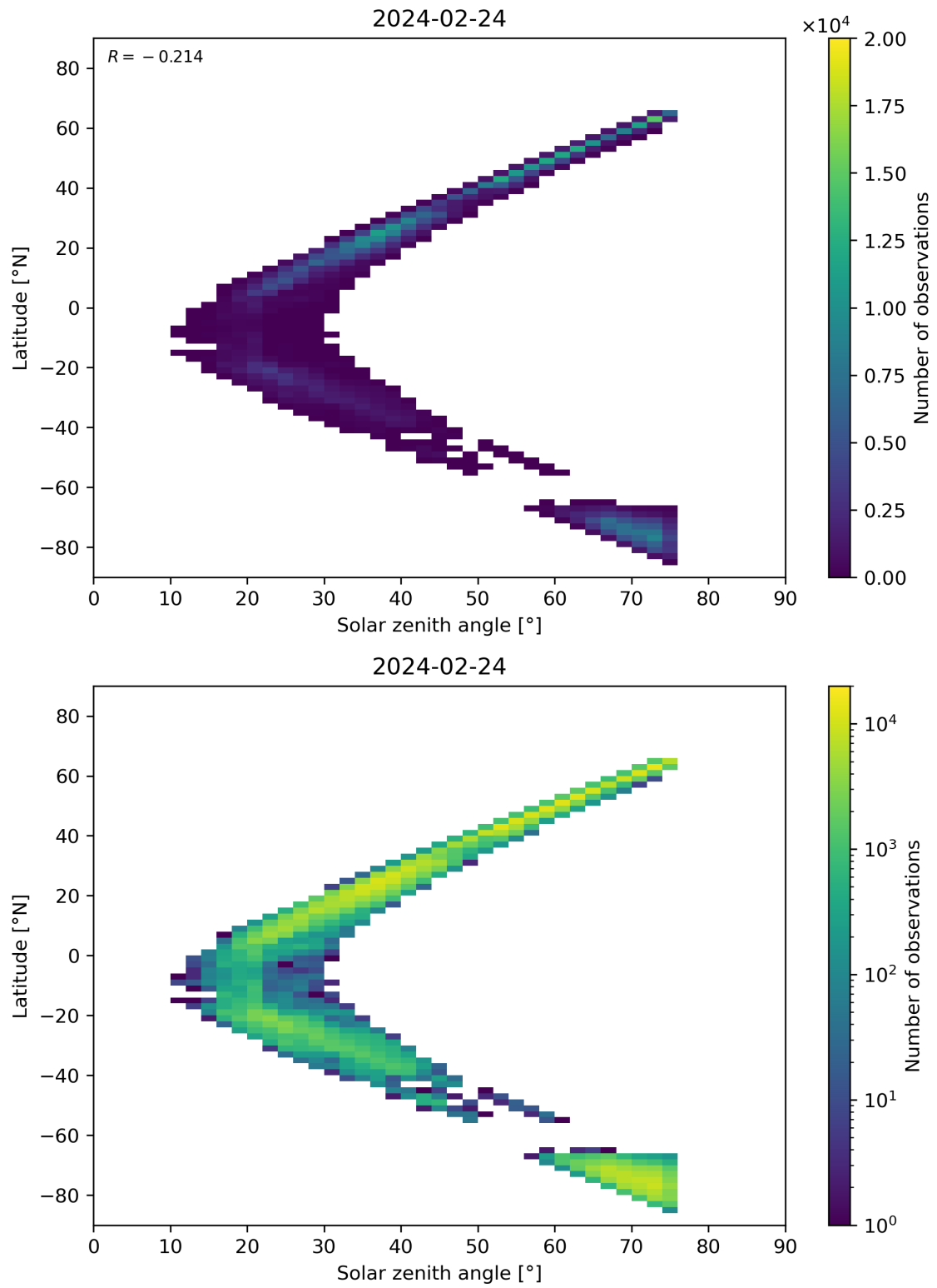
Figure 98: Scatter density plot of “Solar zenith angle” against “Latitude” for 2024-02-23 to 2024-02-25.
