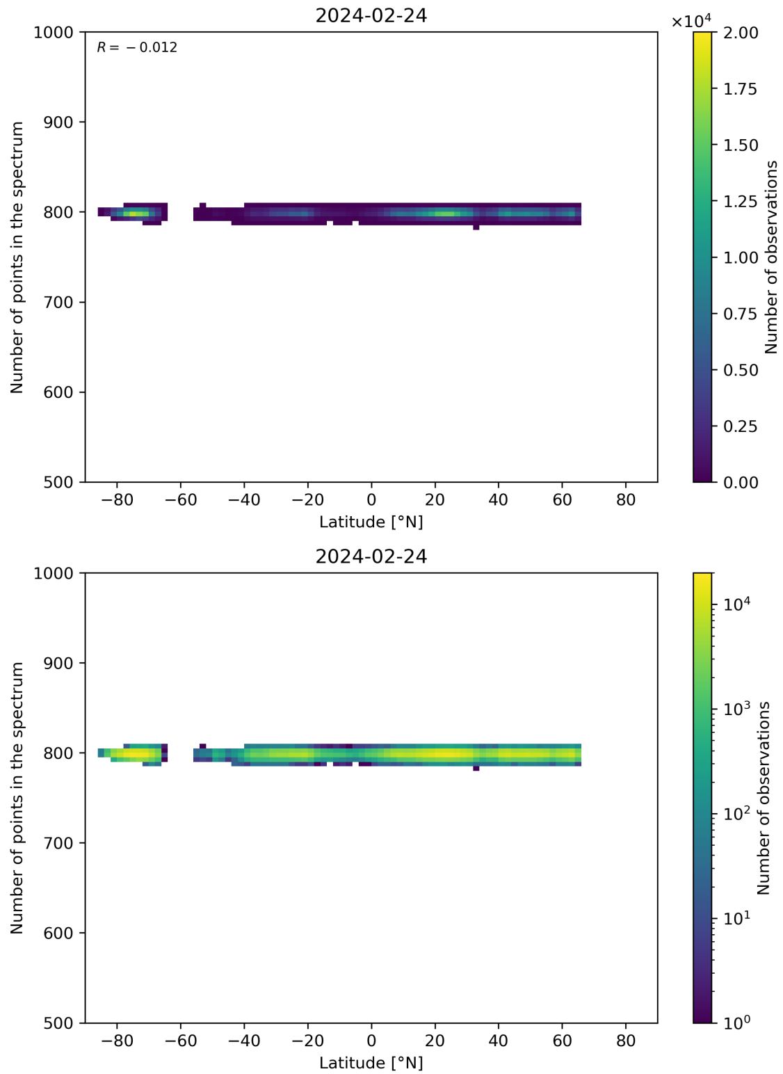
Figure 61: Scatter density plot of “Latitude” against “Number of points in the spectrum” for 2024-02-23 to 2024-02-25.
