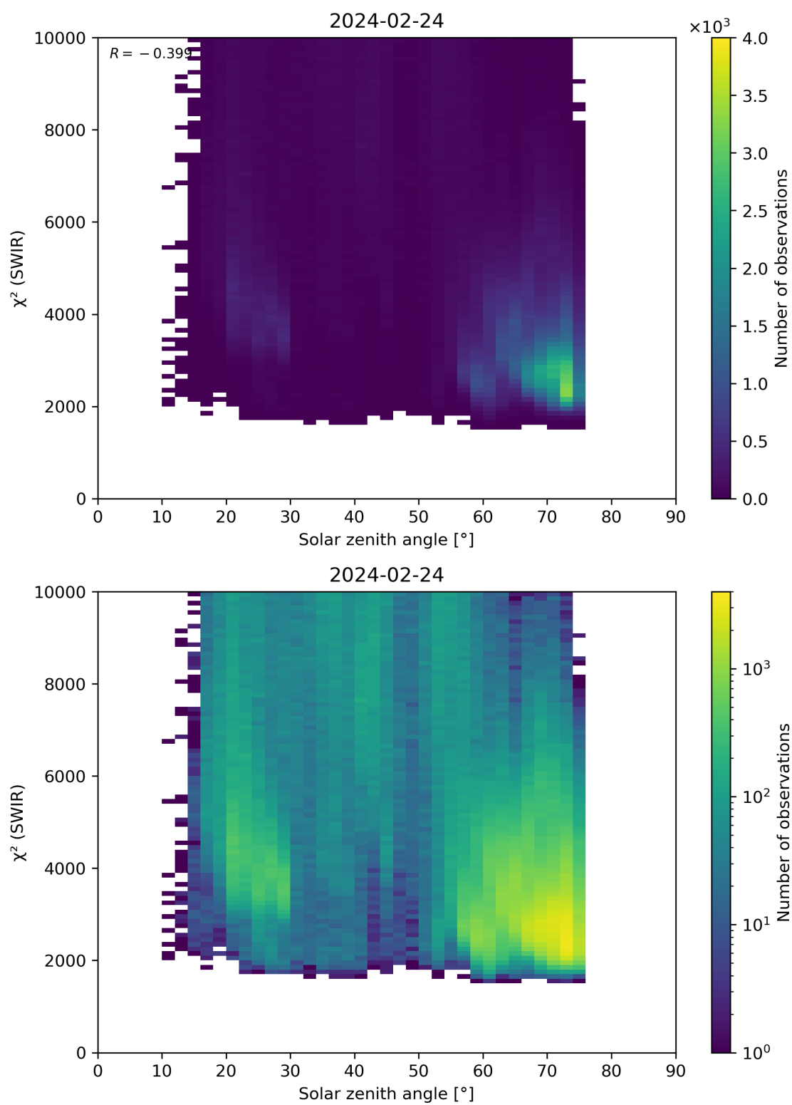
Figure 95: Scatter density plot of “Solar zenith angle” against “ \chi^2 (SWIR)” for 2024-02-23 to 2024-02-25.
