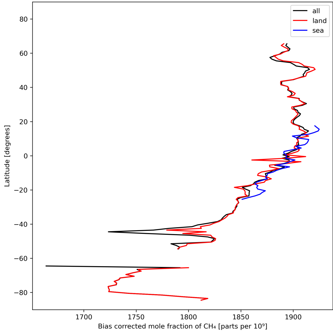
Figure 14: Zonal average of “Bias corrected mole fraction of CH 4 ” for 2024-02-23 to 2024-02-25.
