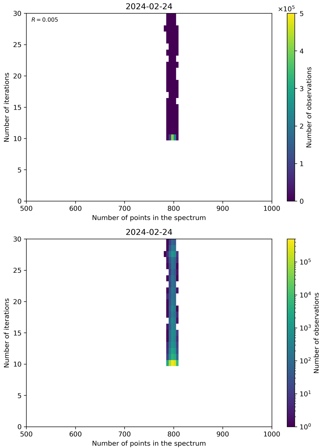
Figure 92: Scatter density plot of “Number of points in the spectrum” against “Number of iterations” for 2024-02-23 to 2024-02-25.
