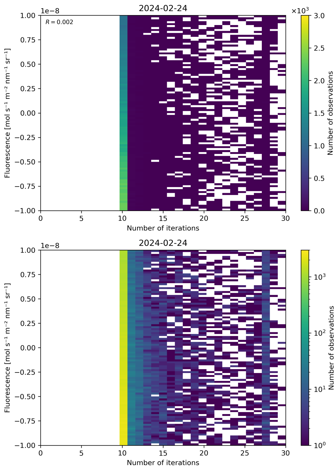
Figure 87: Scatter density plot of “Number of iterations” against “Fluorescence” for 2024-02-23 to 2024-02-25.
