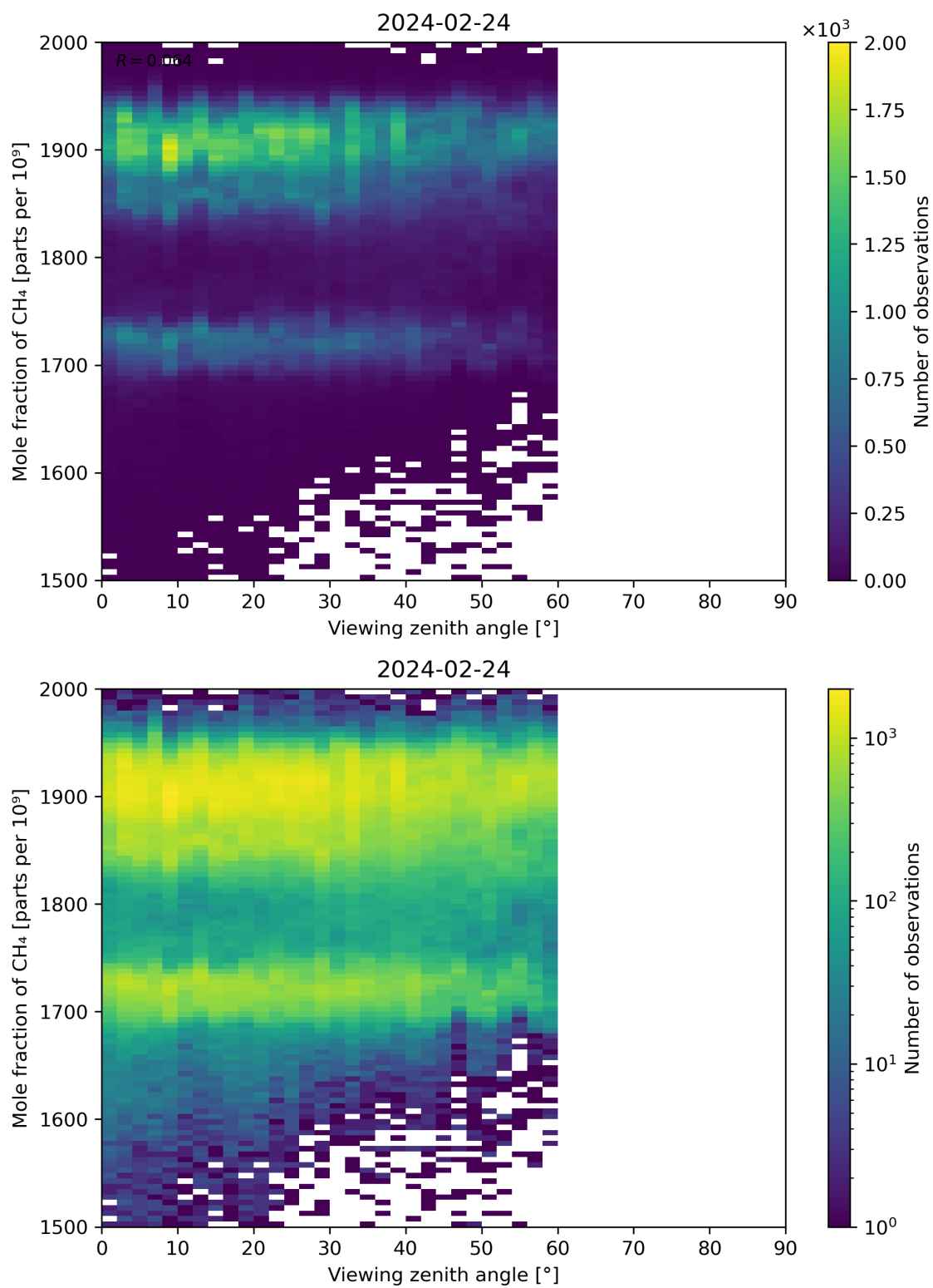
Figure 110: Scatter density plot of “Viewing zenith angle” against “Mole fraction of \text{CH}_4 ” for 2024-02-23 to 2024-02-25.
