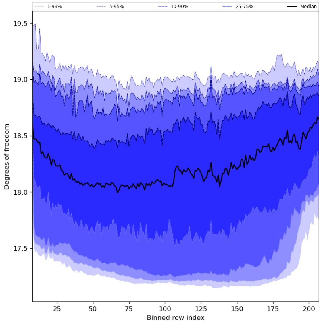
Figure 41: Along track statistics of “Degrees of freedom” for 2024-02-23 to 2024-02-25
