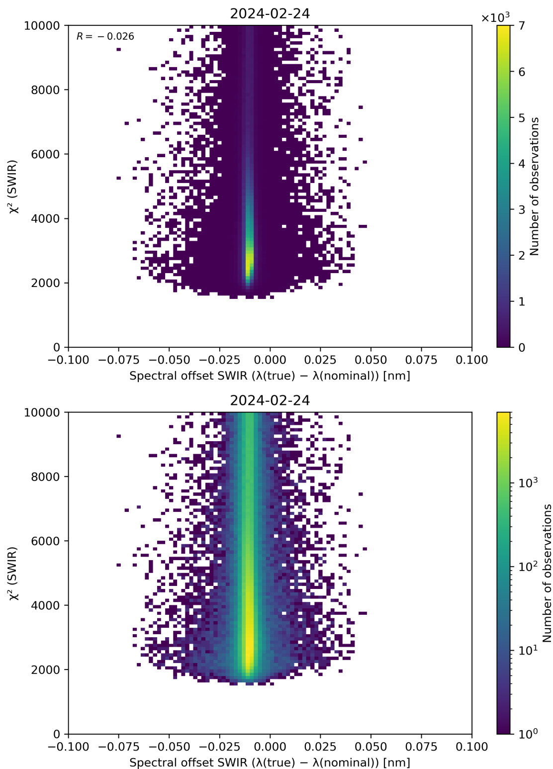
Figure 118: Scatter density plot of “Spectral offset SWIR ( \lambda(\text{true}) - \lambda(\text{nominal}) )” against “ \chi^2 (SWIR)” for 2024-02-23 to 2024-02-25.
