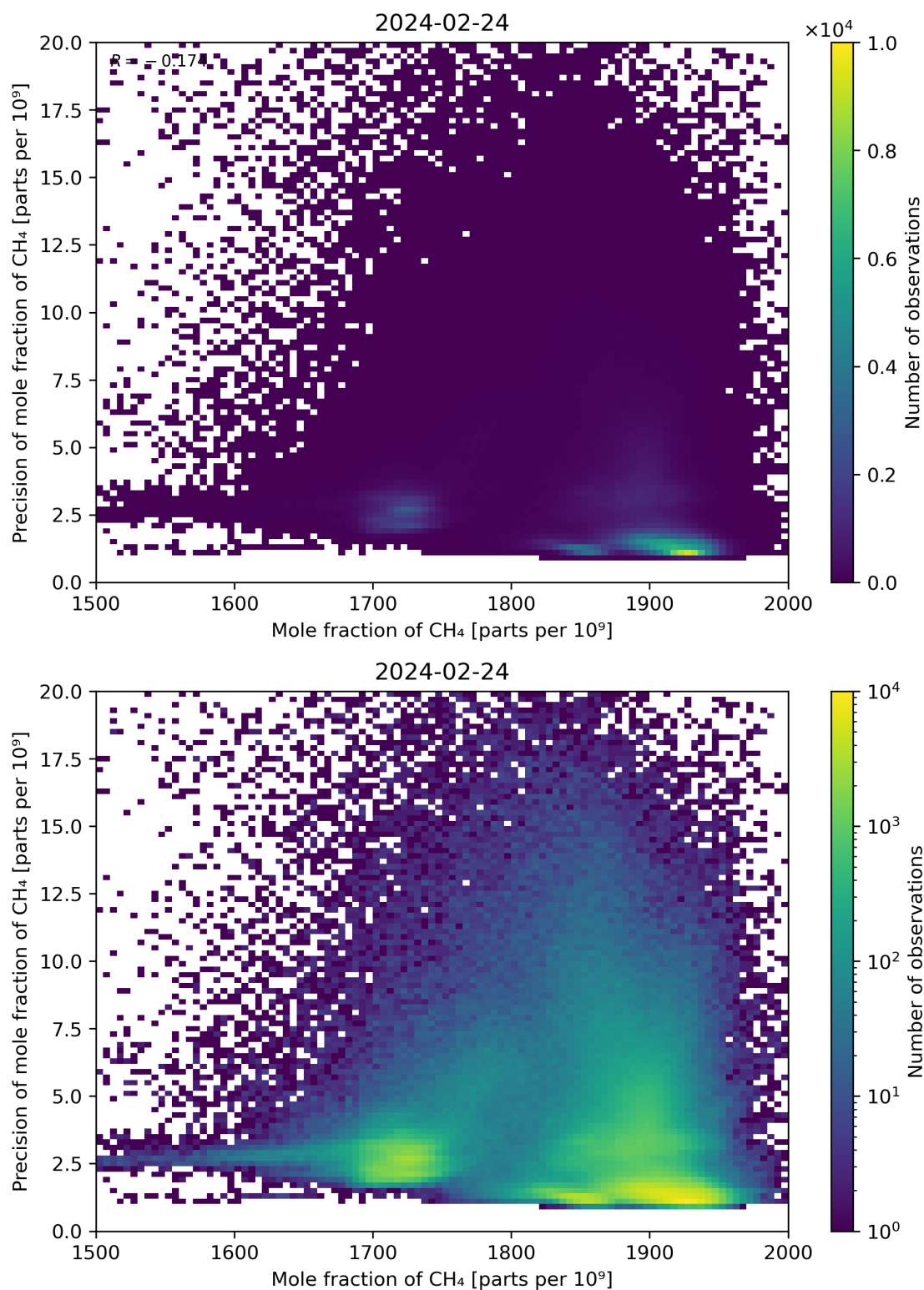
Figure 75: Scatter density plot of “Mole fraction of CH 4 ” against “Precision of mole fraction of CH 4 ” for 2024-02-23 to 2024-02-25.
