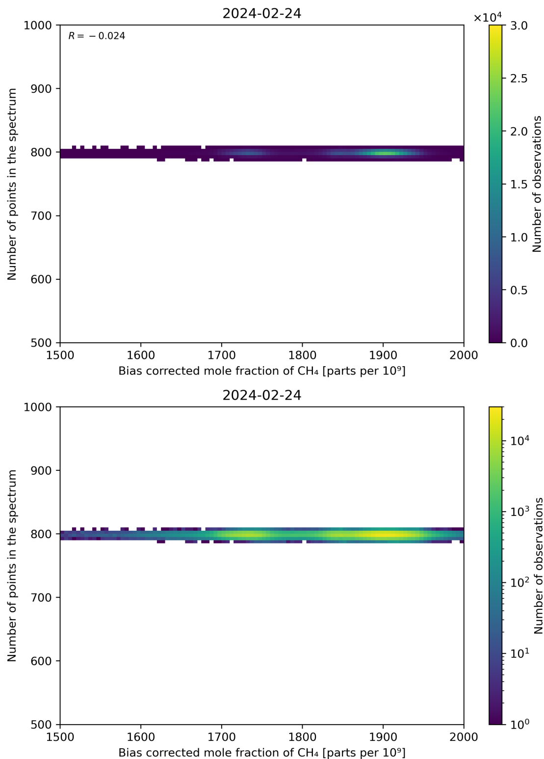
Figure 68: Scatter density plot of “Bias corrected mole fraction of CH 4 ” against “Number of points in the spectrum” for 2024-02-23 to 2024-02-25.
