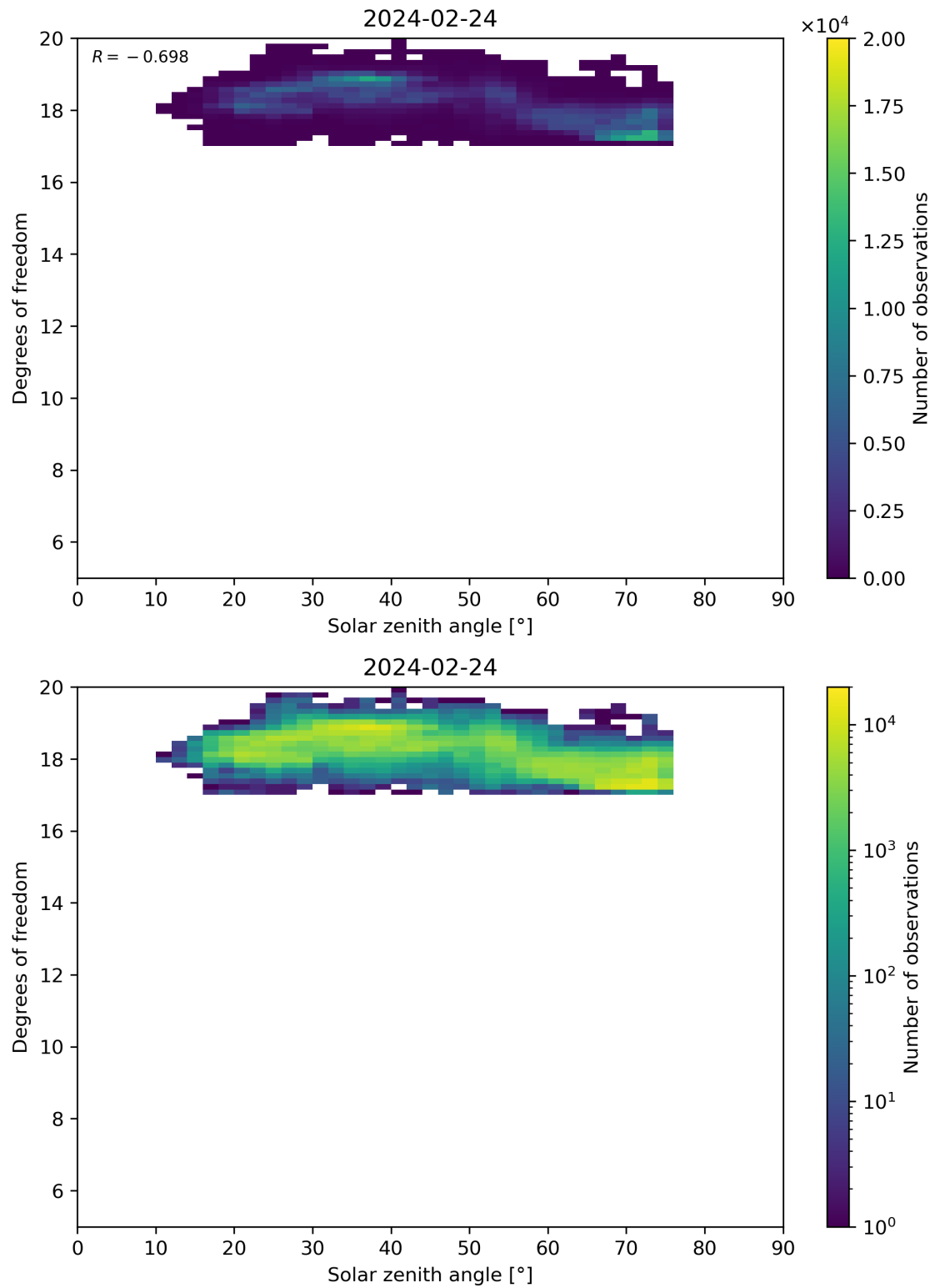
Figure 96: Scatter density plot of “Solar zenith angle” against “Degrees of freedom” for 2024-02-23 to 2024-02-25.
