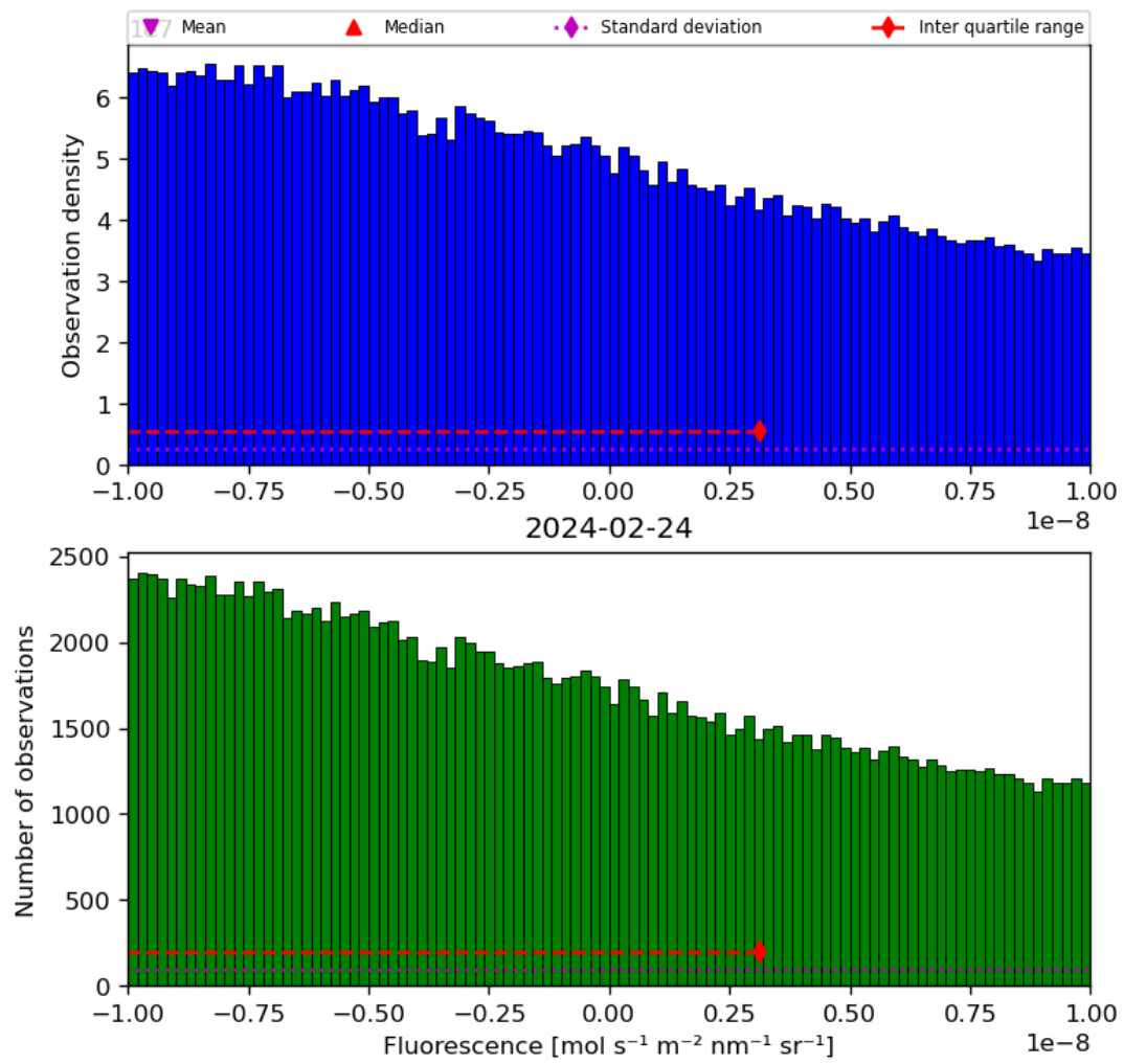
Figure 32: Histogram of “Fluorescence” for 2024-02-23 to 2024-02-25
