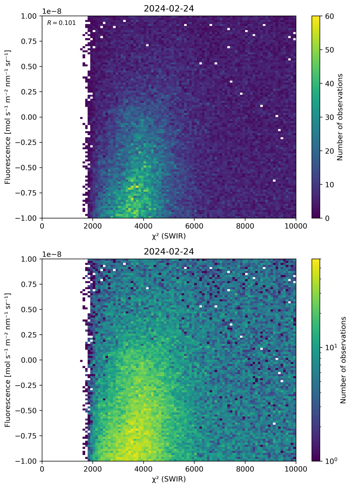
Figure 49: Scatter density plot of “ \chi^2 (SWIR)” against “Fluorescence” for 2024-02-23 to 2024-02-25.
