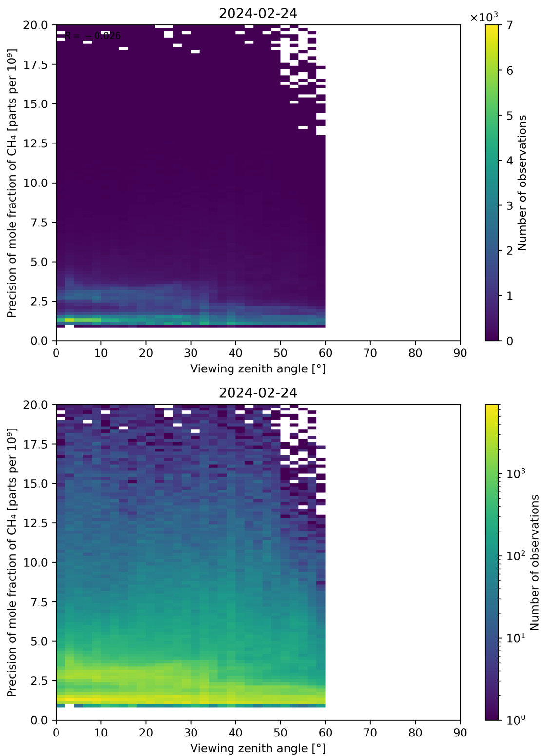
Figure 112: Scatter density plot of “Viewing zenith angle” against “Precision of mole fraction of CH 4 ” for 2024-02-23 to 2024-02-25.
