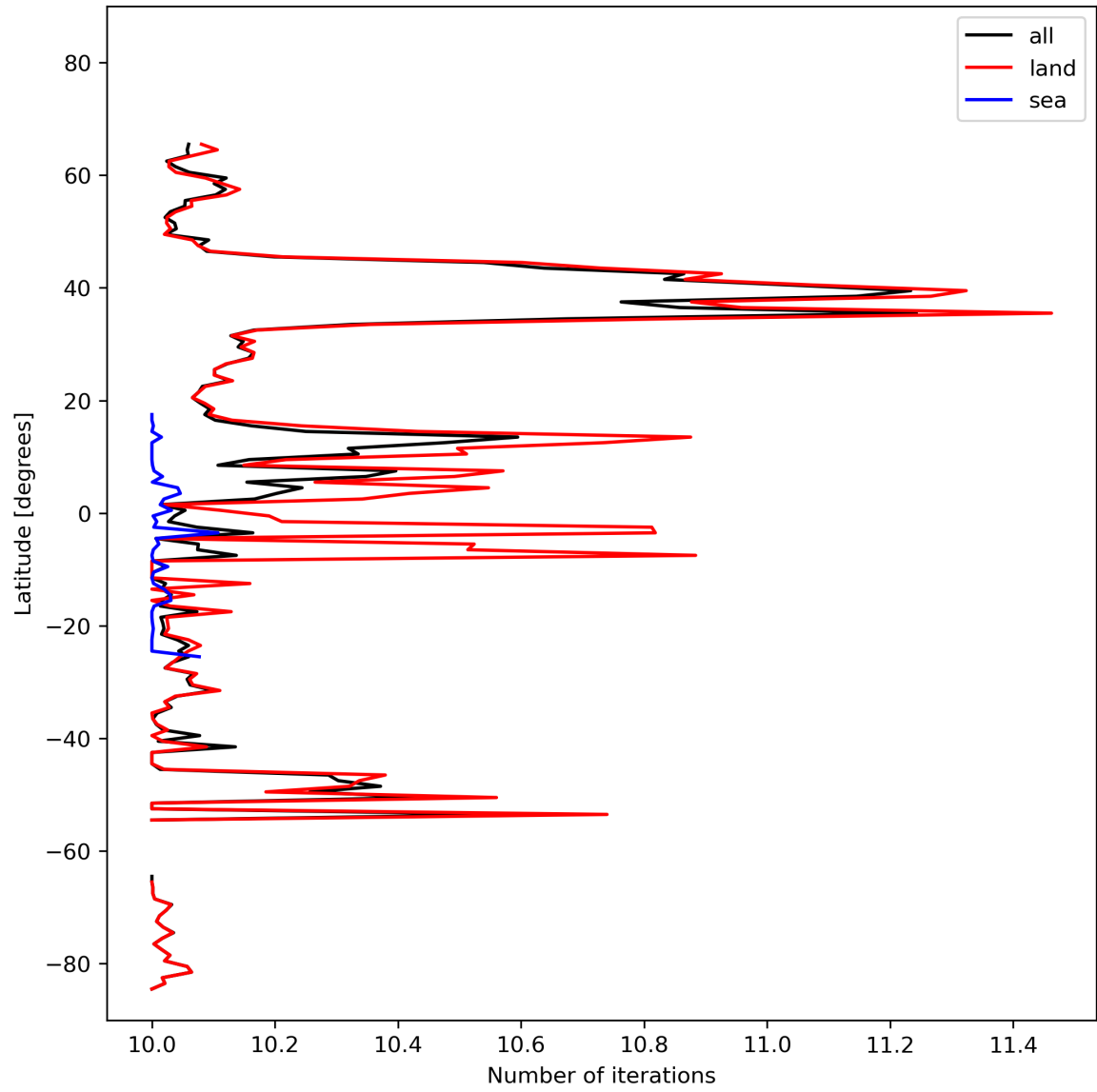
Figure 20: Zonal average of “Number of iterations” for 2024-02-23 to 2024-02-25.
