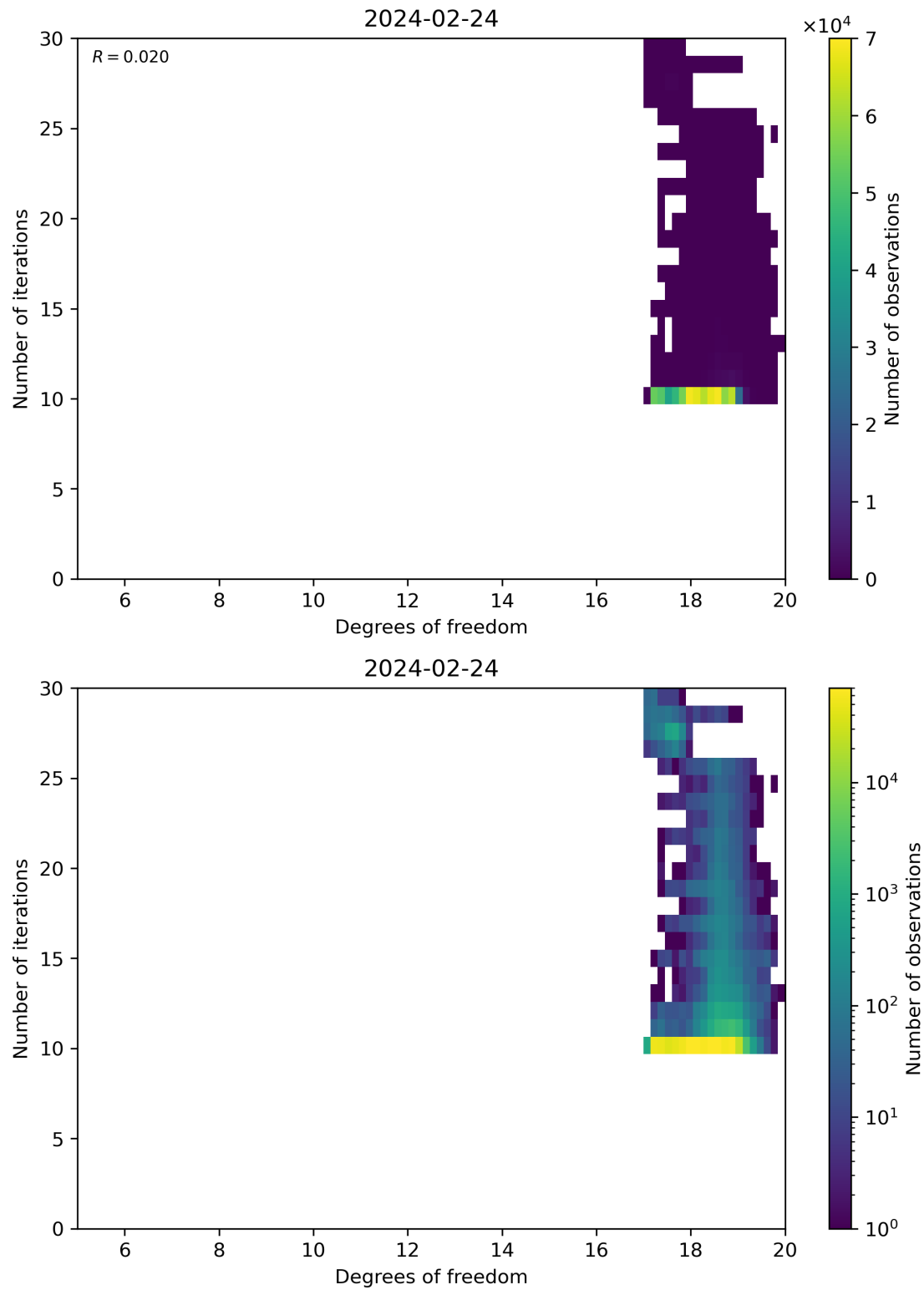
Figure 52: Scatter density plot of “Degrees of freedom” against “Number of iterations” for 2024-02-23 to 2024-02-25.
