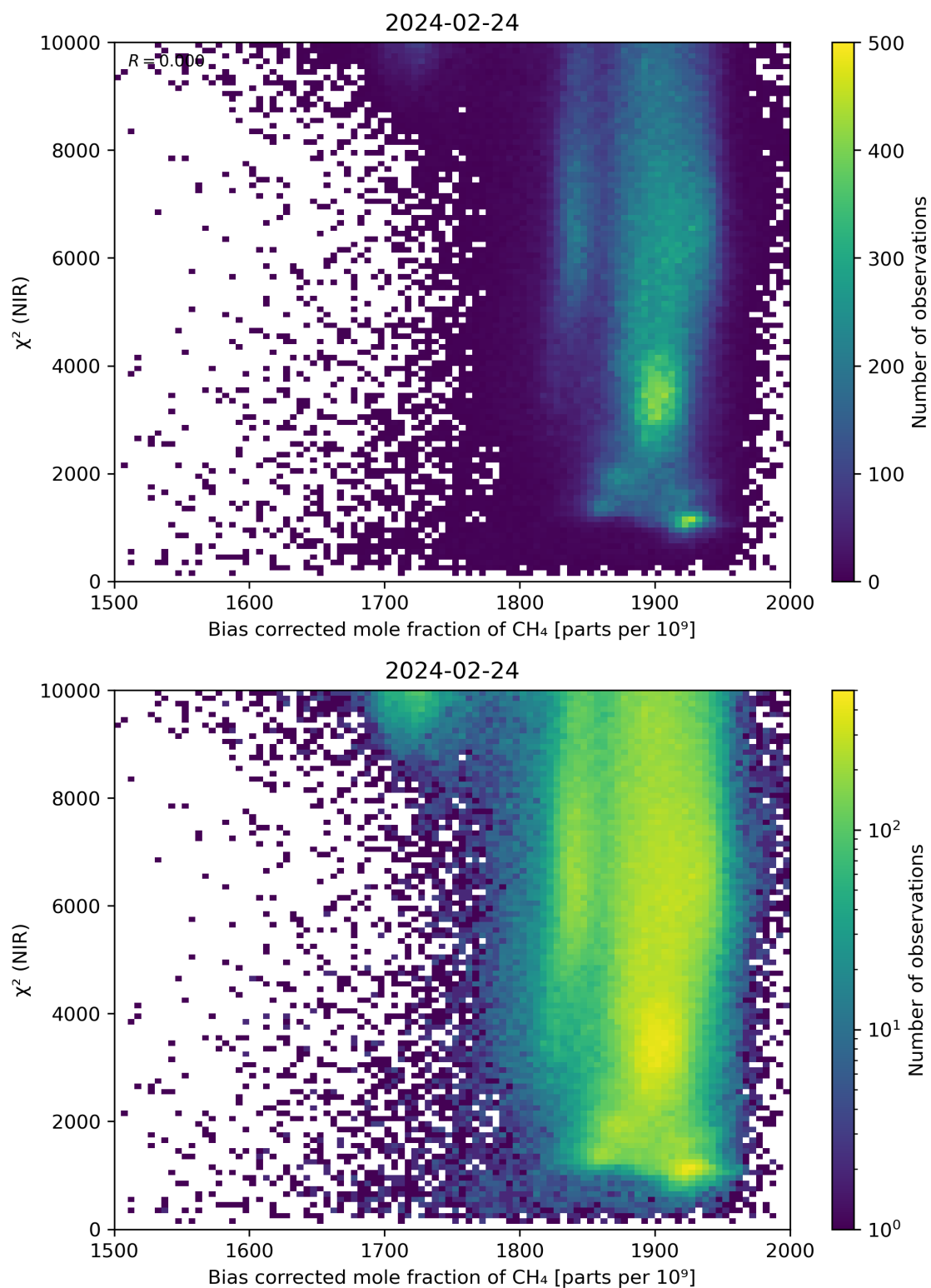
Figure 63: Scatter density plot of “Bias corrected mole fraction of CH 4 ” against “ \chi^2 (NIR)” for 2024-02-23 to 2024-02-25.
