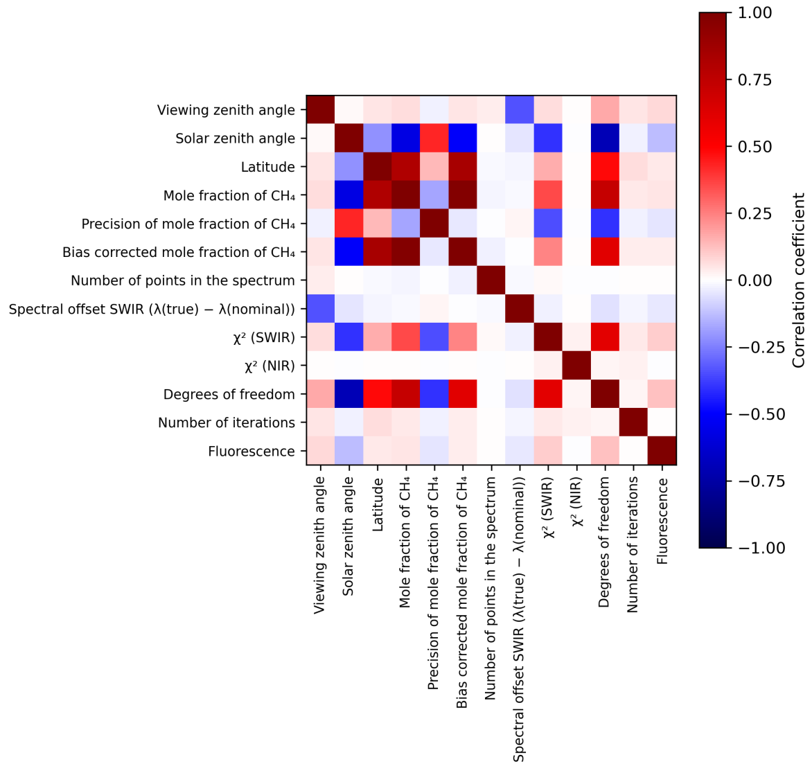
Figure 2: Map of correlation matrix for 2024-02-23 to 2024-02-25.
