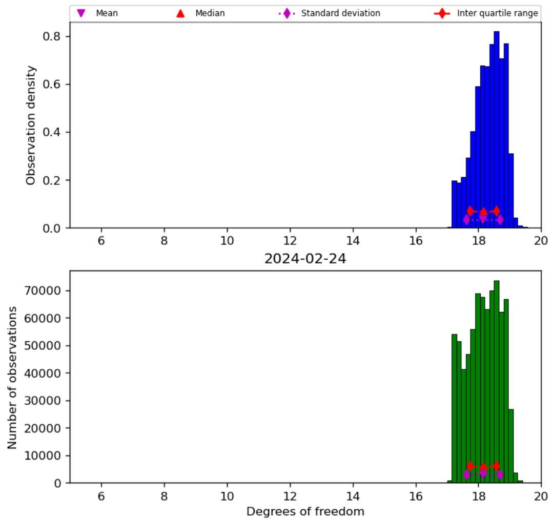
Figure 30: Histogram of “Degrees of freedom” for 2024-02-23 to 2024-02-25
