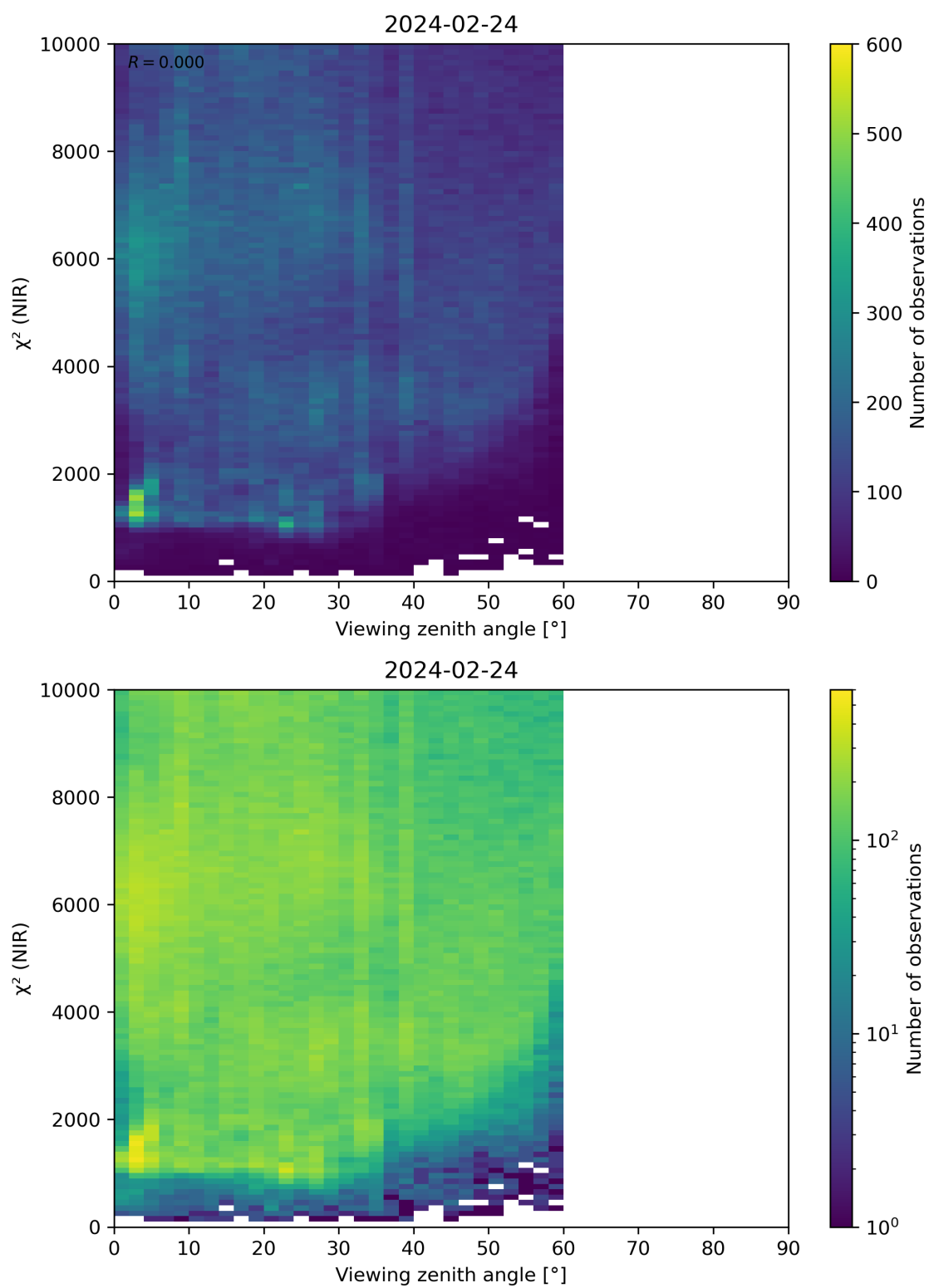
Figure 105: Scatter density plot of “Viewing zenith angle” against “ \chi^2 (NIR)” for 2024-02-23 to 2024-02-25.
