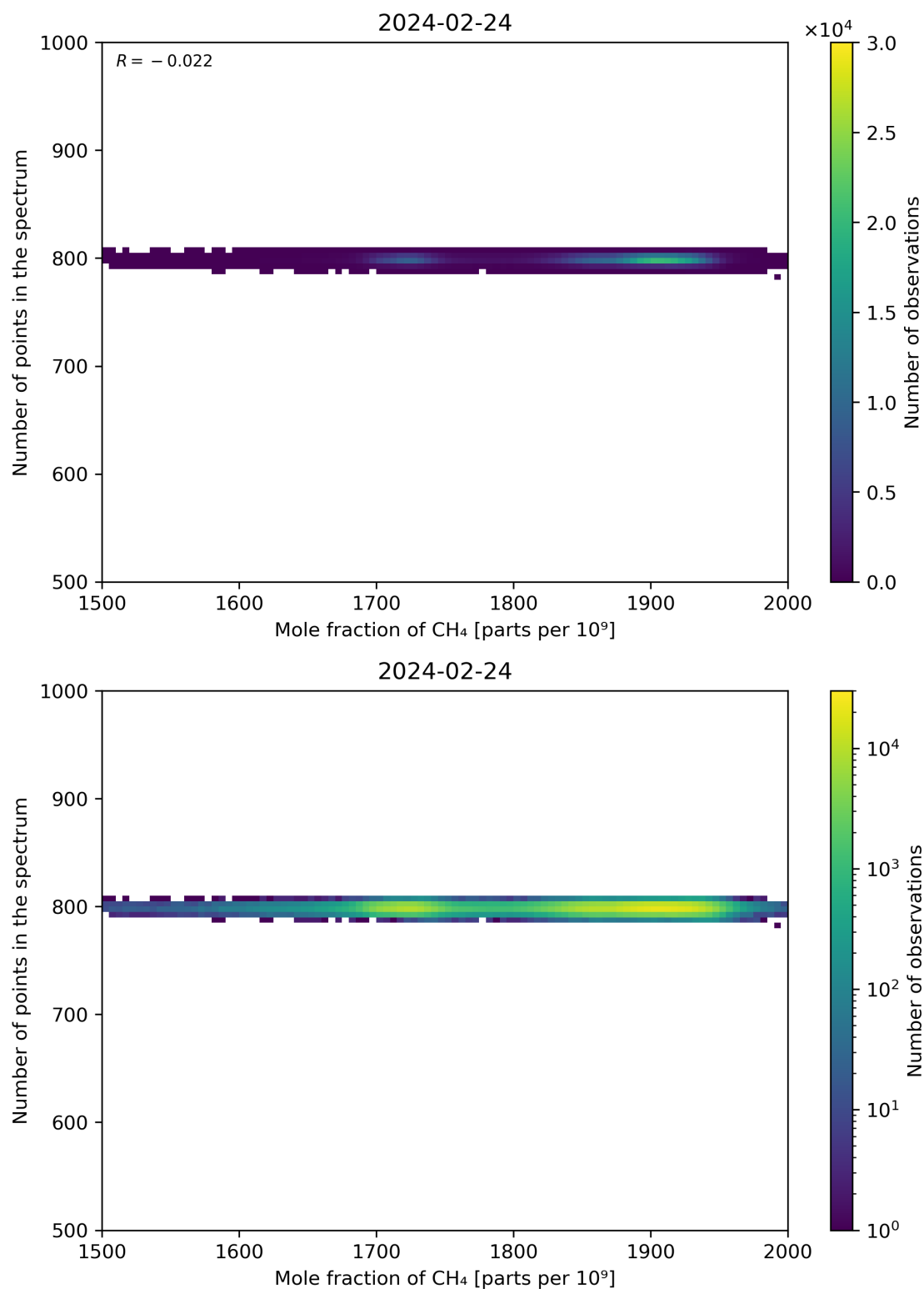
Figure 77: Scatter density plot of “Mole fraction of CH 4 ” against “Number of points in the spectrum” for 2024-02-23 to 2024-02-25.
