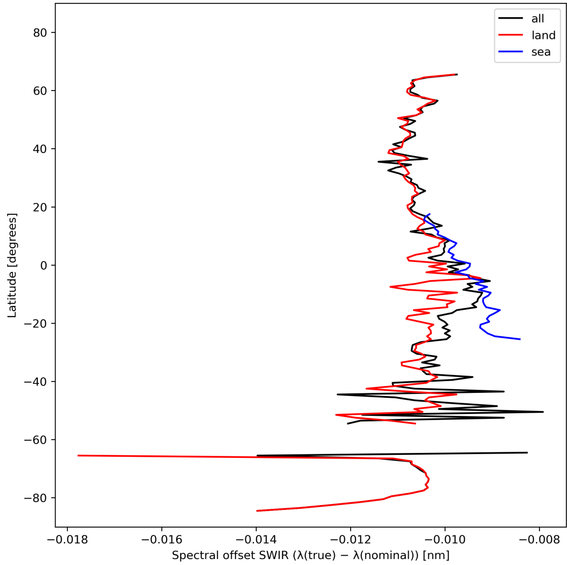
Figure 16: Zonal average of “Spectral offset SWIR ( \lambda(\text{true}) - \lambda(\text{nominal}) )” for 2024-02-23 to 2024-02-25.
