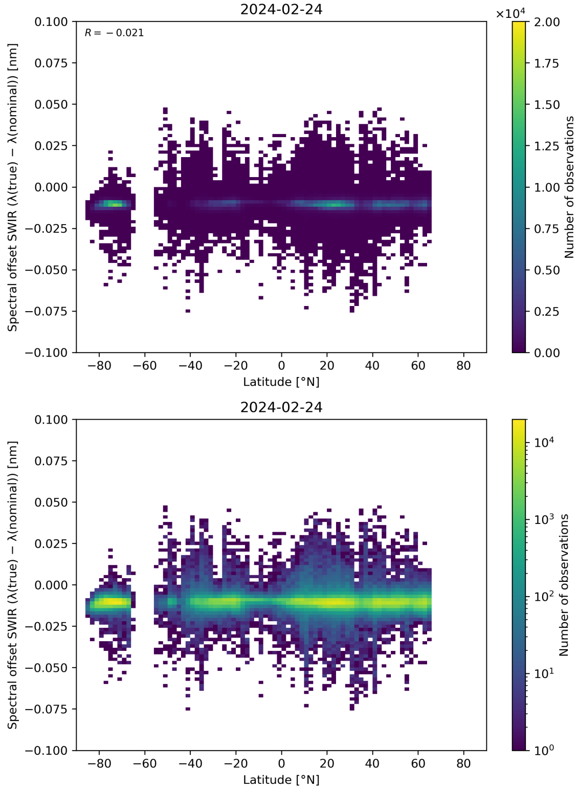
Figure 62: Scatter density plot of “Latitude” against “Spectral offset SWIR ( \lambda(\text{true}) - \lambda(\text{nominal}) )” for 2024-02-23 to 2024-02-25.
