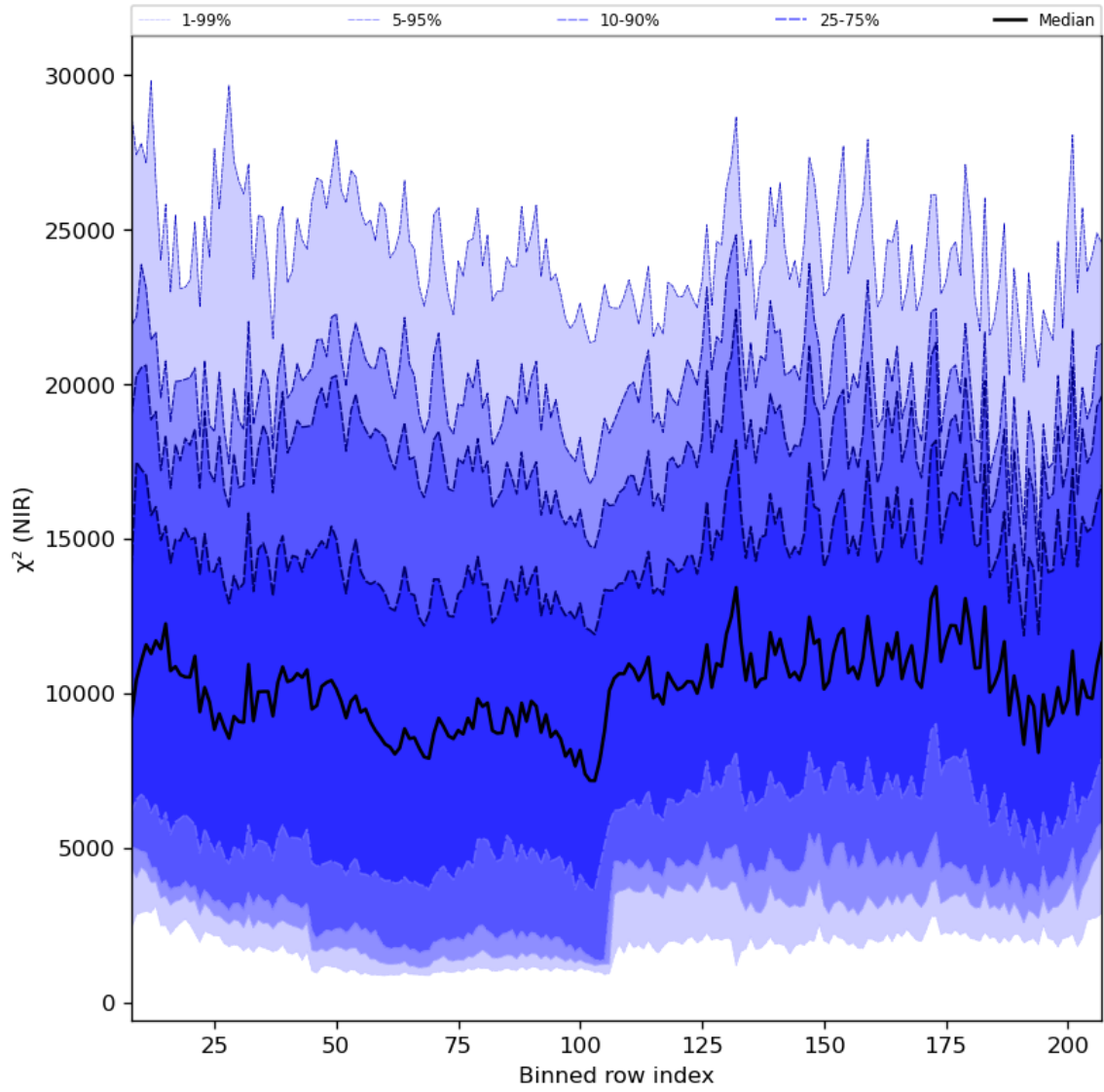
Figure 40: Along track statistics of “ \chi^2 (NIR)” for 2024-02-23 to 2024-02-25
