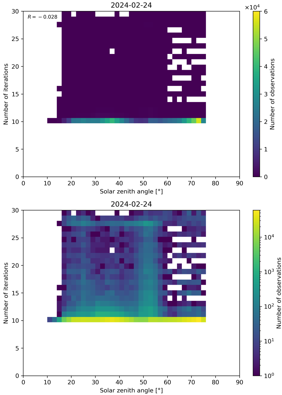
Figure 102: Scatter density plot of “Solar zenith angle” against “Number of iterations” for 2024-02-23 to 2024-02-25.
