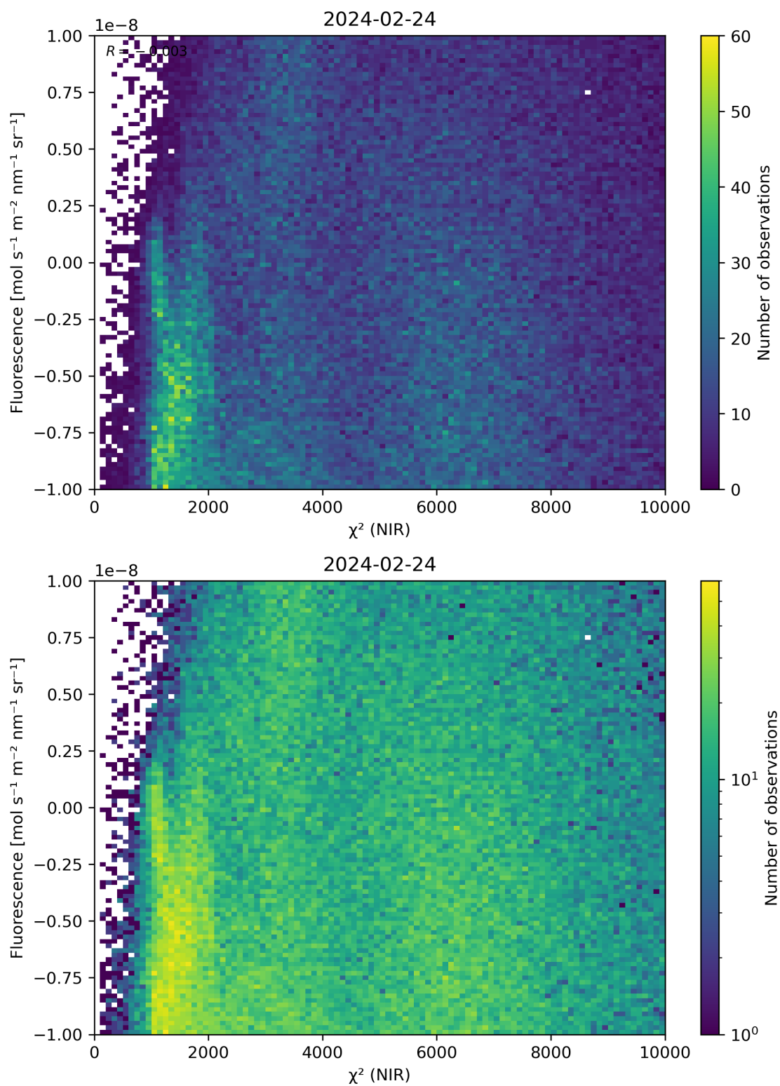
Figure 45: Scatter density plot of “ \chi^2 (NIR)” against “Fluorescence” for 2024-02-23 to 2024-02-25.
