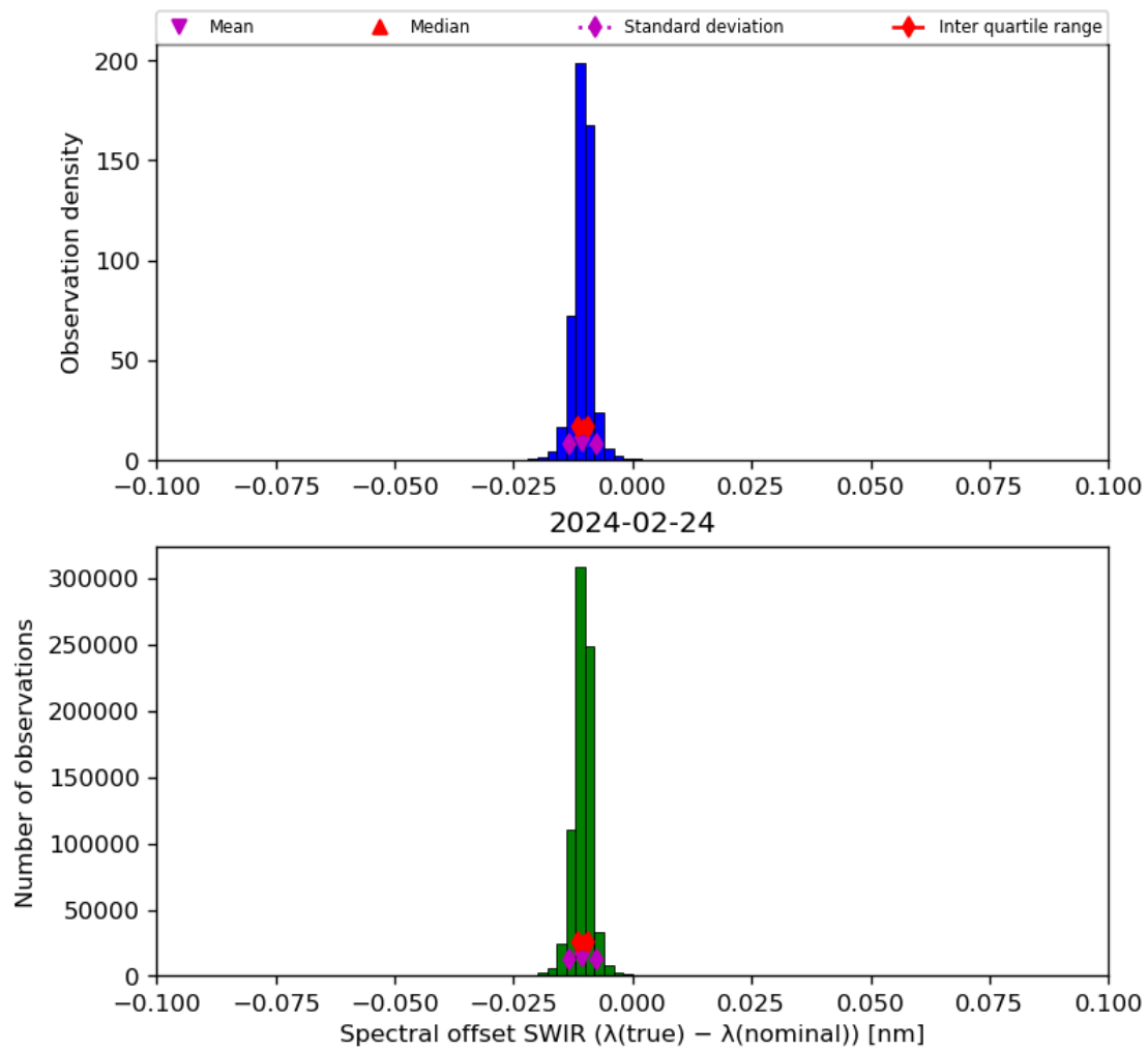
Figure 27: Histogram of “Spectral offset SWIR ( \lambda(\text{true}) - \lambda(\text{nominal}) )” for 2024-02-23 to 2024-02-25
