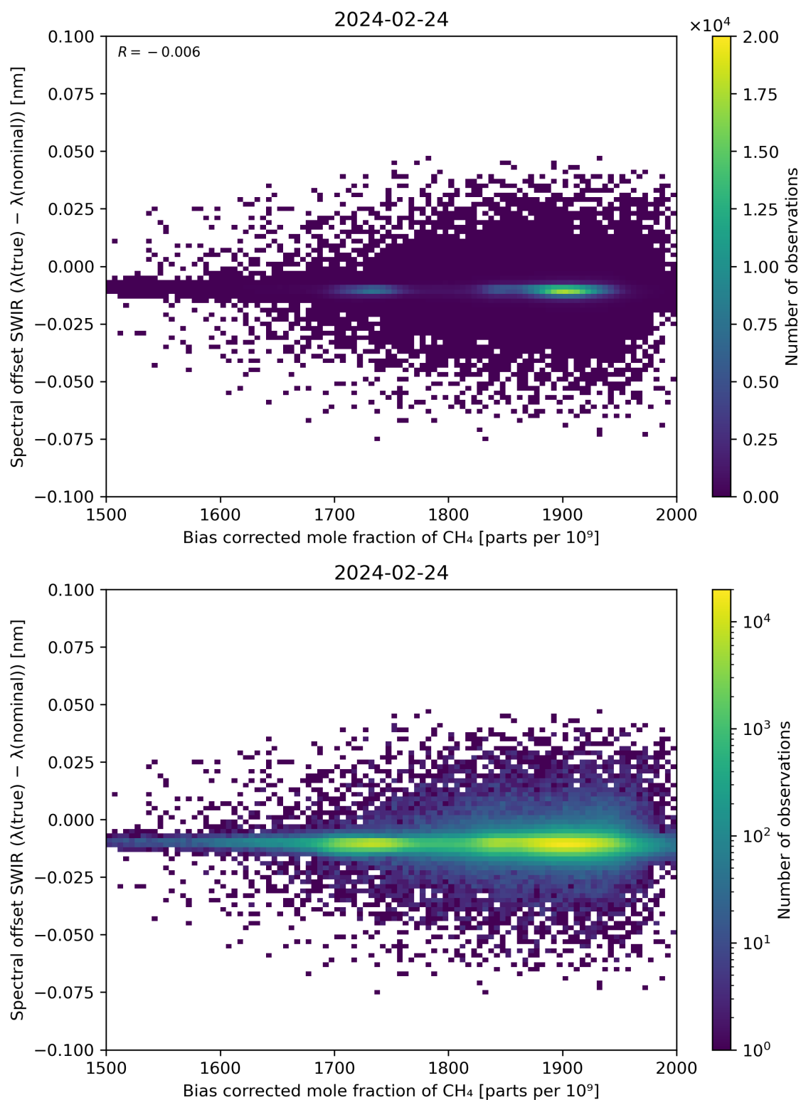
Figure 69: Scatter density plot of “Bias corrected mole fraction of \text{CH}_4 ” against “Spectral offset SWIR ( \lambda(\text{true}) - \lambda(\text{nominal}) )” for 2024-02-23 to 2024-02-25.
