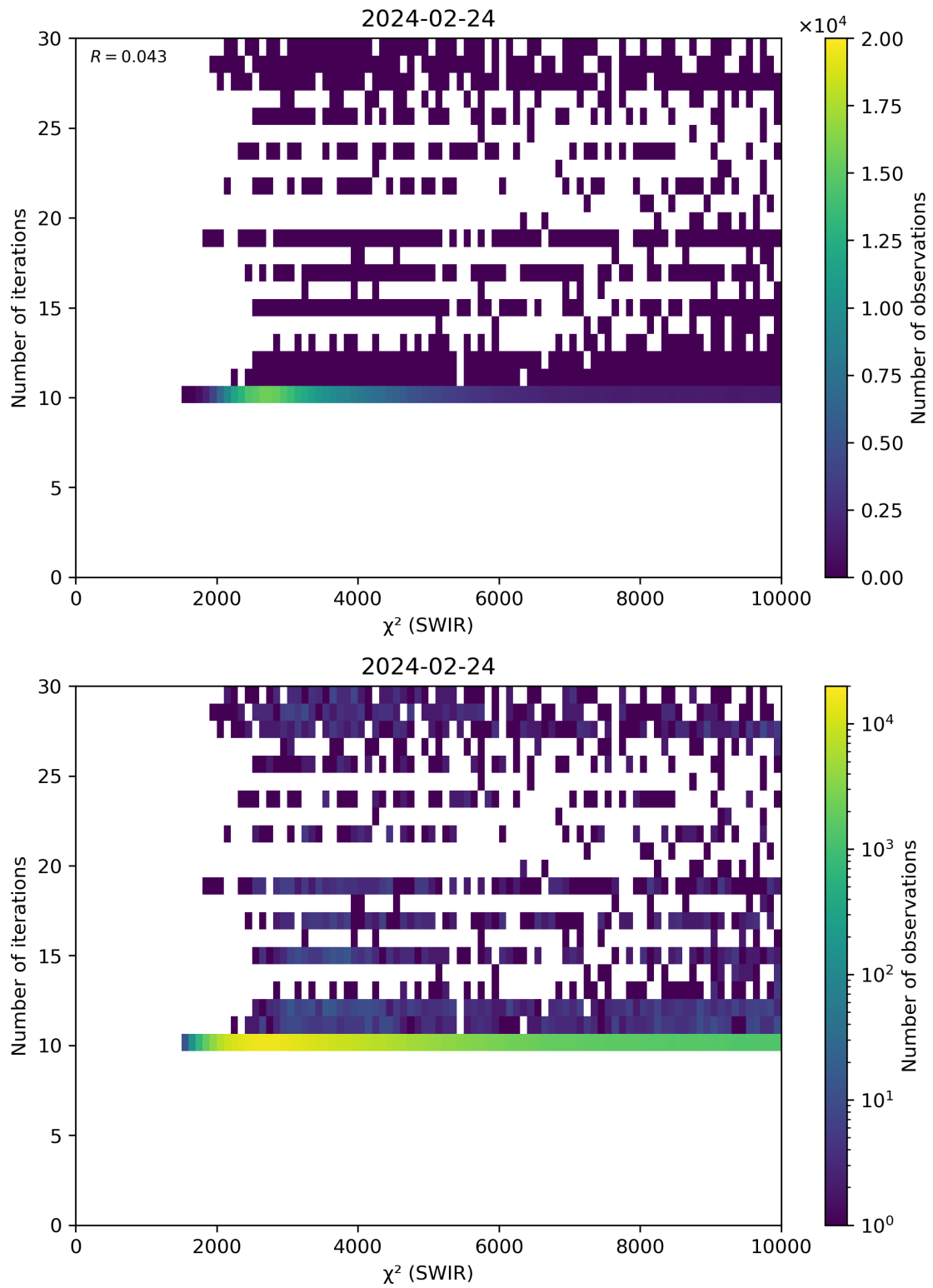
Figure 50: Scatter density plot of “ \chi^2 (SWIR)” against “Number of iterations” for 2024-02-23 to 2024-02-25.
