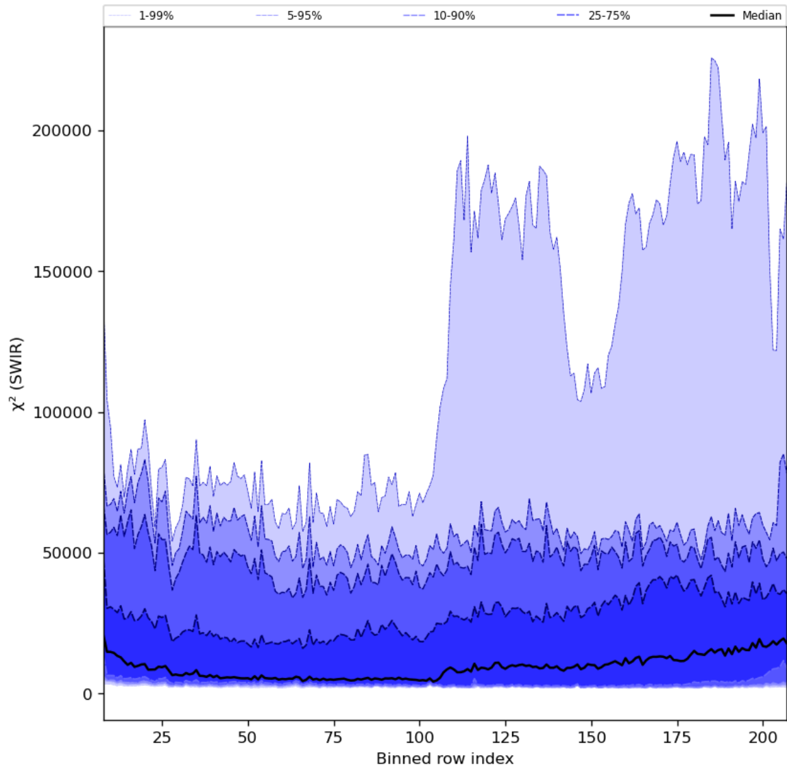
Figure 39: Along track statistics of “ \chi^2 (SWIR)” for 2024-02-23 to 2024-02-25
