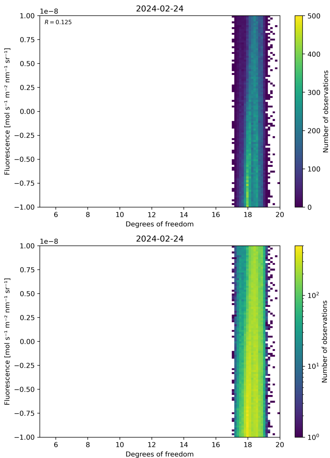
Figure 51: Scatter density plot of “Degrees of freedom” against “Fluorescence” for 2024-02-23 to 2024-02-25.
