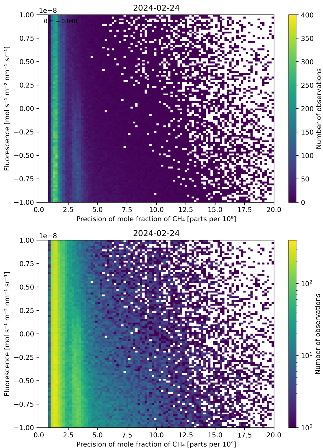
Figure 81: Scatter density plot of “Precision of mole fraction of \text{CH}_4 ” against “Fluorescence” for 2024-02-23 to 2024-02-25.
