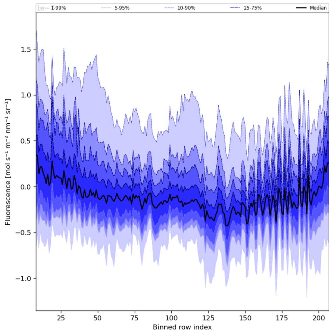
Figure 43: Along track statistics of “Fluorescence” for 2024-02-23 to 2024-02-25
