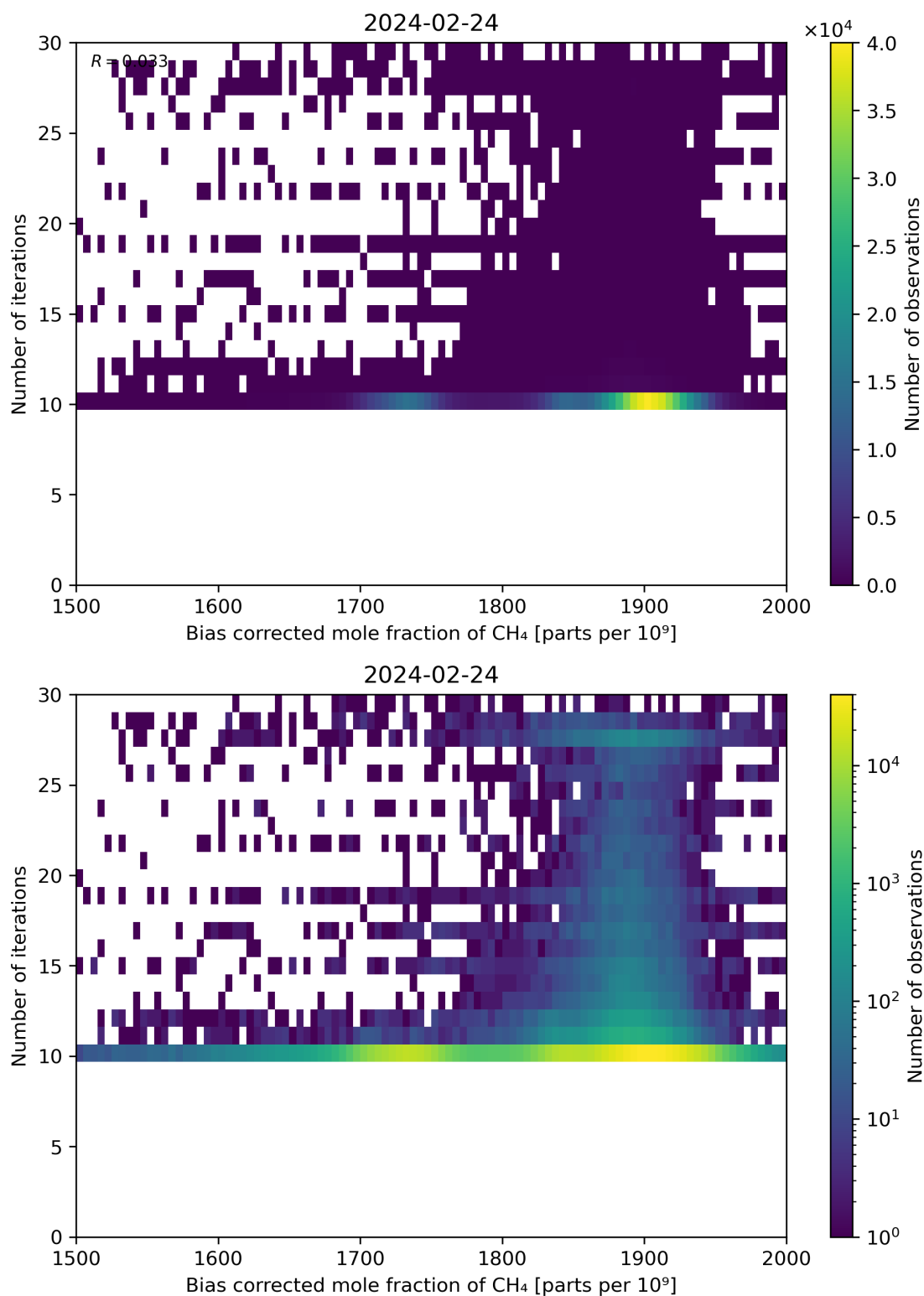
Figure 67: Scatter density plot of “Bias corrected mole fraction of \text{CH}_4 ” against “Number of iterations” for 2024-02-23 to 2024-02-25.
