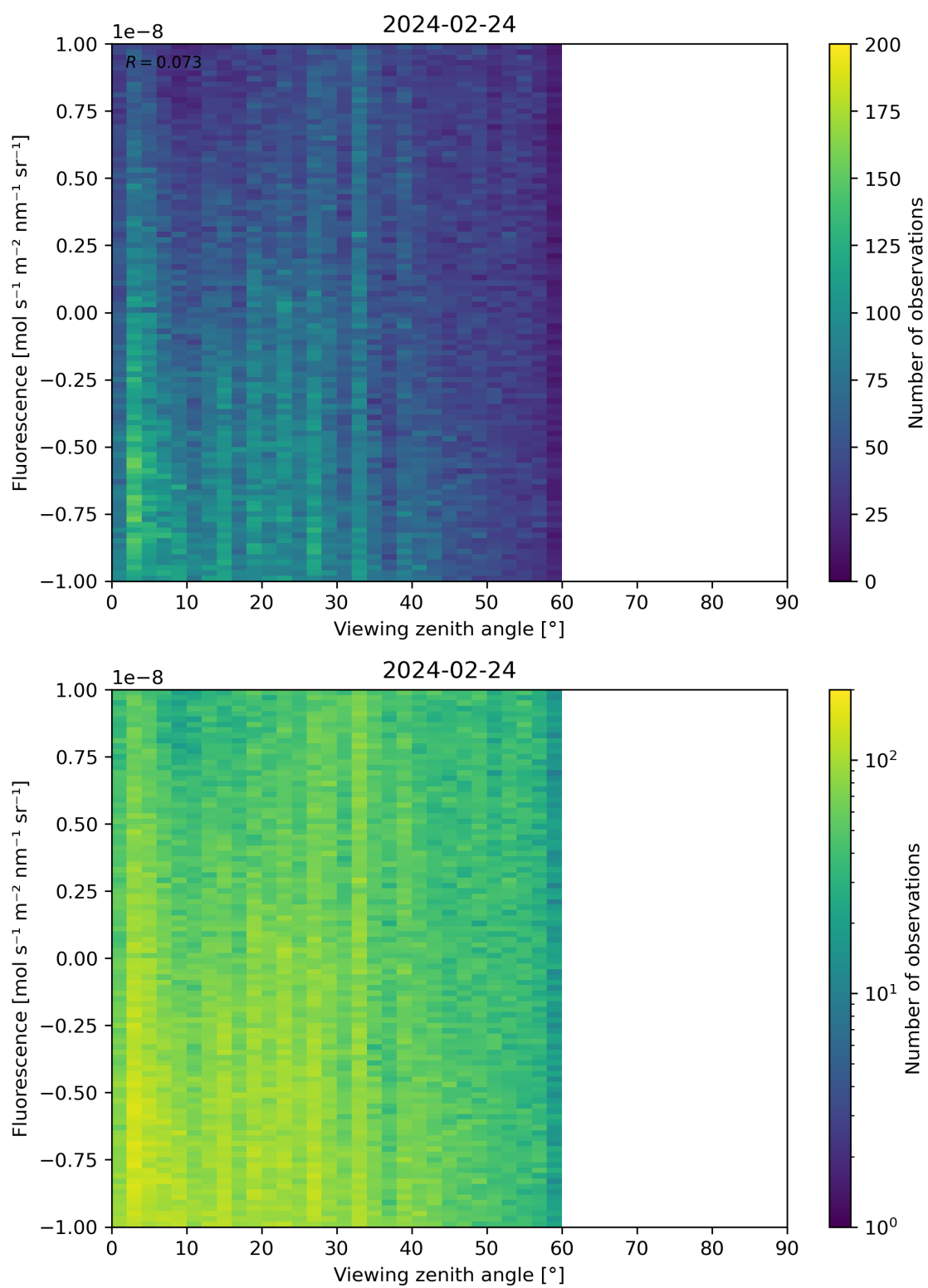
Figure 108: Scatter density plot of “Viewing zenith angle” against “Fluorescence” for 2024-02-23 to 2024-02-25.
