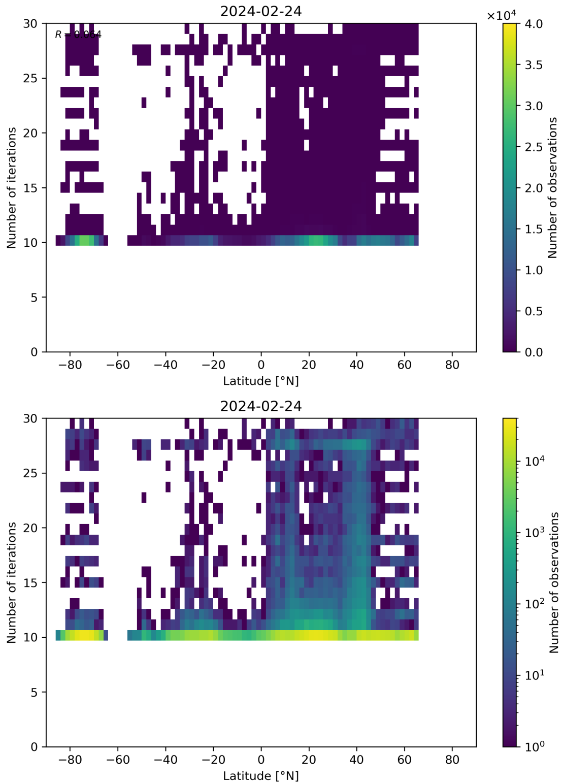
Figure 60: Scatter density plot of “Latitude” against “Number of iterations” for 2024-02-23 to 2024-02-25.
