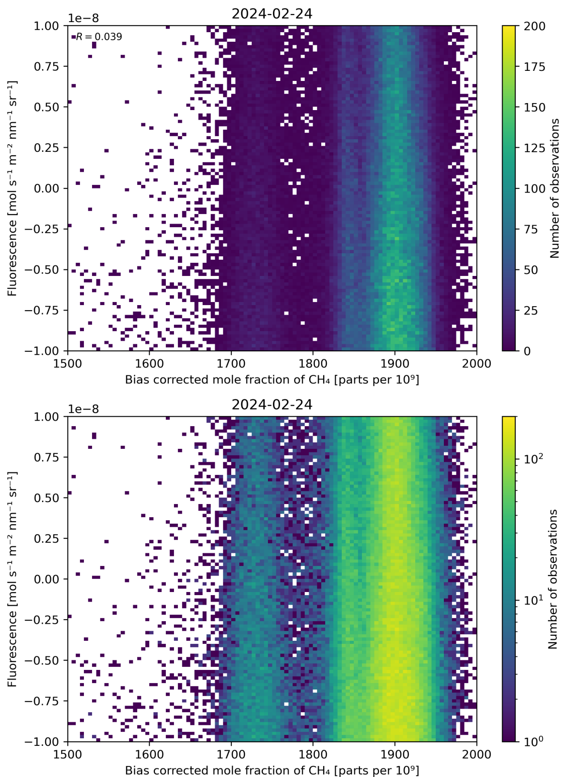
Figure 66: Scatter density plot of “Bias corrected mole fraction of \text{CH}_4 ” against “Fluorescence” for 2024-02-23 to 2024-02-25.
