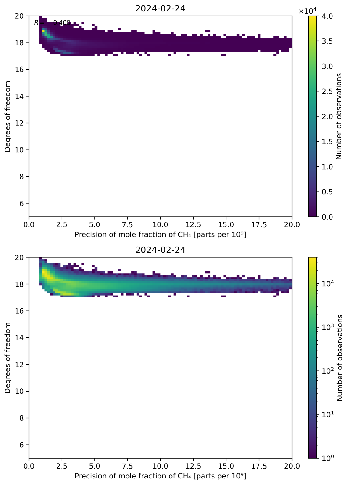
Figure 80: Scatter density plot of “Precision of mole fraction of CH 4 ” against “Degrees of freedom” for 2024-02-23 to 2024-02-25.
