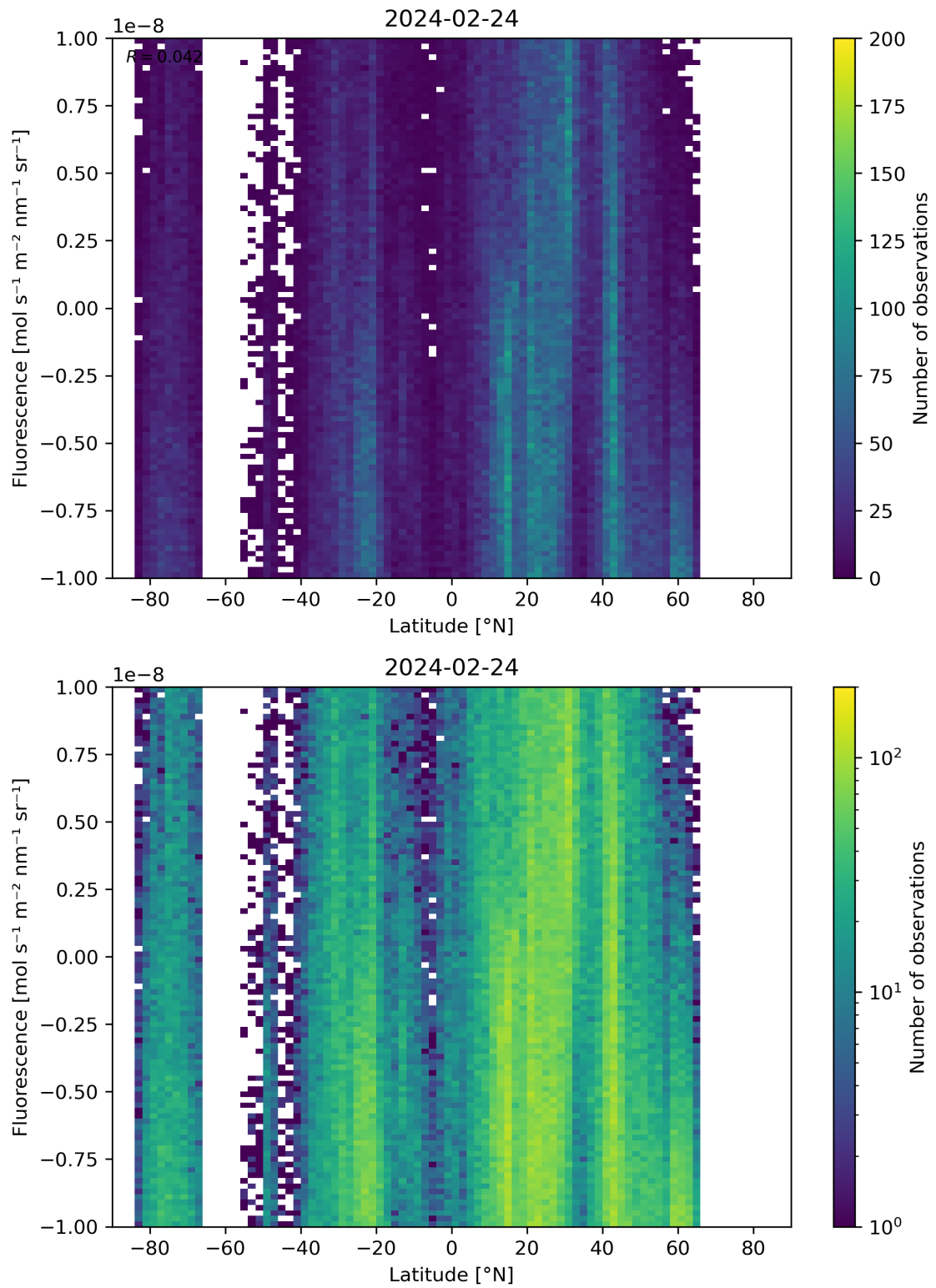
Figure 56: Scatter density plot of “Latitude” against “Fluorescence” for 2024-02-23 to 2024-02-25.
