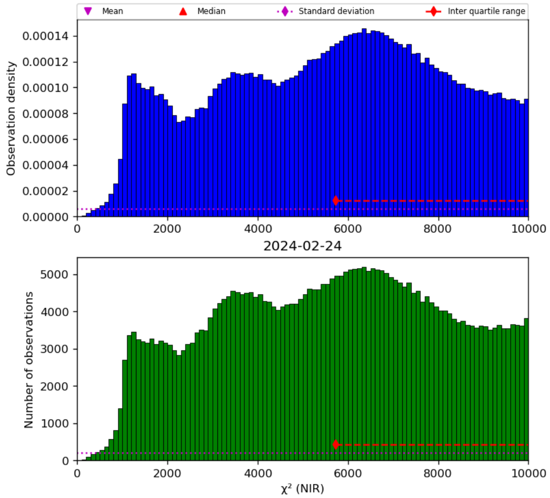
Figure 29: Histogram of “ \chi^2 (NIR)” for 2024-02-23 to 2024-02-25
