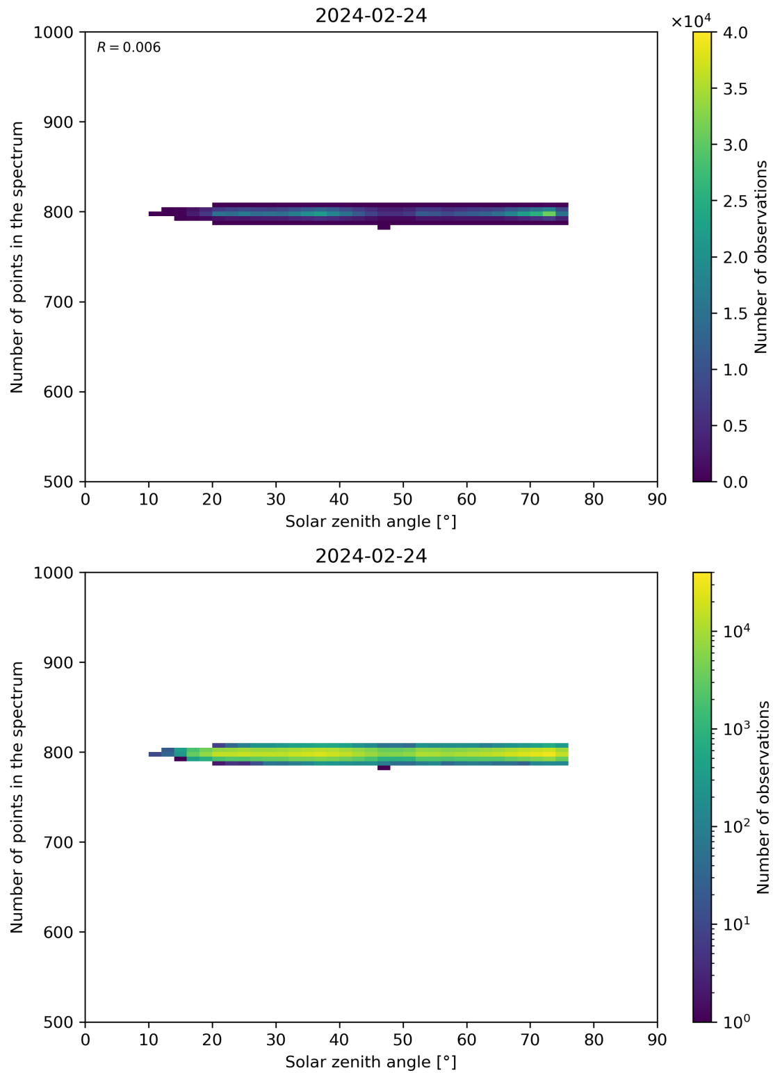
Figure 103: Scatter density plot of “Solar zenith angle” against “Number of points in the spectrum” for 2024-02-23 to 2024-02-25.
