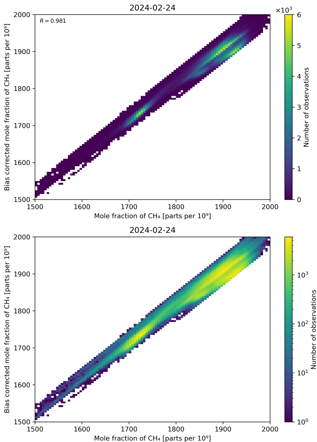
Figure 74: Scatter density plot of “Mole fraction of CH 4 ” against “Bias corrected mole fraction of CH 4 ” for 2024-02-23 to 2024-02-25.
