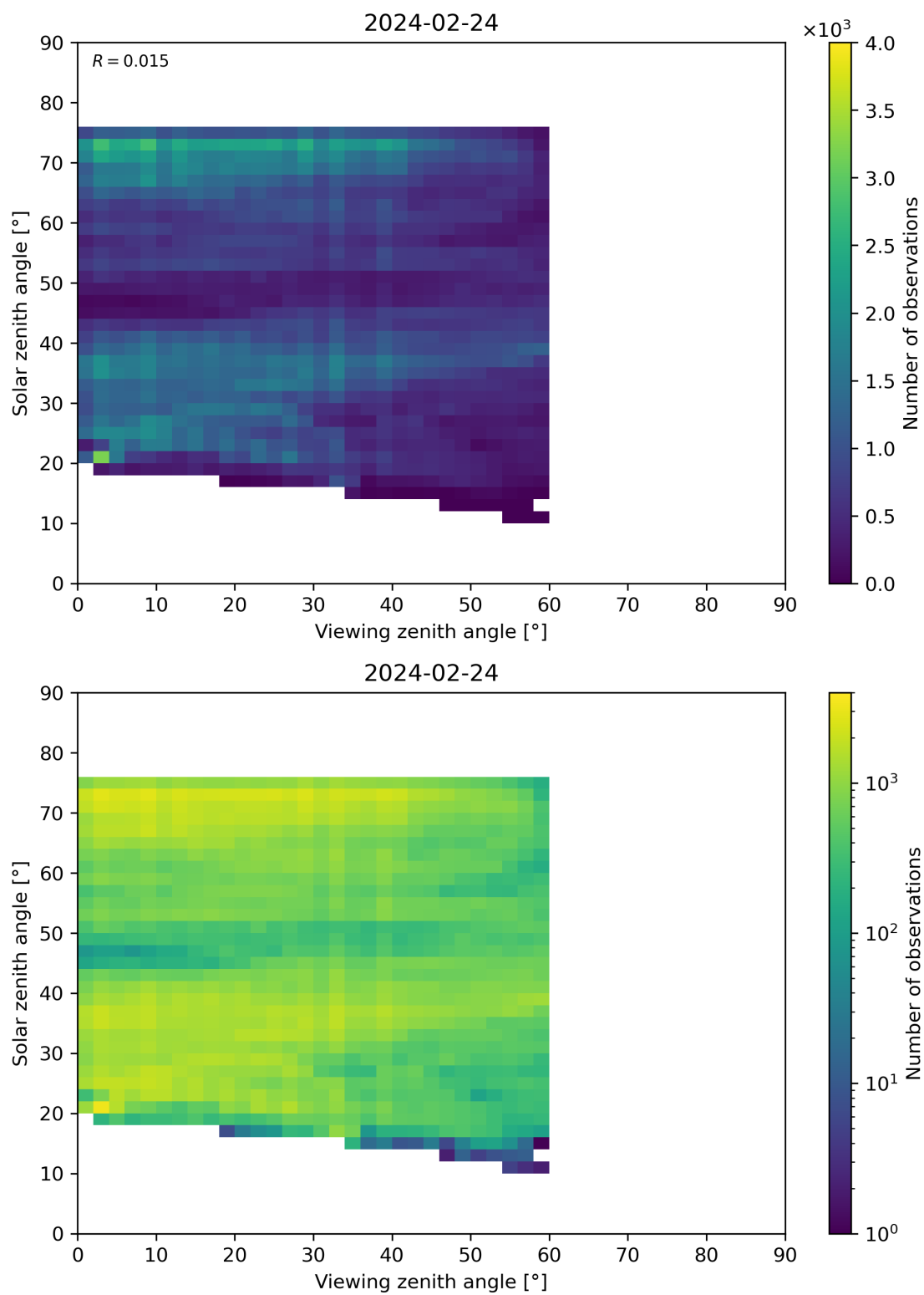
Figure 115: Scatter density plot of “Viewing zenith angle” against “Solar zenith angle” for 2024-02-23 to 2024-02-25.
