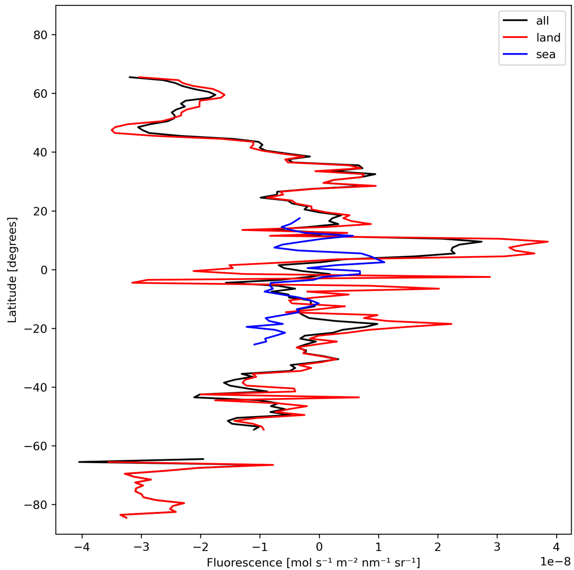
Figure 21: Zonal average of “Fluorescence” for 2024-02-23 to 2024-02-25.
