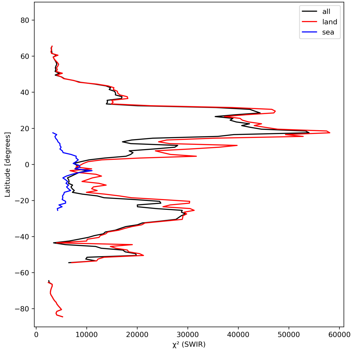
Figure 17: Zonal average of “ \chi^2 (SWIR)” for 2024-02-23 to 2024-02-25.
