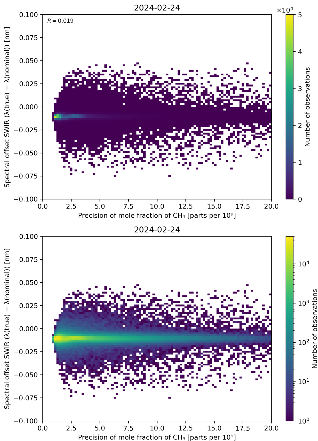
Figure 85: Scatter density plot of “Precision of mole fraction of \text{CH}_4 ” against “Spectral offset SWIR ( \lambda(\text{true}) - \lambda(\text{nominal}) )” for 2024-02-23 to 2024-02-25.
