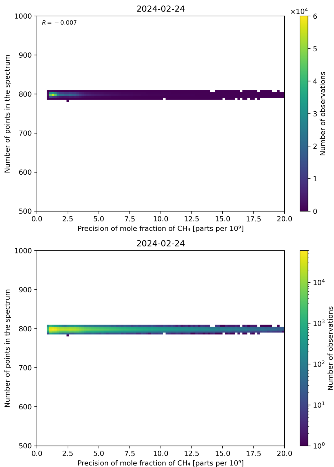
Figure 84: Scatter density plot of “Precision of mole fraction of CH 4 ” against “Number of points in the spectrum” for 2024-02-23 to 2024-02-25.
