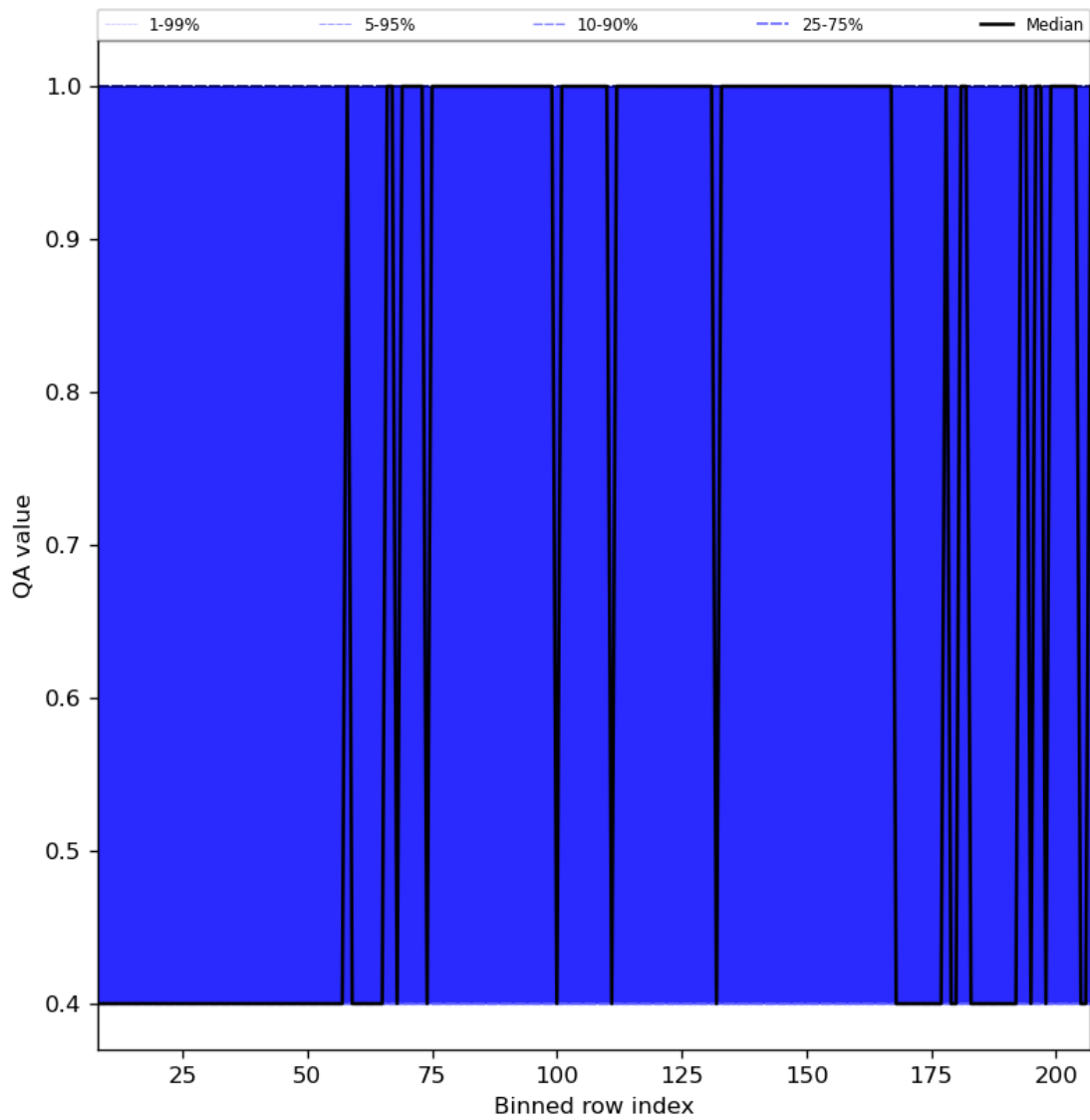
Figure 33: Along track statistics of “QA value” for 2024-02-23 to 2024-02-25
