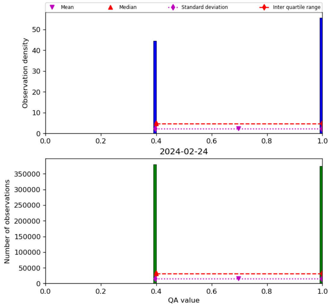
Figure 22: Histogram of “QA value” for 2024-02-23 to 2024-02-25
