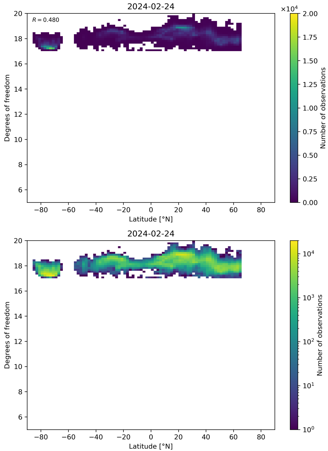
Figure 55: Scatter density plot of “Latitude” against “Degrees of freedom” for 2024-02-23 to 2024-02-25.
