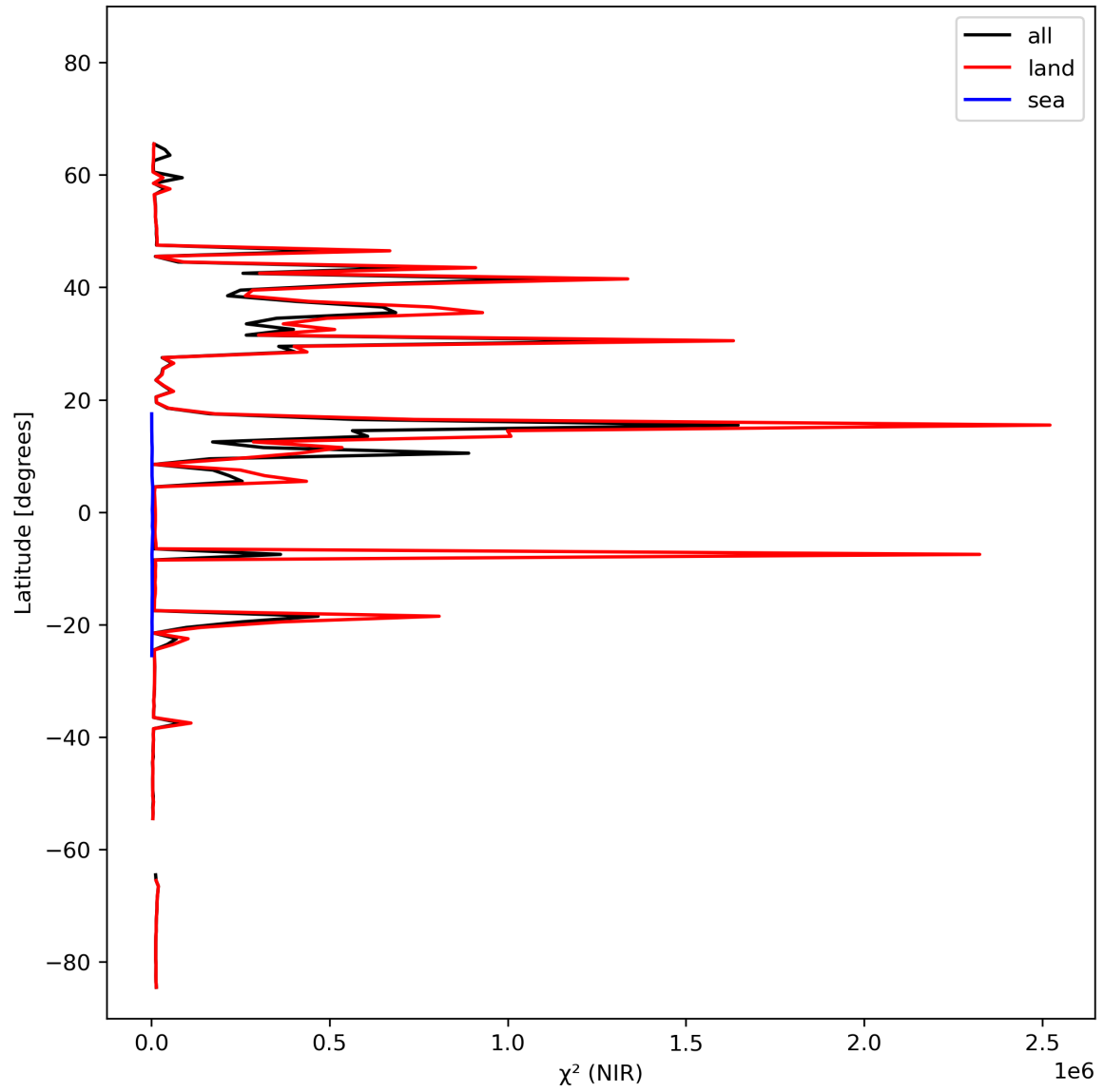
Figure 18: Zonal average of “ \chi^2 (NIR)” for 2024-02-23 to 2024-02-25.
