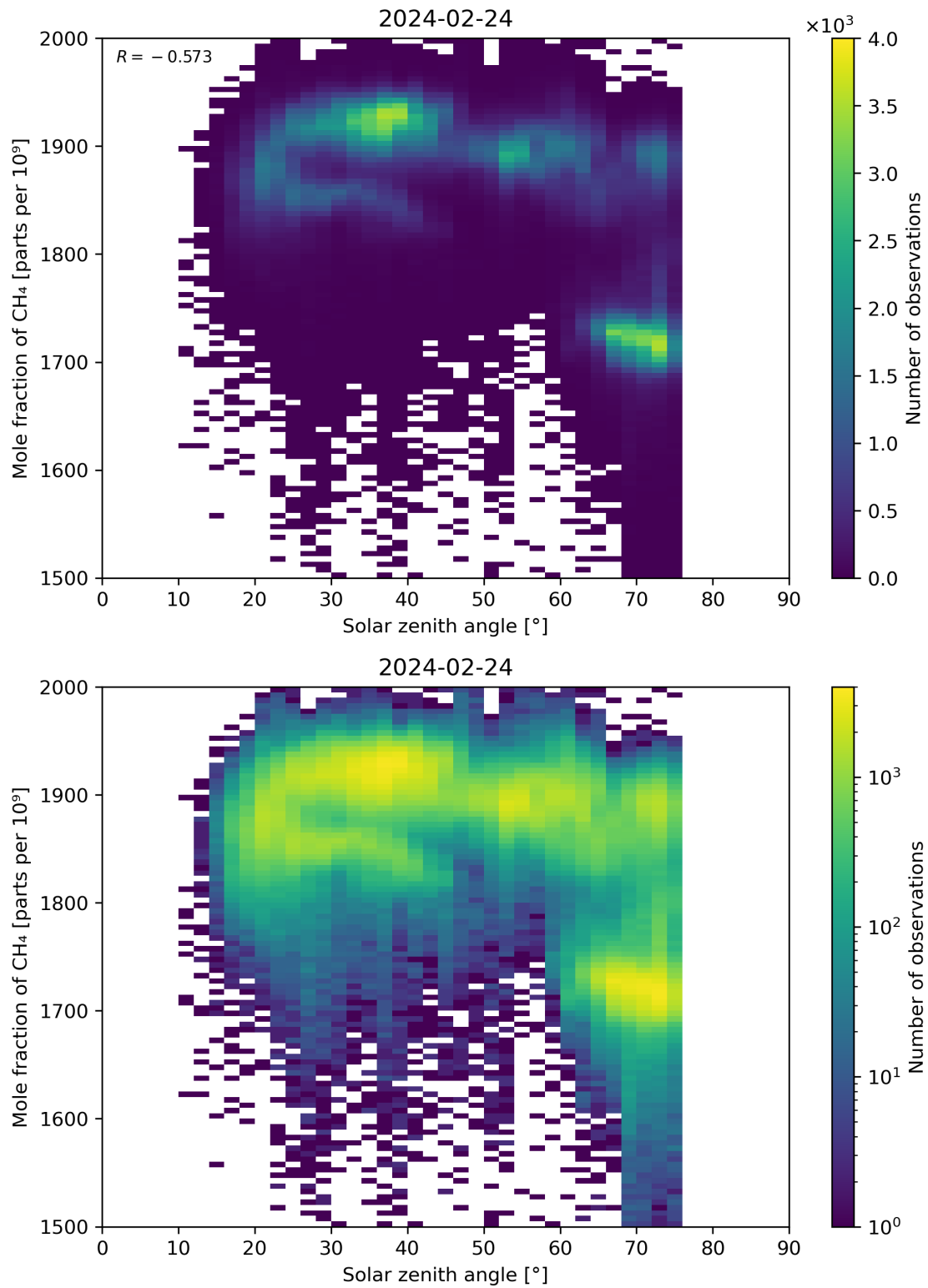
Figure 99: Scatter density plot of “Solar zenith angle” against “Mole fraction of \text{CH}_4 ” for 2024-02-23 to 2024-02-25.
