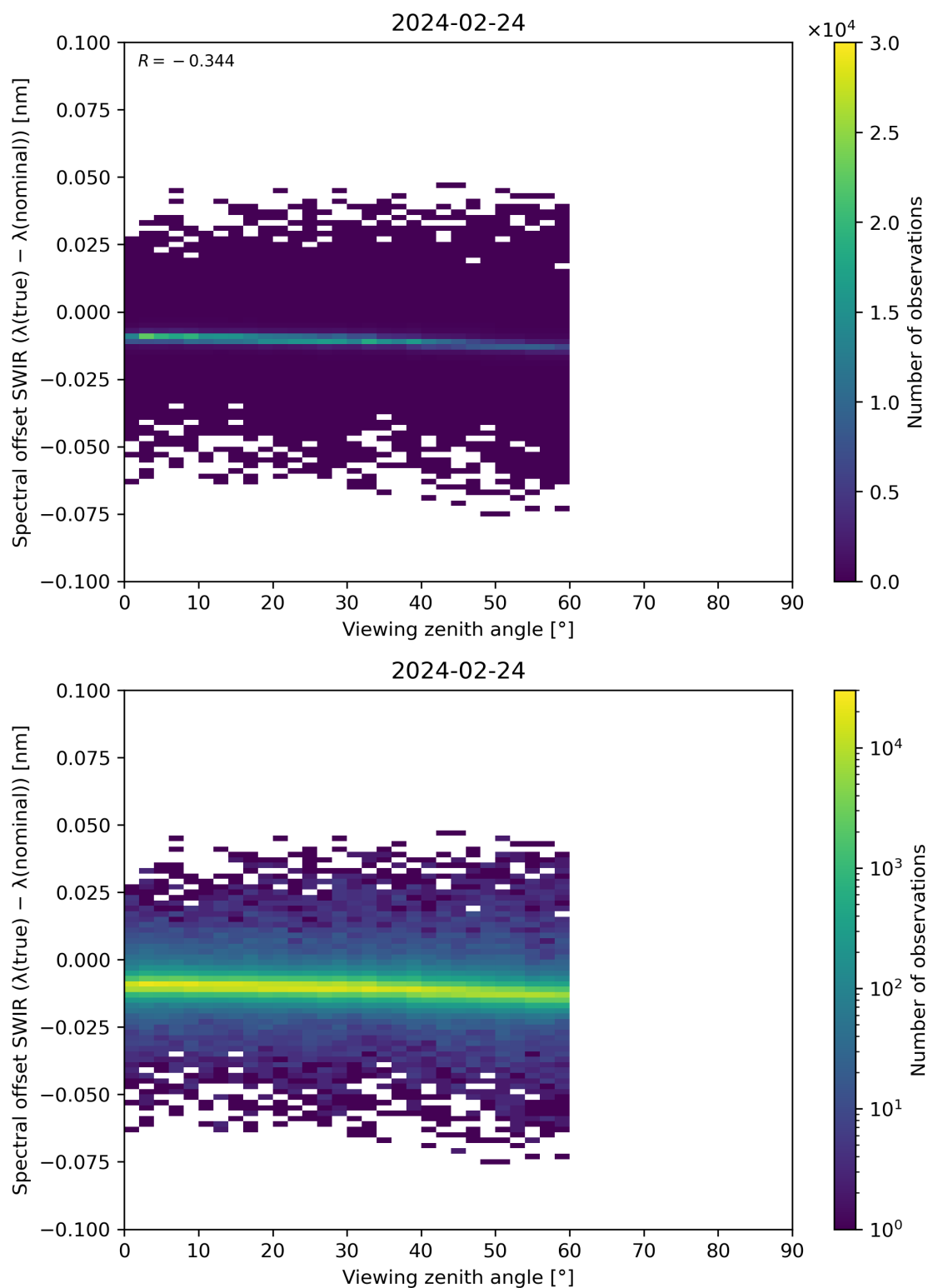
Figure 116: Scatter density plot of “Viewing zenith angle” against “Spectral offset SWIR ( \lambda(\text{true}) - \lambda(\text{nominal}) )” for 2024-02-23 to 2024-02-25.
