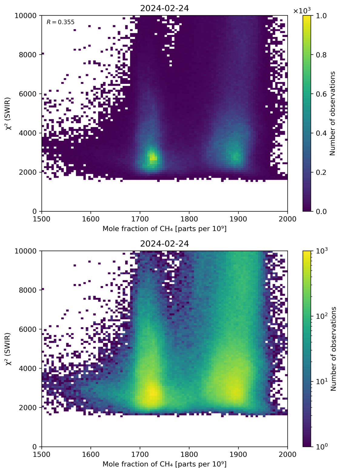
Figure 71: Scatter density plot of “Mole fraction of \text{CH}_4 ” against “ \chi^2 (SWIR)” for 2024-02-23 to 2024-02-25.
