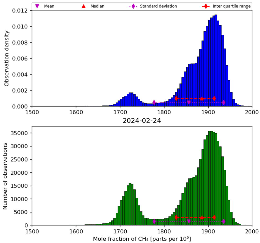
Figure 23: Histogram of “Mole fraction of CH 4 ” for 2024-02-23 to 2024-02-25
