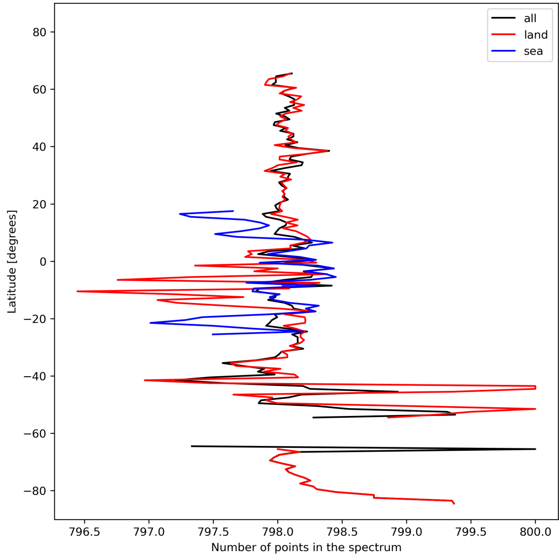
Figure 15: Zonal average of “Number of points in the spectrum” for 2024-02-23 to 2024-02-25.
