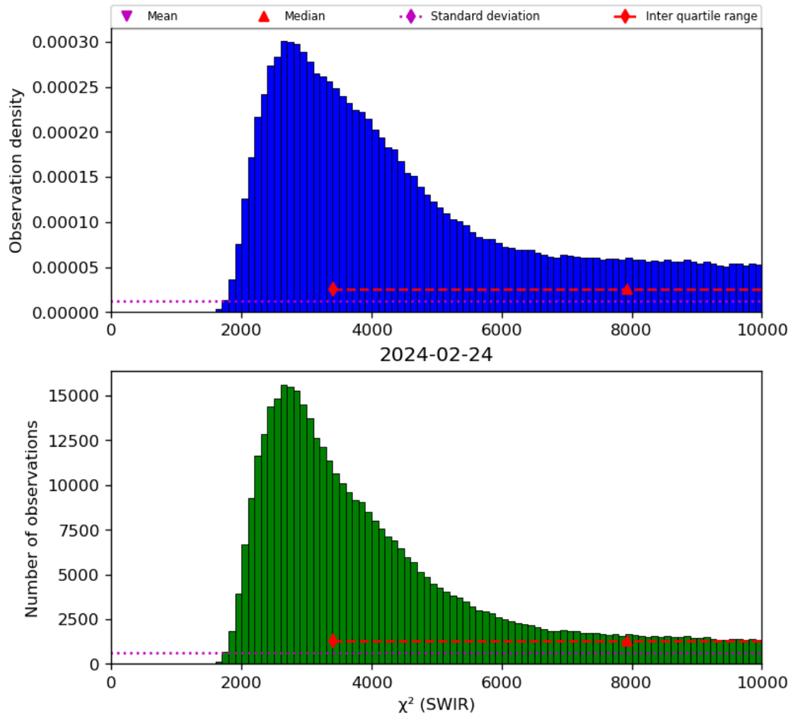
Figure 28: Histogram of “ \chi^2 (SWIR)” for 2024-02-23 to 2024-02-25
