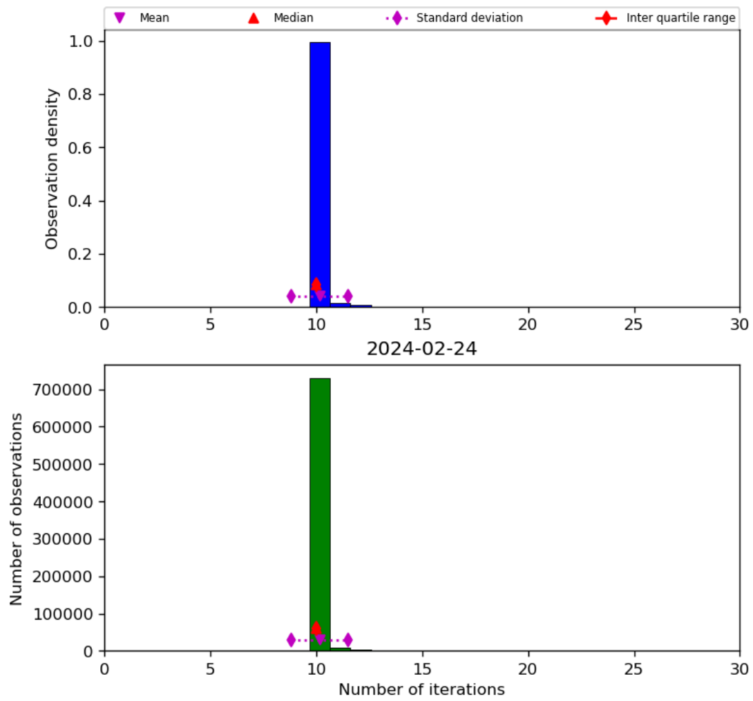
Figure 31: Histogram of "Number of iterations" for 2024-02-23 to 2024-02-25
