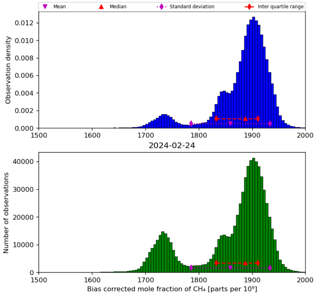
Figure 25: Histogram of “Bias corrected mole fraction of CH 4 ” for 2024-02-23 to 2024-02-25
