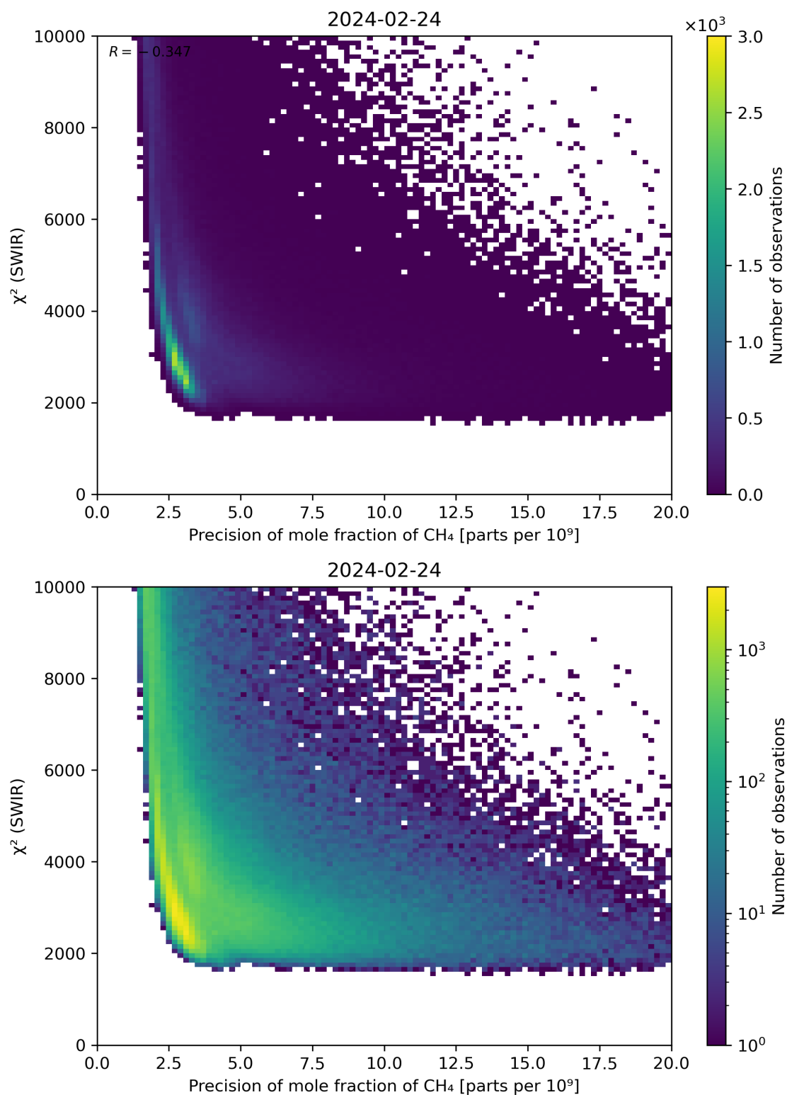
Figure 79: Scatter density plot of “Precision of mole fraction of \text{CH}_4 ” against “ \chi^2 (SWIR)” for 2024-02-23 to 2024-02-25.
