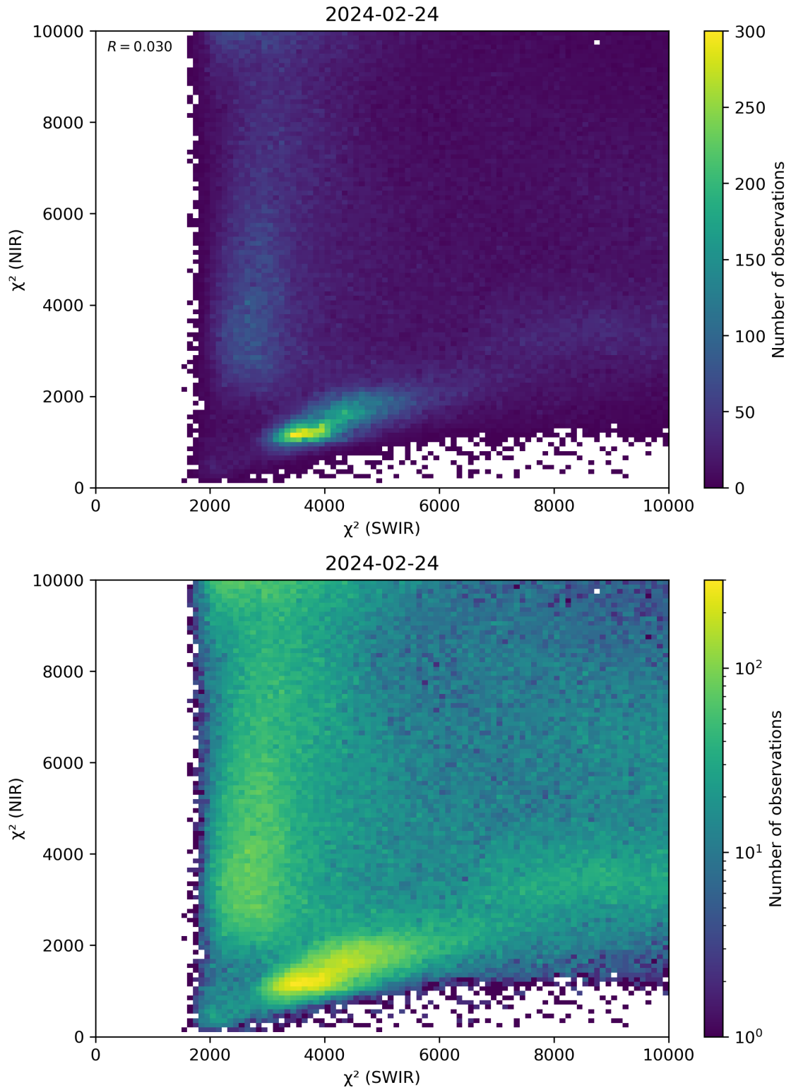
Figure 47: Scatter density plot of “ \chi^2 (SWIR)” against “ \chi^2 (NIR)” for 2024-02-23 to 2024-02-25.
