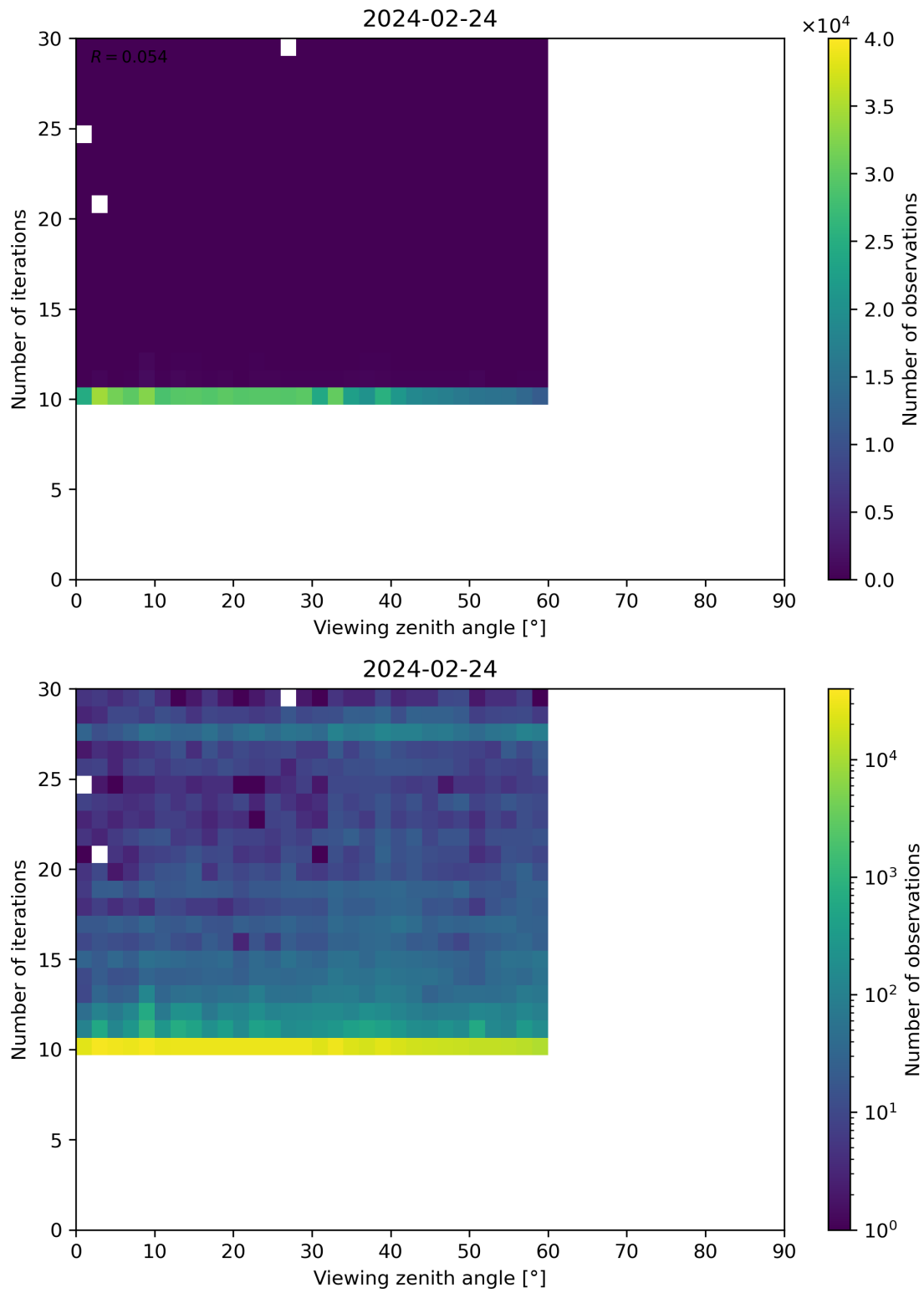
Figure 113: Scatter density plot of “Viewing zenith angle” against “Number of iterations” for 2024-02-23 to 2024-02-25.
