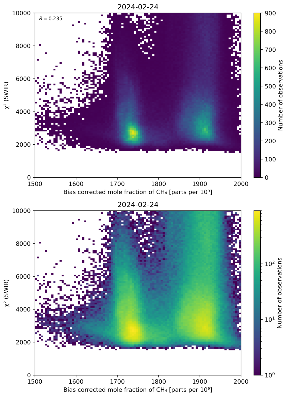
Figure 64: Scatter density plot of “Bias corrected mole fraction of \text{CH}_4 ” against “ \chi^2 (SWIR)” for 2024-02-23 to 2024-02-25.
