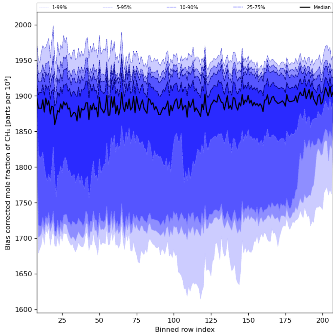
Figure 36: Along track statistics of “Bias corrected mole fraction of CH 4 ” for 2024-02-23 to 2024-02-25
