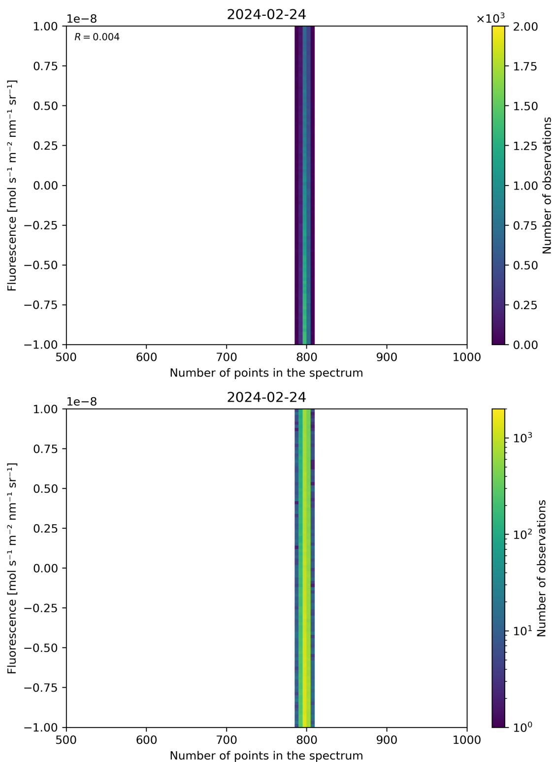
Figure 91: Scatter density plot of “Number of points in the spectrum” against “Fluorescence” for 2024-02-23 to 2024-02-25.
