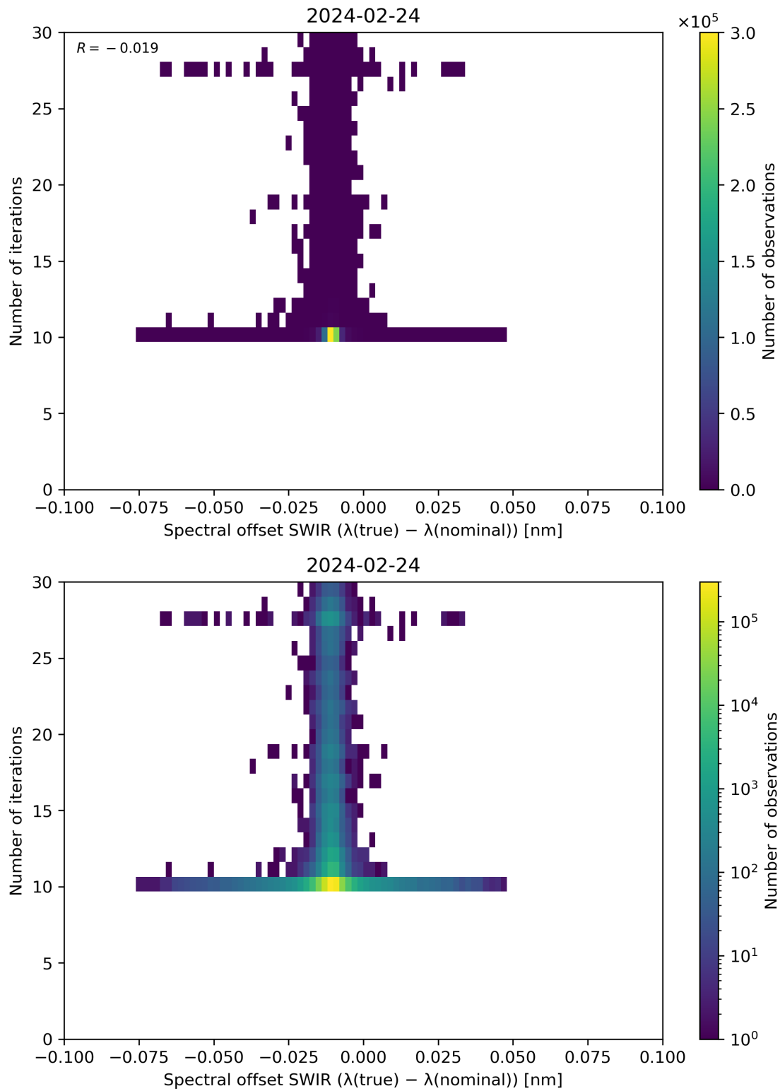
Figure 121: Scatter density plot of “Spectral offset SWIR ( \lambda(\text{true}) - \lambda(\text{nominal}) )” against “Number of iterations” for 2024-02-23 to 2024-02-25.
