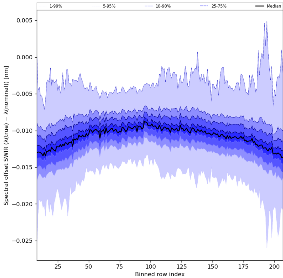
Figure 38: Along track statistics of “Spectral offset SWIR ( \lambda(\text{true}) - \lambda(\text{nominal}) )” for 2024-02-23 to 2024-02-25
