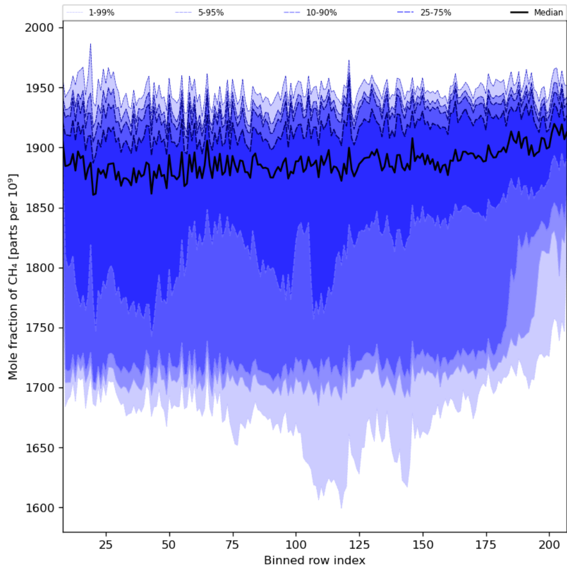
Figure 34: Along track statistics of “Mole fraction of CH 4 ” for 2024-02-23 to 2024-02-25
