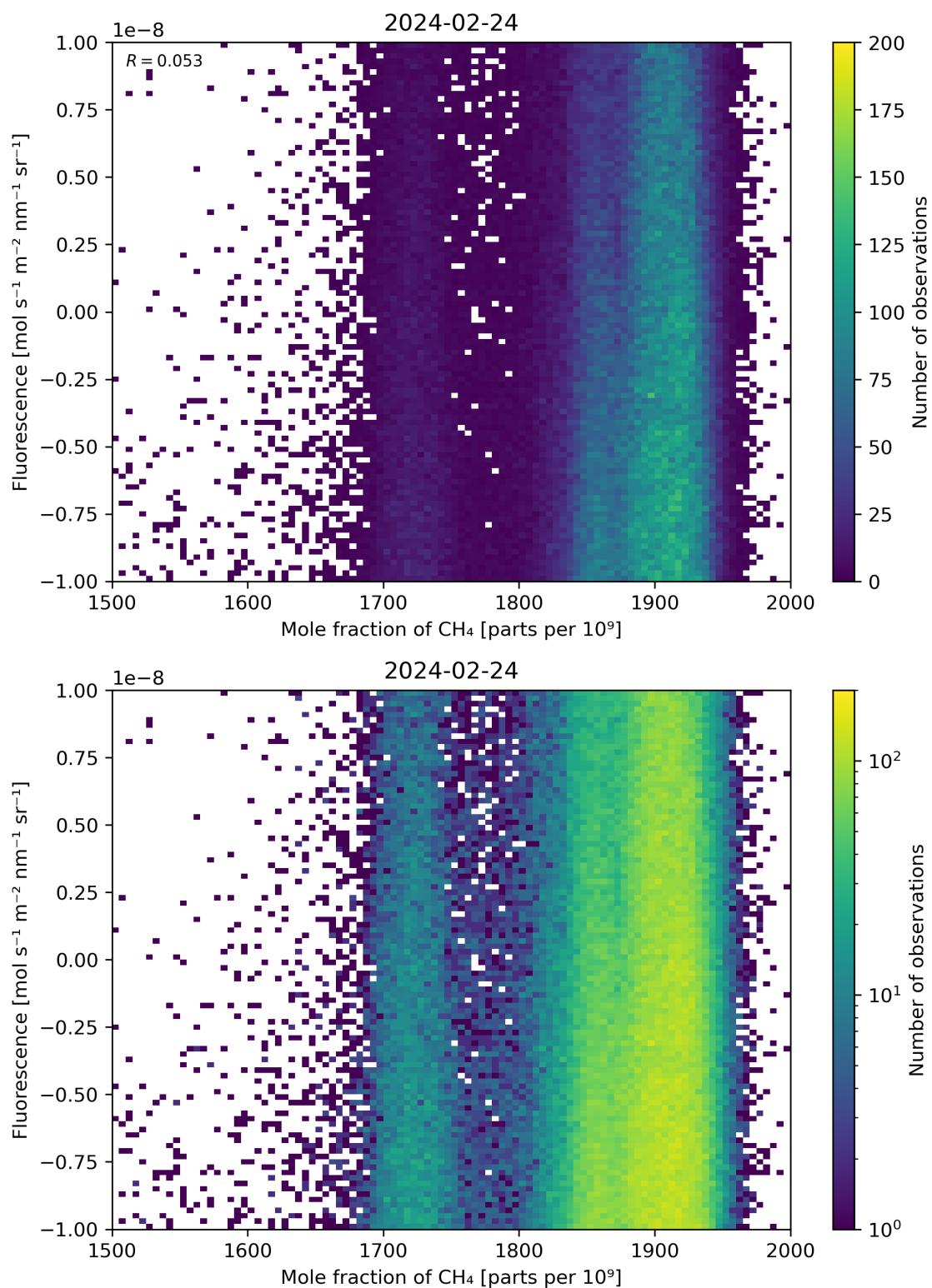
Figure 73: Scatter density plot of “Mole fraction of \text{CH}_4 ” against “Fluorescence” for 2024-02-23 to 2024-02-25.
