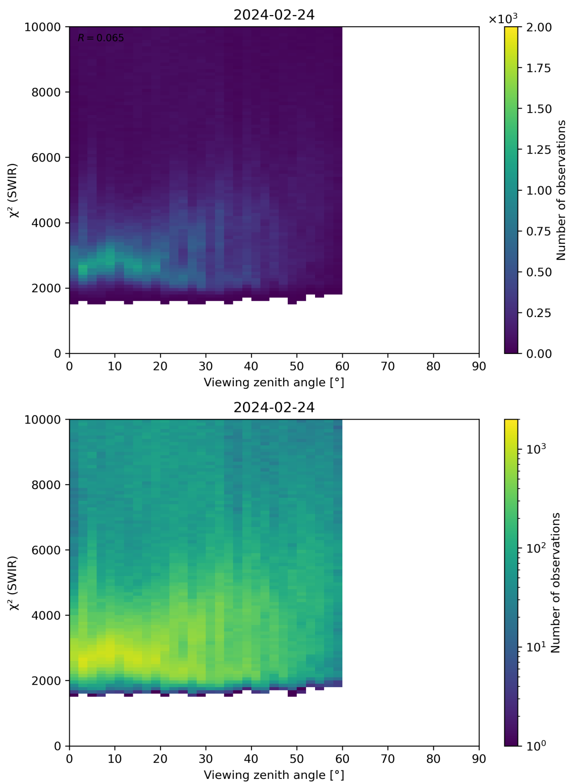
Figure 106: Scatter density plot of “Viewing zenith angle” against “ \chi^2 (SWIR)” for 2024-02-23 to 2024-02-25.
