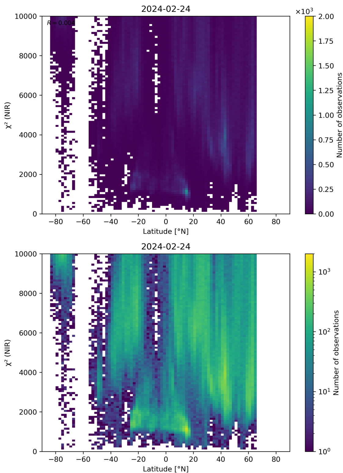
Figure 53: Scatter density plot of “Latitude” against “ \chi^2 (NIR)” for 2024-02-23 to 2024-02-25.
