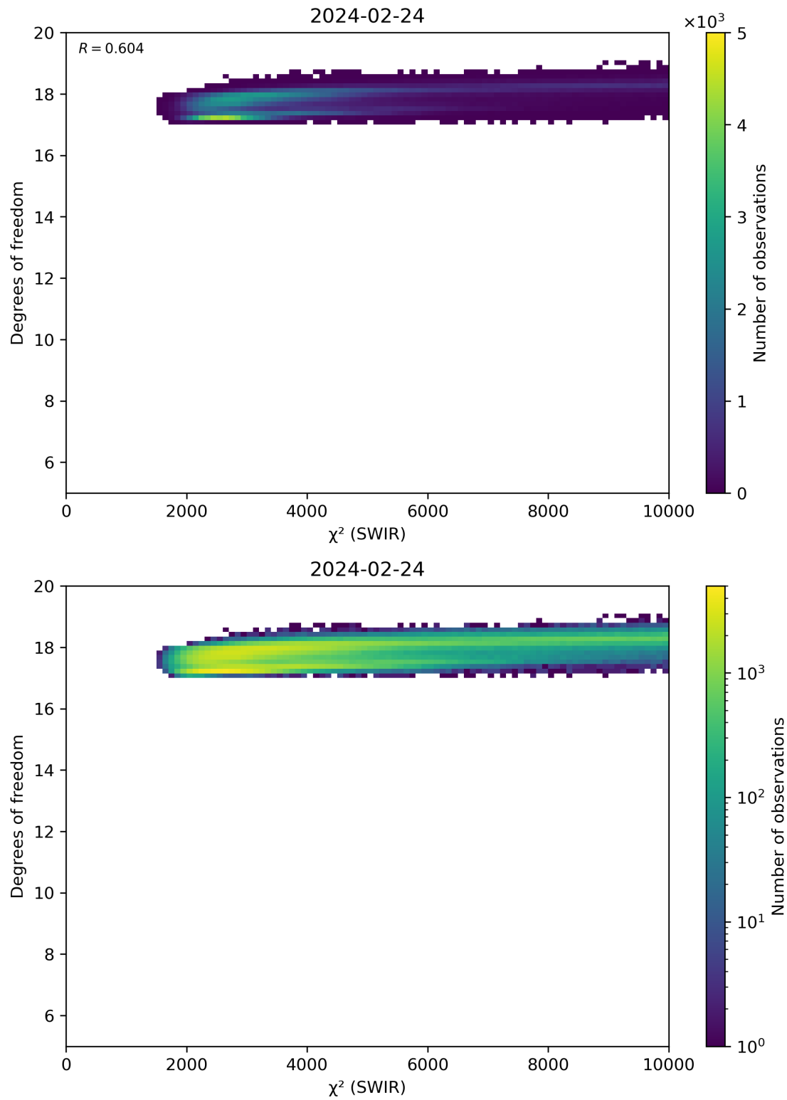
Figure 48: Scatter density plot of “ \chi^2 (SWIR)” against “Degrees of freedom” for 2024-02-23 to 2024-02-25.
