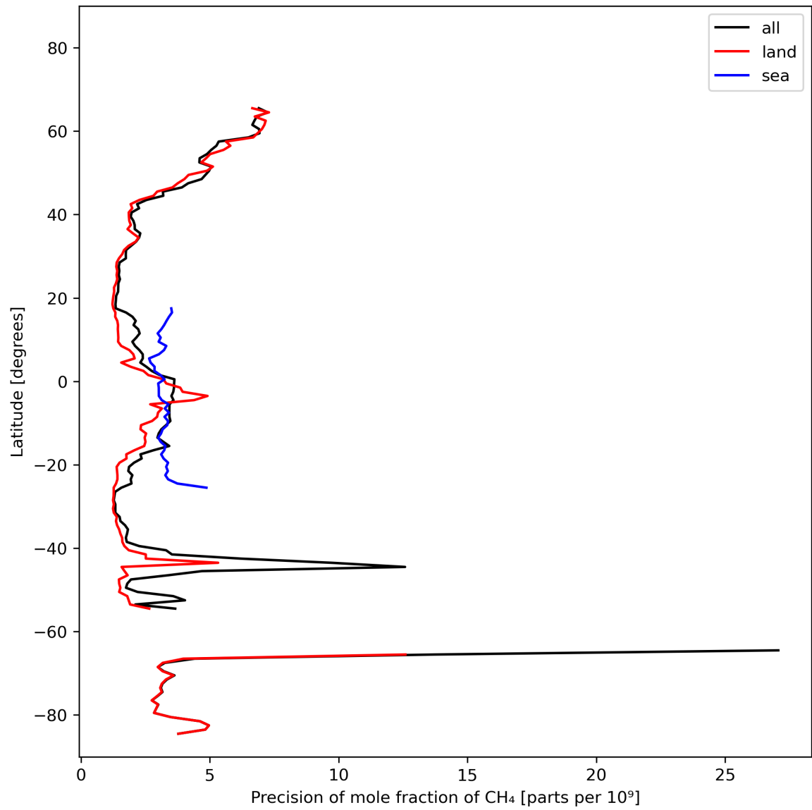
Figure 13: Zonal average of “Precision of mole fraction of CH 4 ” for 2024-02-23 to 2024-02-25.
