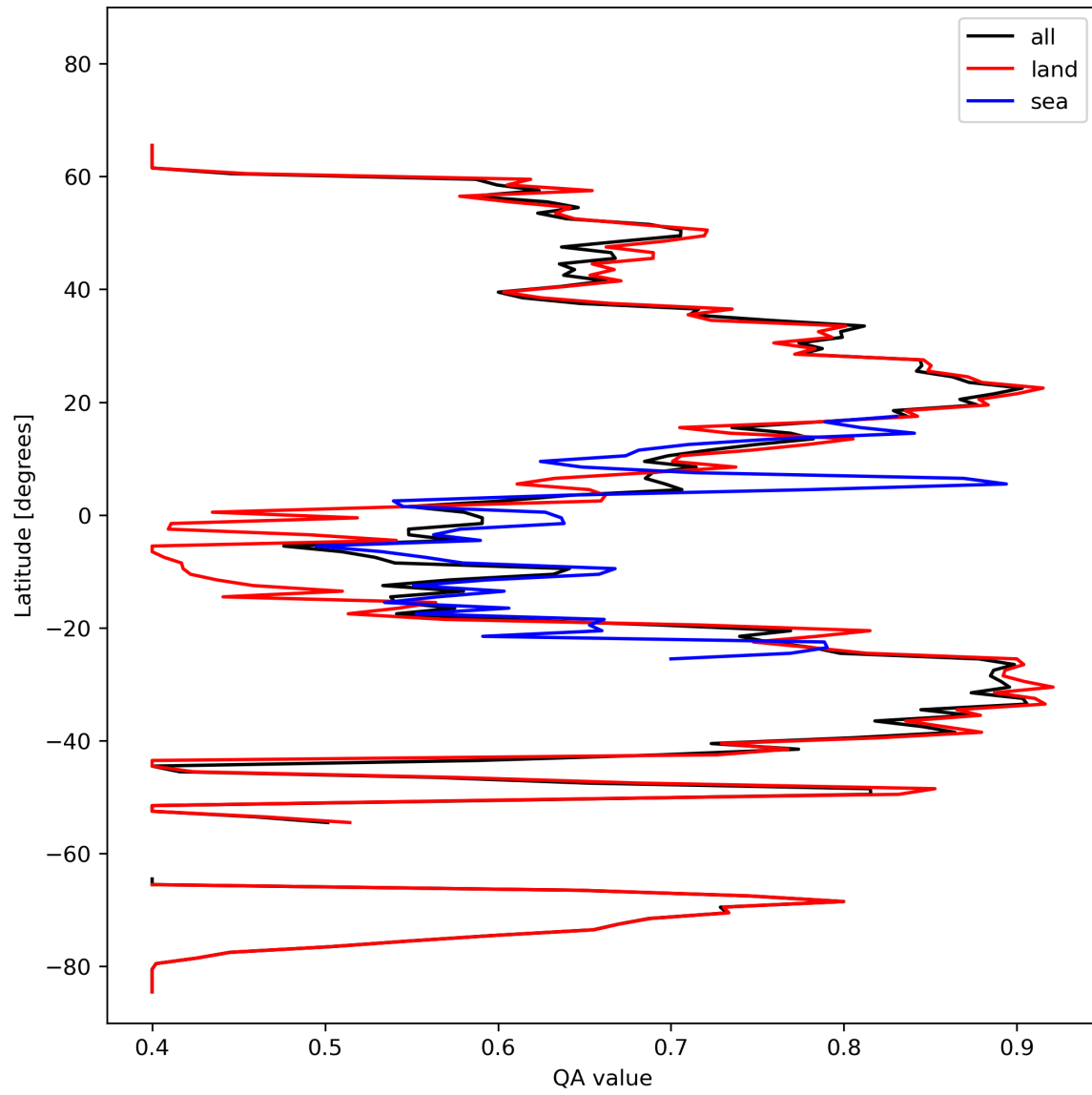
Figure 11: Zonal average of “QA value” for 2024-02-23 to 2024-02-25.
