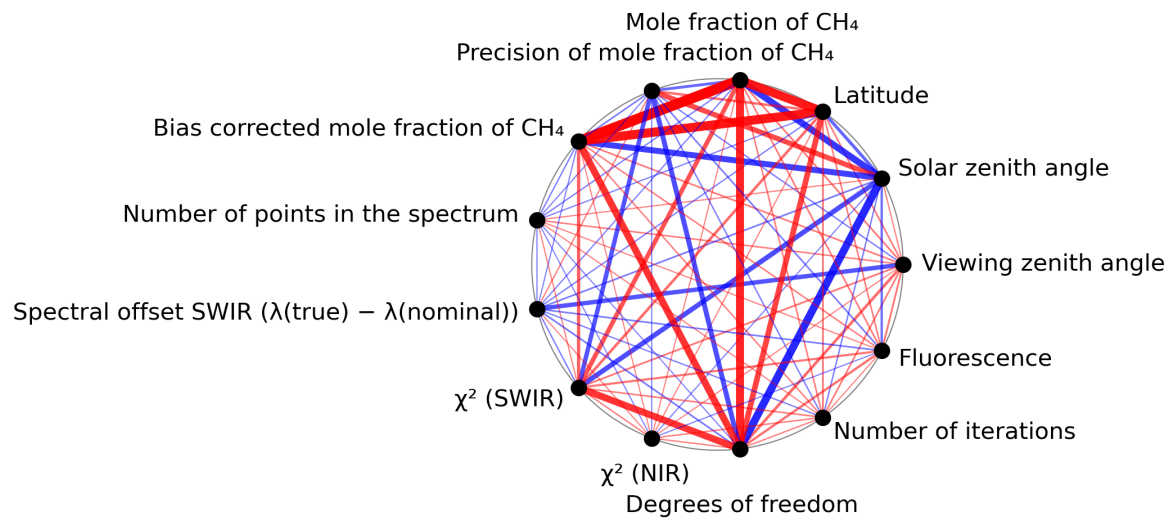
Figure 1: Map of correlation graph for 2024-02-23 to 2024-02-25.
