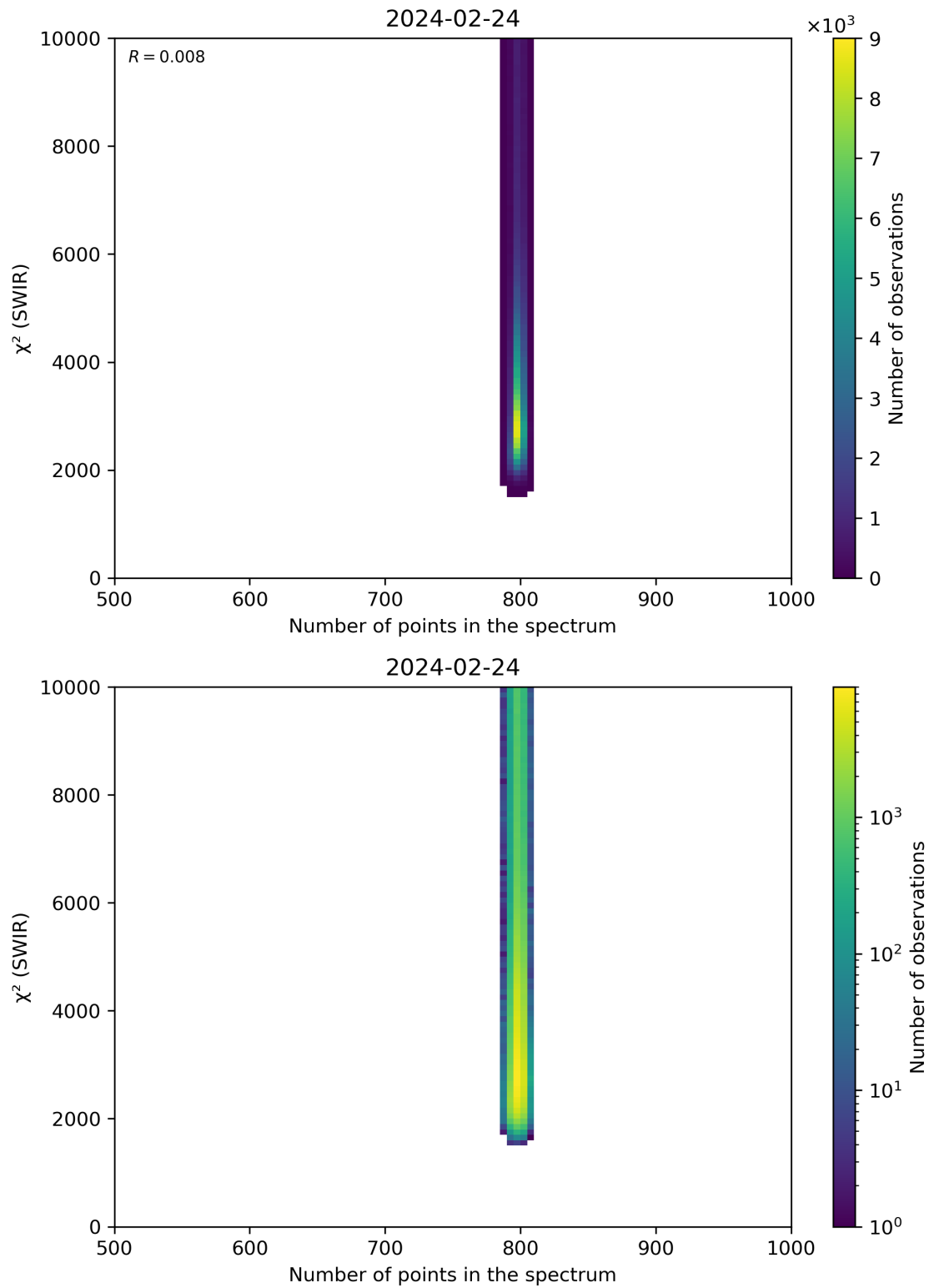
Figure 89: Scatter density plot of “Number of points in the spectrum” against “ \chi^2 (SWIR)” for 2024-02-23 to 2024-02-25.
