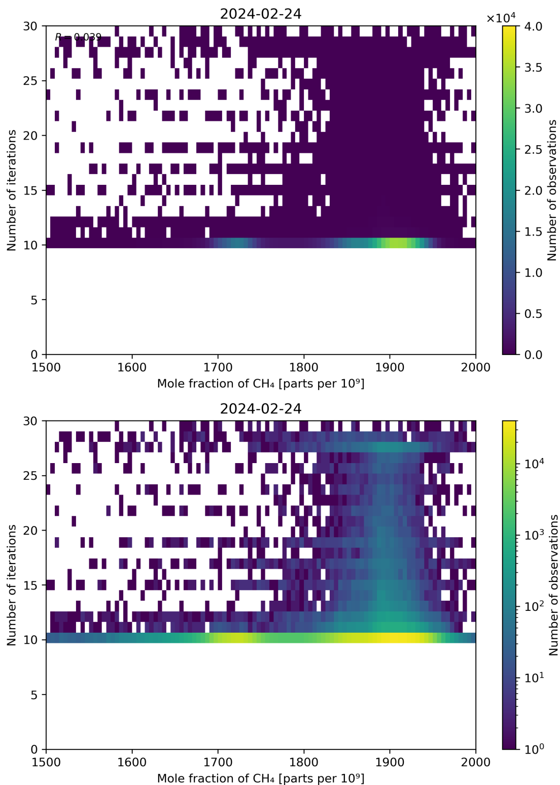
Figure 76: Scatter density plot of “Mole fraction of CH 4 ” against “Number of iterations” for 2024-02-23 to 2024-02-25.
