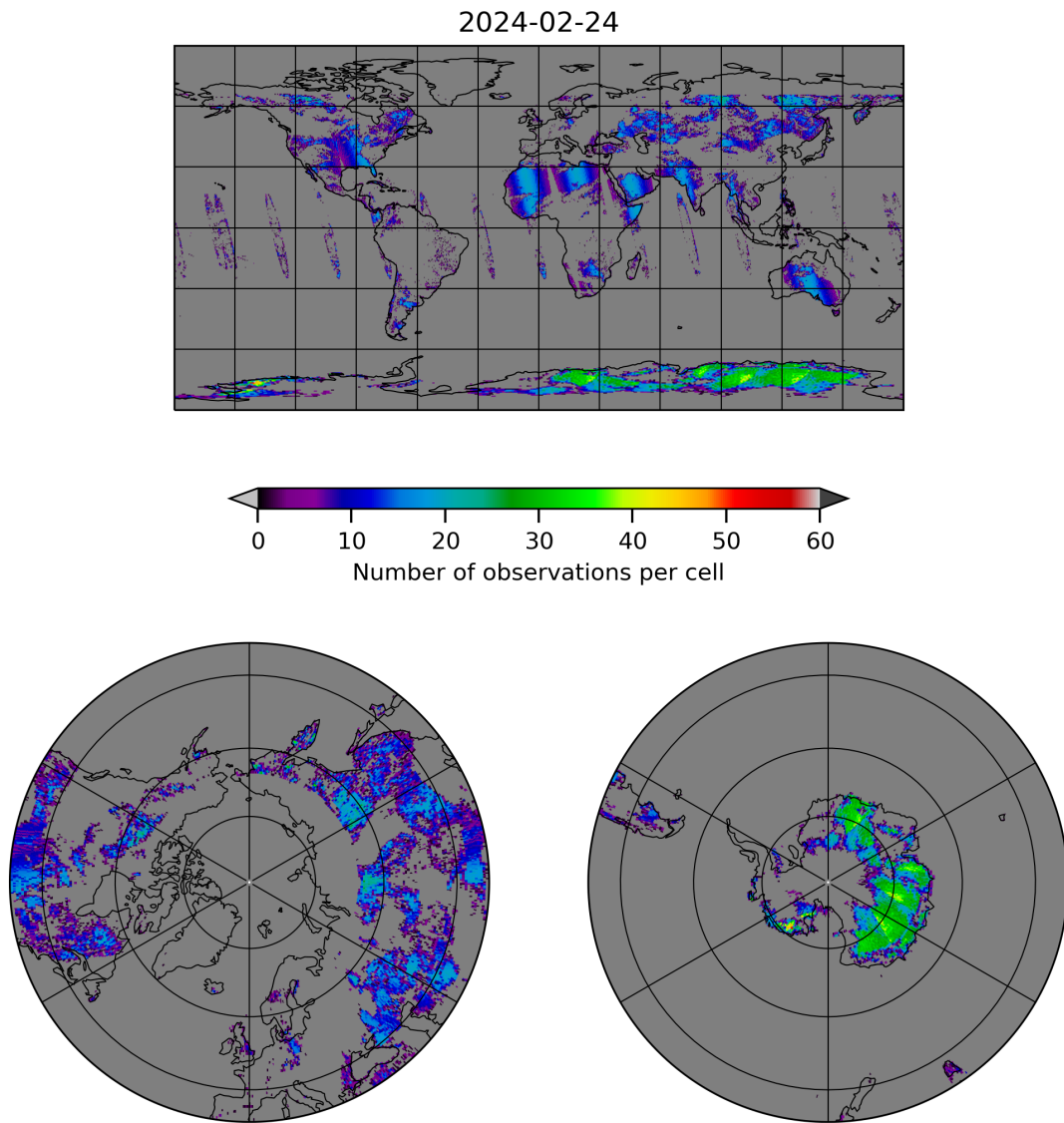
Figure 10: Map of the number of observations for 2024-02-23 to 2024-02-25
