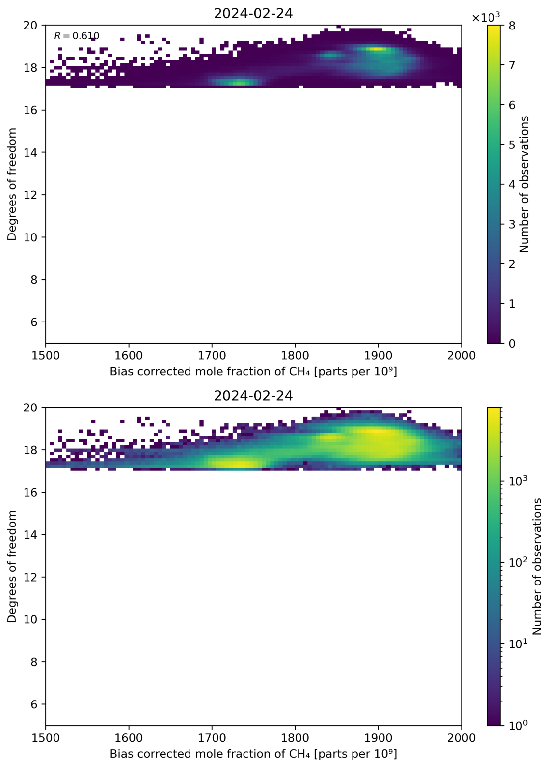
Figure 65: Scatter density plot of “Bias corrected mole fraction of CH 4 ” against “Degrees of freedom” for 2024-02-23 to 2024-02-25.
