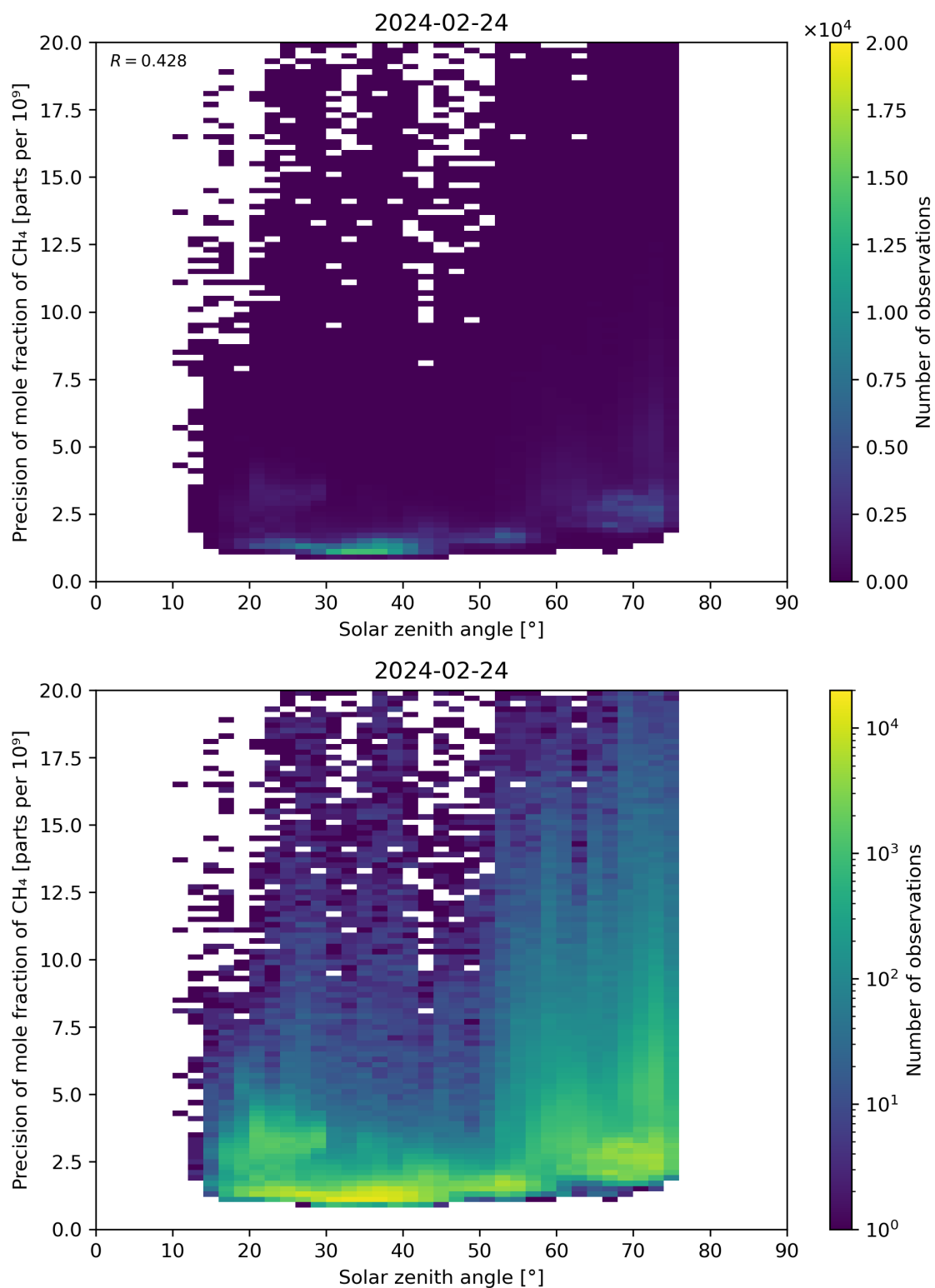
Figure 101: Scatter density plot of “Solar zenith angle” against “Precision of mole fraction of CH 4 ” for 2024-02-23 to 2024-02-25.
