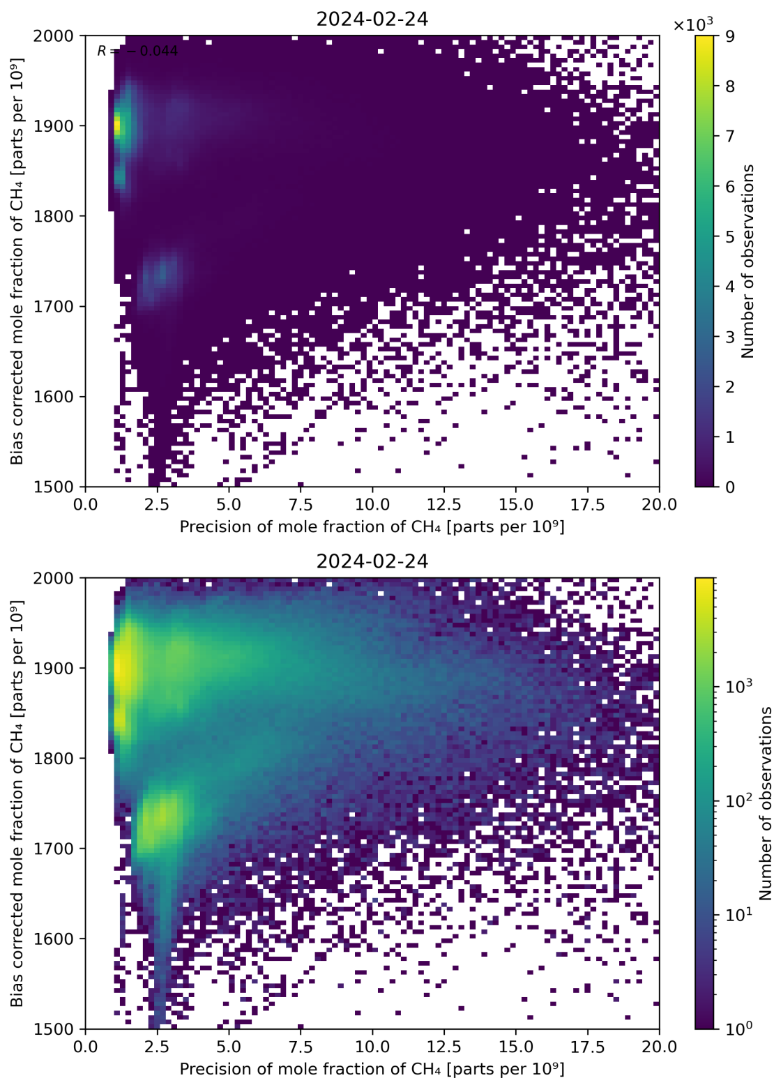
Figure 82: Scatter density plot of “Precision of mole fraction of CH 4 ” against “Bias corrected mole fraction of CH 4 ” for 2024-02-23 to 2024-02-25.
