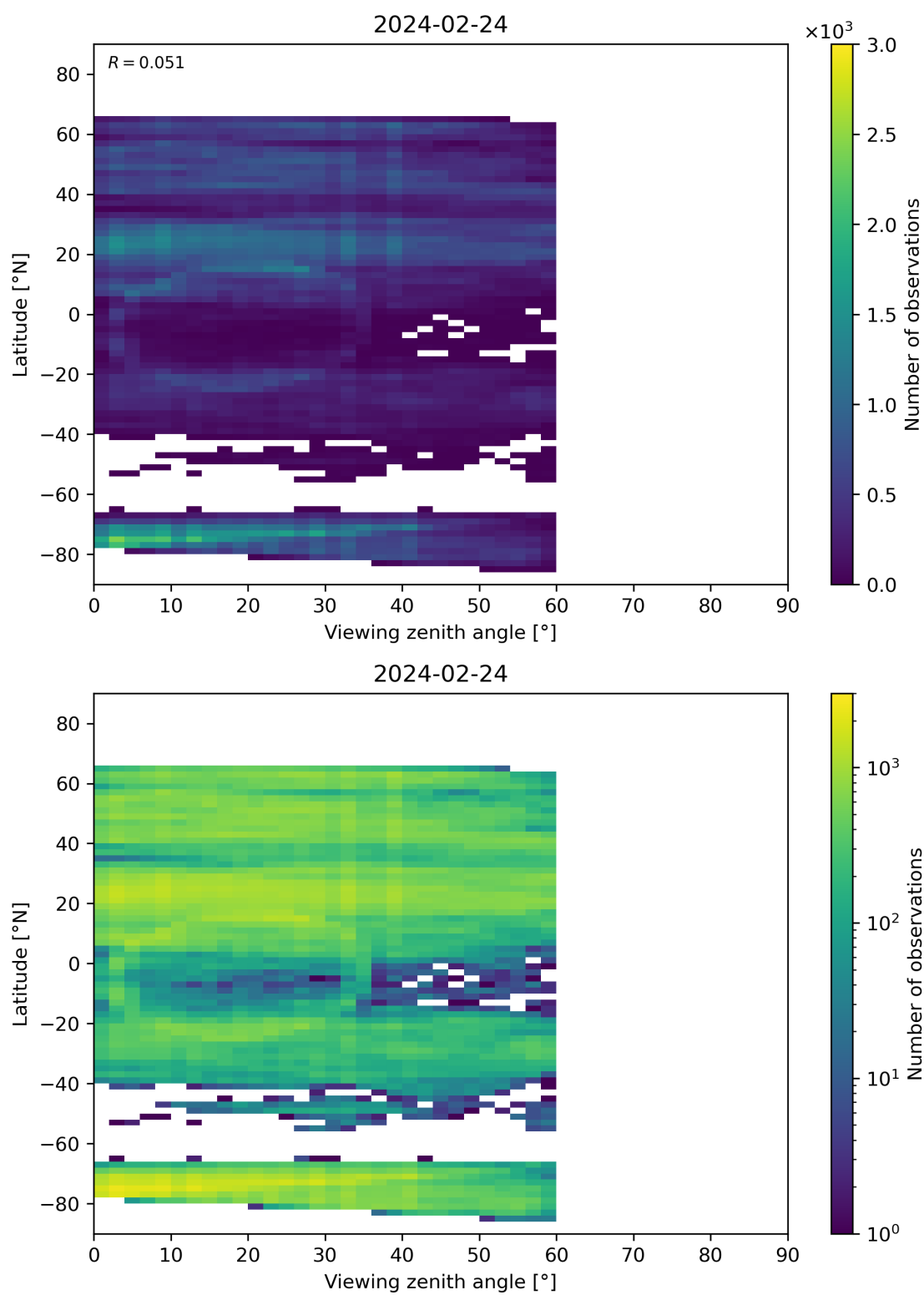
Figure 109: Scatter density plot of “Viewing zenith angle” against “Latitude” for 2024-02-23 to 2024-02-25.
