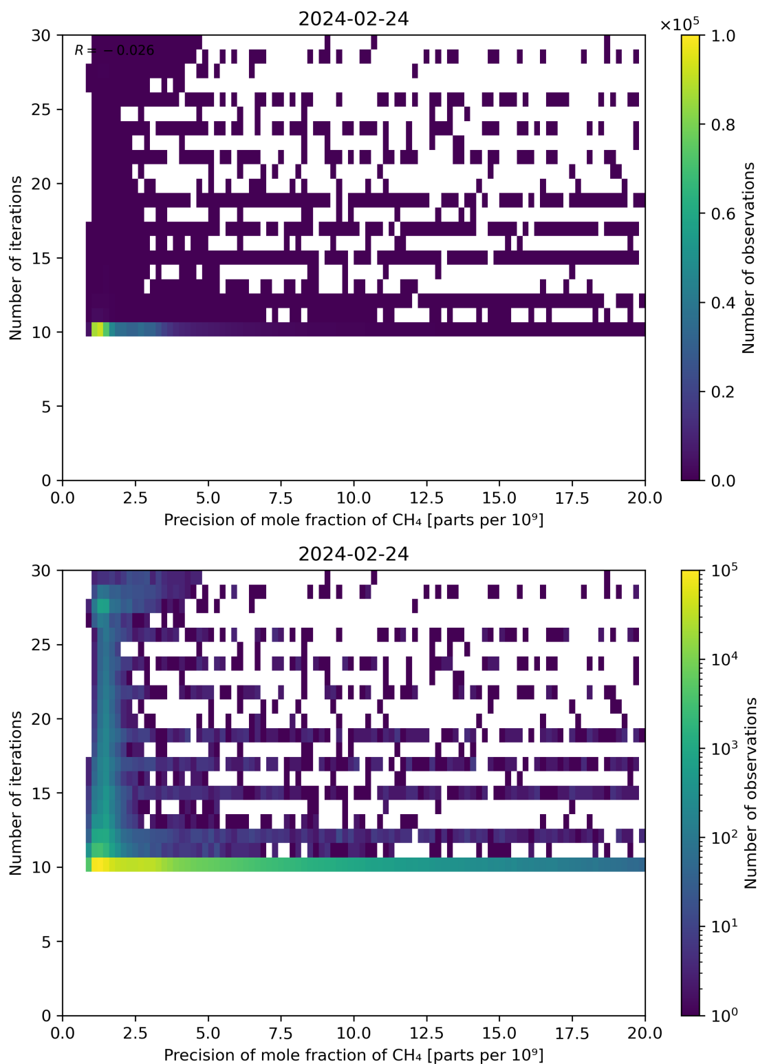
Figure 83: Scatter density plot of “Precision of mole fraction of CH 4 ” against “Number of iterations” for 2024-02-23 to 2024-02-25.
