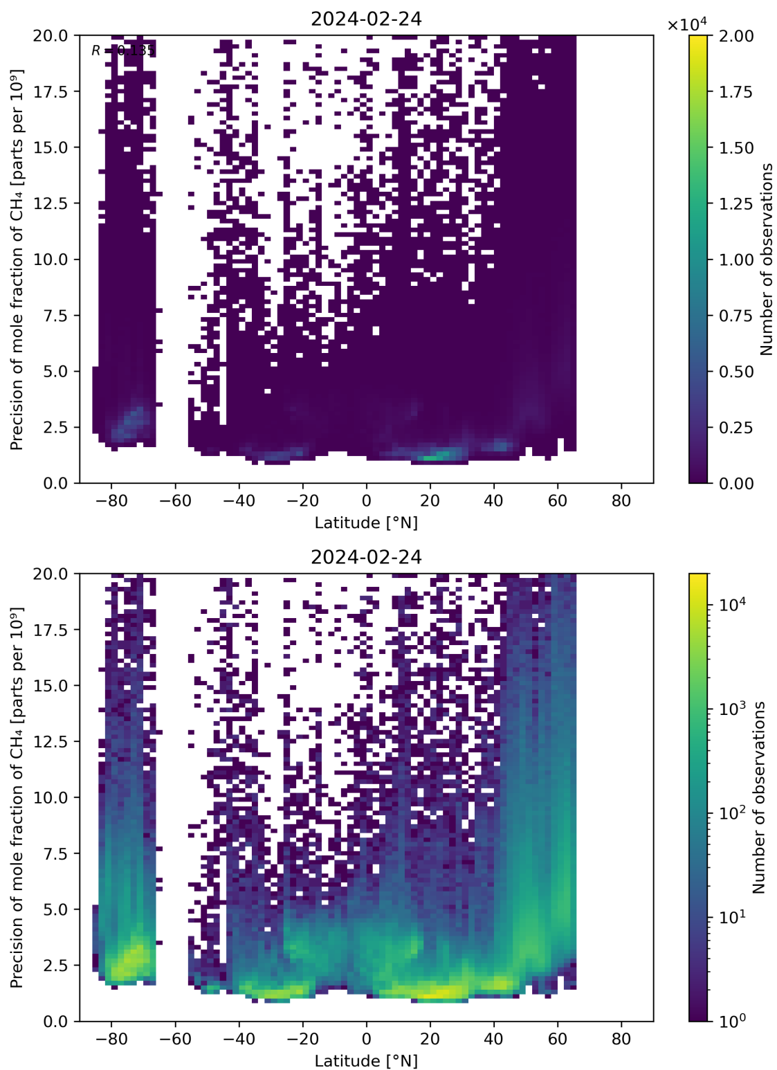
Figure 59: Scatter density plot of “Latitude” against “Precision of mole fraction of CH 4 ” for 2024-02-23 to 2024-02-25.
