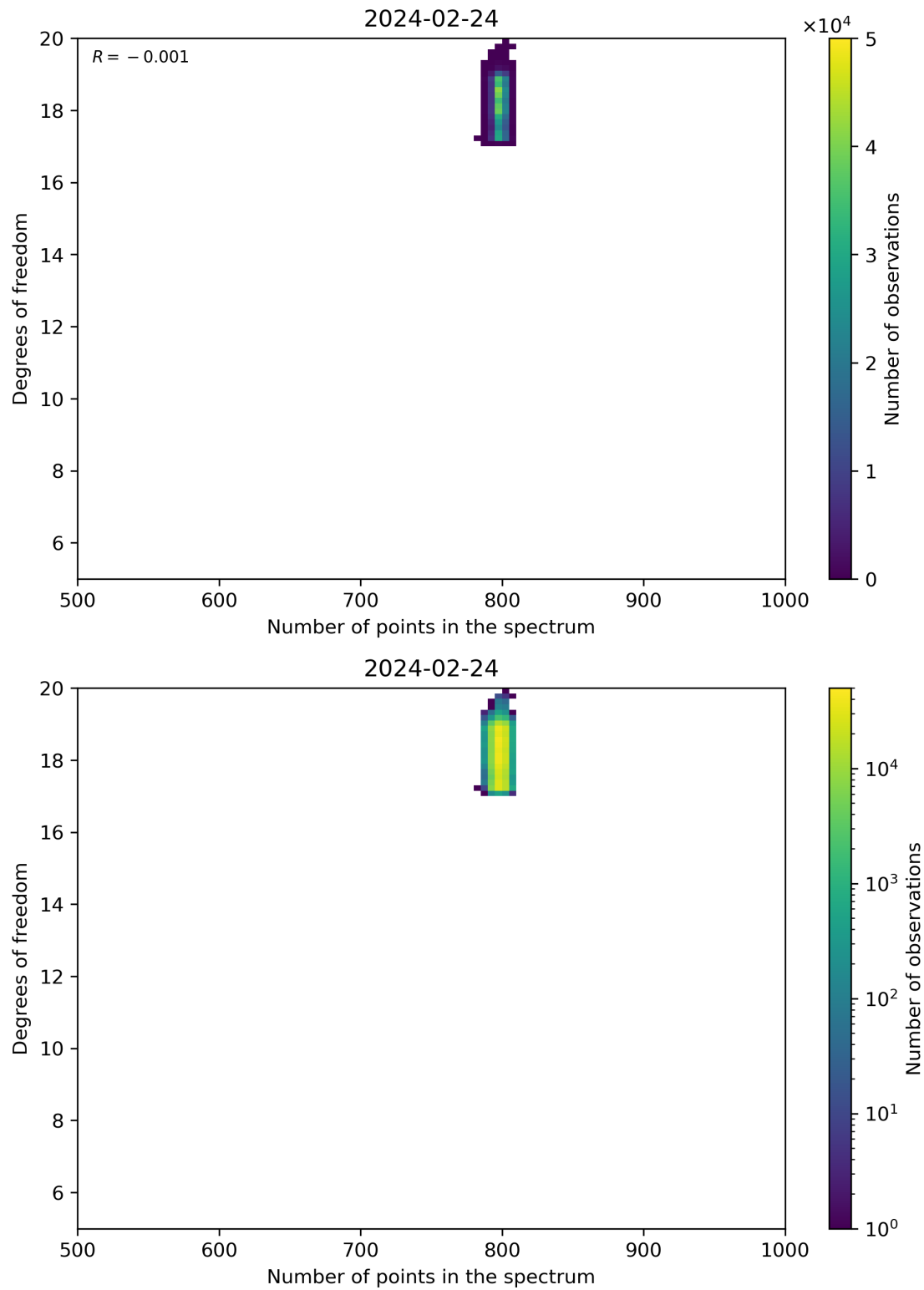
Figure 90: Scatter density plot of “Number of points in the spectrum” against “Degrees of freedom” for 2024-02-23 to 2024-02-25.
