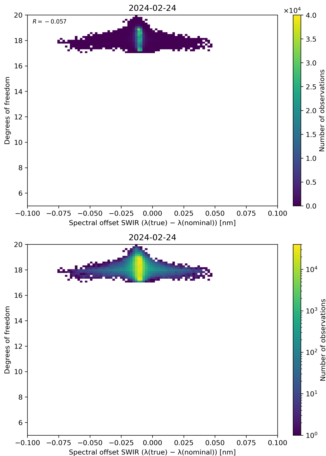
Figure 119: Scatter density plot of “Spectral offset SWIR ( \lambda(\text{true}) - \lambda(\text{nominal}) )” against “Degrees of freedom” for 2024-02-23 to 2024-02-25.
