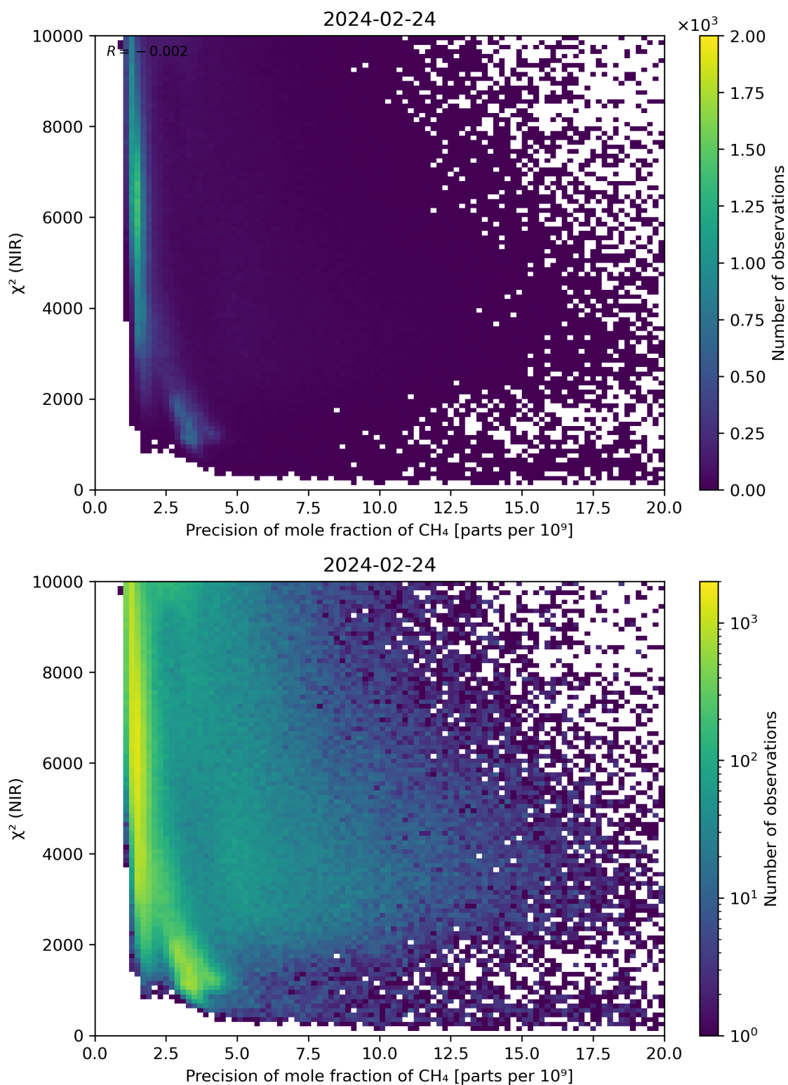
Figure 78: Scatter density plot of “Precision of mole fraction of CH 4 ” against “ \chi^2 (NIR)” for 2024-02-23 to 2024-02-25.
