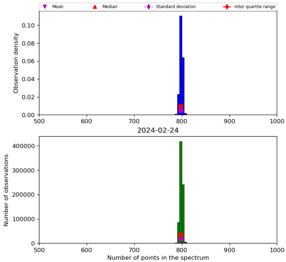
Figure 26: Histogram of “Number of points in the spectrum” for 2024-02-23 to 2024-02-25
