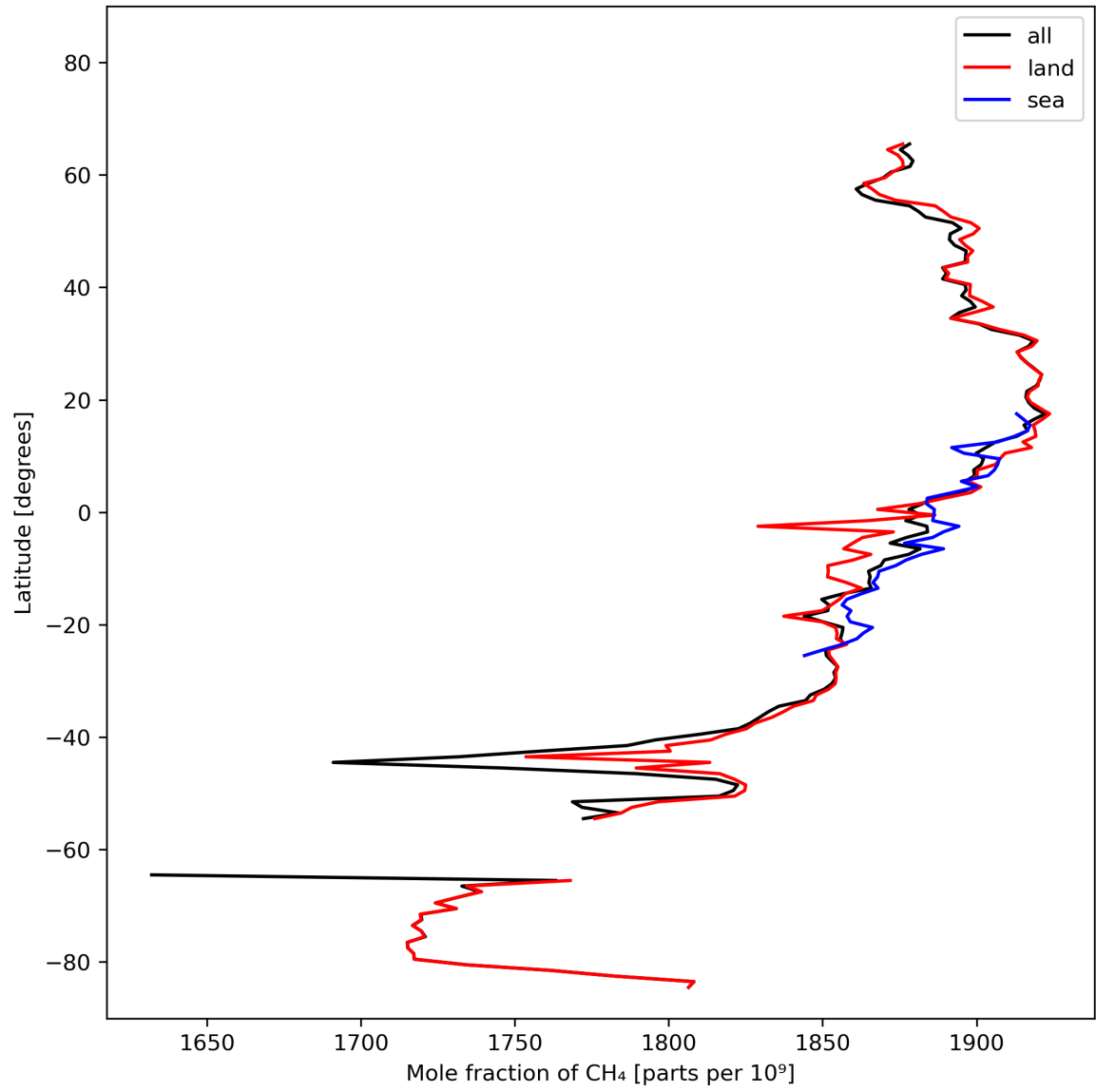
Figure 12: Zonal average of “Mole fraction of \text{CH}_4 ” for 2024-02-23 to 2024-02-25.
