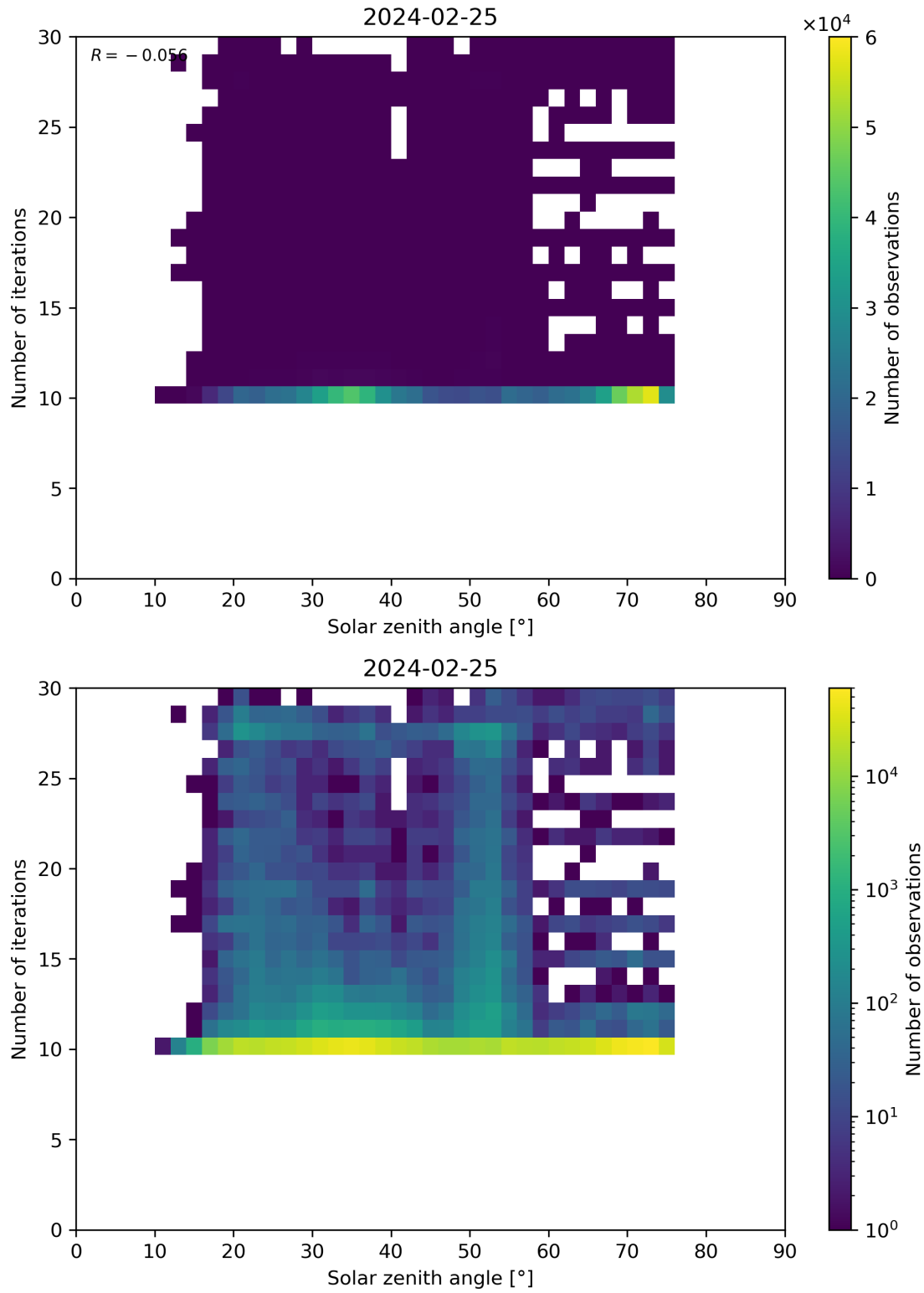
Figure 102: Scatter density plot of “Solar zenith angle” against “Number of iterations” for 2024-02-24 to 2024-02-26.
