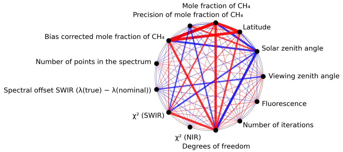
Figure 1: Map of correlation graph for 2024-02-24 to 2024-02-26.
