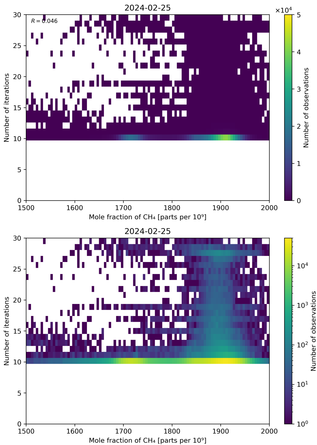
Figure 76: Scatter density plot of “Mole fraction of CH 4 ” against “Number of iterations” for 2024-02-24 to 2024-02-26.
