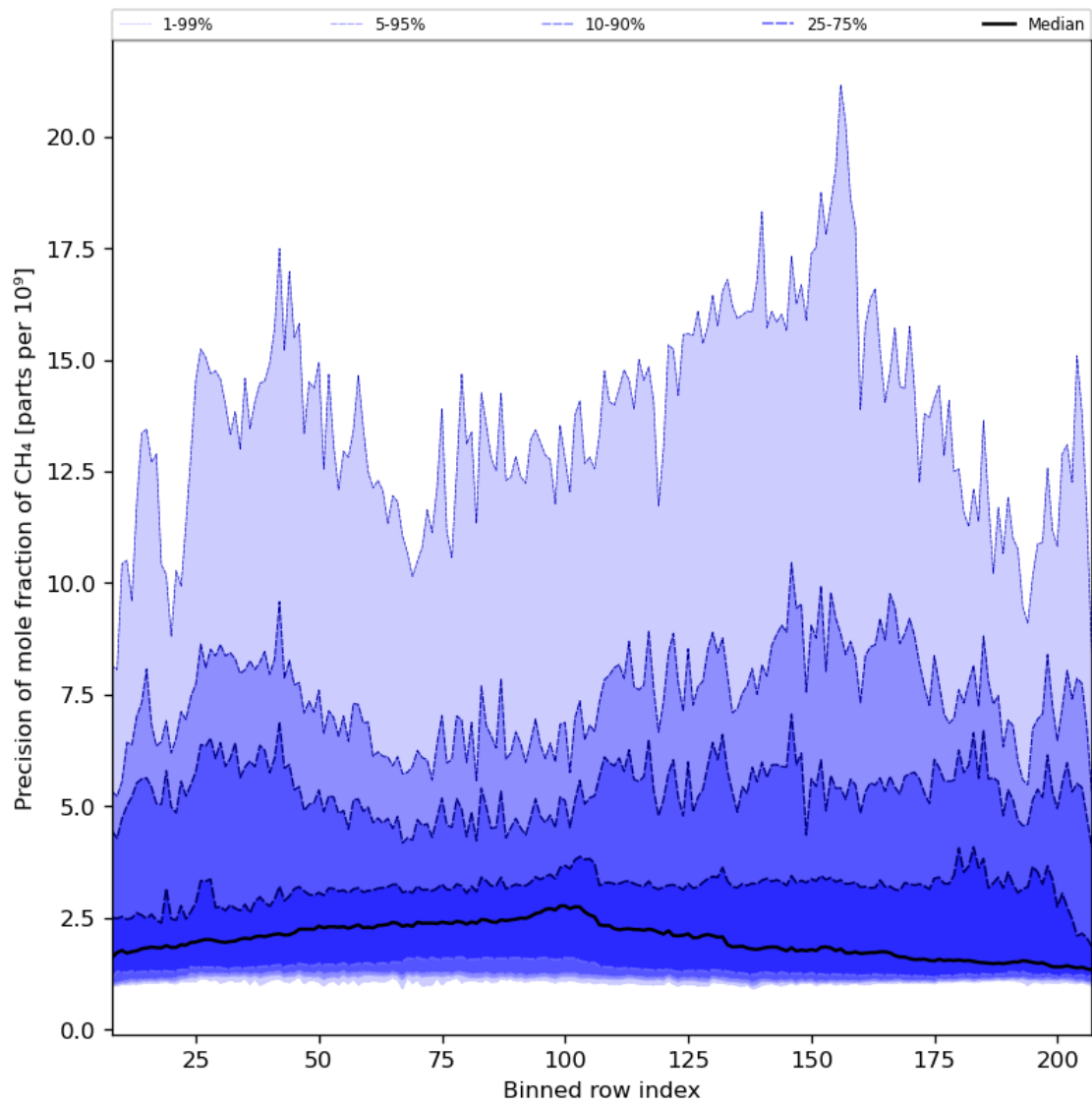
Figure 35: Along track statistics of “Precision of mole fraction of CH 4 ” for 2024-02-24 to 2024-02-26
