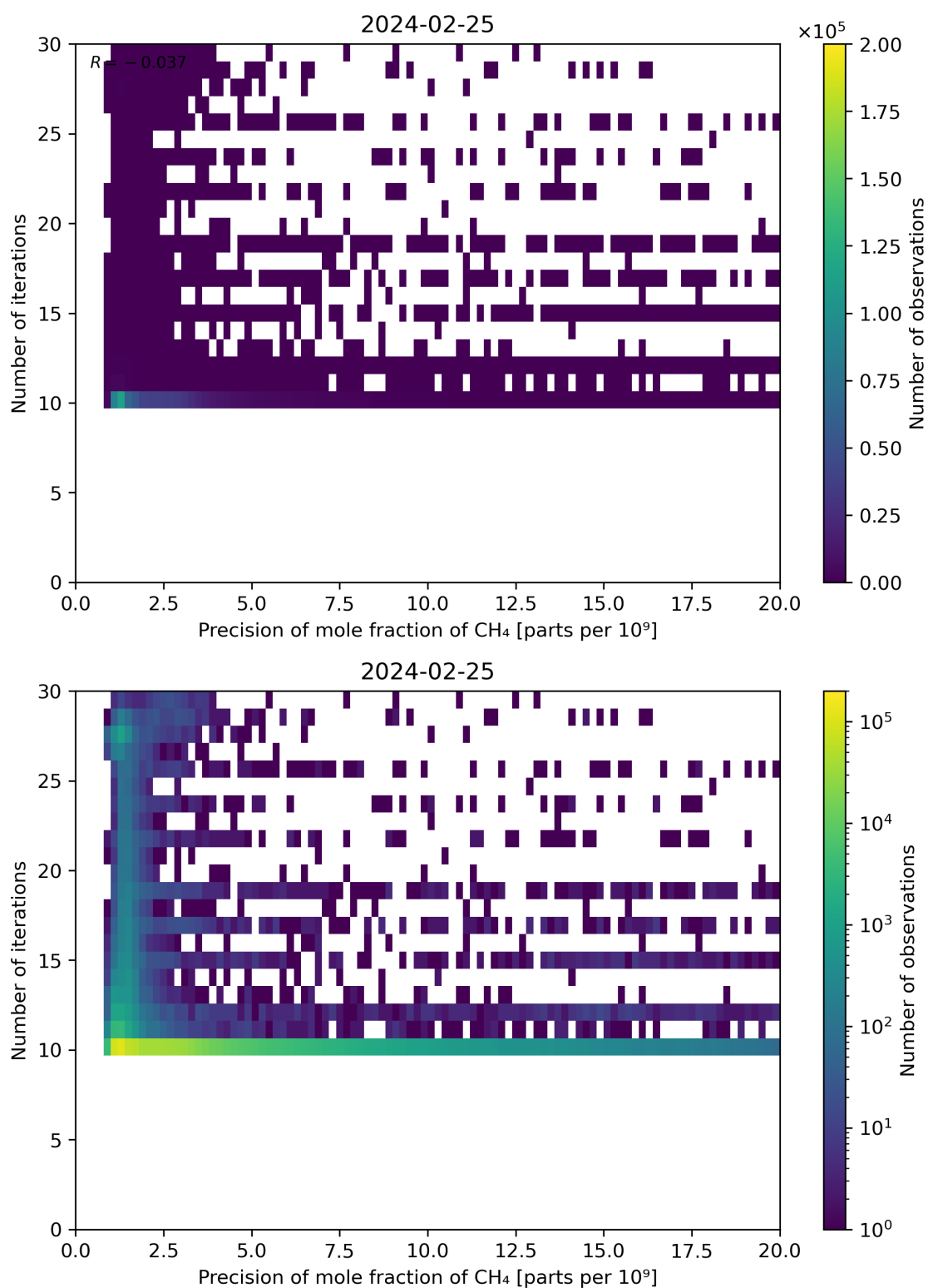
Figure 83: Scatter density plot of “Precision of mole fraction of CH 4 ” against “Number of iterations” for 2024-02-24 to 2024-02-26.
