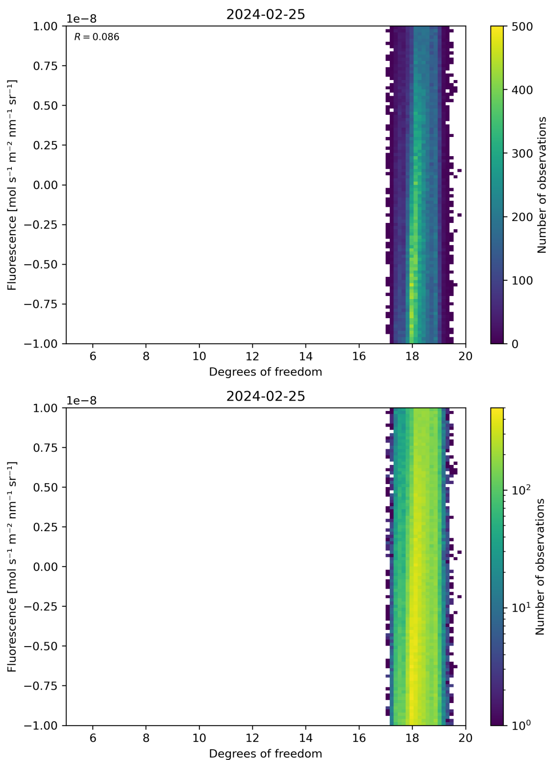
Figure 51: Scatter density plot of “Degrees of freedom” against “Fluorescence” for 2024-02-24 to 2024-02-26.
