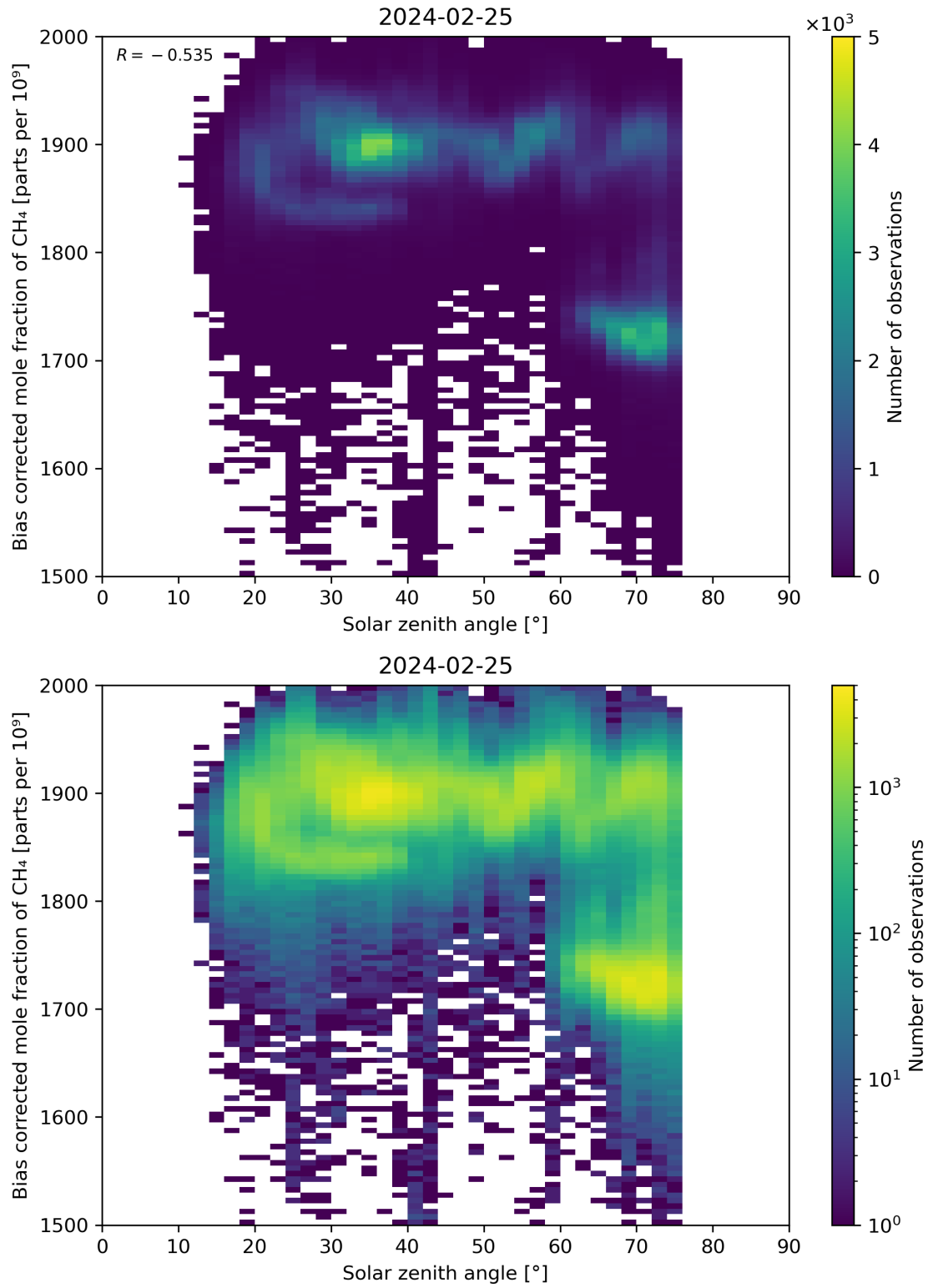
Figure 100: Scatter density plot of “Solar zenith angle” against “Bias corrected mole fraction of \text{CH}_4 ” for 2024-02-24 to 2024-02-26.
