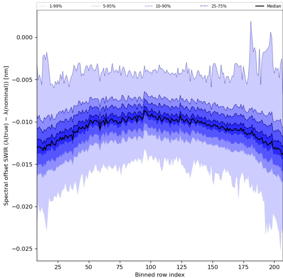
Figure 38: Along track statistics of “Spectral offset SWIR ( \lambda(\text{true}) - \lambda(\text{nominal}) )” for 2024-02-24 to 2024-02-26
