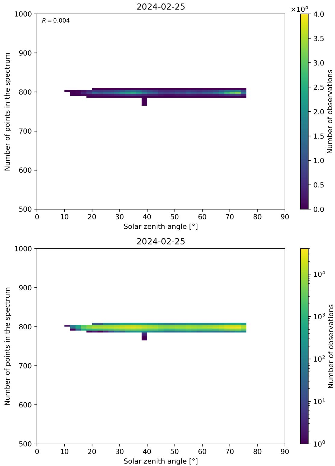
Figure 103: Scatter density plot of “Solar zenith angle” against “Number of points in the spectrum” for 2024-02-24 to 2024-02-26.
