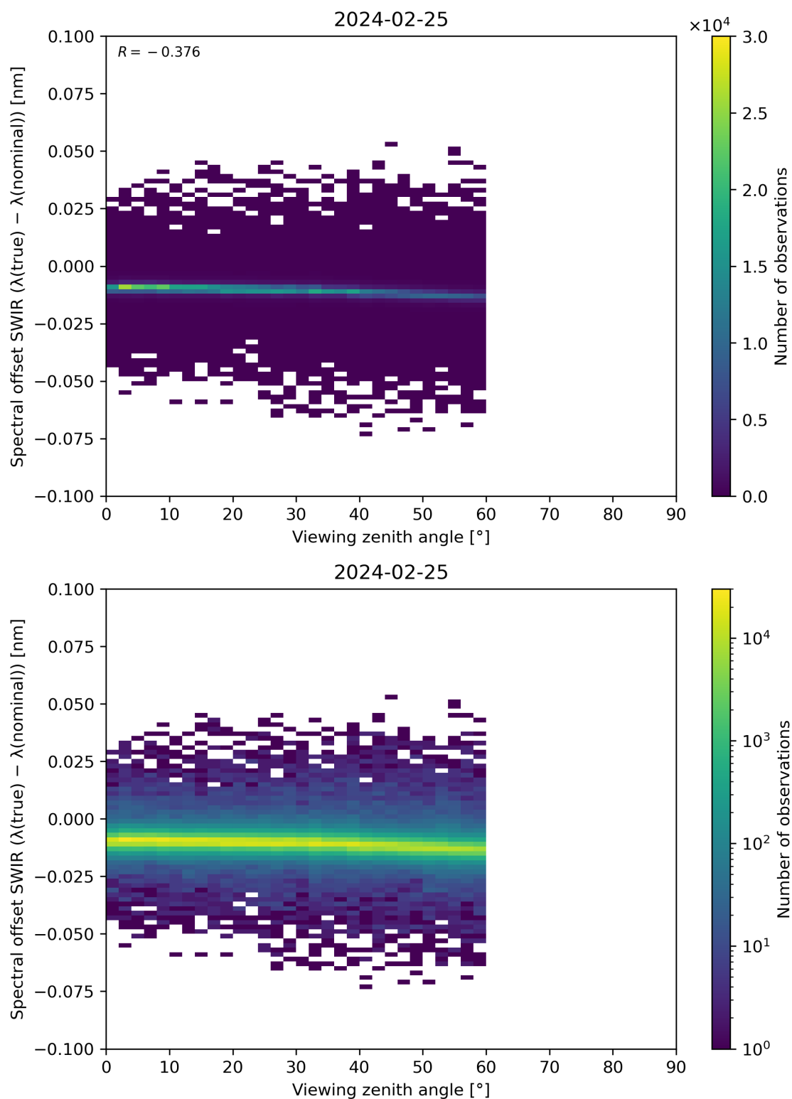
Figure 116: Scatter density plot of “Viewing zenith angle” against “Spectral offset SWIR ( \lambda(\text{true}) - \lambda(\text{nominal}) )” for 2024-02-24 to 2024-02-26.
