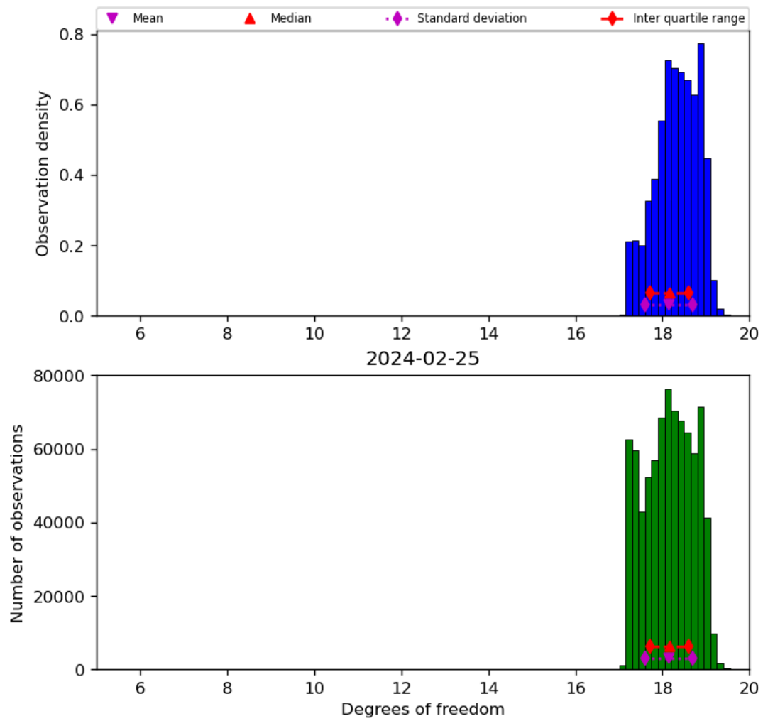
Figure 30: Histogram of “Degrees of freedom” for 2024-02-24 to 2024-02-26
