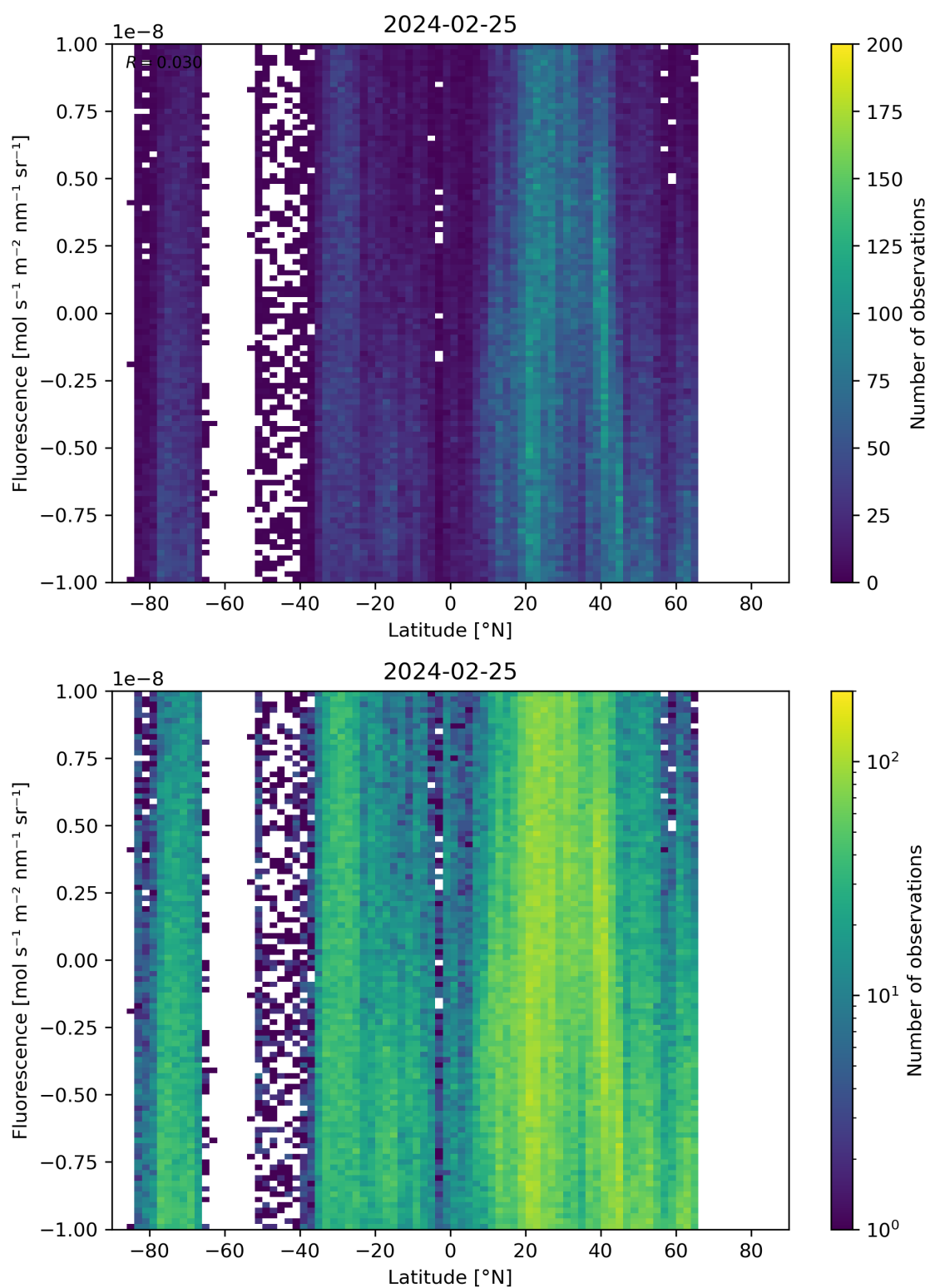
Figure 56: Scatter density plot of “Latitude” against “Fluorescence” for 2024-02-24 to 2024-02-26.
