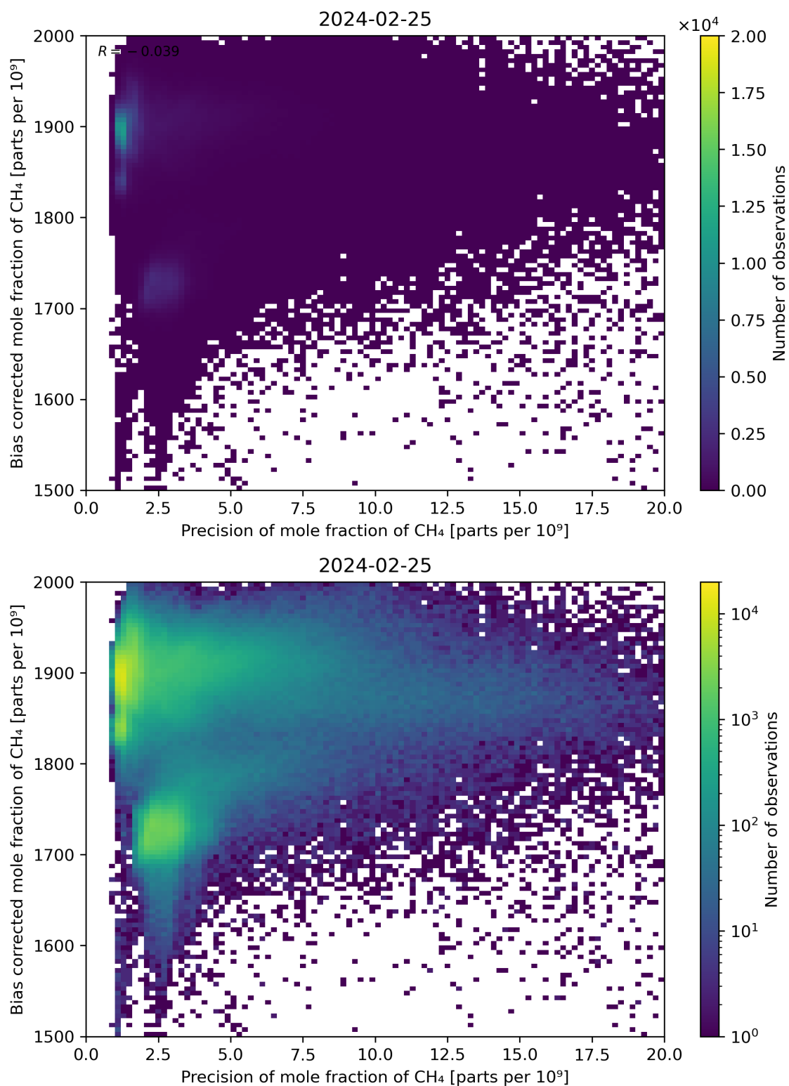
Figure 82: Scatter density plot of “Precision of mole fraction of CH 4 ” against “Bias corrected mole fraction of CH 4 ” for 2024-02-24 to 2024-02-26.
