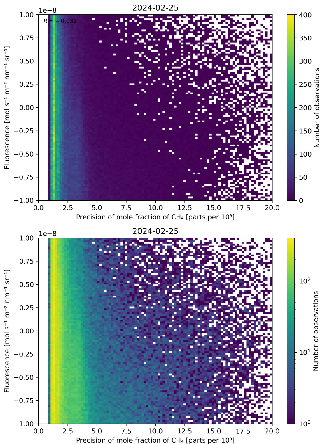
Figure 81: Scatter density plot of “Precision of mole fraction of CH 4 ” against “Fluorescence” for 2024-02-24 to 2024-02-26.
