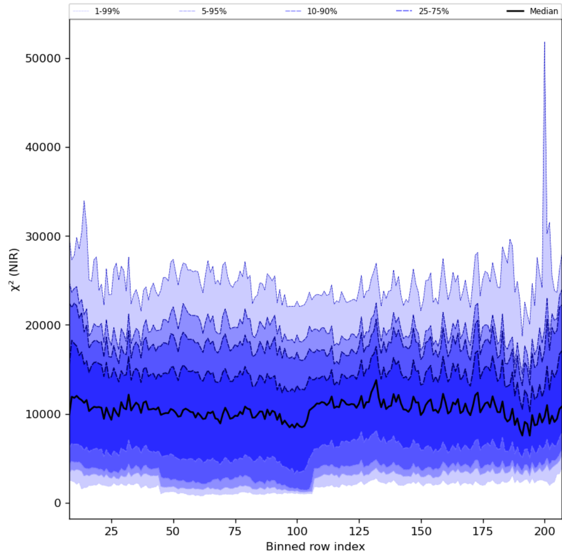
Figure 40: Along track statistics of “ \chi^2 (NIR)” for 2024-02-24 to 2024-02-26
