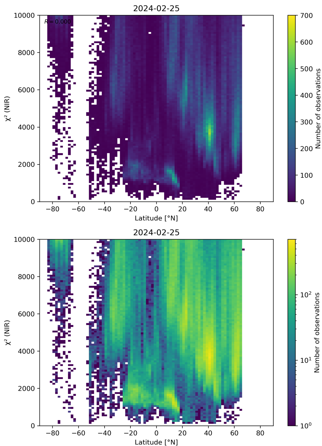
Figure 53: Scatter density plot of “Latitude” against “ \chi^2 (NIR)” for 2024-02-24 to 2024-02-26.
