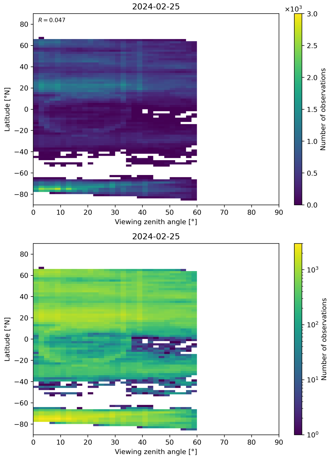
Figure 109: Scatter density plot of “Viewing zenith angle” against “Latitude” for 2024-02-24 to 2024-02-26.
