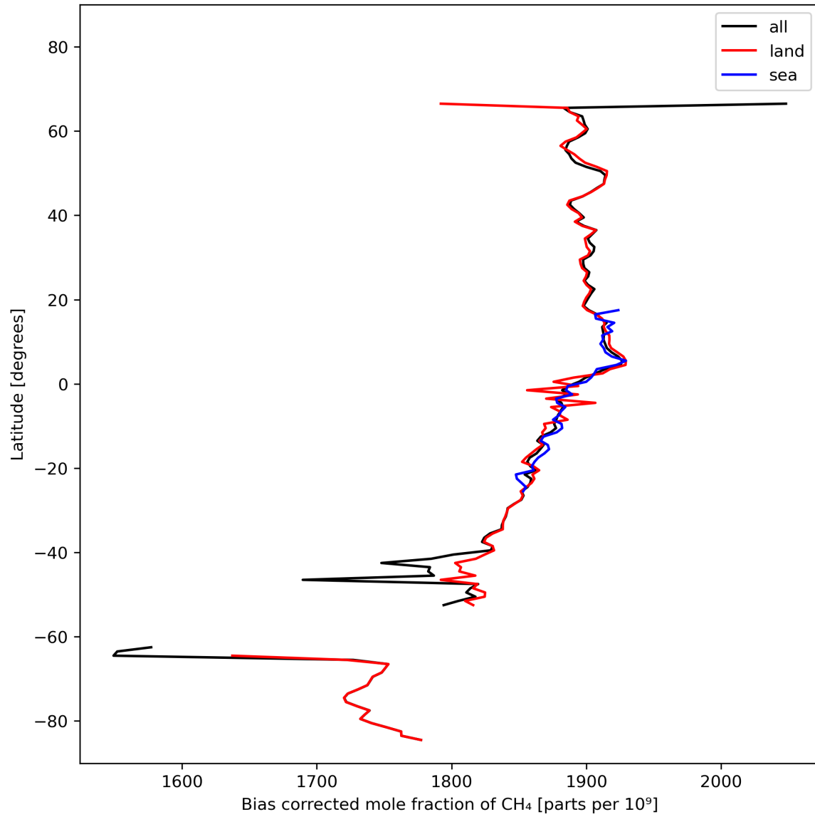
Figure 14: Zonal average of “Bias corrected mole fraction of CH 4 ” for 2024-02-24 to 2024-02-26.
