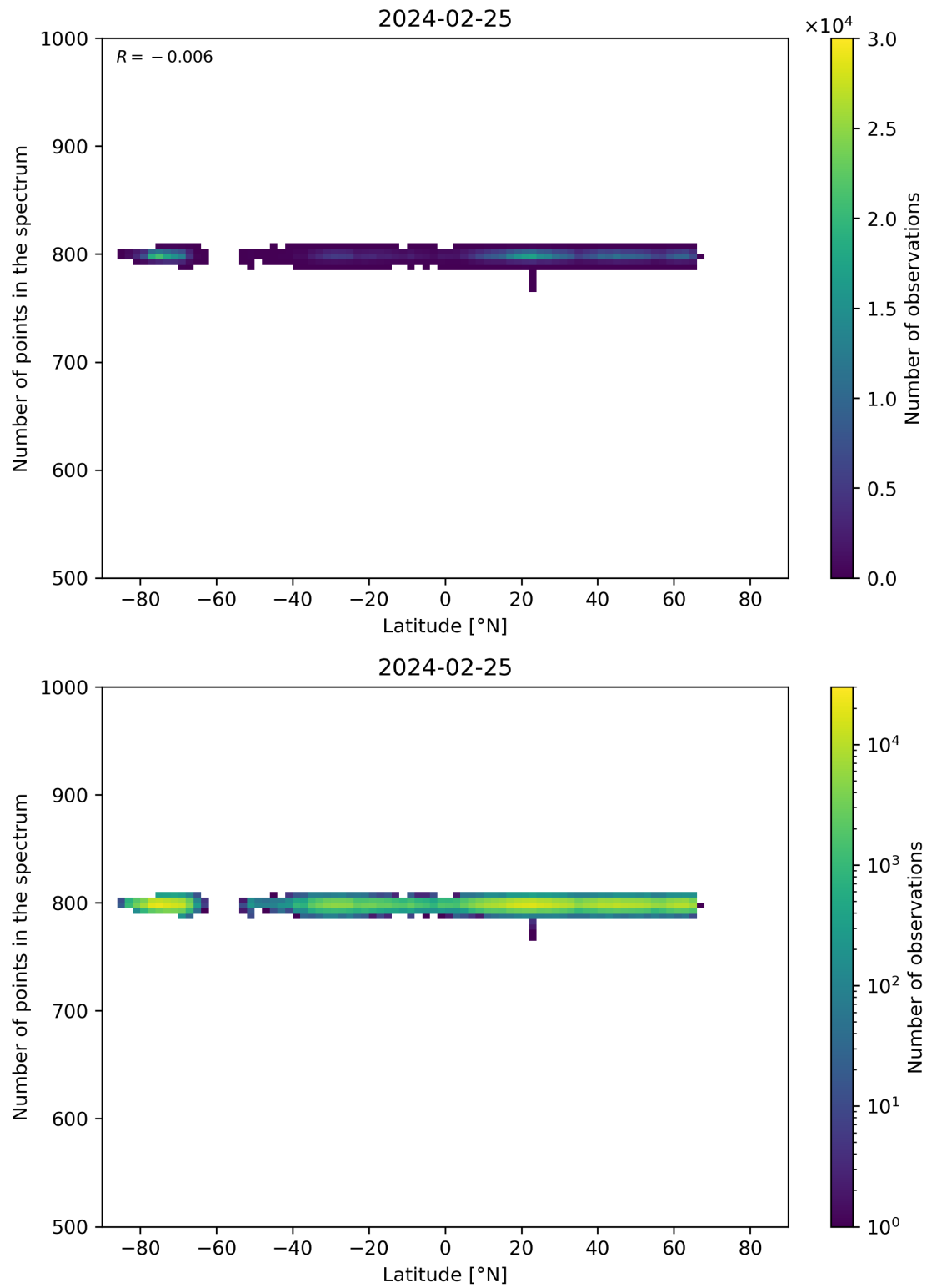
Figure 61: Scatter density plot of “Latitude” against “Number of points in the spectrum” for 2024-02-24 to 2024-02-26.
