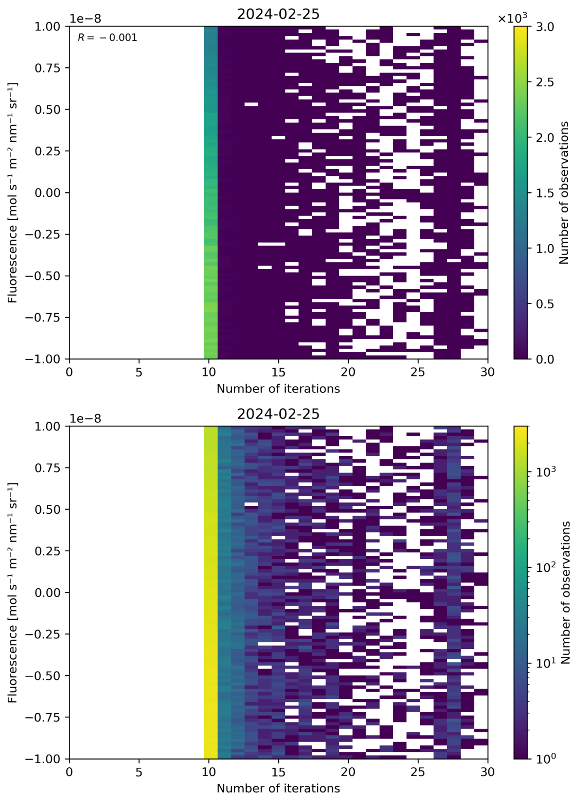
Figure 87: Scatter density plot of “Number of iterations” against “Fluorescence” for 2024-02-24 to 2024-02-26.
