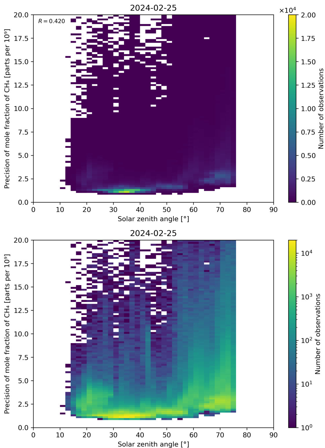
Figure 101: Scatter density plot of “Solar zenith angle” against “Precision of mole fraction of CH 4 ” for 2024-02-24 to 2024-02-26.
