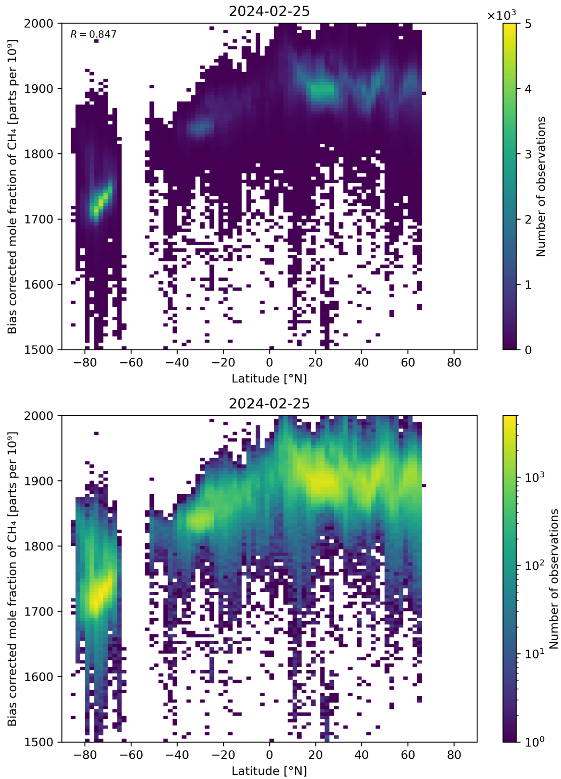
Figure 58: Scatter density plot of “Latitude” against “Bias corrected mole fraction of \text{CH}_4 ” for 2024-02-24 to 2024-02-26.
