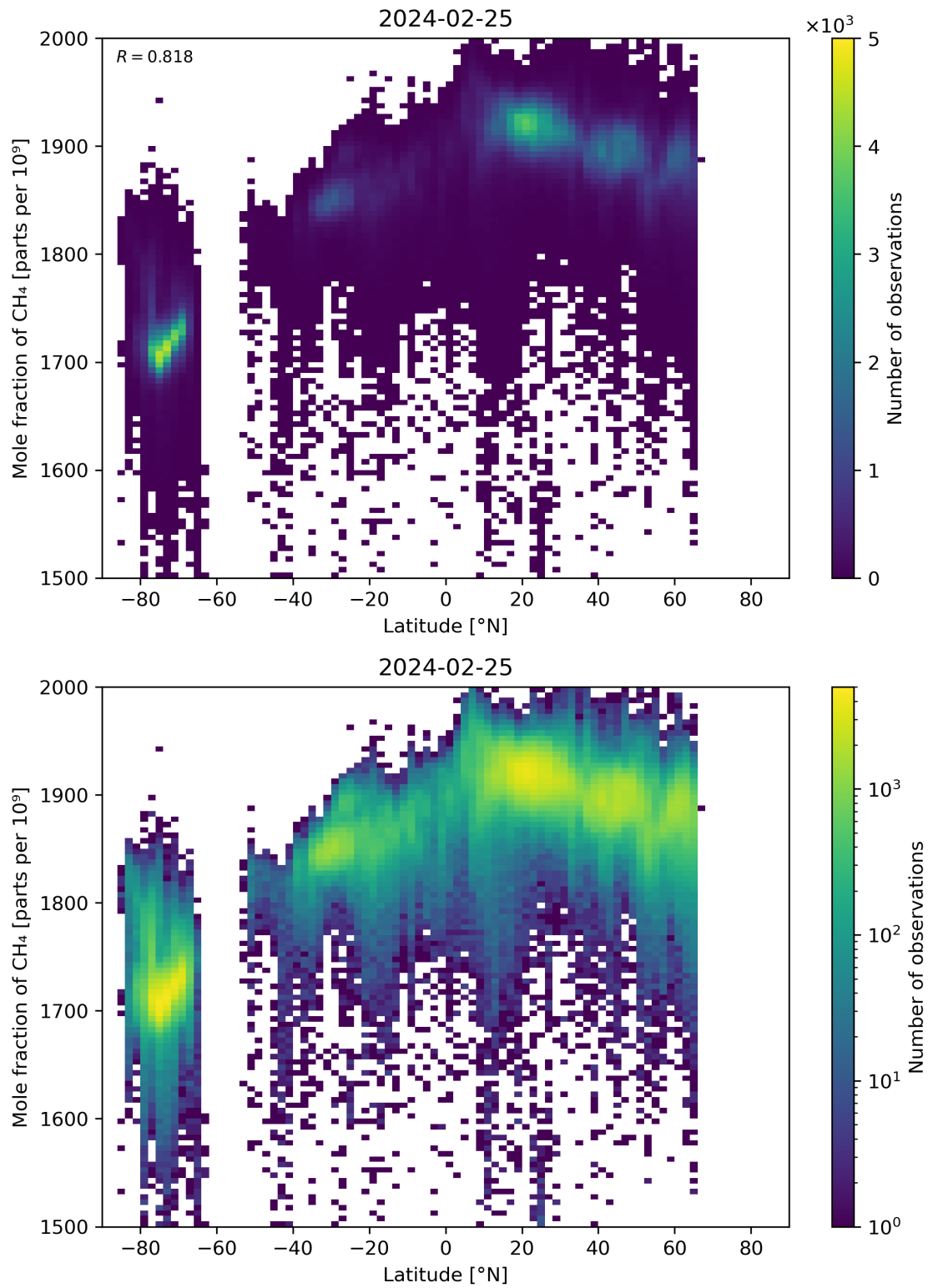
Figure 57: Scatter density plot of “Latitude” against “Mole fraction of CH 4 ” for 2024-02-24 to 2024-02-26.
