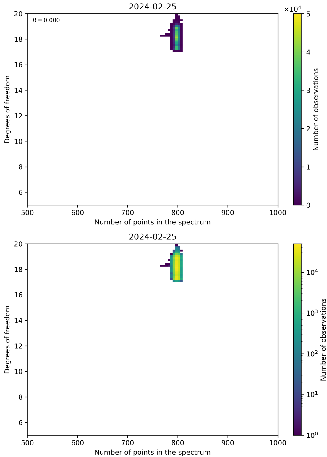
Figure 90: Scatter density plot of “Number of points in the spectrum” against “Degrees of freedom” for 2024-02-24 to 2024-02-26.
