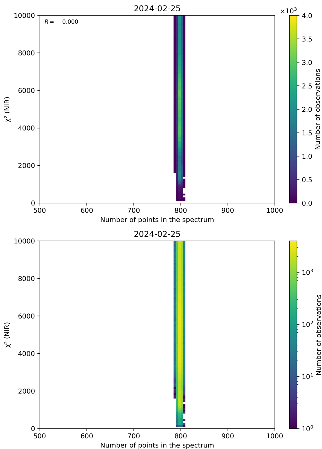
Figure 88: Scatter density plot of “Number of points in the spectrum” against “ \chi^2 (NIR)” for 2024-02-24 to 2024-02-26.
