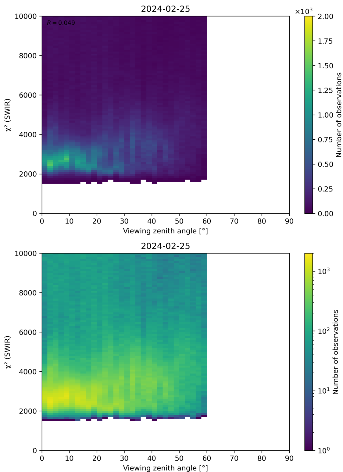
Figure 106: Scatter density plot of “Viewing zenith angle” against “ \chi^2 (SWIR)” for 2024-02-24 to 2024-02-26.
