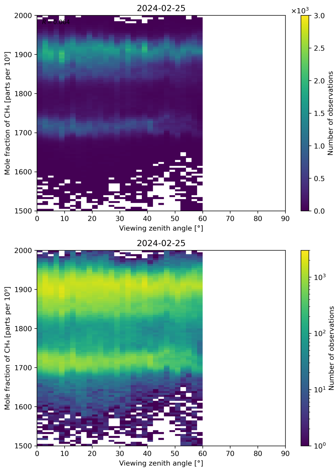
Figure 110: Scatter density plot of “Viewing zenith angle” against “Mole fraction of CH 4 ” for 2024-02-24 to 2024-02-26.
