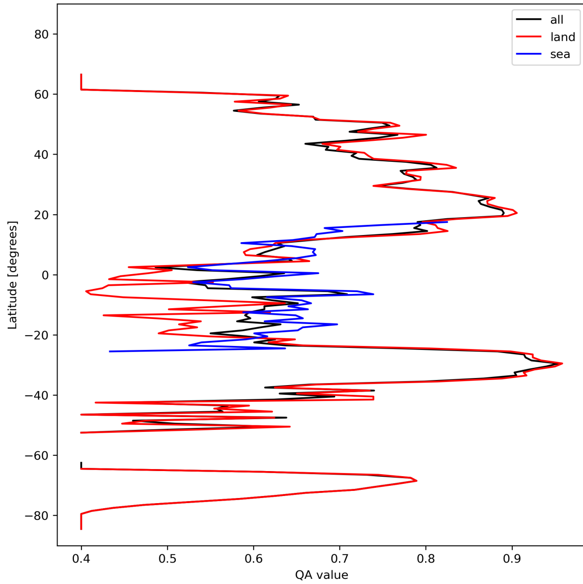
Figure 11: Zonal average of “QA value” for 2024-02-24 to 2024-02-26.
