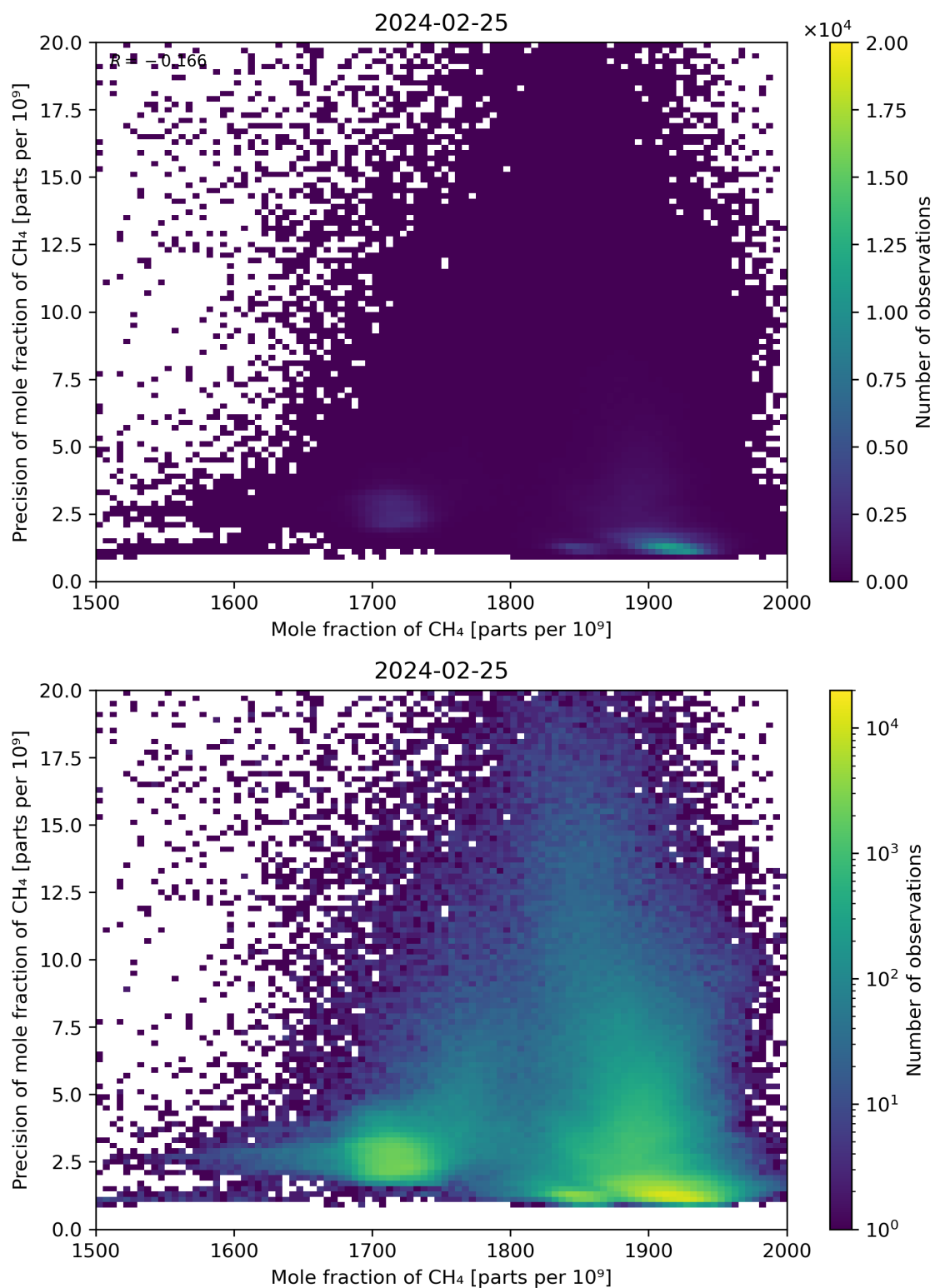
Figure 75: Scatter density plot of “Mole fraction of CH 4 ” against “Precision of mole fraction of CH 4 ” for 2024-02-24 to 2024-02-26.
