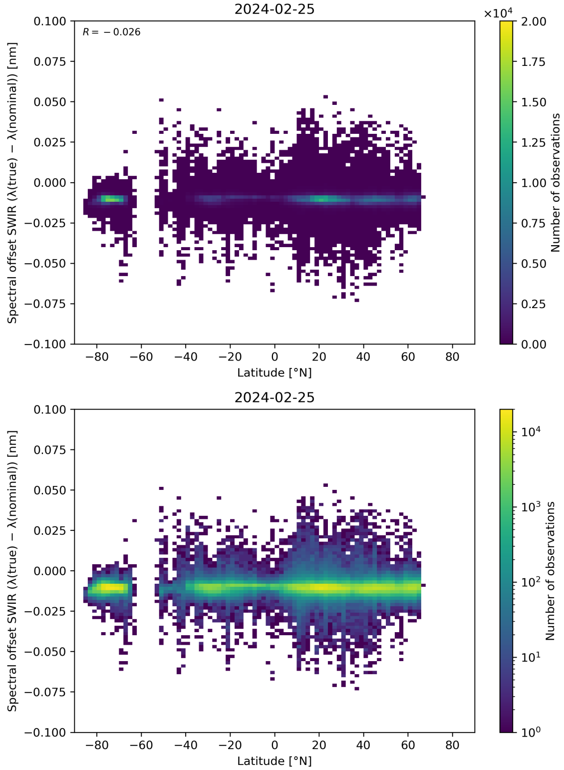
Figure 62: Scatter density plot of “Latitude” against “Spectral offset SWIR ( \lambda(\text{true}) - \lambda(\text{nominal}) )” for 2024-02-24 to 2024-02-26.
