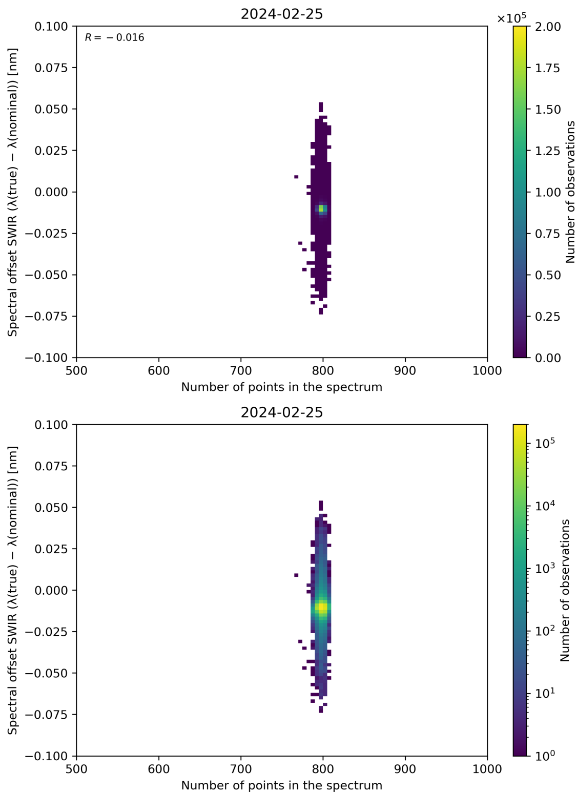
Figure 93: Scatter density plot of “Number of points in the spectrum” against “Spectral offset SWIR ( \lambda(\text{true}) - \lambda(\text{nominal}) )” for 2024-02-24 to 2024-02-26.
