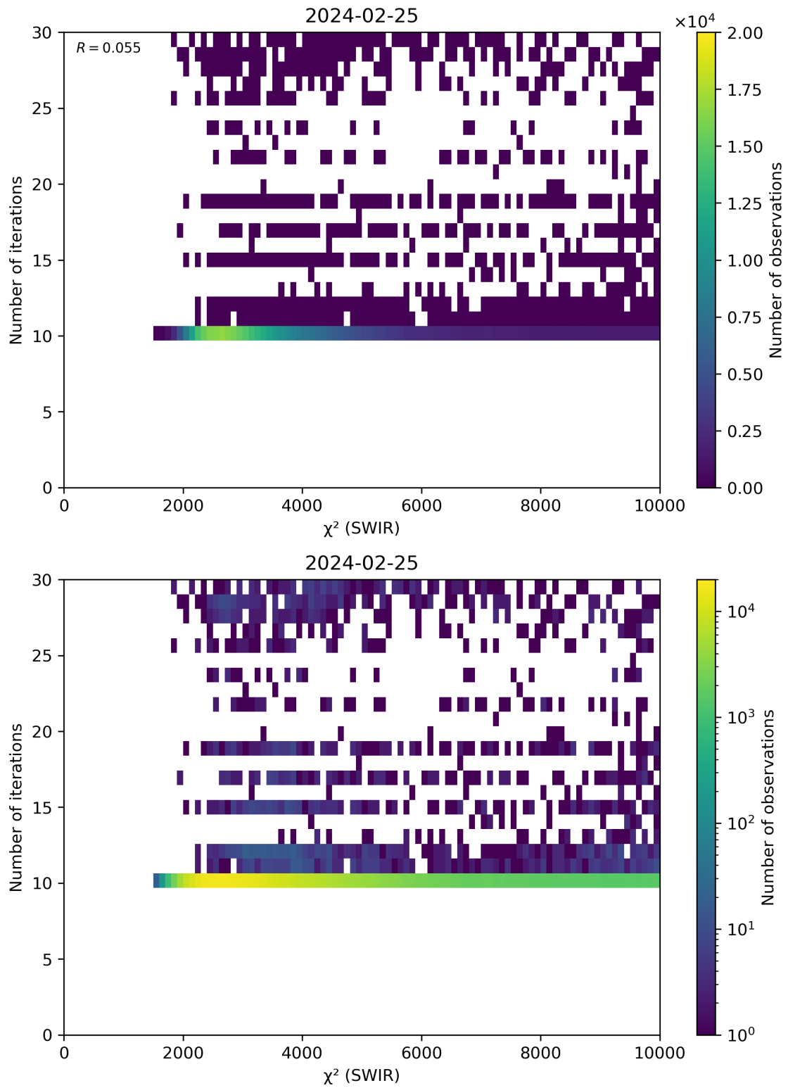
Figure 50: Scatter density plot of “ \chi^2 (SWIR)” against “Number of iterations” for 2024-02-24 to 2024-02-26.
