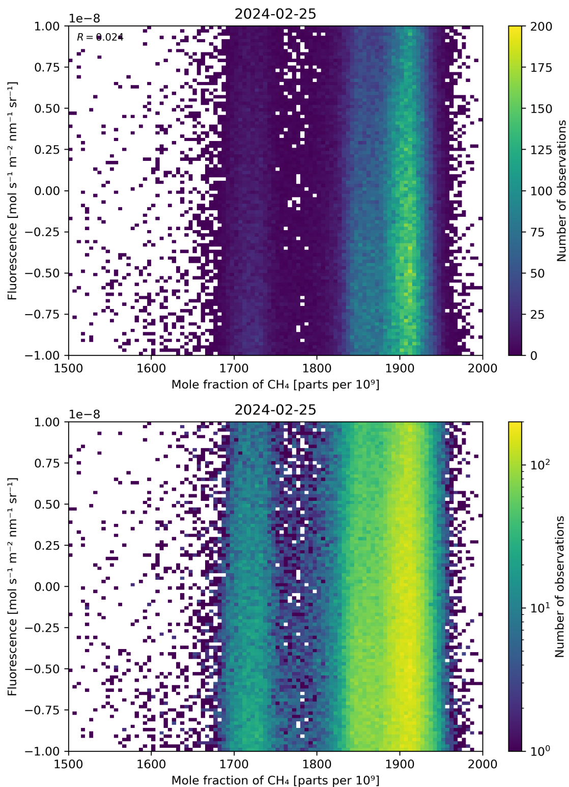
Figure 73: Scatter density plot of “Mole fraction of \text{CH}_4 ” against “Fluorescence” for 2024-02-24 to 2024-02-26.
