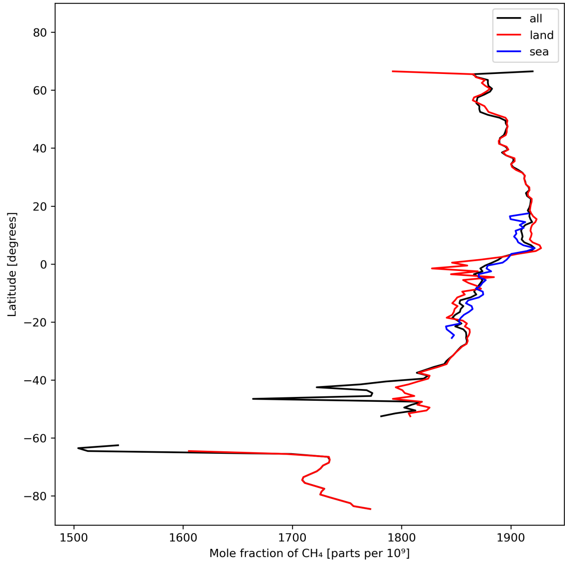
Figure 12: Zonal average of “Mole fraction of \text{CH}_4 ” for 2024-02-24 to 2024-02-26.
