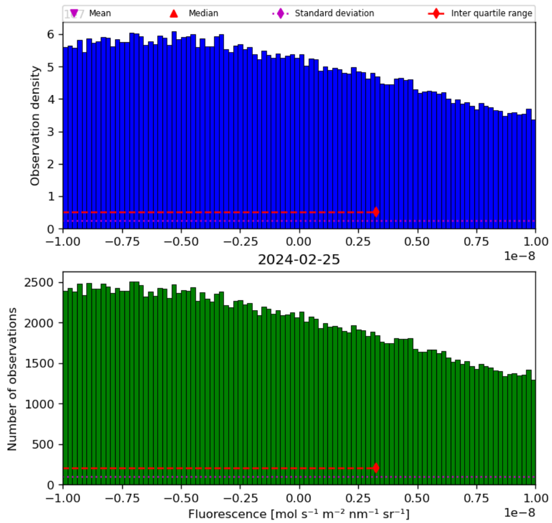
Figure 32: Histogram of “Fluorescence” for 2024-02-24 to 2024-02-26
