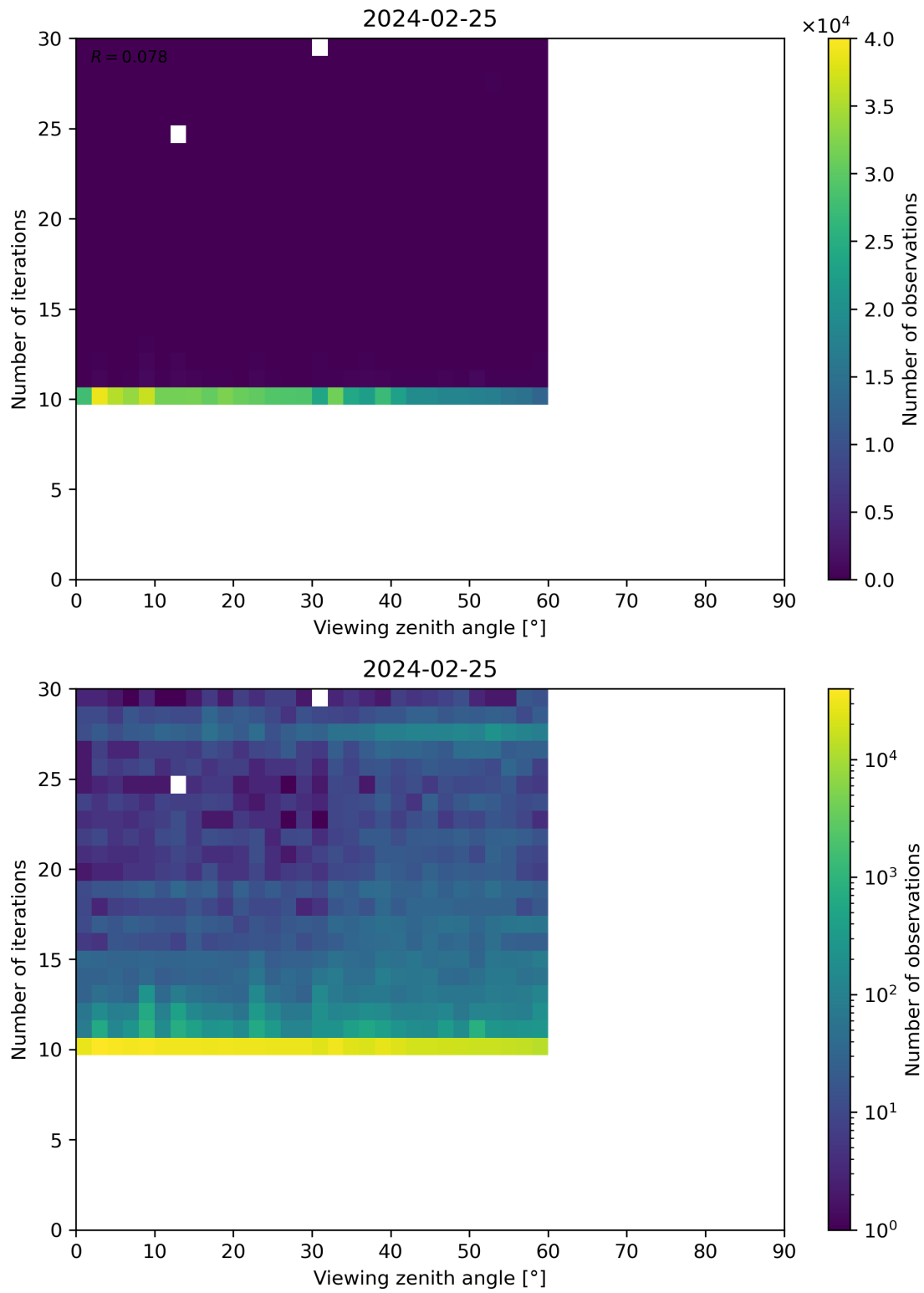
Figure 113: Scatter density plot of “Viewing zenith angle” against “Number of iterations” for 2024-02-24 to 2024-02-26.
