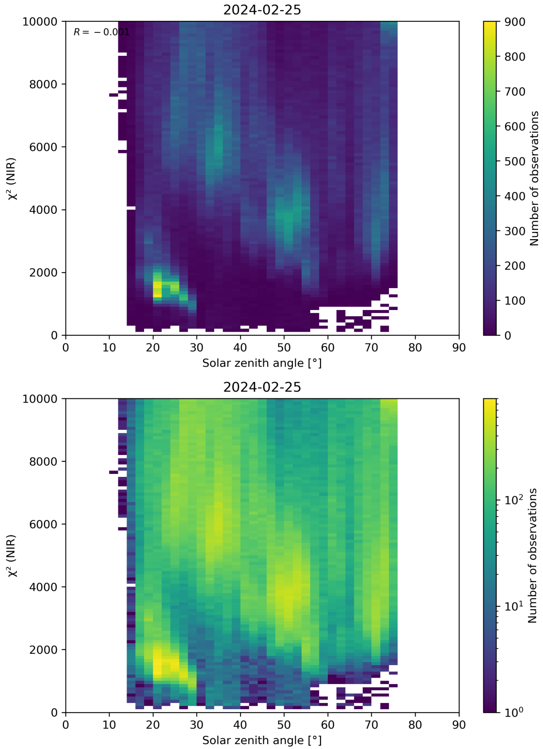
Figure 94: Scatter density plot of “Solar zenith angle” against “ \chi^2 (NIR)” for 2024-02-24 to 2024-02-26.
