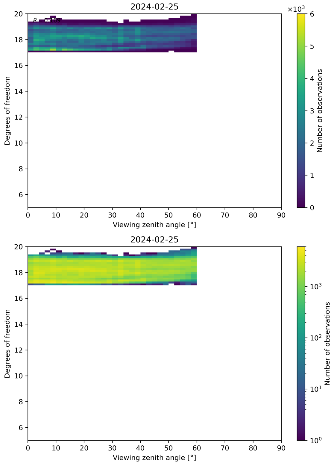
Figure 107: Scatter density plot of “Viewing zenith angle” against “Degrees of freedom” for 2024-02-24 to 2024-02-26.
