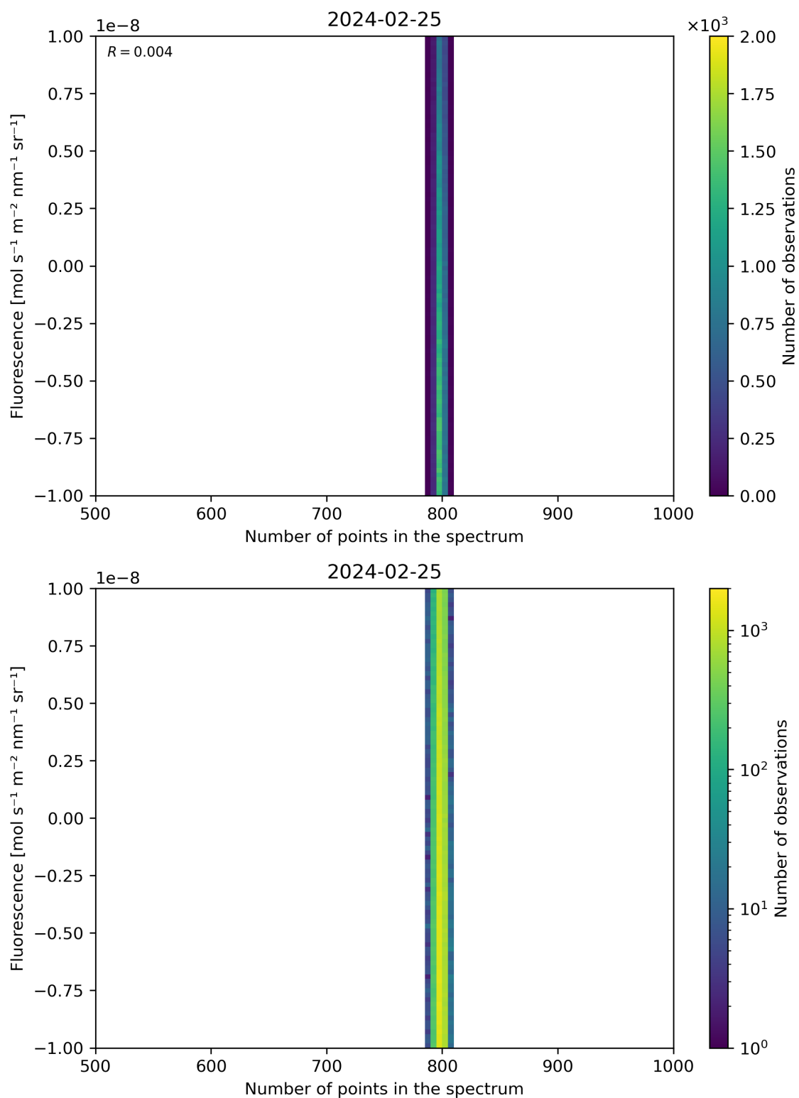
Figure 91: Scatter density plot of “Number of points in the spectrum” against “Fluorescence” for 2024-02-24 to 2024-02-26.
