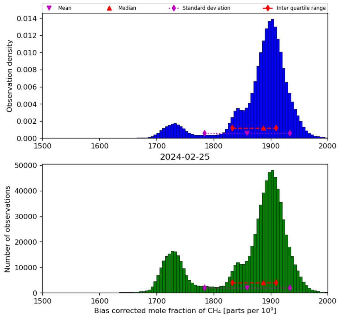
Figure 25: Histogram of “Bias corrected mole fraction of CH 4 ” for 2024-02-24 to 2024-02-26
