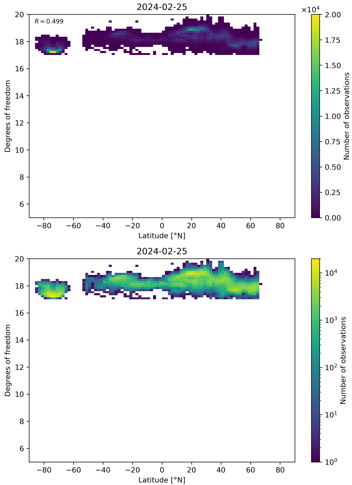
Figure 55: Scatter density plot of “Latitude” against “Degrees of freedom” for 2024-02-24 to 2024-02-26.
