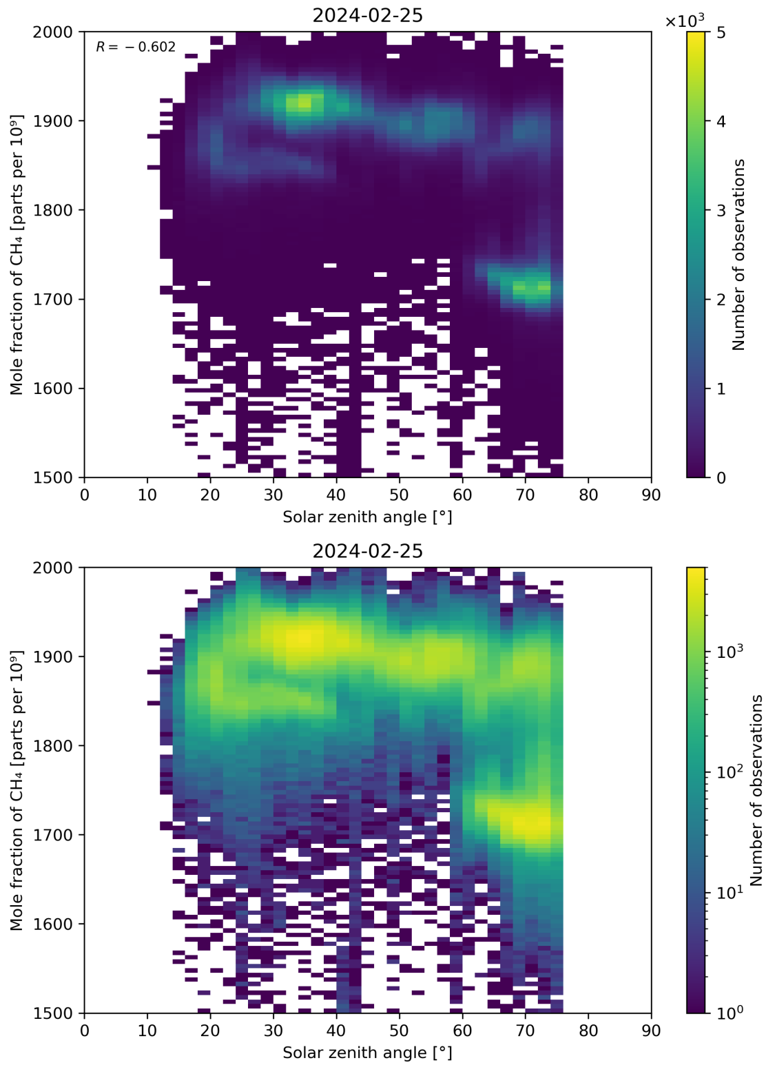
Figure 99: Scatter density plot of “Solar zenith angle” against “Mole fraction of CH 4 ” for 2024-02-24 to 2024-02-26.
