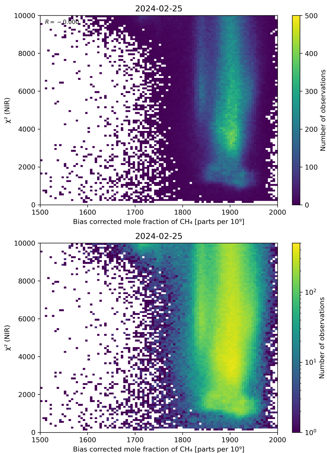
Figure 63: Scatter density plot of “Bias corrected mole fraction of CH 4 ” against “ \chi^2 (NIR)” for 2024-02-24 to 2024-02-26.
