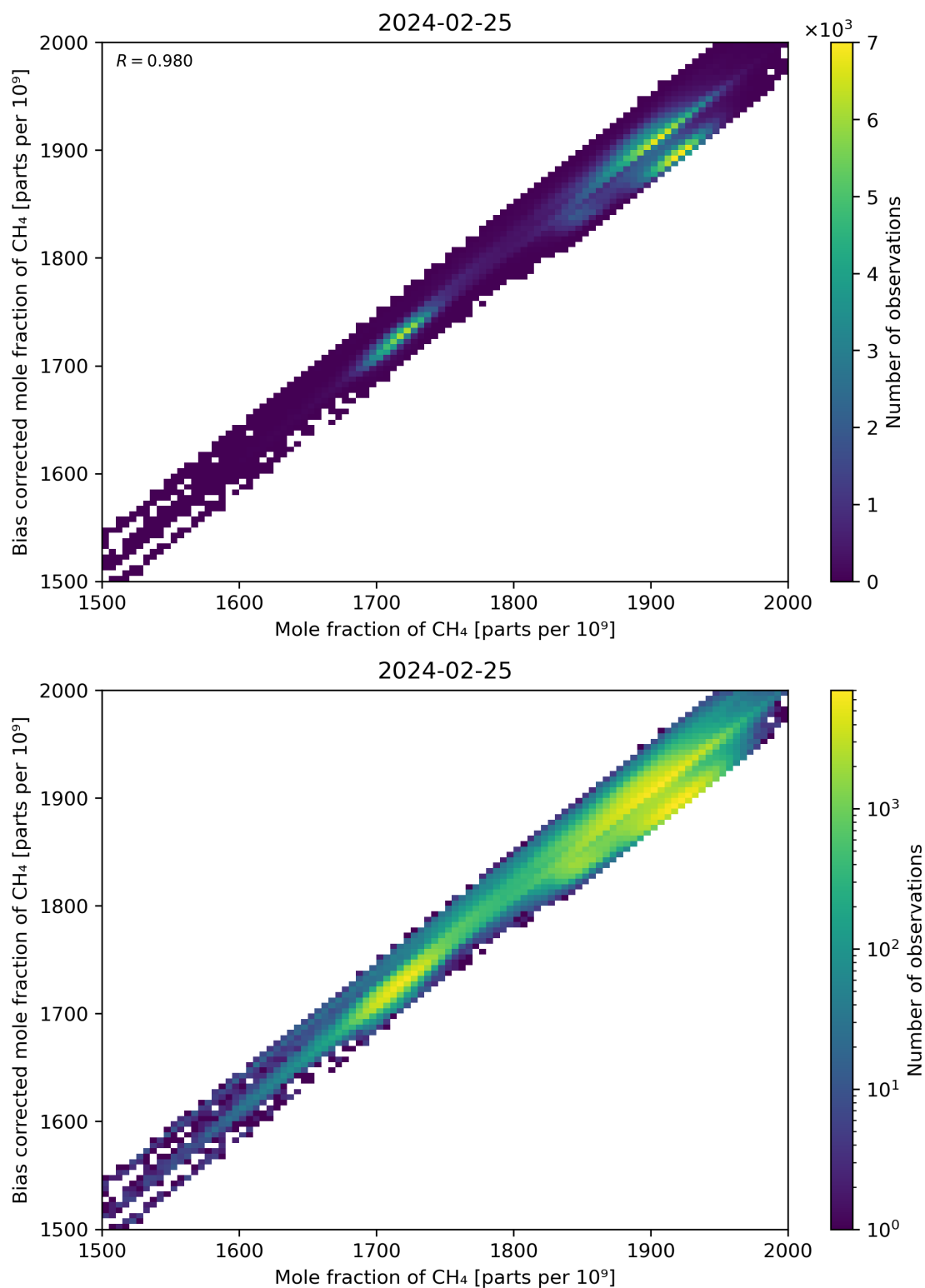
Figure 74: Scatter density plot of “Mole fraction of CH 4 ” against “Bias corrected mole fraction of CH 4 ” for 2024-02-24 to 2024-02-26.
