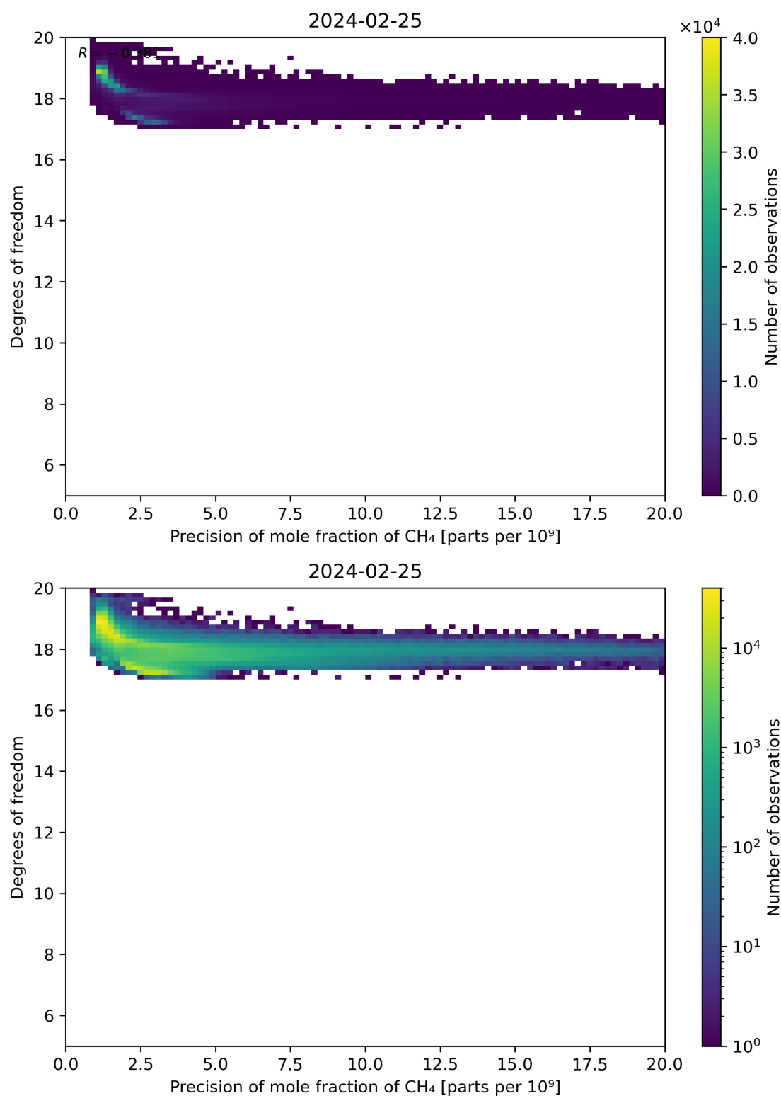
Figure 80: Scatter density plot of “Precision of mole fraction of CH 4 ” against “Degrees of freedom” for 2024-02-24 to 2024-02-26.
