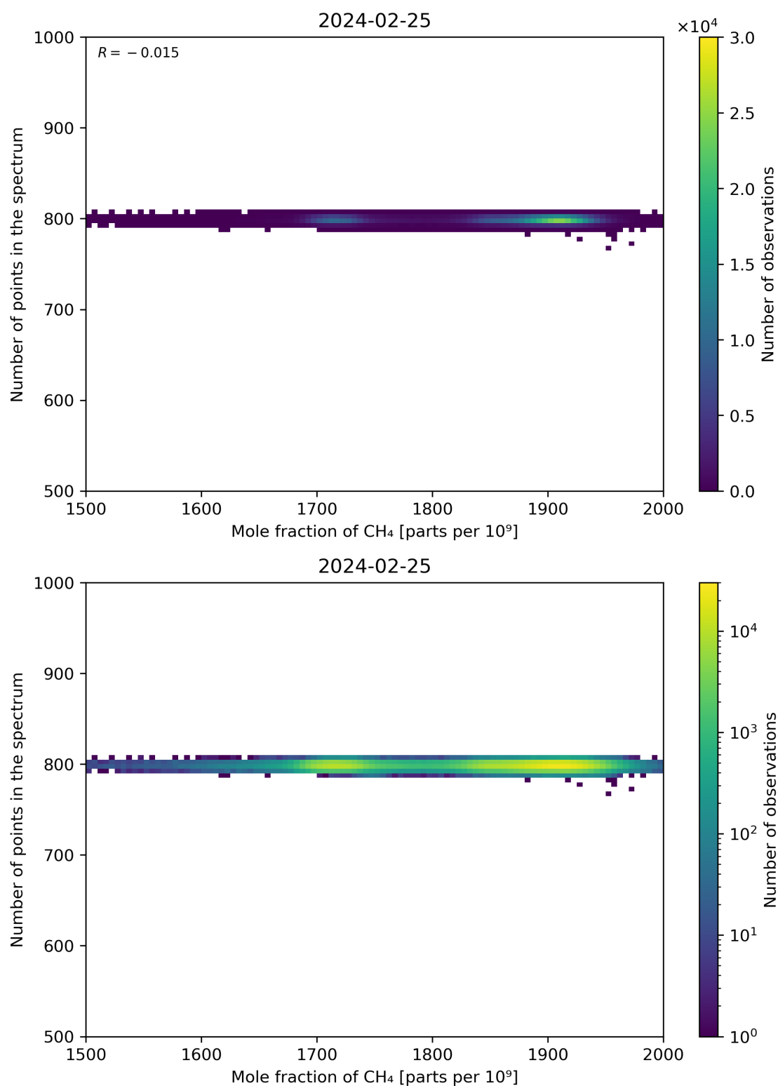
Figure 77: Scatter density plot of “Mole fraction of CH 4 ” against “Number of points in the spectrum” for 2024-02-24 to 2024-02-26.
