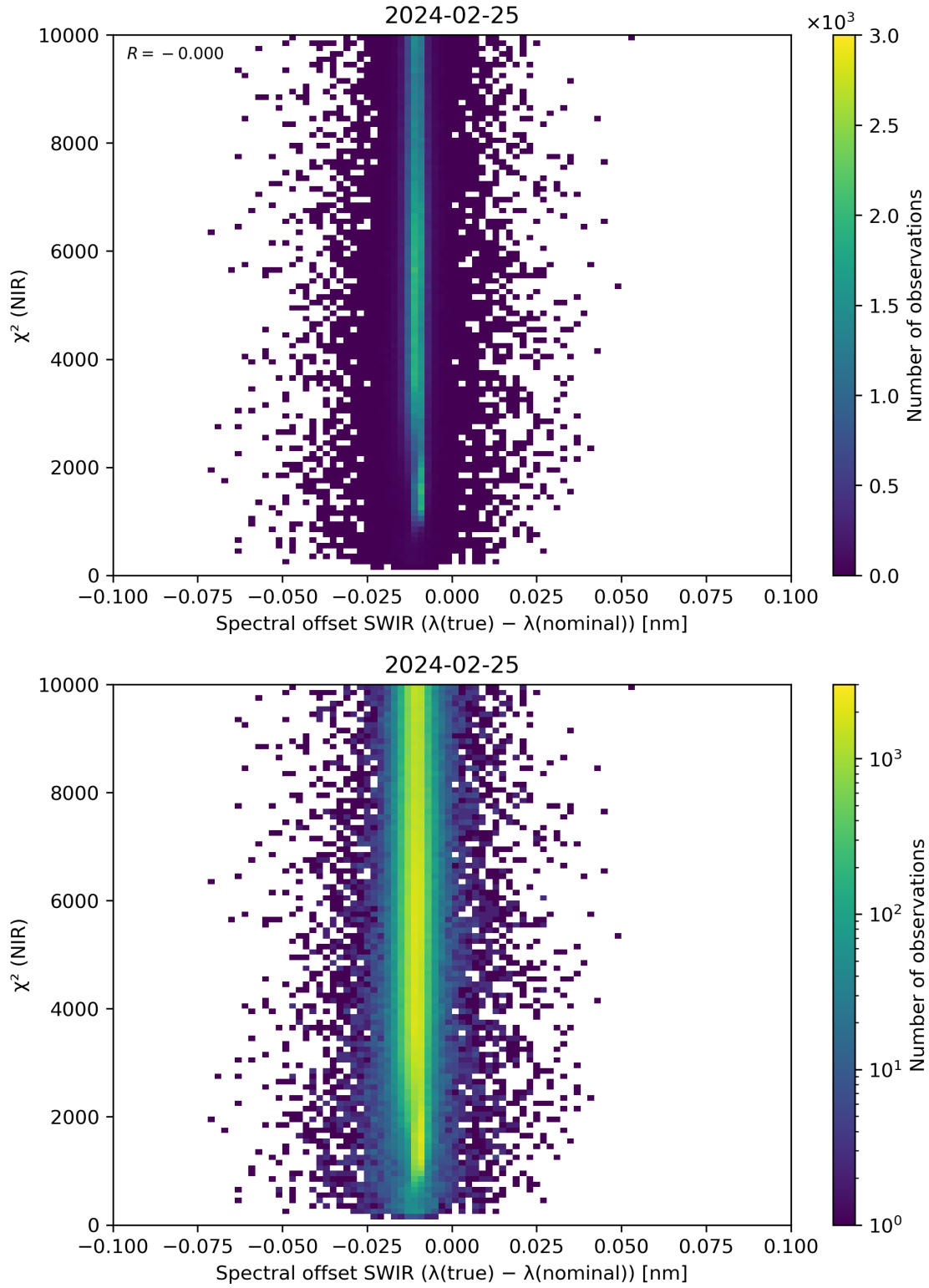
Figure 117: Scatter density plot of “Spectral offset SWIR ( \lambda(\text{true}) - \lambda(\text{nominal}) )” against “ \chi^2 (NIR)” for 2024-02-24 to 2024-02-26.
