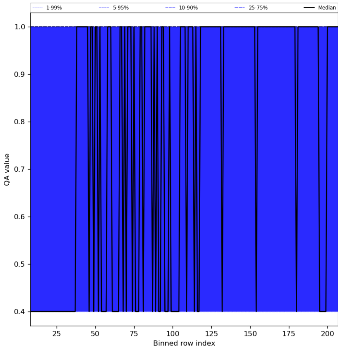
Figure 33: Along track statistics of “QA value” for 2024-02-24 to 2024-02-26
