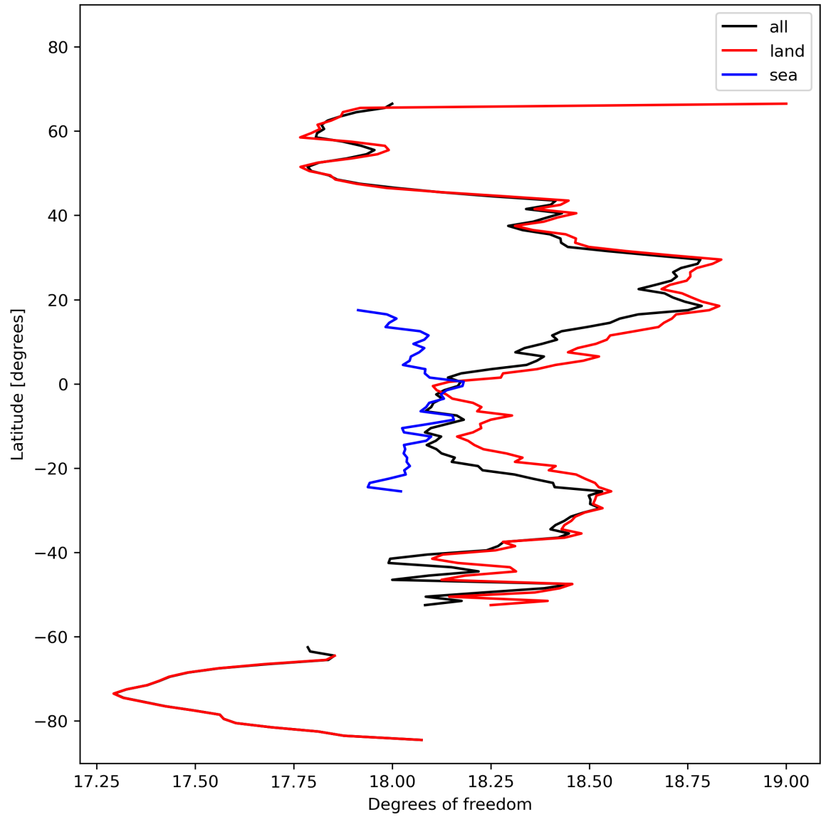
Figure 19: Zonal average of “Degrees of freedom” for 2024-02-24 to 2024-02-26.
