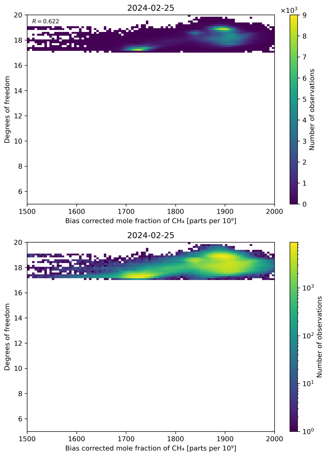
Figure 65: Scatter density plot of “Bias corrected mole fraction of CH 4 ” against “Degrees of freedom” for 2024-02-24 to 2024-02-26.
