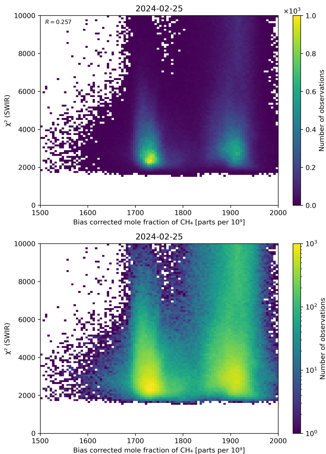
Figure 64: Scatter density plot of “Bias corrected mole fraction of CH 4 ” against “ \chi^2 (SWIR)” for 2024-02-24 to 2024-02-26.
