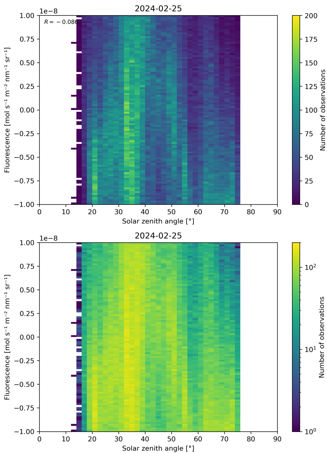
Figure 97: Scatter density plot of “Solar zenith angle” against “Fluorescence” for 2024-02-24 to 2024-02-26.
