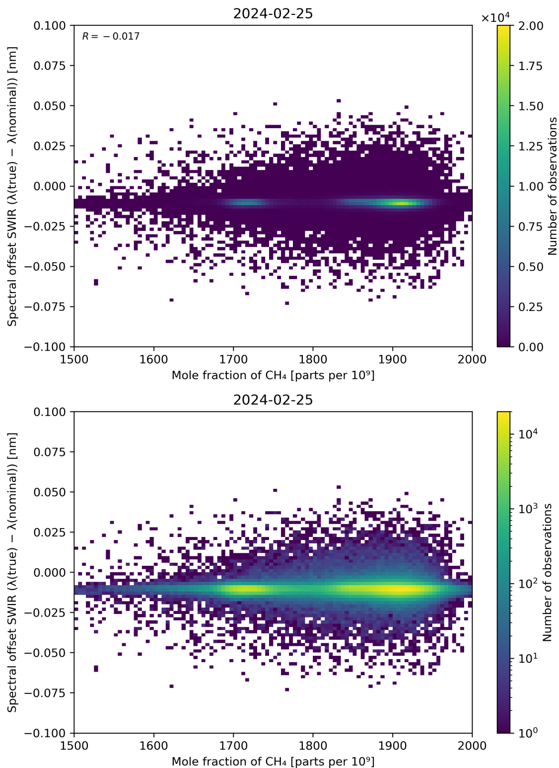
Figure 86: Scatter density plot of “Mole fraction of CH 4 ” against “Spectral offset SWIR ( \lambda(\text{true}) - \lambda(\text{nominal}) )” for 2024-02-24 to 2024-02-26.
