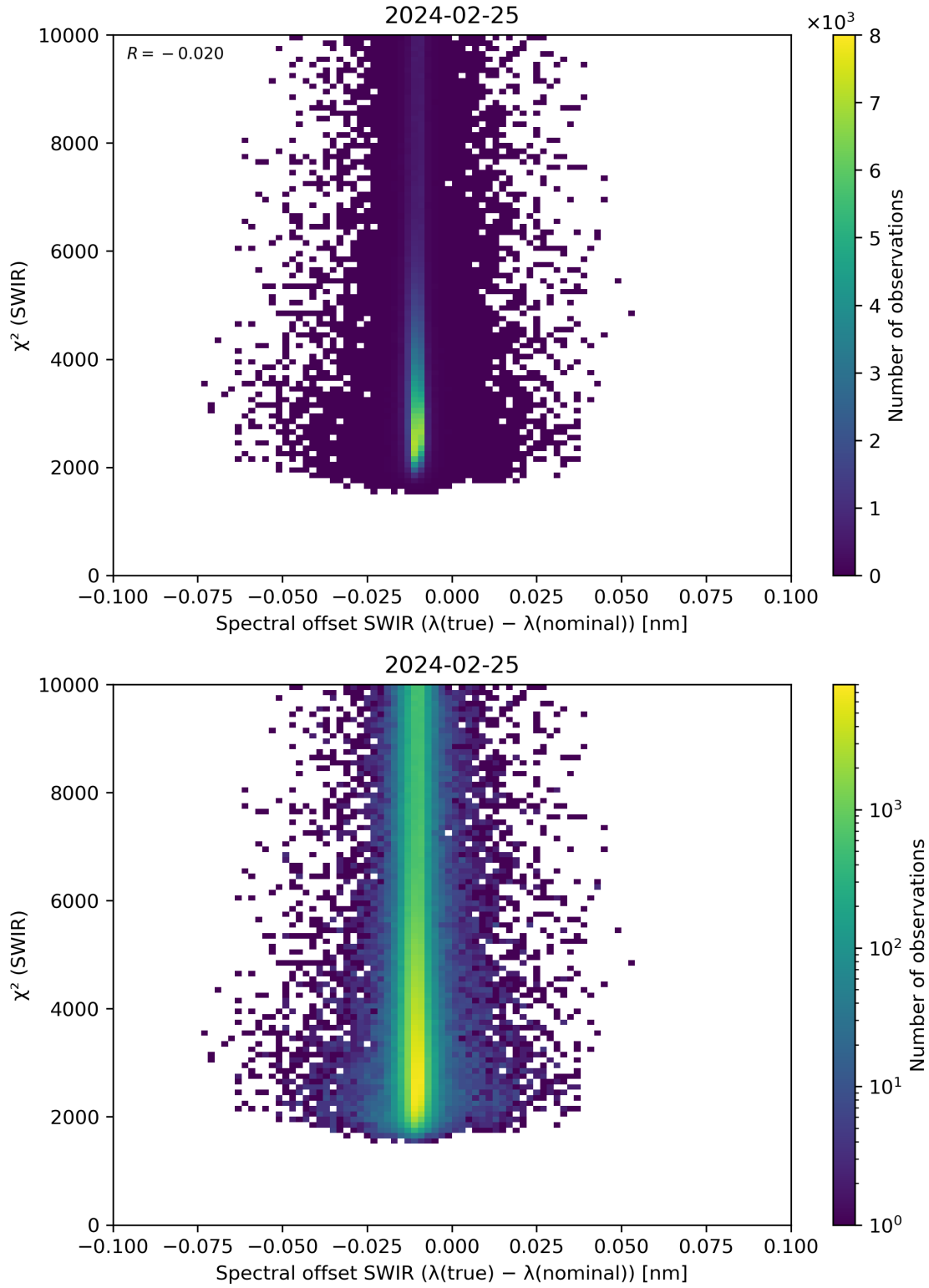
Figure 118: Scatter density plot of “Spectral offset SWIR ( \lambda(\text{true}) - \lambda(\text{nominal}) )” against “ \chi^2 (SWIR)” for 2024-02-24 to 2024-02-26.
