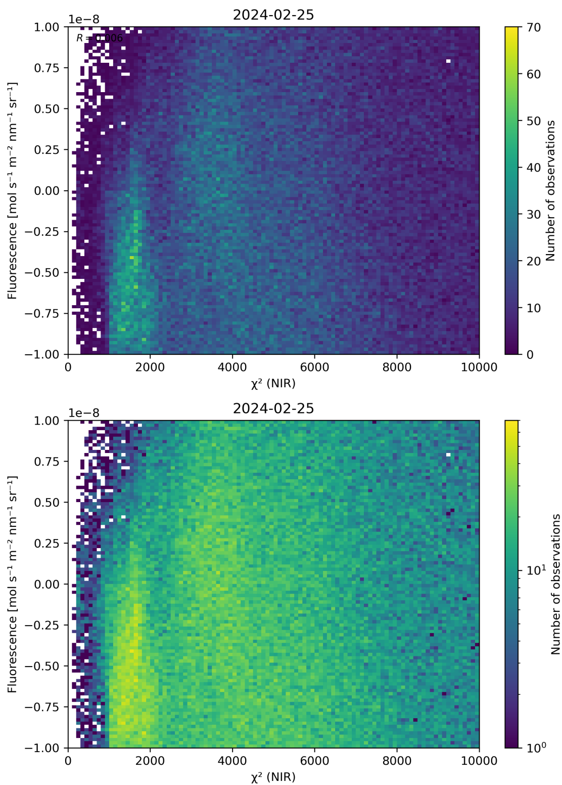
Figure 45: Scatter density plot of “ \chi^2 (NIR)” against “Fluorescence” for 2024-02-24 to 2024-02-26.
