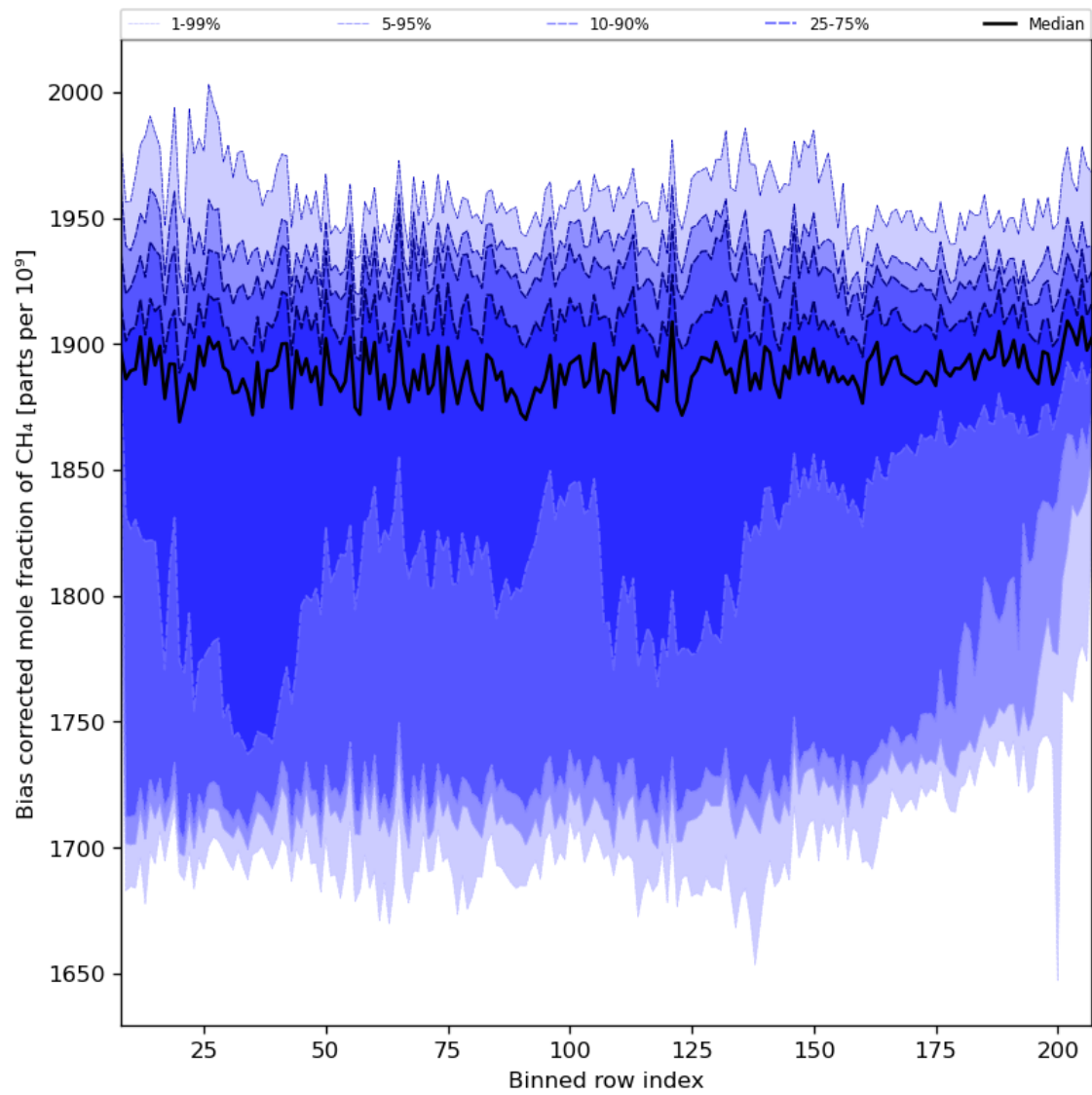
Figure 36: Along track statistics of “Bias corrected mole fraction of CH 4 ” for 2024-02-24 to 2024-02-26
