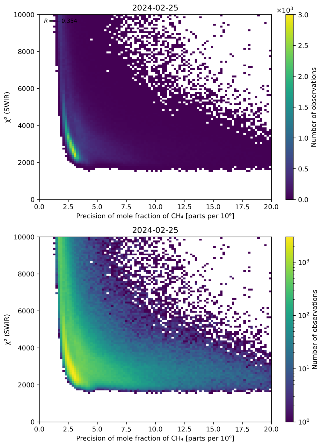
Figure 79: Scatter density plot of “Precision of mole fraction of CH 4 ” against “ \chi^2 (SWIR)” for 2024-02-24 to 2024-02-26.
