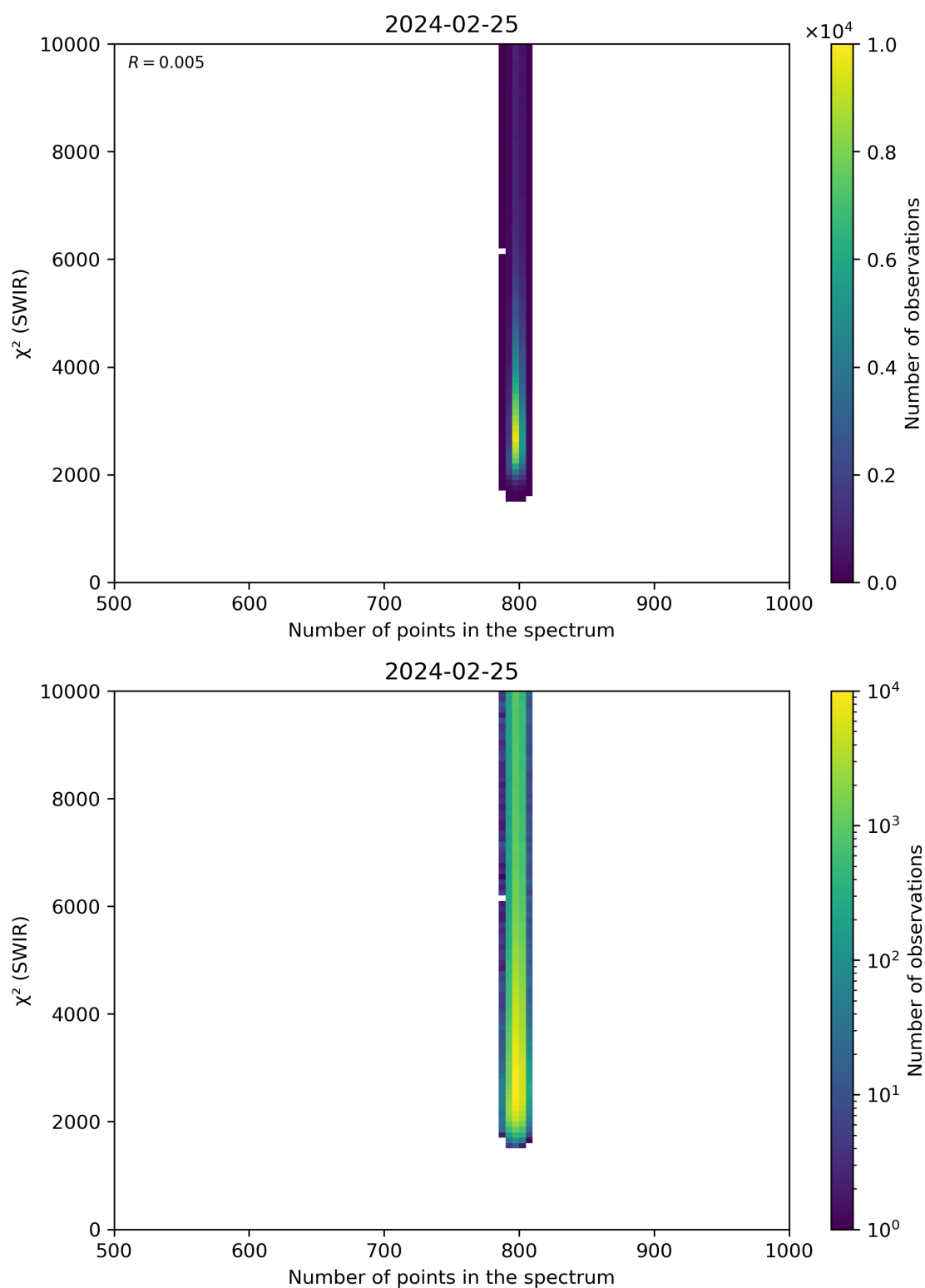
Figure 89: Scatter density plot of “Number of points in the spectrum” against “ \chi^2 (SWIR)” for 2024-02-24 to 2024-02-26.
