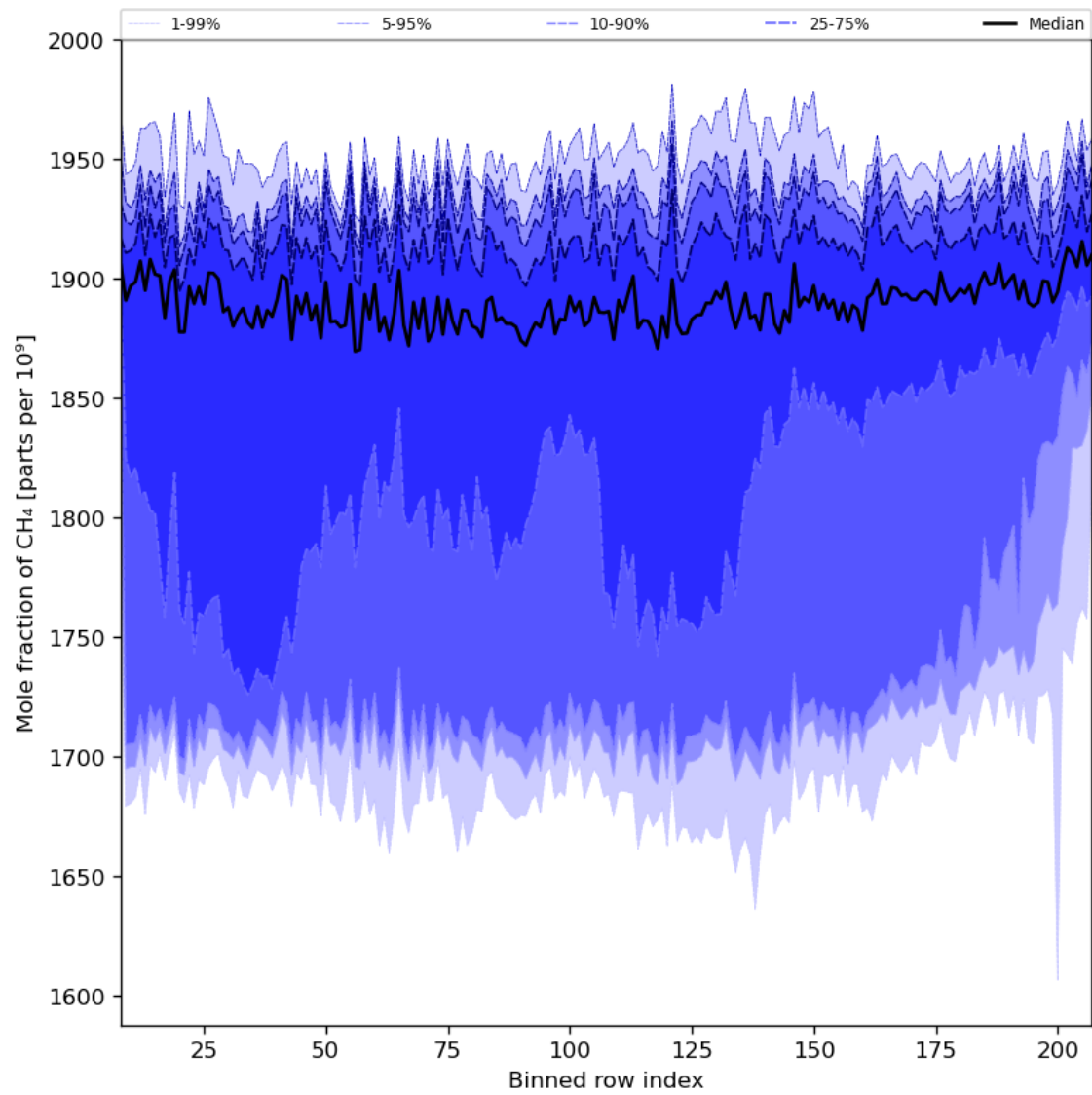
Figure 34: Along track statistics of “Mole fraction of CH 4 ” for 2024-02-24 to 2024-02-26
