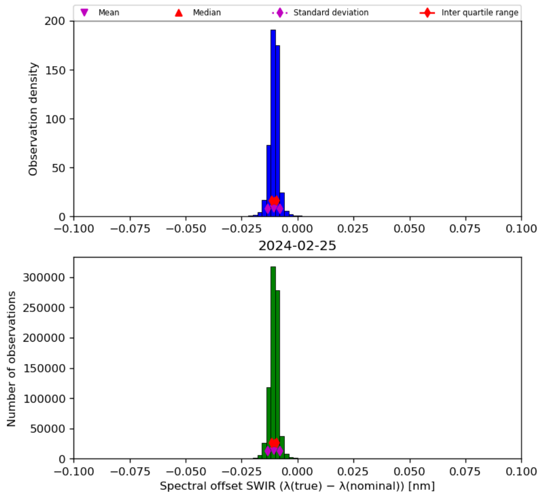
Figure 27: Histogram of “Spectral offset SWIR ( \lambda(\text{true}) - \lambda(\text{nominal}) )” for 2024-02-24 to 2024-02-26
