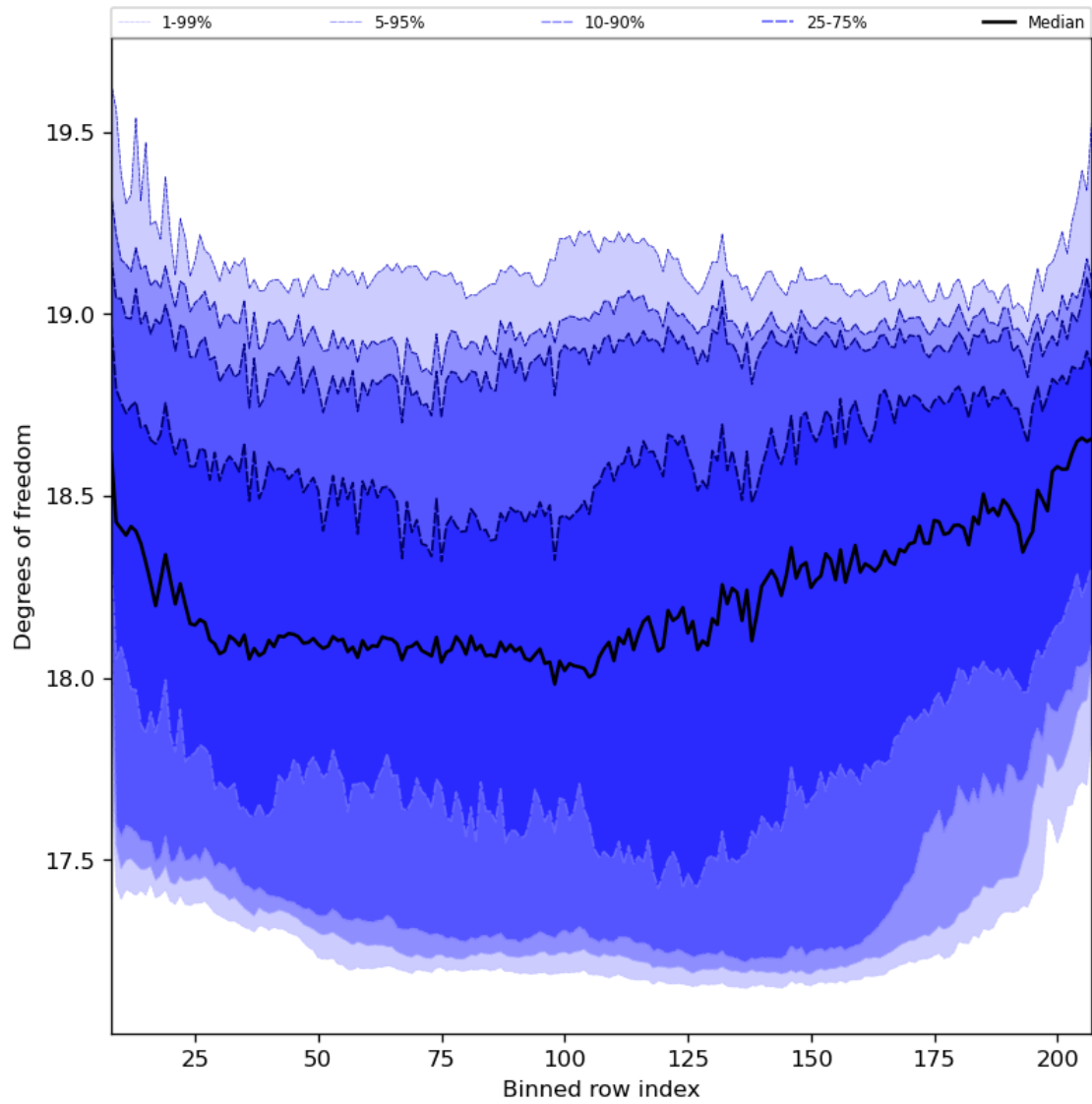
Figure 41: Along track statistics of “Degrees of freedom” for 2024-02-24 to 2024-02-26
