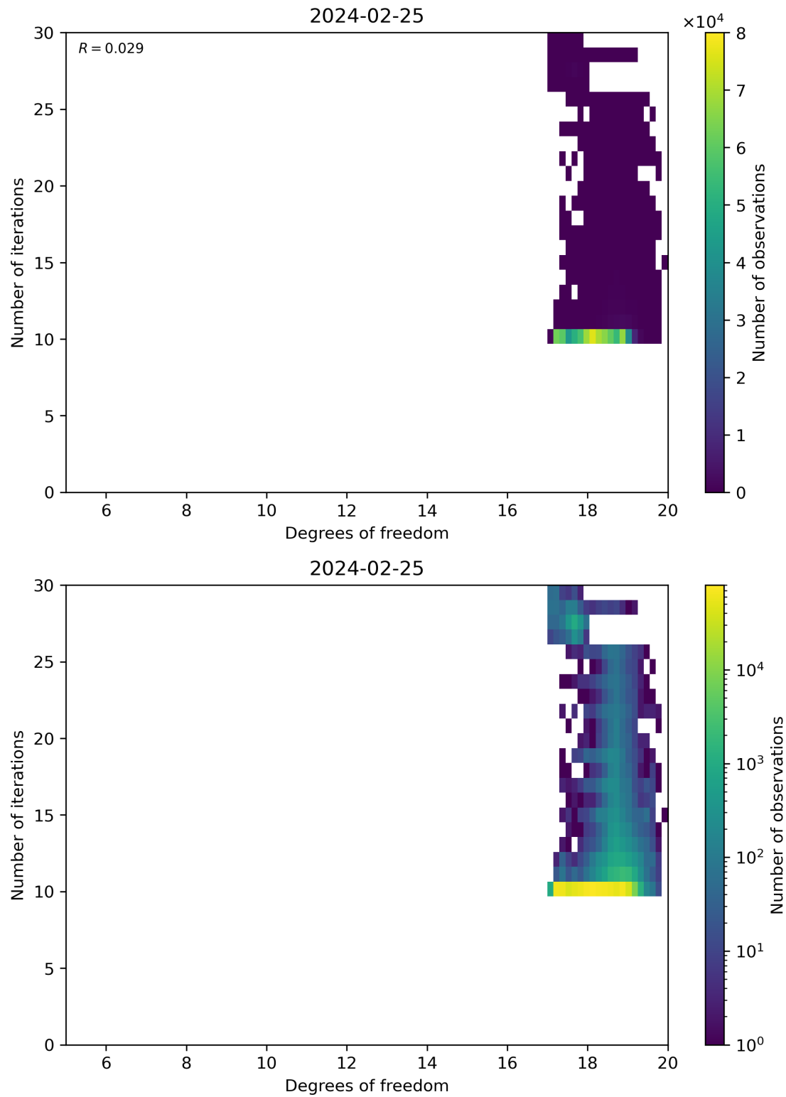
Figure 52: Scatter density plot of “Degrees of freedom” against “Number of iterations” for 2024-02-24 to 2024-02-26.
