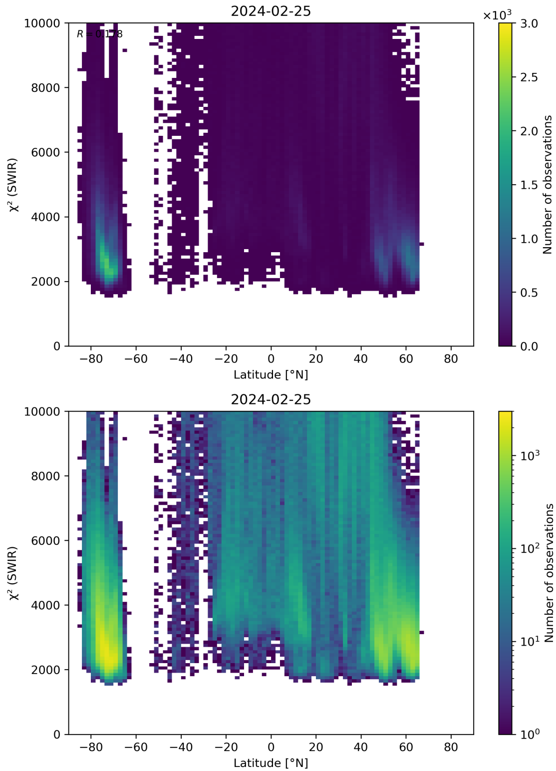
Figure 54: Scatter density plot of “Latitude” against “ \chi^2 (SWIR)” for 2024-02-24 to 2024-02-26.
