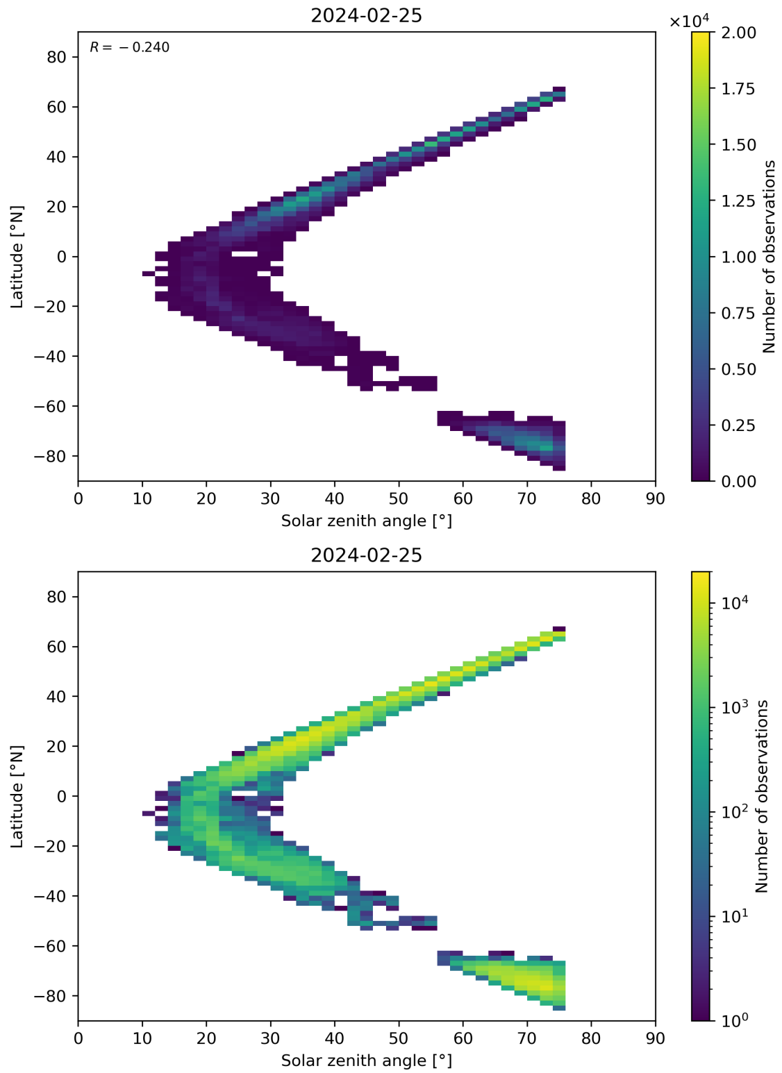
Figure 98: Scatter density plot of “Solar zenith angle” against “Latitude” for 2024-02-24 to 2024-02-26.
