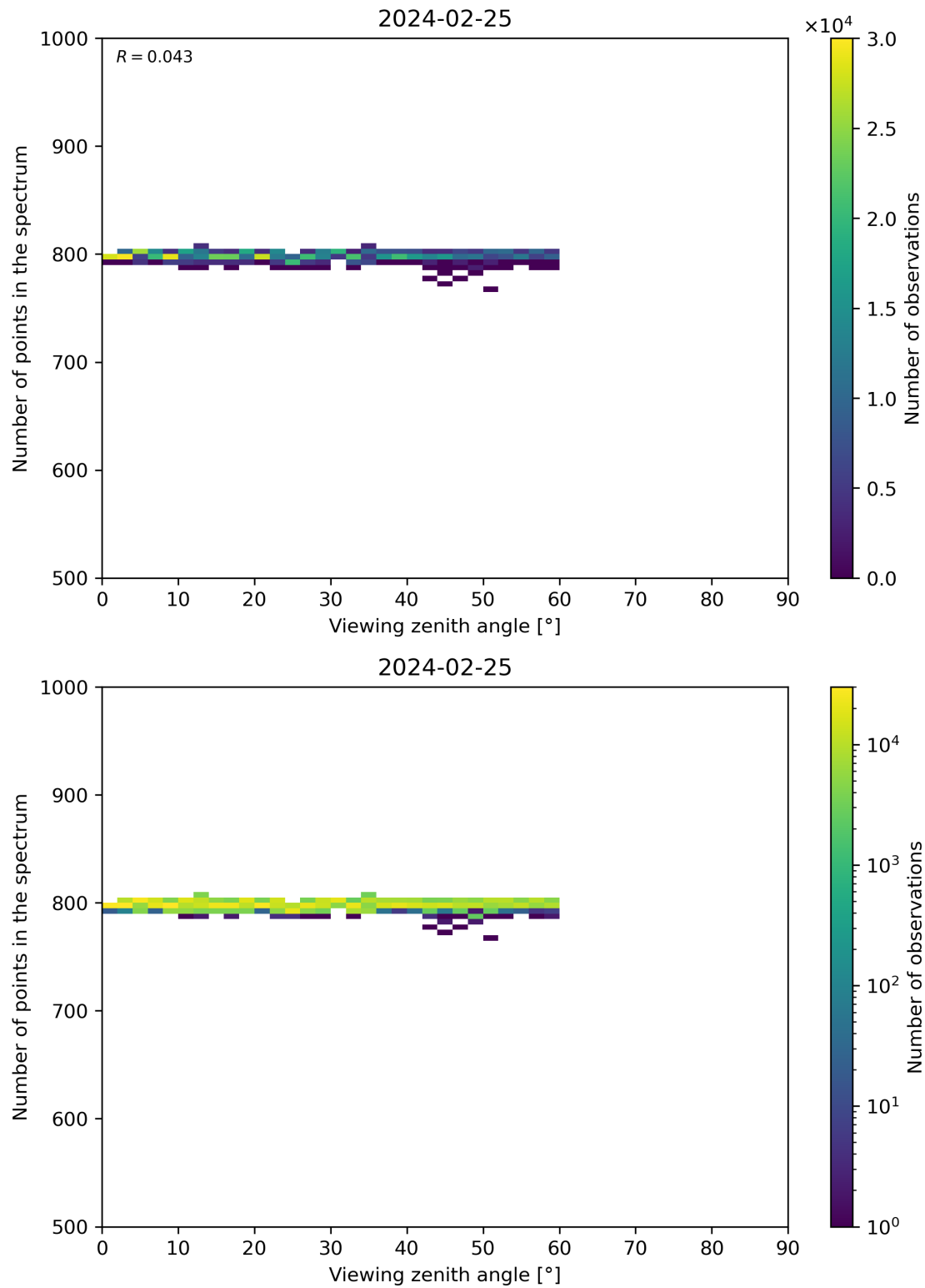
Figure 114: Scatter density plot of “Viewing zenith angle” against “Number of points in the spectrum” for 2024-02-24 to 2024-02-26.
