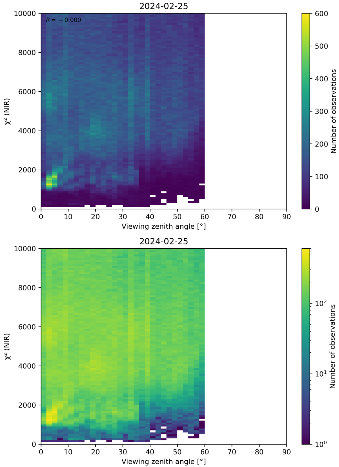
Figure 105: Scatter density plot of “Viewing zenith angle” against “ \chi^2 (NIR)” for 2024-02-24 to 2024-02-26.
