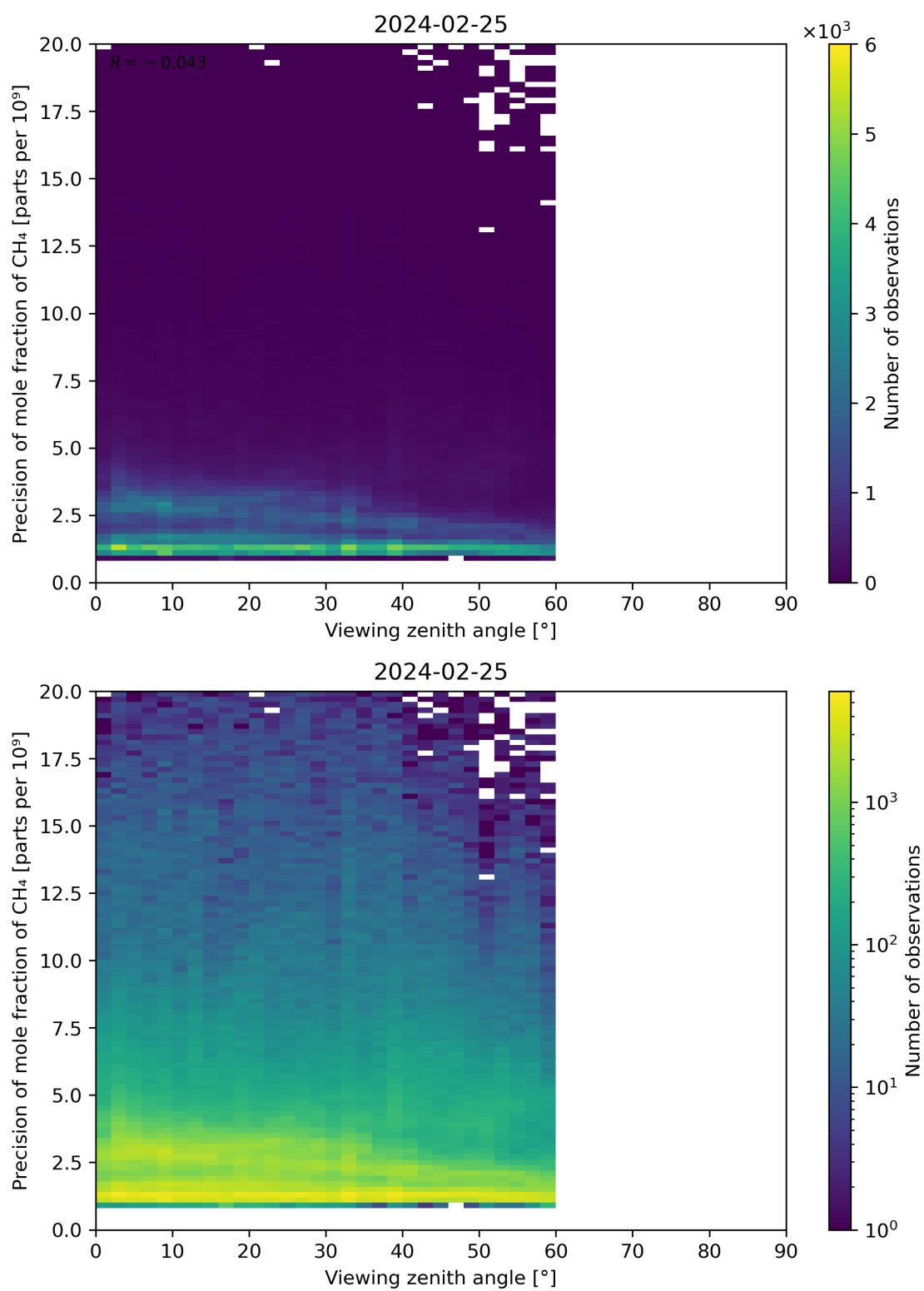
Figure 112: Scatter density plot of “Viewing zenith angle” against “Precision of mole fraction of CH 4 ” for 2024-02-24 to 2024-02-26.
