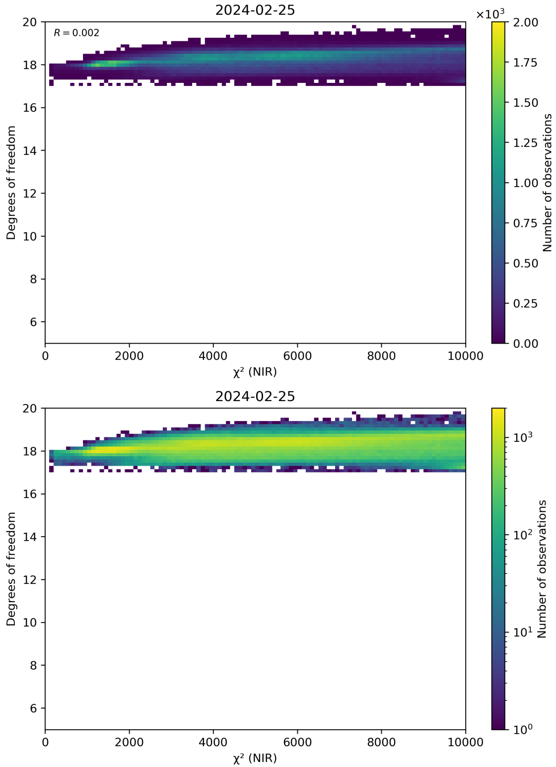
Figure 44: Scatter density plot of “ \chi^2 (NIR)” against “Degrees of freedom” for 2024-02-24 to 2024-02-26.
