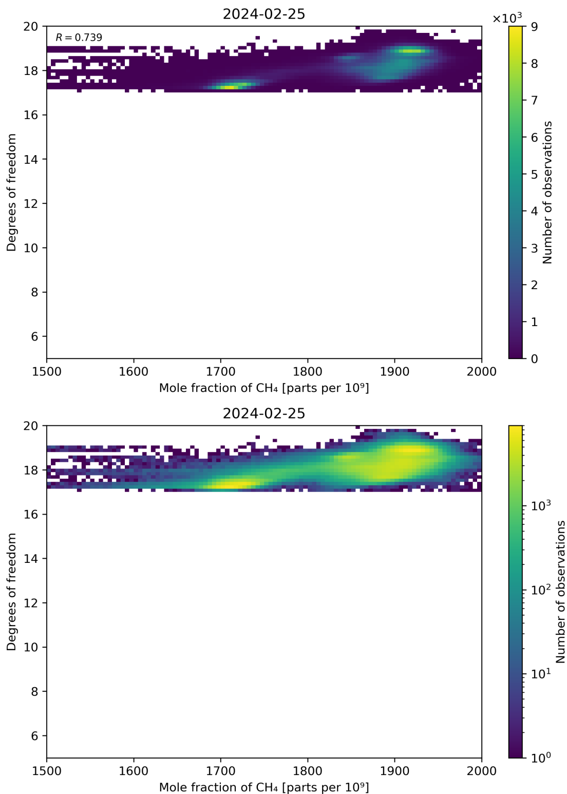
Figure 72: Scatter density plot of “Mole fraction of CH 4 ” against “Degrees of freedom” for 2024-02-24 to 2024-02-26.
