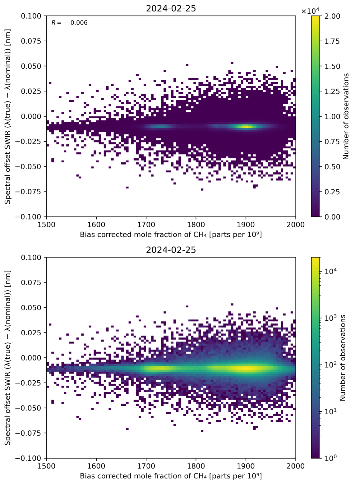
Figure 69: Scatter density plot of “Bias corrected mole fraction of \text{CH}_4 ” against “Spectral offset SWIR ( \lambda(\text{true}) - \lambda(\text{nominal}) )” for 2024-02-24 to 2024-02-26.
