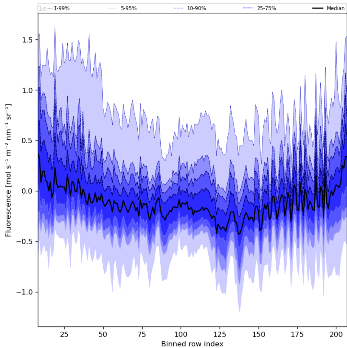
Figure 43: Along track statistics of “Fluorescence” for 2024-02-24 to 2024-02-26
