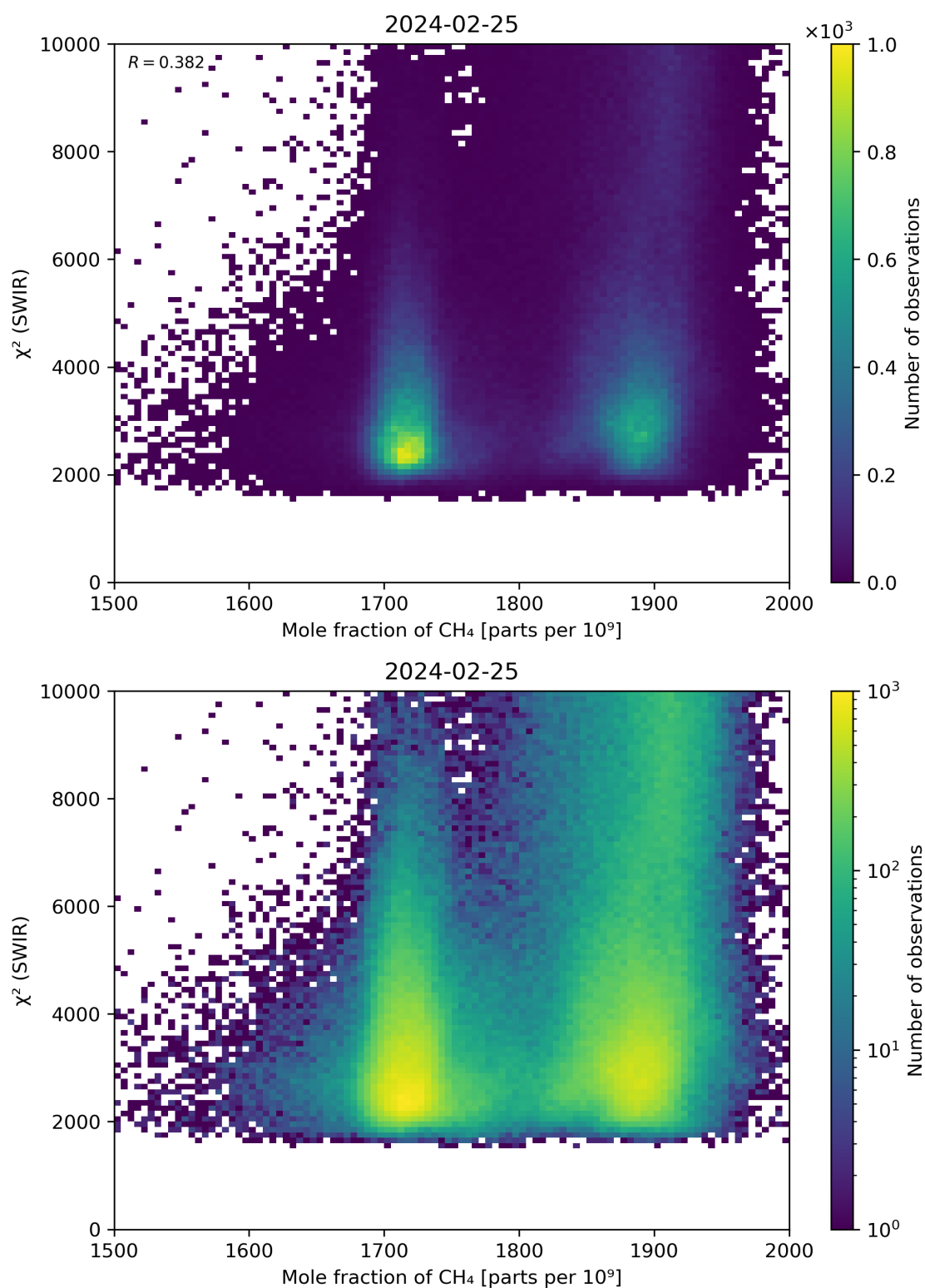
Figure 71: Scatter density plot of “Mole fraction of \text{CH}_4 ” against “ \chi^2 (SWIR)” for 2024-02-24 to 2024-02-26.
