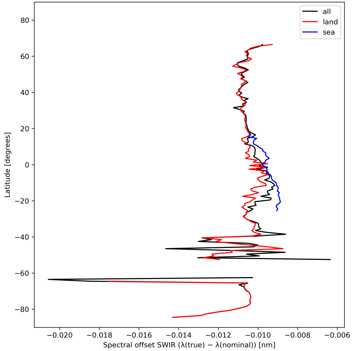
Figure 16: Zonal average of “Spectral offset SWIR ( \lambda(\text{true}) - \lambda(\text{nominal}) )” for 2024-02-24 to 2024-02-26.
