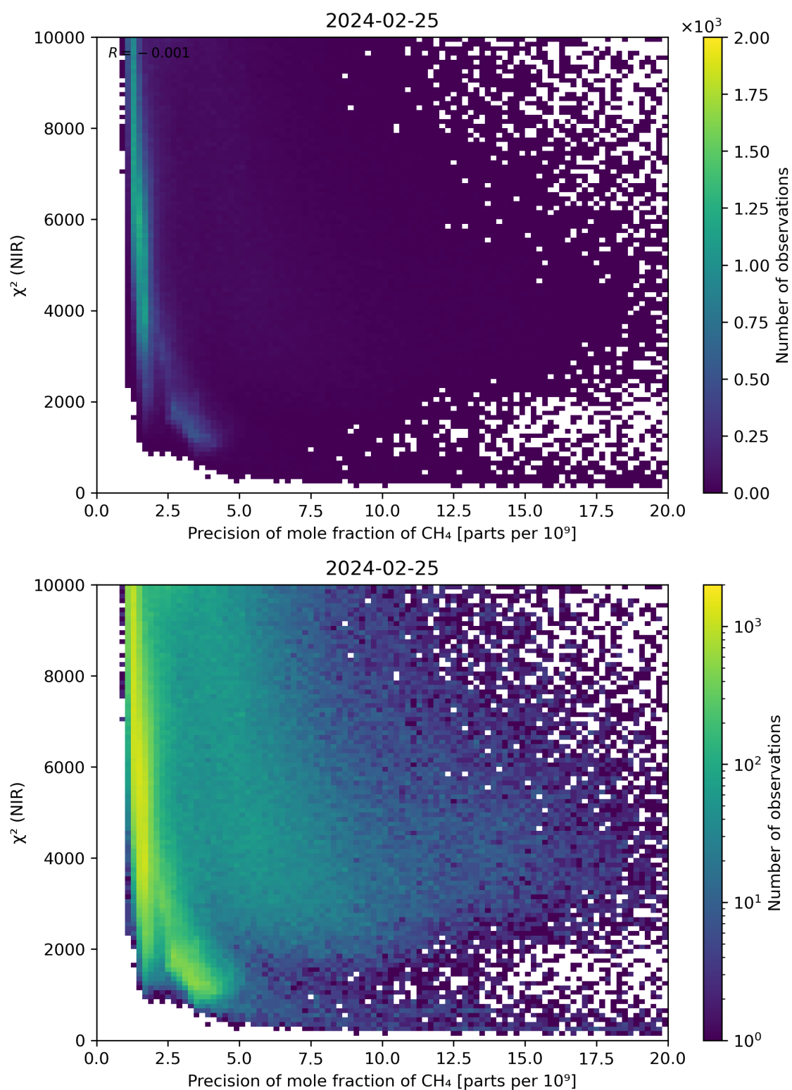
Figure 78: Scatter density plot of “Precision of mole fraction of CH 4 ” against “ \chi^2 (NIR)” for 2024-02-24 to 2024-02-26.
