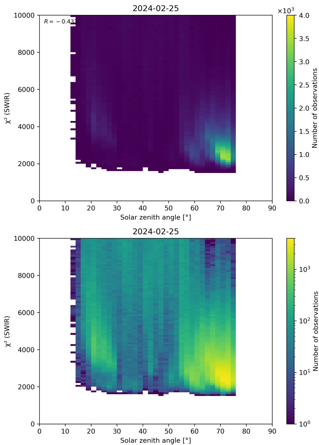
Figure 95: Scatter density plot of “Solar zenith angle” against “ \chi^2 (SWIR)” for 2024-02-24 to 2024-02-26.
