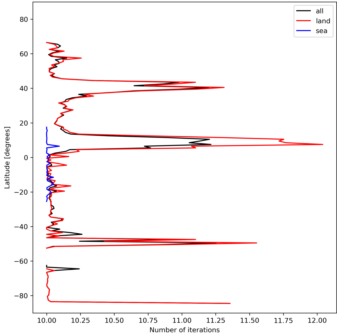
Figure 20: Zonal average of “Number of iterations” for 2024-02-24 to 2024-02-26.
