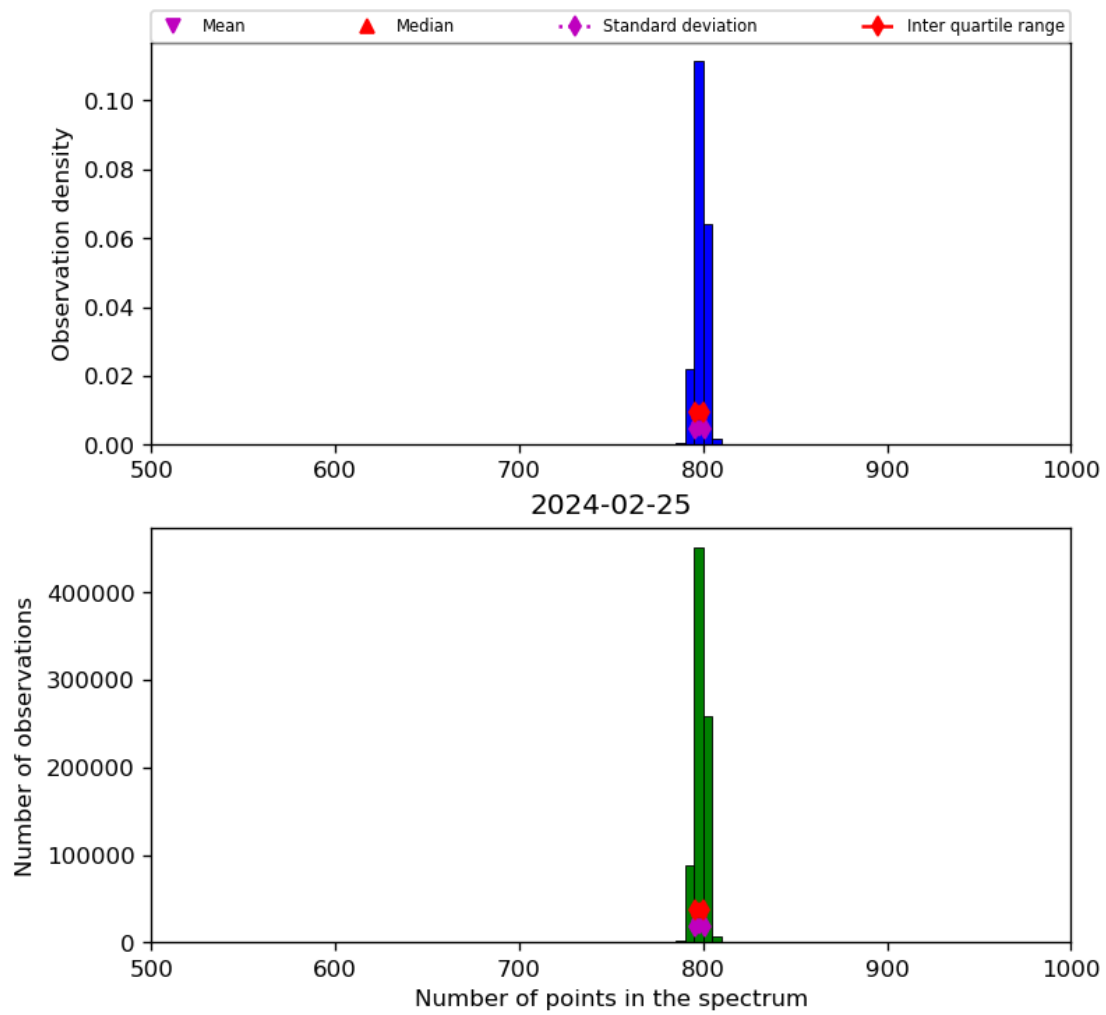
Figure 26: Histogram of “Number of points in the spectrum” for 2024-02-24 to 2024-02-26
