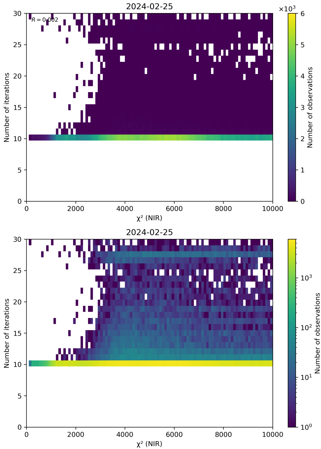
Figure 46: Scatter density plot of “ \chi^2 (NIR)” against “Number of iterations” for 2024-02-24 to 2024-02-26.
