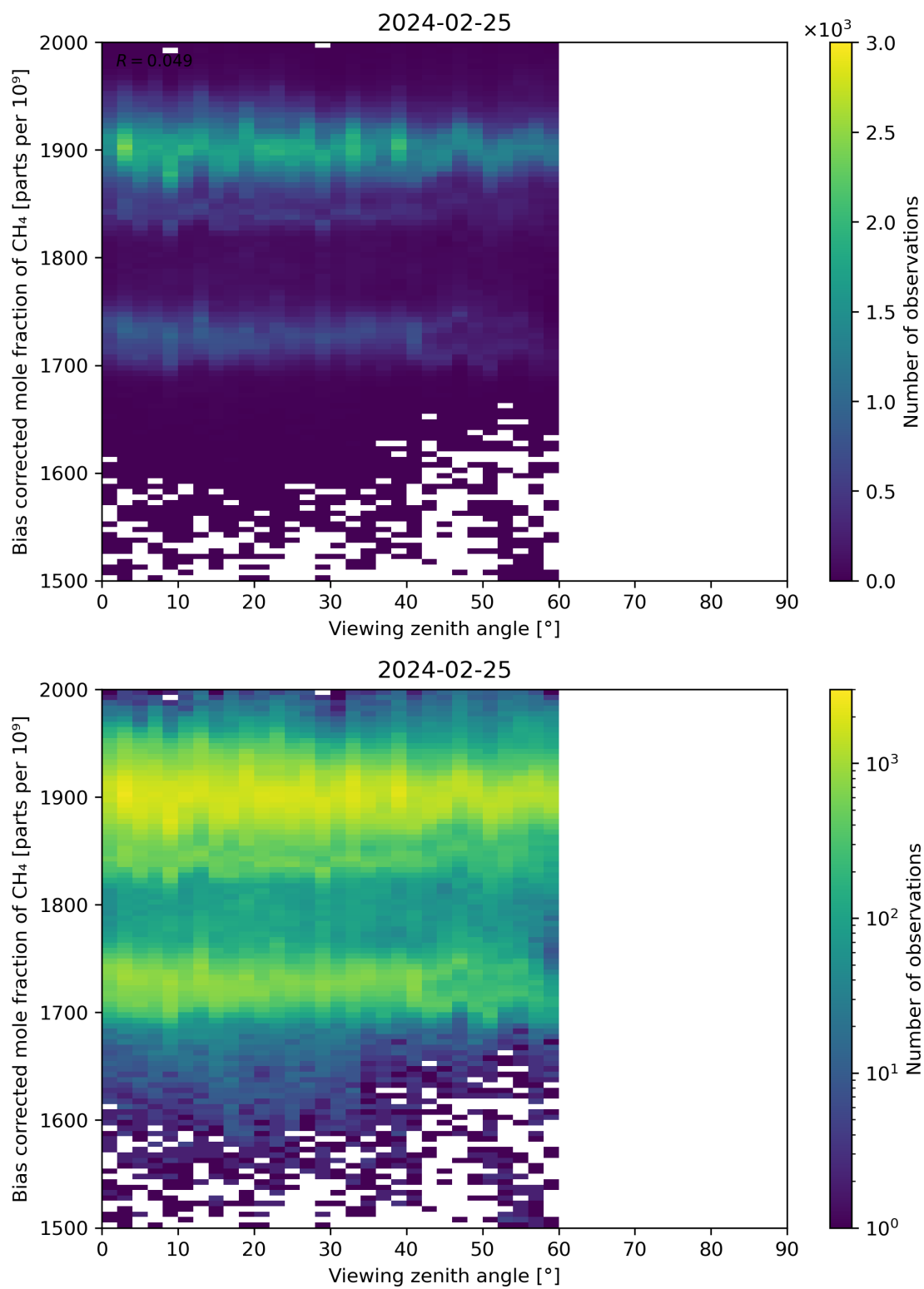
Figure 111: Scatter density plot of “Viewing zenith angle” against “Bias corrected mole fraction of CH 4 ” for 2024-02-24 to 2024-02-26.
