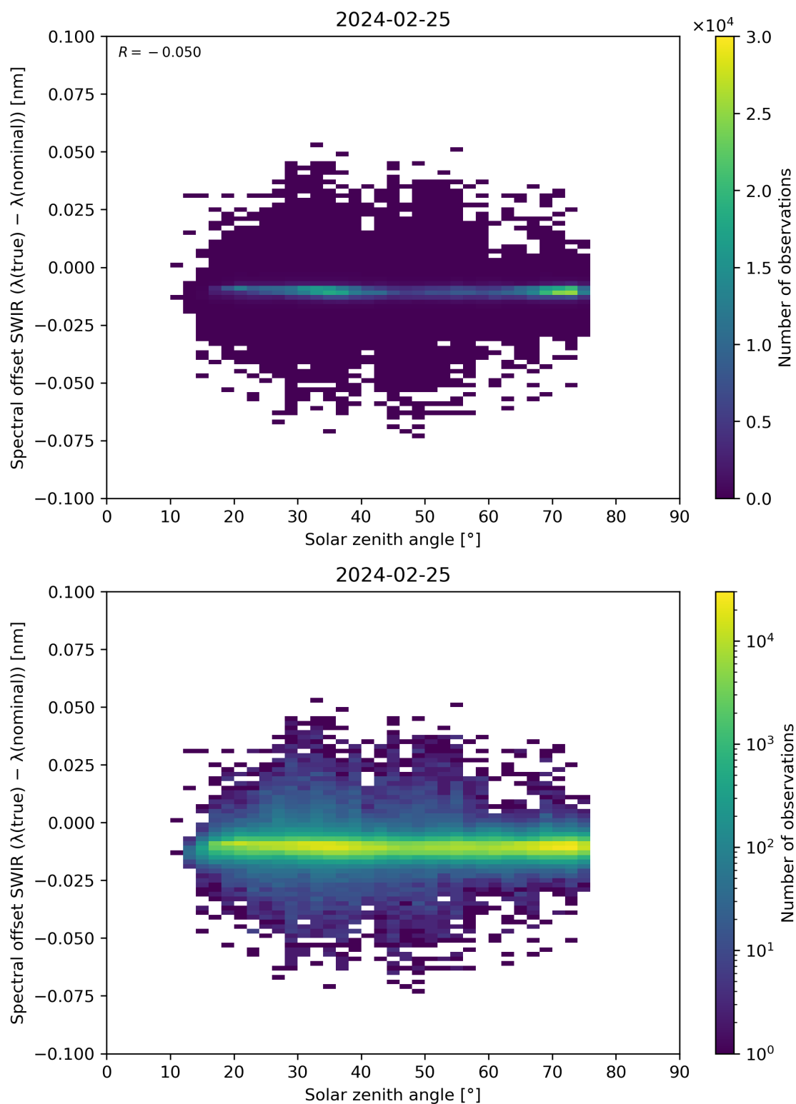
Figure 104: Scatter density plot of “Solar zenith angle” against “Spectral offset SWIR ( \lambda(\text{true}) - \lambda(\text{nominal}) )” for 2024-02-24 to 2024-02-26.
