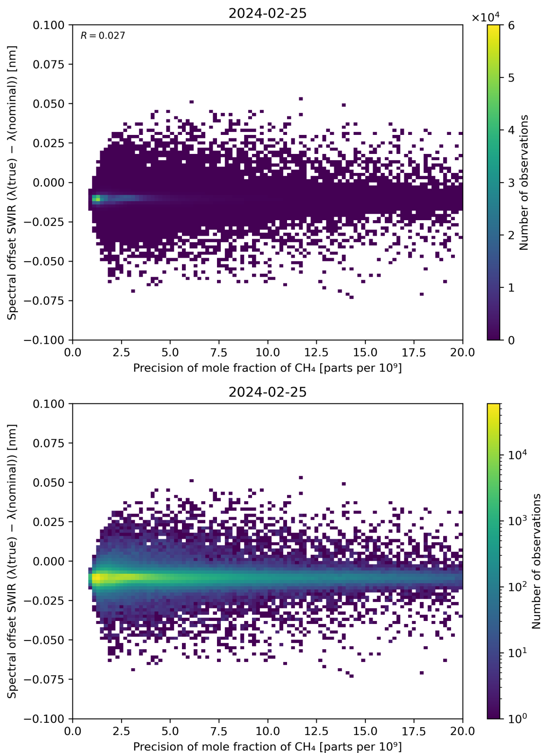
Figure 85: Scatter density plot of “Precision of mole fraction of \text{CH}_4 ” against “Spectral offset SWIR ( \lambda(\text{true}) - \lambda(\text{nominal}) )” for 2024-02-24 to 2024-02-26.
