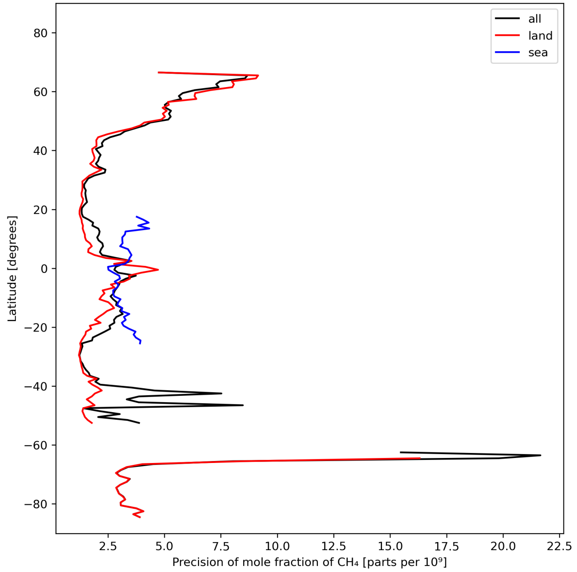
Figure 13: Zonal average of “Precision of mole fraction of CH 4 ” for 2024-02-24 to 2024-02-26.
