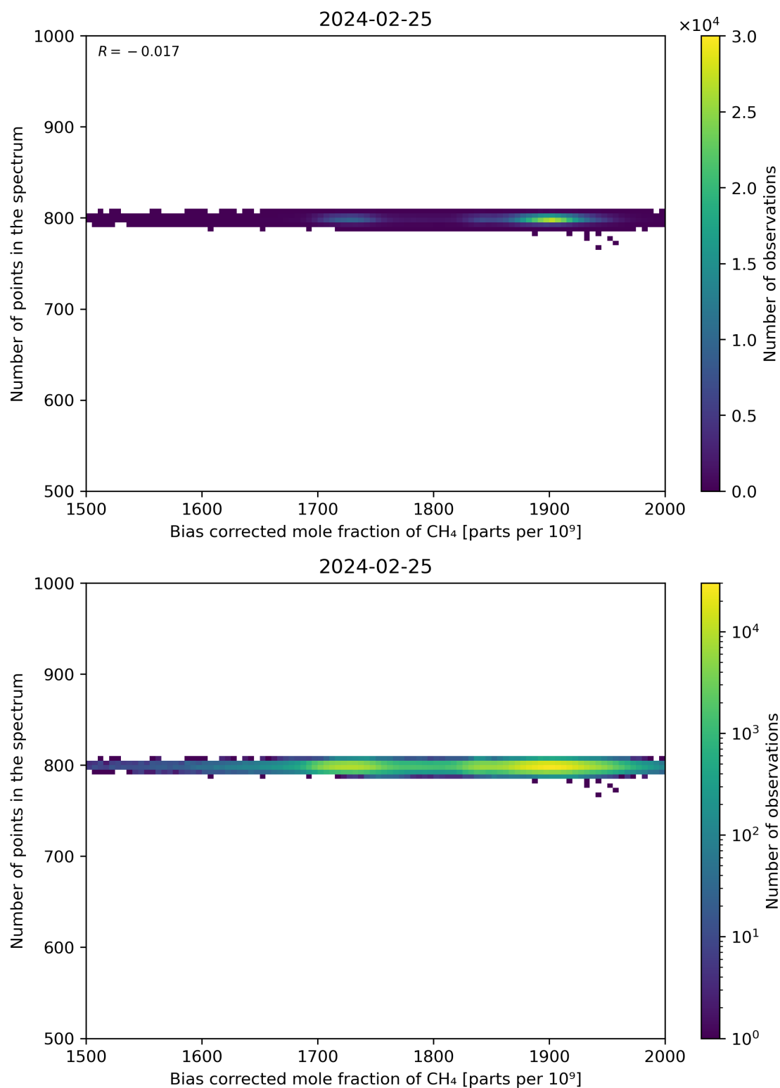
Figure 68: Scatter density plot of “Bias corrected mole fraction of CH 4 ” against “Number of points in the spectrum” for 2024-02-24 to 2024-02-26.
