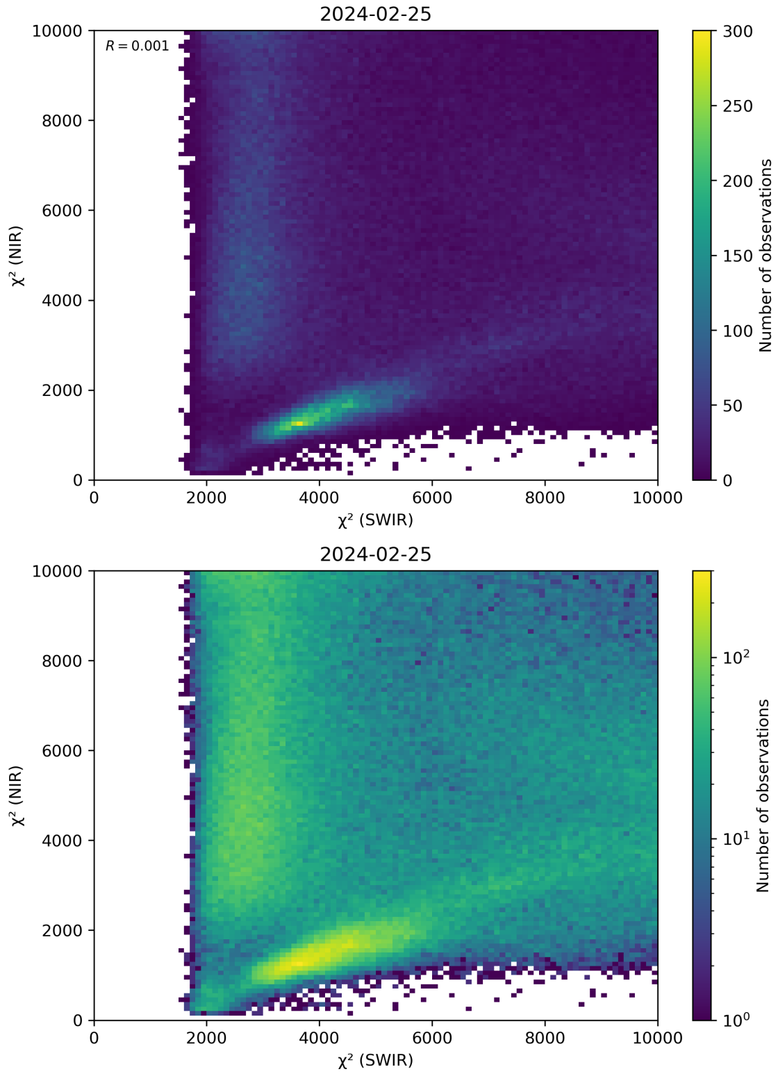
Figure 47: Scatter density plot of “ \chi^2 (SWIR)” against “ \chi^2 (NIR)” for 2024-02-24 to 2024-02-26.
