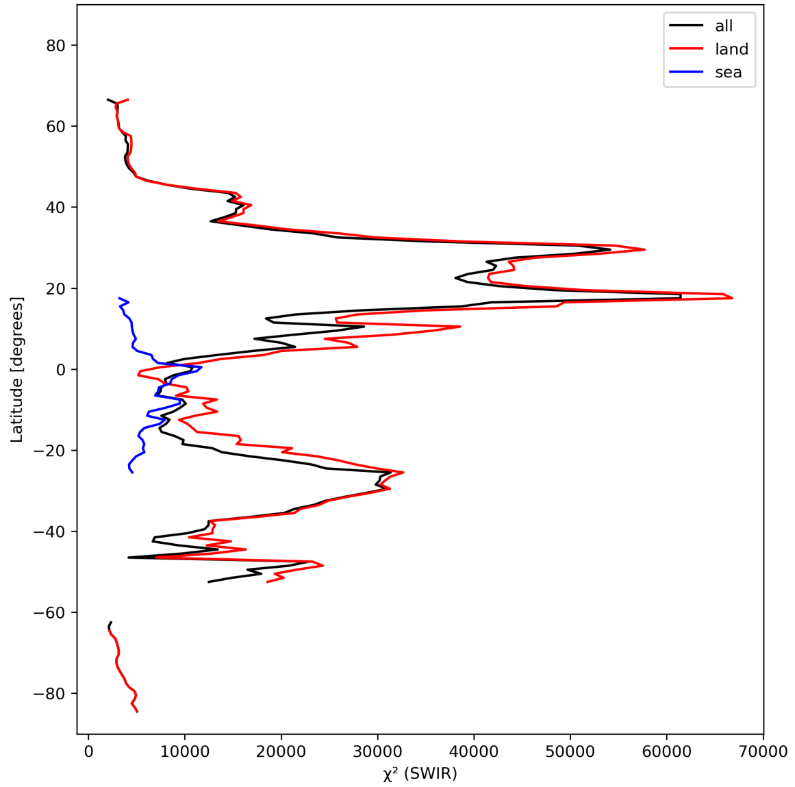
Figure 17: Zonal average of “ \chi^2 (SWIR)” for 2024-02-24 to 2024-02-26.
