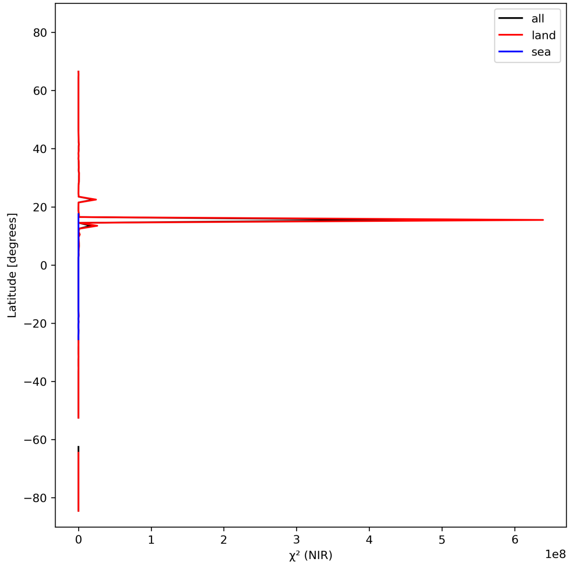
Figure 18: Zonal average of “ \chi^2 (NIR)” for 2024-02-24 to 2024-02-26.
