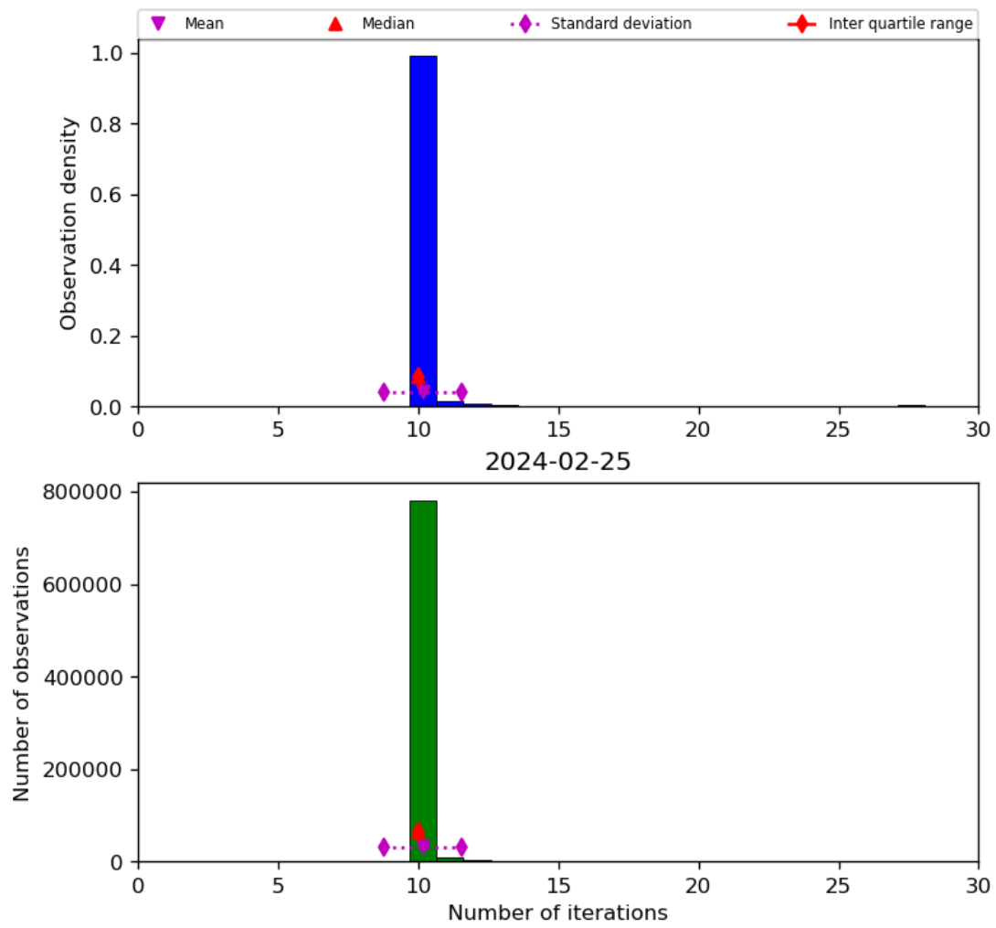
Figure 31: Histogram of “Number of iterations” for 2024-02-24 to 2024-02-26
