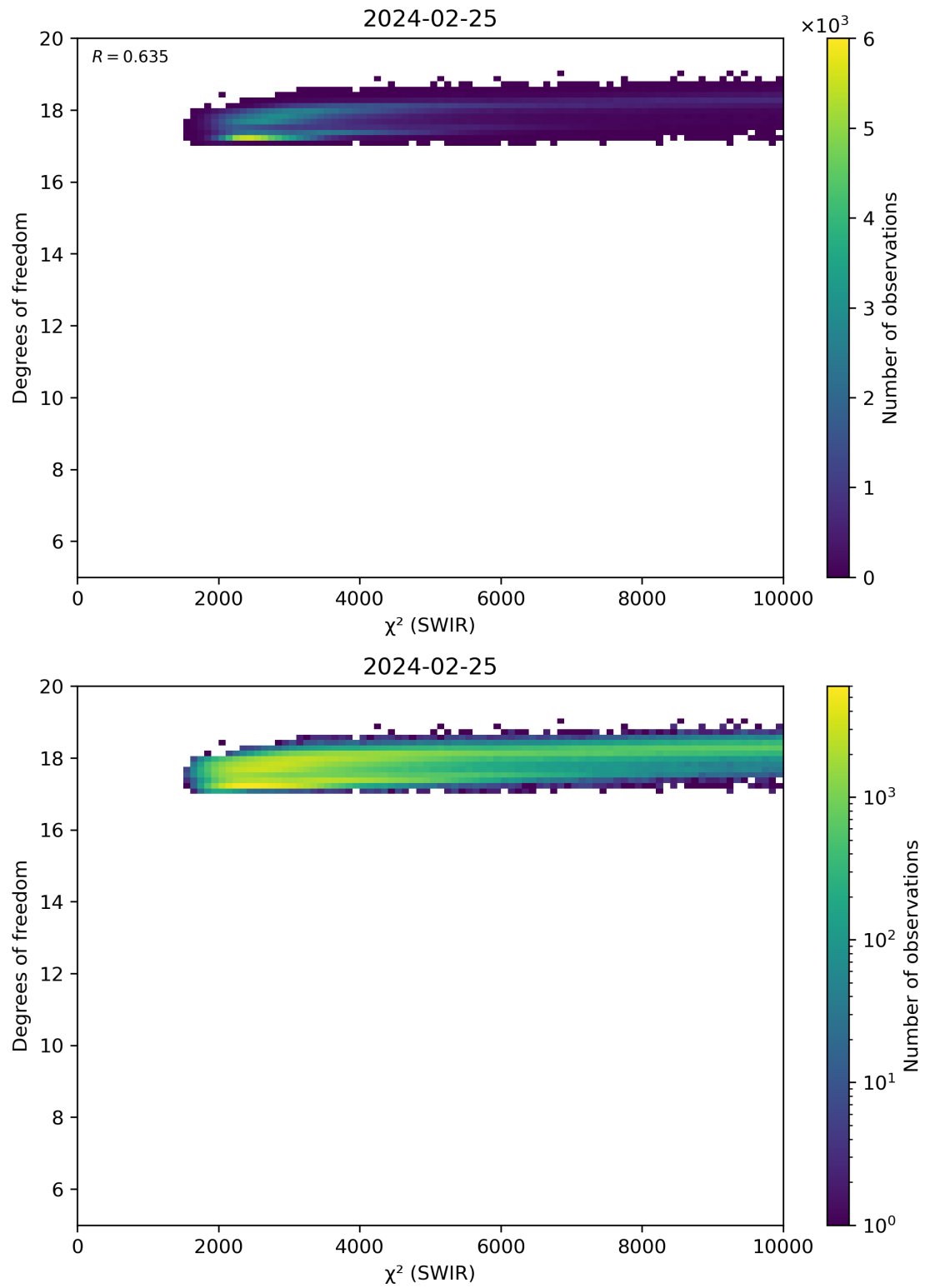
Figure 48: Scatter density plot of “ \chi^2 (SWIR)” against “Degrees of freedom” for 2024-02-24 to 2024-02-26.
