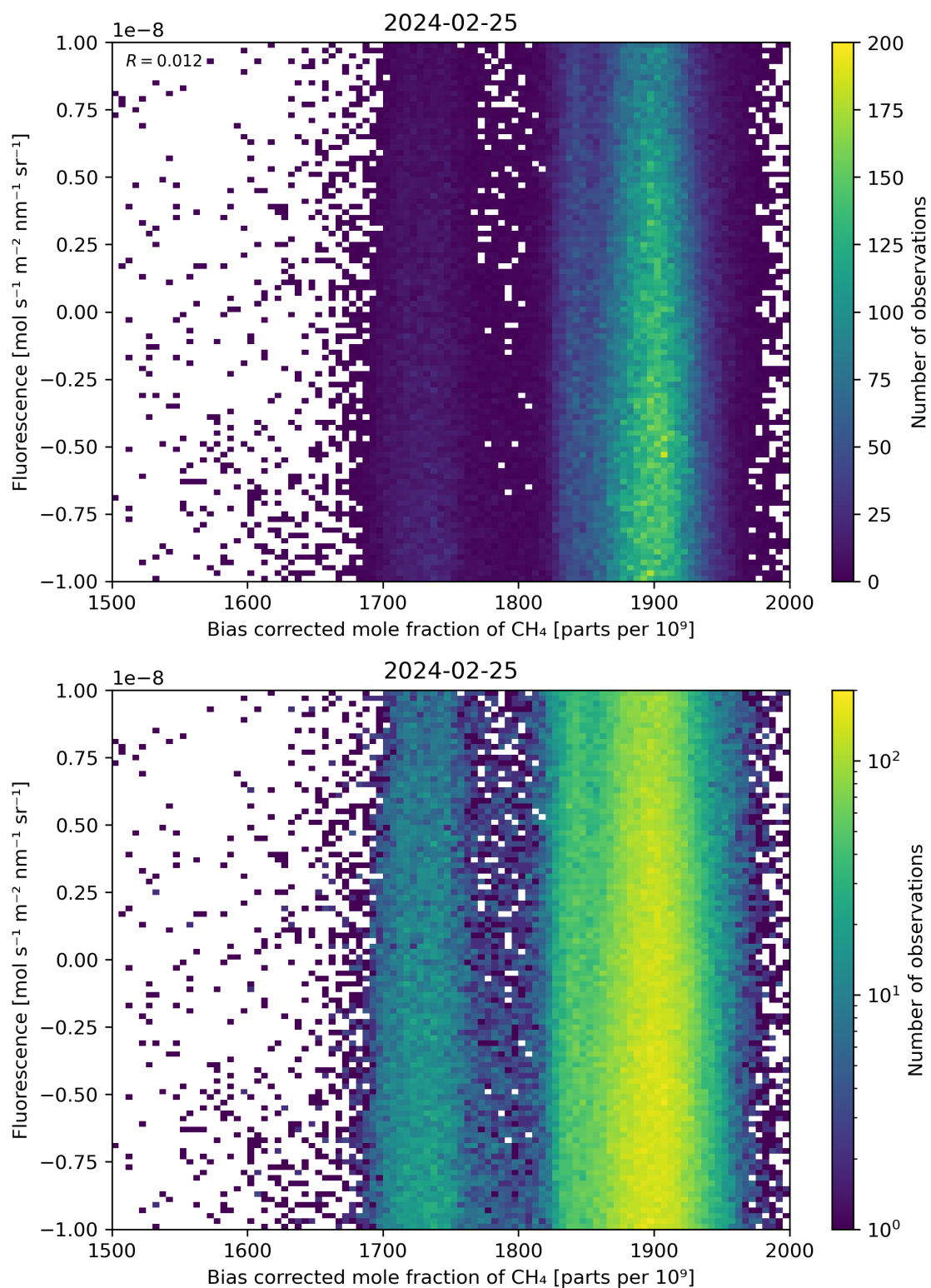
Figure 66: Scatter density plot of “Bias corrected mole fraction of \text{CH}_4 ” against “Fluorescence” for 2024-02-24 to 2024-02-26.
