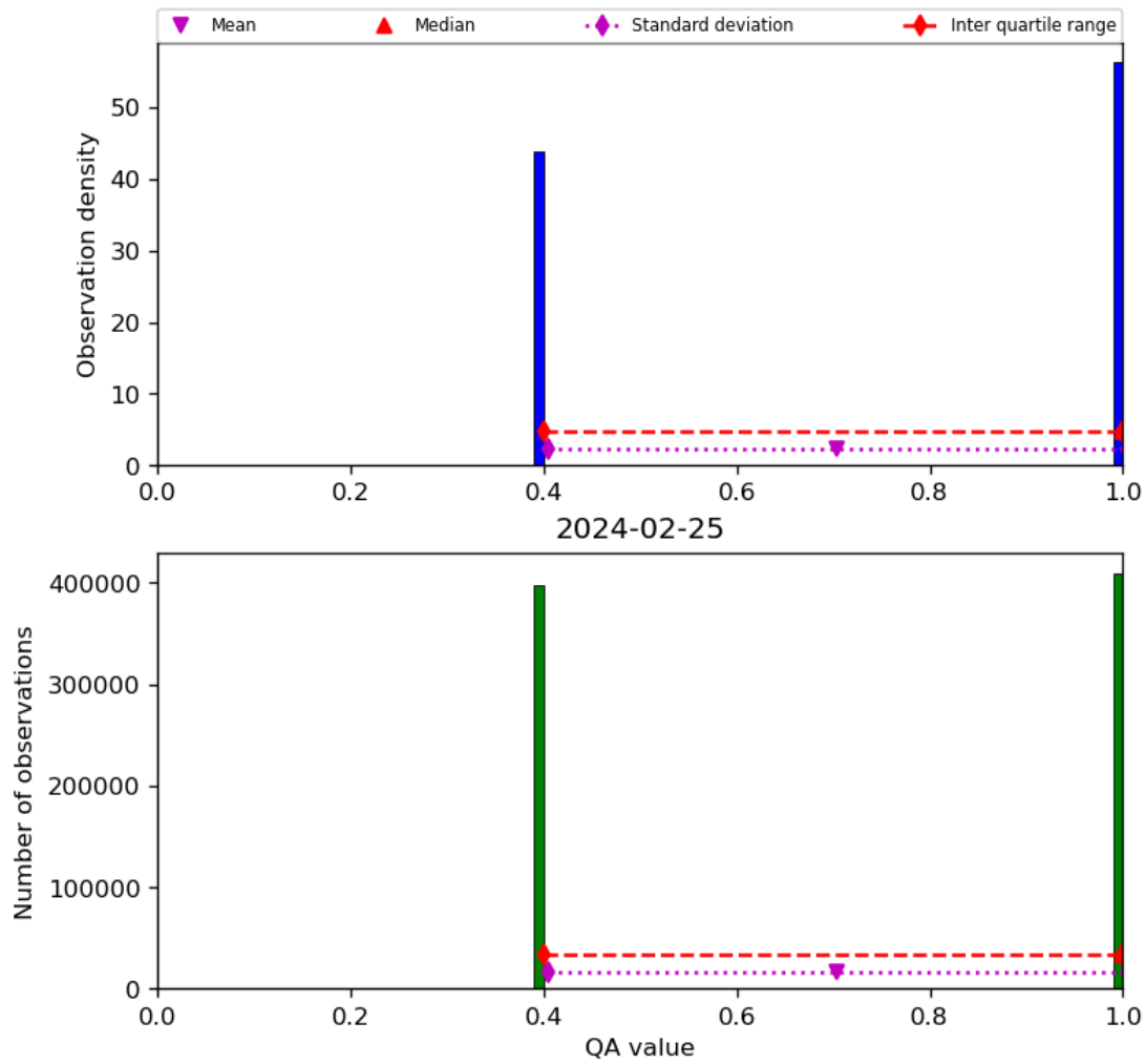
Figure 22: Histogram of “QA value” for 2024-02-24 to 2024-02-26
