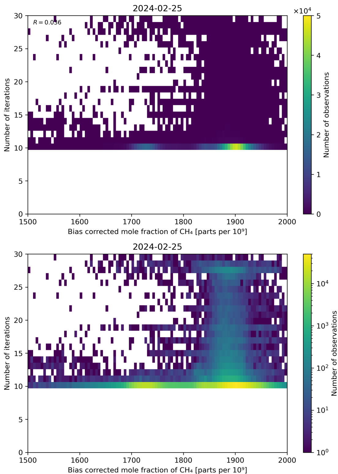
Figure 67: Scatter density plot of “Bias corrected mole fraction of \text{CH}_4 ” against “Number of iterations” for 2024-02-24 to 2024-02-26.
