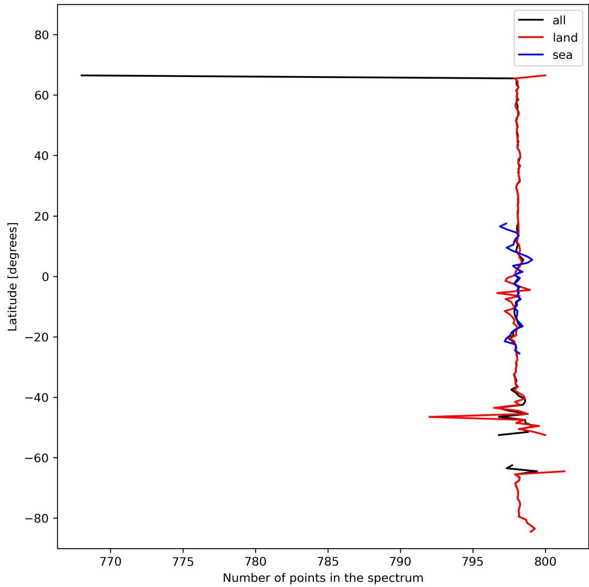
Figure 15: Zonal average of “Number of points in the spectrum” for 2024-02-24 to 2024-02-26.
