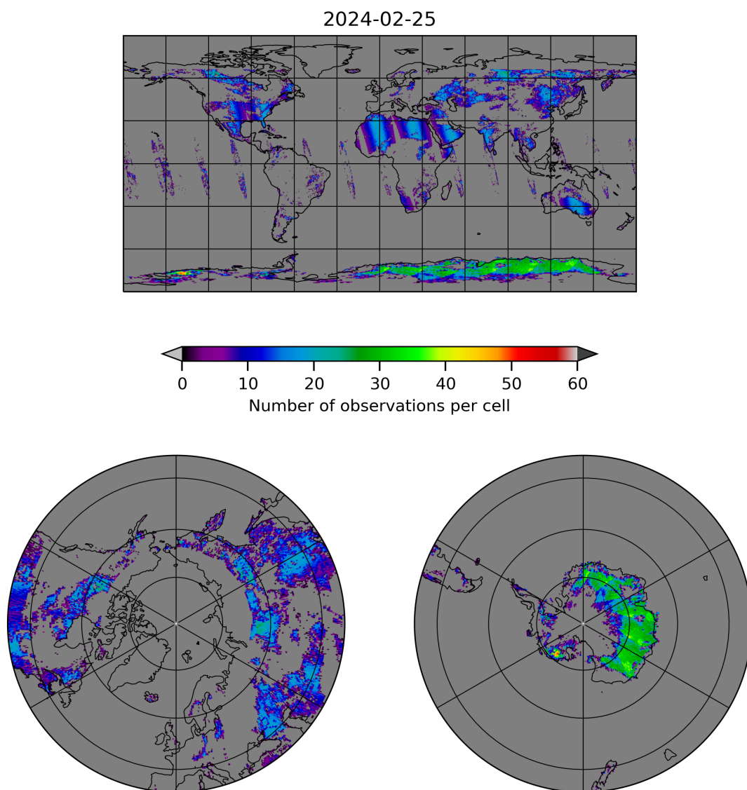
Figure 10: Map of the number of observations for 2024-02-24 to 2024-02-26
