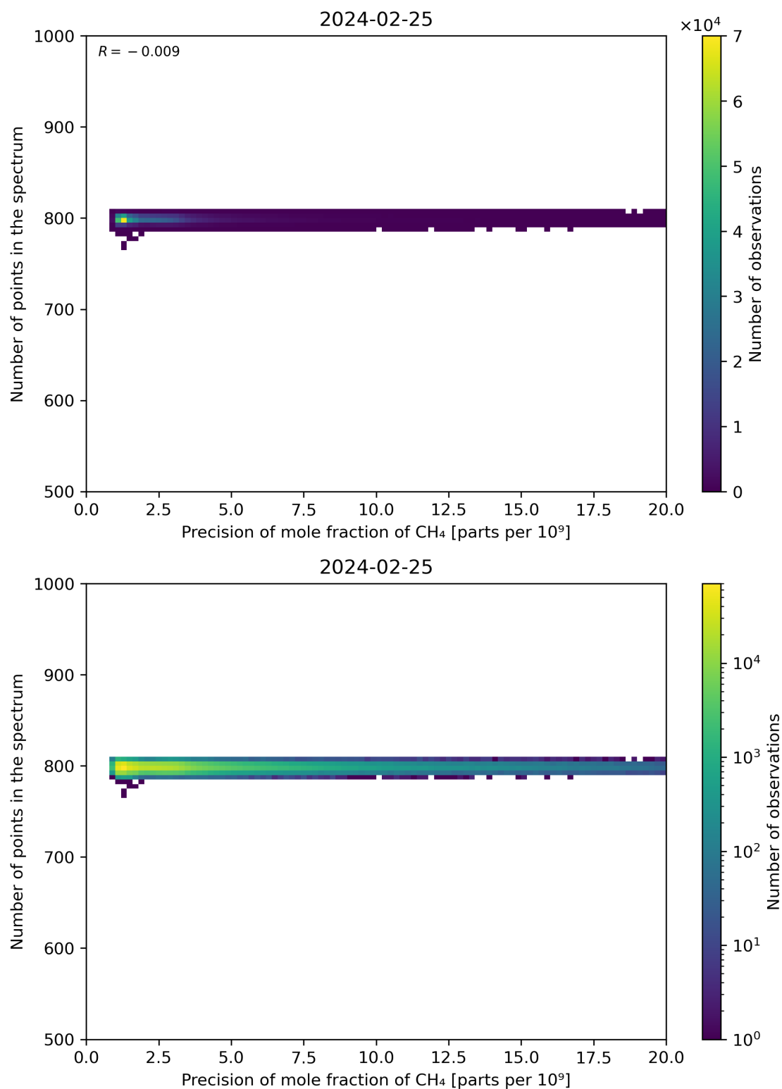
Figure 84: Scatter density plot of “Precision of mole fraction of CH 4 ” against “Number of points in the spectrum” for 2024-02-24 to 2024-02-26.
