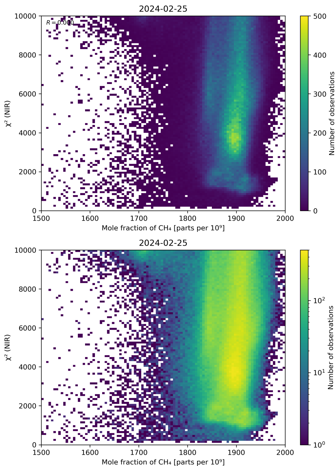
Figure 70: Scatter density plot of “Mole fraction of \text{CH}_4 ” against “ \chi^2 (NIR)” for 2024-02-24 to 2024-02-26.
