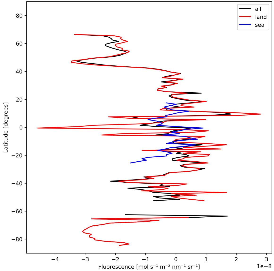
Figure 21: Zonal average of “Fluorescence” for 2024-02-24 to 2024-02-26.
