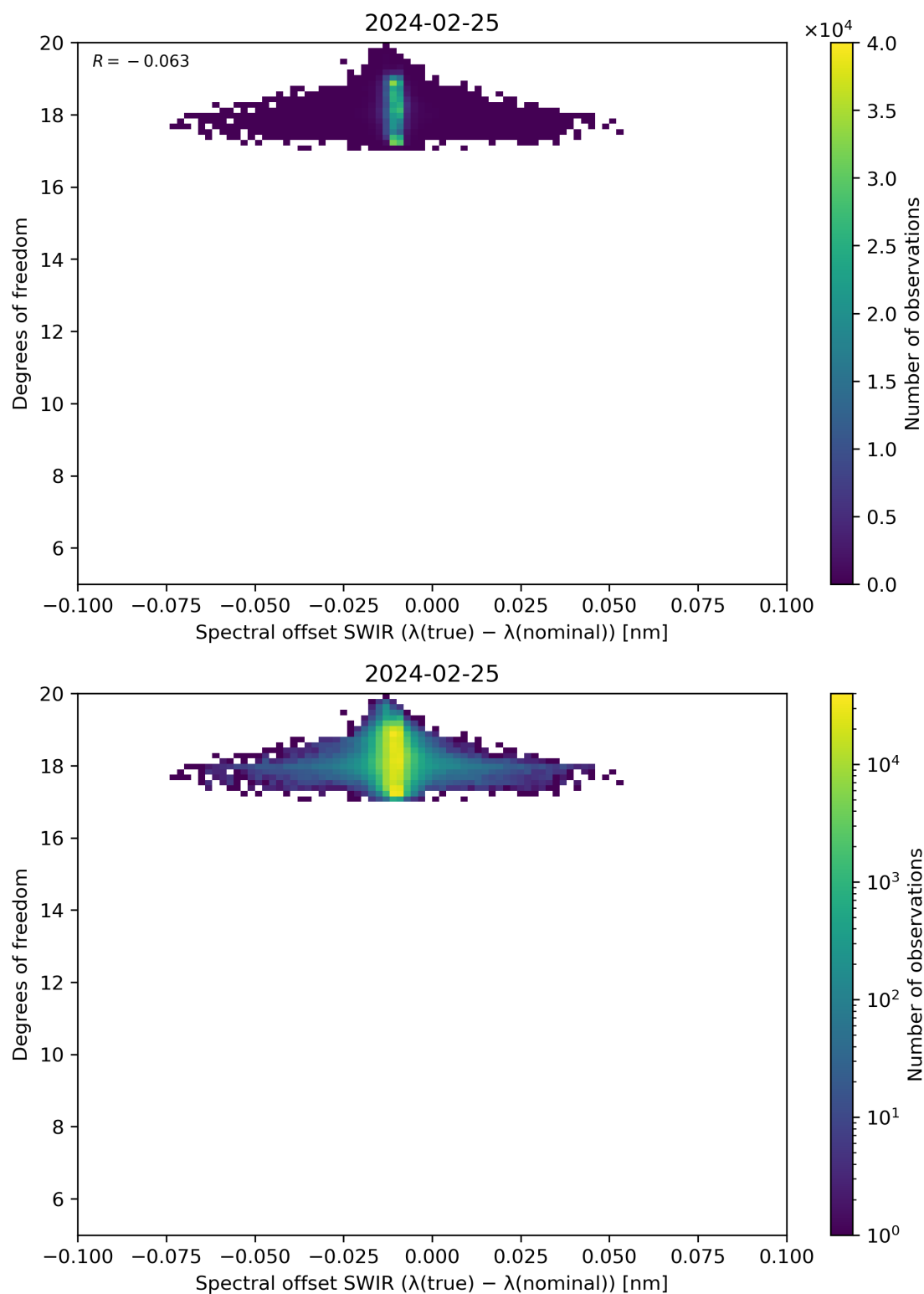
Figure 119: Scatter density plot of “Spectral offset SWIR ( \lambda(\text{true}) - \lambda(\text{nominal}) )” against “Degrees of freedom” for 2024-02-24 to 2024-02-26.
