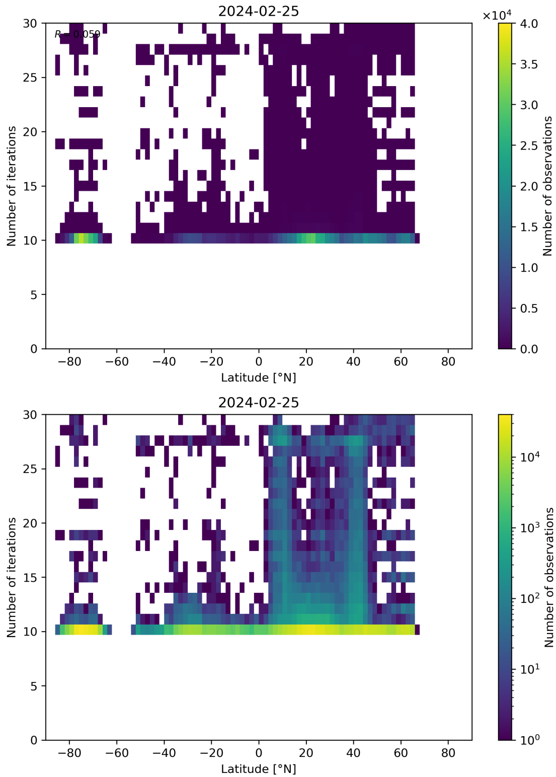
Figure 60: Scatter density plot of “Latitude” against “Number of iterations” for 2024-02-24 to 2024-02-26.
