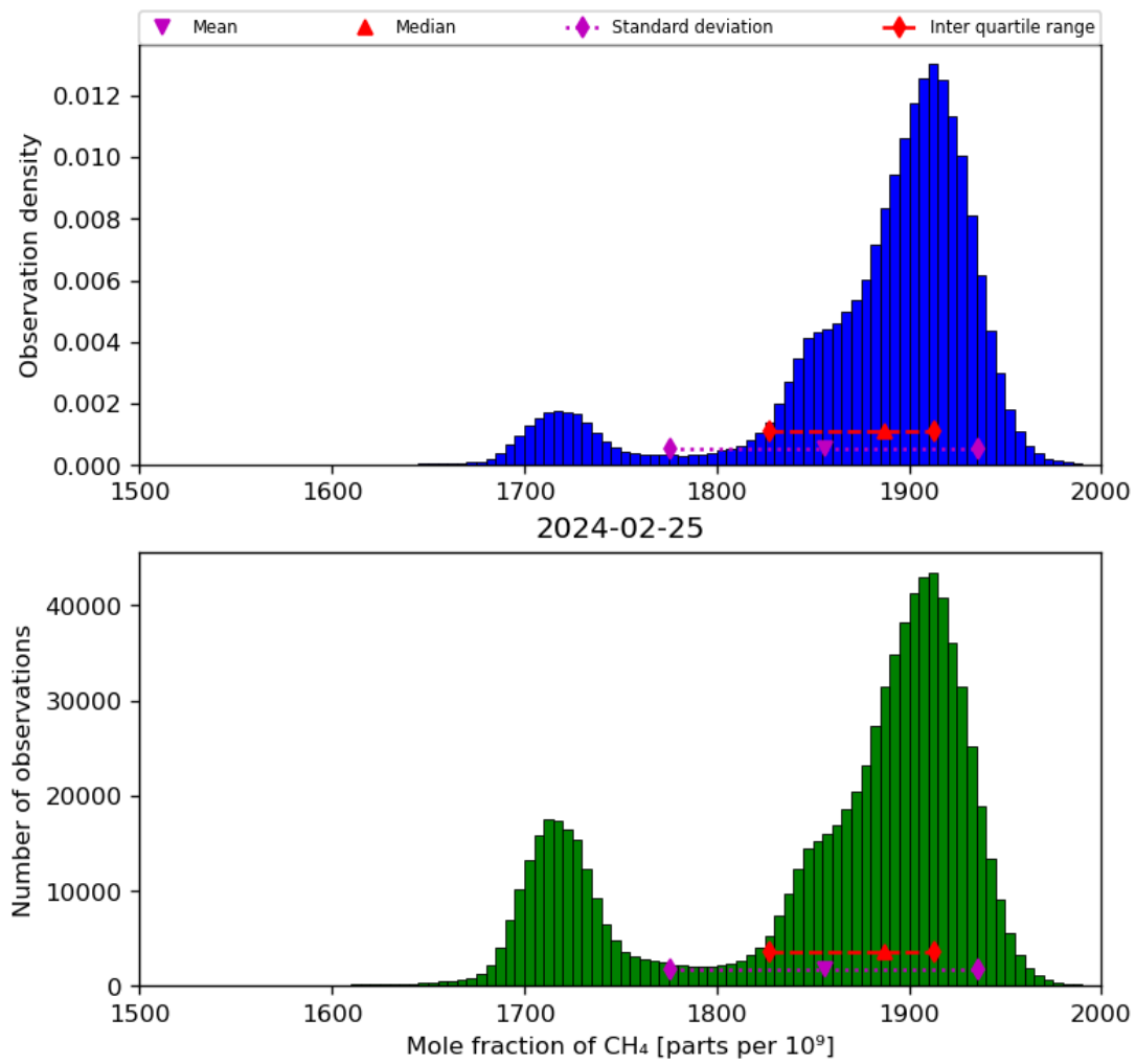
Figure 23: Histogram of “Mole fraction of CH 4 ” for 2024-02-24 to 2024-02-26
