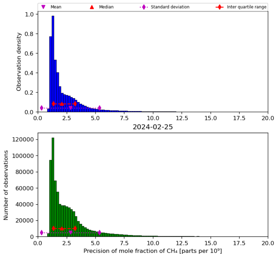
Figure 24: Histogram of “Precision of mole fraction of CH 4 ” for 2024-02-24 to 2024-02-26
