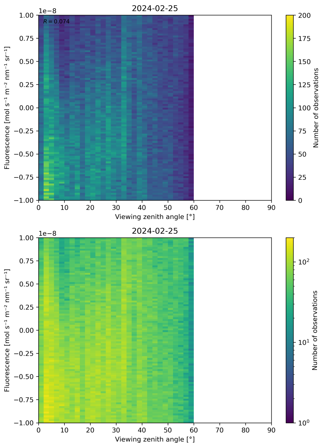
Figure 108: Scatter density plot of “Viewing zenith angle” against “Fluorescence” for 2024-02-24 to 2024-02-26.
