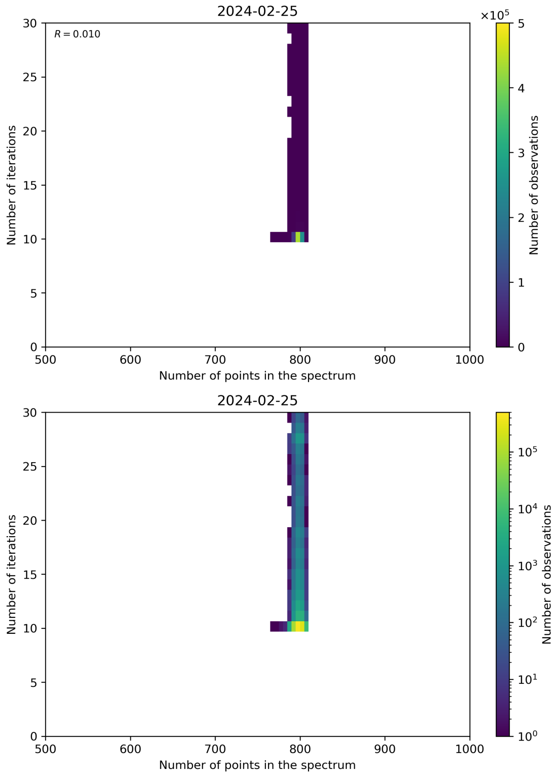
Figure 92: Scatter density plot of “Number of points in the spectrum” against “Number of iterations” for 2024-02-24 to 2024-02-26.
