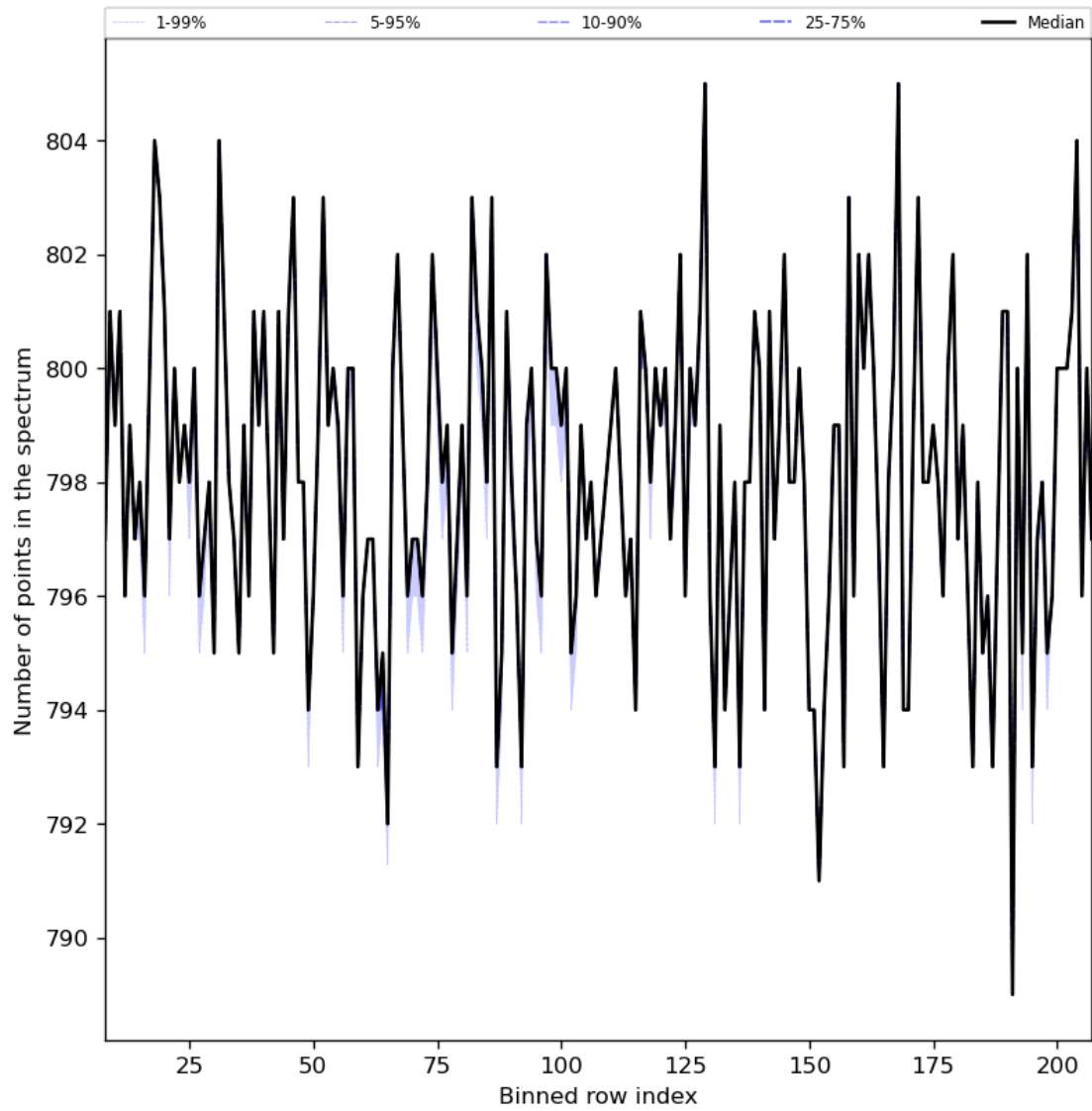
Figure 37: Along track statistics of “Number of points in the spectrum” for 2024-02-24 to 2024-02-26
