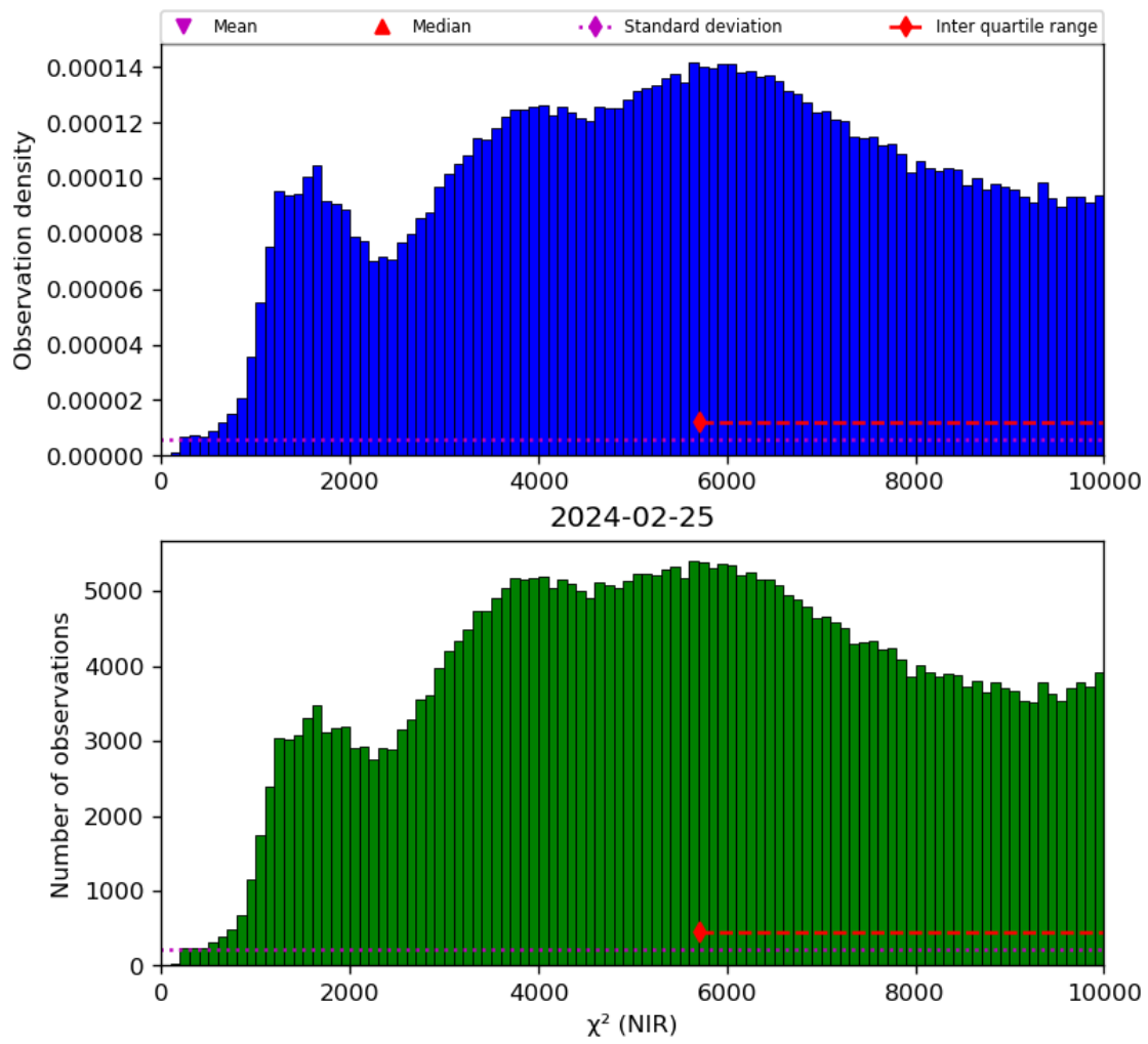
Figure 29: Histogram of " \chi^2 (NIR)" for 2024-02-24 to 2024-02-26
