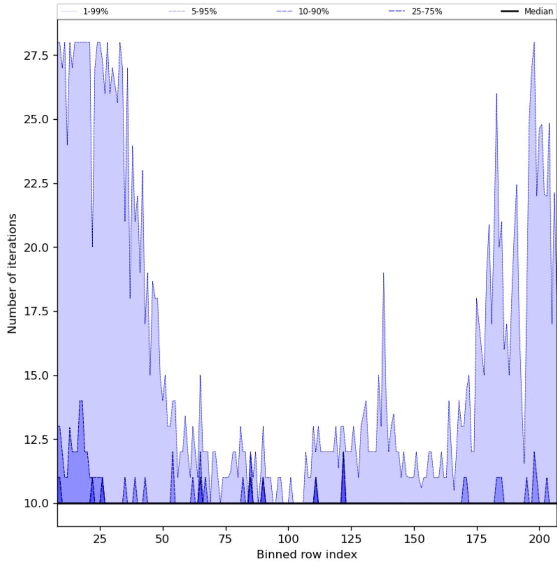
Figure 42: Along track statistics of “Number of iterations” for 2024-02-24 to 2024-02-26
