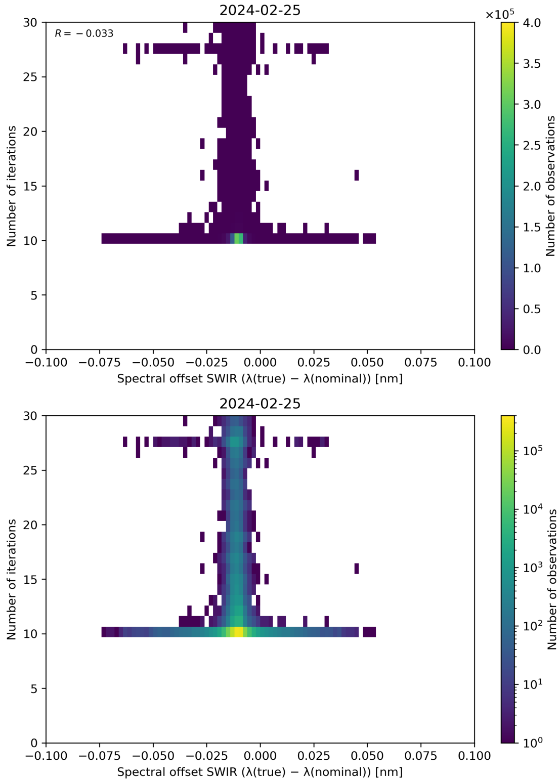
Figure 121: Scatter density plot of “Spectral offset SWIR ( \lambda(\text{true}) - \lambda(\text{nominal}) )” against “Number of iterations” for 2024-02-24 to 2024-02-26.
