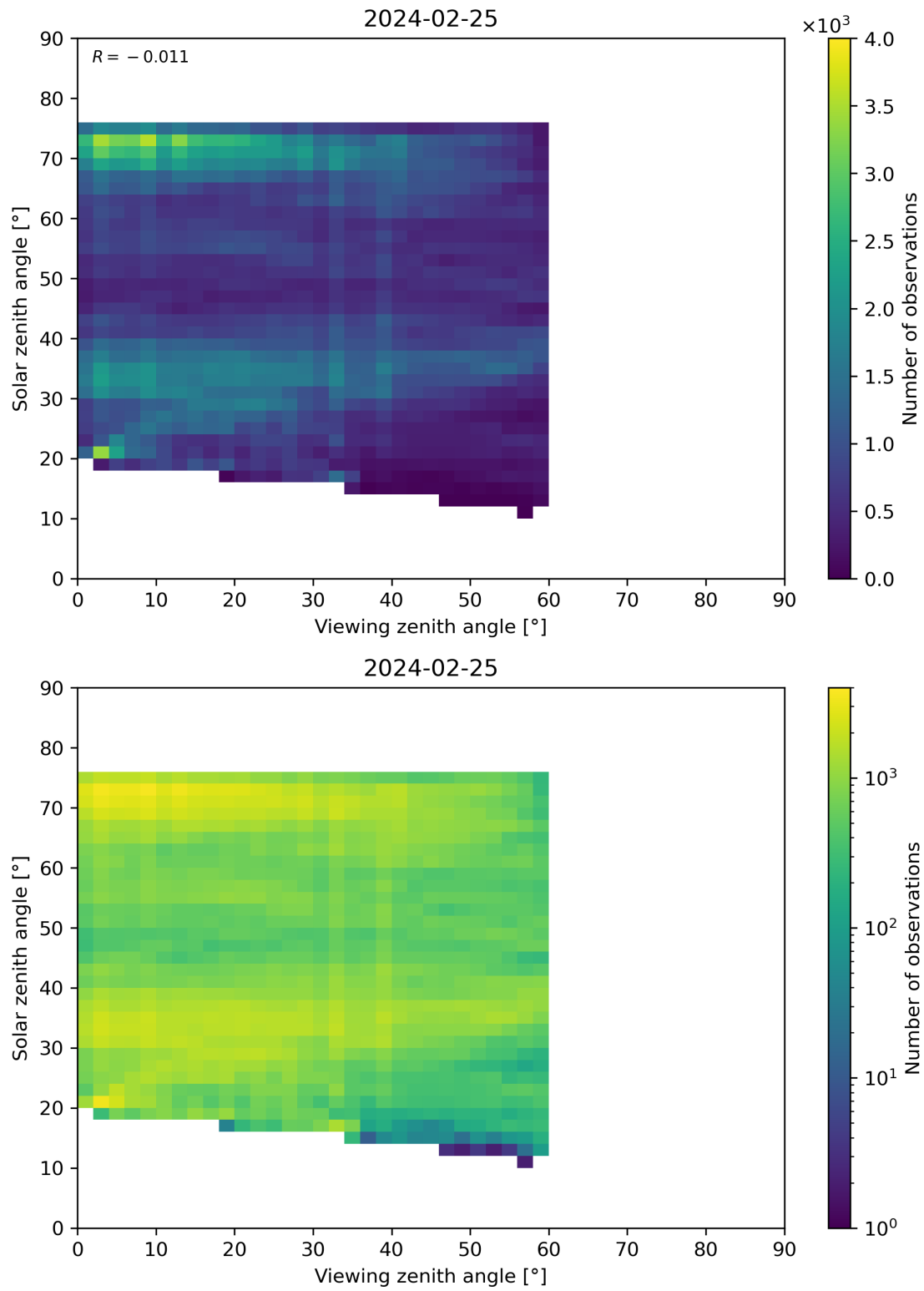
Figure 115: Scatter density plot of “Viewing zenith angle” against “Solar zenith angle” for 2024-02-24 to 2024-02-26.
