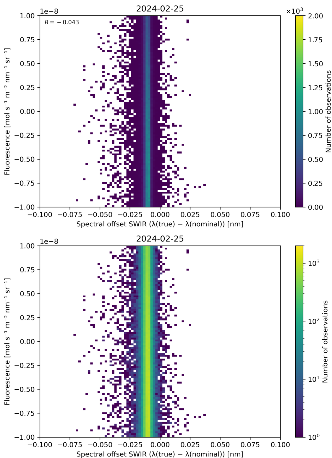
Figure 120: Scatter density plot of “Spectral offset SWIR ( \lambda(\text{true}) - \lambda(\text{nominal}) )” against “Fluorescence” for 2024-02-24 to 2024-02-26.
