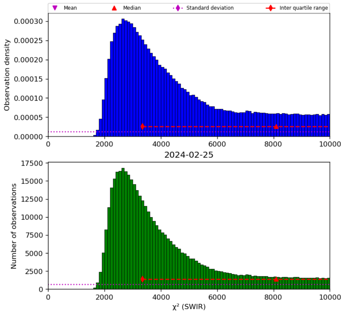
Figure 28: Histogram of “ \chi^2 (SWIR)” for 2024-02-24 to 2024-02-26
