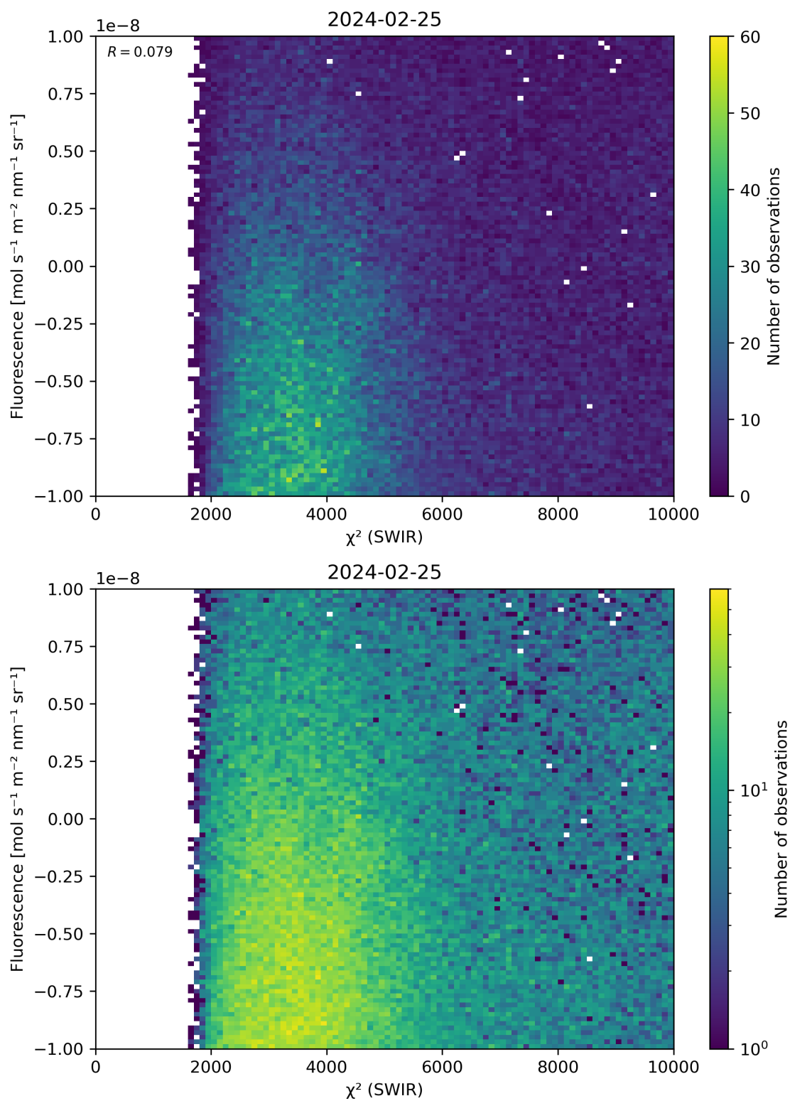
Figure 49: Scatter density plot of “ \chi^2 (SWIR)” against “Fluorescence” for 2024-02-24 to 2024-02-26.
