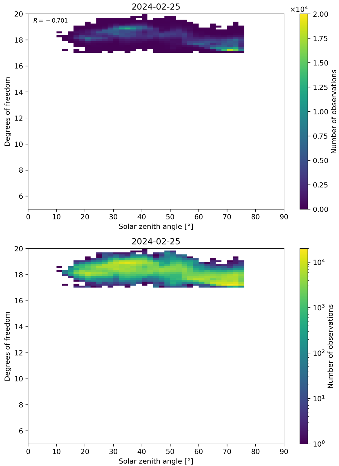
Figure 96: Scatter density plot of “Solar zenith angle” against “Degrees of freedom” for 2024-02-24 to 2024-02-26.
