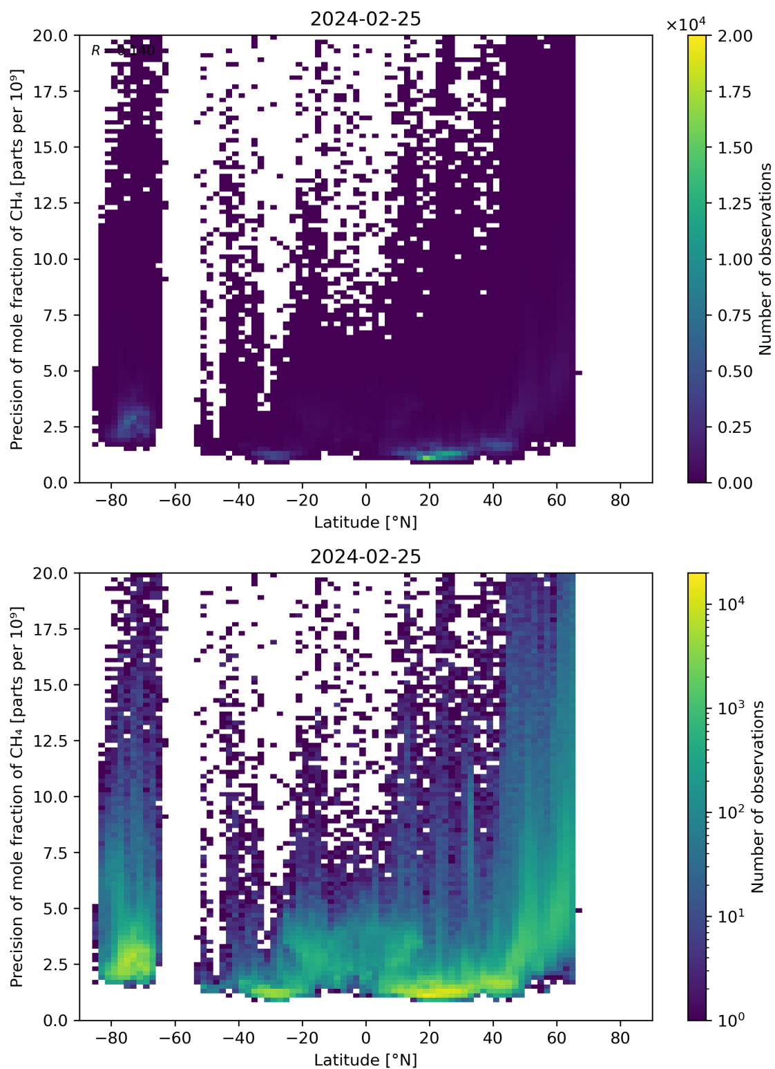
Figure 59: Scatter density plot of “Latitude” against “Precision of mole fraction of CH 4 ” for 2024-02-24 to 2024-02-26.
