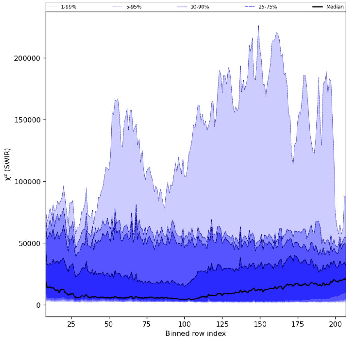
Figure 39: Along track statistics of " \chi^2 (SWIR)" for 2024-02-24 to 2024-02-26
