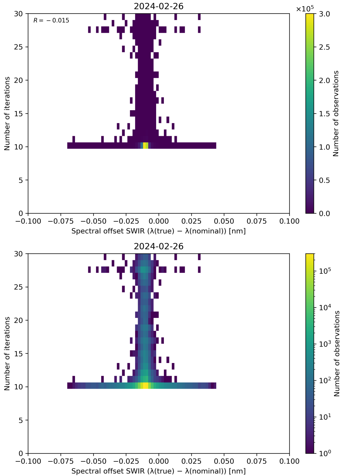
Figure 121: Scatter density plot of “Spectral offset SWIR ( \lambda(\text{true}) - \lambda(\text{nominal}) )” against “Number of iterations” for 2024-02-25 to 2024-02-27.
