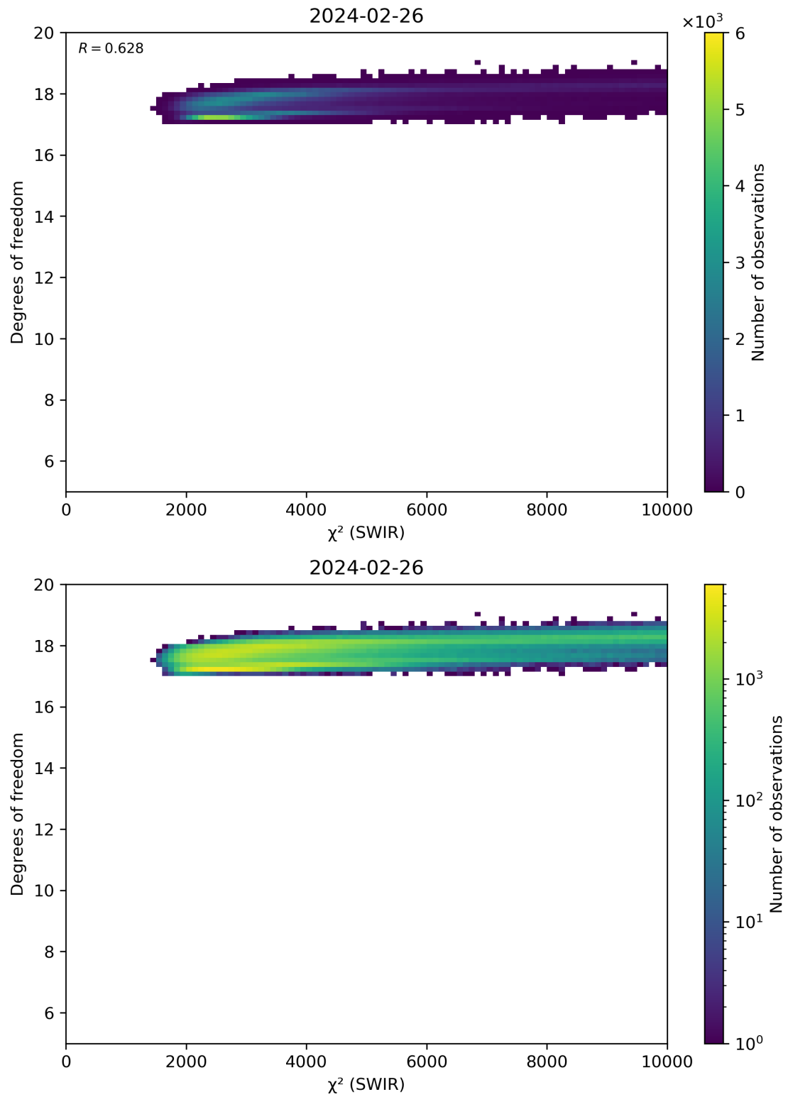
Figure 48: Scatter density plot of “ \chi^2 (SWIR)” against “Degrees of freedom” for 2024-02-25 to 2024-02-27.
