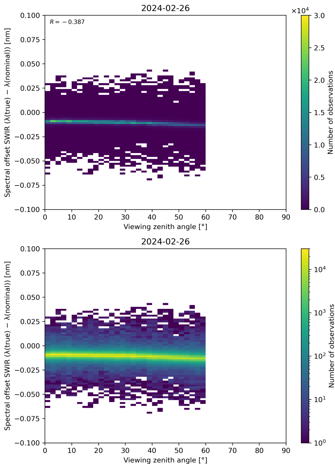
Figure 116: Scatter density plot of “Viewing zenith angle” against “Spectral offset SWIR ( \lambda(\text{true}) - \lambda(\text{nominal}) )” for 2024-02-25 to 2024-02-27.
