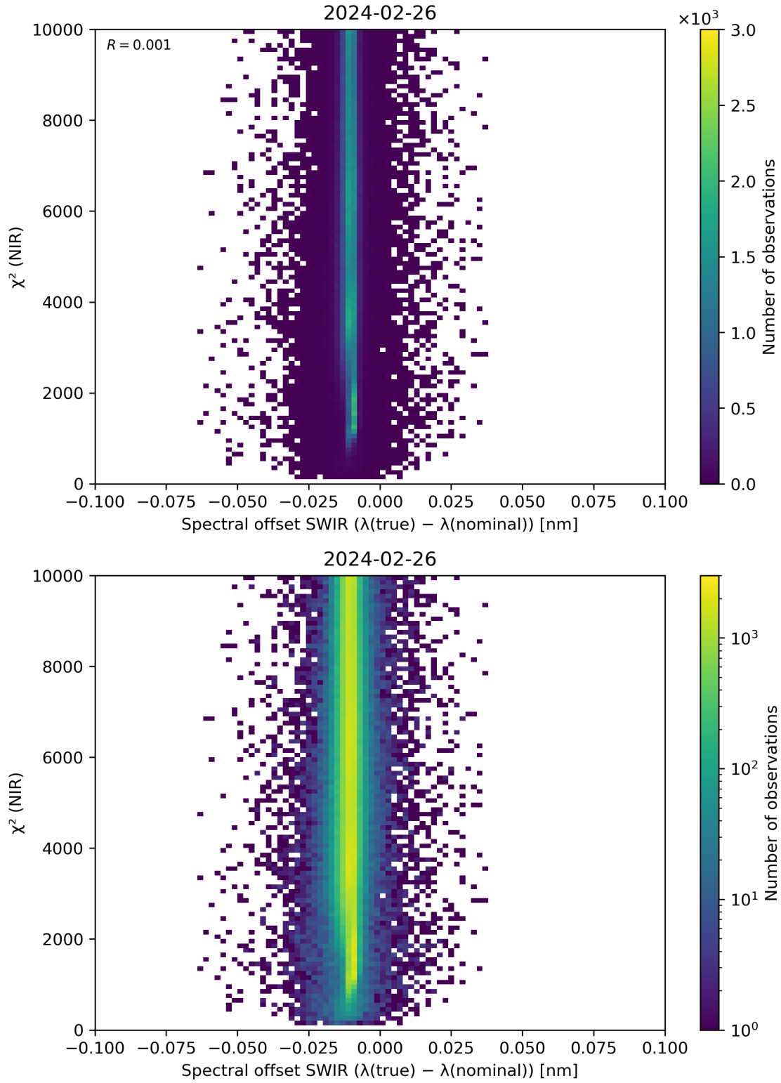
Figure 117: Scatter density plot of “Spectral offset SWIR ( \lambda(\text{true}) - \lambda(\text{nominal}) )” against “ \chi^2 (NIR)” for 2024-02-25 to 2024-02-27.
