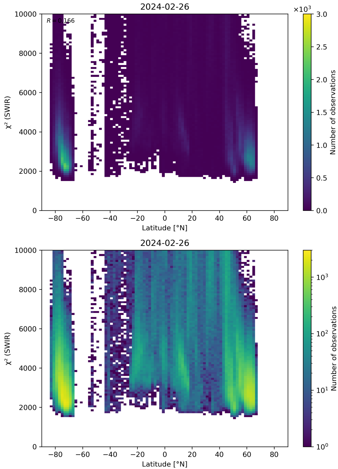
Figure 54: Scatter density plot of “Latitude” against “ \chi^2 (SWIR)” for 2024-02-25 to 2024-02-27.
