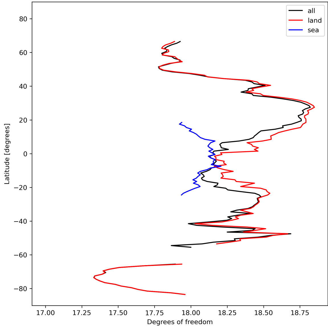
Figure 19: Zonal average of “Degrees of freedom” for 2024-02-25 to 2024-02-27.
