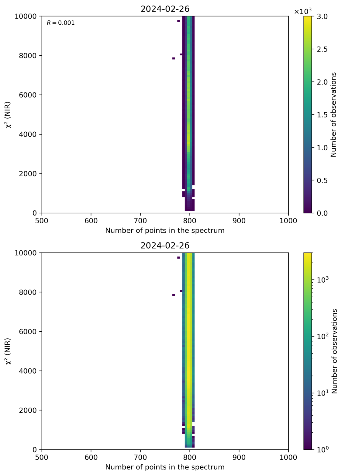
Figure 88: Scatter density plot of “Number of points in the spectrum” against “ \chi^2 (NIR)” for 2024-02-25 to 2024-02-27.
