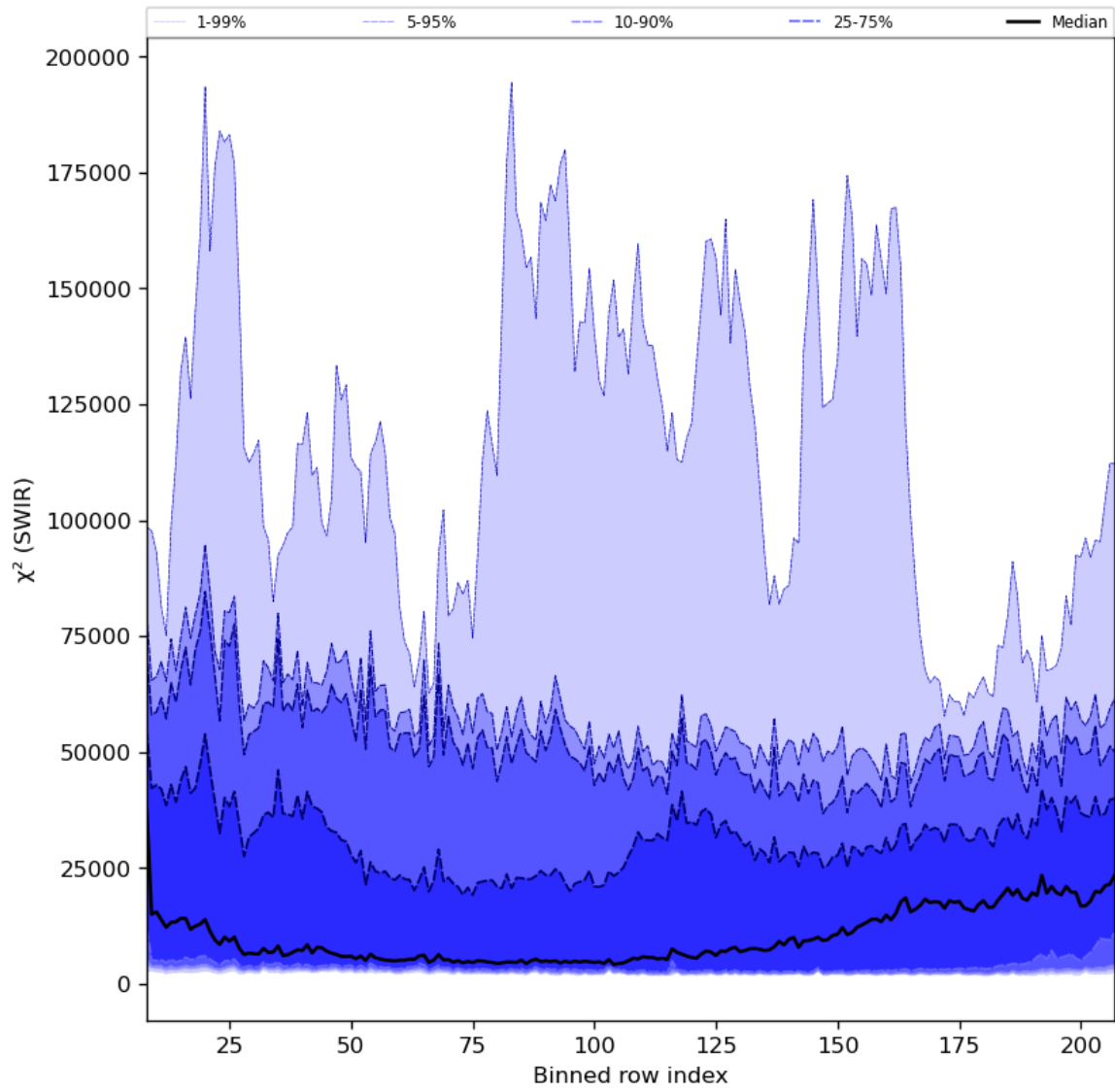
Figure 39: Along track statistics of “ \chi^2 (SWIR)” for 2024-02-25 to 2024-02-27
