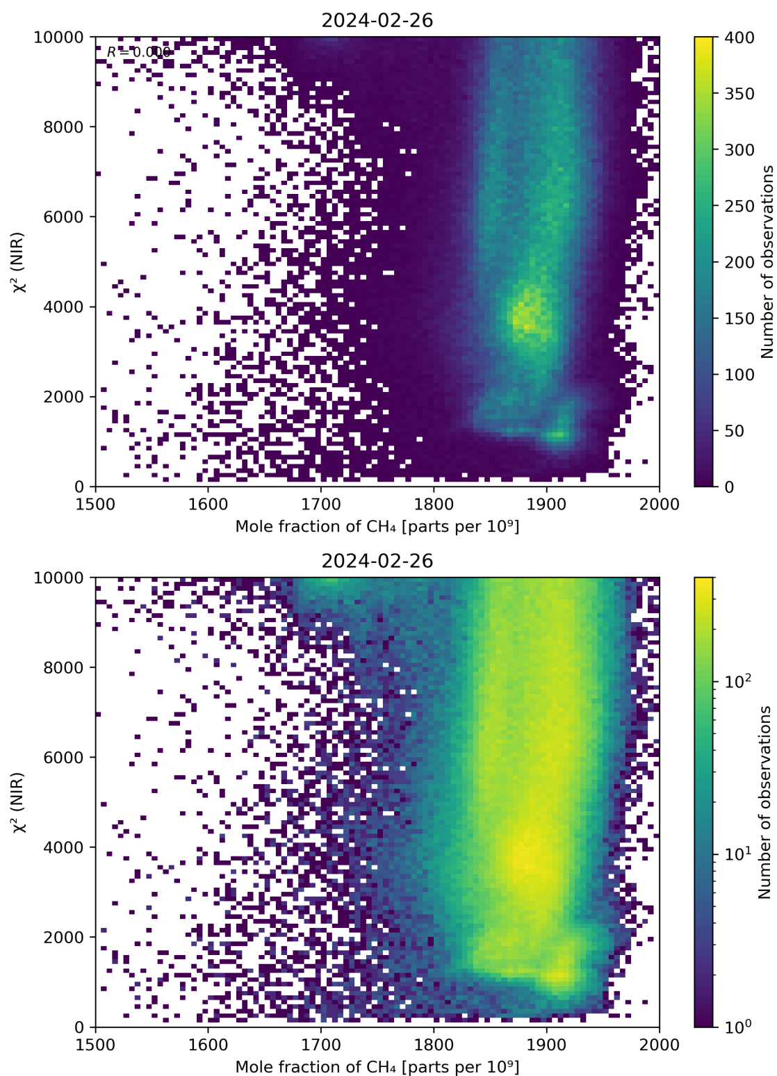
Figure 70: Scatter density plot of “Mole fraction of \text{CH}_4 ” against “ \chi^2 (NIR)” for 2024-02-25 to 2024-02-27.
