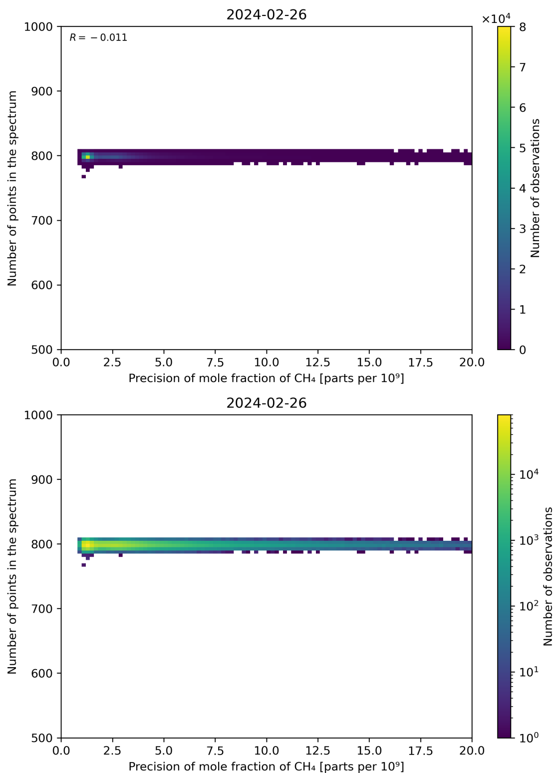
Figure 84: Scatter density plot of “Precision of mole fraction of CH 4 ” against “Number of points in the spectrum” for 2024-02-25 to 2024-02-27.
