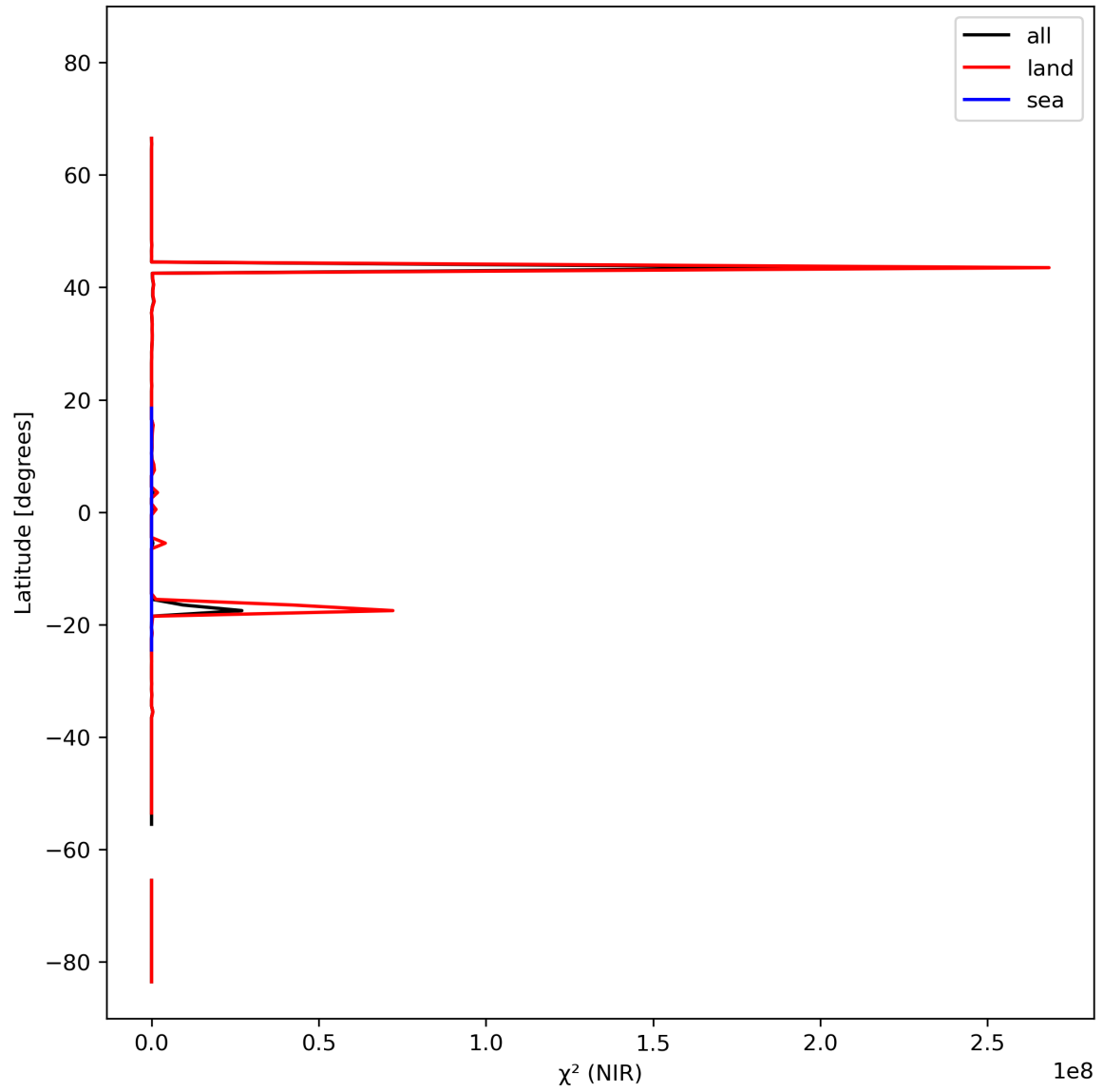
Figure 18: Zonal average of “ \chi^2 (NIR)” for 2024-02-25 to 2024-02-27.
