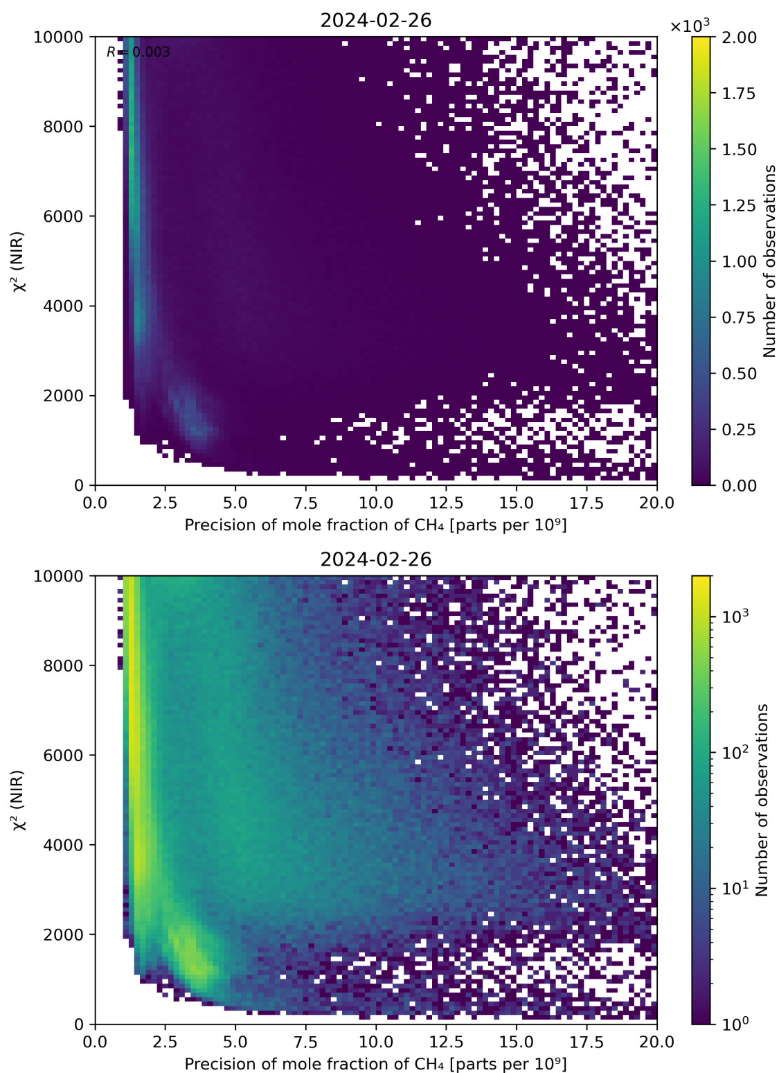
Figure 78: Scatter density plot of “Precision of mole fraction of CH 4 ” against “ \chi^2 (NIR)” for 2024-02-25 to 2024-02-27.
