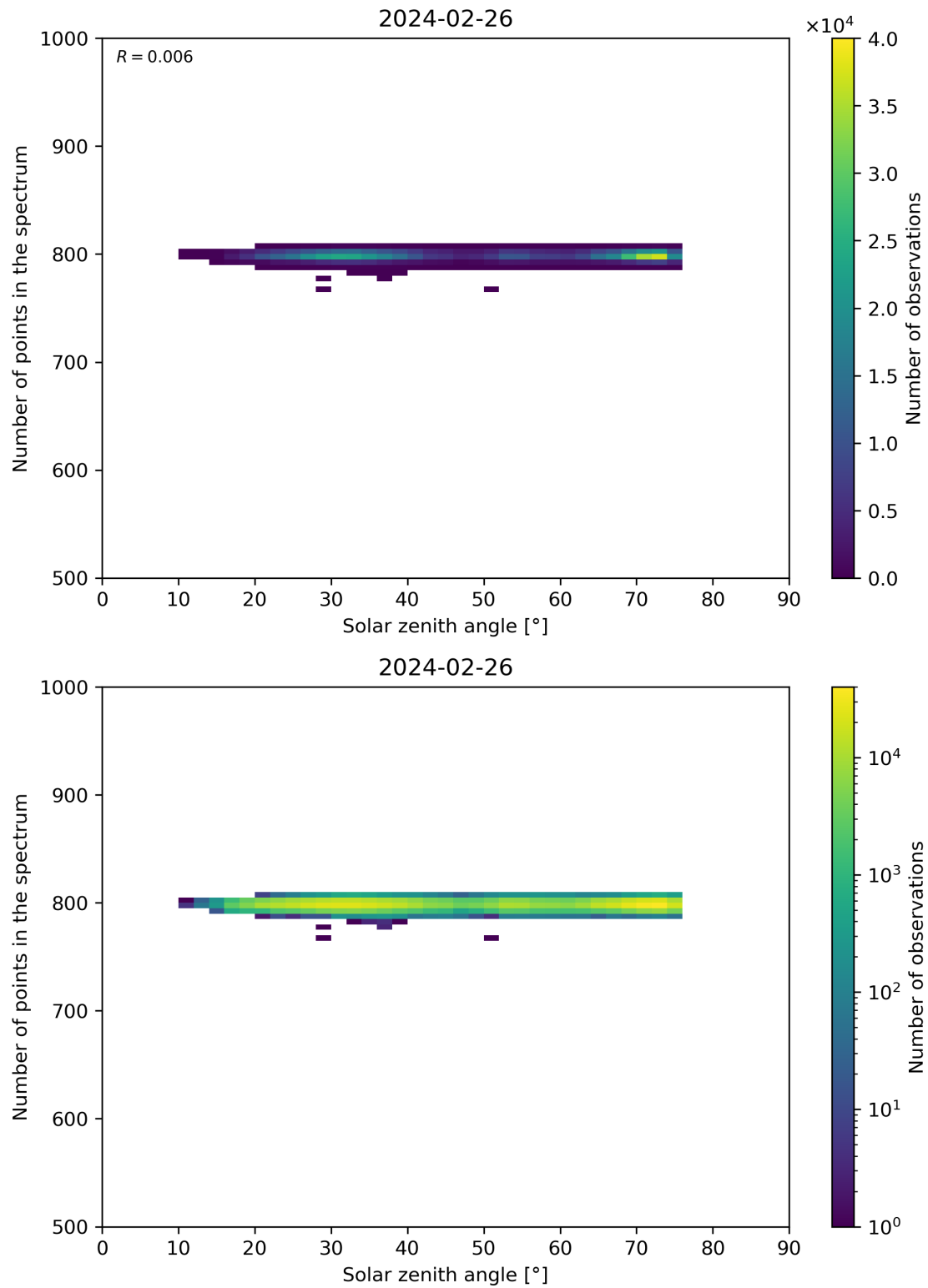
Figure 103: Scatter density plot of “Solar zenith angle” against “Number of points in the spectrum” for 2024-02-25 to 2024-02-27.
