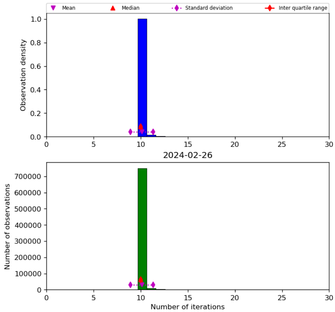
Figure 31: Histogram of “Number of iterations” for 2024-02-25 to 2024-02-27
