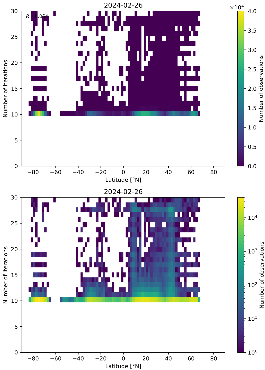
Figure 60: Scatter density plot of “Latitude” against “Number of iterations” for 2024-02-25 to 2024-02-27.
