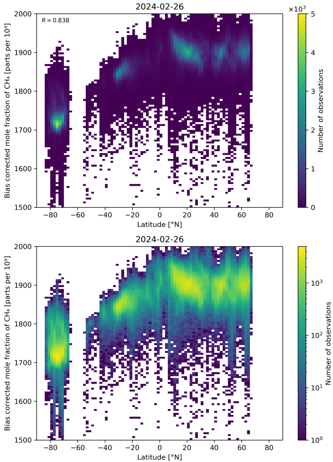
Figure 58: Scatter density plot of “Latitude” against “Bias corrected mole fraction of CH 4 ” for 2024-02-25 to 2024-02-27.
