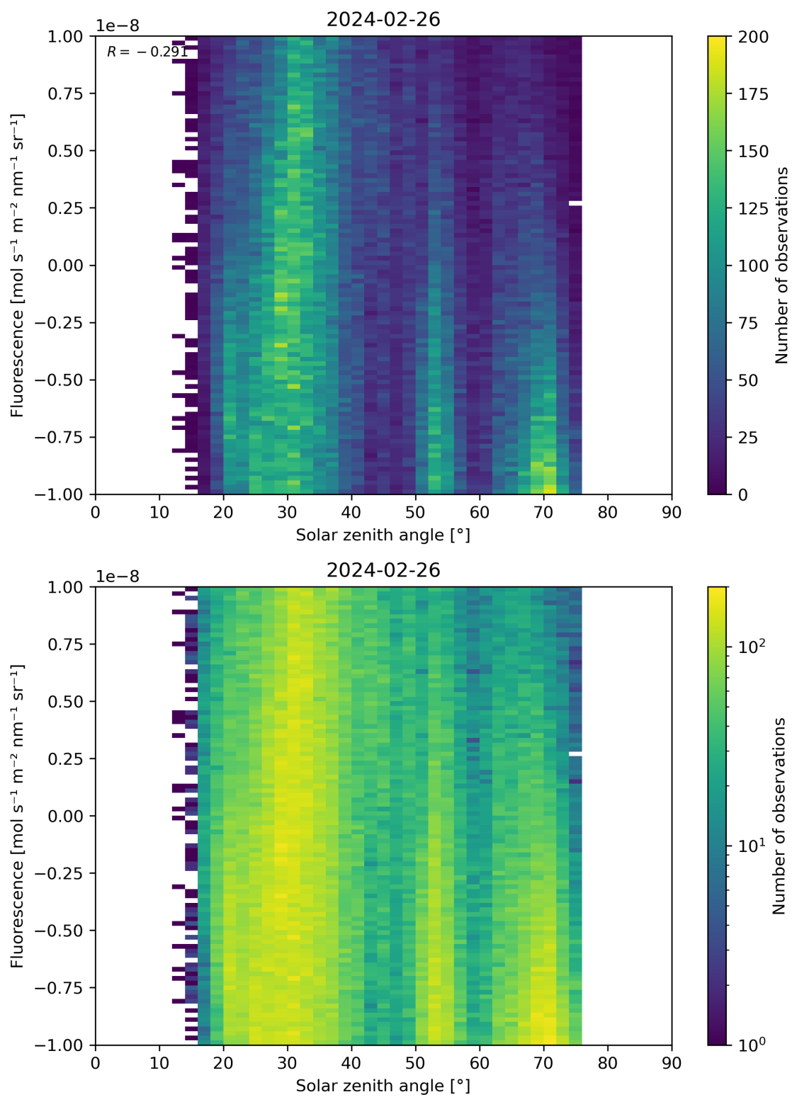
Figure 97: Scatter density plot of “Solar zenith angle” against “Fluorescence” for 2024-02-25 to 2024-02-27.
