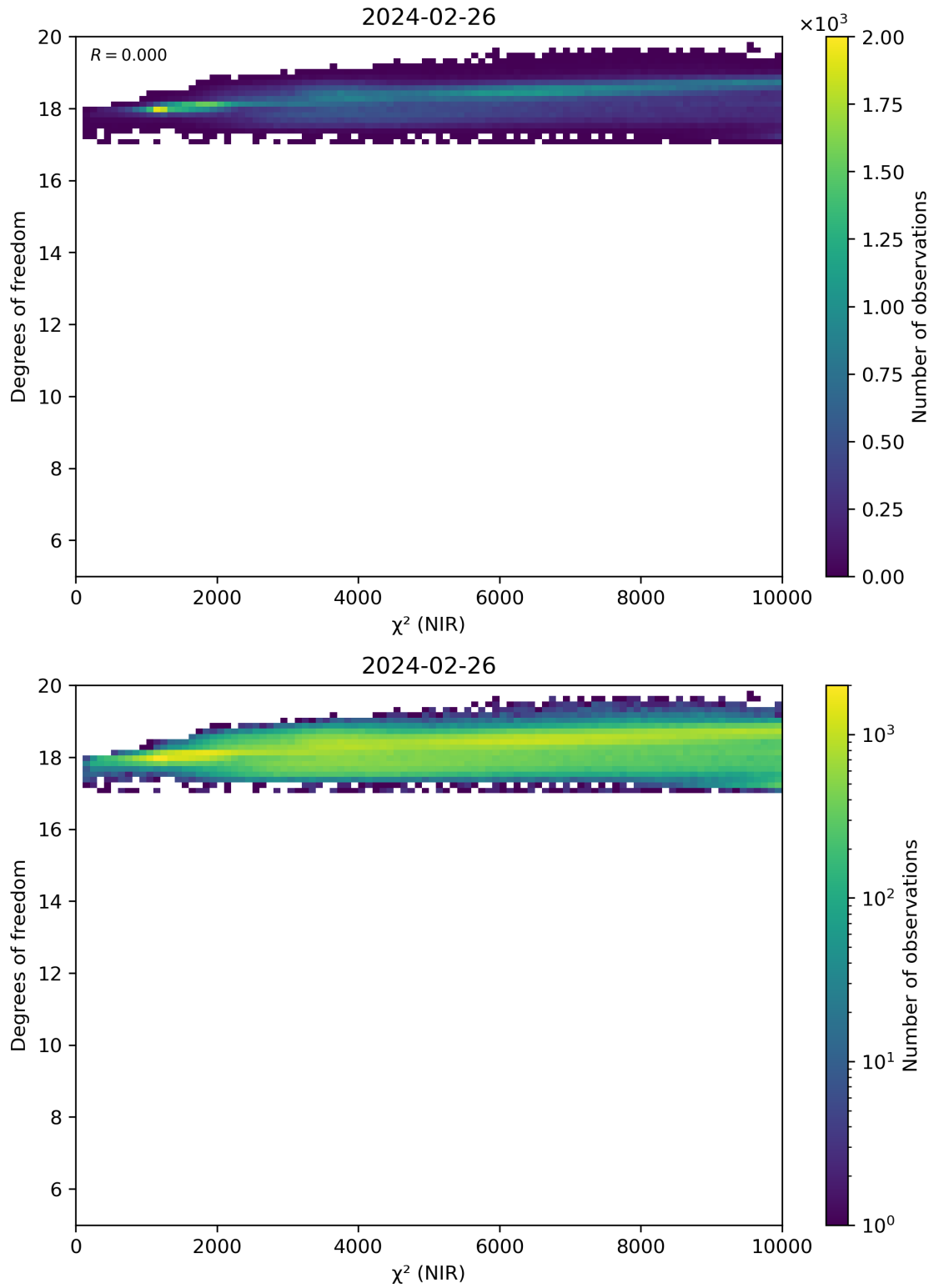
Figure 44: Scatter density plot of “ \chi^2 (NIR)” against “Degrees of freedom” for 2024-02-25 to 2024-02-27.
