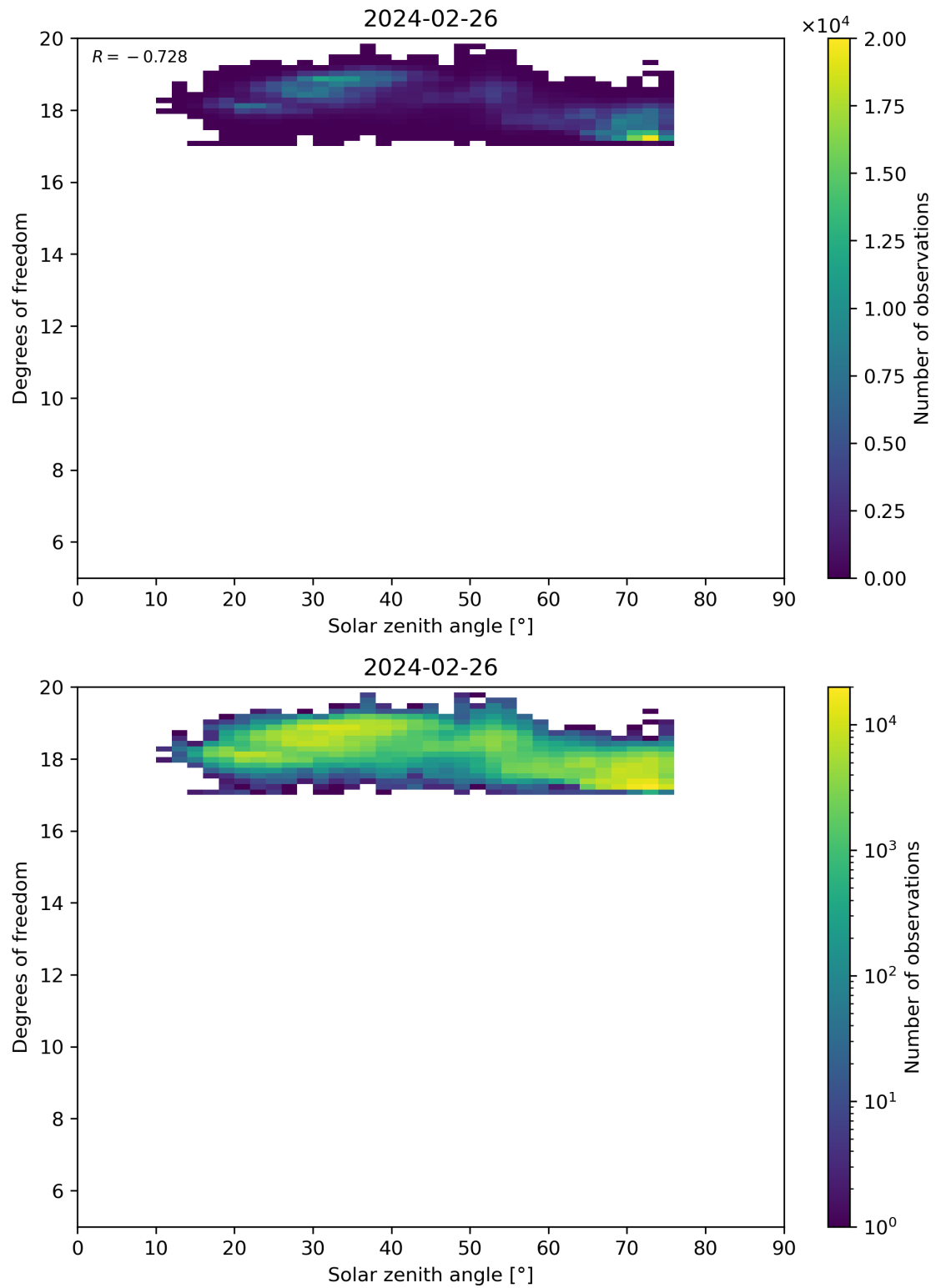
Figure 96: Scatter density plot of “Solar zenith angle” against “Degrees of freedom” for 2024-02-25 to 2024-02-27.
