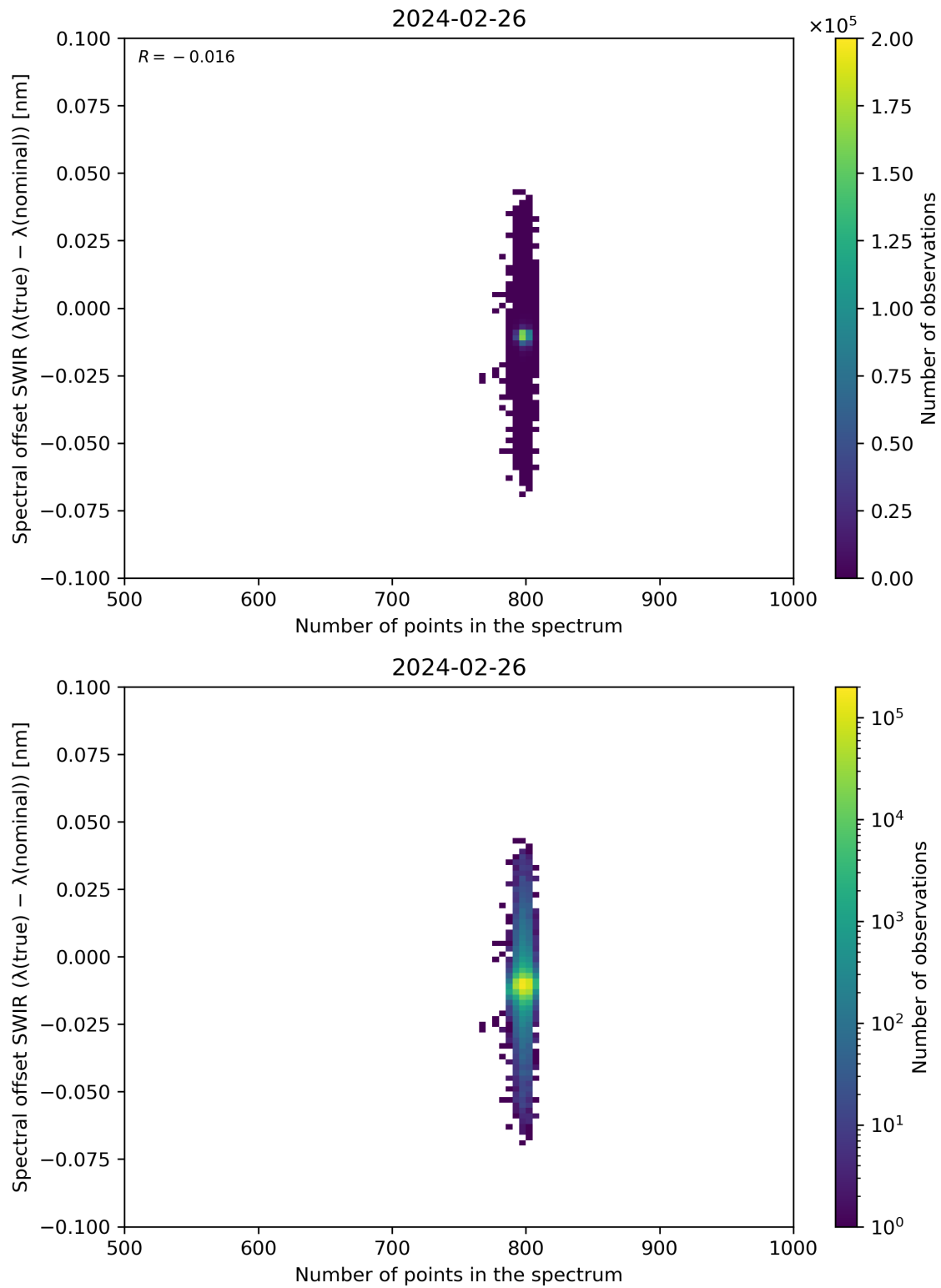
Figure 93: Scatter density plot of “Number of points in the spectrum” against “Spectral offset SWIR ( \lambda(\text{true}) - \lambda(\text{nominal}) )” for 2024-02-25 to 2024-02-27.
