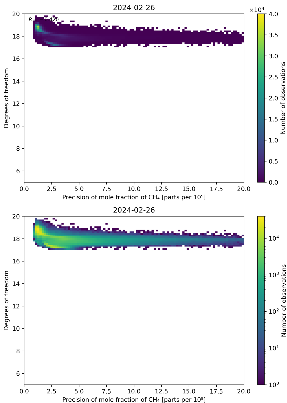
Figure 80: Scatter density plot of “Precision of mole fraction of CH 4 ” against “Degrees of freedom” for 2024-02-25 to 2024-02-27.
