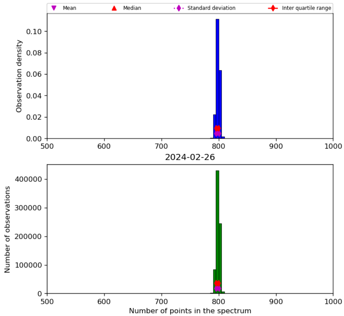
Figure 26: Histogram of “Number of points in the spectrum” for 2024-02-25 to 2024-02-27
