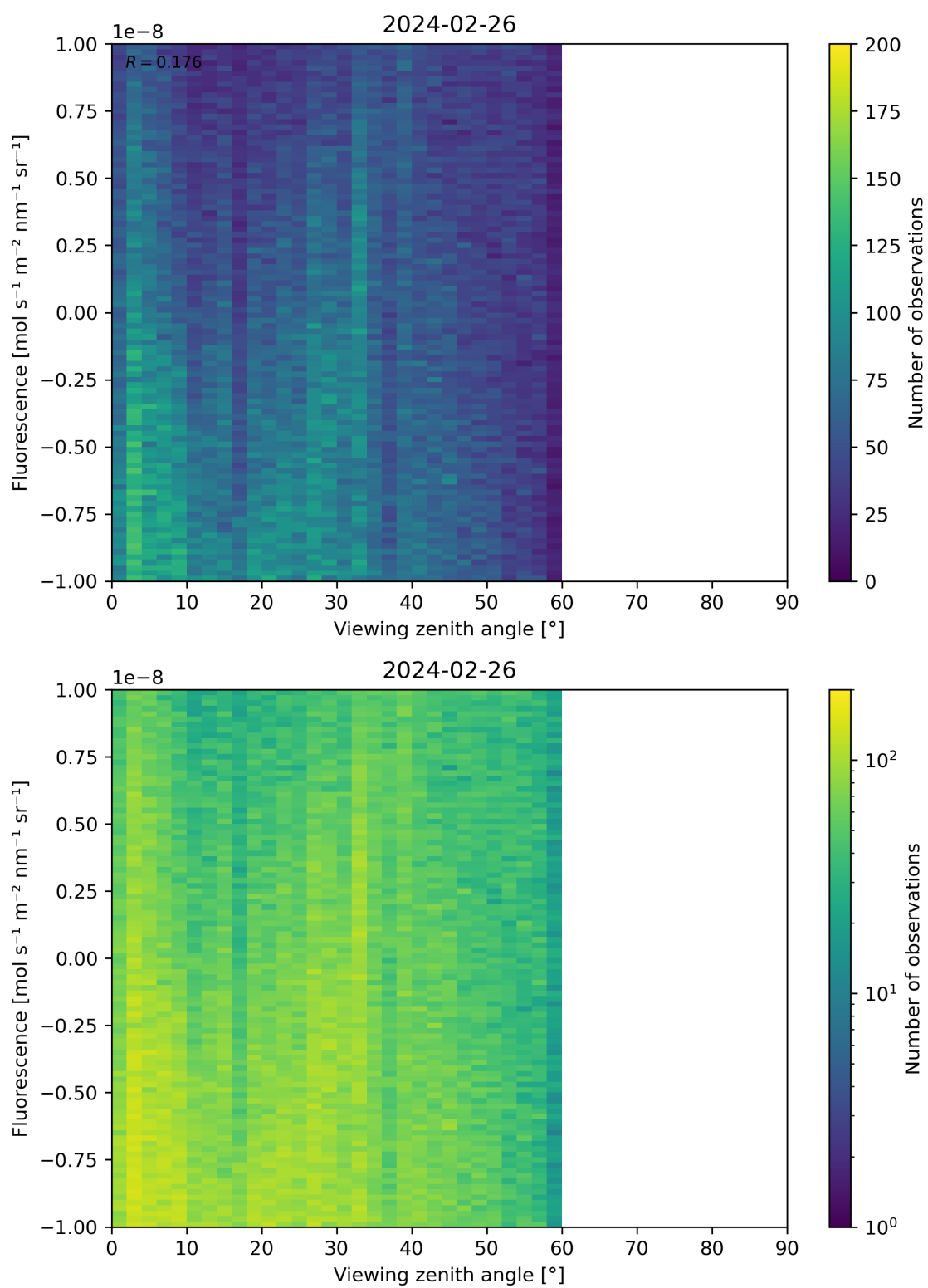
Figure 108: Scatter density plot of “Viewing zenith angle” against “Fluorescence” for 2024-02-25 to 2024-02-27.
