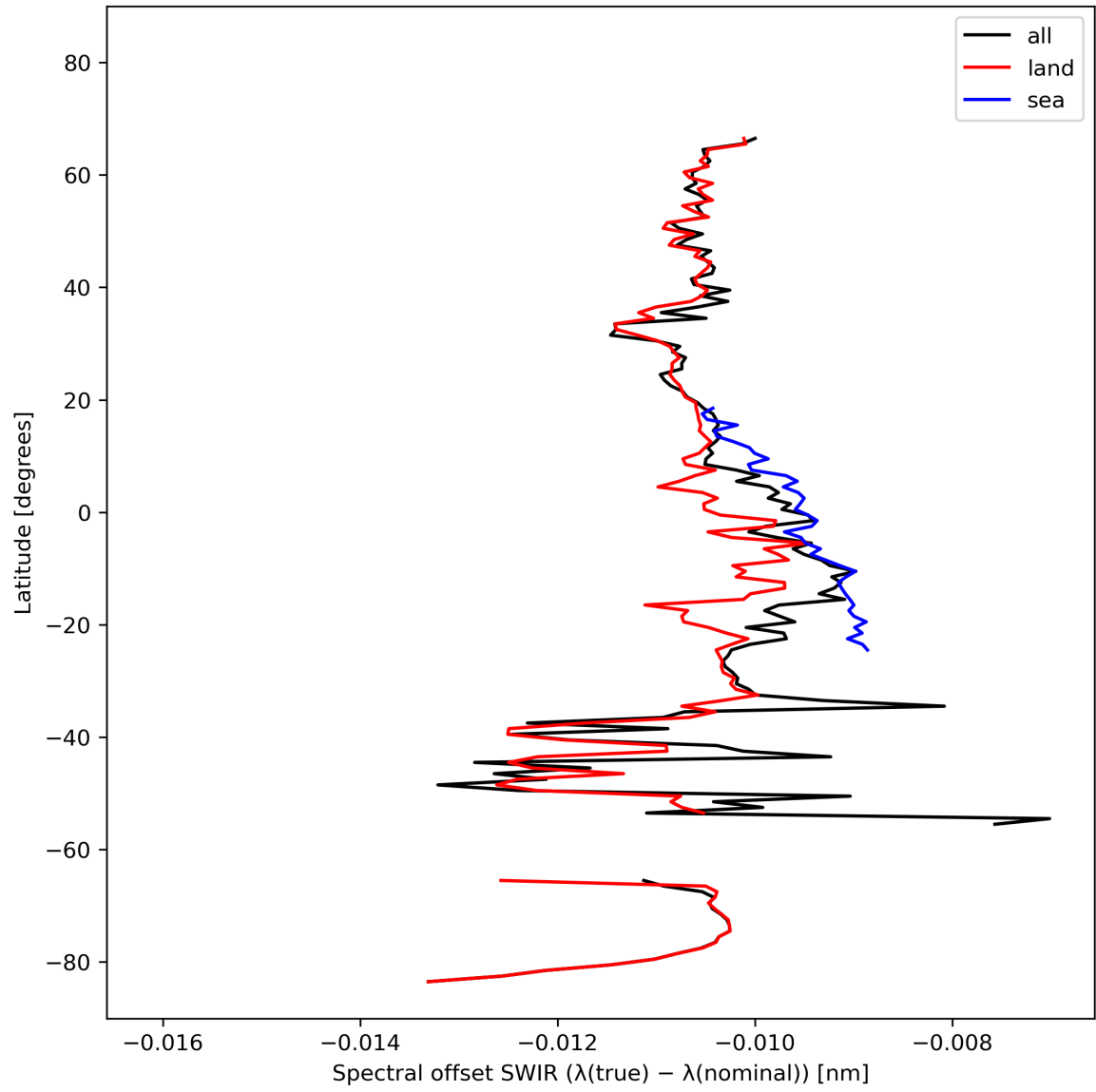
Figure 16: Zonal average of “Spectral offset SWIR ( \lambda(\text{true}) - \lambda(\text{nominal}) )” for 2024-02-25 to 2024-02-27.
