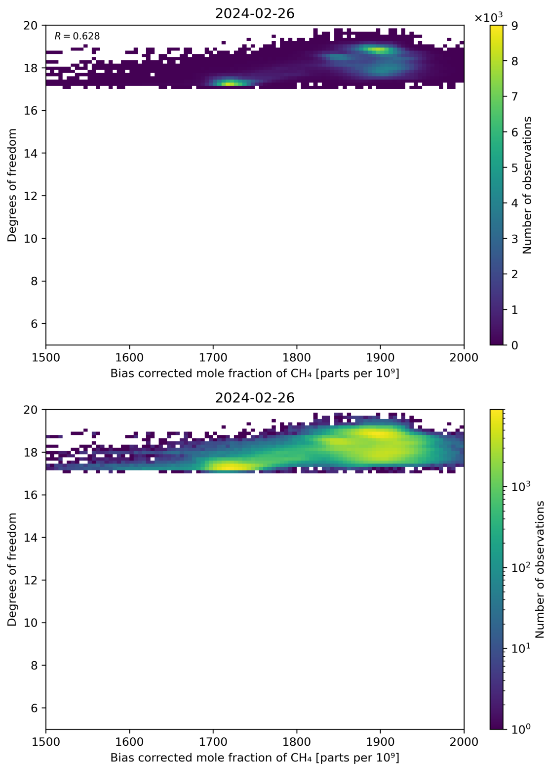
Figure 65: Scatter density plot of “Bias corrected mole fraction of CH 4 ” against “Degrees of freedom” for 2024-02-25 to 2024-02-27.
