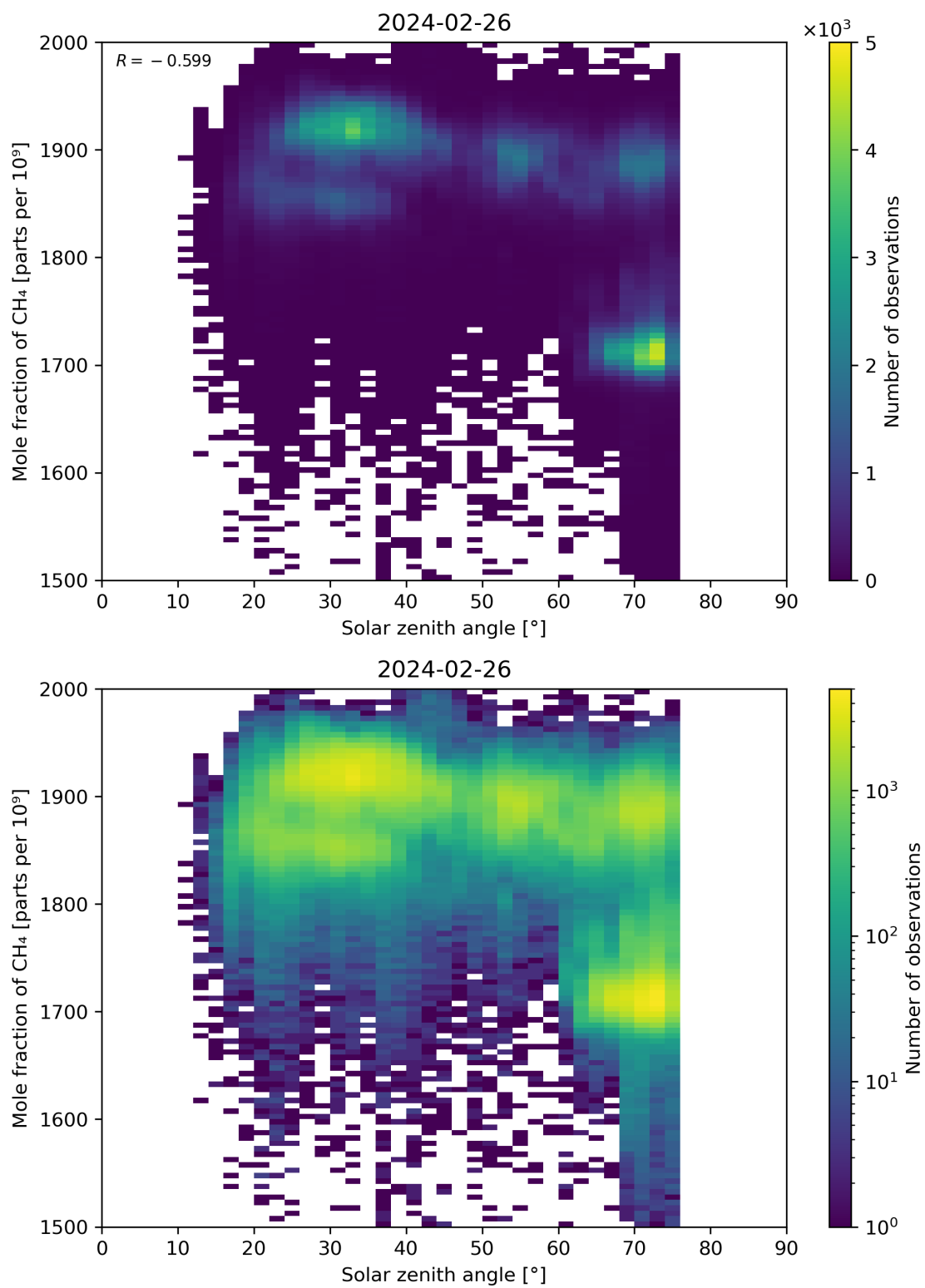
Figure 99: Scatter density plot of “Solar zenith angle” against “Mole fraction of CH 4 ” for 2024-02-25 to 2024-02-27.
