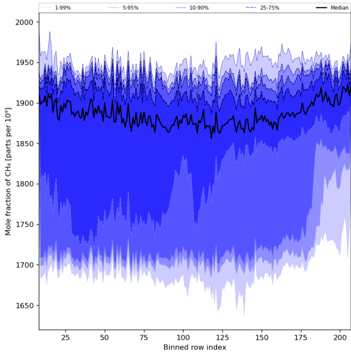
Figure 34: Along track statistics of “Mole fraction of CH 4 ” for 2024-02-25 to 2024-02-27
