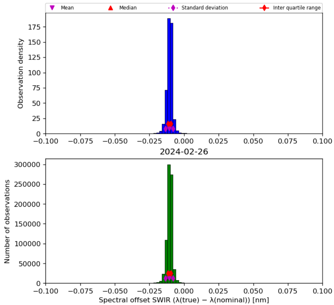
Figure 27: Histogram of “Spectral offset SWIR ( \lambda(\text{true}) - \lambda(\text{nominal}) )” for 2024-02-25 to 2024-02-27
