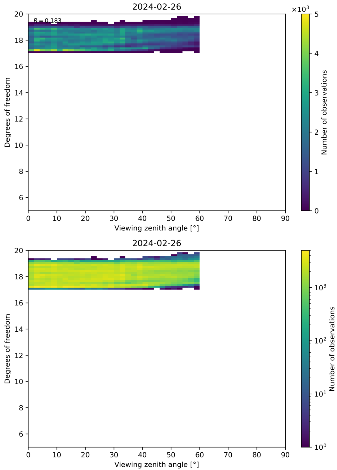
Figure 107: Scatter density plot of “Viewing zenith angle” against “Degrees of freedom” for 2024-02-25 to 2024-02-27.
