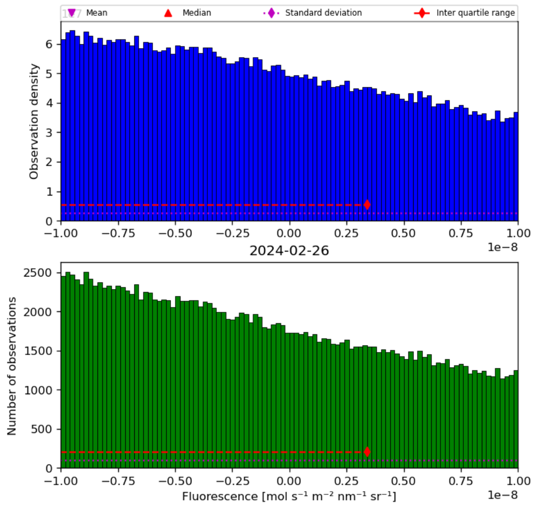
Figure 32: Histogram of “Fluorescence” for 2024-02-25 to 2024-02-27
