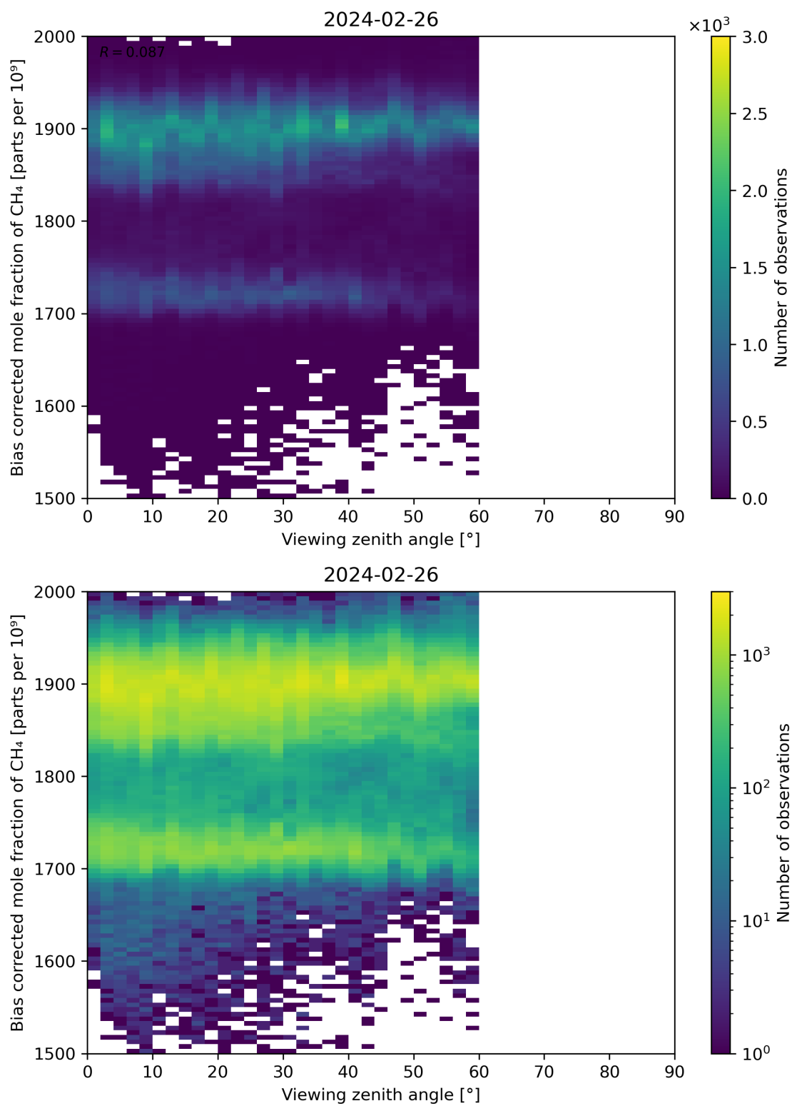
Figure 111: Scatter density plot of “Viewing zenith angle” against “Bias corrected mole fraction of \text{CH}_4 ” for 2024-02-25 to 2024-02-27.
