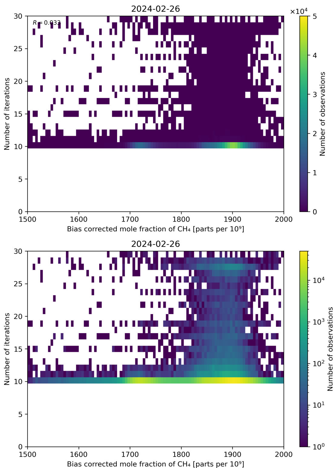
Figure 67: Scatter density plot of “Bias corrected mole fraction of \text{CH}_4 ” against “Number of iterations” for 2024-02-25 to 2024-02-27.
