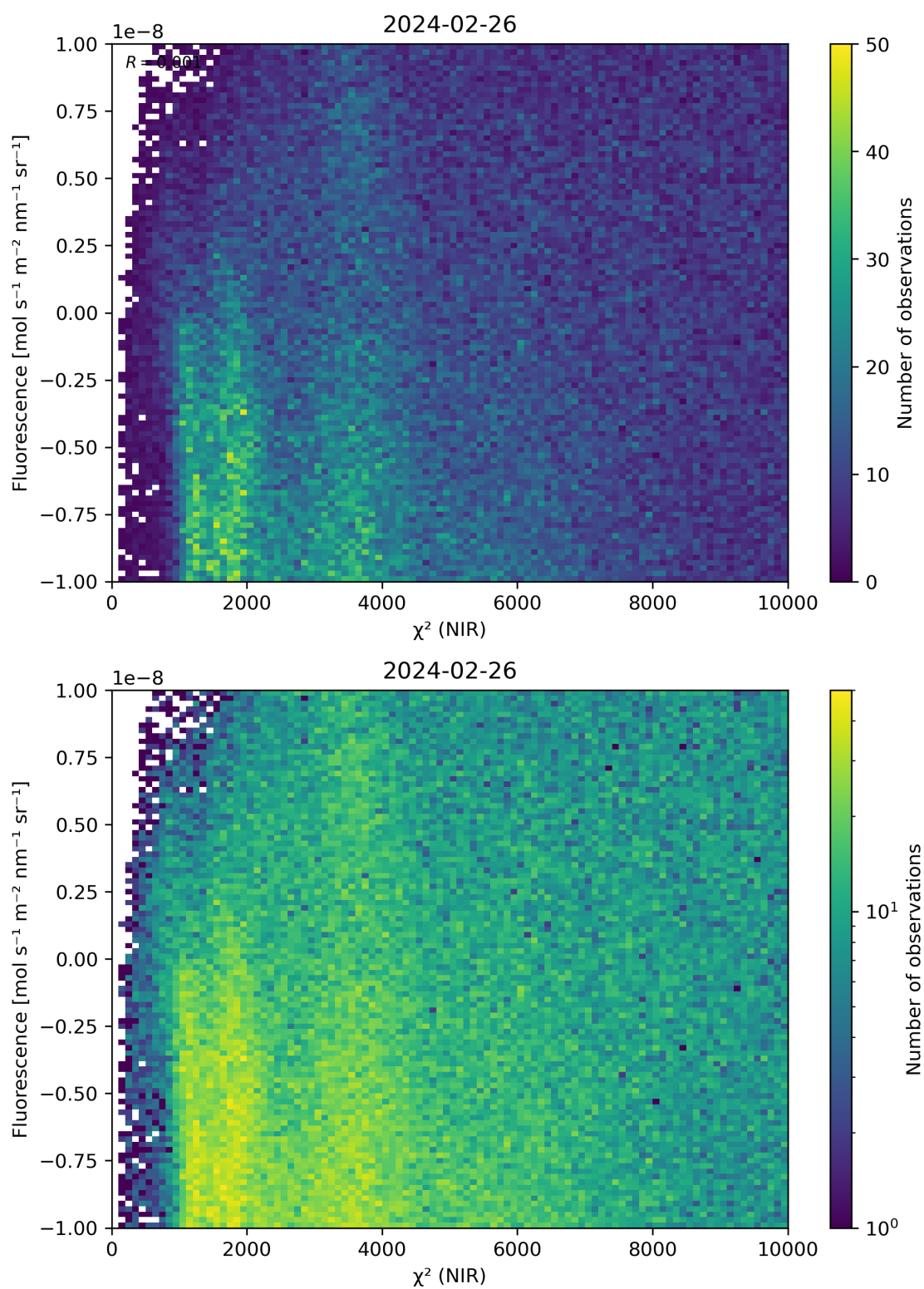
Figure 45: Scatter density plot of “ \chi^2 (NIR)” against “Fluorescence” for 2024-02-25 to 2024-02-27.
