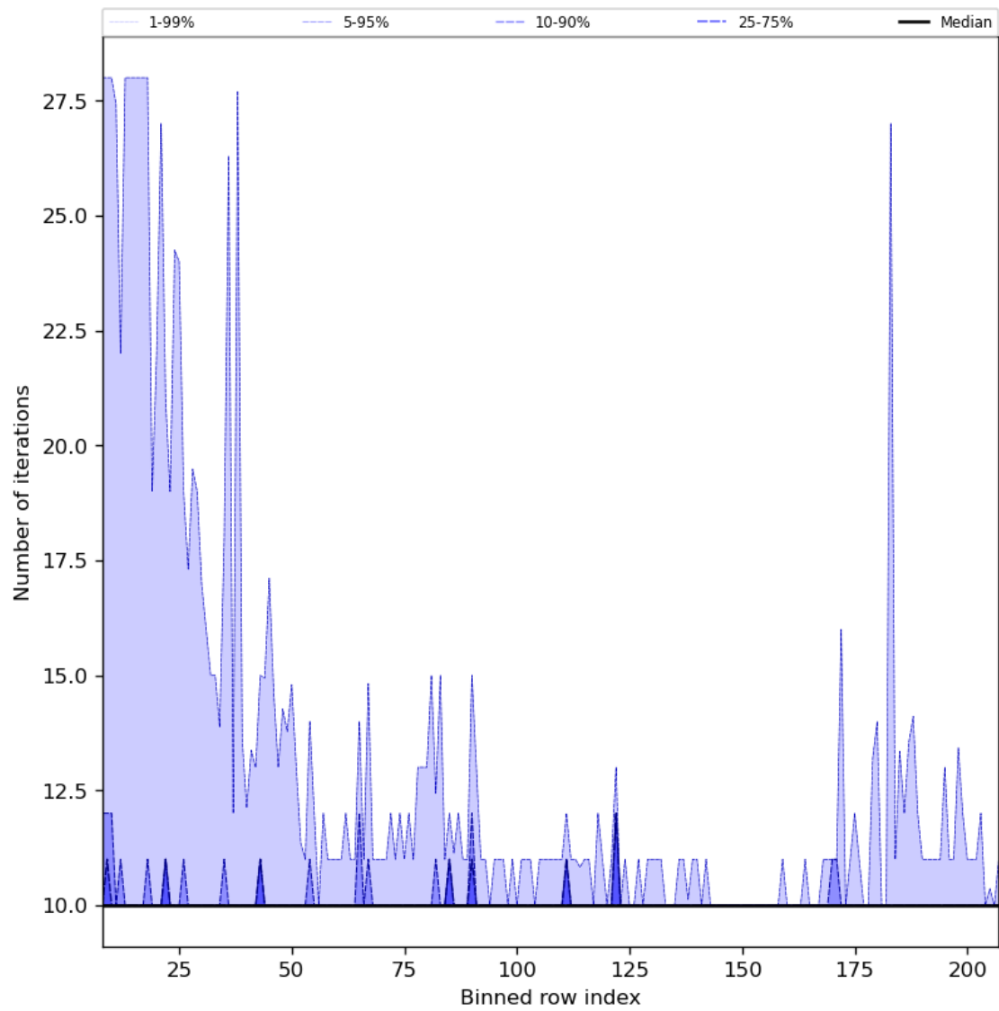
Figure 42: Along track statistics of “Number of iterations” for 2024-02-25 to 2024-02-27
