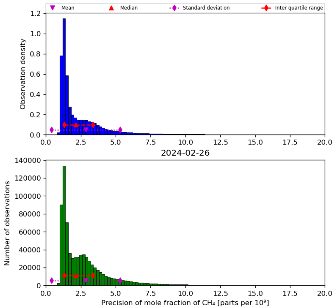
Figure 24: Histogram of “Precision of mole fraction of CH 4 ” for 2024-02-25 to 2024-02-27
