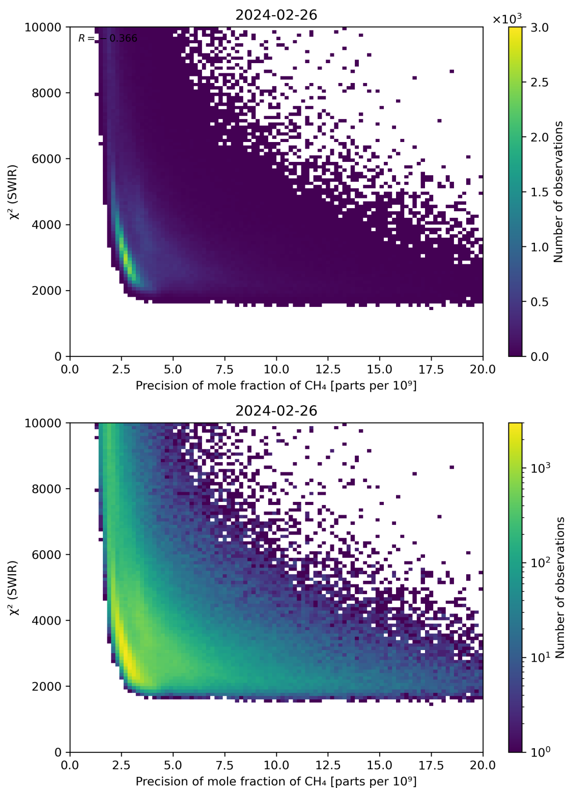
Figure 79: Scatter density plot of “Precision of mole fraction of \text{CH}_4 ” against “ \chi^2 (SWIR)” for 2024-02-25 to 2024-02-27.
