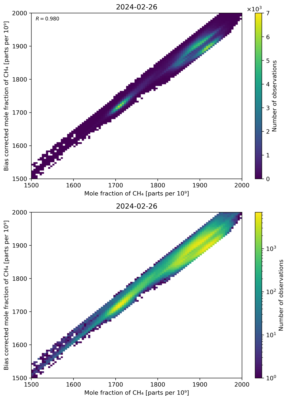
Figure 74: Scatter density plot of “Mole fraction of CH 4 ” against “Bias corrected mole fraction of CH 4 ” for 2024-02-25 to 2024-02-27.
