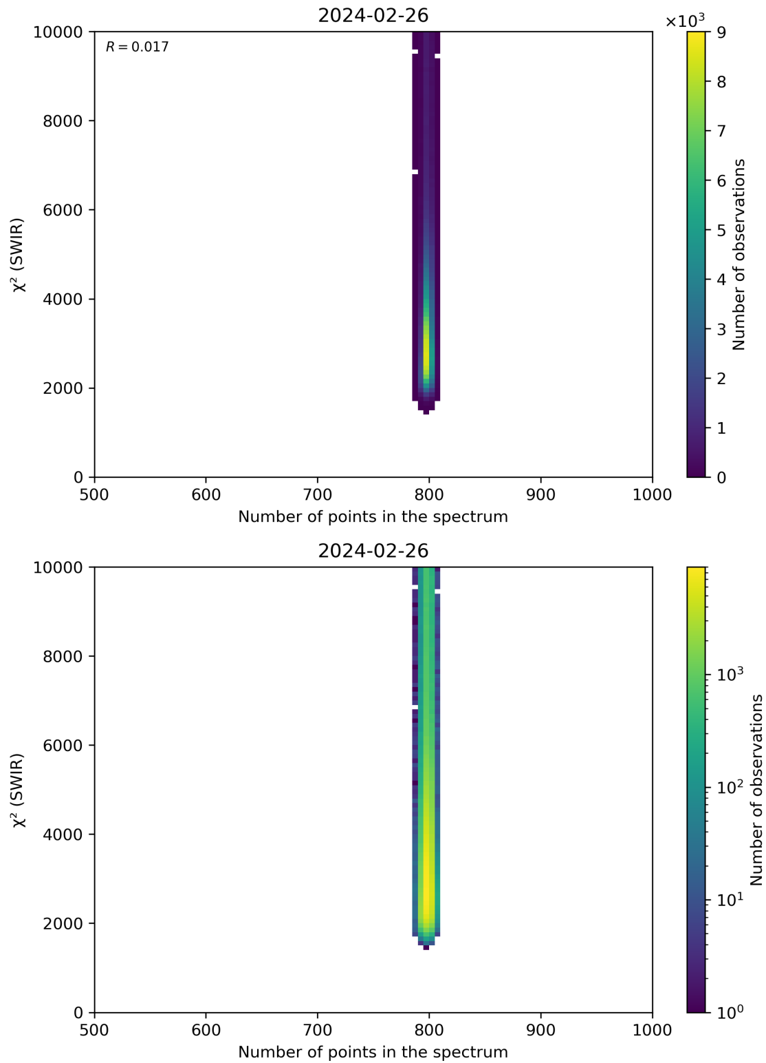
Figure 89: Scatter density plot of “Number of points in the spectrum” against “ \chi^2 (SWIR)” for 2024-02-25 to 2024-02-27.
