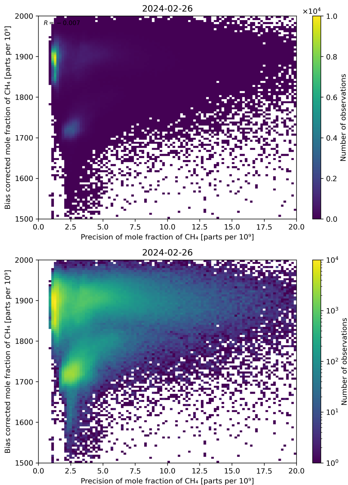
Figure 82: Scatter density plot of “Precision of mole fraction of \text{CH}_4 ” against “Bias corrected mole fraction of \text{CH}_4 ” for 2024-02-25 to 2024-02-27.
