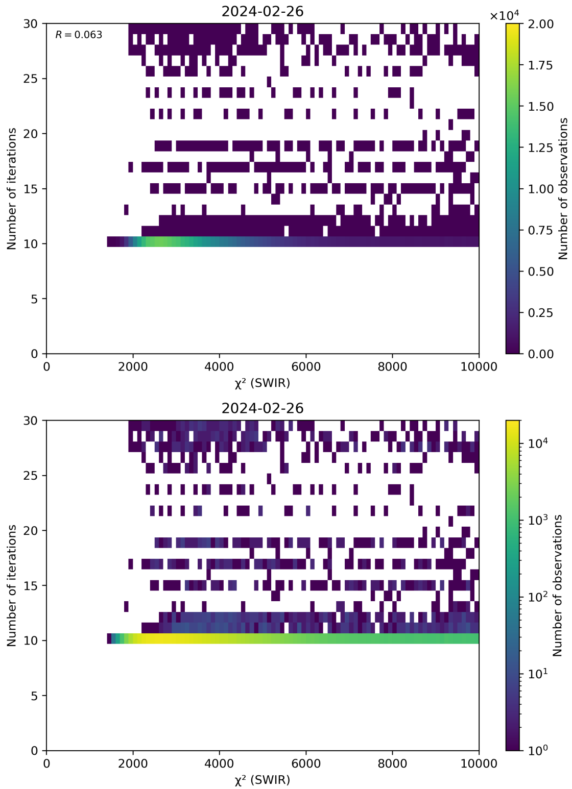
Figure 50: Scatter density plot of “ \chi^2 (SWIR)” against “Number of iterations” for 2024-02-25 to 2024-02-27.
