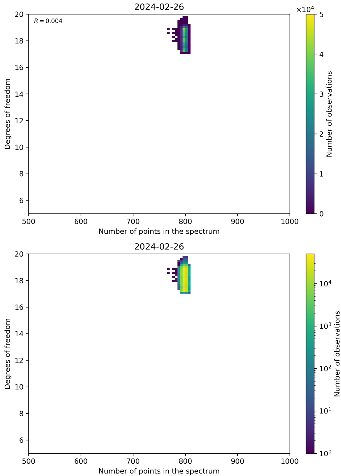
Figure 90: Scatter density plot of “Number of points in the spectrum” against “Degrees of freedom” for 2024-02-25 to 2024-02-27.
