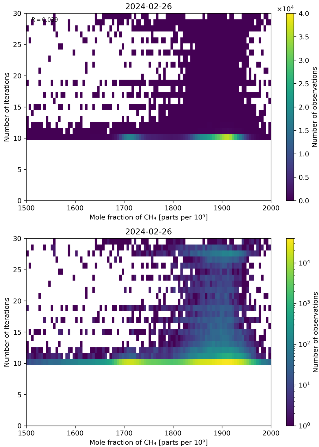
Figure 76: Scatter density plot of “Mole fraction of CH 4 ” against “Number of iterations” for 2024-02-25 to 2024-02-27.
