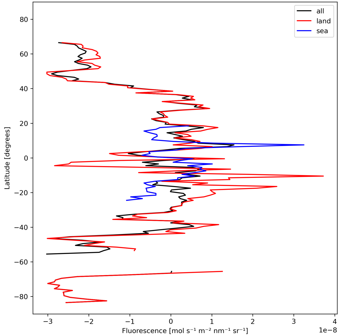
Figure 21: Zonal average of “Fluorescence” for 2024-02-25 to 2024-02-27.
