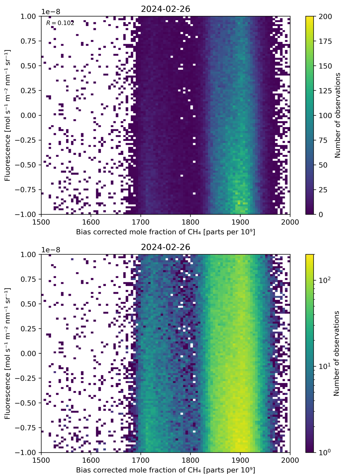
Figure 66: Scatter density plot of “Bias corrected mole fraction of \text{CH}_4 ” against “Fluorescence” for 2024-02-25 to 2024-02-27.
