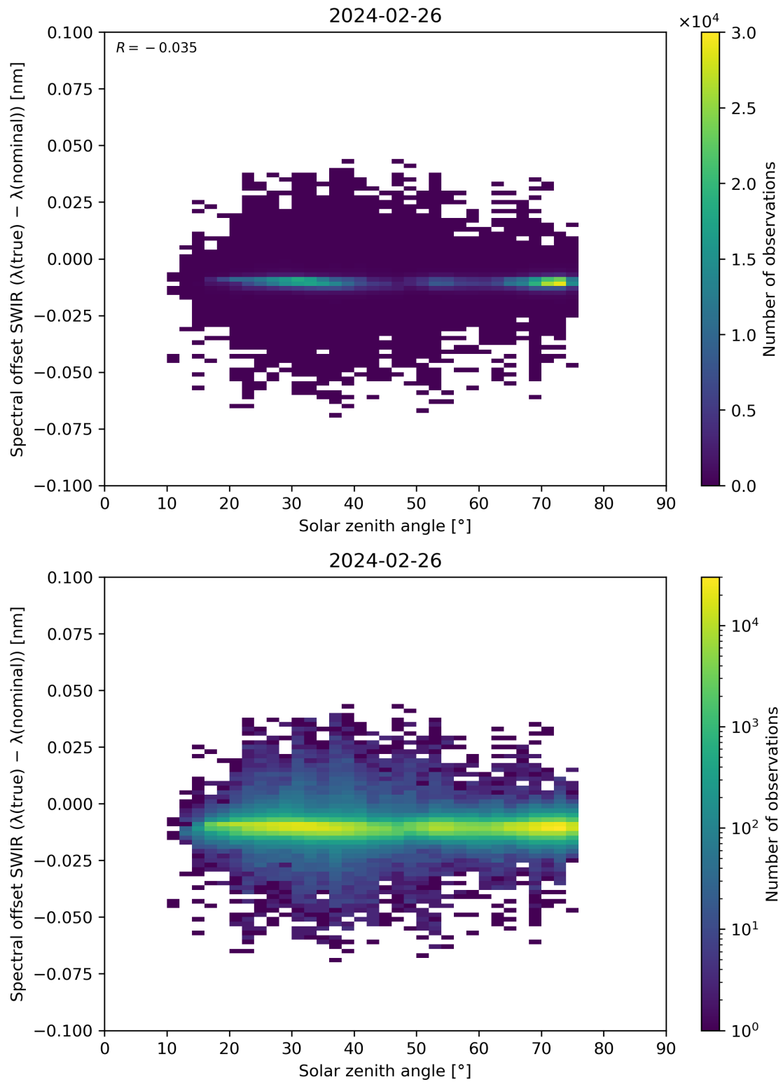
Figure 104: Scatter density plot of “Solar zenith angle” against “Spectral offset SWIR ( \lambda(\text{true}) - \lambda(\text{nominal}) )” for 2024-02-25 to 2024-02-27.
