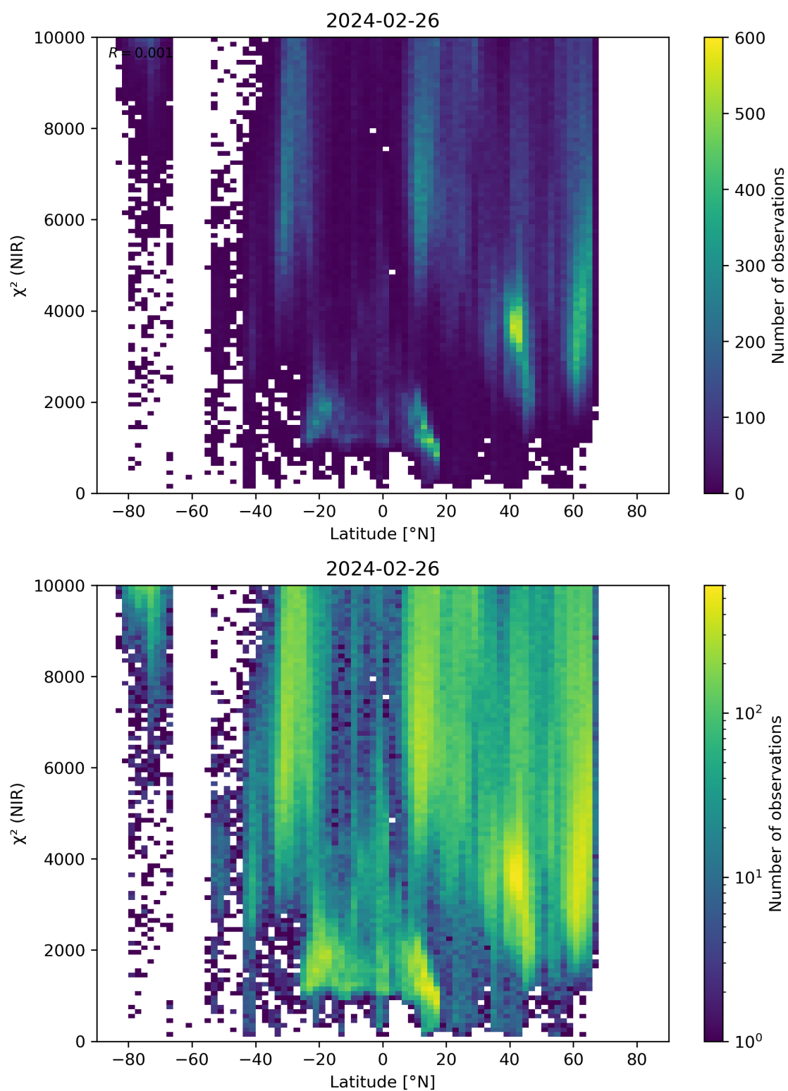
Figure 53: Scatter density plot of “Latitude” against “ \chi^2 (NIR)” for 2024-02-25 to 2024-02-27.
