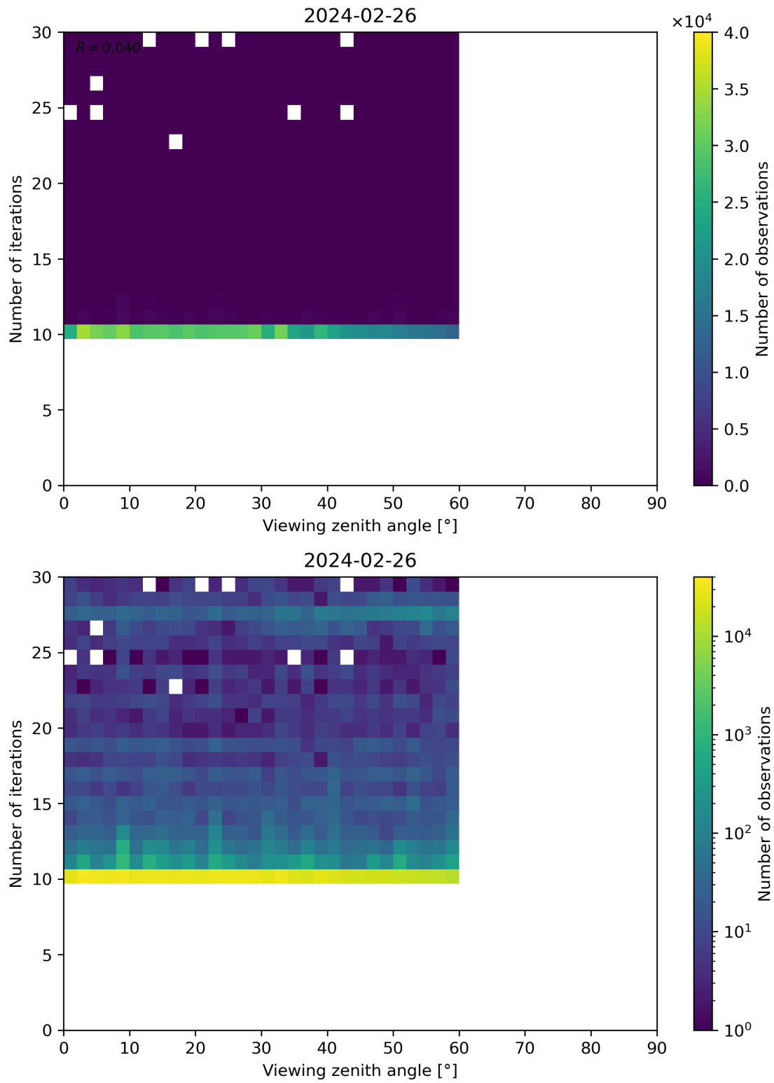
Figure 113: Scatter density plot of “Viewing zenith angle” against “Number of iterations” for 2024-02-25 to 2024-02-27.
