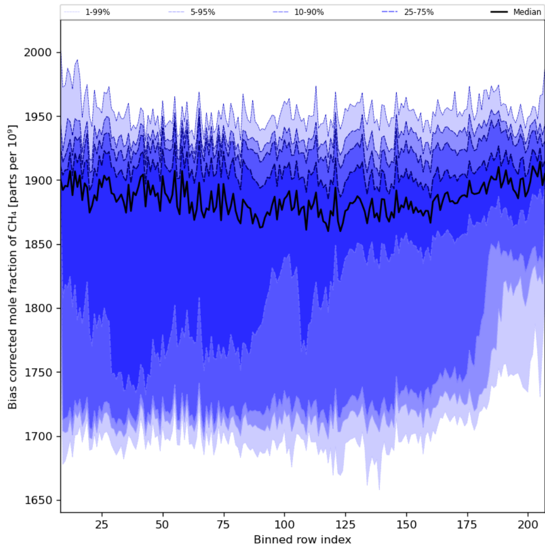
Figure 36: Along track statistics of “Bias corrected mole fraction of CH 4 ” for 2024-02-25 to 2024-02-27
