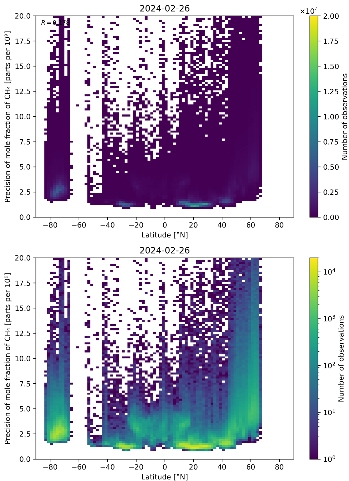
Figure 59: Scatter density plot of “Latitude” against “Precision of mole fraction of CH 4 ” for 2024-02-25 to 2024-02-27.
