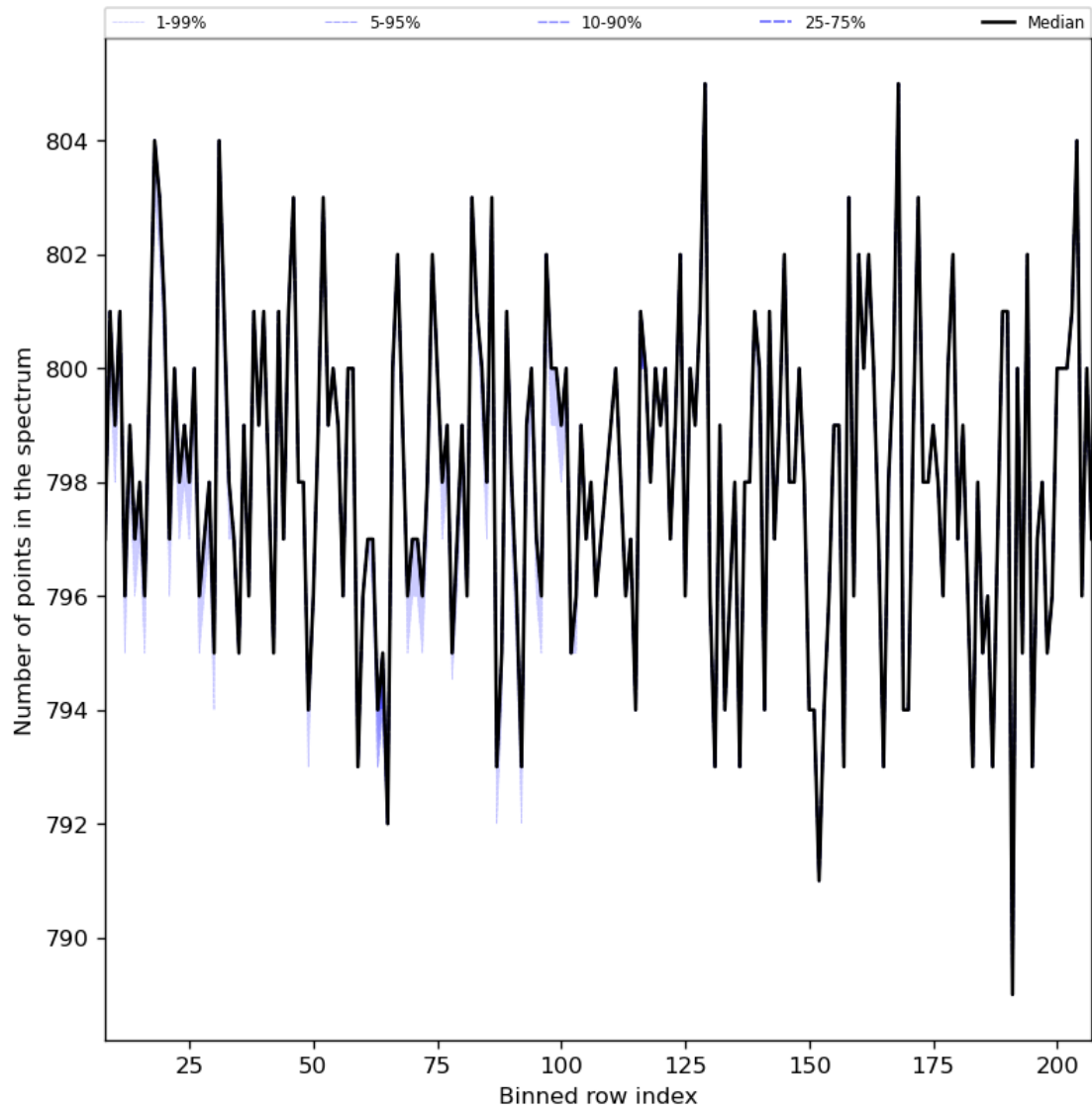
Figure 37: Along track statistics of “Number of points in the spectrum” for 2024-02-25 to 2024-02-27
