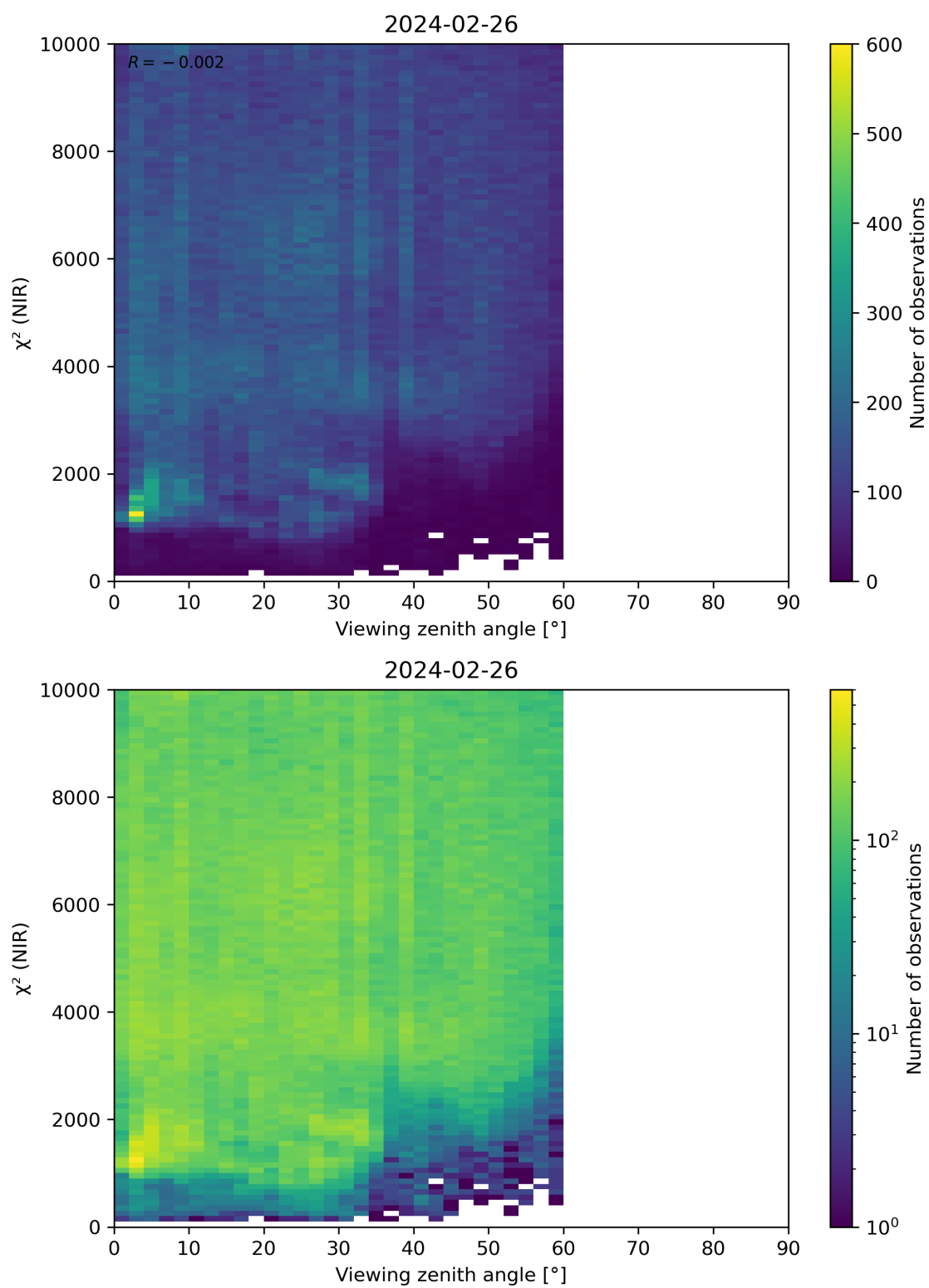
Figure 105: Scatter density plot of “Viewing zenith angle” against “ \chi^2 (NIR)” for 2024-02-25 to 2024-02-27.
