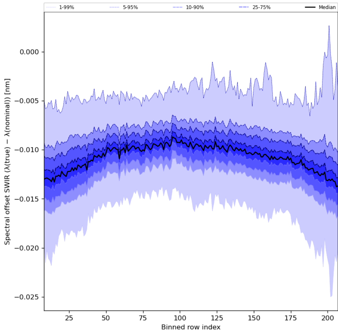
Figure 38: Along track statistics of “Spectral offset SWIR ( \lambda(\text{true}) - \lambda(\text{nominal}) )” for 2024-02-25 to 2024-02-27
