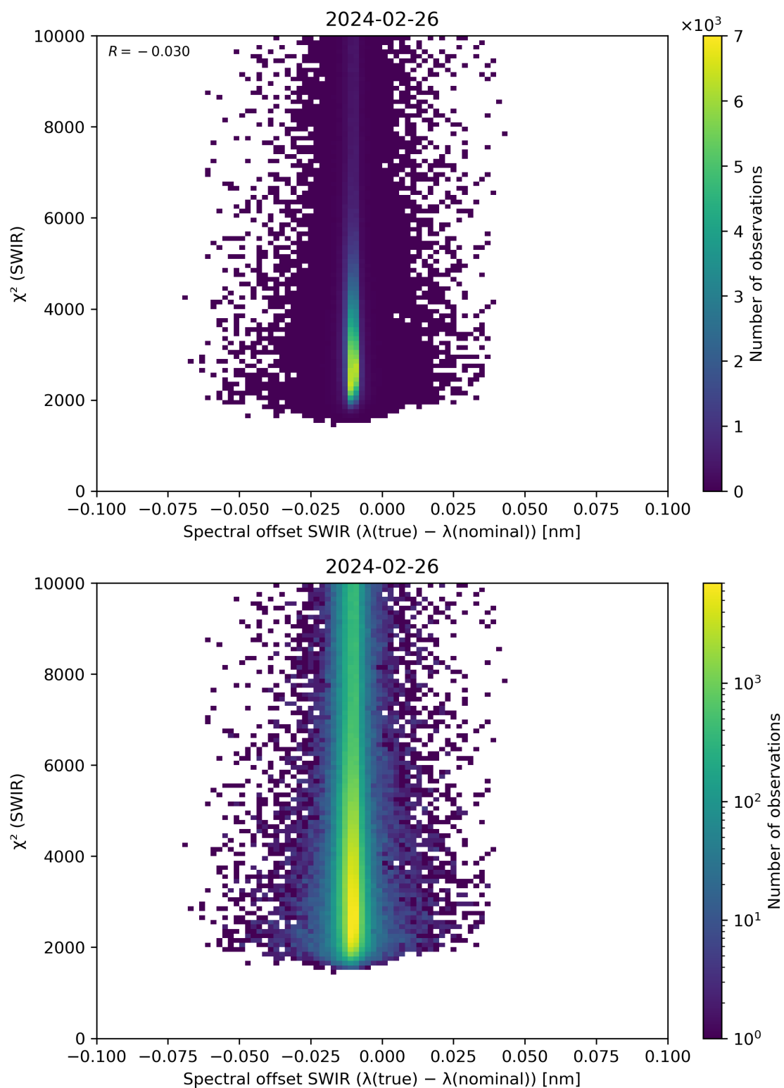
Figure 118: Scatter density plot of “Spectral offset SWIR ( \lambda(\text{true}) - \lambda(\text{nominal}) )” against “ \chi^2 (SWIR)” for 2024-02-25 to 2024-02-27.
