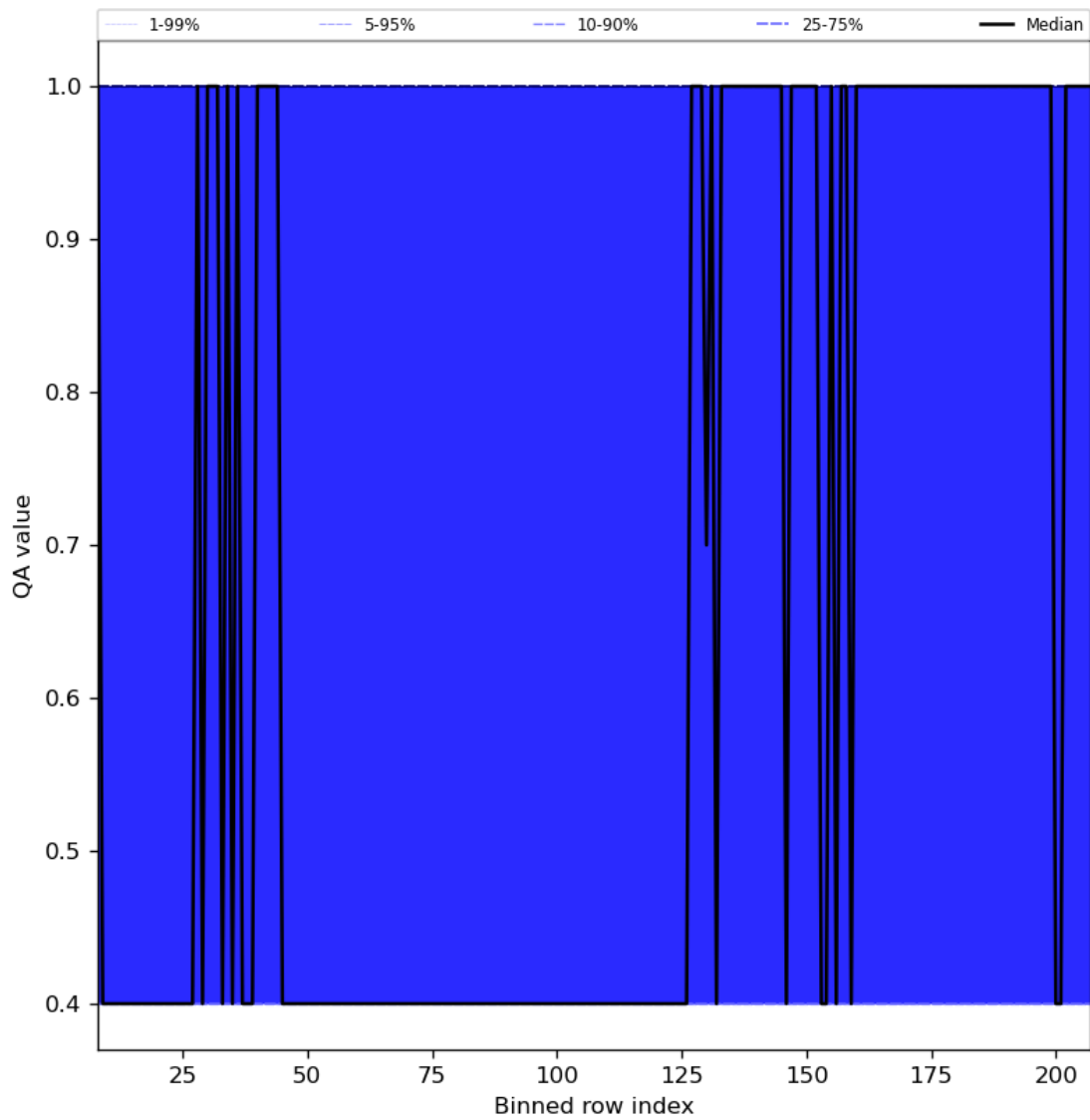
Figure 33: Along track statistics of “QA value” for 2024-02-25 to 2024-02-27
