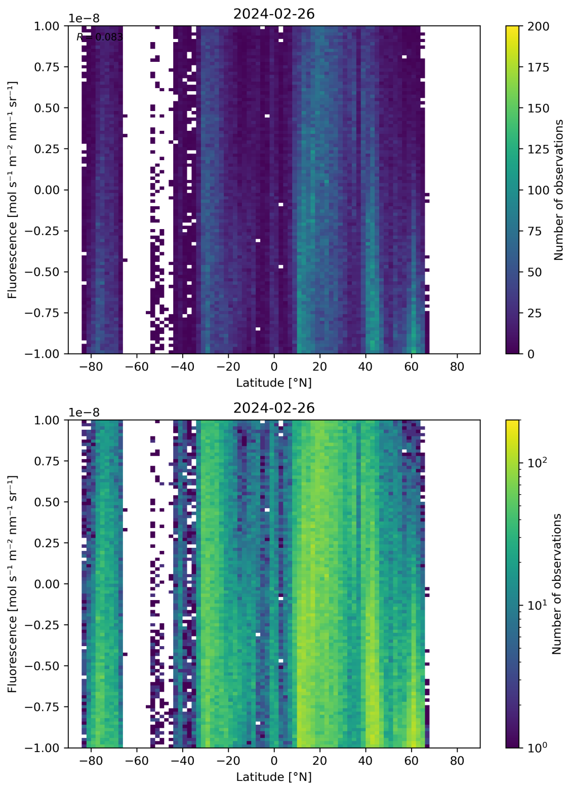
Figure 56: Scatter density plot of “Latitude” against “Fluorescence” for 2024-02-25 to 2024-02-27.
