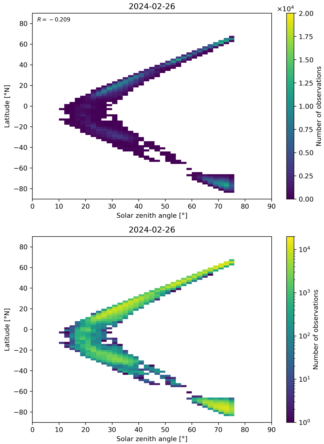
Figure 98: Scatter density plot of “Solar zenith angle” against “Latitude” for 2024-02-25 to 2024-02-27.
