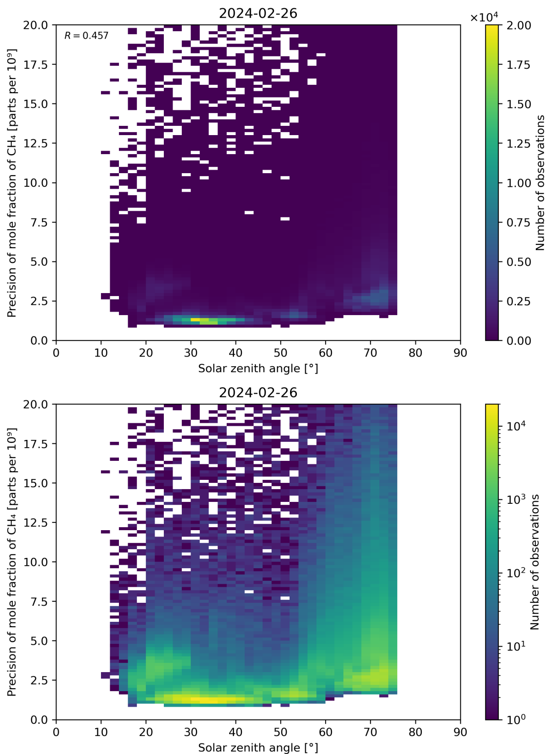
Figure 101: Scatter density plot of “Solar zenith angle” against “Precision of mole fraction of CH 4 ” for 2024-02-25 to 2024-02-27.
