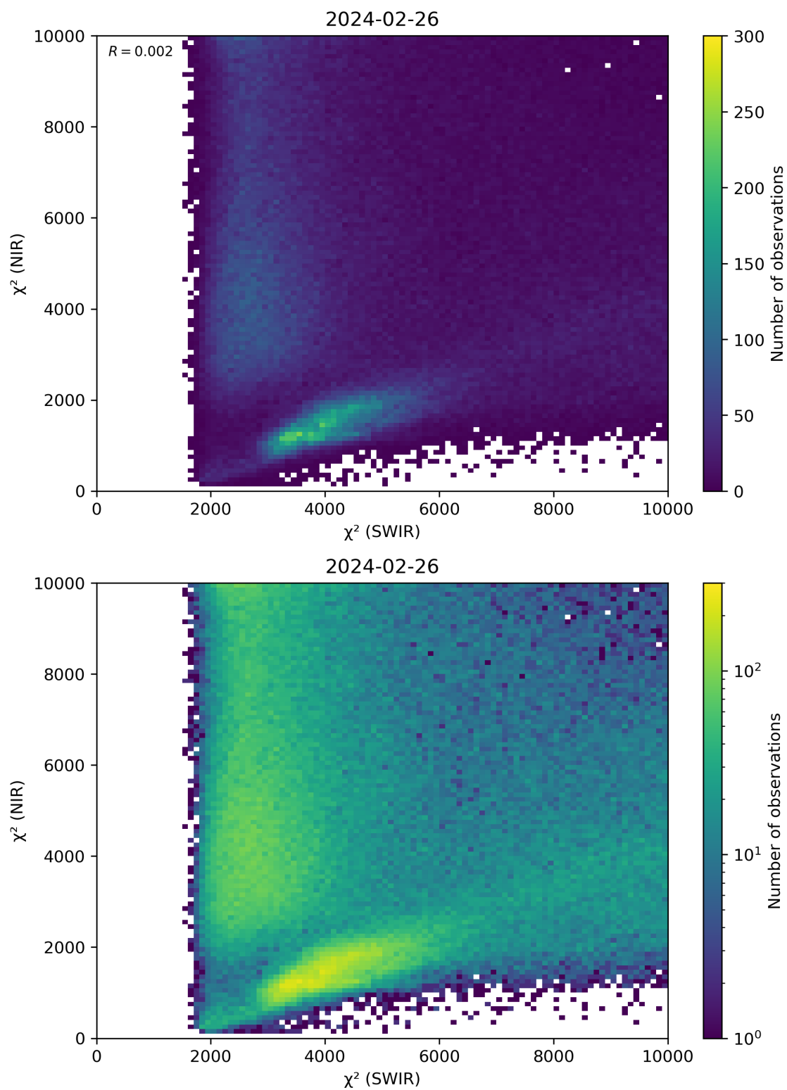
Figure 47: Scatter density plot of “ \chi^2 (SWIR)” against “ \chi^2 (NIR)” for 2024-02-25 to 2024-02-27.
