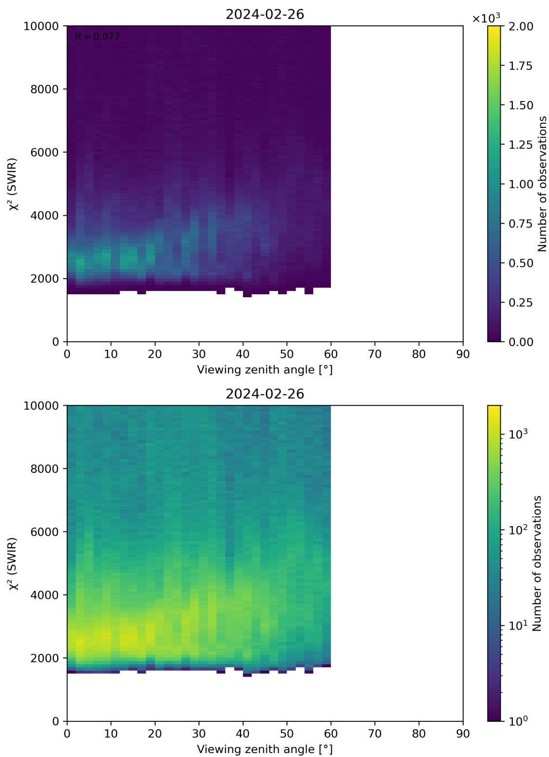
Figure 106: Scatter density plot of “Viewing zenith angle” against “ \chi^2 (SWIR)” for 2024-02-25 to 2024-02-27.
