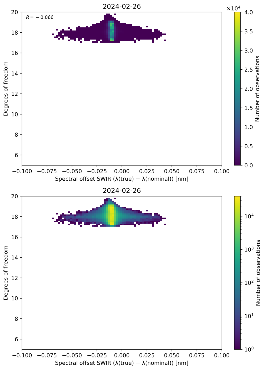
Figure 119: Scatter density plot of “Spectral offset SWIR ( \lambda(\text{true}) - \lambda(\text{nominal}) )” against “Degrees of freedom” for 2024-02-25 to 2024-02-27.
