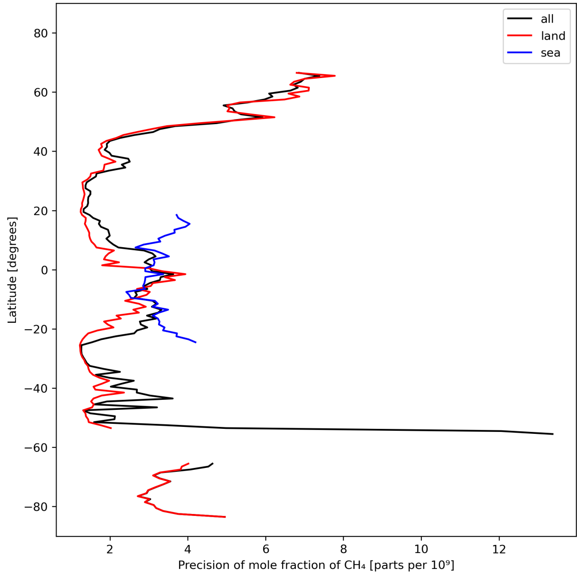
Figure 13: Zonal average of “Precision of mole fraction of CH 4 ” for 2024-02-25 to 2024-02-27.
