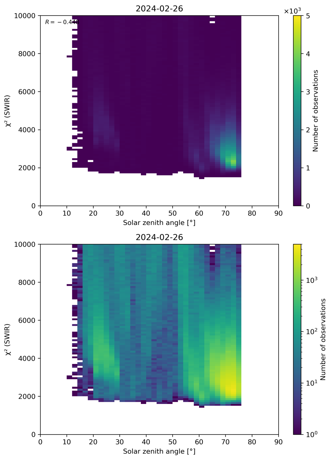
Figure 95: Scatter density plot of “Solar zenith angle” against “ \chi^2 (SWIR)” for 2024-02-25 to 2024-02-27.
