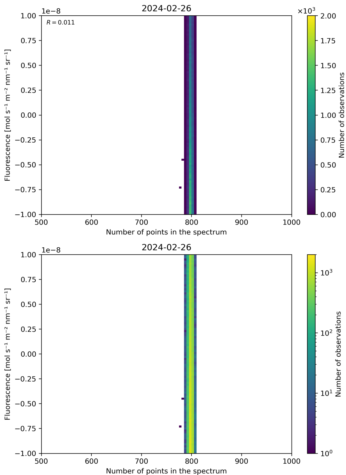
Figure 91: Scatter density plot of “Number of points in the spectrum” against “Fluorescence” for 2024-02-25 to 2024-02-27.
