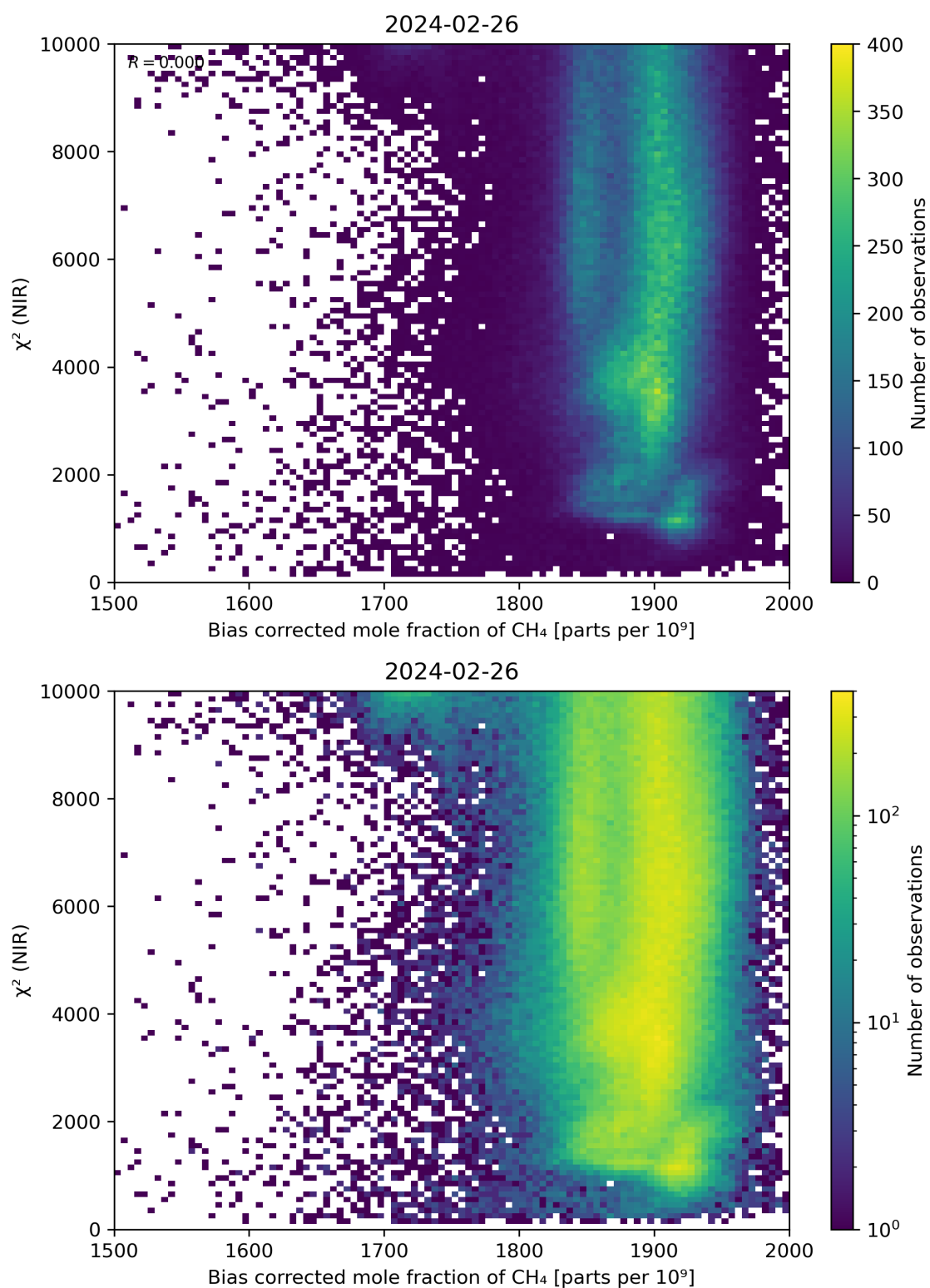
Figure 63: Scatter density plot of “Bias corrected mole fraction of \text{CH}_4 ” against “ \chi^2 (NIR)” for 2024-02-25 to 2024-02-27.
