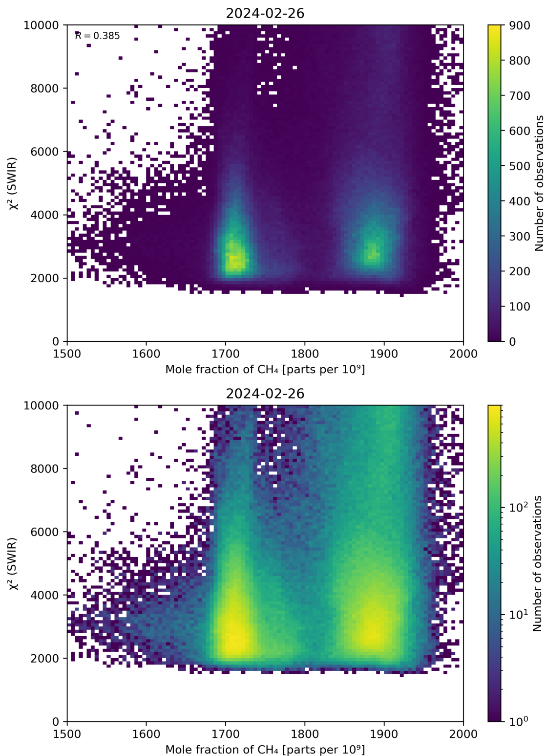
Figure 71: Scatter density plot of “Mole fraction of \text{CH}_4 ” against “ \chi^2 (SWIR)” for 2024-02-25 to 2024-02-27.
