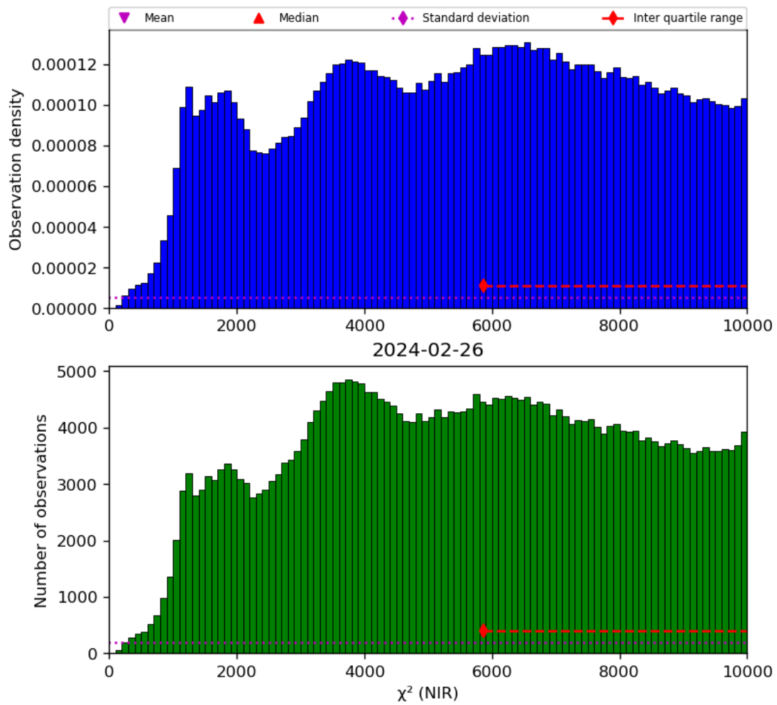
Figure 29: Histogram of “ \chi^2 (NIR)” for 2024-02-25 to 2024-02-27
