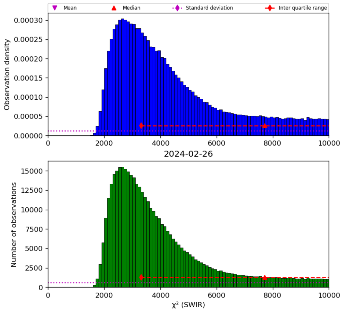
Figure 28: Histogram of “ \chi^2 (SWIR)” for 2024-02-25 to 2024-02-27
