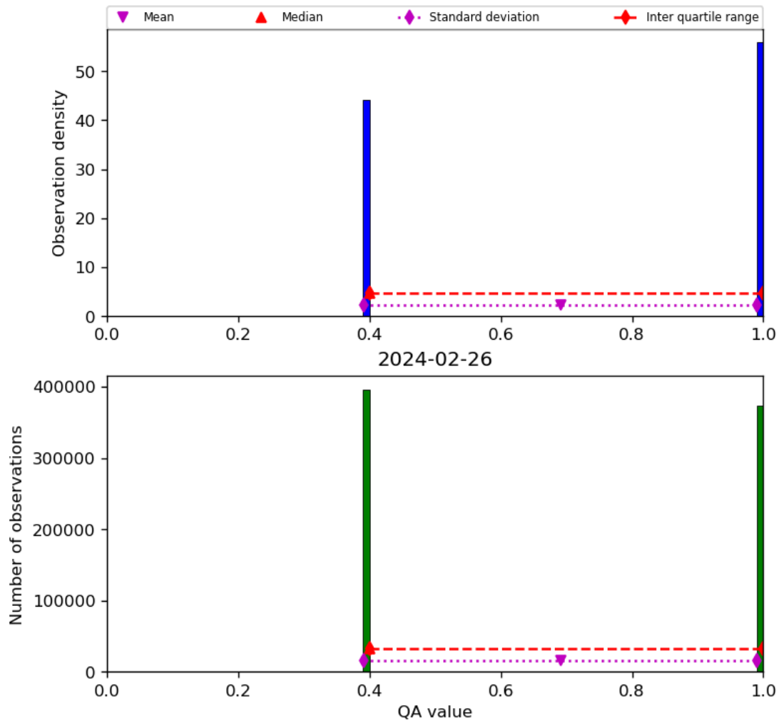
Figure 22: Histogram of "QA value" for 2024-02-25 to 2024-02-27
