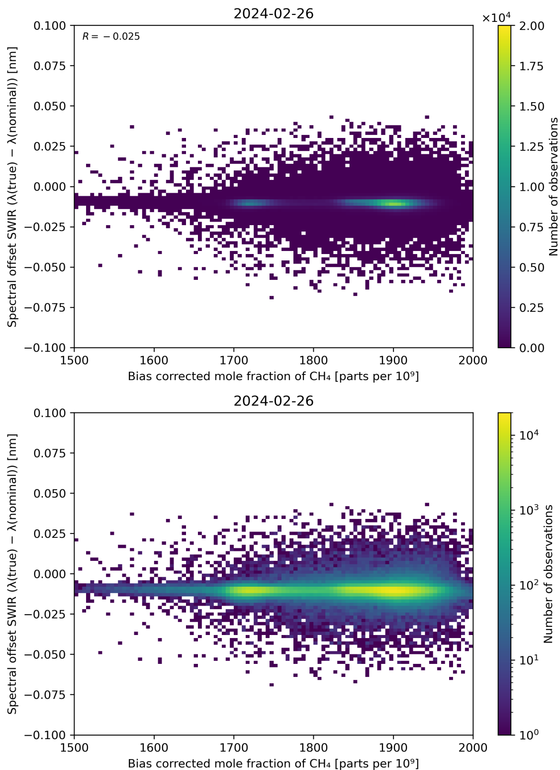
Figure 69: Scatter density plot of “Bias corrected mole fraction of \text{CH}_4 ” against “Spectral offset SWIR ( \lambda(\text{true}) - \lambda(\text{nominal}) )” for 2024-02-25 to 2024-02-27.
