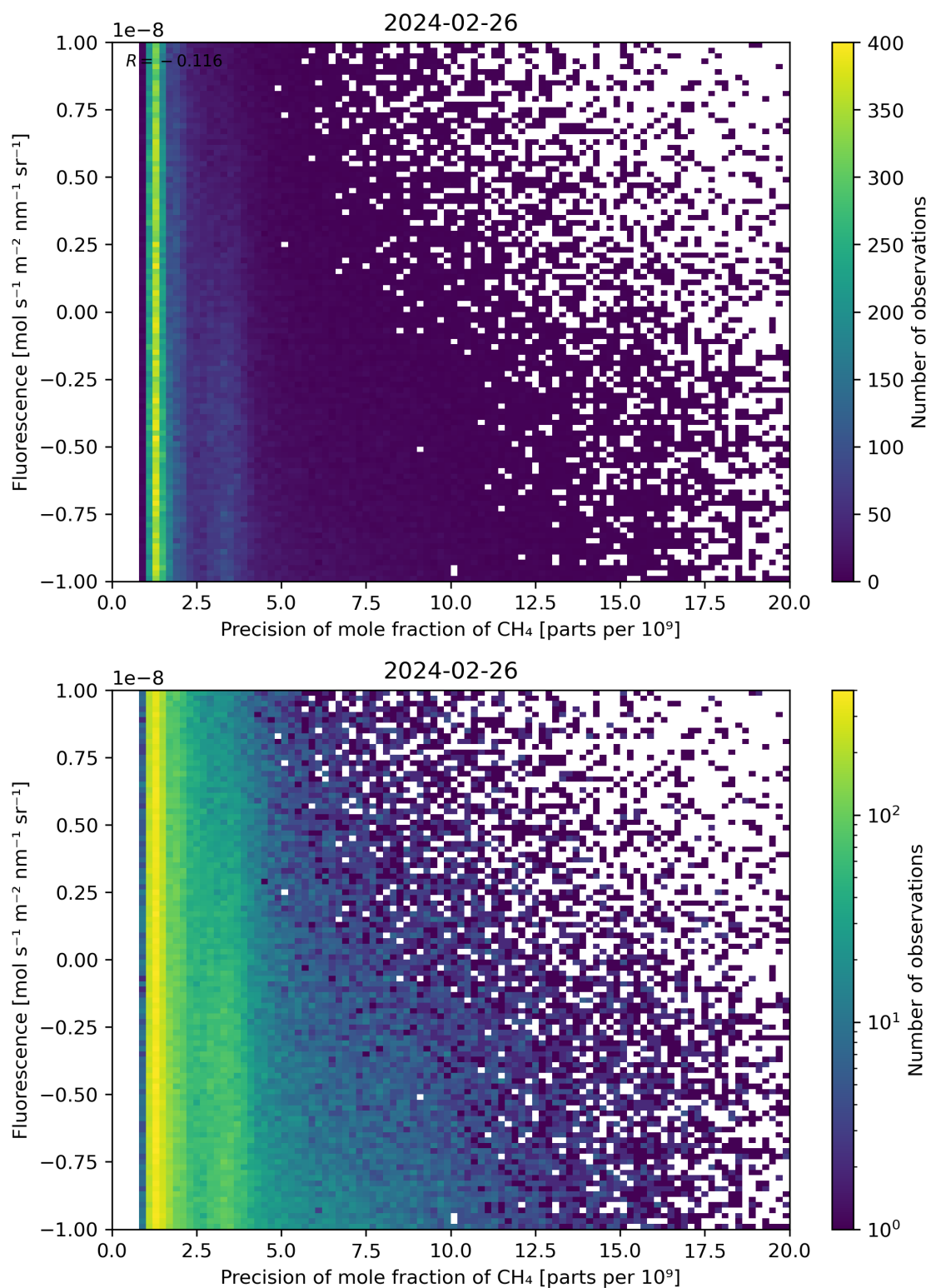
Figure 81: Scatter density plot of “Precision of mole fraction of \text{CH}_4 ” against “Fluorescence” for 2024-02-25 to 2024-02-27.
