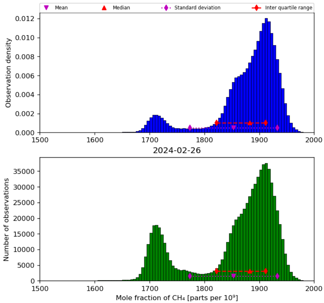
Figure 23: Histogram of “Mole fraction of CH 4 ” for 2024-02-25 to 2024-02-27
