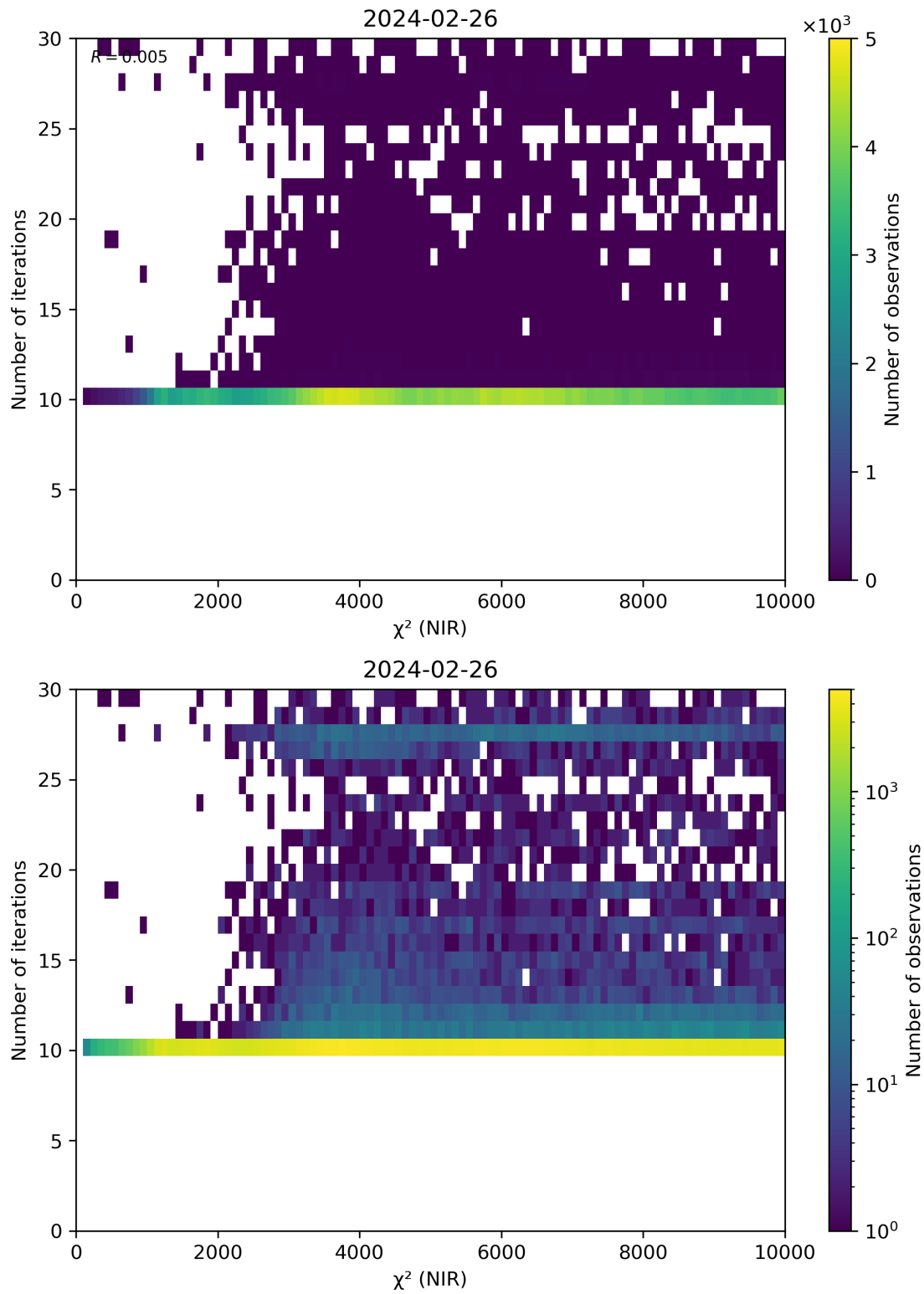
Figure 46: Scatter density plot of “ \chi^2 (NIR)” against “Number of iterations” for 2024-02-25 to 2024-02-27.
