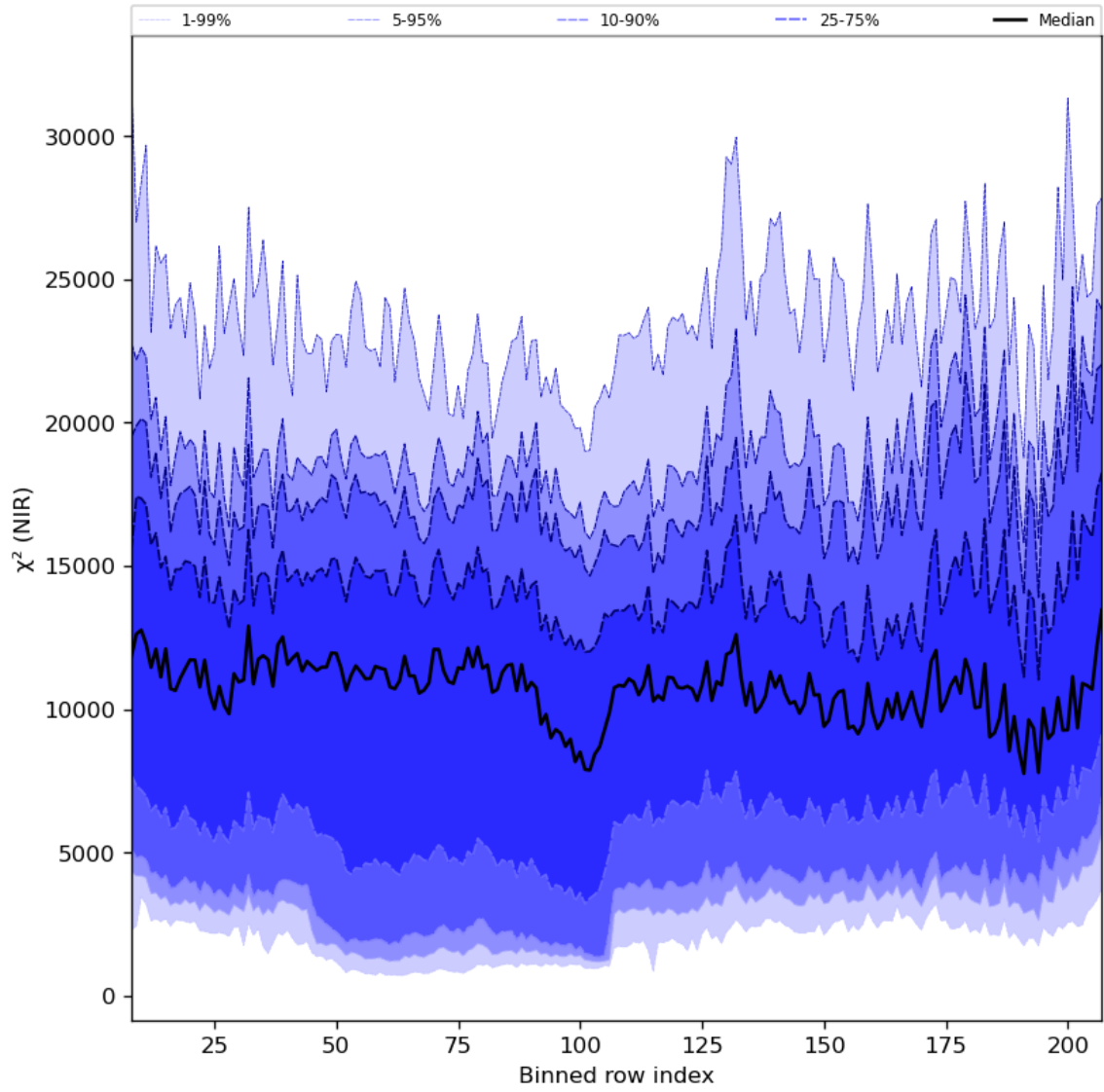
Figure 40: Along track statistics of " \chi^2 (NIR)" for 2024-02-25 to 2024-02-27
