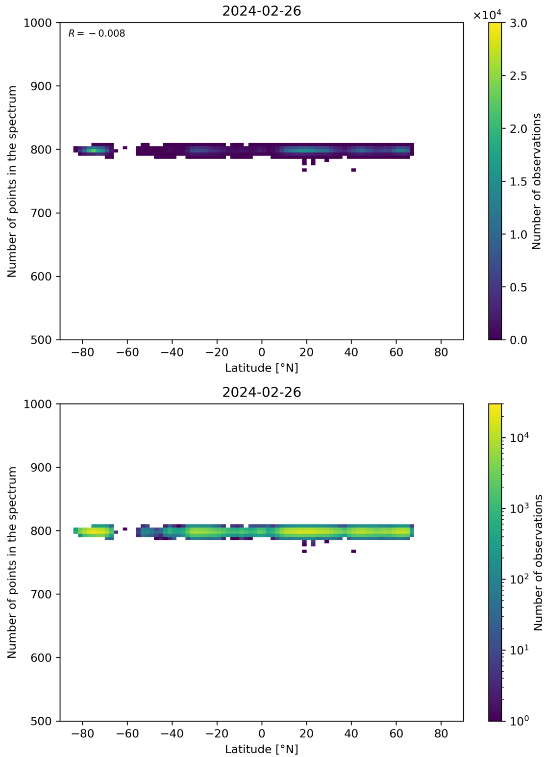
Figure 61: Scatter density plot of “Latitude” against “Number of points in the spectrum” for 2024-02-25 to 2024-02-27.
