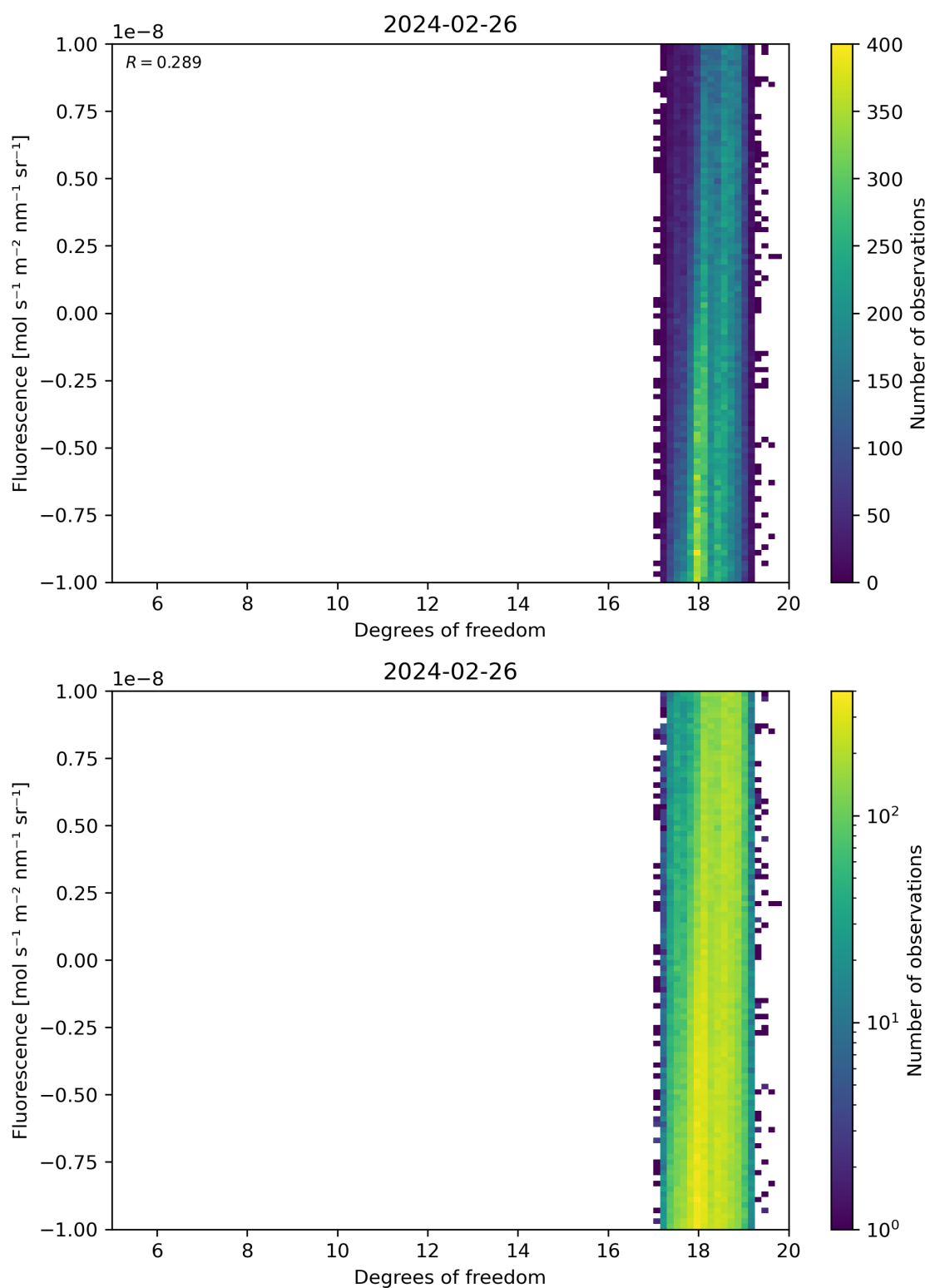
Figure 51: Scatter density plot of “Degrees of freedom” against “Fluorescence” for 2024-02-25 to 2024-02-27.
