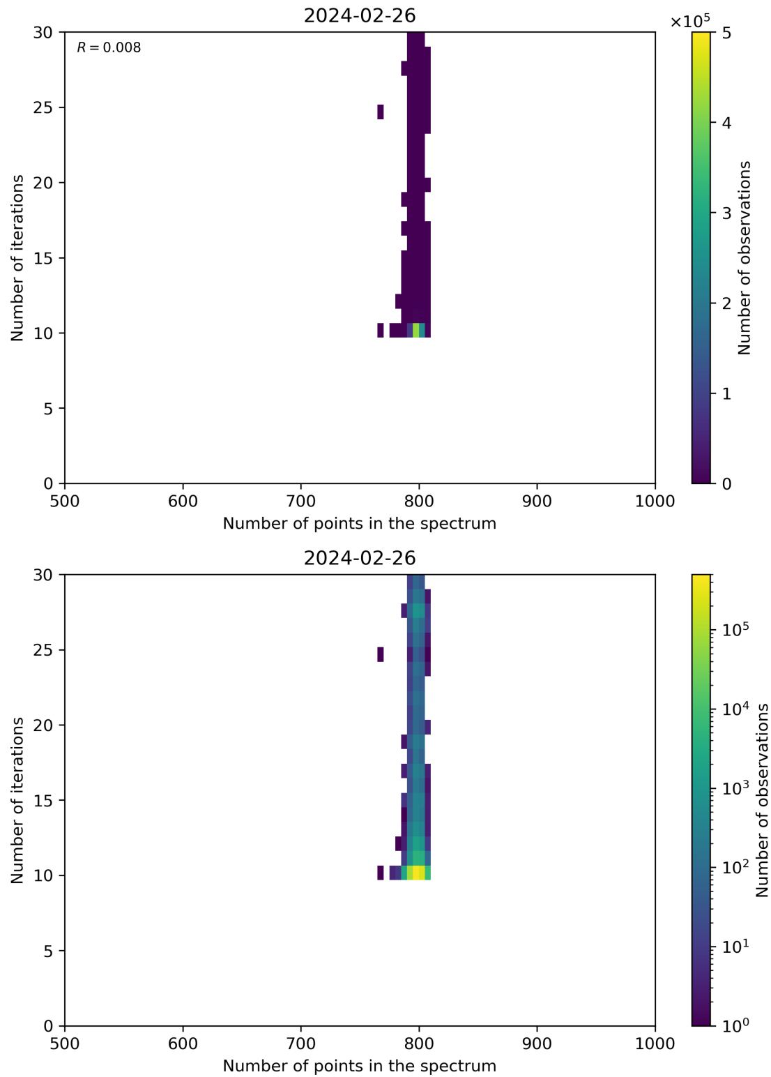
Figure 92: Scatter density plot of “Number of points in the spectrum” against “Number of iterations” for 2024-02-25 to 2024-02-27.
