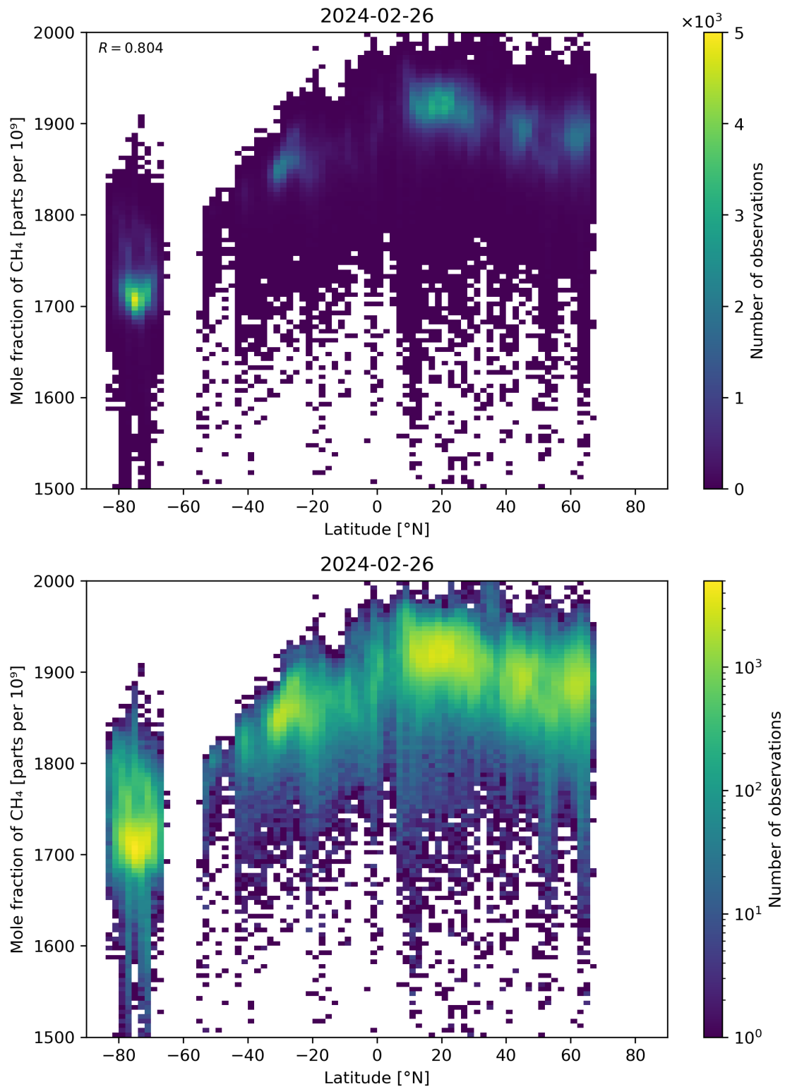
Figure 57: Scatter density plot of “Latitude” against “Mole fraction of \text{CH}_4 ” for 2024-02-25 to 2024-02-27.
