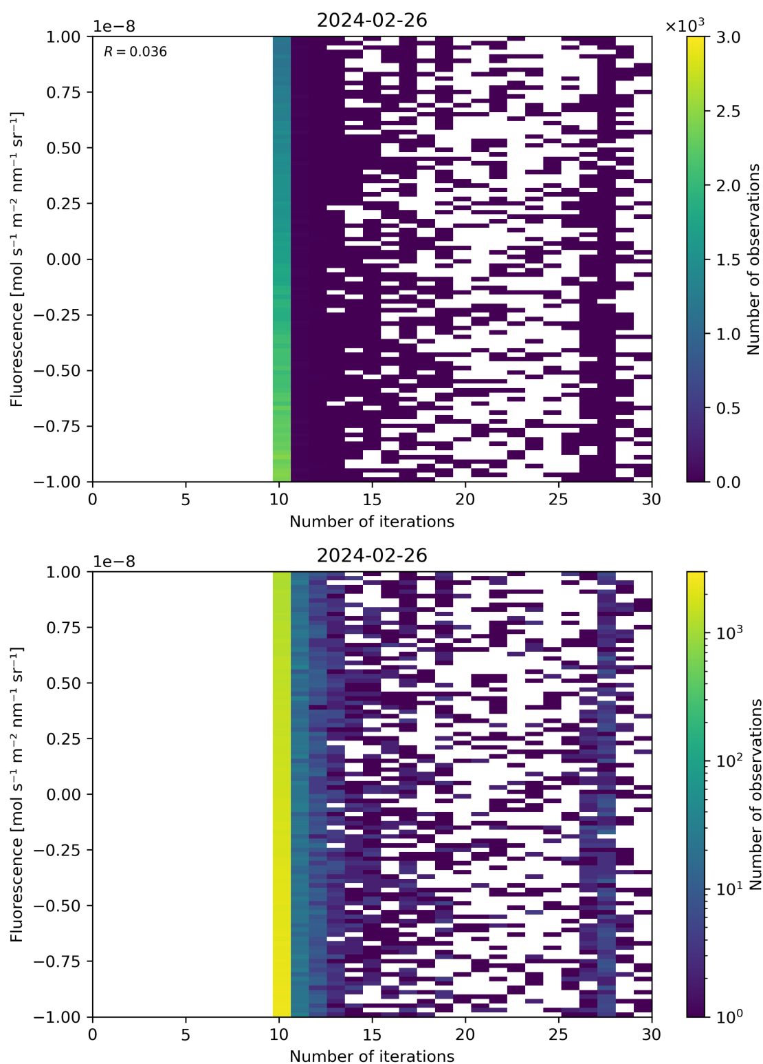
Figure 87: Scatter density plot of “Number of iterations” against “Fluorescence” for 2024-02-25 to 2024-02-27.
