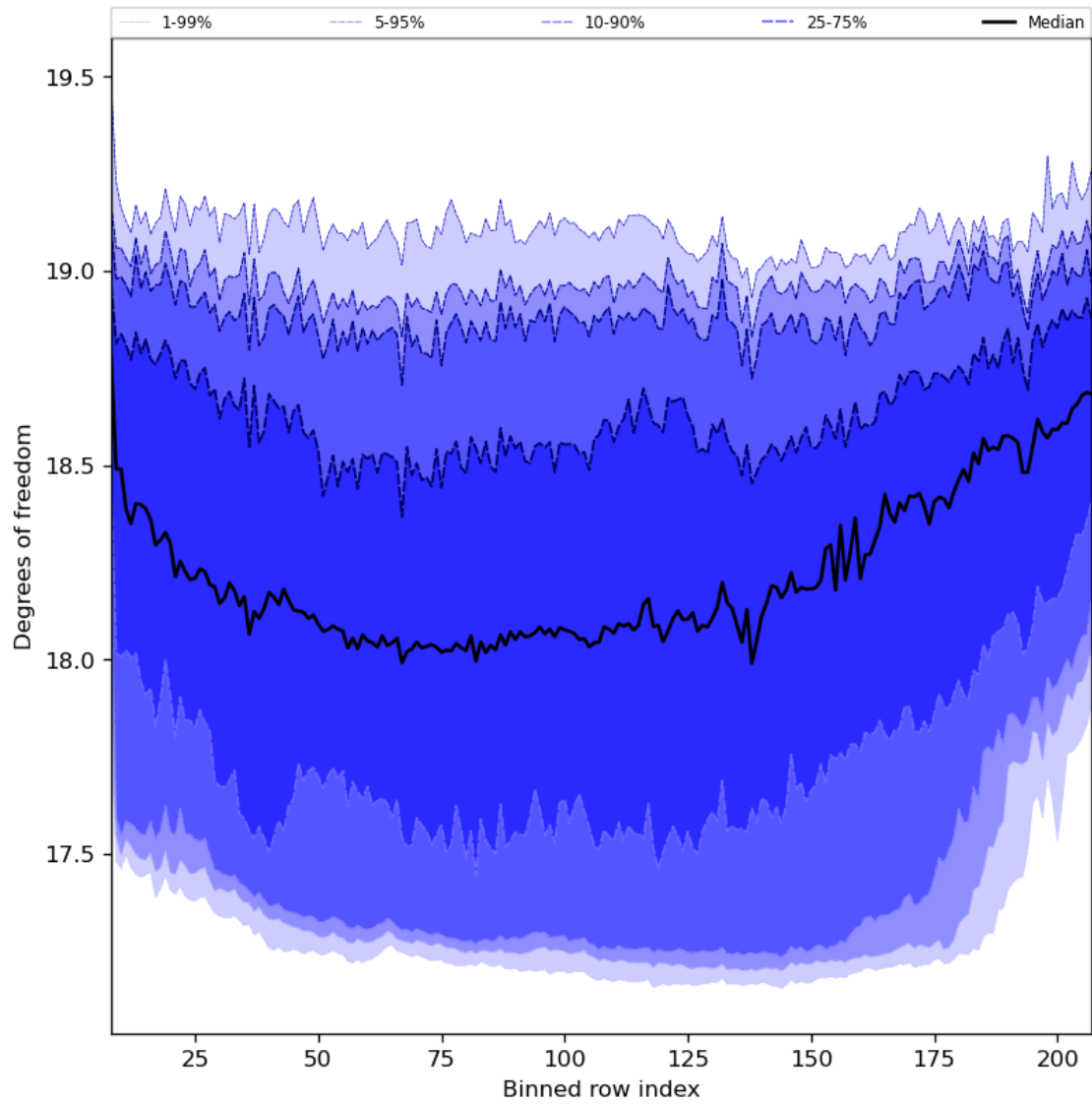
Figure 41: Along track statistics of “Degrees of freedom” for 2024-02-25 to 2024-02-27
