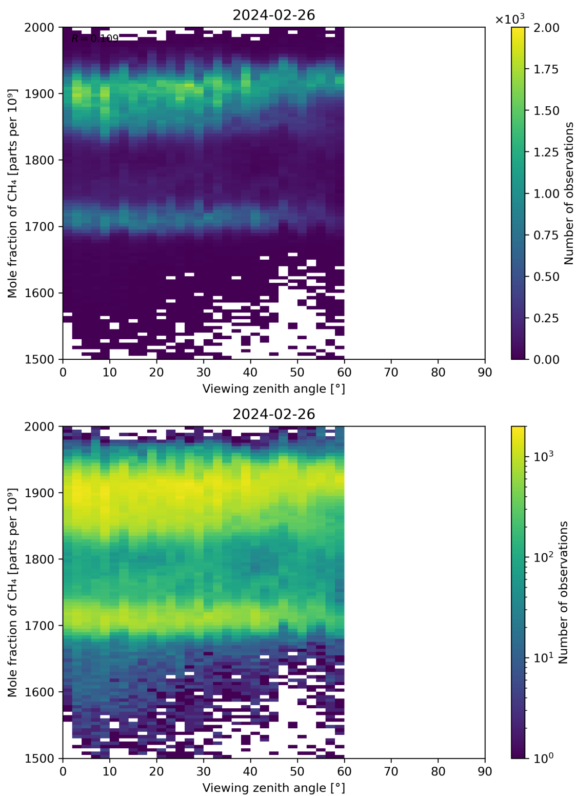
Figure 110: Scatter density plot of “Viewing zenith angle” against “Mole fraction of CH 4 ” for 2024-02-25 to 2024-02-27.
