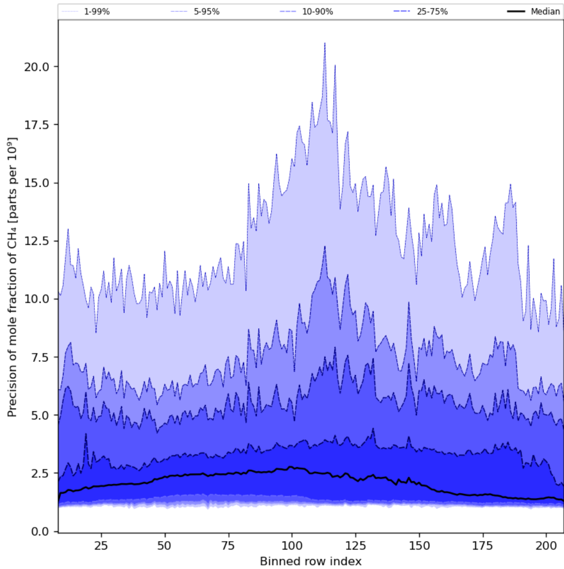
Figure 35: Along track statistics of “Precision of mole fraction of CH 4 ” for 2024-02-25 to 2024-02-27
