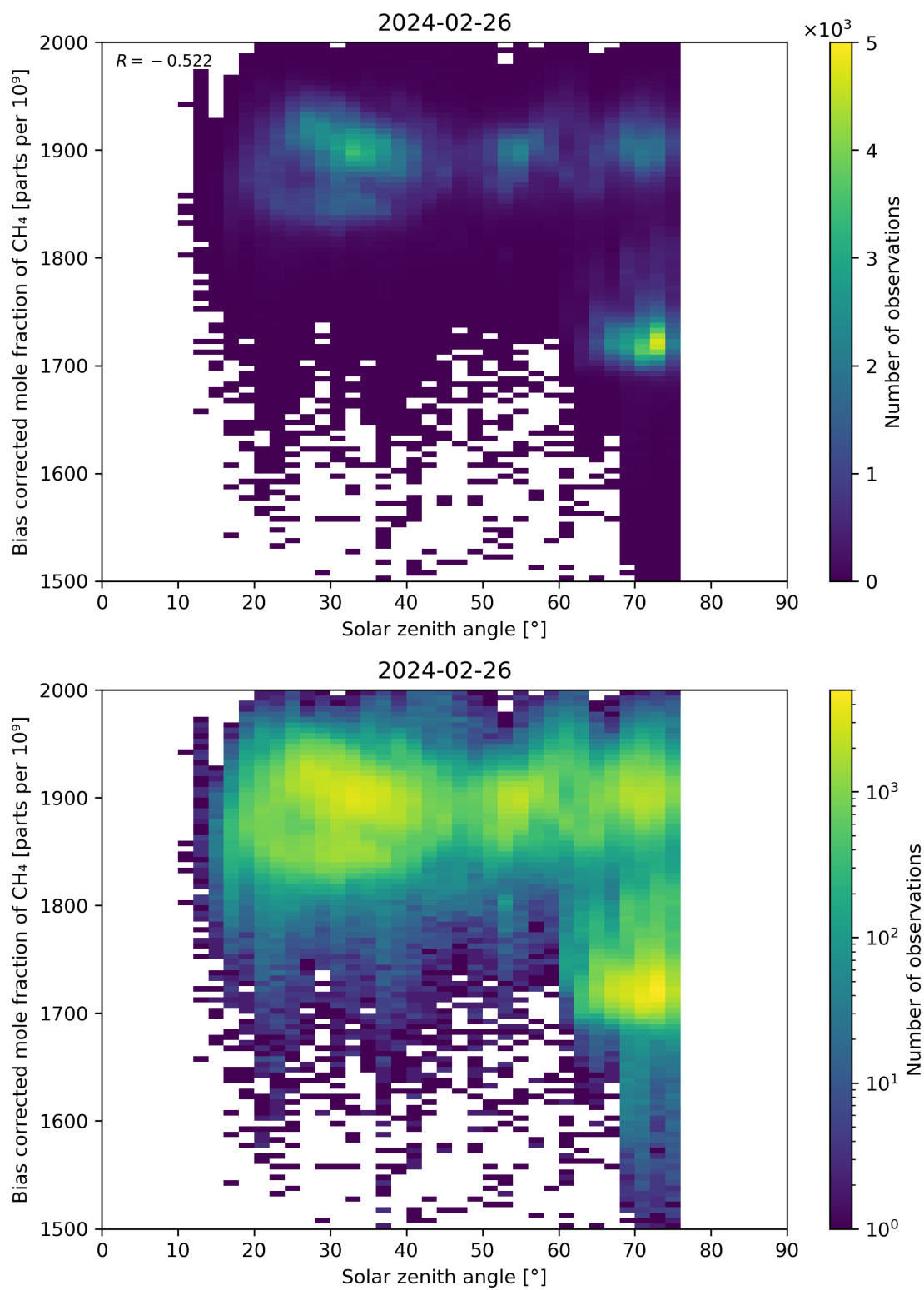
Figure 100: Scatter density plot of “Solar zenith angle” against “Bias corrected mole fraction of \text{CH}_4 ” for 2024-02-25 to 2024-02-27.
