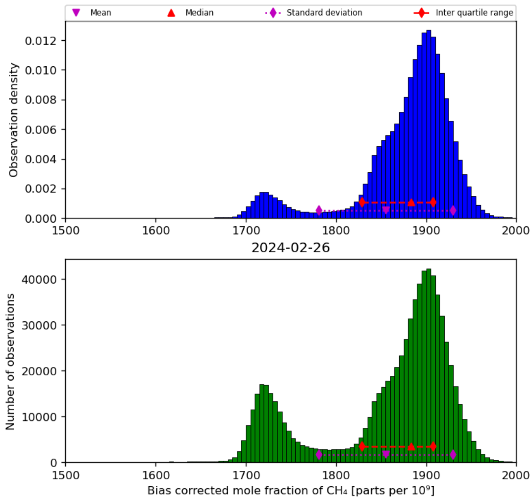
Figure 25: Histogram of “Bias corrected mole fraction of CH 4 ” for 2024-02-25 to 2024-02-27
