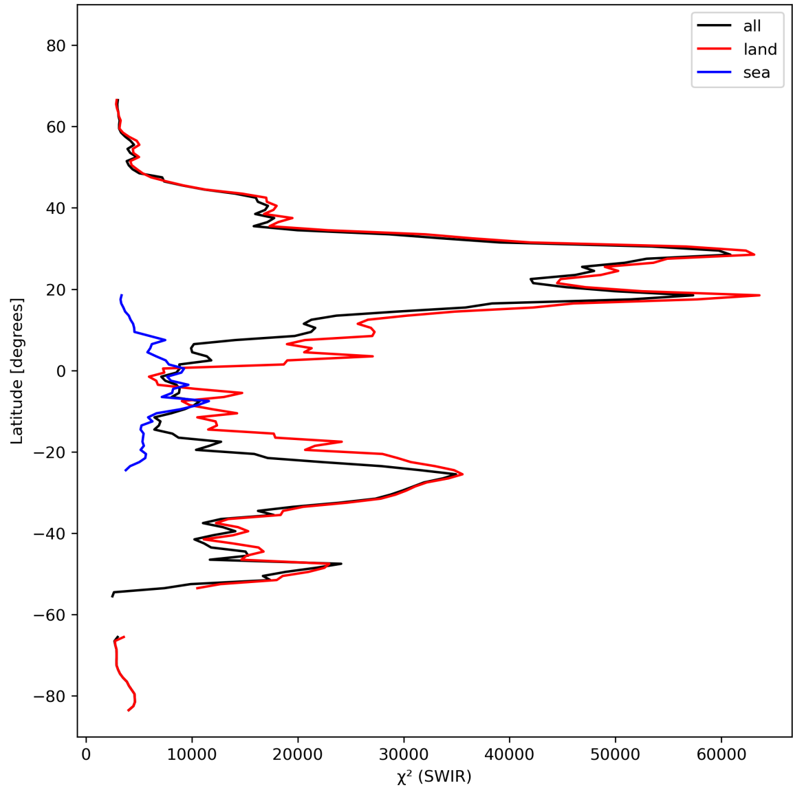
Figure 17: Zonal average of “ \chi^2 (SWIR)” for 2024-02-25 to 2024-02-27.
