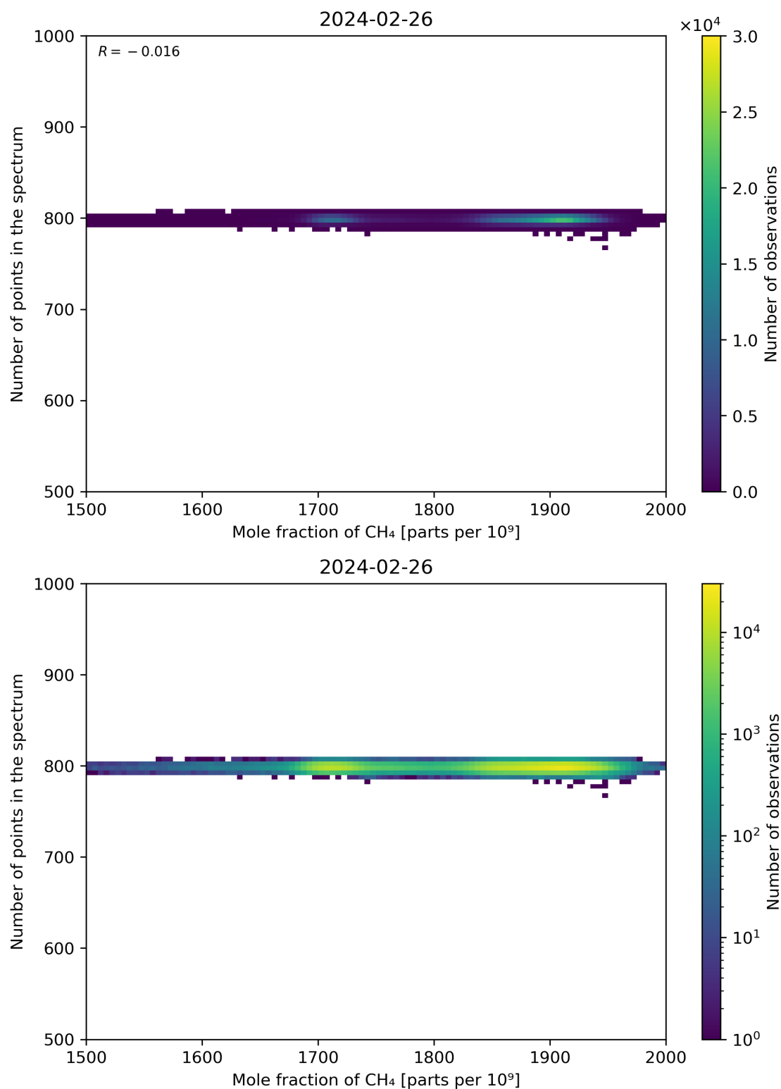
Figure 77: Scatter density plot of “Mole fraction of CH 4 ” against “Number of points in the spectrum” for 2024-02-25 to 2024-02-27.
