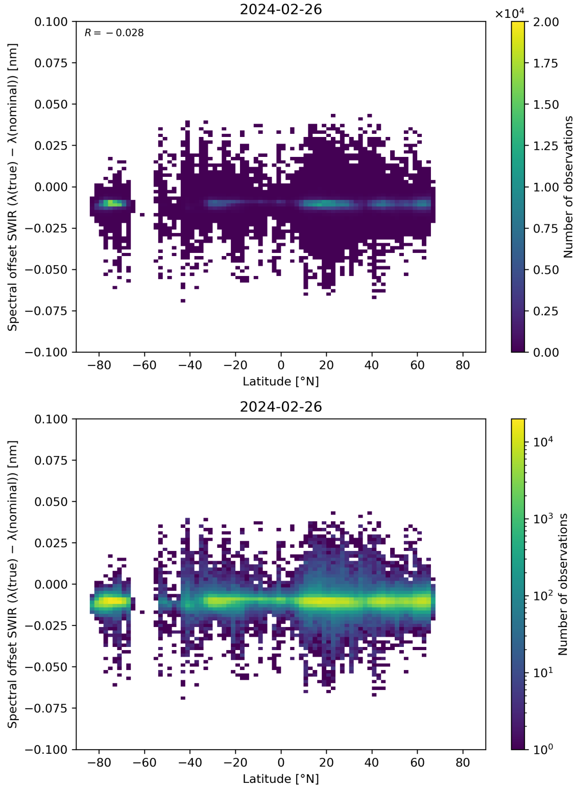
Figure 62: Scatter density plot of “Latitude” against “Spectral offset SWIR ( \lambda(\text{true}) - \lambda(\text{nominal}) )” for 2024-02-25 to 2024-02-27.
