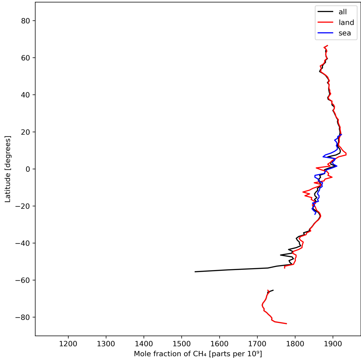
Figure 12: Zonal average of “Mole fraction of \text{CH}_4 ” for 2024-02-25 to 2024-02-27.
