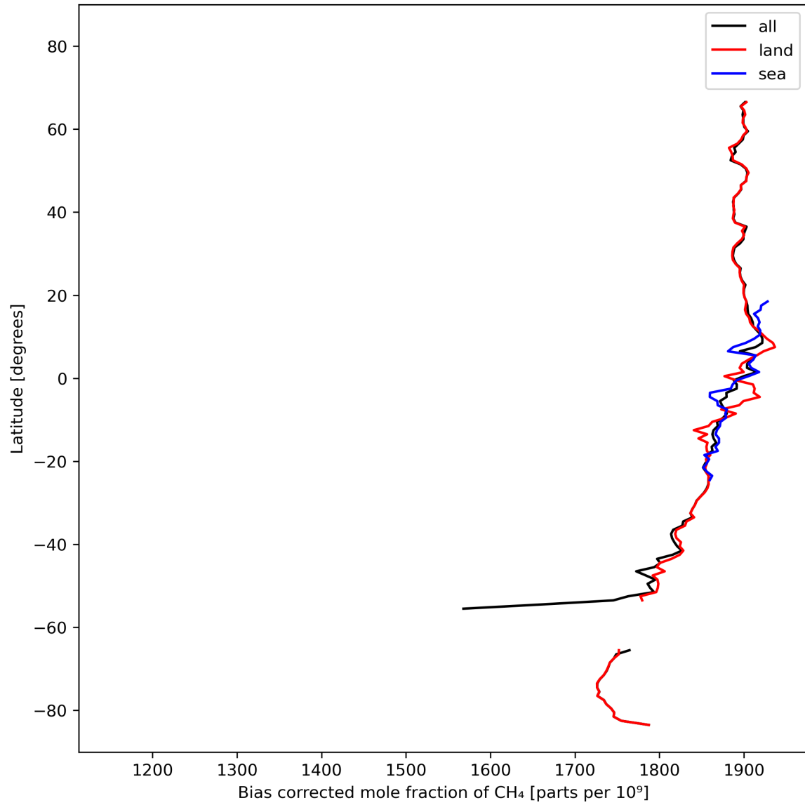
Figure 14: Zonal average of “Bias corrected mole fraction of CH 4 ” for 2024-02-25 to 2024-02-27.
