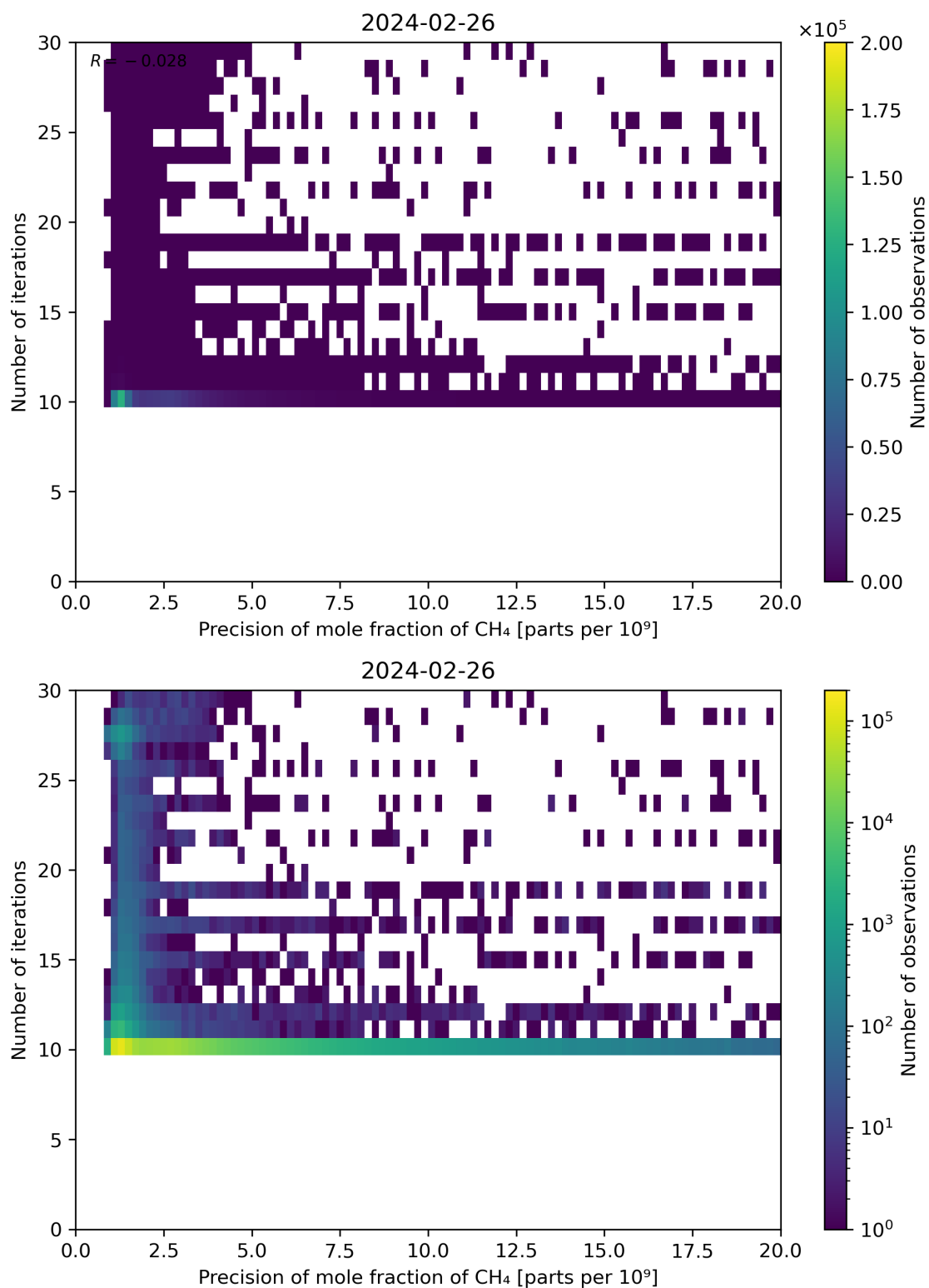
Figure 83: Scatter density plot of “Precision of mole fraction of CH 4 ” against “Number of iterations” for 2024-02-25 to 2024-02-27.
