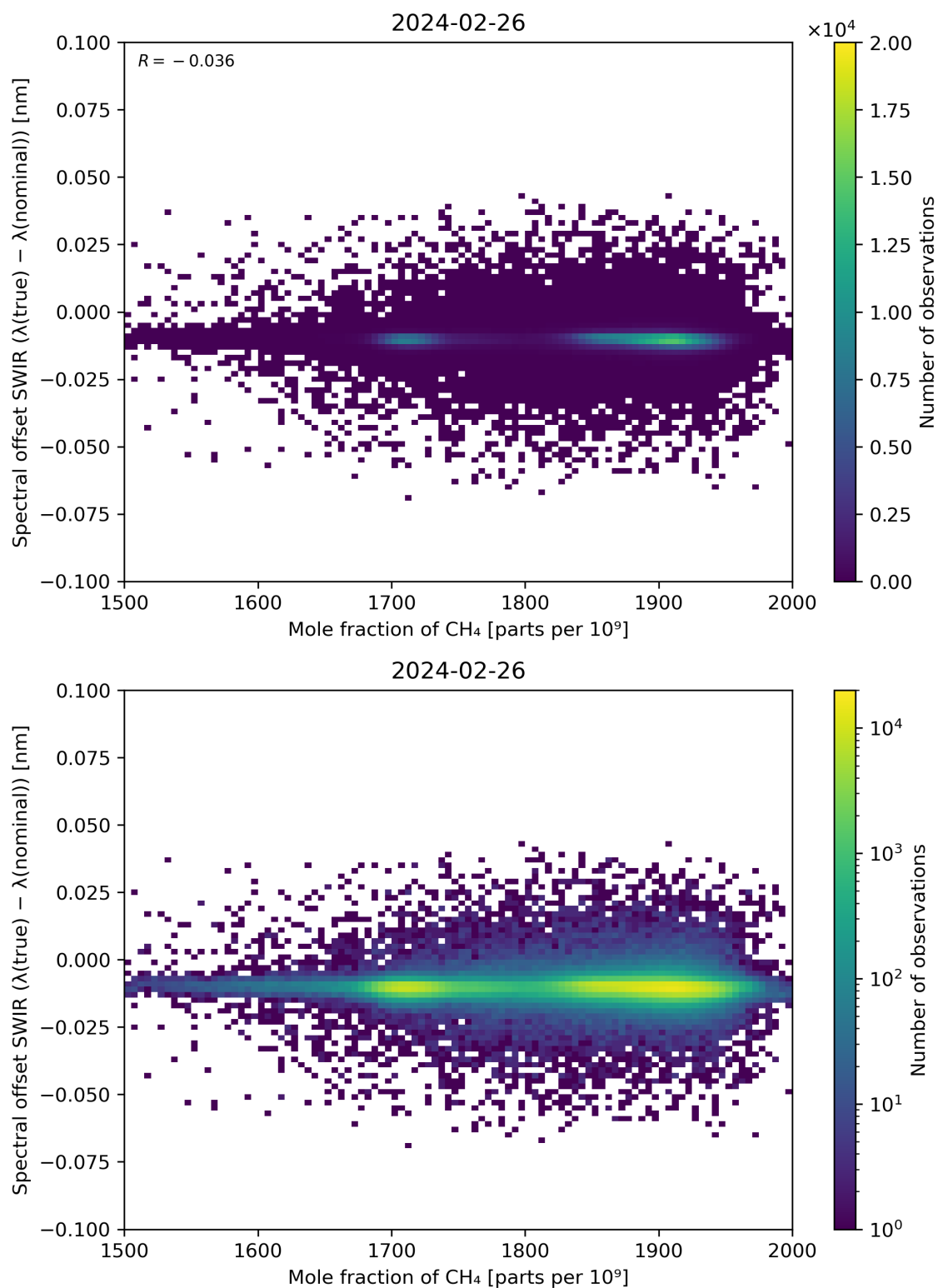
Figure 86: Scatter density plot of “Mole fraction of CH 4 ” against “Spectral offset SWIR ( \lambda(\text{true}) - \lambda(\text{nominal}) )” for 2024-02-25 to 2024-02-27.
