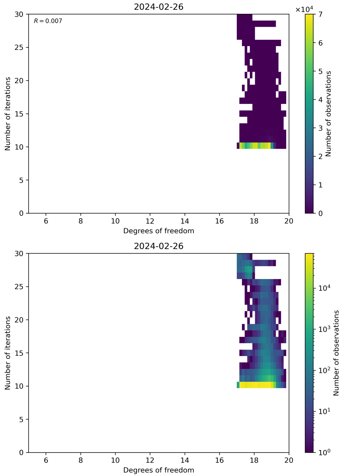
Figure 52: Scatter density plot of “Degrees of freedom” against “Number of iterations” for 2024-02-25 to 2024-02-27.
