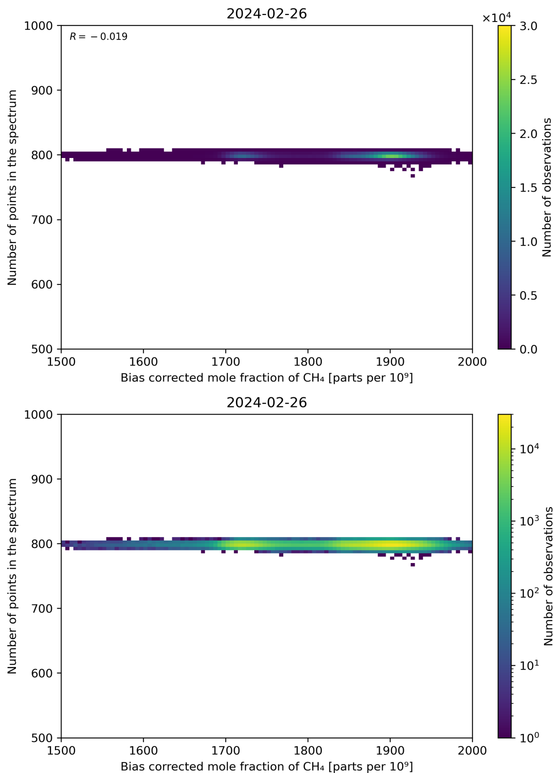
Figure 68: Scatter density plot of “Bias corrected mole fraction of CH 4 ” against “Number of points in the spectrum” for 2024-02-25 to 2024-02-27.
