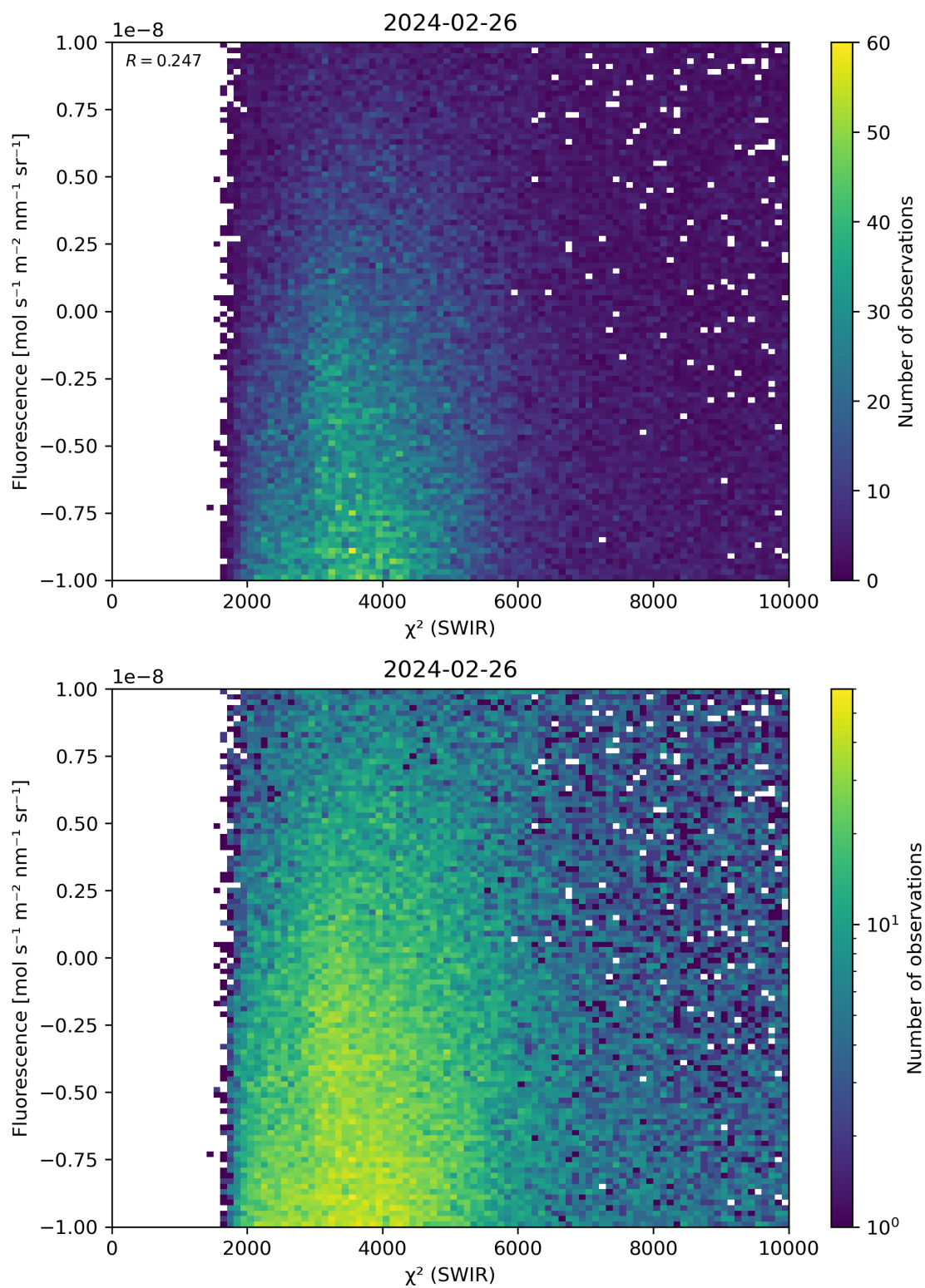
Figure 49: Scatter density plot of “ \chi^2 (SWIR)” against “Fluorescence” for 2024-02-25 to 2024-02-27.
