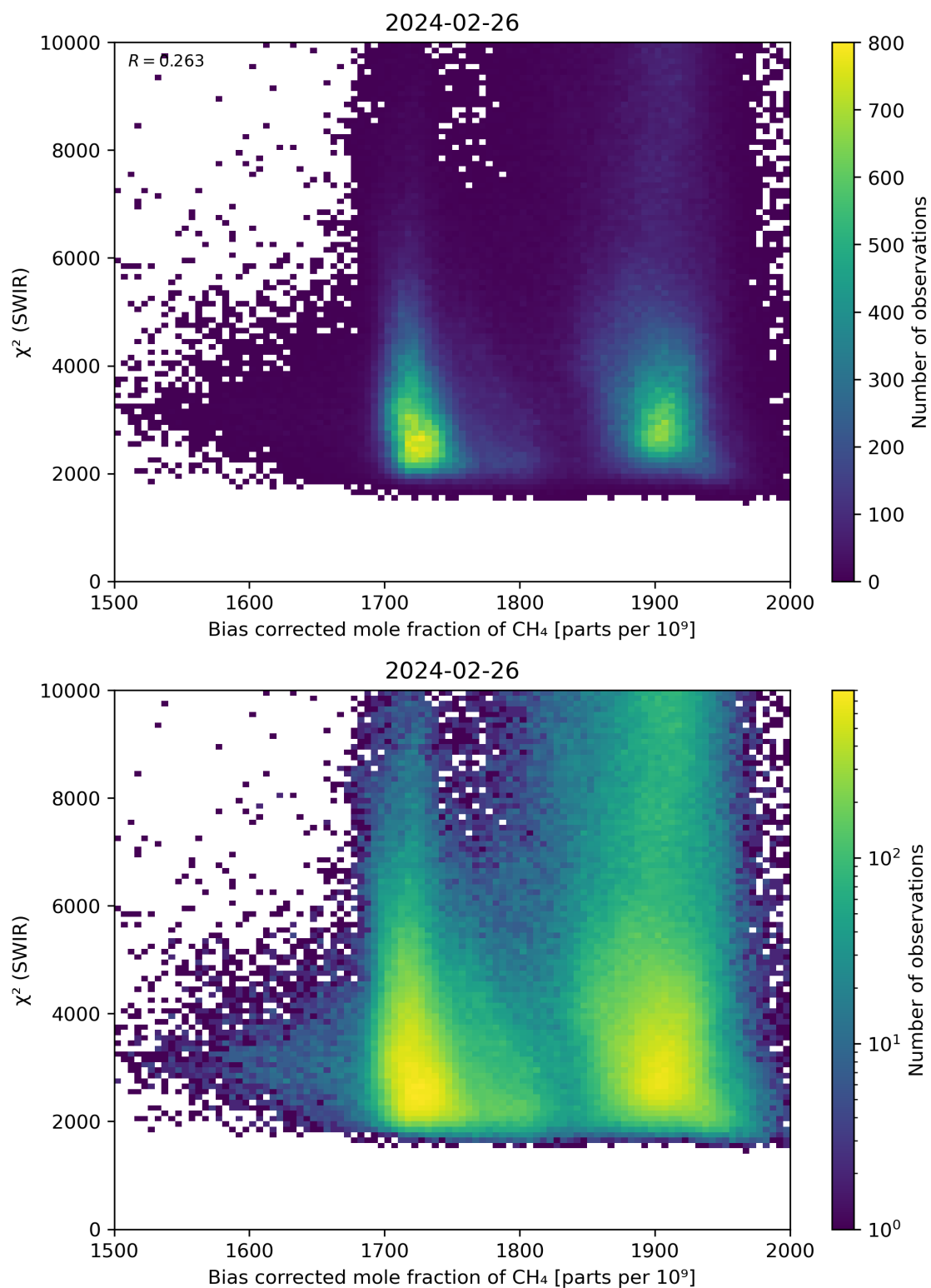
Figure 64: Scatter density plot of “Bias corrected mole fraction of CH 4 ” against “ \chi^2 (SWIR)” for 2024-02-25 to 2024-02-27.
