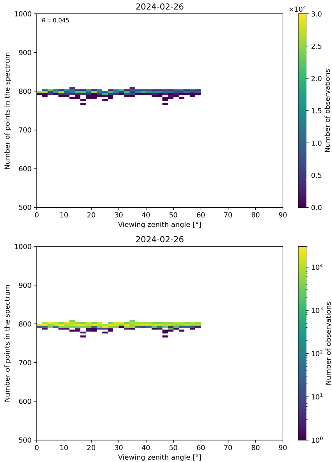
Figure 114: Scatter density plot of “Viewing zenith angle” against “Number of points in the spectrum” for 2024-02-25 to 2024-02-27.
