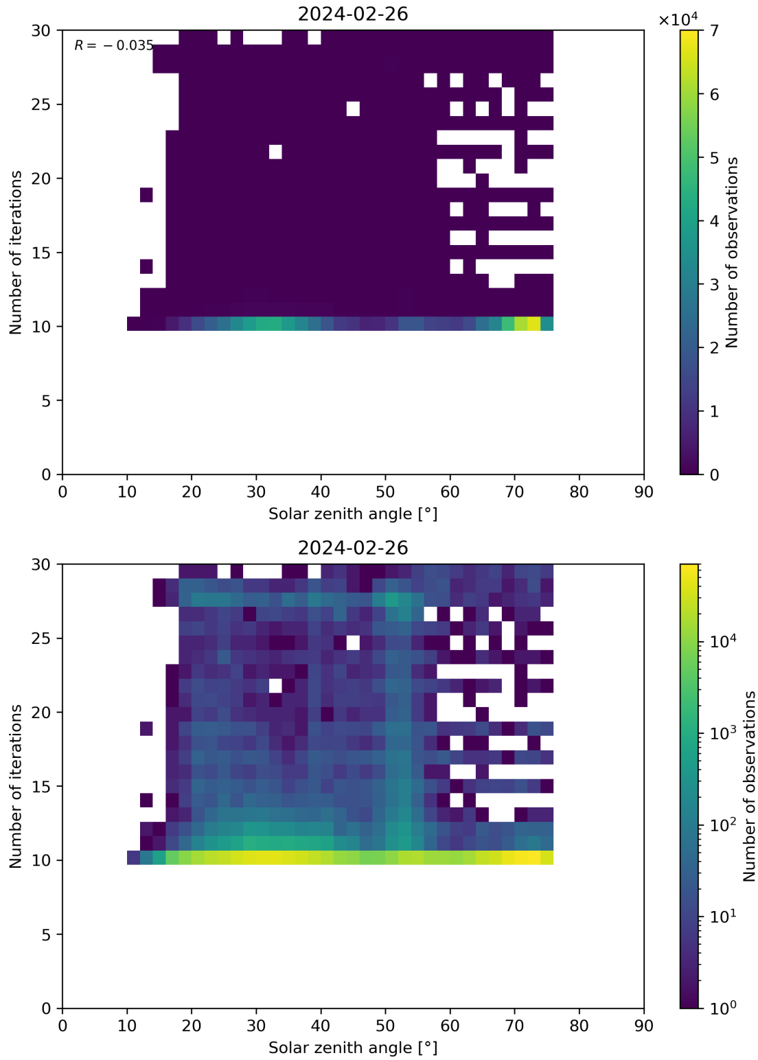
Figure 102: Scatter density plot of “Solar zenith angle” against “Number of iterations” for 2024-02-25 to 2024-02-27.
