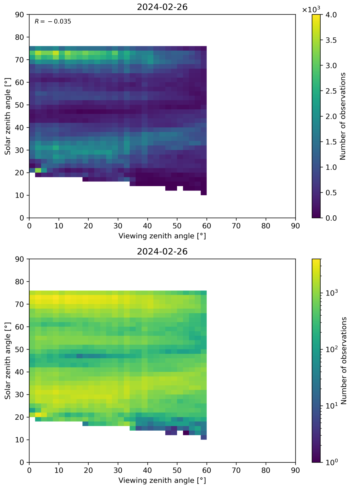
Figure 115: Scatter density plot of “Viewing zenith angle” against “Solar zenith angle” for 2024-02-25 to 2024-02-27.
