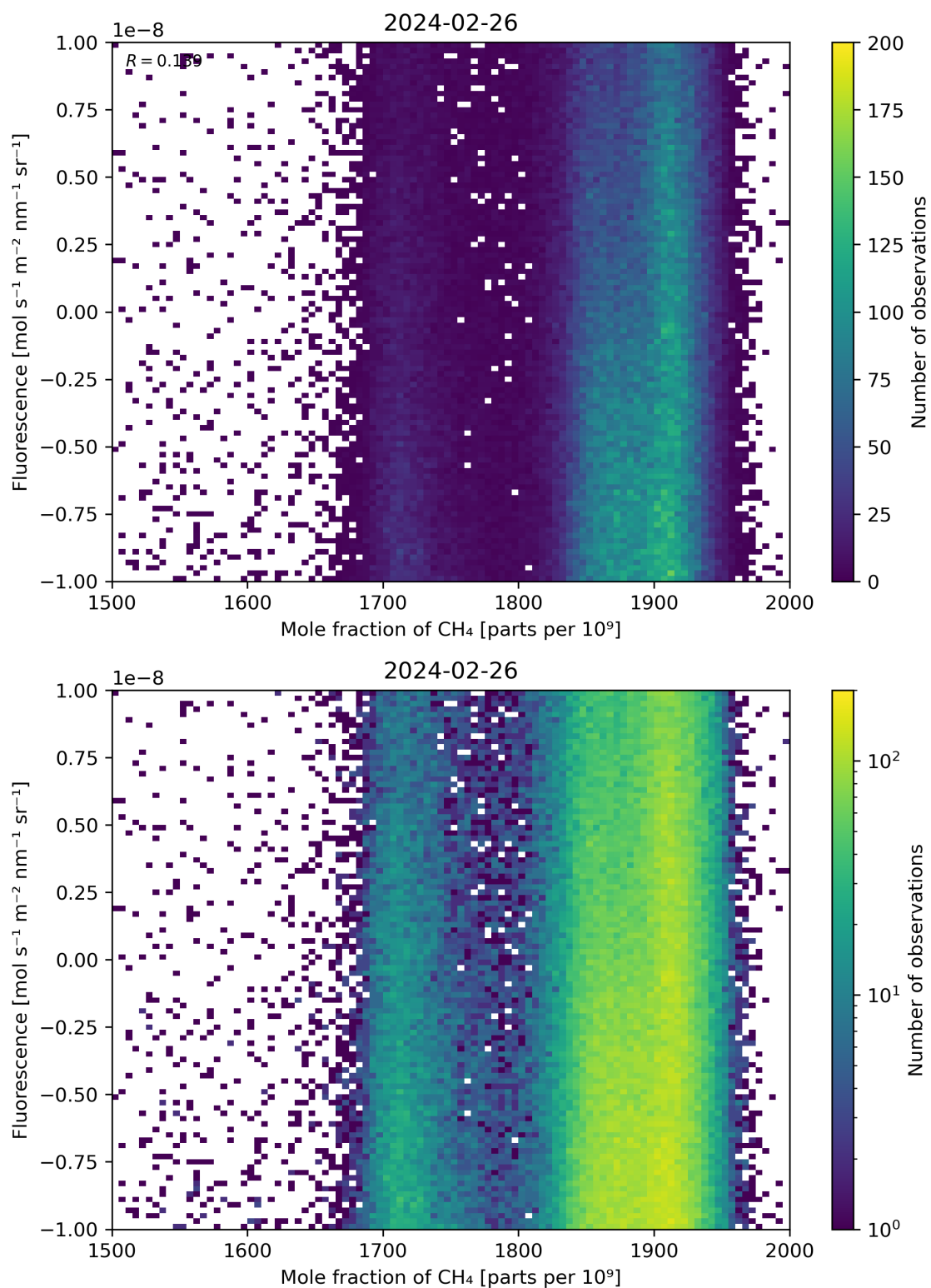
Figure 73: Scatter density plot of “Mole fraction of \text{CH}_4 ” against “Fluorescence” for 2024-02-25 to 2024-02-27.
