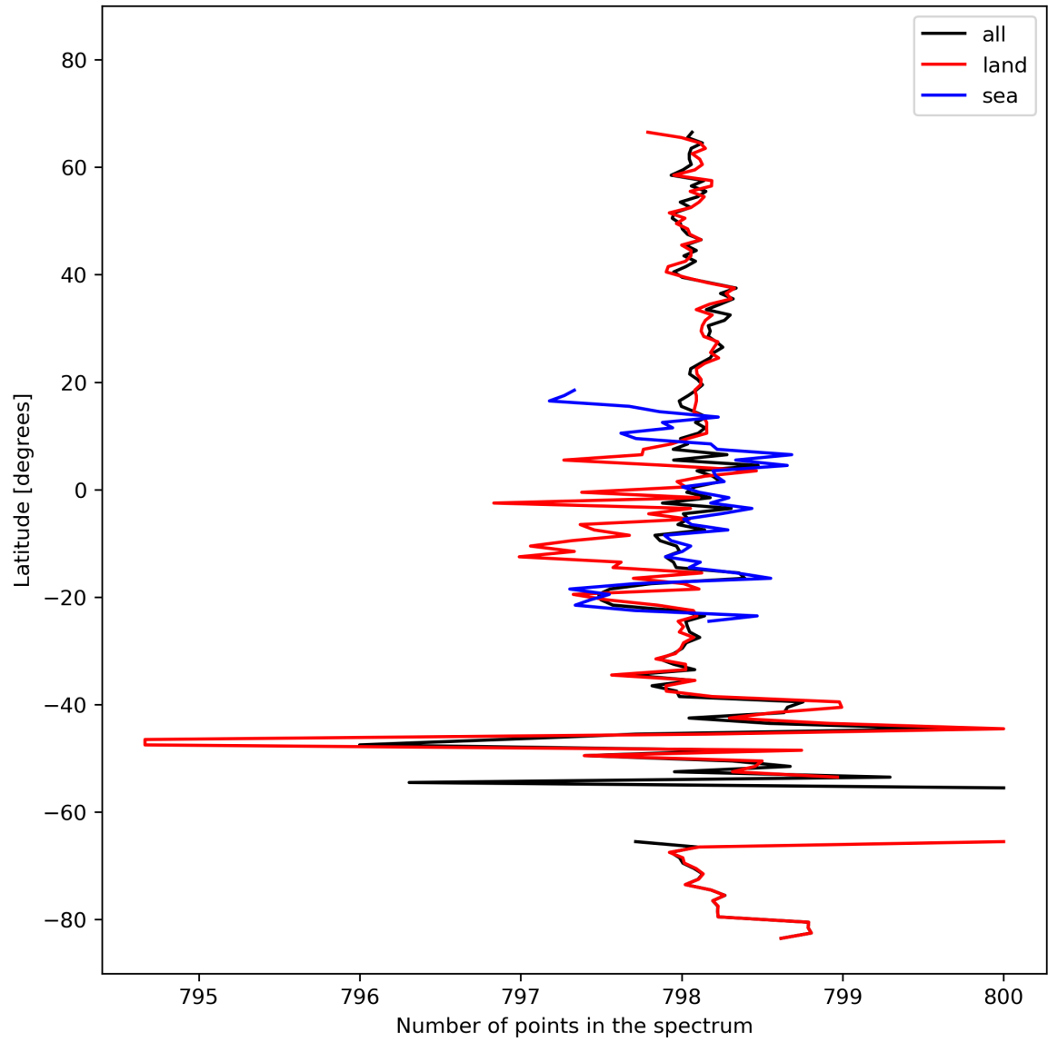
Figure 15: Zonal average of “Number of points in the spectrum” for 2024-02-25 to 2024-02-27.
