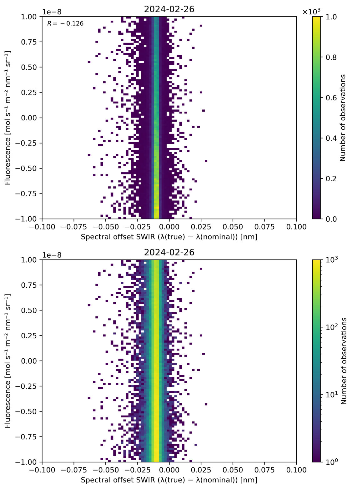
Figure 120: Scatter density plot of “Spectral offset SWIR ( \lambda(\text{true}) - \lambda(\text{nominal}) )” against “Fluorescence” for 2024-02-25 to 2024-02-27.
