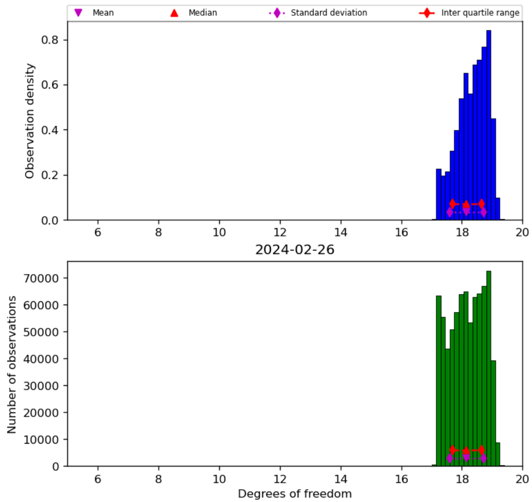
Figure 30: Histogram of “Degrees of freedom” for 2024-02-25 to 2024-02-27
