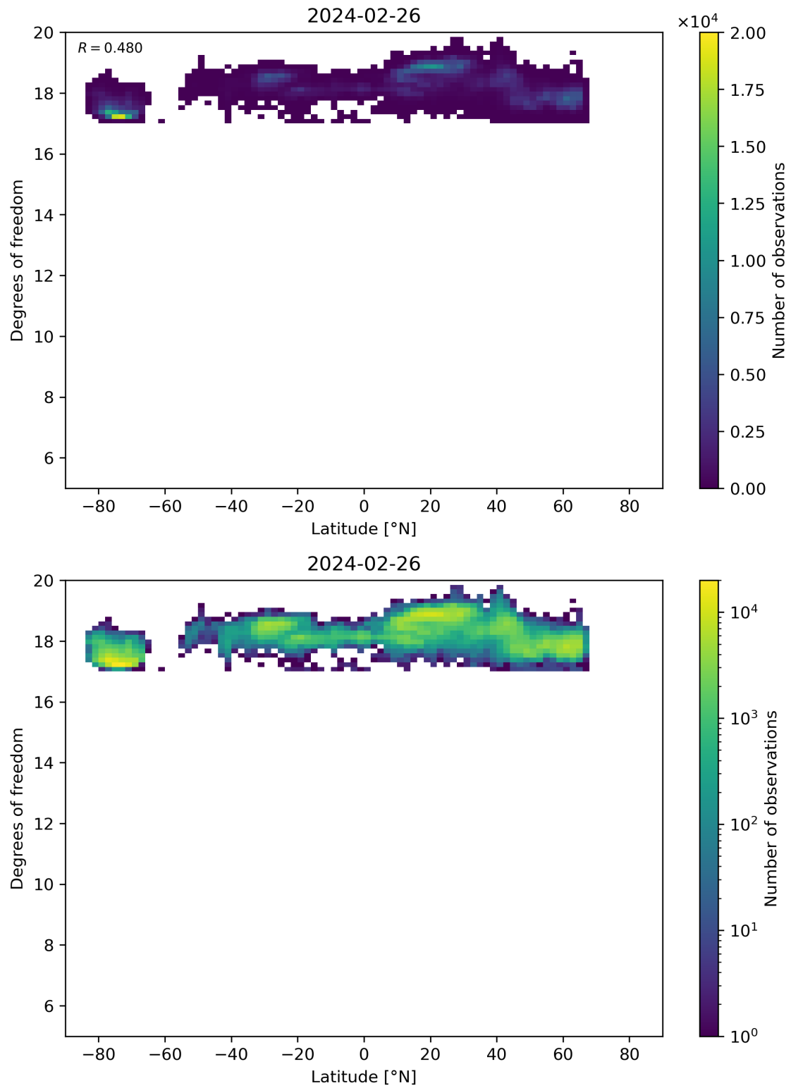
Figure 55: Scatter density plot of “Latitude” against “Degrees of freedom” for 2024-02-25 to 2024-02-27.
