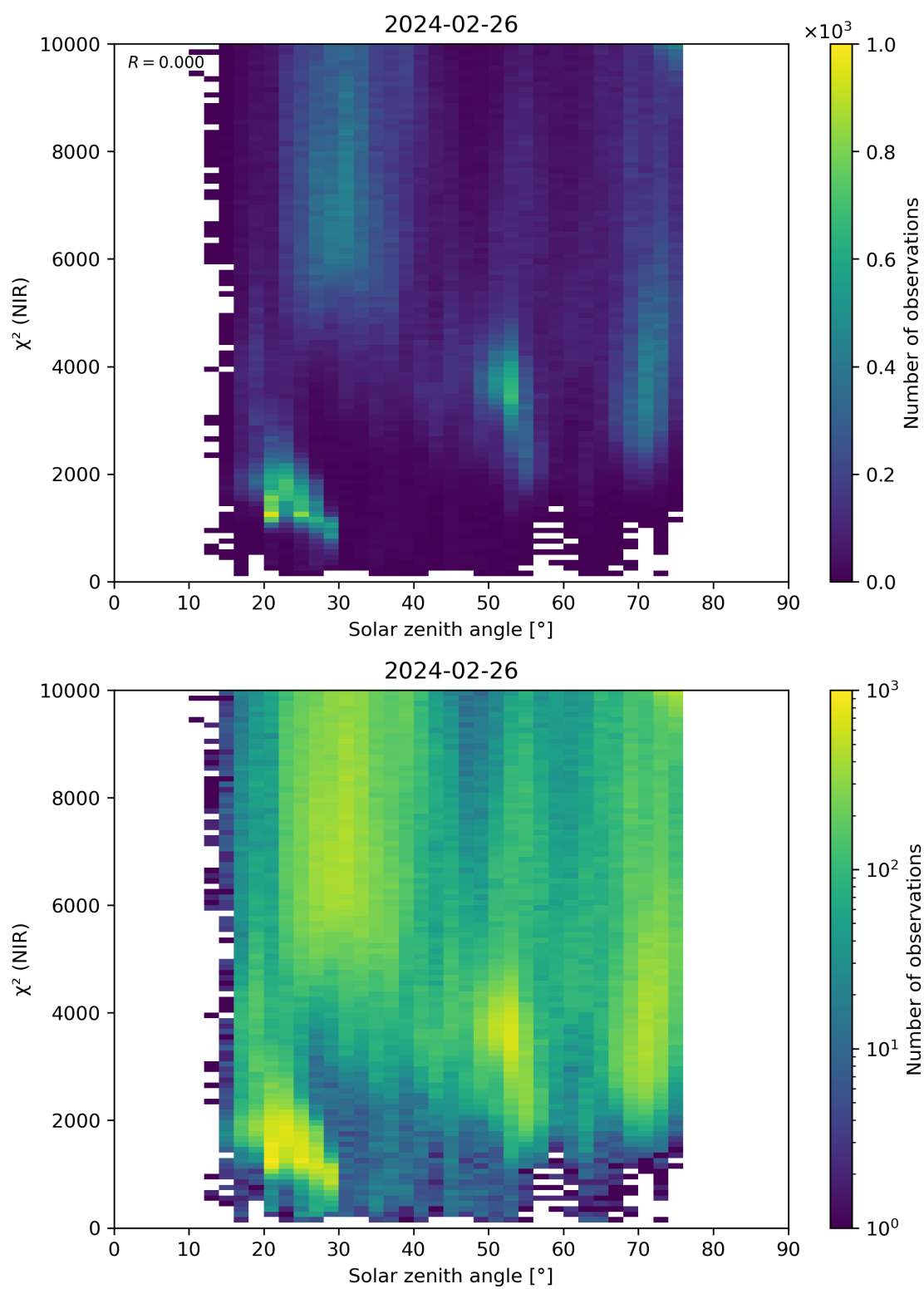
Figure 94: Scatter density plot of “Solar zenith angle” against “ \chi^2 (NIR)” for 2024-02-25 to 2024-02-27.
