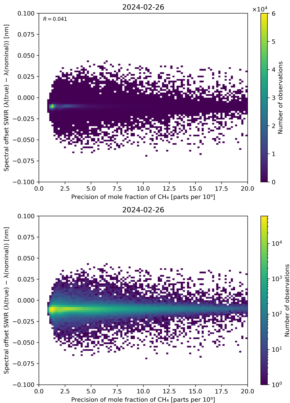
Figure 85: Scatter density plot of “Precision of mole fraction of CH 4 ” against “Spectral offset SWIR ( \lambda(\text{true}) - \lambda(\text{nominal}) )” for 2024-02-25 to 2024-02-27.
