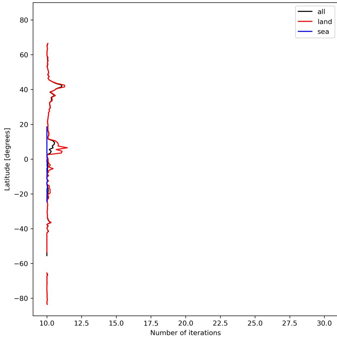
Figure 20: Zonal average of “Number of iterations” for 2024-02-25 to 2024-02-27.
