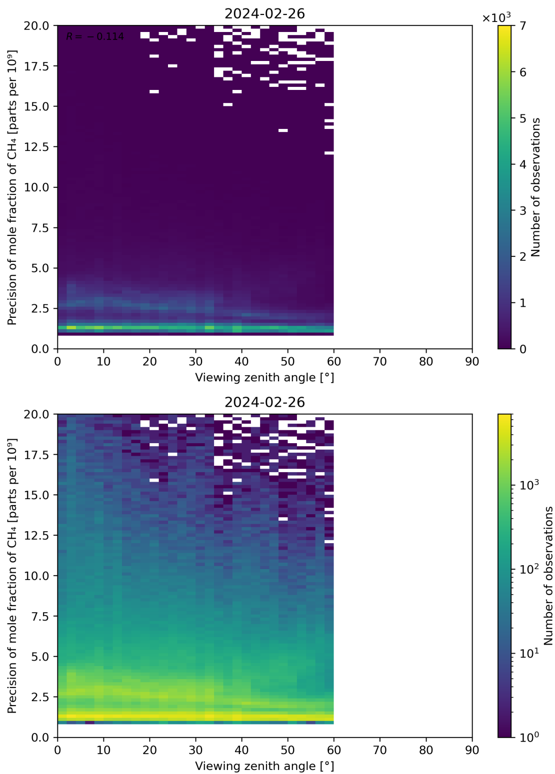
Figure 112: Scatter density plot of “Viewing zenith angle” against “Precision of mole fraction of \text{CH}_4 ” for 2024-02-25 to 2024-02-27.
