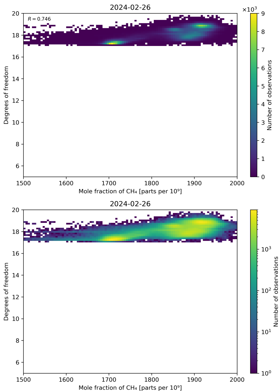
Figure 72: Scatter density plot of “Mole fraction of CH 4 ” against “Degrees of freedom” for 2024-02-25 to 2024-02-27.
