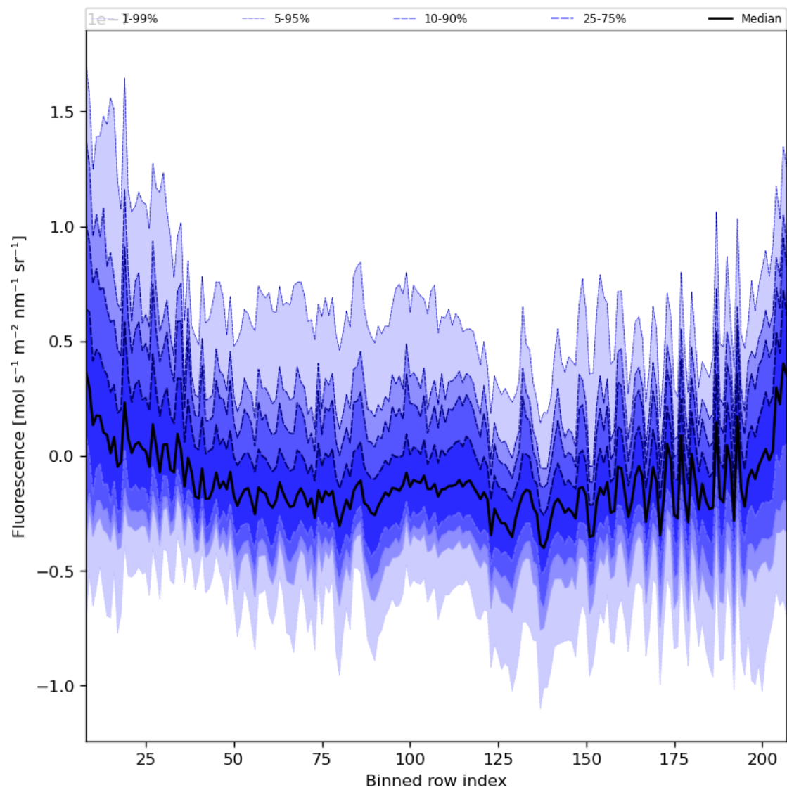
Figure 43: Along track statistics of “Fluorescence” for 2024-02-25 to 2024-02-27
