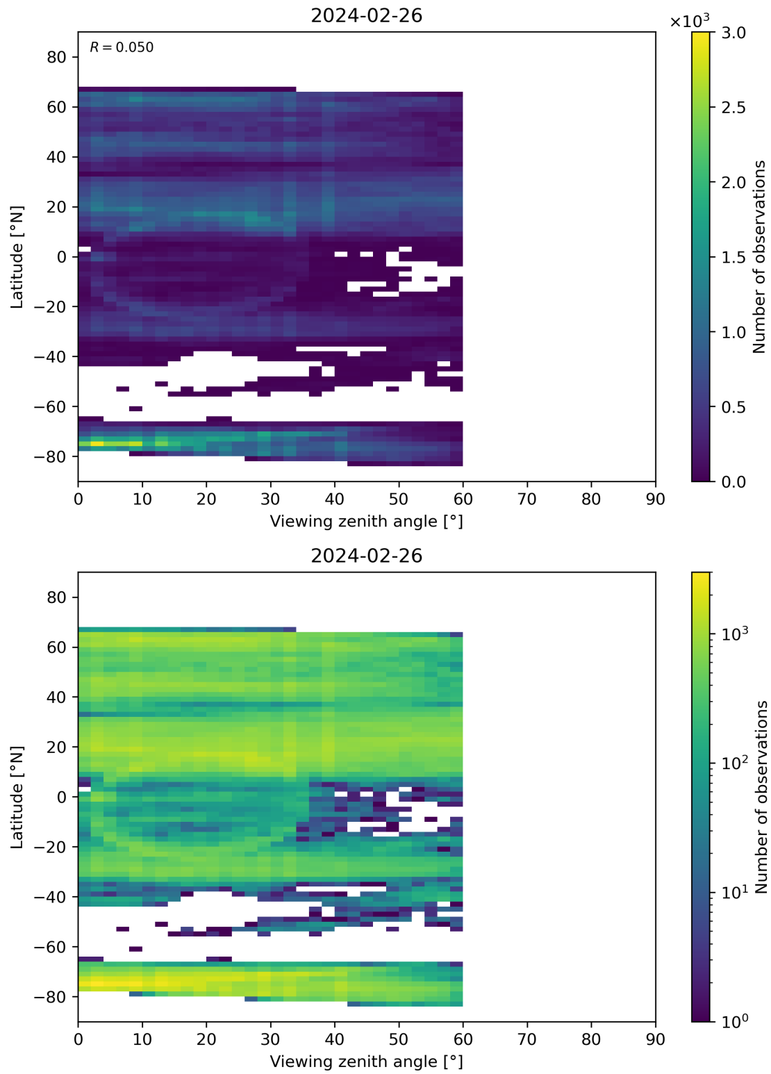
Figure 109: Scatter density plot of “Viewing zenith angle” against “Latitude” for 2024-02-25 to 2024-02-27.
