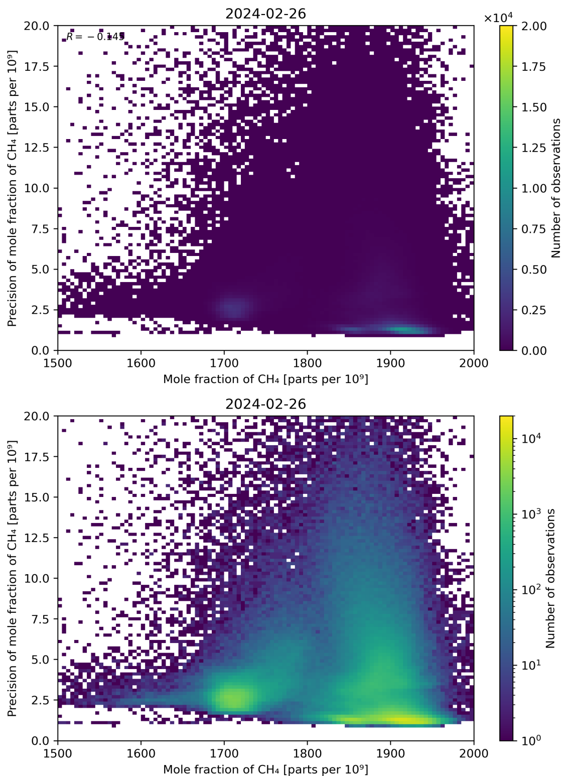
Figure 75: Scatter density plot of “Mole fraction of CH 4 ” against “Precision of mole fraction of CH 4 ” for 2024-02-25 to 2024-02-27.
