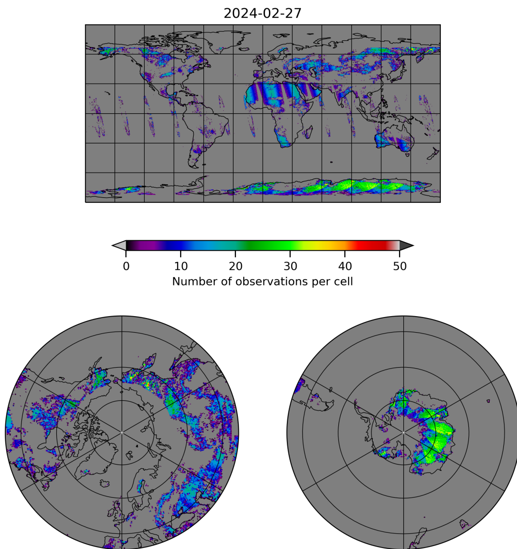
Figure 10: Map of the number of observations for 2024-02-27 to 2024-02-28
