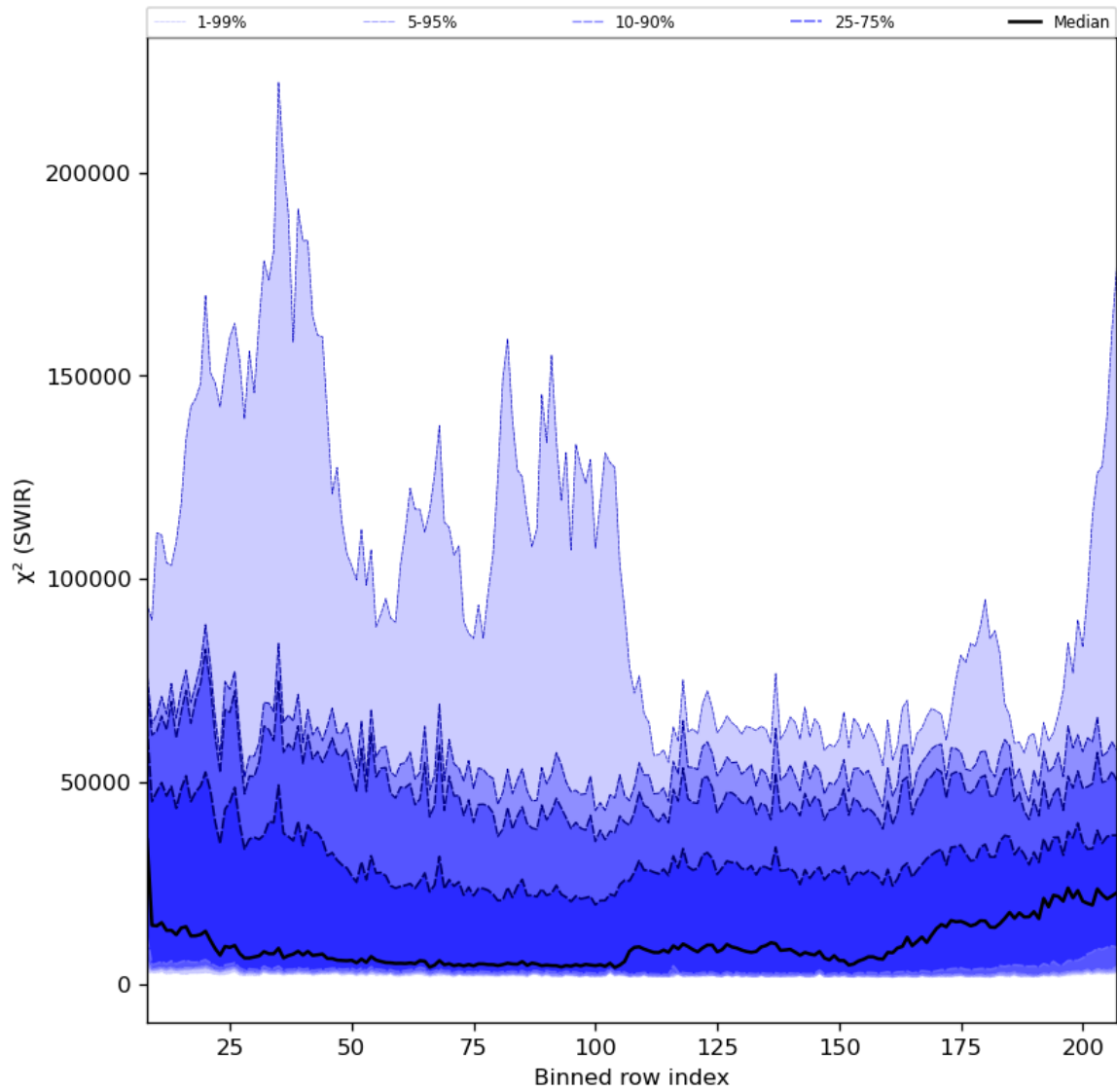
Figure 39: Along track statistics of “ \chi^2 (SWIR)” for 2024-02-27 to 2024-02-28
