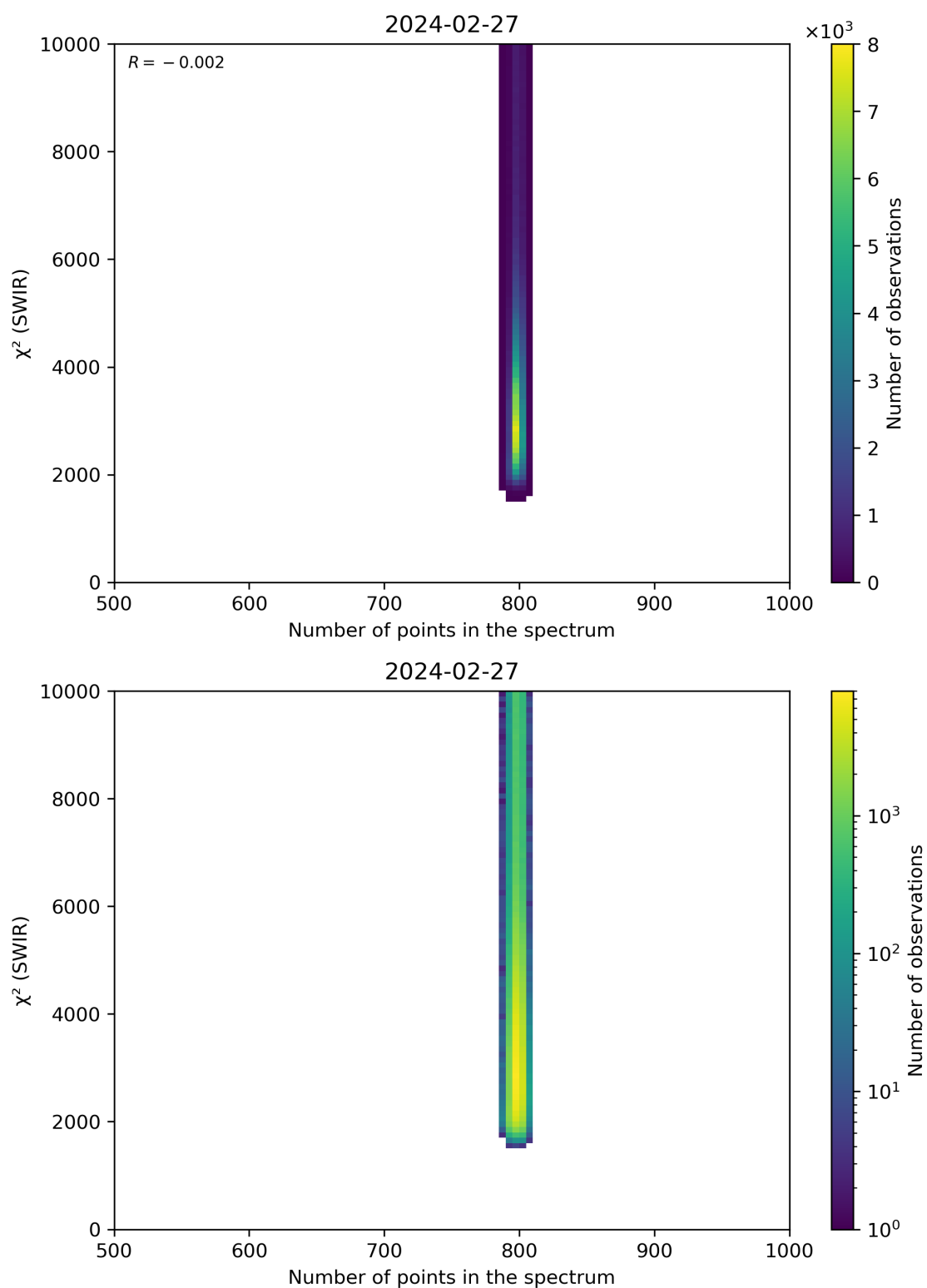
Figure 89: Scatter density plot of “Number of points in the spectrum” against “ \chi^2 (SWIR)” for 2024-02-27 to 2024-02-28.
