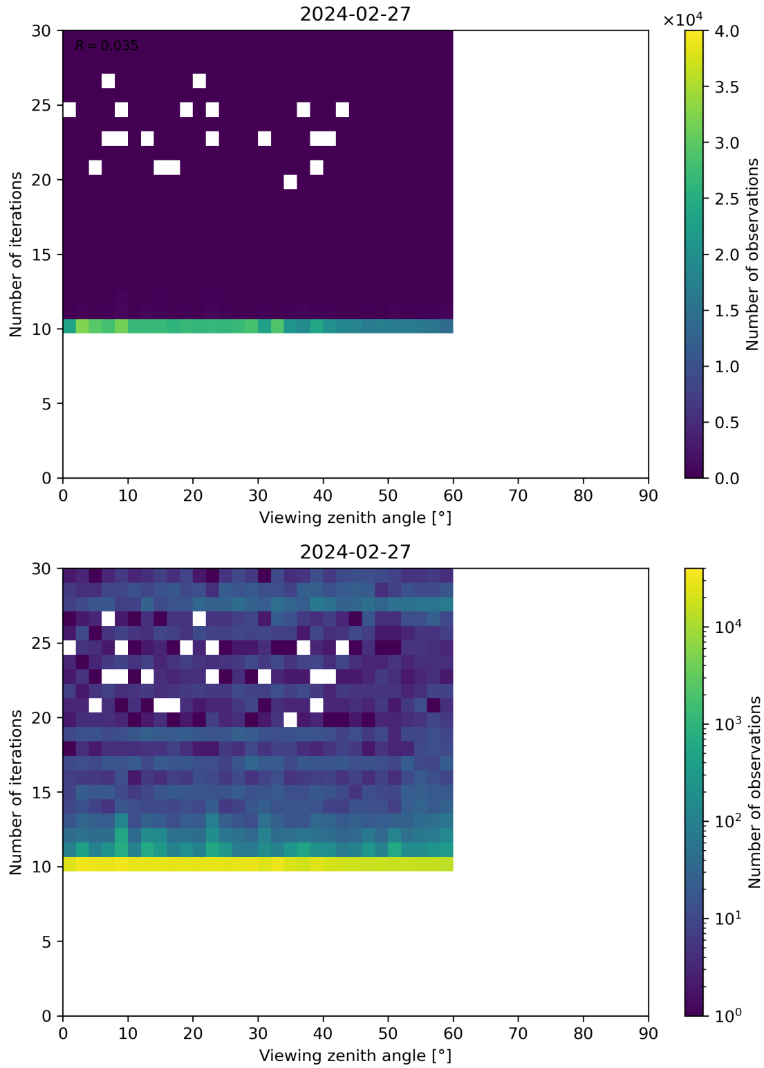
Figure 113: Scatter density plot of “Viewing zenith angle” against “Number of iterations” for 2024-02-27 to 2024-02-28.
