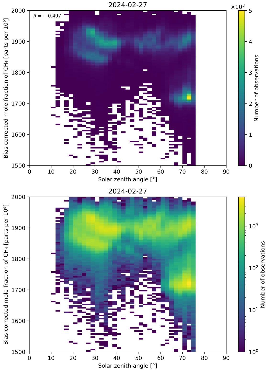
Figure 100: Scatter density plot of “Solar zenith angle” against “Bias corrected mole fraction of \text{CH}_4 ” for 2024-02-27 to 2024-02-28.
