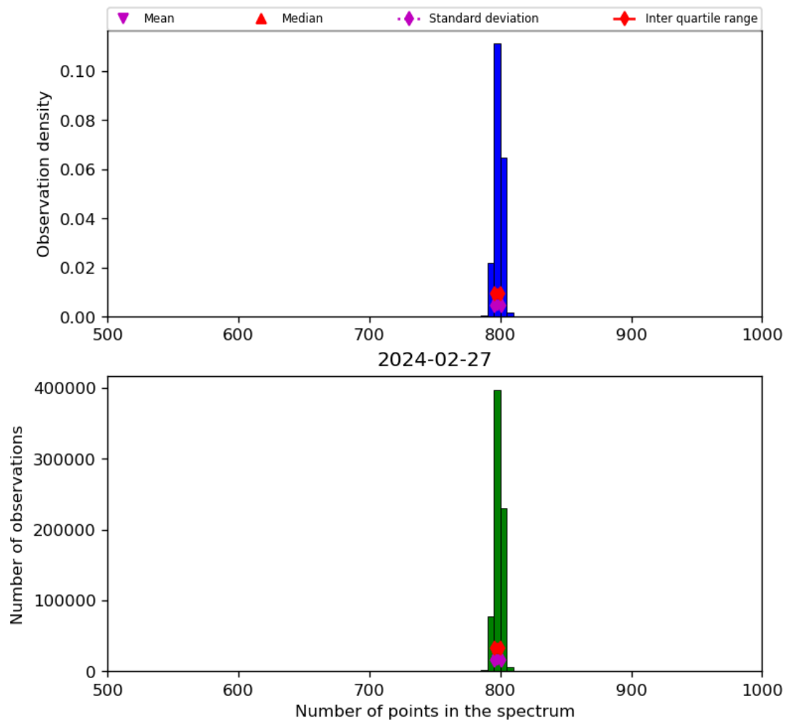
Figure 26: Histogram of “Number of points in the spectrum” for 2024-02-27 to 2024-02-28
