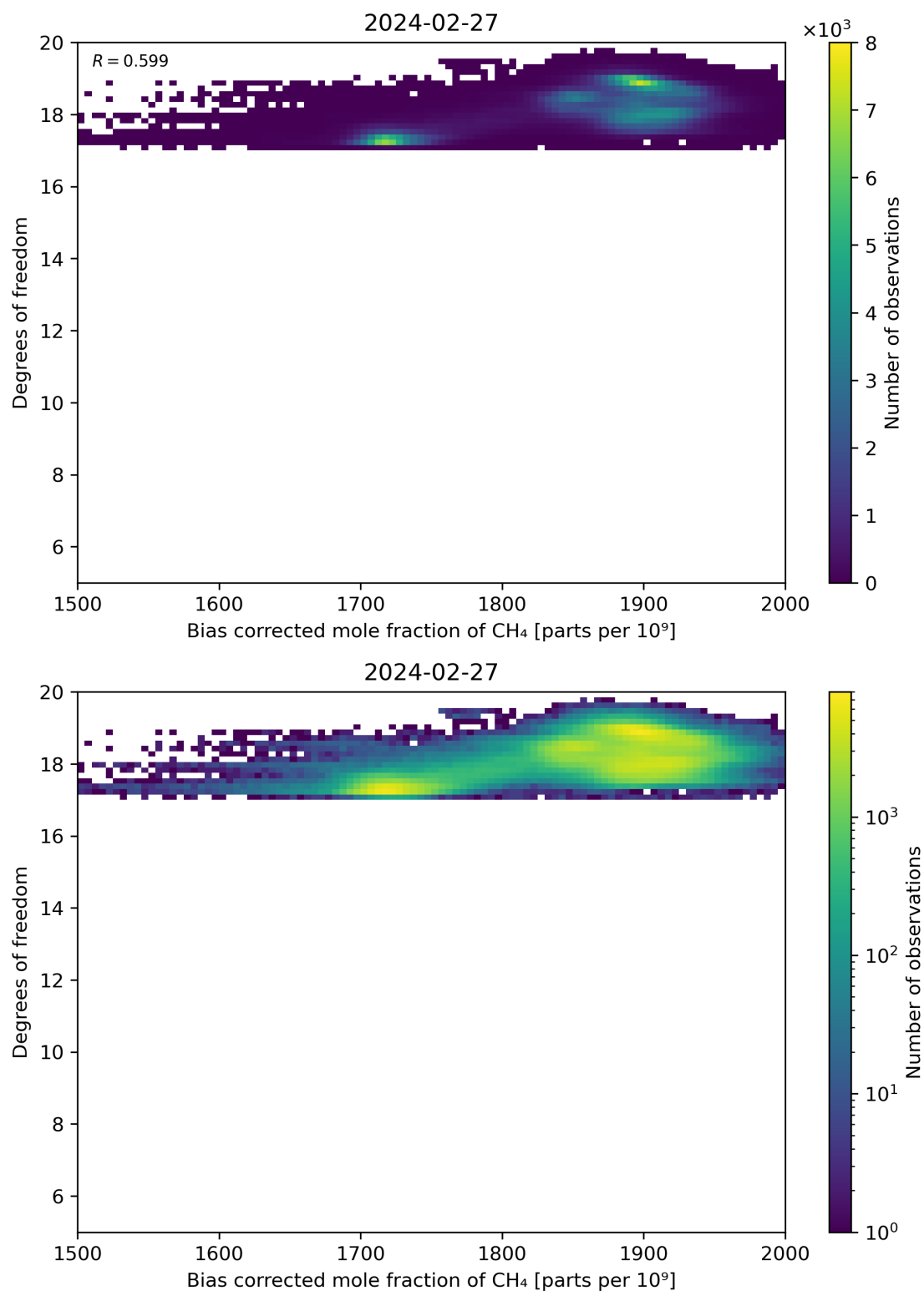
Figure 65: Scatter density plot of “Bias corrected mole fraction of CH 4 ” against “Degrees of freedom” for 2024-02-27 to 2024-02-28.
