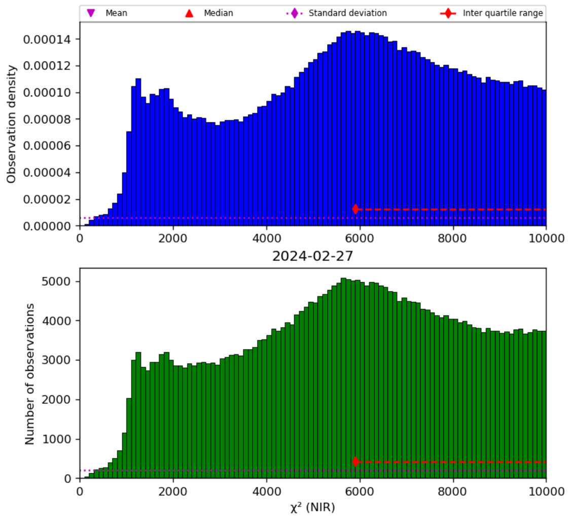
Figure 29: Histogram of “ \chi^2 (NIR)” for 2024-02-27 to 2024-02-28
