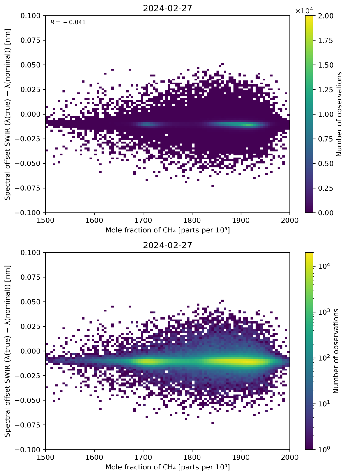
Figure 86: Scatter density plot of “Mole fraction of CH 4 ” against “Spectral offset SWIR ( \lambda(\text{true}) - \lambda(\text{nominal}) )” for 2024-02-27 to 2024-02-28.
