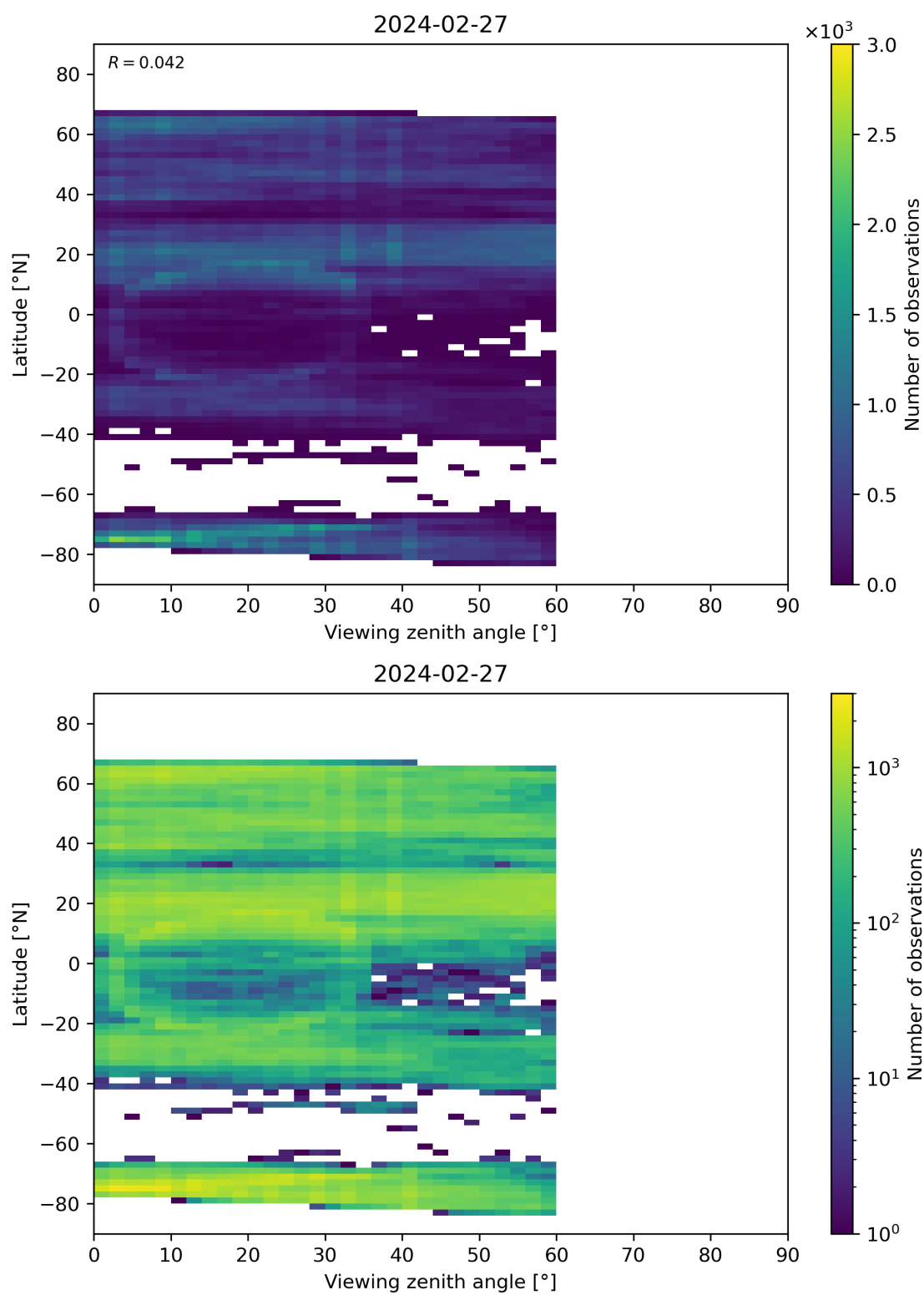
Figure 109: Scatter density plot of “Viewing zenith angle” against “Latitude” for 2024-02-27 to 2024-02-28.
