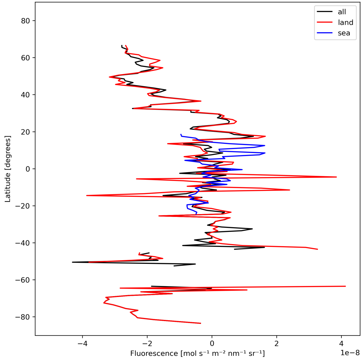
Figure 21: Zonal average of “Fluorescence” for 2024-02-27 to 2024-02-28.
