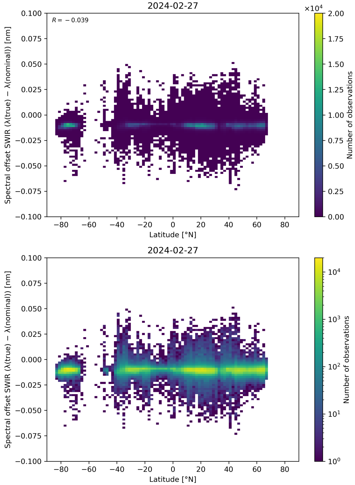
Figure 62: Scatter density plot of “Latitude” against “Spectral offset SWIR ( \lambda(\text{true}) - \lambda(\text{nominal}) )” for 2024-02-27 to 2024-02-28.
