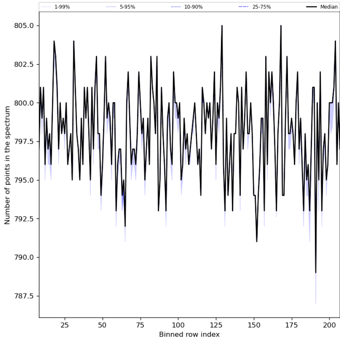
Figure 37: Along track statistics of “Number of points in the spectrum” for 2024-02-27 to 2024-02-28
