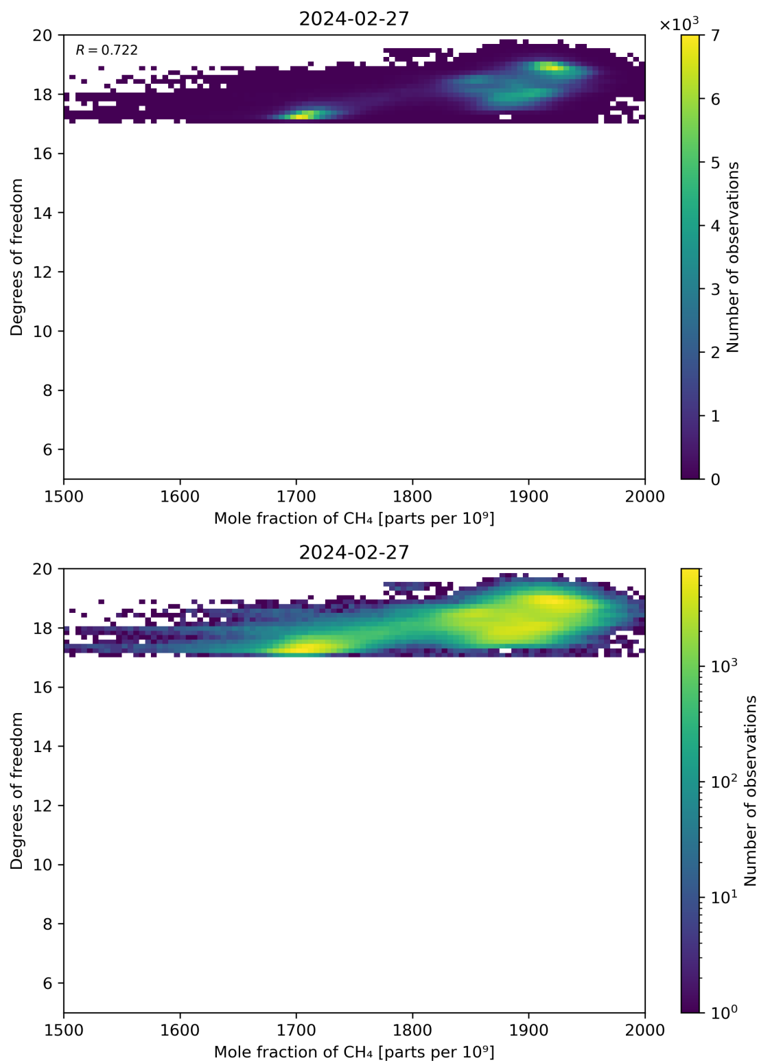
Figure 72: Scatter density plot of “Mole fraction of CH 4 ” against “Degrees of freedom” for 2024-02-27 to 2024-02-28.
