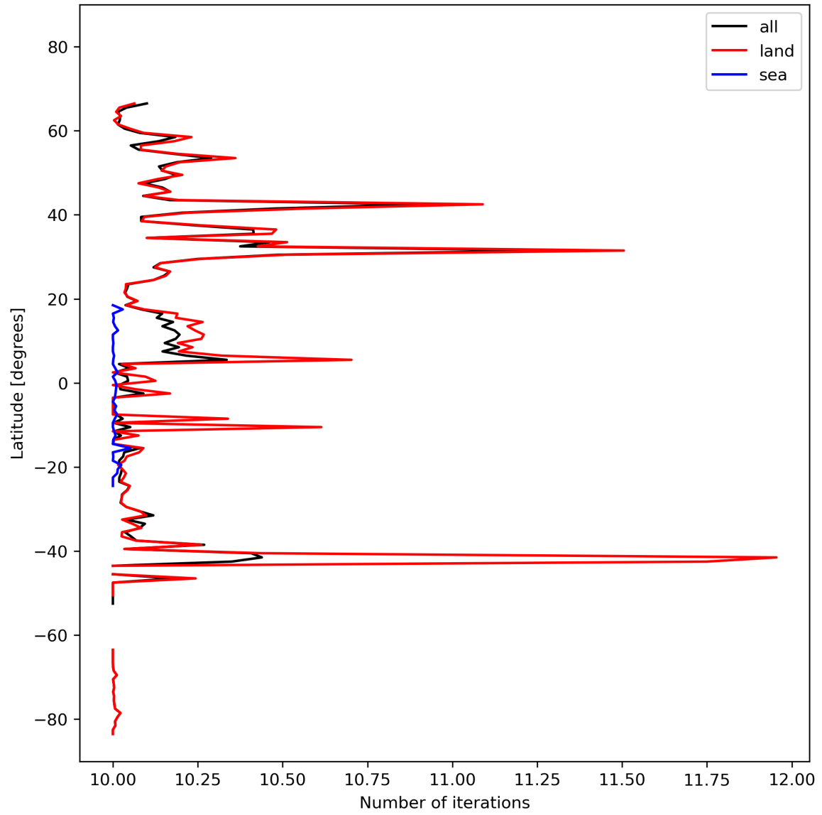
Figure 20: Zonal average of “Number of iterations” for 2024-02-27 to 2024-02-28.
