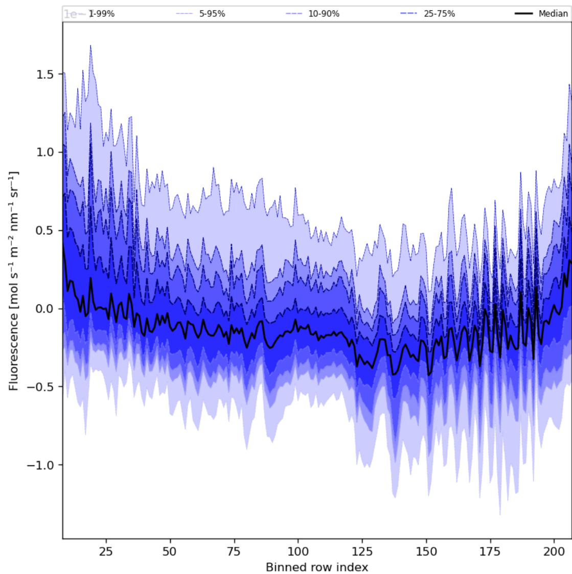
Figure 43: Along track statistics of “Fluorescence” for 2024-02-27 to 2024-02-28
