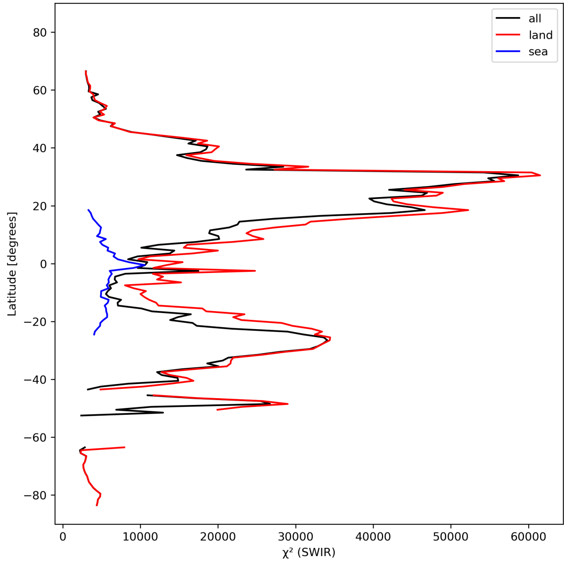
Figure 17: Zonal average of “ \chi^2 (SWIR)” for 2024-02-27 to 2024-02-28.
