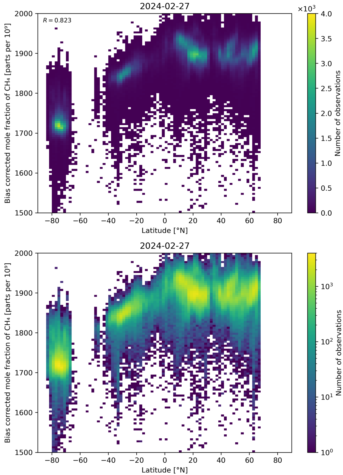
Figure 58: Scatter density plot of “Latitude” against “Bias corrected mole fraction of CH 4 ” for 2024-02-27 to 2024-02-28.
