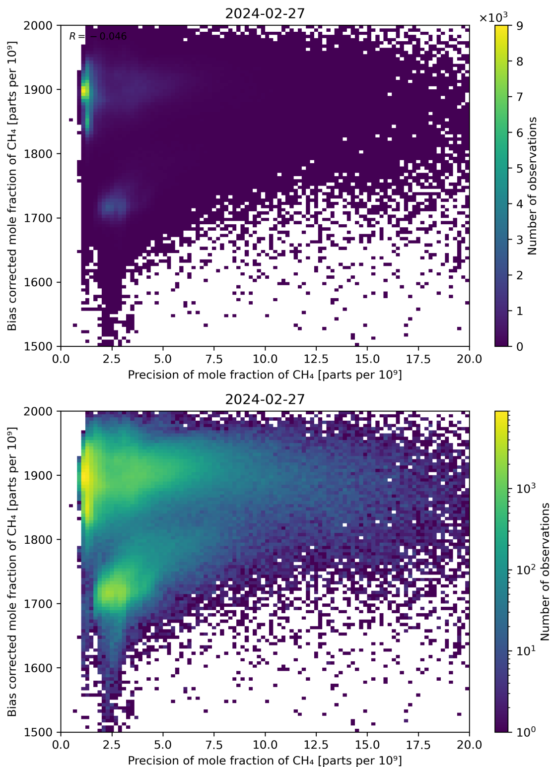
Figure 82: Scatter density plot of “Precision of mole fraction of \text{CH}_4 ” against “Bias corrected mole fraction of \text{CH}_4 ” for 2024-02-27 to 2024-02-28.
