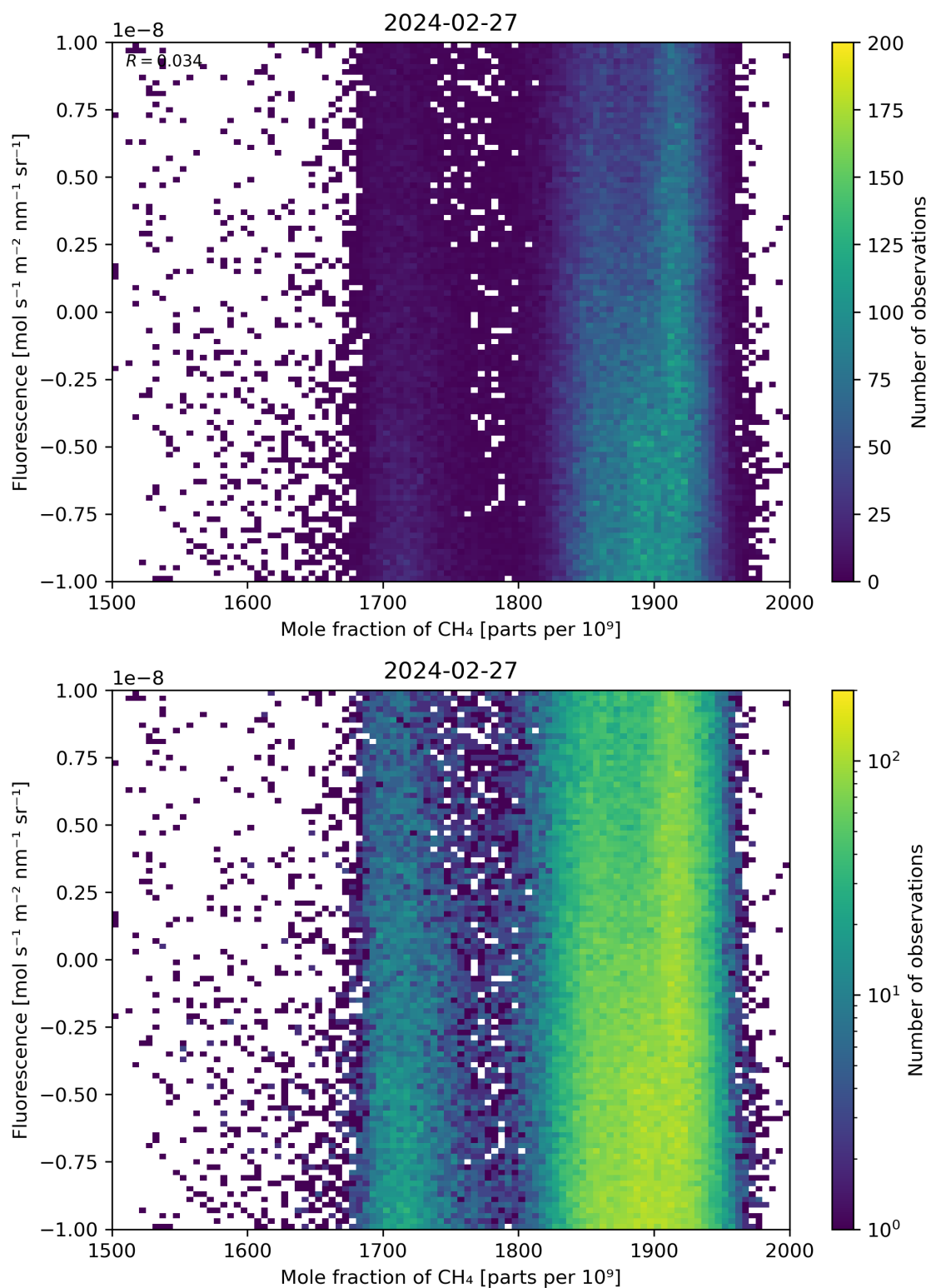
Figure 73: Scatter density plot of “Mole fraction of \text{CH}_4 ” against “Fluorescence” for 2024-02-27 to 2024-02-28.
