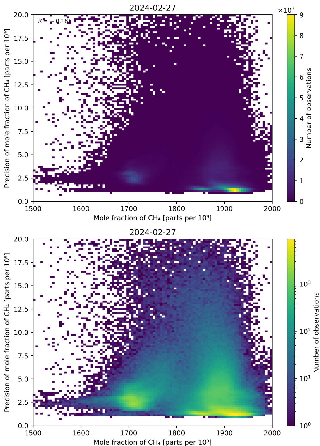
Figure 75: Scatter density plot of “Mole fraction of CH 4 ” against “Precision of mole fraction of CH 4 ” for 2024-02-27 to 2024-02-28.
