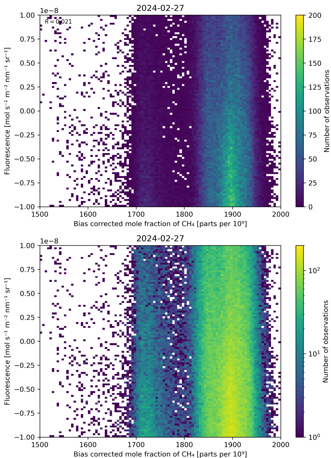
Figure 66: Scatter density plot of “Bias corrected mole fraction of CH 4 ” against “Fluorescence” for 2024-02-27 to 2024-02-28.
