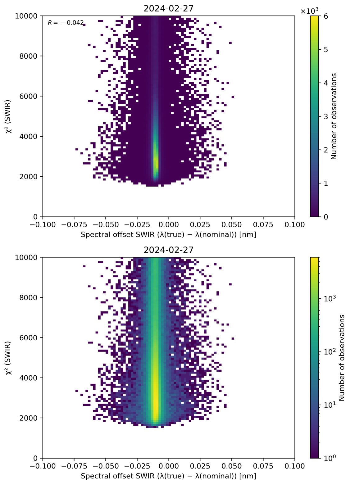
Figure 118: Scatter density plot of “Spectral offset SWIR ( \lambda(\text{true}) - \lambda(\text{nominal}) )” against “ \chi^2 (SWIR)” for 2024-02-27 to 2024-02-28.
