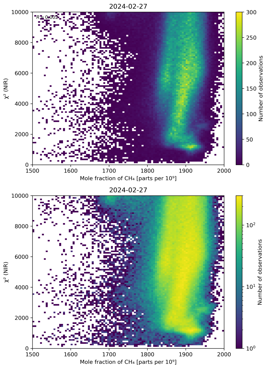
Figure 70: Scatter density plot of “Mole fraction of \text{CH}_4 ” against “ \chi^2 (NIR)” for 2024-02-27 to 2024-02-28.
