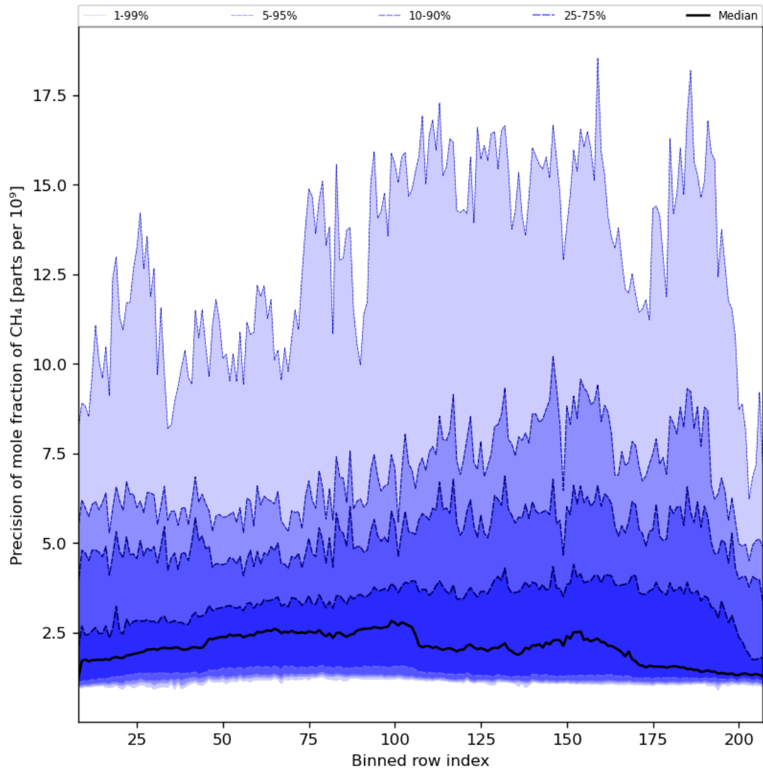
Figure 35: Along track statistics of “Precision of mole fraction of CH 4 ” for 2024-02-27 to 2024-02-28
