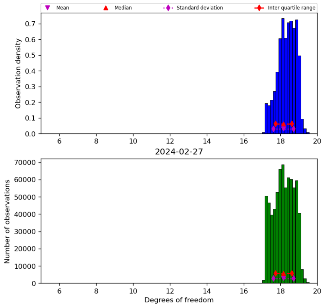
Figure 30: Histogram of “Degrees of freedom” for 2024-02-27 to 2024-02-28
