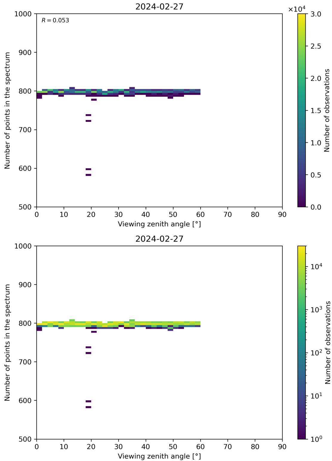
Figure 114: Scatter density plot of “Viewing zenith angle” against “Number of points in the spectrum” for 2024-02-27 to 2024-02-28.
