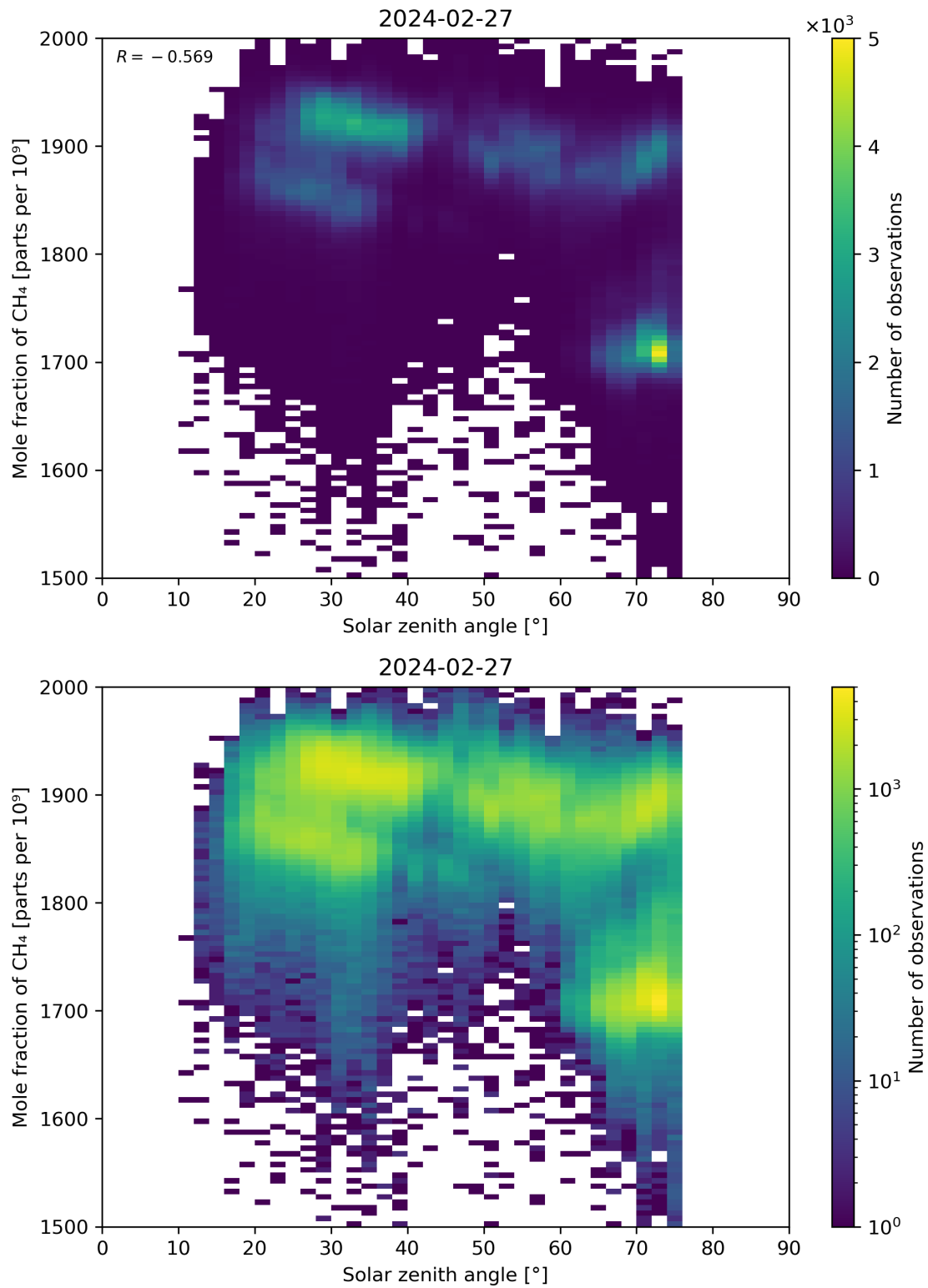
Figure 99: Scatter density plot of “Solar zenith angle” against “Mole fraction of \text{CH}_4 ” for 2024-02-27 to 2024-02-28.
