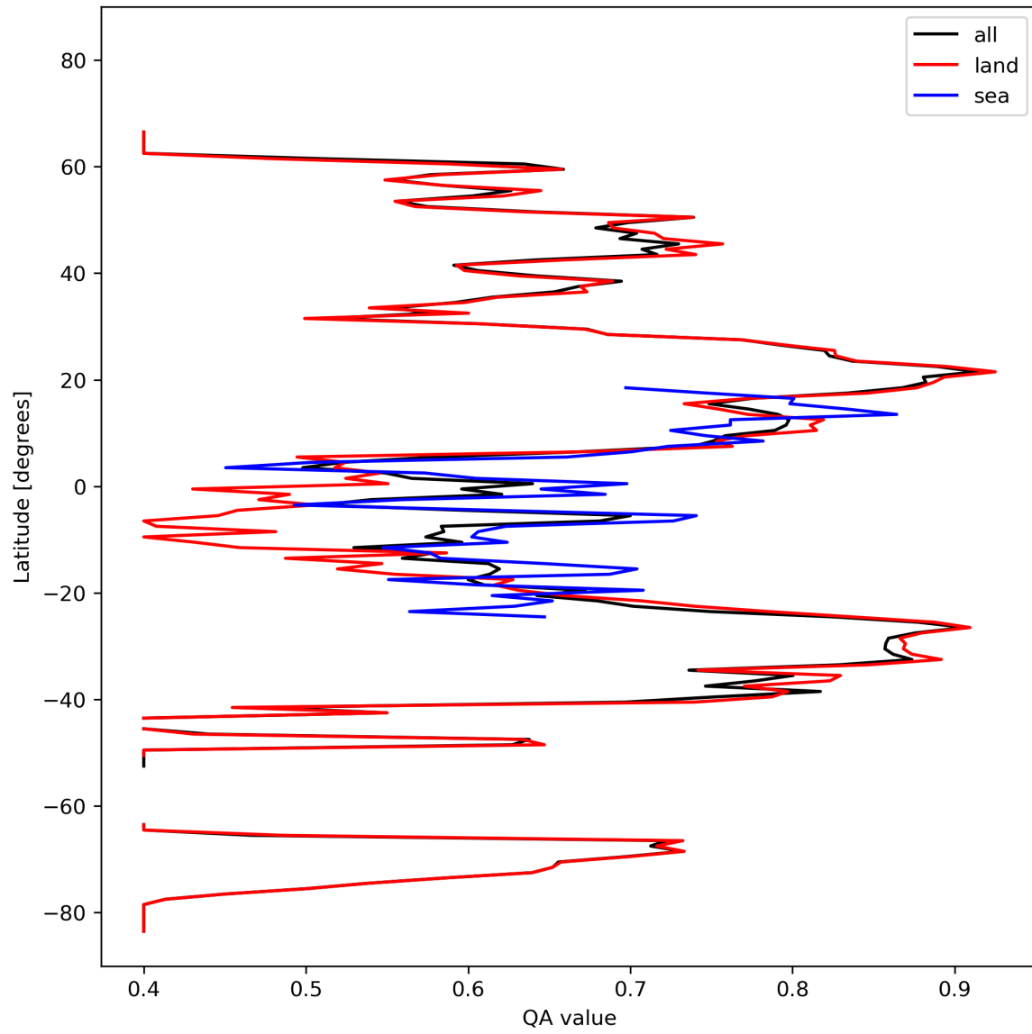
Figure 11: Zonal average of “QA value” for 2024-02-27 to 2024-02-28.
