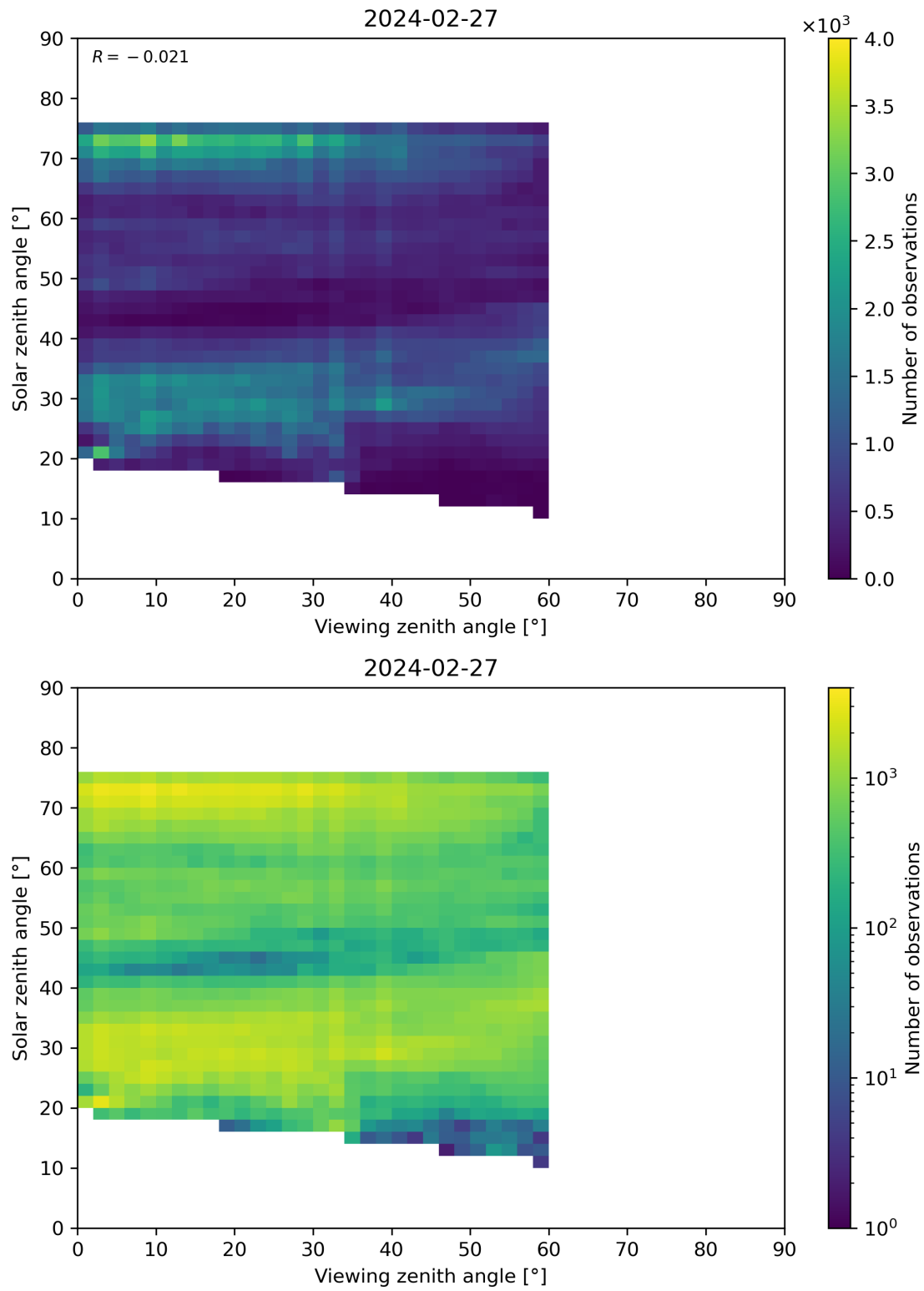
Figure 115: Scatter density plot of “Viewing zenith angle” against “Solar zenith angle” for 2024-02-27 to 2024-02-28.
