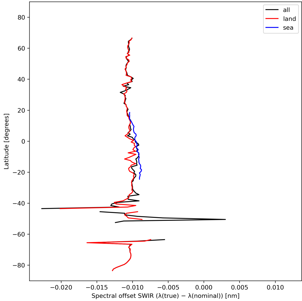
Figure 16: Zonal average of “Spectral offset SWIR ( \lambda(\text{true}) - \lambda(\text{nominal}) )” for 2024-02-27 to 2024-02-28.
