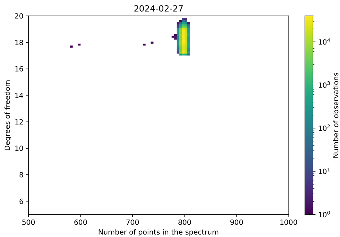
Figure 90: Scatter density plot of “Number of points in the spectrum” against “Degrees of freedom” for 2024-02-27 to 2024-02-28.
