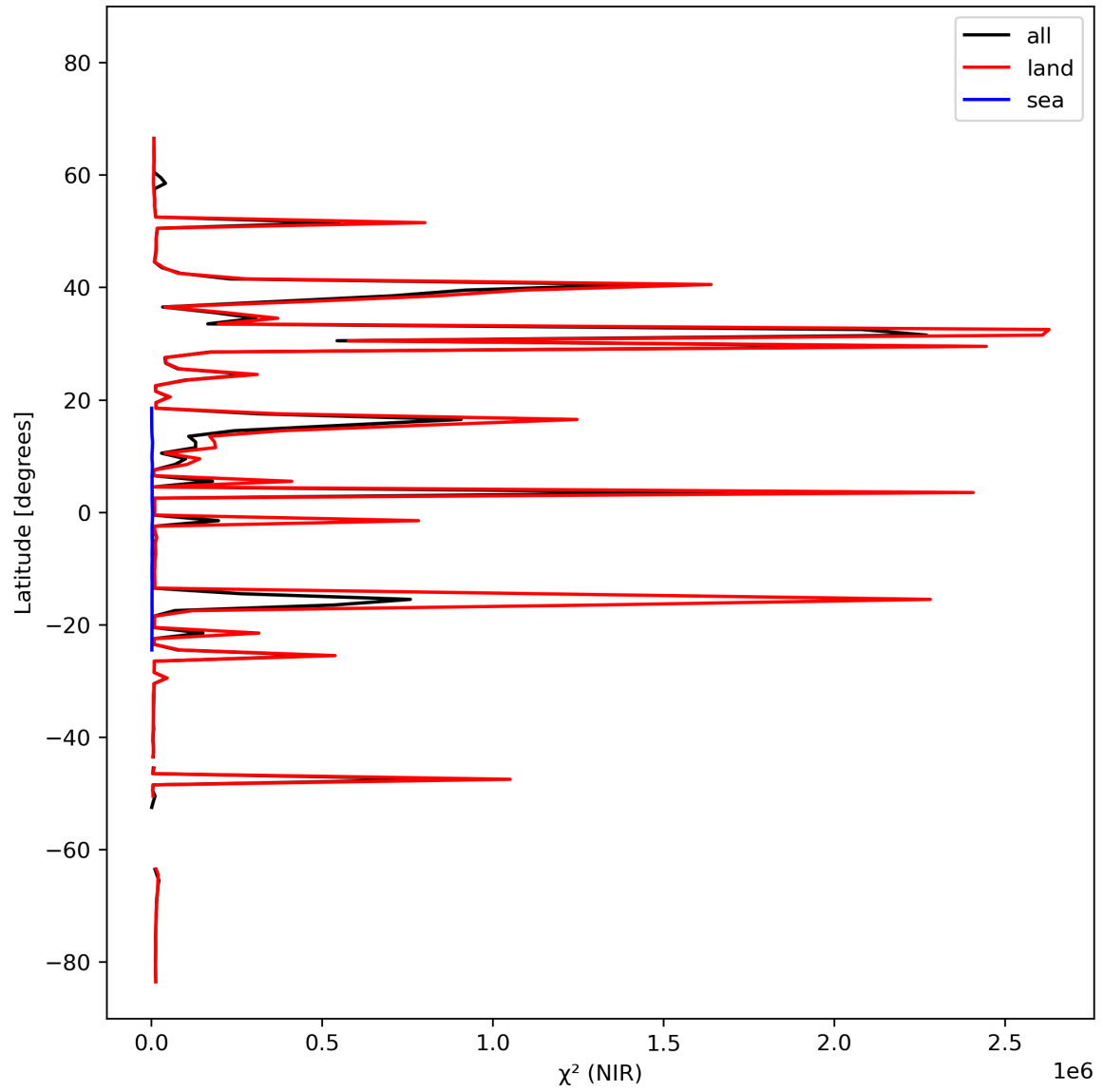
Figure 18: Zonal average of “ \chi^2 (NIR)” for 2024-02-27 to 2024-02-28.
