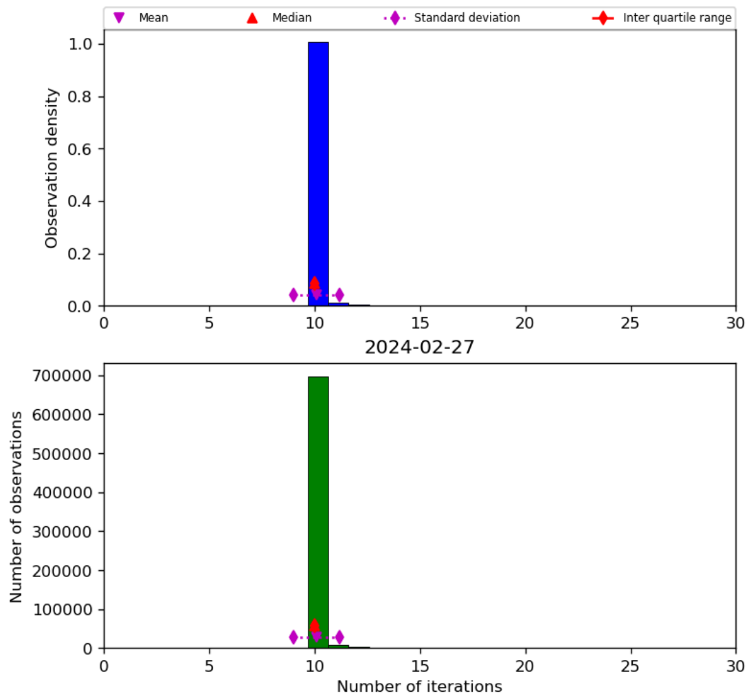
Figure 31: Histogram of “Number of iterations” for 2024-02-27 to 2024-02-28
