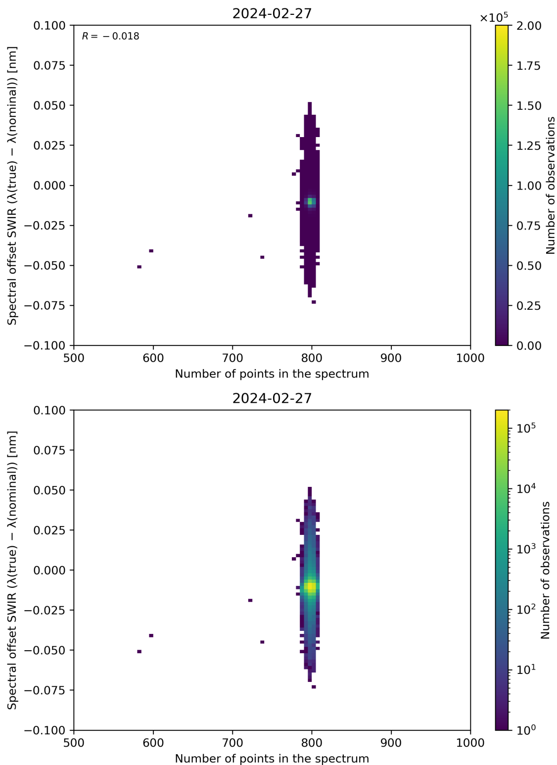
Figure 93: Scatter density plot of “Number of points in the spectrum” against “Spectral offset SWIR ( \lambda(\text{true}) - \lambda(\text{nominal}) )” for 2024-02-27 to 2024-02-28.
