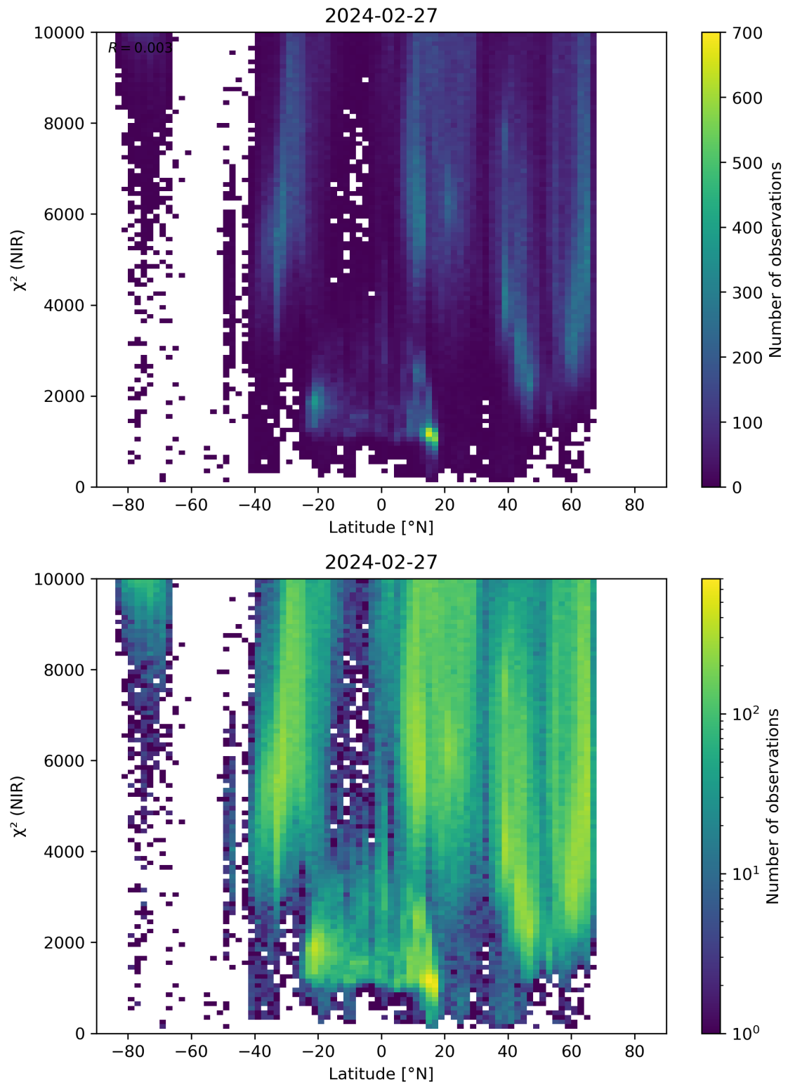
Figure 53: Scatter density plot of “Latitude” against “ \chi^2 (NIR)” for 2024-02-27 to 2024-02-28.
