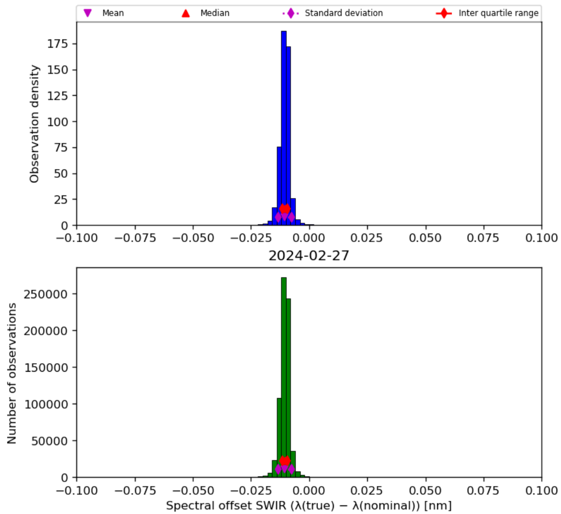
Figure 27: Histogram of “Spectral offset SWIR ( \lambda(\text{true}) - \lambda(\text{nominal}) )” for 2024-02-27 to 2024-02-28
