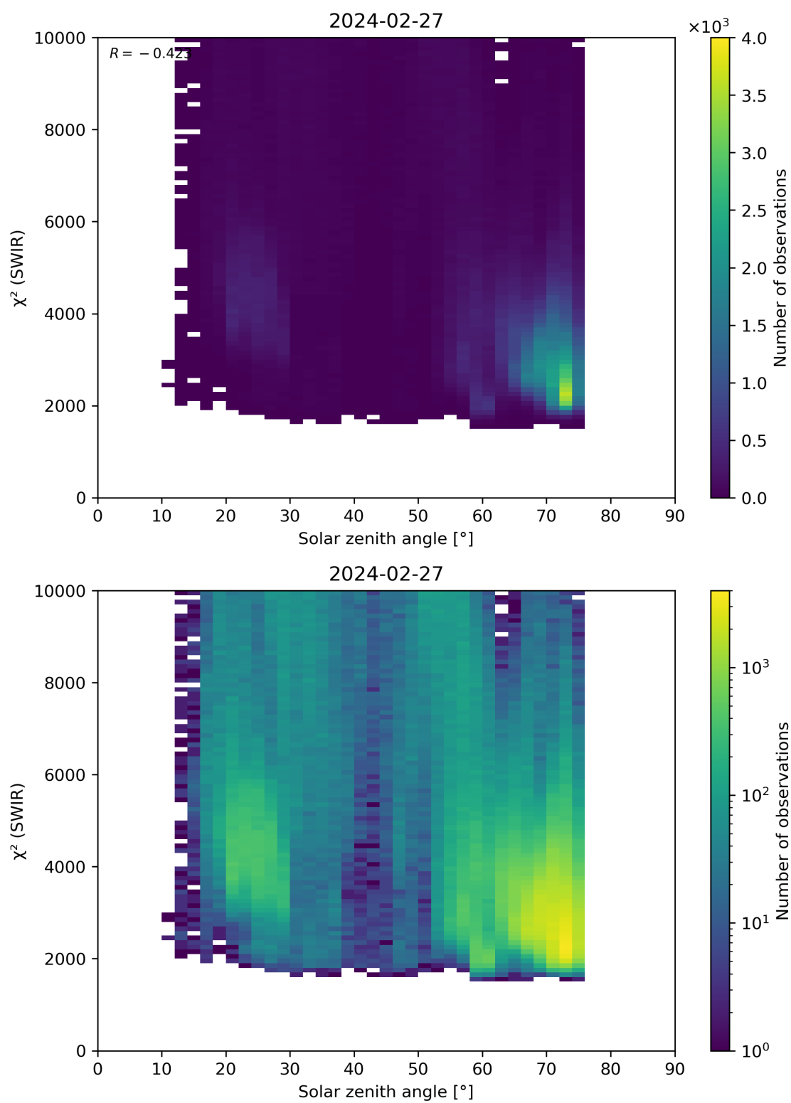
Figure 95: Scatter density plot of “Solar zenith angle” against “ \chi^2 (SWIR)” for 2024-02-27 to 2024-02-28.
