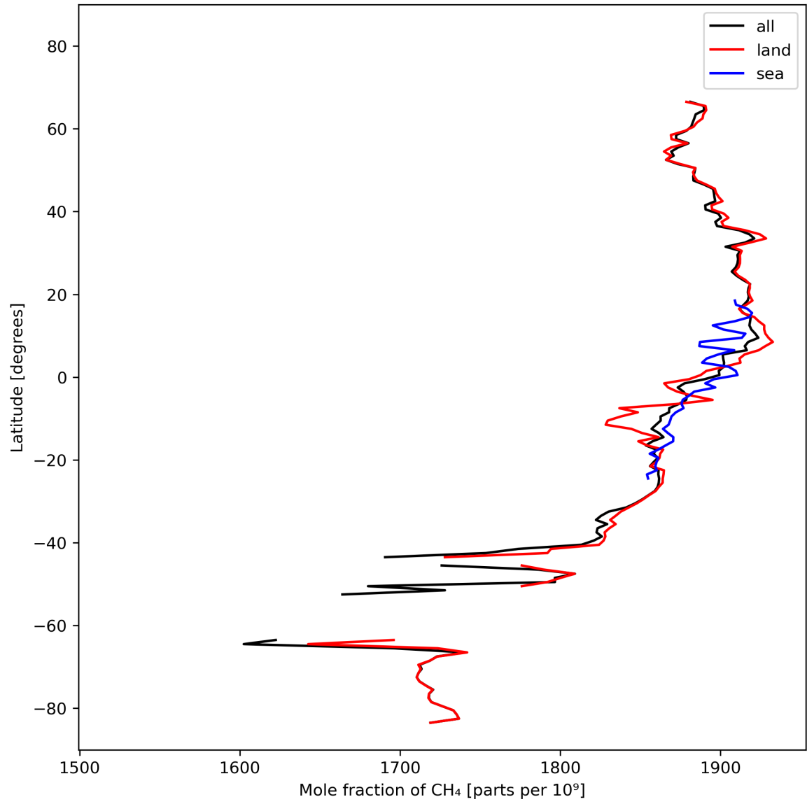
Figure 12: Zonal average of “Mole fraction of \text{CH}_4 ” for 2024-02-27 to 2024-02-28.
