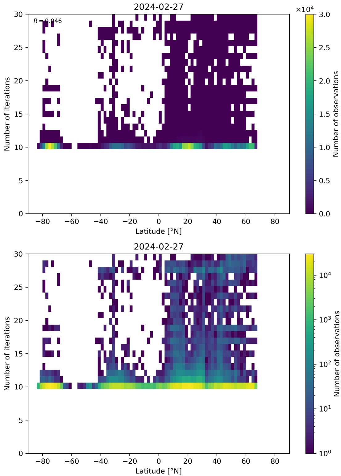
Figure 60: Scatter density plot of “Latitude” against “Number of iterations” for 2024-02-27 to 2024-02-28.
