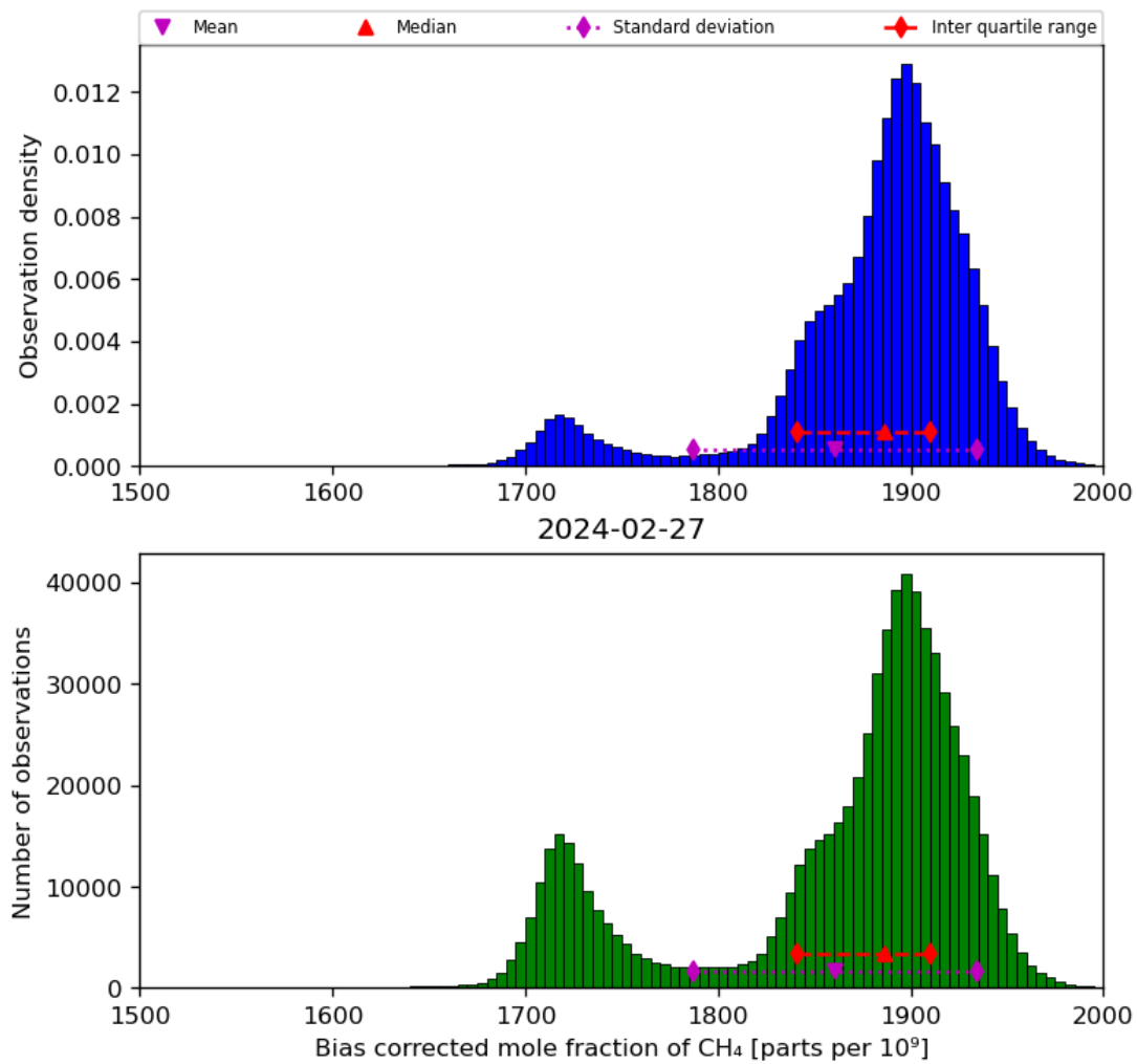
Figure 25: Histogram of “Bias corrected mole fraction of CH 4 ” for 2024-02-27 to 2024-02-28
