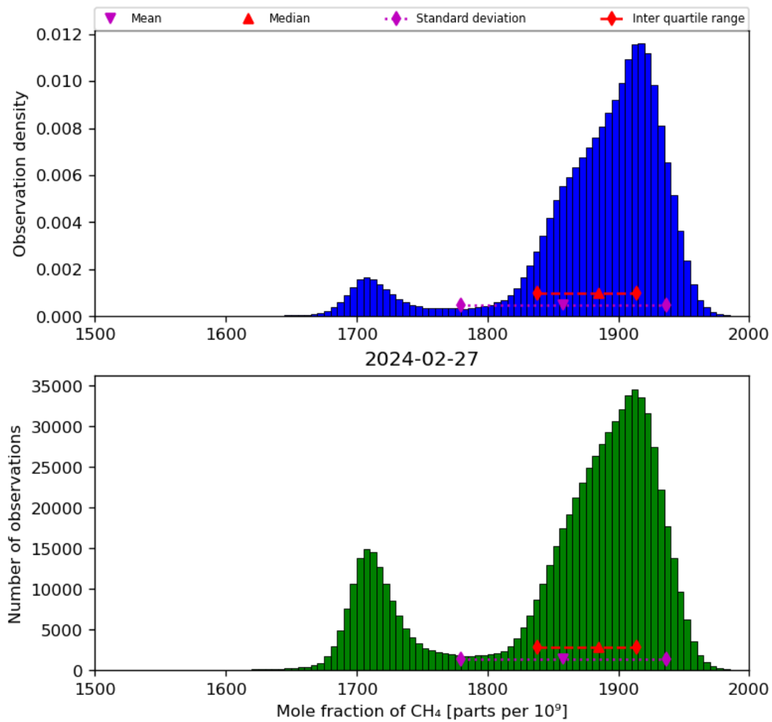
Figure 23: Histogram of “Mole fraction of CH 4 ” for 2024-02-27 to 2024-02-28
