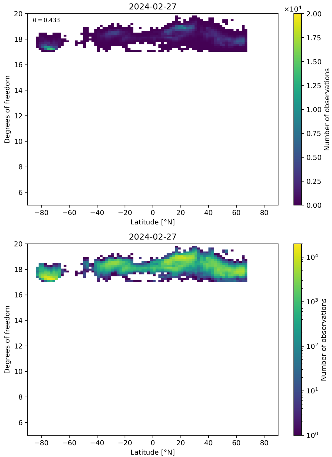
Figure 55: Scatter density plot of “Latitude” against “Degrees of freedom” for 2024-02-27 to 2024-02-28.
