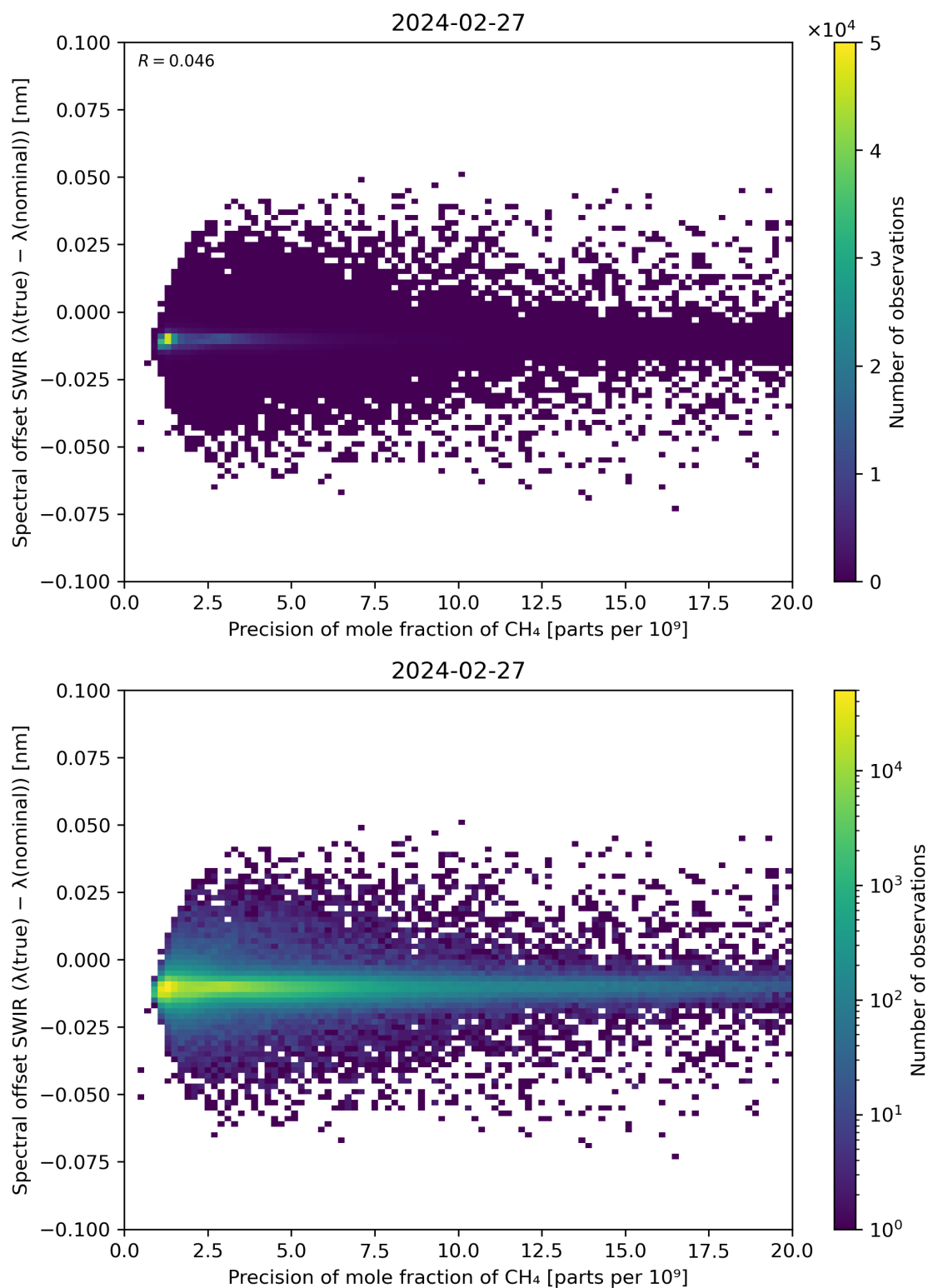
Figure 85: Scatter density plot of “Precision of mole fraction of \text{CH}_4 ” against “Spectral offset SWIR ( \lambda(\text{true}) - \lambda(\text{nominal}) )” for 2024-02-27 to 2024-02-28.
