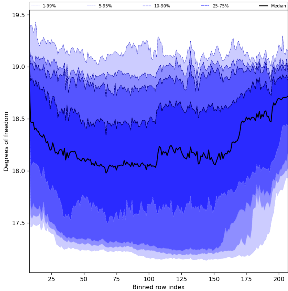
Figure 41: Along track statistics of “Degrees of freedom” for 2024-02-27 to 2024-02-28
