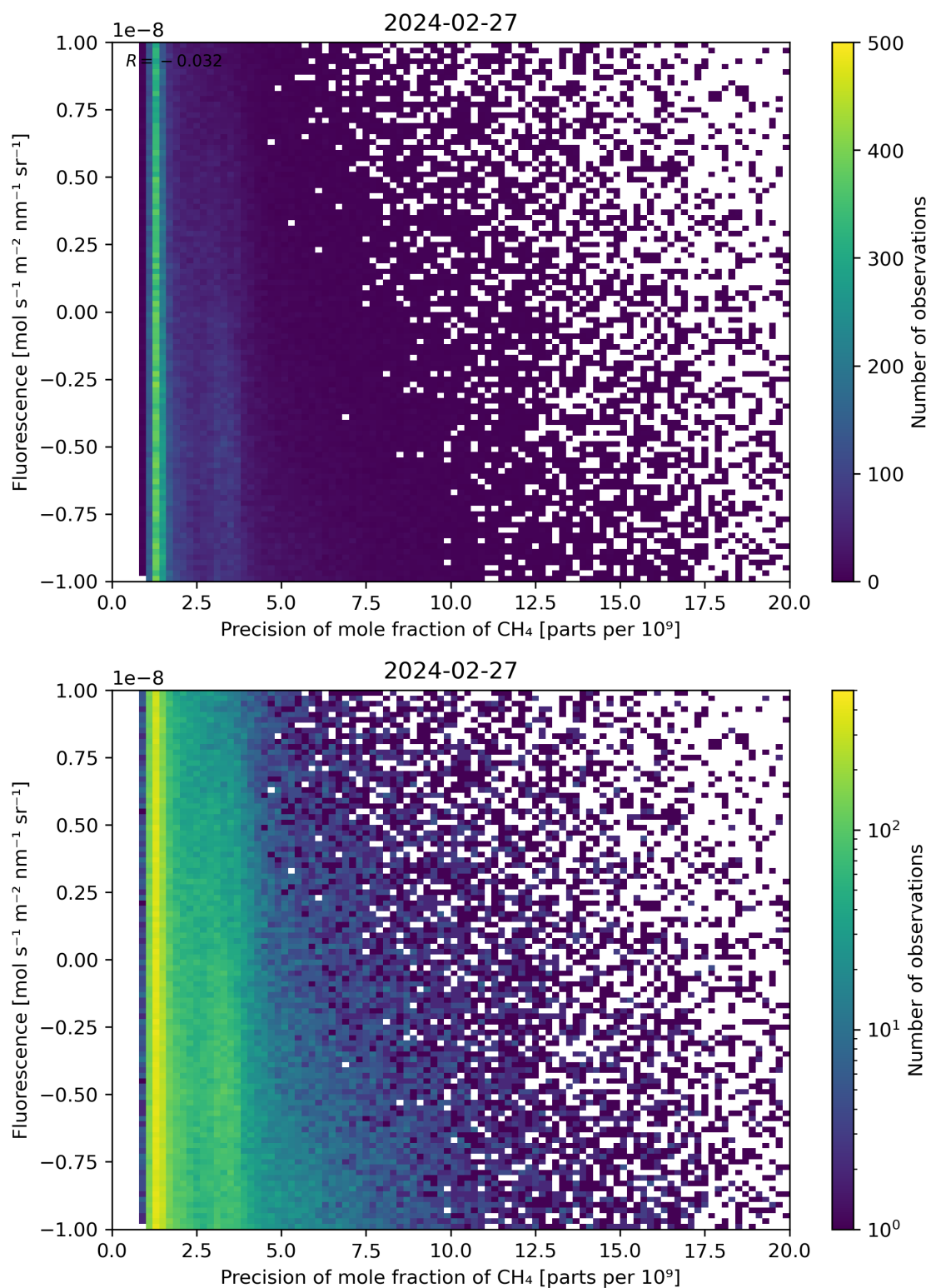
Figure 81: Scatter density plot of “Precision of mole fraction of CH 4 ” against “Fluorescence” for 2024-02-27 to 2024-02-28.
