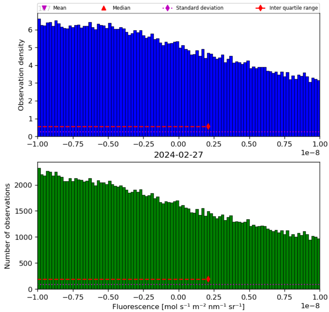
Figure 32: Histogram of “Fluorescence” for 2024-02-27 to 2024-02-28
