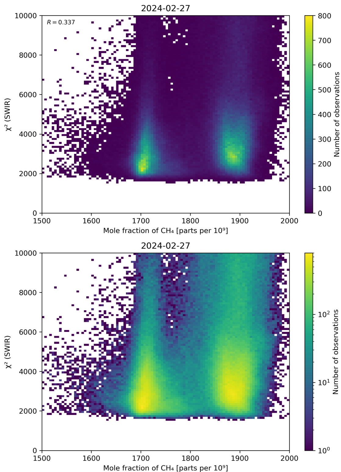
Figure 71: Scatter density plot of “Mole fraction of \text{CH}_4 ” against “ \chi^2 (SWIR)” for 2024-02-27 to 2024-02-28.
