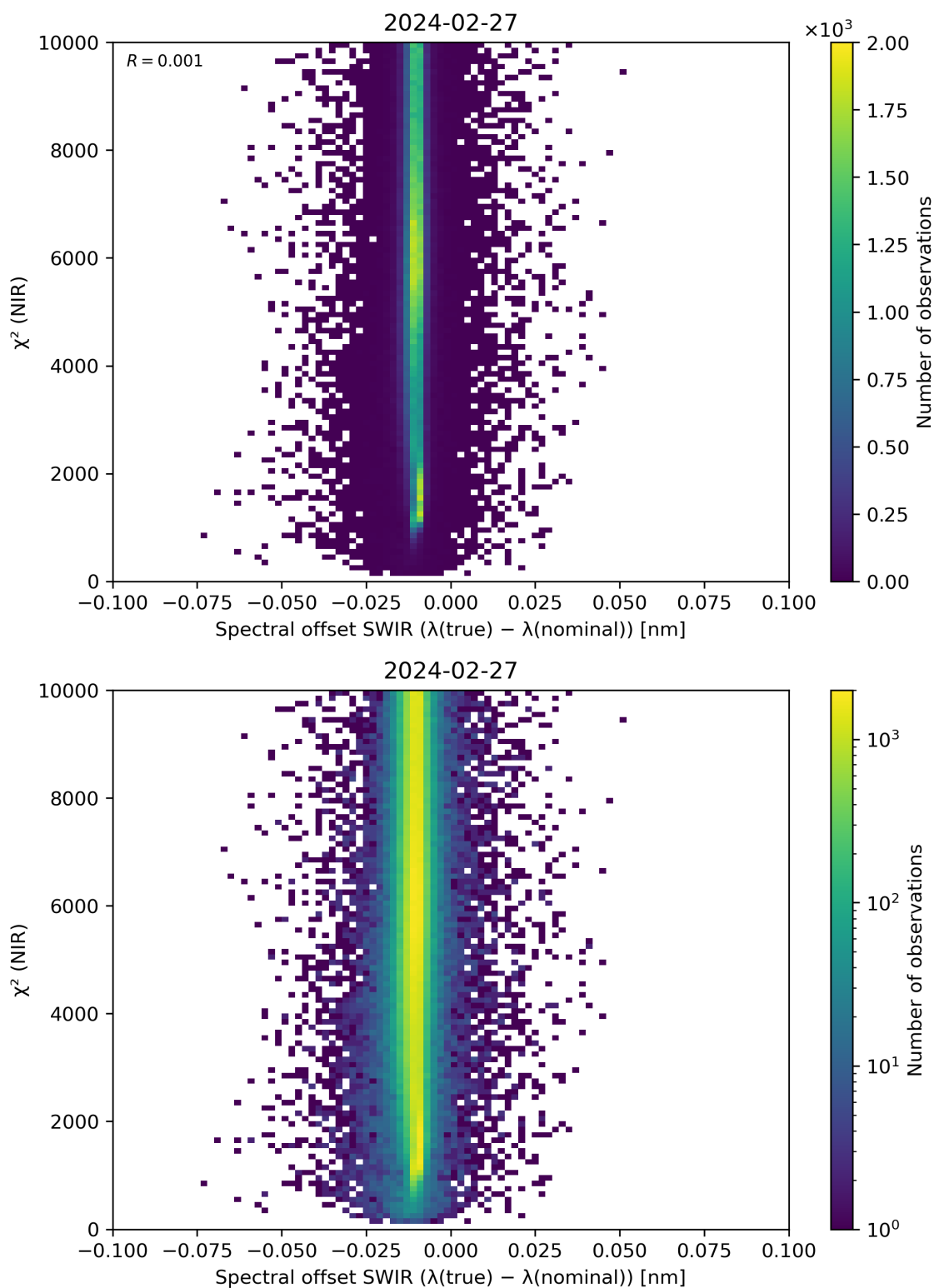
Figure 117: Scatter density plot of “Spectral offset SWIR ( \lambda(\text{true}) - \lambda(\text{nominal}) )” against “ \chi^2 (NIR)” for 2024-02-27 to 2024-02-28.
