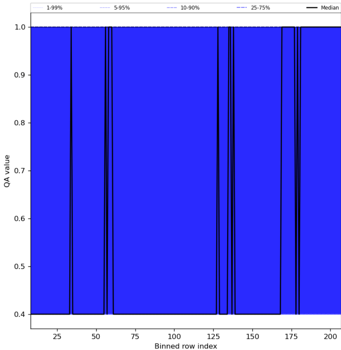
Figure 33: Along track statistics of “QA value” for 2024-02-27 to 2024-02-28
