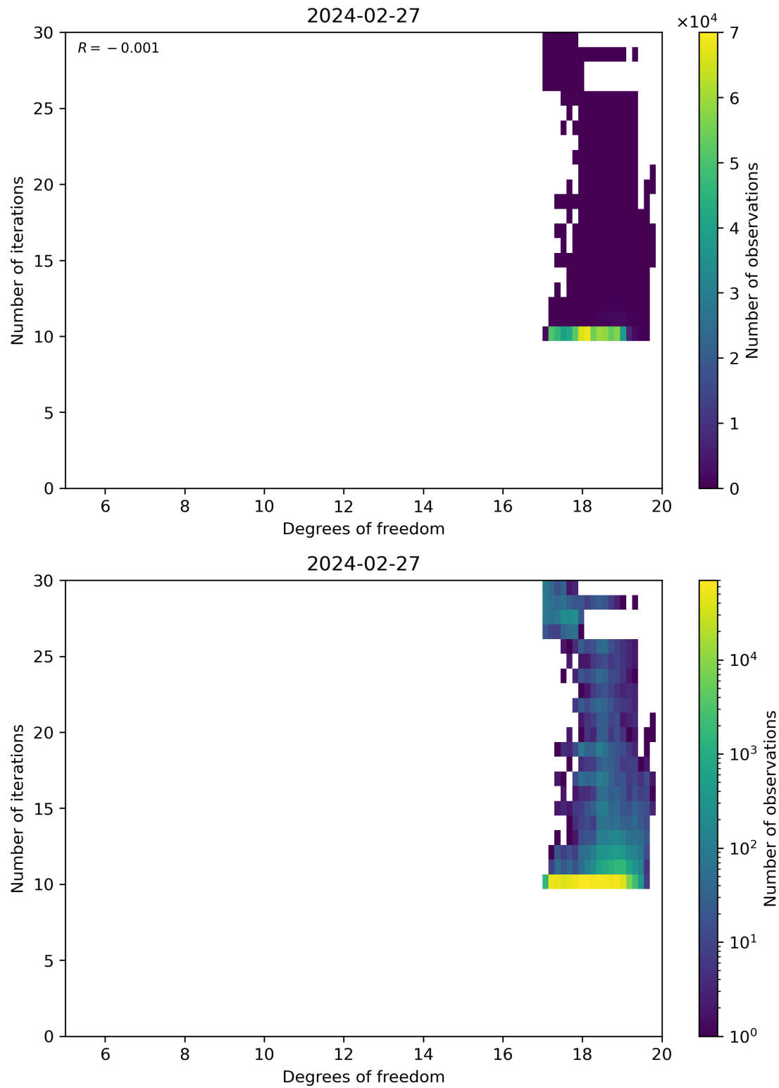
Figure 52: Scatter density plot of “Degrees of freedom” against “Number of iterations” for 2024-02-27 to 2024-02-28.
