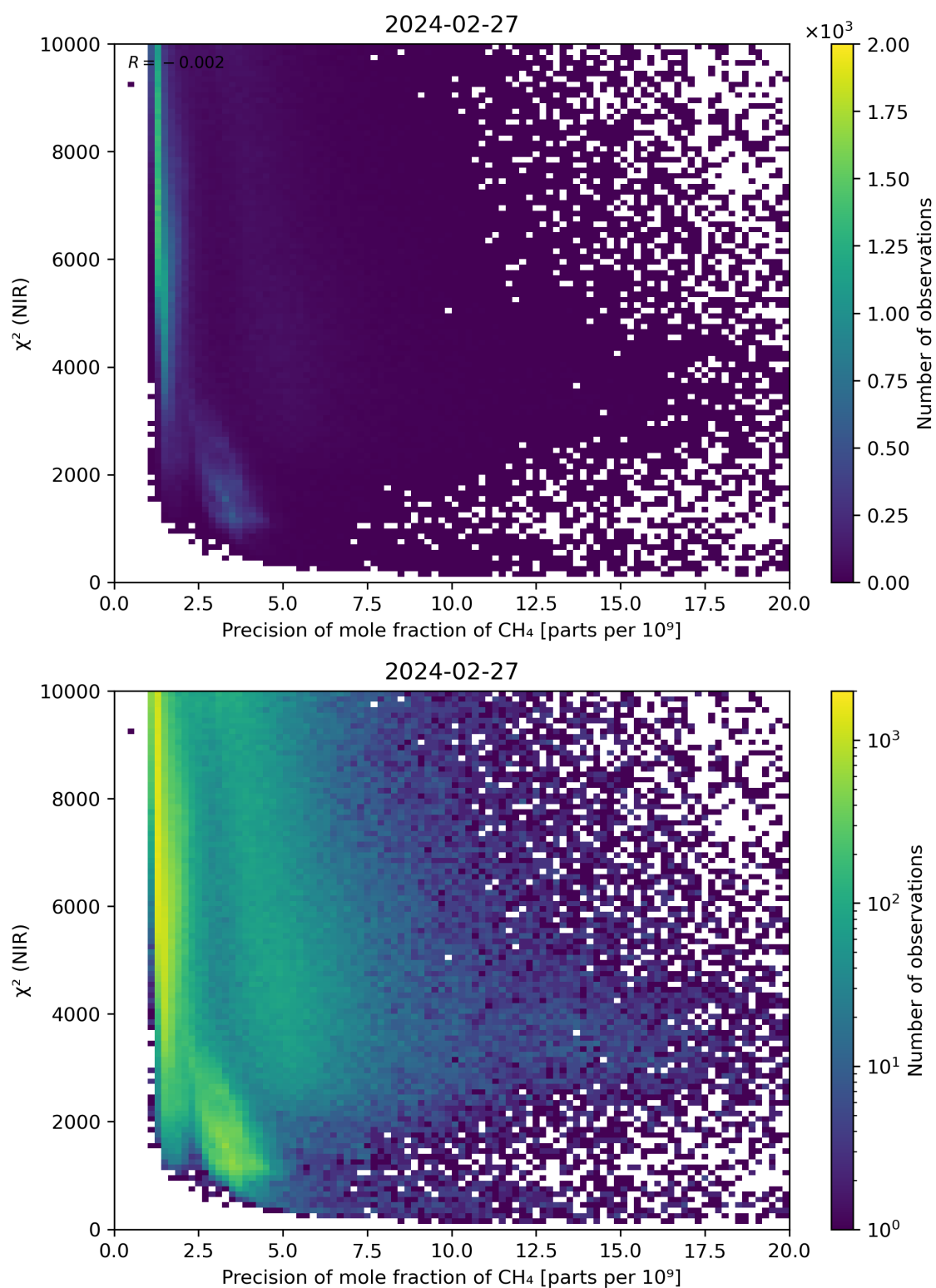
Figure 78: Scatter density plot of “Precision of mole fraction of CH 4 ” against “ \chi^2 (NIR)” for 2024-02-27 to 2024-02-28.
