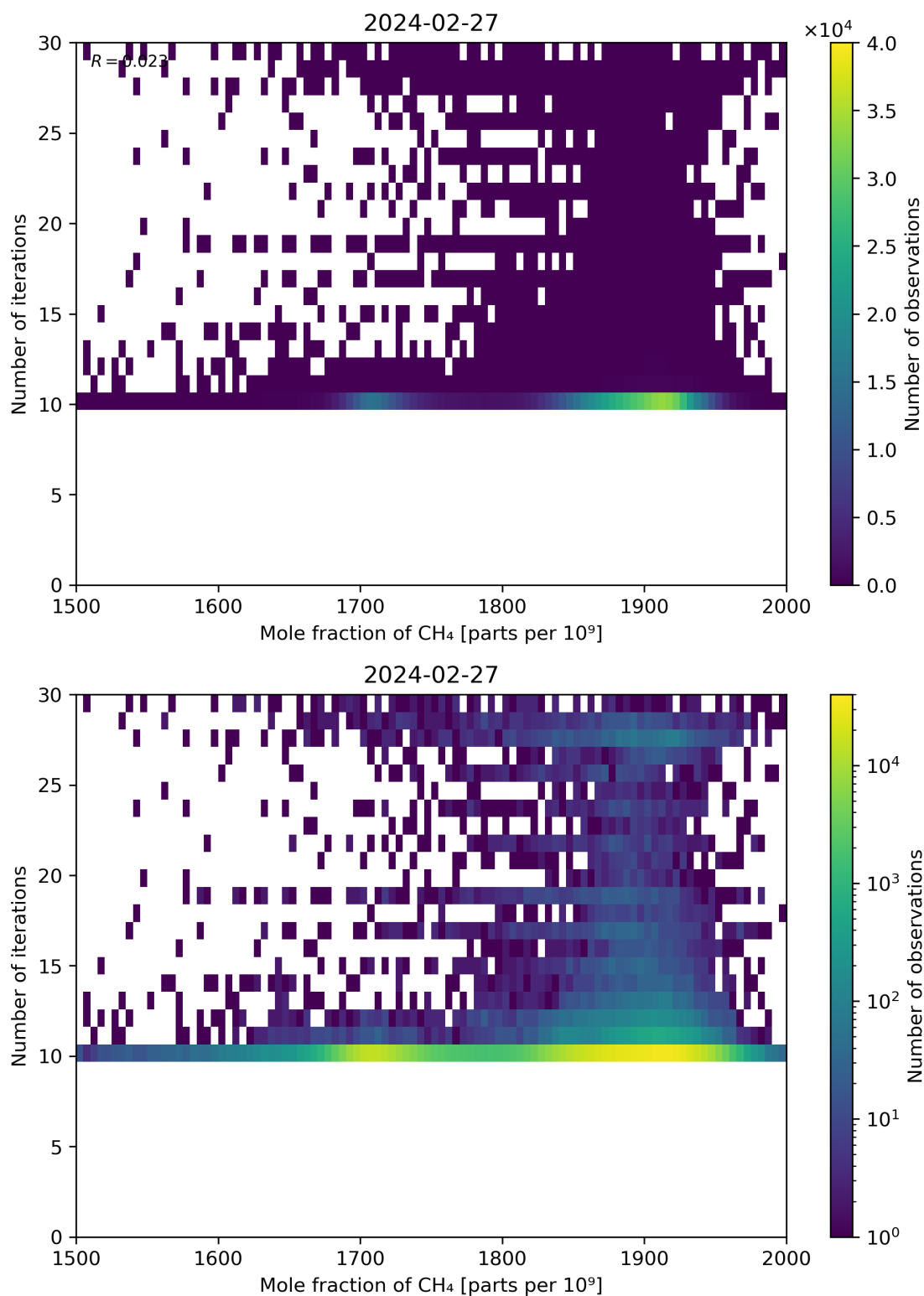
Figure 76: Scatter density plot of “Mole fraction of CH 4 ” against “Number of iterations” for 2024-02-27 to 2024-02-28.
