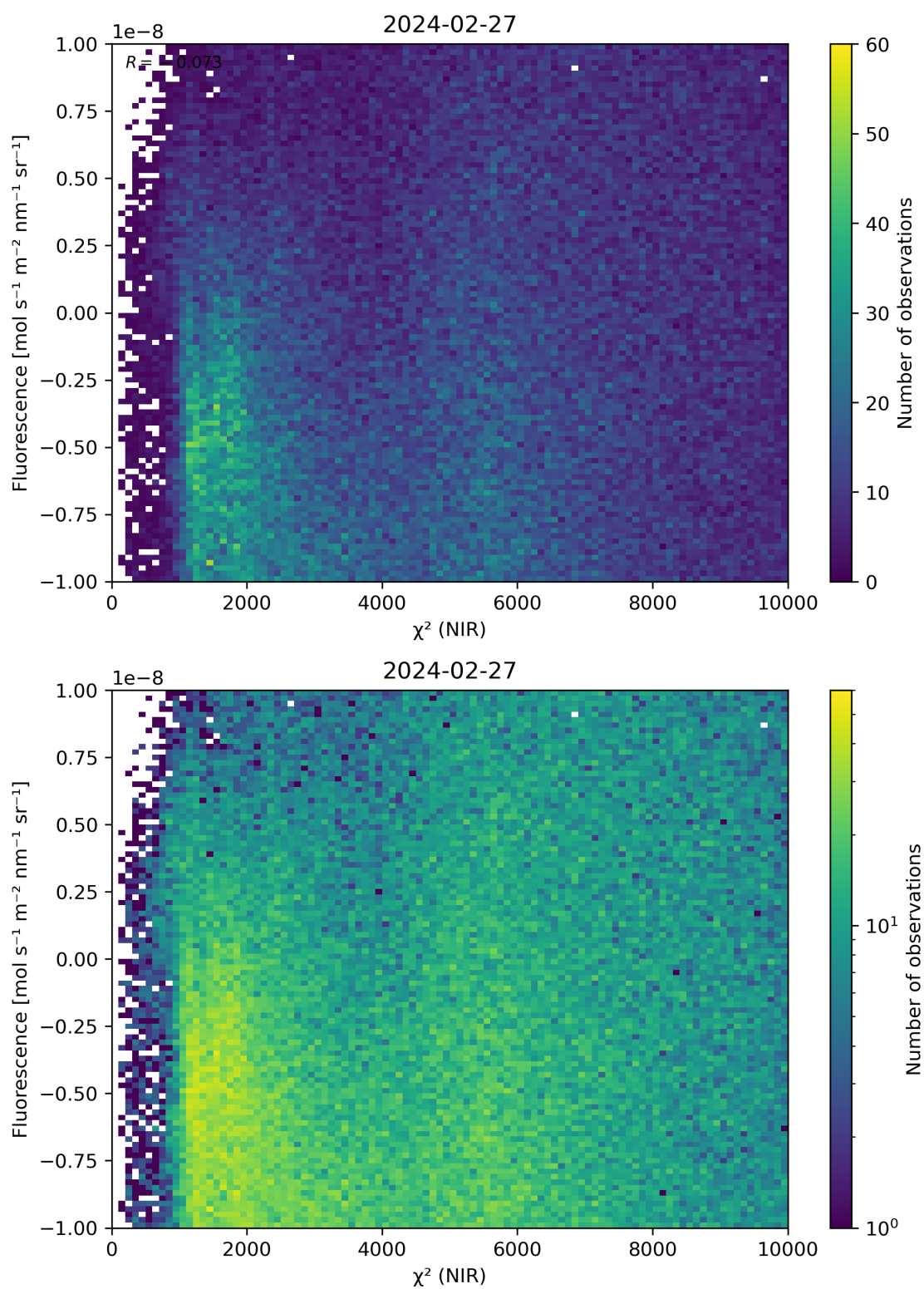
Figure 45: Scatter density plot of “ \chi^2 (NIR)” against “Fluorescence” for 2024-02-27 to 2024-02-28.
