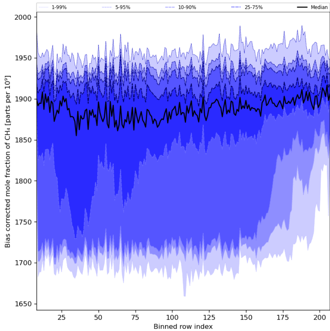
Figure 36: Along track statistics of “Bias corrected mole fraction of CH 4 ” for 2024-02-27 to 2024-02-28
