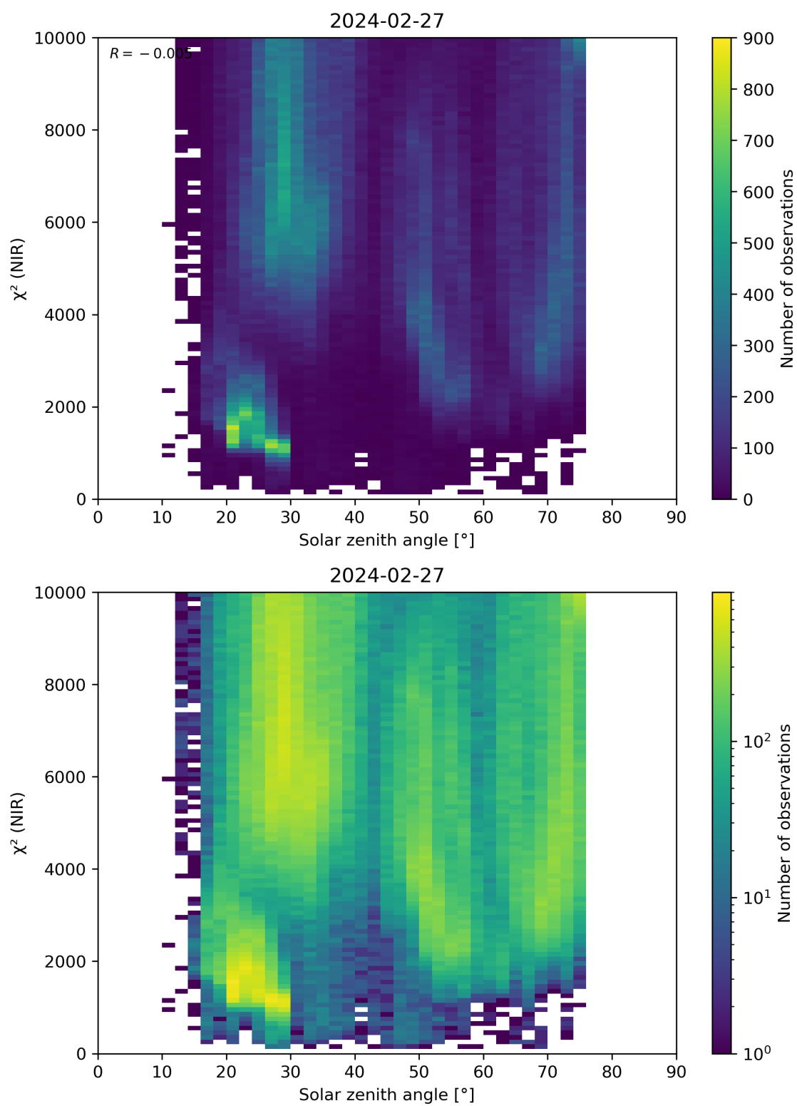
Figure 94: Scatter density plot of “Solar zenith angle” against “ \chi^2 (NIR)” for 2024-02-27 to 2024-02-28.
