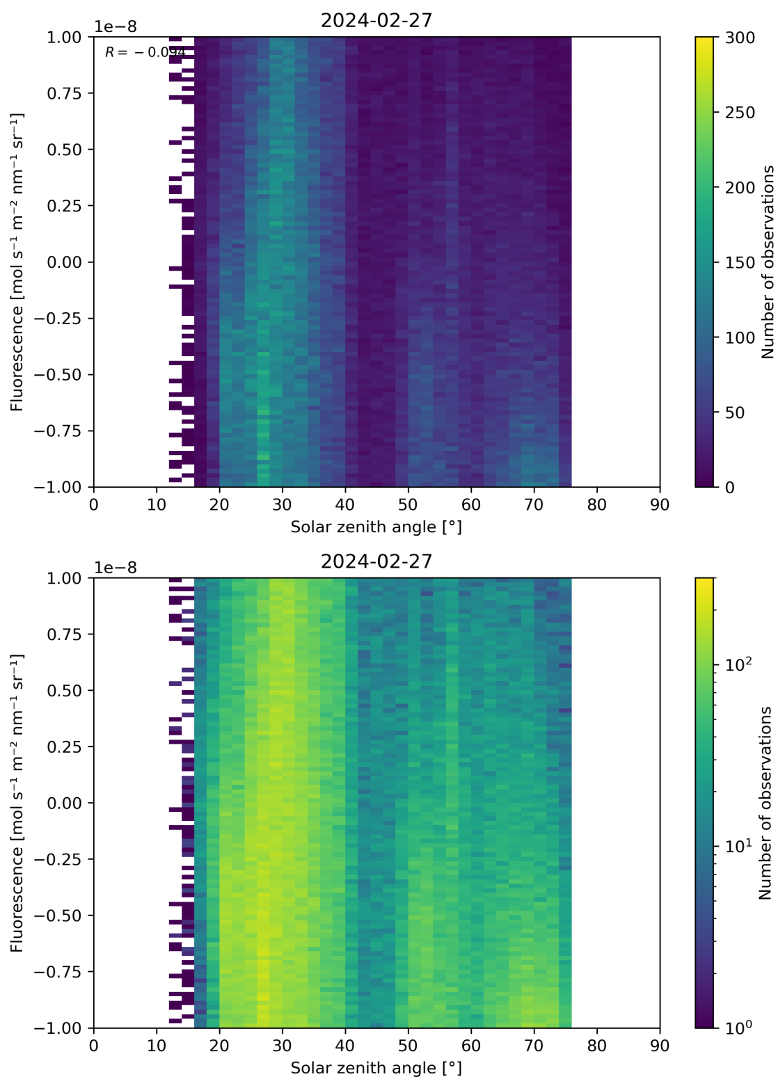
Figure 97: Scatter density plot of “Solar zenith angle” against “Fluorescence” for 2024-02-27 to 2024-02-28.
