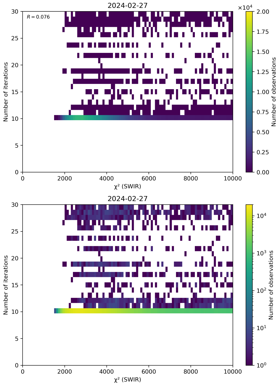
Figure 50: Scatter density plot of “ \chi^2 (SWIR)” against “Number of iterations” for 2024-02-27 to 2024-02-28.
