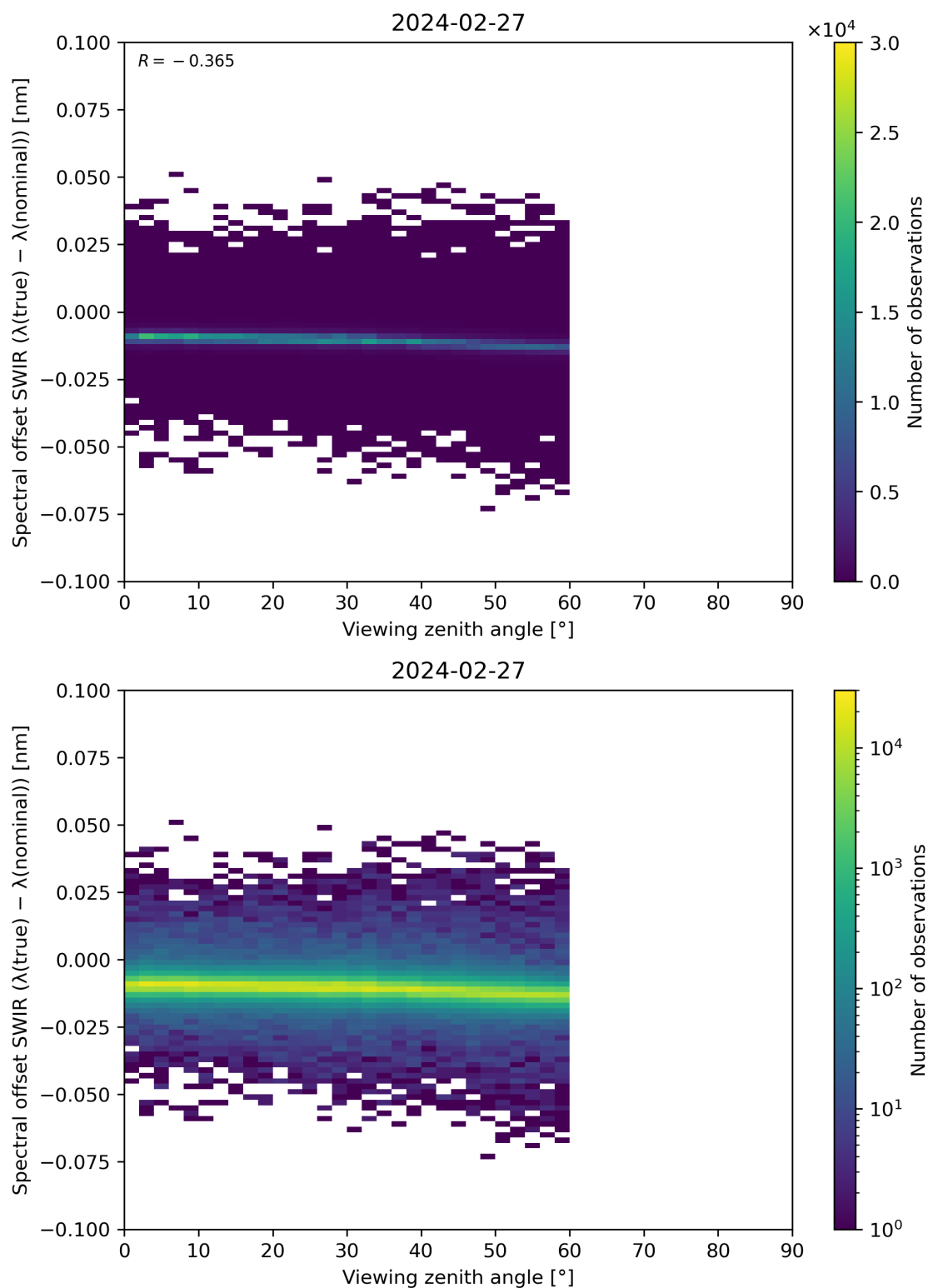
Figure 116: Scatter density plot of “Viewing zenith angle” against “Spectral offset SWIR ( \lambda(\text{true}) - \lambda(\text{nominal}) )” for 2024-02-27 to 2024-02-28.
