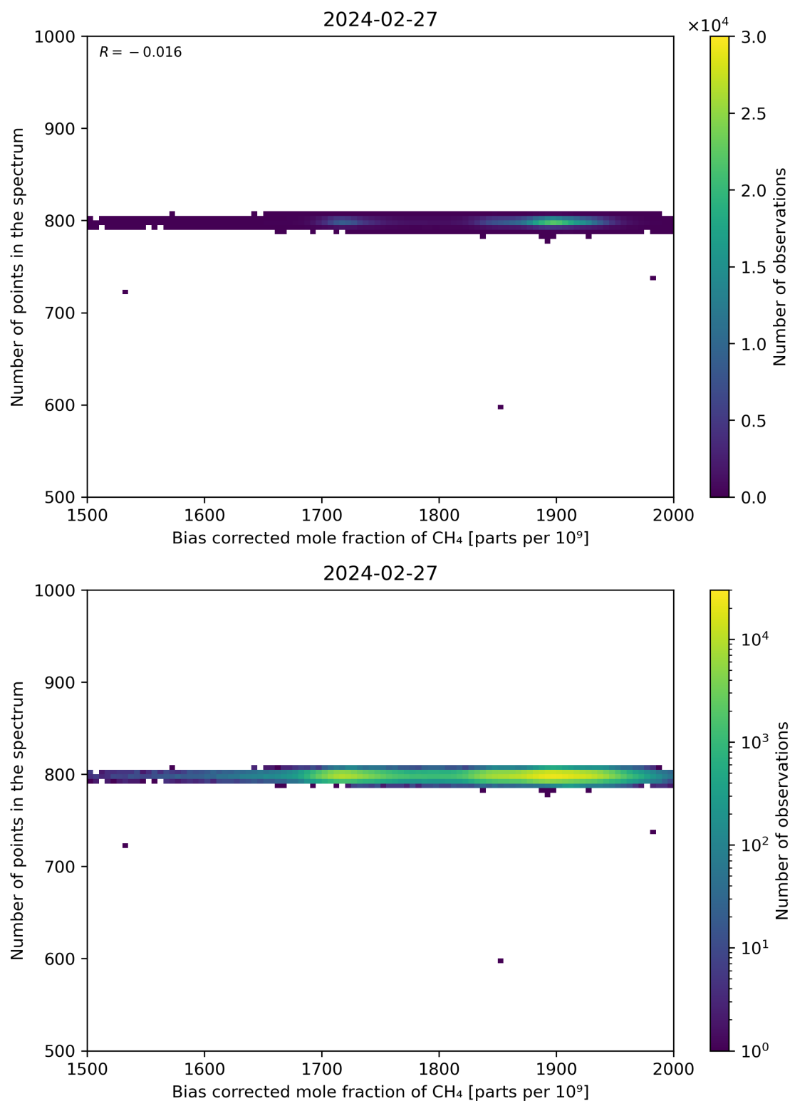
Figure 68: Scatter density plot of “Bias corrected mole fraction of CH 4 ” against “Number of points in the spectrum” for 2024-02-27 to 2024-02-28.
