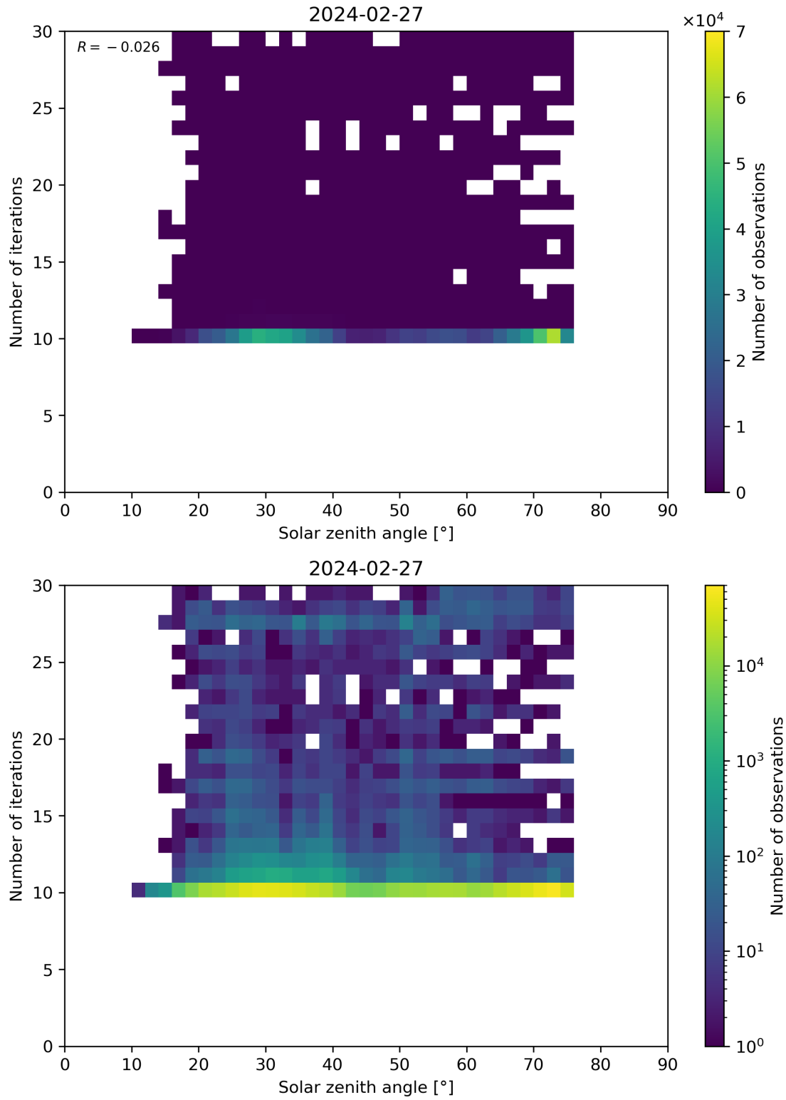
Figure 102: Scatter density plot of “Solar zenith angle” against “Number of iterations” for 2024-02-27 to 2024-02-28.
