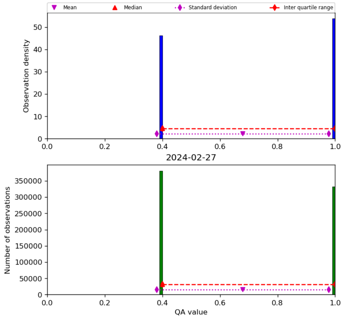
Figure 22: Histogram of “QA value” for 2024-02-27 to 2024-02-28
