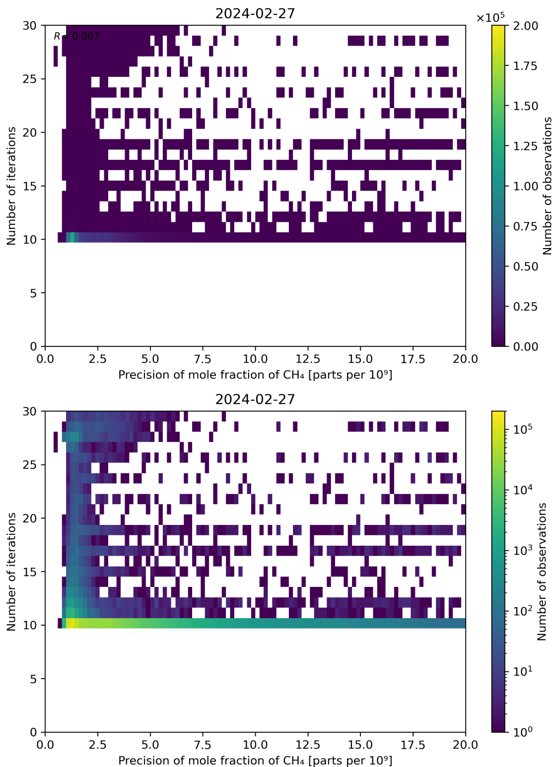
Figure 83: Scatter density plot of “Precision of mole fraction of CH 4 ” against “Number of iterations” for 2024-02-27 to 2024-02-28.
