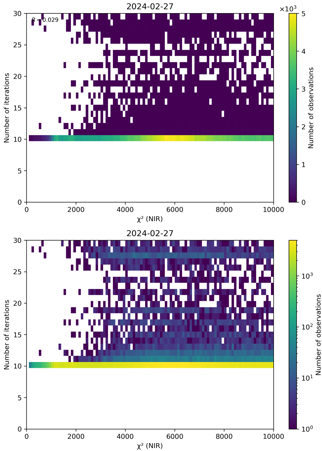
Figure 46: Scatter density plot of “ \chi^2 (NIR)” against “Number of iterations” for 2024-02-27 to 2024-02-28.
