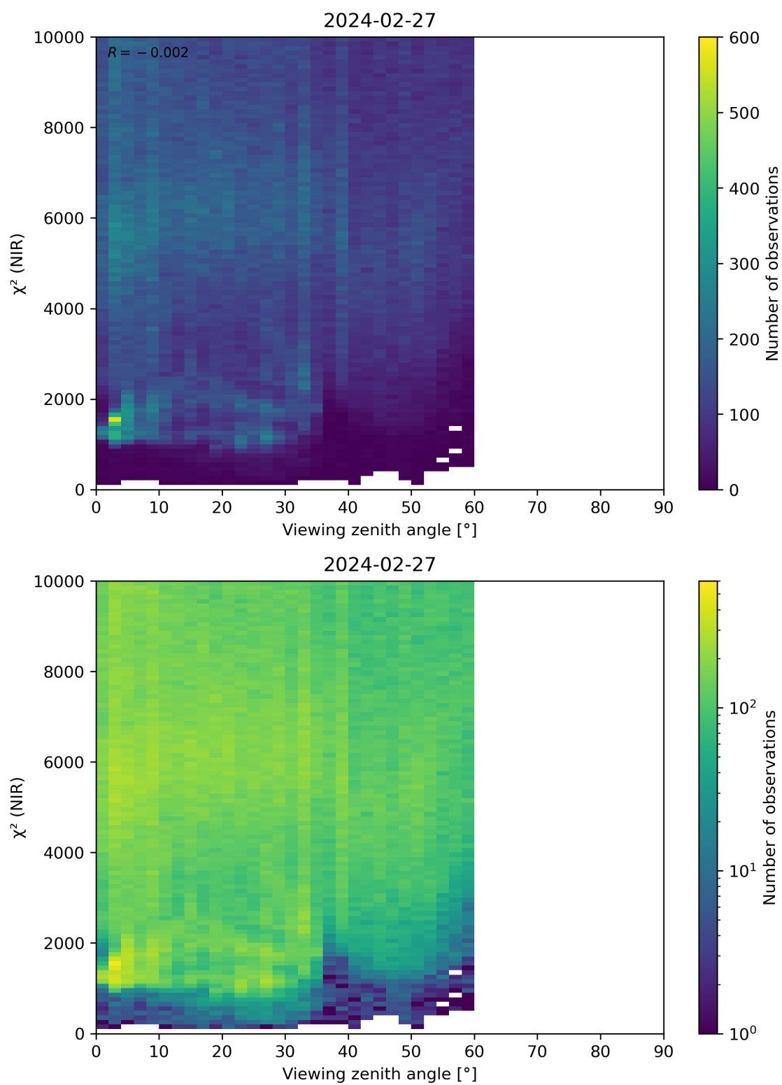
Figure 105: Scatter density plot of “Viewing zenith angle” against “ \chi^2 (NIR)” for 2024-02-27 to 2024-02-28.
