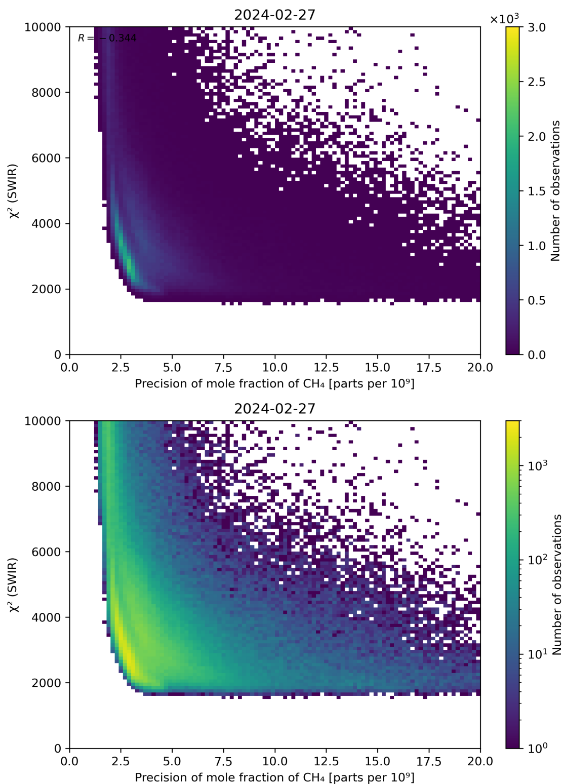
Figure 79: Scatter density plot of “Precision of mole fraction of \text{CH}_4 ” against “ \chi^2 (SWIR)” for 2024-02-27 to 2024-02-28.
