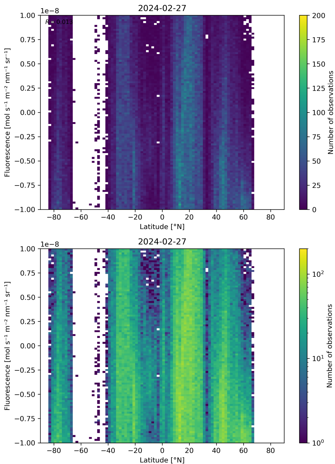
Figure 56: Scatter density plot of “Latitude” against “Fluorescence” for 2024-02-27 to 2024-02-28.
