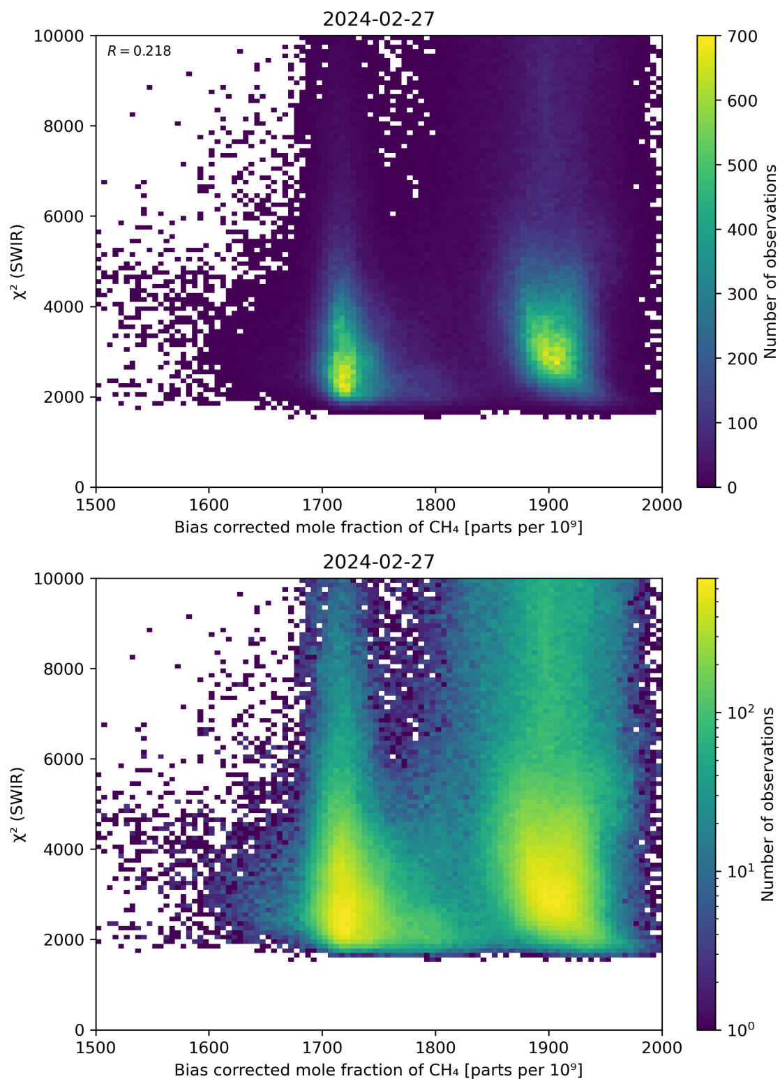
Figure 64: Scatter density plot of “Bias corrected mole fraction of \text{CH}_4 ” against “ \chi^2 (SWIR)” for 2024-02-27 to 2024-02-28.
