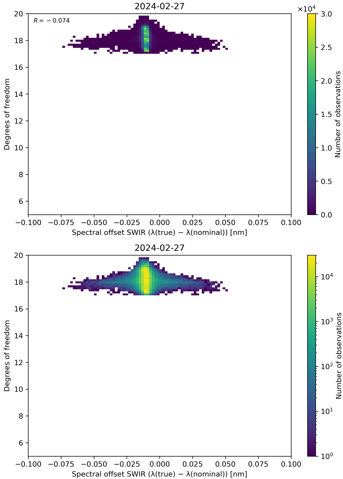
Figure 119: Scatter density plot of “Spectral offset SWIR ( \lambda(\text{true}) - \lambda(\text{nominal}) )” against “Degrees of freedom” for 2024-02-27 to 2024-02-28.
