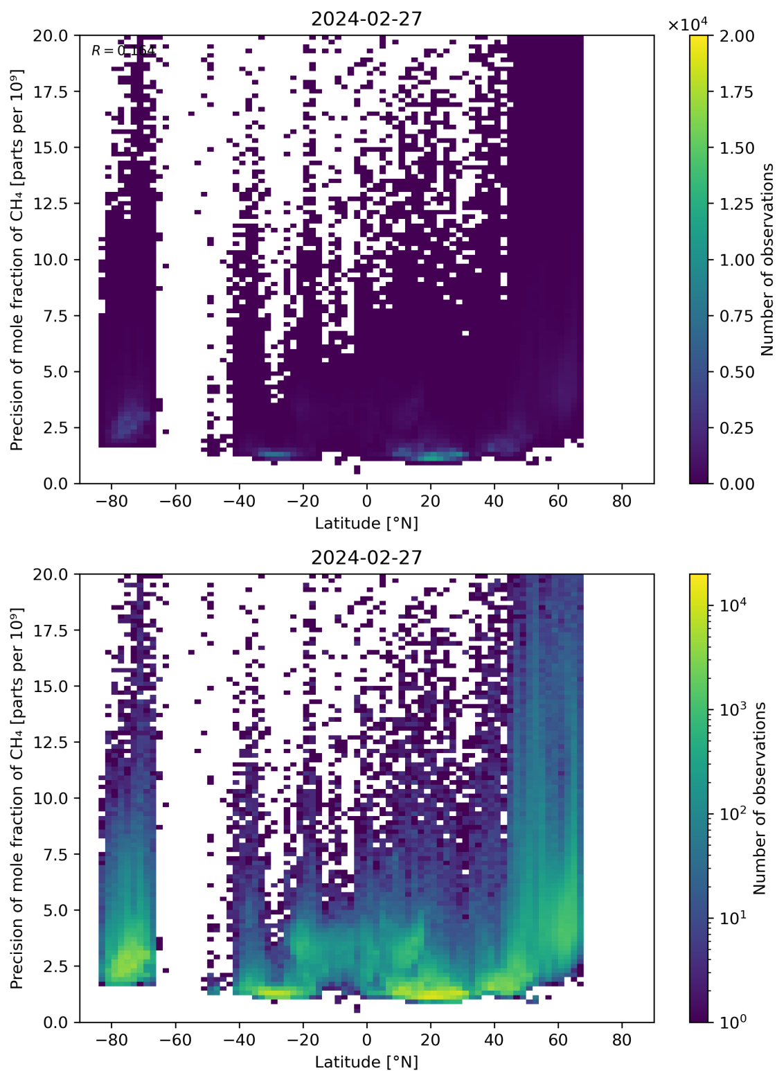
Figure 59: Scatter density plot of “Latitude” against “Precision of mole fraction of CH 4 ” for 2024-02-27 to 2024-02-28.
