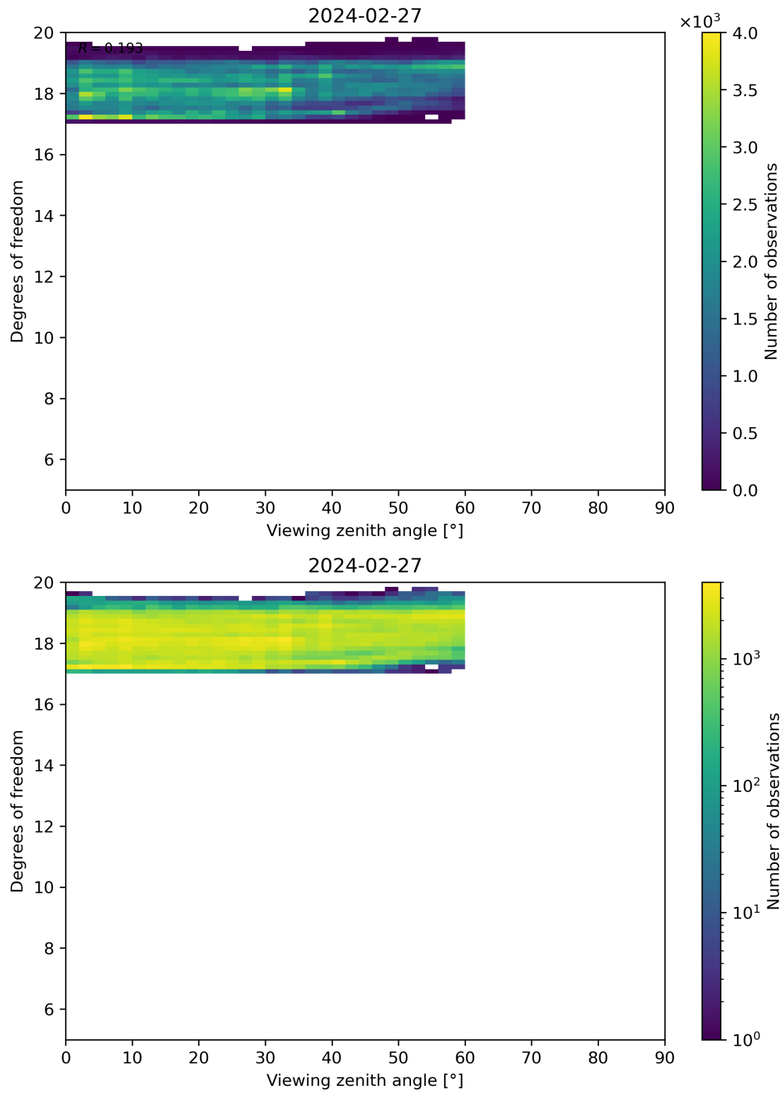
Figure 107: Scatter density plot of “Viewing zenith angle” against “Degrees of freedom” for 2024-02-27 to 2024-02-28.
