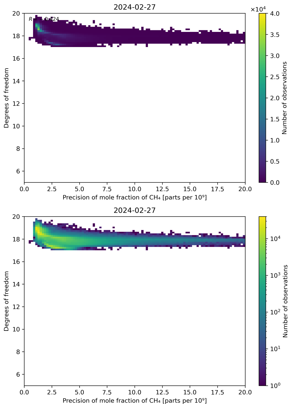
Figure 80: Scatter density plot of “Precision of mole fraction of CH 4 ” against “Degrees of freedom” for 2024-02-27 to 2024-02-28.
