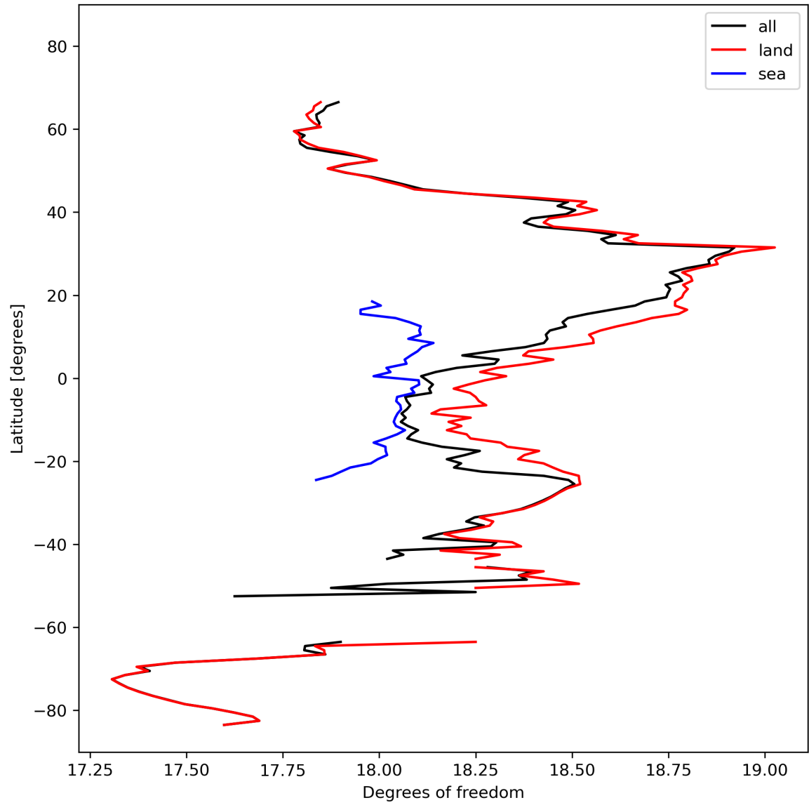
Figure 19: Zonal average of “Degrees of freedom” for 2024-02-27 to 2024-02-28.
