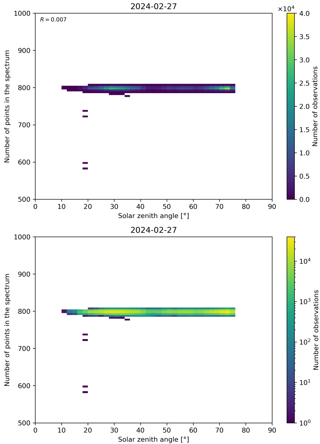
Figure 103: Scatter density plot of “Solar zenith angle” against “Number of points in the spectrum” for 2024-02-27 to 2024-02-28.
