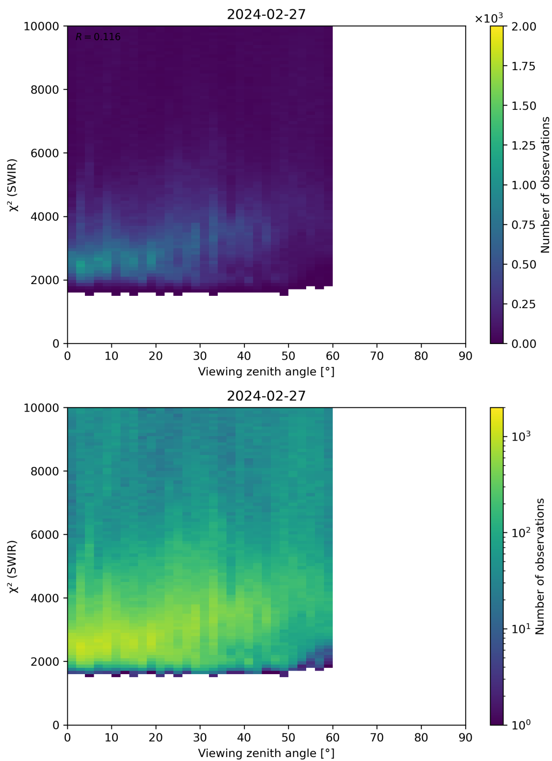
Figure 106: Scatter density plot of “Viewing zenith angle” against “ \chi^2 (SWIR)” for 2024-02-27 to 2024-02-28.
