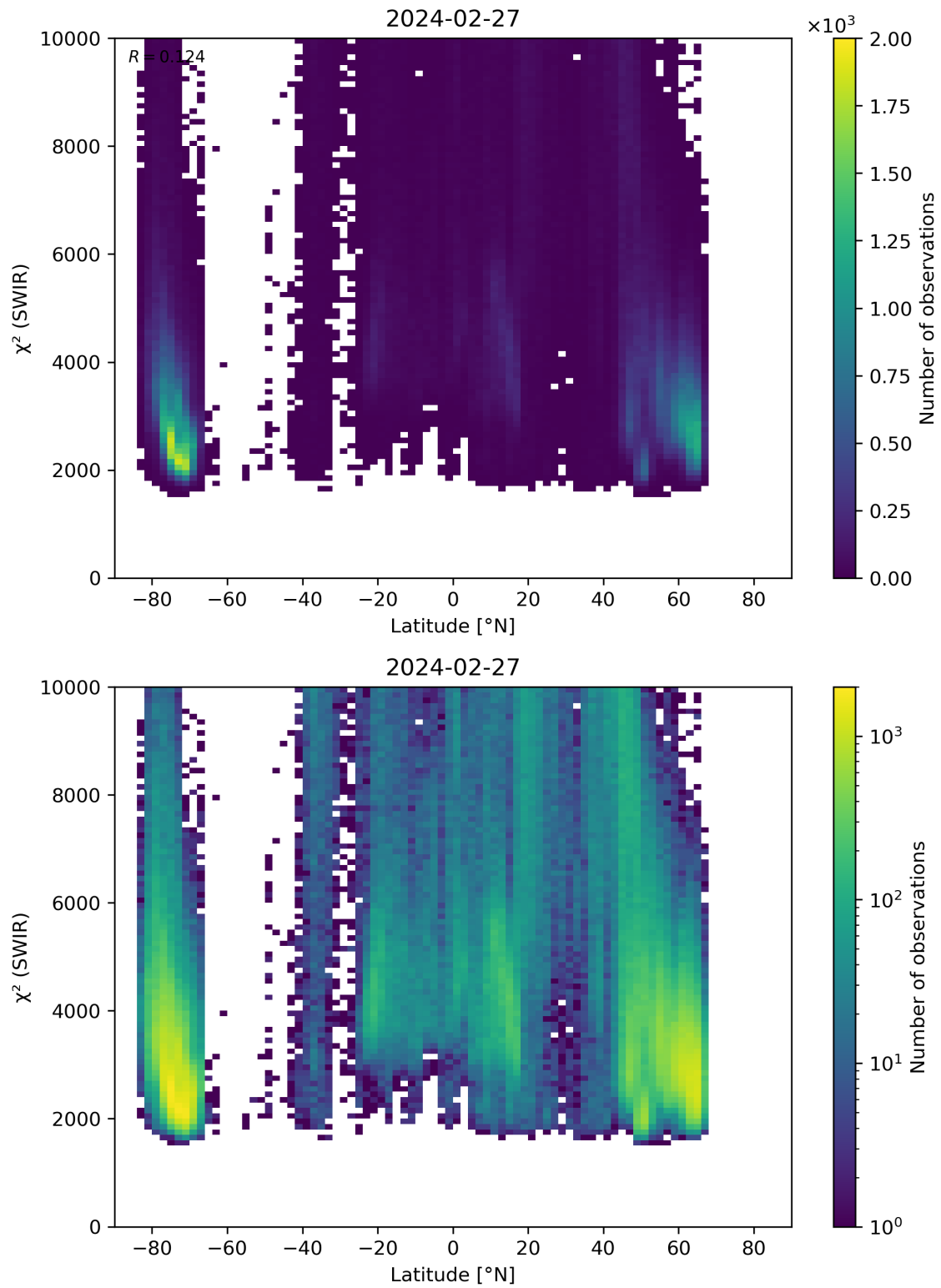
Figure 54: Scatter density plot of “Latitude” against “ \chi^2 (SWIR)” for 2024-02-27 to 2024-02-28.
