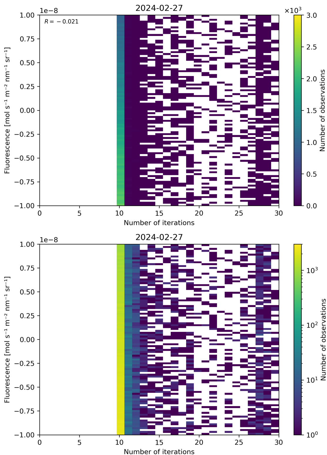
Figure 87: Scatter density plot of “Number of iterations” against “Fluorescence” for 2024-02-27 to 2024-02-28.
