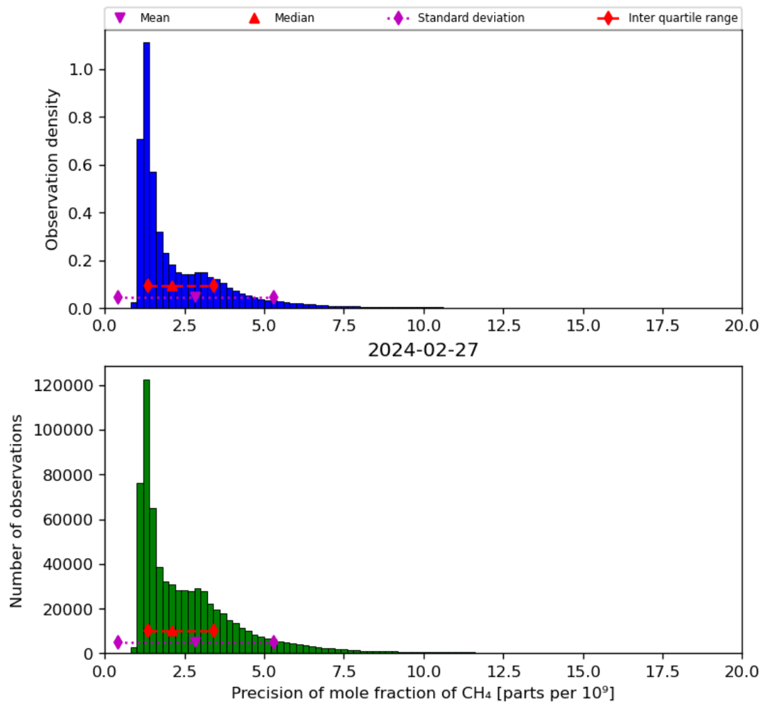
Figure 24: Histogram of “Precision of mole fraction of CH 4 ” for 2024-02-27 to 2024-02-28
