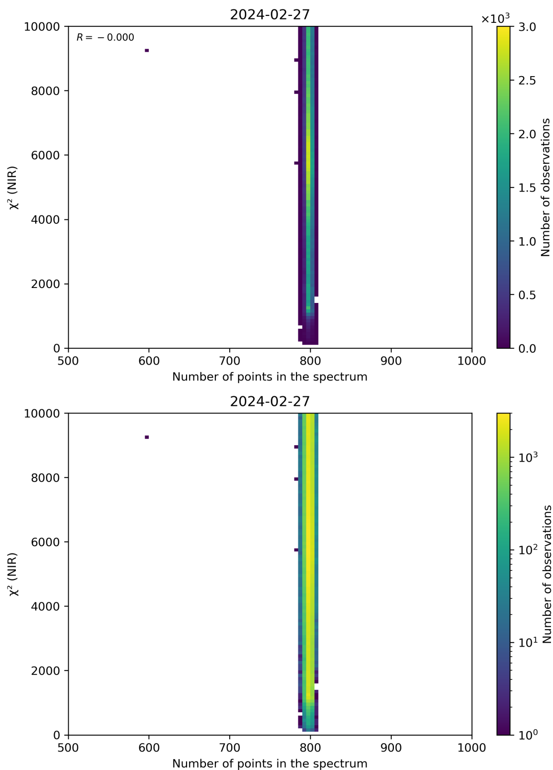
Figure 88: Scatter density plot of “Number of points in the spectrum” against “ \chi^2 (NIR)” for 2024-02-27 to 2024-02-28.
