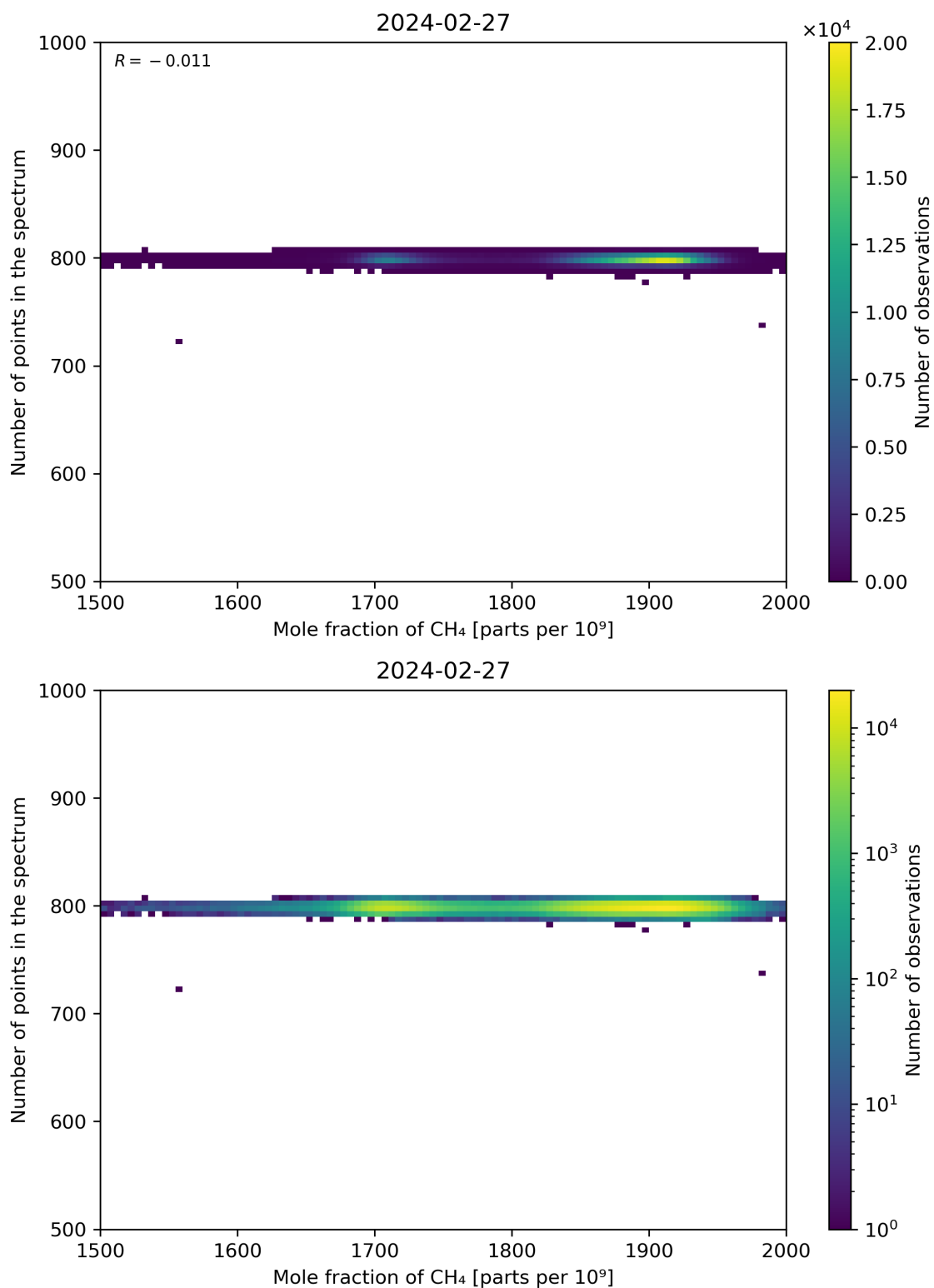
Figure 77: Scatter density plot of “Mole fraction of CH 4 ” against “Number of points in the spectrum” for 2024-02-27 to 2024-02-28.
