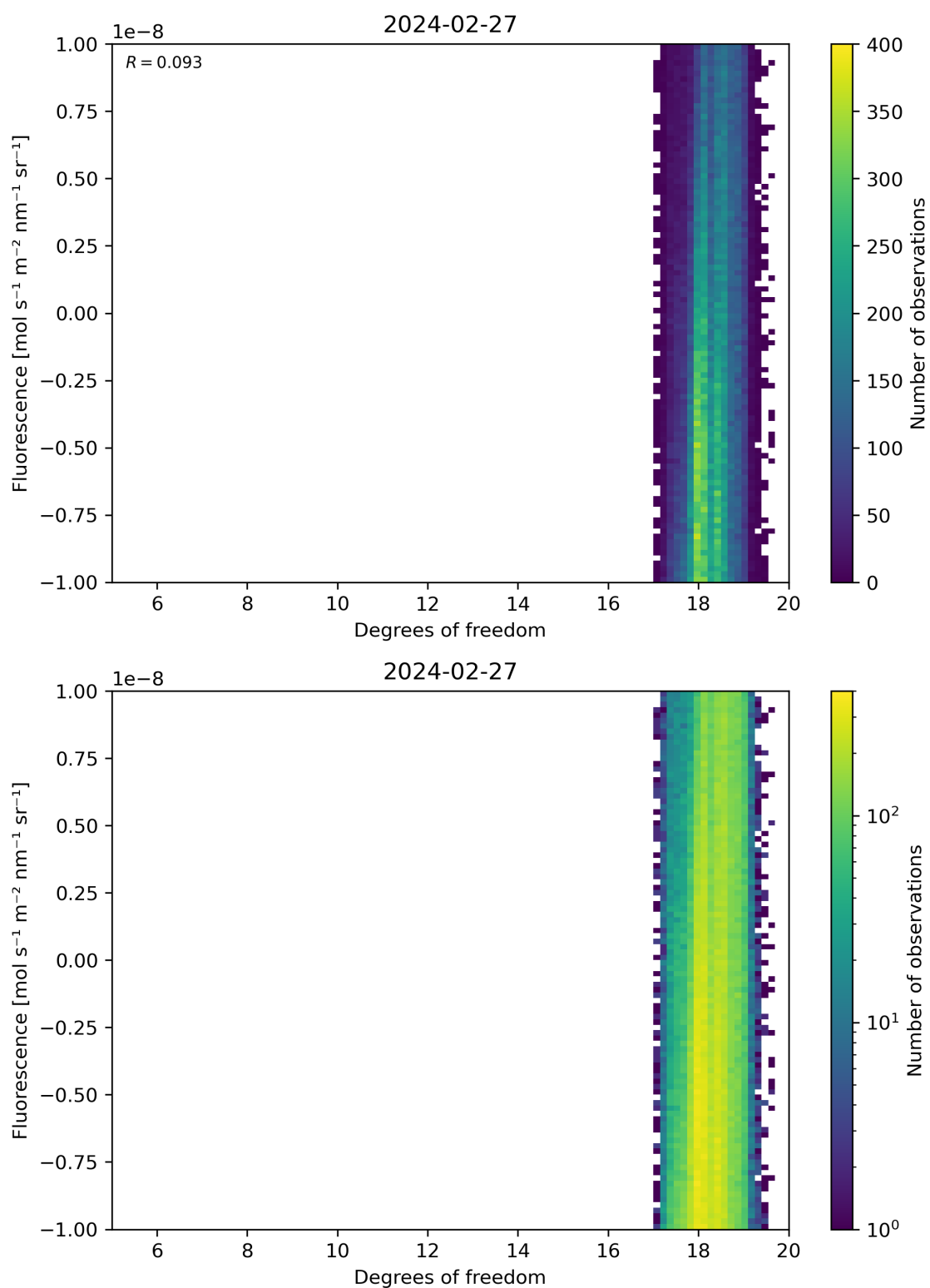
Figure 51: Scatter density plot of “Degrees of freedom” against “Fluorescence” for 2024-02-27 to 2024-02-28.
