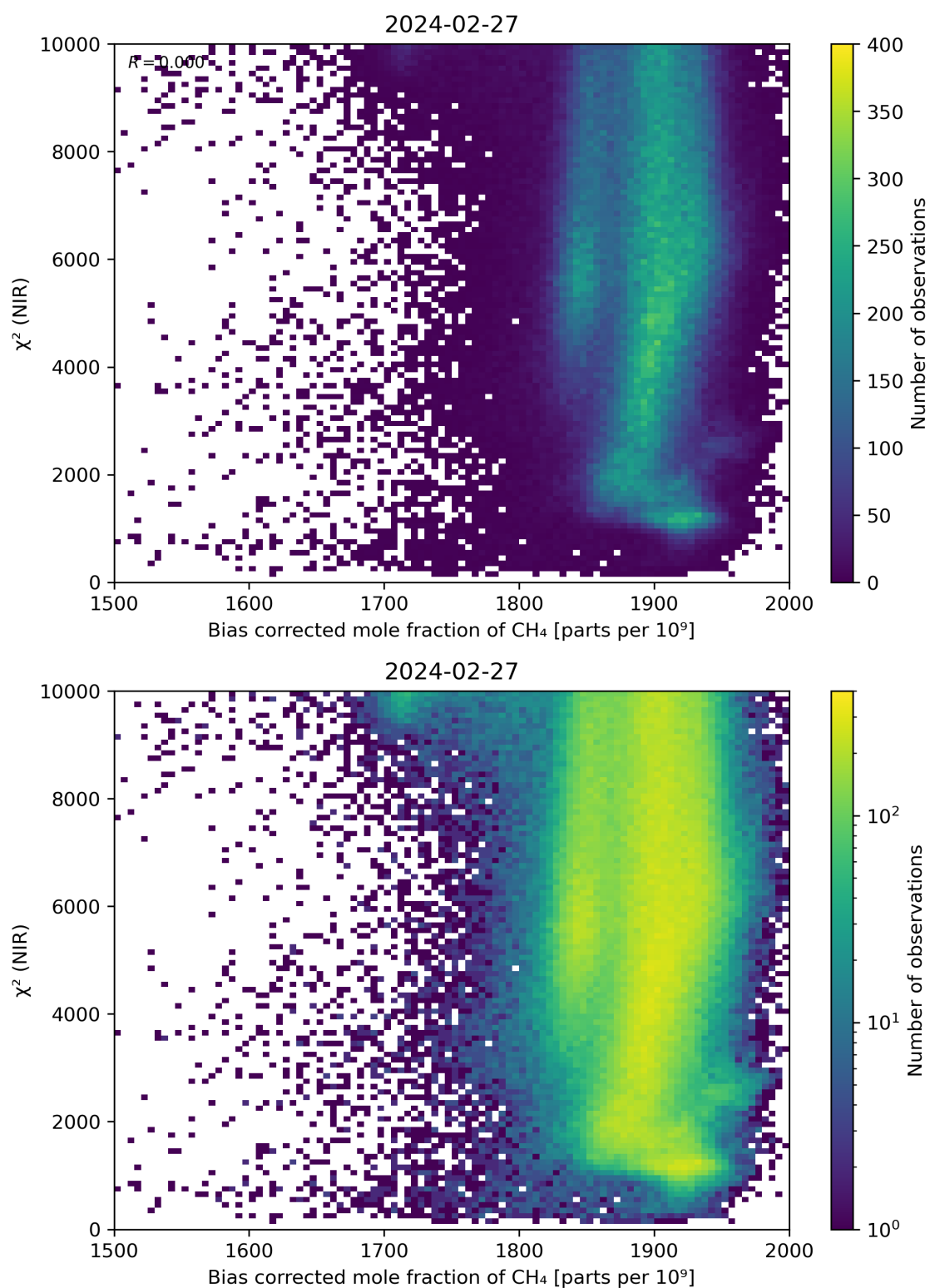
Figure 63: Scatter density plot of “Bias corrected mole fraction of \text{CH}_4 ” against “ \chi^2 (NIR)” for 2024-02-27 to 2024-02-28.
