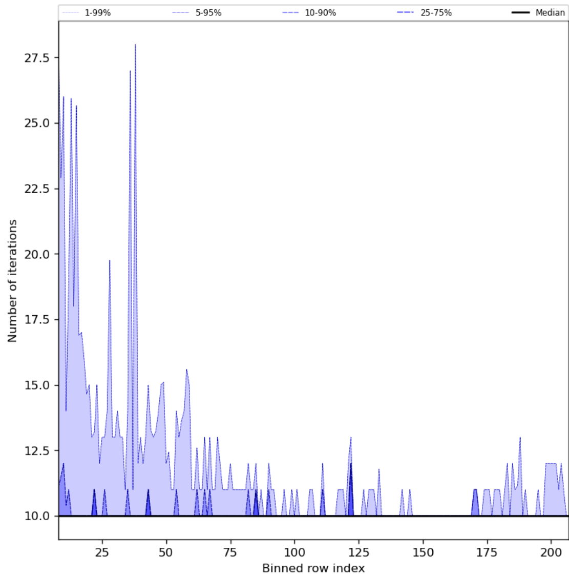
Figure 42: Along track statistics of “Number of iterations” for 2024-02-27 to 2024-02-28
