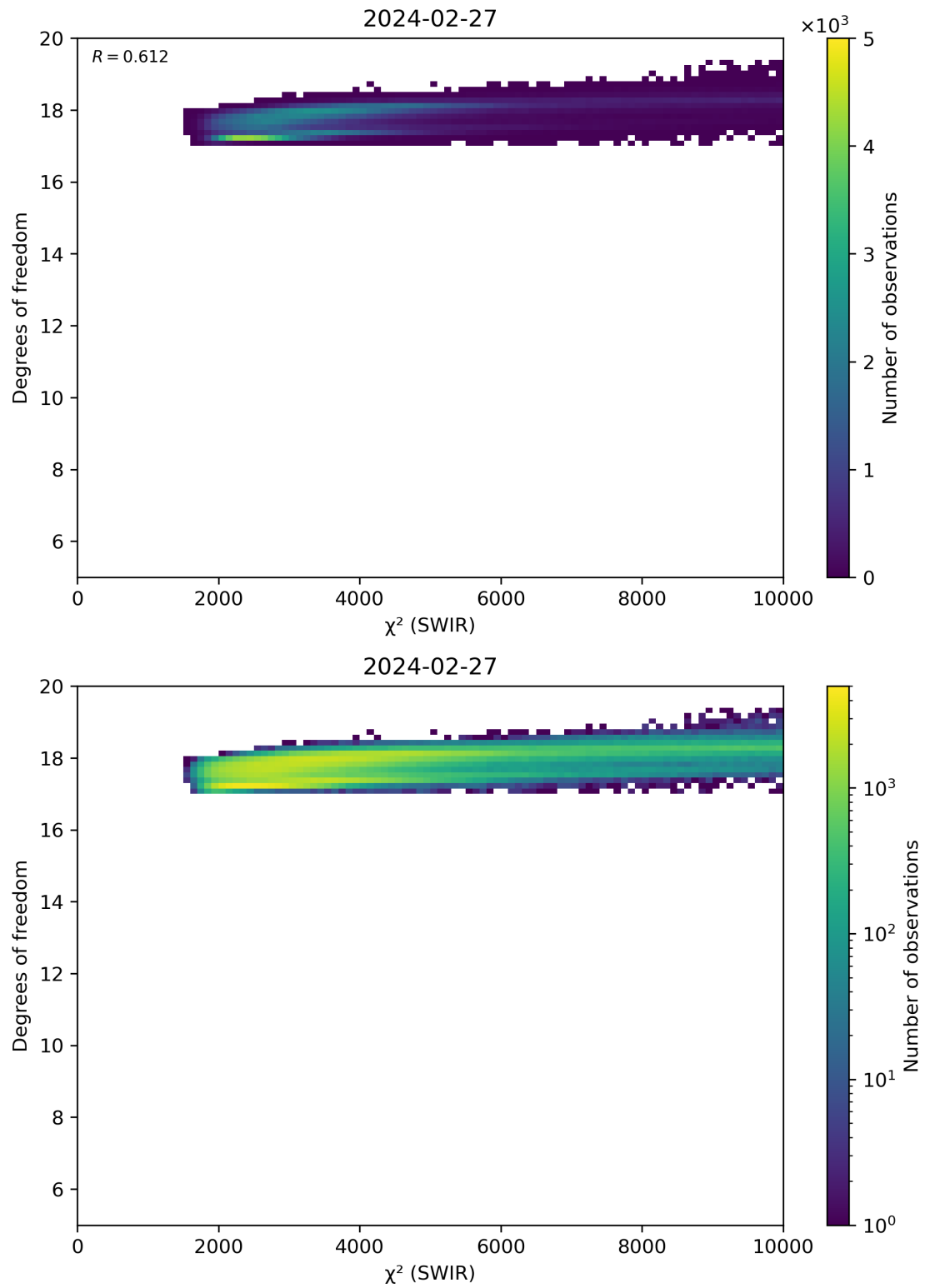
Figure 48: Scatter density plot of “ \chi^2 (SWIR)” against “Degrees of freedom” for 2024-02-27 to 2024-02-28.
