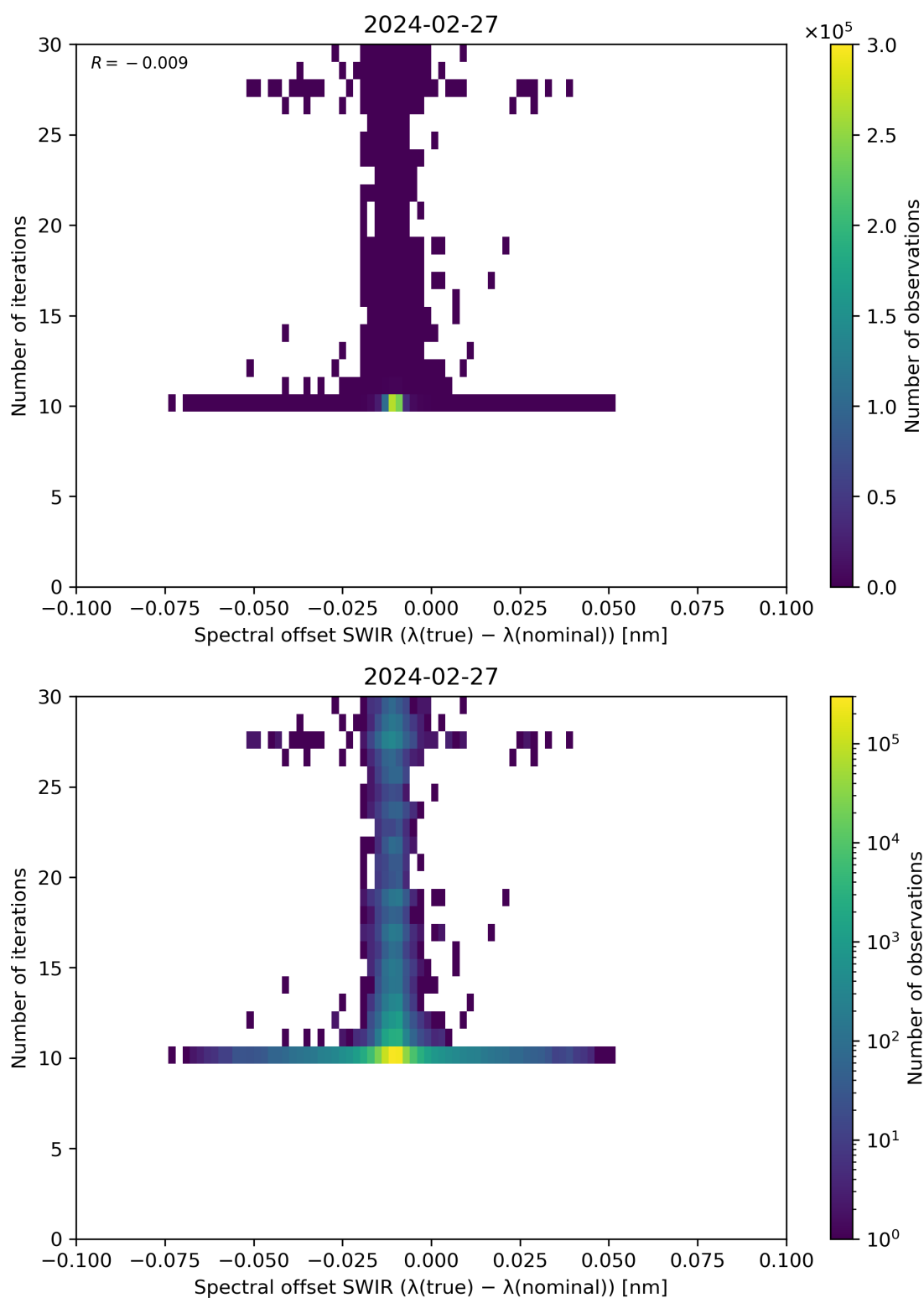
Figure 121: Scatter density plot of “Spectral offset SWIR ( \lambda(\text{true}) - \lambda(\text{nominal}) )” against “Number of iterations” for 2024-02-27 to 2024-02-28.
