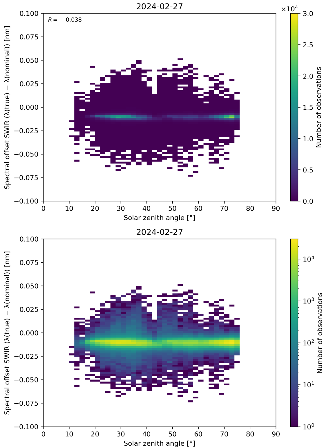
Figure 104: Scatter density plot of “Solar zenith angle” against “Spectral offset SWIR ( \lambda(\text{true}) - \lambda(\text{nominal}) )” for 2024-02-27 to 2024-02-28.
