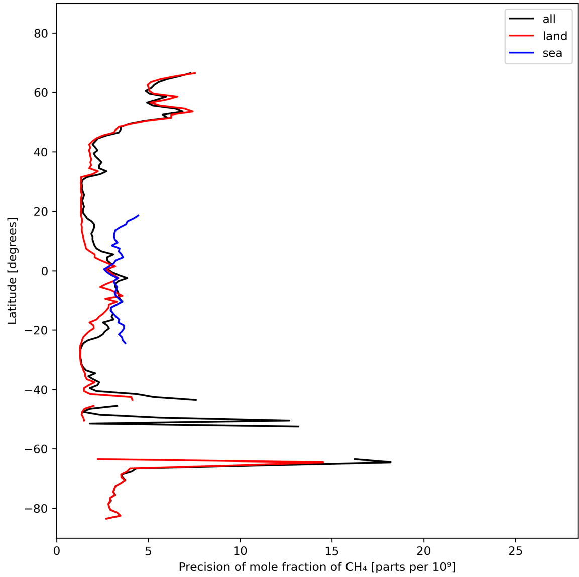
Figure 13: Zonal average of “Precision of mole fraction of CH 4 ” for 2024-02-27 to 2024-02-28.
