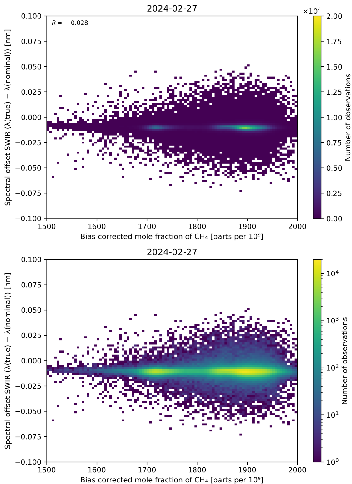
Figure 69: Scatter density plot of “Bias corrected mole fraction of \text{CH}_4 ” against “Spectral offset SWIR ( \lambda(\text{true}) - \lambda(\text{nominal}) )” for 2024-02-27 to 2024-02-28.
