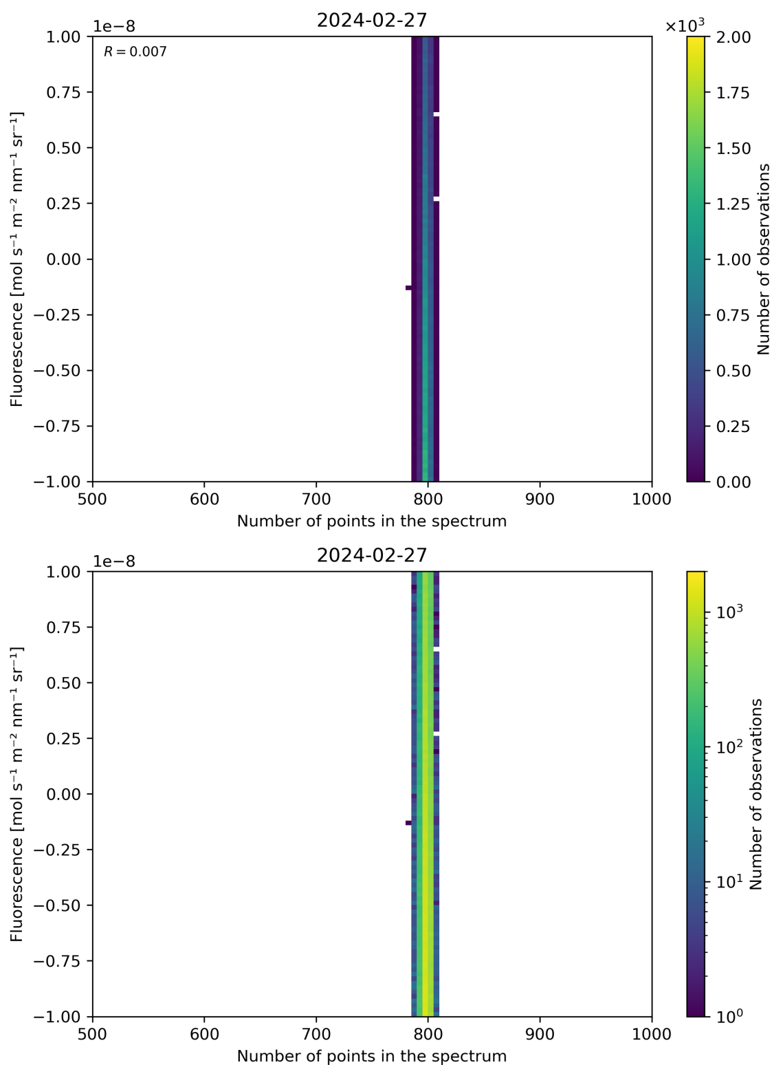
Figure 91: Scatter density plot of “Number of points in the spectrum” against “Fluorescence” for 2024-02-27 to 2024-02-28.
