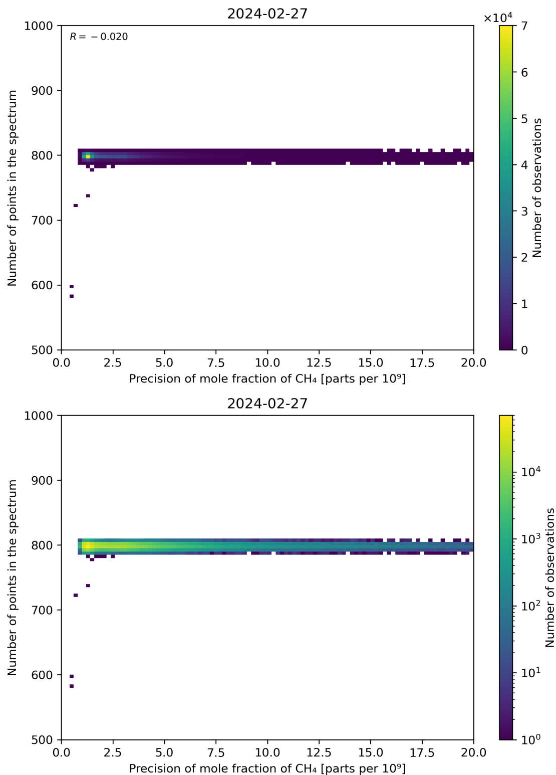
Figure 84: Scatter density plot of “Precision of mole fraction of CH 4 ” against “Number of points in the spectrum” for 2024-02-27 to 2024-02-28.
