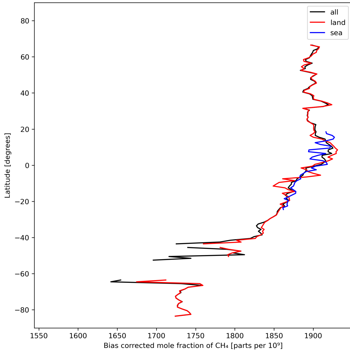
Figure 14: Zonal average of “Bias corrected mole fraction of CH 4 ” for 2024-02-27 to 2024-02-28.
