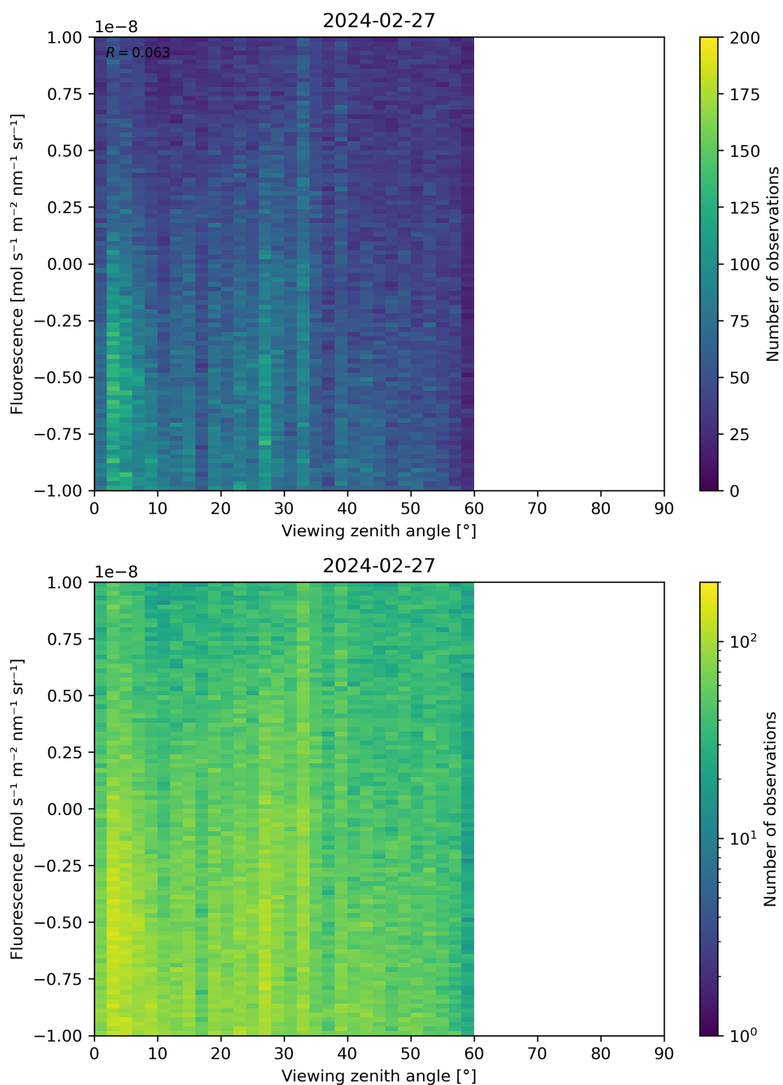
Figure 108: Scatter density plot of “Viewing zenith angle” against “Fluorescence” for 2024-02-27 to 2024-02-28.
