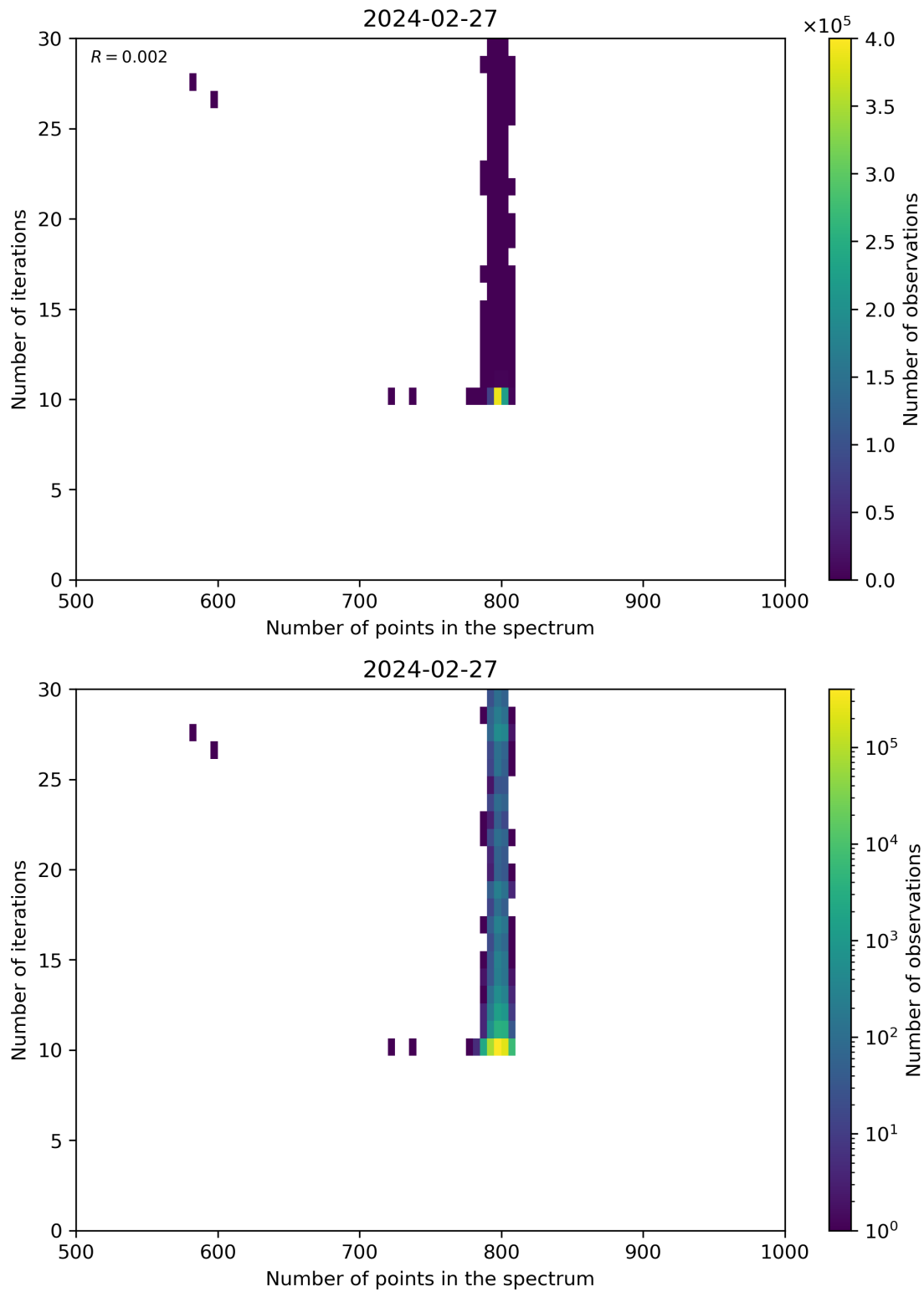
Figure 92: Scatter density plot of “Number of points in the spectrum” against “Number of iterations” for 2024-02-27 to 2024-02-28.
