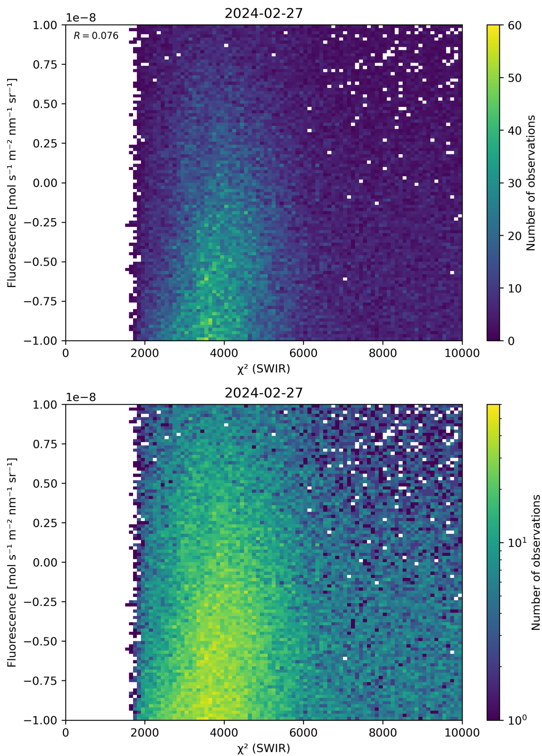
Figure 49: Scatter density plot of “ \chi^2 (SWIR)” against “Fluorescence” for 2024-02-27 to 2024-02-28.
