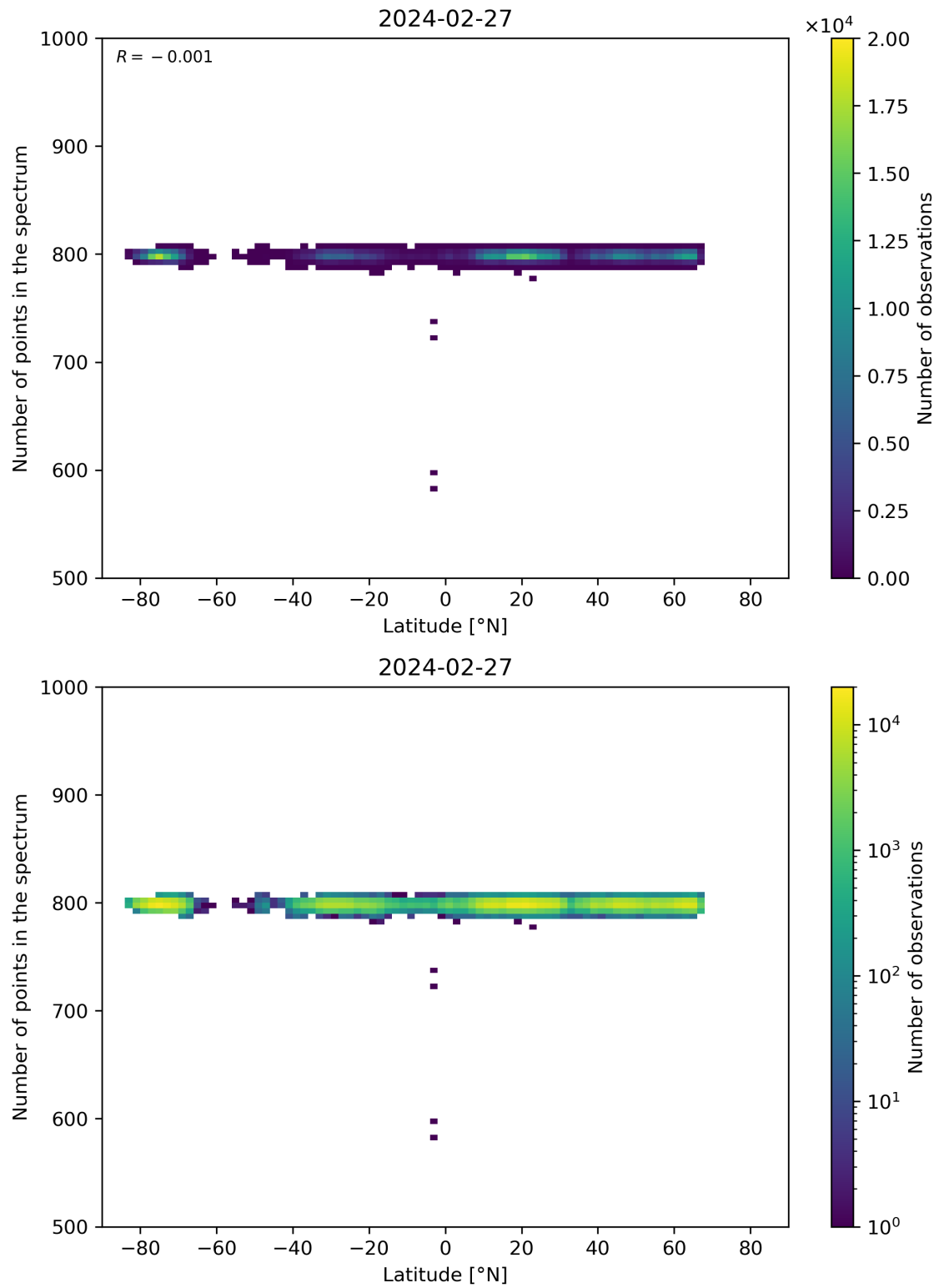
Figure 61: Scatter density plot of “Latitude” against “Number of points in the spectrum” for 2024-02-27 to 2024-02-28.
