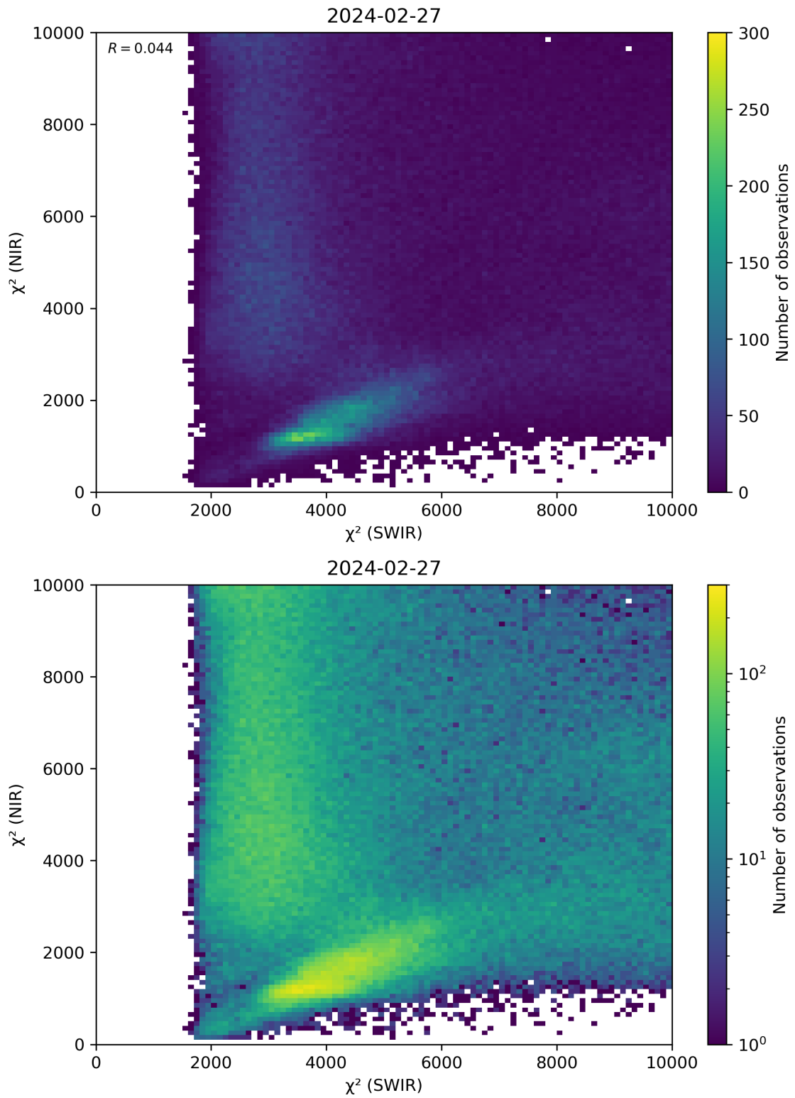
Figure 47: Scatter density plot of “ \chi^2 (SWIR)” against “ \chi^2 (NIR)” for 2024-02-27 to 2024-02-28.
