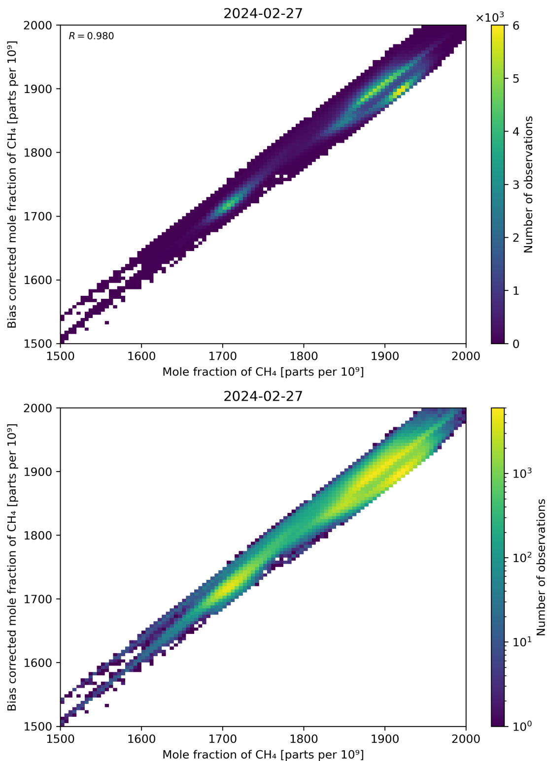
Figure 74: Scatter density plot of “Mole fraction of CH 4 ” against “Bias corrected mole fraction of CH 4 ” for 2024-02-27 to 2024-02-28.
