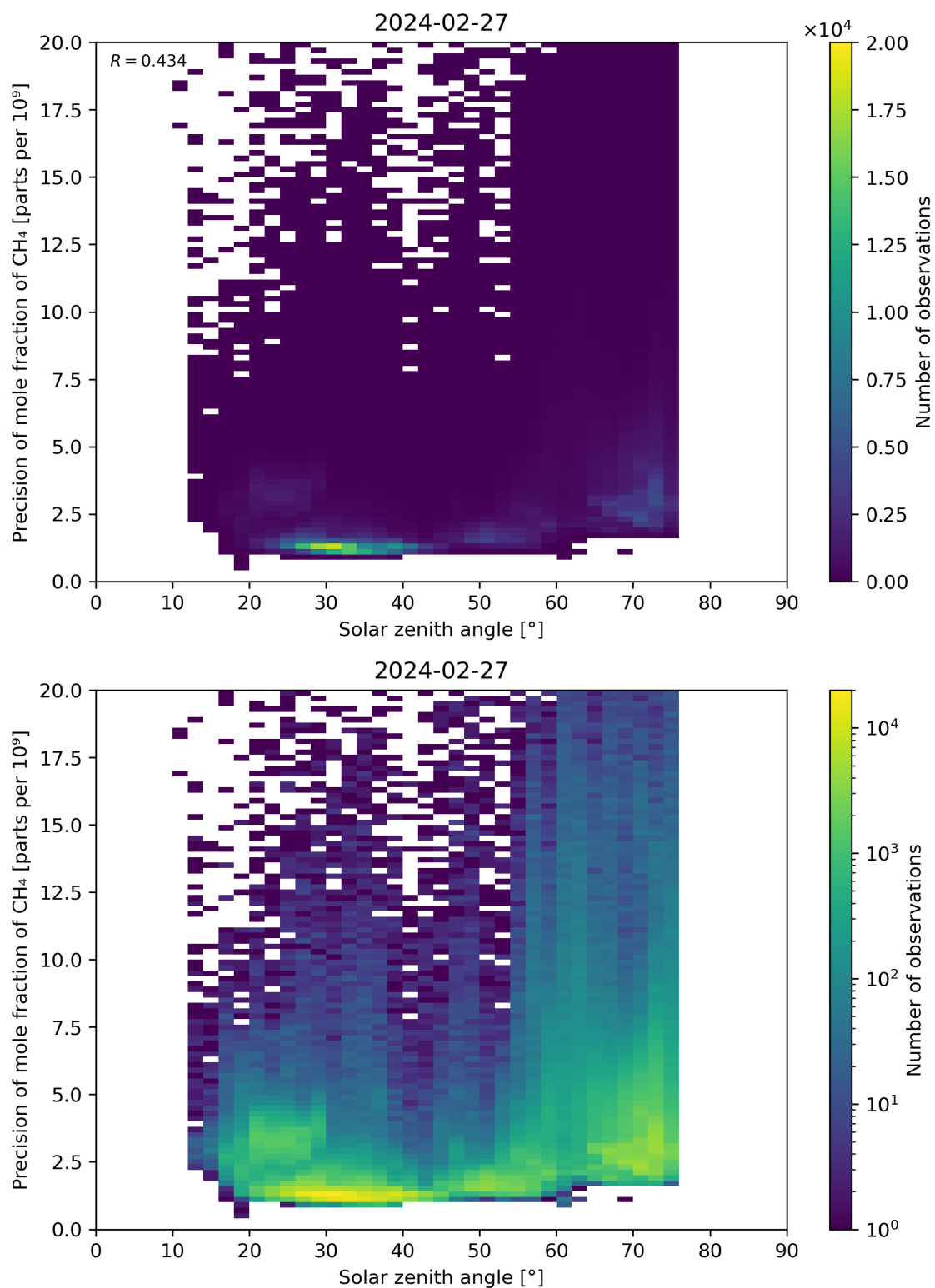
Figure 101: Scatter density plot of “Solar zenith angle” against “Precision of mole fraction of CH 4 ” for 2024-02-27 to 2024-02-28.
