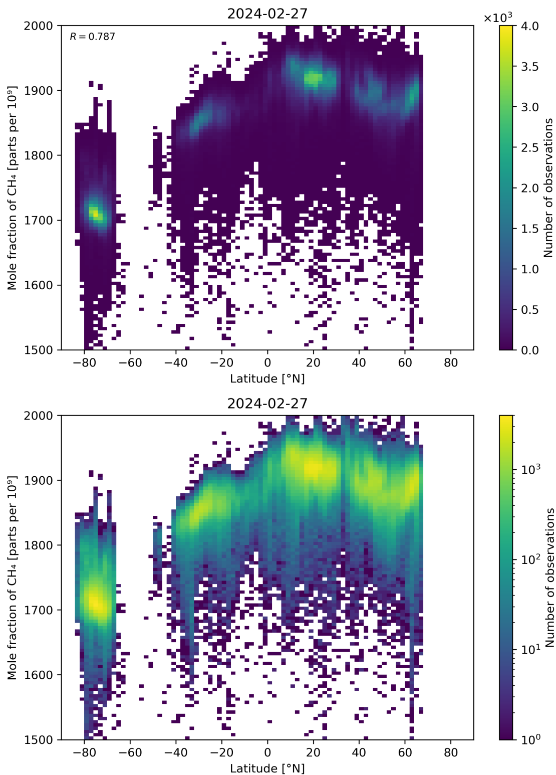
Figure 57: Scatter density plot of “Latitude” against “Mole fraction of CH 4 ” for 2024-02-27 to 2024-02-28.
