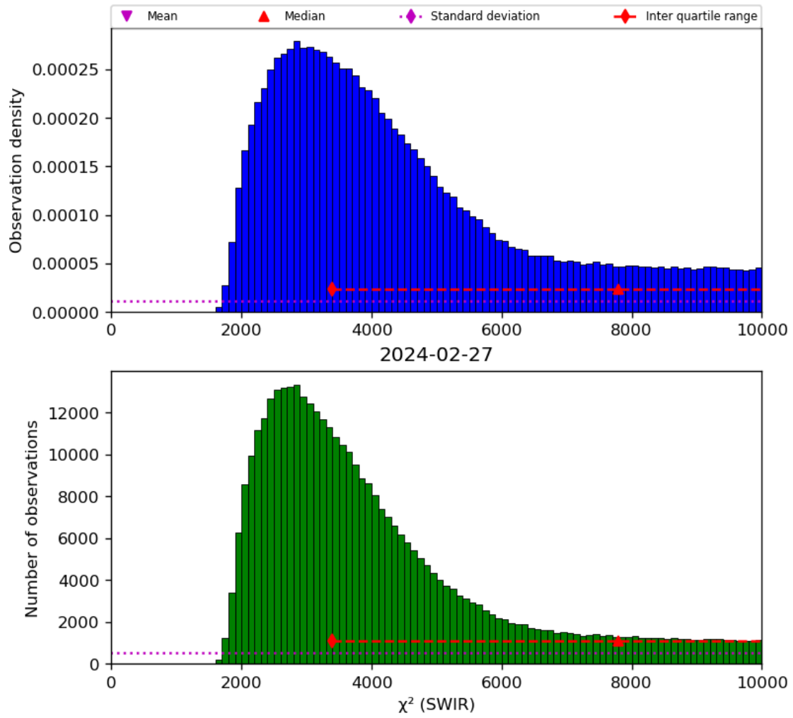
Figure 28: Histogram of “ \chi^2 (SWIR)” for 2024-02-27 to 2024-02-28
