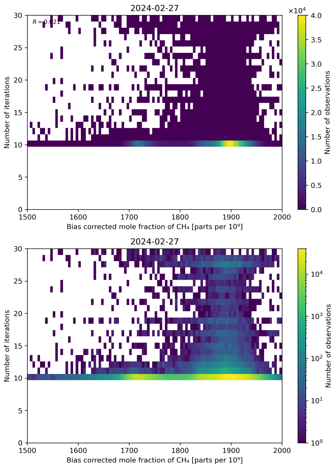
Figure 67: Scatter density plot of “Bias corrected mole fraction of \text{CH}_4 ” against “Number of iterations” for 2024-02-27 to 2024-02-28.
