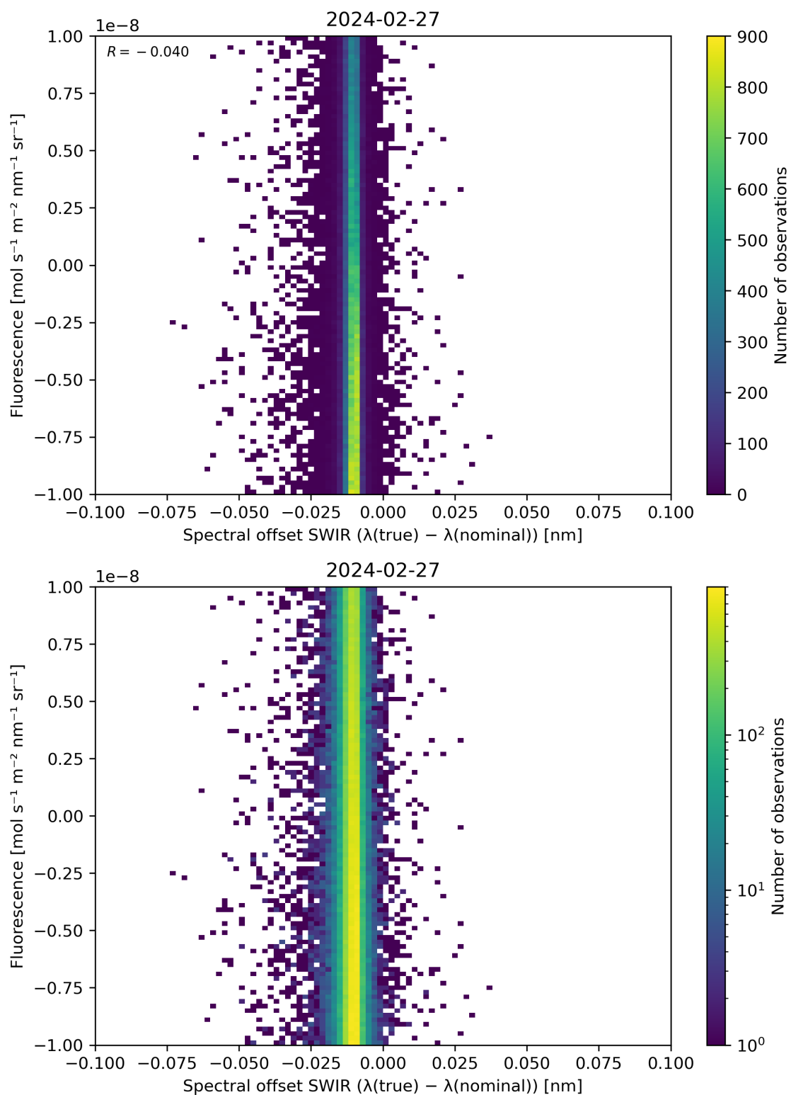
Figure 120: Scatter density plot of “Spectral offset SWIR ( \lambda(\text{true}) - \lambda(\text{nominal}) )” against “Fluorescence” for 2024-02-27 to 2024-02-28.
