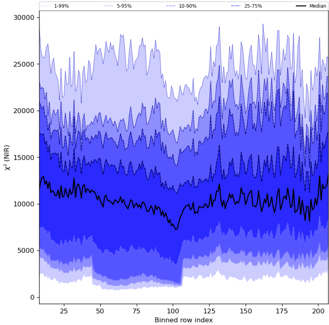
Figure 40: Along track statistics of “ \chi^2 (NIR)” for 2024-02-27 to 2024-02-28
