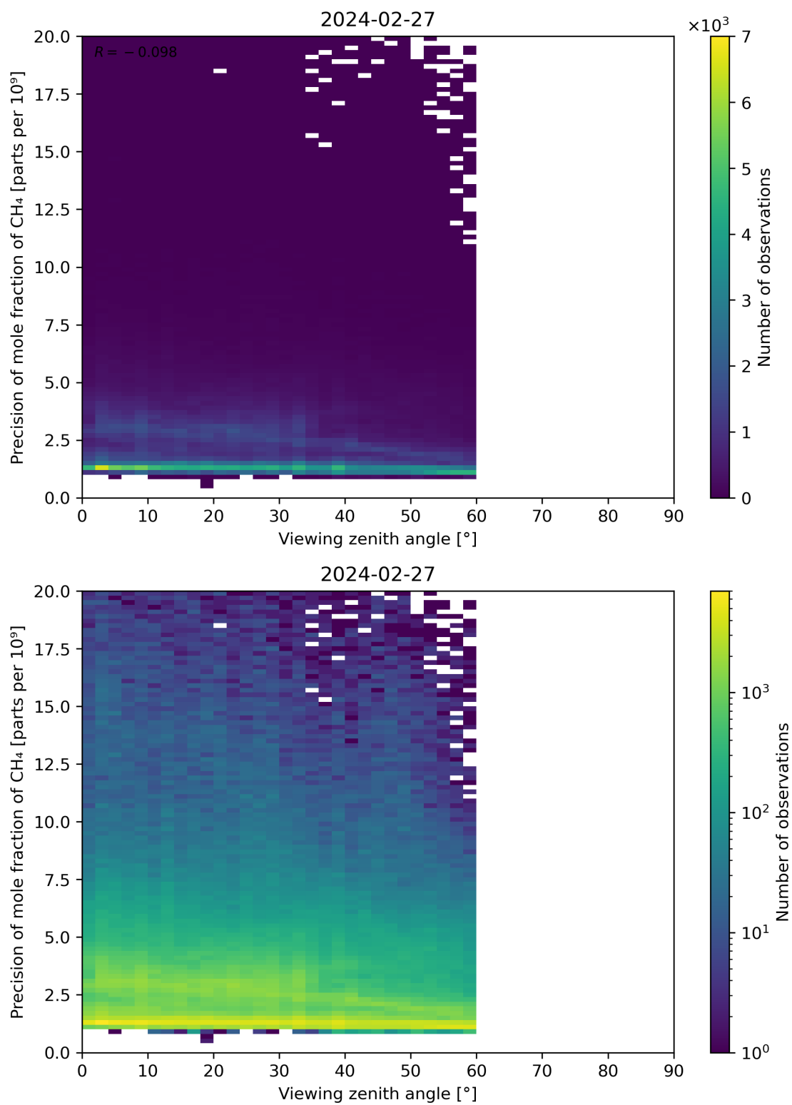
Figure 112: Scatter density plot of “Viewing zenith angle” against “Precision of mole fraction of CH 4 ” for 2024-02-27 to 2024-02-28.
