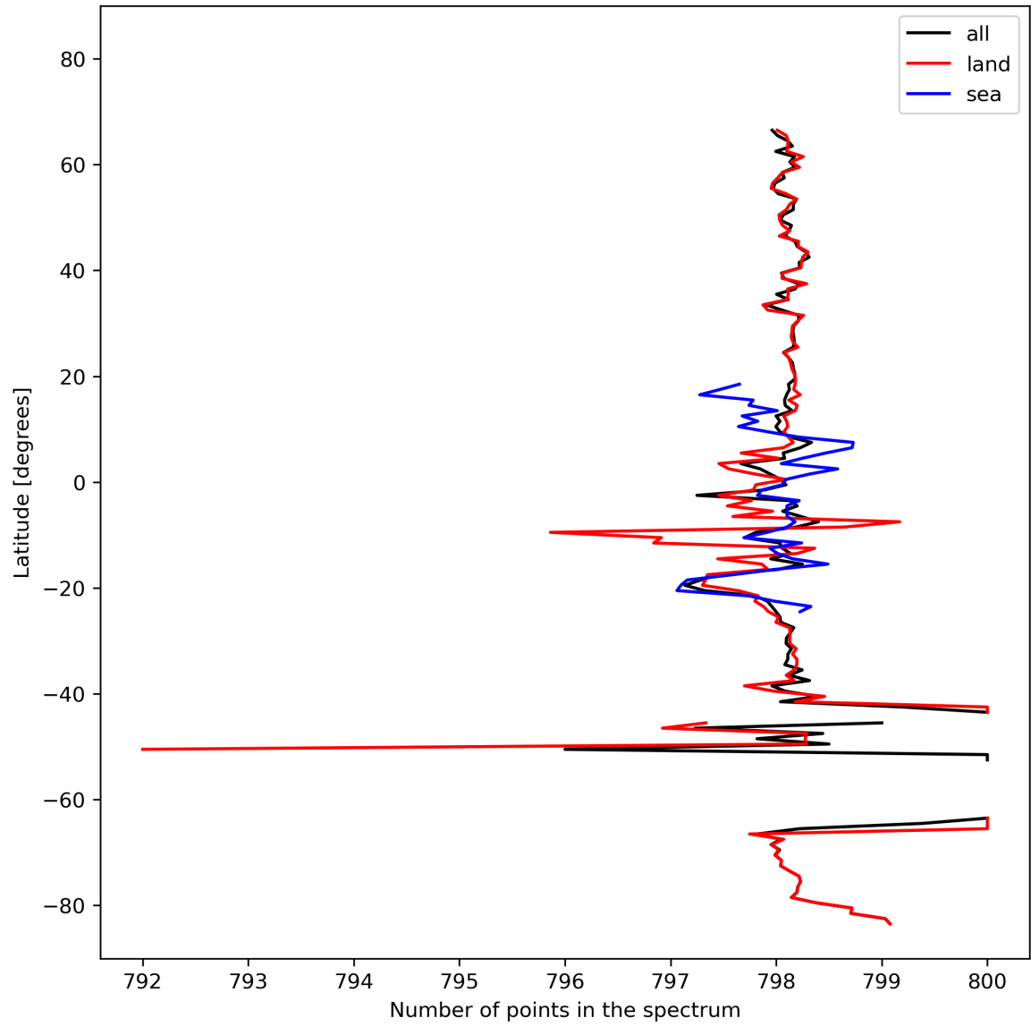
Figure 15: Zonal average of “Number of points in the spectrum” for 2024-02-27 to 2024-02-28.
