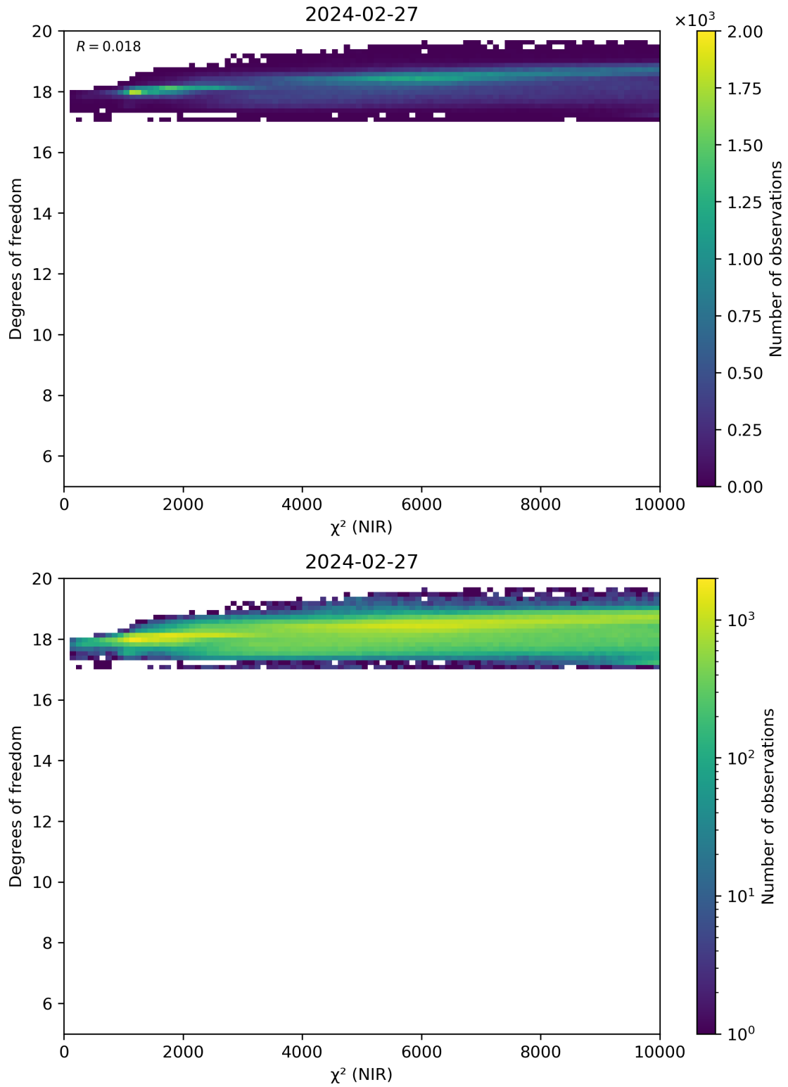
Figure 44: Scatter density plot of “ \chi^2 (NIR)” against “Degrees of freedom” for 2024-02-27 to 2024-02-28.
