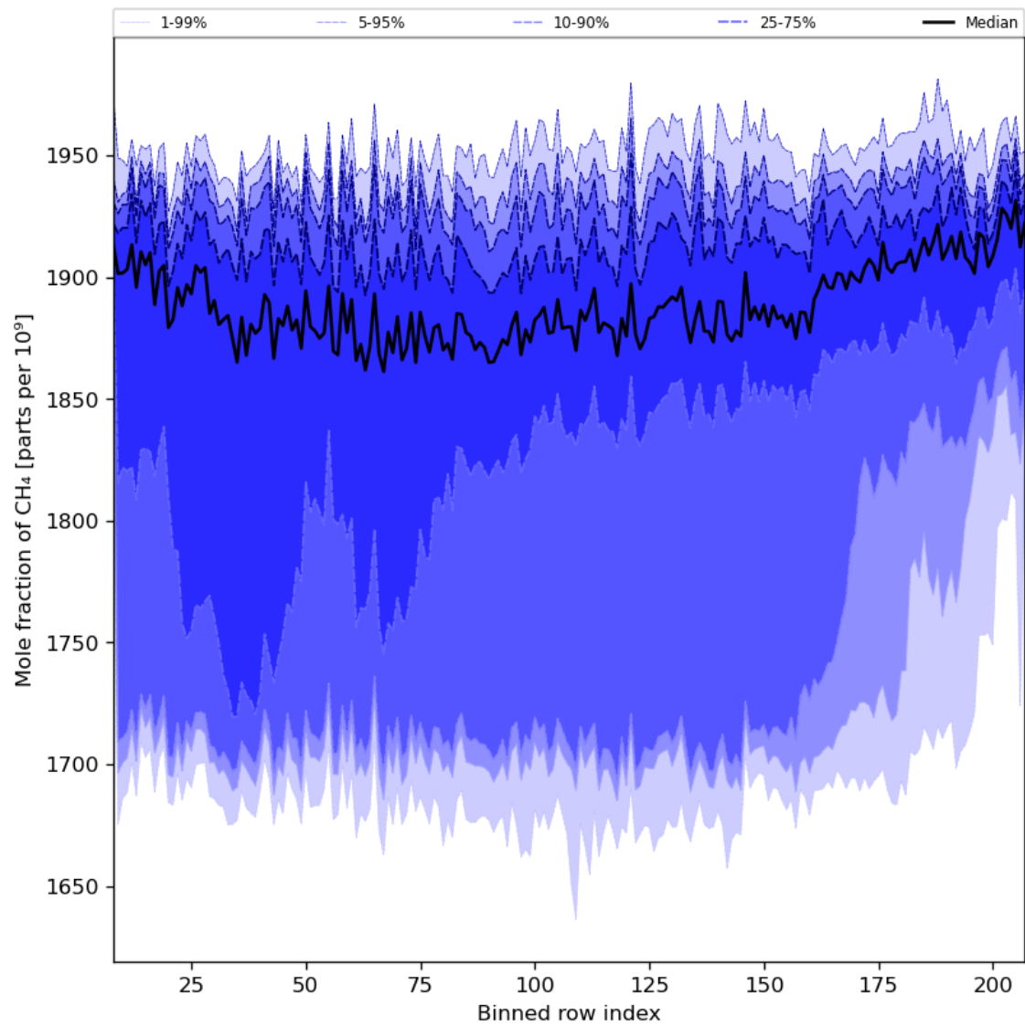
Figure 34: Along track statistics of “Mole fraction of CH 4 ” for 2024-02-27 to 2024-02-28
