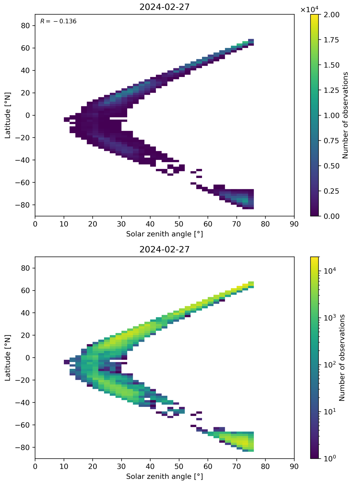
Figure 98: Scatter density plot of “Solar zenith angle” against “Latitude” for 2024-02-27 to 2024-02-28.
