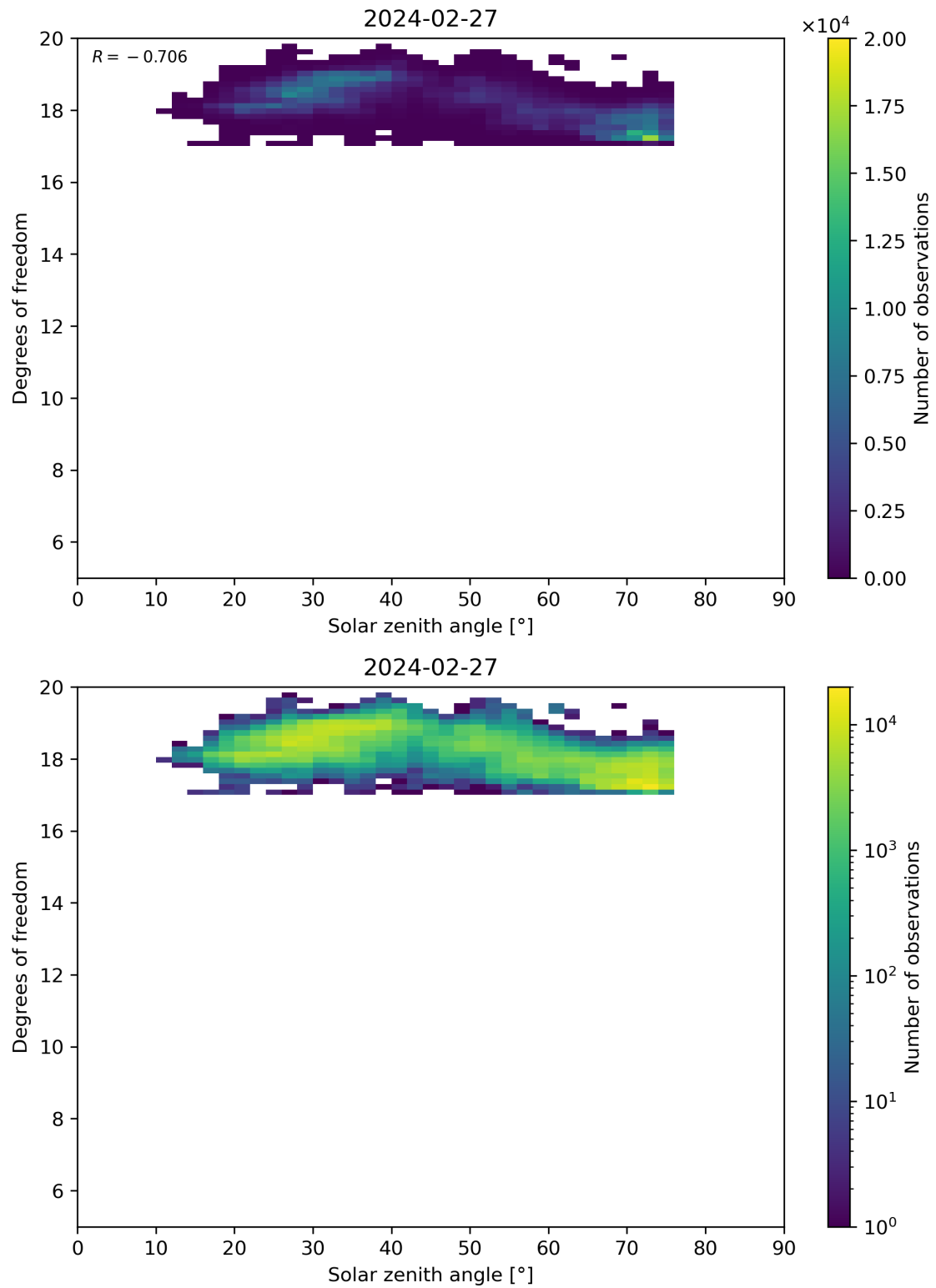
Figure 96: Scatter density plot of “Solar zenith angle” against “Degrees of freedom” for 2024-02-27 to 2024-02-28.
