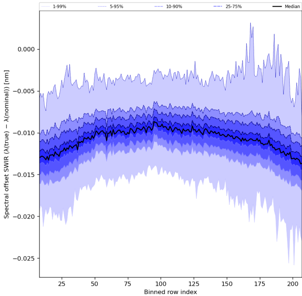
Figure 38: Along track statistics of “Spectral offset SWIR ( \lambda(\text{true}) - \lambda(\text{nominal}) )” for 2024-02-27 to 2024-02-28
