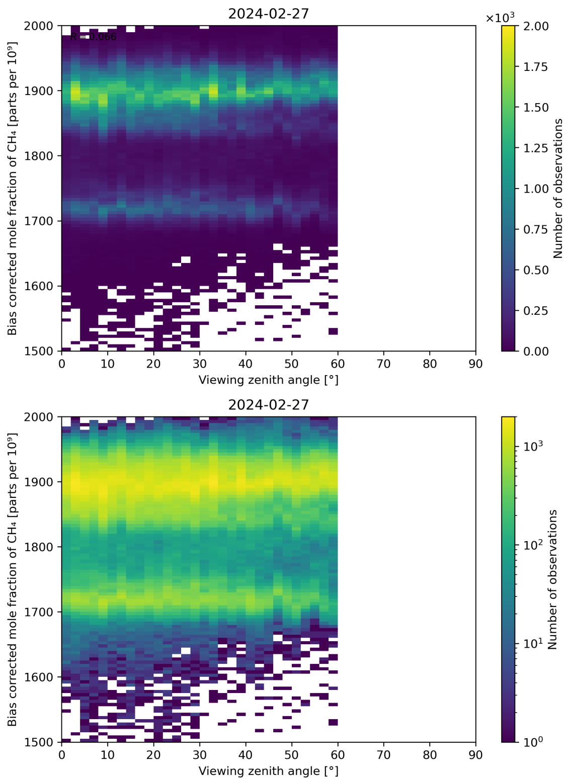
Figure 111: Scatter density plot of “Viewing zenith angle” against “Bias corrected mole fraction of CH 4 ” for 2024-02-27 to 2024-02-28.
