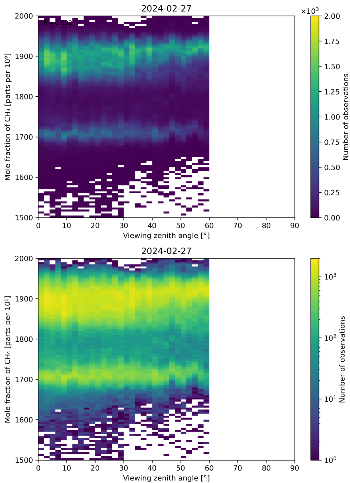
Figure 110: Scatter density plot of “Viewing zenith angle” against “Mole fraction of CH 4 ” for 2024-02-27 to 2024-02-28.
