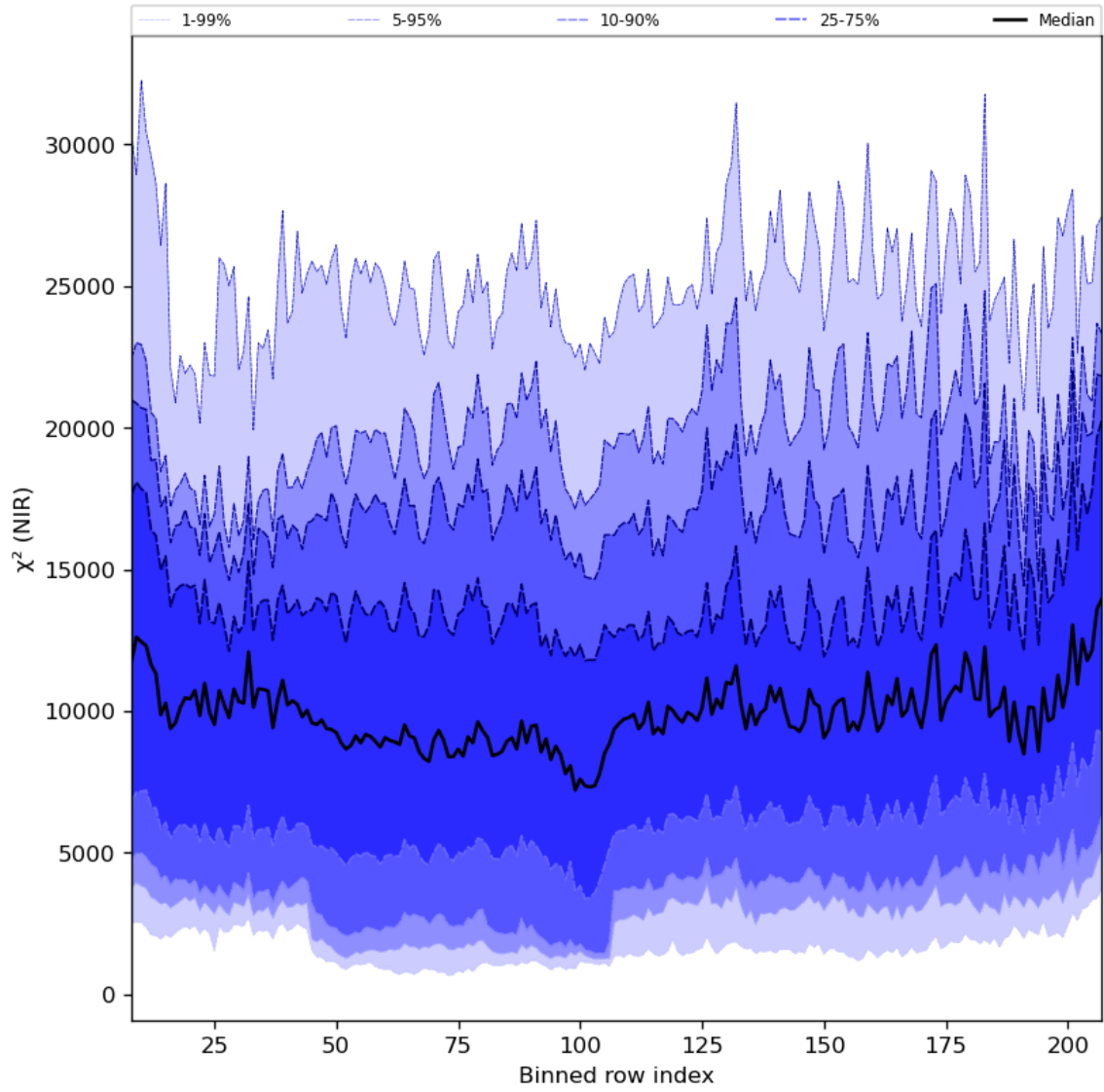
Figure 40: Along track statistics of “ \chi^2 (NIR)” for 2024-02-27 to 2024-02-29
