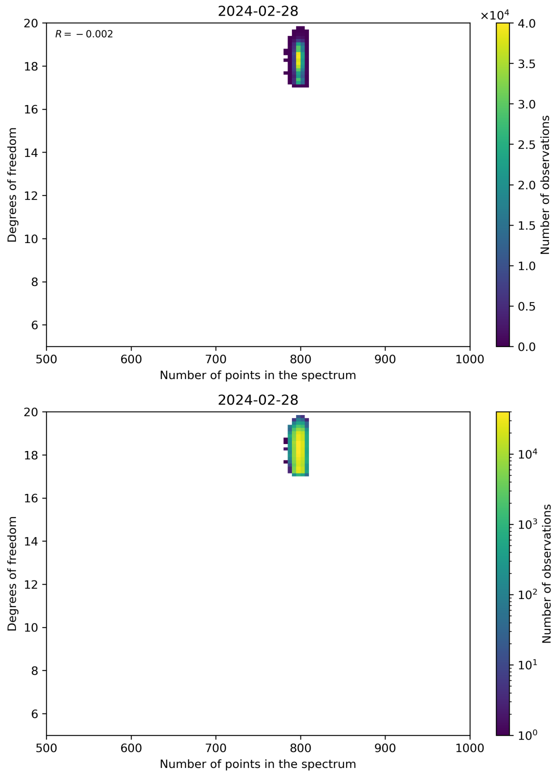
Figure 90: Scatter density plot of “Number of points in the spectrum” against “Degrees of freedom” for 2024-02-27 to 2024-02-29.
