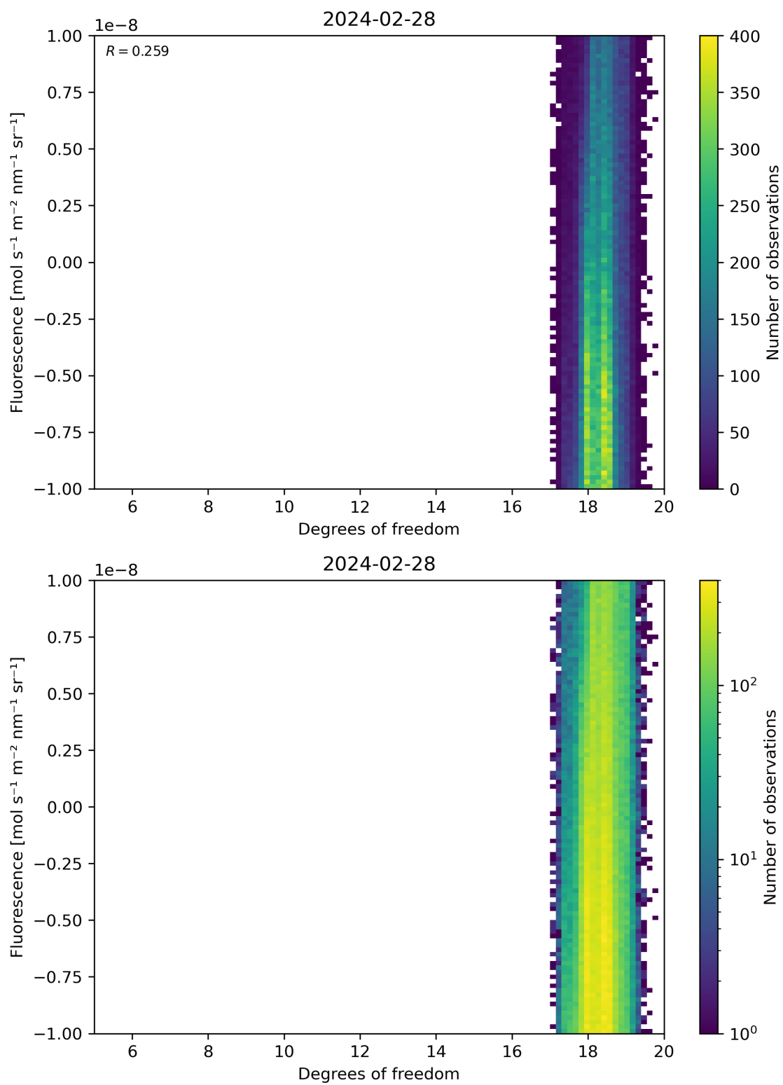
Figure 51: Scatter density plot of “Degrees of freedom” against “Fluorescence” for 2024-02-27 to 2024-02-29.
