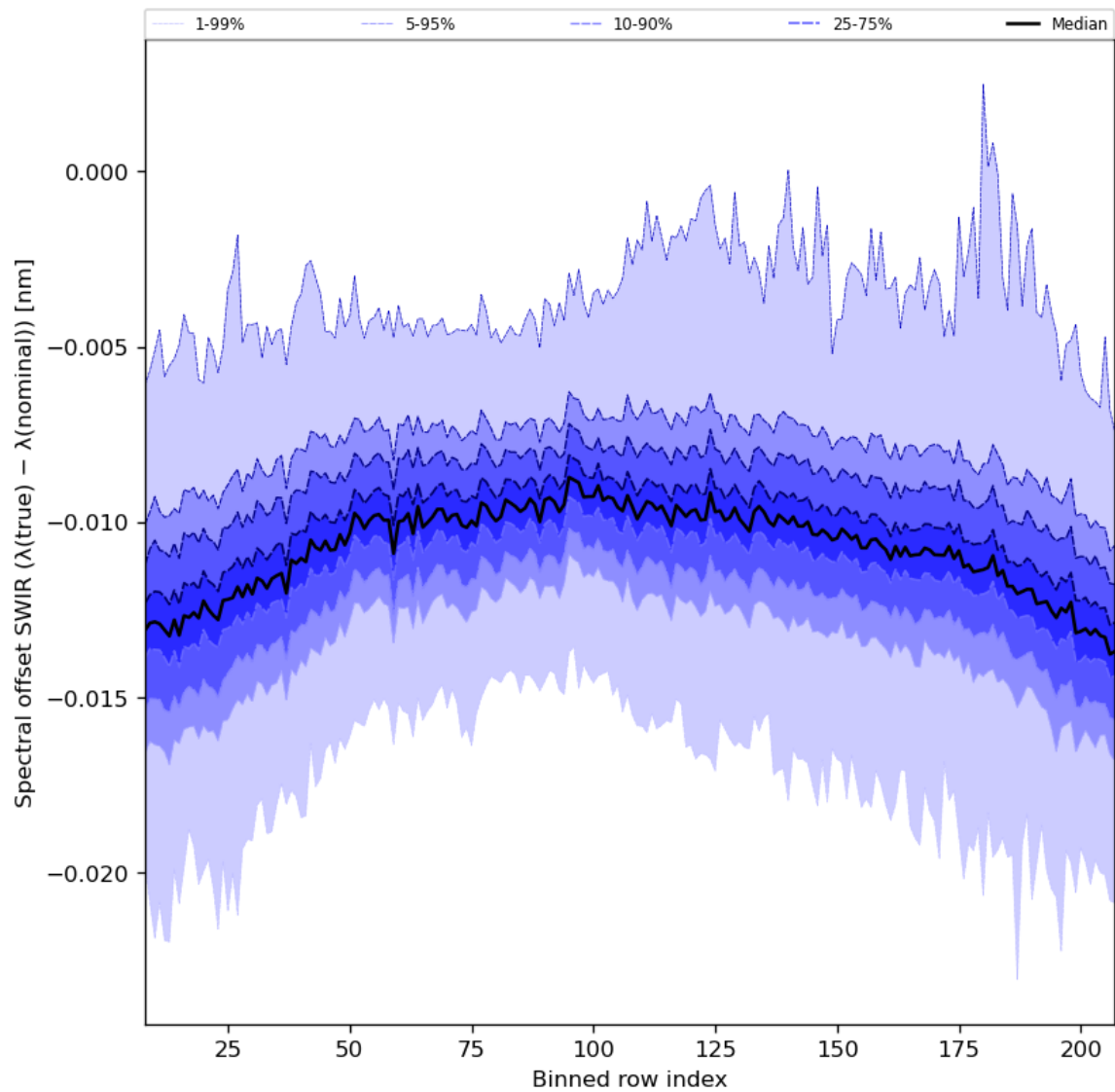
Figure 38: Along track statistics of “Spectral offset SWIR ( \lambda(\text{true}) - \lambda(\text{nominal}) )” for 2024-02-27 to 2024-02-29
