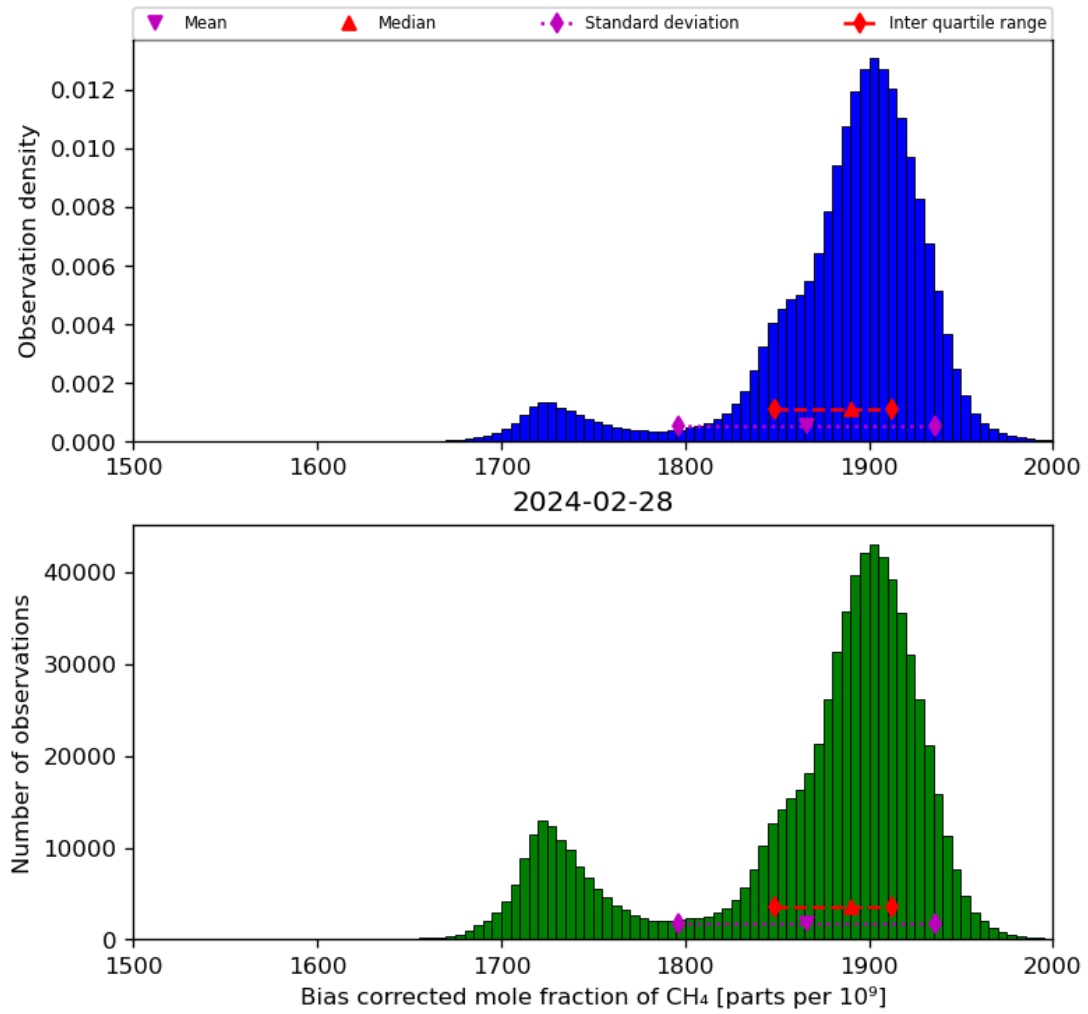
Figure 25: Histogram of “Bias corrected mole fraction of CH 4 ” for 2024-02-27 to 2024-02-29
