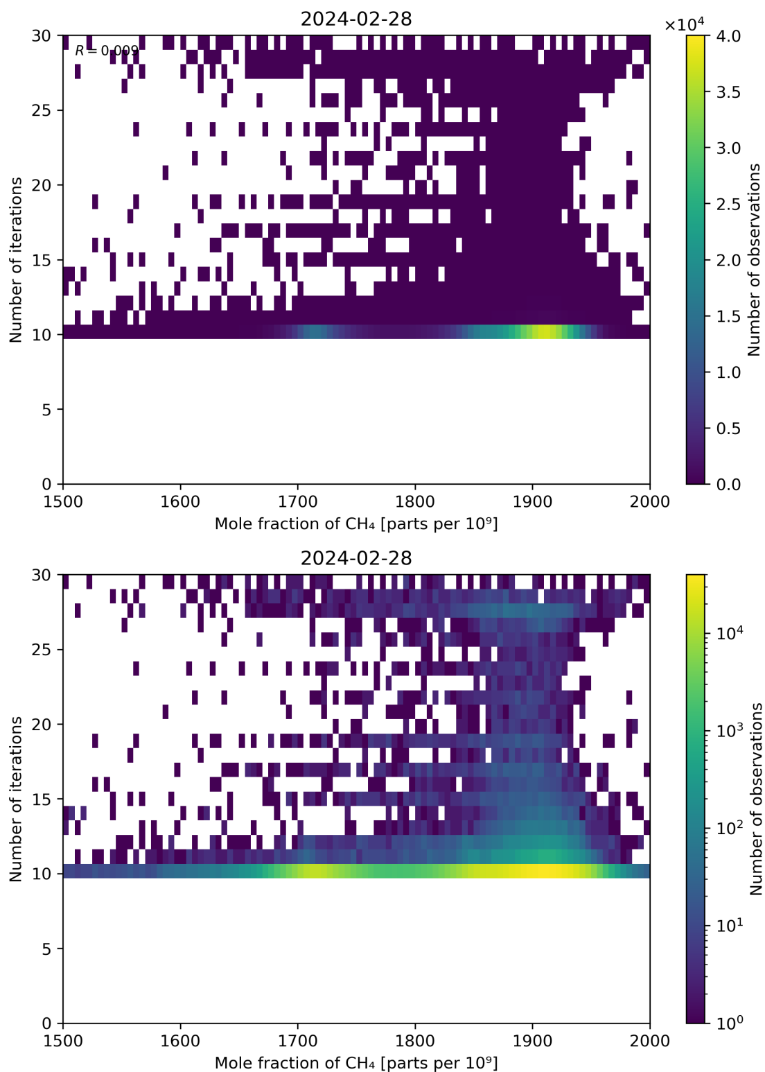
Figure 76: Scatter density plot of “Mole fraction of CH 4 ” against “Number of iterations” for 2024-02-27 to 2024-02-29.
