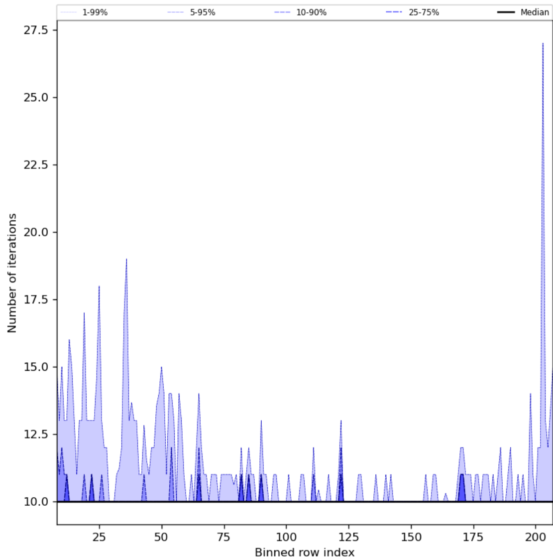
Figure 42: Along track statistics of “Number of iterations” for 2024-02-27 to 2024-02-29
