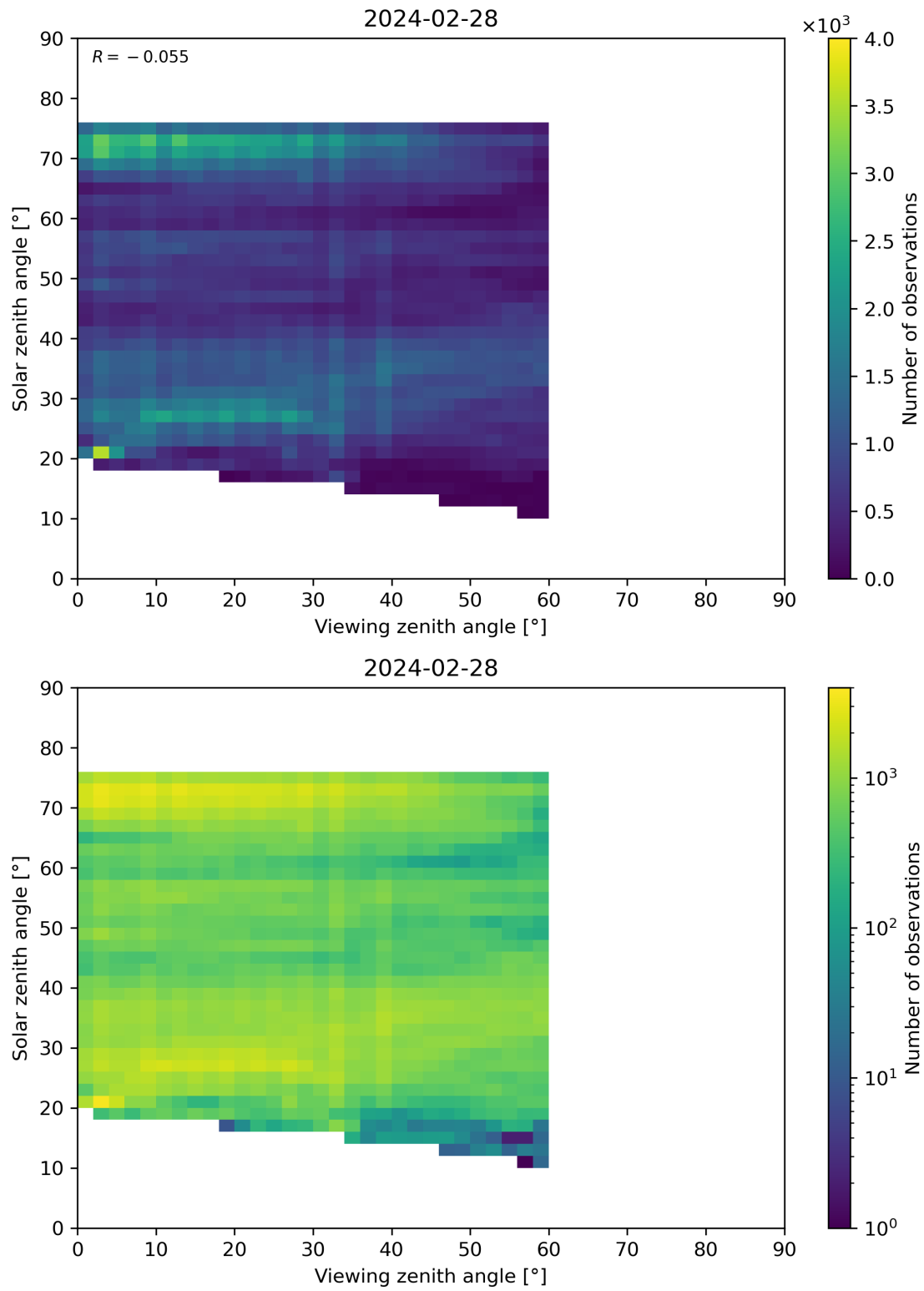
Figure 115: Scatter density plot of “Viewing zenith angle” against “Solar zenith angle” for 2024-02-27 to 2024-02-29.
