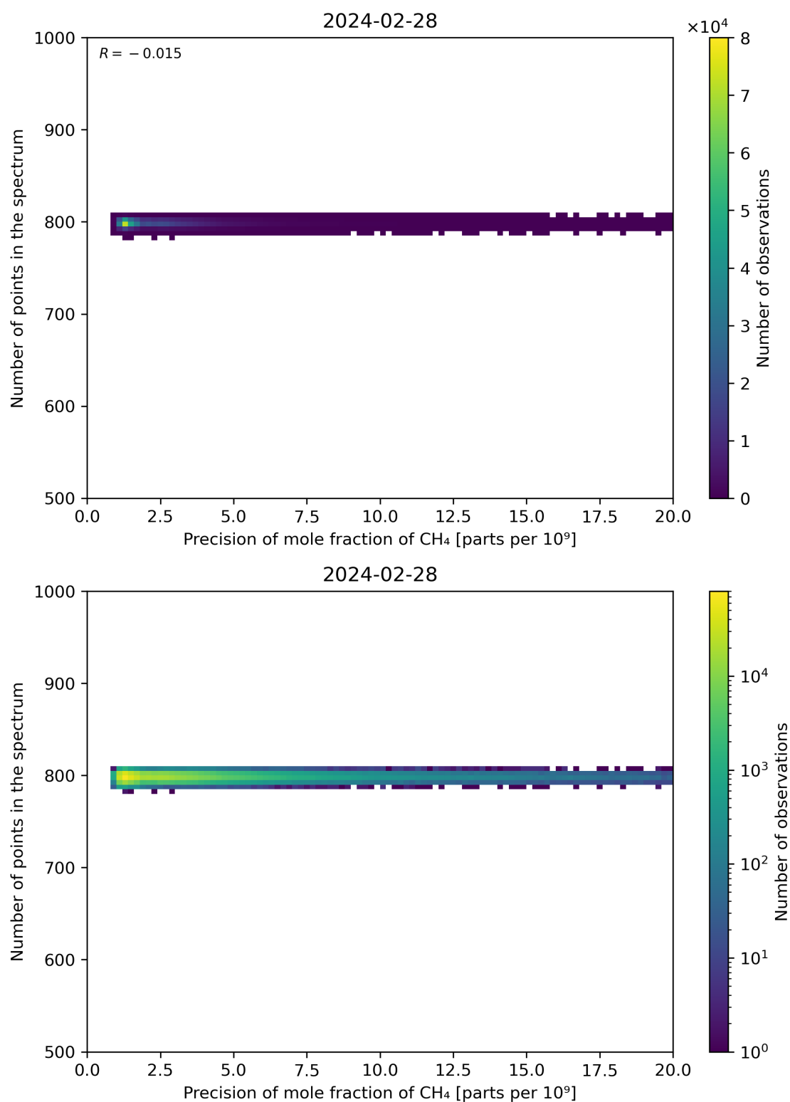
Figure 84: Scatter density plot of “Precision of mole fraction of CH 4 ” against “Number of points in the spectrum” for 2024-02-27 to 2024-02-29.
