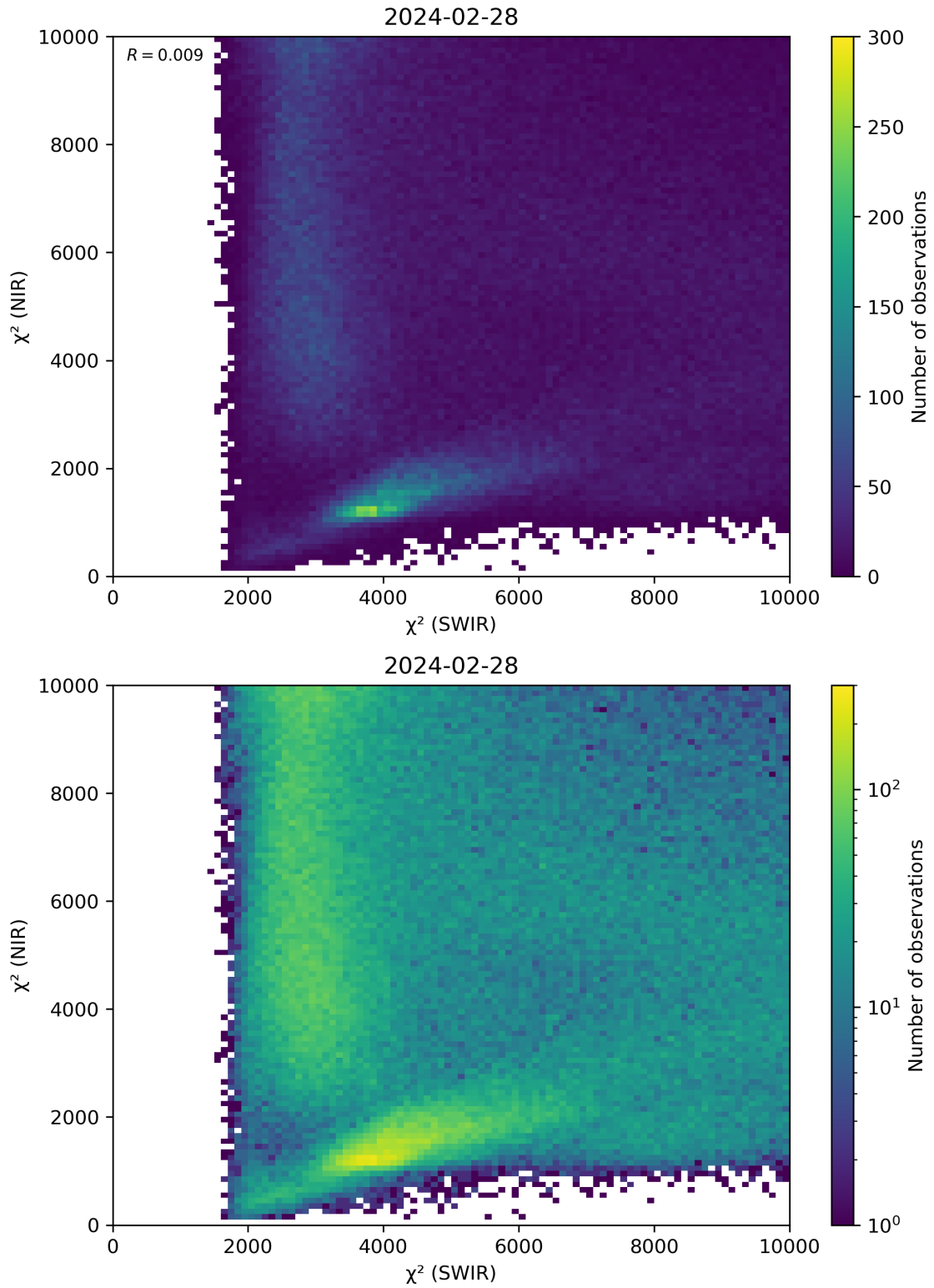
Figure 47: Scatter density plot of “ \chi^2 (SWIR)” against “ \chi^2 (NIR)” for 2024-02-27 to 2024-02-29.
