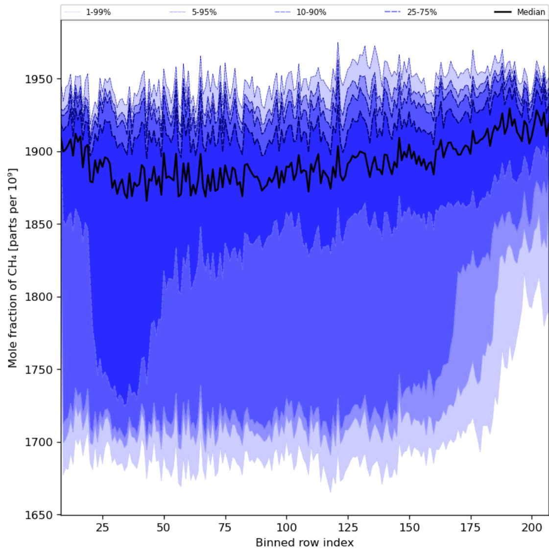
Figure 34: Along track statistics of “Mole fraction of CH 4 ” for 2024-02-27 to 2024-02-29
