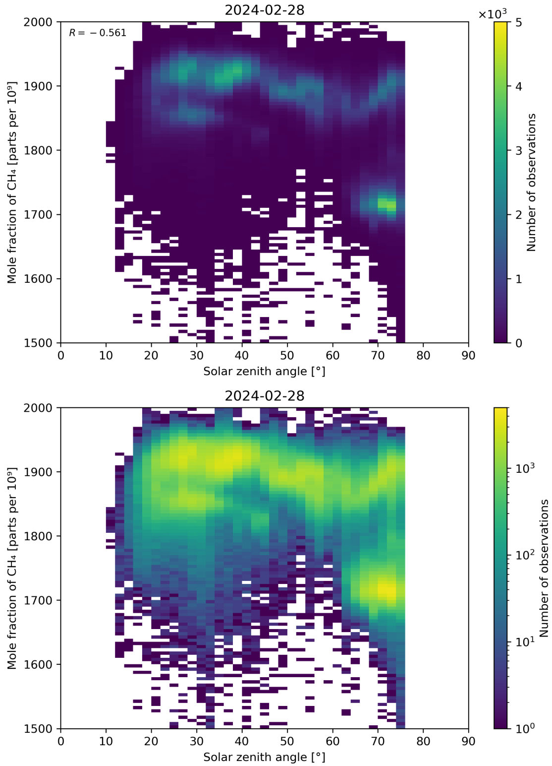
Figure 99: Scatter density plot of “Solar zenith angle” against “Mole fraction of \text{CH}_4 ” for 2024-02-27 to 2024-02-29.
