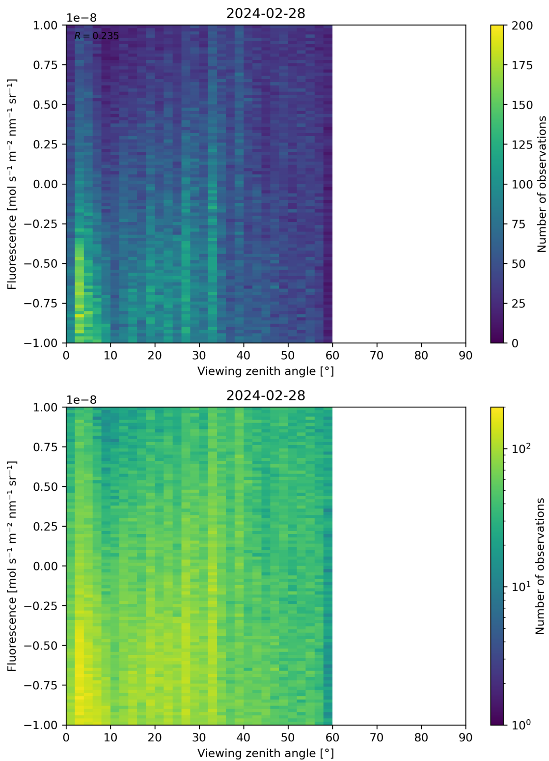
Figure 108: Scatter density plot of “Viewing zenith angle” against “Fluorescence” for 2024-02-27 to 2024-02-29.
