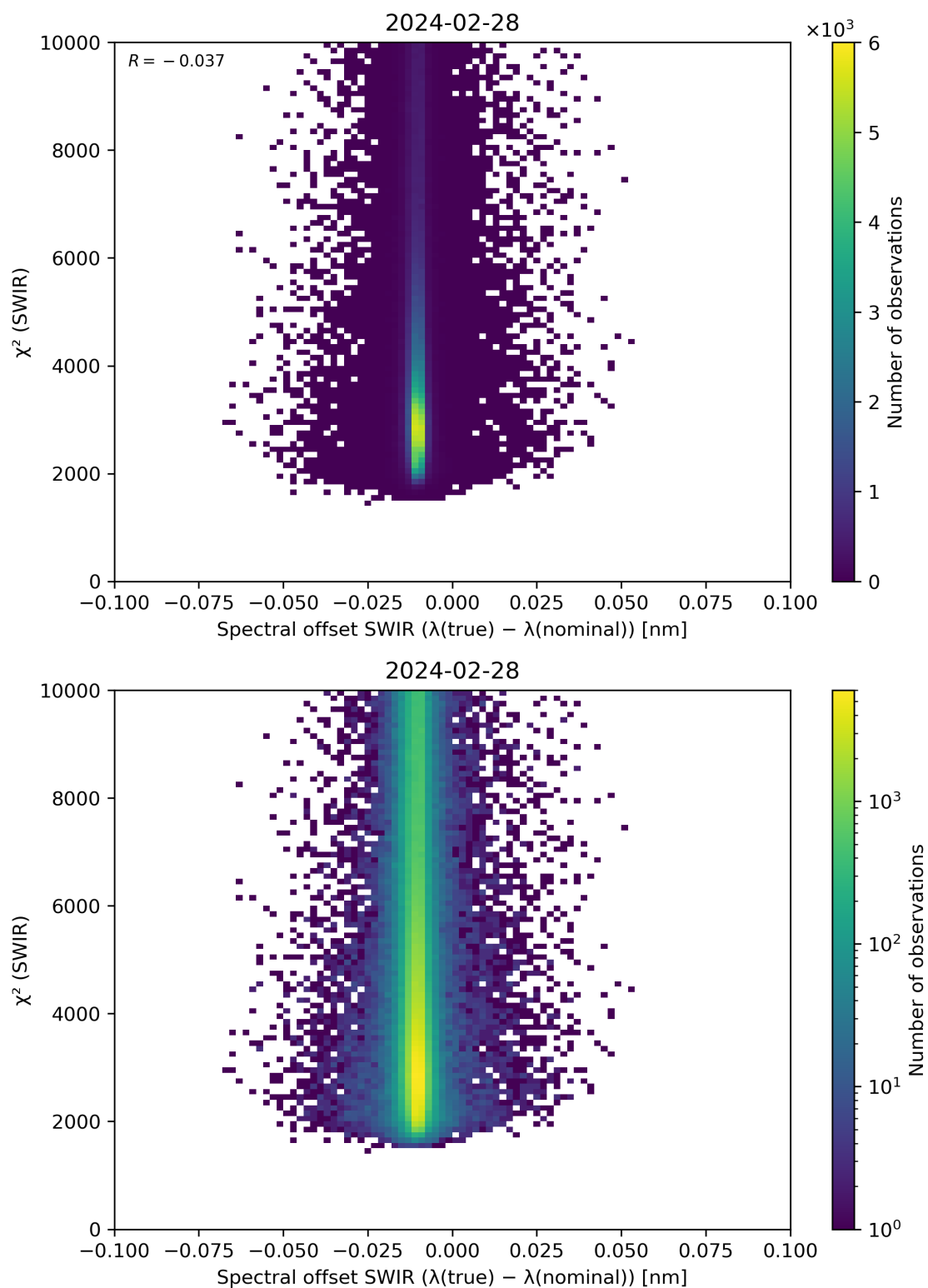
Figure 118: Scatter density plot of “Spectral offset SWIR ( \lambda(\text{true}) - \lambda(\text{nominal}) )” against “ \chi^2 (SWIR)” for 2024-02-27 to 2024-02-29.
