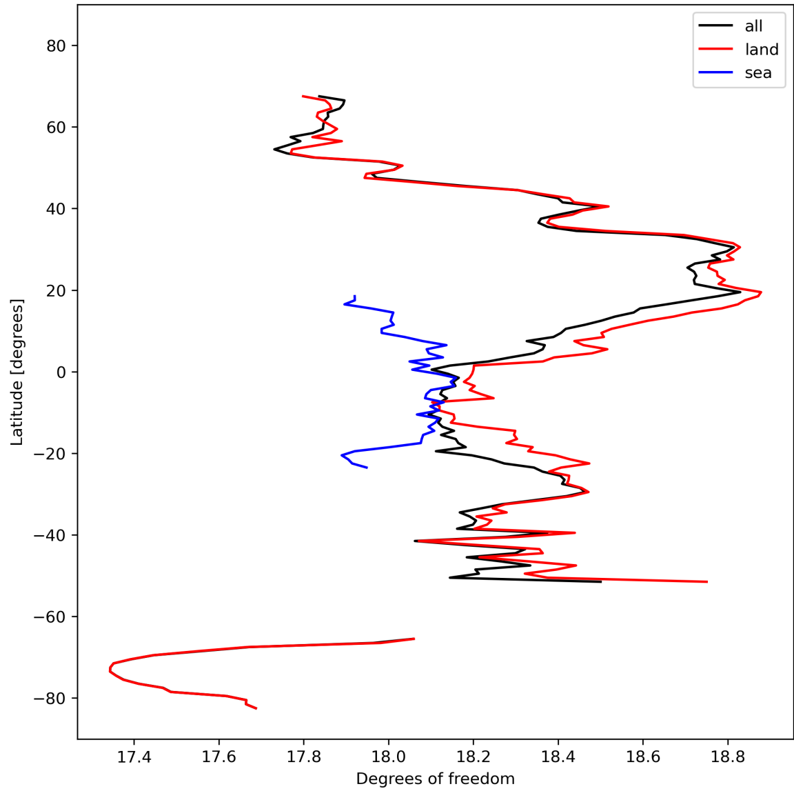
Figure 19: Zonal average of “Degrees of freedom” for 2024-02-27 to 2024-02-29.
