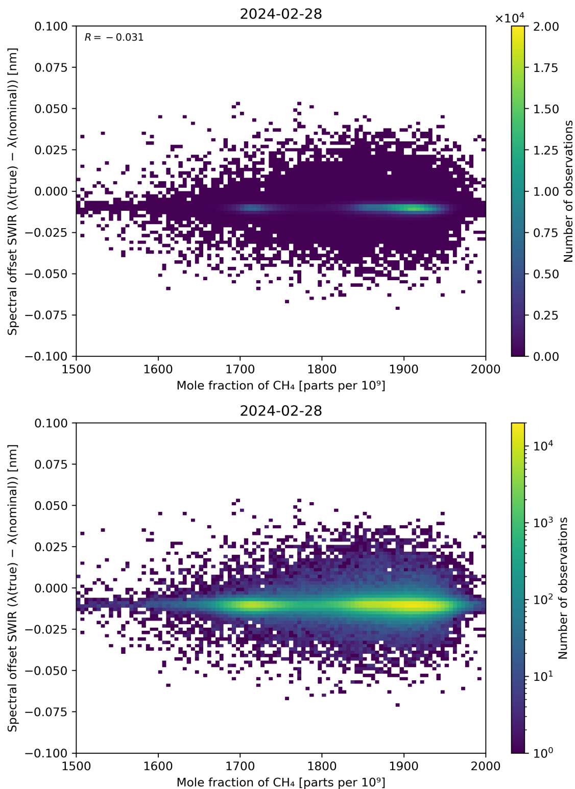
Figure 86: Scatter density plot of “Mole fraction of CH 4 ” against “Spectral offset SWIR ( \lambda(\text{true}) - \lambda(\text{nominal}) )” for 2024-02-27 to 2024-02-29.
