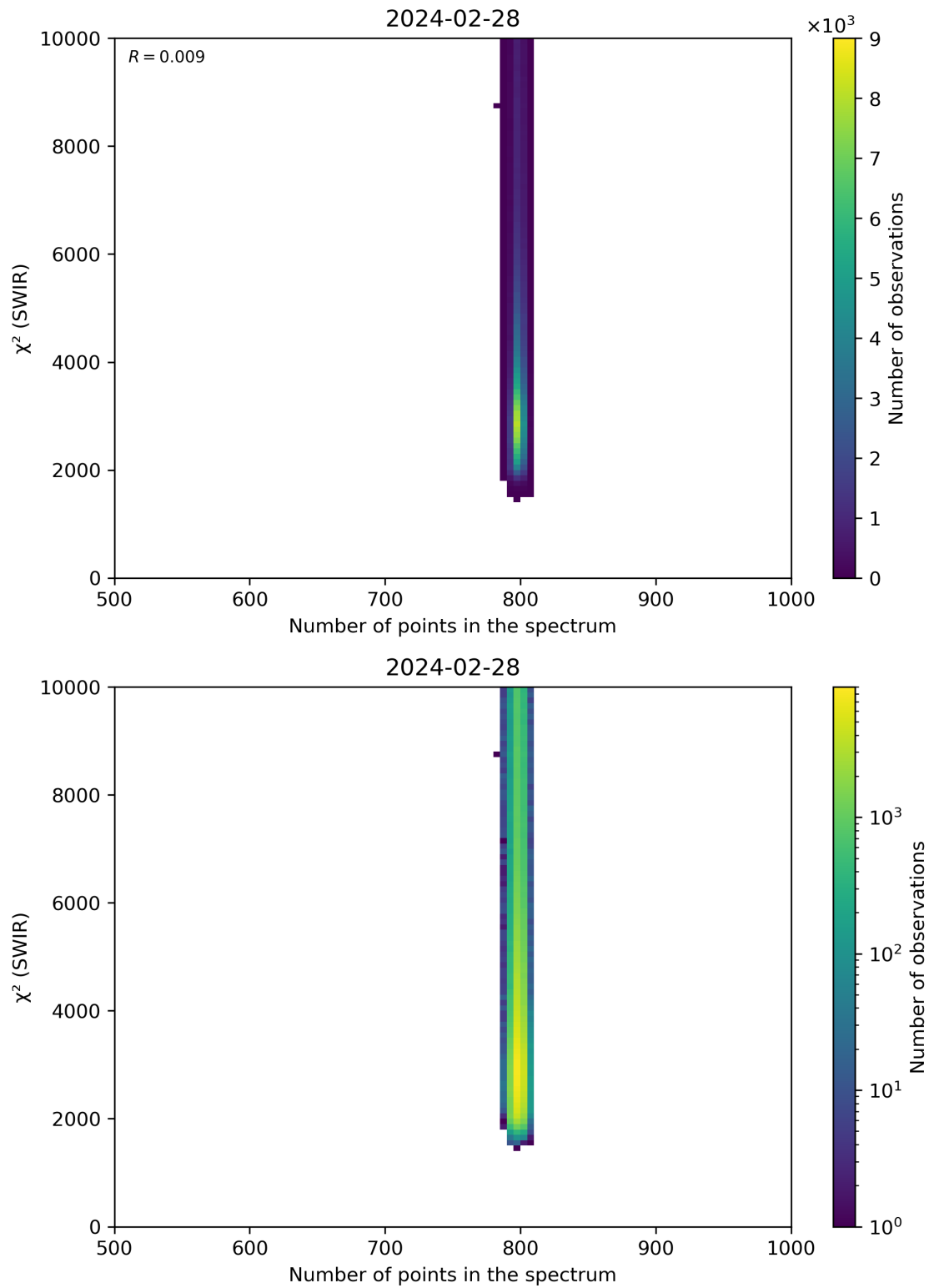
Figure 89: Scatter density plot of “Number of points in the spectrum” against “ \chi^2 (SWIR)” for 2024-02-27 to 2024-02-29.
