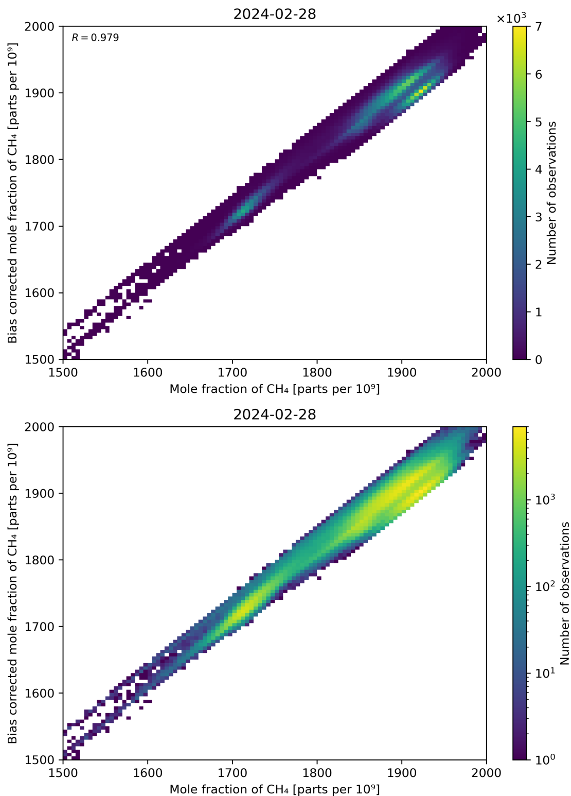
Figure 74: Scatter density plot of “Mole fraction of CH 4 ” against “Bias corrected mole fraction of CH 4 ” for 2024-02-27 to 2024-02-29.
