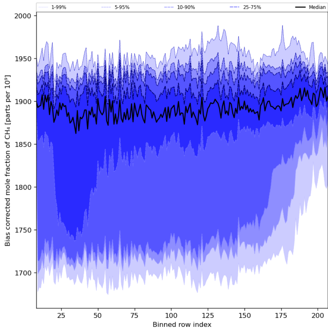
Figure 36: Along track statistics of “Bias corrected mole fraction of CH 4 ” for 2024-02-27 to 2024-02-29
