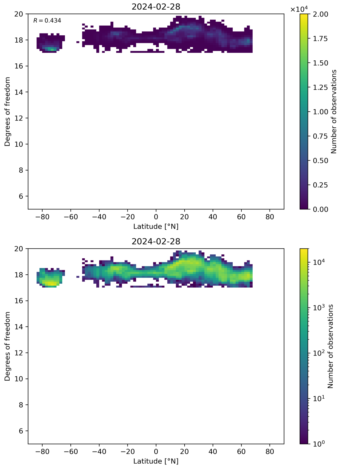
Figure 55: Scatter density plot of “Latitude” against “Degrees of freedom” for 2024-02-27 to 2024-02-29.
