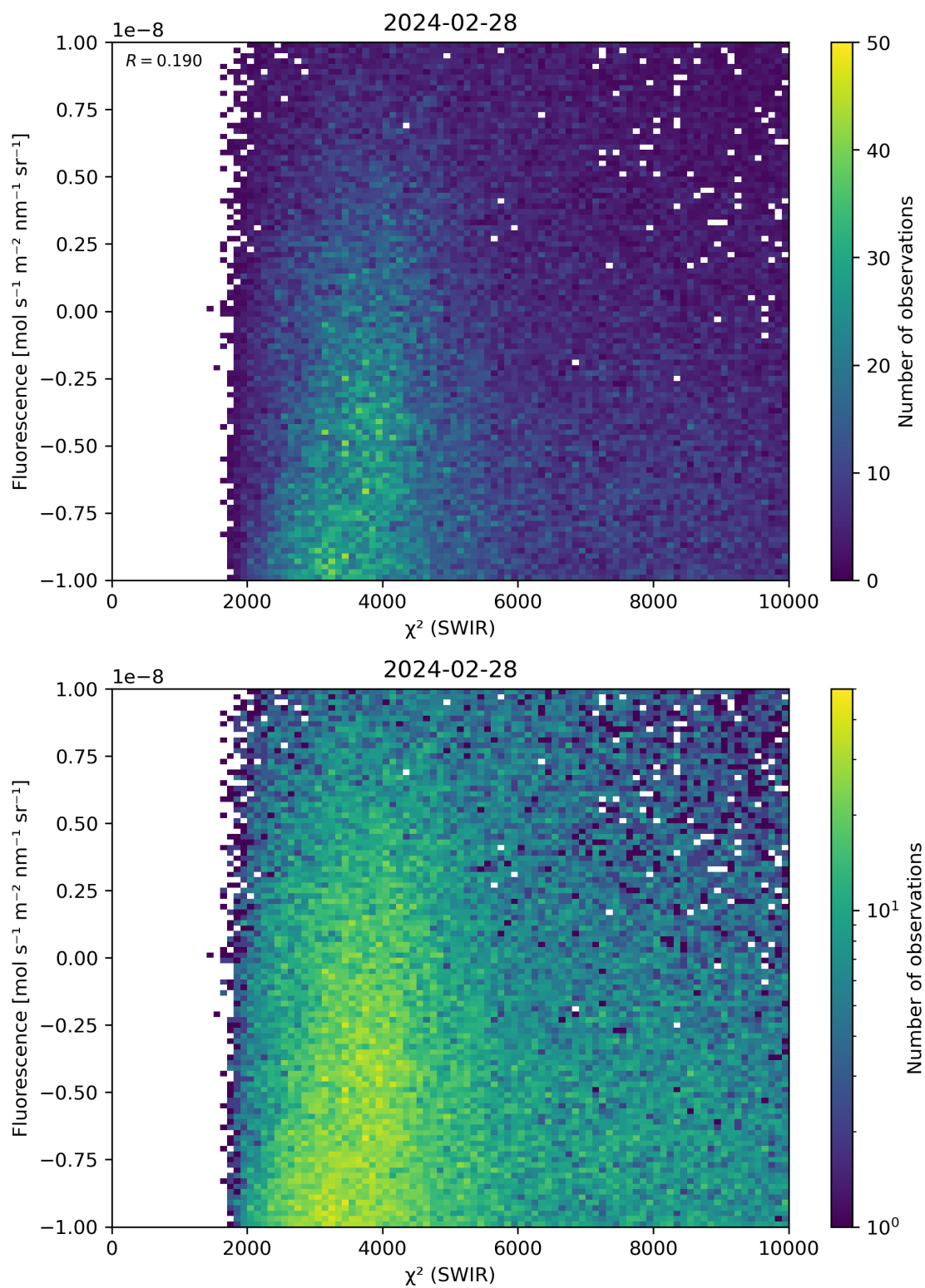
Figure 49: Scatter density plot of “ \chi^2 (SWIR)” against “Fluorescence” for 2024-02-27 to 2024-02-29.
