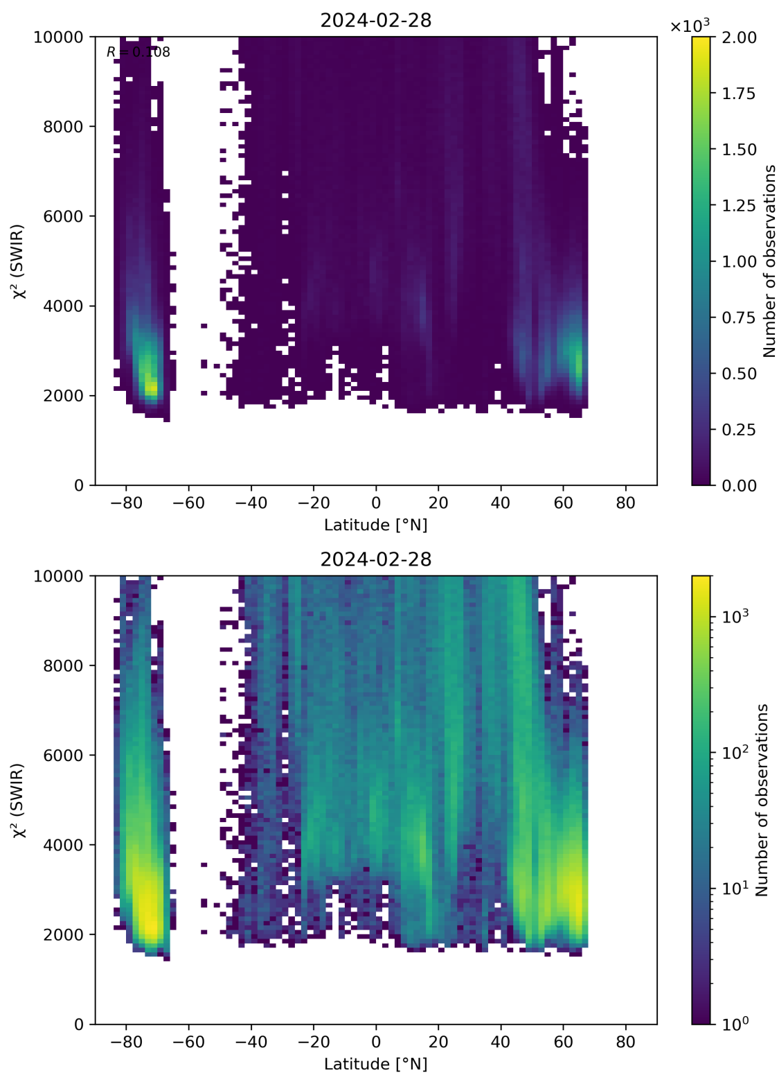
Figure 54: Scatter density plot of “Latitude” against “ \chi^2 (SWIR)” for 2024-02-27 to 2024-02-29.
