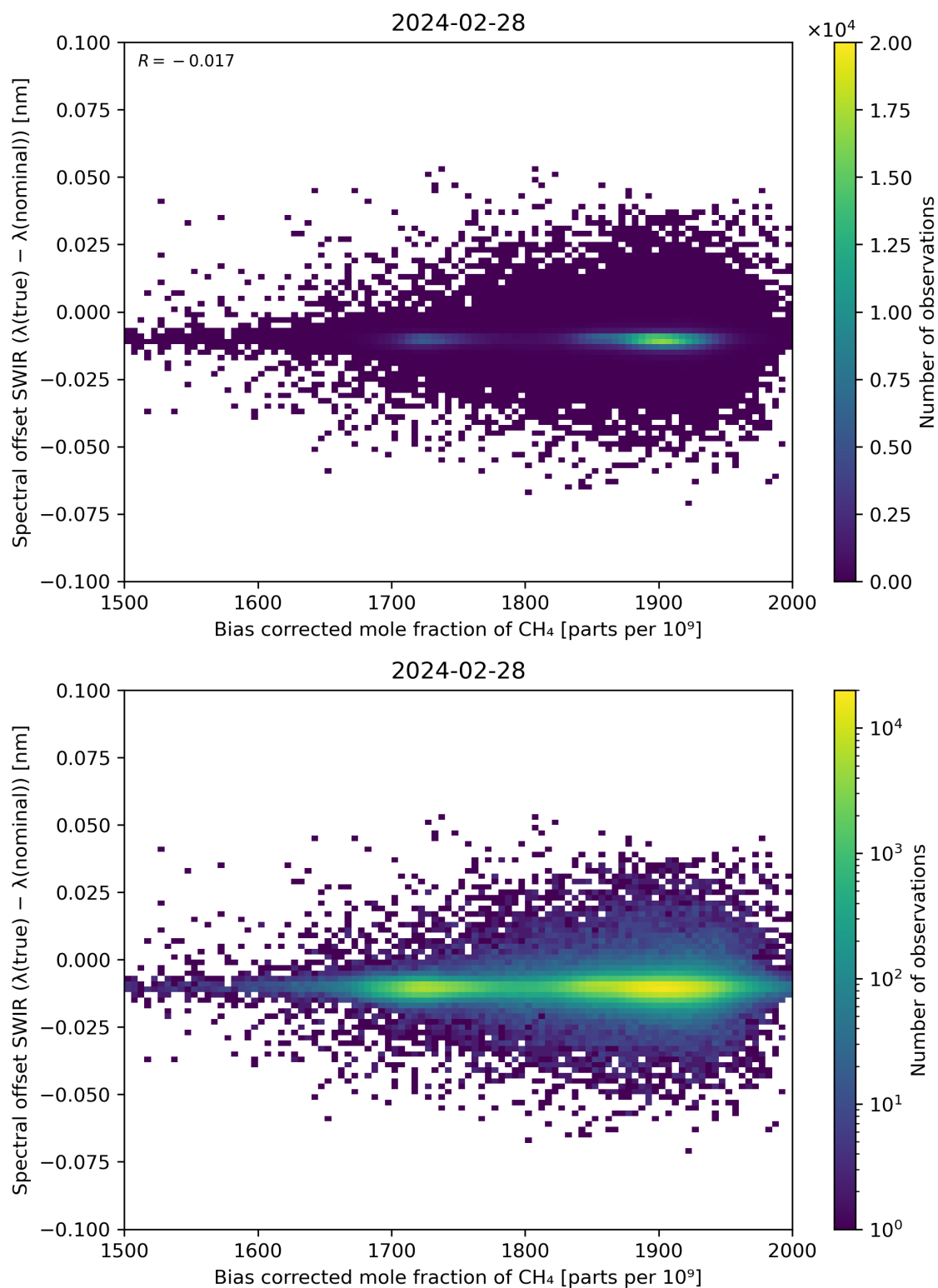
Figure 69: Scatter density plot of “Bias corrected mole fraction of \text{CH}_4 ” against “Spectral offset SWIR ( \lambda(\text{true}) - \lambda(\text{nominal}) )” for 2024-02-27 to 2024-02-29.
