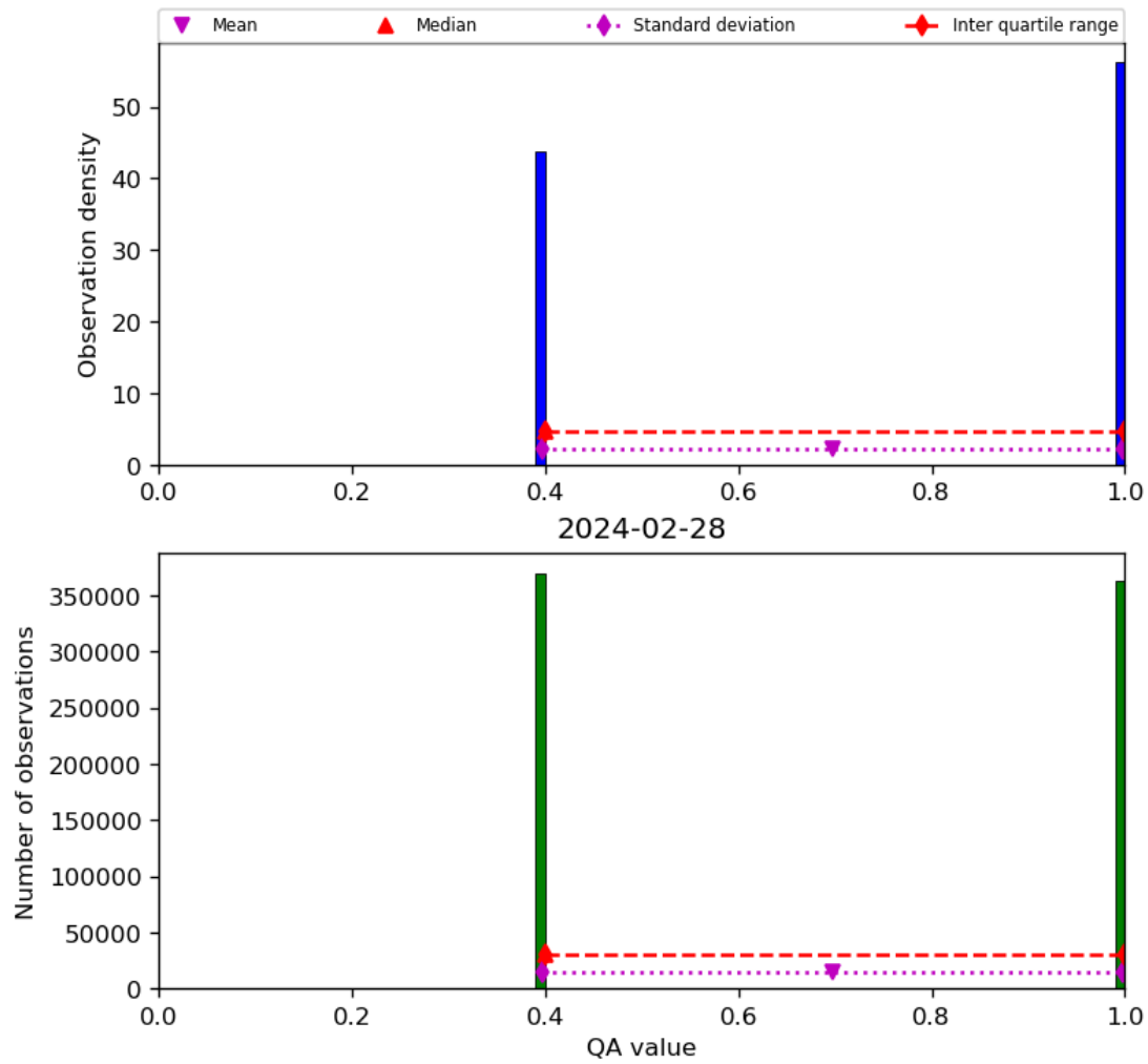
Figure 22: Histogram of “QA value” for 2024-02-27 to 2024-02-29
