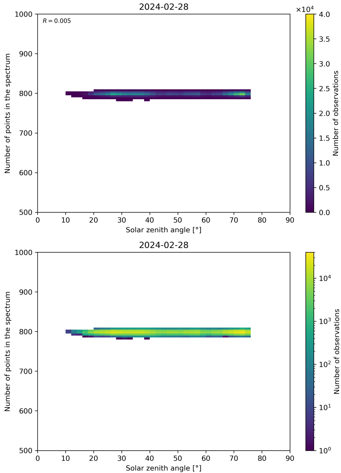
Figure 103: Scatter density plot of “Solar zenith angle” against “Number of points in the spectrum” for 2024-02-27 to 2024-02-29.
