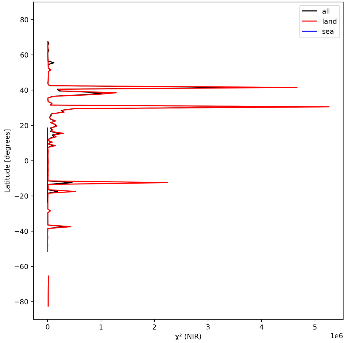
Figure 18: Zonal average of “ \chi^2 (NIR)” for 2024-02-27 to 2024-02-29.
