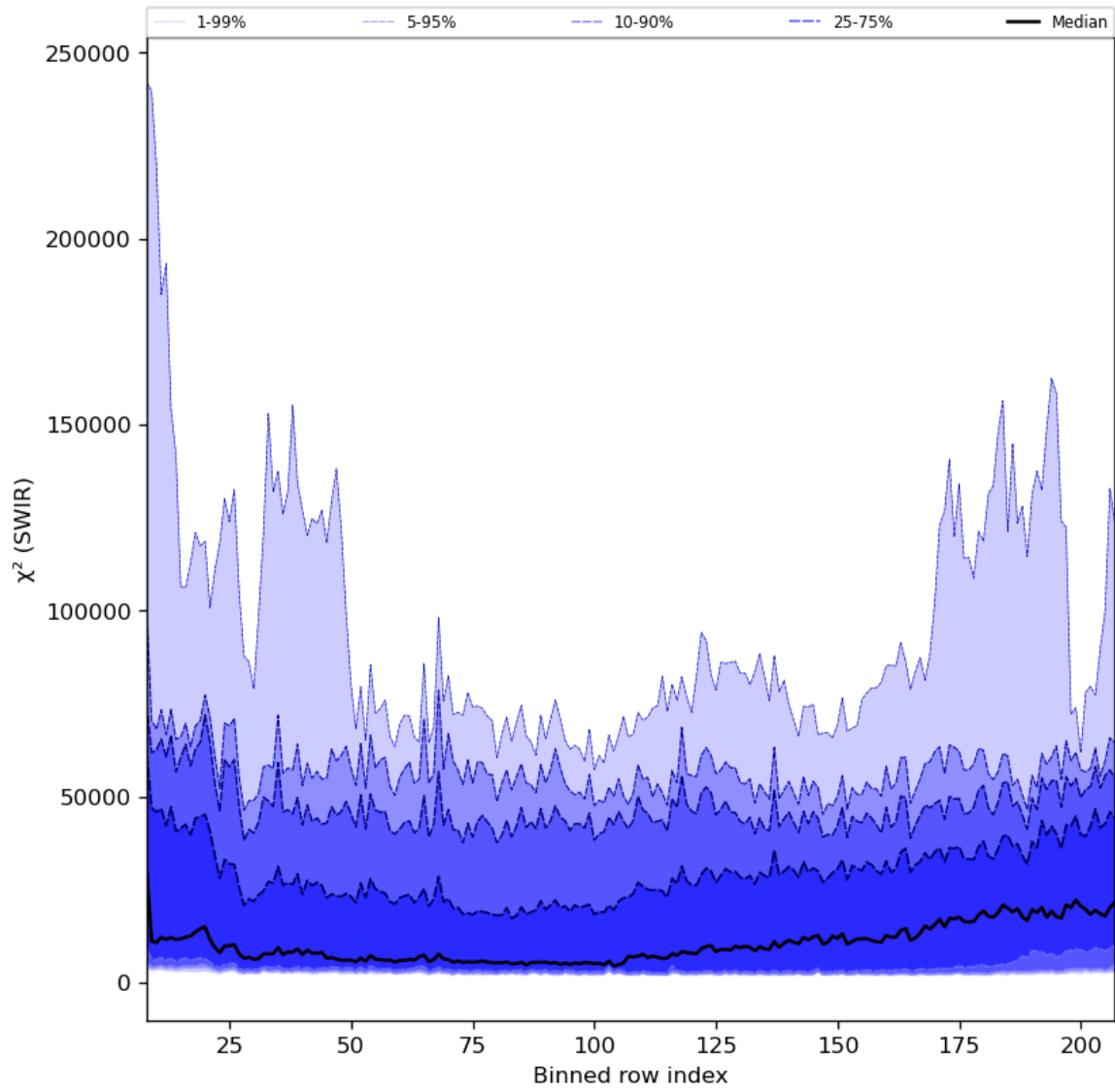
Figure 39: Along track statistics of “ \chi^2 (SWIR)” for 2024-02-27 to 2024-02-29
