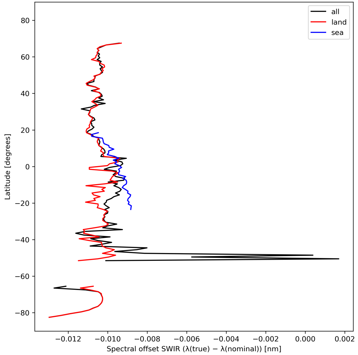
Figure 16: Zonal average of “Spectral offset SWIR ( \lambda(\text{true}) - \lambda(\text{nominal}) )” for 2024-02-27 to 2024-02-29.
