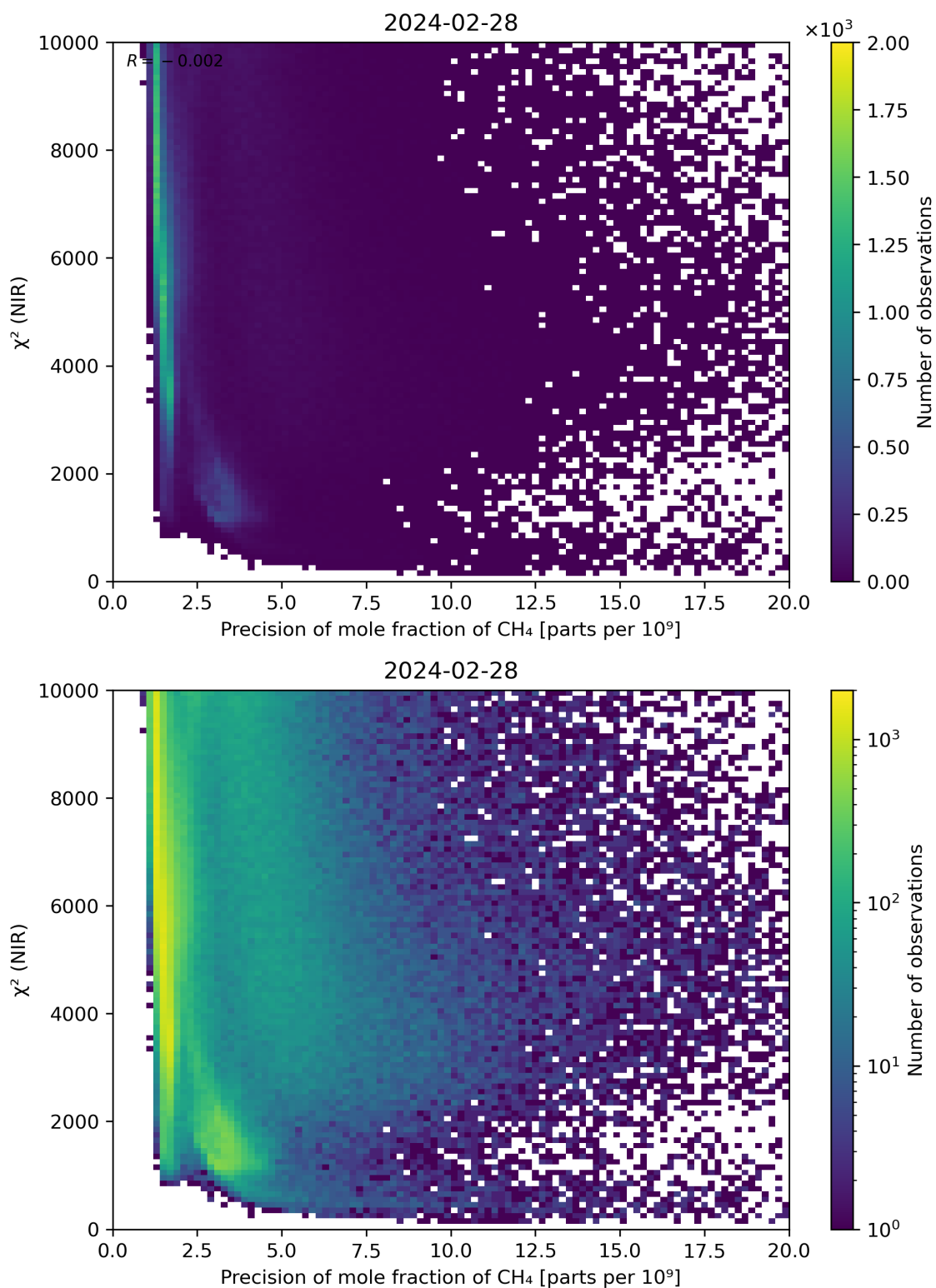
Figure 78: Scatter density plot of “Precision of mole fraction of CH 4 ” against “ \chi^2 (NIR)” for 2024-02-27 to 2024-02-29.
