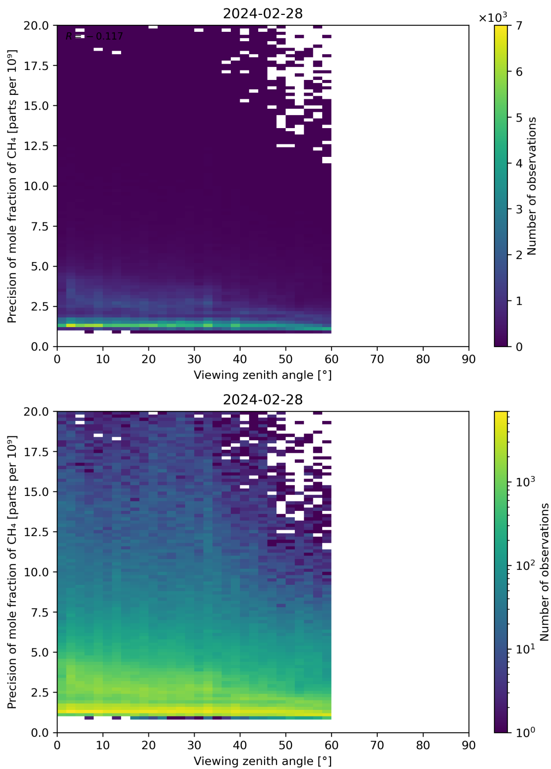
Figure 112: Scatter density plot of “Viewing zenith angle” against “Precision of mole fraction of CH 4 ” for 2024-02-27 to 2024-02-29.
