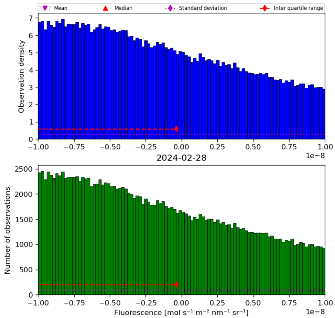
Figure 32: Histogram of “Fluorescence” for 2024-02-27 to 2024-02-29
