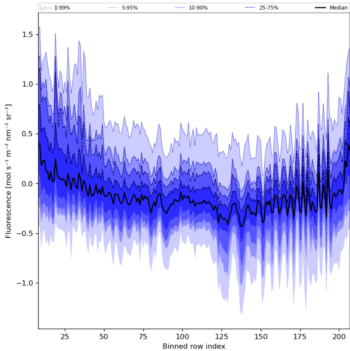
Figure 43: Along track statistics of “Fluorescence” for 2024-02-27 to 2024-02-29
