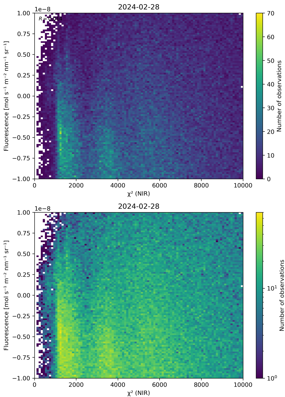
Figure 45: Scatter density plot of “ \chi^2 (NIR)” against “Fluorescence” for 2024-02-27 to 2024-02-29.
