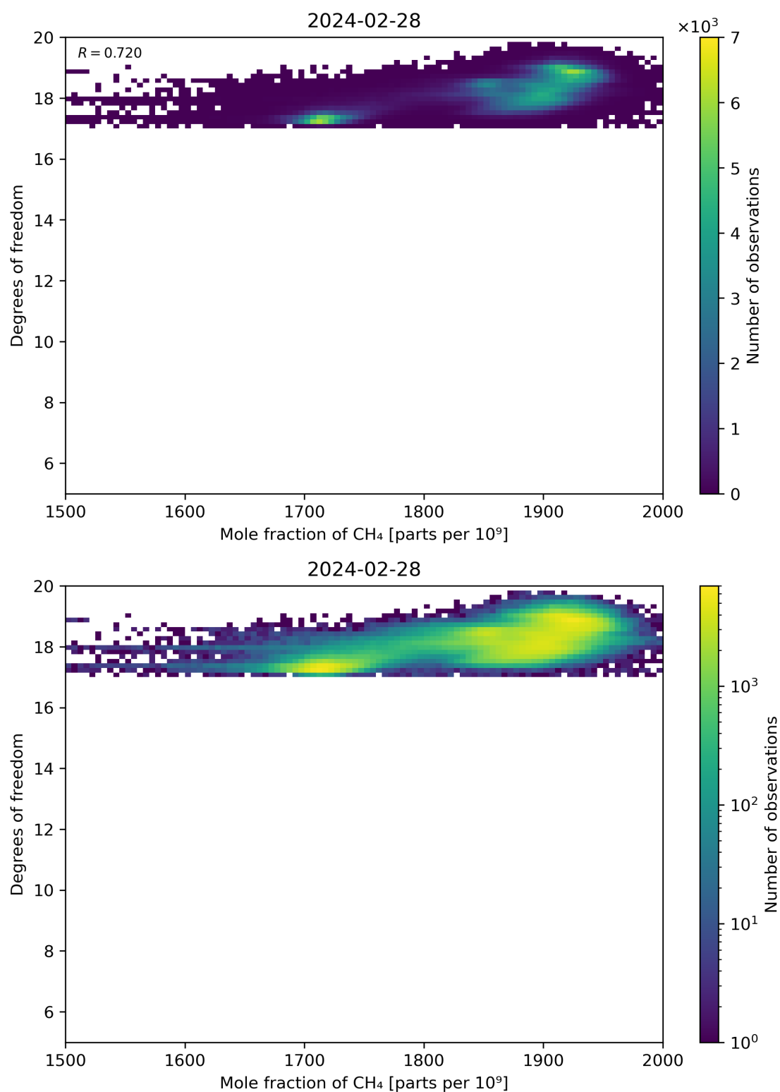
Figure 72: Scatter density plot of “Mole fraction of CH 4 ” against “Degrees of freedom” for 2024-02-27 to 2024-02-29.
