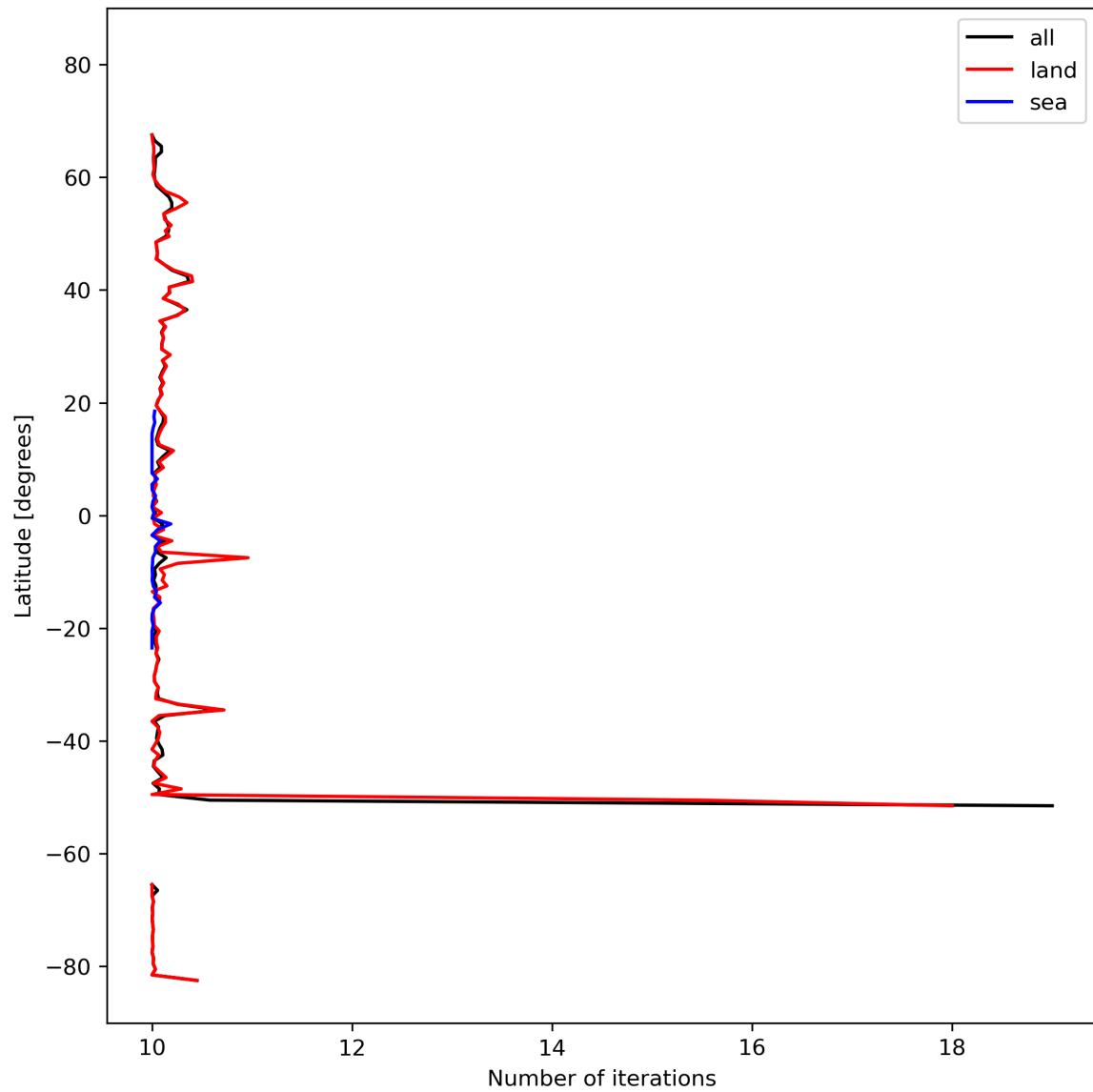
Figure 20: Zonal average of “Number of iterations” for 2024-02-27 to 2024-02-29.
