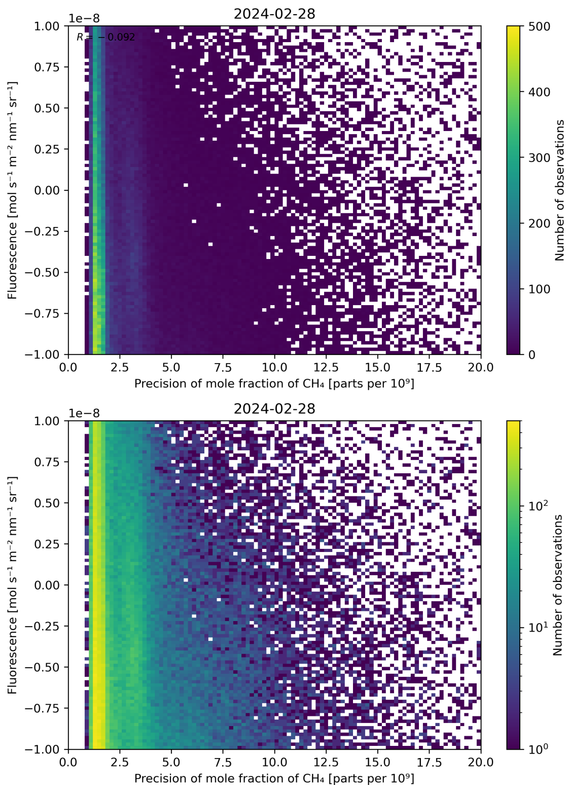
Figure 81: Scatter density plot of “Precision of mole fraction of \text{CH}_4 ” against “Fluorescence” for 2024-02-27 to 2024-02-29.
