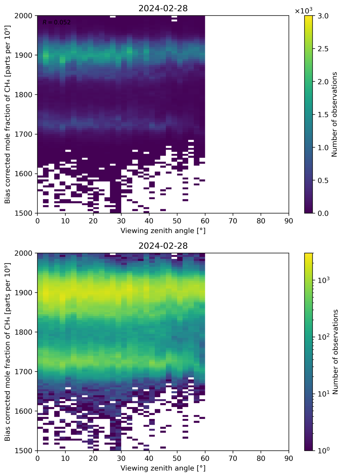
Figure 111: Scatter density plot of “Viewing zenith angle” against “Bias corrected mole fraction of CH 4 ” for 2024-02-27 to 2024-02-29.
