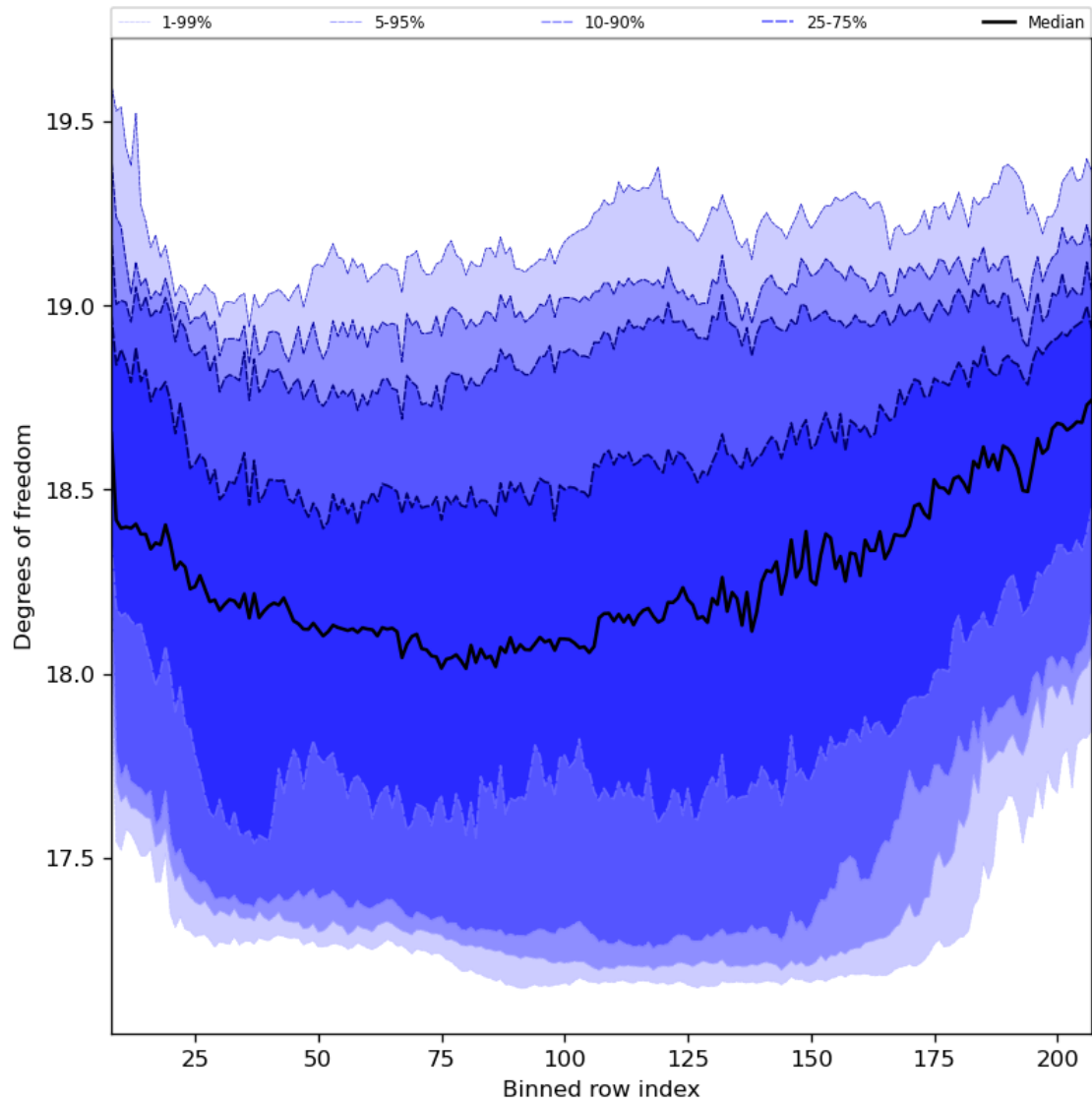
Figure 41: Along track statistics of “Degrees of freedom” for 2024-02-27 to 2024-02-29
