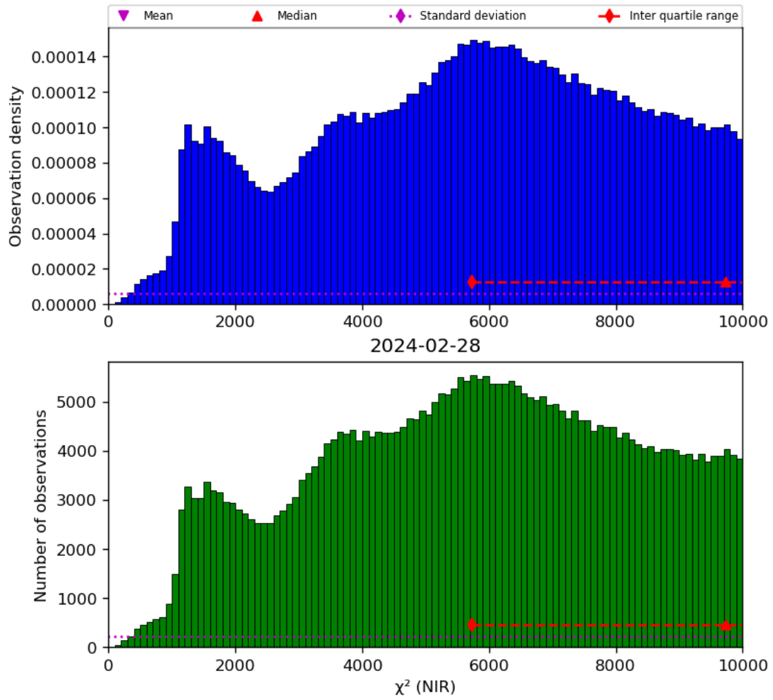
Figure 29: Histogram of “ \chi^2 (NIR)” for 2024-02-27 to 2024-02-29
