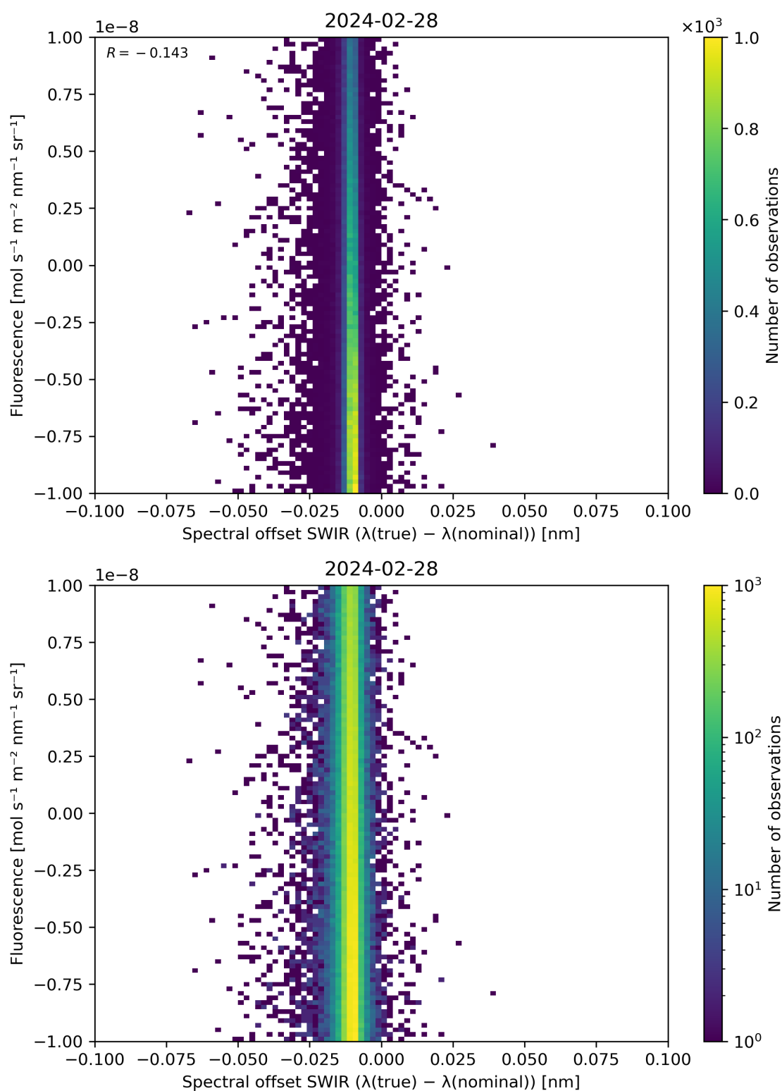
Figure 120: Scatter density plot of “Spectral offset SWIR ( \lambda(\text{true}) - \lambda(\text{nominal}) )” against “Fluorescence” for 2024-02-27 to 2024-02-29.
