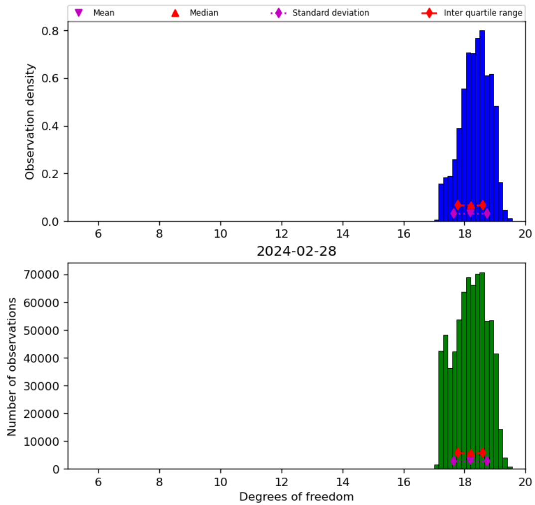
Figure 30: Histogram of “Degrees of freedom” for 2024-02-27 to 2024-02-29
