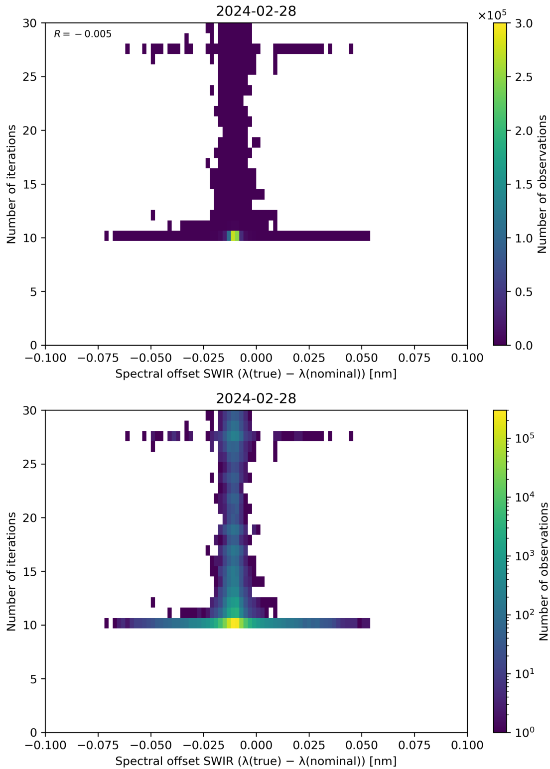
Figure 121: Scatter density plot of “Spectral offset SWIR ( \lambda(\text{true}) - \lambda(\text{nominal}) )” against “Number of iterations” for 2024-02-27 to 2024-02-29.
