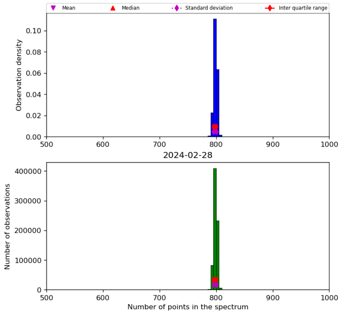
Figure 26: Histogram of “Number of points in the spectrum” for 2024-02-27 to 2024-02-29
