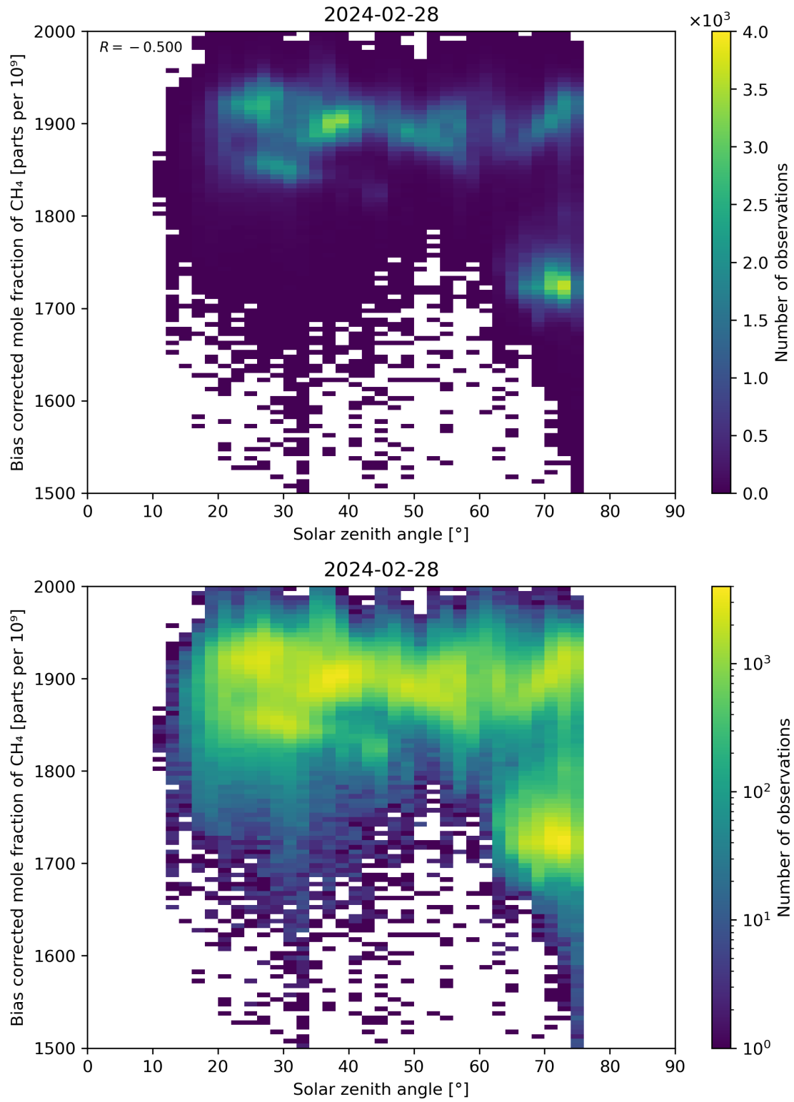
Figure 100: Scatter density plot of “Solar zenith angle” against “Bias corrected mole fraction of \text{CH}_4 ” for 2024-02-27 to 2024-02-29.
