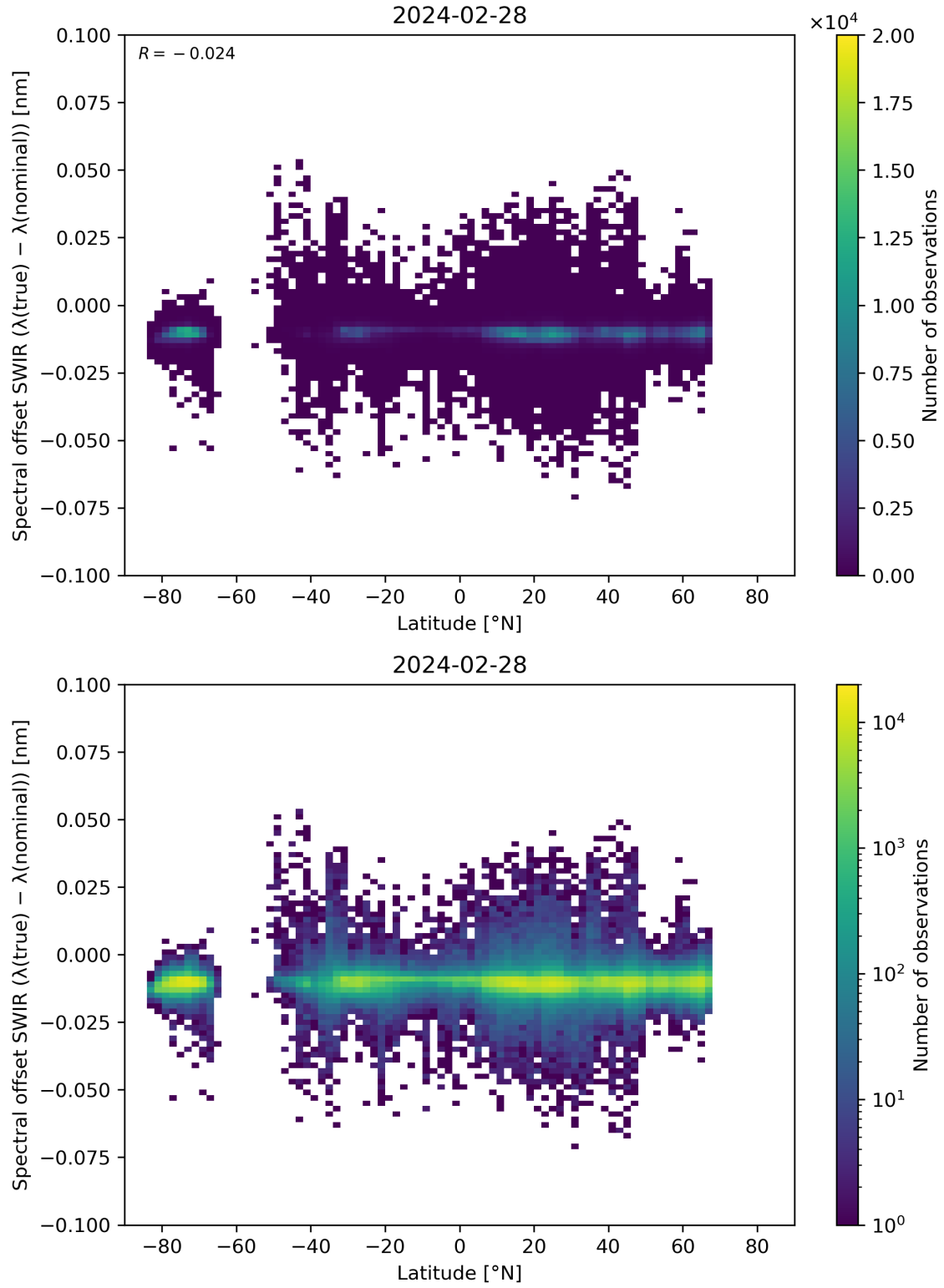
Figure 62: Scatter density plot of “Latitude” against “Spectral offset SWIR ( \lambda(\text{true}) - \lambda(\text{nominal}) )” for 2024-02-27 to 2024-02-29.
