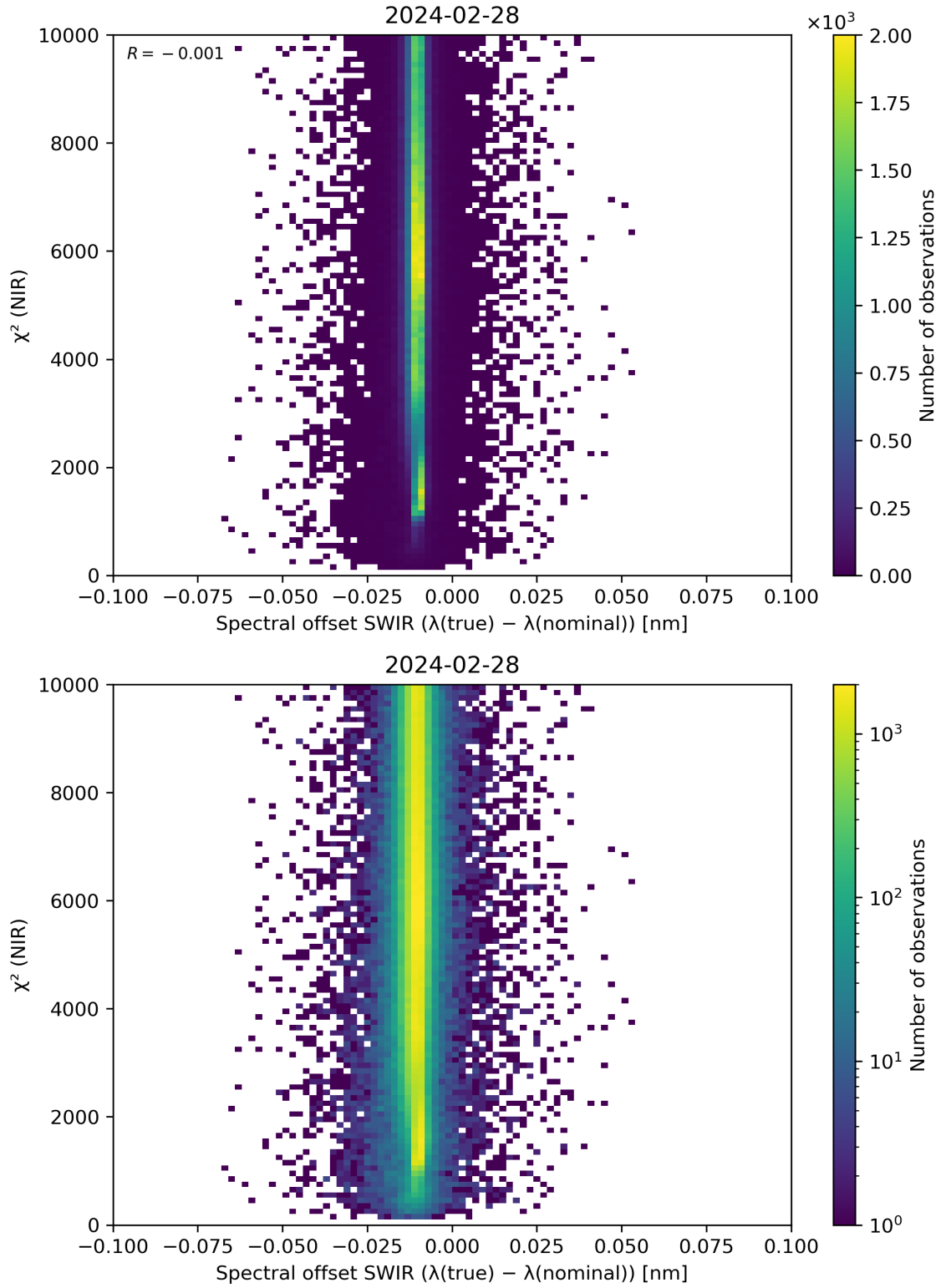
Figure 117: Scatter density plot of “Spectral offset SWIR ( \lambda(\text{true}) - \lambda(\text{nominal}) )” against “ \chi^2 (NIR)” for 2024-02-27 to 2024-02-29.
