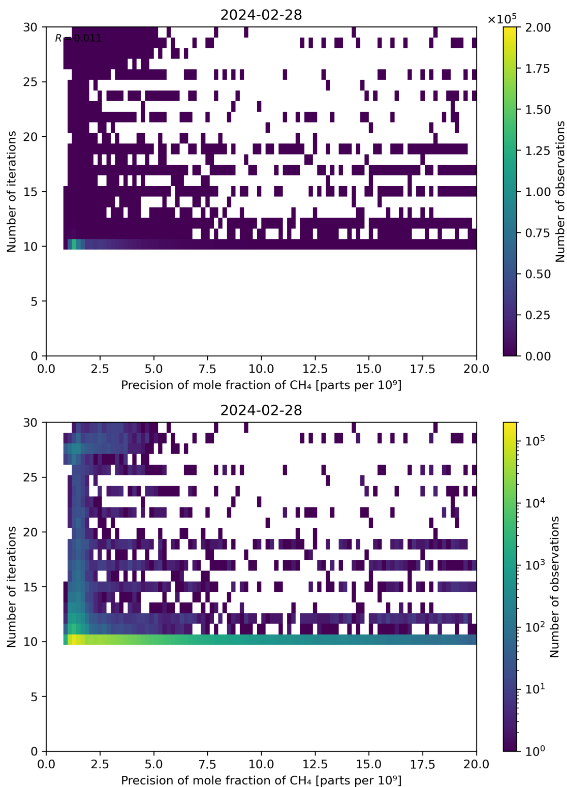
Figure 83: Scatter density plot of “Precision of mole fraction of CH 4 ” against “Number of iterations” for 2024-02-27 to 2024-02-29.
