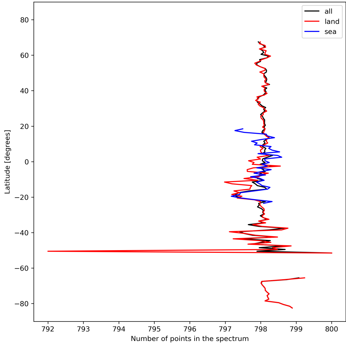
Figure 15: Zonal average of “Number of points in the spectrum” for 2024-02-27 to 2024-02-29.
