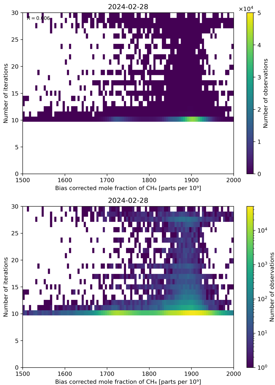
Figure 67: Scatter density plot of “Bias corrected mole fraction of \text{CH}_4 ” against “Number of iterations” for 2024-02-27 to 2024-02-29.
