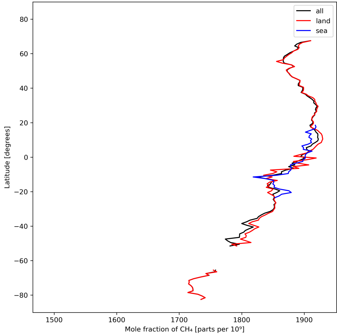
Figure 12: Zonal average of “Mole fraction of \text{CH}_4 ” for 2024-02-27 to 2024-02-29.
