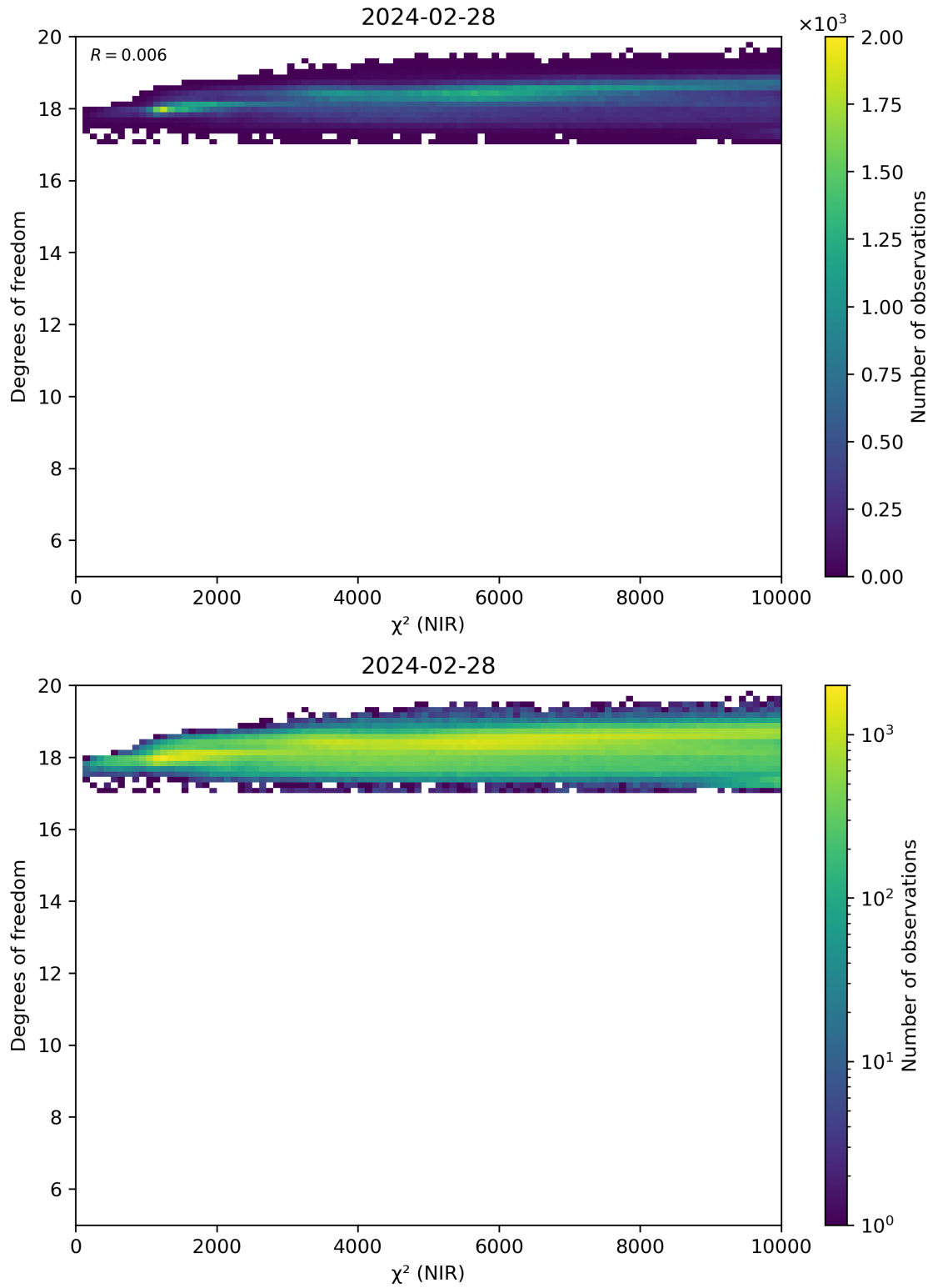
Figure 44: Scatter density plot of “ \chi^2 (NIR)” against “Degrees of freedom” for 2024-02-27 to 2024-02-29.
