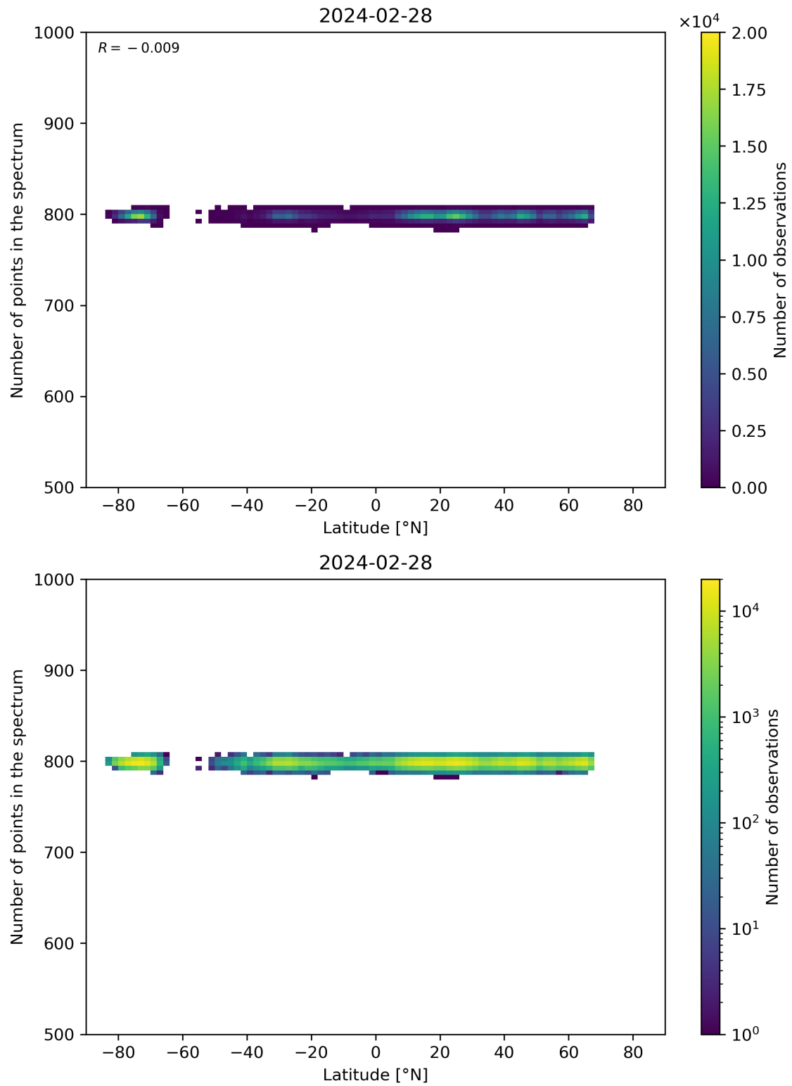
Figure 61: Scatter density plot of “Latitude” against “Number of points in the spectrum” for 2024-02-27 to 2024-02-29.
