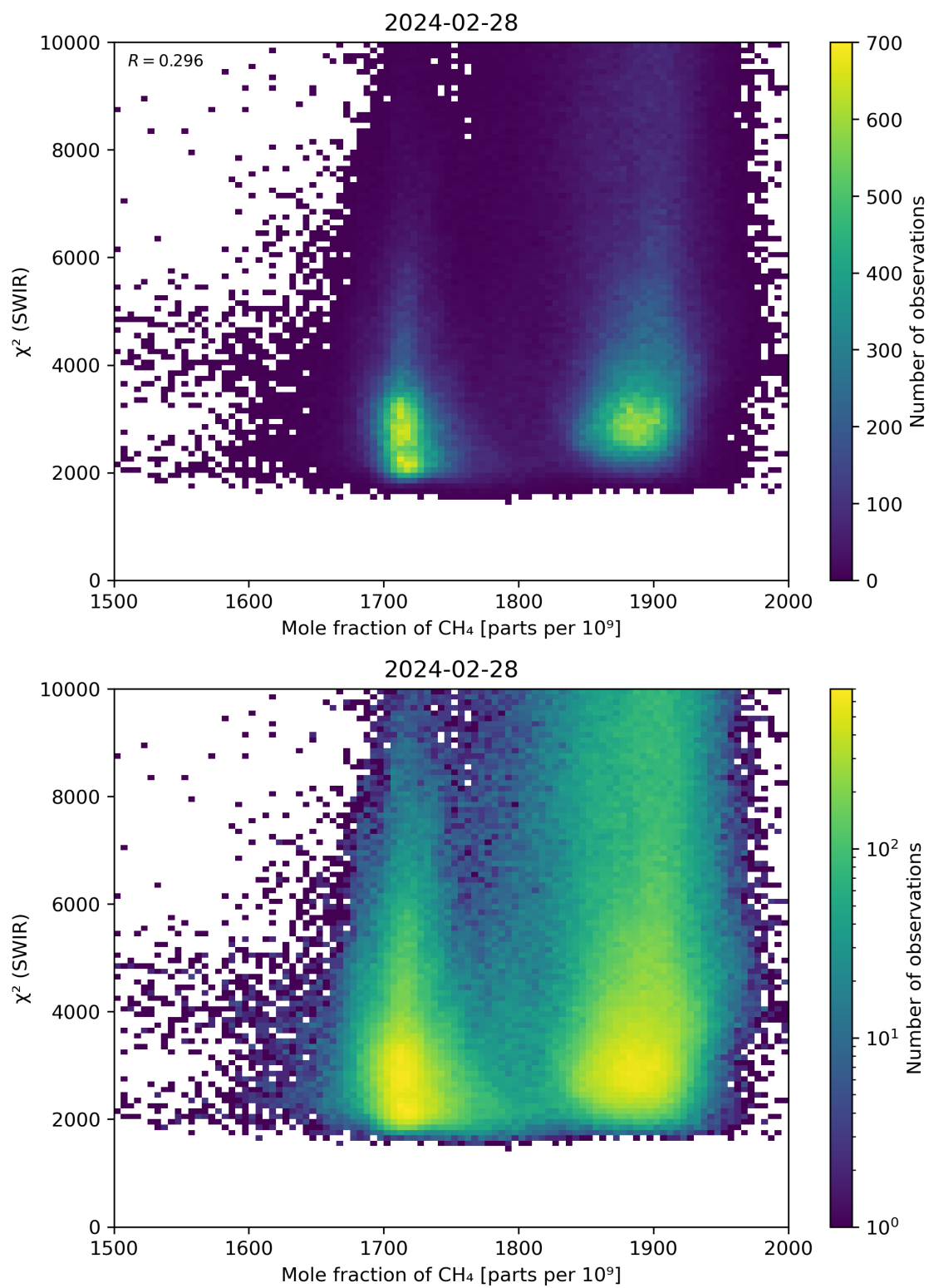
Figure 71: Scatter density plot of “Mole fraction of \text{CH}_4 ” against “ \chi^2 (SWIR)” for 2024-02-27 to 2024-02-29.
