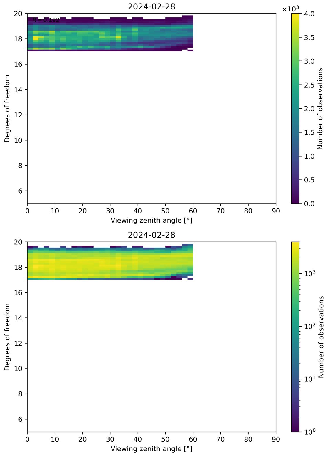
Figure 107: Scatter density plot of “Viewing zenith angle” against “Degrees of freedom” for 2024-02-27 to 2024-02-29.
