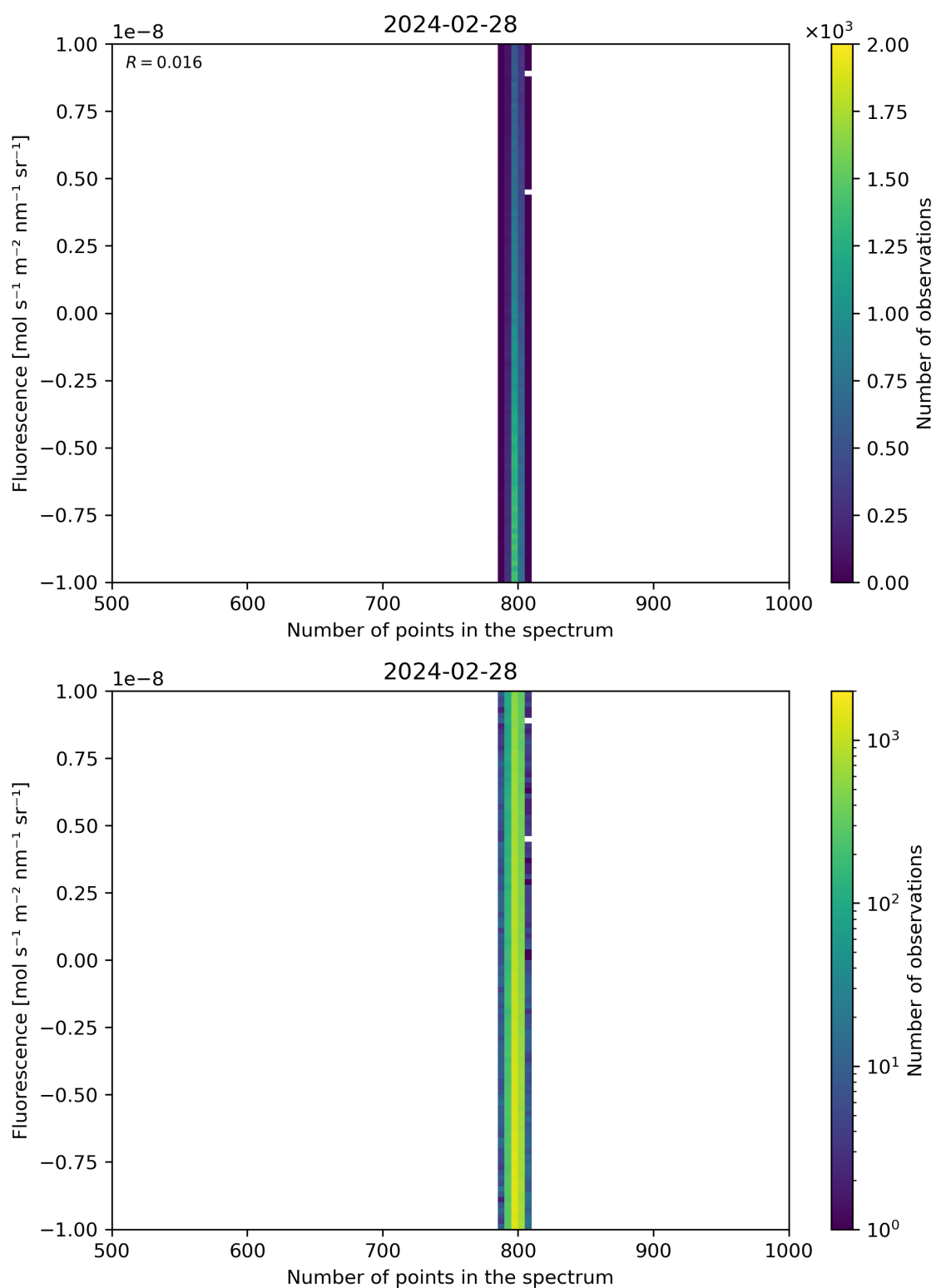
Figure 91: Scatter density plot of “Number of points in the spectrum” against “Fluorescence” for 2024-02-27 to 2024-02-29.
