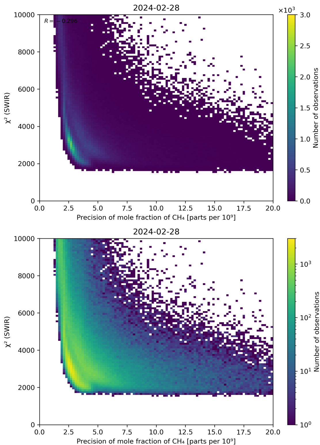
Figure 79: Scatter density plot of “Precision of mole fraction of \text{CH}_4 ” against “ \chi^2 (SWIR)” for 2024-02-27 to 2024-02-29.
