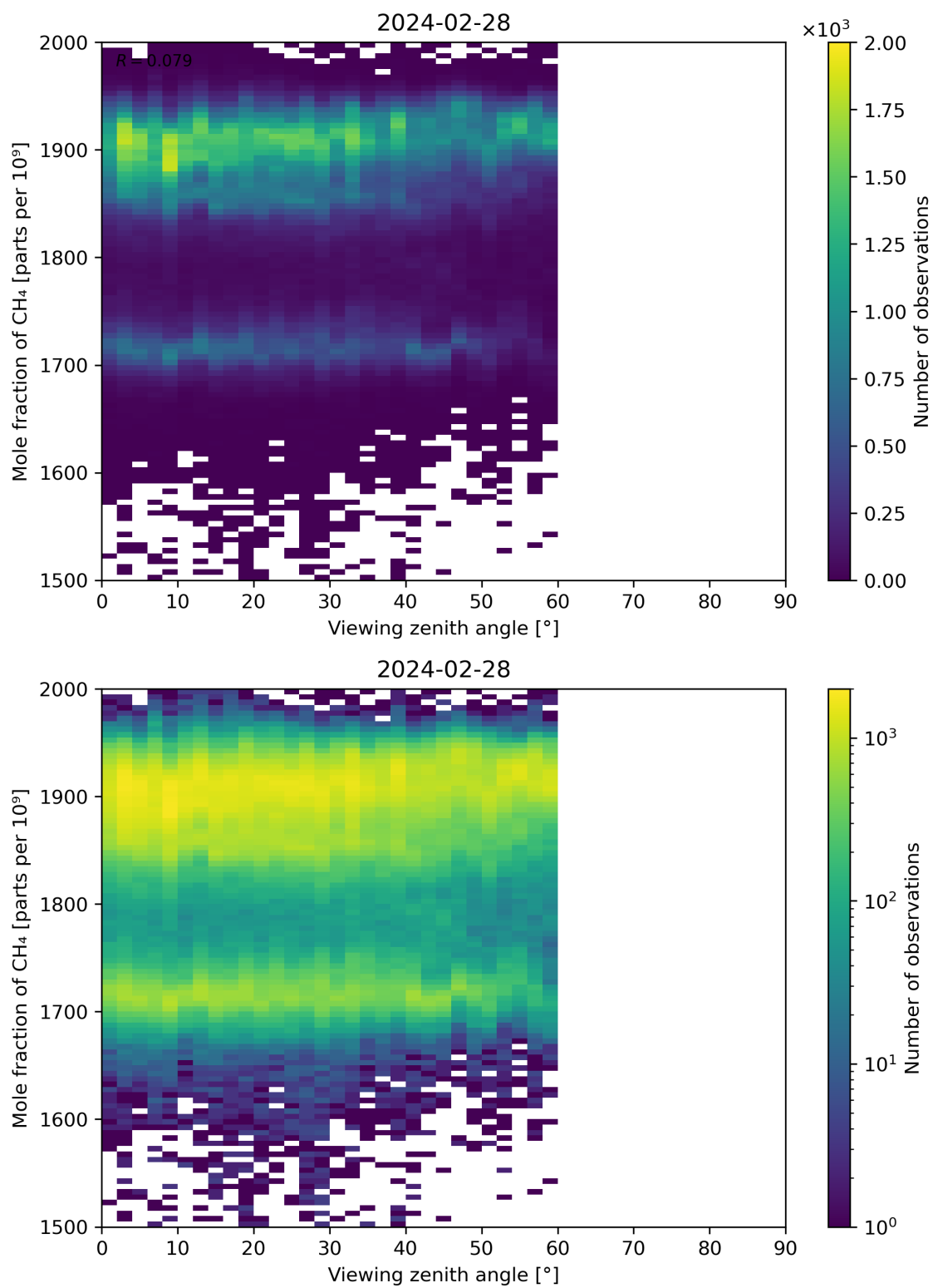
Figure 110: Scatter density plot of “Viewing zenith angle” against “Mole fraction of CH 4 ” for 2024-02-27 to 2024-02-29.
