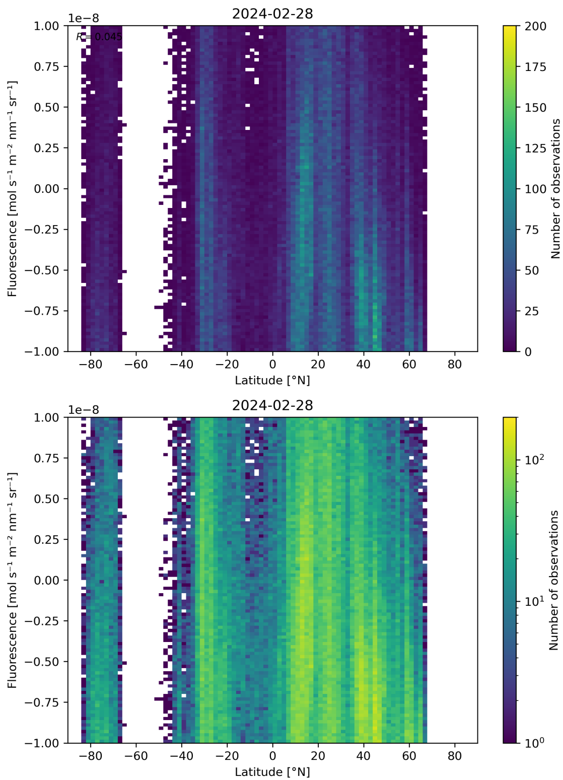
Figure 56: Scatter density plot of “Latitude” against “Fluorescence” for 2024-02-27 to 2024-02-29.
