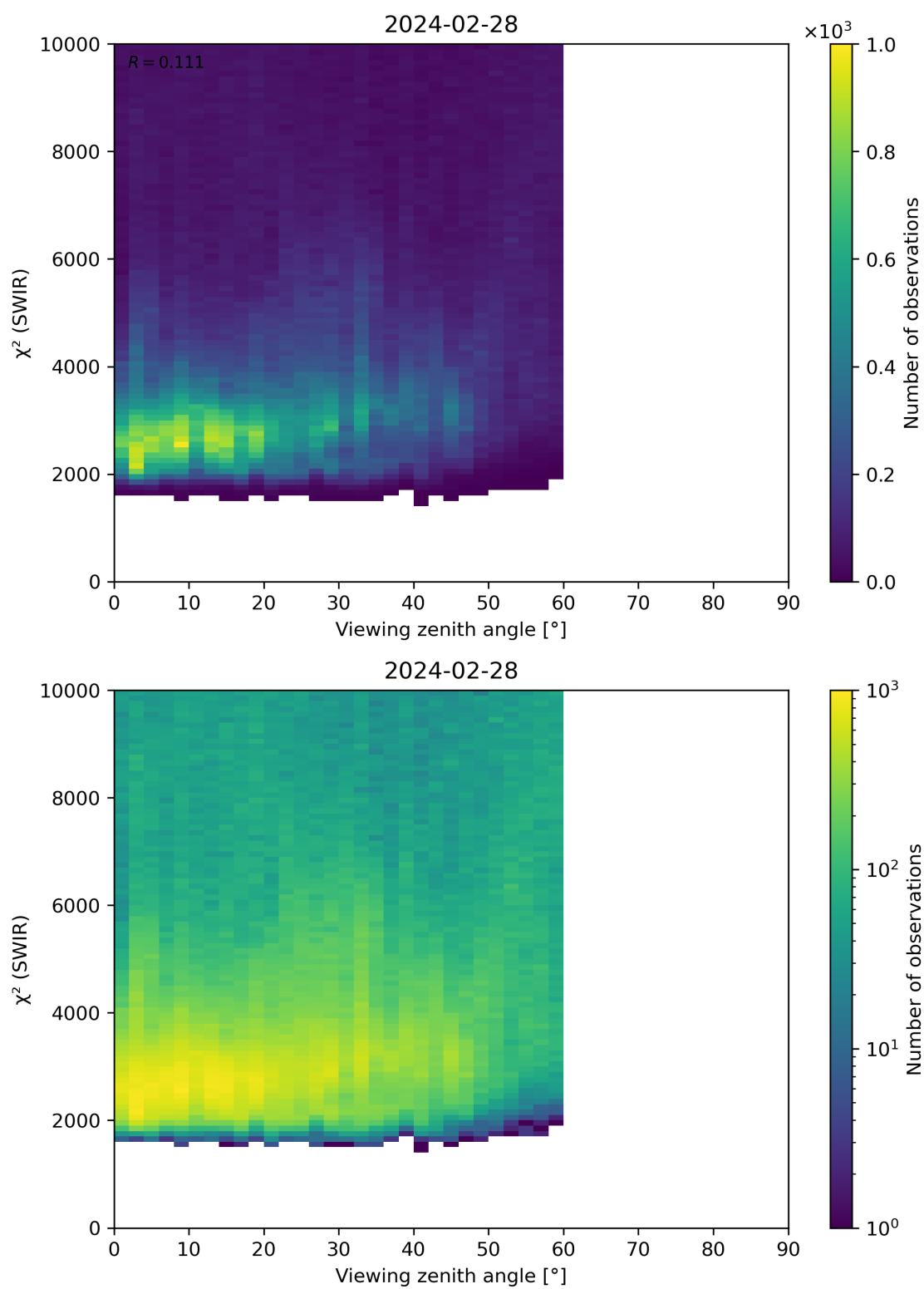
Figure 106: Scatter density plot of “Viewing zenith angle” against “ \chi^2 (SWIR)” for 2024-02-27 to 2024-02-29.
