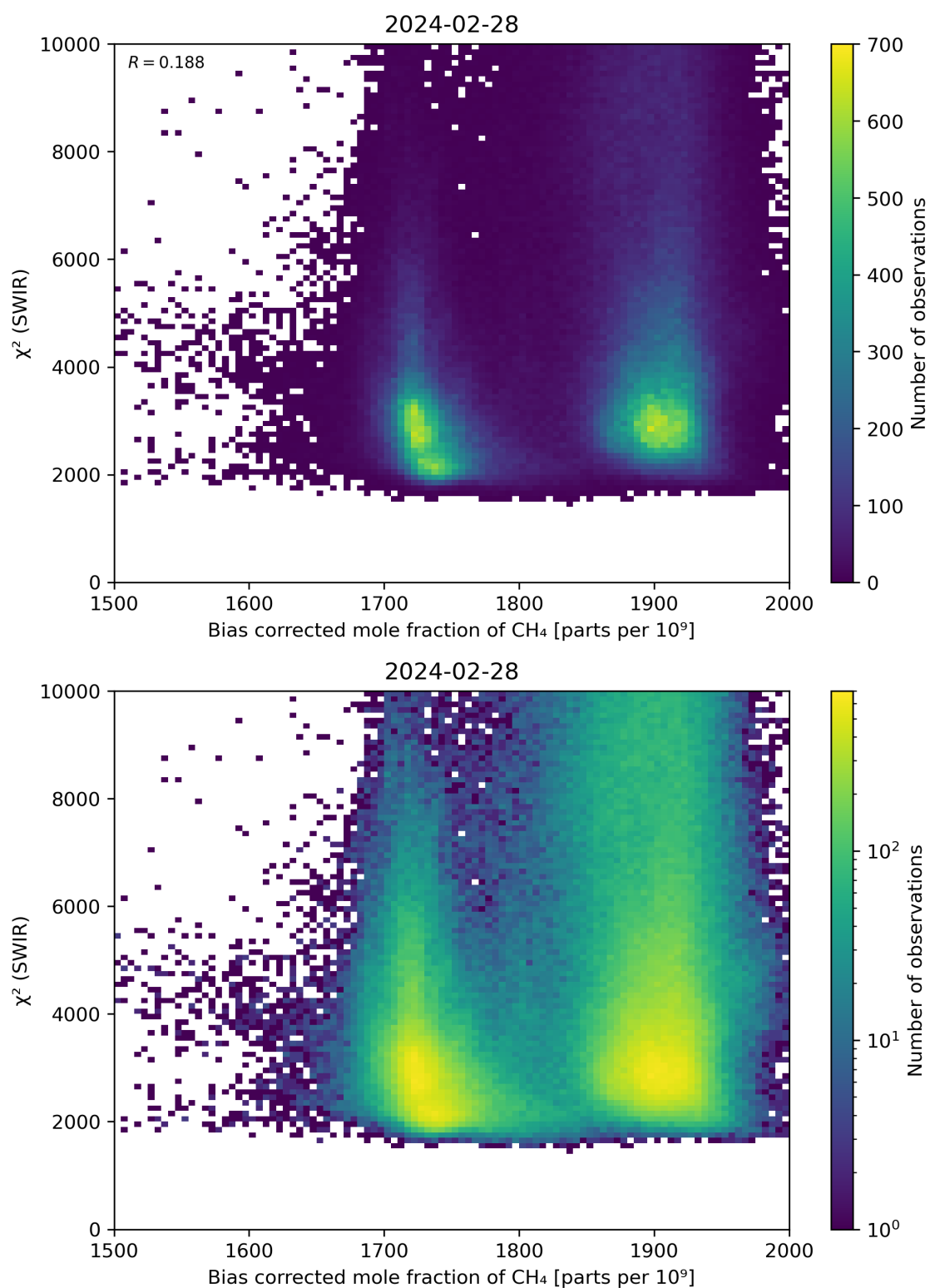
Figure 64: Scatter density plot of “Bias corrected mole fraction of CH 4 ” against “ \chi^2 (SWIR)” for 2024-02-27 to 2024-02-29.
