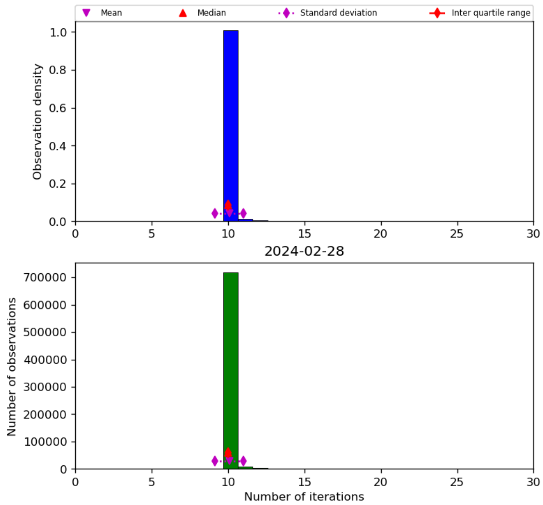
Figure 31: Histogram of “Number of iterations” for 2024-02-27 to 2024-02-29
