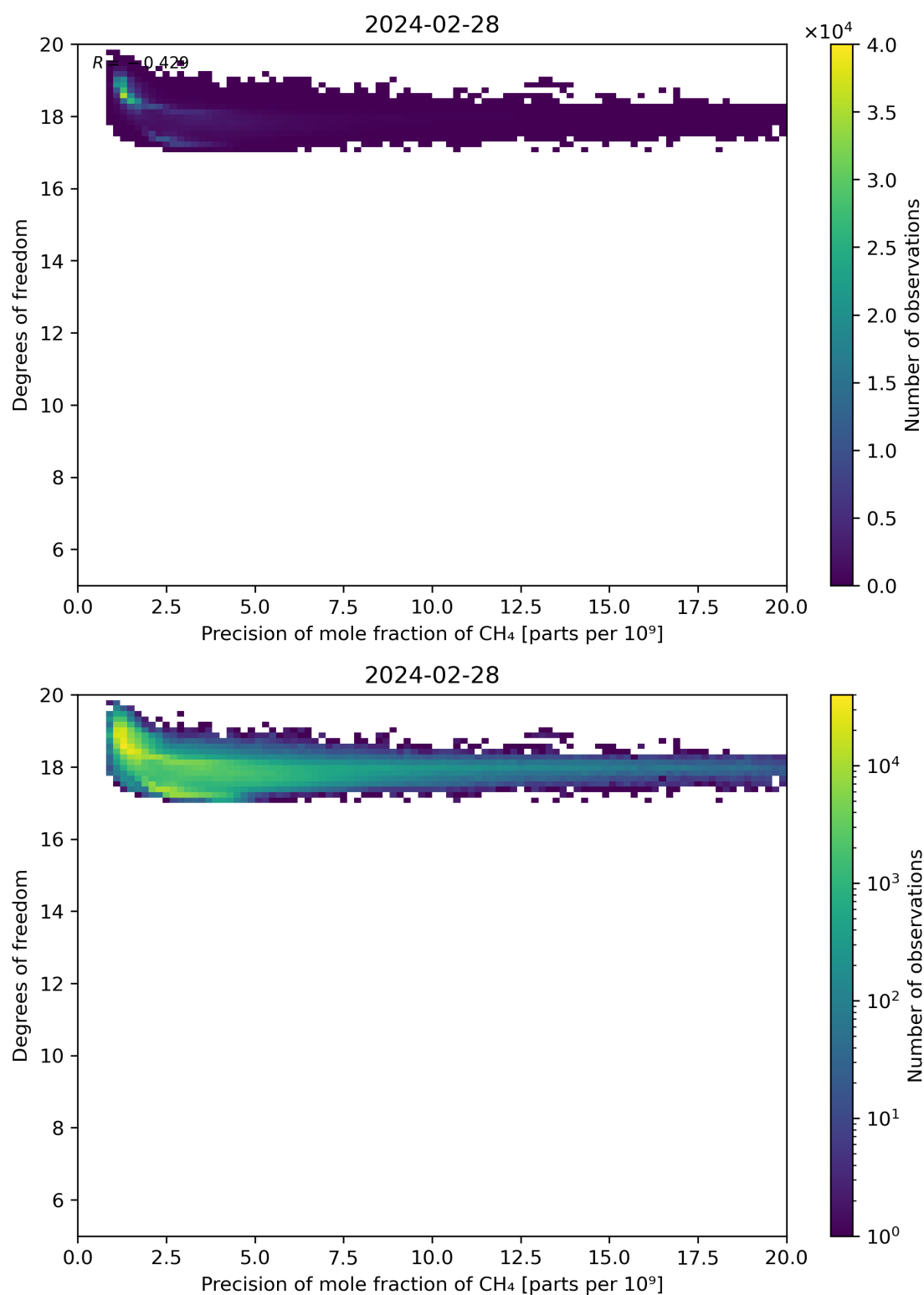
Figure 80: Scatter density plot of “Precision of mole fraction of CH 4 ” against “Degrees of freedom” for 2024-02-27 to 2024-02-29.
