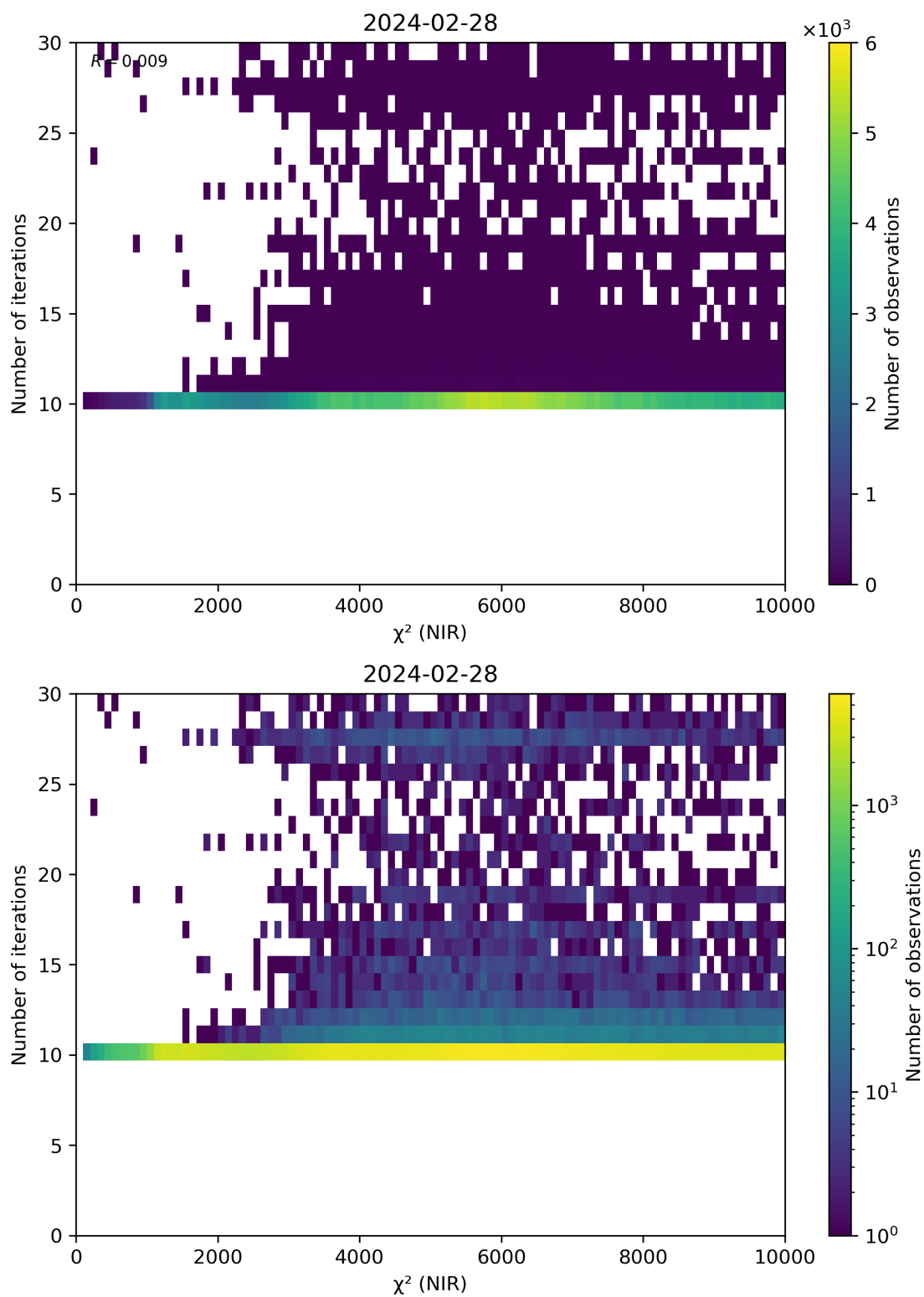
Figure 46: Scatter density plot of “ \chi^2 (NIR)” against “Number of iterations” for 2024-02-27 to 2024-02-29.
