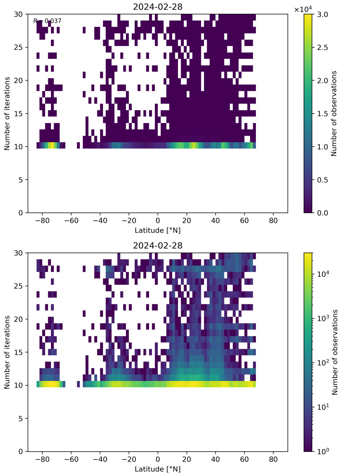
Figure 60: Scatter density plot of “Latitude” against “Number of iterations” for 2024-02-27 to 2024-02-29.
