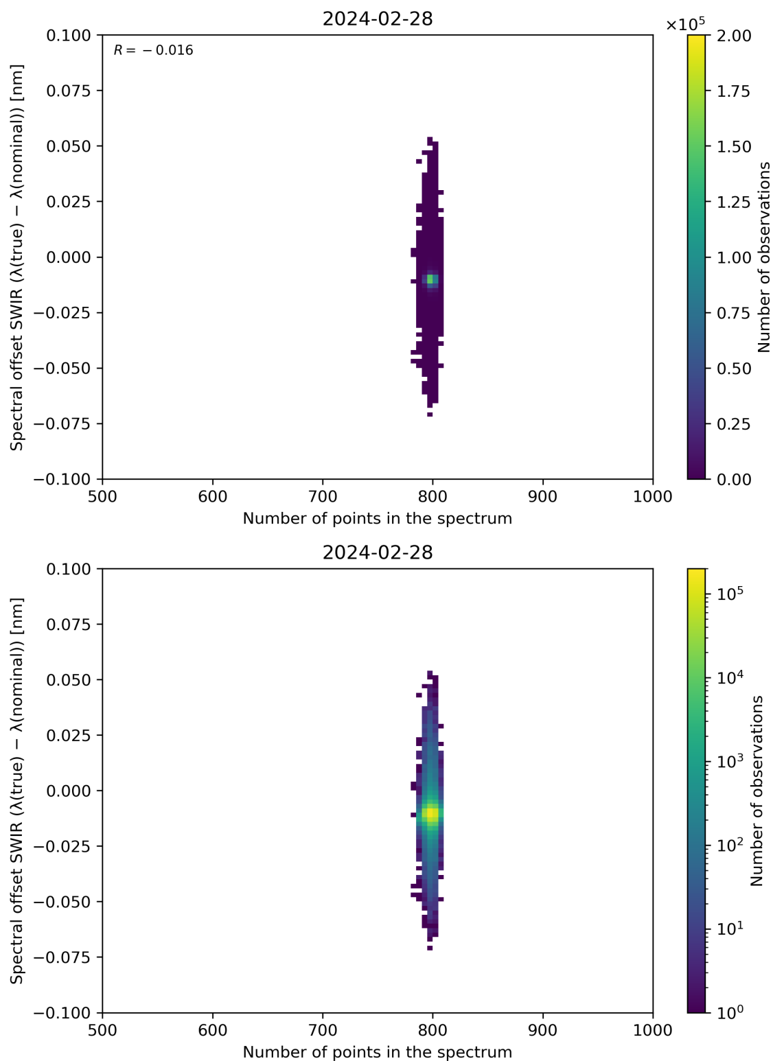
Figure 93: Scatter density plot of “Number of points in the spectrum” against “Spectral offset SWIR ( \lambda(\text{true}) - \lambda(\text{nominal}) )” for 2024-02-27 to 2024-02-29.
