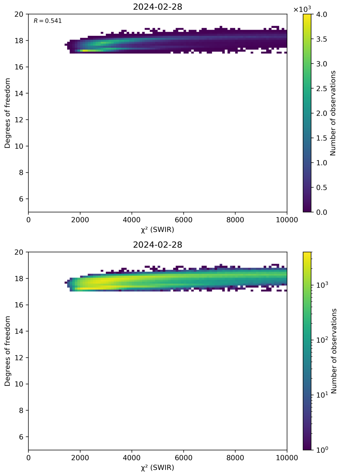
Figure 48: Scatter density plot of “ \chi^2 (SWIR)” against “Degrees of freedom” for 2024-02-27 to 2024-02-29.
