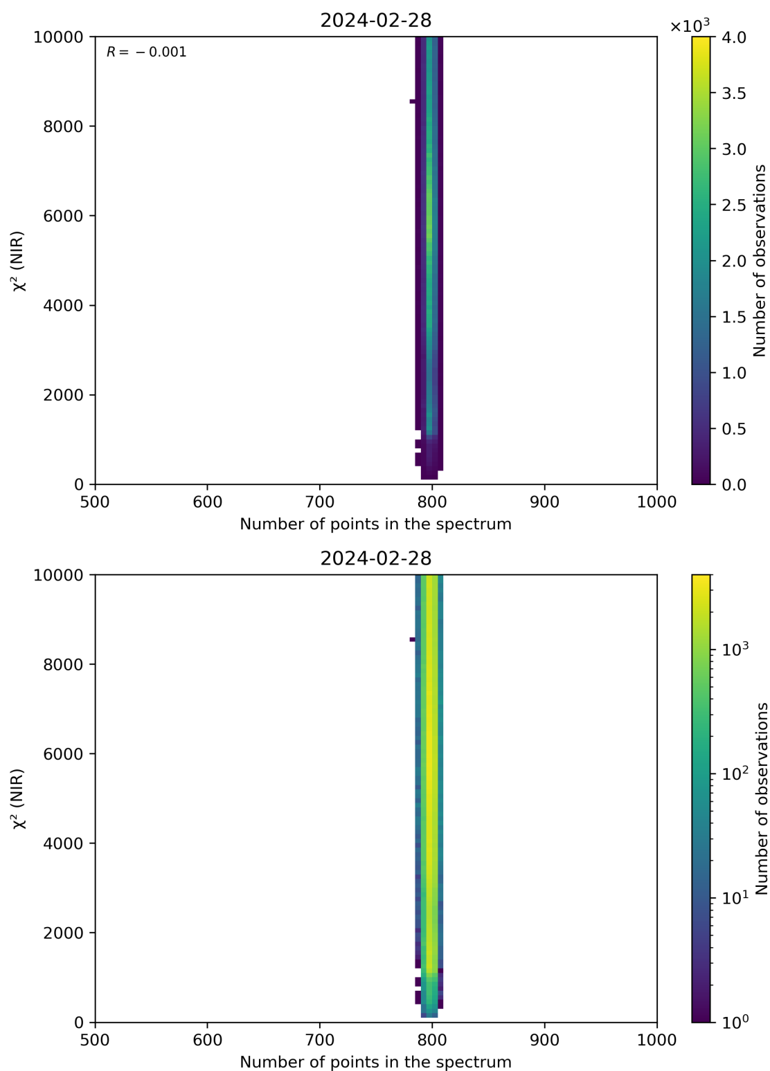
Figure 88: Scatter density plot of “Number of points in the spectrum” against “ \chi^2 (NIR)” for 2024-02-27 to 2024-02-29.
