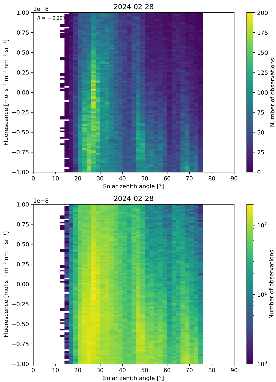
Figure 97: Scatter density plot of “Solar zenith angle” against “Fluorescence” for 2024-02-27 to 2024-02-29.
