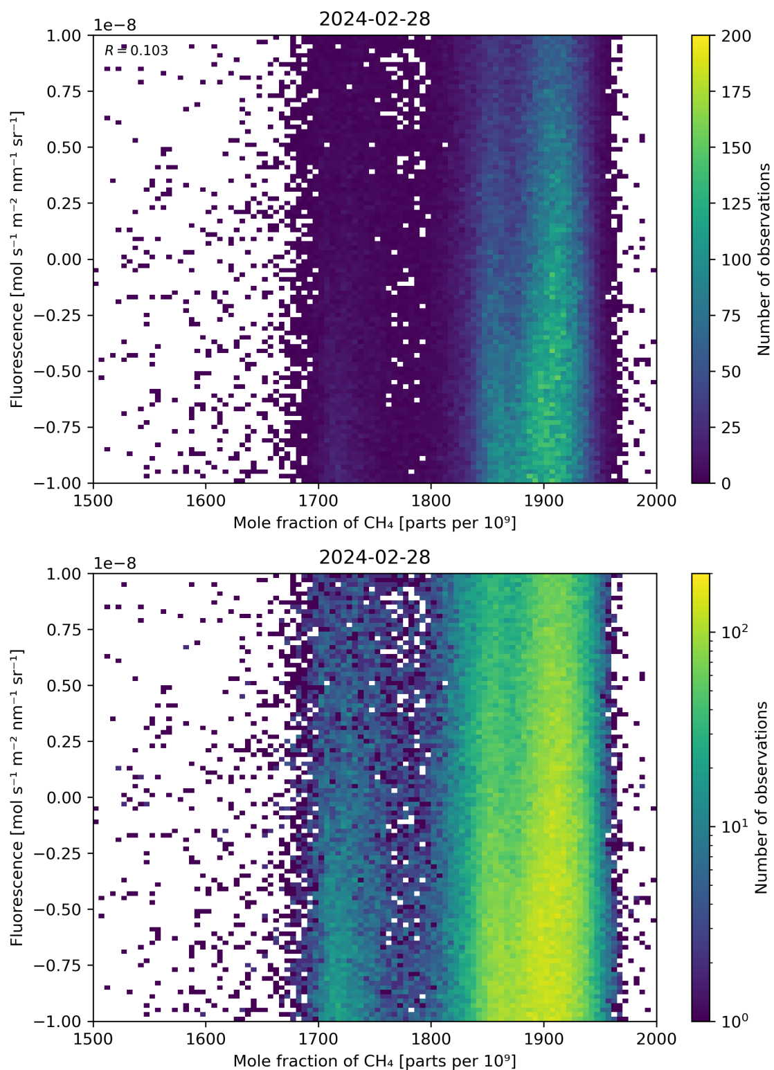
Figure 73: Scatter density plot of “Mole fraction of \text{CH}_4 ” against “Fluorescence” for 2024-02-27 to 2024-02-29.
