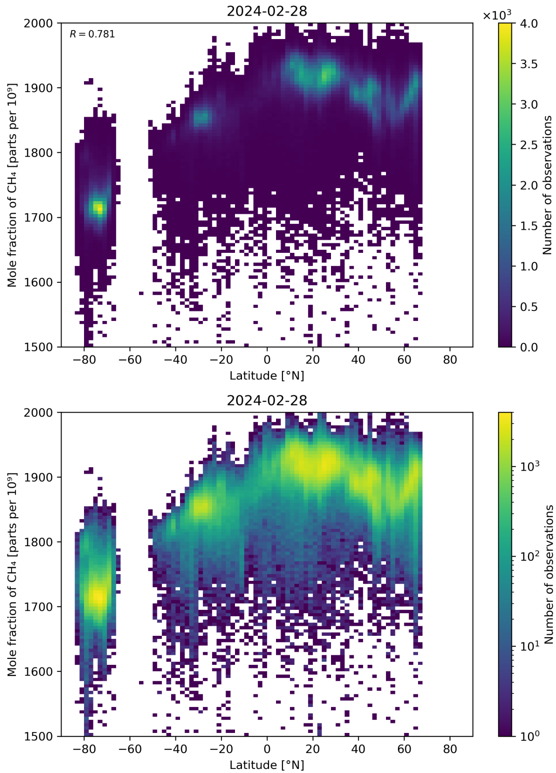
Figure 57: Scatter density plot of “Latitude” against “Mole fraction of CH 4 ” for 2024-02-27 to 2024-02-29.
