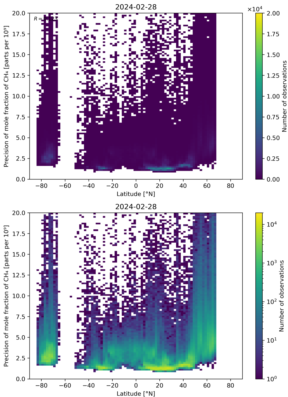
Figure 59: Scatter density plot of “Latitude” against “Precision of mole fraction of CH 4 ” for 2024-02-27 to 2024-02-29.
