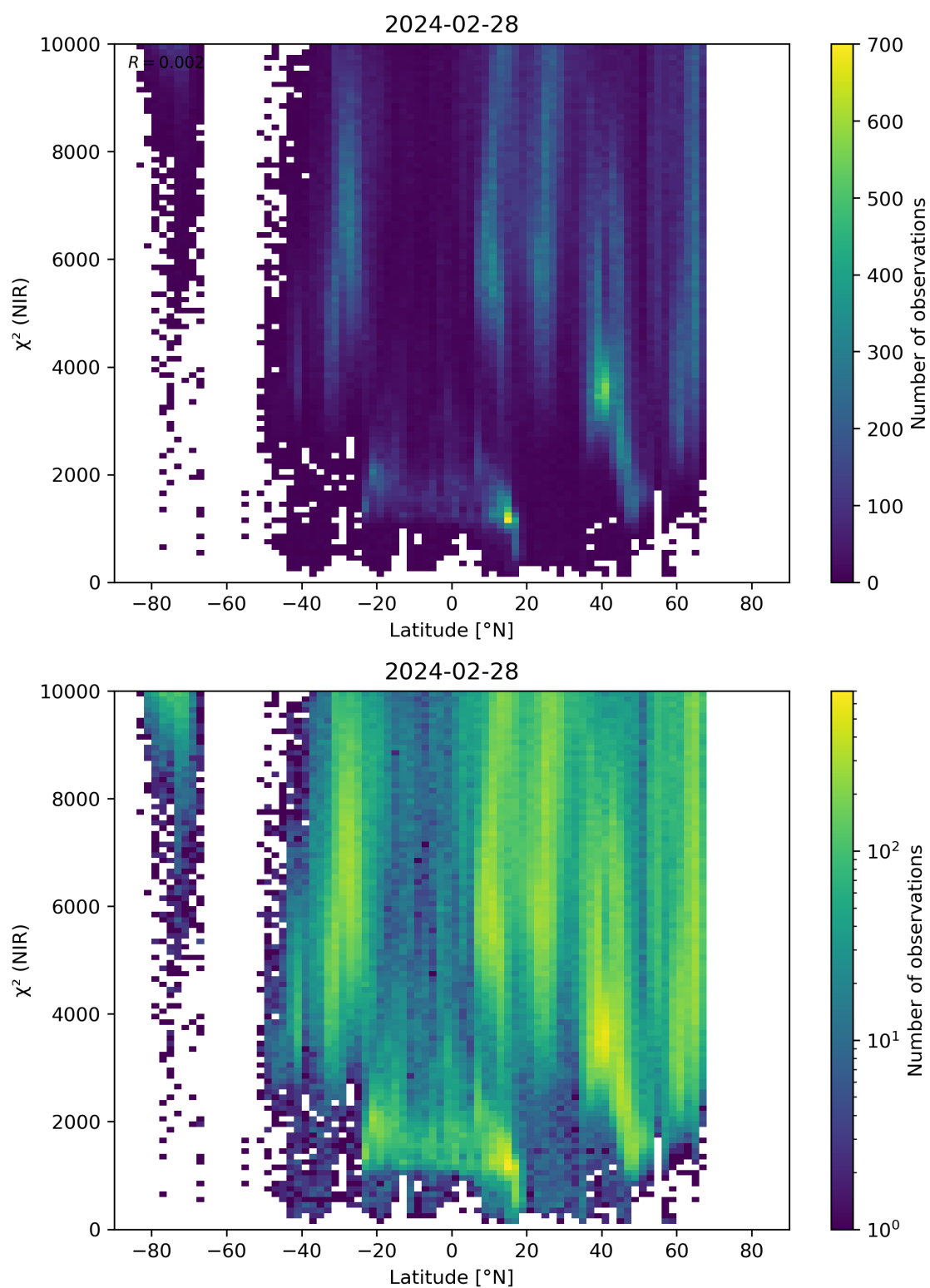
Figure 53: Scatter density plot of “Latitude” against “ \chi^2 (NIR)” for 2024-02-27 to 2024-02-29.
