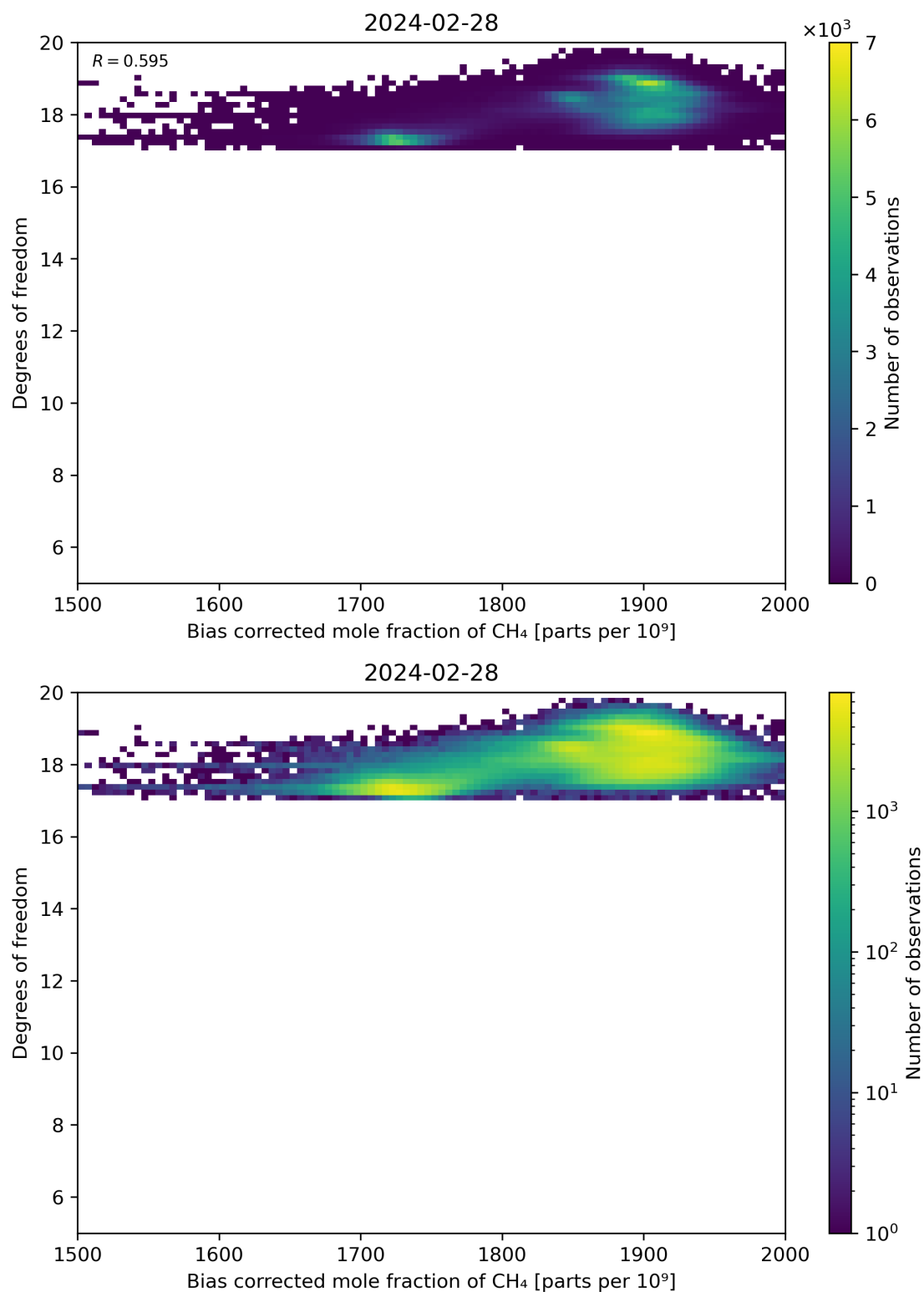
Figure 65: Scatter density plot of “Bias corrected mole fraction of CH 4 ” against “Degrees of freedom” for 2024-02-27 to 2024-02-29.
