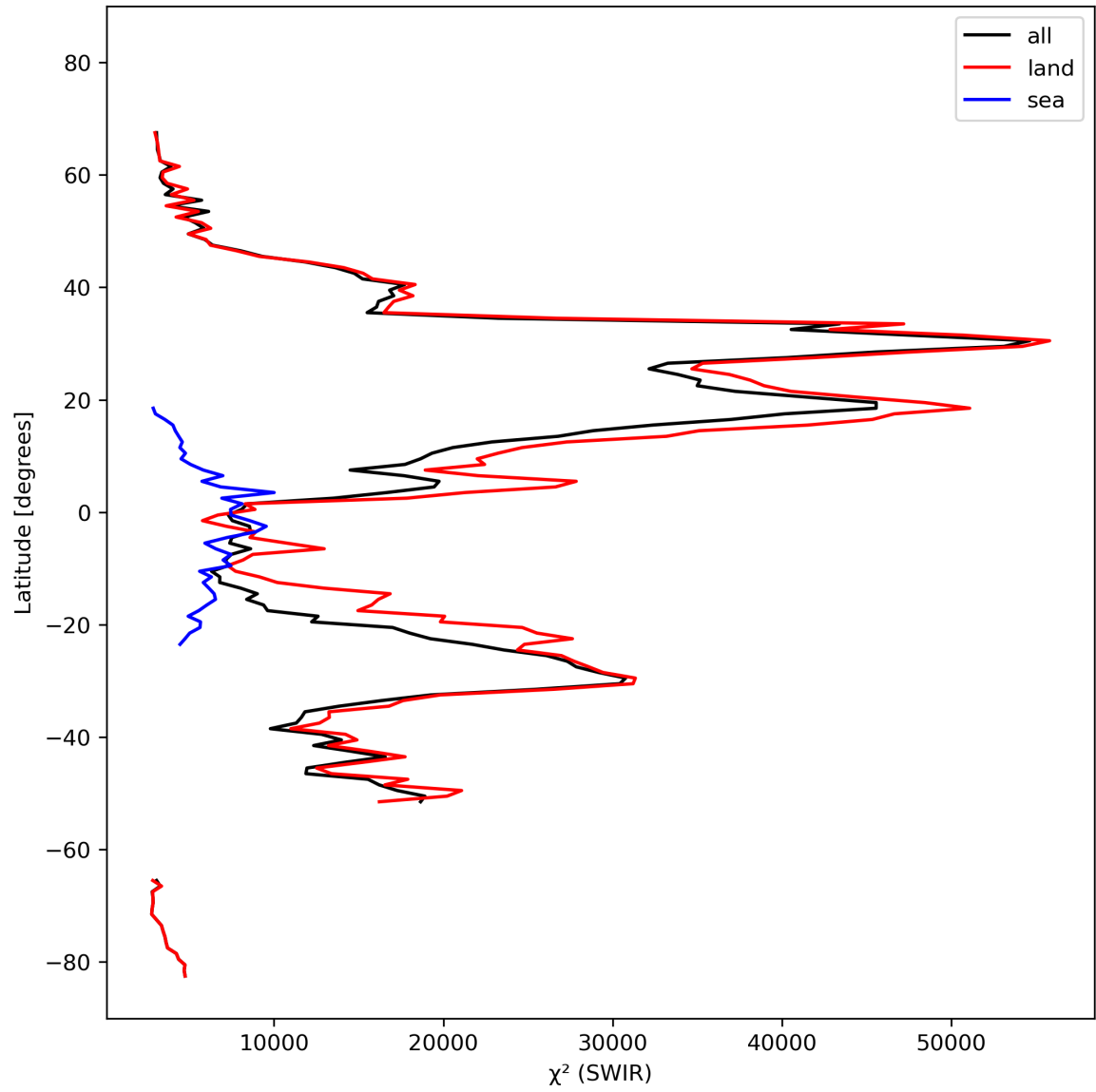
Figure 17: Zonal average of “ \chi^2 (SWIR)” for 2024-02-27 to 2024-02-29.
