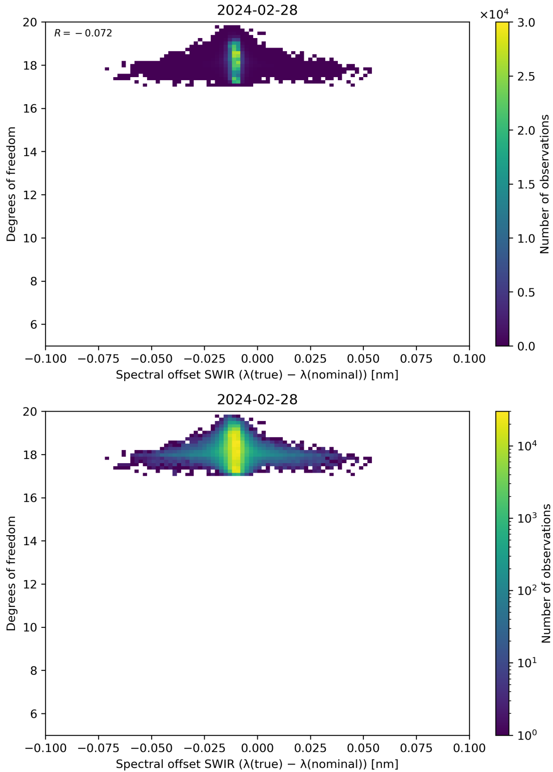
Figure 119: Scatter density plot of “Spectral offset SWIR ( \lambda(\text{true}) - \lambda(\text{nominal}) )” against “Degrees of freedom” for 2024-02-27 to 2024-02-29.
