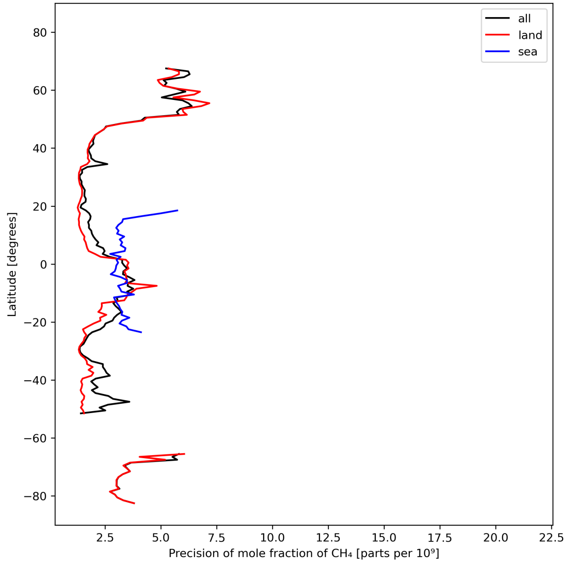
Figure 13: Zonal average of “Precision of mole fraction of CH 4 ” for 2024-02-27 to 2024-02-29.
