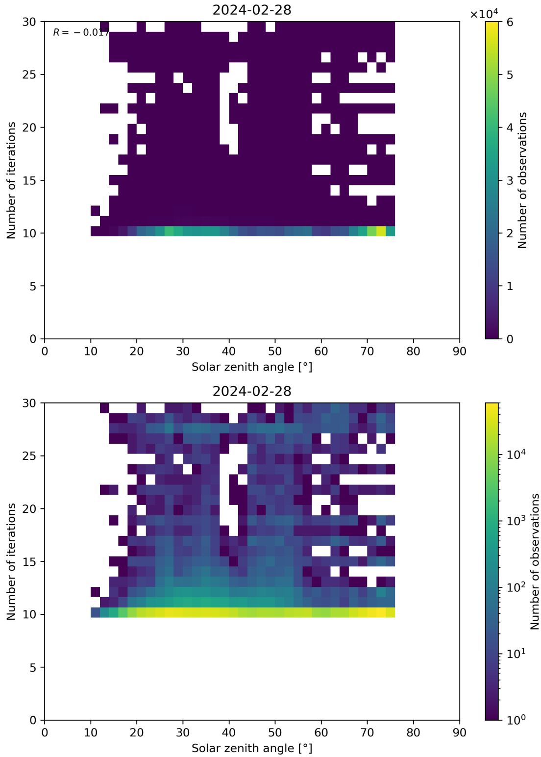
Figure 102: Scatter density plot of “Solar zenith angle” against “Number of iterations” for 2024-02-27 to 2024-02-29.
