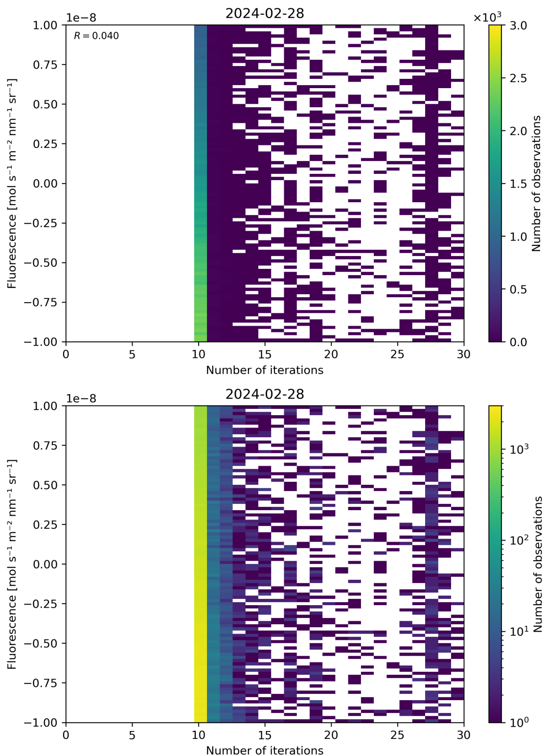
Figure 87: Scatter density plot of “Number of iterations” against “Fluorescence” for 2024-02-27 to 2024-02-29.
