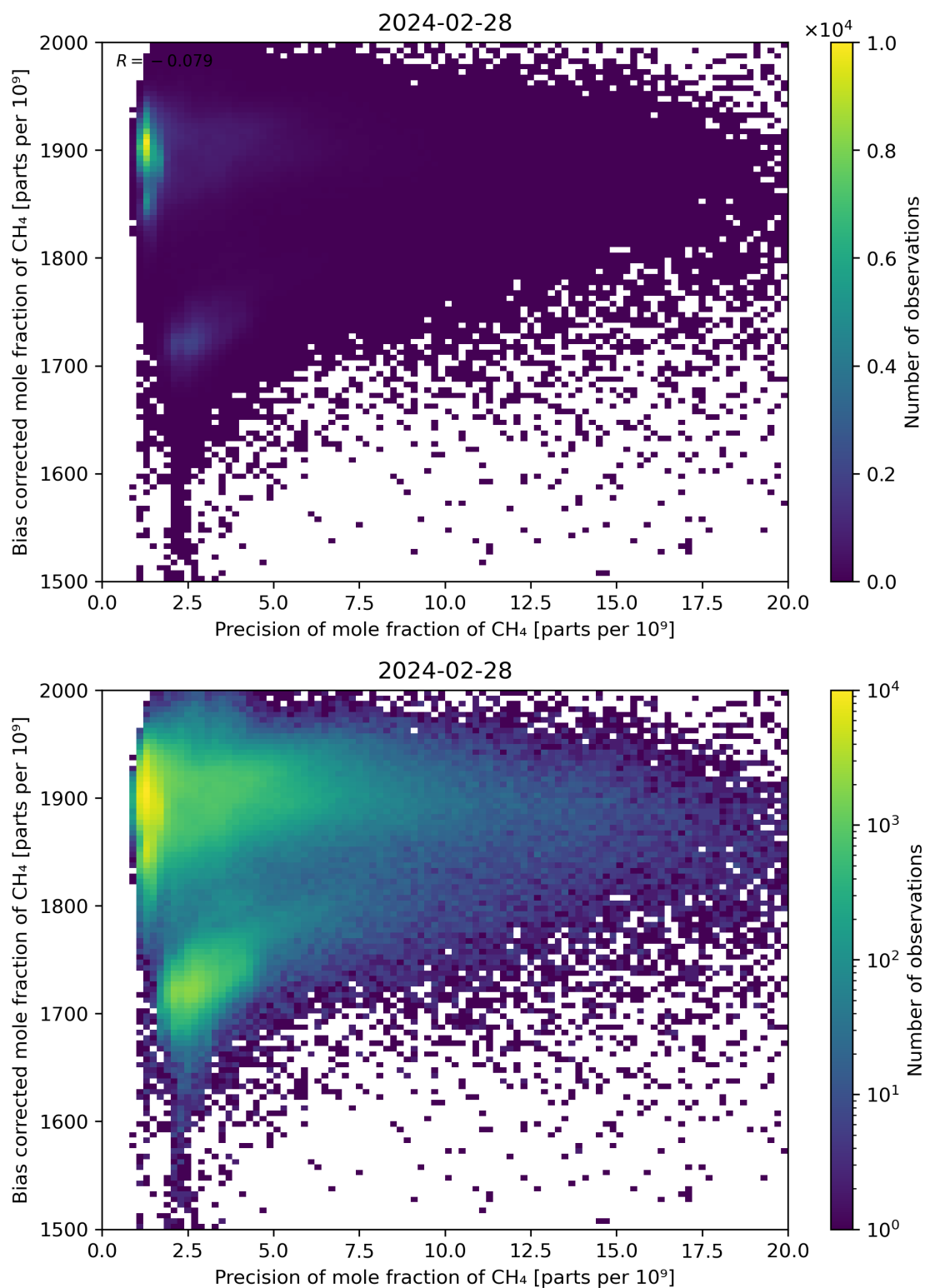
Figure 82: Scatter density plot of “Precision of mole fraction of CH 4 ” against “Bias corrected mole fraction of CH 4 ” for 2024-02-27 to 2024-02-29.
