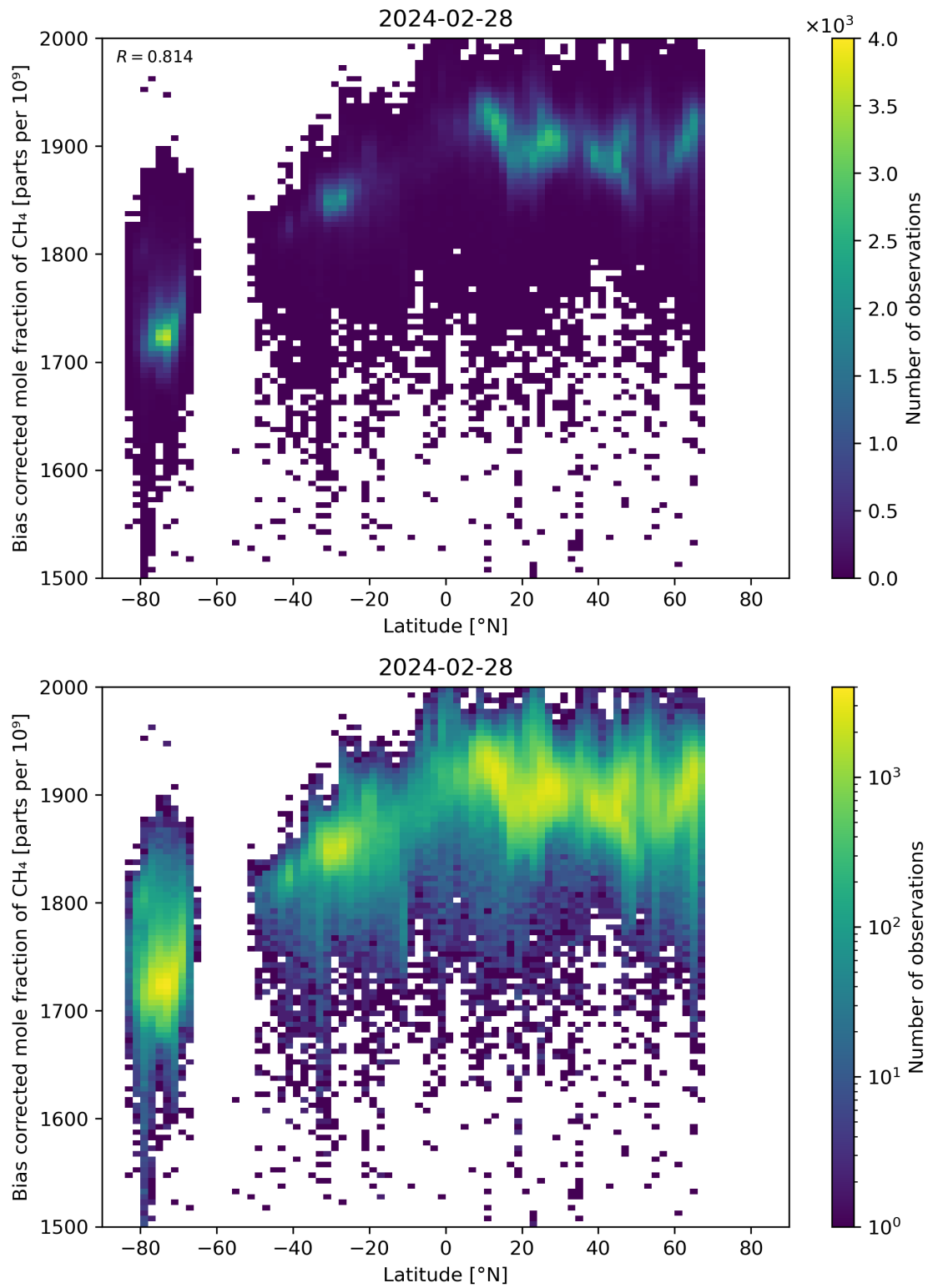
Figure 58: Scatter density plot of “Latitude” against “Bias corrected mole fraction of CH 4 ” for 2024-02-27 to 2024-02-29.
