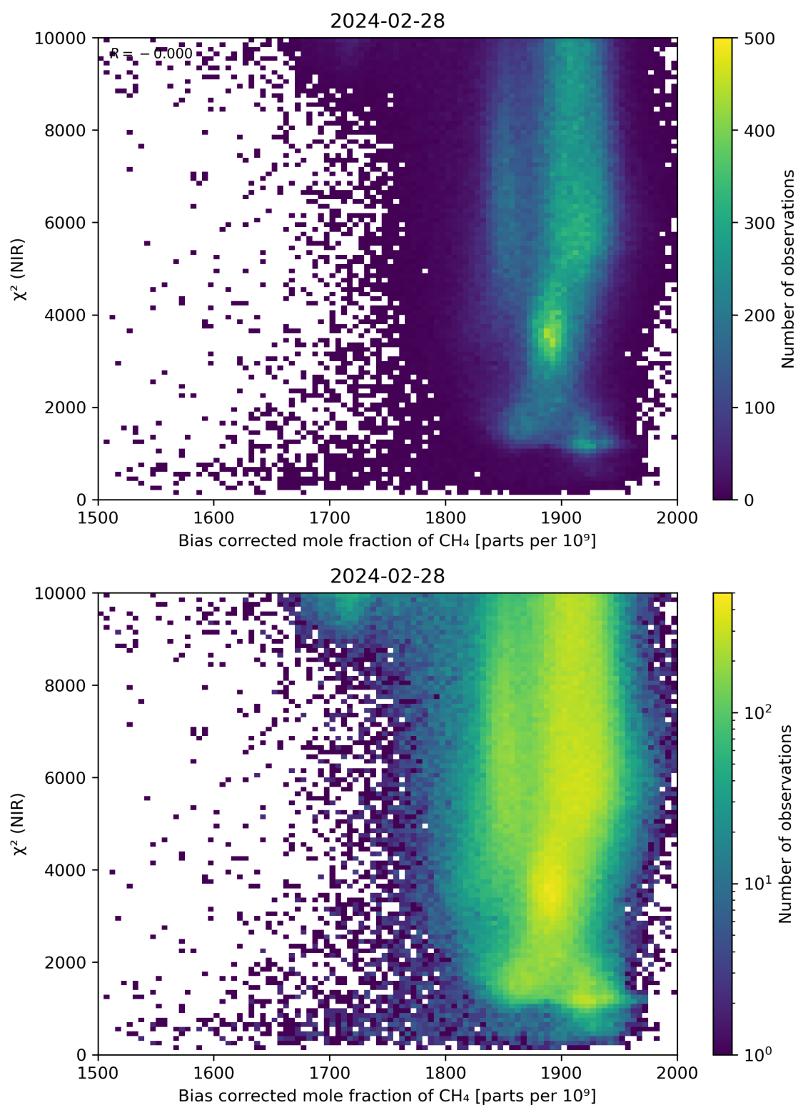
Figure 63: Scatter density plot of “Bias corrected mole fraction of \text{CH}_4 ” against “ \chi^2 (NIR)” for 2024-02-27 to 2024-02-29.
