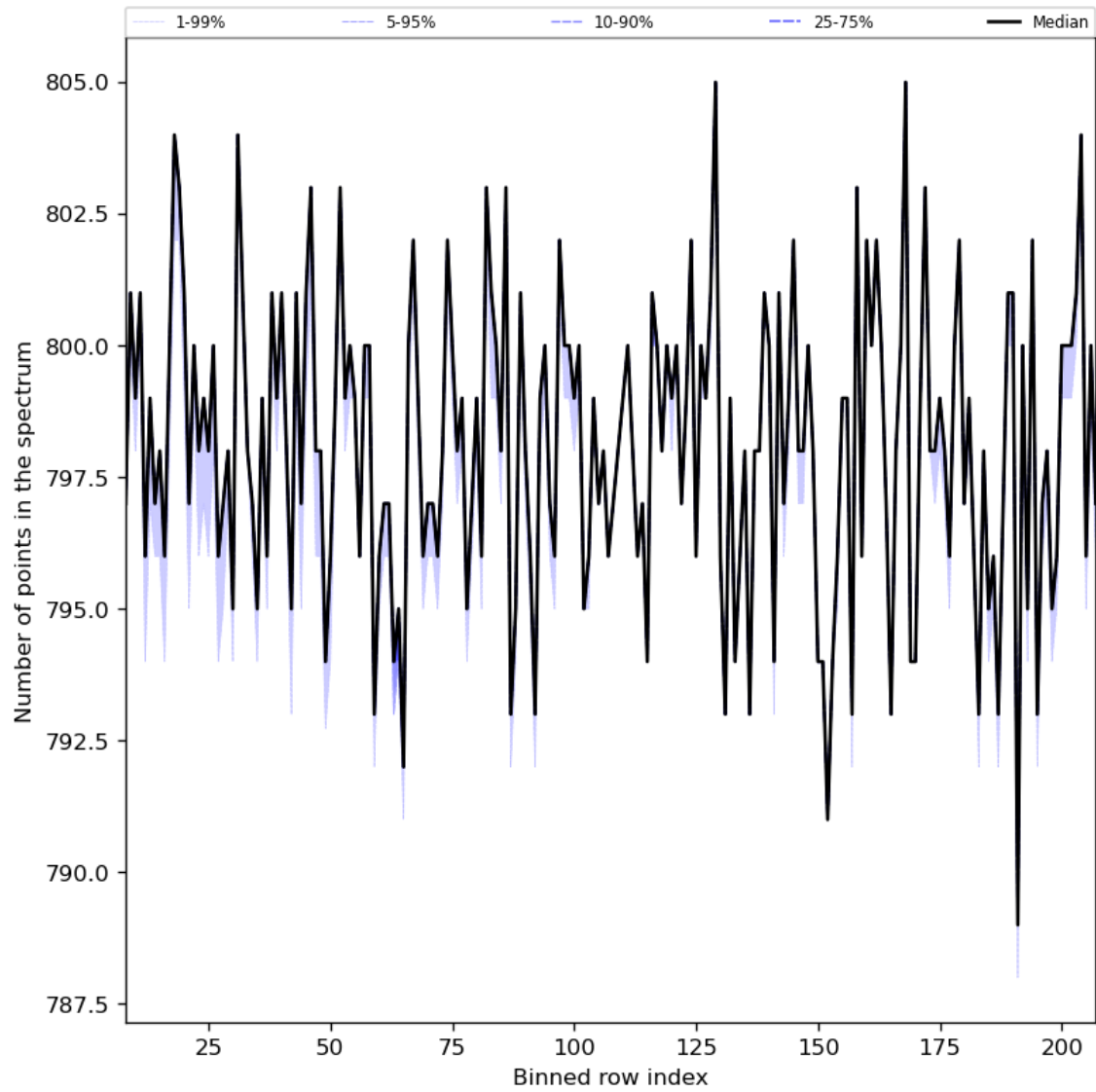
Figure 37: Along track statistics of “Number of points in the spectrum” for 2024-02-27 to 2024-02-29
