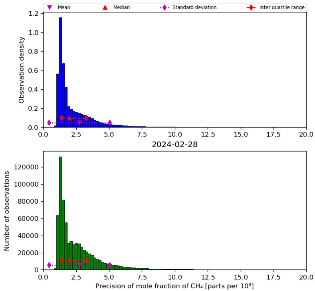
Figure 24: Histogram of “Precision of mole fraction of CH 4 ” for 2024-02-27 to 2024-02-29
