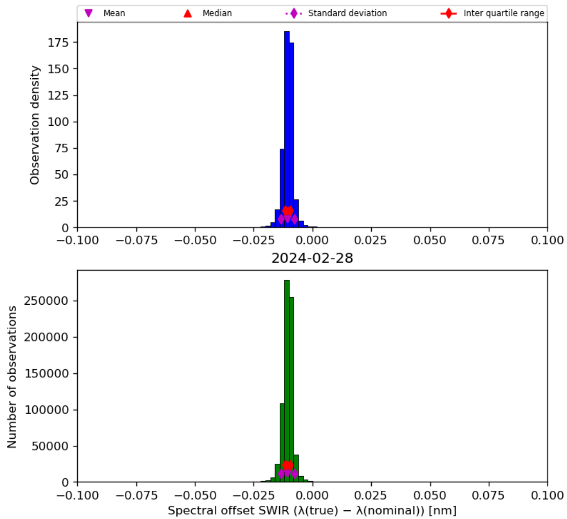
Figure 27: Histogram of “Spectral offset SWIR ( \lambda(\text{true}) - \lambda(\text{nominal}) )” for 2024-02-27 to 2024-02-29
