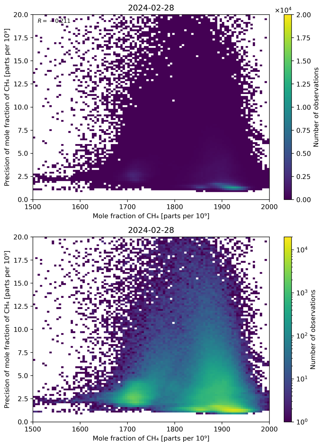
Figure 75: Scatter density plot of “Mole fraction of CH 4 ” against “Precision of mole fraction of CH 4 ” for 2024-02-27 to 2024-02-29.
