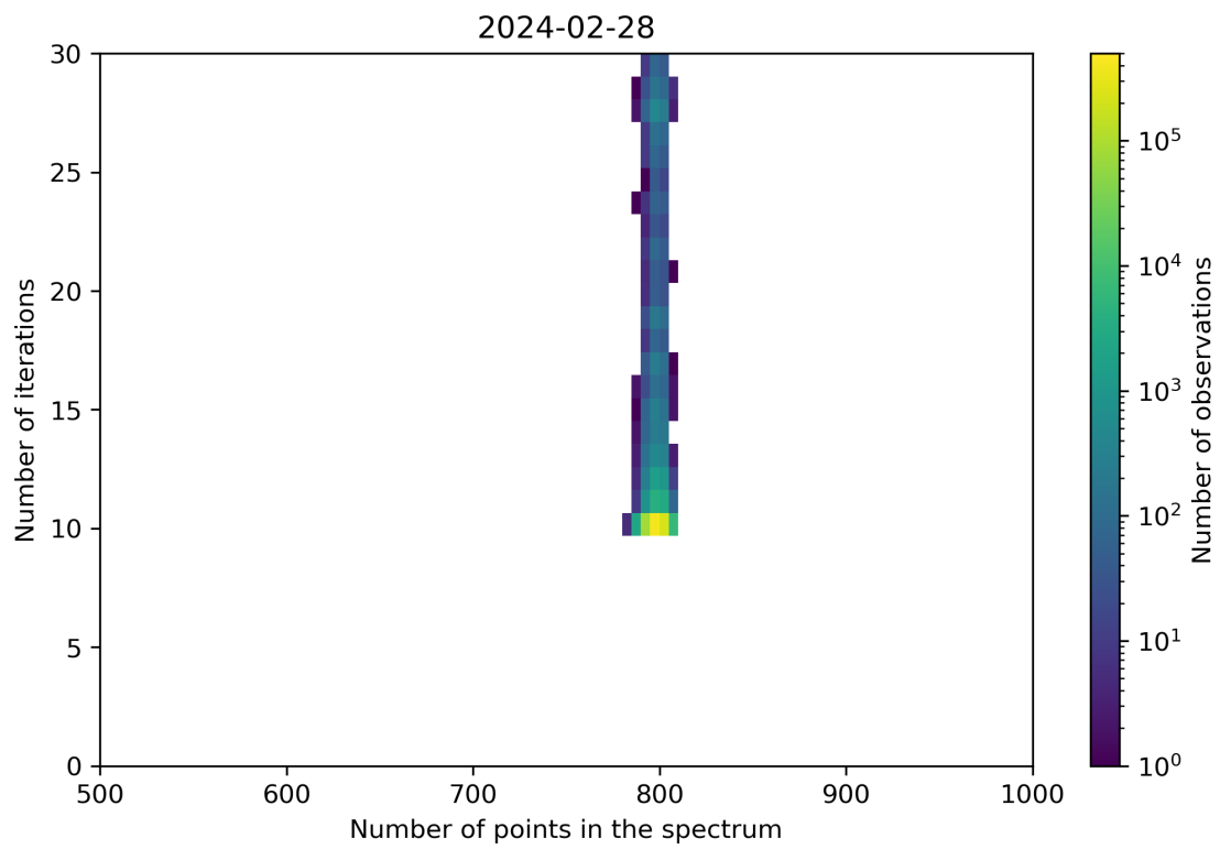
Figure 92: Scatter density plot of “Number of points in the spectrum” against “Number of iterations” for 2024-02-27 to 2024-02-29.
