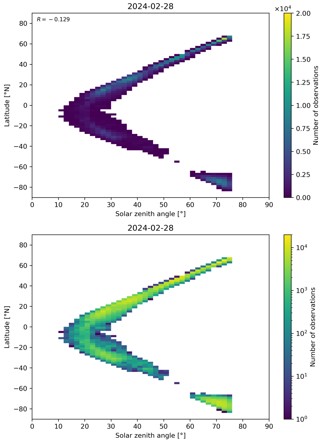
Figure 98: Scatter density plot of “Solar zenith angle” against “Latitude” for 2024-02-27 to 2024-02-29.
