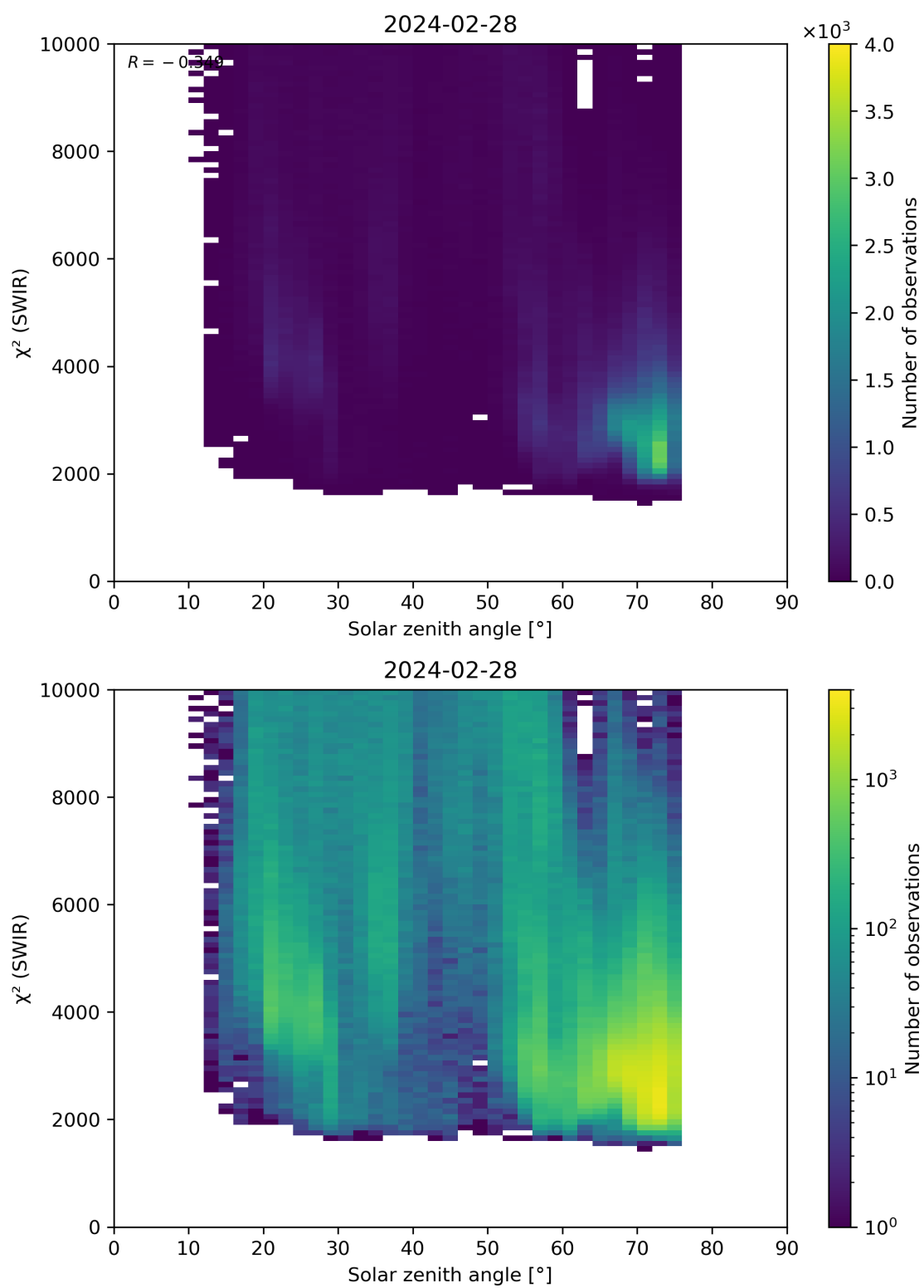
Figure 95: Scatter density plot of “Solar zenith angle” against “ \chi^2 (SWIR)” for 2024-02-27 to 2024-02-29.
