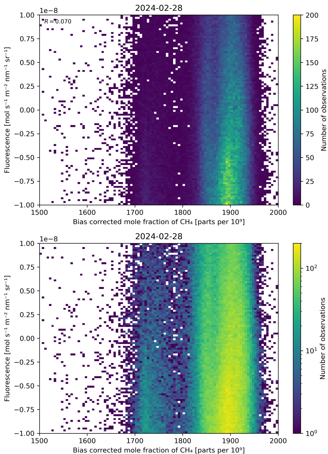
Figure 66: Scatter density plot of “Bias corrected mole fraction of \text{CH}_4 ” against “Fluorescence” for 2024-02-27 to 2024-02-29.
