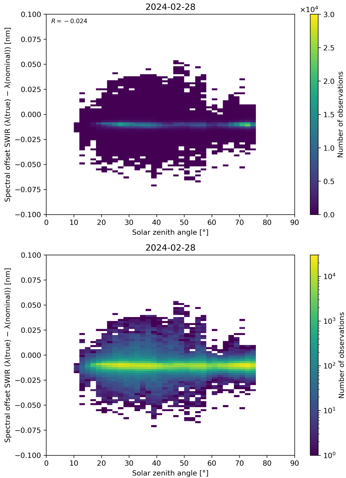
Figure 104: Scatter density plot of “Solar zenith angle” against “Spectral offset SWIR ( \lambda(\text{true}) - \lambda(\text{nominal}) )” for 2024-02-27 to 2024-02-29.
