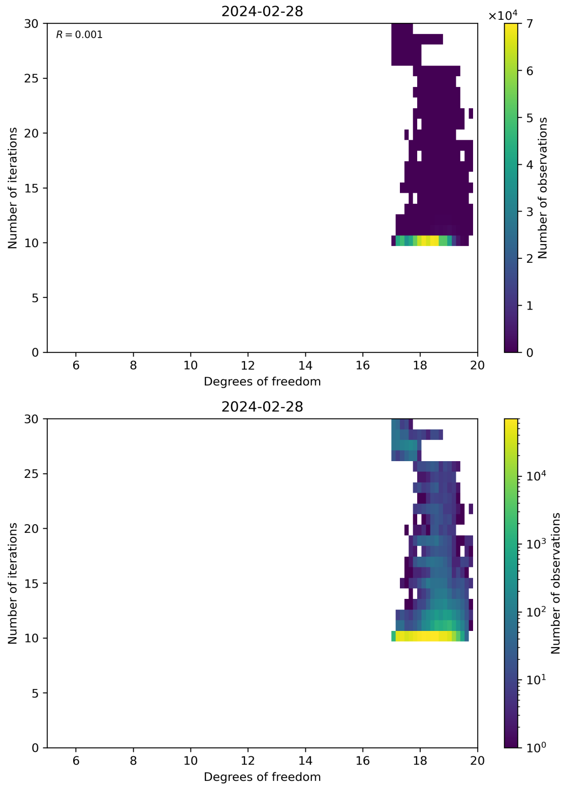
Figure 52: Scatter density plot of “Degrees of freedom” against “Number of iterations” for 2024-02-27 to 2024-02-29.
