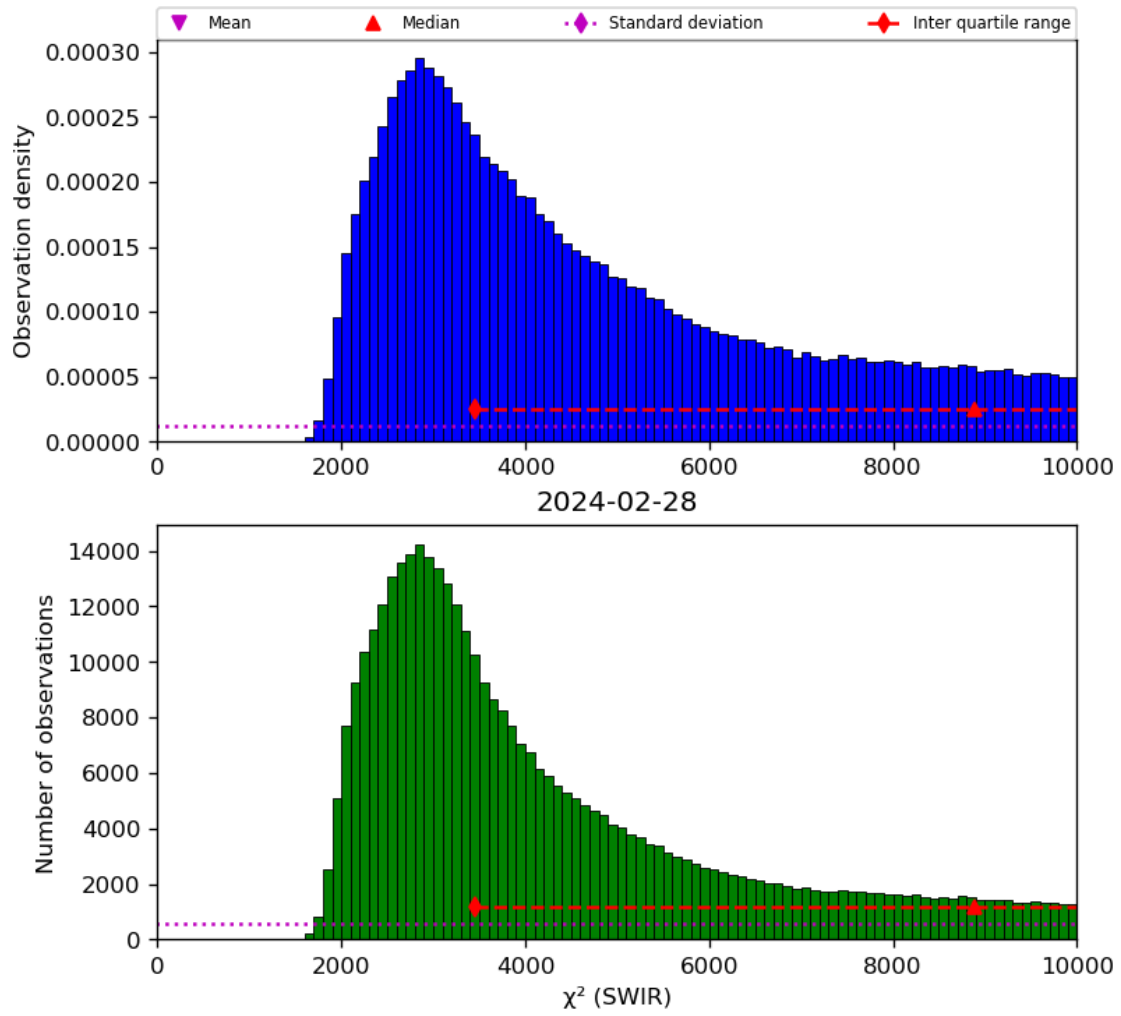
Figure 28: Histogram of “ \chi^2 (SWIR)” for 2024-02-27 to 2024-02-29
