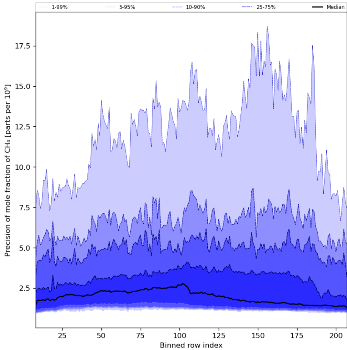
Figure 35: Along track statistics of “Precision of mole fraction of CH 4 ” for 2024-02-27 to 2024-02-29
