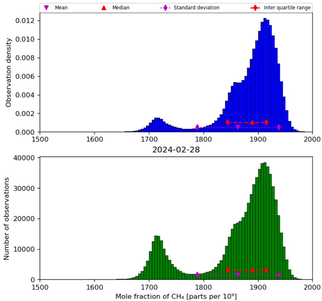
Figure 23: Histogram of “Mole fraction of CH 4 ” for 2024-02-27 to 2024-02-29
