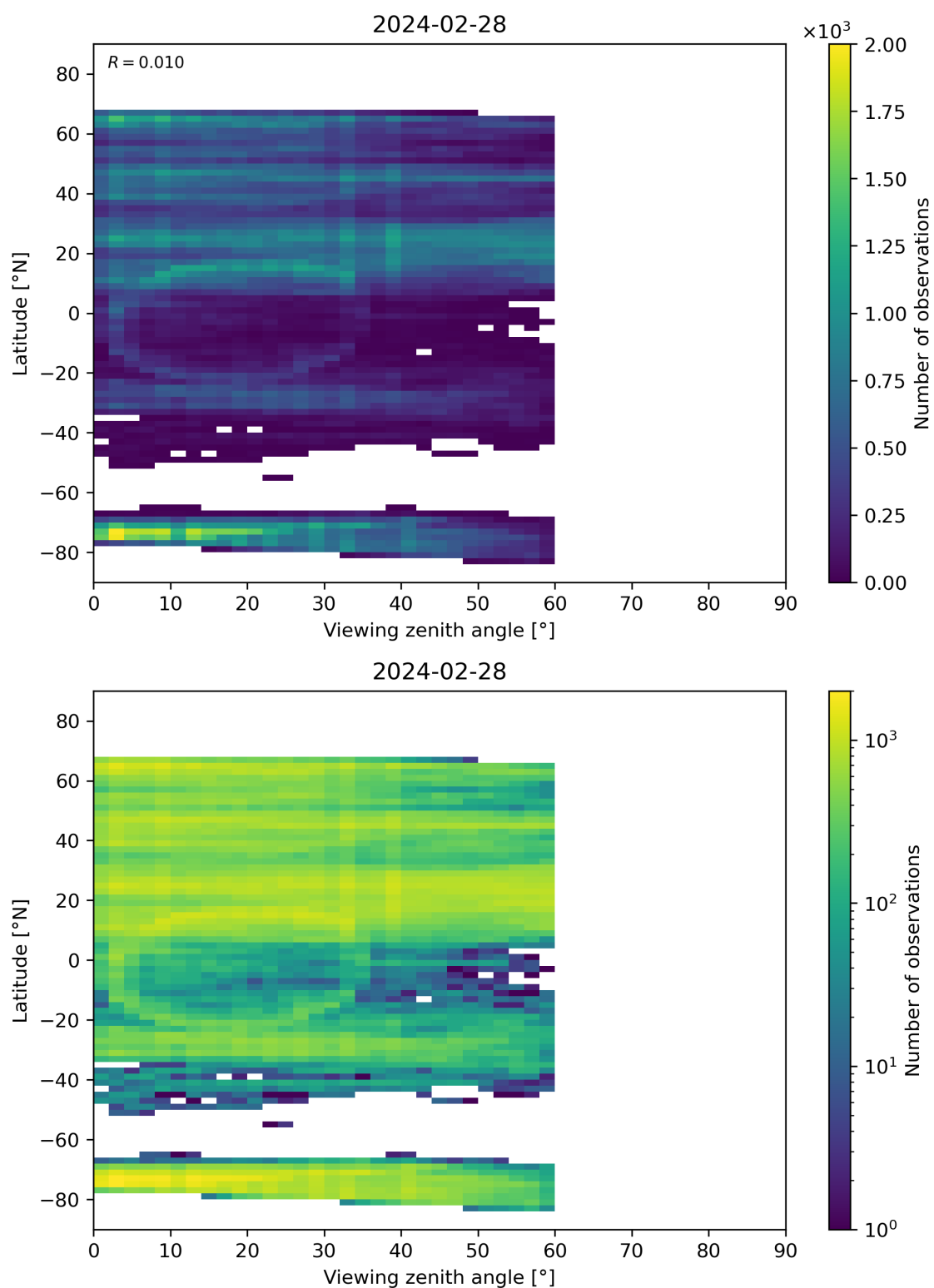
Figure 109: Scatter density plot of “Viewing zenith angle” against “Latitude” for 2024-02-27 to 2024-02-29.
