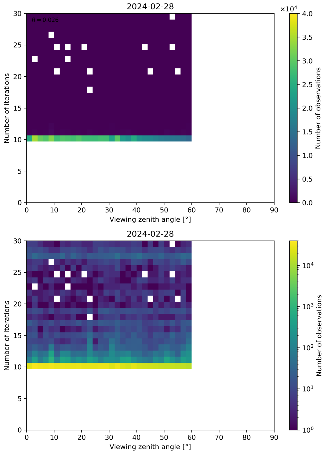
Figure 113: Scatter density plot of “Viewing zenith angle” against “Number of iterations” for 2024-02-27 to 2024-02-29.
