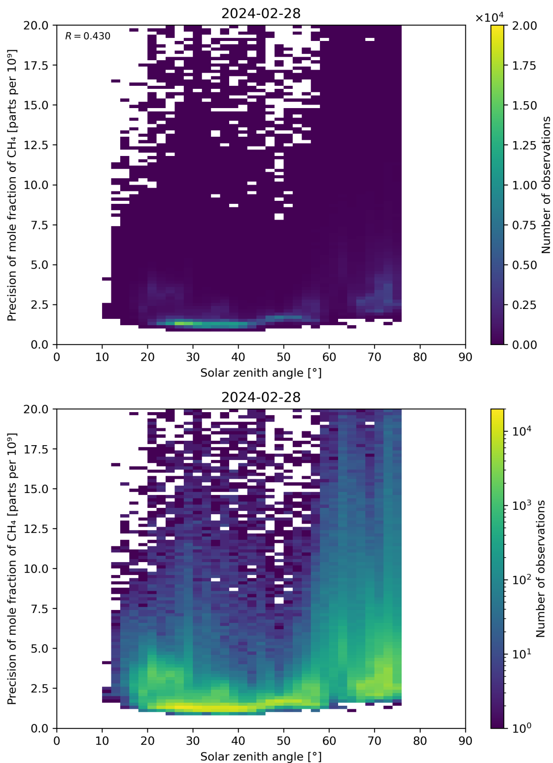
Figure 101: Scatter density plot of “Solar zenith angle” against “Precision of mole fraction of CH 4 ” for 2024-02-27 to 2024-02-29.
