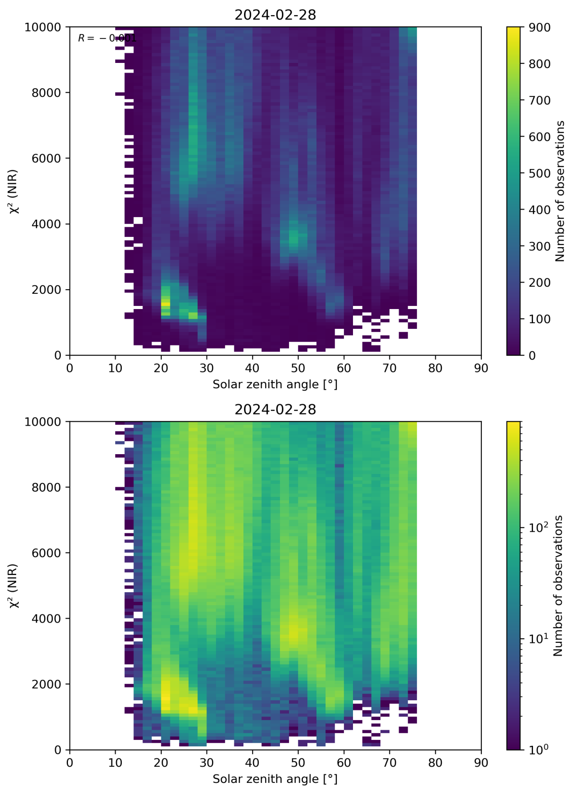
Figure 94: Scatter density plot of “Solar zenith angle” against “ \chi^2 (NIR)” for 2024-02-27 to 2024-02-29.
