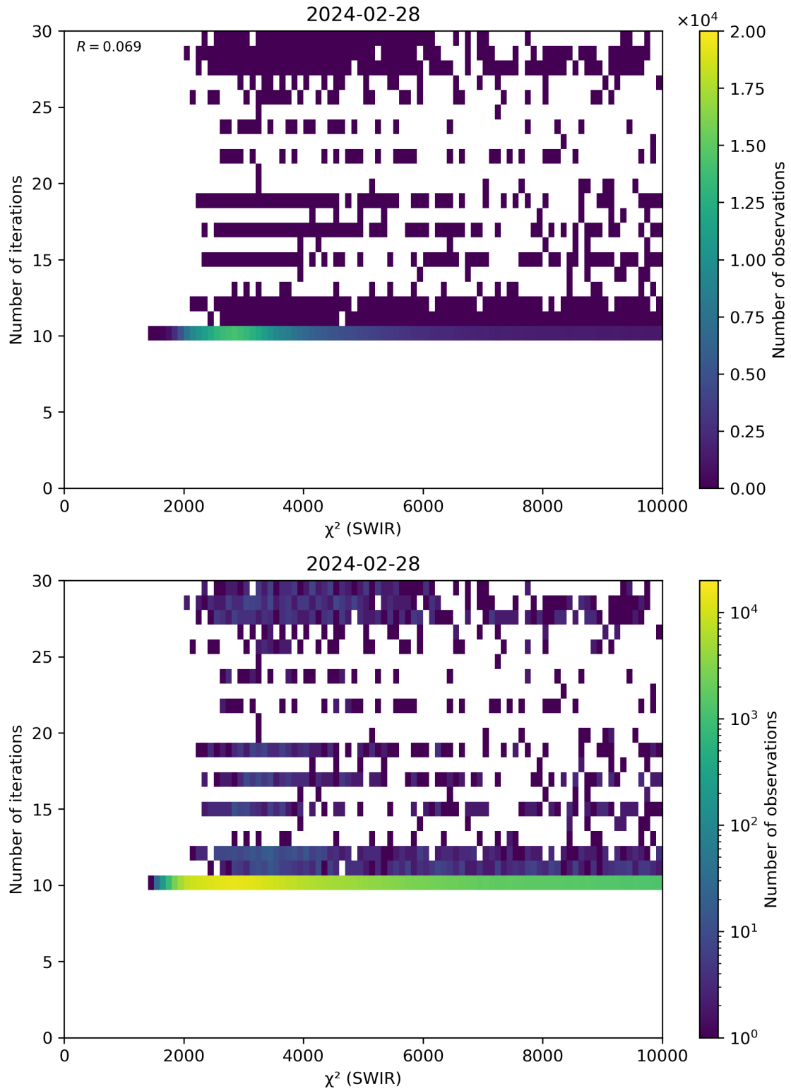
Figure 50: Scatter density plot of “ \chi^2 (SWIR)” against “Number of iterations” for 2024-02-27 to 2024-02-29.
