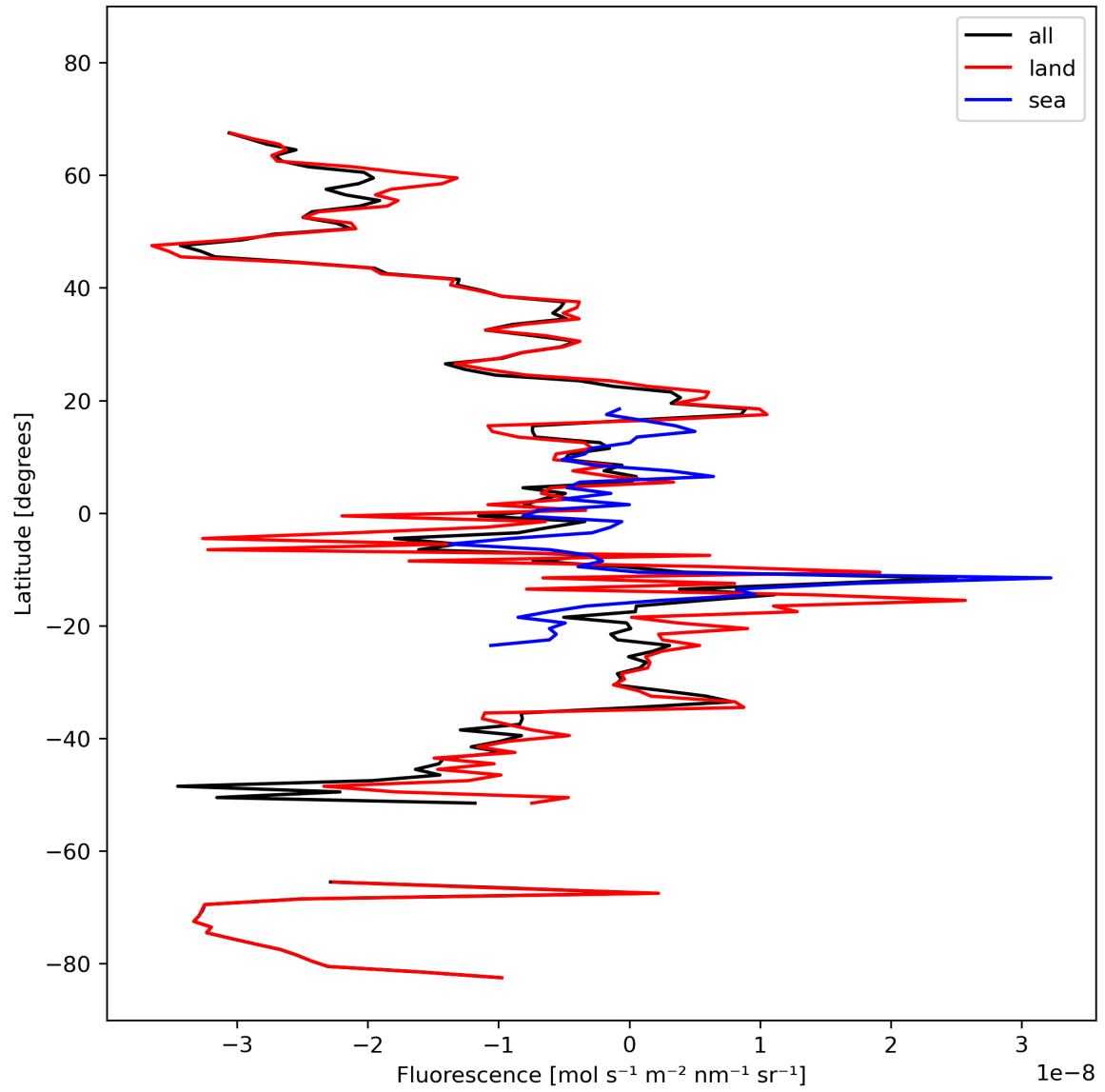
Figure 21: Zonal average of “Fluorescence” for 2024-02-27 to 2024-02-29.
