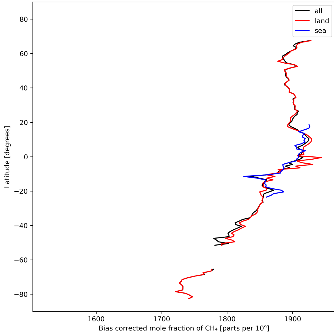
Figure 14: Zonal average of “Bias corrected mole fraction of CH 4 ” for 2024-02-27 to 2024-02-29.
