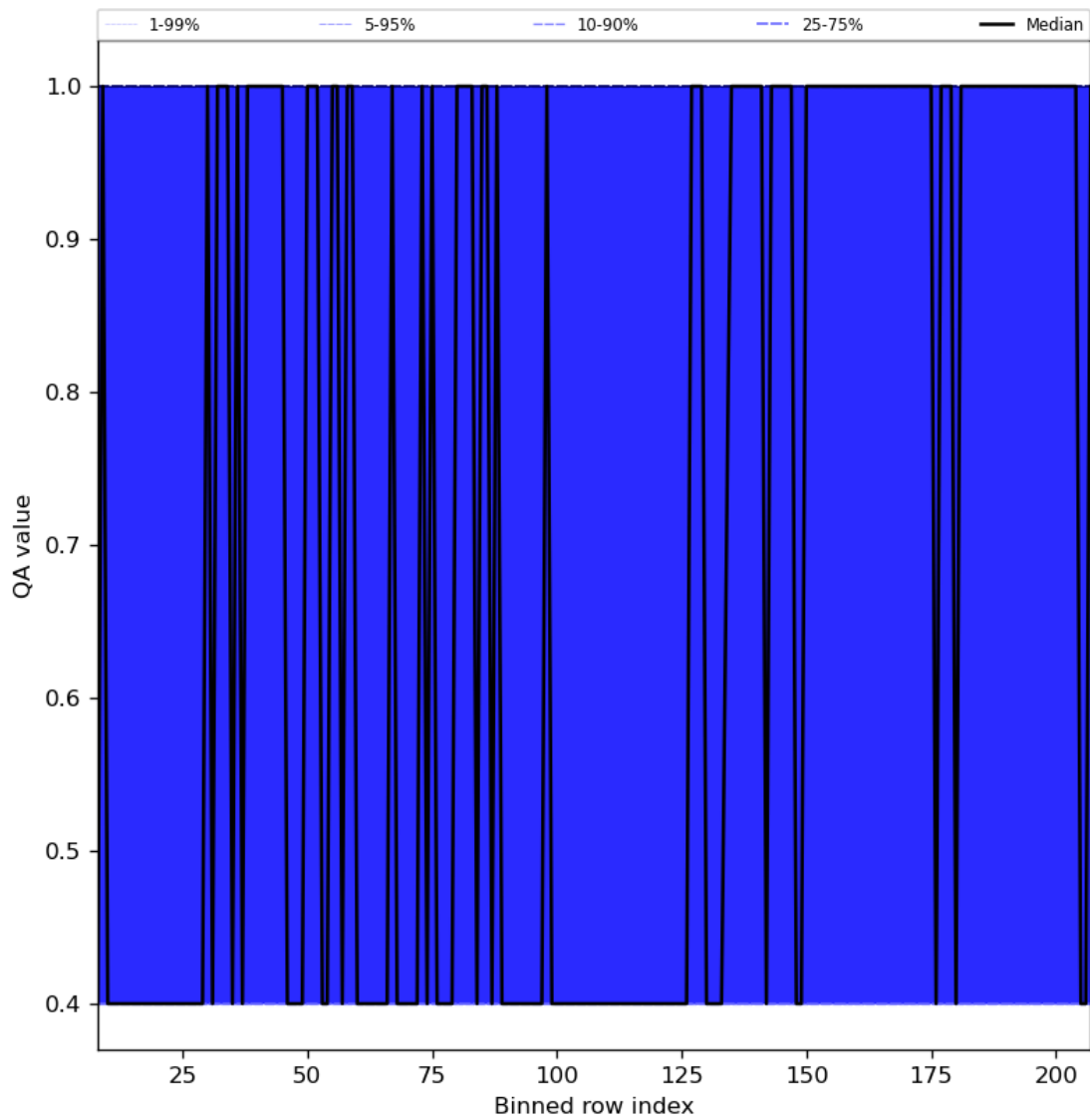
Figure 33: Along track statistics of “QA value” for 2024-02-27 to 2024-02-29
