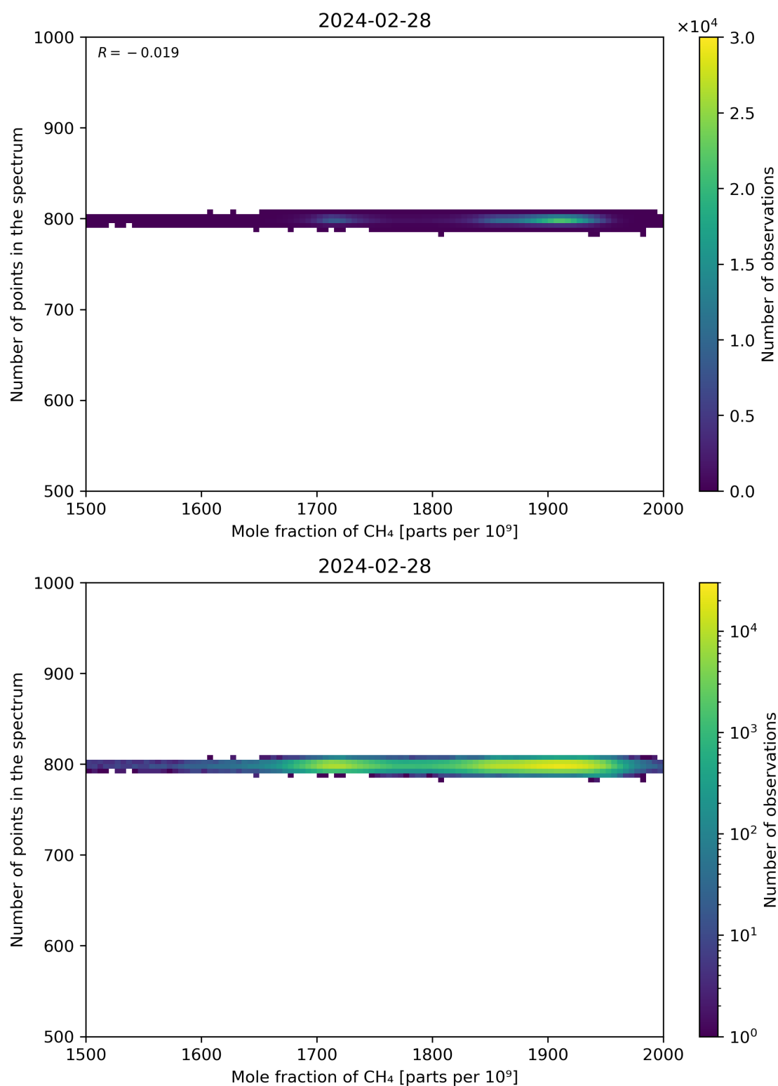
Figure 77: Scatter density plot of “Mole fraction of CH 4 ” against “Number of points in the spectrum” for 2024-02-27 to 2024-02-29.
