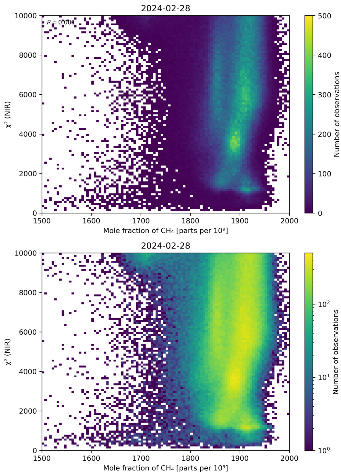
Figure 70: Scatter density plot of “Mole fraction of \text{CH}_4 ” against “ \chi^2 (NIR)” for 2024-02-27 to 2024-02-29.
