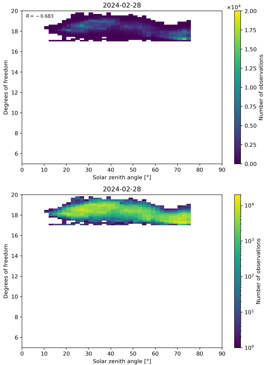
Figure 96: Scatter density plot of “Solar zenith angle” against “Degrees of freedom” for 2024-02-27 to 2024-02-29.
