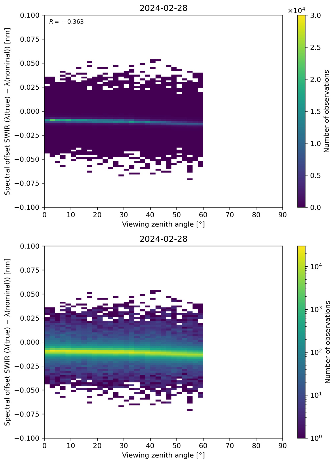
Figure 116: Scatter density plot of “Viewing zenith angle” against “Spectral offset SWIR ( \lambda(\text{true}) - \lambda(\text{nominal}) )” for 2024-02-27 to 2024-02-29.
