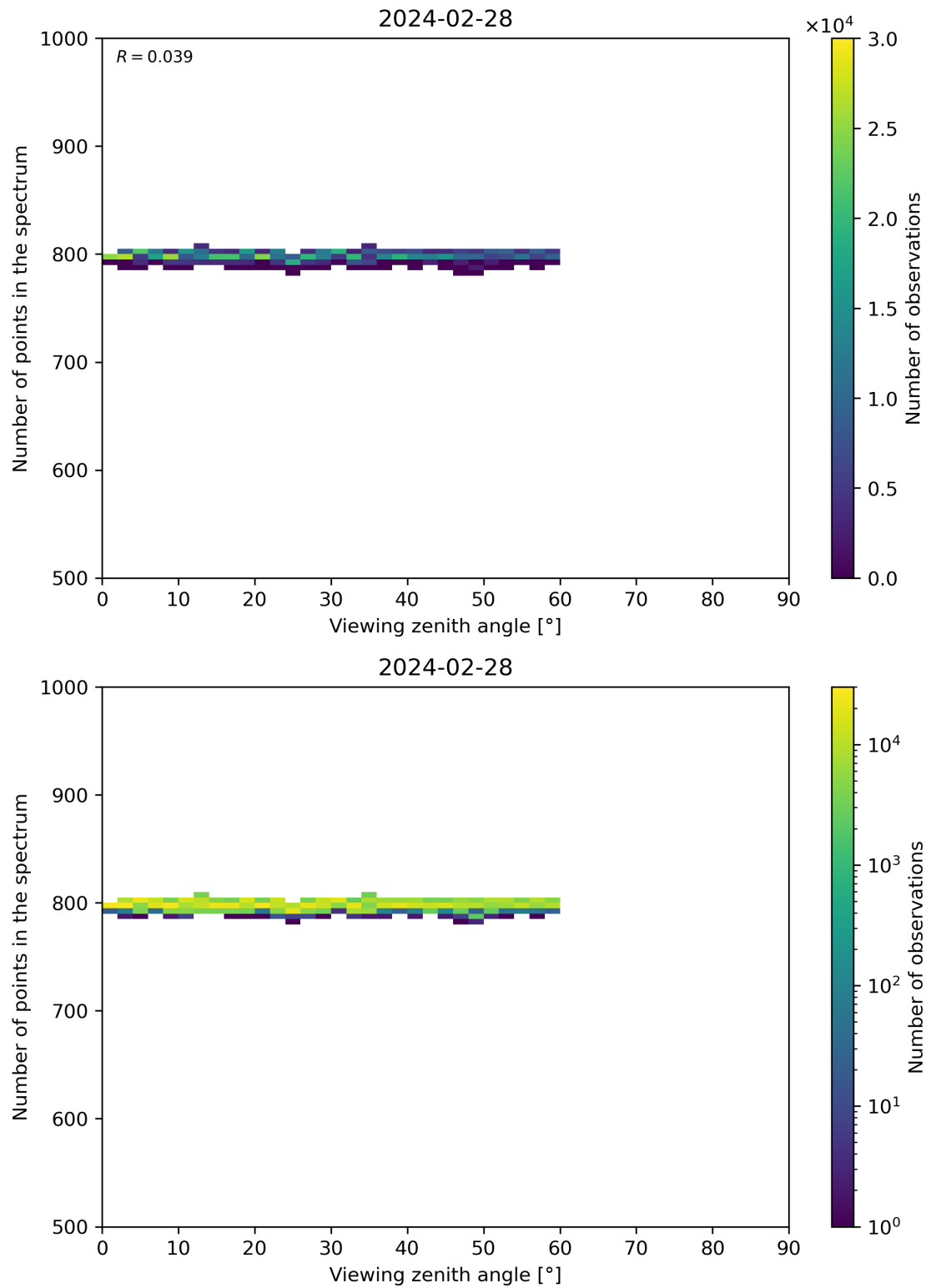
Figure 114: Scatter density plot of “Viewing zenith angle” against “Number of points in the spectrum” for 2024-02-27 to 2024-02-29.
