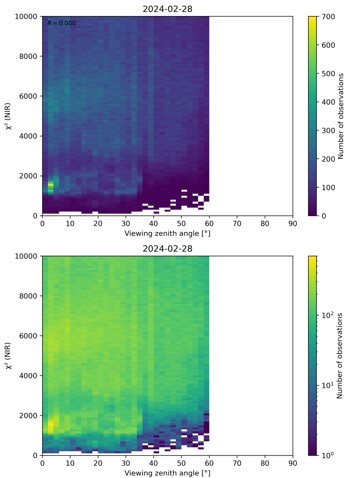
Figure 105: Scatter density plot of “Viewing zenith angle” against “ \chi^2 (NIR)” for 2024-02-27 to 2024-02-29.
