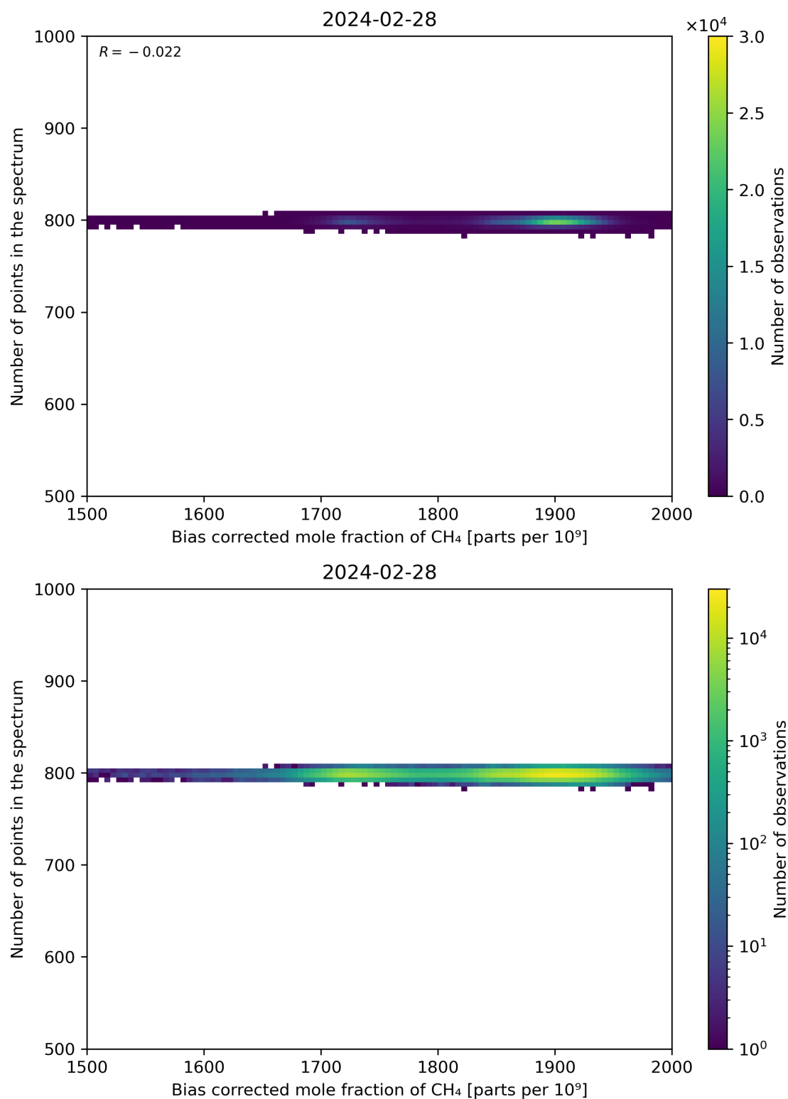
Figure 68: Scatter density plot of “Bias corrected mole fraction of CH 4 ” against “Number of points in the spectrum” for 2024-02-27 to 2024-02-29.
