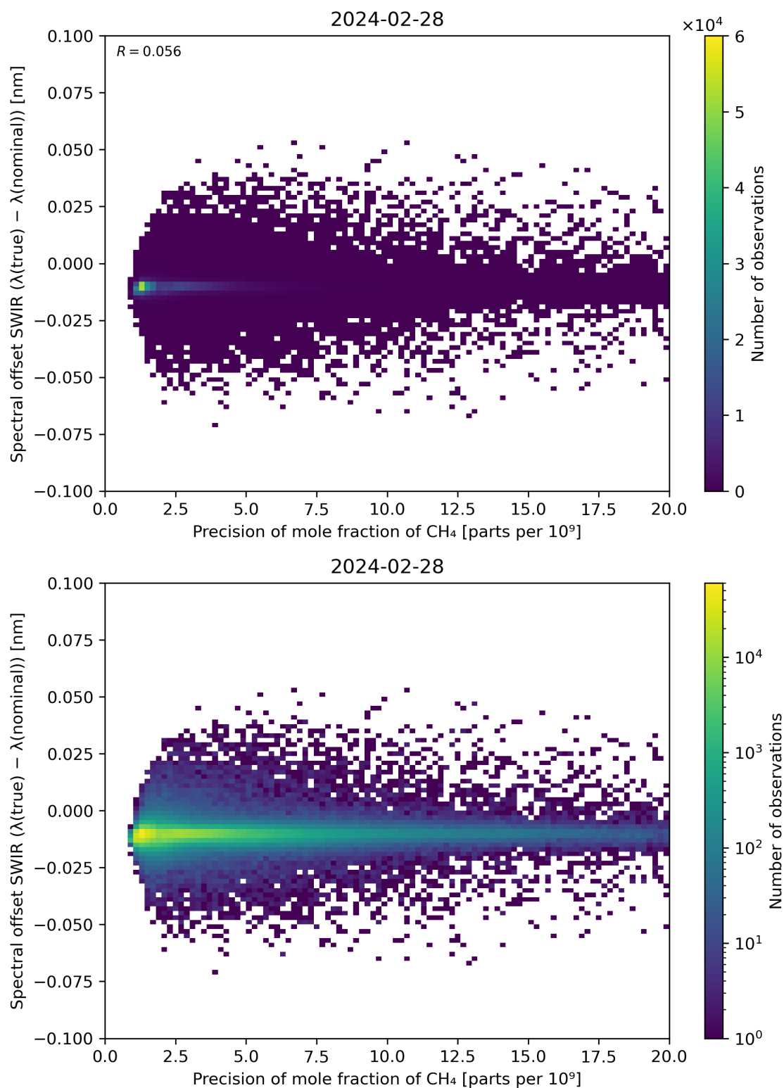
Figure 85: Scatter density plot of “Precision of mole fraction of \text{CH}_4 ” against “Spectral offset SWIR ( \lambda(\text{true}) - \lambda(\text{nominal}) )” for 2024-02-27 to 2024-02-29.
