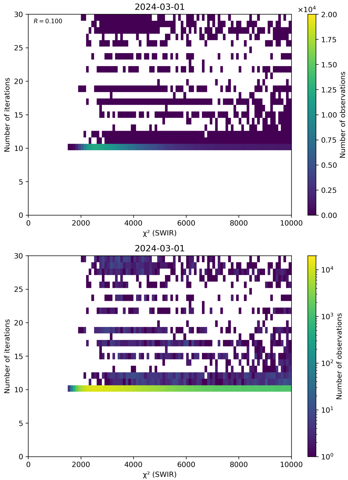
Figure 50: Scatter density plot of “ \chi^2 (SWIR)” against “Number of iterations” for 2024-02-29 to 2024-03-02.
