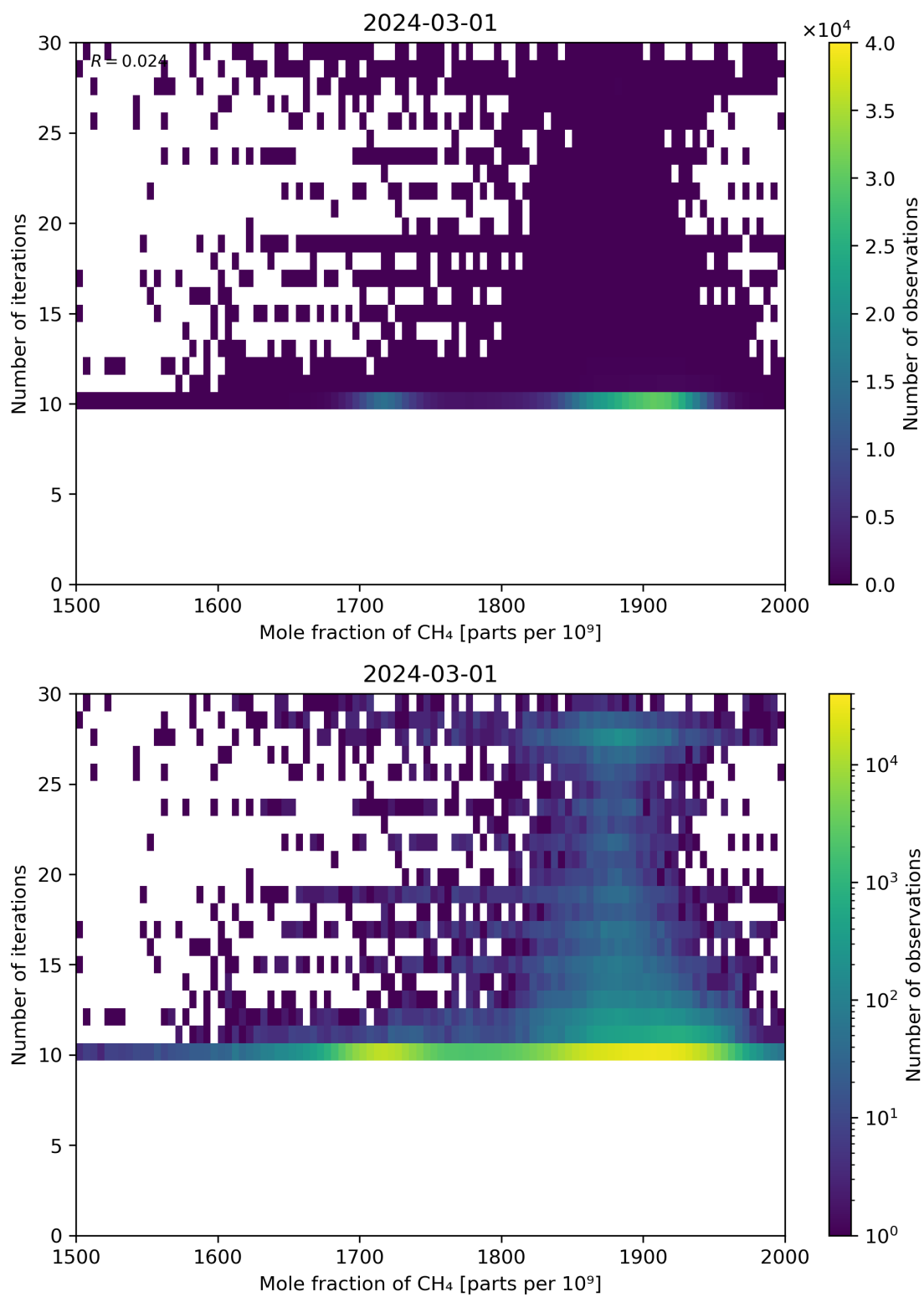
Figure 76: Scatter density plot of “Mole fraction of CH 4 ” against “Number of iterations” for 2024-02-29 to 2024-03-02.
