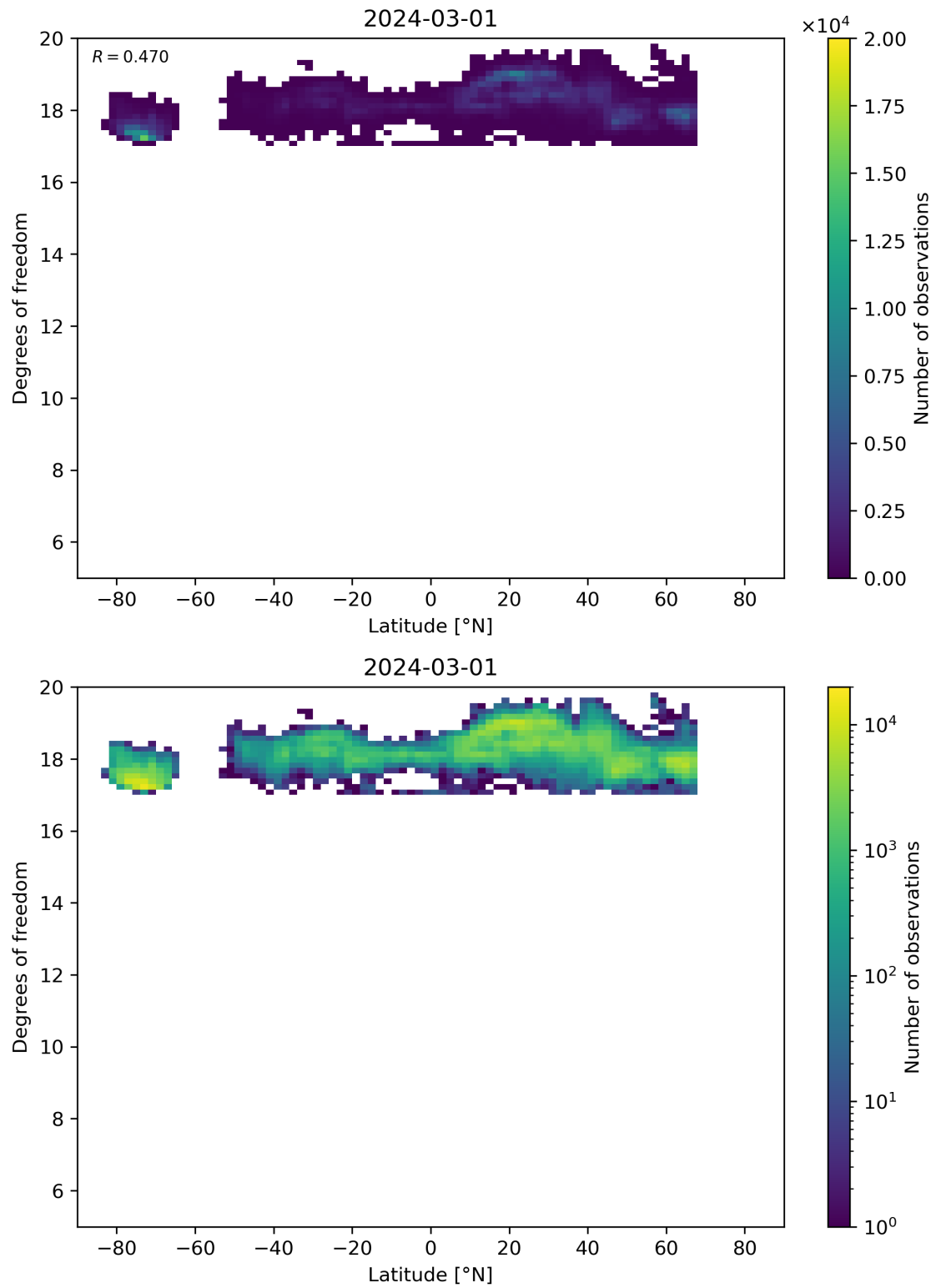
Figure 55: Scatter density plot of “Latitude” against “Degrees of freedom” for 2024-02-29 to 2024-03-02.
