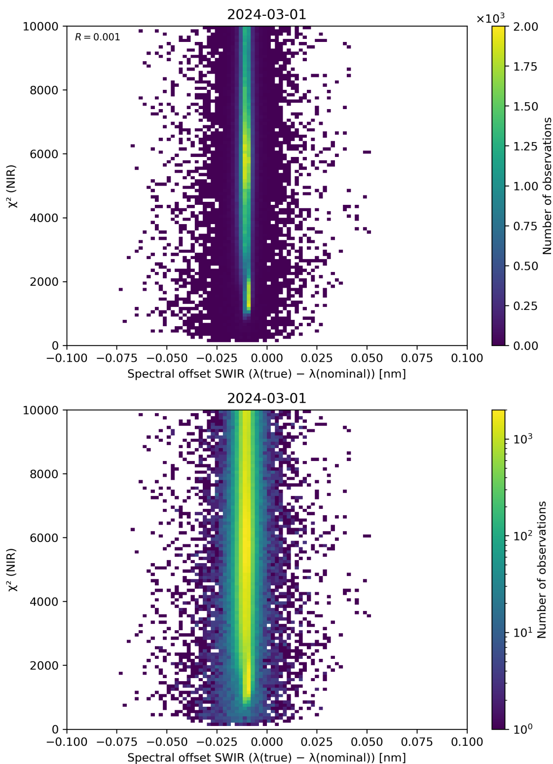
Figure 117: Scatter density plot of “Spectral offset SWIR ( \lambda(\text{true}) - \lambda(\text{nominal}) )” against “ \chi^2 (NIR)” for 2024-02-29 to 2024-03-02.
