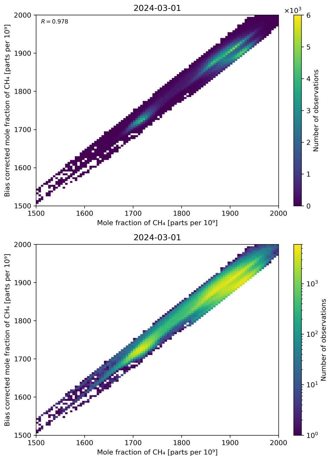
Figure 74: Scatter density plot of “Mole fraction of CH 4 ” against “Bias corrected mole fraction of CH 4 ” for 2024-02-29 to 2024-03-02.
