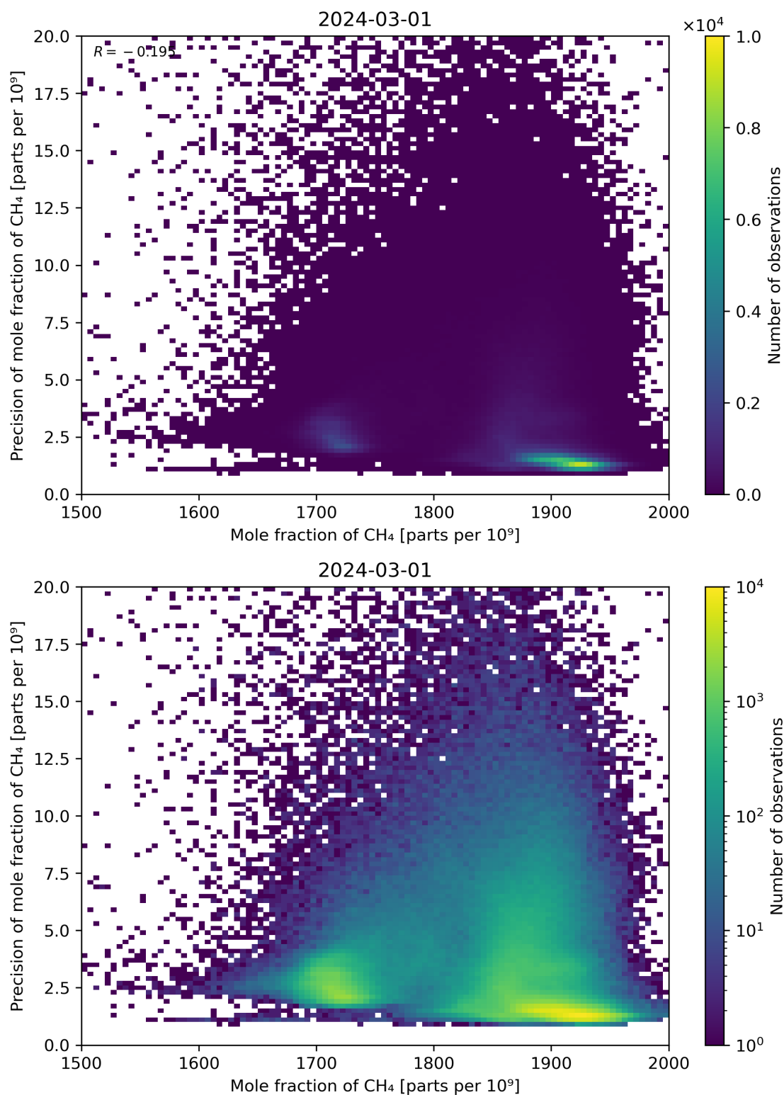
Figure 75: Scatter density plot of “Mole fraction of CH 4 ” against “Precision of mole fraction of CH 4 ” for 2024-02-29 to 2024-03-02.
