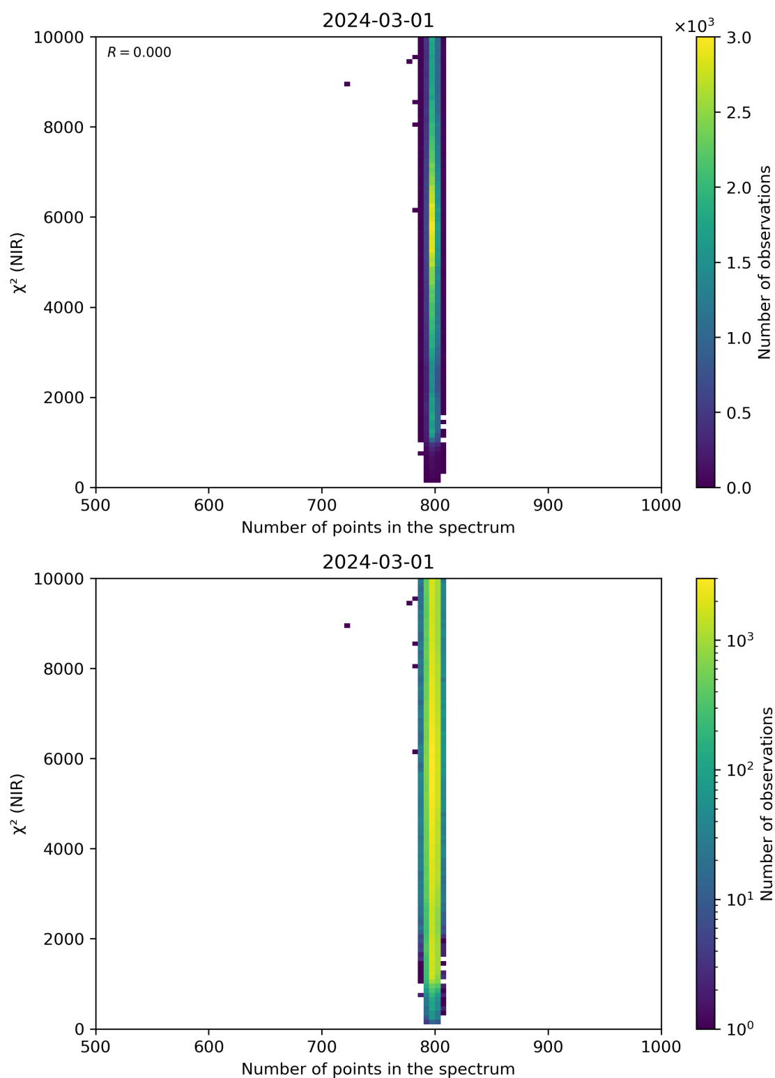
Figure 88: Scatter density plot of “Number of points in the spectrum” against “ \chi^2 (NIR)” for 2024-02-29 to 2024-03-02.
