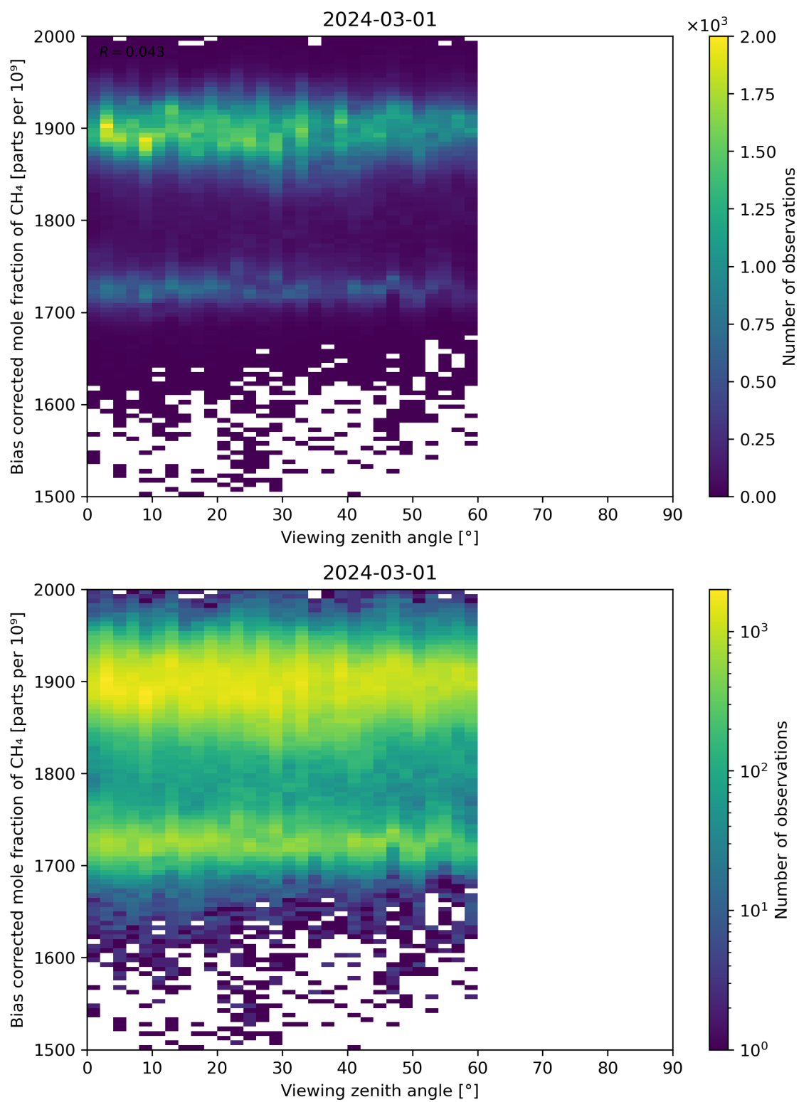
Figure 111: Scatter density plot of “Viewing zenith angle” against “Bias corrected mole fraction of CH 4 ” for 2024-02-29 to 2024-03-02.
