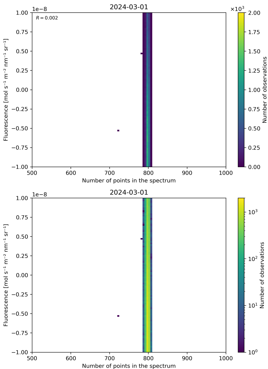
Figure 91: Scatter density plot of “Number of points in the spectrum” against “Fluorescence” for 2024-02-29 to 2024-03-02.
