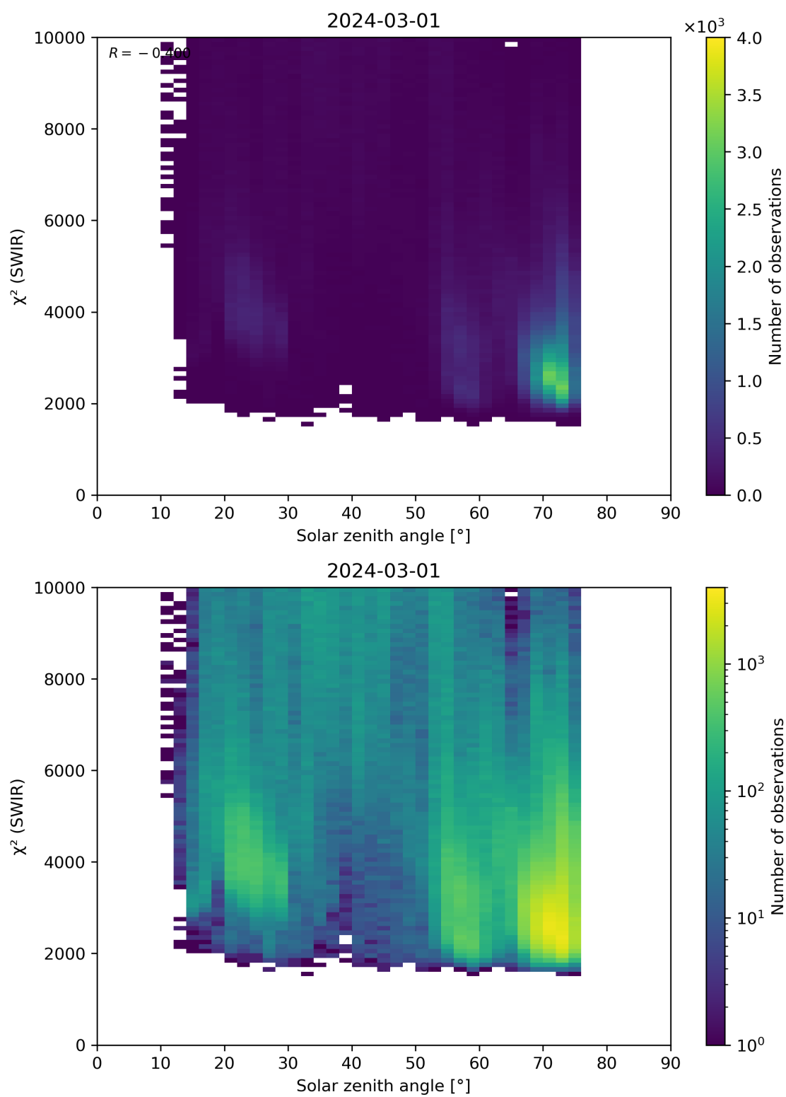
Figure 95: Scatter density plot of “Solar zenith angle” against “ \chi^2 (SWIR)” for 2024-02-29 to 2024-03-02.
