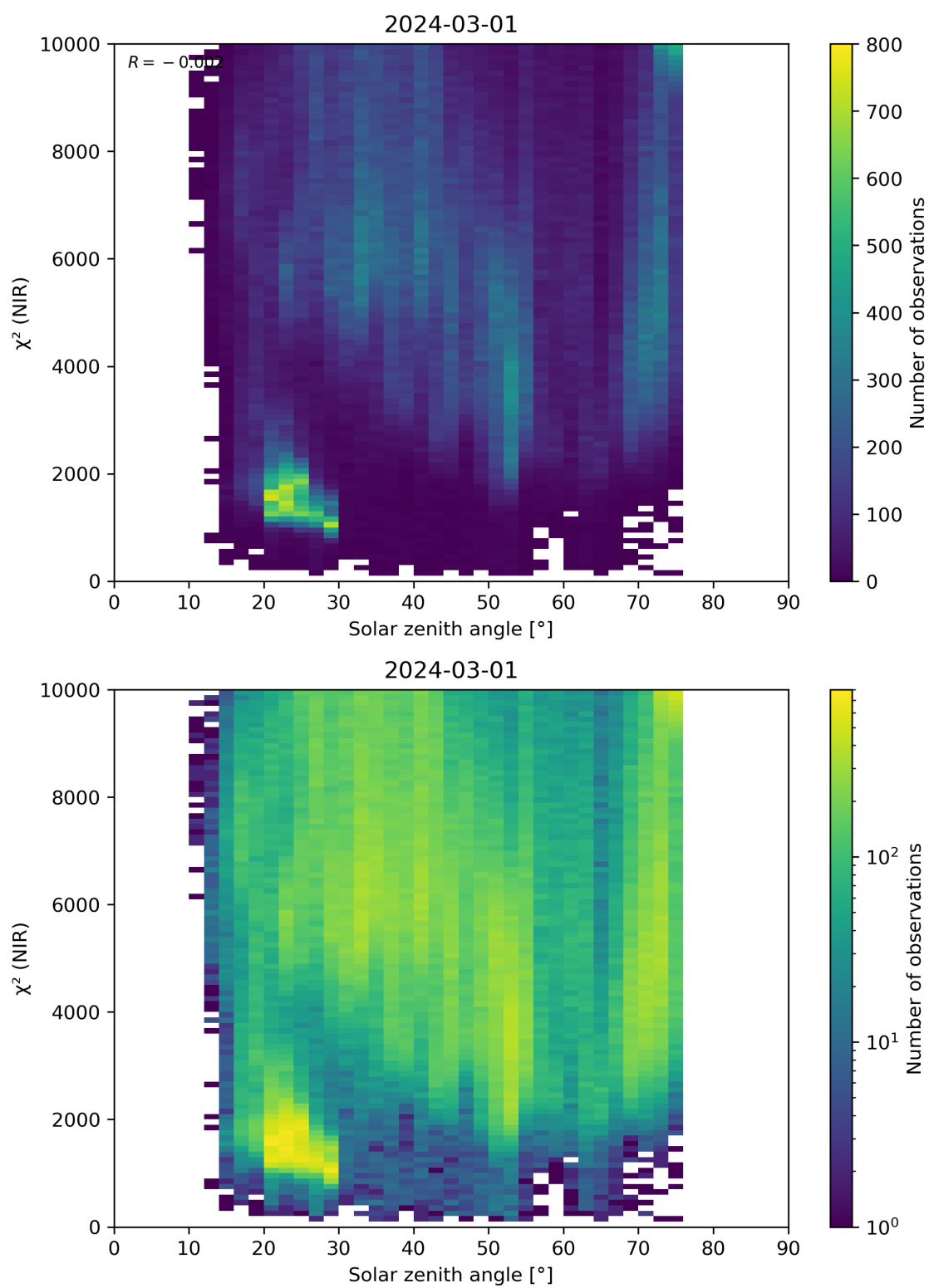
Figure 94: Scatter density plot of “Solar zenith angle” against “ \chi^2 (NIR)” for 2024-02-29 to 2024-03-02.
