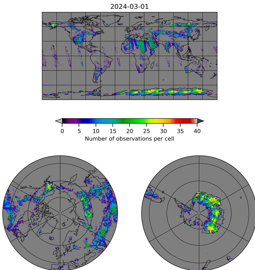
Figure 10: Map of the number of observations for 2024-02-29 to 2024-03-02
