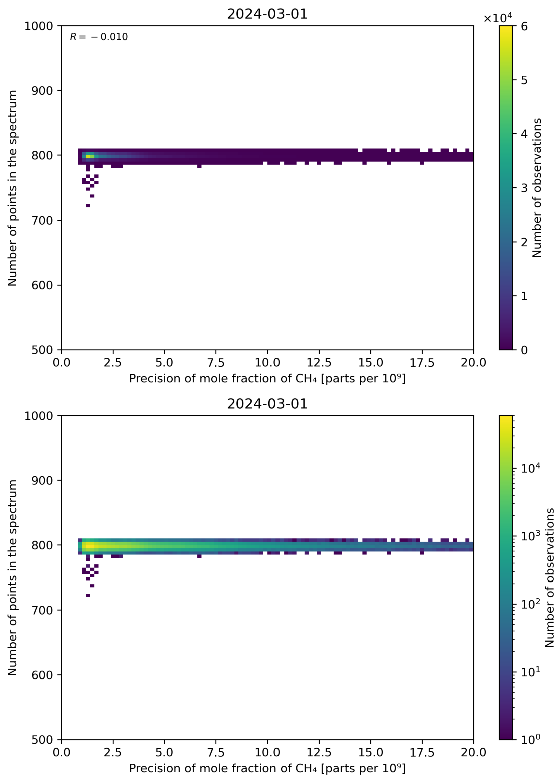
Figure 84: Scatter density plot of “Precision of mole fraction of CH 4 ” against “Number of points in the spectrum” for 2024-02-29 to 2024-03-02.
