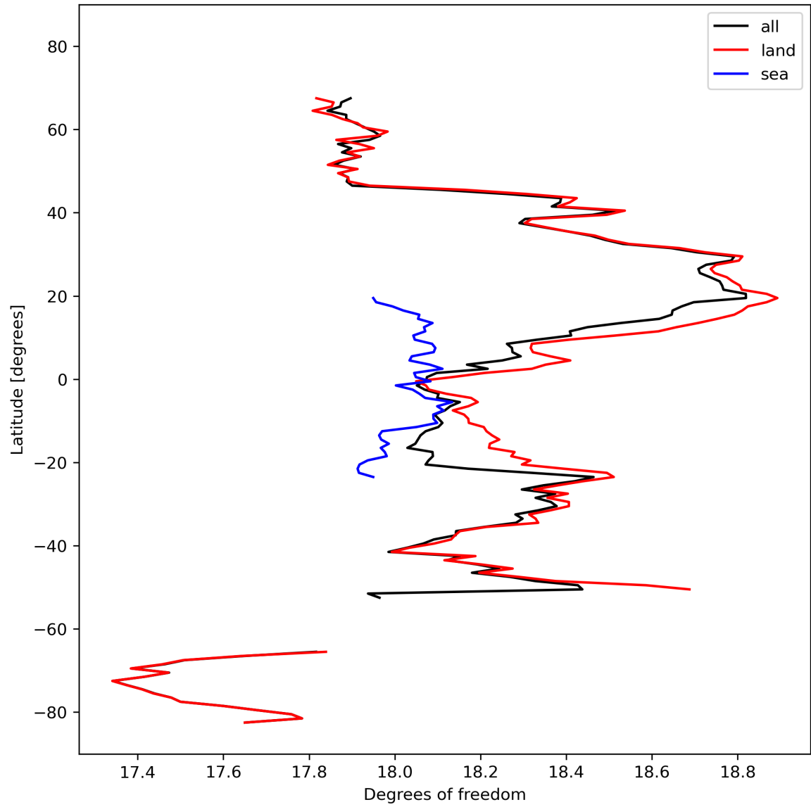
Figure 19: Zonal average of “Degrees of freedom” for 2024-02-29 to 2024-03-02.
