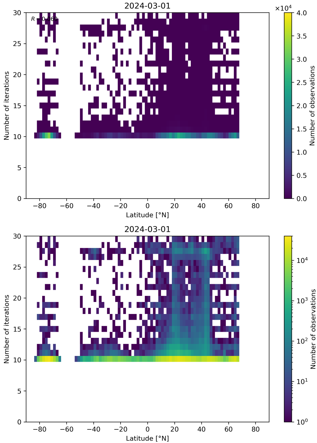
Figure 60: Scatter density plot of “Latitude” against “Number of iterations” for 2024-02-29 to 2024-03-02.
