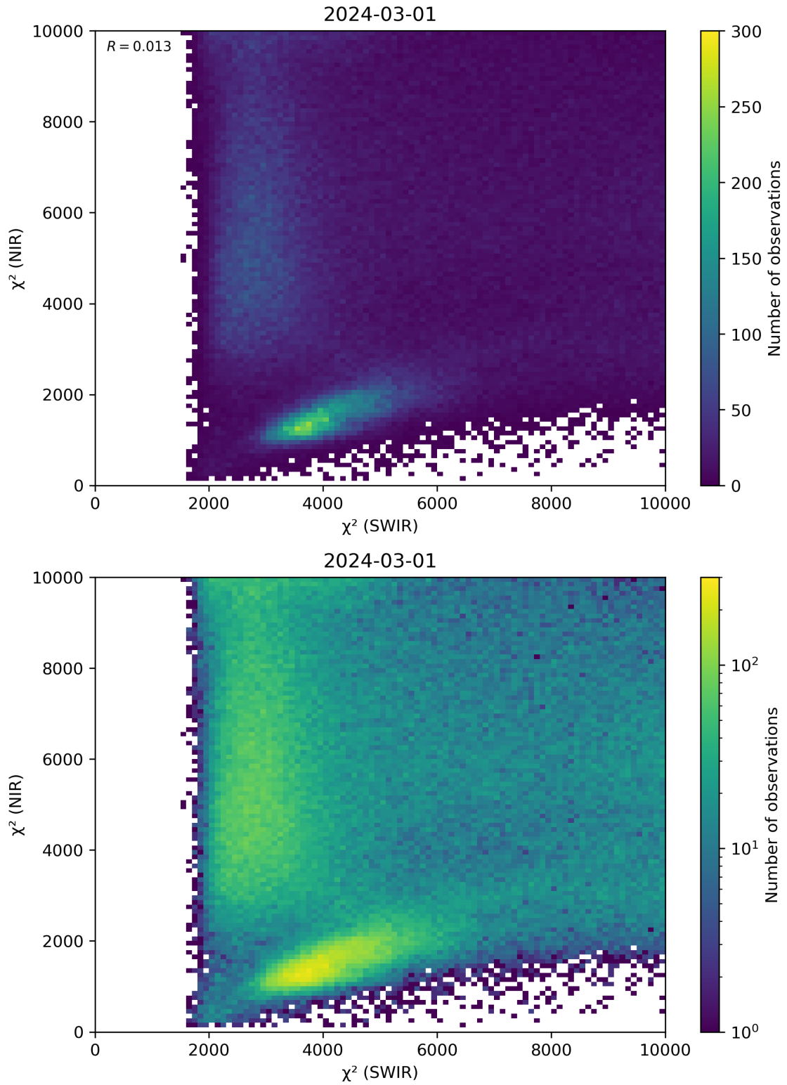
Figure 47: Scatter density plot of “ \chi^2 (SWIR)” against “ \chi^2 (NIR)” for 2024-02-29 to 2024-03-02.
