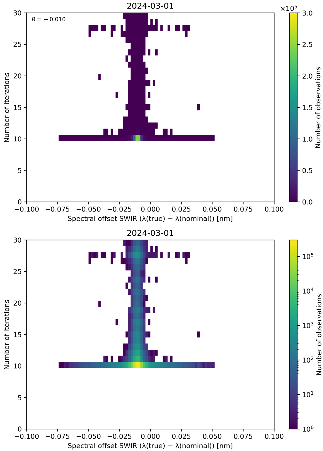
Figure 121: Scatter density plot of “Spectral offset SWIR ( \lambda(\text{true}) - \lambda(\text{nominal}) )” against “Number of iterations” for 2024-02-29 to 2024-03-02.
