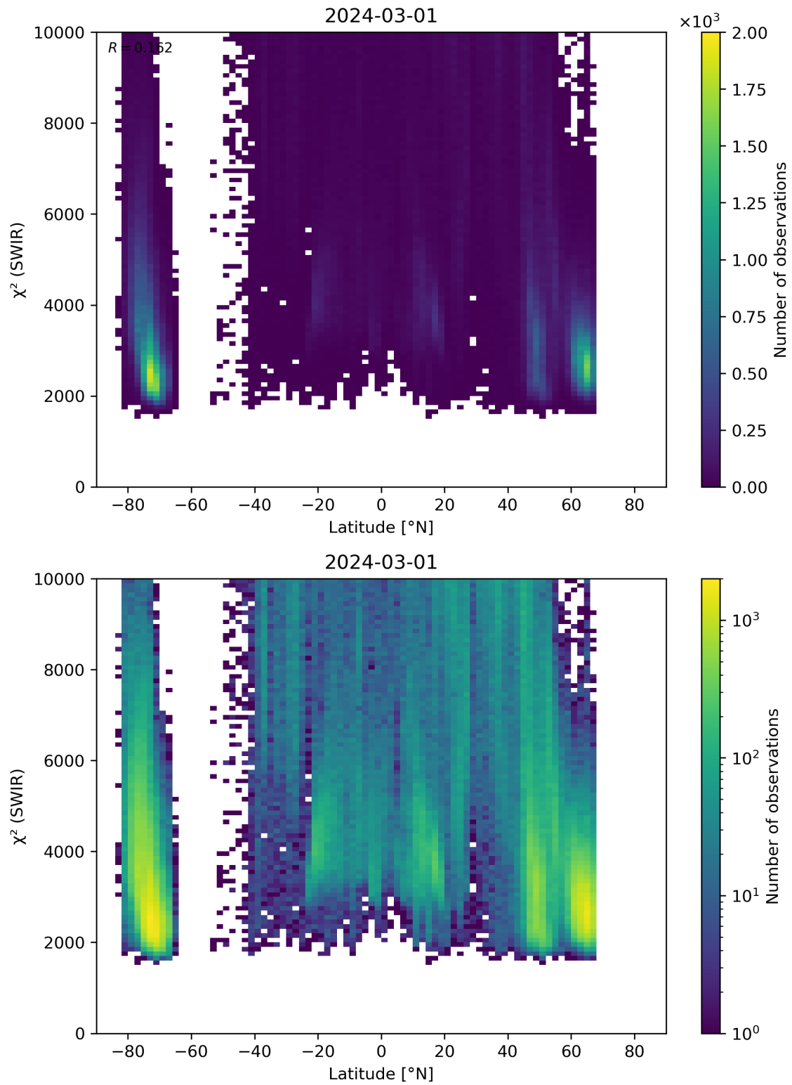
Figure 54: Scatter density plot of “Latitude” against “ \chi^2 (SWIR)” for 2024-02-29 to 2024-03-02.
