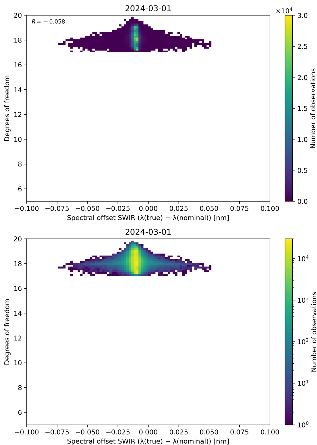
Figure 119: Scatter density plot of “Spectral offset SWIR ( \lambda(\text{true}) - \lambda(\text{nominal}) )” against “Degrees of freedom” for 2024-02-29 to 2024-03-02.
