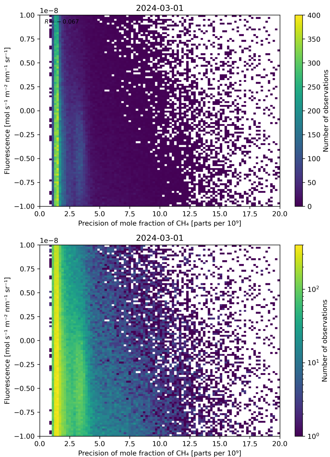
Figure 81: Scatter density plot of “Precision of mole fraction of \text{CH}_4 ” against “Fluorescence” for 2024-02-29 to 2024-03-02.
