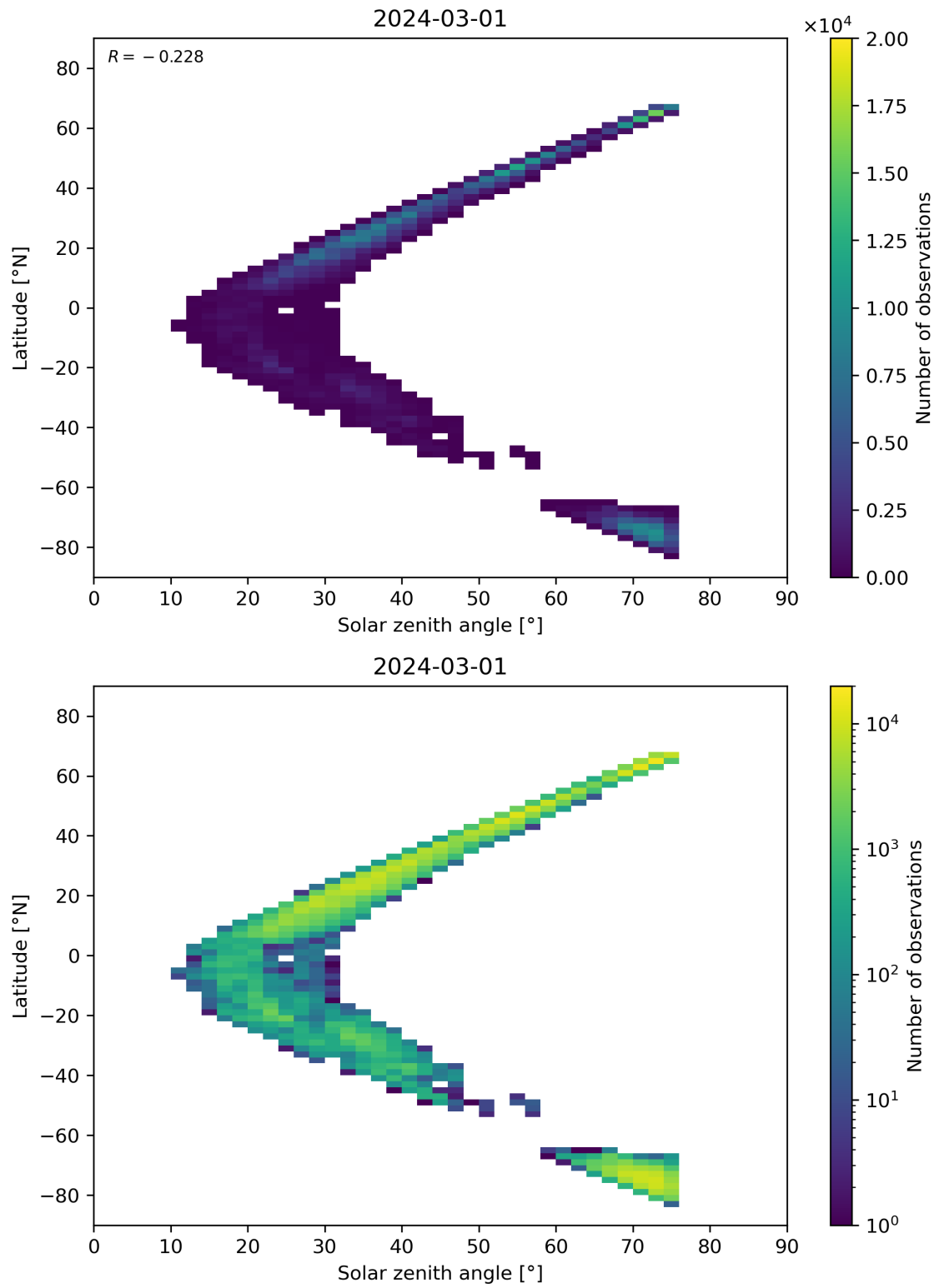
Figure 98: Scatter density plot of “Solar zenith angle” against “Latitude” for 2024-02-29 to 2024-03-02.
