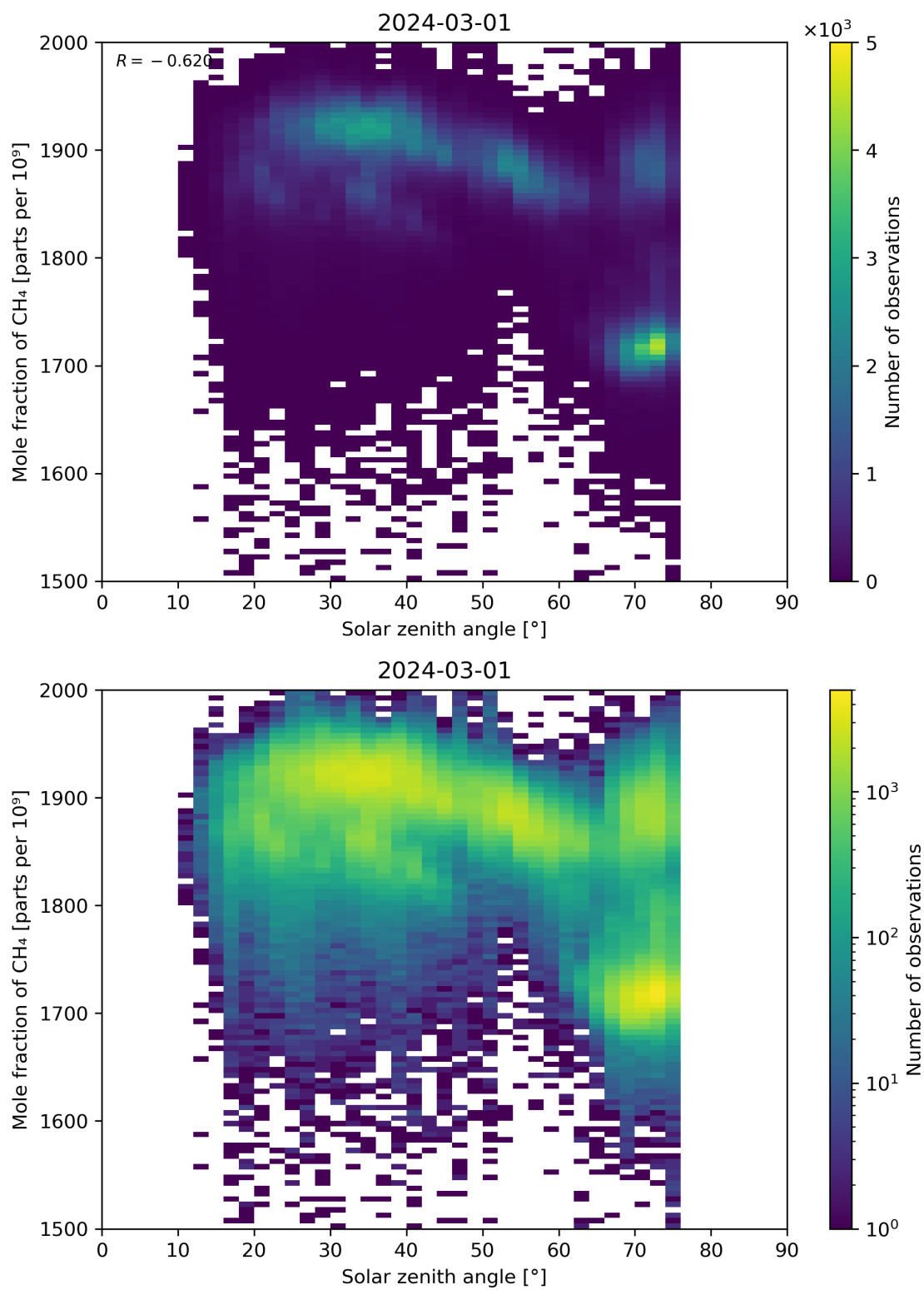
Figure 99: Scatter density plot of “Solar zenith angle” against “Mole fraction of CH 4 ” for 2024-02-29 to 2024-03-02.
