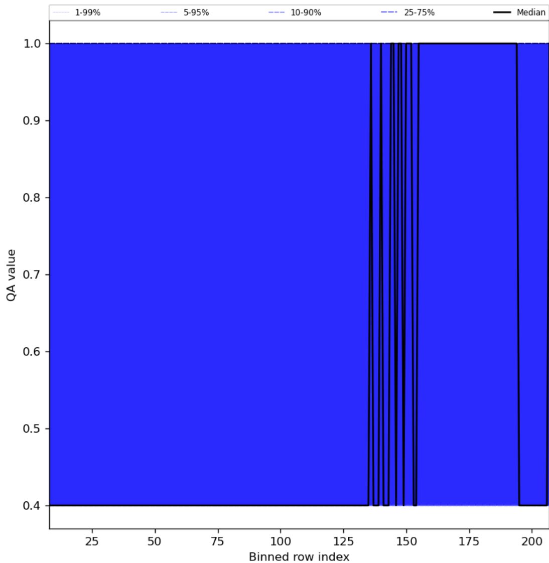
Figure 33: Along track statistics of “QA value” for 2024-02-29 to 2024-03-02
