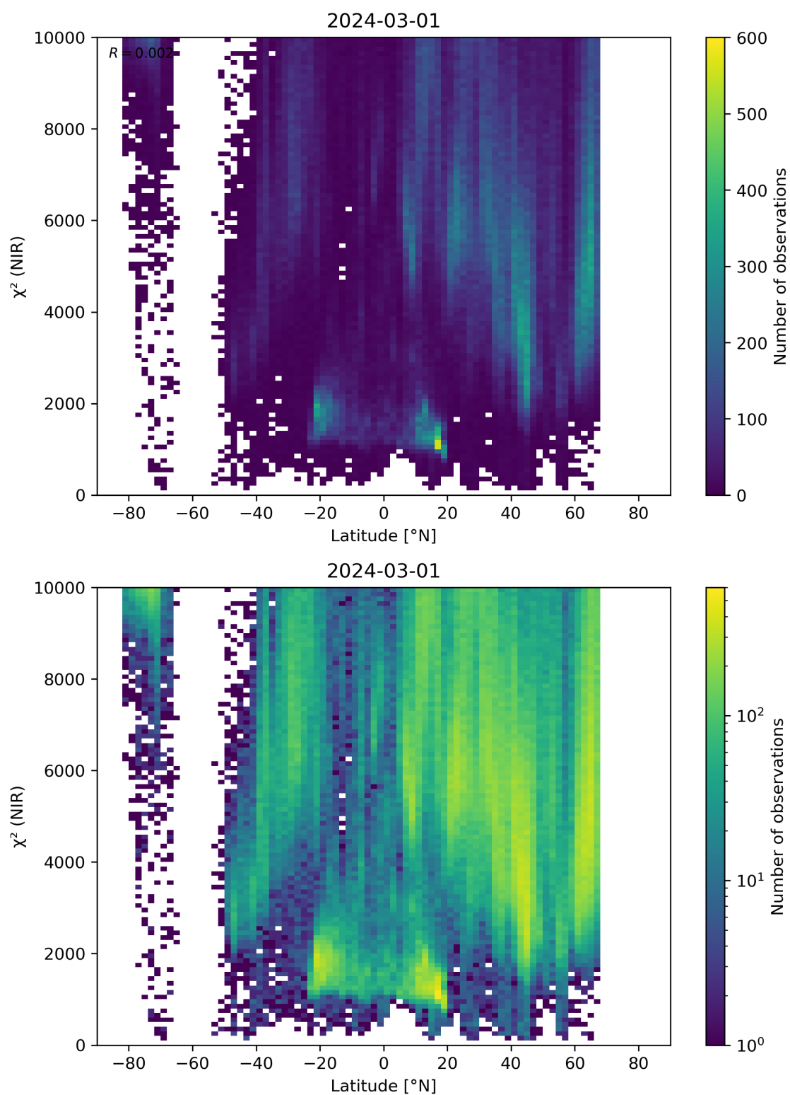
Figure 53: Scatter density plot of “Latitude” against “ \chi^2 (NIR)” for 2024-02-29 to 2024-03-02.
