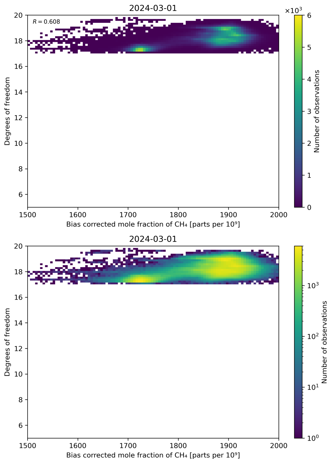
Figure 65: Scatter density plot of “Bias corrected mole fraction of CH 4 ” against “Degrees of freedom” for 2024-02-29 to 2024-03-02.
