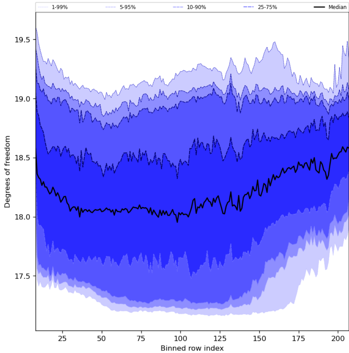
Figure 41: Along track statistics of “Degrees of freedom” for 2024-02-29 to 2024-03-02
