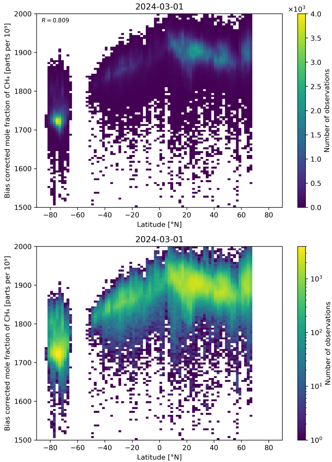
Figure 58: Scatter density plot of “Latitude” against “Bias corrected mole fraction of CH 4 ” for 2024-02-29 to 2024-03-02.
