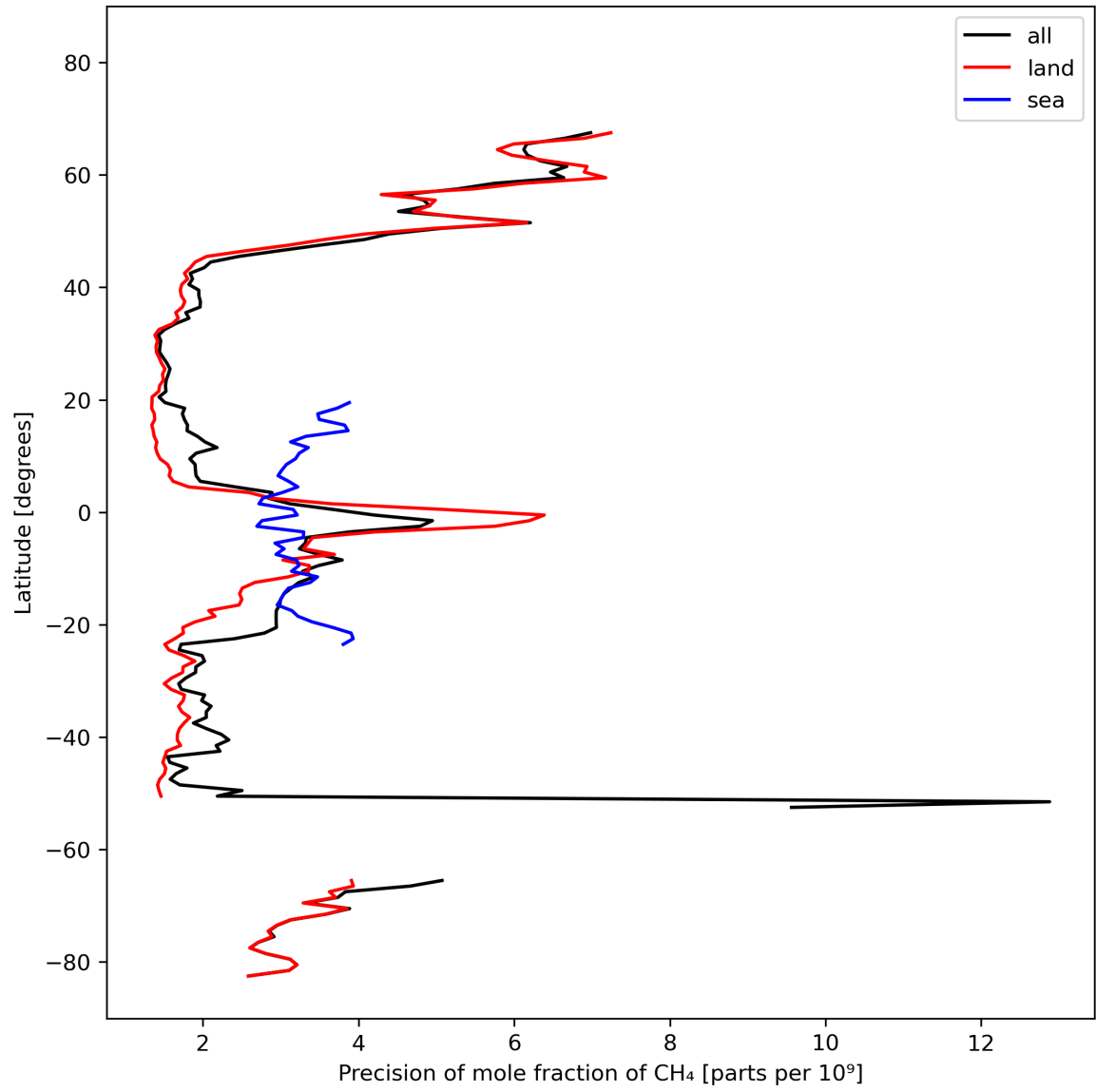
Figure 13: Zonal average of “Precision of mole fraction of CH 4 ” for 2024-02-29 to 2024-03-02.
