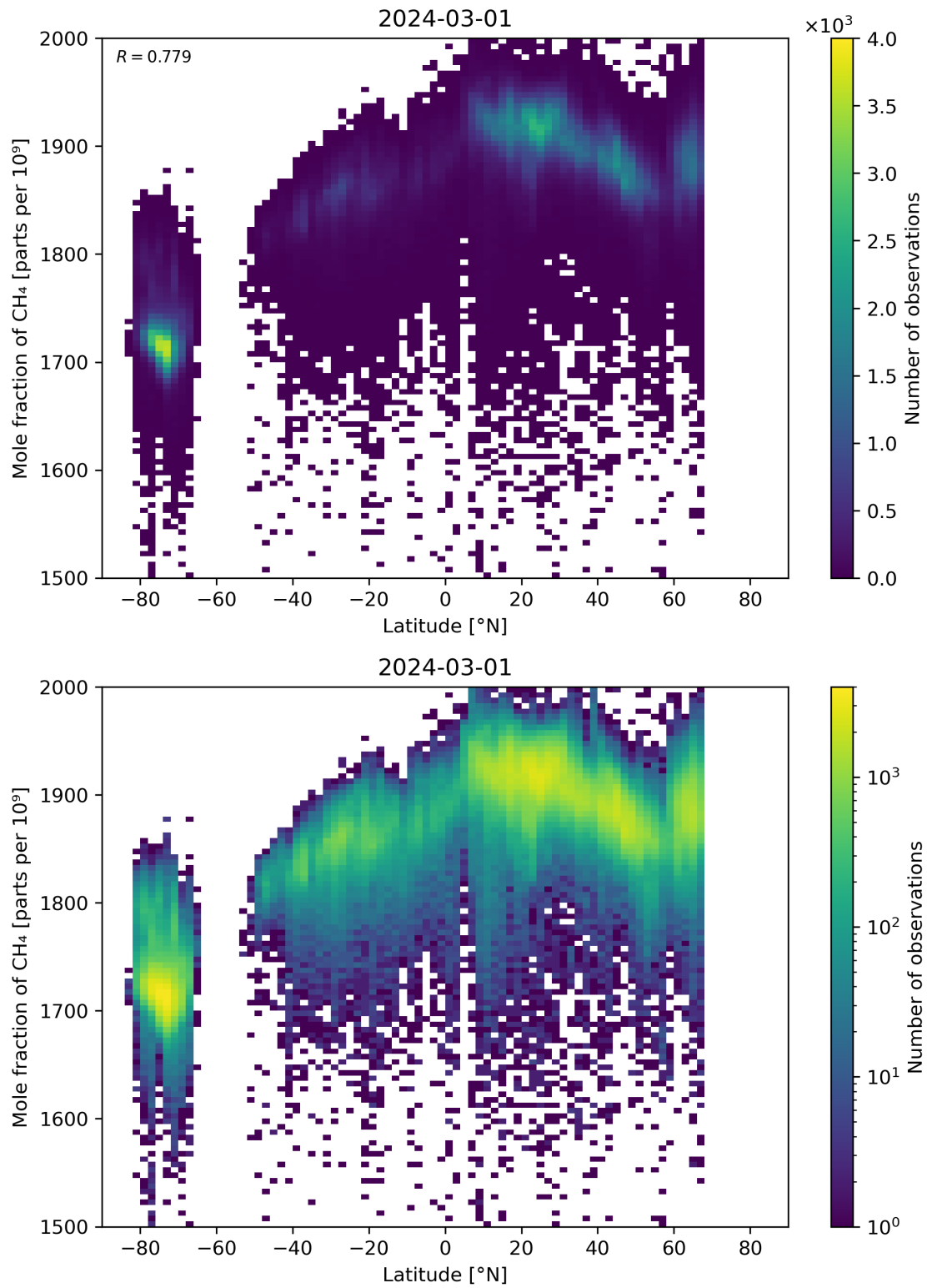
Figure 57: Scatter density plot of “Latitude” against “Mole fraction of CH 4 ” for 2024-02-29 to 2024-03-02.
