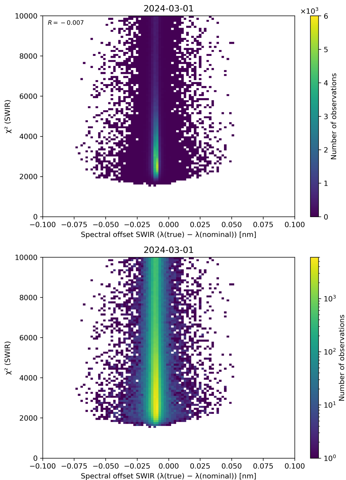
Figure 118: Scatter density plot of “Spectral offset SWIR ( \lambda(\text{true}) - \lambda(\text{nominal}) )” against “ \chi^2 (SWIR)” for 2024-02-29 to 2024-03-02.
