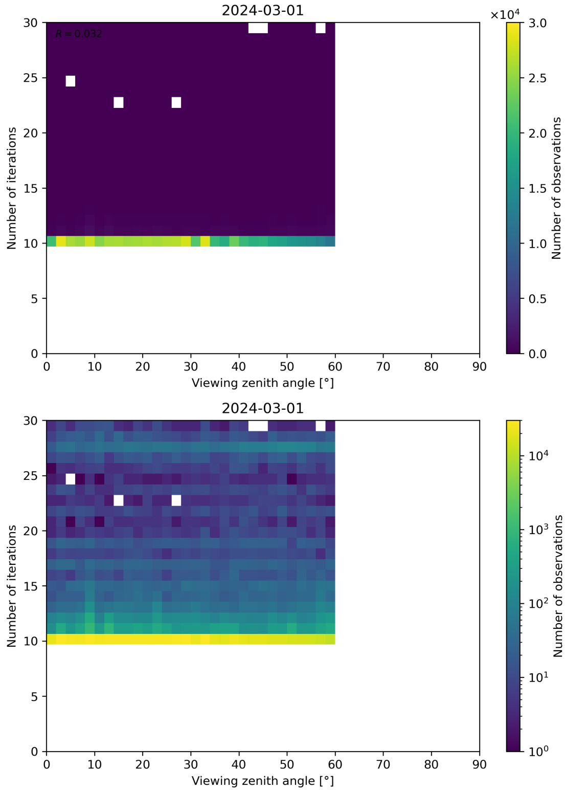
Figure 113: Scatter density plot of “Viewing zenith angle” against “Number of iterations” for 2024-02-29 to 2024-03-02.
