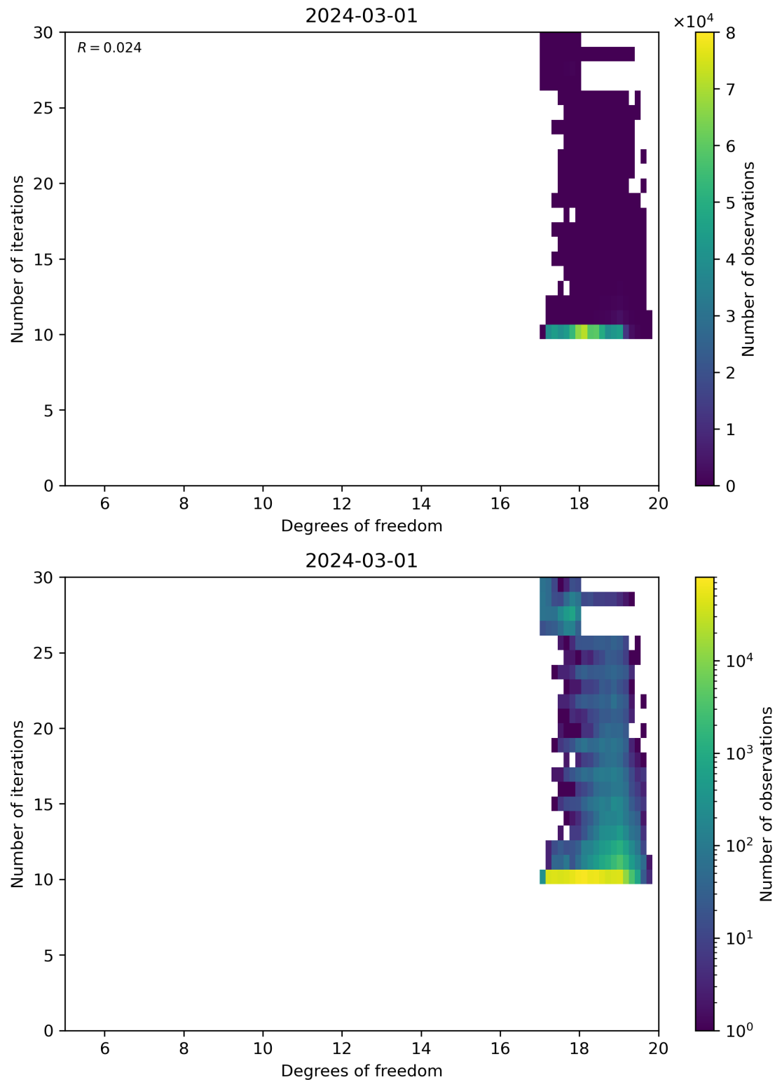
Figure 52: Scatter density plot of “Degrees of freedom” against “Number of iterations” for 2024-02-29 to 2024-03-02.
