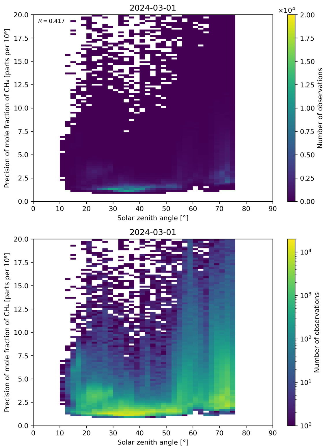
Figure 101: Scatter density plot of “Solar zenith angle” against “Precision of mole fraction of CH 4 ” for 2024-02-29 to 2024-03-02.
