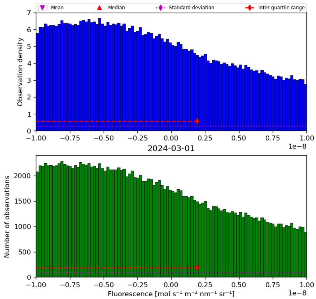
Figure 32: Histogram of “Fluorescence” for 2024-02-29 to 2024-03-02
