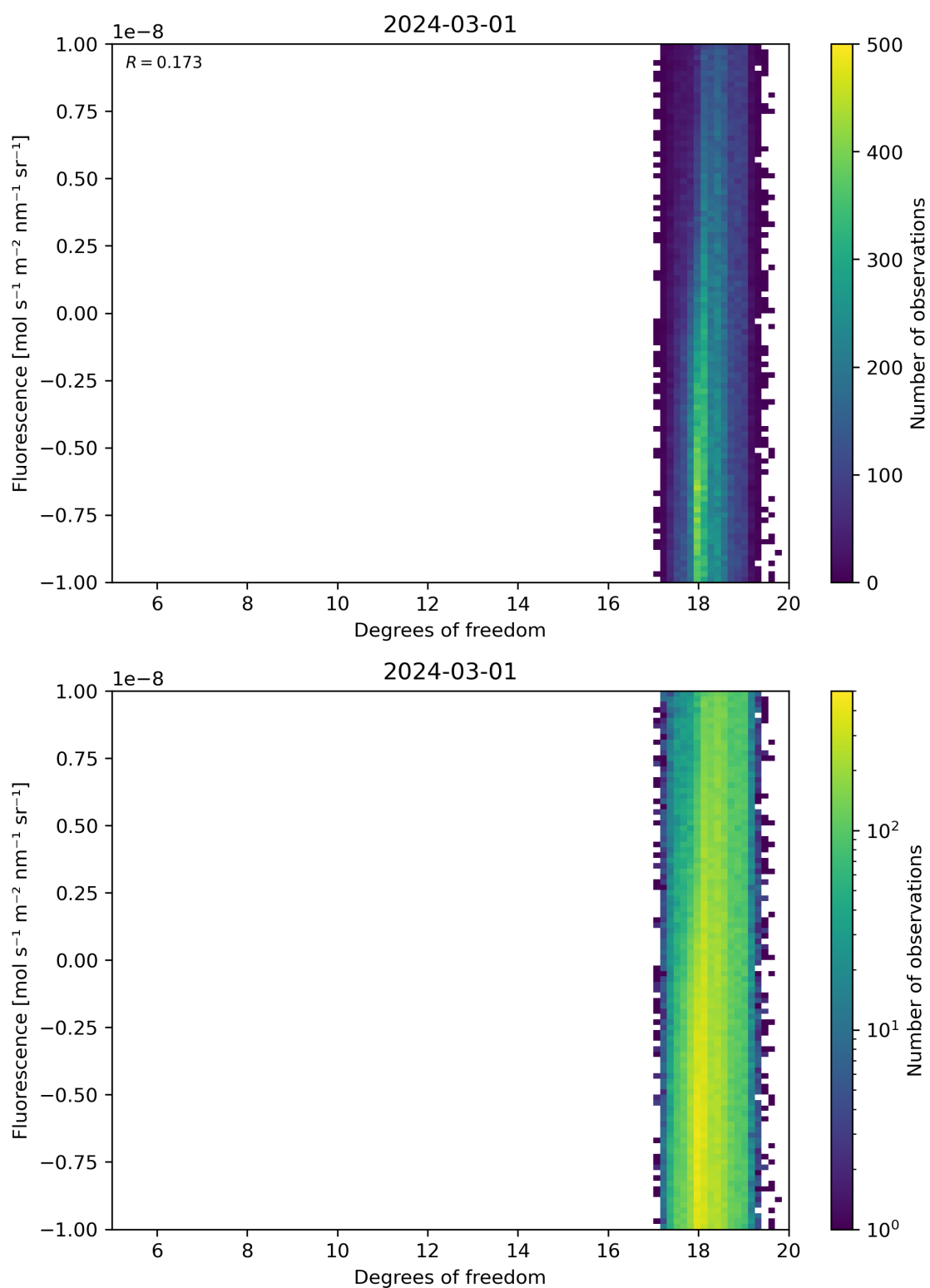
Figure 51: Scatter density plot of “Degrees of freedom” against “Fluorescence” for 2024-02-29 to 2024-03-02.
