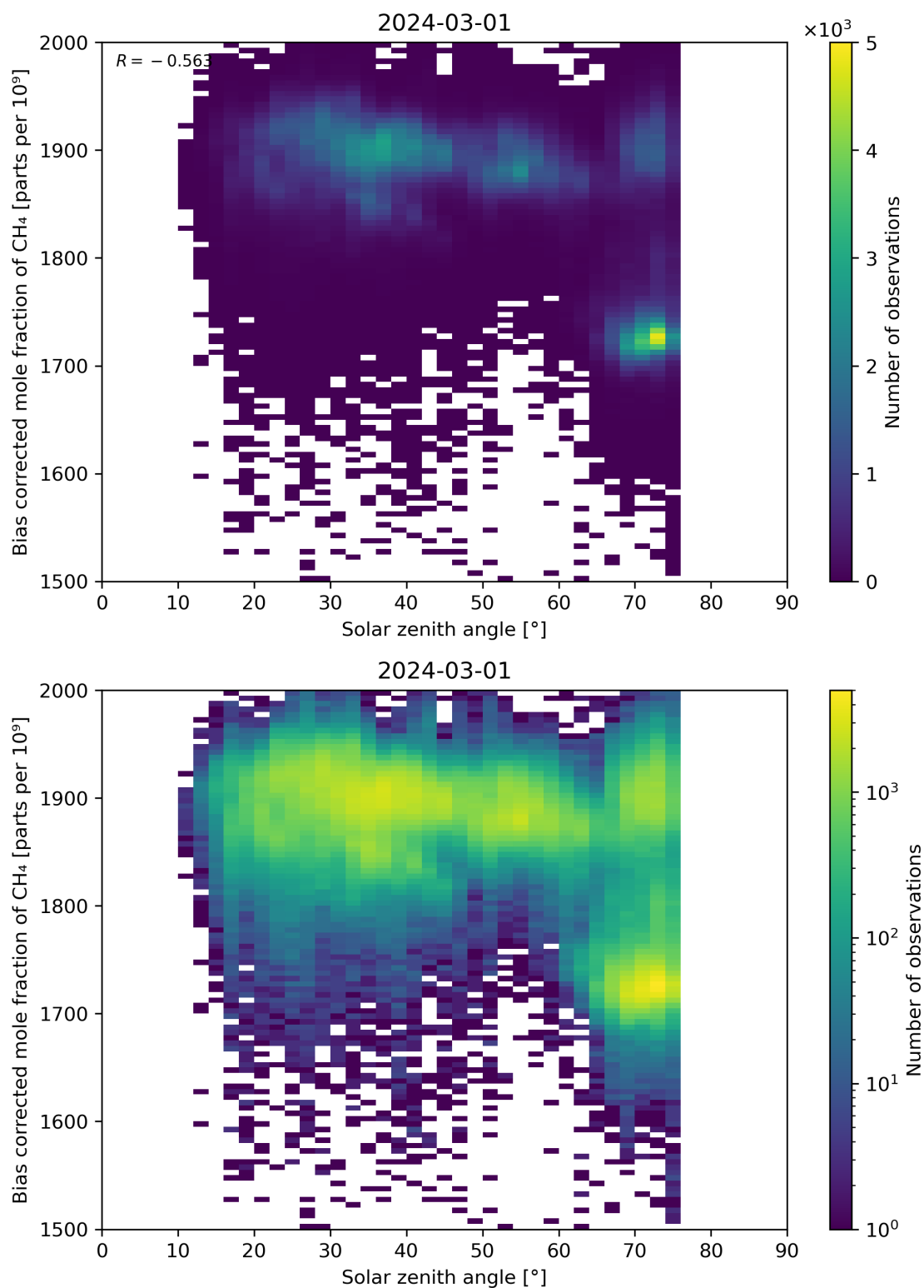
Figure 100: Scatter density plot of “Solar zenith angle” against “Bias corrected mole fraction of CH 4 ” for 2024-02-29 to 2024-03-02.
