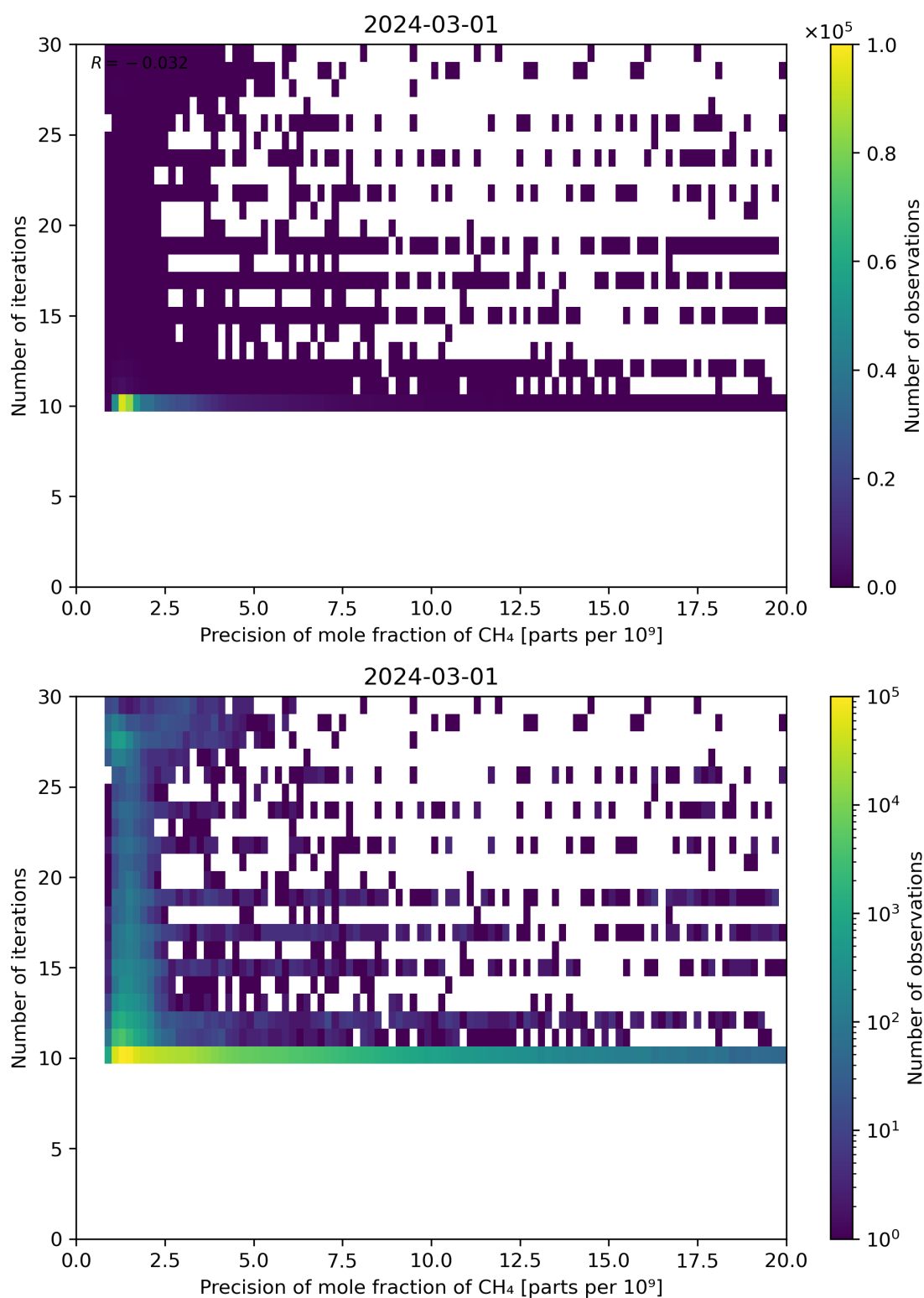
Figure 83: Scatter density plot of “Precision of mole fraction of CH 4 ” against “Number of iterations” for 2024-02-29 to 2024-03-02.
