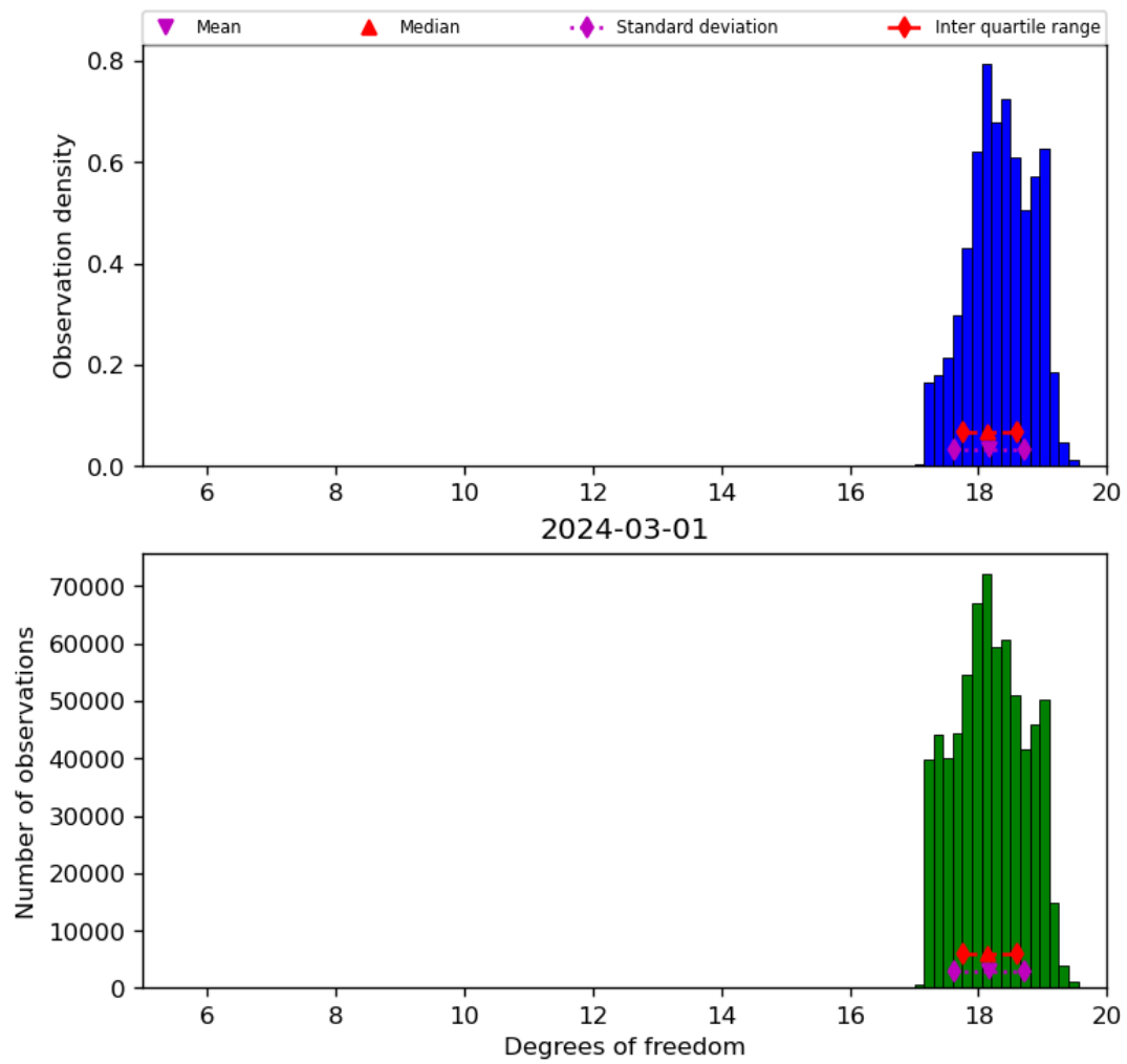
Figure 30: Histogram of “Degrees of freedom” for 2024-02-29 to 2024-03-02
