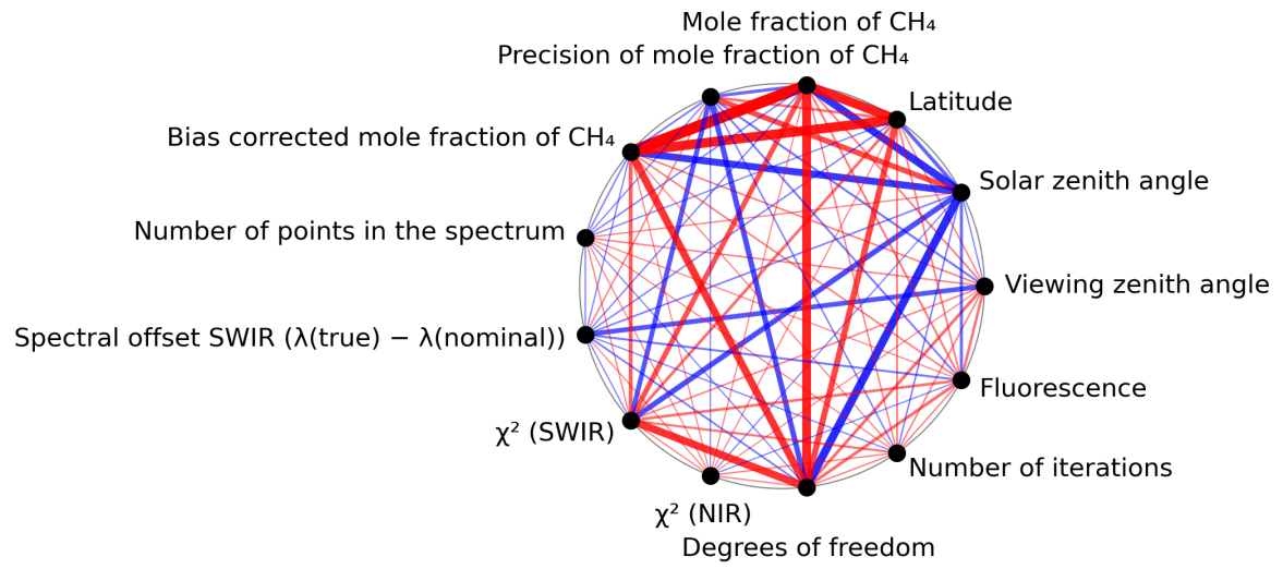
Figure 1: Map of correlation graph for 2024-02-29 to 2024-03-02.
