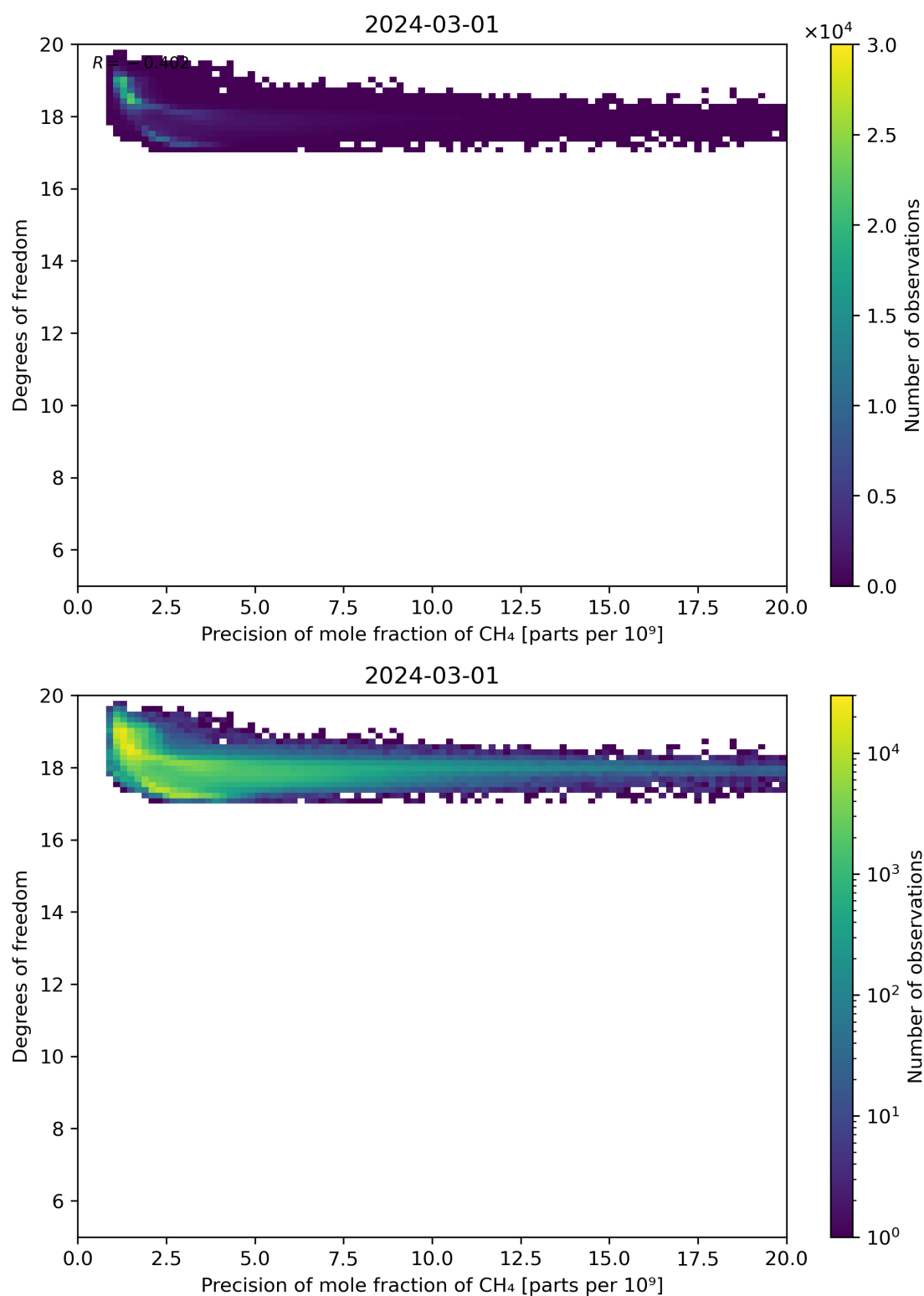
Figure 80: Scatter density plot of “Precision of mole fraction of CH 4 ” against “Degrees of freedom” for 2024-02-29 to 2024-03-02.
