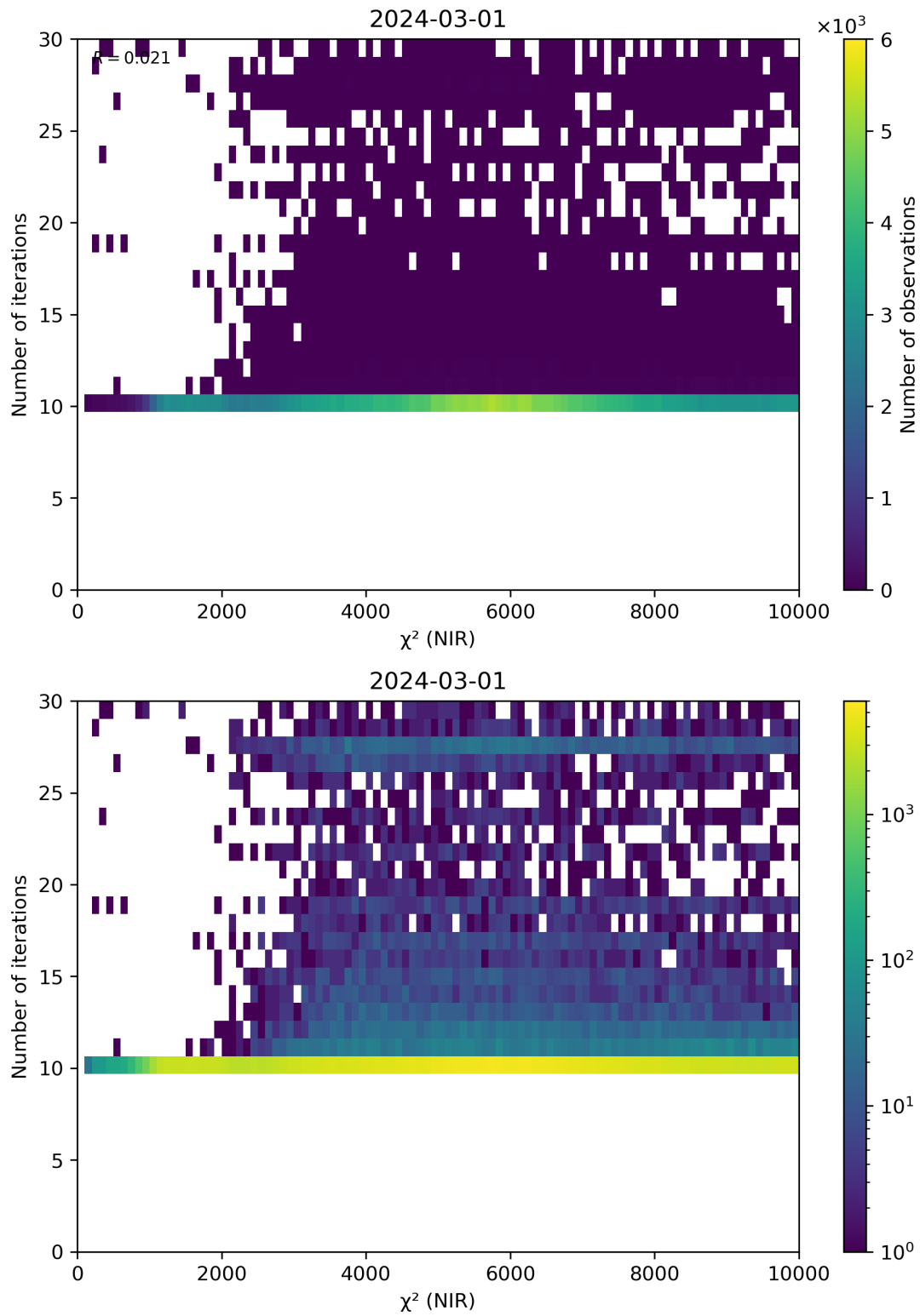
Figure 46: Scatter density plot of “ \chi^2 (NIR)” against “Number of iterations” for 2024-02-29 to 2024-03-02.
