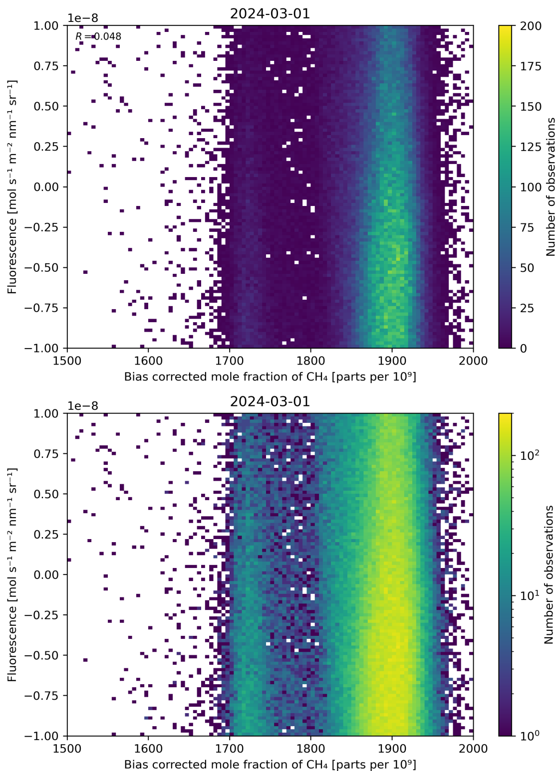
Figure 66: Scatter density plot of “Bias corrected mole fraction of CH 4 ” against “Fluorescence” for 2024-02-29 to 2024-03-02.
