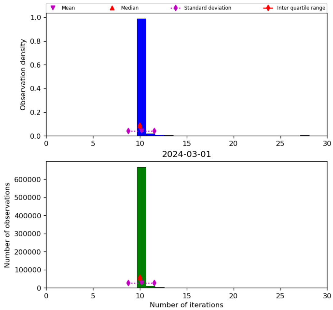
Figure 31: Histogram of “Number of iterations” for 2024-02-29 to 2024-03-02
