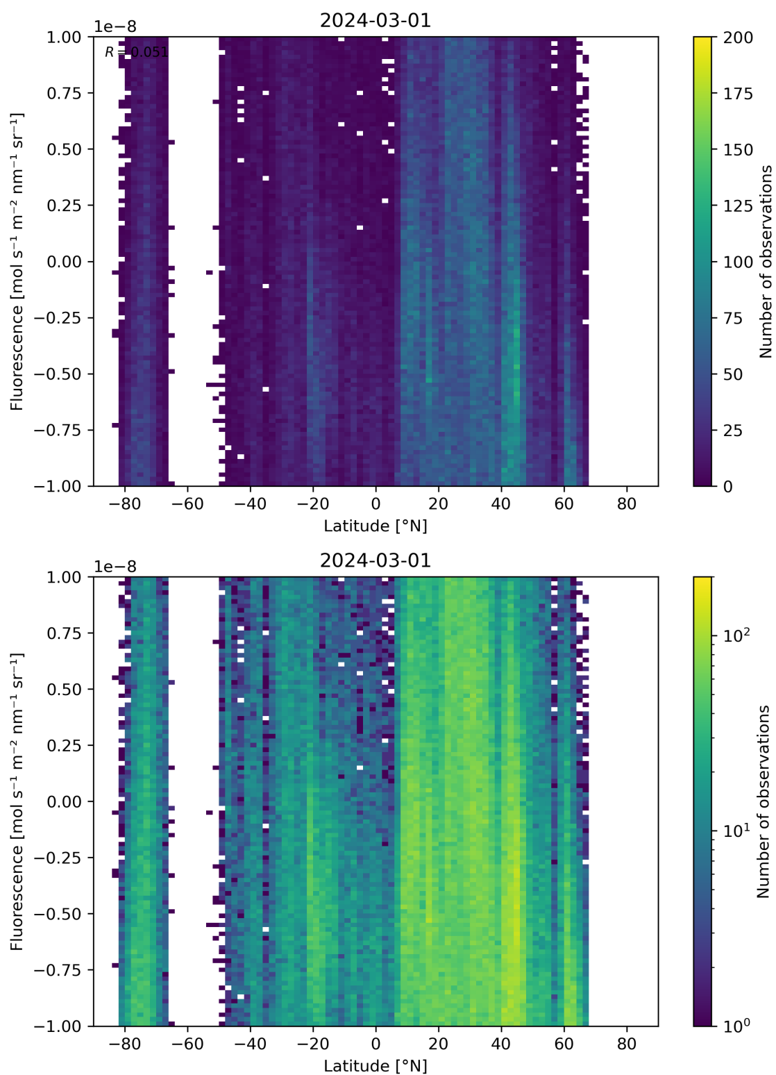
Figure 56: Scatter density plot of “Latitude” against “Fluorescence” for 2024-02-29 to 2024-03-02.
