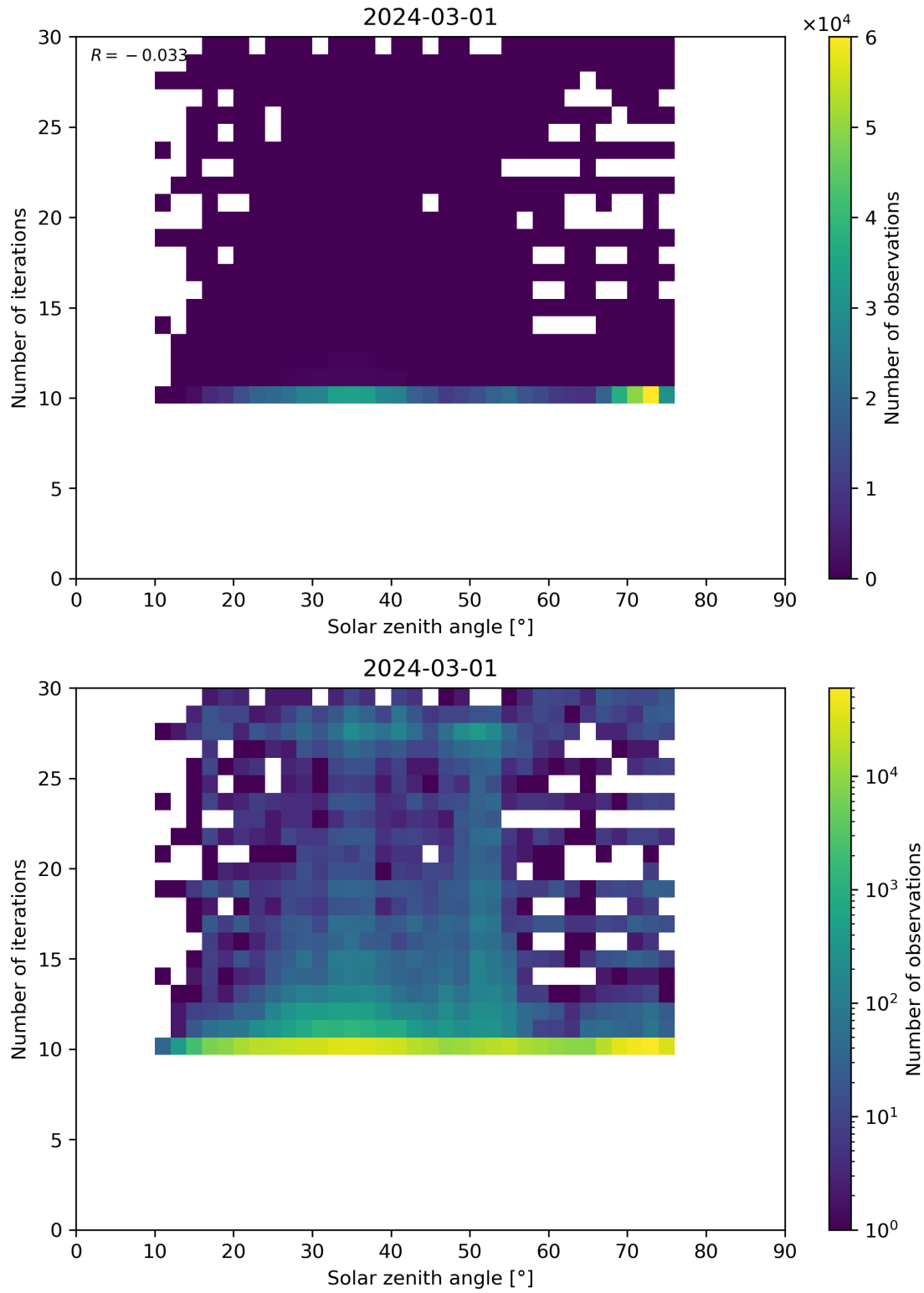
Figure 102: Scatter density plot of “Solar zenith angle” against “Number of iterations” for 2024-02-29 to 2024-03-02.
