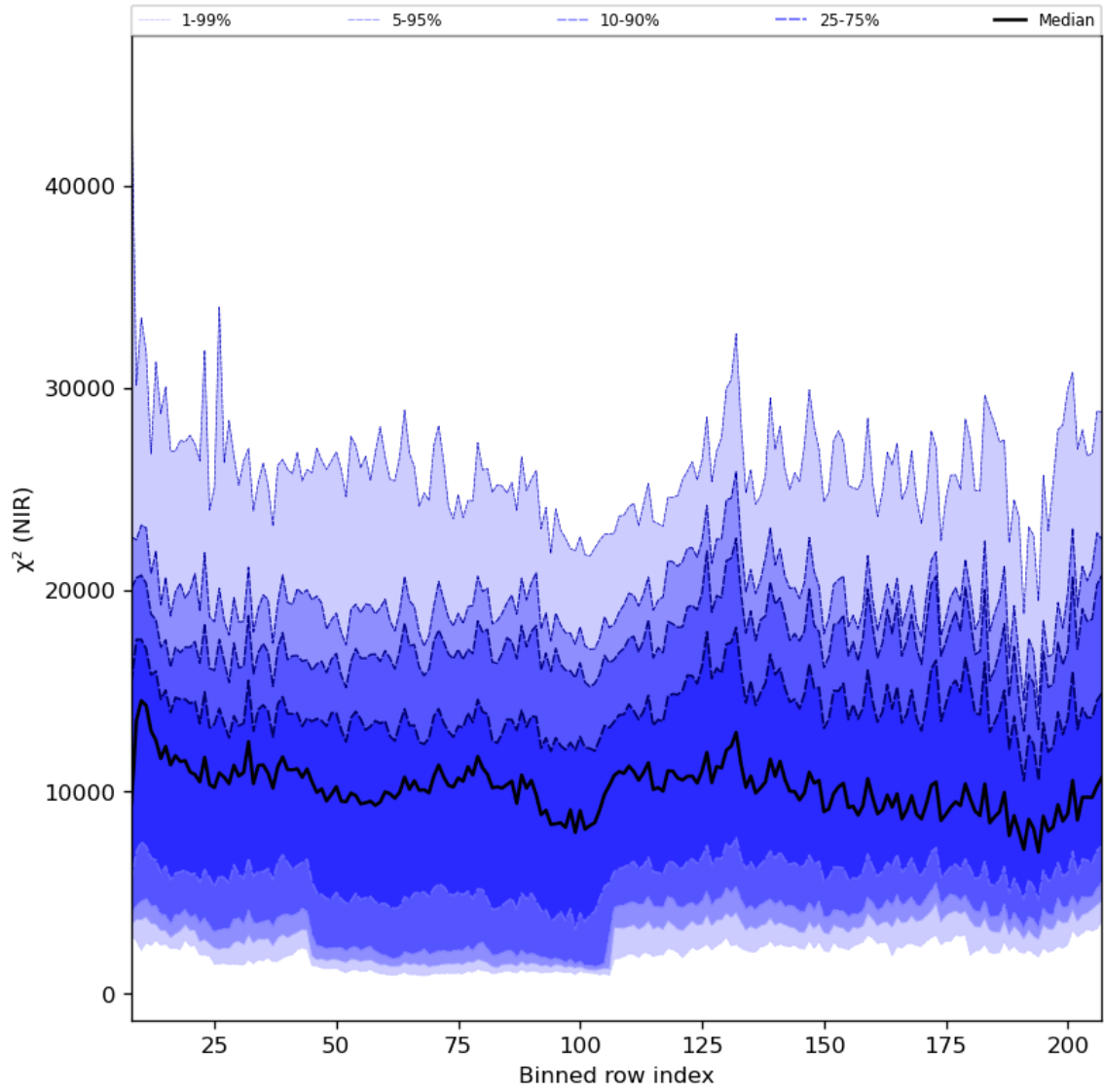
Figure 40: Along track statistics of “ \chi^2 (NIR)” for 2024-02-29 to 2024-03-02
