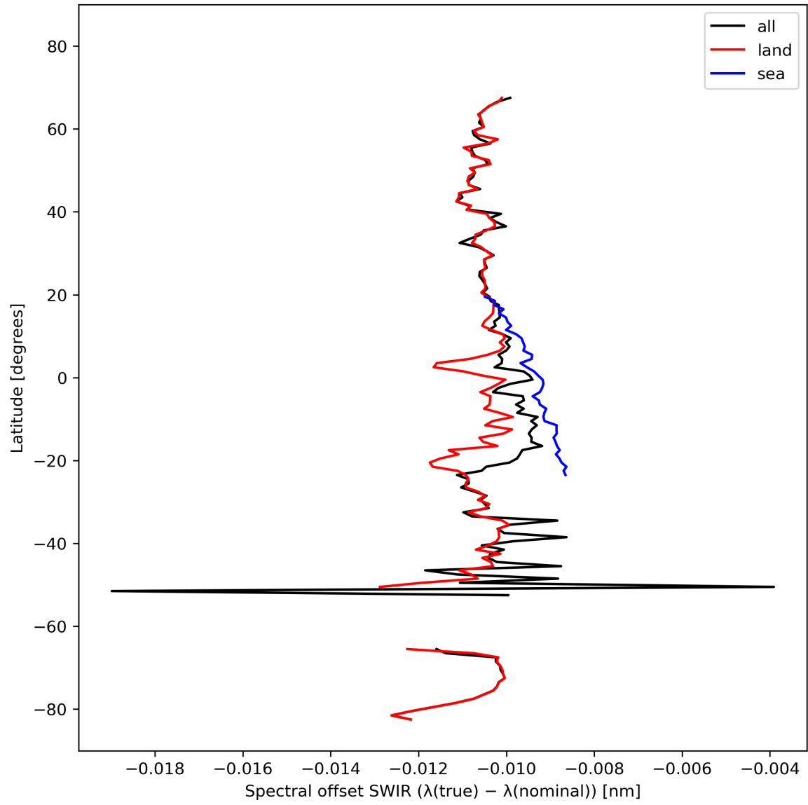
Figure 16: Zonal average of “Spectral offset SWIR ( \lambda(\text{true}) - \lambda(\text{nominal}) )” for 2024-02-29 to 2024-03-02.
