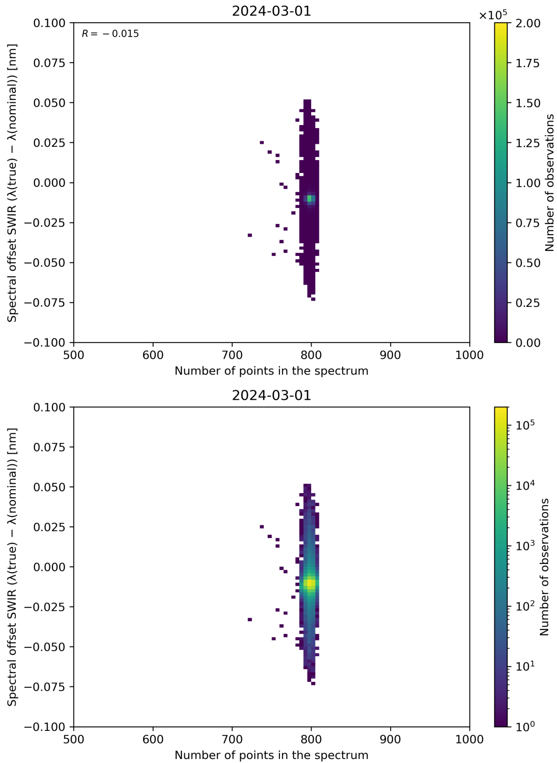
Figure 93: Scatter density plot of “Number of points in the spectrum” against “Spectral offset SWIR ( \lambda(\text{true}) - \lambda(\text{nominal}) )” for 2024-02-29 to 2024-03-02.
