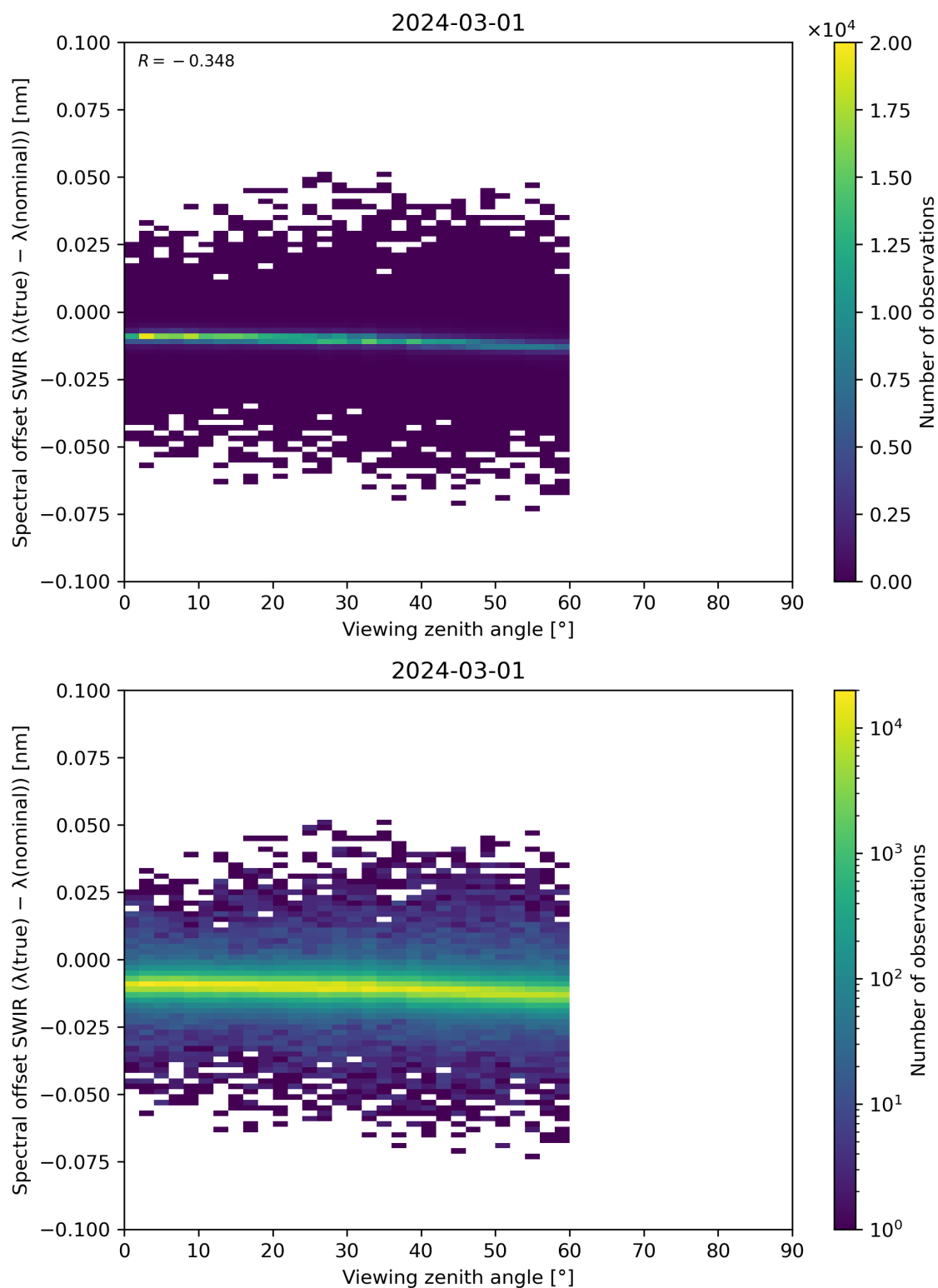
Figure 116: Scatter density plot of “Viewing zenith angle” against “Spectral offset SWIR ( \lambda(\text{true}) - \lambda(\text{nominal}) )” for 2024-02-29 to 2024-03-02.
