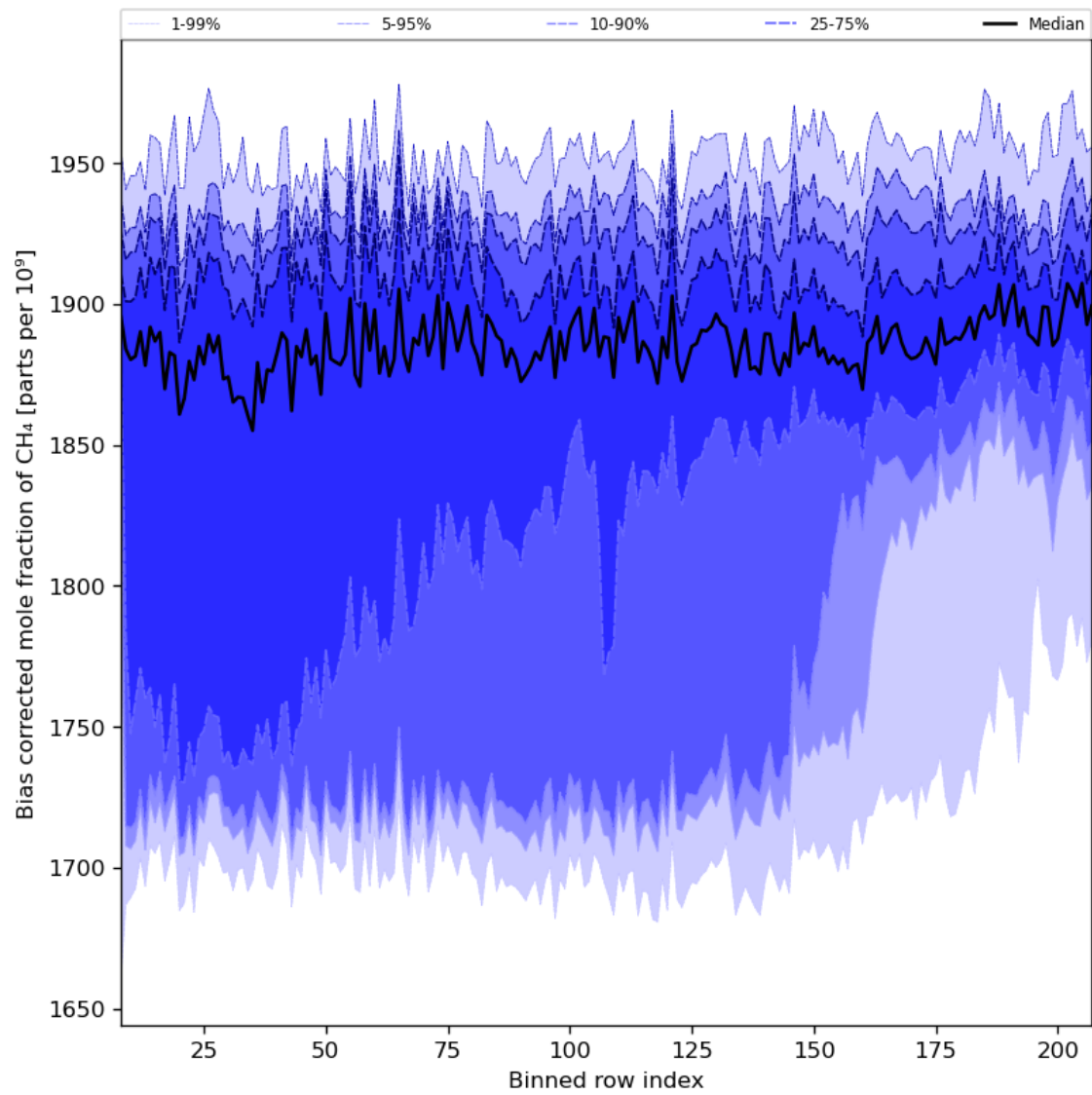
Figure 36: Along track statistics of “Bias corrected mole fraction of CH 4 ” for 2024-02-29 to 2024-03-02
