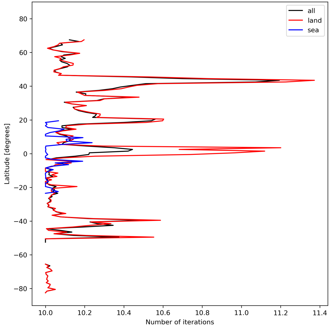
Figure 20: Zonal average of “Number of iterations” for 2024-02-29 to 2024-03-02.
