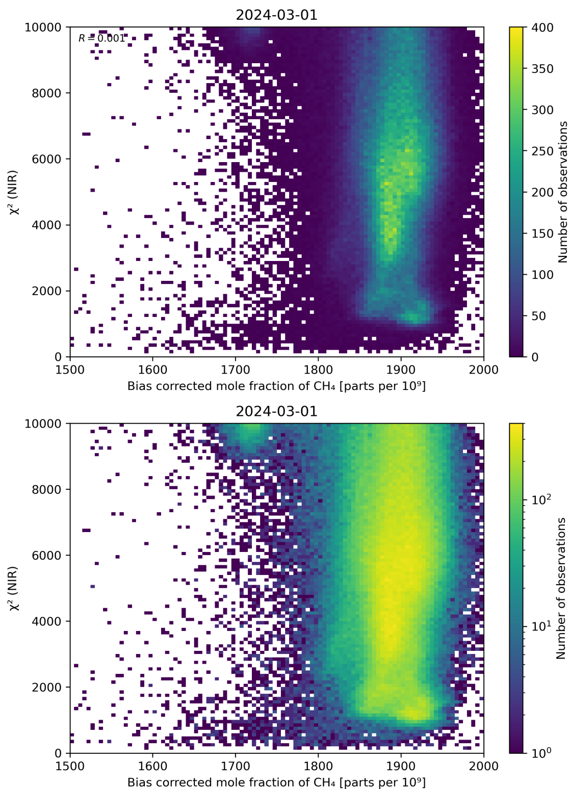
Figure 63: Scatter density plot of “Bias corrected mole fraction of CH 4 ” against “ \chi^2 (NIR)” for 2024-02-29 to 2024-03-02.
