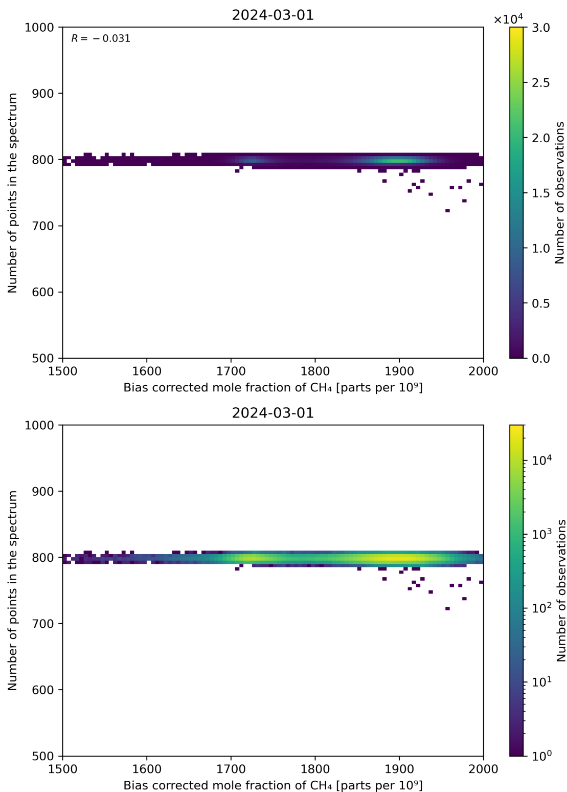
Figure 68: Scatter density plot of “Bias corrected mole fraction of CH 4 ” against “Number of points in the spectrum” for 2024-02-29 to 2024-03-02.
