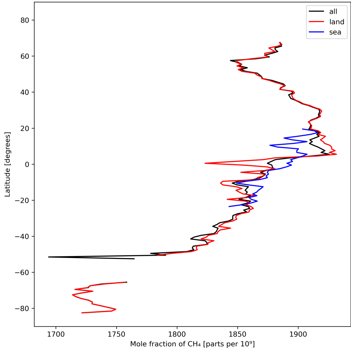
Figure 12: Zonal average of “Mole fraction of CH 4 ” for 2024-02-29 to 2024-03-02.
