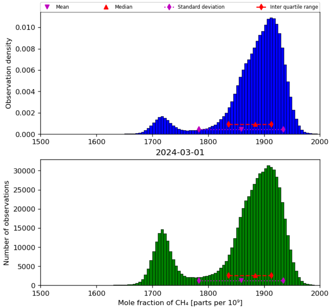
Figure 23: Histogram of “Mole fraction of CH 4 ” for 2024-02-29 to 2024-03-02
