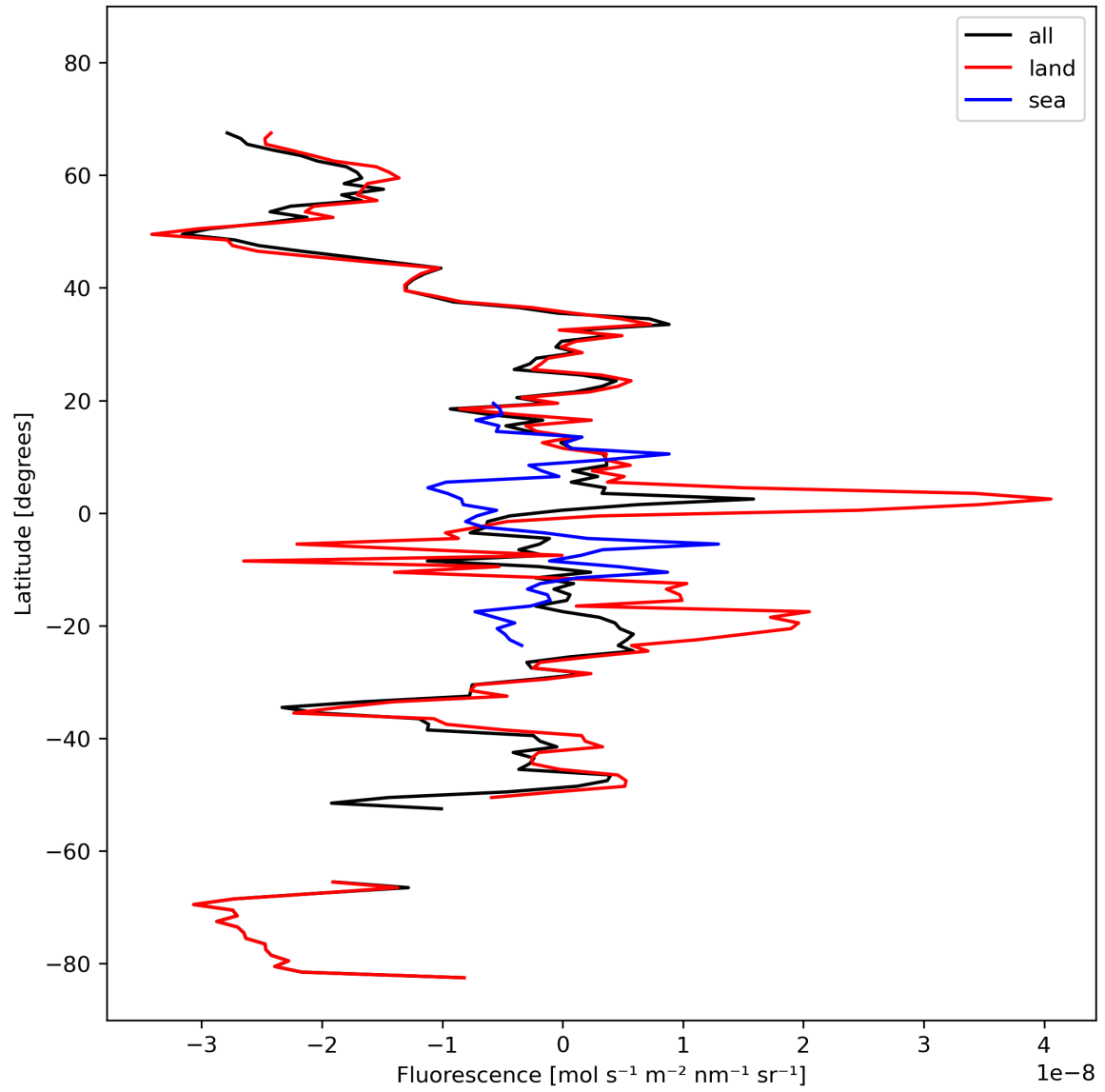
Figure 21: Zonal average of “Fluorescence” for 2024-02-29 to 2024-03-02.
