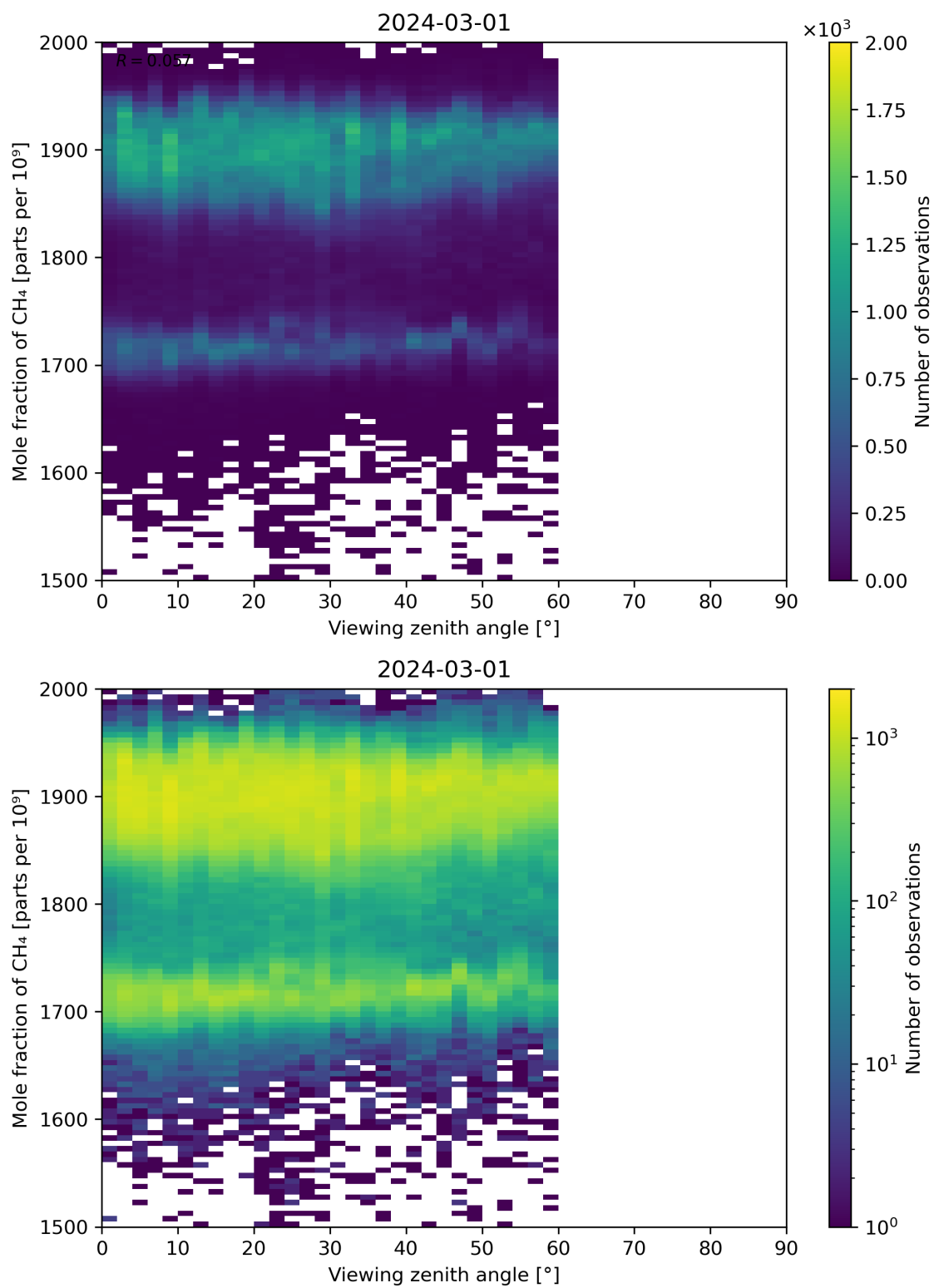
Figure 110: Scatter density plot of “Viewing zenith angle” against “Mole fraction of CH 4 ” for 2024-02-29 to 2024-03-02.
