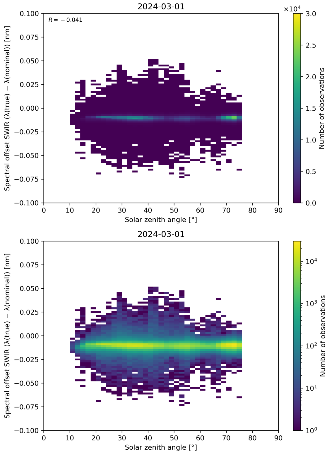
Figure 104: Scatter density plot of “Solar zenith angle” against “Spectral offset SWIR ( \lambda(\text{true}) - \lambda(\text{nominal}) )” for 2024-02-29 to 2024-03-02.
