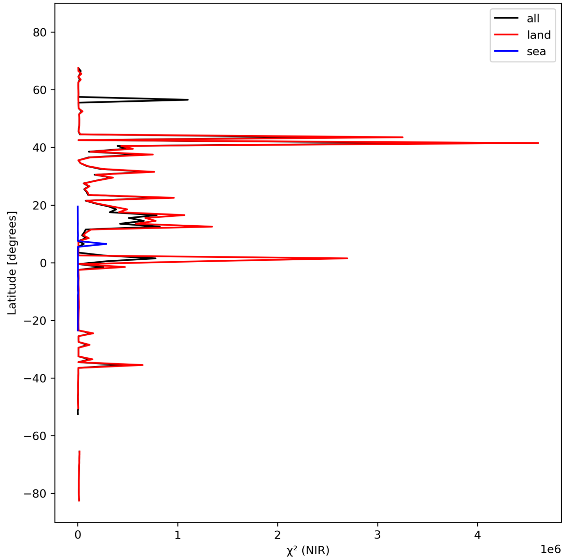
Figure 18: Zonal average of “ \chi^2 (NIR)” for 2024-02-29 to 2024-03-02.
