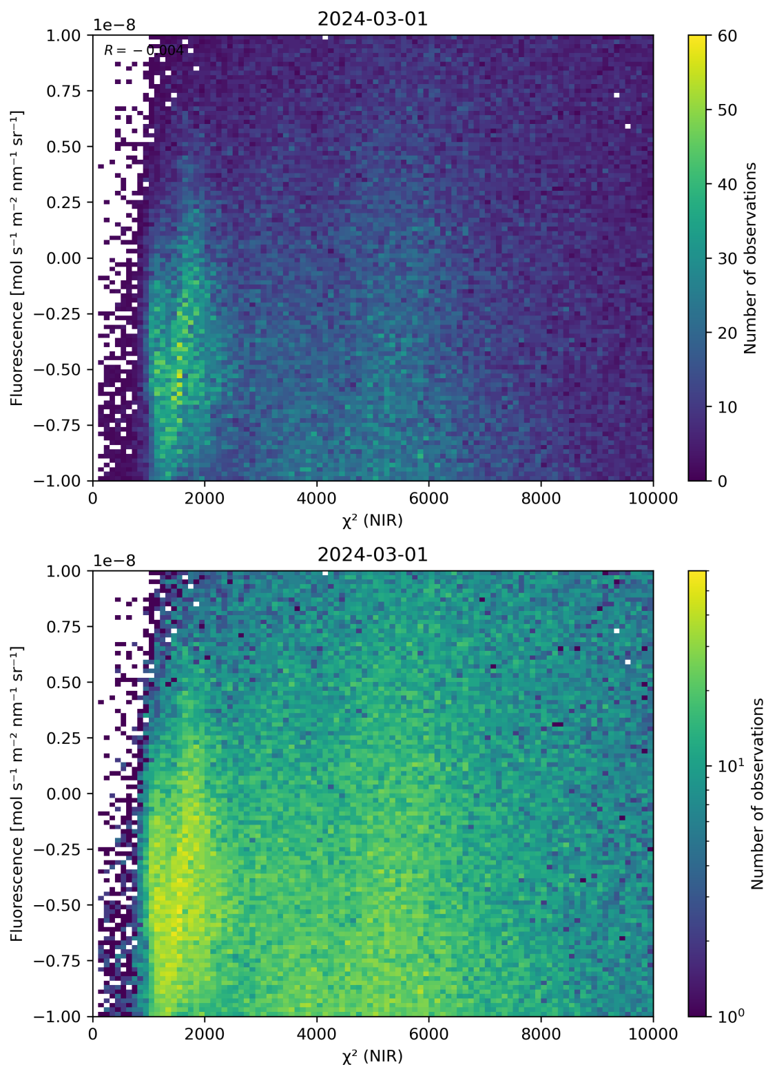
Figure 45: Scatter density plot of “ \chi^2 (NIR)” against “Fluorescence” for 2024-02-29 to 2024-03-02.
