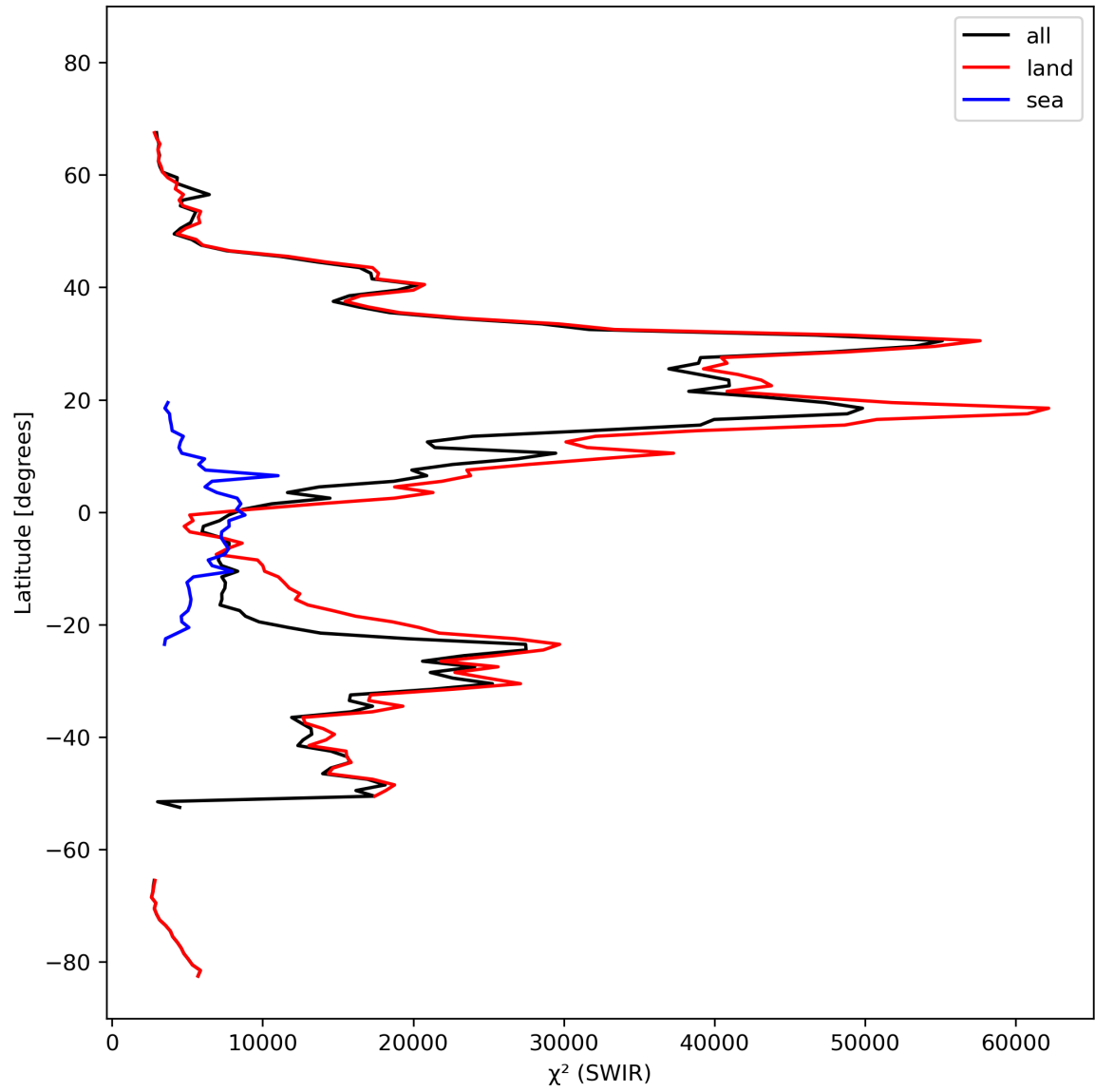
Figure 17: Zonal average of “ \chi^2 (SWIR)” for 2024-02-29 to 2024-03-02.
