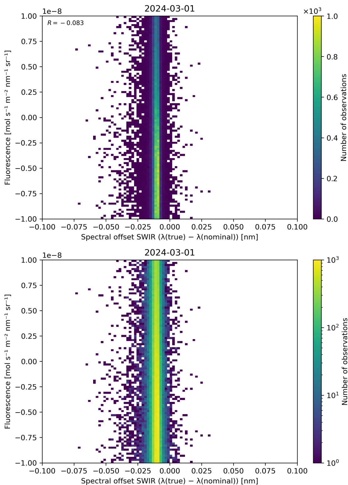
Figure 120: Scatter density plot of “Spectral offset SWIR ( \lambda(\text{true}) - \lambda(\text{nominal}) )” against “Fluorescence” for 2024-02-29 to 2024-03-02.
