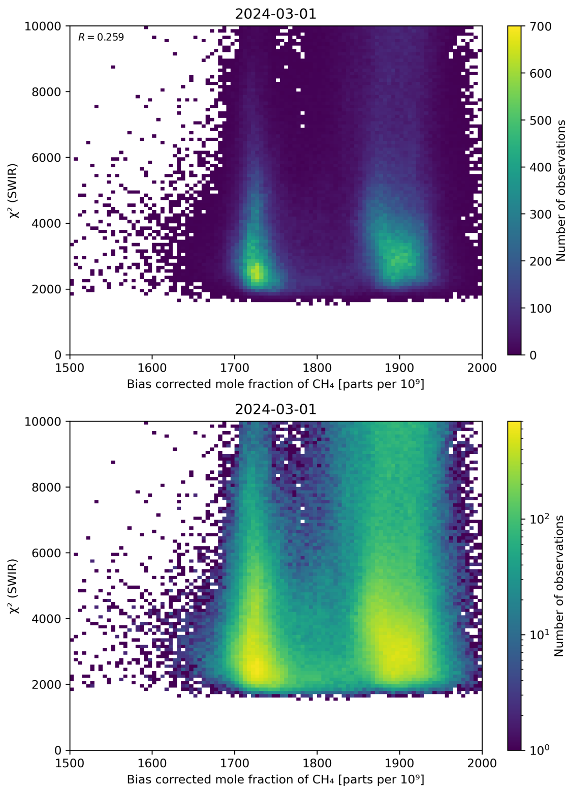
Figure 64: Scatter density plot of “Bias corrected mole fraction of CH 4 ” against “ \chi^2 (SWIR)” for 2024-02-29 to 2024-03-02.
