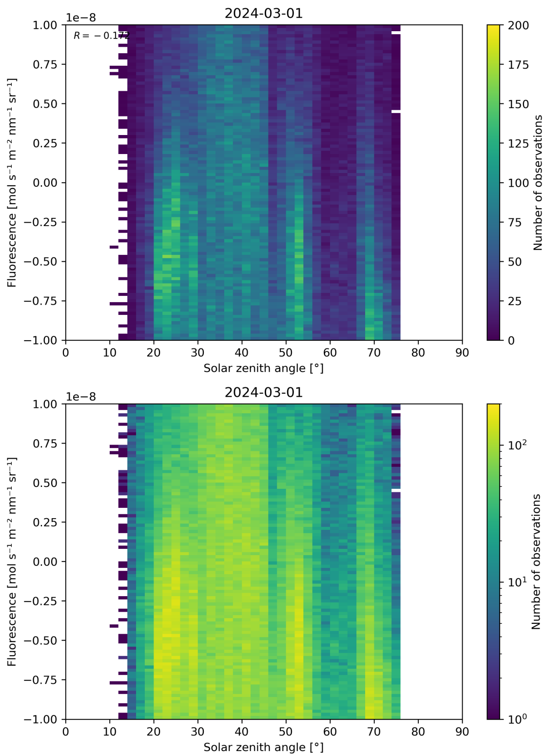
Figure 97: Scatter density plot of “Solar zenith angle” against “Fluorescence” for 2024-02-29 to 2024-03-02.
