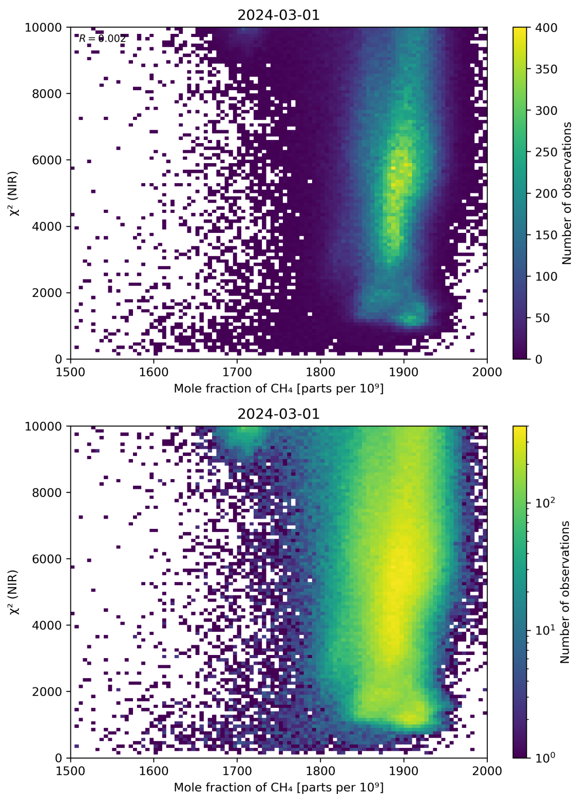
Figure 70: Scatter density plot of “Mole fraction of CH 4 ” against “ \chi^2 (NIR)” for 2024-02-29 to 2024-03-02.
