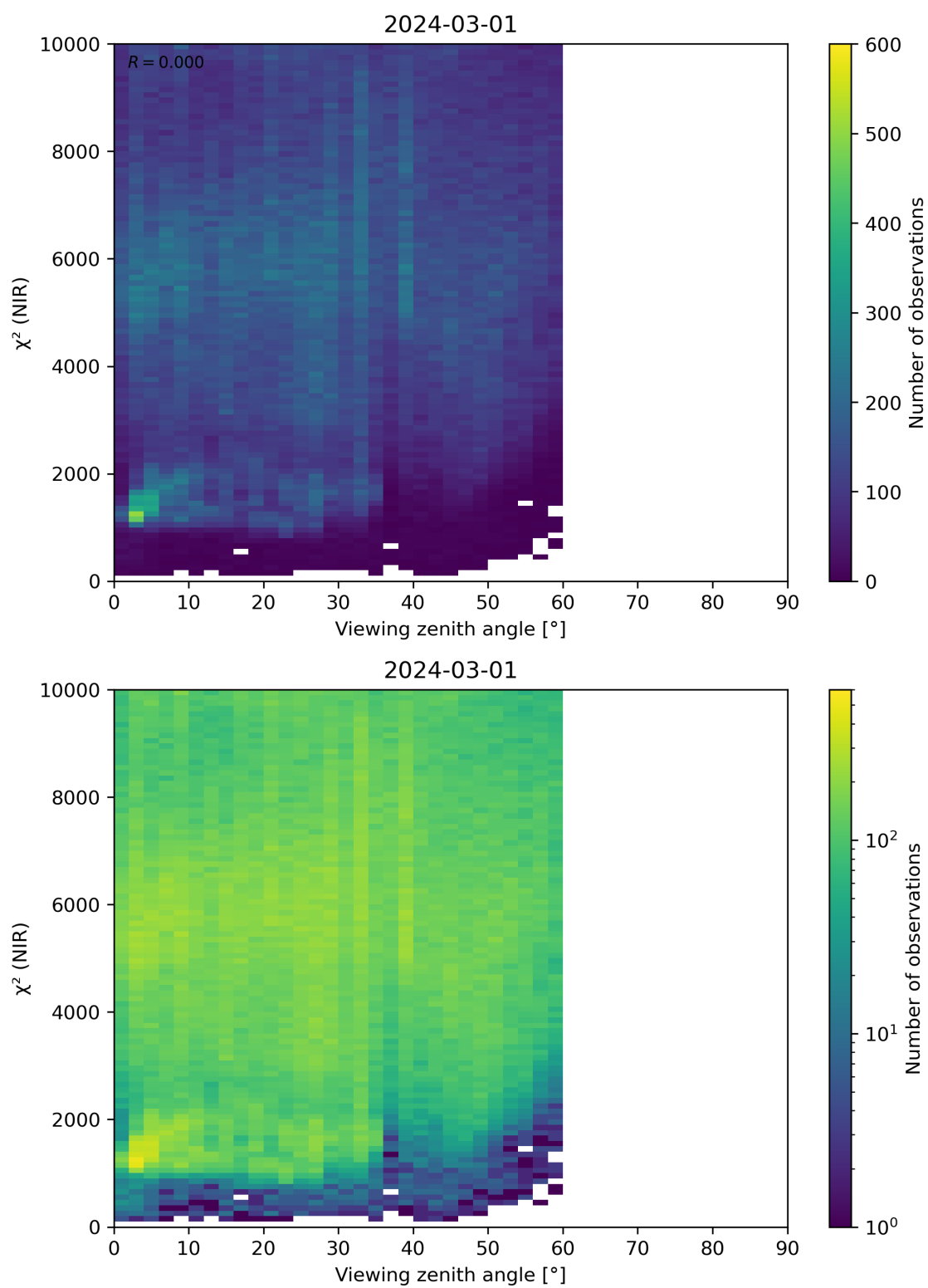
Figure 105: Scatter density plot of “Viewing zenith angle” against “ \chi^2 (NIR)” for 2024-02-29 to 2024-03-02.
