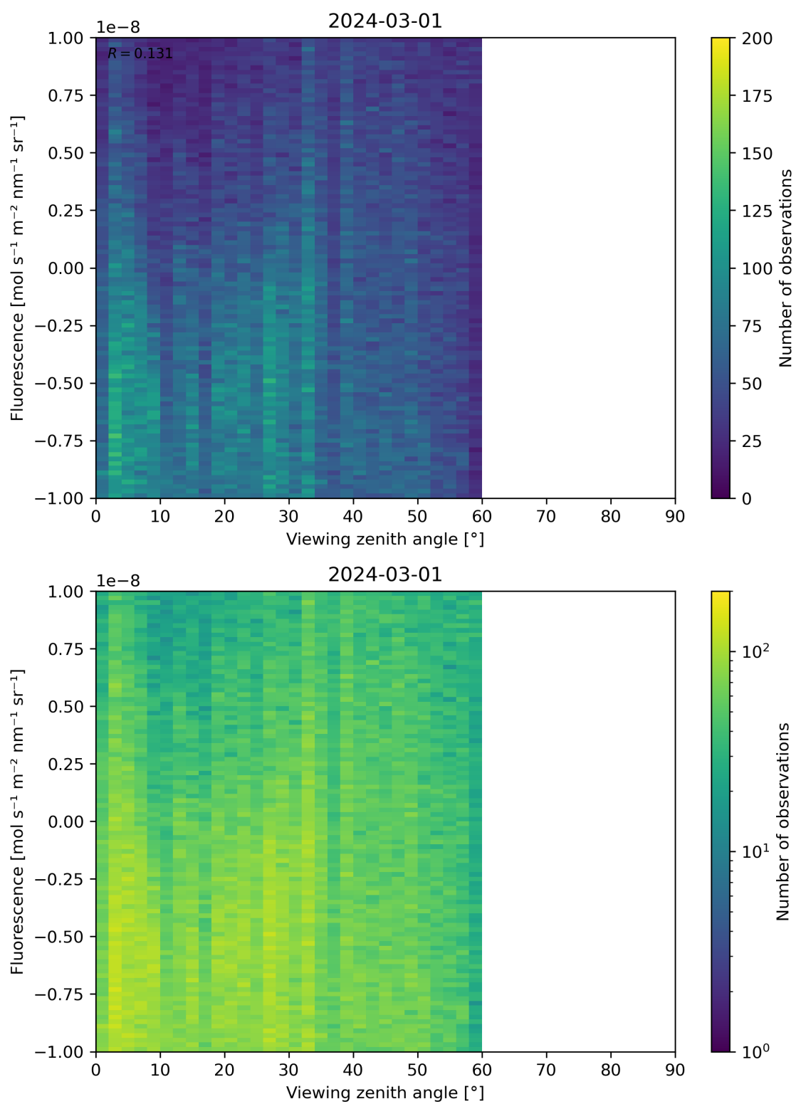
Figure 108: Scatter density plot of “Viewing zenith angle” against “Fluorescence” for 2024-02-29 to 2024-03-02.
