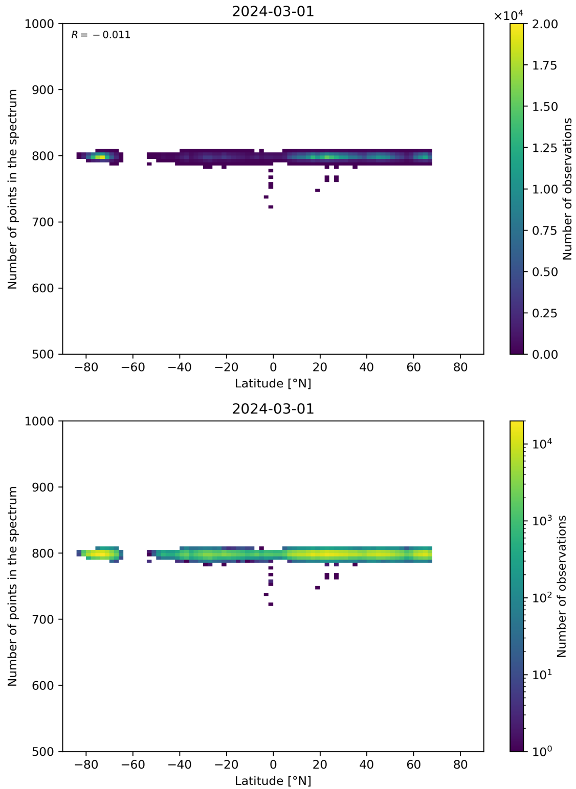
Figure 61: Scatter density plot of “Latitude” against “Number of points in the spectrum” for 2024-02-29 to 2024-03-02.
