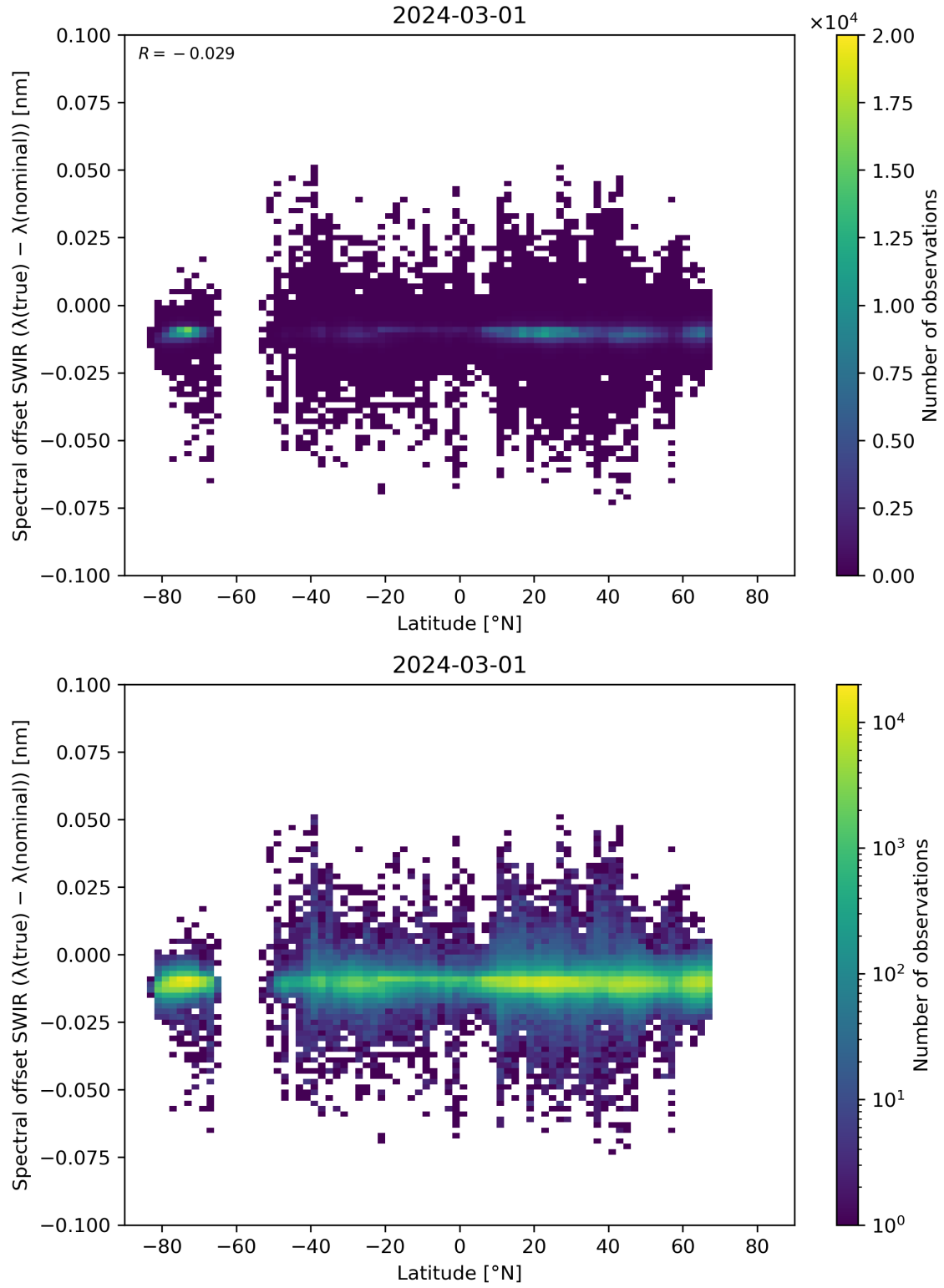
Figure 62: Scatter density plot of “Latitude” against “Spectral offset SWIR ( \lambda(\text{true}) - \lambda(\text{nominal}) )” for 2024-02-29 to 2024-03-02.
