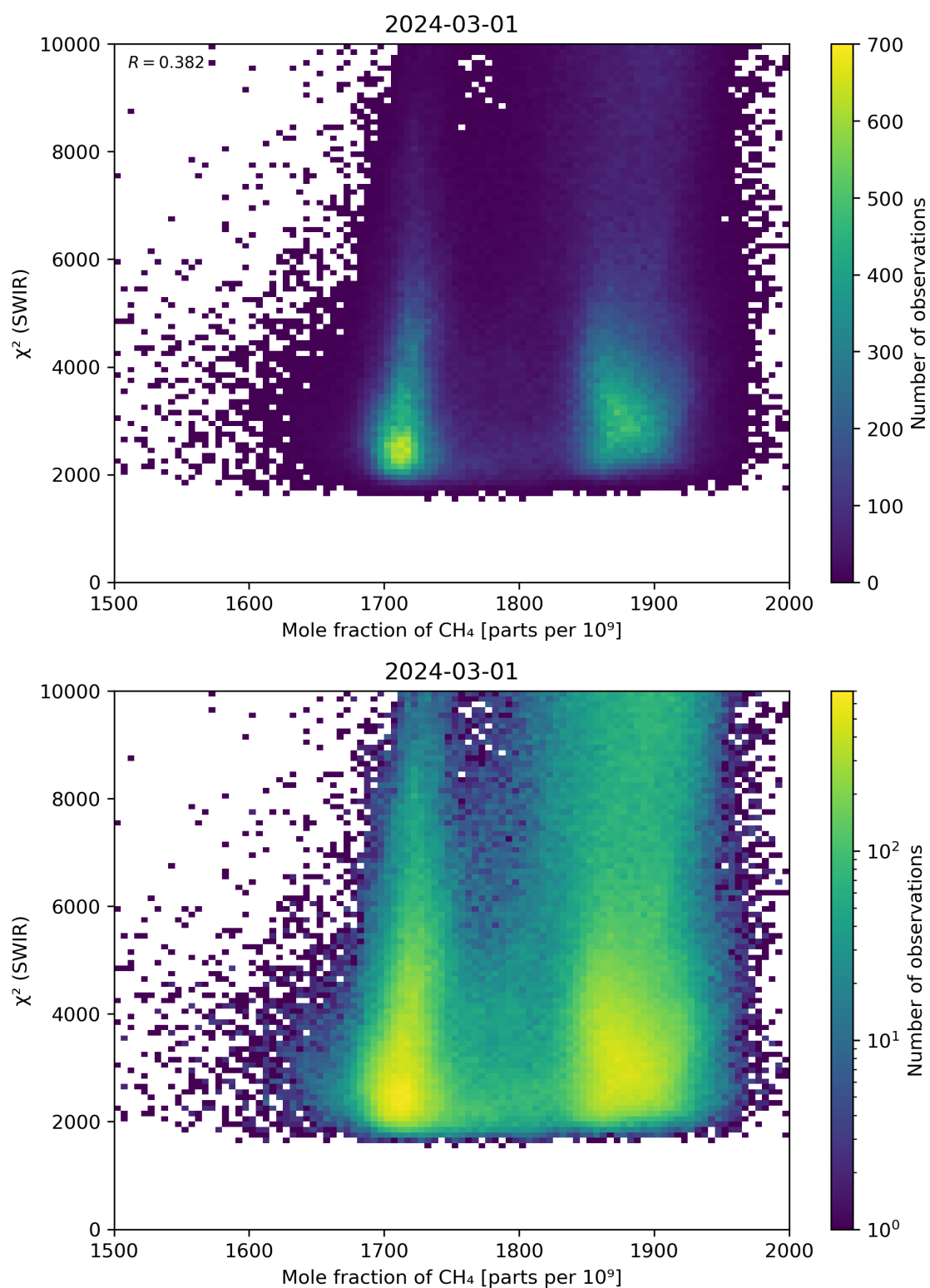
Figure 71: Scatter density plot of “Mole fraction of \text{CH}_4 ” against “ \chi^2 (SWIR)” for 2024-02-29 to 2024-03-02.
