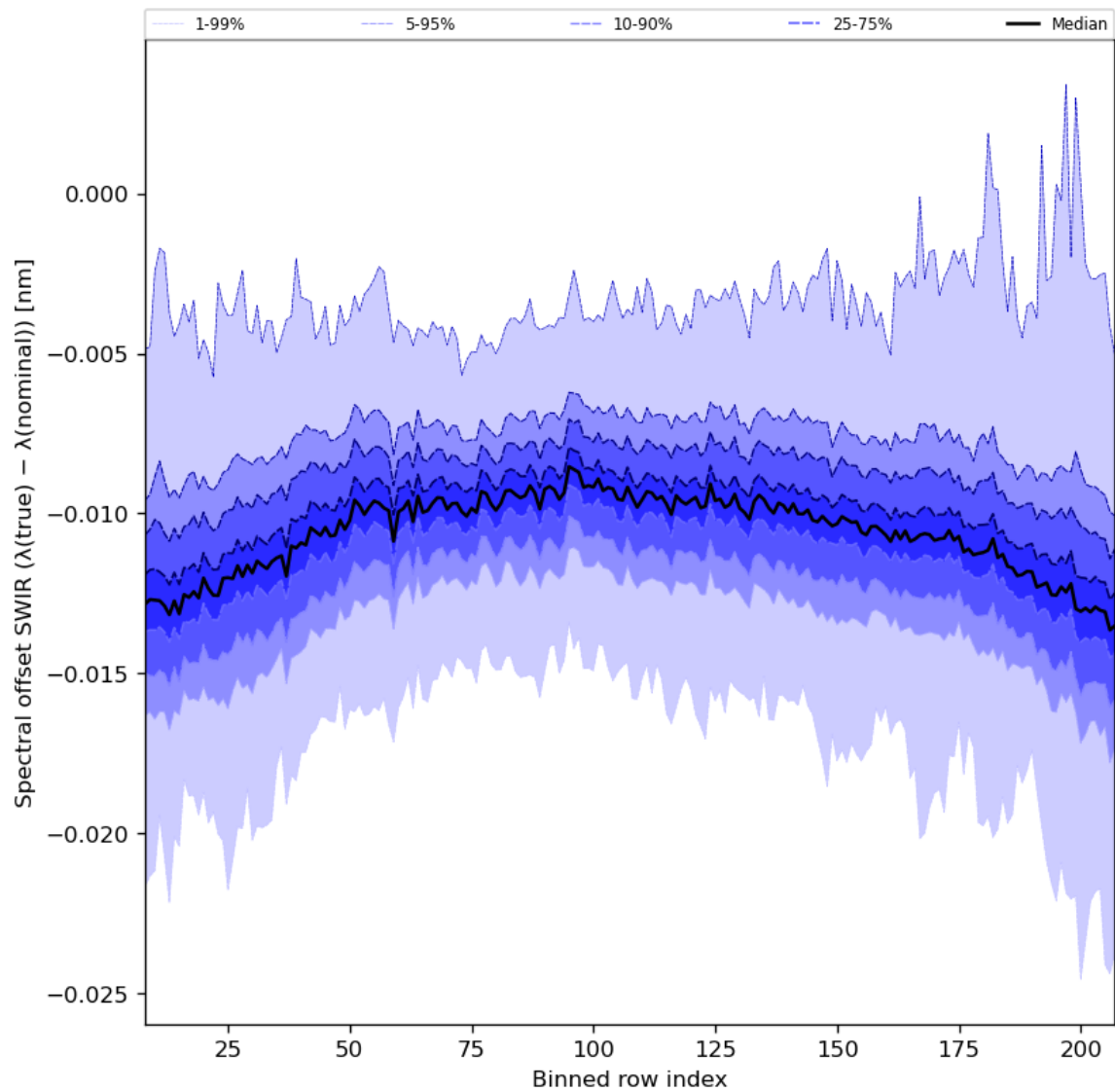
Figure 38: Along track statistics of “Spectral offset SWIR ( \lambda(\text{true}) - \lambda(\text{nominal}) )” for 2024-02-29 to 2024-03-02
