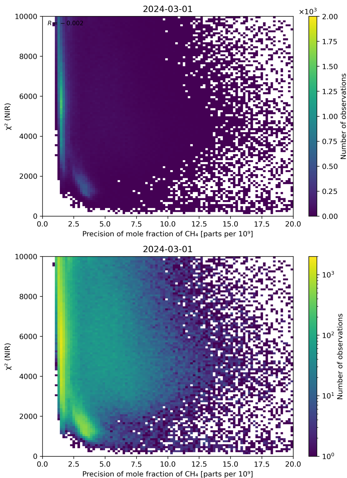
Figure 78: Scatter density plot of “Precision of mole fraction of CH 4 ” against “ \chi^2 (NIR)” for 2024-02-29 to 2024-03-02.
