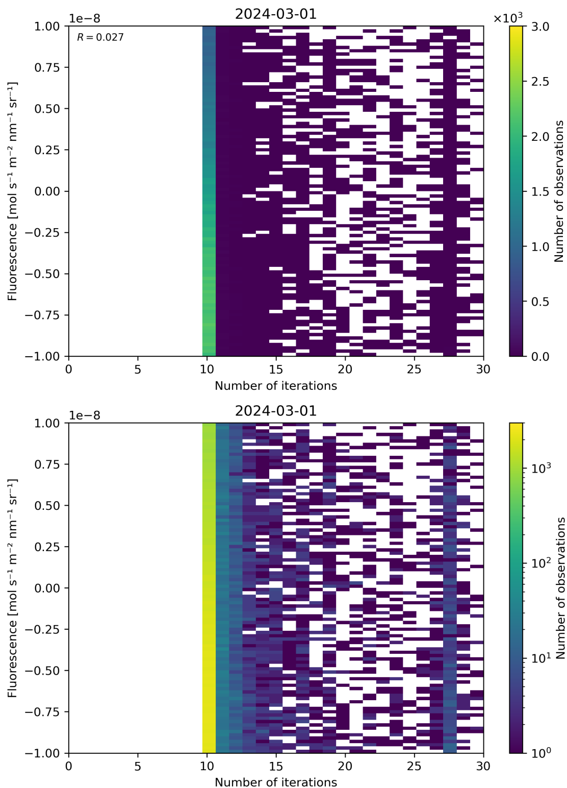
Figure 87: Scatter density plot of “Number of iterations” against “Fluorescence” for 2024-02-29 to 2024-03-02.
