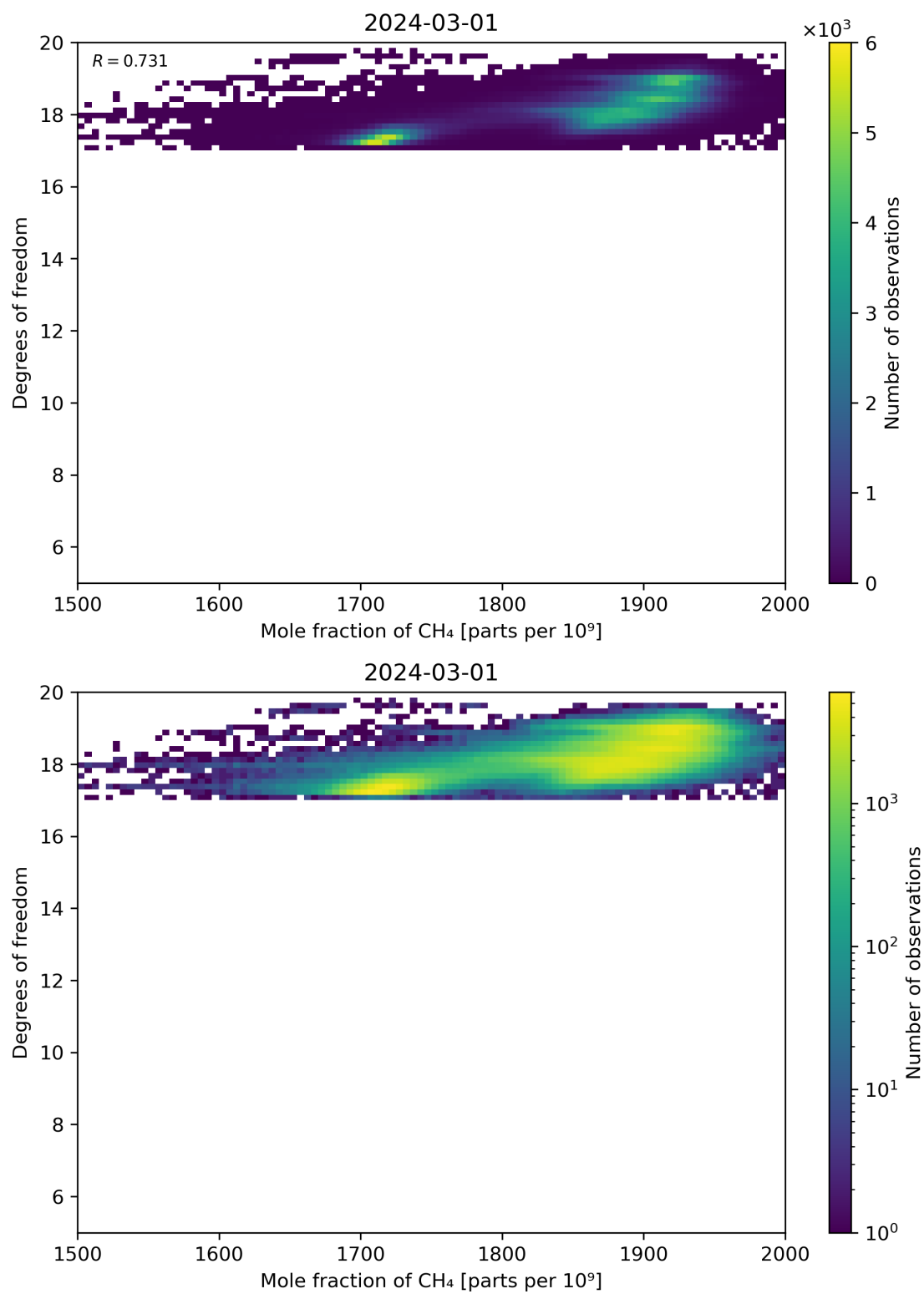
Figure 72: Scatter density plot of “Mole fraction of CH 4 ” against “Degrees of freedom” for 2024-02-29 to 2024-03-02.
