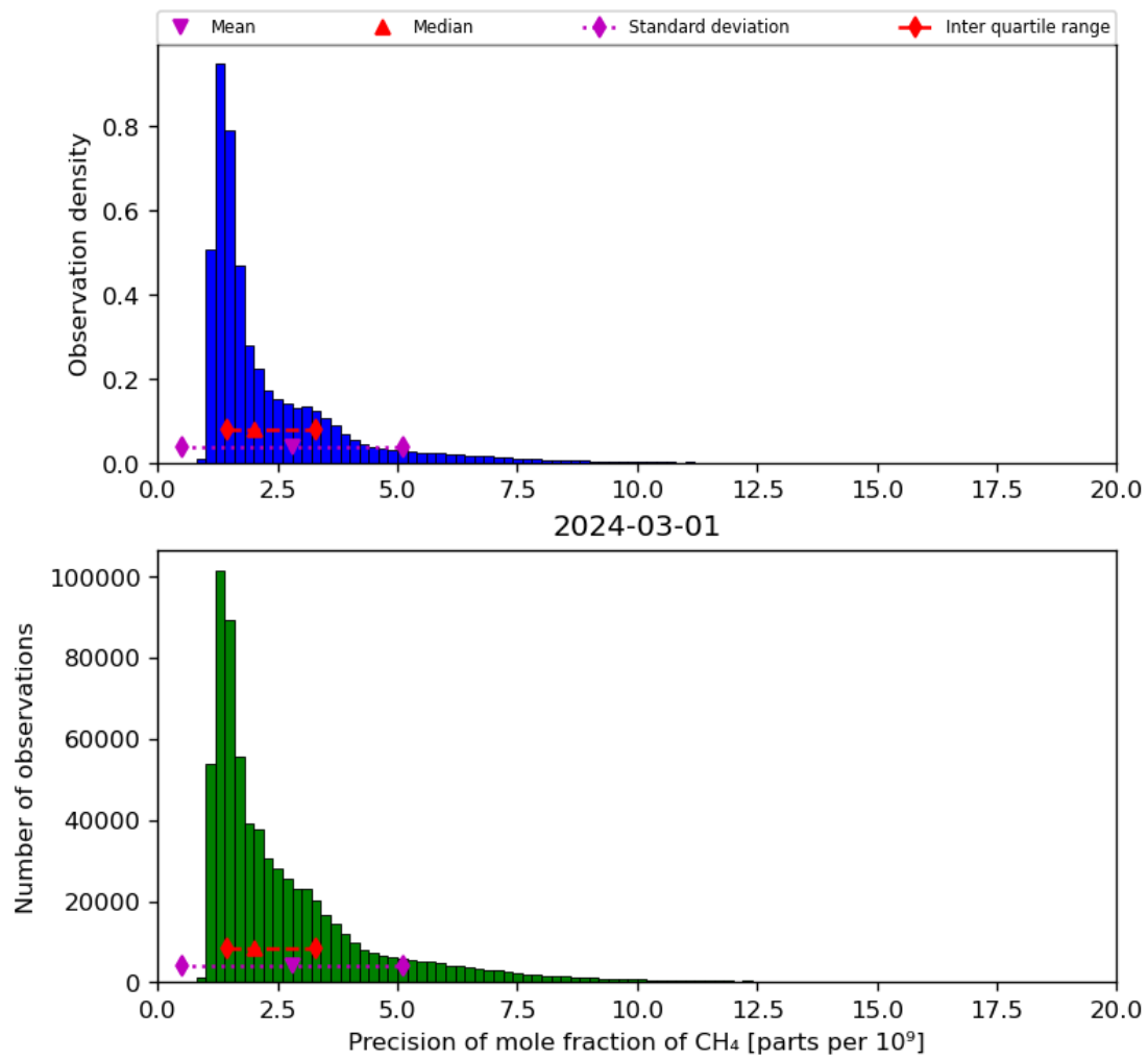
Figure 24: Histogram of “Precision of mole fraction of CH 4 ” for 2024-02-29 to 2024-03-02
