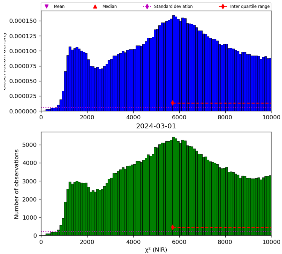
Figure 29: Histogram of “ \chi^2 (NIR)” for 2024-02-29 to 2024-03-02
