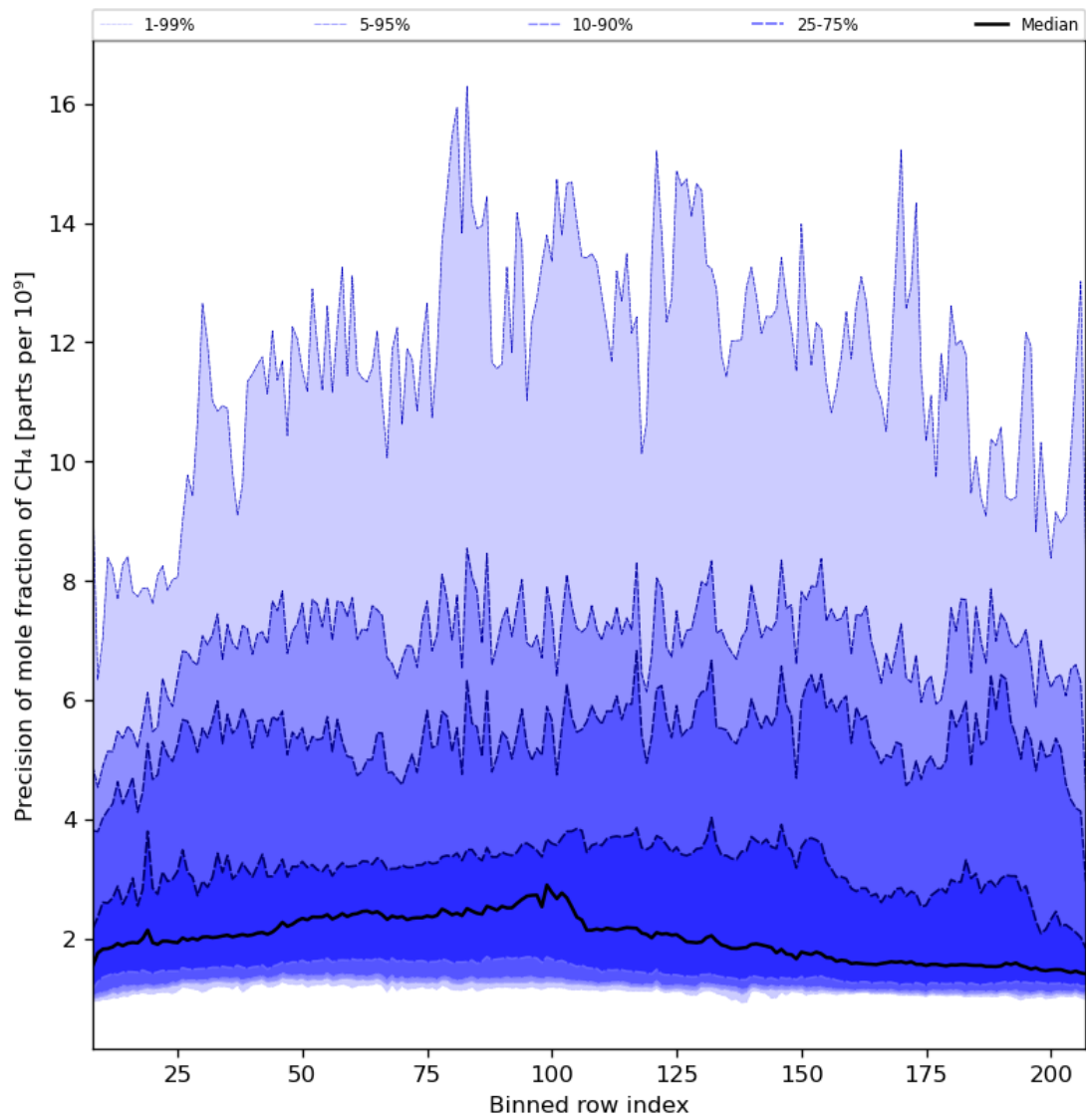
Figure 35: Along track statistics of “Precision of mole fraction of CH 4 ” for 2024-02-29 to 2024-03-02
