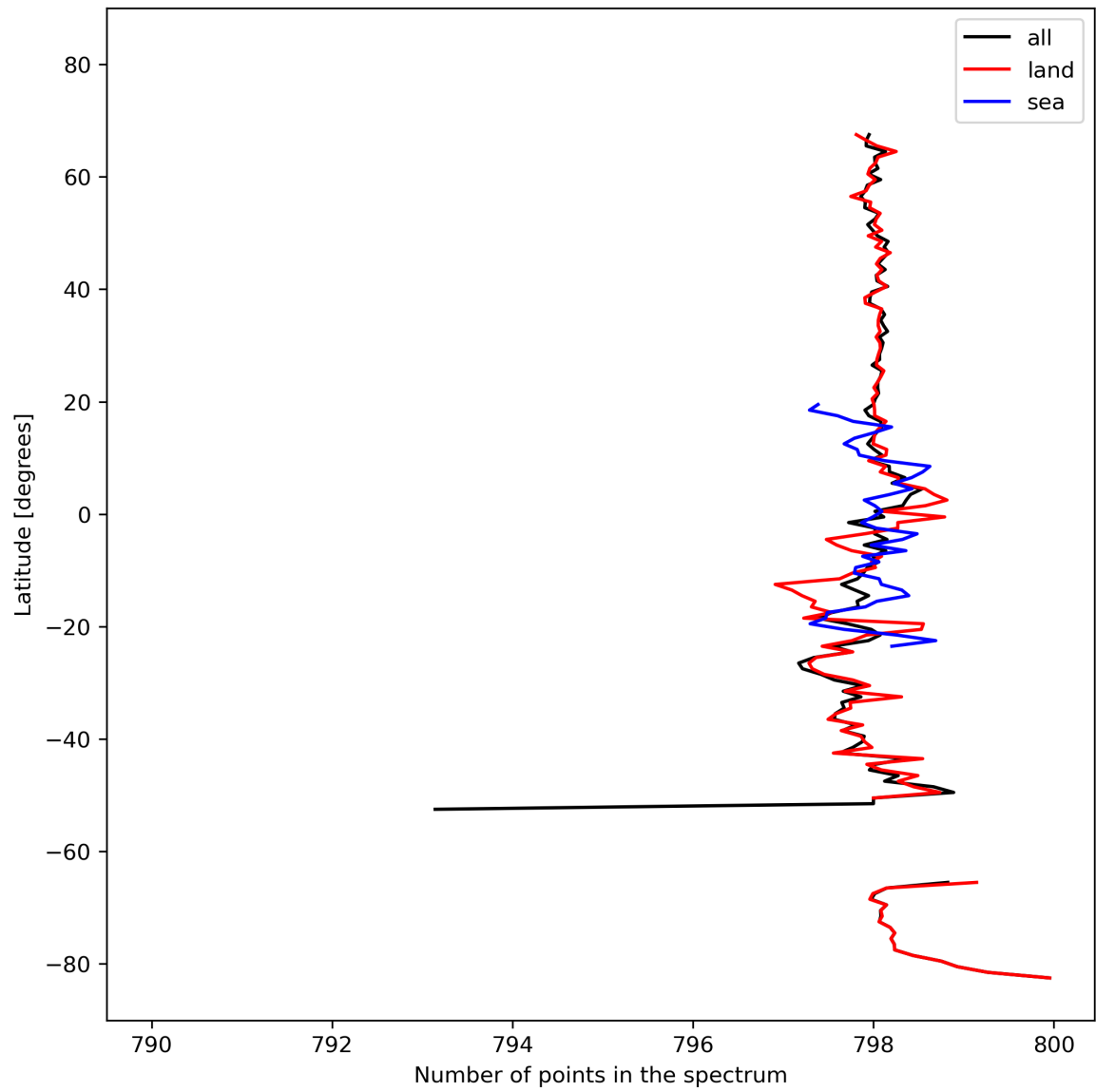
Figure 15: Zonal average of “Number of points in the spectrum” for 2024-02-29 to 2024-03-02.
