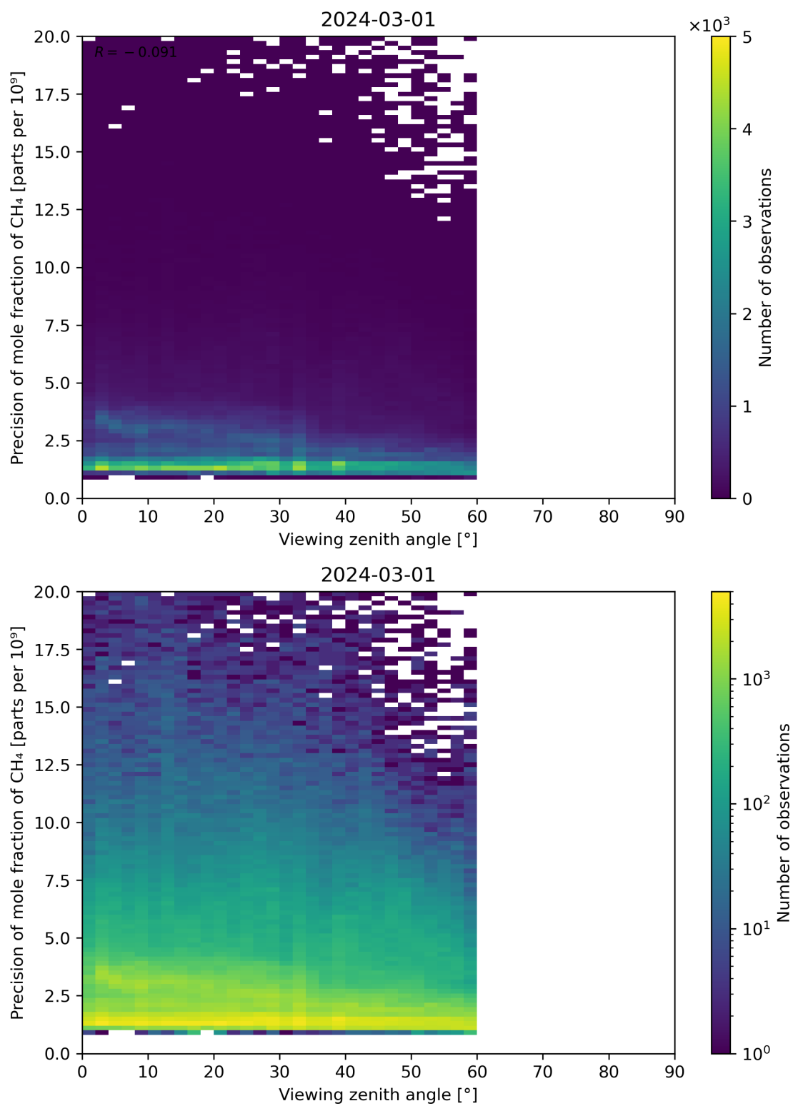
Figure 112: Scatter density plot of “Viewing zenith angle” against “Precision of mole fraction of CH 4 ” for 2024-02-29 to 2024-03-02.
