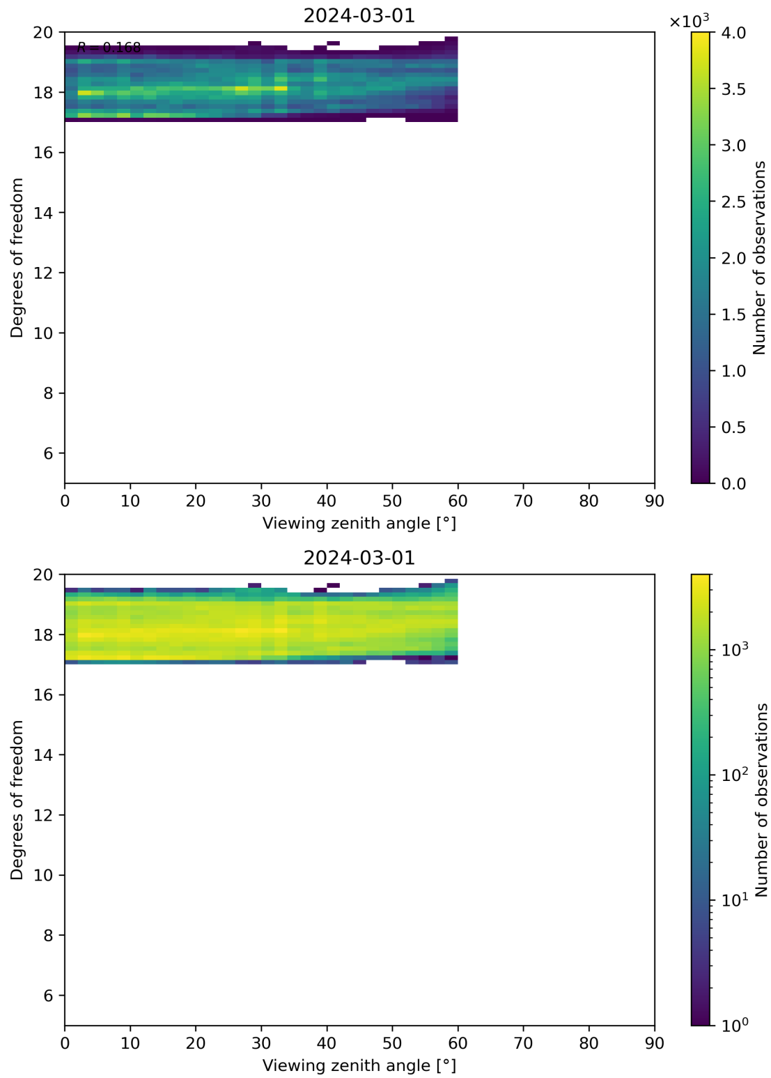
Figure 107: Scatter density plot of “Viewing zenith angle” against “Degrees of freedom” for 2024-02-29 to 2024-03-02.
