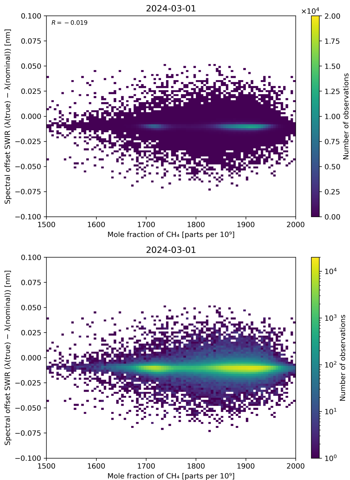
Figure 86: Scatter density plot of “Mole fraction of CH 4 ” against “Spectral offset SWIR ( \lambda(\text{true}) - \lambda(\text{nominal}) )” for 2024-02-29 to 2024-03-02.
