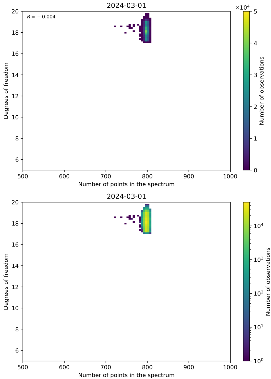
Figure 90: Scatter density plot of “Number of points in the spectrum” against “Degrees of freedom” for 2024-02-29 to 2024-03-02.
