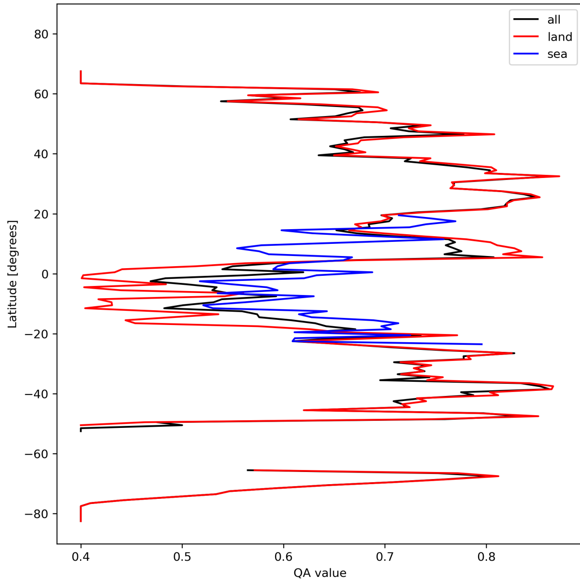
Figure 11: Zonal average of “QA value” for 2024-02-29 to 2024-03-02.
