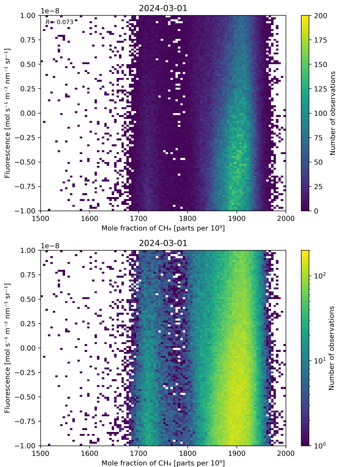
Figure 73: Scatter density plot of “Mole fraction of \text{CH}_4 ” against “Fluorescence” for 2024-02-29 to 2024-03-02.
