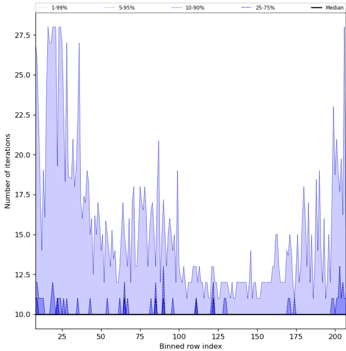
Figure 42: Along track statistics of “Number of iterations” for 2024-02-29 to 2024-03-02
