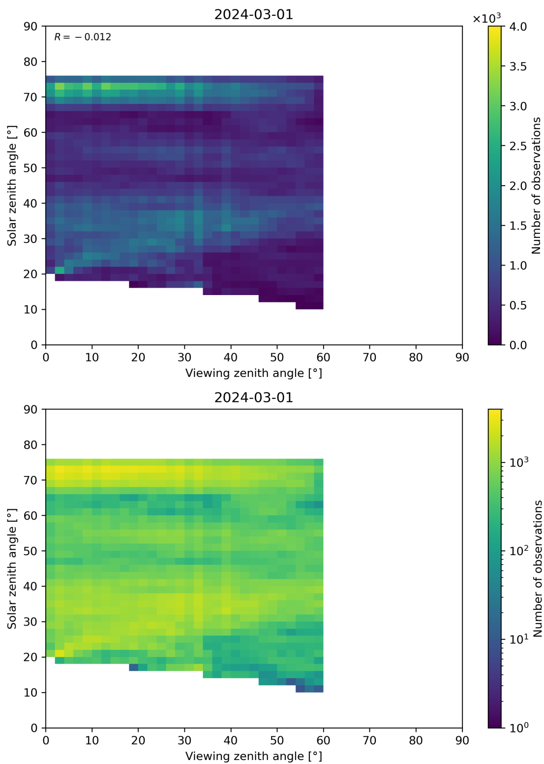
Figure 115: Scatter density plot of “Viewing zenith angle” against “Solar zenith angle” for 2024-02-29 to 2024-03-02.
