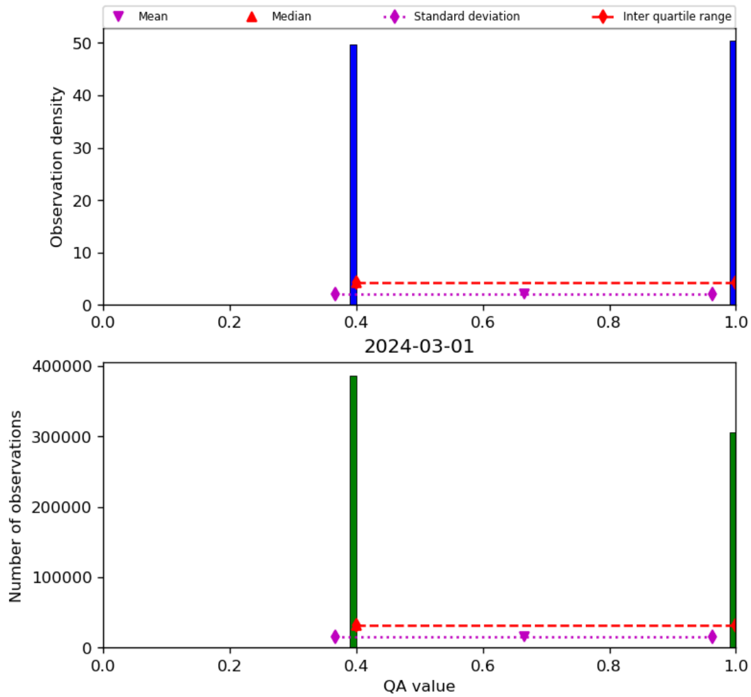
Figure 22: Histogram of “QA value” for 2024-02-29 to 2024-03-02
