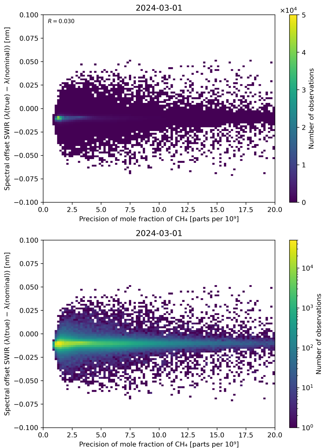
Figure 85: Scatter density plot of “Precision of mole fraction of \text{CH}_4 ” against “Spectral offset SWIR ( \lambda(\text{true}) - \lambda(\text{nominal}) )” for 2024-02-29 to 2024-03-02.
