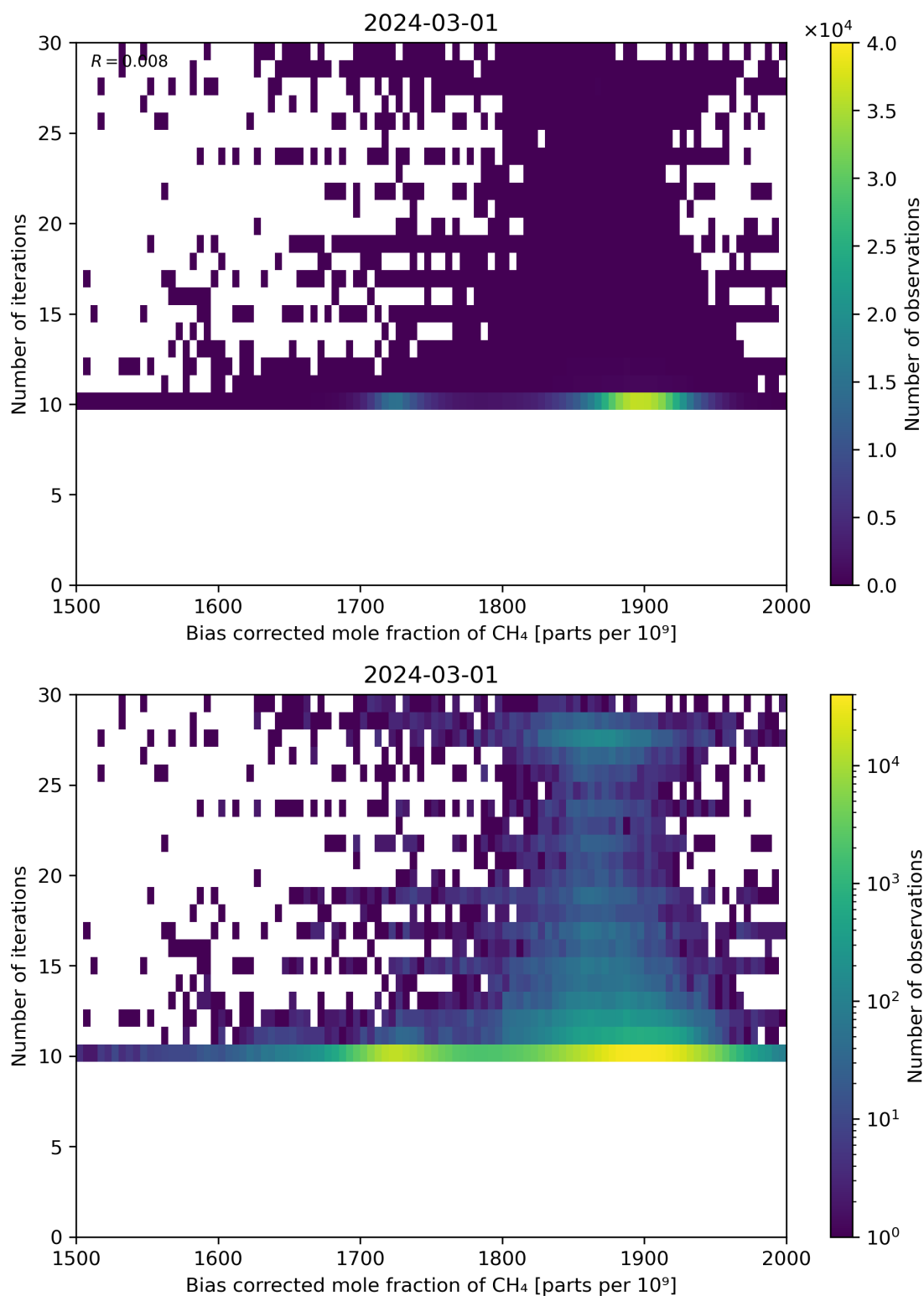
Figure 67: Scatter density plot of “Bias corrected mole fraction of \text{CH}_4 ” against “Number of iterations” for 2024-02-29 to 2024-03-02.
