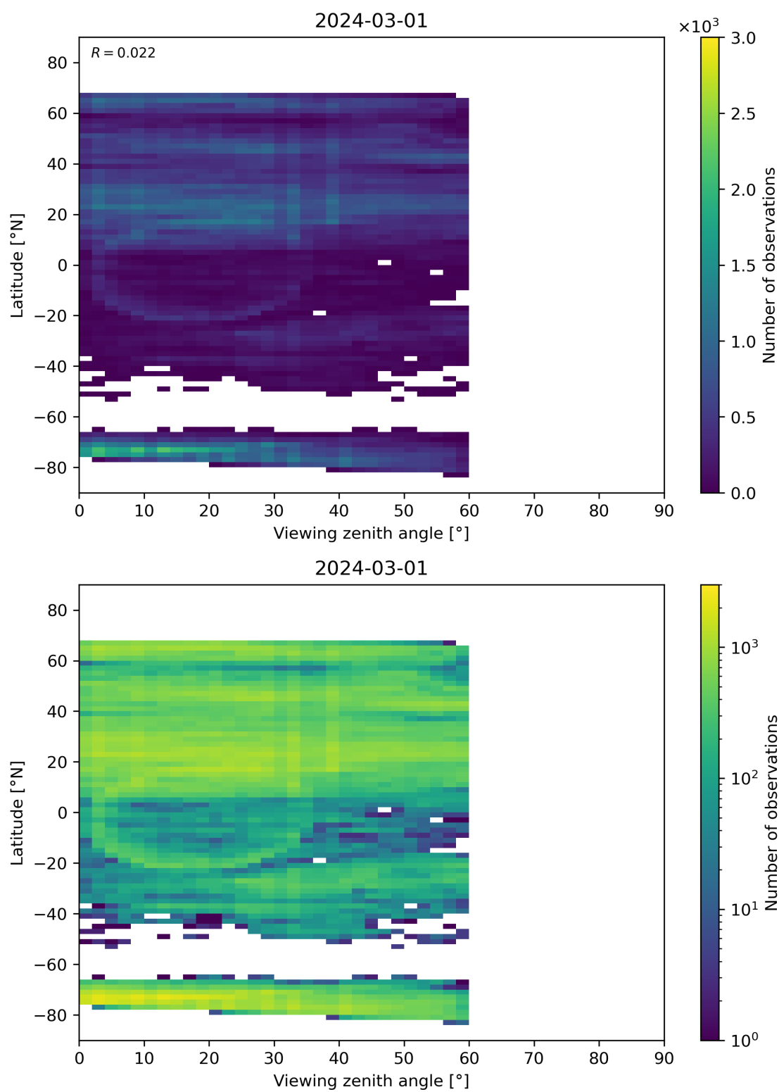
Figure 109: Scatter density plot of “Viewing zenith angle” against “Latitude” for 2024-02-29 to 2024-03-02.
