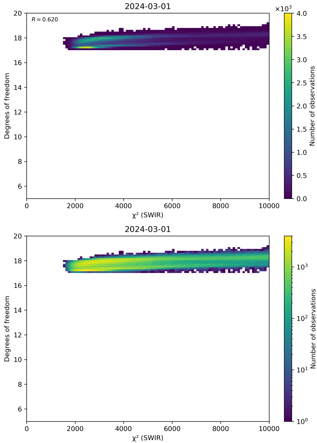
Figure 48: Scatter density plot of “ \chi^2 (SWIR)” against “Degrees of freedom” for 2024-02-29 to 2024-03-02.
