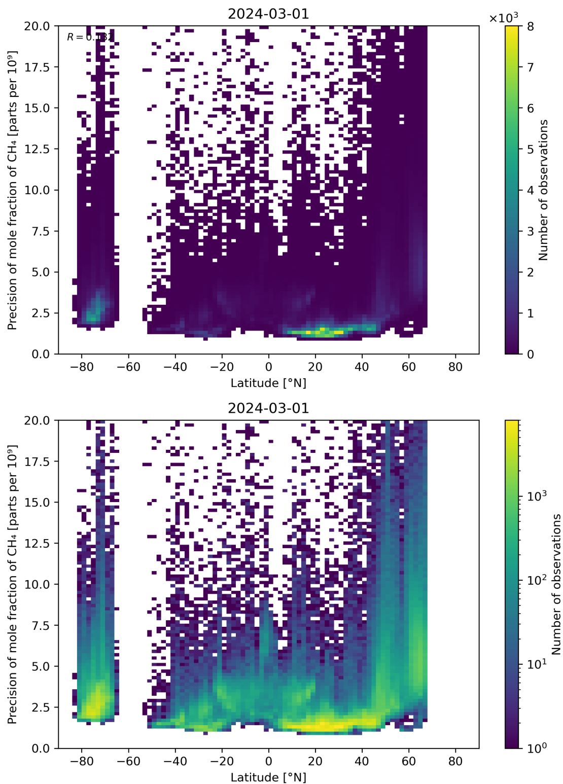
Figure 59: Scatter density plot of “Latitude” against “Precision of mole fraction of CH 4 ” for 2024-02-29 to 2024-03-02.
