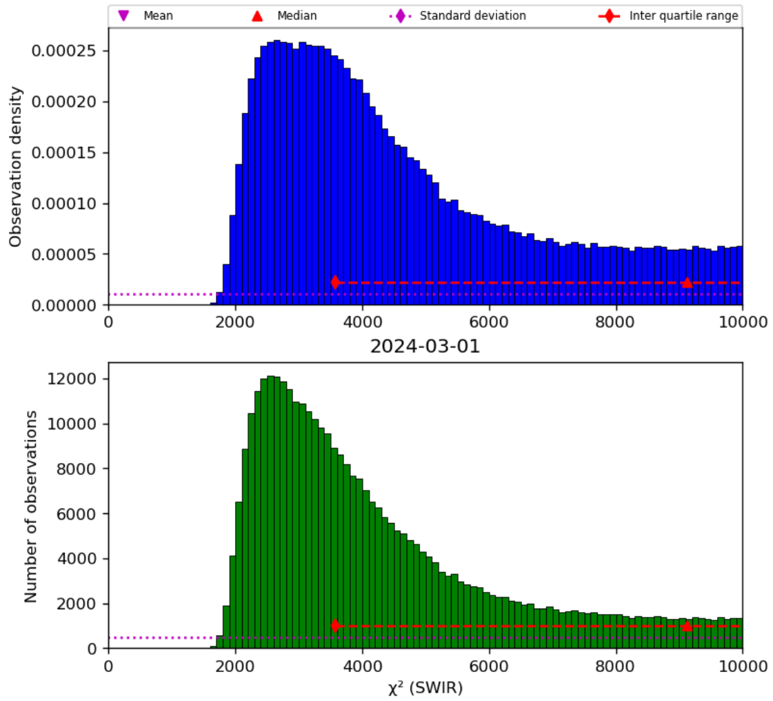
Figure 28: Histogram of “ \chi^2 (SWIR)” for 2024-02-29 to 2024-03-02
