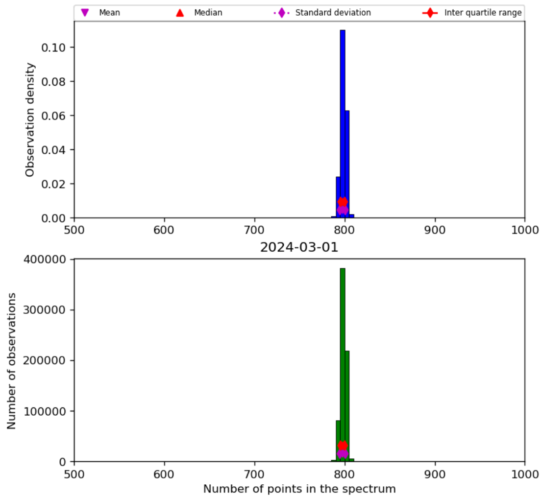
Figure 26: Histogram of “Number of points in the spectrum” for 2024-02-29 to 2024-03-02
