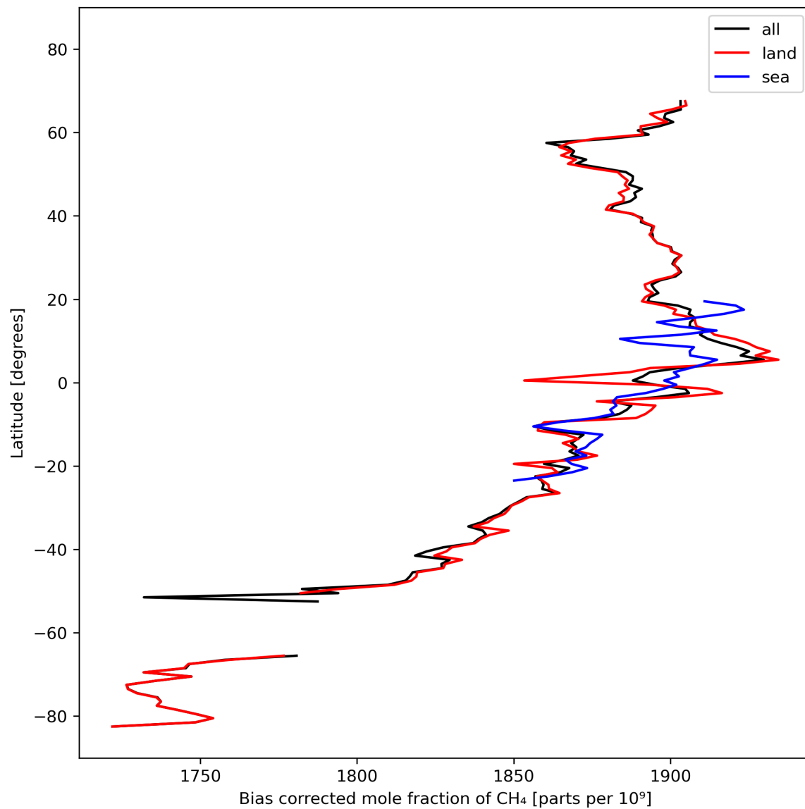
Figure 14: Zonal average of “Bias corrected mole fraction of CH 4 ” for 2024-02-29 to 2024-03-02.
