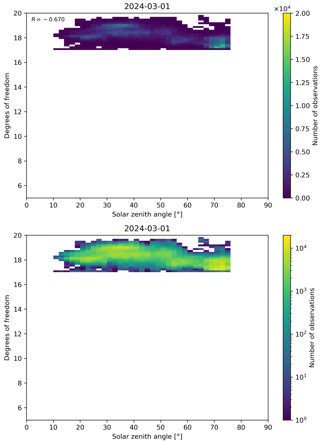
Figure 96: Scatter density plot of “Solar zenith angle” against “Degrees of freedom” for 2024-02-29 to 2024-03-02.
