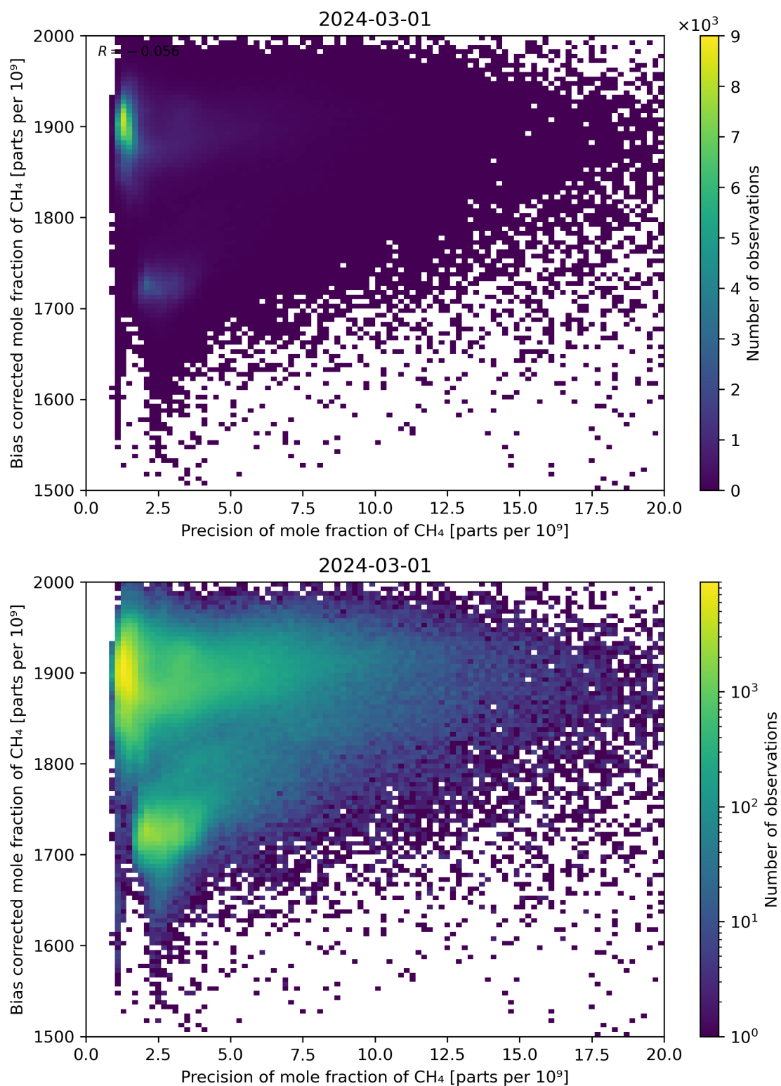
Figure 82: Scatter density plot of “Precision of mole fraction of CH 4 ” against “Bias corrected mole fraction of CH 4 ” for 2024-02-29 to 2024-03-02.
