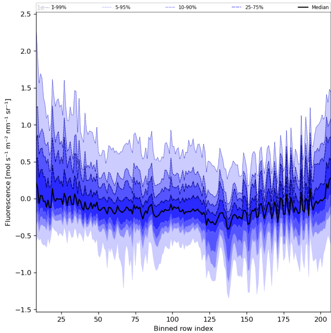
Figure 43: Along track statistics of “Fluorescence” for 2024-02-29 to 2024-03-02
