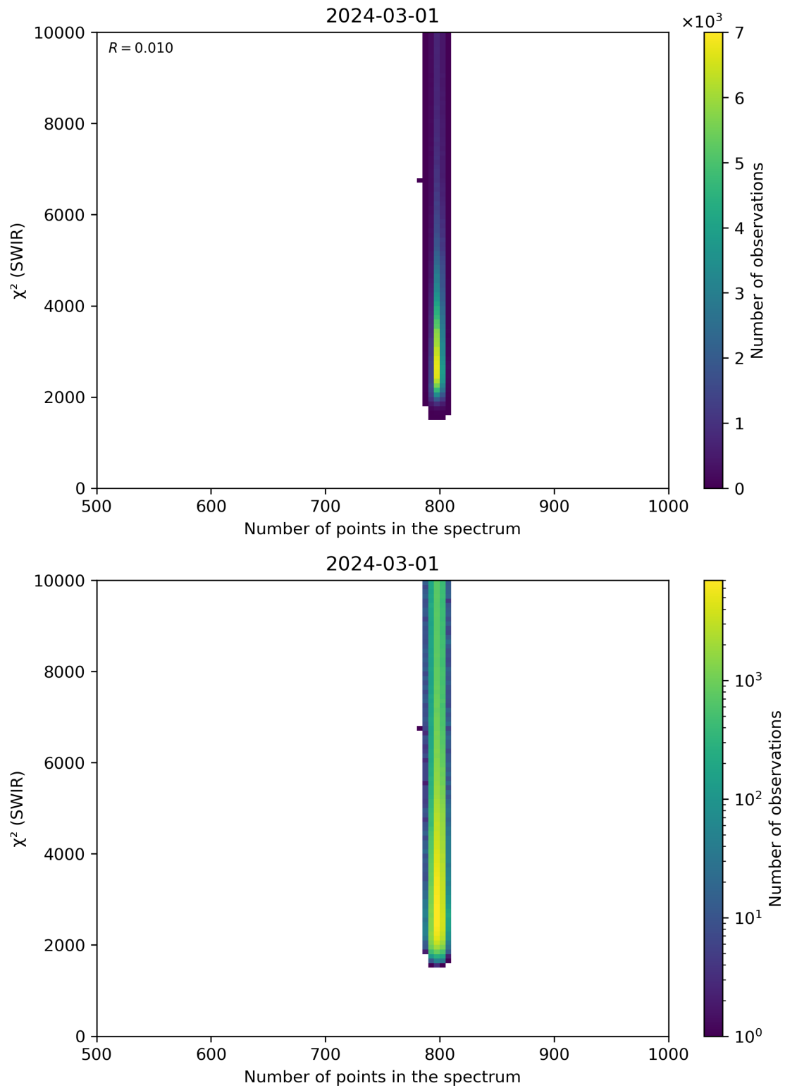
Figure 89: Scatter density plot of “Number of points in the spectrum” against “ \chi^2 (SWIR)” for 2024-02-29 to 2024-03-02.
