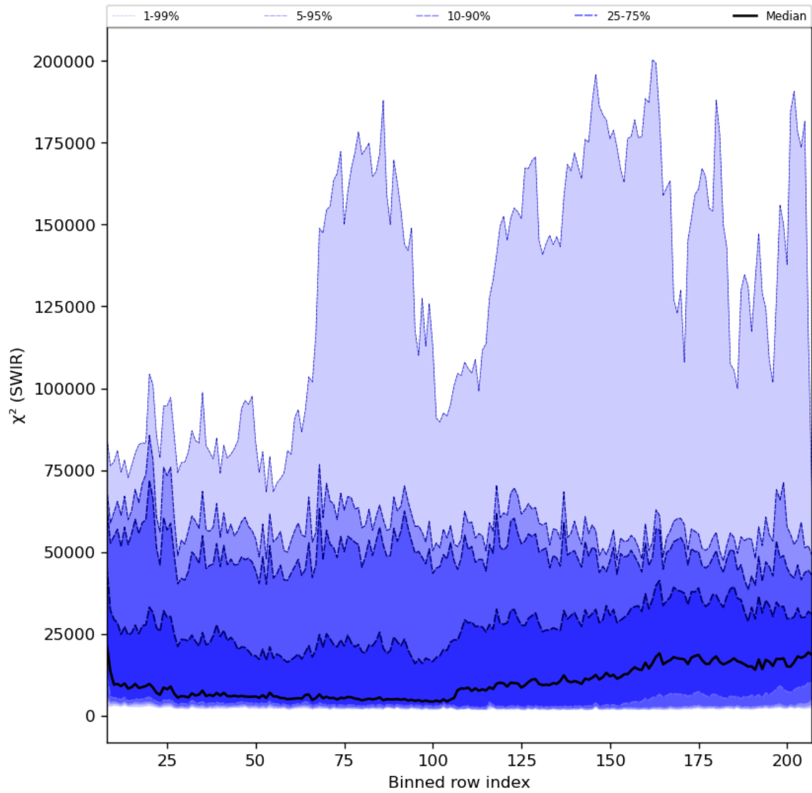
Figure 39: Along track statistics of “ \chi^2 (SWIR)” for 2024-02-29 to 2024-03-02
