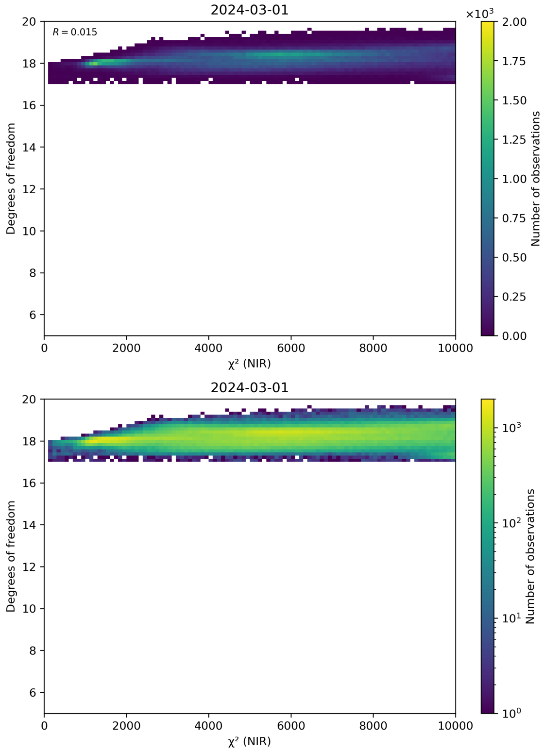
Figure 44: Scatter density plot of “ \chi^2 (NIR)” against “Degrees of freedom” for 2024-02-29 to 2024-03-02.
