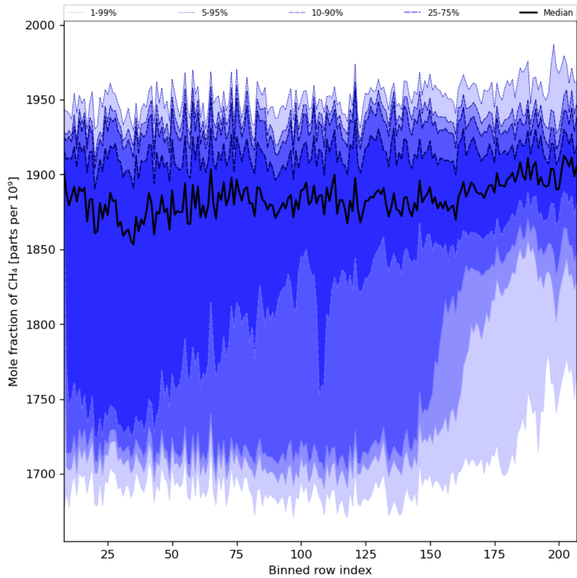
Figure 34: Along track statistics of “Mole fraction of CH 4 ” for 2024-02-29 to 2024-03-02
