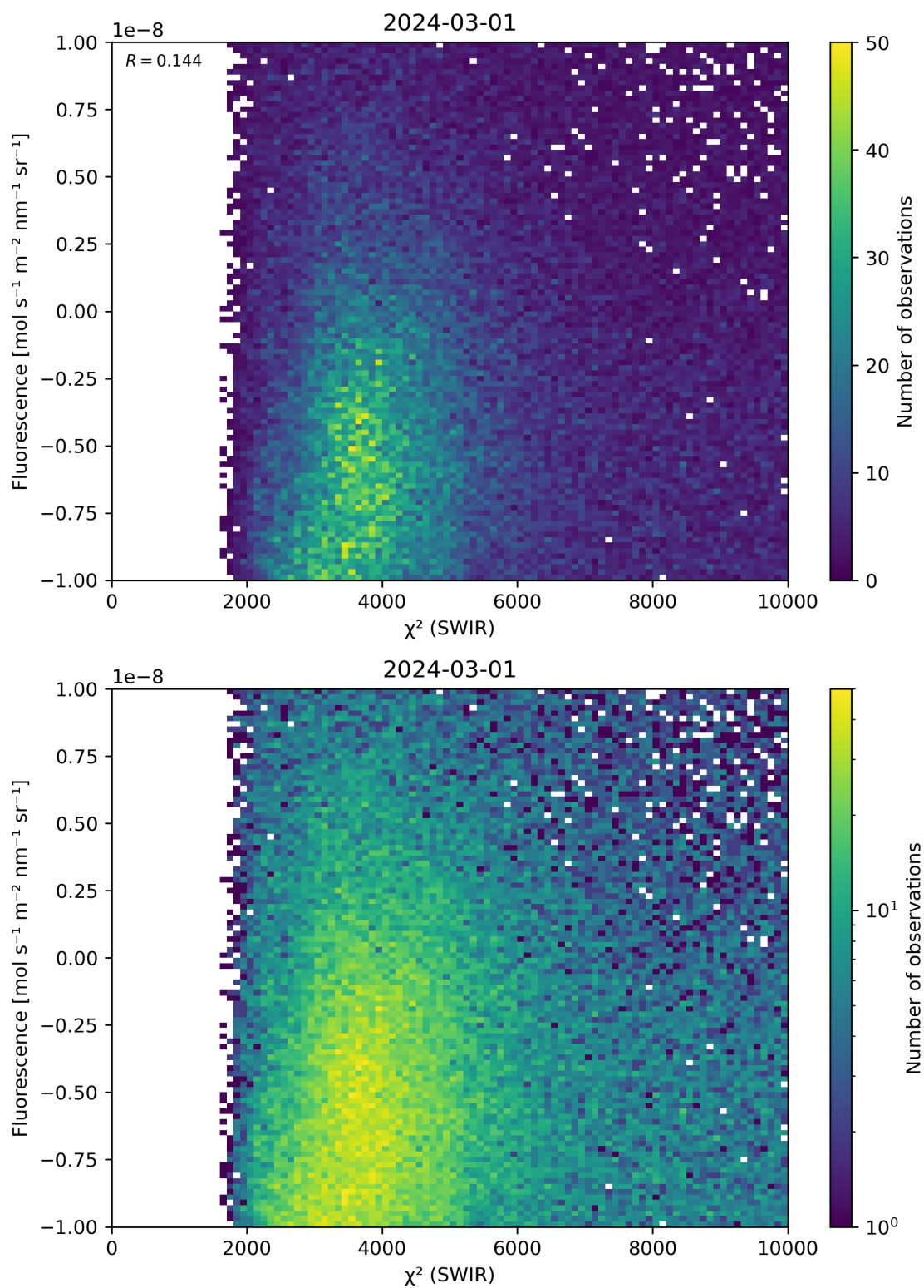
Figure 49: Scatter density plot of “ \chi^2 (SWIR)” against “Fluorescence” for 2024-02-29 to 2024-03-02.
