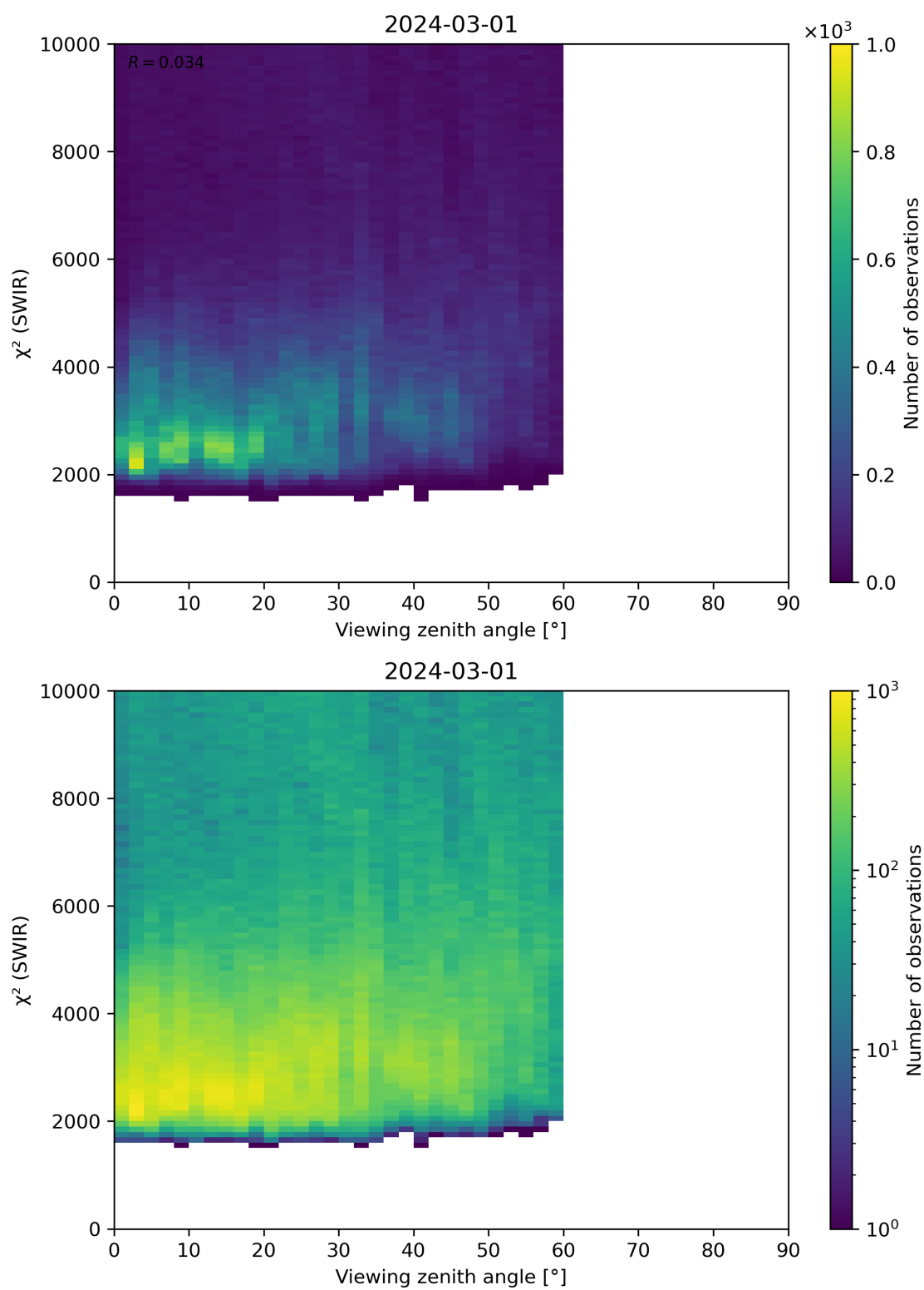
Figure 106: Scatter density plot of “Viewing zenith angle” against “ \chi^2 (SWIR)” for 2024-02-29 to 2024-03-02.
