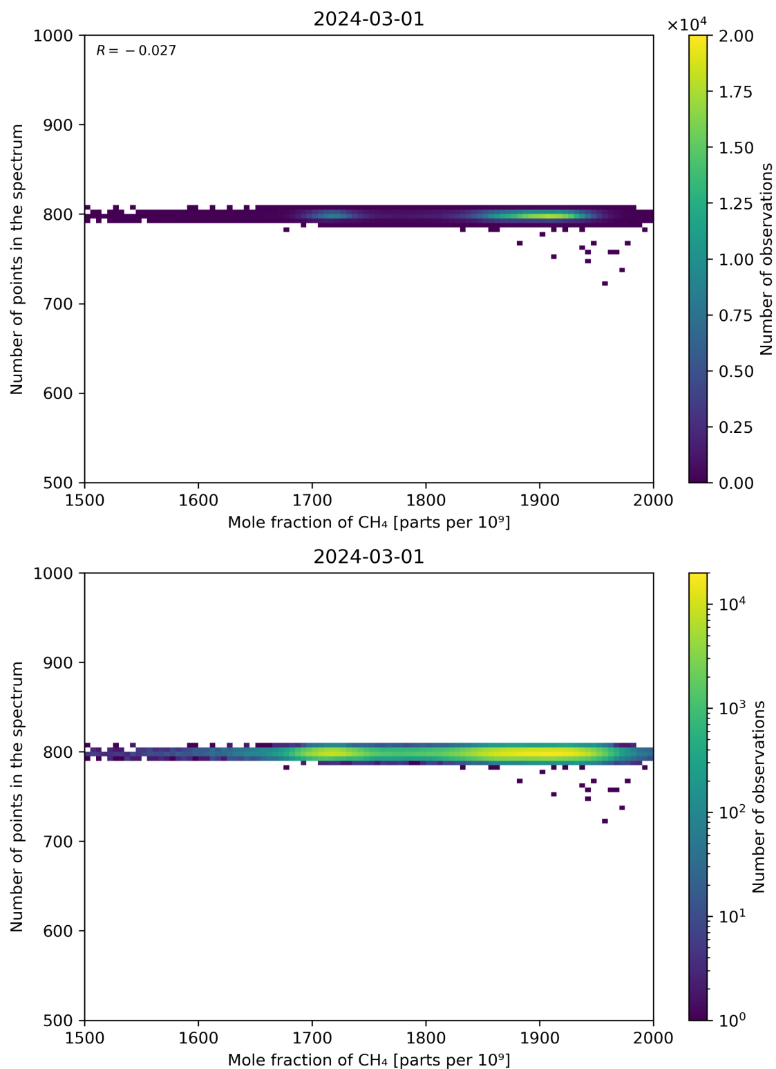
Figure 77: Scatter density plot of “Mole fraction of CH 4 ” against “Number of points in the spectrum” for 2024-02-29 to 2024-03-02.
