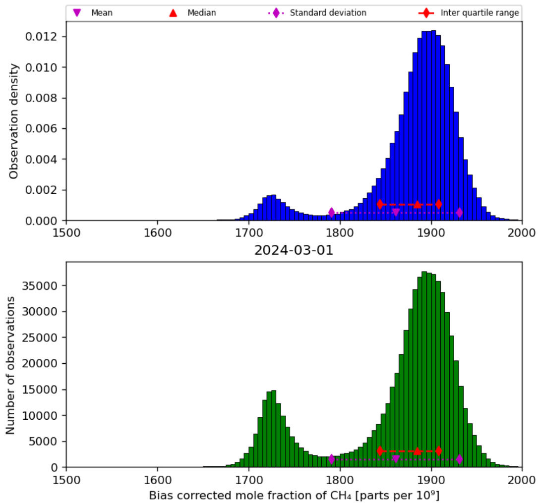
Figure 25: Histogram of “Bias corrected mole fraction of CH 4 ” for 2024-02-29 to 2024-03-02
