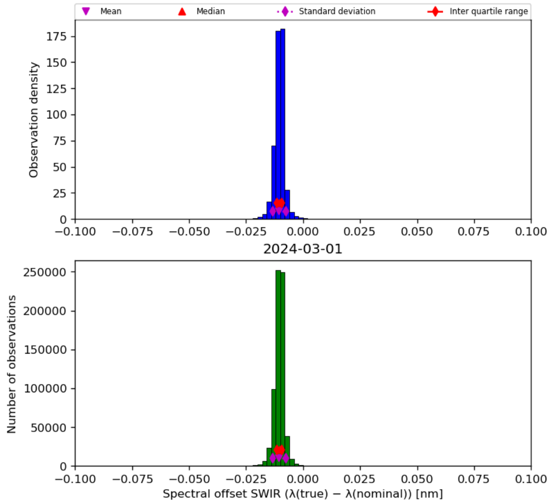
Figure 27: Histogram of “Spectral offset SWIR ( \lambda(\text{true}) - \lambda(\text{nominal}) )” for 2024-02-29 to 2024-03-02
