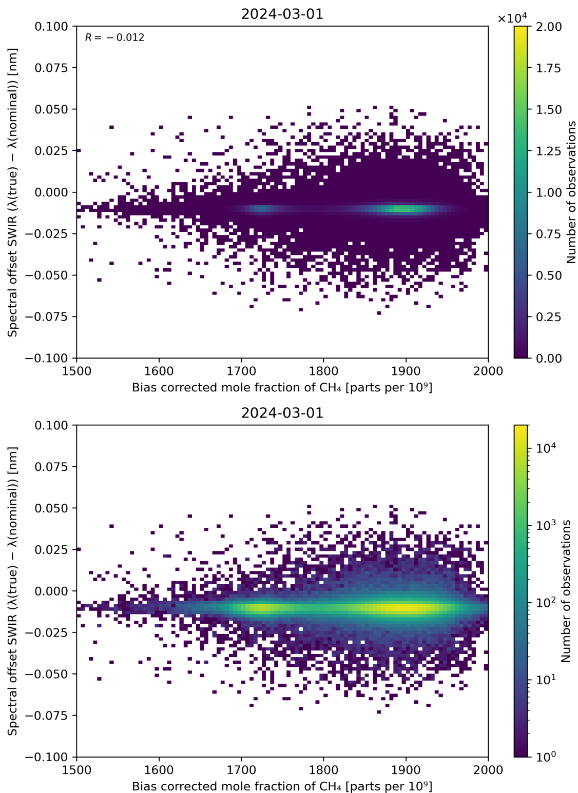
Figure 69: Scatter density plot of “Bias corrected mole fraction of \text{CH}_4 ” against “Spectral offset SWIR ( \lambda(\text{true}) - \lambda(\text{nominal}) )” for 2024-02-29 to 2024-03-02.
