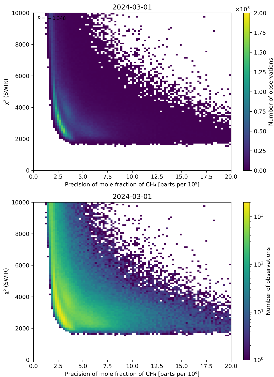
Figure 79: Scatter density plot of “Precision of mole fraction of CH 4 ” against “ \chi^2 (SWIR)” for 2024-02-29 to 2024-03-02.
