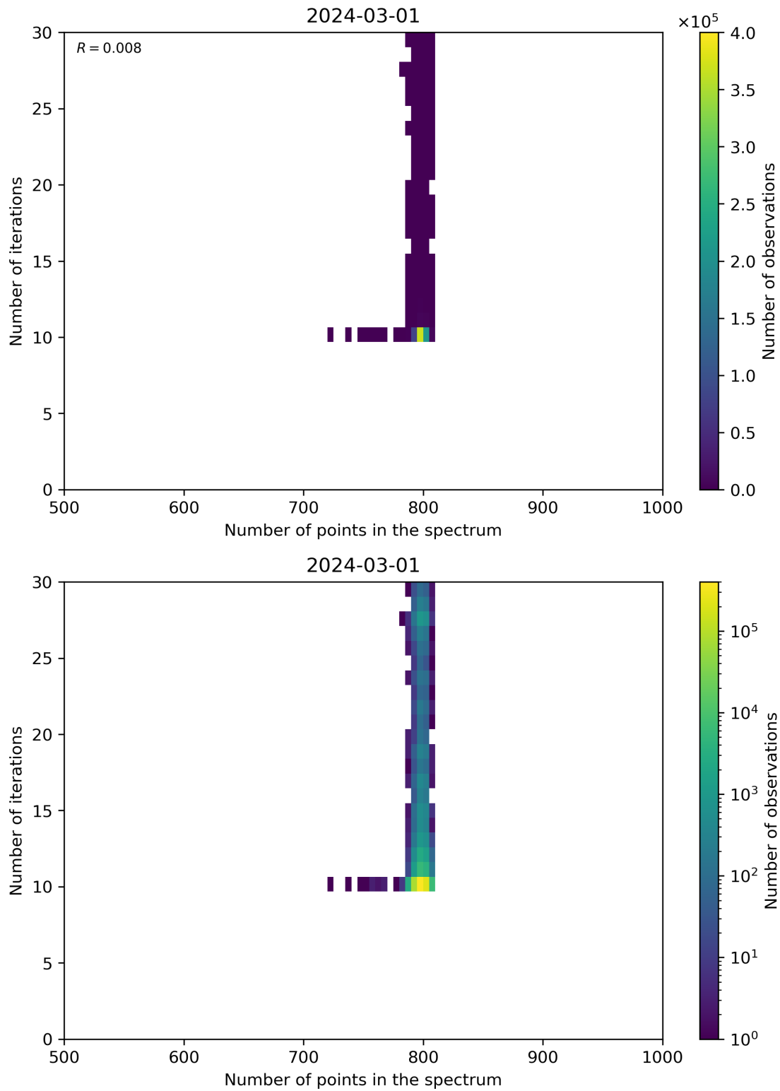
Figure 92: Scatter density plot of “Number of points in the spectrum” against “Number of iterations” for 2024-02-29 to 2024-03-02.
