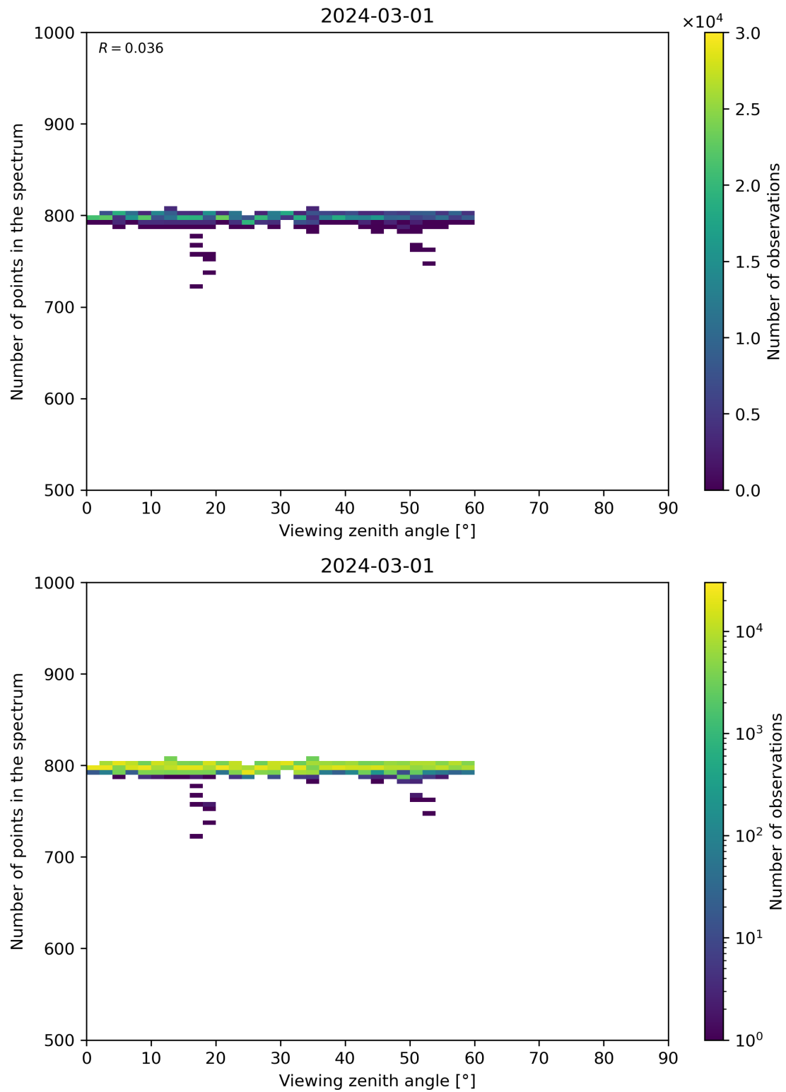
Figure 114: Scatter density plot of “Viewing zenith angle” against “Number of points in the spectrum” for 2024-02-29 to 2024-03-02.
