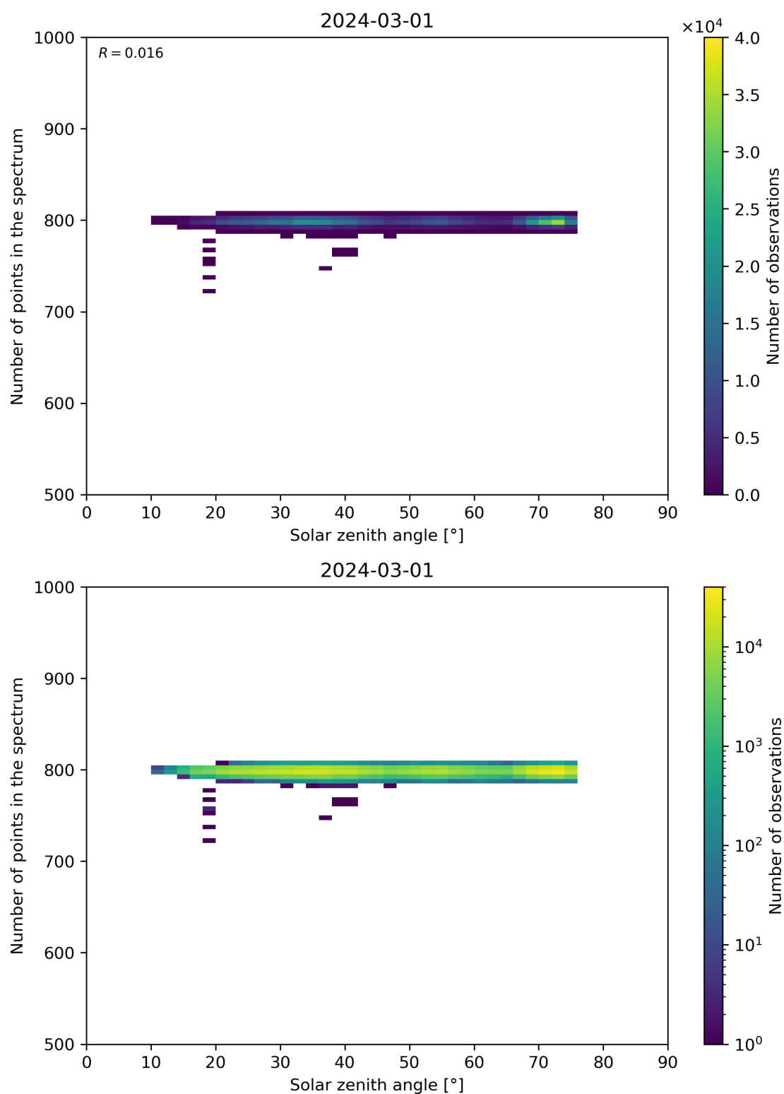
Figure 103: Scatter density plot of “Solar zenith angle” against “Number of points in the spectrum” for 2024-02-29 to 2024-03-02.
