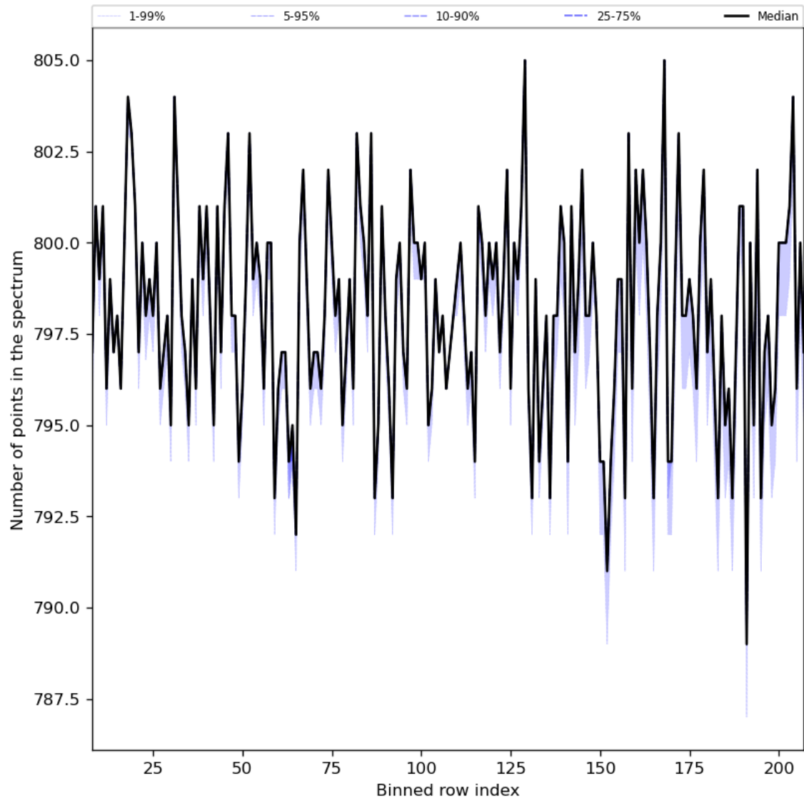
Figure 37: Along track statistics of “Number of points in the spectrum” for 2024-02-29 to 2024-03-02
