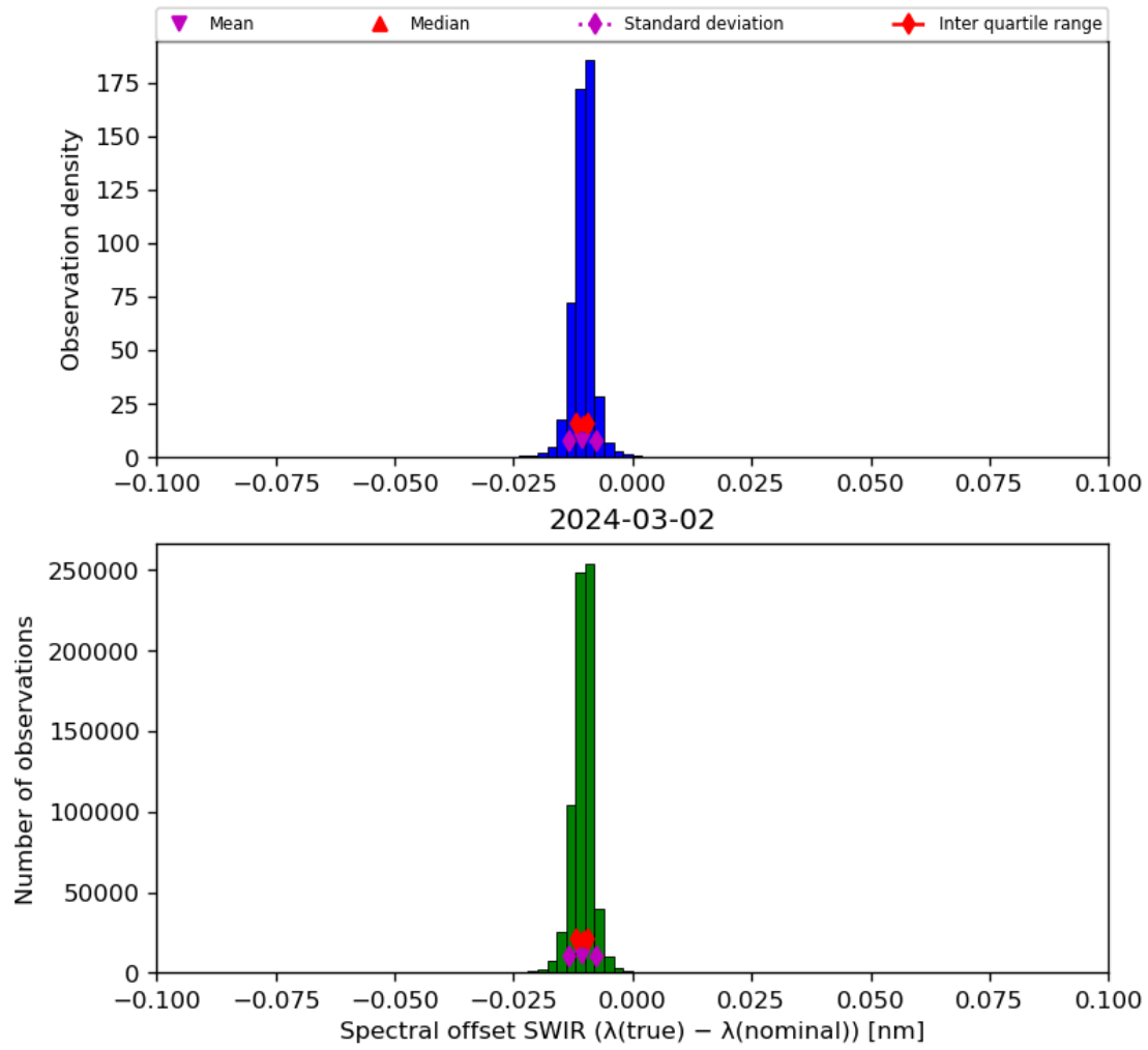
Figure 27: Histogram of “Spectral offset SWIR ( \lambda(\text{true}) - \lambda(\text{nominal}) )” for 2024-03-01 to 2024-03-03
