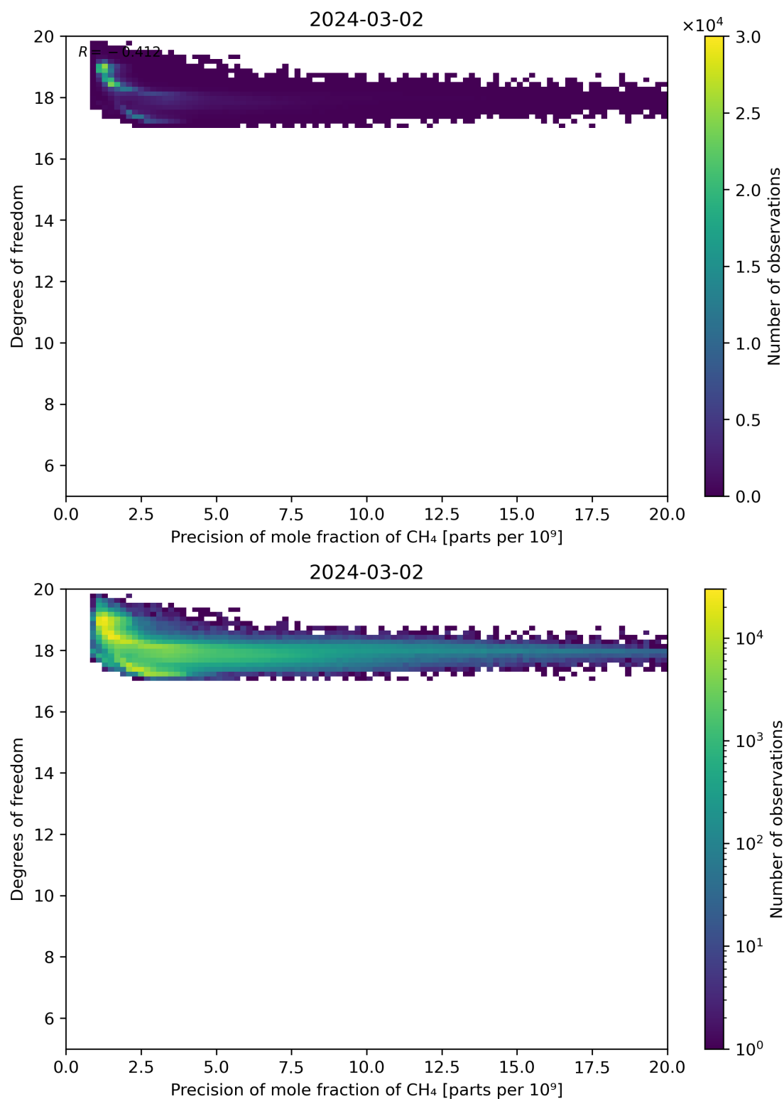
Figure 80: Scatter density plot of “Precision of mole fraction of CH 4 ” against “Degrees of freedom” for 2024-03-01 to 2024-03-03.
