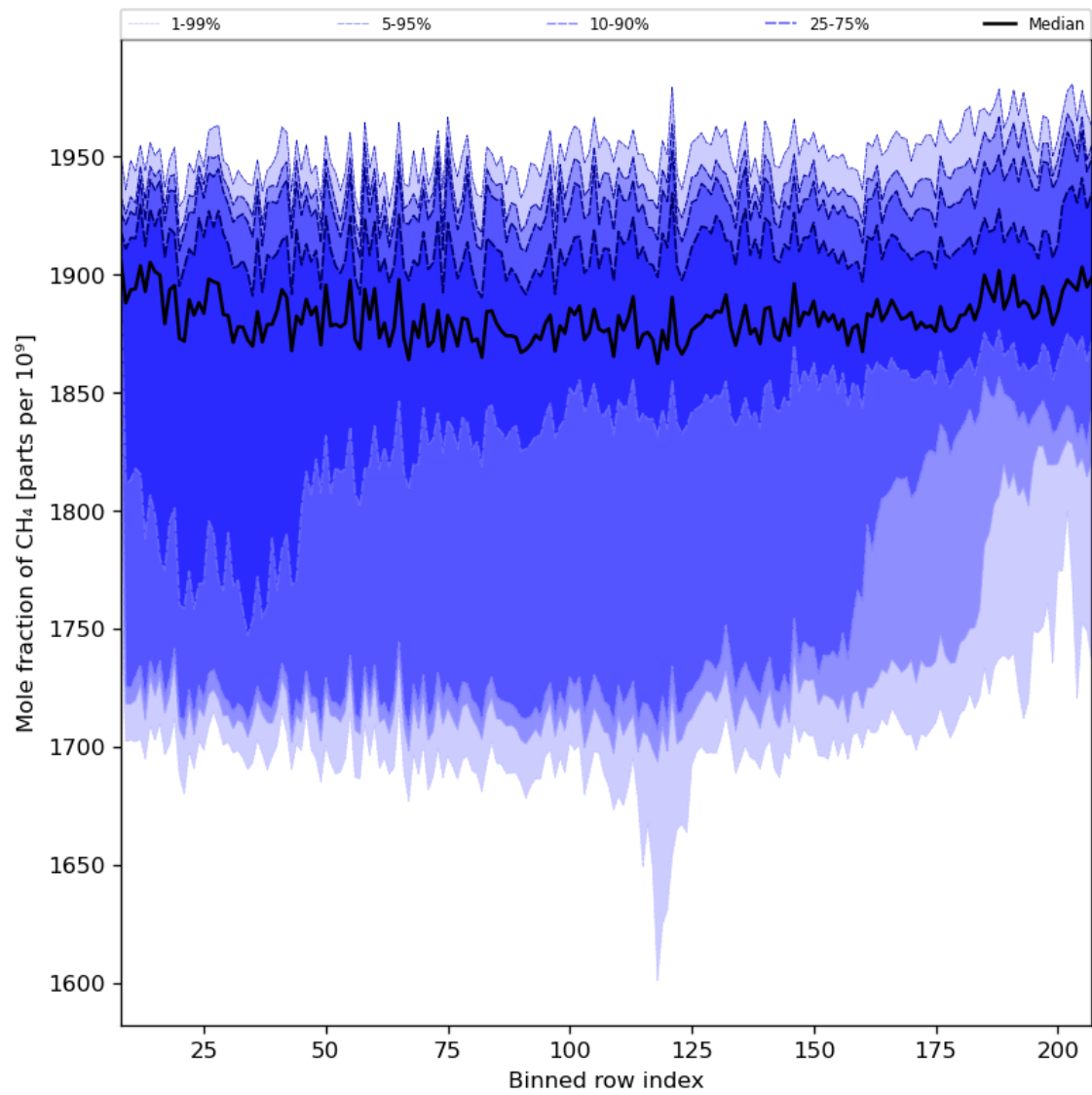
Figure 34: Along track statistics of “Mole fraction of CH 4 ” for 2024-03-01 to 2024-03-03
