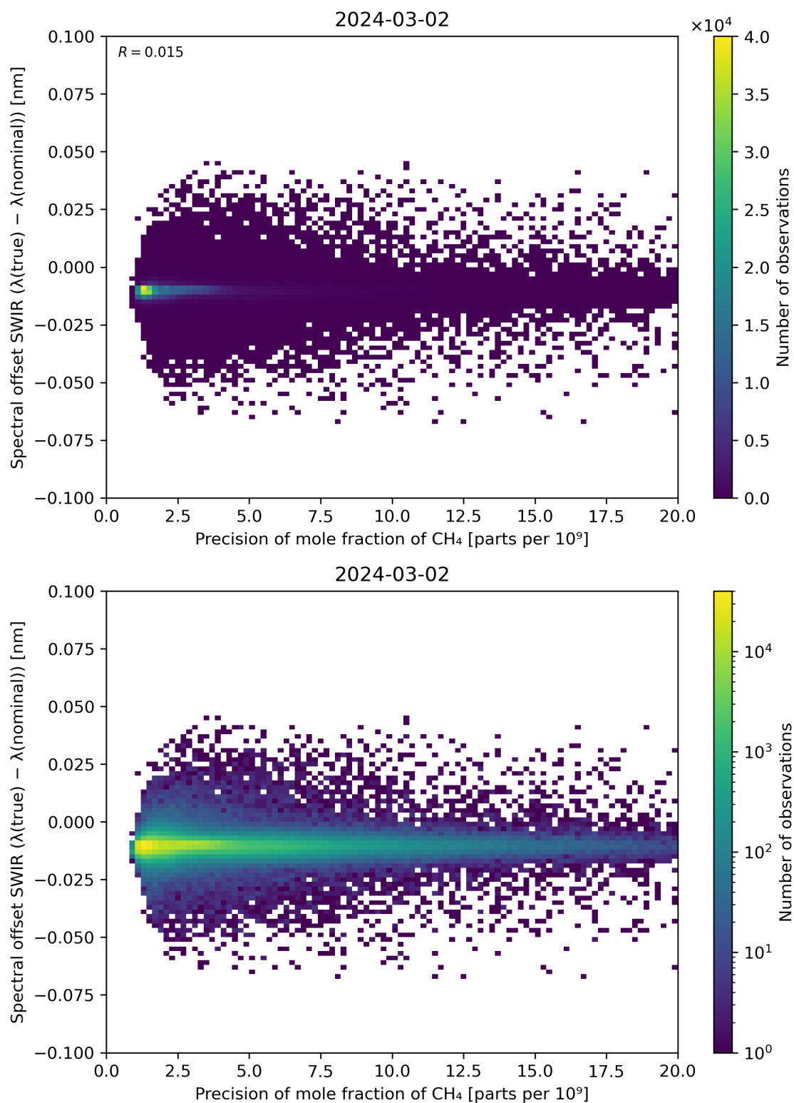
Figure 85: Scatter density plot of “Precision of mole fraction of \text{CH}_4 ” against “Spectral offset SWIR ( \lambda(\text{true}) - \lambda(\text{nominal}) )” for 2024-03-01 to 2024-03-03.
