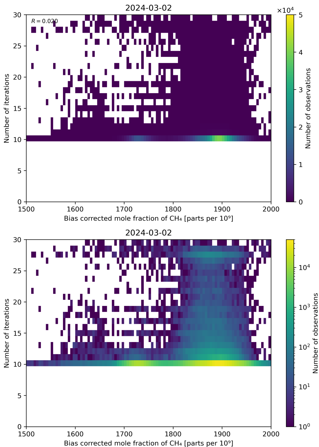
Figure 67: Scatter density plot of “Bias corrected mole fraction of \text{CH}_4 ” against “Number of iterations” for 2024-03-01 to 2024-03-03.
