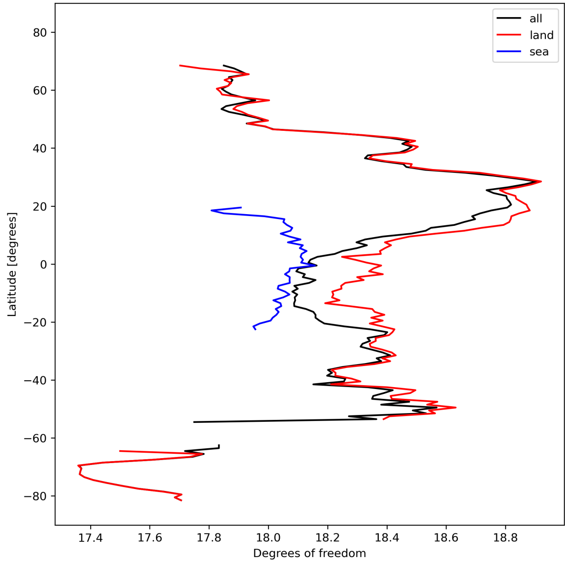
Figure 19: Zonal average of “Degrees of freedom” for 2024-03-01 to 2024-03-03.
