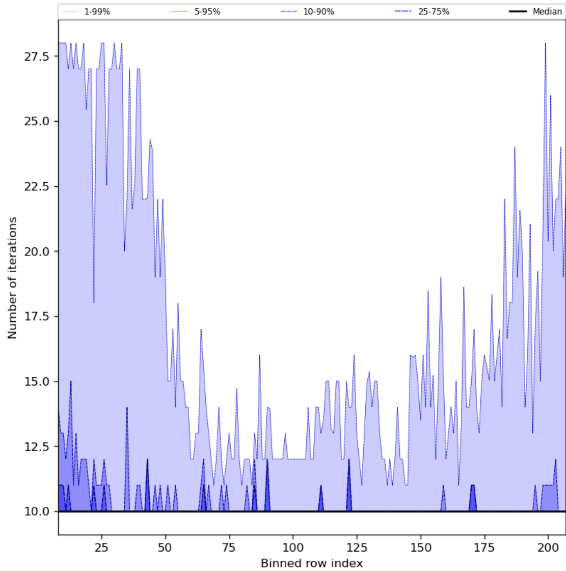
Figure 42: Along track statistics of “Number of iterations” for 2024-03-01 to 2024-03-03
