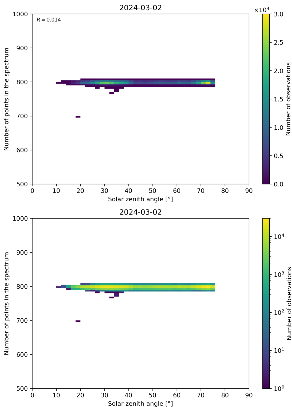
Figure 103: Scatter density plot of “Solar zenith angle” against “Number of points in the spectrum” for 2024-03-01 to 2024-03-03.
