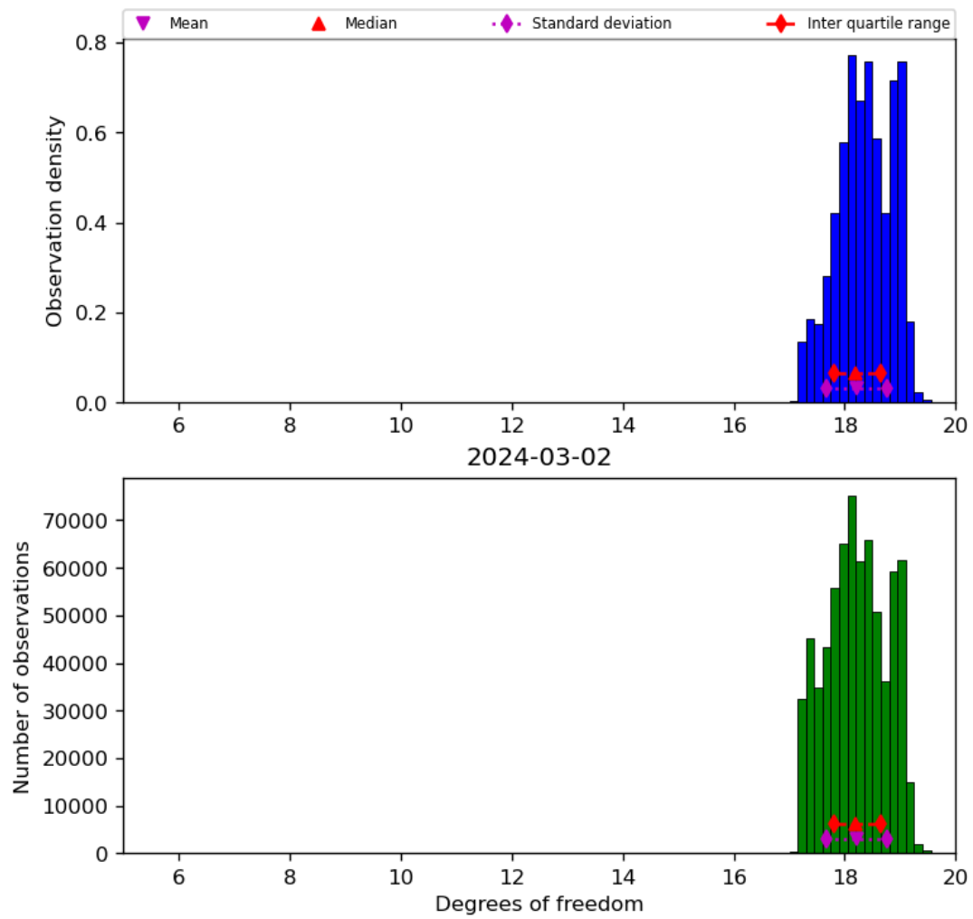
Figure 30: Histogram of “Degrees of freedom” for 2024-03-01 to 2024-03-03
