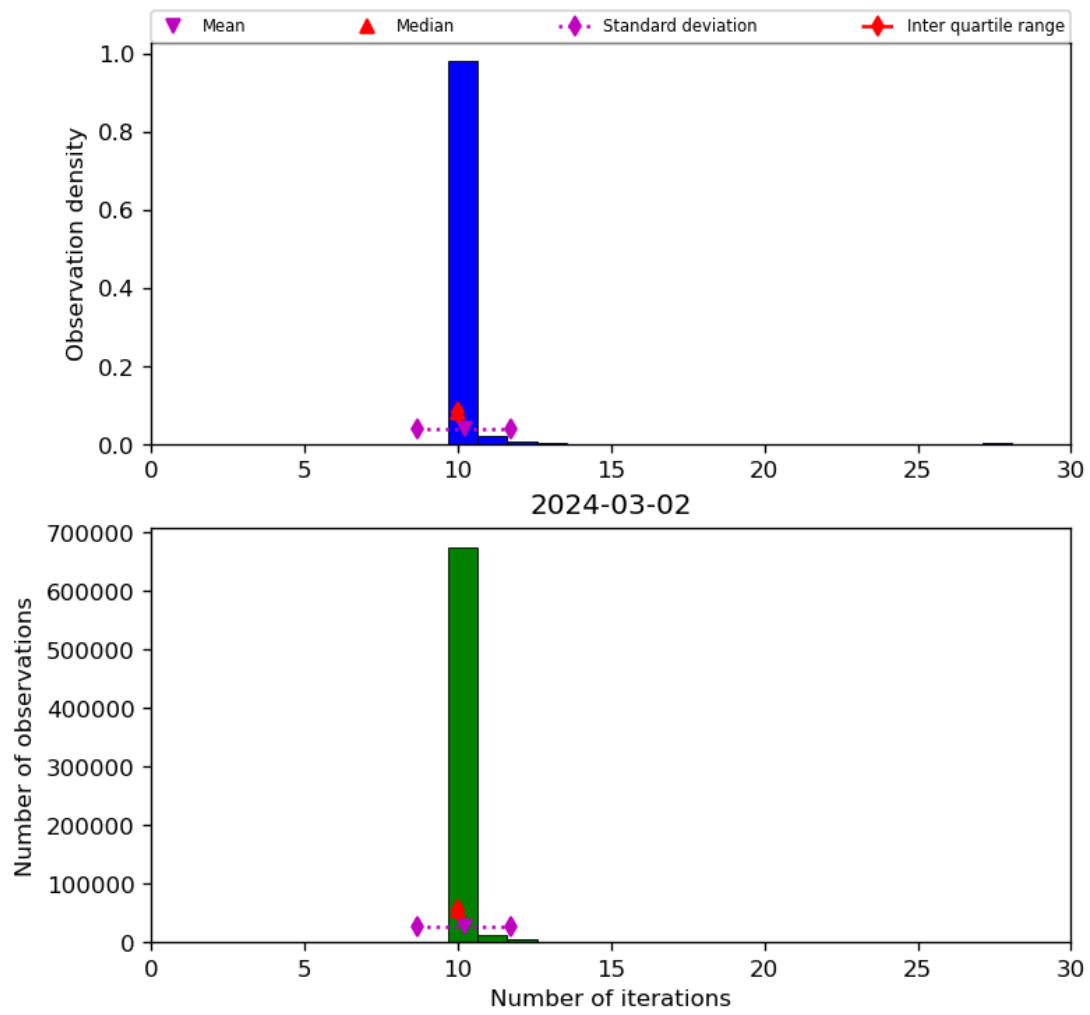
Figure 31: Histogram of “Number of iterations” for 2024-03-01 to 2024-03-03
