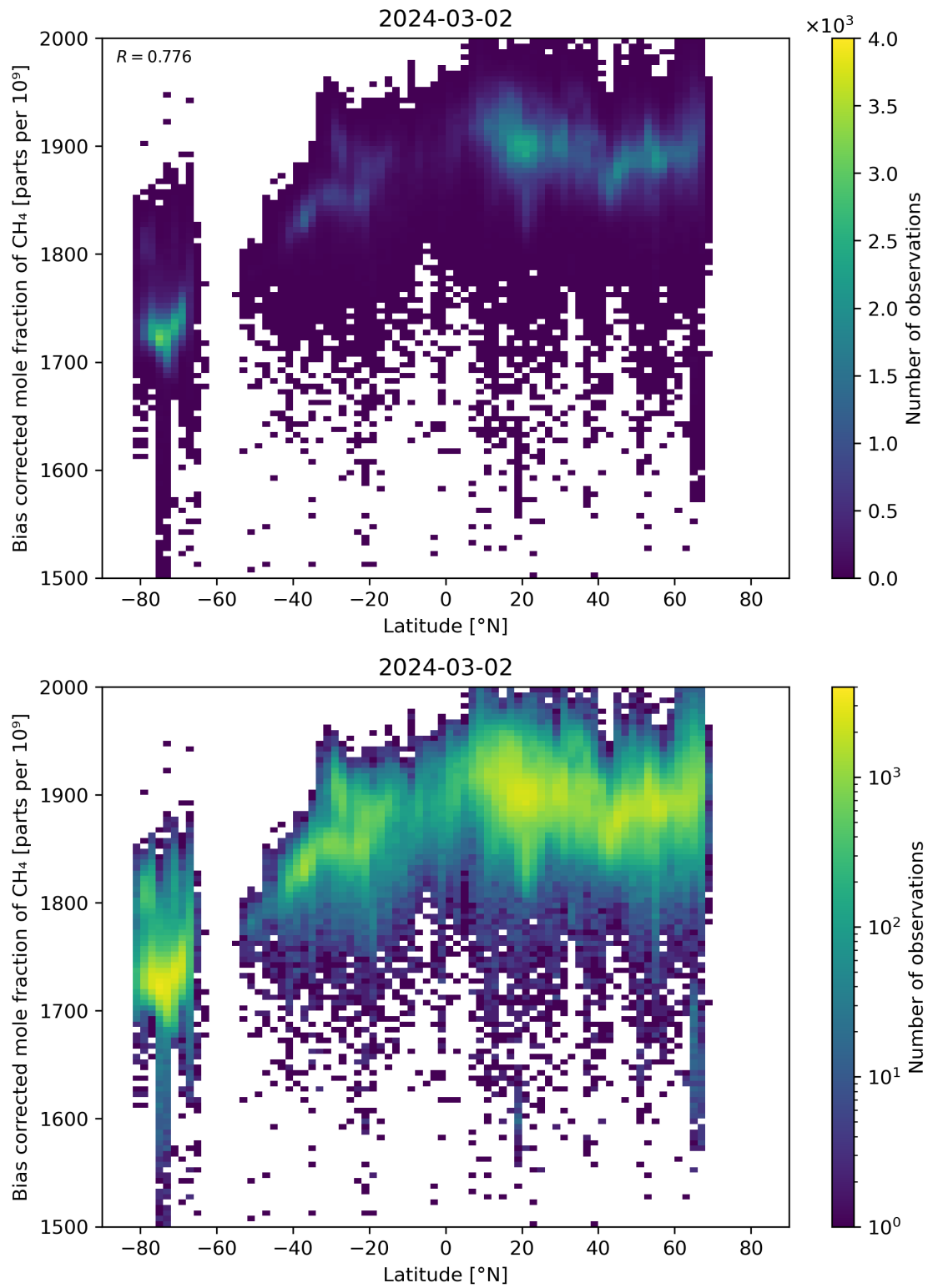
Figure 58: Scatter density plot of “Latitude” against “Bias corrected mole fraction of CH 4 ” for 2024-03-01 to 2024-03-03.
