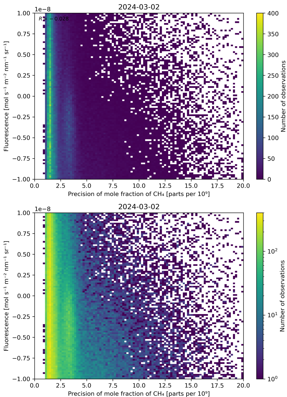
Figure 81: Scatter density plot of “Precision of mole fraction of \text{CH}_4 ” against “Fluorescence” for 2024-03-01 to 2024-03-03.
