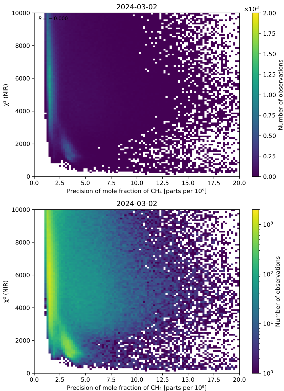
Figure 78: Scatter density plot of “Precision of mole fraction of CH 4 ” against “ \chi^2 (NIR)” for 2024-03-01 to 2024-03-03.
