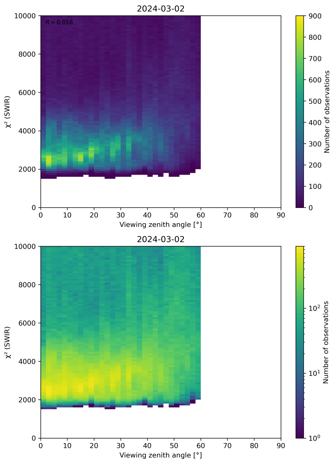
Figure 106: Scatter density plot of “Viewing zenith angle” against “ \chi^2 (SWIR)” for 2024-03-01 to 2024-03-03.
