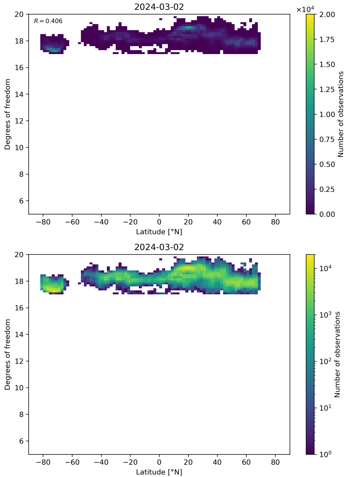
Figure 55: Scatter density plot of “Latitude” against “Degrees of freedom” for 2024-03-01 to 2024-03-03.
