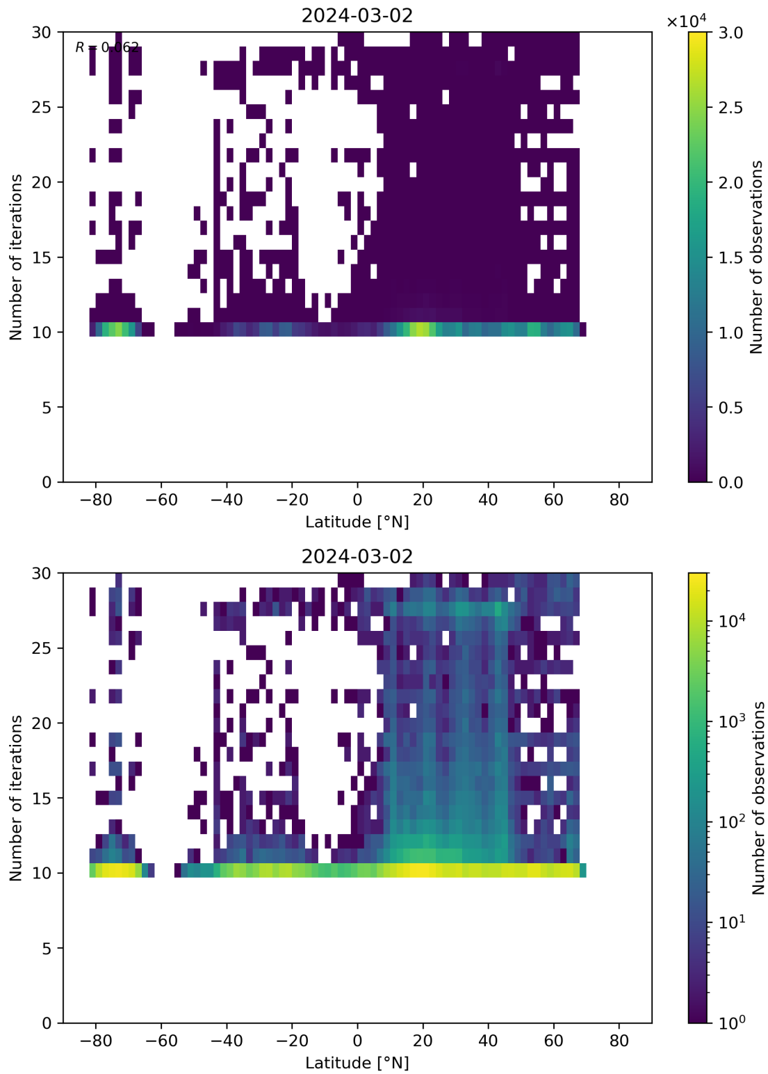
Figure 60: Scatter density plot of “Latitude” against “Number of iterations” for 2024-03-01 to 2024-03-03.
