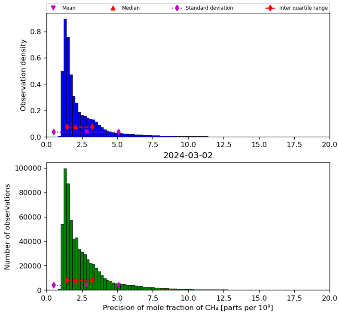
Figure 24: Histogram of “Precision of mole fraction of CH 4 ” for 2024-03-01 to 2024-03-03
