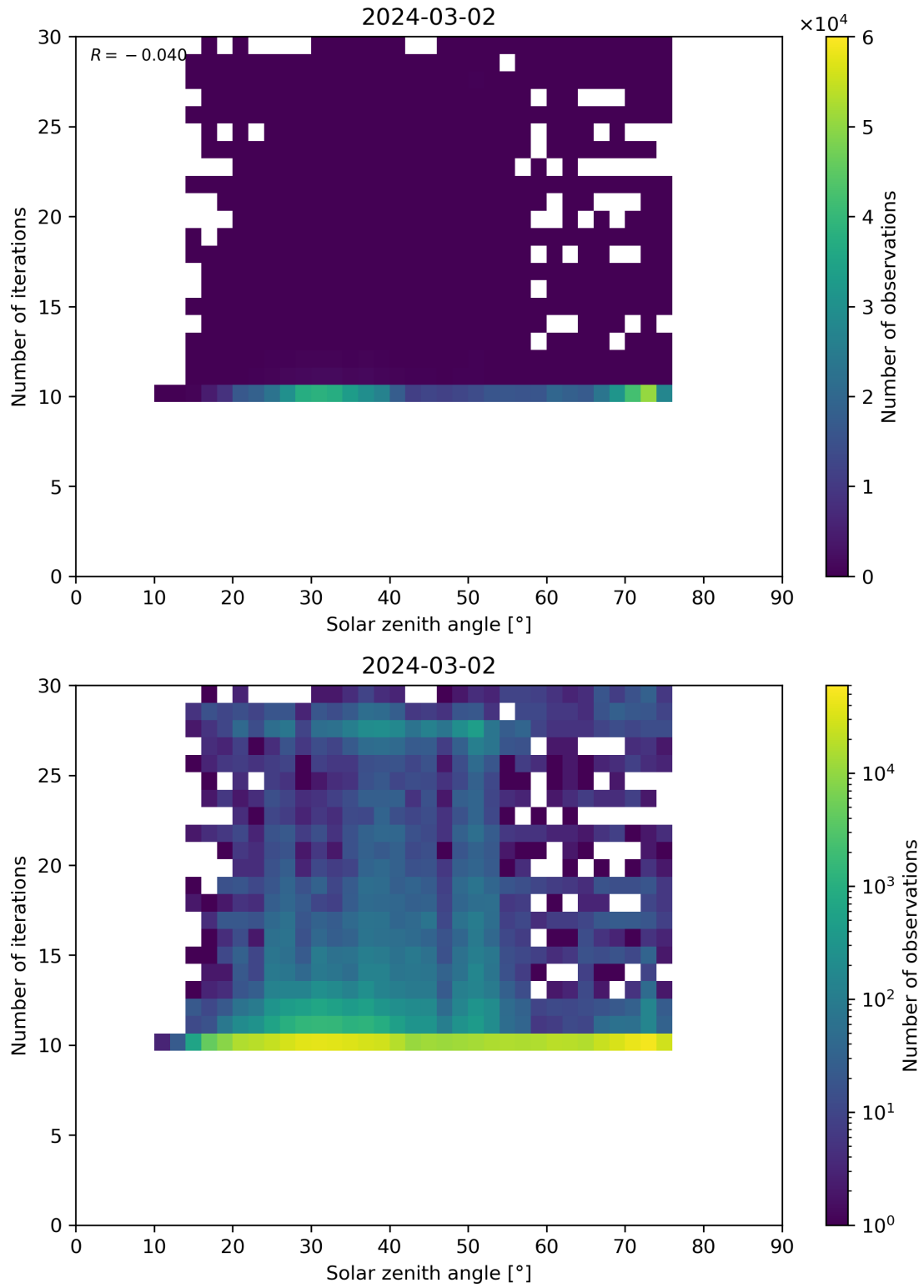
Figure 102: Scatter density plot of “Solar zenith angle” against “Number of iterations” for 2024-03-01 to 2024-03-03.
