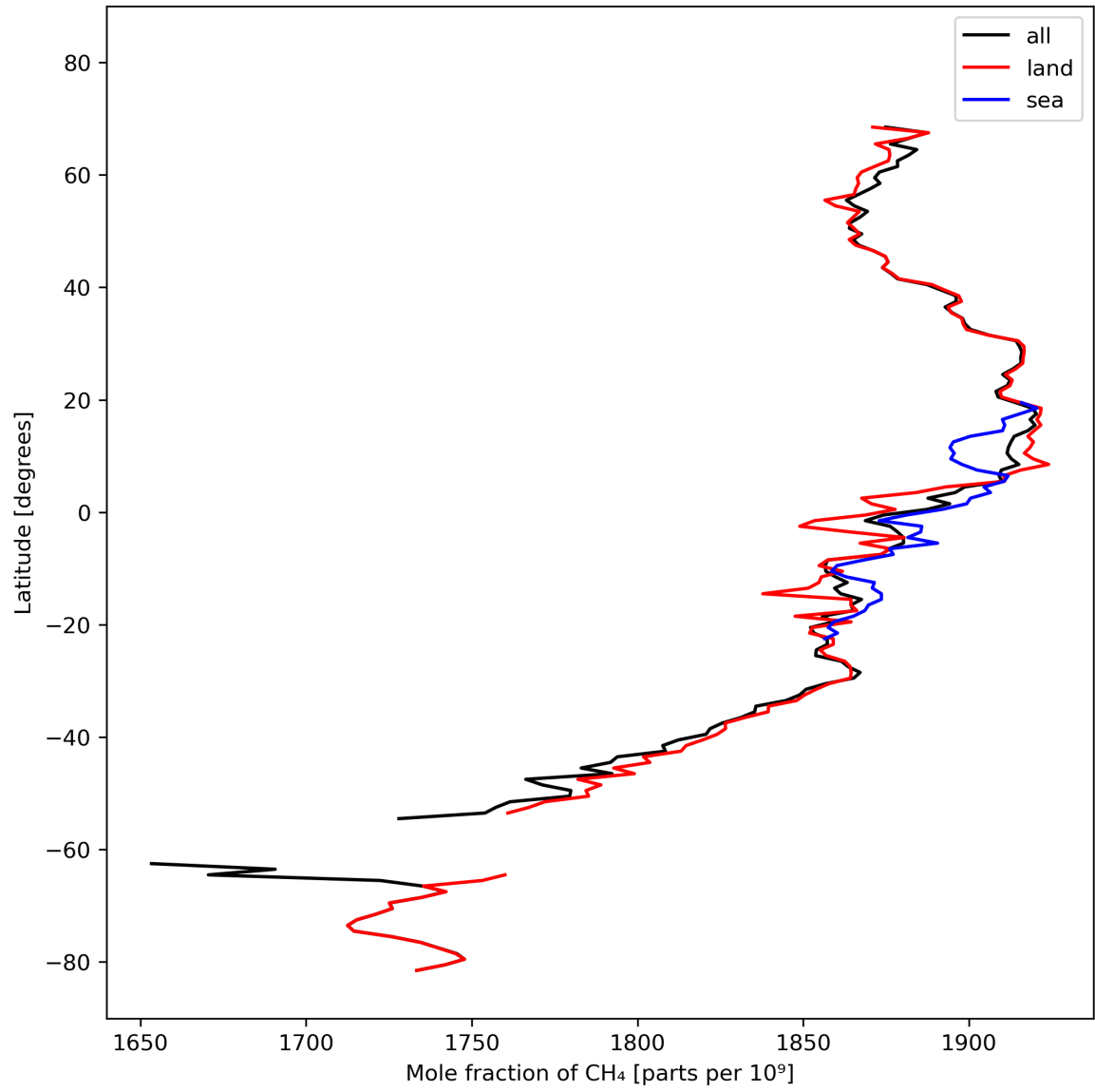
Figure 12: Zonal average of “Mole fraction of \text{CH}_4 ” for 2024-03-01 to 2024-03-03.
