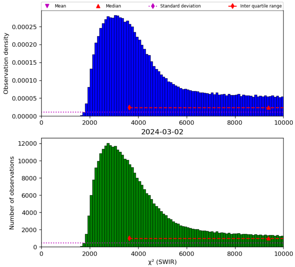
Figure 28: Histogram of “ \chi^2 (SWIR)” for 2024-03-01 to 2024-03-03
