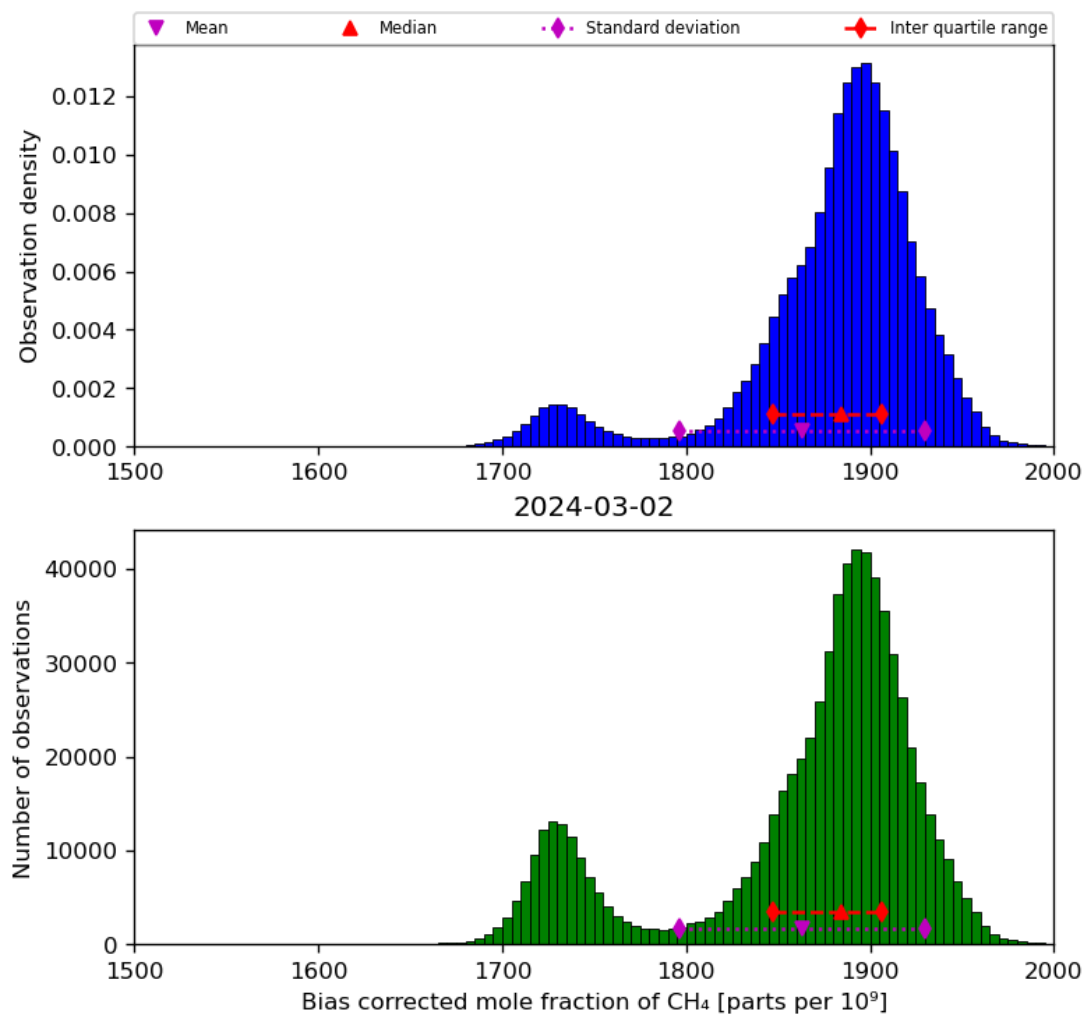
Figure 25: Histogram of “Bias corrected mole fraction of CH 4 ” for 2024-03-01 to 2024-03-03
