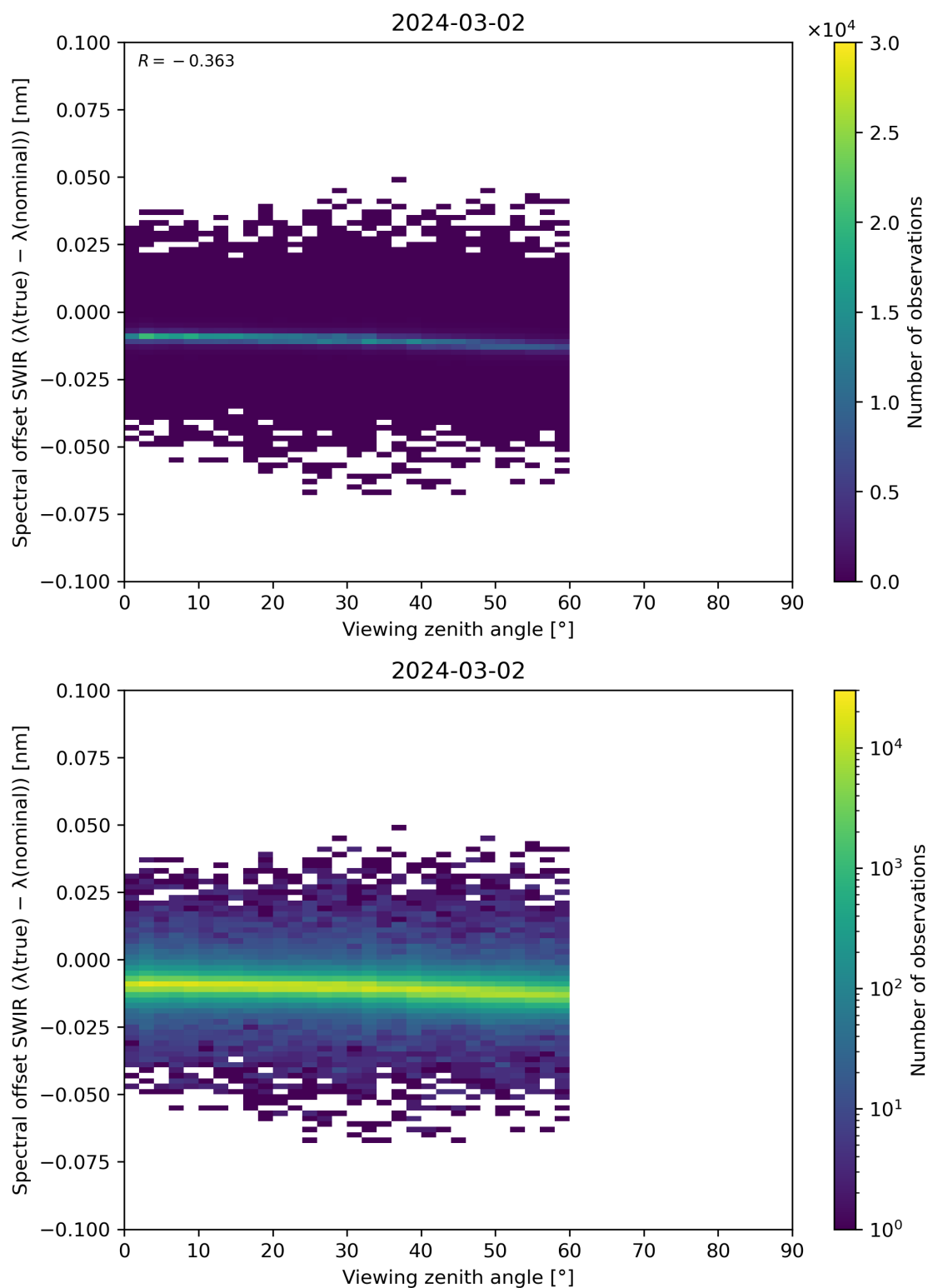
Figure 116: Scatter density plot of “Viewing zenith angle” against “Spectral offset SWIR ( \lambda(\text{true}) - \lambda(\text{nominal}) )” for 2024-03-01 to 2024-03-03.
