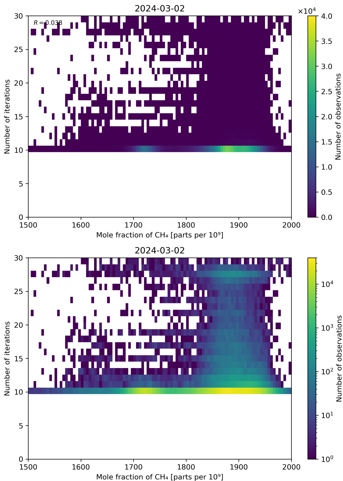
Figure 76: Scatter density plot of “Mole fraction of CH 4 ” against “Number of iterations” for 2024-03-01 to 2024-03-03.
