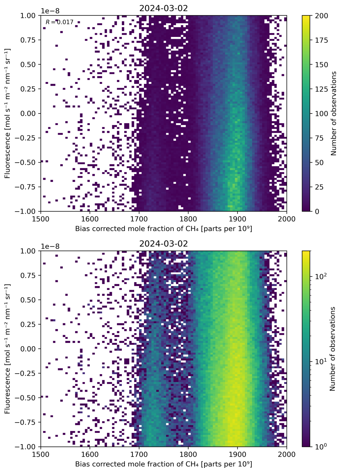
Figure 66: Scatter density plot of “Bias corrected mole fraction of \text{CH}_4 ” against “Fluorescence” for 2024-03-01 to 2024-03-03.
