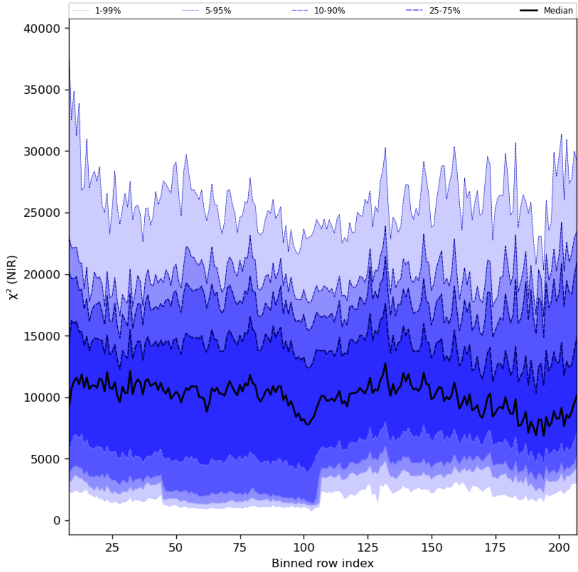
Figure 40: Along track statistics of “ \chi^2 (NIR)” for 2024-03-01 to 2024-03-03
