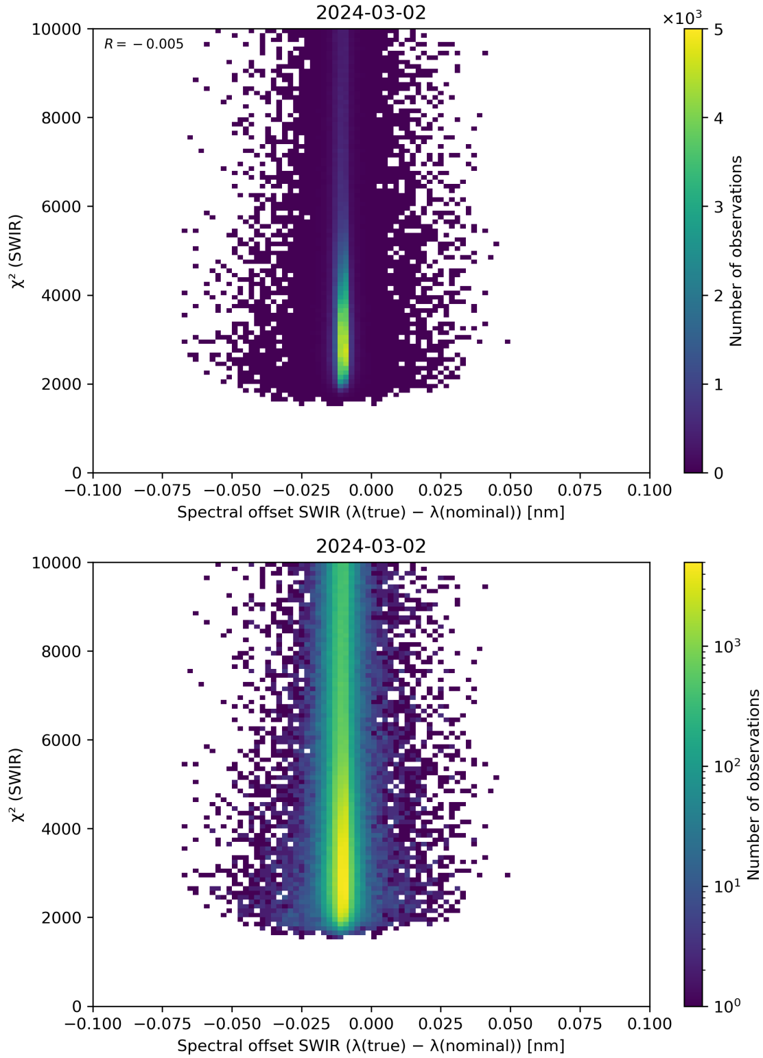
Figure 118: Scatter density plot of “Spectral offset SWIR ( \lambda(\text{true}) - \lambda(\text{nominal}) )” against “ \chi^2 (SWIR)” for 2024-03-01 to 2024-03-03.
