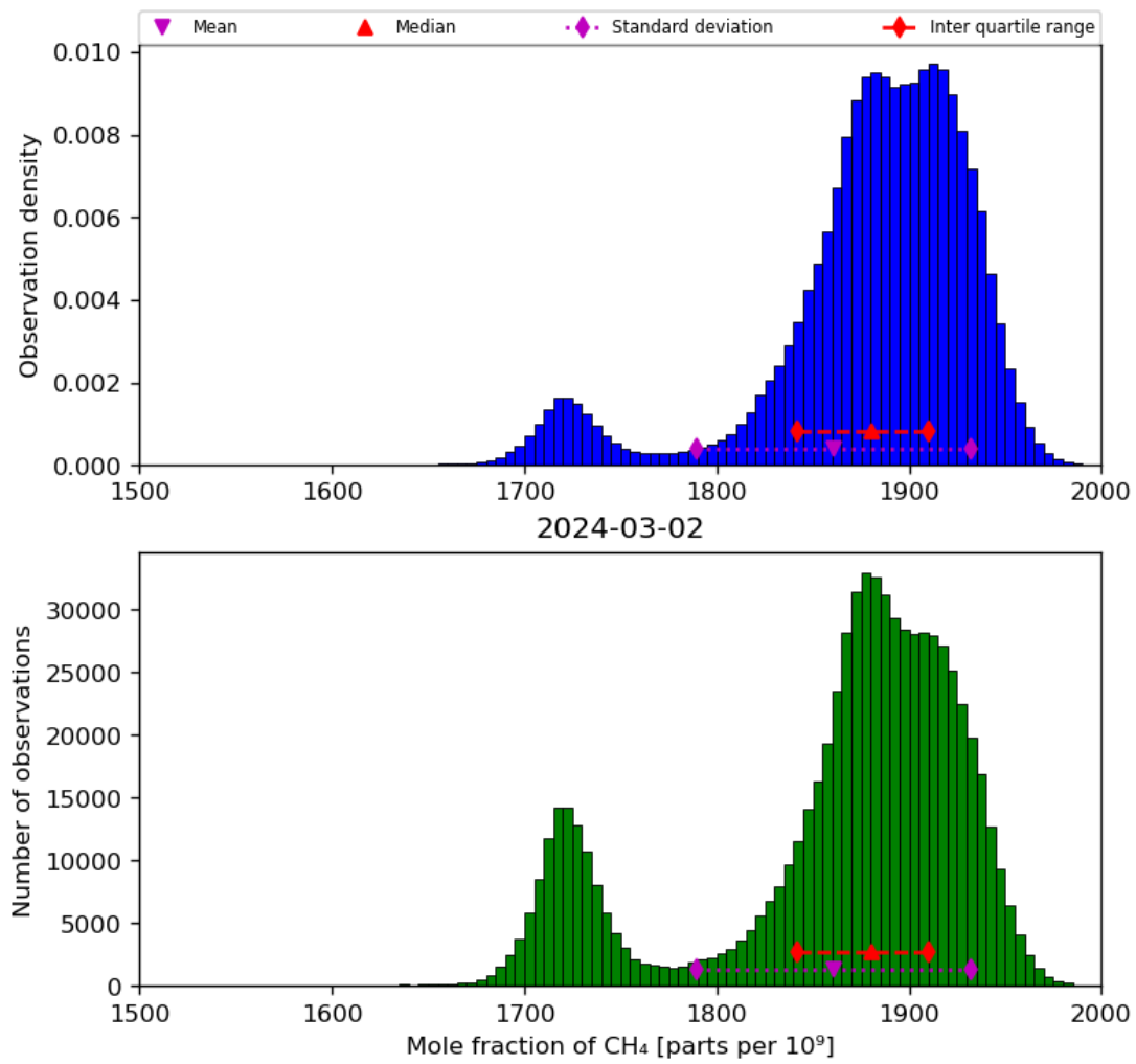
Figure 23: Histogram of “Mole fraction of CH 4 ” for 2024-03-01 to 2024-03-03
