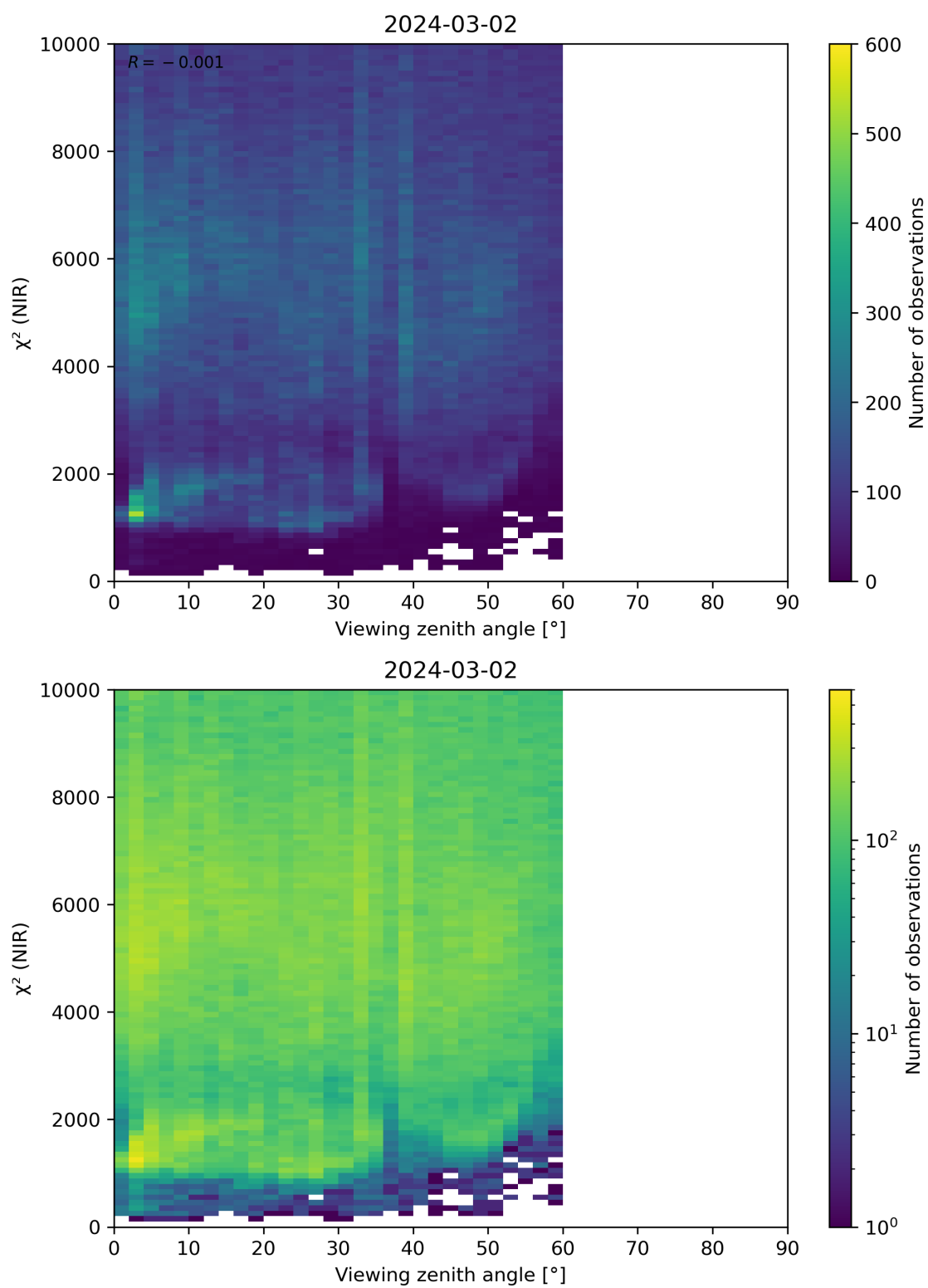
Figure 105: Scatter density plot of “Viewing zenith angle” against “ \chi^2 (NIR)” for 2024-03-01 to 2024-03-03.
