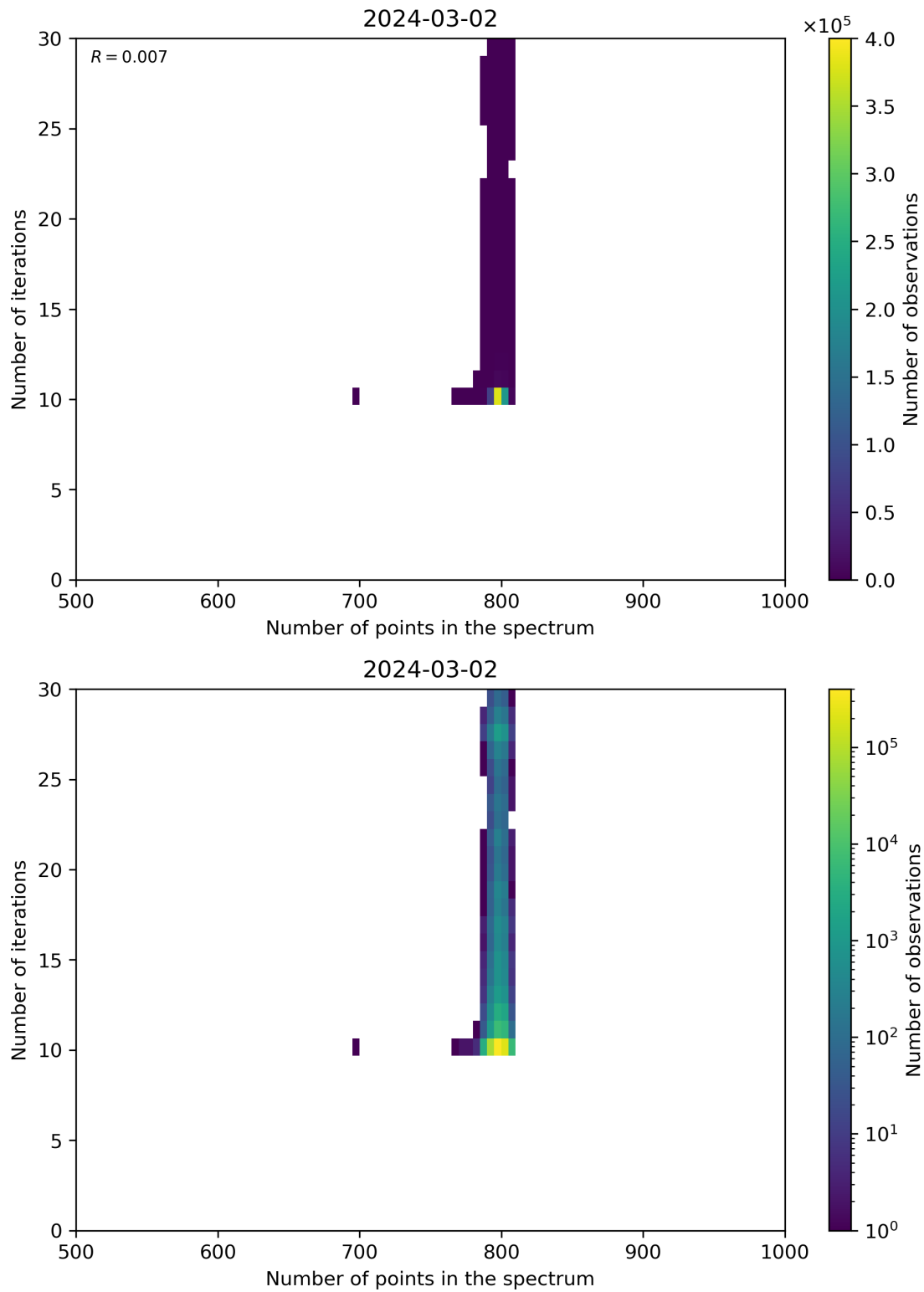
Figure 92: Scatter density plot of “Number of points in the spectrum” against “Number of iterations” for 2024-03-01 to 2024-03-03.
