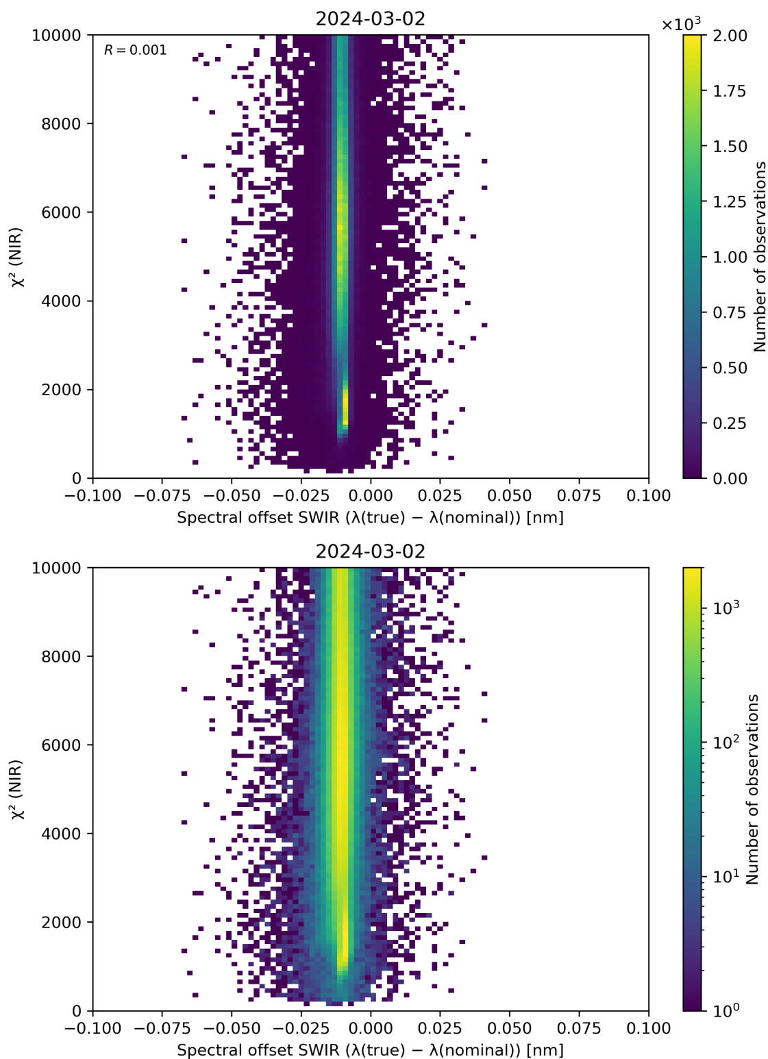
Figure 117: Scatter density plot of “Spectral offset SWIR ( \lambda(\text{true}) - \lambda(\text{nominal}) )” against “ \chi^2 (NIR)” for 2024-03-01 to 2024-03-03.
