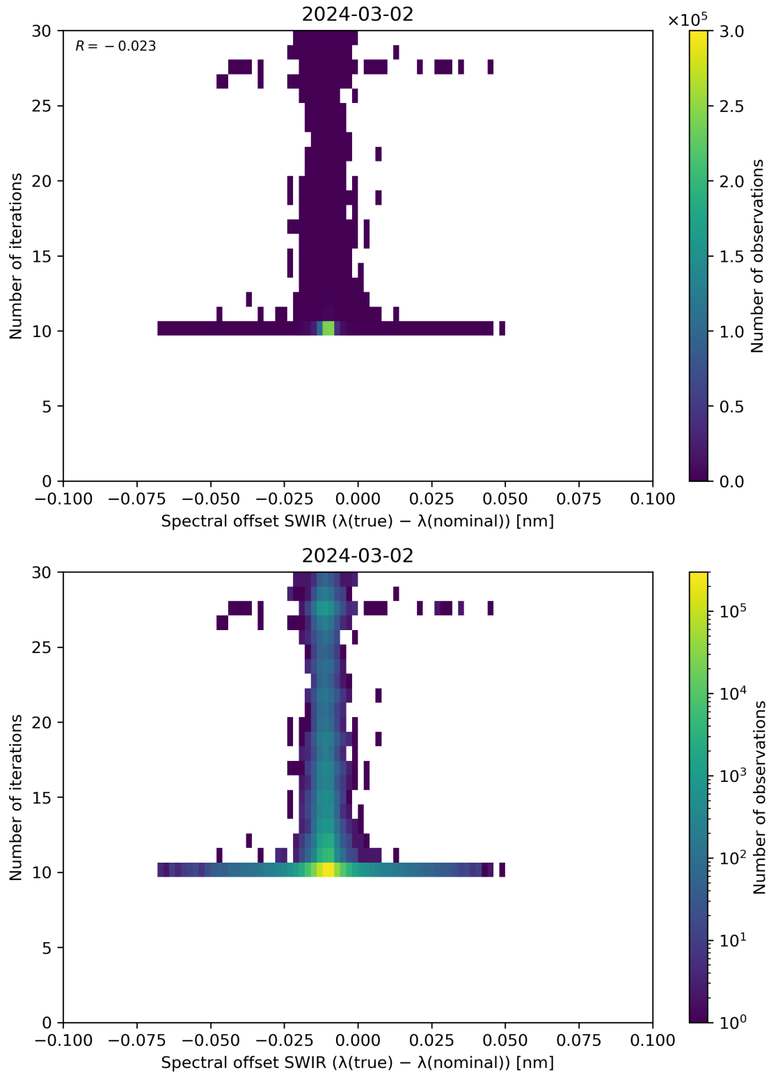
Figure 121: Scatter density plot of “Spectral offset SWIR ( \lambda(\text{true}) - \lambda(\text{nominal}) )” against “Number of iterations” for 2024-03-01 to 2024-03-03.
