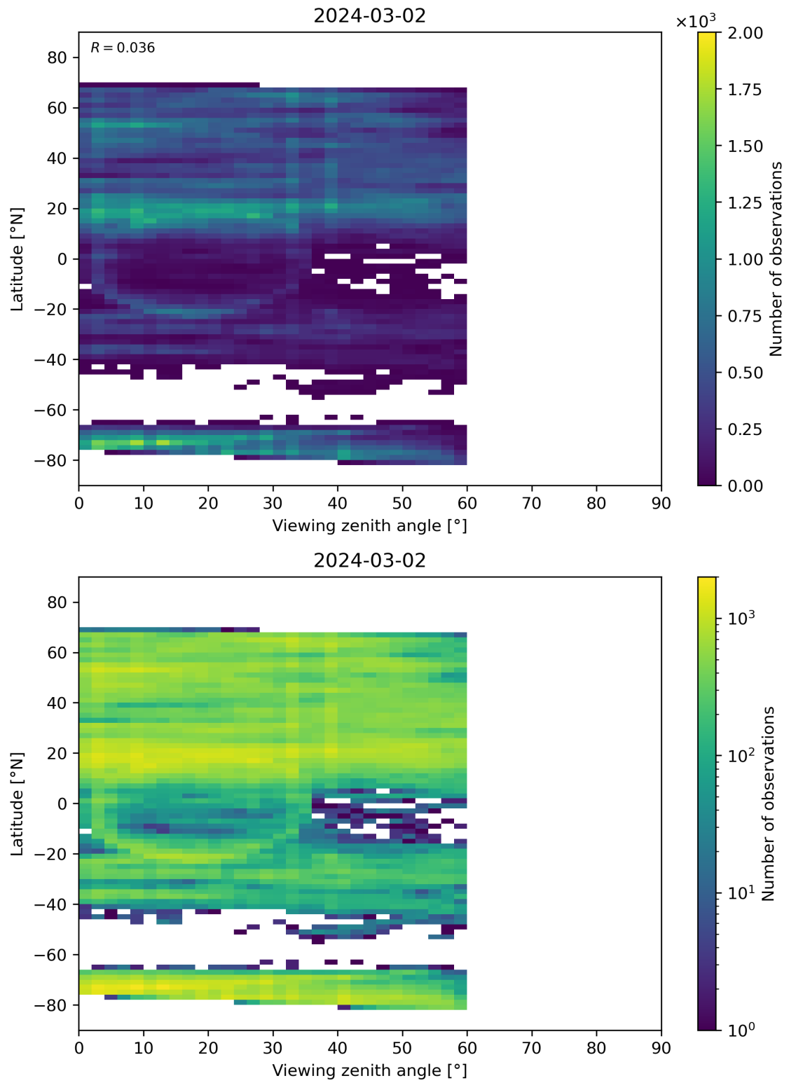
Figure 109: Scatter density plot of “Viewing zenith angle” against “Latitude” for 2024-03-01 to 2024-03-03.
