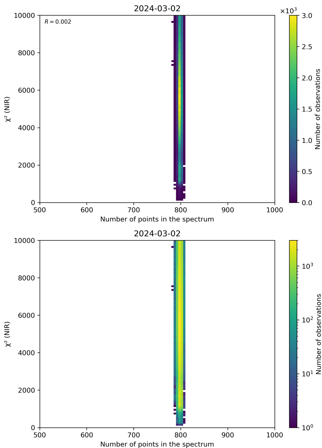
Figure 88: Scatter density plot of “Number of points in the spectrum” against “ \chi^2 (NIR)” for 2024-03-01 to 2024-03-03.
