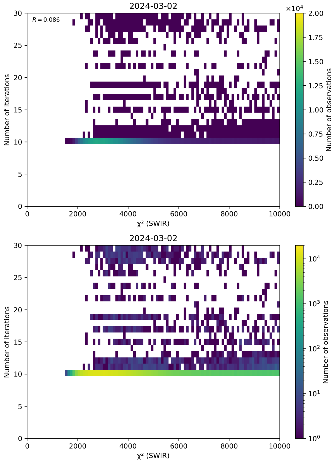
Figure 50: Scatter density plot of “ \chi^2 (SWIR)” against “Number of iterations” for 2024-03-01 to 2024-03-03.
