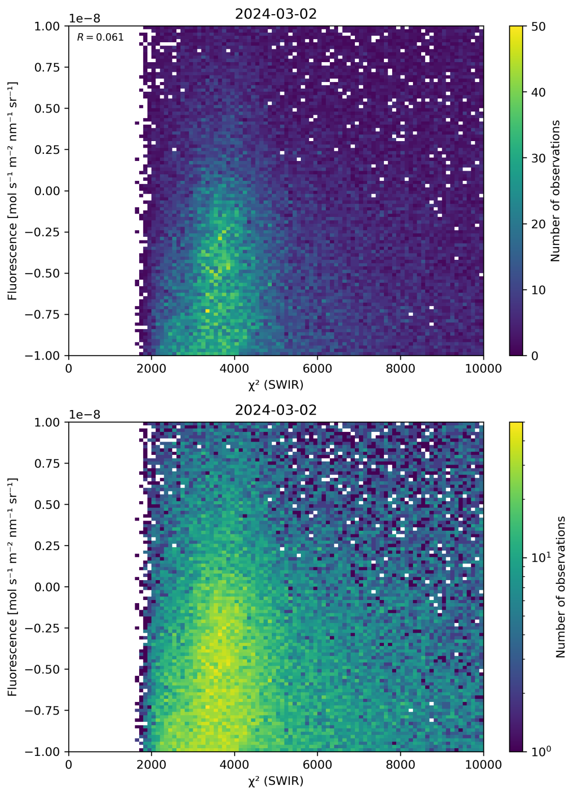
Figure 49: Scatter density plot of “ \chi^2 (SWIR)” against “Fluorescence” for 2024-03-01 to 2024-03-03.
