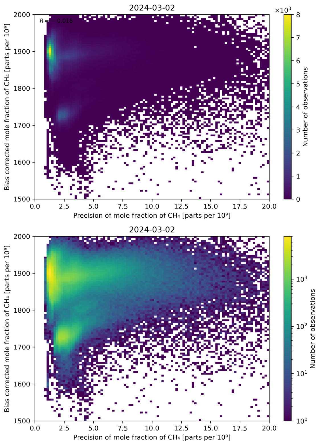
Figure 82: Scatter density plot of “Precision of mole fraction of \text{CH}_4 ” against “Bias corrected mole fraction of \text{CH}_4 ” for 2024-03-01 to 2024-03-03.
