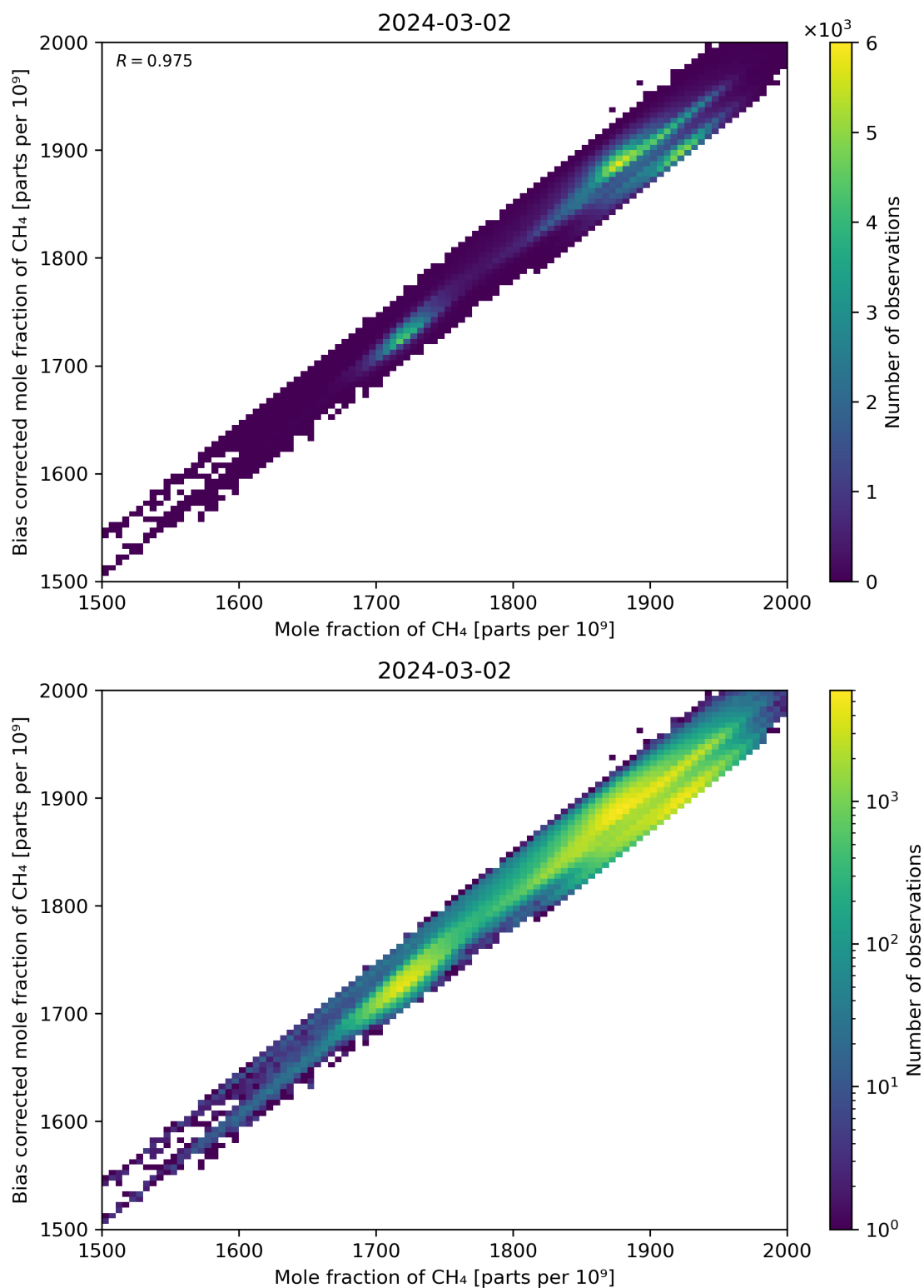
Figure 74: Scatter density plot of “Mole fraction of CH 4 ” against “Bias corrected mole fraction of CH 4 ” for 2024-03-01 to 2024-03-03.
