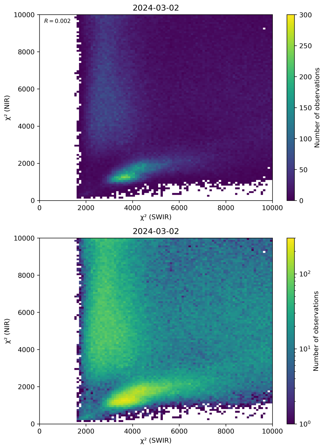
Figure 47: Scatter density plot of “ \chi^2 (SWIR)” against “ \chi^2 (NIR)” for 2024-03-01 to 2024-03-03.
