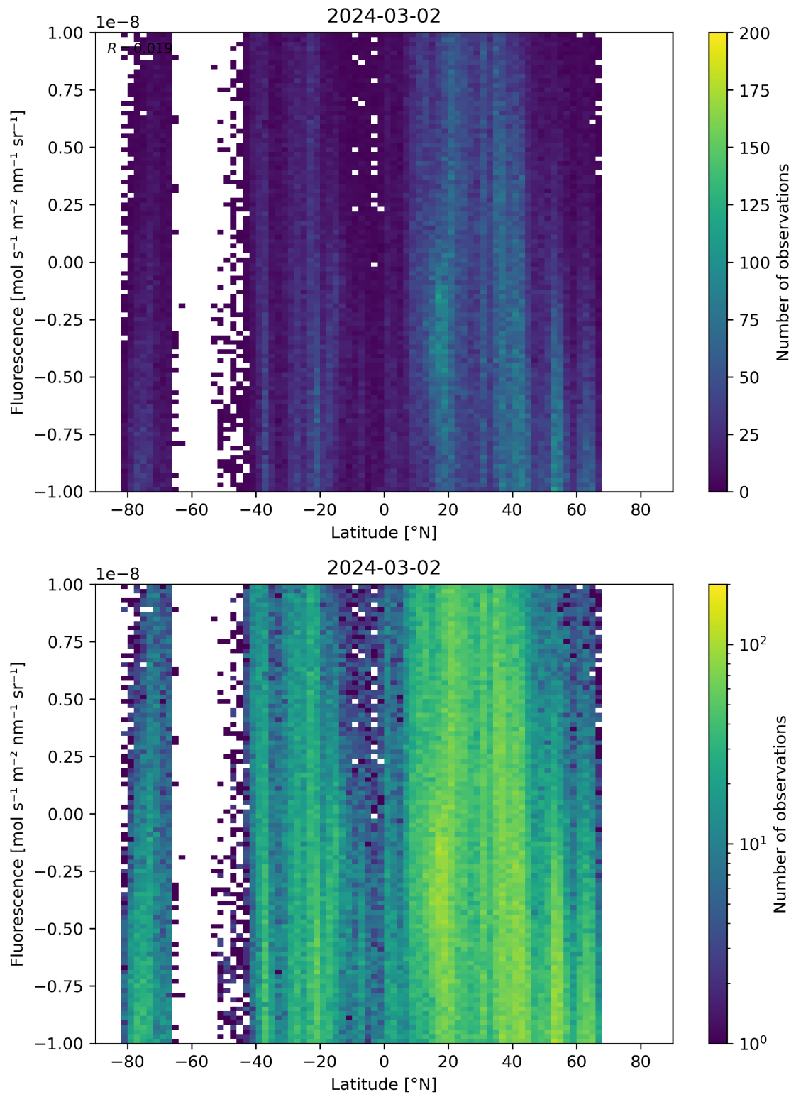
Figure 56: Scatter density plot of “Latitude” against “Fluorescence” for 2024-03-01 to 2024-03-03.
