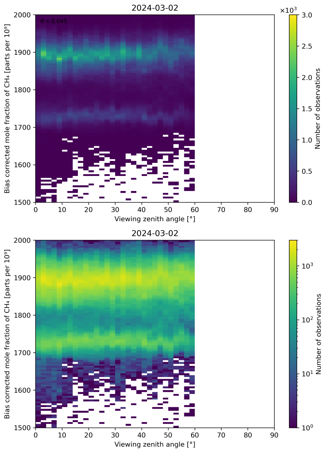
Figure 111: Scatter density plot of “Viewing zenith angle” against “Bias corrected mole fraction of CH 4 ” for 2024-03-01 to 2024-03-03.
