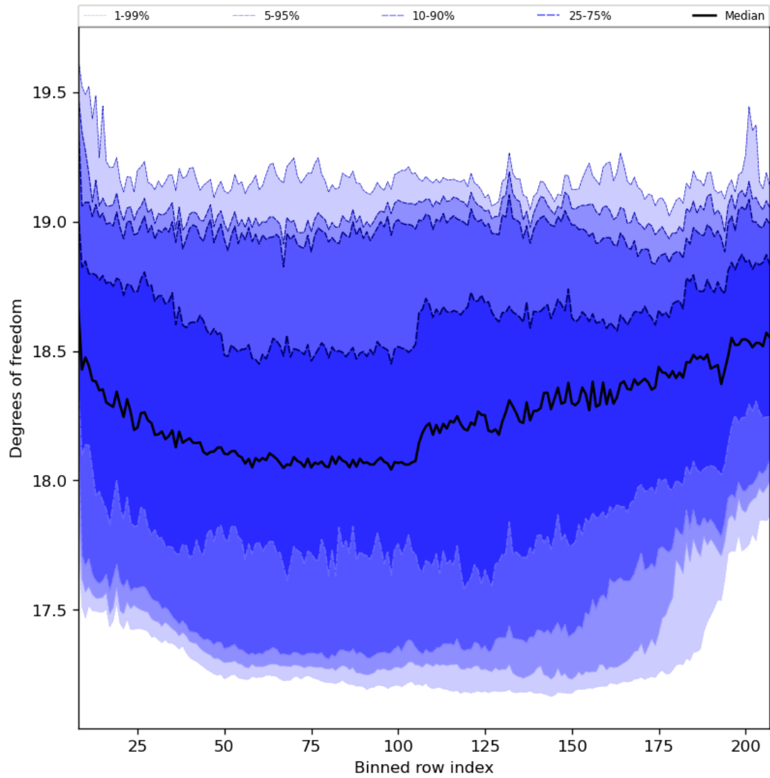
Figure 41: Along track statistics of “Degrees of freedom” for 2024-03-01 to 2024-03-03
