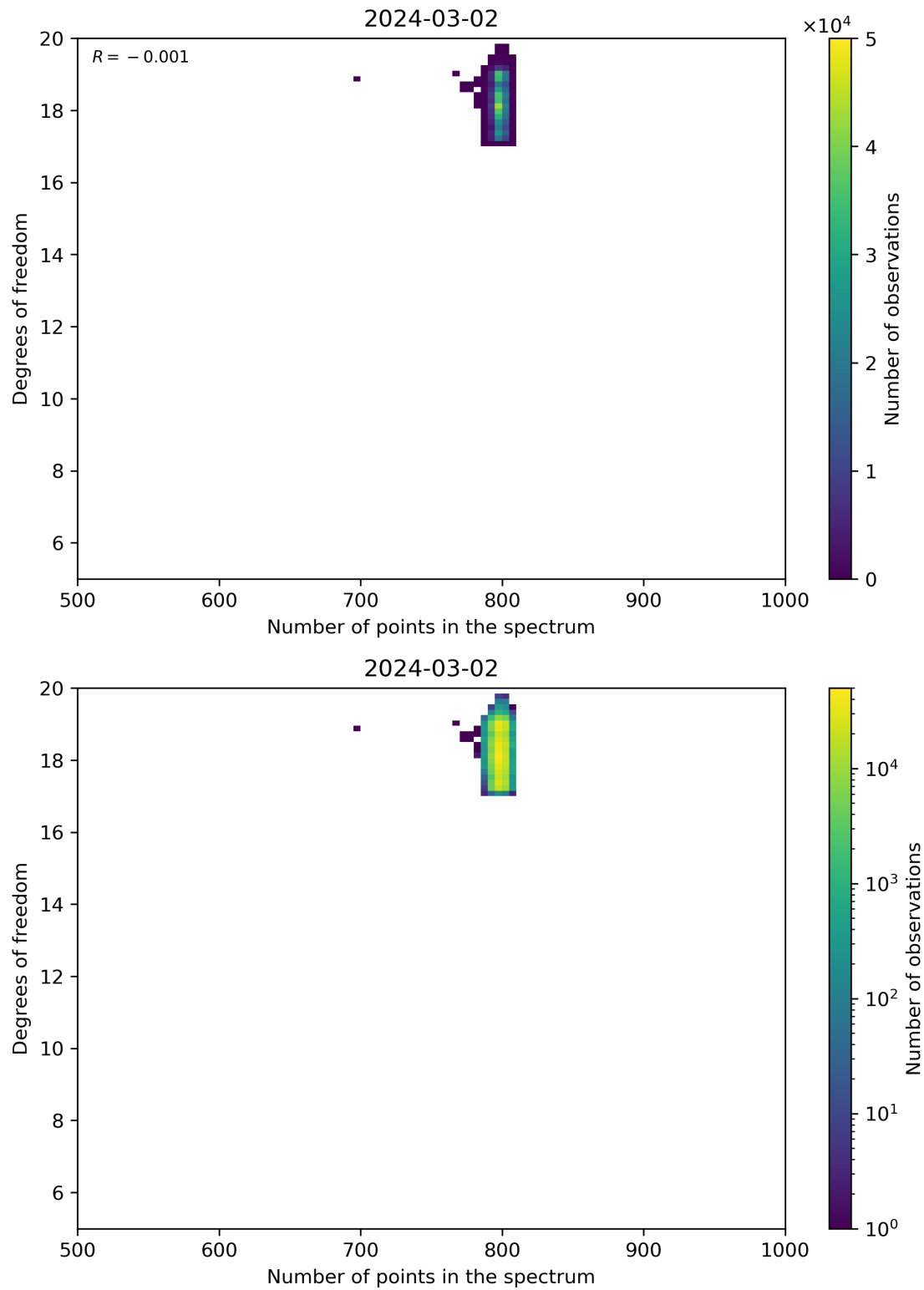
Figure 90: Scatter density plot of “Number of points in the spectrum” against “Degrees of freedom” for 2024-03-01 to 2024-03-03.
