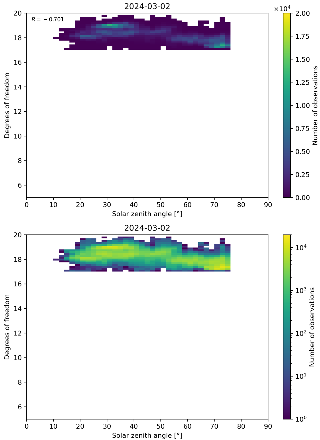
Figure 96: Scatter density plot of “Solar zenith angle” against “Degrees of freedom” for 2024-03-01 to 2024-03-03.
