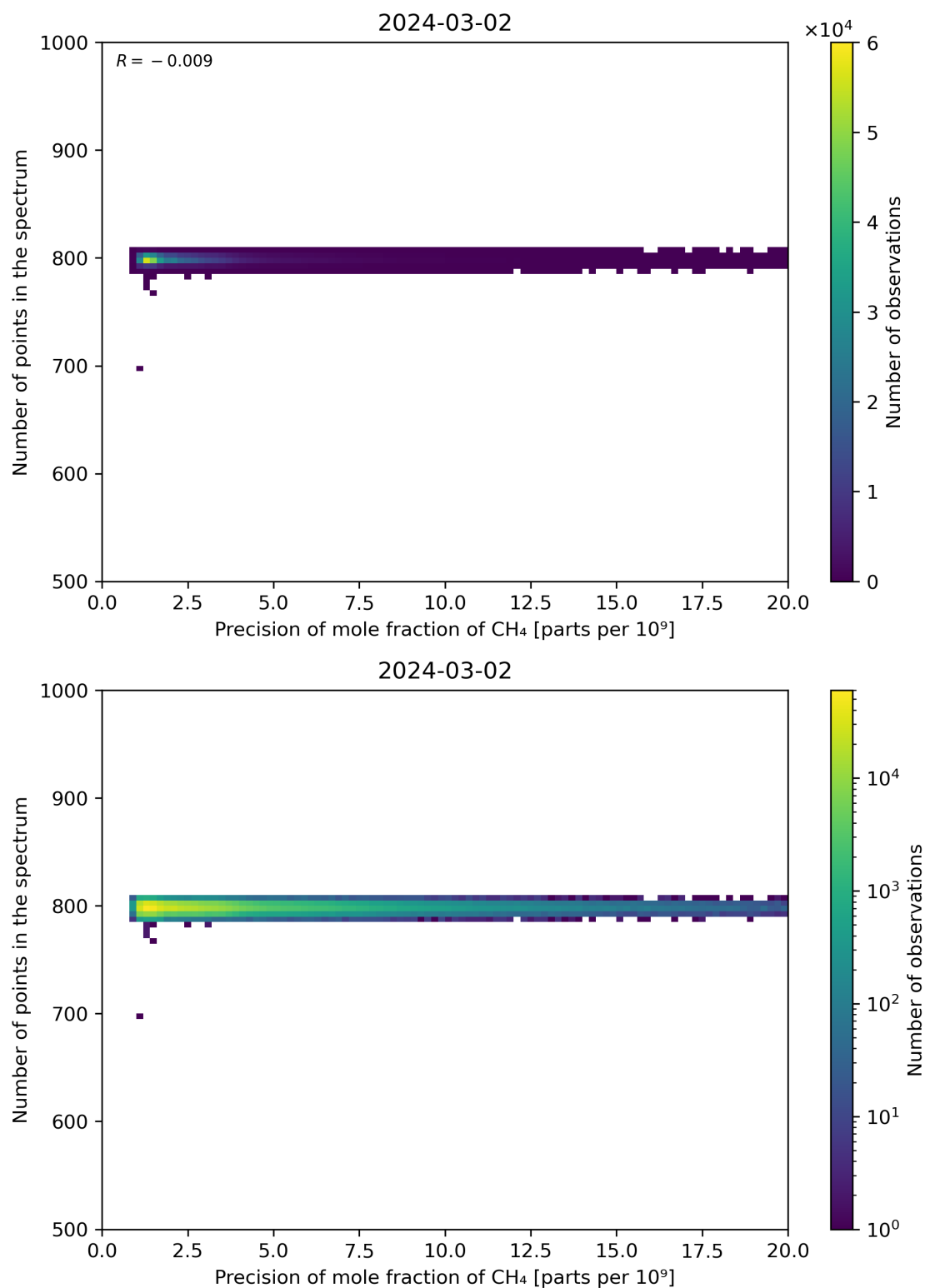
Figure 84: Scatter density plot of “Precision of mole fraction of CH 4 ” against “Number of points in the spectrum” for 2024-03-01 to 2024-03-03.
