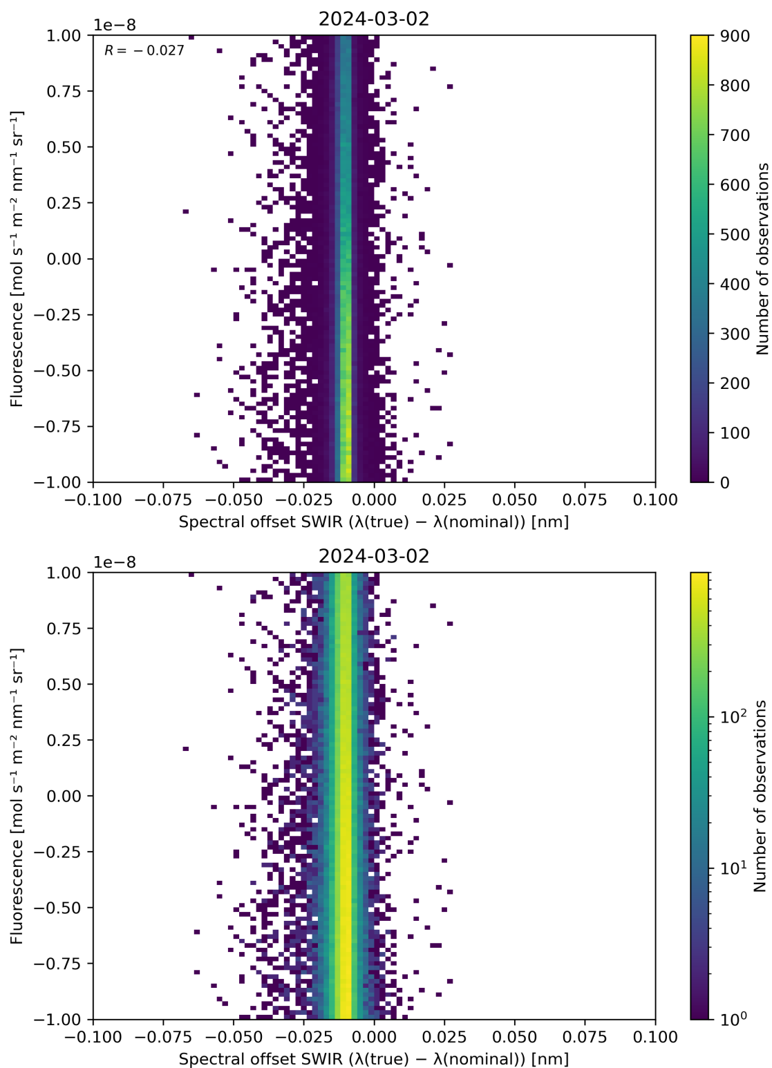
Figure 120: Scatter density plot of “Spectral offset SWIR ( \lambda(\text{true}) - \lambda(\text{nominal}) )” against “Fluorescence” for 2024-03-01 to 2024-03-03.
