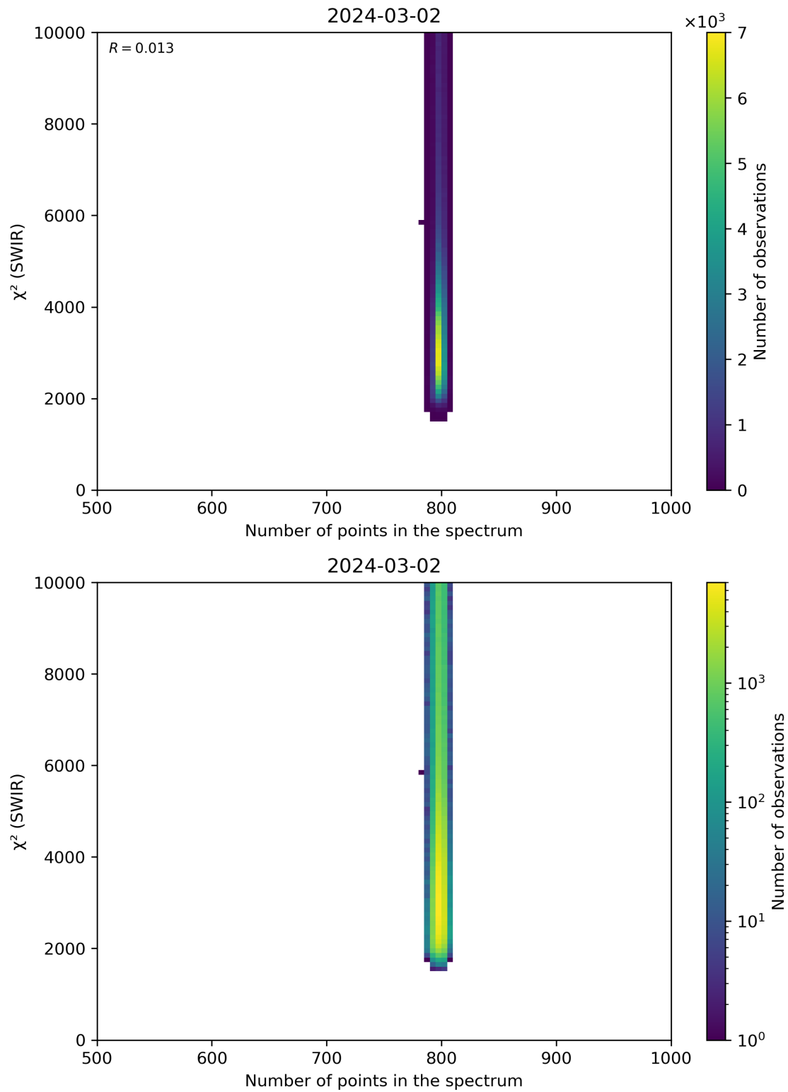
Figure 89: Scatter density plot of “Number of points in the spectrum” against “ \chi^2 (SWIR)” for 2024-03-01 to 2024-03-03.
