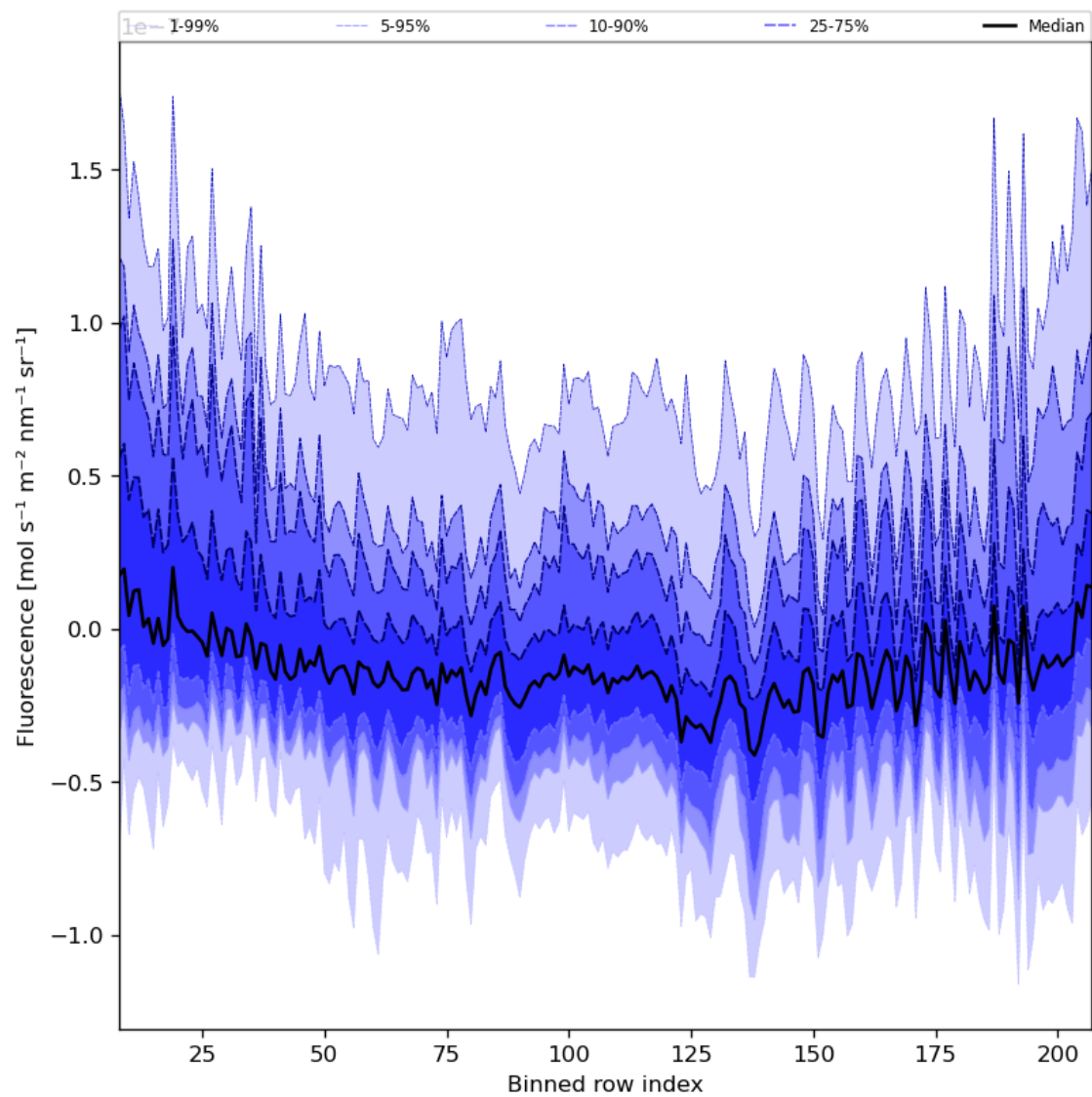
Figure 43: Along track statistics of “Fluorescence” for 2024-03-01 to 2024-03-03
