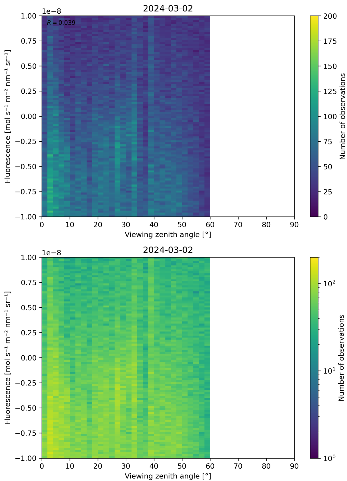
Figure 108: Scatter density plot of “Viewing zenith angle” against “Fluorescence” for 2024-03-01 to 2024-03-03.
