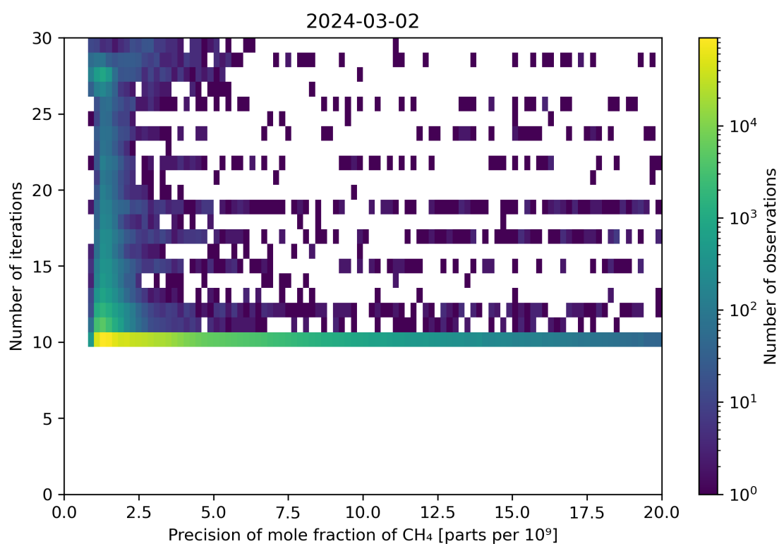
Figure 83: Scatter density plot of “Precision of mole fraction of CH 4 ” against “Number of iterations” for 2024-03-01 to 2024-03-03.
