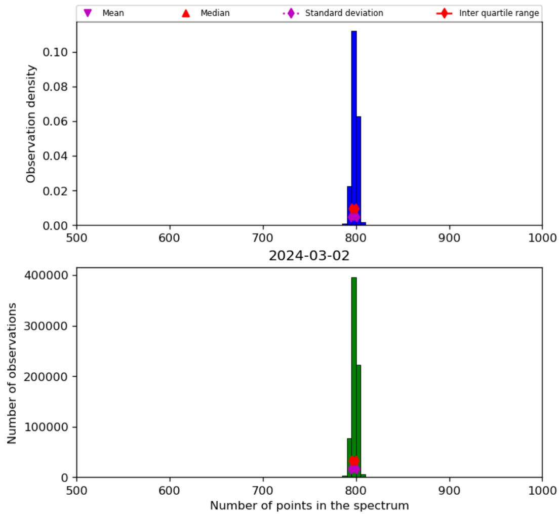
Figure 26: Histogram of “Number of points in the spectrum” for 2024-03-01 to 2024-03-03
