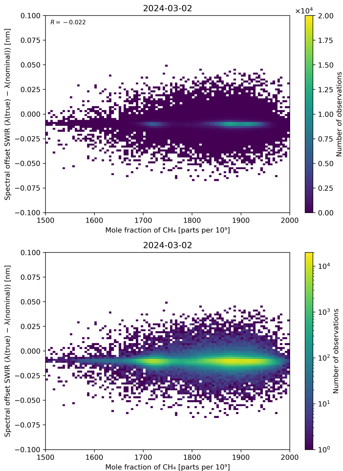
Figure 86: Scatter density plot of “Mole fraction of CH 4 ” against “Spectral offset SWIR ( \lambda(\text{true}) - \lambda(\text{nominal}) )” for 2024-03-01 to 2024-03-03.
