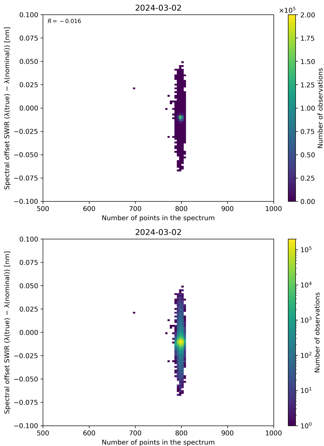
Figure 93: Scatter density plot of “Number of points in the spectrum” against “Spectral offset SWIR ( \lambda(\text{true}) - \lambda(\text{nominal}) )” for 2024-03-01 to 2024-03-03.
