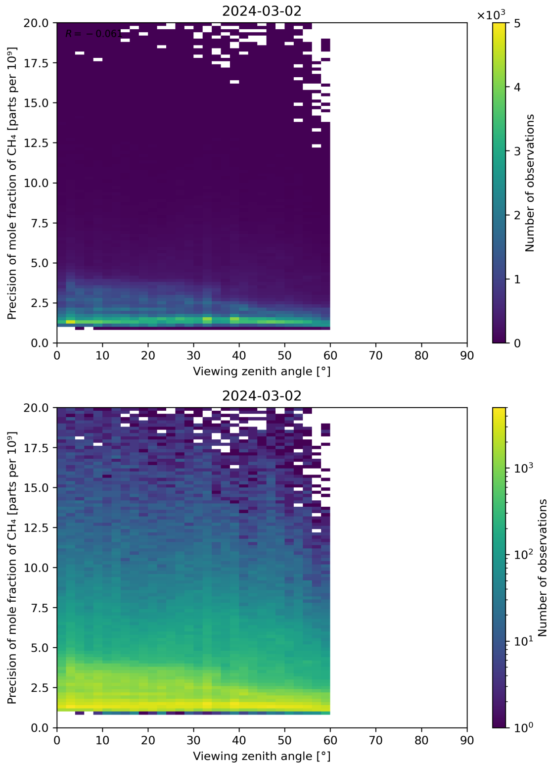
Figure 112: Scatter density plot of “Viewing zenith angle” against “Precision of mole fraction of CH 4 ” for 2024-03-01 to 2024-03-03.
