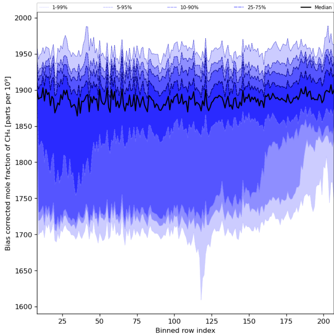
Figure 36: Along track statistics of “Bias corrected mole fraction of CH 4 ” for 2024-03-01 to 2024-03-03
