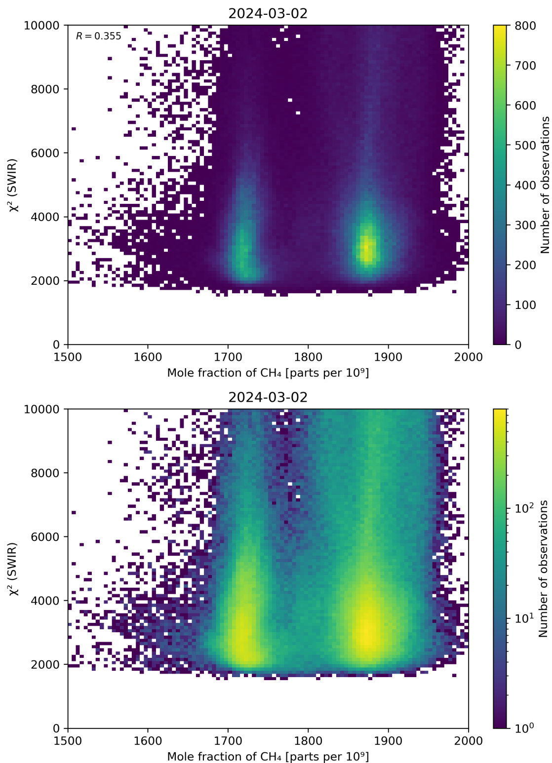
Figure 71: Scatter density plot of “Mole fraction of \text{CH}_4 ” against “ \chi^2 (SWIR)” for 2024-03-01 to 2024-03-03.
