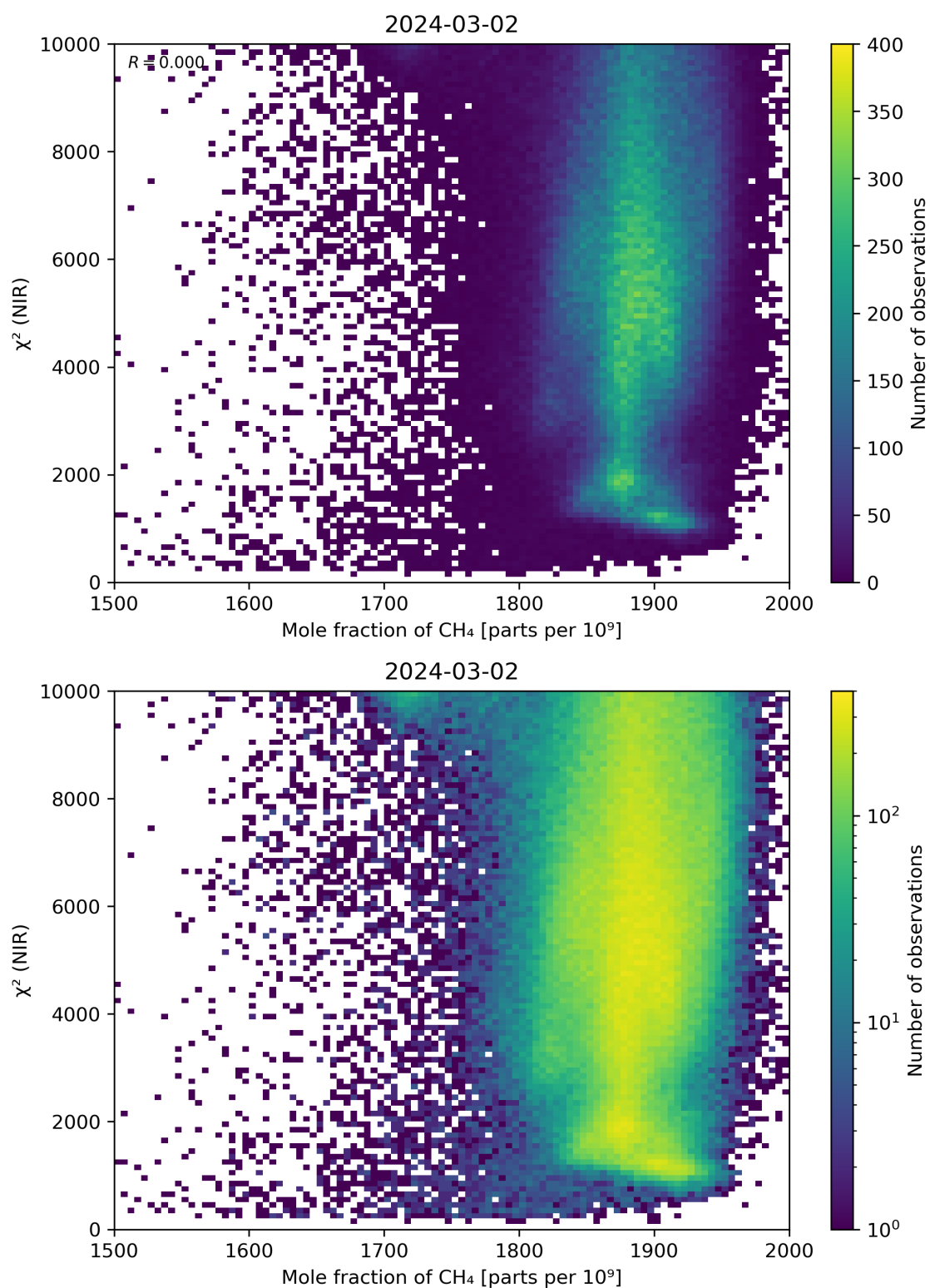
Figure 70: Scatter density plot of “Mole fraction of CH 4 ” against “ \chi^2 (NIR)” for 2024-03-01 to 2024-03-03.
