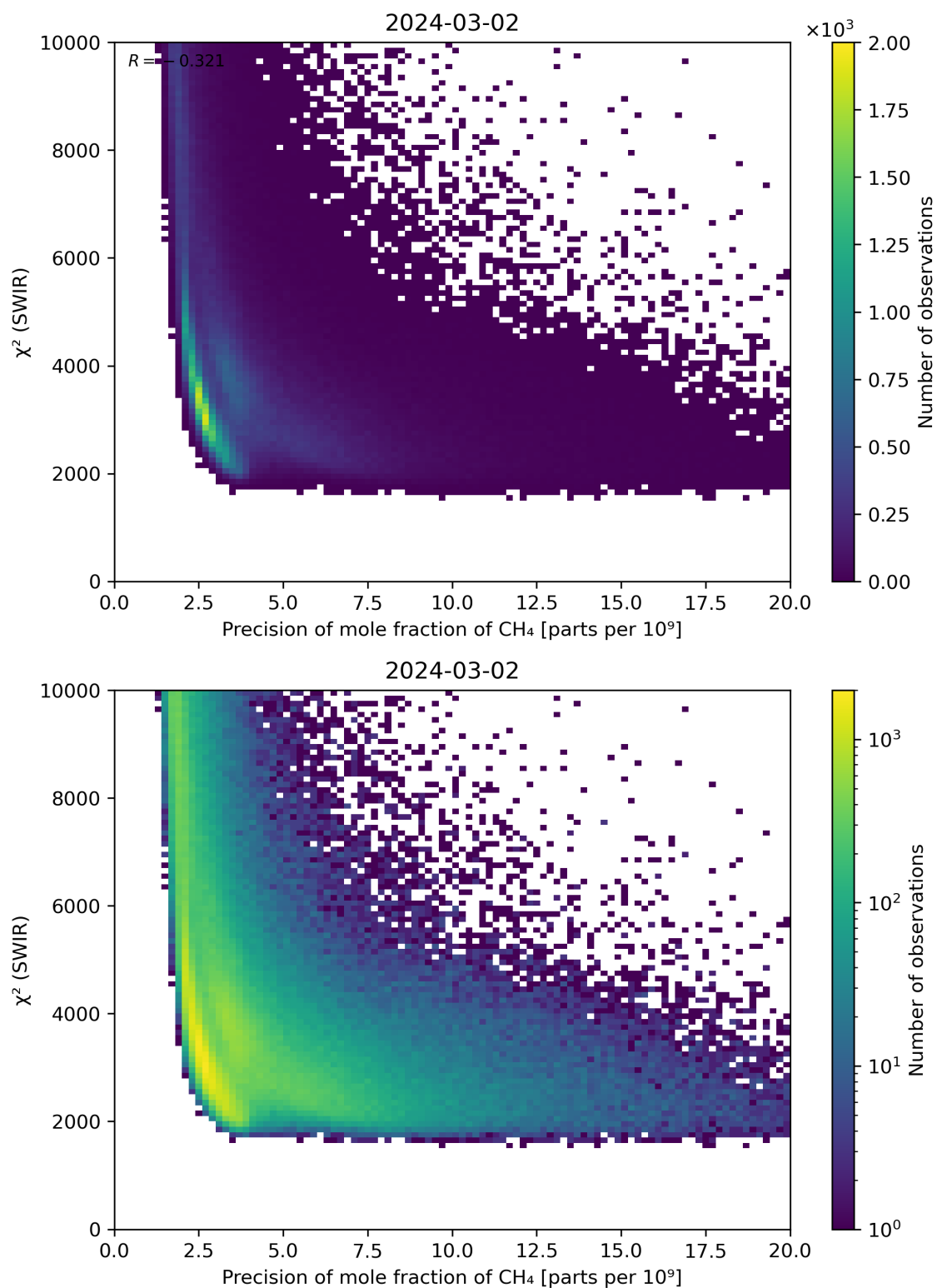
Figure 79: Scatter density plot of “Precision of mole fraction of CH 4 ” against “ \chi^2 (SWIR)” for 2024-03-01 to 2024-03-03.
