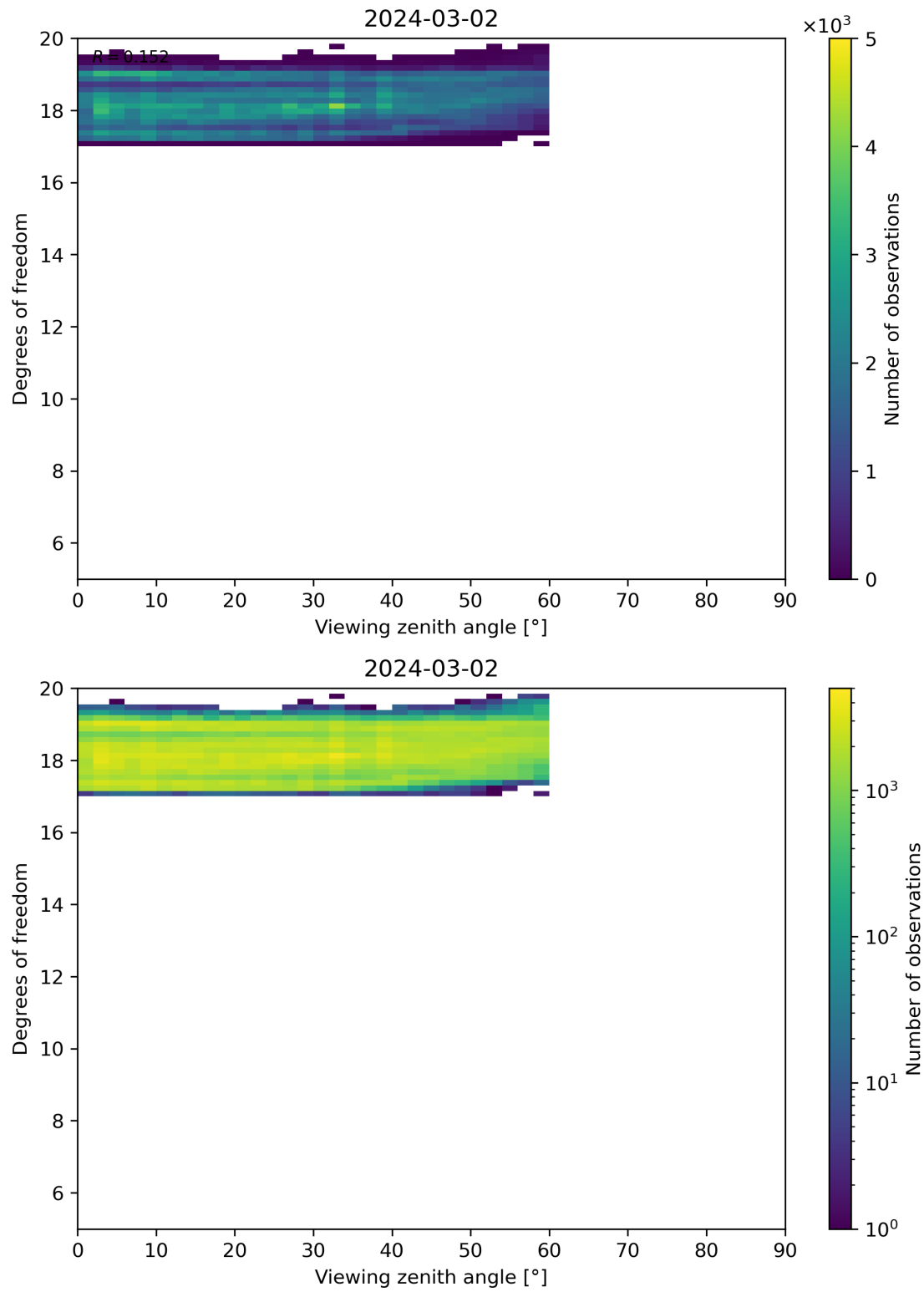
Figure 107: Scatter density plot of “Viewing zenith angle” against “Degrees of freedom” for 2024-03-01 to 2024-03-03.
