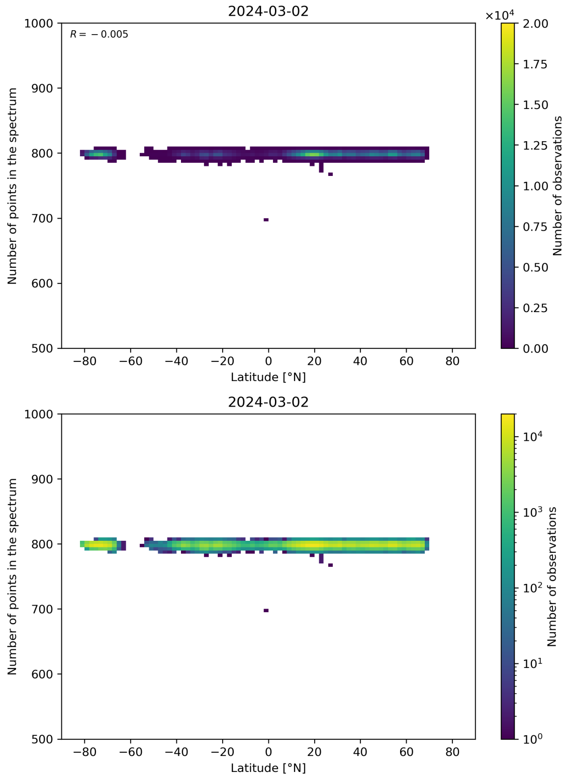
Figure 61: Scatter density plot of “Latitude” against “Number of points in the spectrum” for 2024-03-01 to 2024-03-03.
