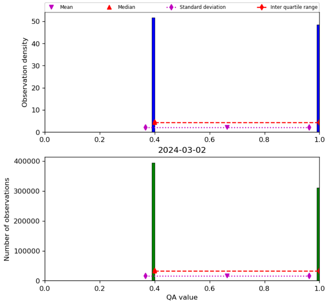
Figure 22: Histogram of “QA value” for 2024-03-01 to 2024-03-03
