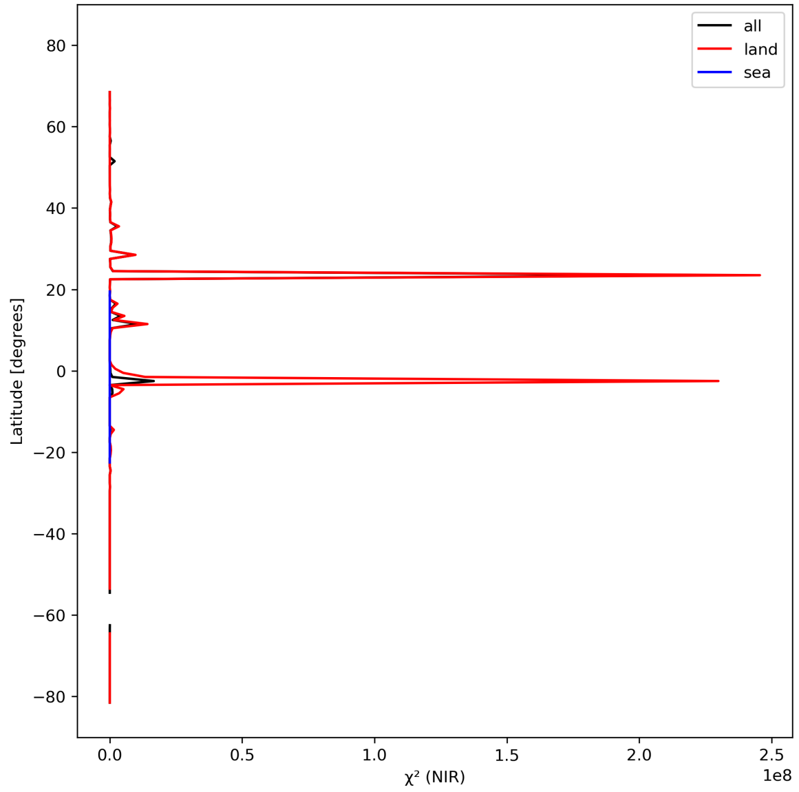
Figure 18: Zonal average of “ \chi^2 (NIR)” for 2024-03-01 to 2024-03-03.
