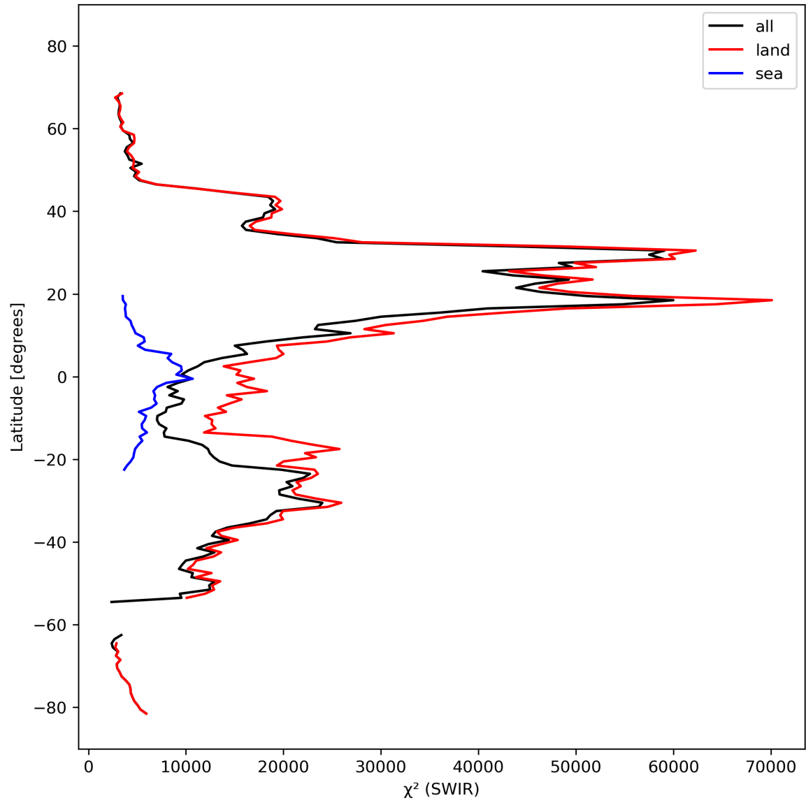
Figure 17: Zonal average of “ \chi^2 (SWIR)” for 2024-03-01 to 2024-03-03.
