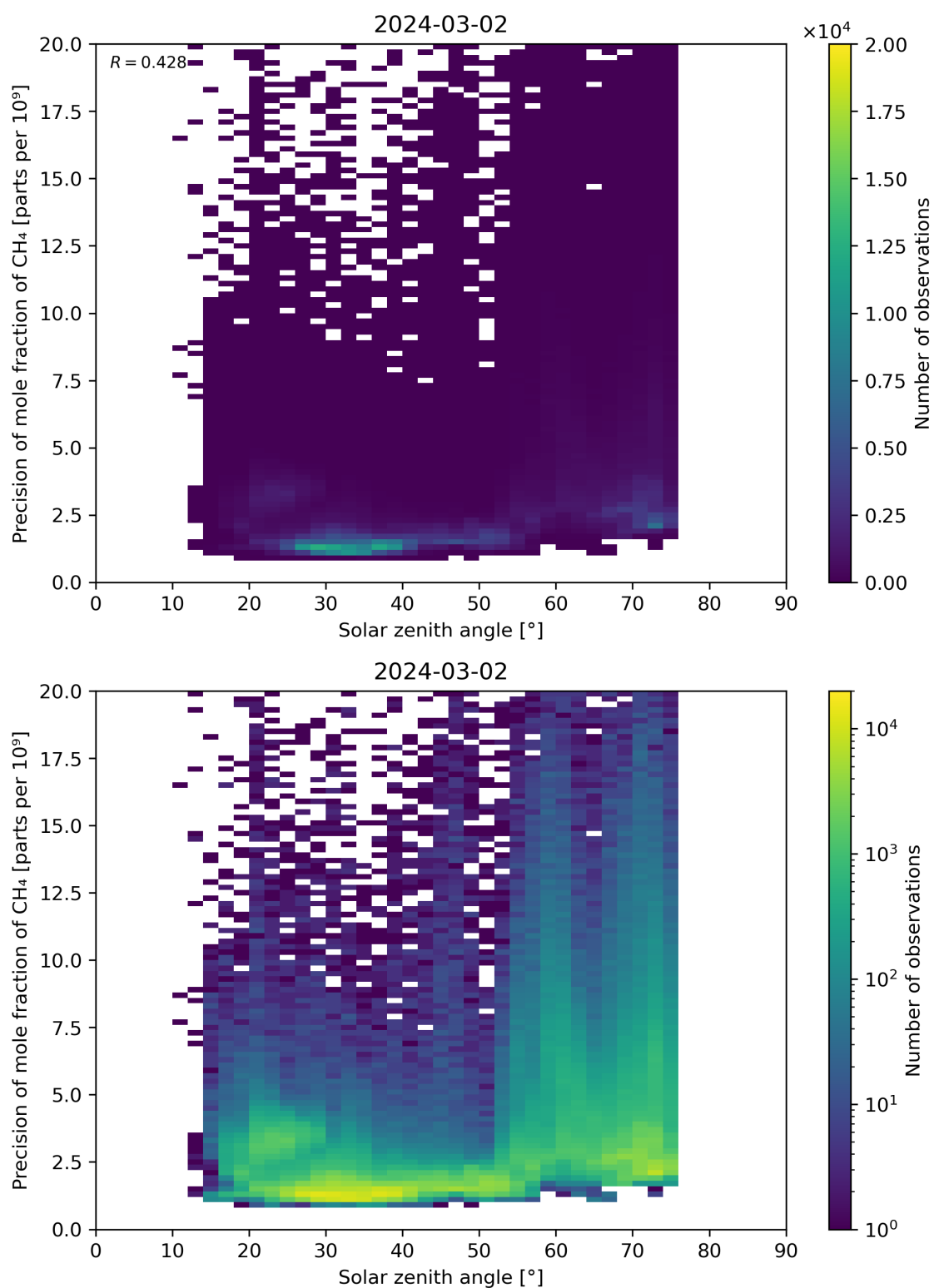
Figure 101: Scatter density plot of “Solar zenith angle” against “Precision of mole fraction of CH 4 ” for 2024-03-01 to 2024-03-03.
