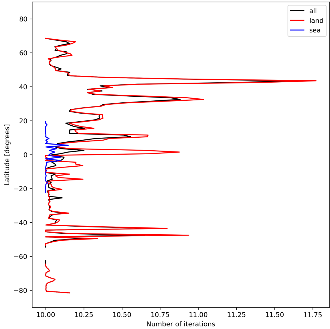
Figure 20: Zonal average of “Number of iterations” for 2024-03-01 to 2024-03-03.
