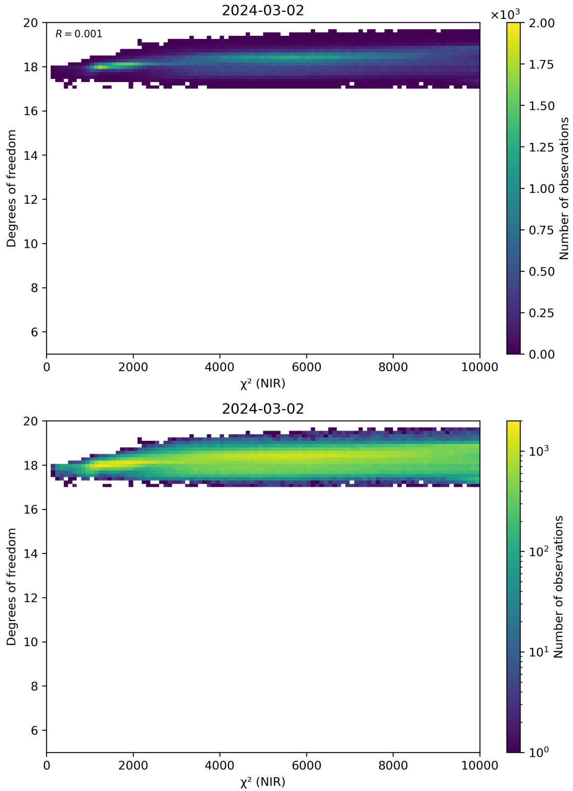
Figure 44: Scatter density plot of “ \chi^2 (NIR)” against “Degrees of freedom” for 2024-03-01 to 2024-03-03.
