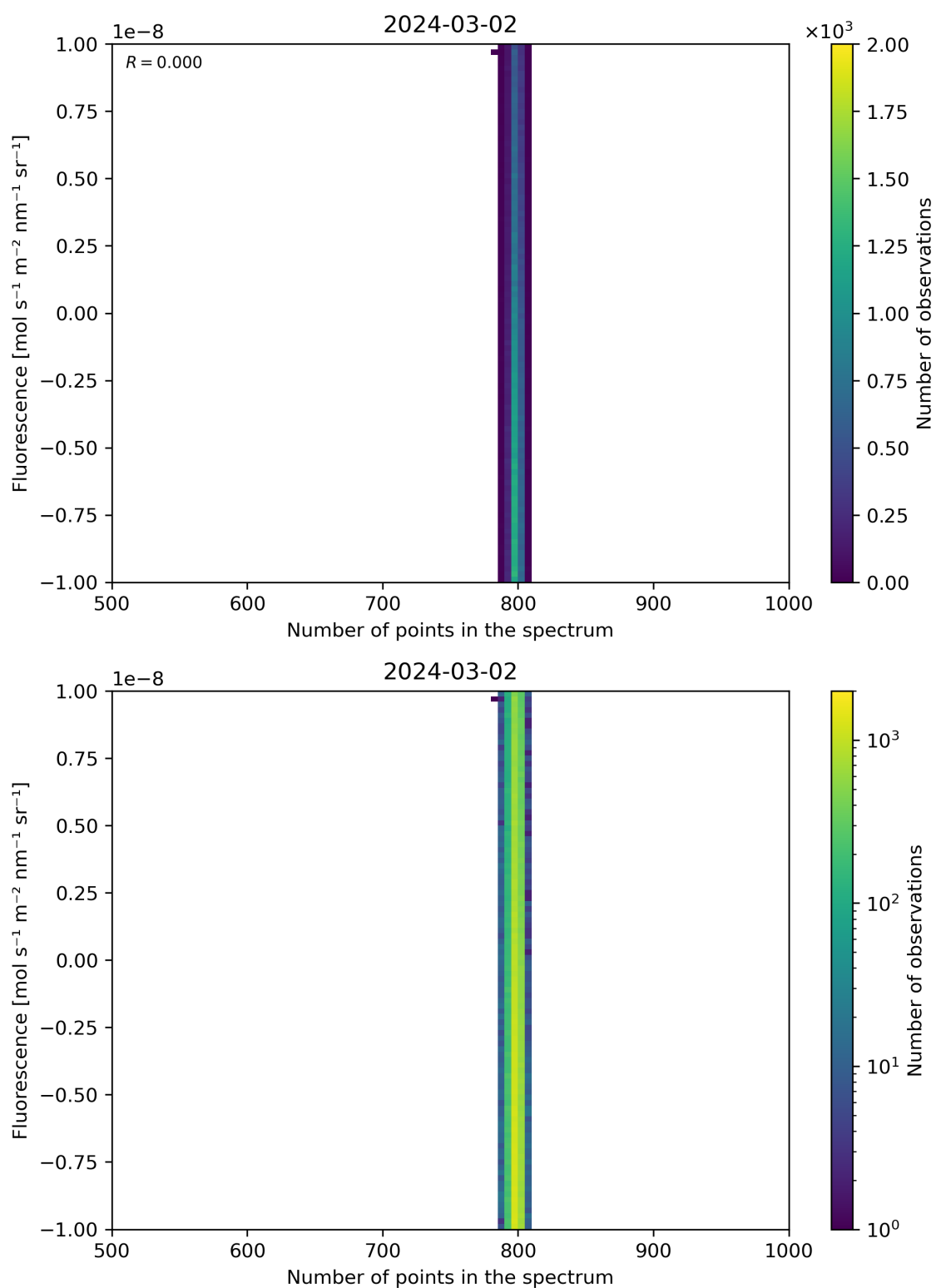
Figure 91: Scatter density plot of “Number of points in the spectrum” against “Fluorescence” for 2024-03-01 to 2024-03-03.
