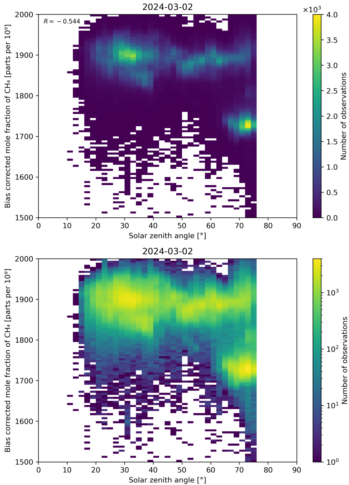
Figure 100: Scatter density plot of “Solar zenith angle” against “Bias corrected mole fraction of \text{CH}_4 ” for 2024-03-01 to 2024-03-03.
