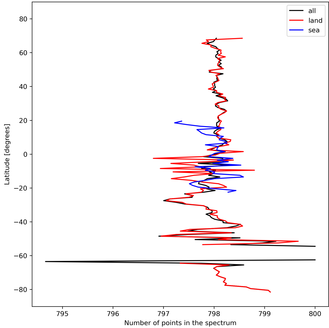
Figure 15: Zonal average of “Number of points in the spectrum” for 2024-03-01 to 2024-03-03.
