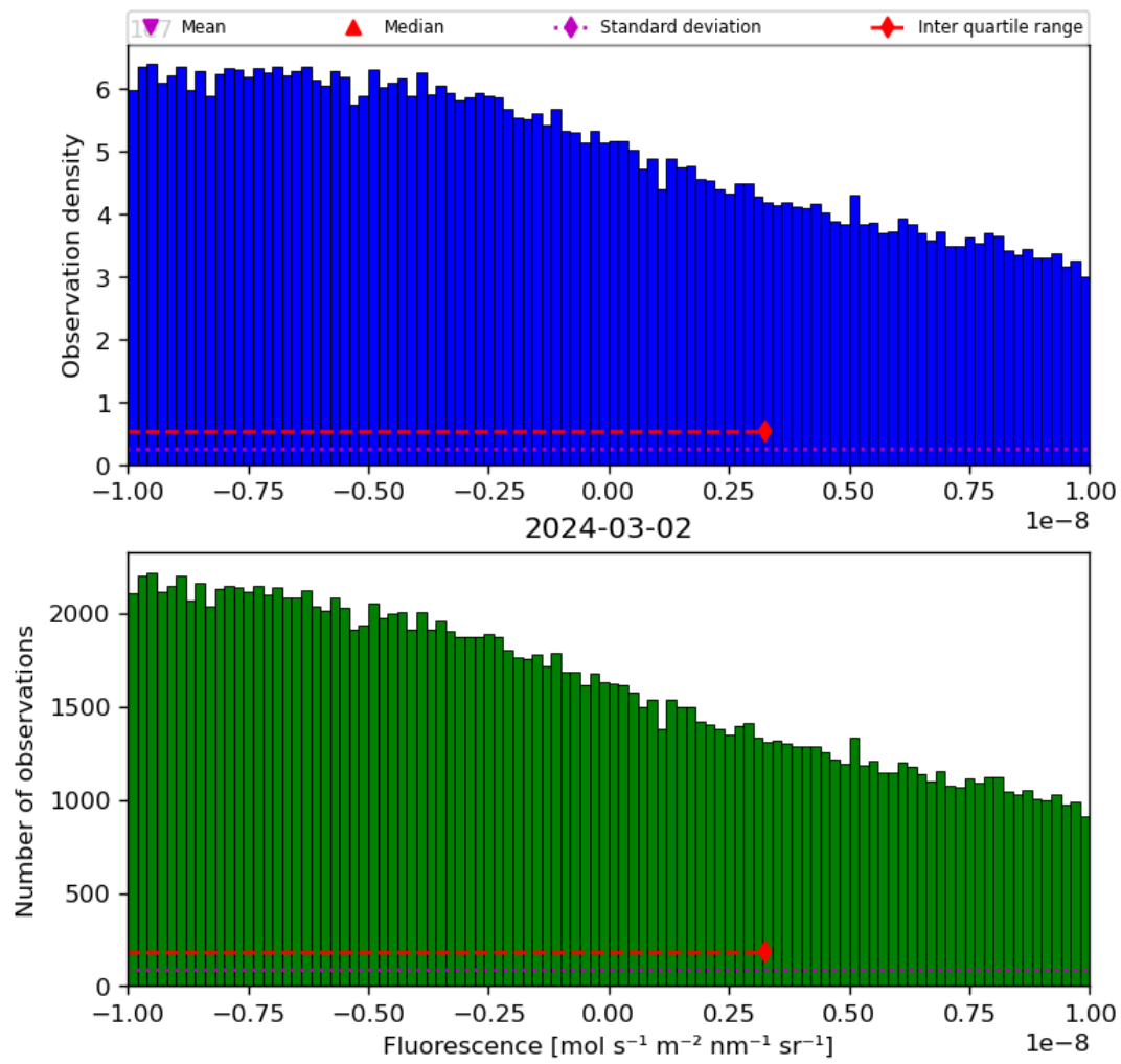
Figure 32: Histogram of “Fluorescence” for 2024-03-01 to 2024-03-03
