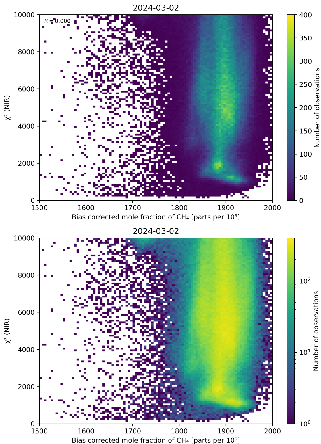
Figure 63: Scatter density plot of “Bias corrected mole fraction of CH 4 ” against “ \chi^2 (NIR)” for 2024-03-01 to 2024-03-03.
