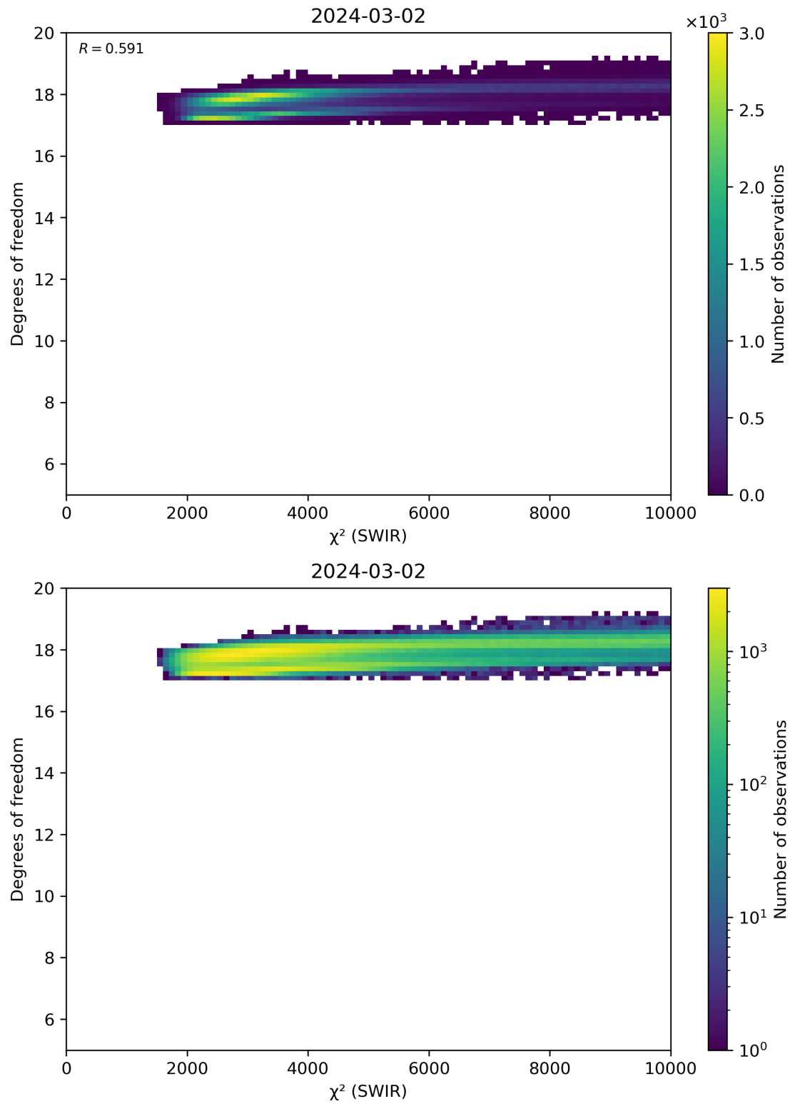
Figure 48: Scatter density plot of “ \chi^2 (SWIR)” against “Degrees of freedom” for 2024-03-01 to 2024-03-03.
