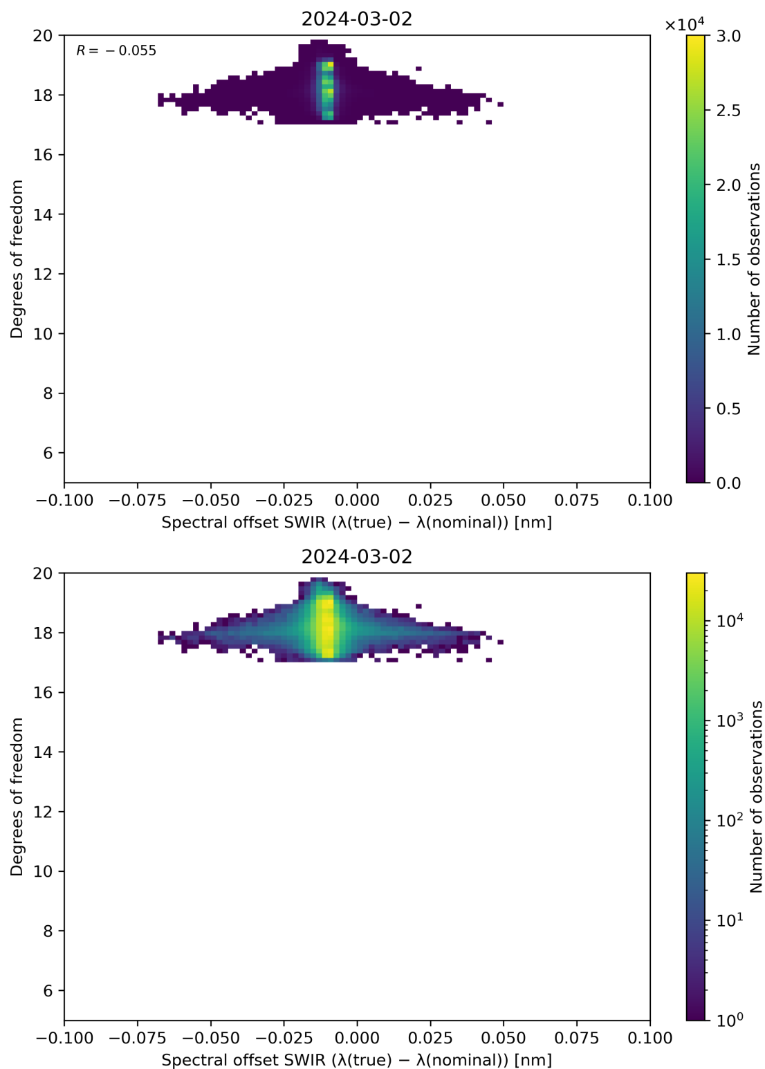
Figure 119: Scatter density plot of “Spectral offset SWIR ( \lambda(\text{true}) - \lambda(\text{nominal}) )” against “Degrees of freedom” for 2024-03-01 to 2024-03-03.
