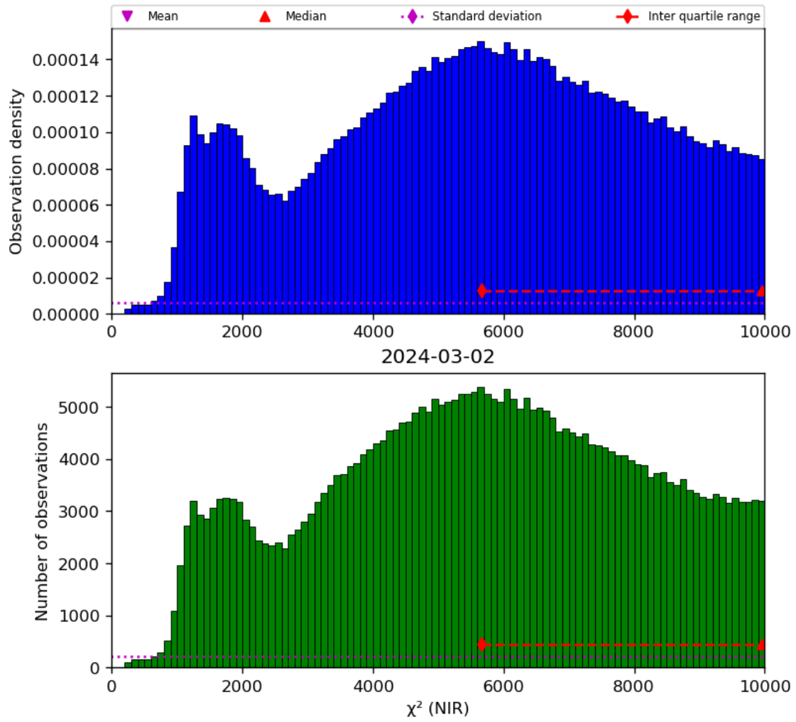
Figure 29: Histogram of “ \chi^2 (NIR)” for 2024-03-01 to 2024-03-03
