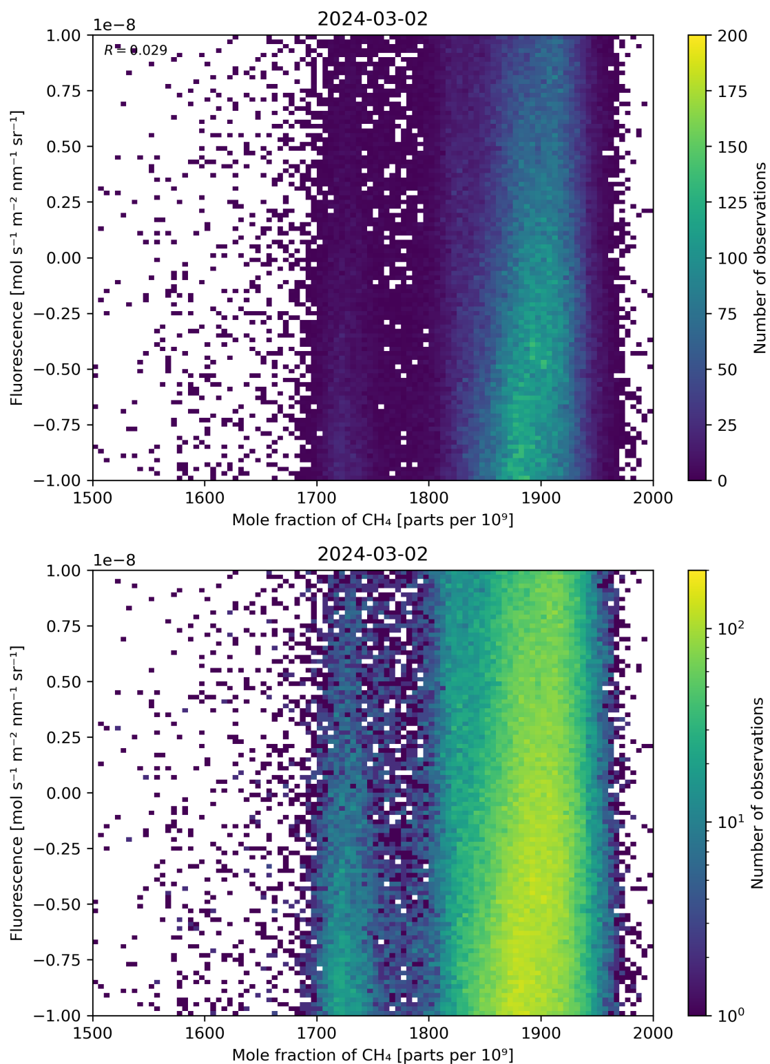
Figure 73: Scatter density plot of “Mole fraction of \text{CH}_4 ” against “Fluorescence” for 2024-03-01 to 2024-03-03.
