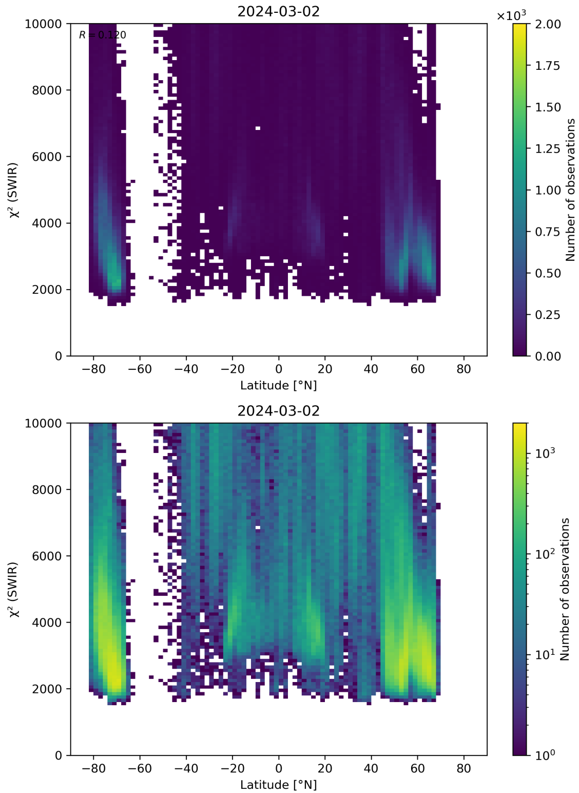
Figure 54: Scatter density plot of “Latitude” against “ \chi^2 (SWIR)” for 2024-03-01 to 2024-03-03.
