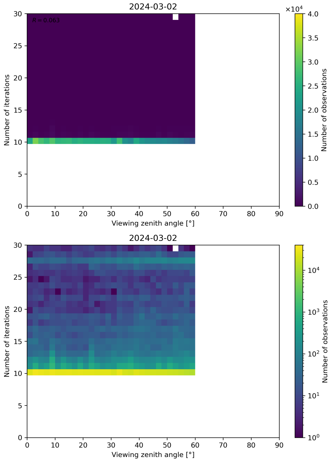
Figure 113: Scatter density plot of “Viewing zenith angle” against “Number of iterations” for 2024-03-01 to 2024-03-03.
