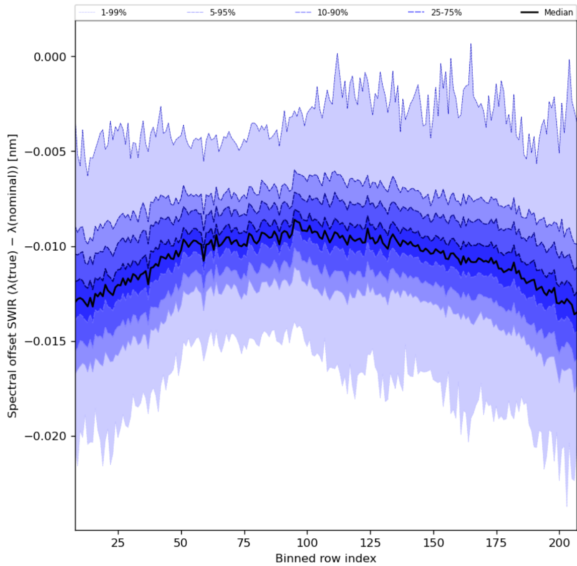
Figure 38: Along track statistics of “Spectral offset SWIR ( \lambda(\text{true}) - \lambda(\text{nominal}) )” for 2024-03-01 to 2024-03-03
