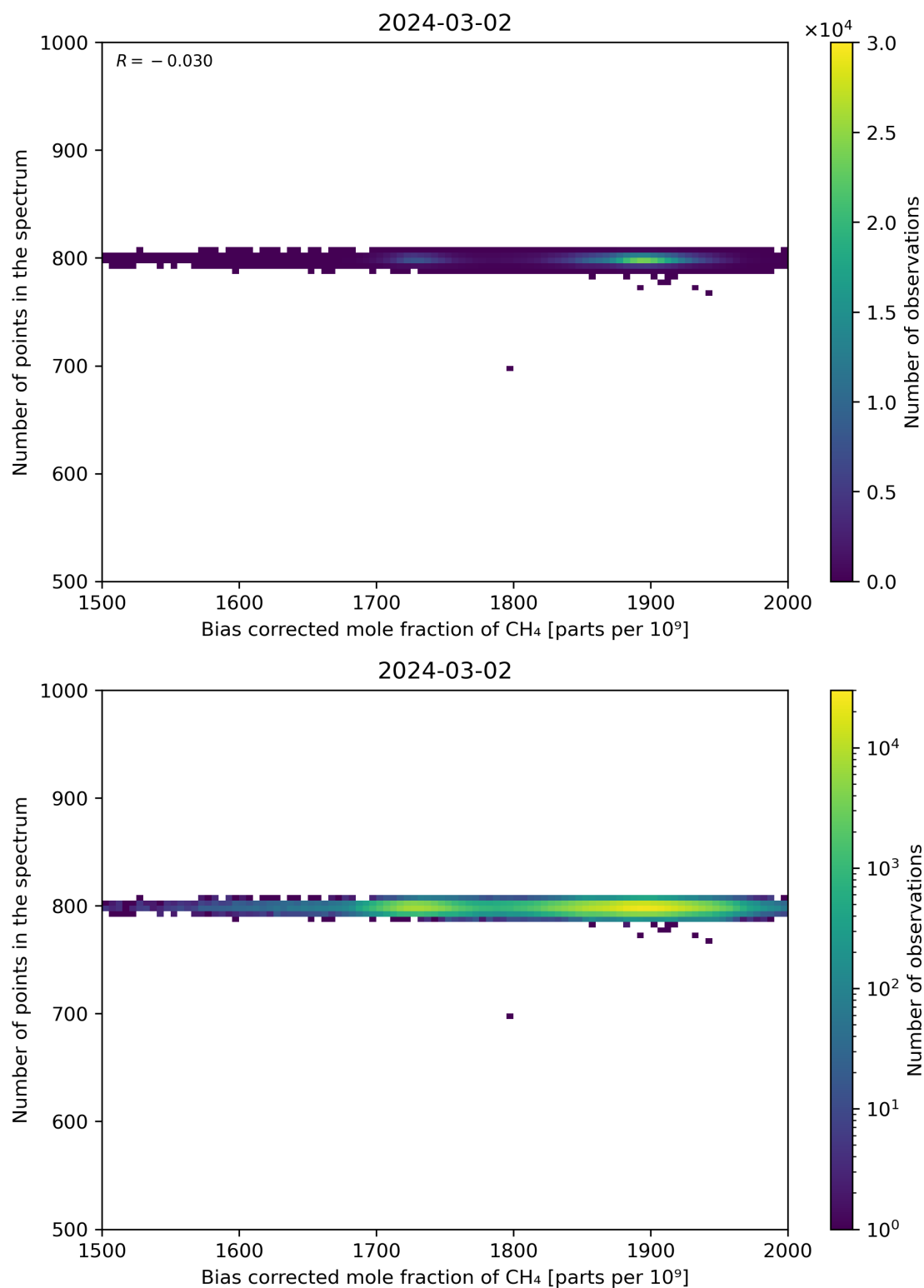
Figure 68: Scatter density plot of “Bias corrected mole fraction of CH 4 ” against “Number of points in the spectrum” for 2024-03-01 to 2024-03-03.
