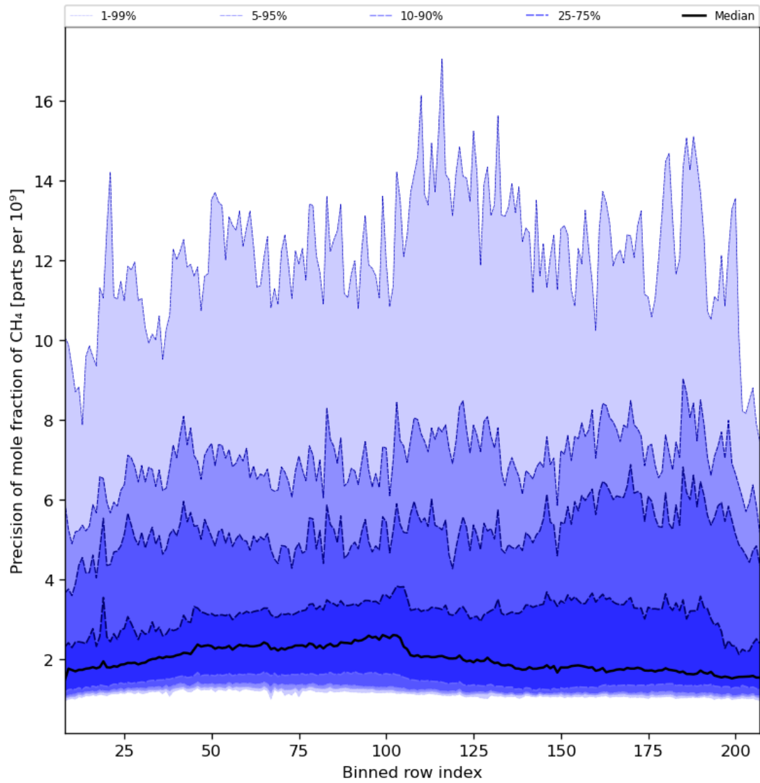
Figure 35: Along track statistics of “Precision of mole fraction of CH 4 ” for 2024-03-01 to 2024-03-03
