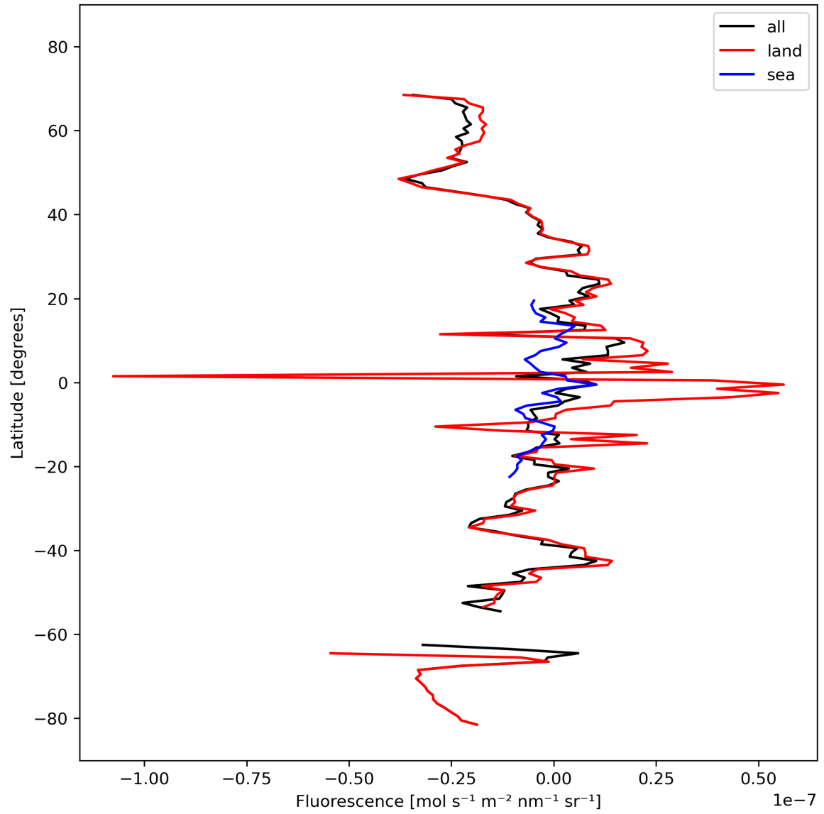
Figure 21: Zonal average of “Fluorescence” for 2024-03-01 to 2024-03-03.
