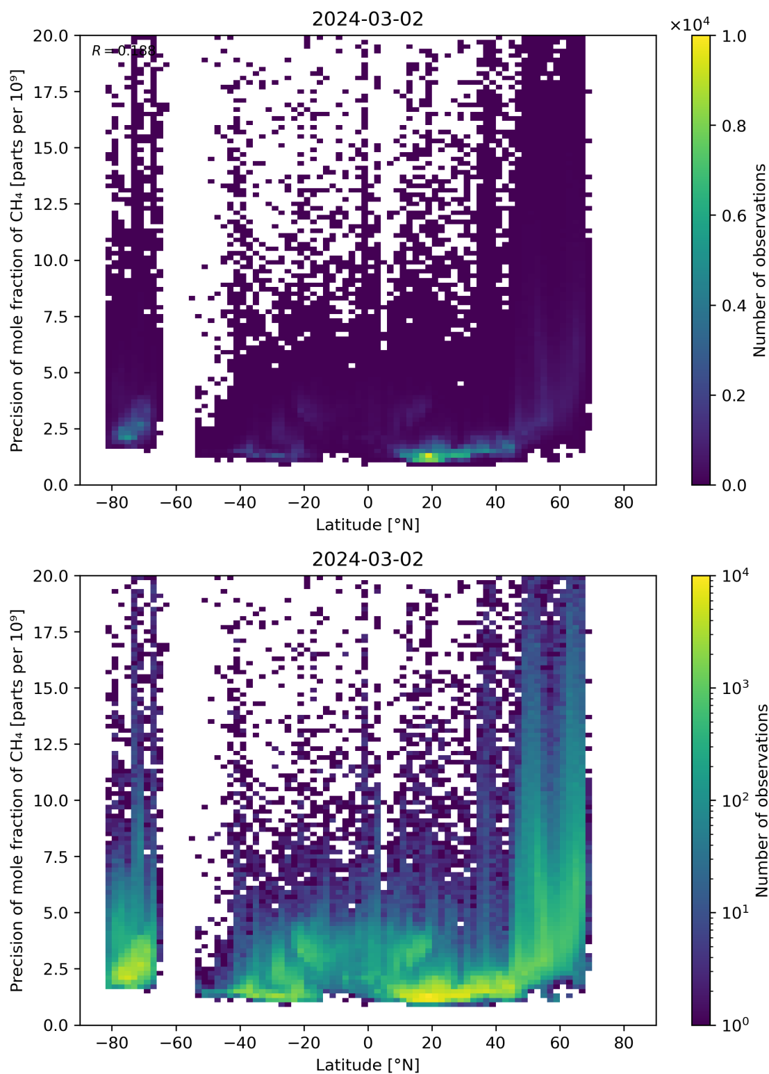
Figure 59: Scatter density plot of “Latitude” against “Precision of mole fraction of CH 4 ” for 2024-03-01 to 2024-03-03.
