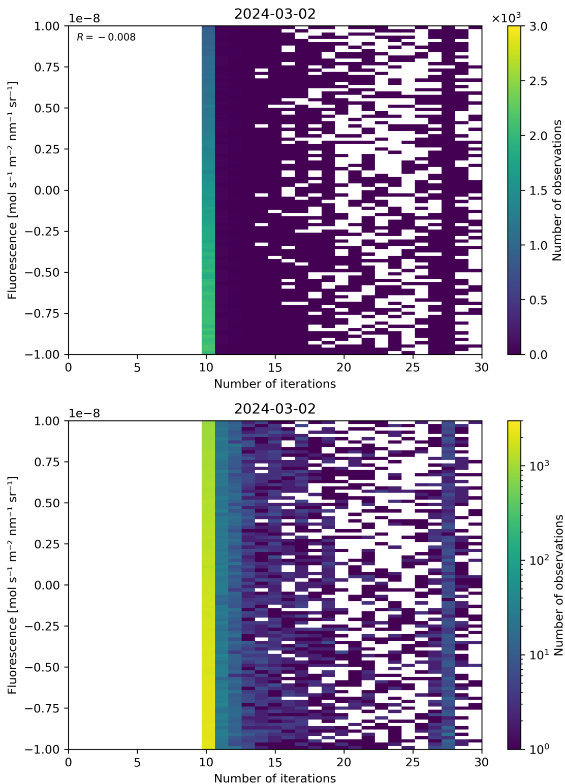
Figure 87: Scatter density plot of “Number of iterations” against “Fluorescence” for 2024-03-01 to 2024-03-03.
