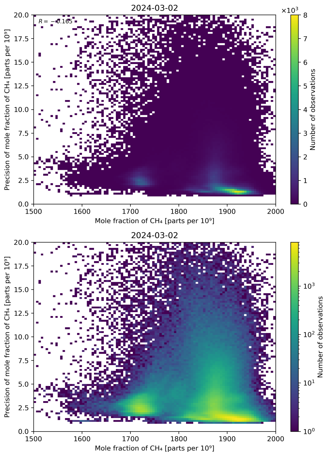
Figure 75: Scatter density plot of “Mole fraction of CH 4 ” against “Precision of mole fraction of CH 4 ” for 2024-03-01 to 2024-03-03.
