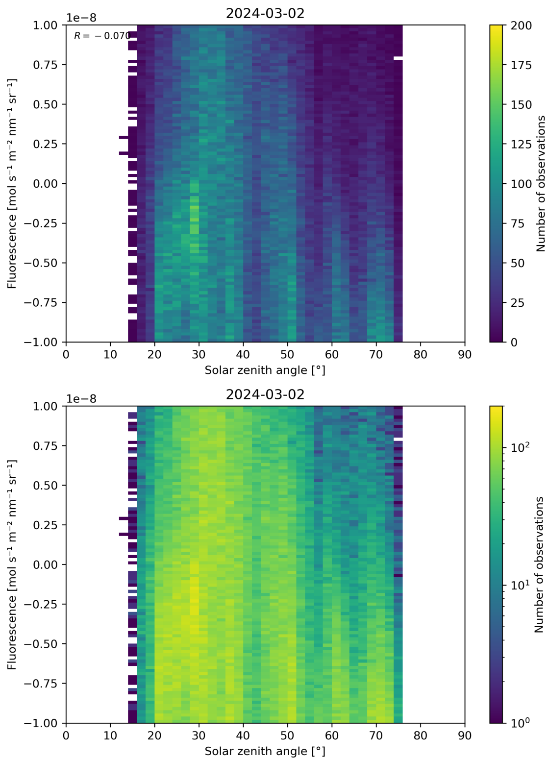
Figure 97: Scatter density plot of “Solar zenith angle” against “Fluorescence” for 2024-03-01 to 2024-03-03.
