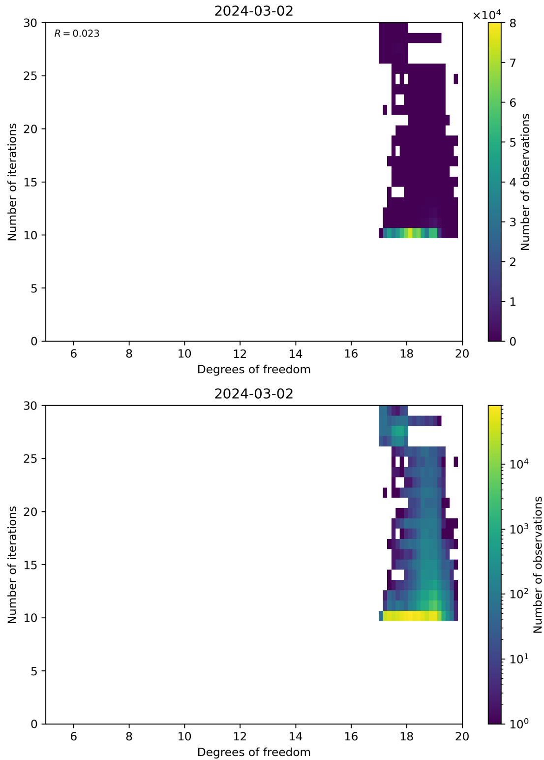
Figure 52: Scatter density plot of “Degrees of freedom” against “Number of iterations” for 2024-03-01 to 2024-03-03.
