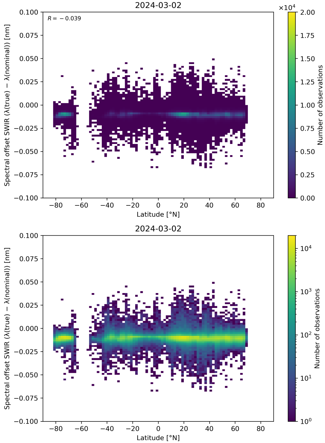
Figure 62: Scatter density plot of “Latitude” against “Spectral offset SWIR ( \lambda(\text{true}) - \lambda(\text{nominal}) )” for 2024-03-01 to 2024-03-03.
