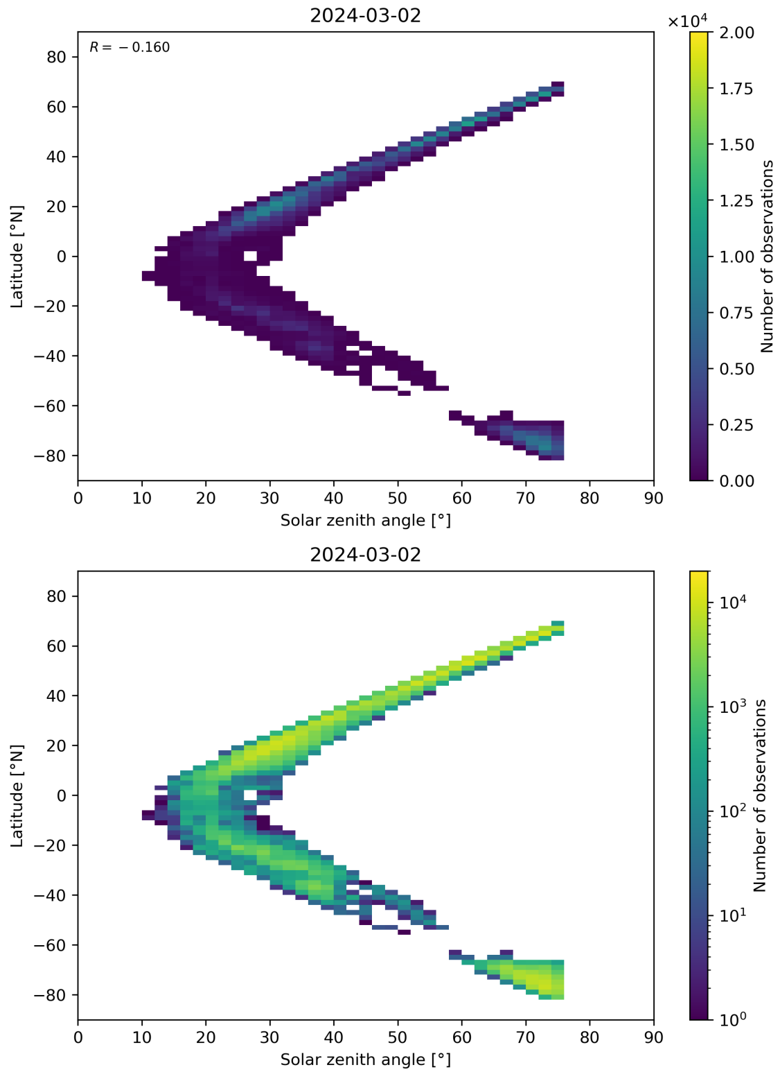
Figure 98: Scatter density plot of “Solar zenith angle” against “Latitude” for 2024-03-01 to 2024-03-03.
