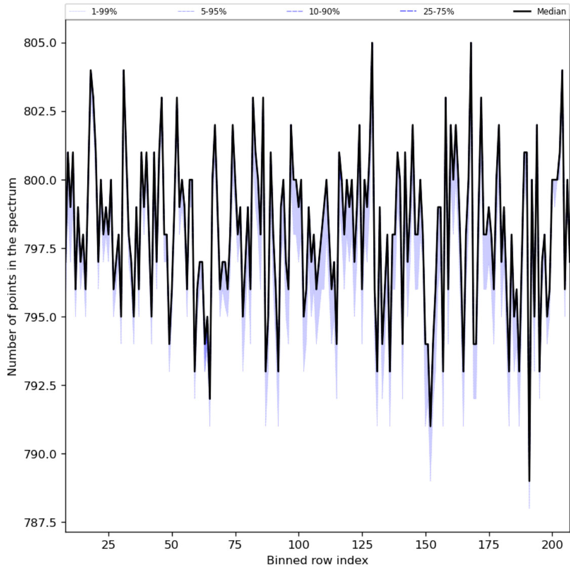
Figure 37: Along track statistics of “Number of points in the spectrum” for 2024-03-01 to 2024-03-03
