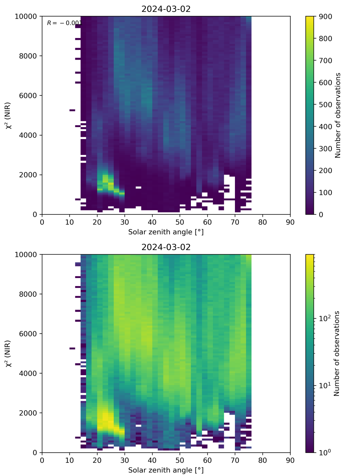
Figure 94: Scatter density plot of “Solar zenith angle” against “ \chi^2 (NIR)” for 2024-03-01 to 2024-03-03.
