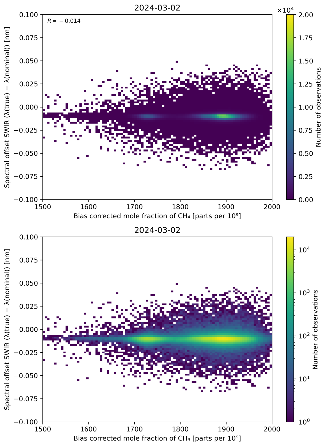
Figure 69: Scatter density plot of “Bias corrected mole fraction of \text{CH}_4 ” against “Spectral offset SWIR ( \lambda(\text{true}) - \lambda(\text{nominal}) )” for 2024-03-01 to 2024-03-03.
