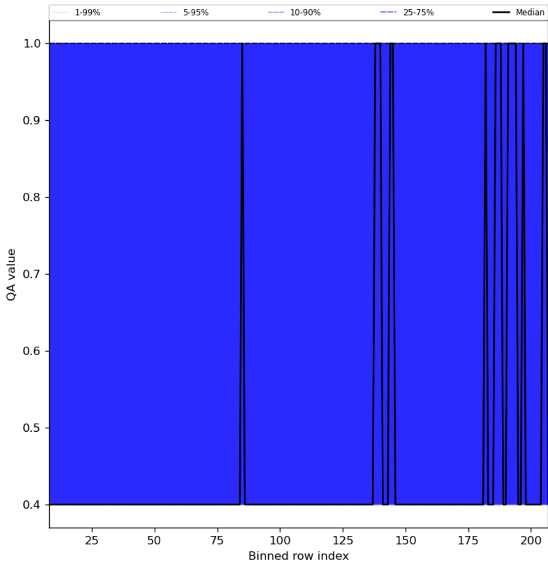
Figure 33: Along track statistics of “QA value” for 2024-03-01 to 2024-03-03
