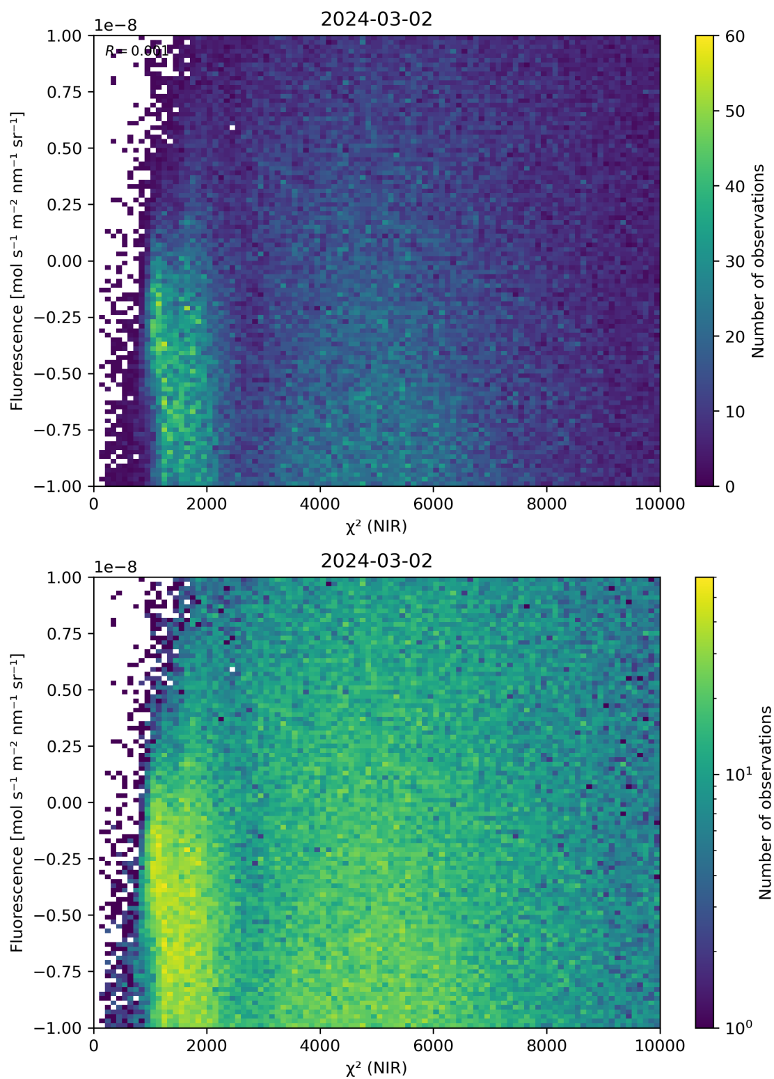
Figure 45: Scatter density plot of “ \chi^2 (NIR)” against “Fluorescence” for 2024-03-01 to 2024-03-03.
