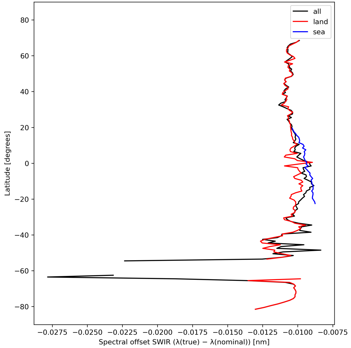
Figure 16: Zonal average of “Spectral offset SWIR ( \lambda(\text{true}) - \lambda(\text{nominal}) )” for 2024-03-01 to 2024-03-03.
