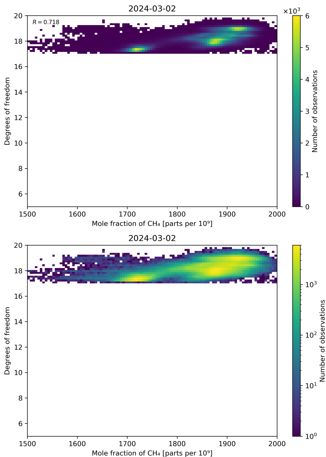
Figure 72: Scatter density plot of “Mole fraction of CH 4 ” against “Degrees of freedom” for 2024-03-01 to 2024-03-03.
