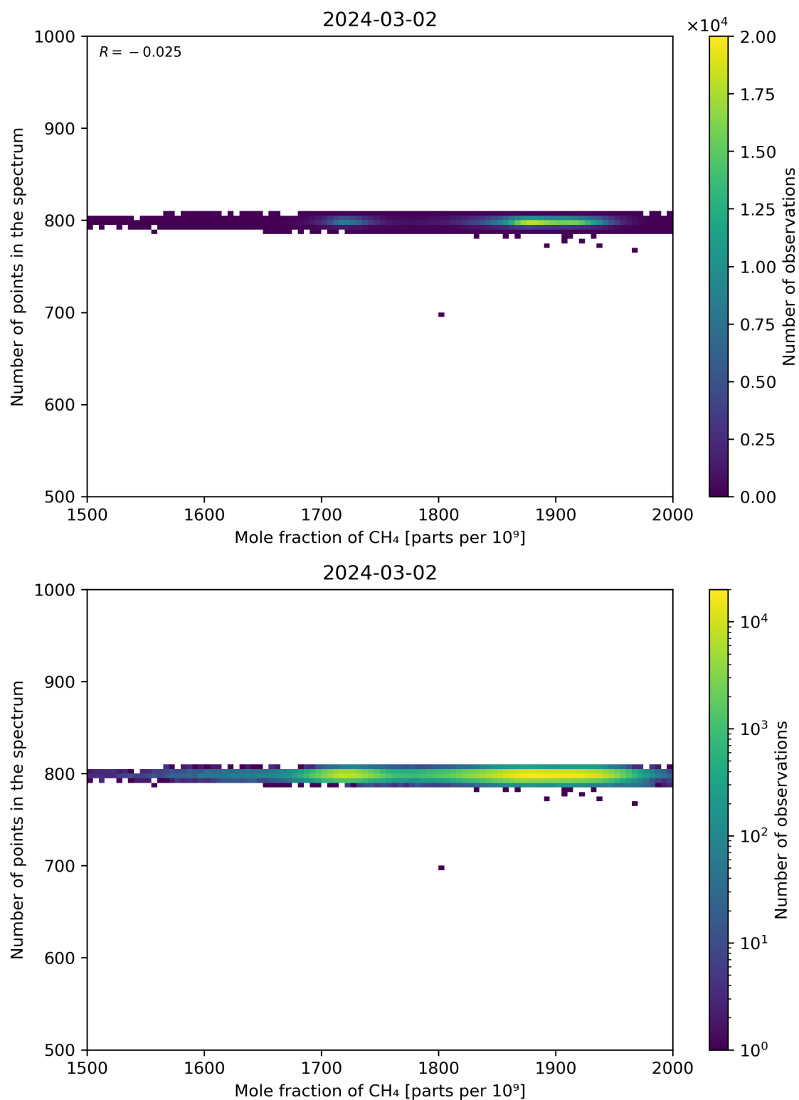
Figure 77: Scatter density plot of “Mole fraction of CH 4 ” against “Number of points in the spectrum” for 2024-03-01 to 2024-03-03.
