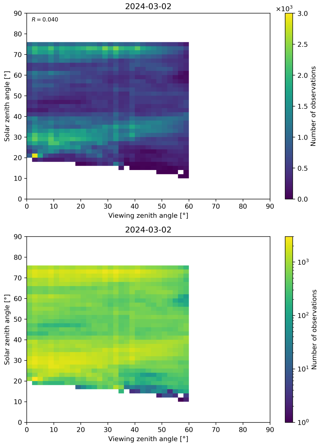
Figure 115: Scatter density plot of “Viewing zenith angle” against “Solar zenith angle” for 2024-03-01 to 2024-03-03.
