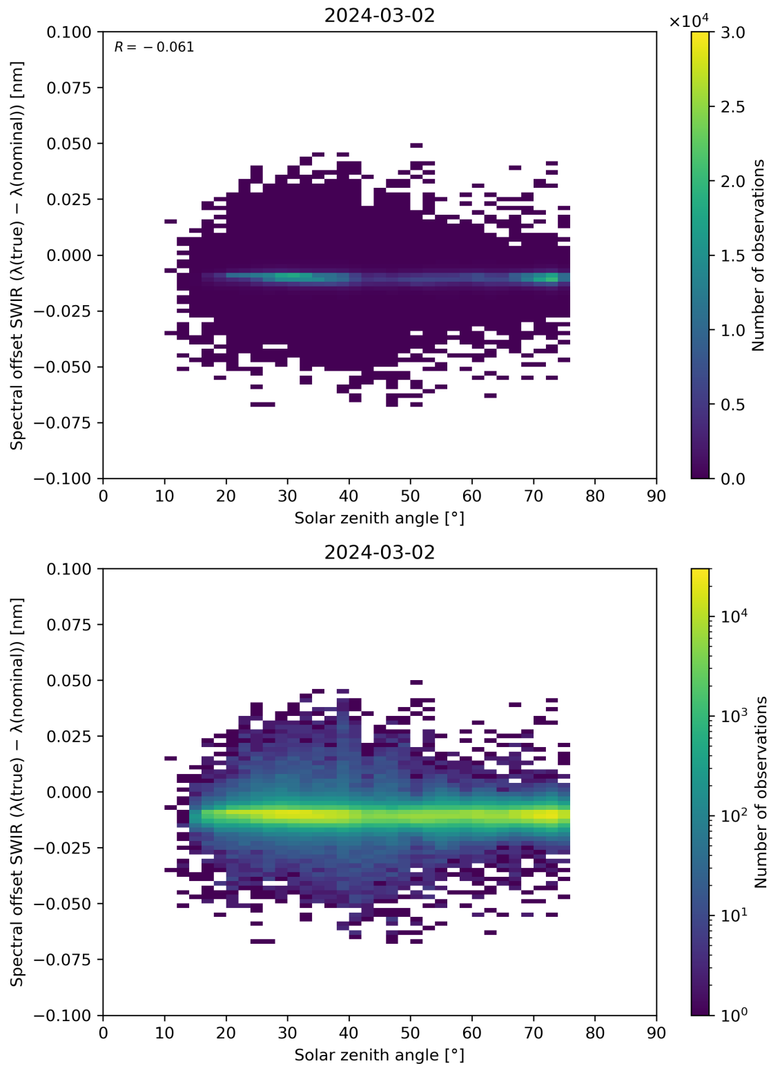
Figure 104: Scatter density plot of “Solar zenith angle” against “Spectral offset SWIR ( \lambda(\text{true}) - \lambda(\text{nominal}) )” for 2024-03-01 to 2024-03-03.
