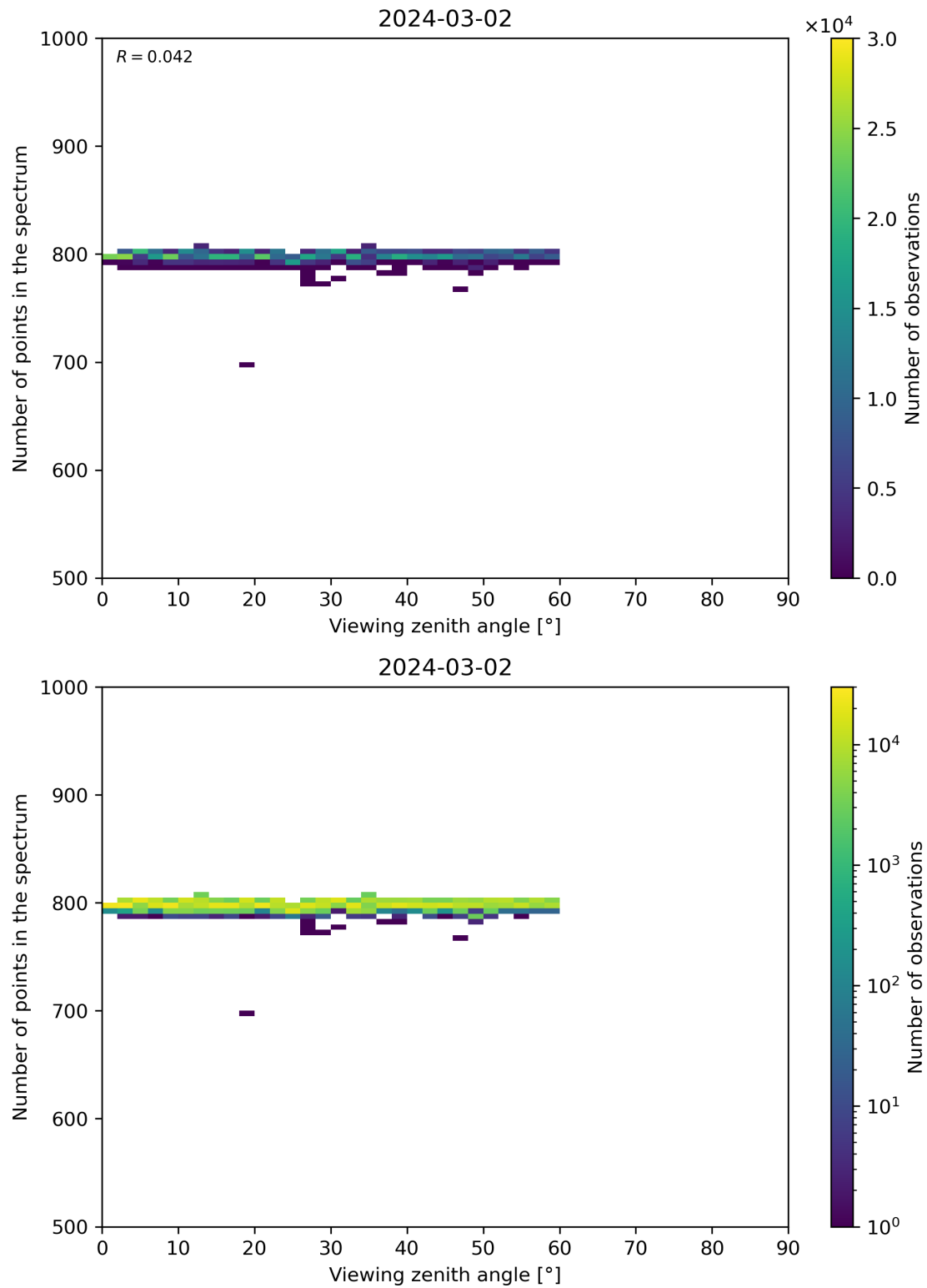
Figure 114: Scatter density plot of “Viewing zenith angle” against “Number of points in the spectrum” for 2024-03-01 to 2024-03-03.
