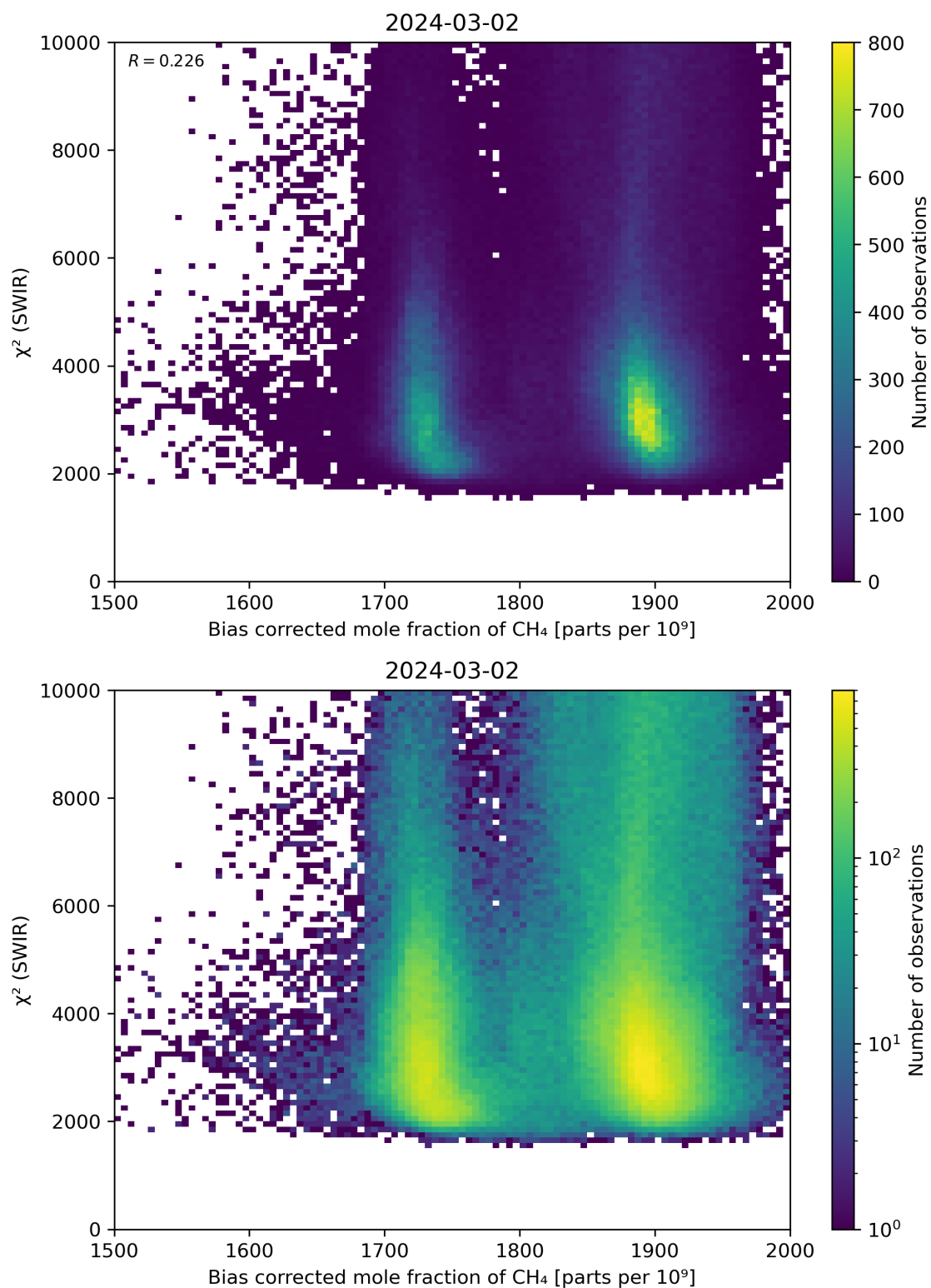
Figure 64: Scatter density plot of “Bias corrected mole fraction of \text{CH}_4 ” against “ \chi^2 (SWIR)” for 2024-03-01 to 2024-03-03.
