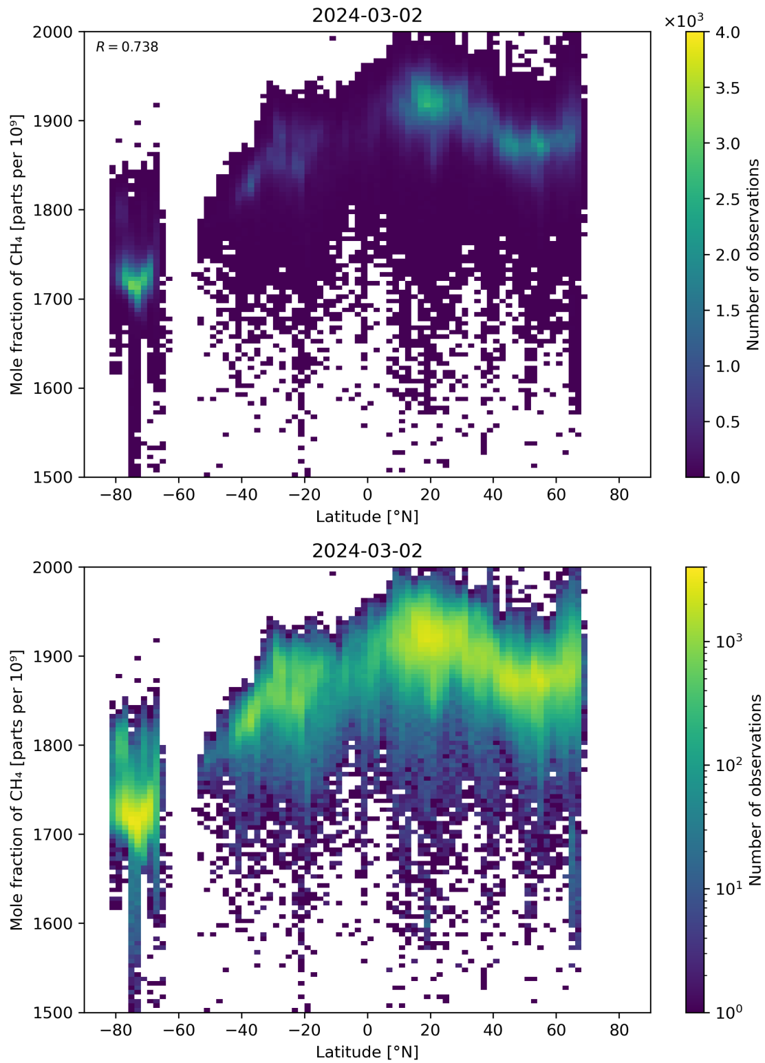
Figure 57: Scatter density plot of “Latitude” against “Mole fraction of CH 4 ” for 2024-03-01 to 2024-03-03.
