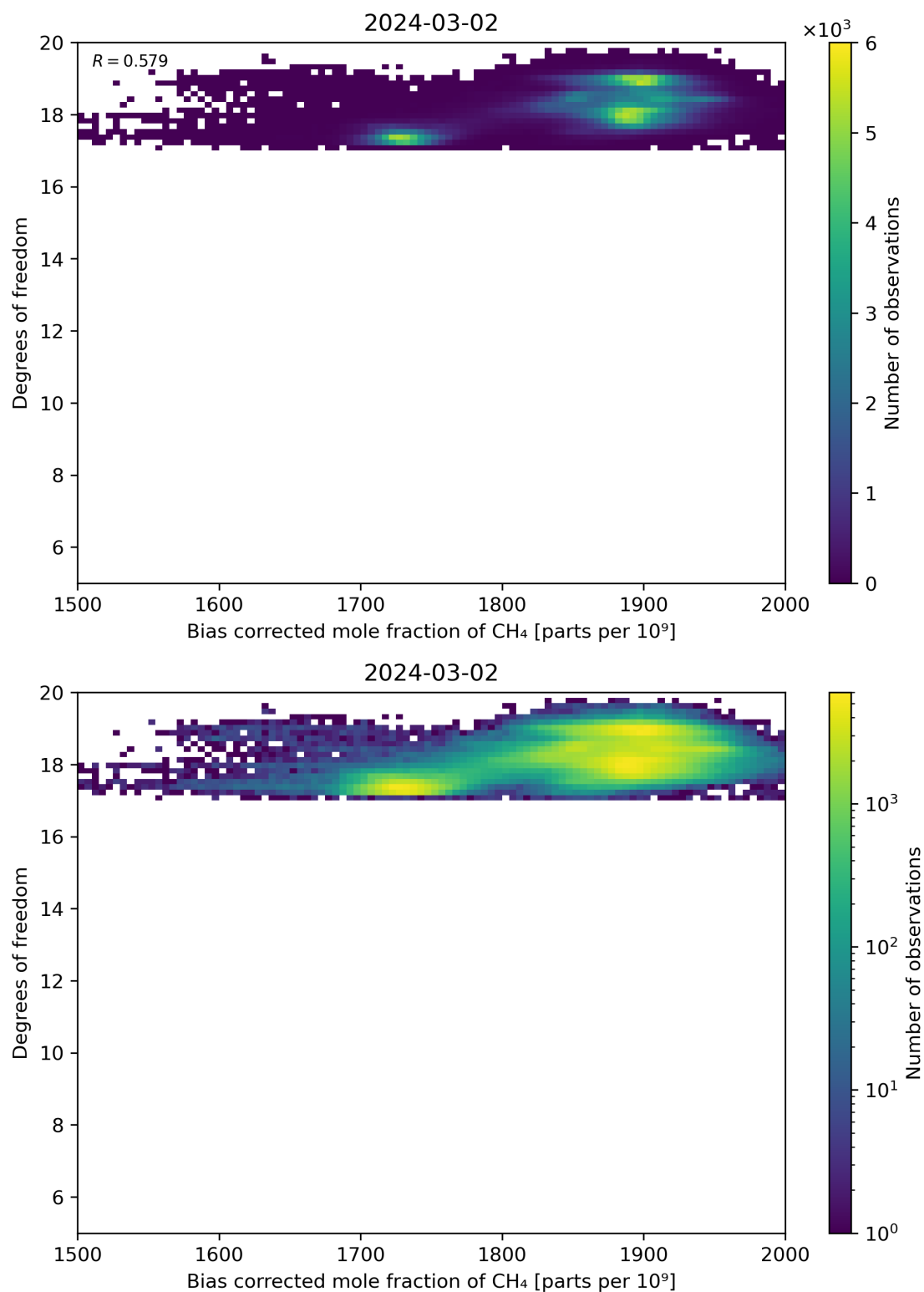
Figure 65: Scatter density plot of “Bias corrected mole fraction of CH 4 ” against “Degrees of freedom” for 2024-03-01 to 2024-03-03.
