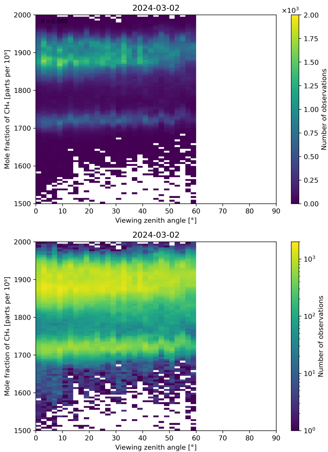
Figure 110: Scatter density plot of “Viewing zenith angle” against “Mole fraction of CH 4 ” for 2024-03-01 to 2024-03-03.
