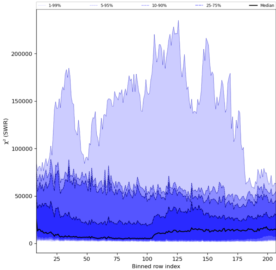
Figure 39: Along track statistics of “ \chi^2 (SWIR)” for 2024-03-01 to 2024-03-03
