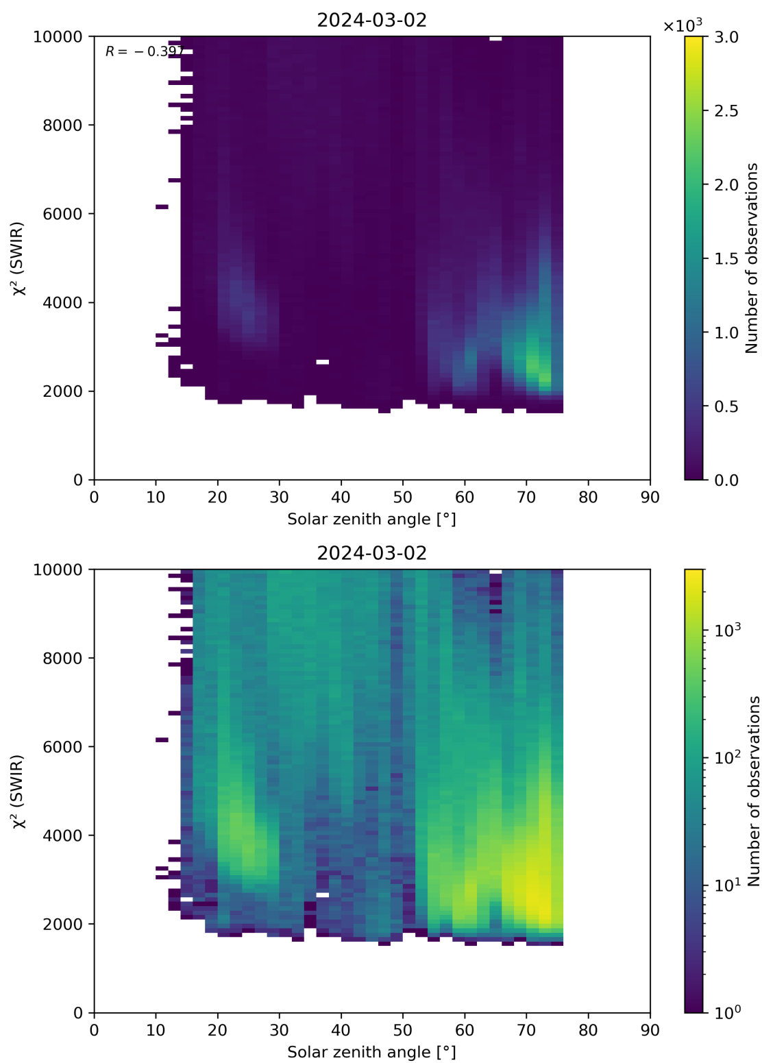
Figure 95: Scatter density plot of “Solar zenith angle” against “ \chi^2 (SWIR)” for 2024-03-01 to 2024-03-03.
