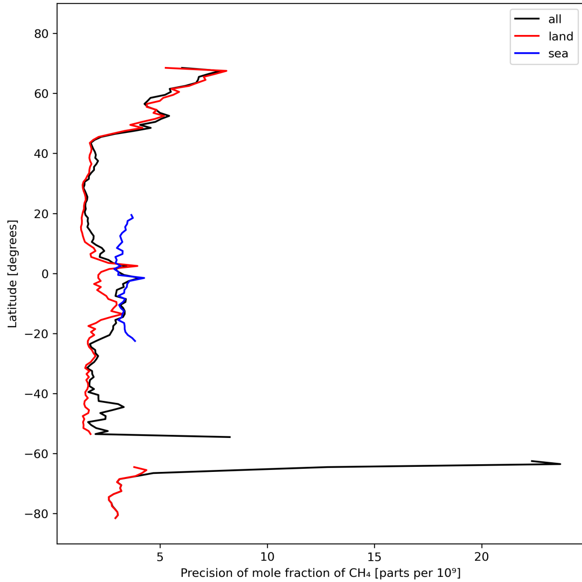
Figure 13: Zonal average of “Precision of mole fraction of CH 4 ” for 2024-03-01 to 2024-03-03.
