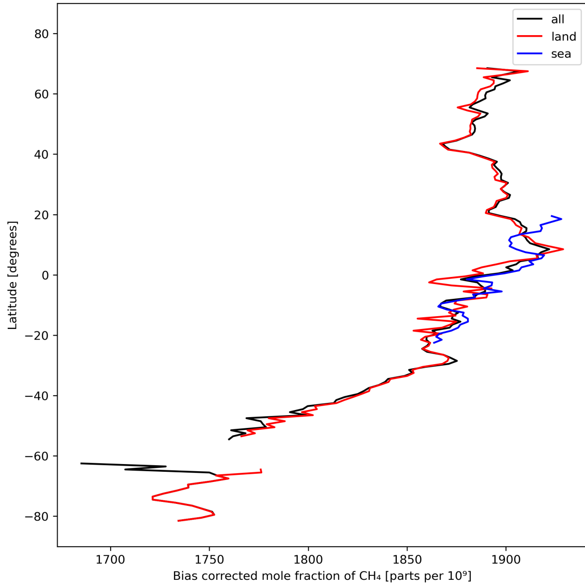
Figure 14: Zonal average of “Bias corrected mole fraction of CH 4 ” for 2024-03-01 to 2024-03-03.
