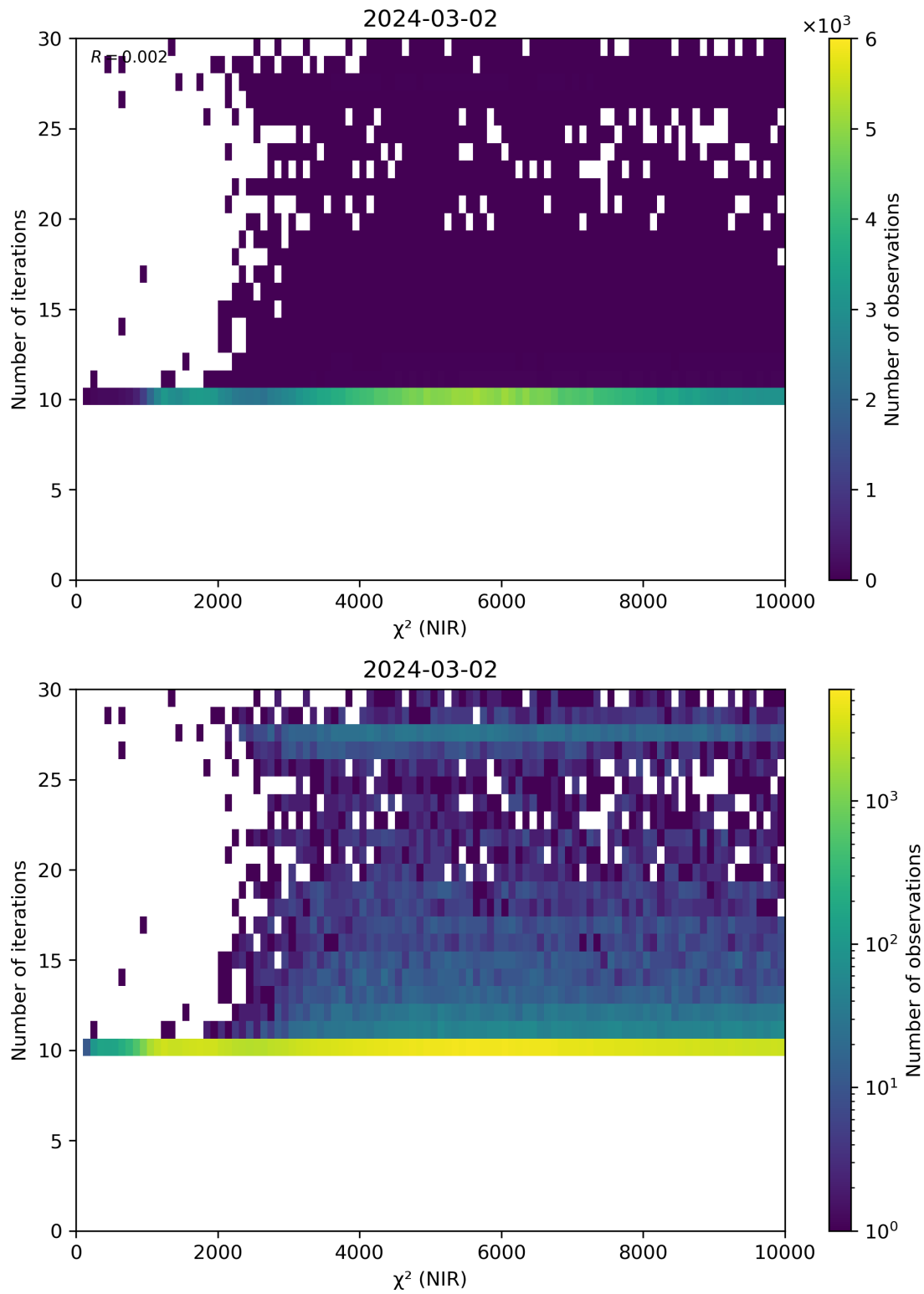
Figure 46: Scatter density plot of “ \chi^2 (NIR)” against “Number of iterations” for 2024-03-01 to 2024-03-03.
