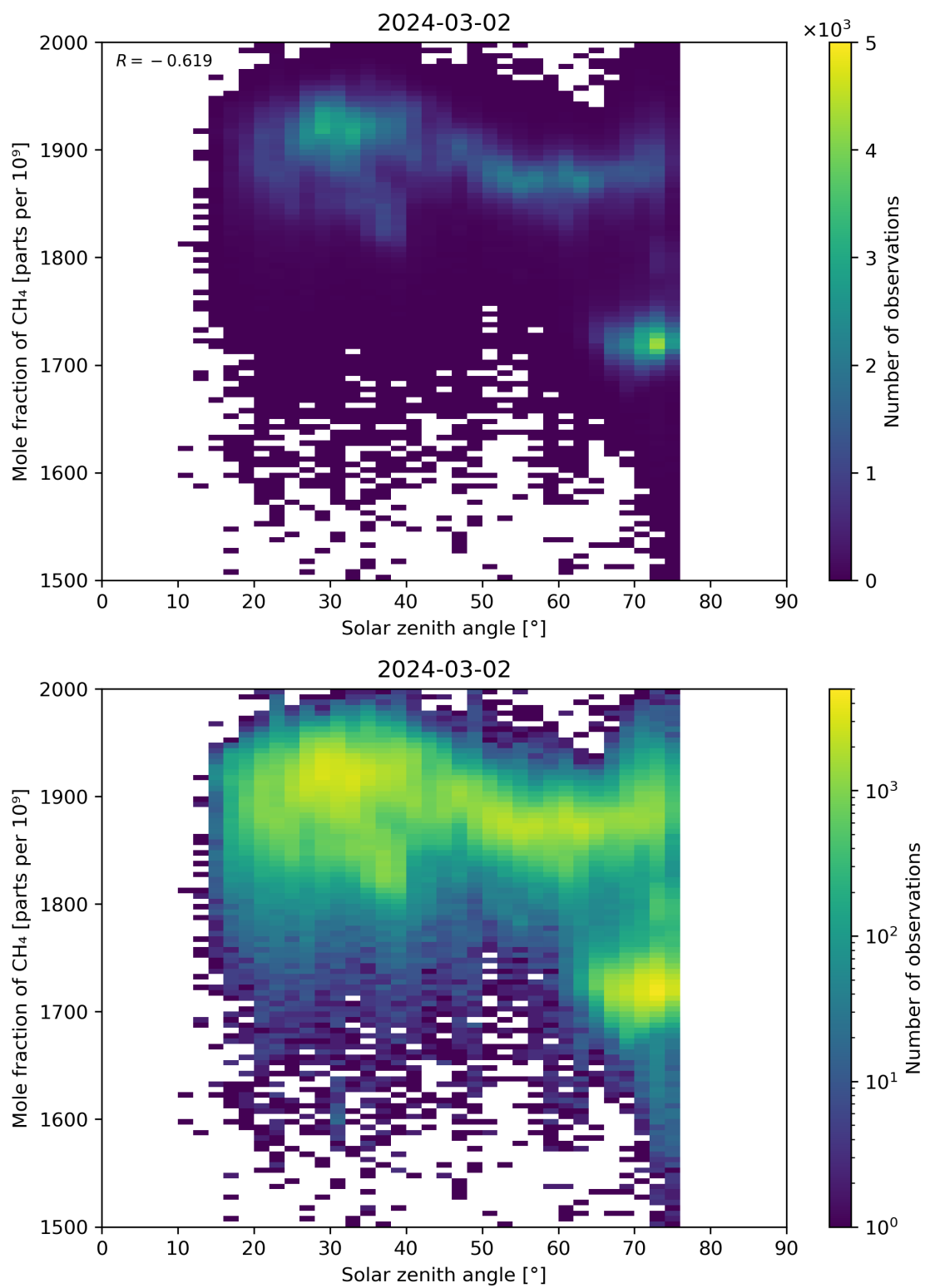
Figure 99: Scatter density plot of “Solar zenith angle” against “Mole fraction of CH 4 ” for 2024-03-01 to 2024-03-03.
