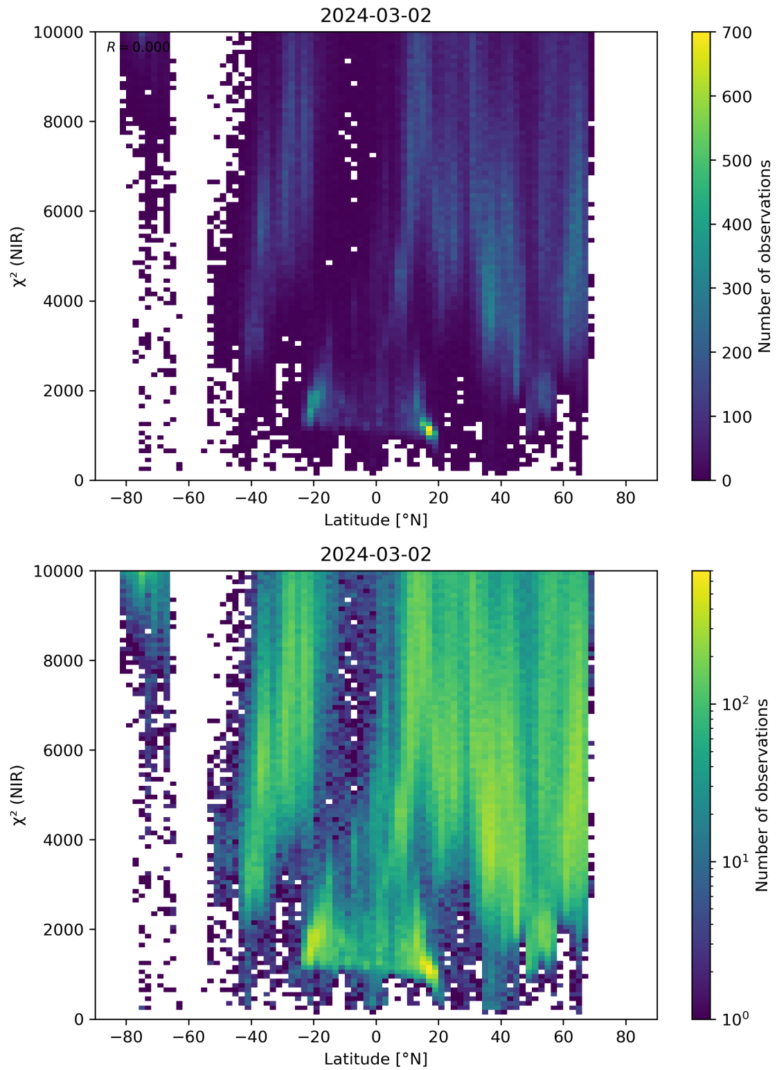
Figure 53: Scatter density plot of “Latitude” against “ \chi^2 (NIR)” for 2024-03-01 to 2024-03-03.
