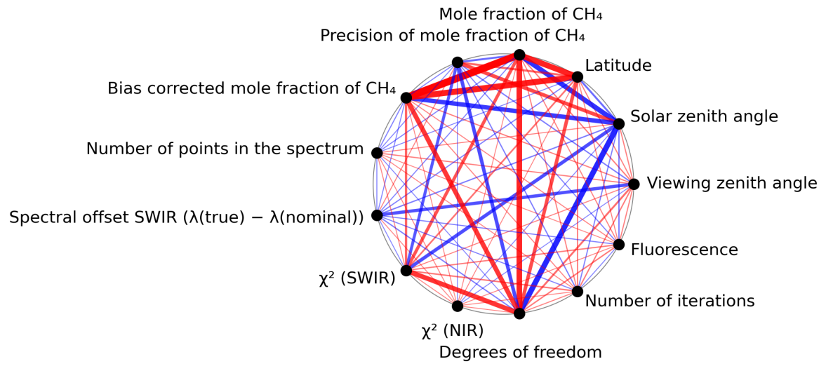
Figure 1: Map of correlation graph for 2024-03-01 to 2024-03-03.
