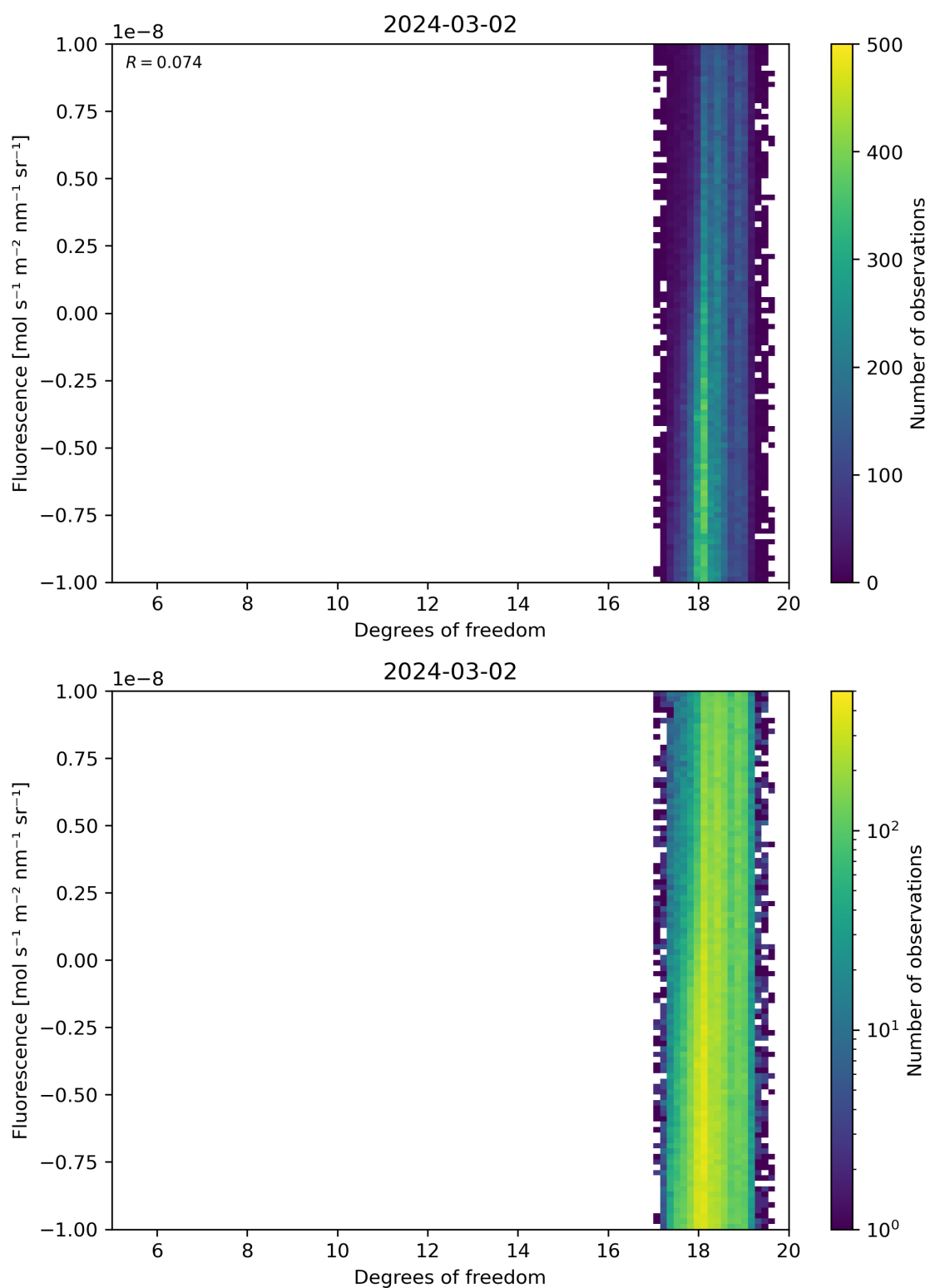
Figure 51: Scatter density plot of “Degrees of freedom” against “Fluorescence” for 2024-03-01 to 2024-03-03.
