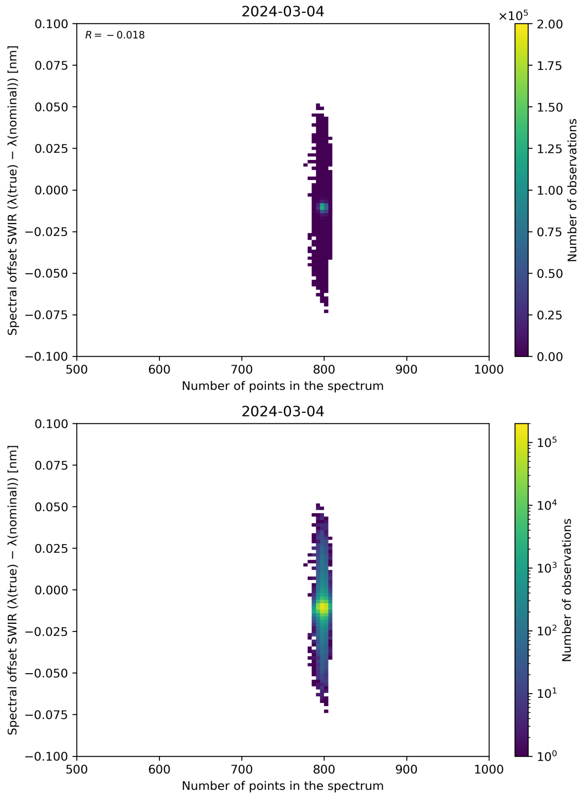
Figure 93: Scatter density plot of “Number of points in the spectrum” against “Spectral offset SWIR ( \lambda(\text{true}) - \lambda(\text{nominal}) )” for 2024-03-04 to 2024-03-05.
