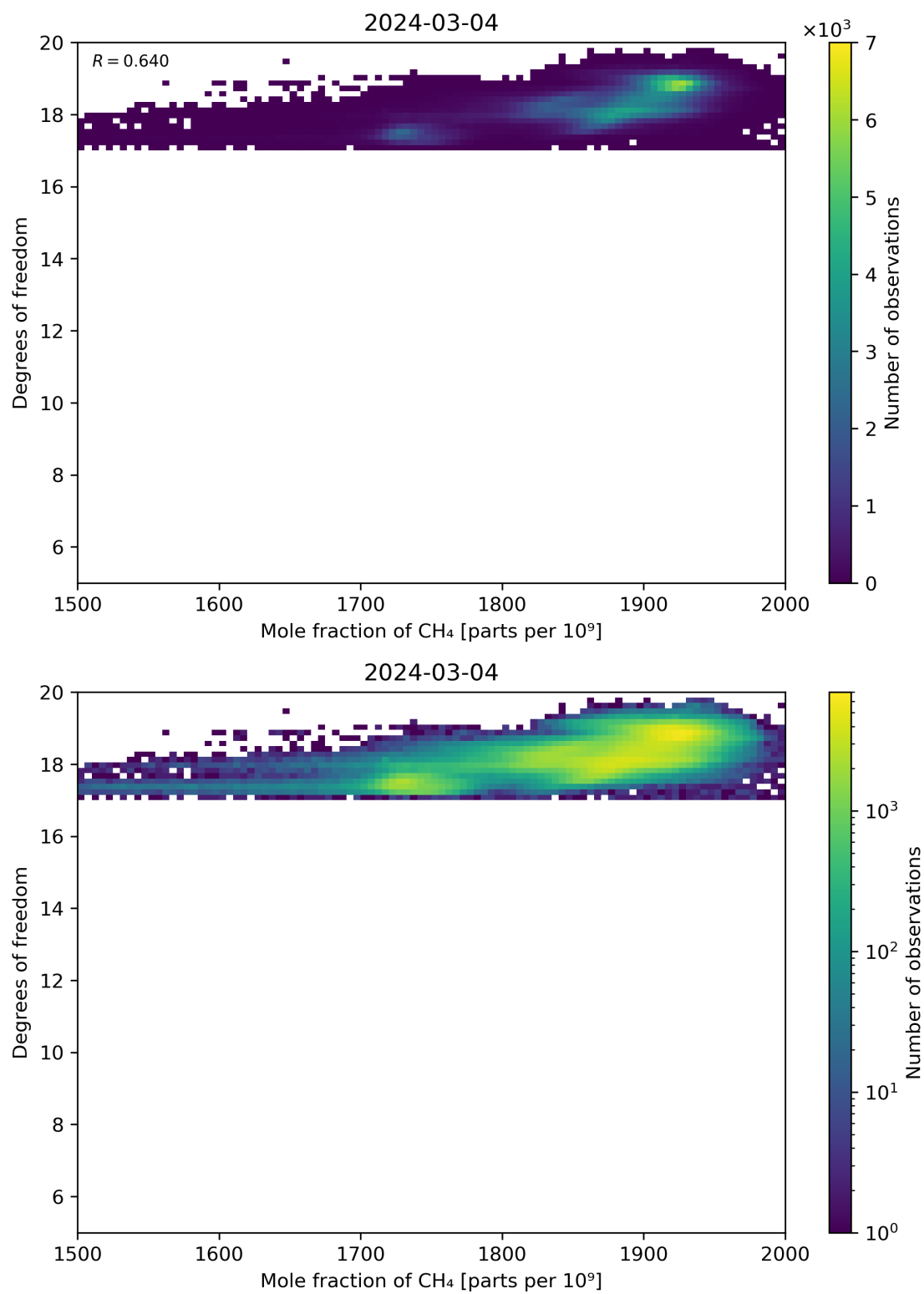
Figure 72: Scatter density plot of “Mole fraction of CH 4 ” against “Degrees of freedom” for 2024-03-04 to 2024-03-05.
