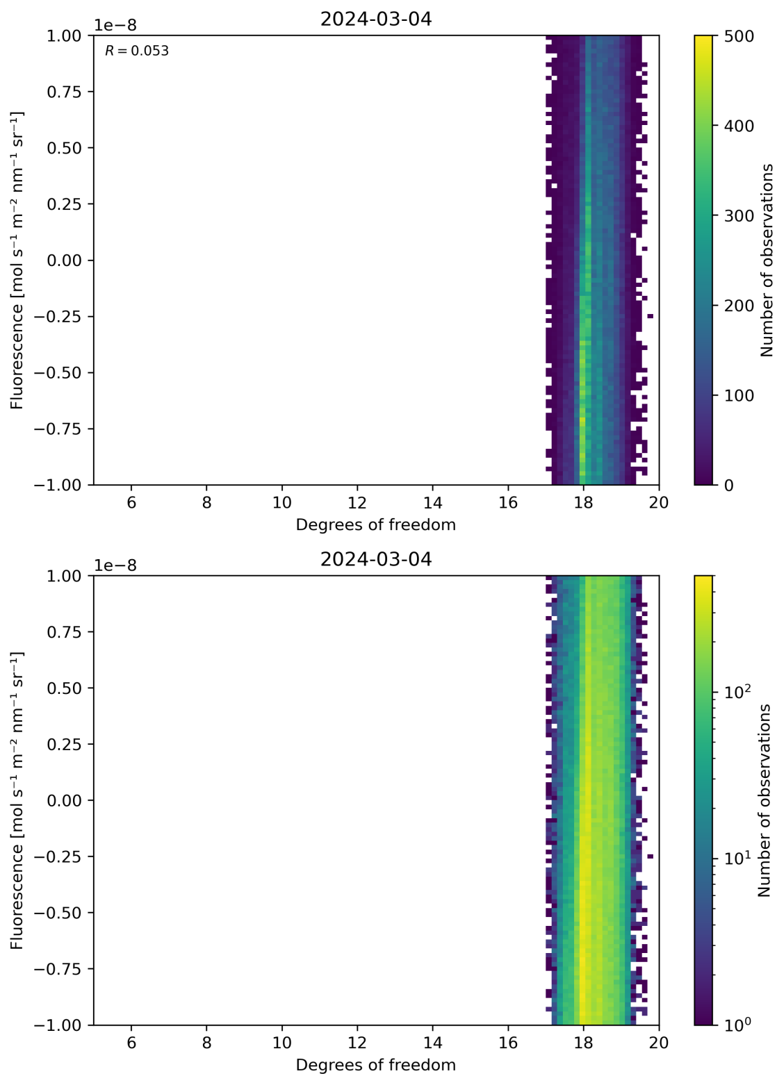
Figure 51: Scatter density plot of “Degrees of freedom” against “Fluorescence” for 2024-03-04 to 2024-03-05.
