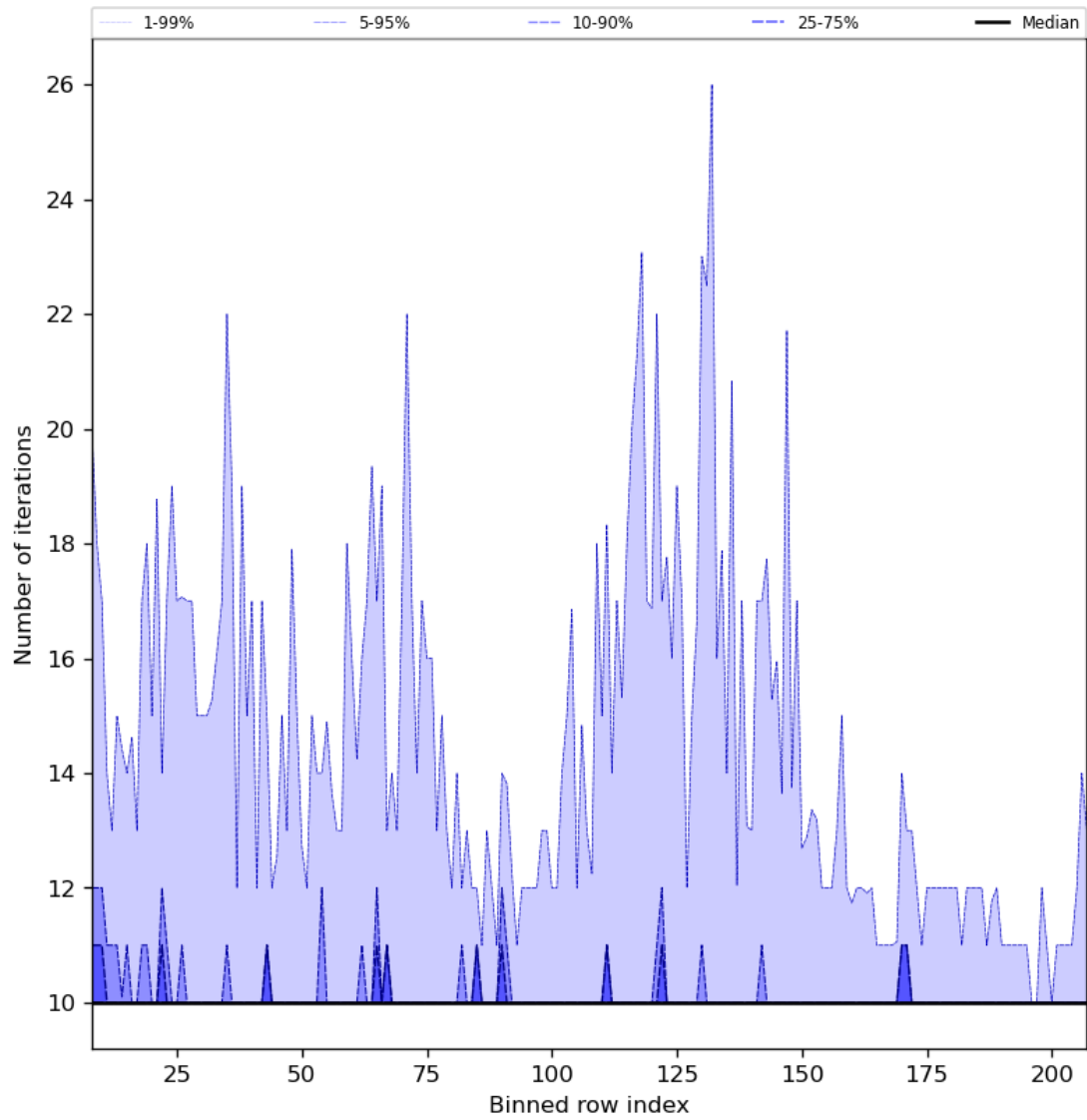
Figure 42: Along track statistics of “Number of iterations” for 2024-03-04 to 2024-03-05
