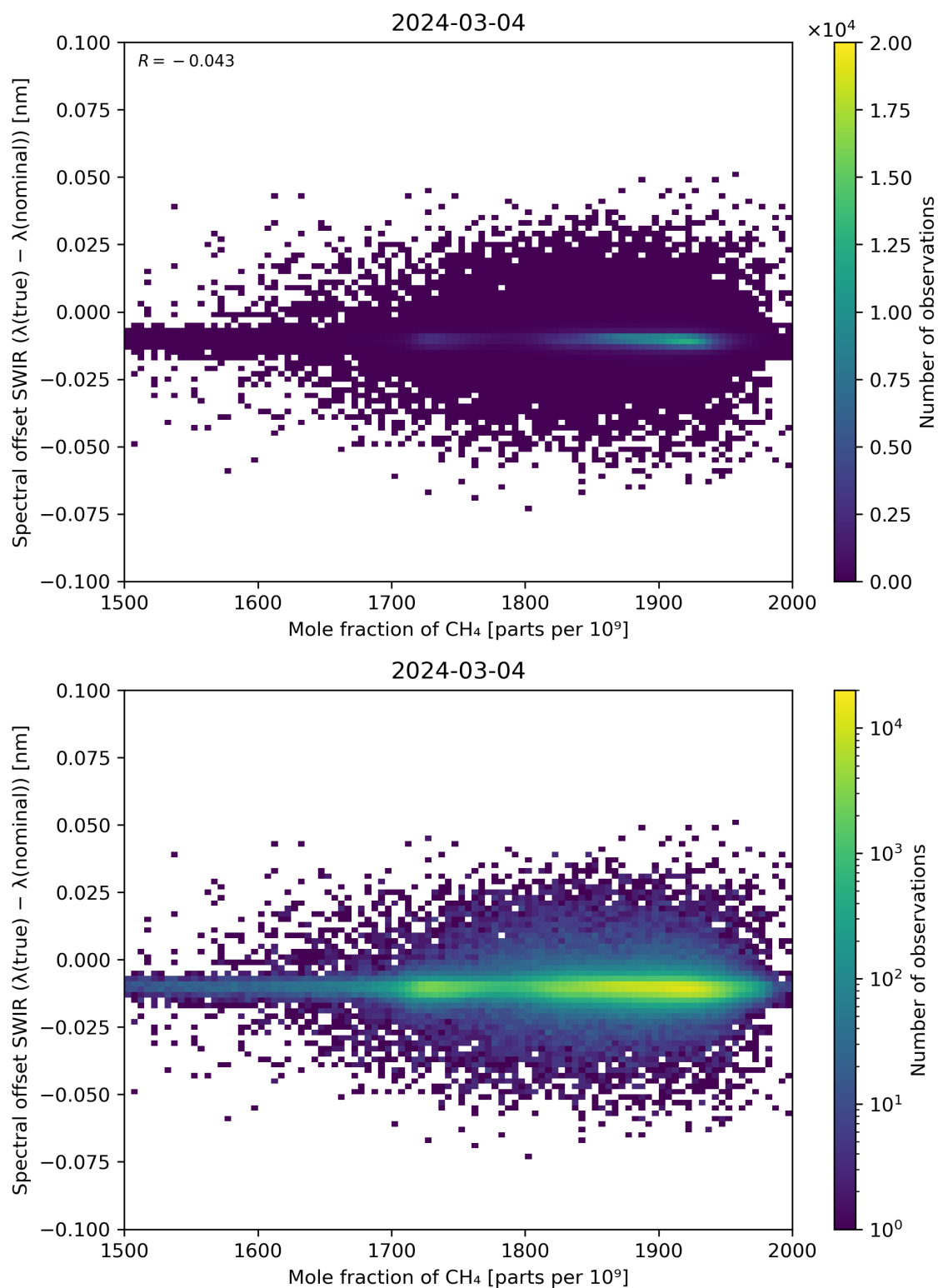
Figure 86: Scatter density plot of “Mole fraction of CH 4 ” against “Spectral offset SWIR ( \lambda(\text{true}) - \lambda(\text{nominal}) )” for 2024-03-04 to 2024-03-05.
