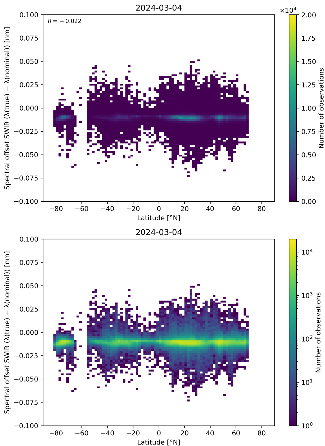
Figure 62: Scatter density plot of “Latitude” against “Spectral offset SWIR ( \lambda(\text{true}) - \lambda(\text{nominal}) )” for 2024-03-04 to 2024-03-05.
