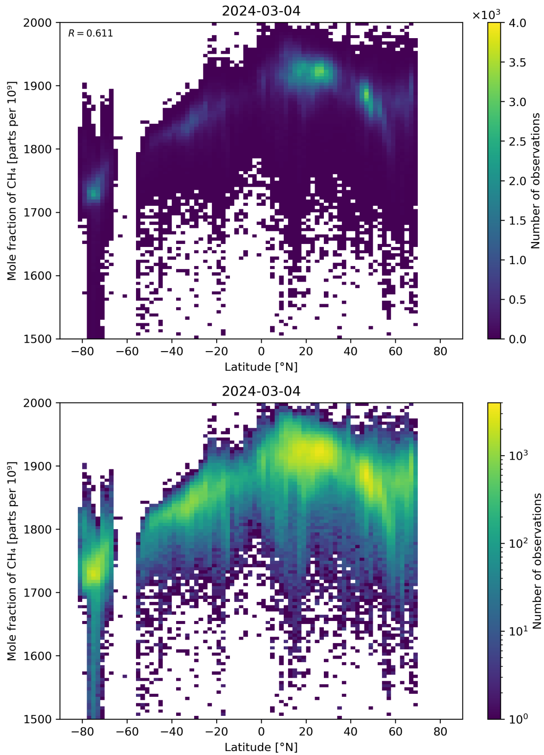
Figure 57: Scatter density plot of “Latitude” against “Mole fraction of \text{CH}_4 ” for 2024-03-04 to 2024-03-05.
