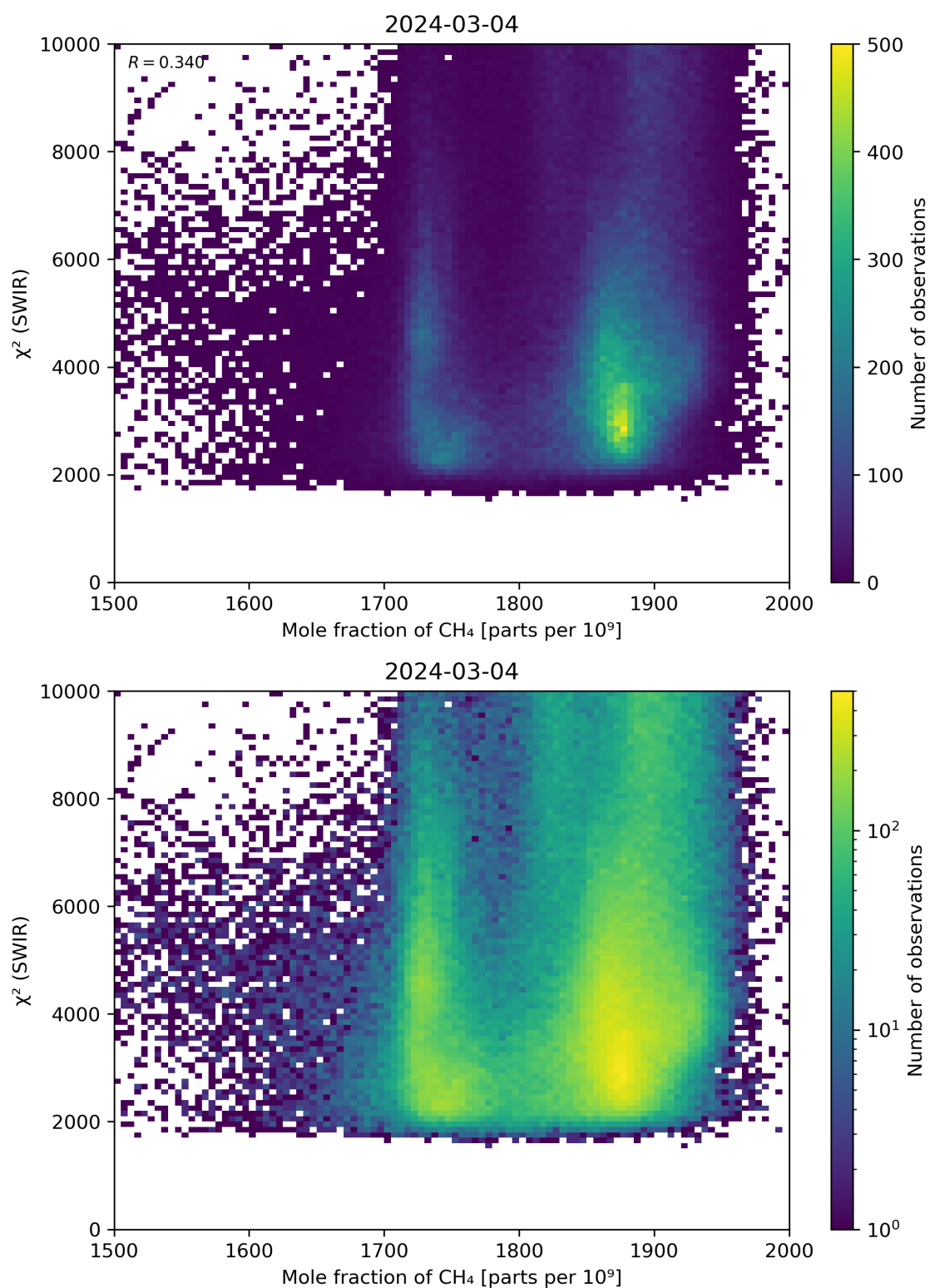
Figure 71: Scatter density plot of “Mole fraction of \text{CH}_4 ” against “ \chi^2 (SWIR)” for 2024-03-04 to 2024-03-05.
