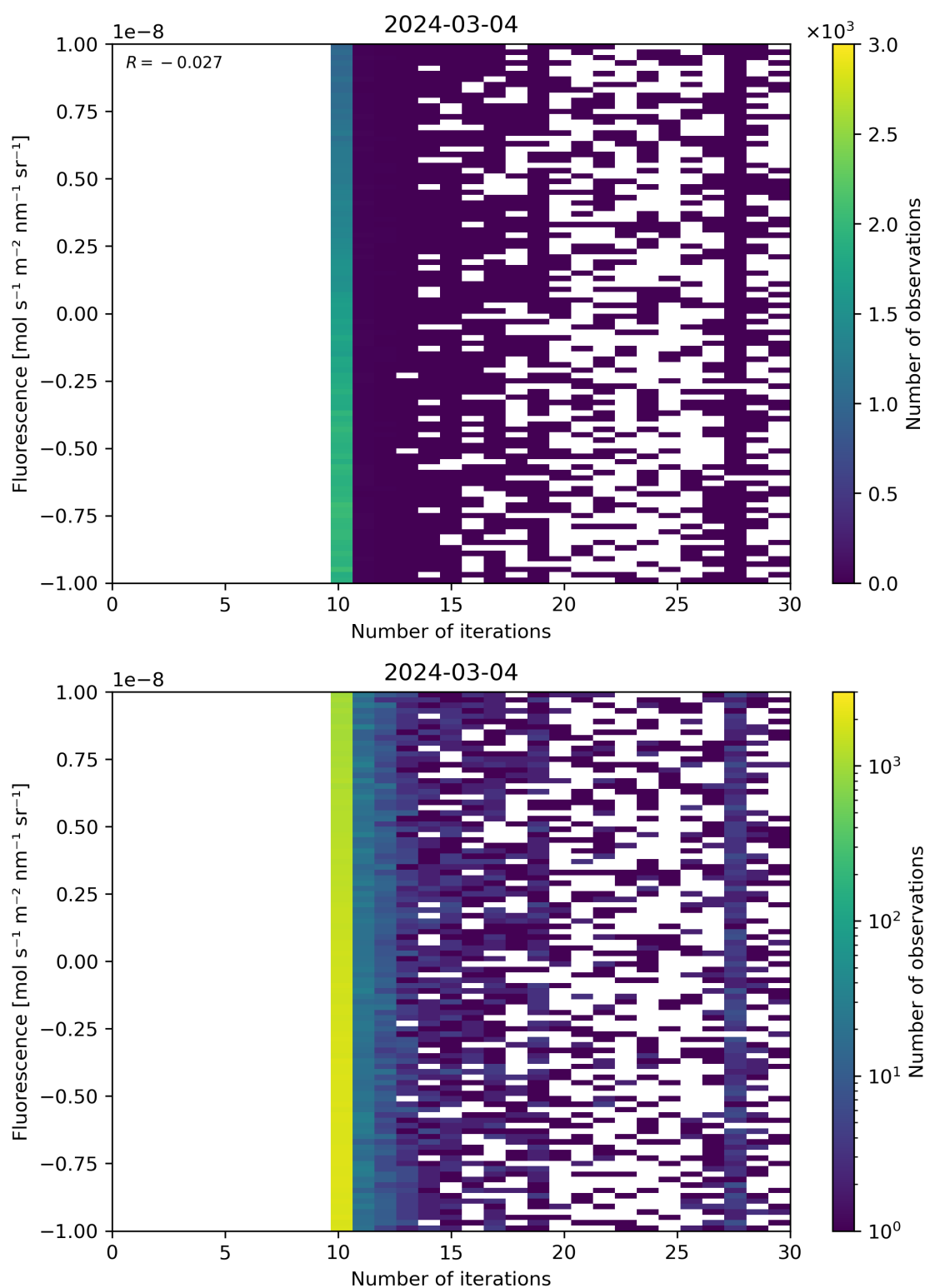
Figure 87: Scatter density plot of “Number of iterations” against “Fluorescence” for 2024-03-04 to 2024-03-05.
