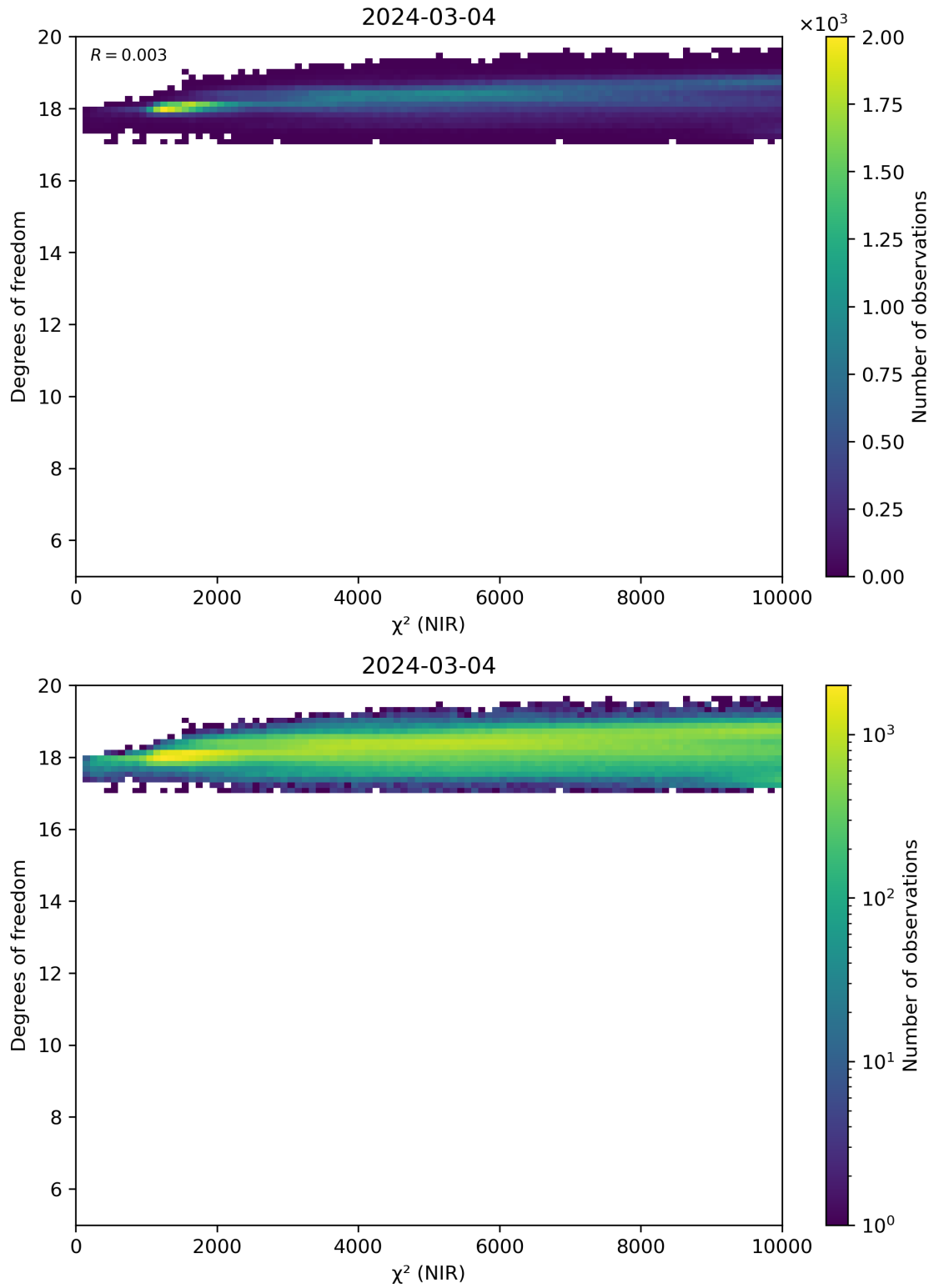
Figure 44: Scatter density plot of “ \chi^2 (NIR)” against “Degrees of freedom” for 2024-03-04 to 2024-03-05.
