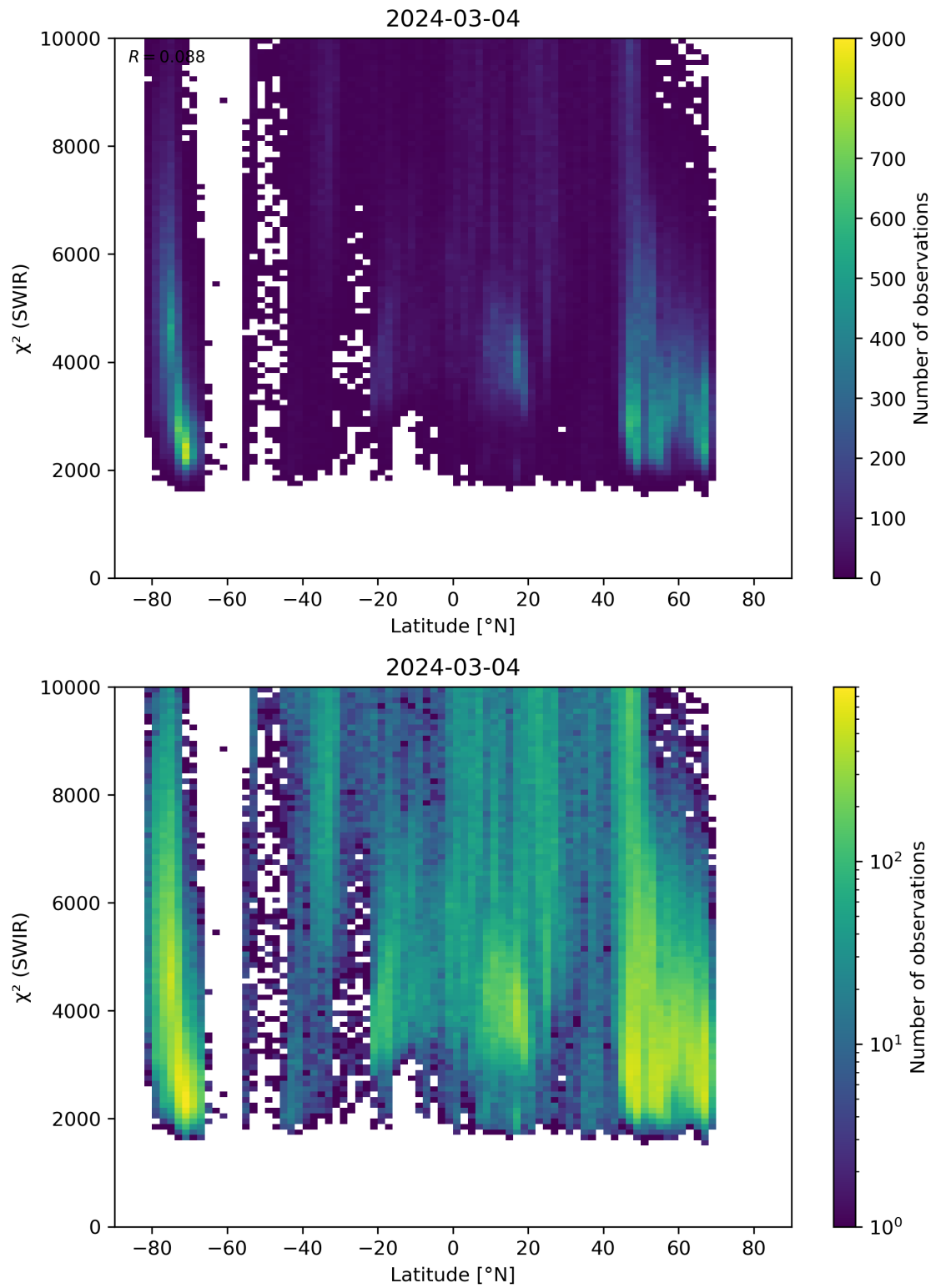
Figure 54: Scatter density plot of “Latitude” against “ \chi^2 (SWIR)” for 2024-03-04 to 2024-03-05.
