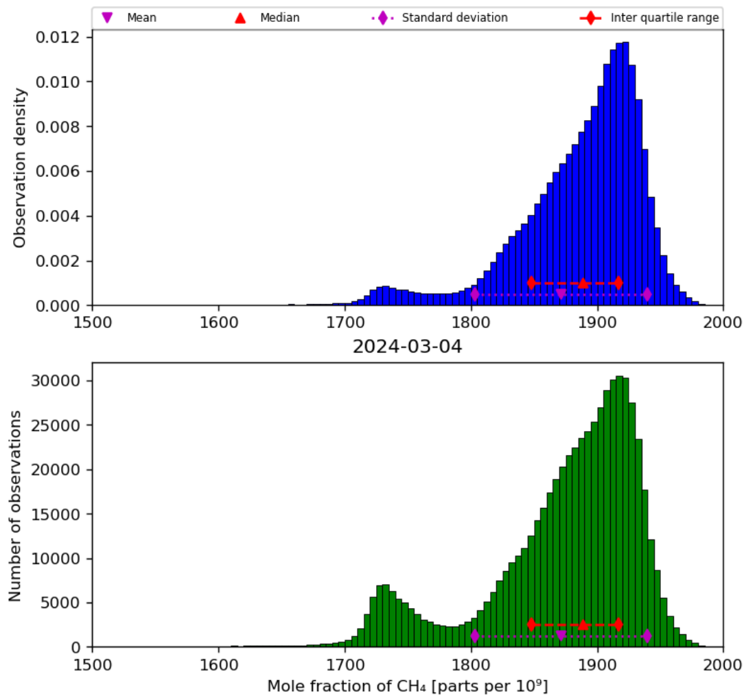
Figure 23: Histogram of “Mole fraction of CH 4 ” for 2024-03-04 to 2024-03-05
