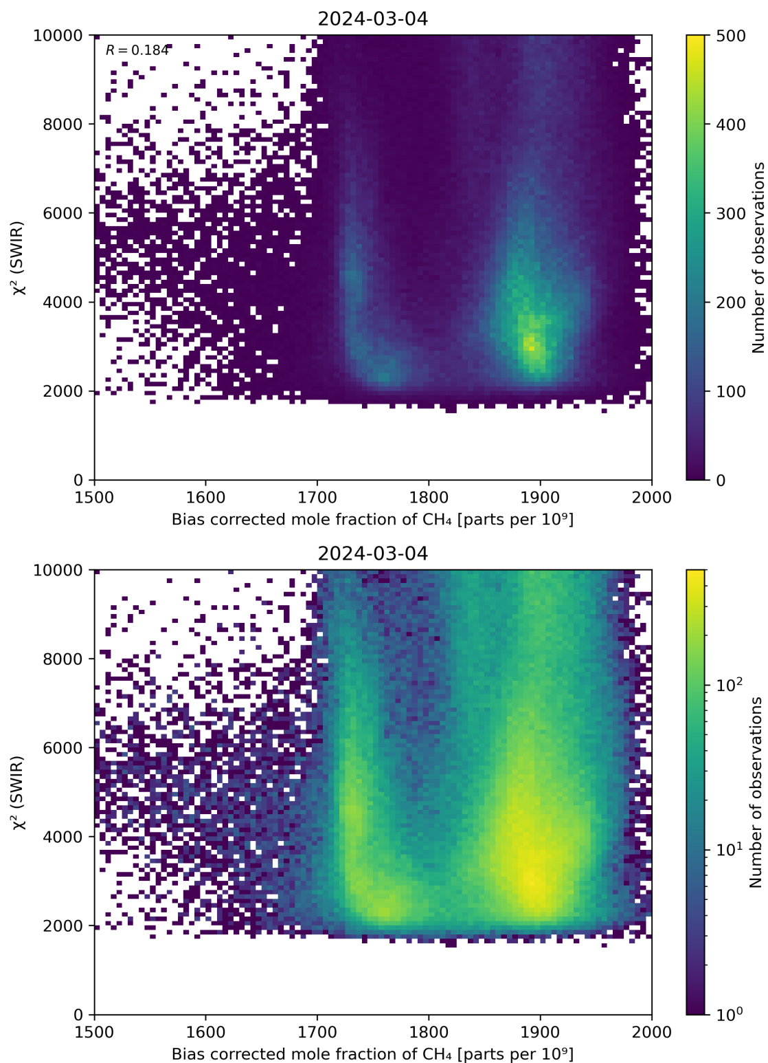
Figure 64: Scatter density plot of “Bias corrected mole fraction of CH 4 ” against “ \chi^2 (SWIR)” for 2024-03-04 to 2024-03-05.
