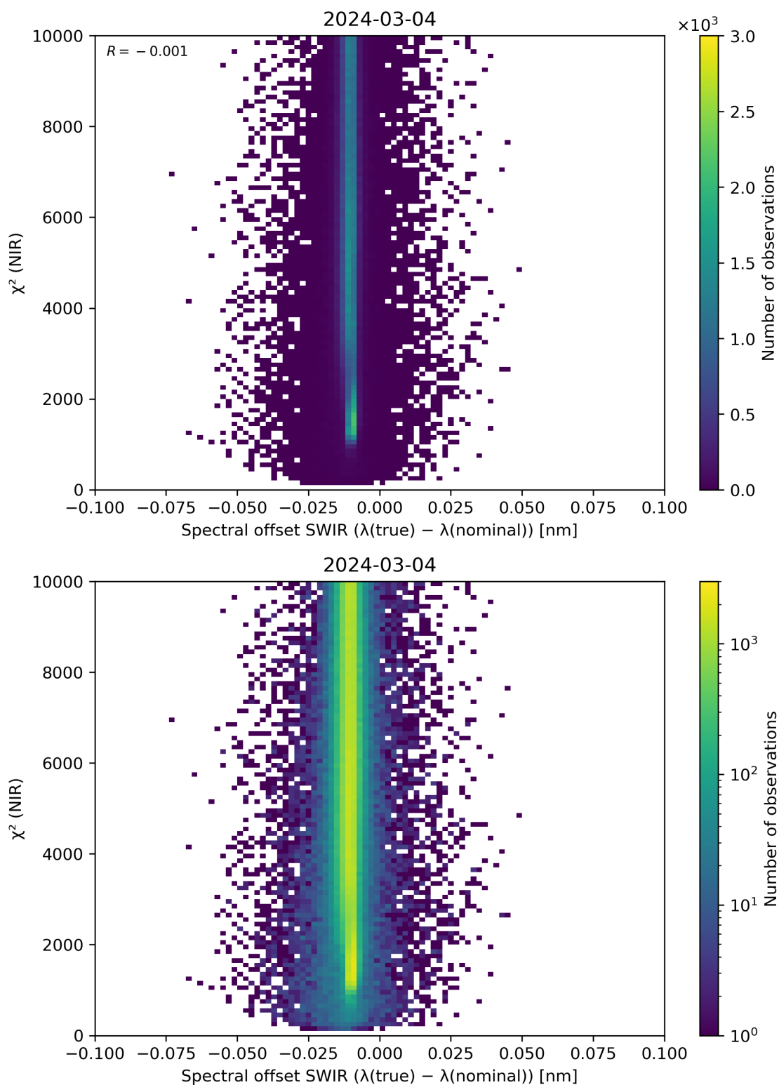
Figure 117: Scatter density plot of “Spectral offset SWIR ( \lambda(\text{true}) - \lambda(\text{nominal}) )” against “ \chi^2 (NIR)” for 2024-03-04 to 2024-03-05.
