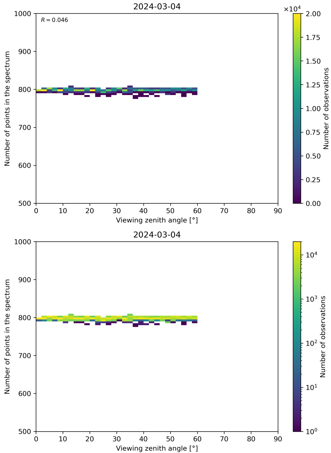
Figure 114: Scatter density plot of “Viewing zenith angle” against “Number of points in the spectrum” for 2024-03-04 to 2024-03-05.
