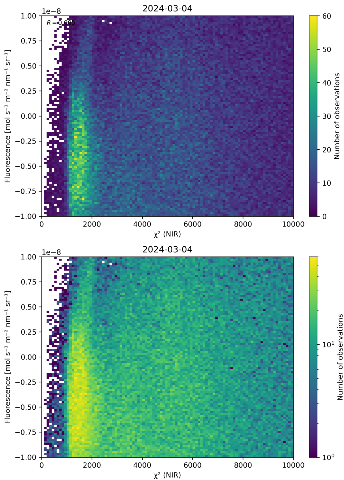
Figure 45: Scatter density plot of “ \chi^2 (NIR)” against “Fluorescence” for 2024-03-04 to 2024-03-05.
