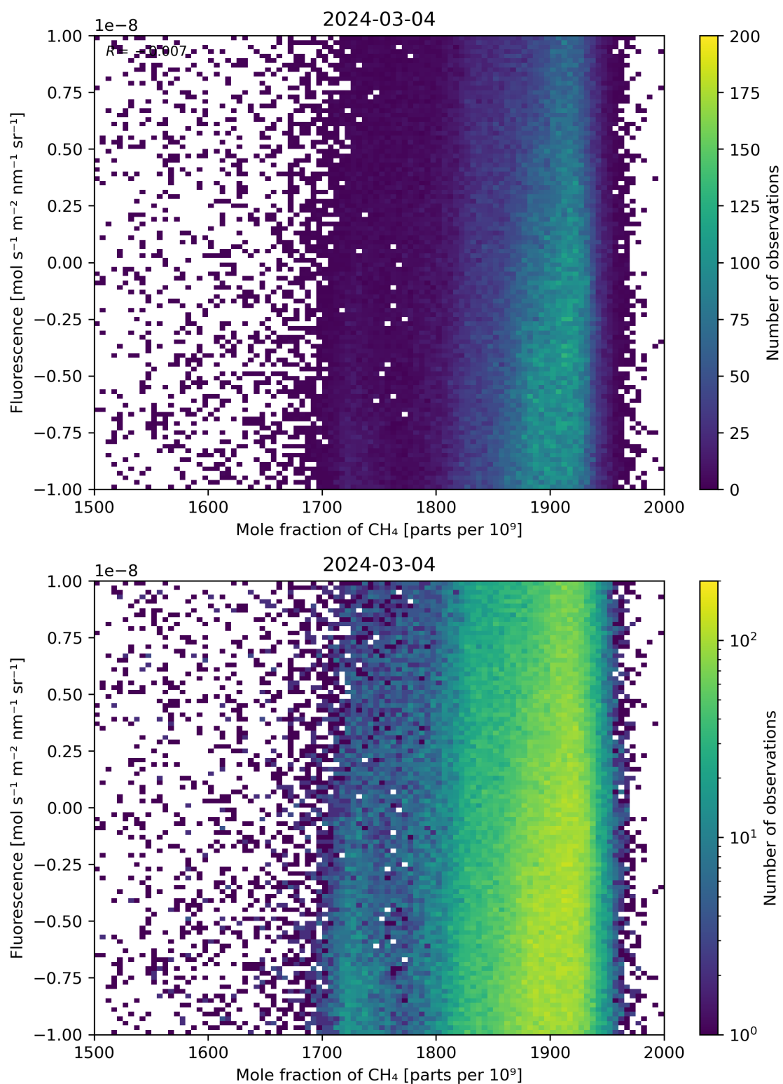
Figure 73: Scatter density plot of “Mole fraction of \text{CH}_4 ” against “Fluorescence” for 2024-03-04 to 2024-03-05.
