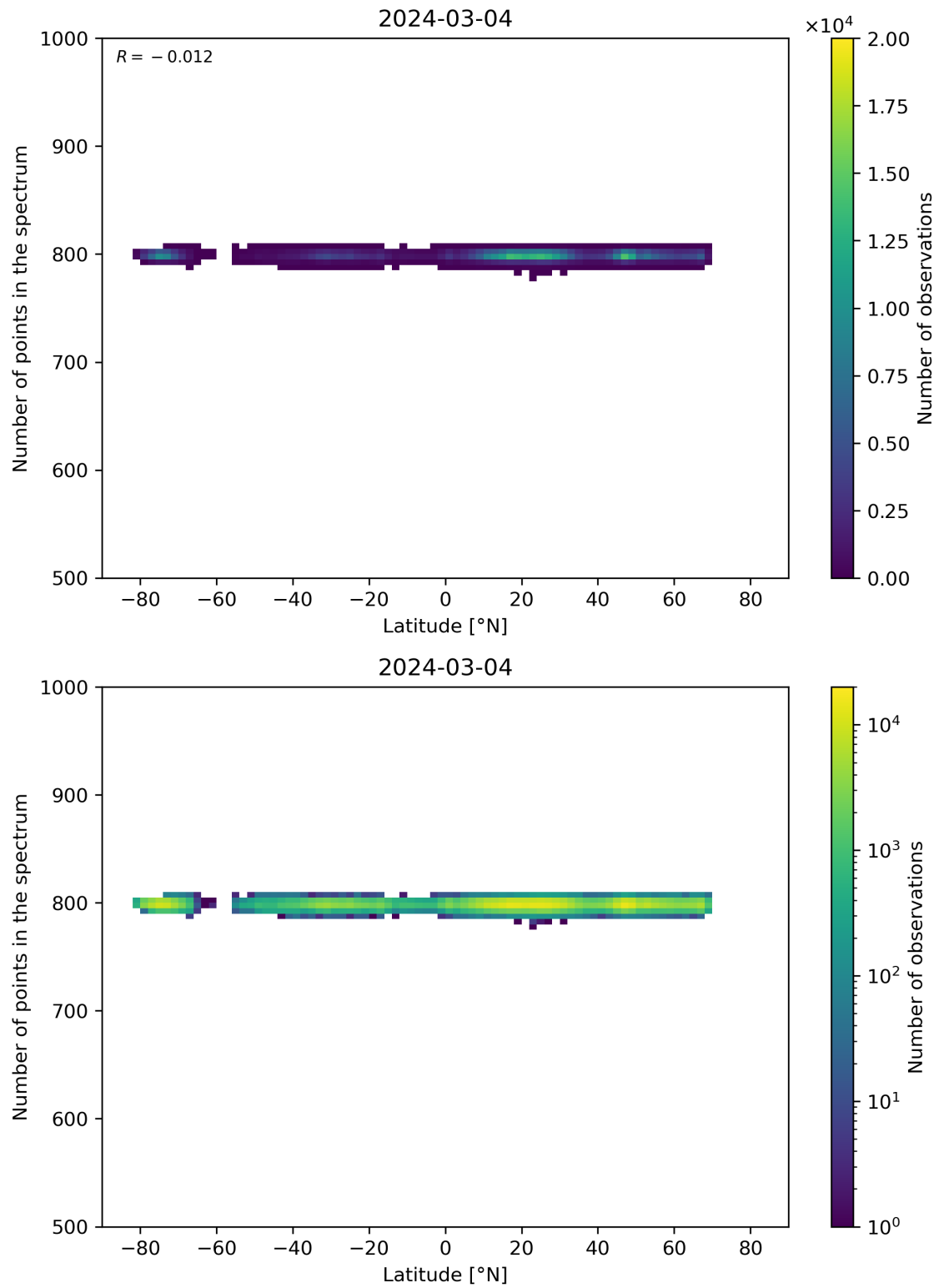
Figure 61: Scatter density plot of “Latitude” against “Number of points in the spectrum” for 2024-03-04 to 2024-03-05.
