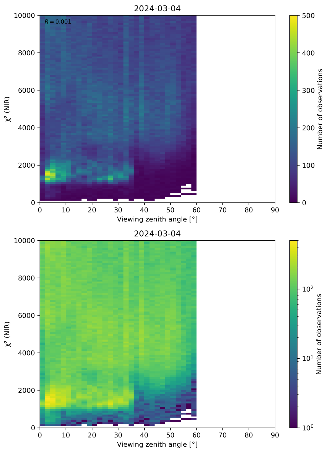
Figure 105: Scatter density plot of “Viewing zenith angle” against “ \chi^2 (NIR)” for 2024-03-04 to 2024-03-05.
