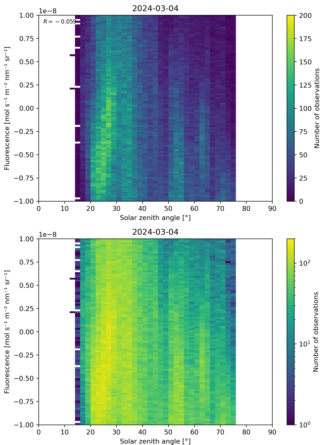
Figure 97: Scatter density plot of “Solar zenith angle” against “Fluorescence” for 2024-03-04 to 2024-03-05.
