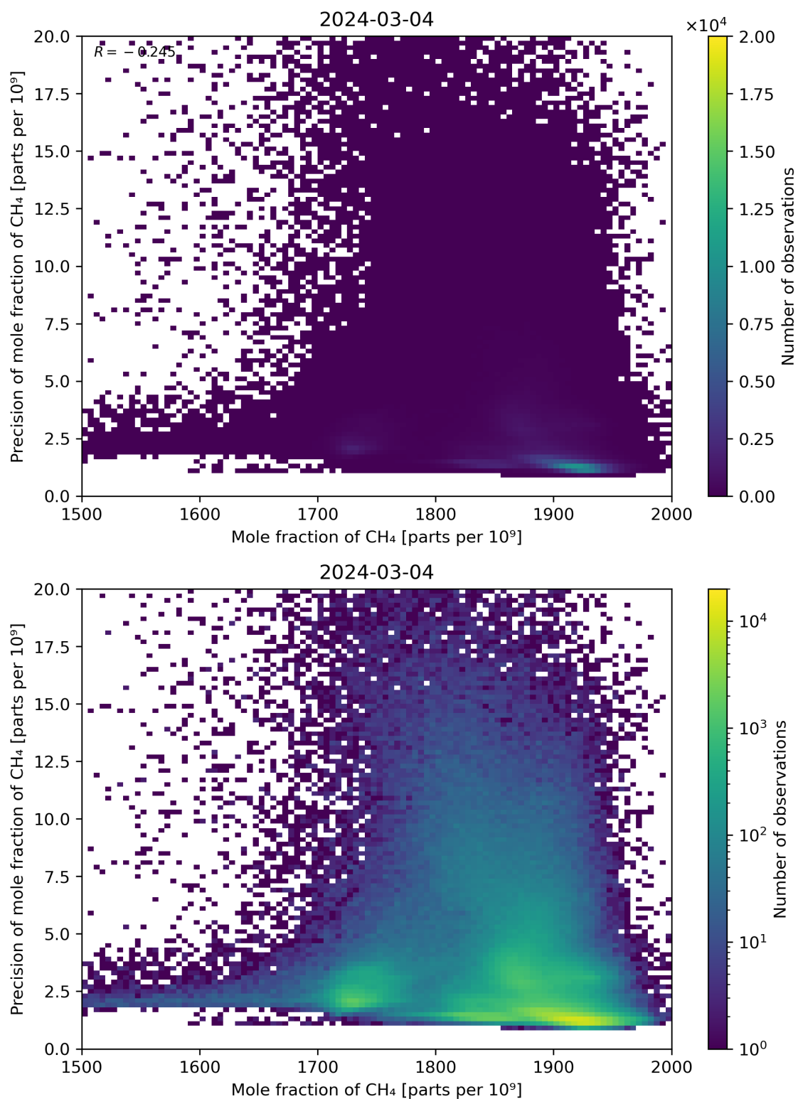
Figure 75: Scatter density plot of “Mole fraction of CH 4 ” against “Precision of mole fraction of CH 4 ” for 2024-03-04 to 2024-03-05.
