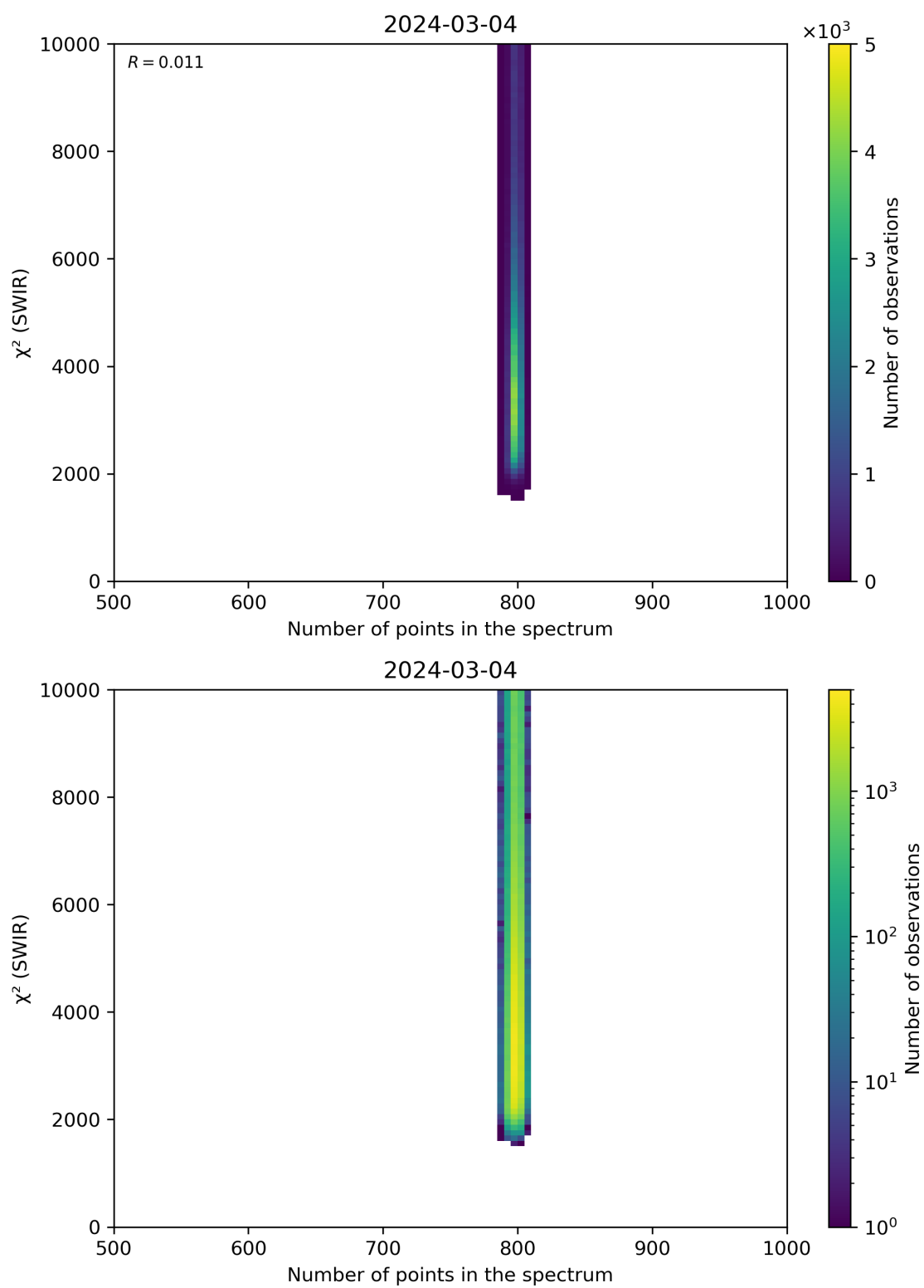
Figure 89: Scatter density plot of “Number of points in the spectrum” against “ \chi^2 (SWIR)” for 2024-03-04 to 2024-03-05.
