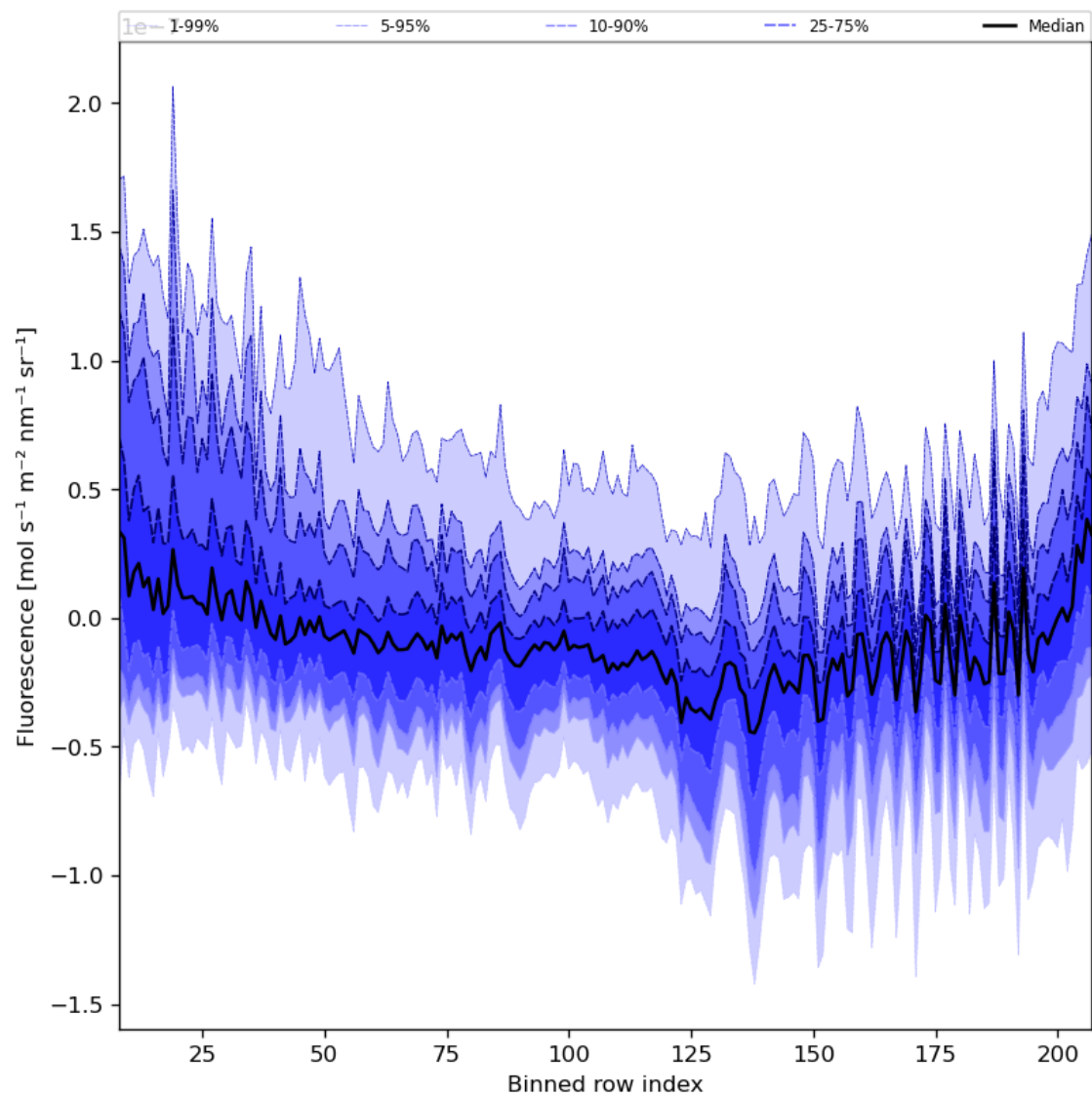
Figure 43: Along track statistics of “Fluorescence” for 2024-03-04 to 2024-03-05
