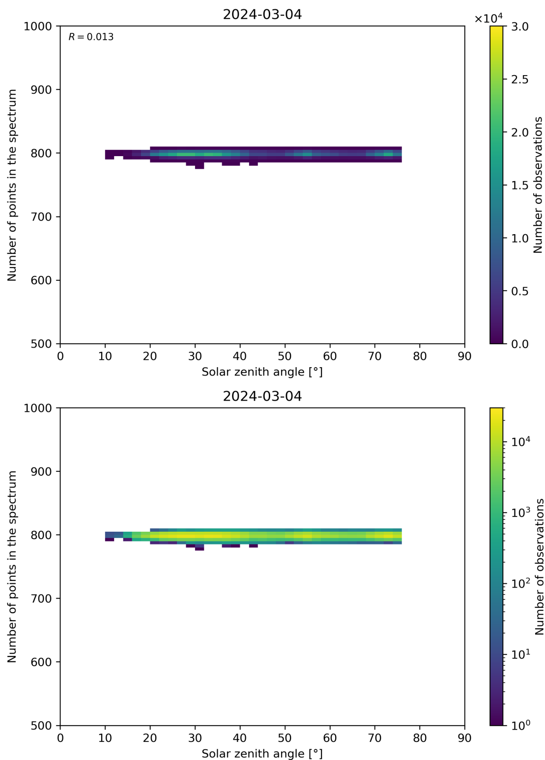
Figure 103: Scatter density plot of “Solar zenith angle” against “Number of points in the spectrum” for 2024-03-04 to 2024-03-05.
