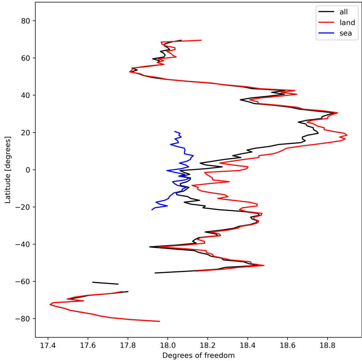
Figure 19: Zonal average of “Degrees of freedom” for 2024-03-04 to 2024-03-05.
