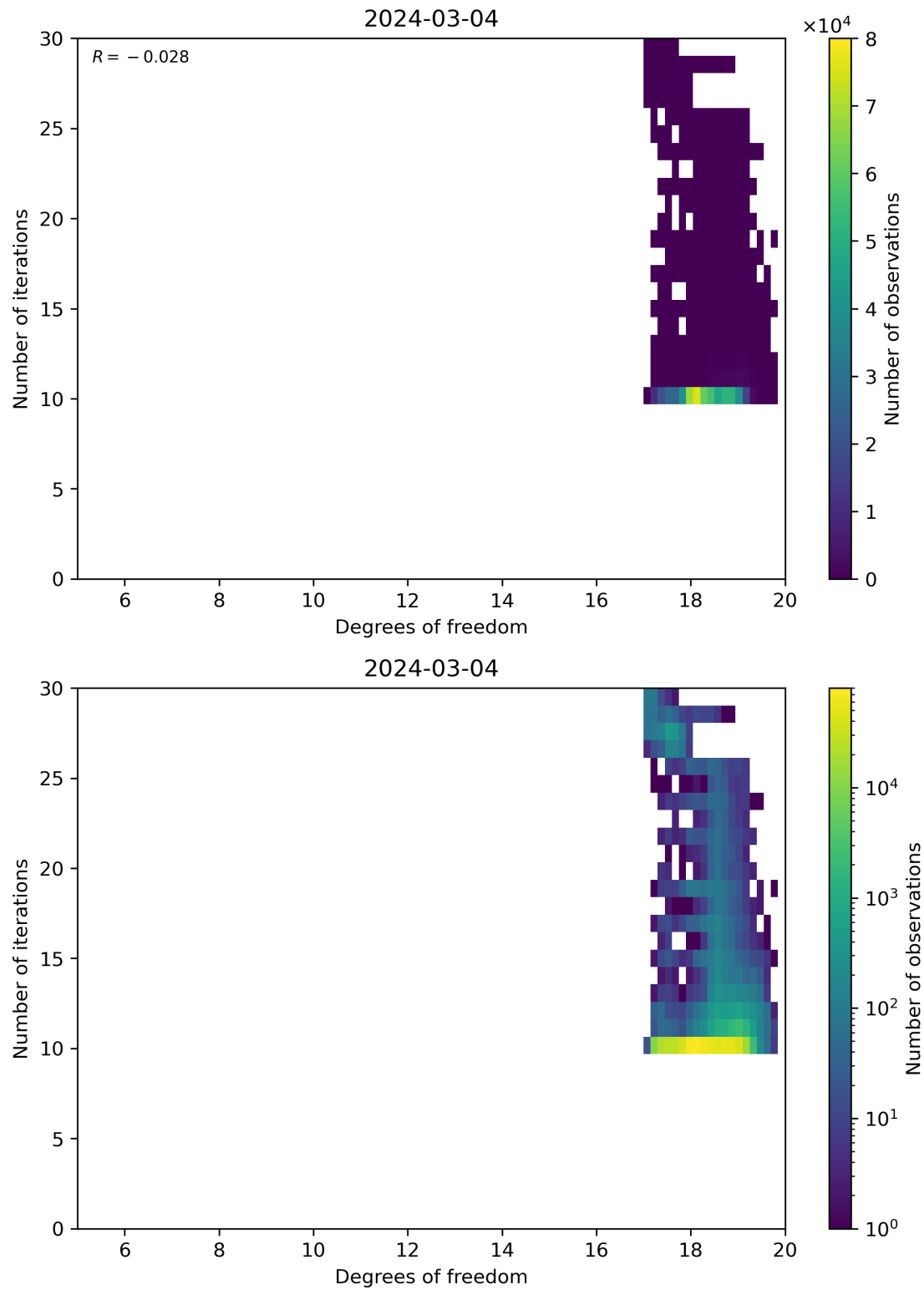
Figure 52: Scatter density plot of “Degrees of freedom” against “Number of iterations” for 2024-03-04 to 2024-03-05.
