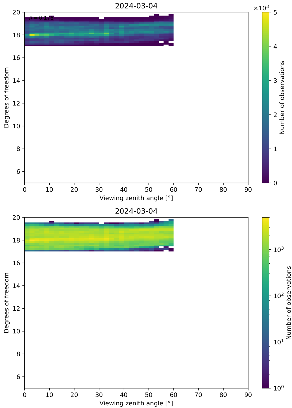
Figure 107: Scatter density plot of “Viewing zenith angle” against “Degrees of freedom” for 2024-03-04 to 2024-03-05.
