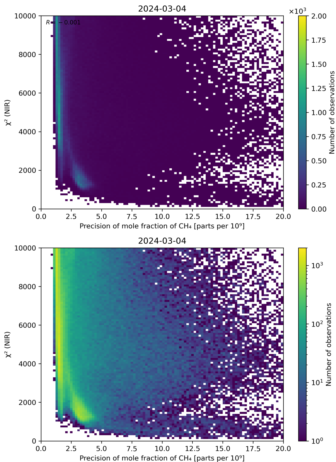
Figure 78: Scatter density plot of “Precision of mole fraction of CH 4 ” against “ \chi^2 (NIR)” for 2024-03-04 to 2024-03-05.
