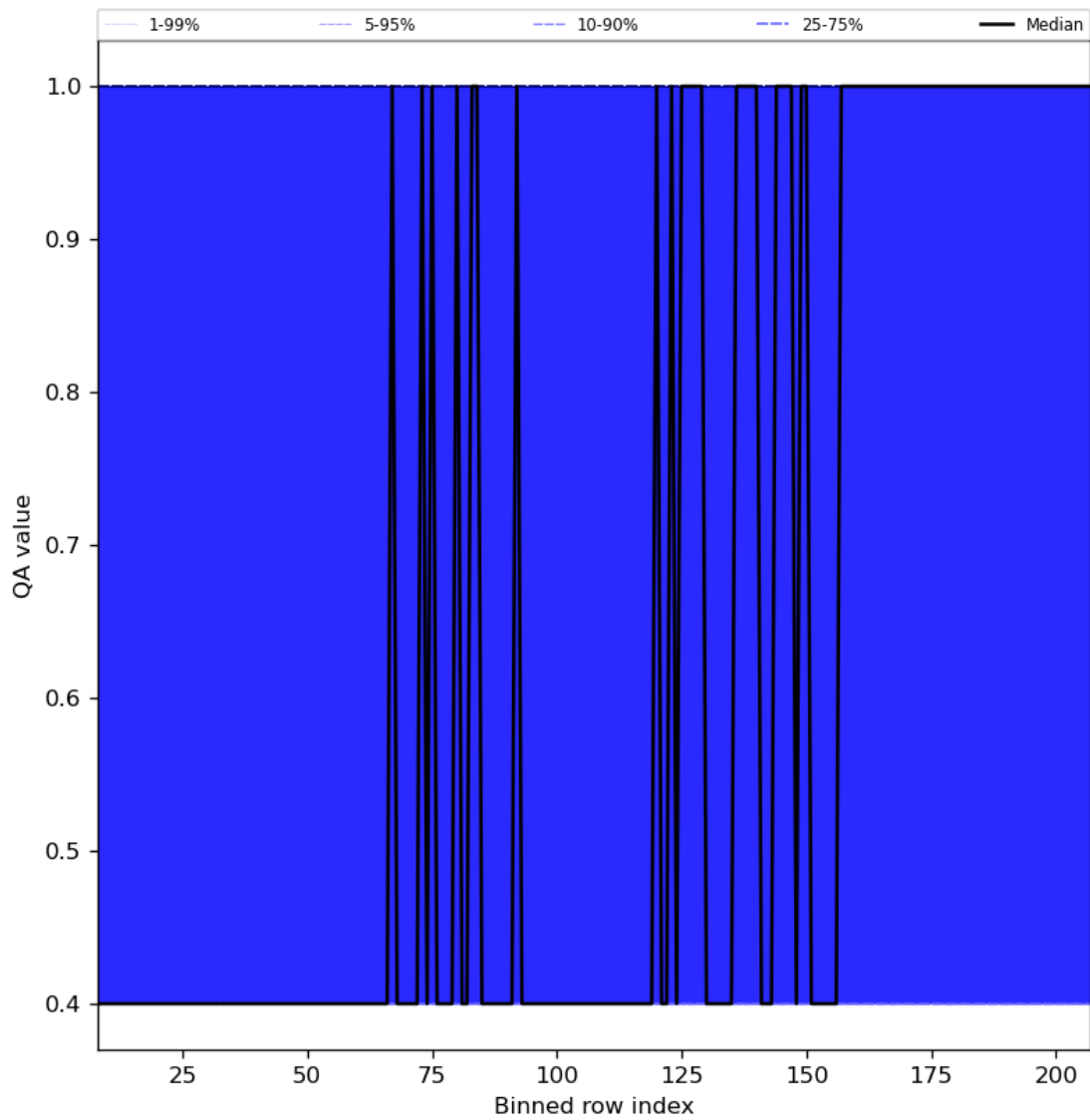
Figure 33: Along track statistics of “QA value” for 2024-03-04 to 2024-03-05
