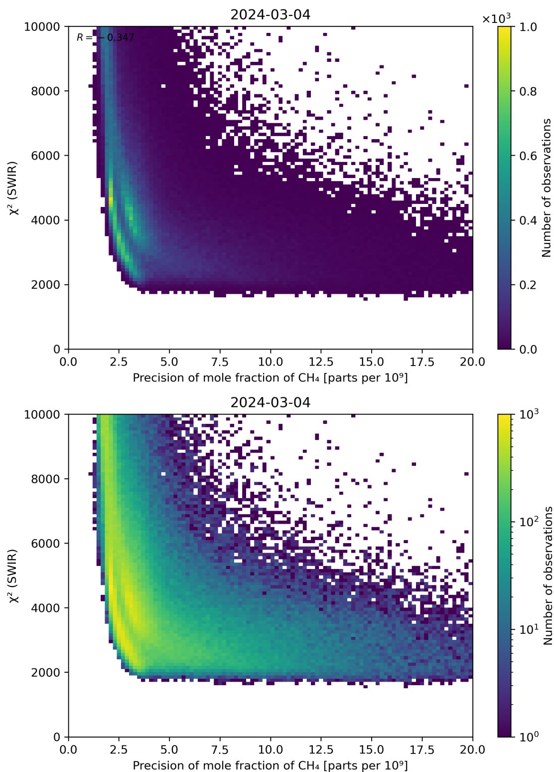
Figure 79: Scatter density plot of “Precision of mole fraction of \text{CH}_4 ” against “ \chi^2 (SWIR)” for 2024-03-04 to 2024-03-05.
