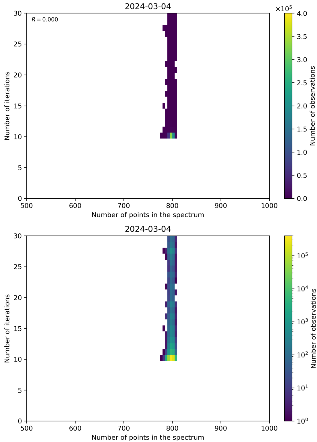
Figure 92: Scatter density plot of “Number of points in the spectrum” against “Number of iterations” for 2024-03-04 to 2024-03-05.
