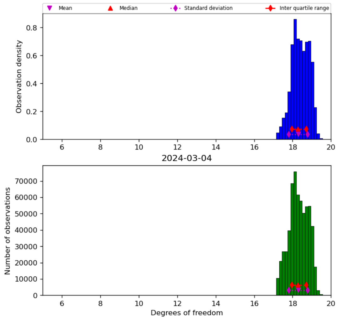
Figure 30: Histogram of “Degrees of freedom” for 2024-03-04 to 2024-03-05
