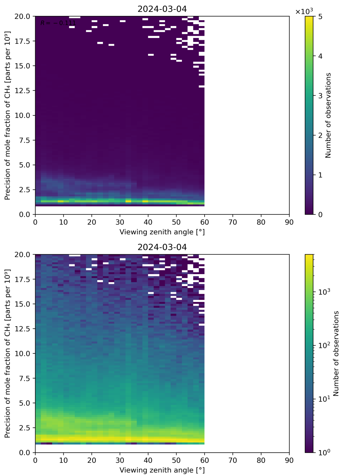
Figure 112: Scatter density plot of “Viewing zenith angle” against “Precision of mole fraction of CH 4 ” for 2024-03-04 to 2024-03-05.
