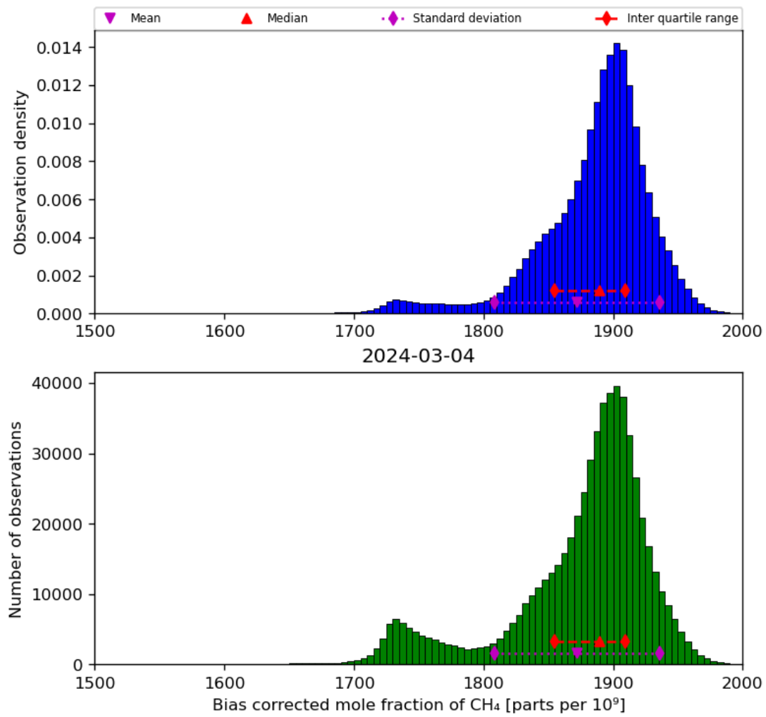
Figure 25: Histogram of “Bias corrected mole fraction of CH 4 ” for 2024-03-04 to 2024-03-05
