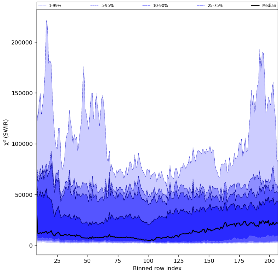
Figure 39: Along track statistics of “ \chi^2 (SWIR)” for 2024-03-04 to 2024-03-05
