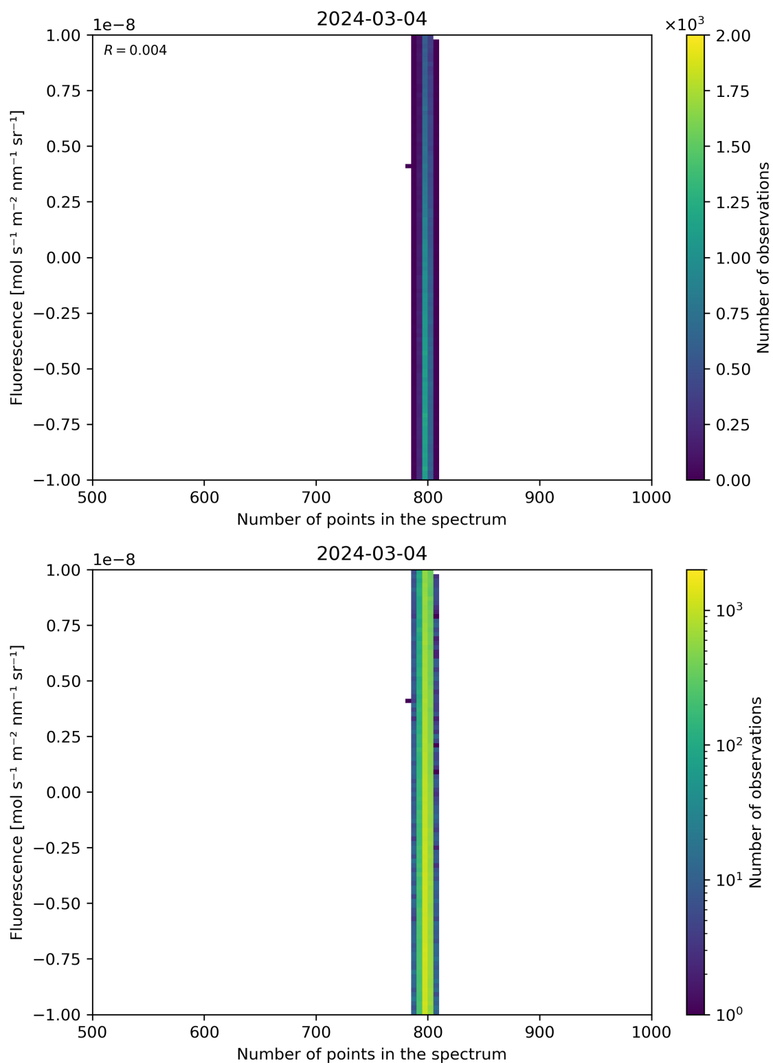
Figure 91: Scatter density plot of “Number of points in the spectrum” against “Fluorescence” for 2024-03-04 to 2024-03-05.
