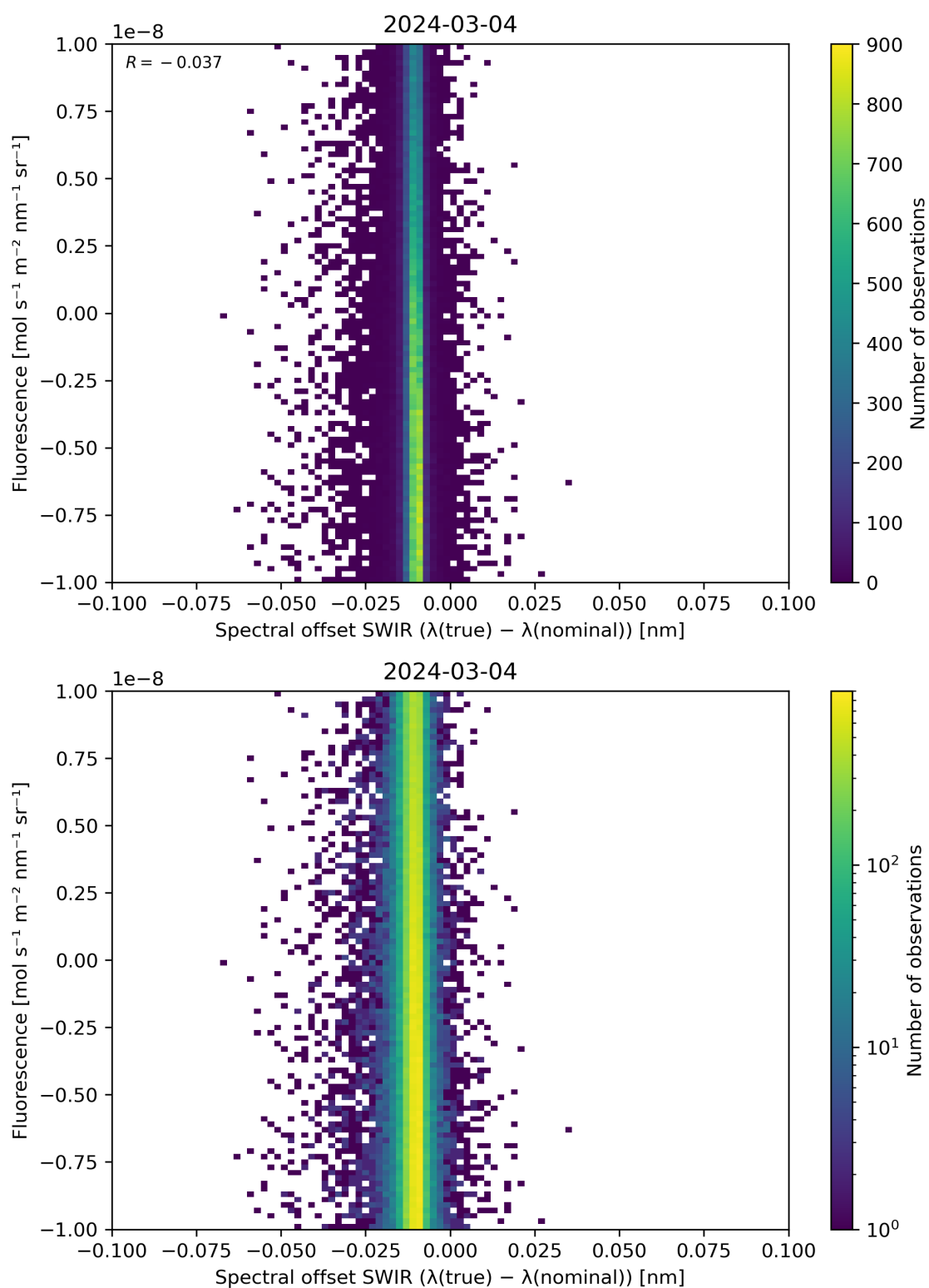
Figure 120: Scatter density plot of “Spectral offset SWIR ( \lambda(\text{true}) - \lambda(\text{nominal}) )” against “Fluorescence” for 2024-03-04 to 2024-03-05.
