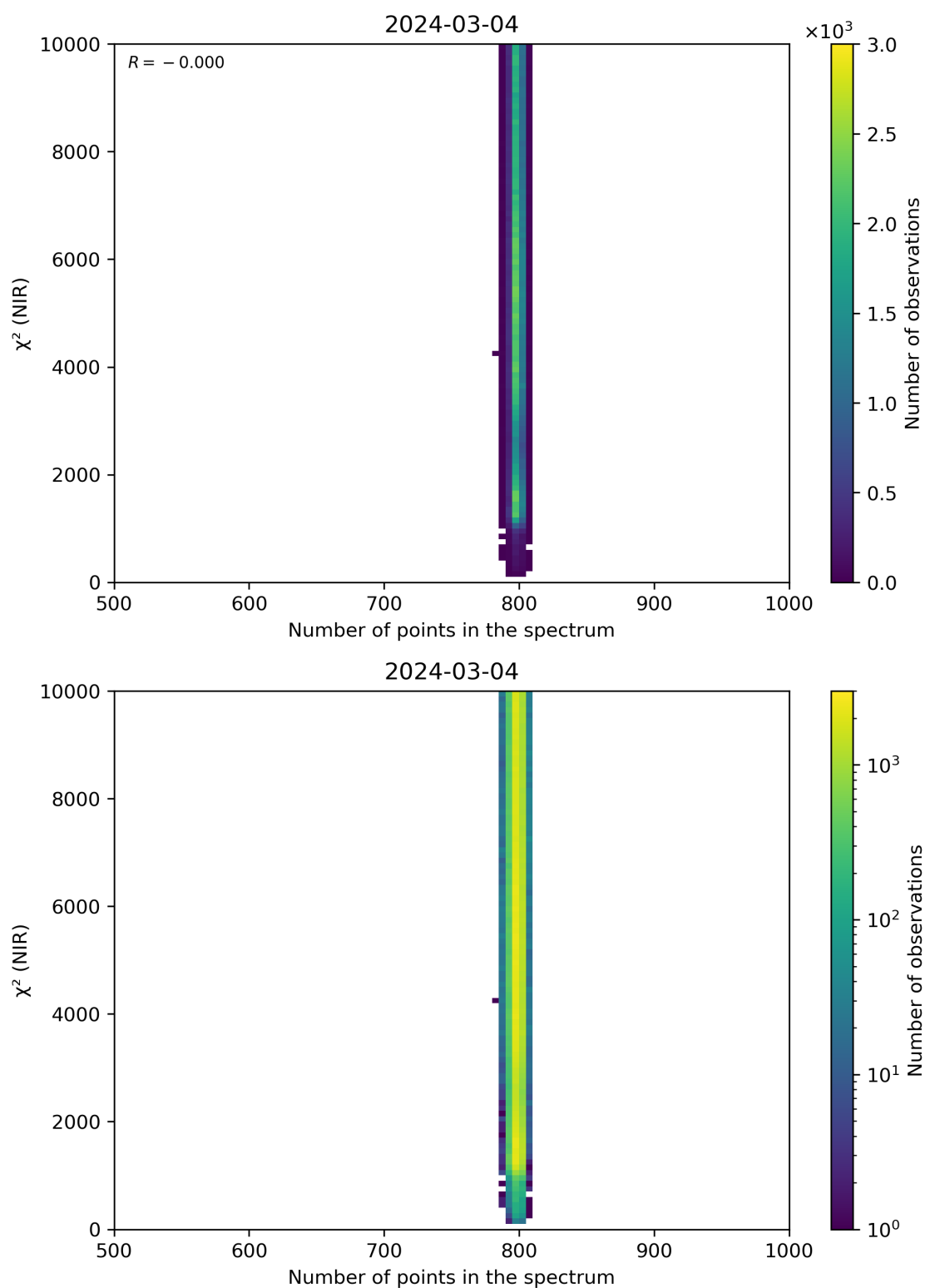
Figure 88: Scatter density plot of “Number of points in the spectrum” against “ \chi^2 (NIR)” for 2024-03-04 to 2024-03-05.
