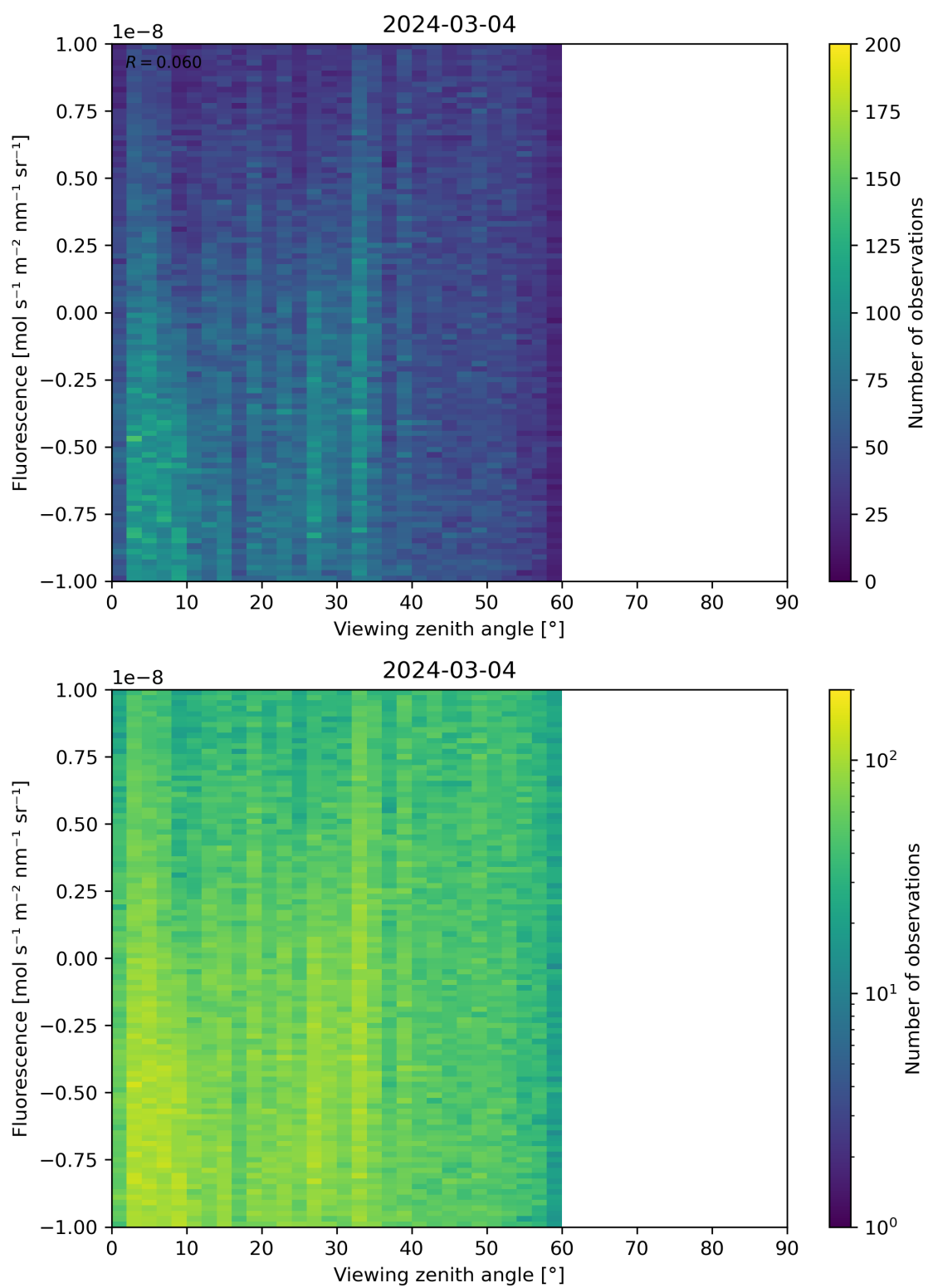
Figure 108: Scatter density plot of “Viewing zenith angle” against “Fluorescence” for 2024-03-04 to 2024-03-05.
