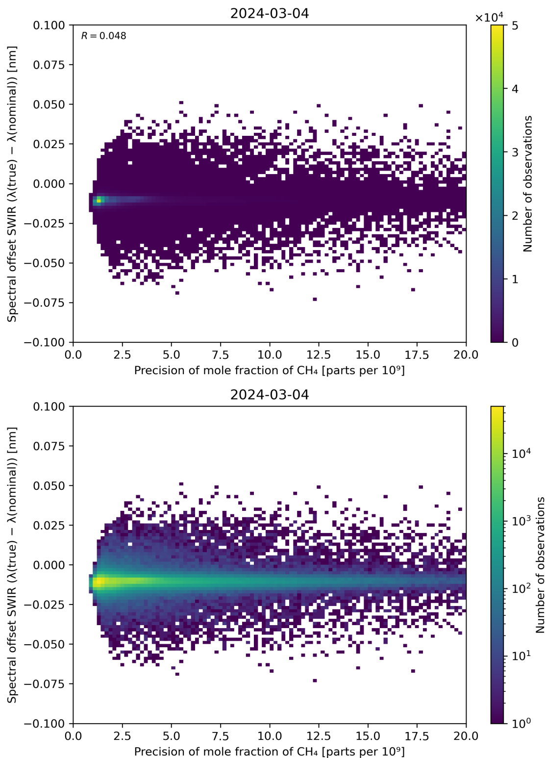
Figure 85: Scatter density plot of “Precision of mole fraction of CH 4 ” against “Spectral offset SWIR ( \lambda(\text{true}) - \lambda(\text{nominal}) )” for 2024-03-04 to 2024-03-05.
