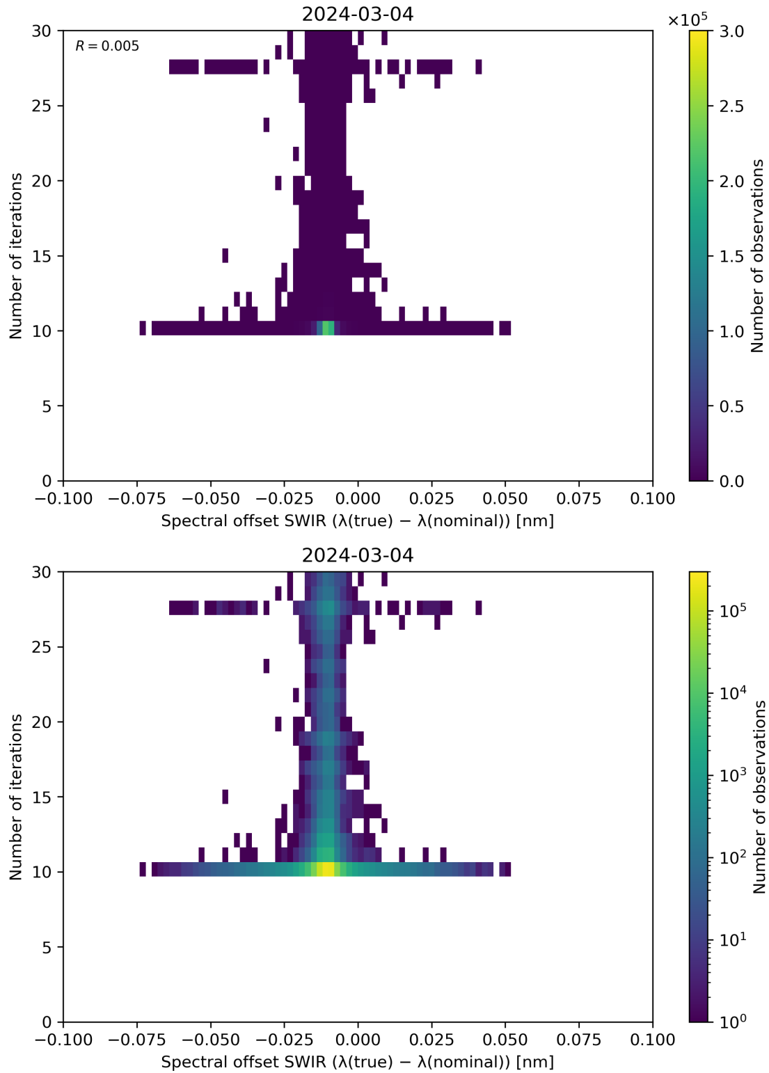
Figure 121: Scatter density plot of “Spectral offset SWIR ( \lambda(\text{true}) - \lambda(\text{nominal}) )” against “Number of iterations” for 2024-03-04 to 2024-03-05.
