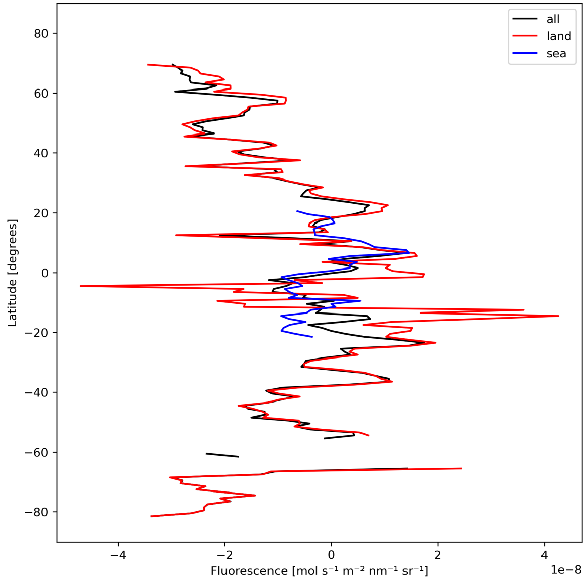
Figure 21: Zonal average of “Fluorescence” for 2024-03-04 to 2024-03-05.
