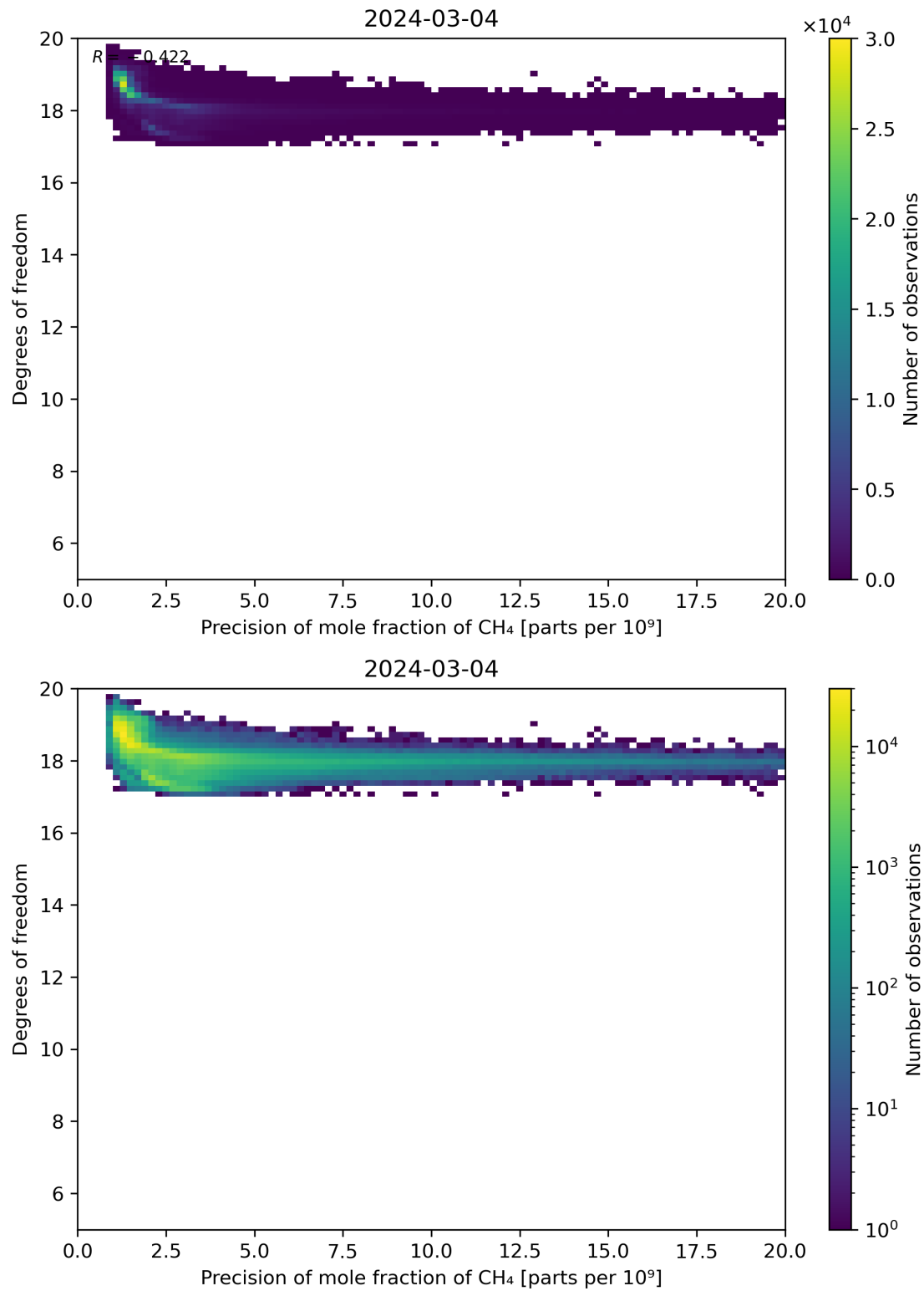
Figure 80: Scatter density plot of “Precision of mole fraction of CH 4 ” against “Degrees of freedom” for 2024-03-04 to 2024-03-05.
