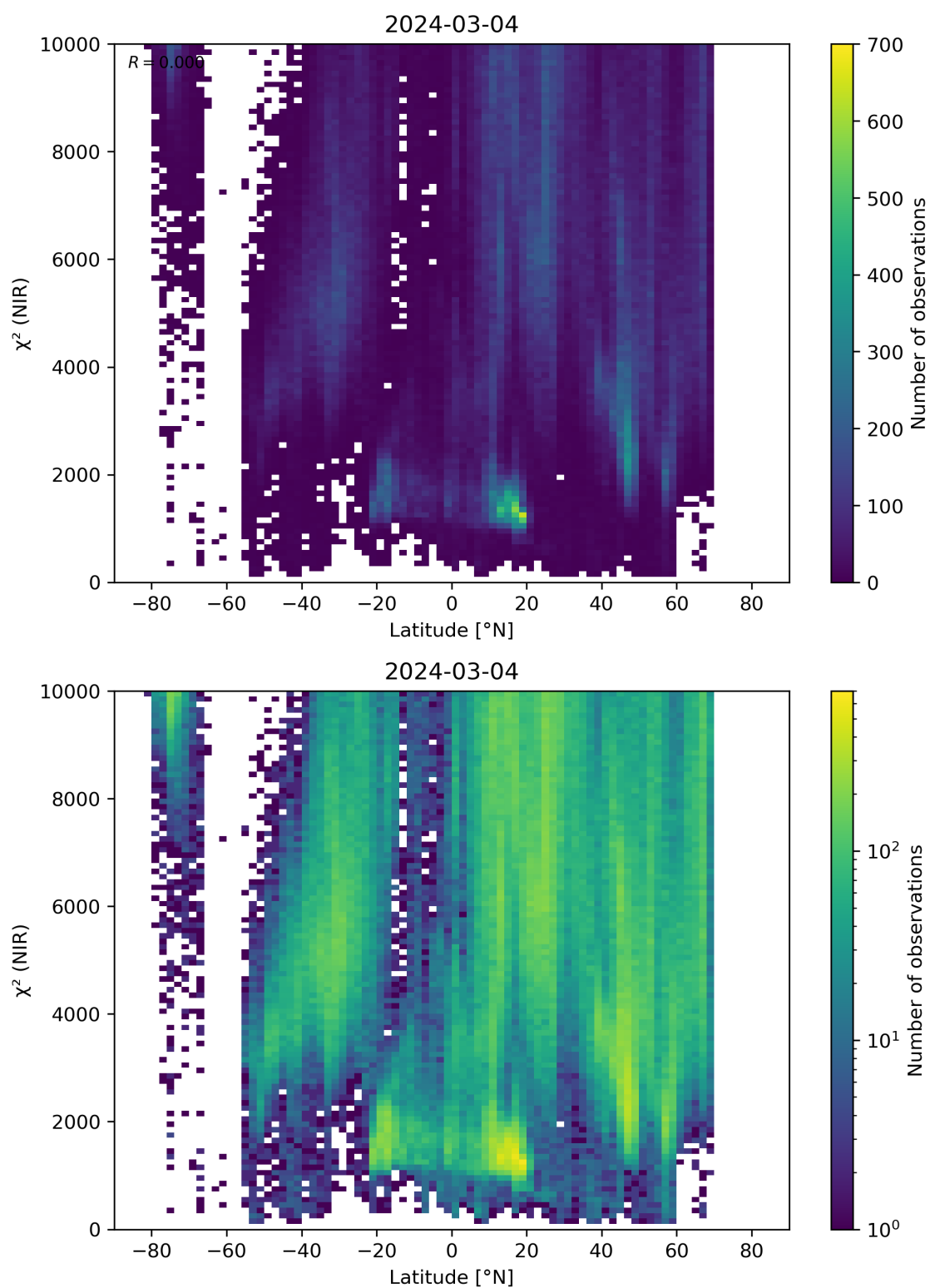
Figure 53: Scatter density plot of “Latitude” against “ \chi^2 (NIR)” for 2024-03-04 to 2024-03-05.
