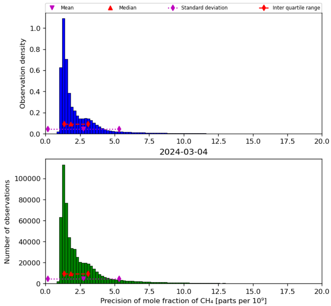
Figure 24: Histogram of “Precision of mole fraction of CH 4 ” for 2024-03-04 to 2024-03-05
