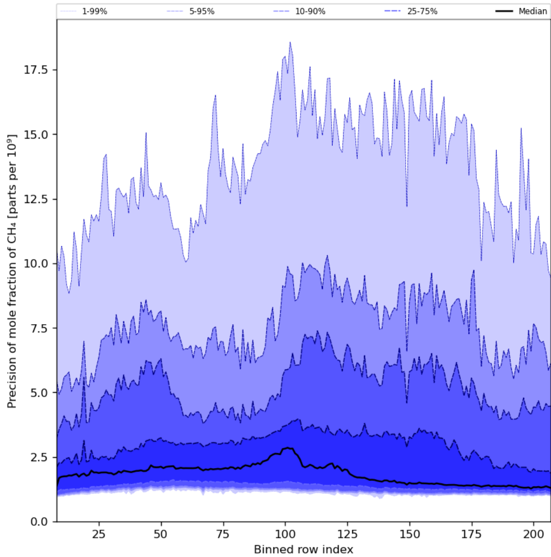
Figure 35: Along track statistics of “Precision of mole fraction of CH 4 ” for 2024-03-04 to 2024-03-05
