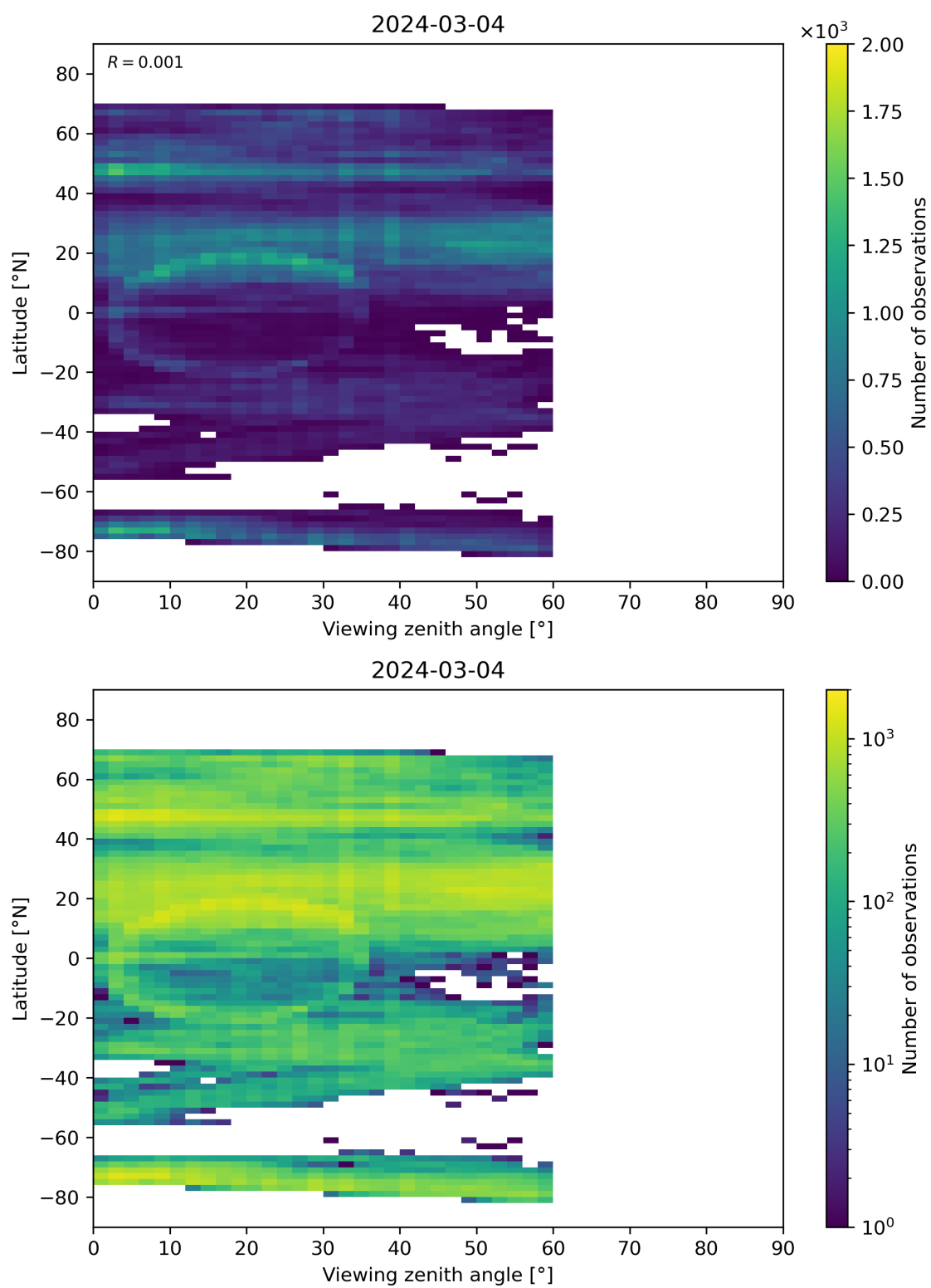
Figure 109: Scatter density plot of “Viewing zenith angle” against “Latitude” for 2024-03-04 to 2024-03-05.
