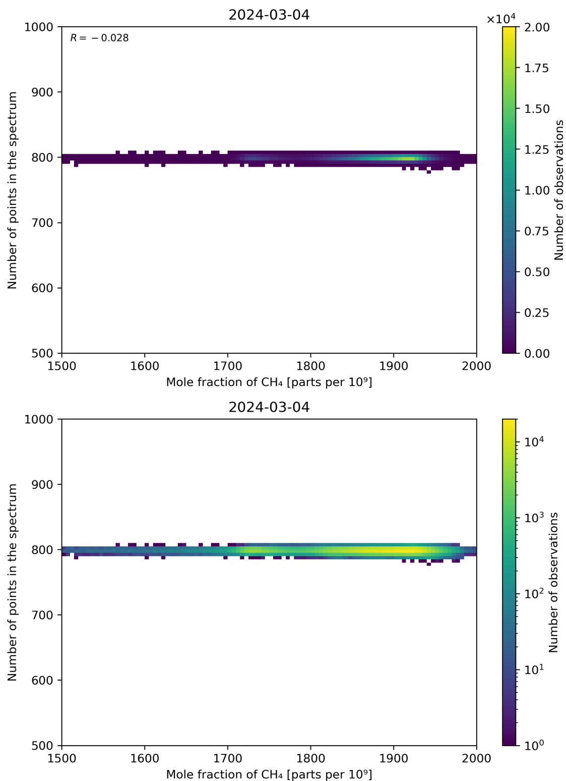
Figure 77: Scatter density plot of “Mole fraction of CH 4 ” against “Number of points in the spectrum” for 2024-03-04 to 2024-03-05.
