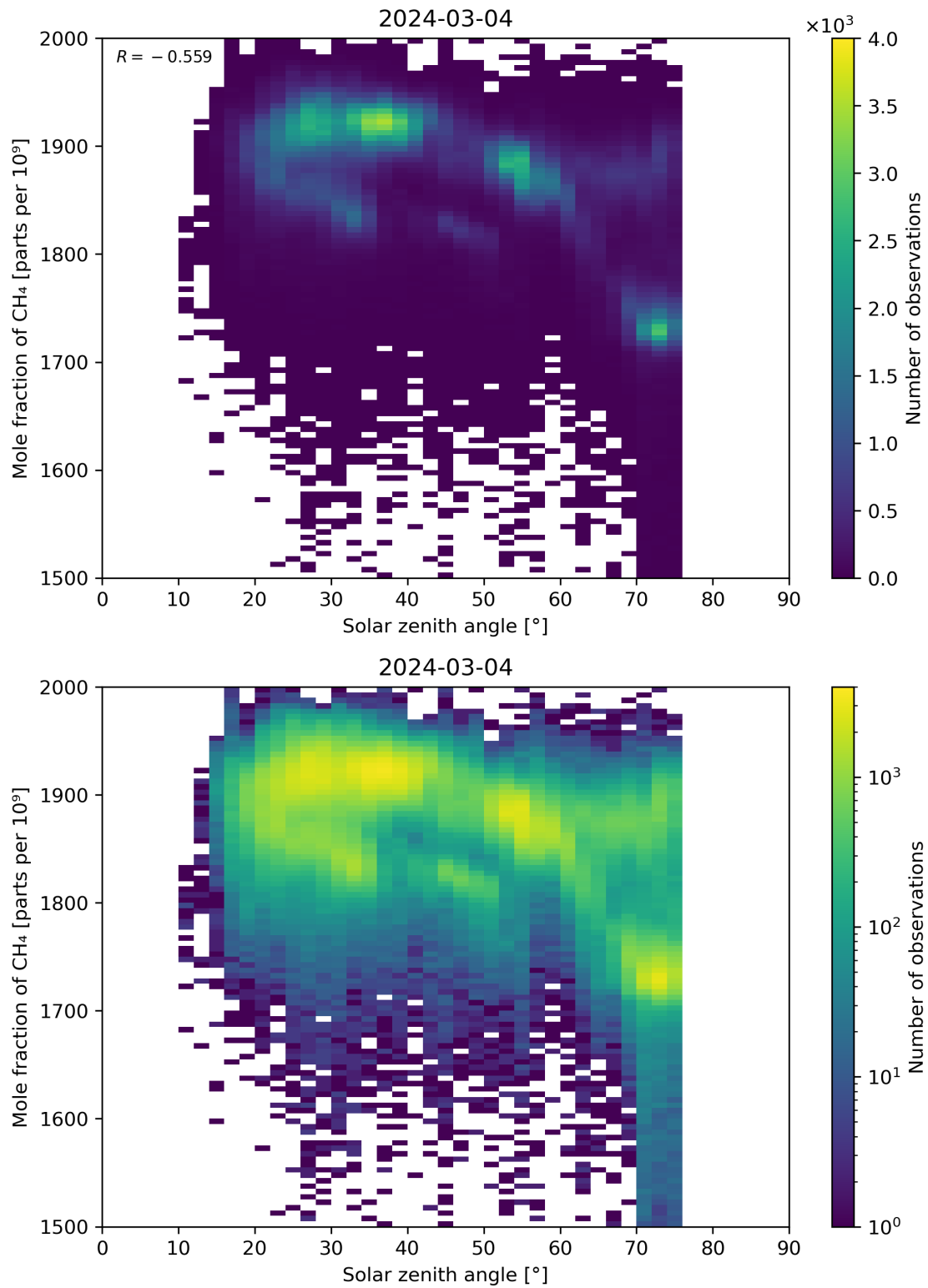
Figure 99: Scatter density plot of “Solar zenith angle” against “Mole fraction of CH 4 ” for 2024-03-04 to 2024-03-05.
