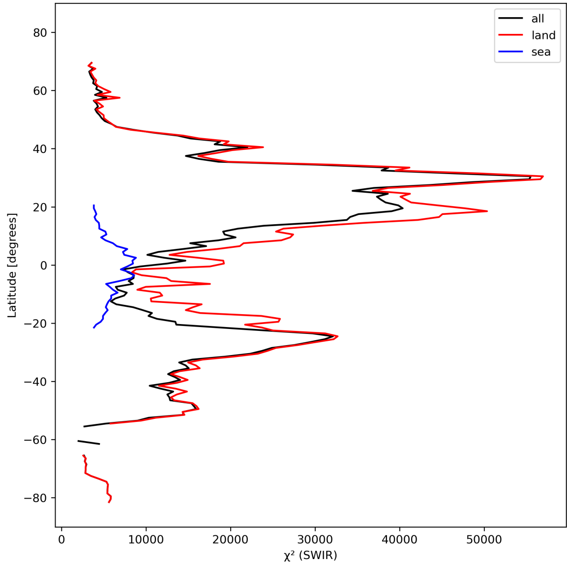
Figure 17: Zonal average of “ \chi^2 (SWIR)” for 2024-03-04 to 2024-03-05.
