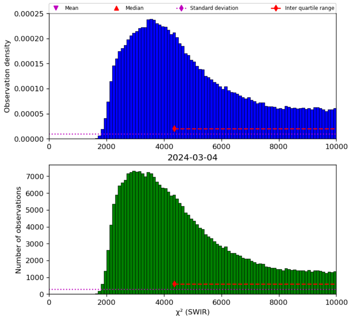
Figure 28: Histogram of “ \chi^2 (SWIR)” for 2024-03-04 to 2024-03-05
