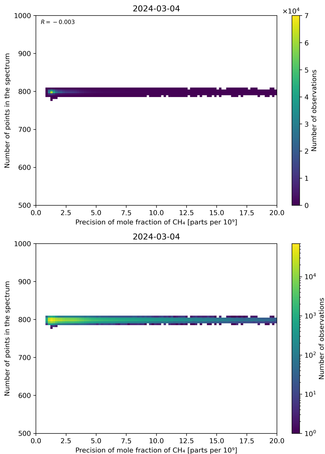
Figure 84: Scatter density plot of “Precision of mole fraction of CH 4 ” against “Number of points in the spectrum” for 2024-03-04 to 2024-03-05.
