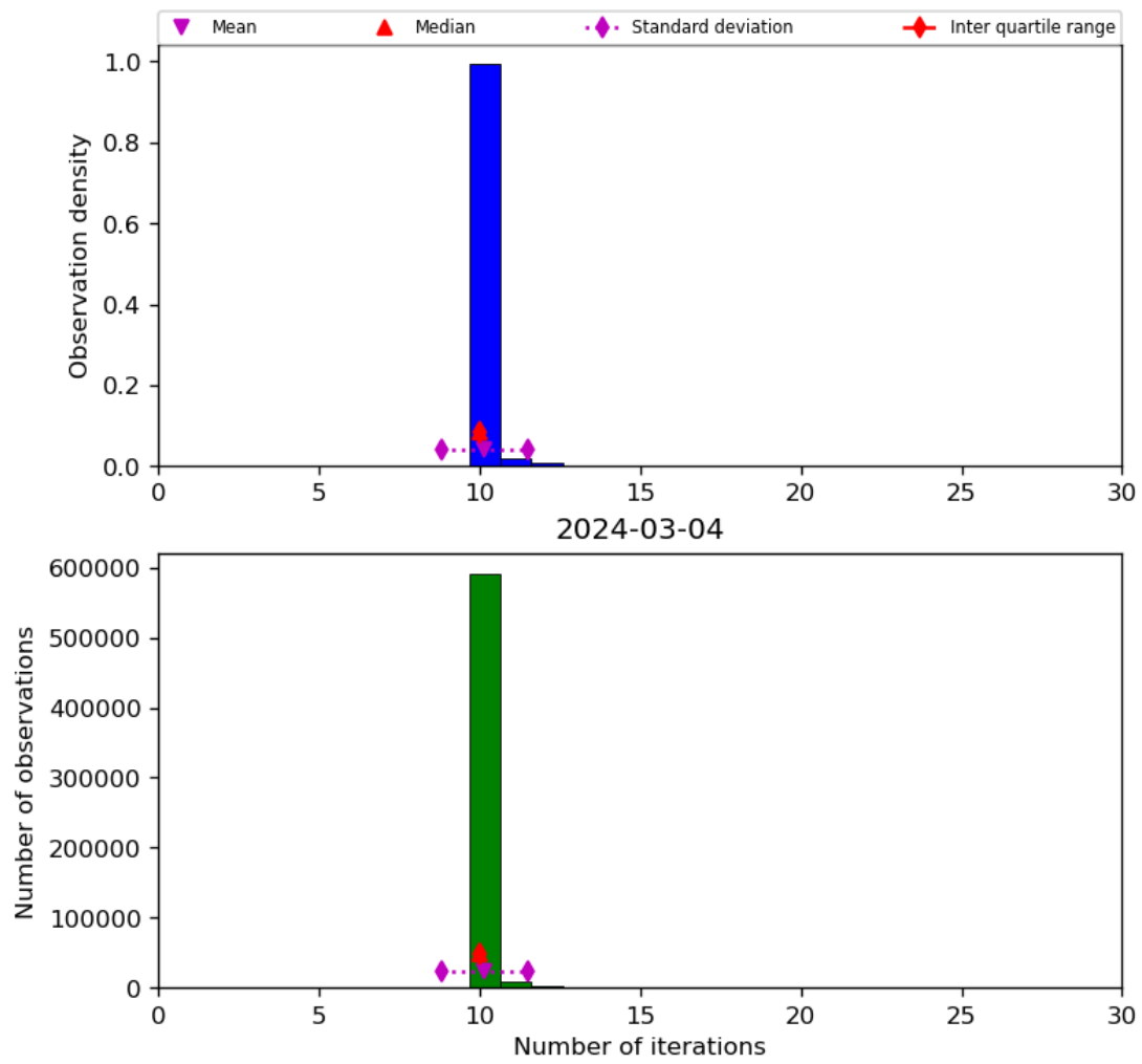
Figure 31: Histogram of “Number of iterations” for 2024-03-04 to 2024-03-05
