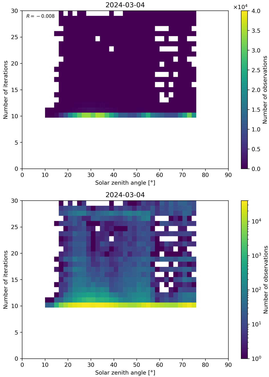
Figure 102: Scatter density plot of “Solar zenith angle” against “Number of iterations” for 2024-03-04 to 2024-03-05.
