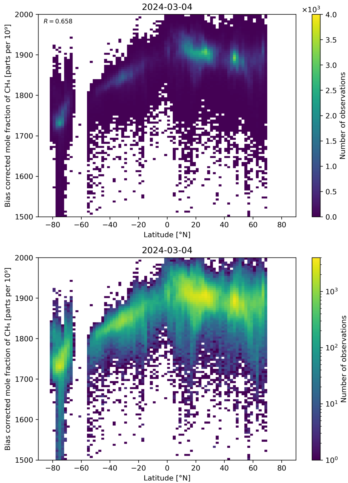
Figure 58: Scatter density plot of “Latitude” against “Bias corrected mole fraction of CH 4 ” for 2024-03-04 to 2024-03-05.
