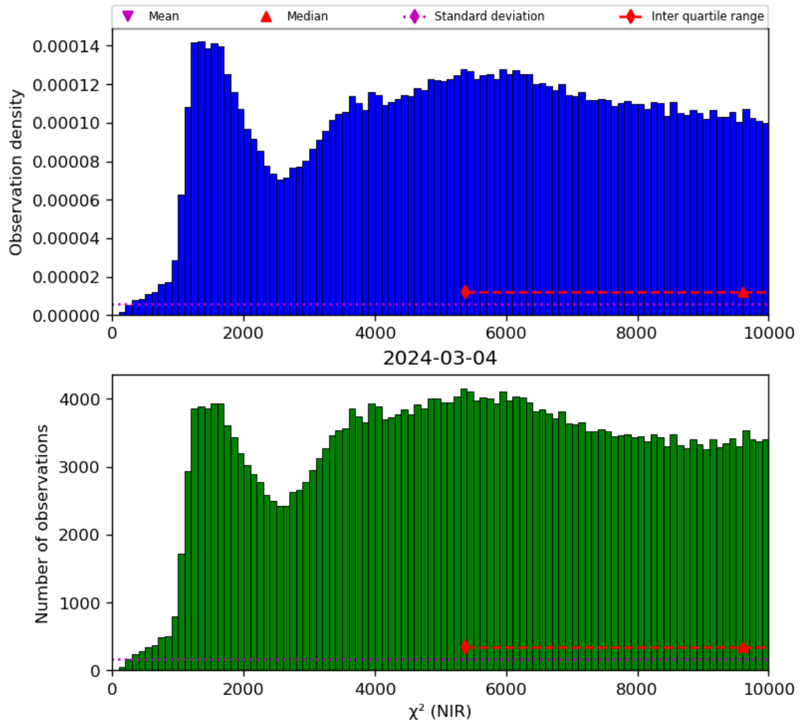
Figure 29: Histogram of “ \chi^2 (NIR)” for 2024-03-04 to 2024-03-05
