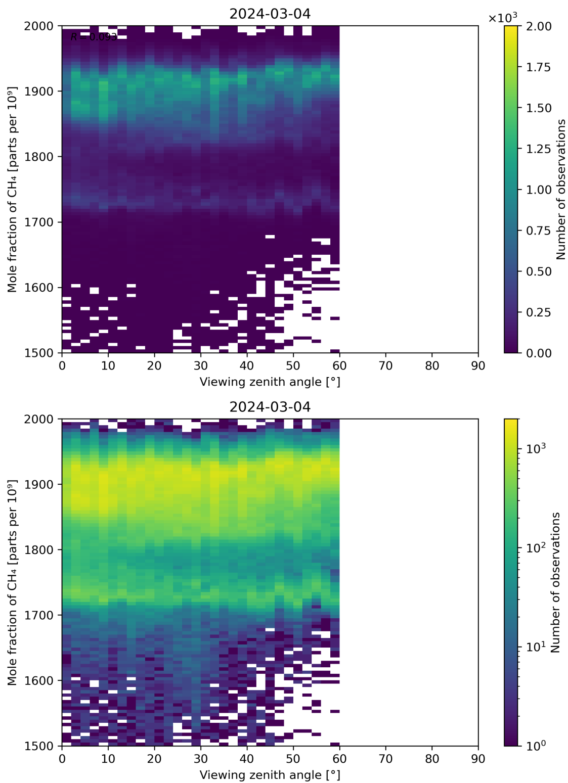
Figure 110: Scatter density plot of “Viewing zenith angle” against “Mole fraction of CH 4 ” for 2024-03-04 to 2024-03-05.
