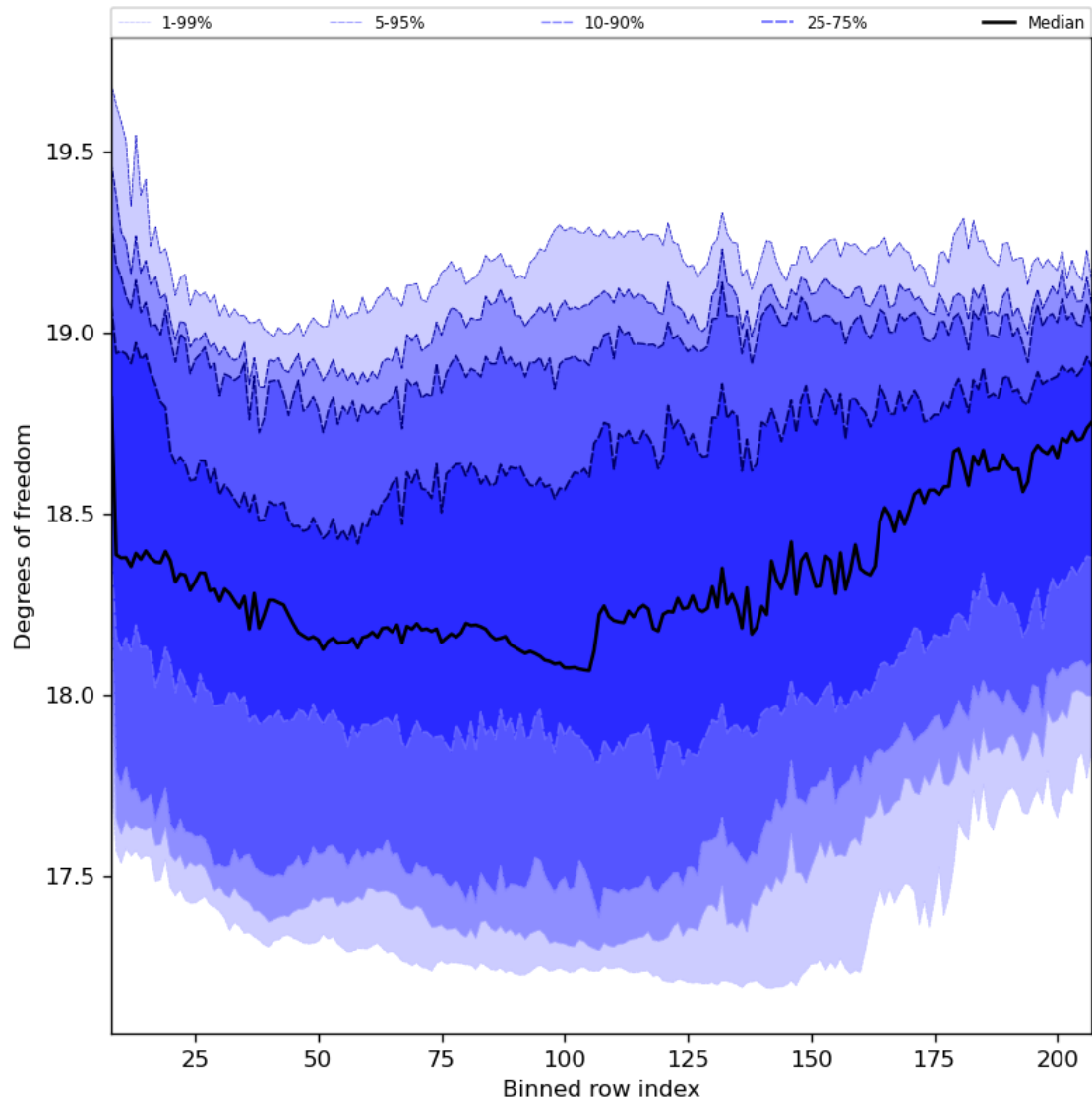
Figure 41: Along track statistics of “Degrees of freedom” for 2024-03-04 to 2024-03-05
