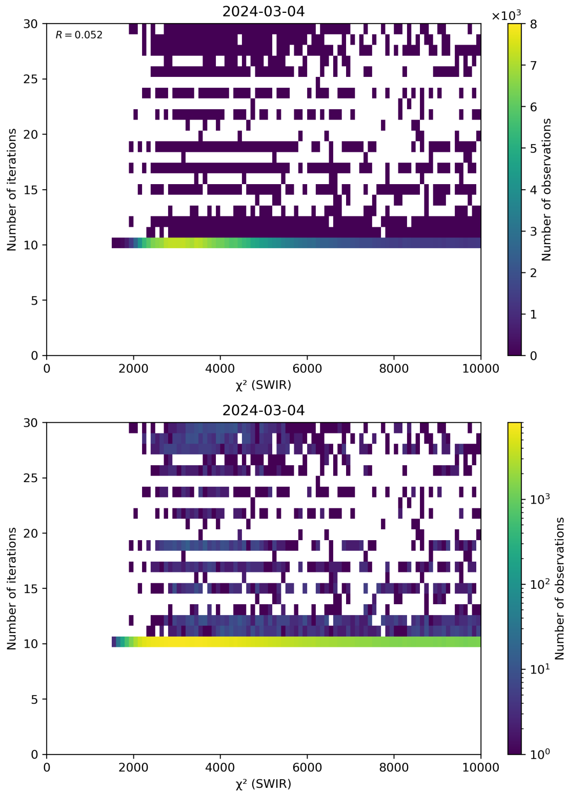
Figure 50: Scatter density plot of “ \chi^2 (SWIR)” against “Number of iterations” for 2024-03-04 to 2024-03-05.
