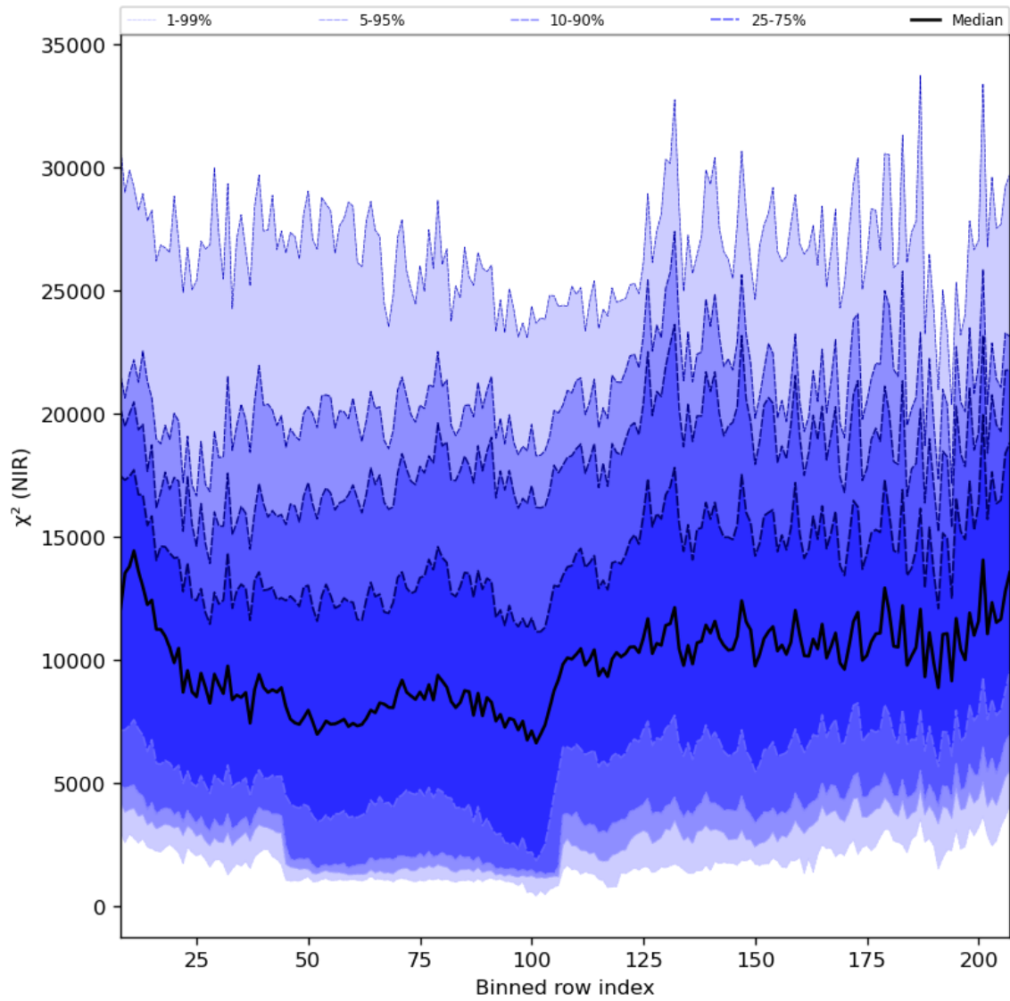
Figure 40: Along track statistics of “ \chi^2 (NIR)” for 2024-03-04 to 2024-03-05
