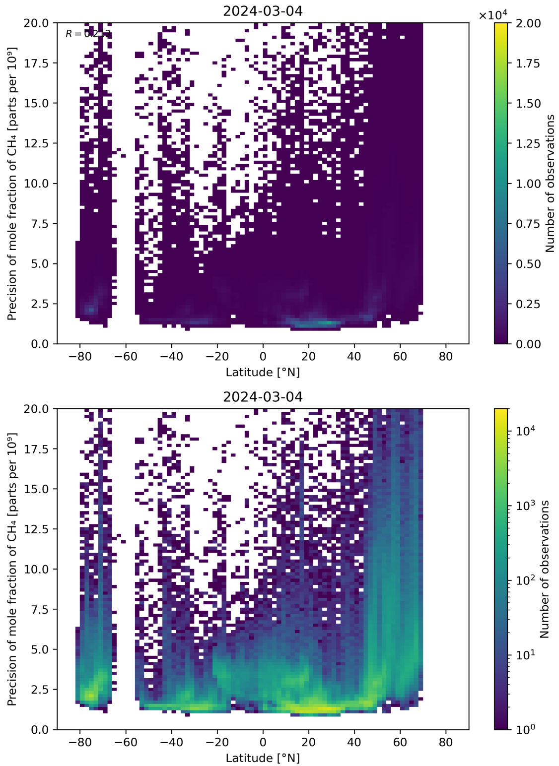
Figure 59: Scatter density plot of “Latitude” against “Precision of mole fraction of CH 4 ” for 2024-03-04 to 2024-03-05.
