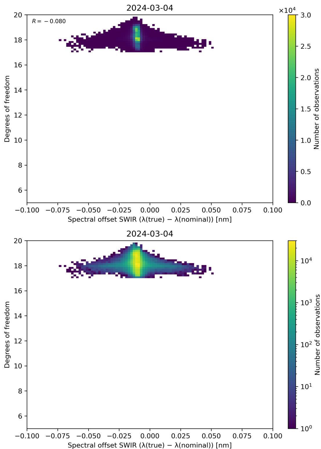
Figure 119: Scatter density plot of “Spectral offset SWIR ( \lambda(\text{true}) - \lambda(\text{nominal}) )” against “Degrees of freedom” for 2024-03-04 to 2024-03-05.
