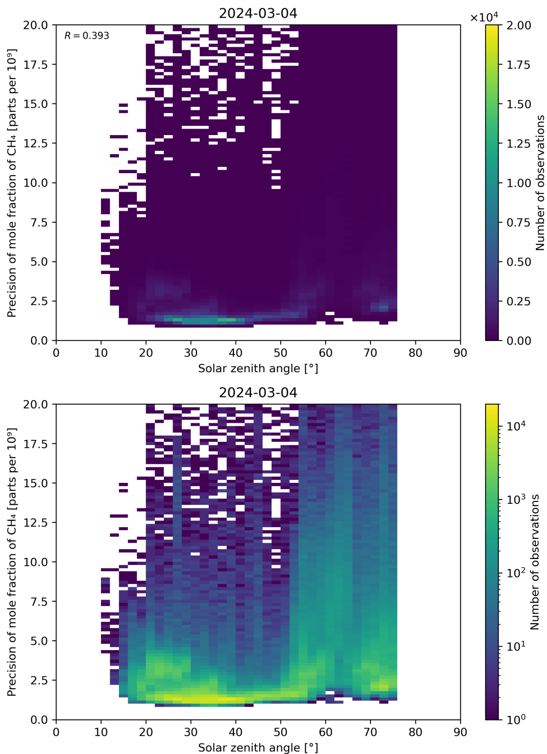
Figure 101: Scatter density plot of “Solar zenith angle” against “Precision of mole fraction of CH 4 ” for 2024-03-04 to 2024-03-05.
