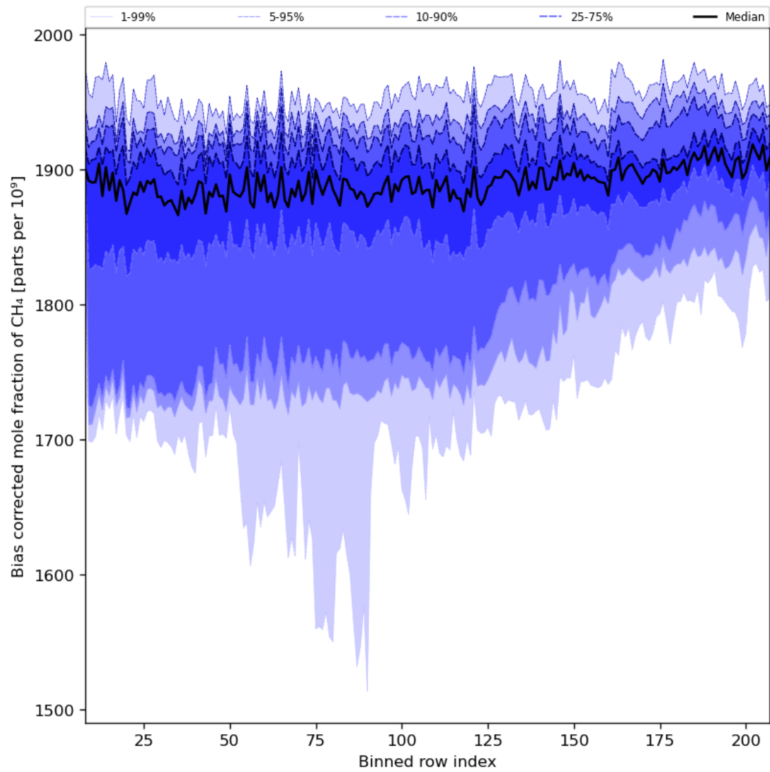
Figure 36: Along track statistics of “Bias corrected mole fraction of CH 4 ” for 2024-03-04 to 2024-03-05
