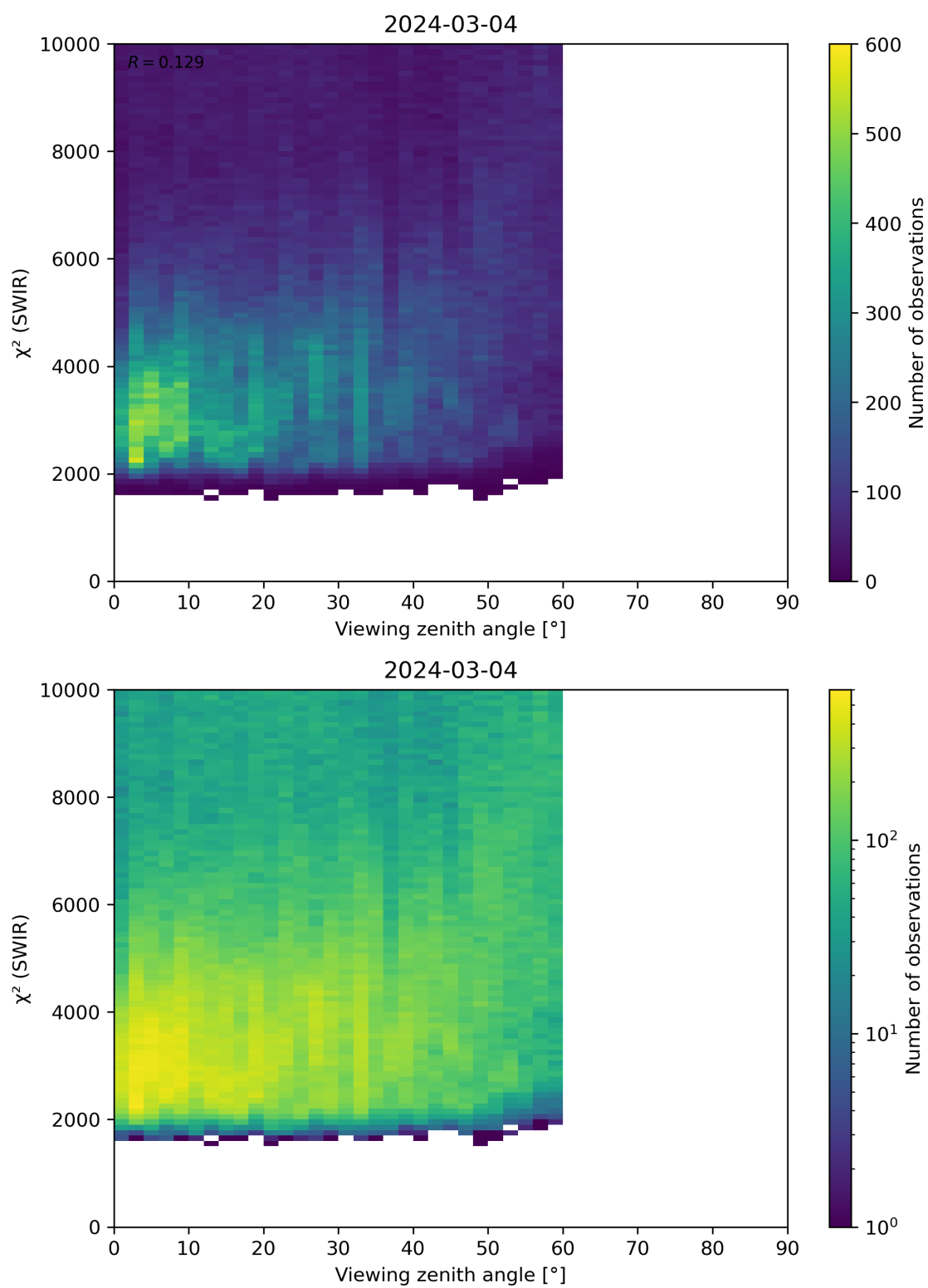
Figure 106: Scatter density plot of “Viewing zenith angle” against “ \chi^2 (SWIR)” for 2024-03-04 to 2024-03-05.
