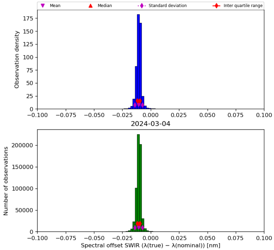
Figure 27: Histogram of “Spectral offset SWIR ( \lambda(\text{true}) - \lambda(\text{nominal}) )” for 2024-03-04 to 2024-03-05
