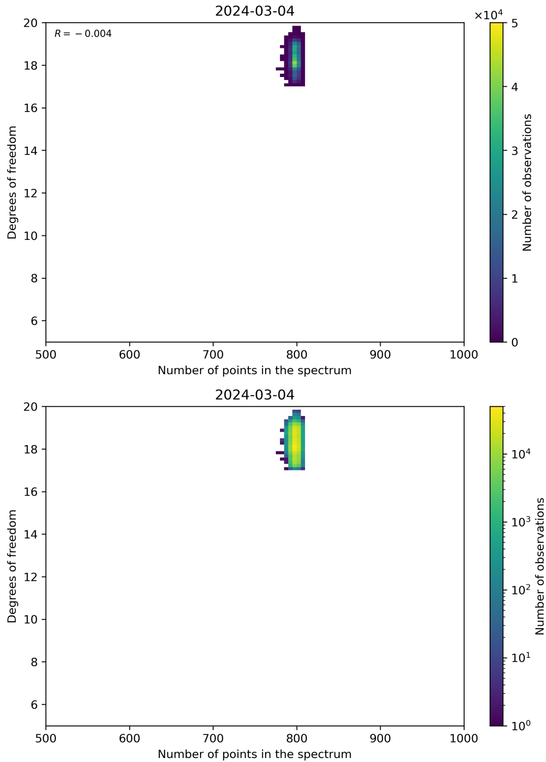
Figure 90: Scatter density plot of “Number of points in the spectrum” against “Degrees of freedom” for 2024-03-04 to 2024-03-05.
