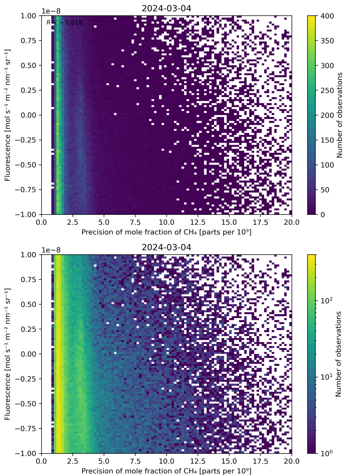
Figure 81: Scatter density plot of “Precision of mole fraction of \text{CH}_4 ” against “Fluorescence” for 2024-03-04 to 2024-03-05.
