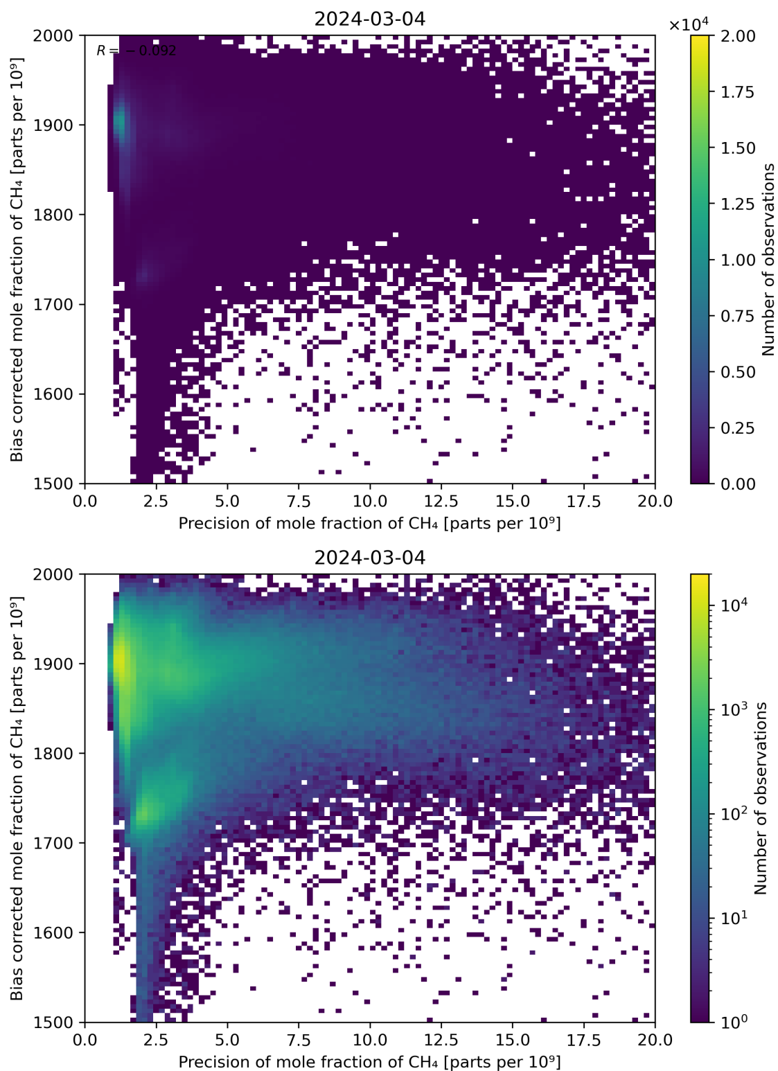
Figure 82: Scatter density plot of “Precision of mole fraction of CH 4 ” against “Bias corrected mole fraction of CH 4 ” for 2024-03-04 to 2024-03-05.
