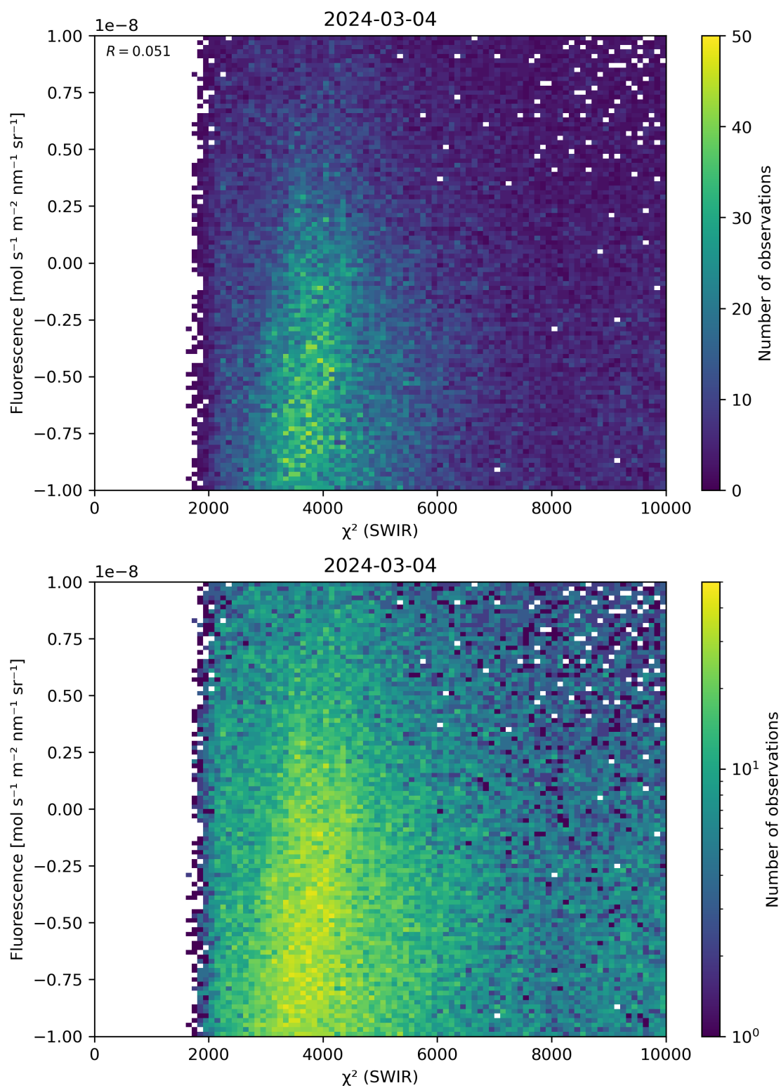
Figure 49: Scatter density plot of “ \chi^2 (SWIR)” against “Fluorescence” for 2024-03-04 to 2024-03-05.
