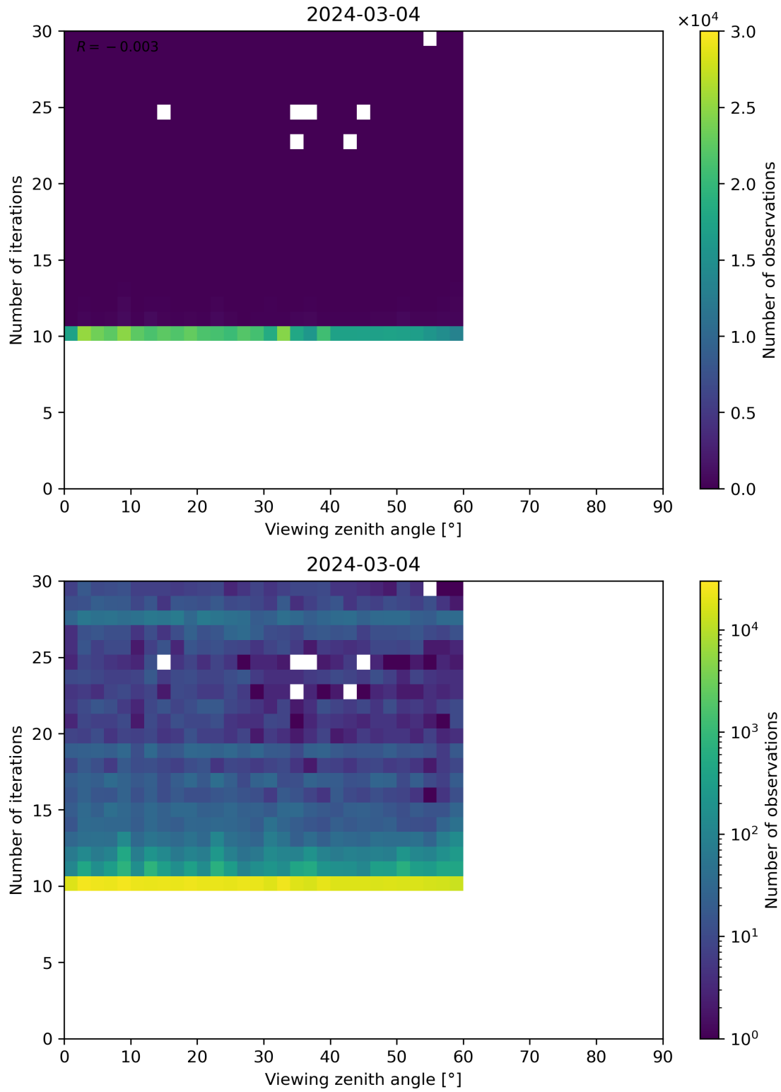
Figure 113: Scatter density plot of “Viewing zenith angle” against “Number of iterations” for 2024-03-04 to 2024-03-05.
