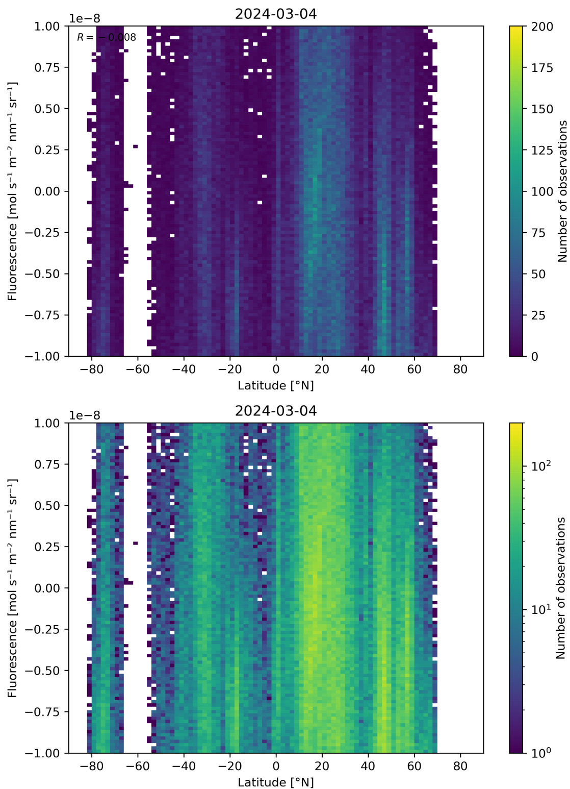
Figure 56: Scatter density plot of “Latitude” against “Fluorescence” for 2024-03-04 to 2024-03-05.
