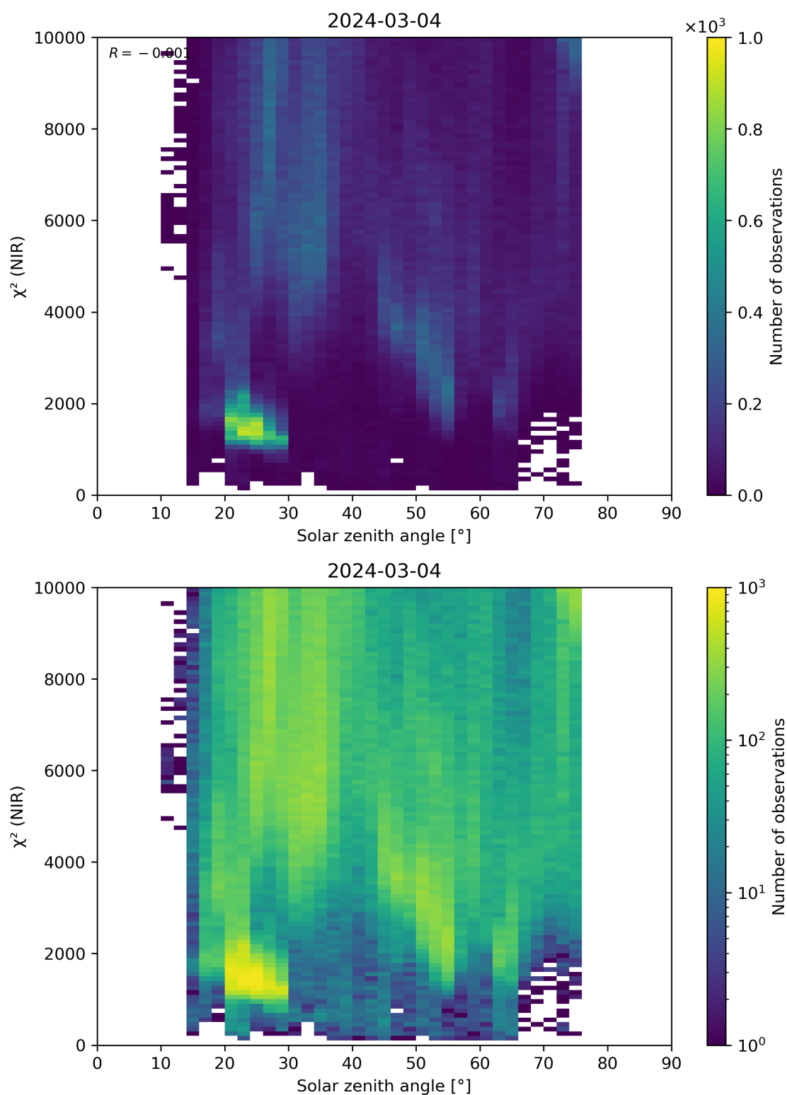
Figure 94: Scatter density plot of “Solar zenith angle” against “ \chi^2 (NIR)” for 2024-03-04 to 2024-03-05.
