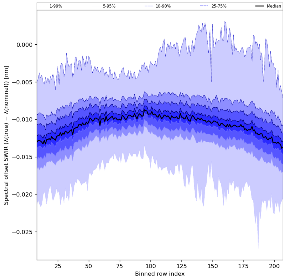
Figure 38: Along track statistics of “Spectral offset SWIR ( \lambda(\text{true}) - \lambda(\text{nominal}) )” for 2024-03-04 to 2024-03-05
