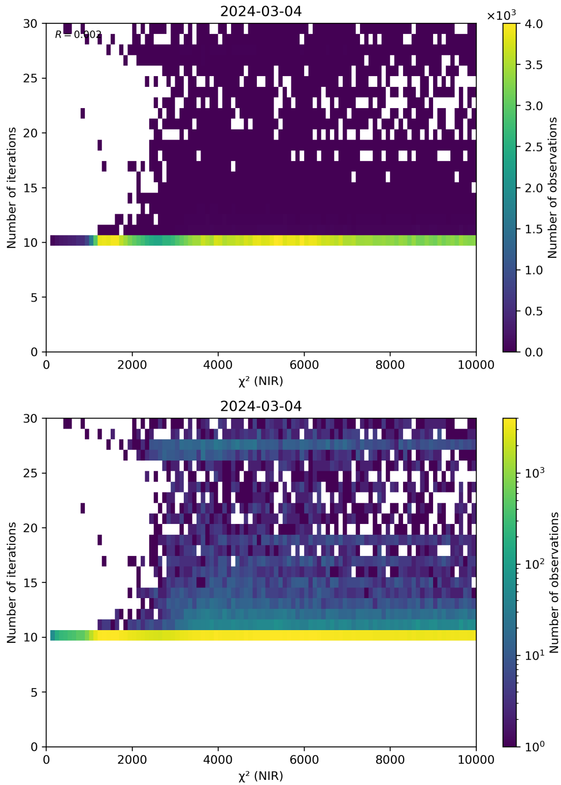
Figure 46: Scatter density plot of “ \chi^2 (NIR)” against “Number of iterations” for 2024-03-04 to 2024-03-05.
