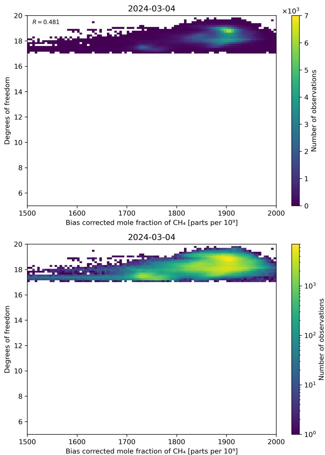
Figure 65: Scatter density plot of “Bias corrected mole fraction of CH 4 ” against “Degrees of freedom” for 2024-03-04 to 2024-03-05.
