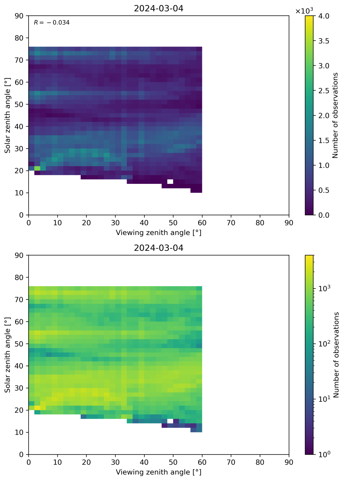
Figure 115: Scatter density plot of “Viewing zenith angle” against “Solar zenith angle” for 2024-03-04 to 2024-03-05.
