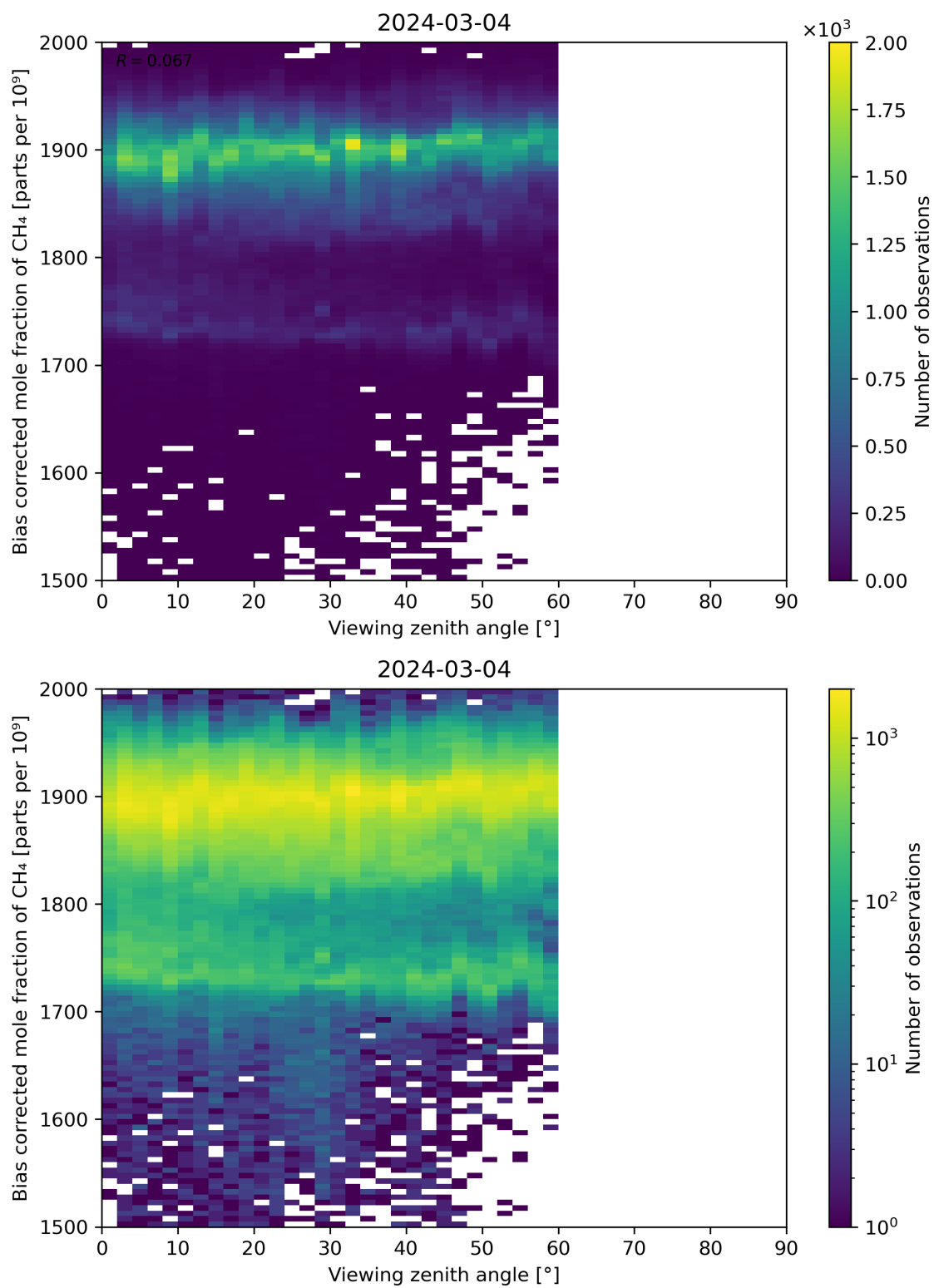
Figure 111: Scatter density plot of “Viewing zenith angle” against “Bias corrected mole fraction of CH 4 ” for 2024-03-04 to 2024-03-05.
