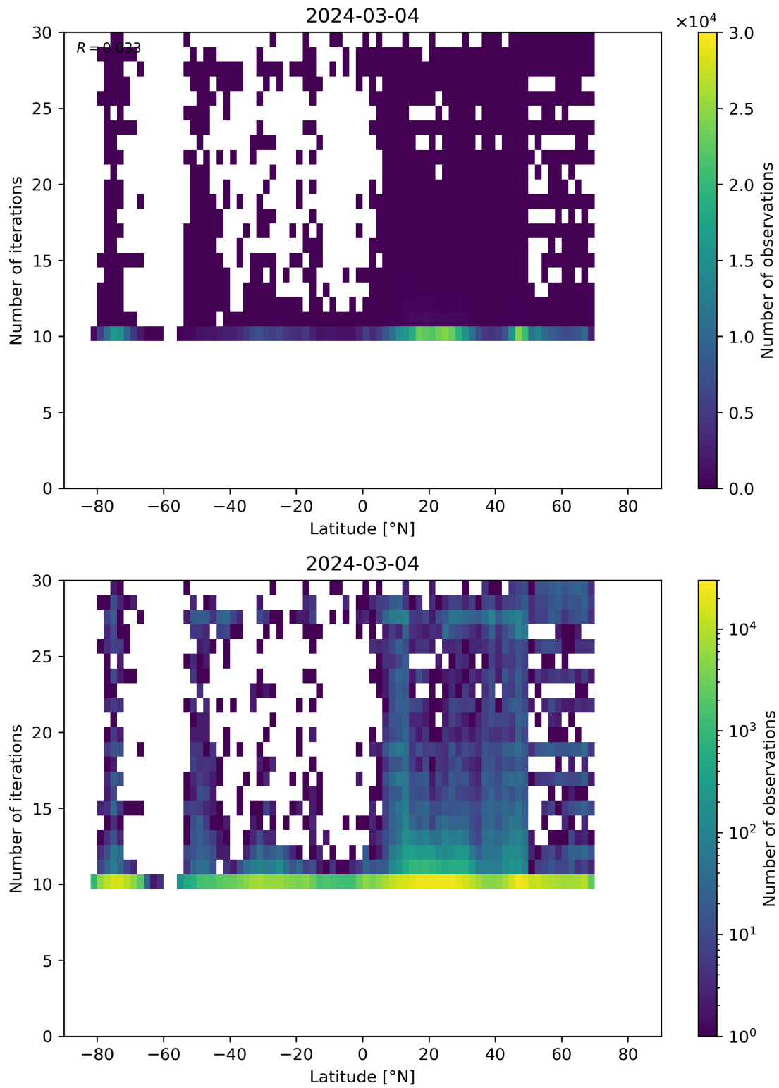
Figure 60: Scatter density plot of “Latitude” against “Number of iterations” for 2024-03-04 to 2024-03-05.
