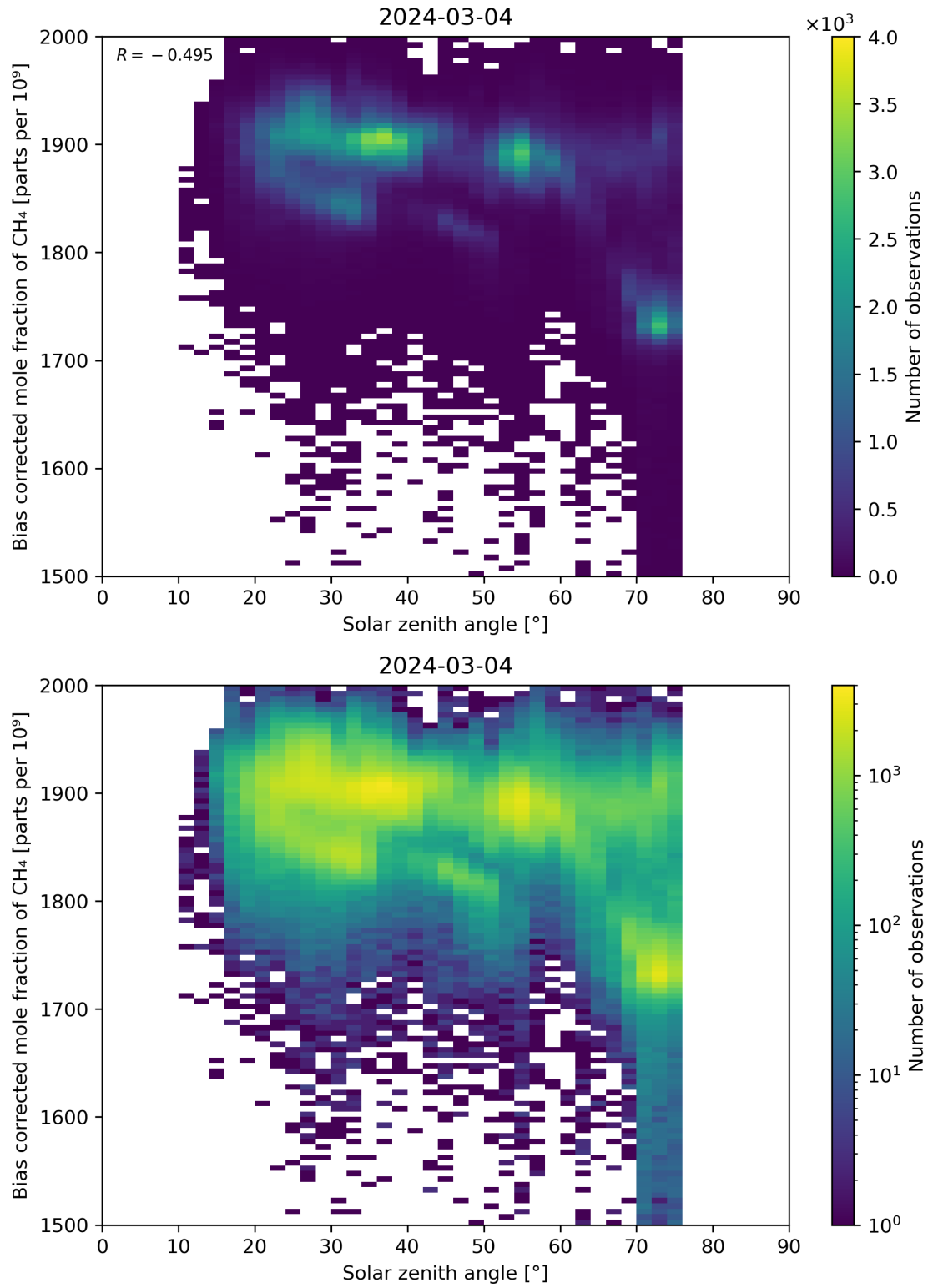
Figure 100: Scatter density plot of “Solar zenith angle” against “Bias corrected mole fraction of \text{CH}_4 ” for 2024-03-04 to 2024-03-05.
