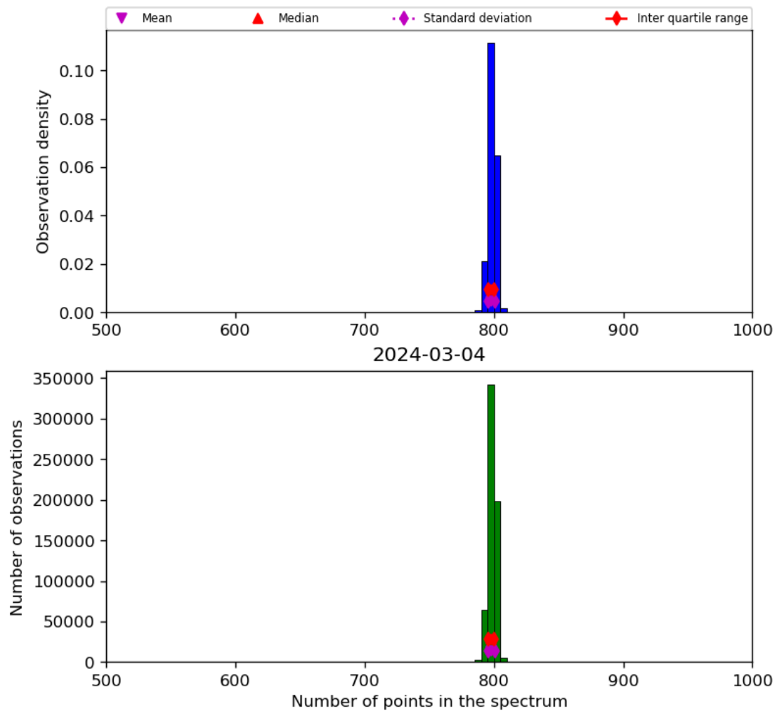
Figure 26: Histogram of “Number of points in the spectrum” for 2024-03-04 to 2024-03-05
