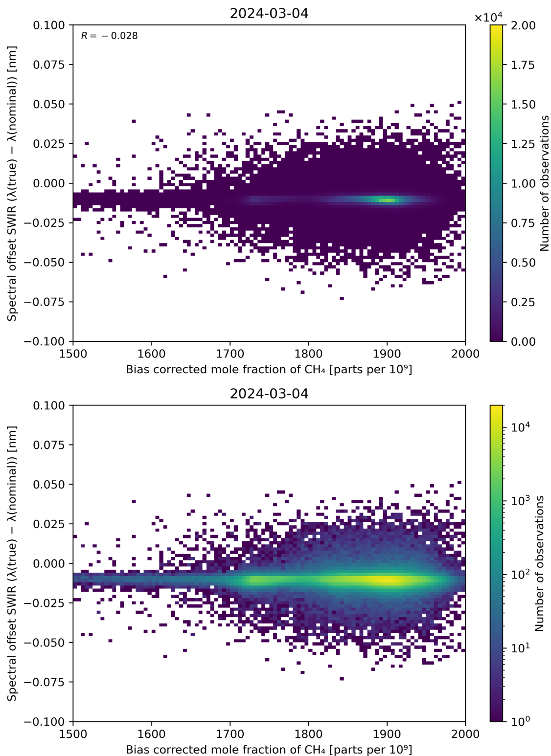
Figure 69: Scatter density plot of “Bias corrected mole fraction of \text{CH}_4 ” against “Spectral offset SWIR ( \lambda(\text{true}) - \lambda(\text{nominal}) )” for 2024-03-04 to 2024-03-05.
