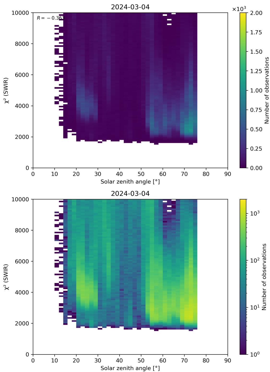
Figure 95: Scatter density plot of “Solar zenith angle” against “ \chi^2 (SWIR)” for 2024-03-04 to 2024-03-05.
