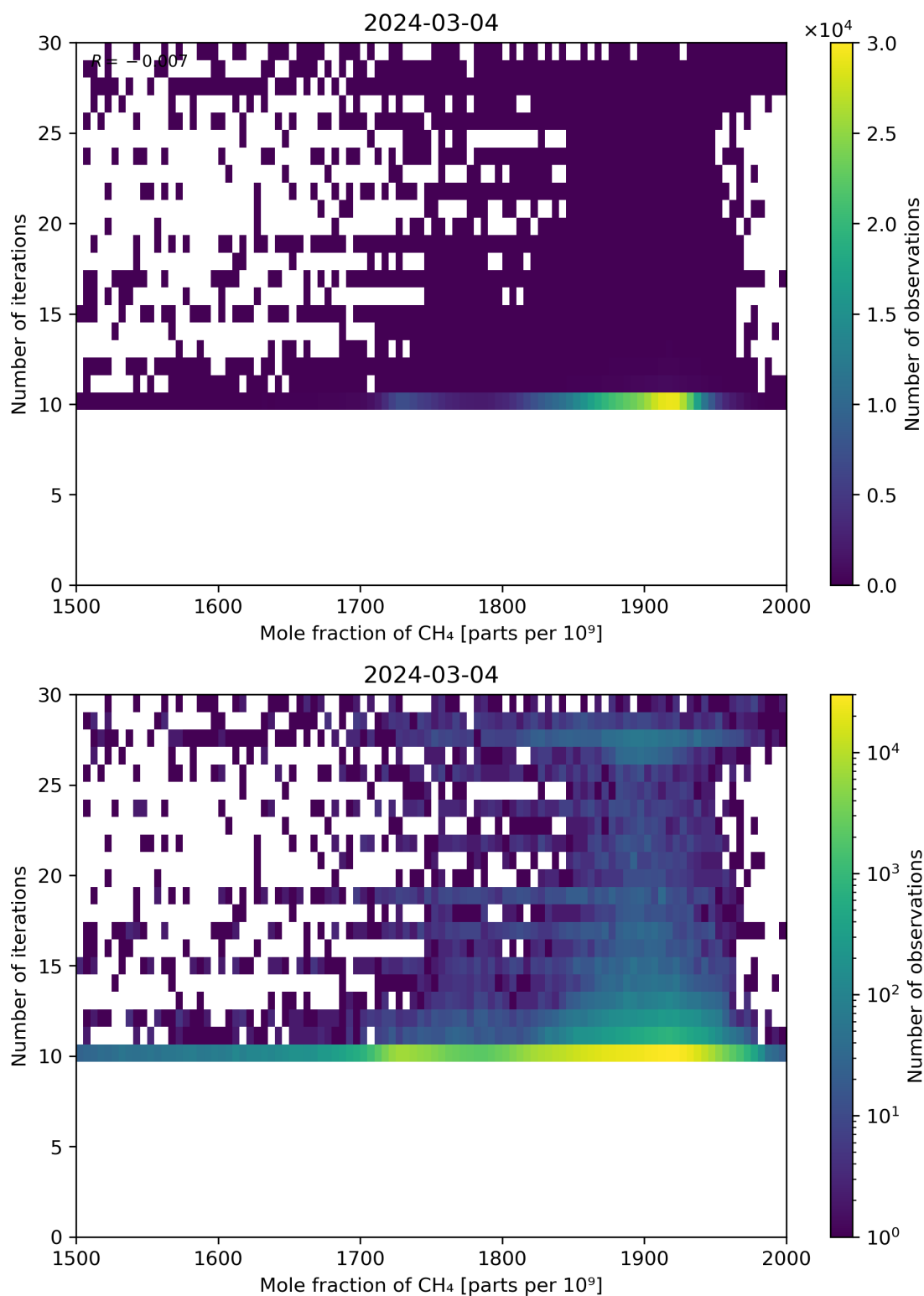
Figure 76: Scatter density plot of “Mole fraction of CH 4 ” against “Number of iterations” for 2024-03-04 to 2024-03-05.
