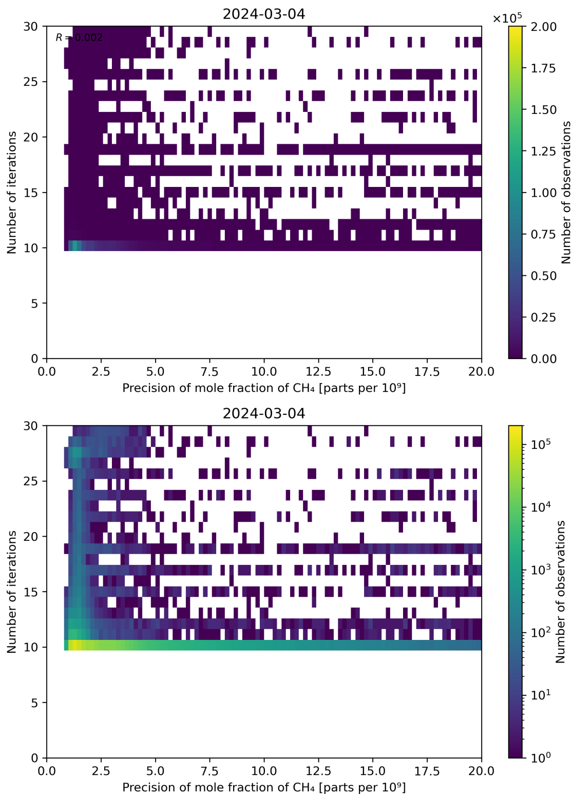
Figure 83: Scatter density plot of “Precision of mole fraction of CH 4 ” against “Number of iterations” for 2024-03-04 to 2024-03-05.
