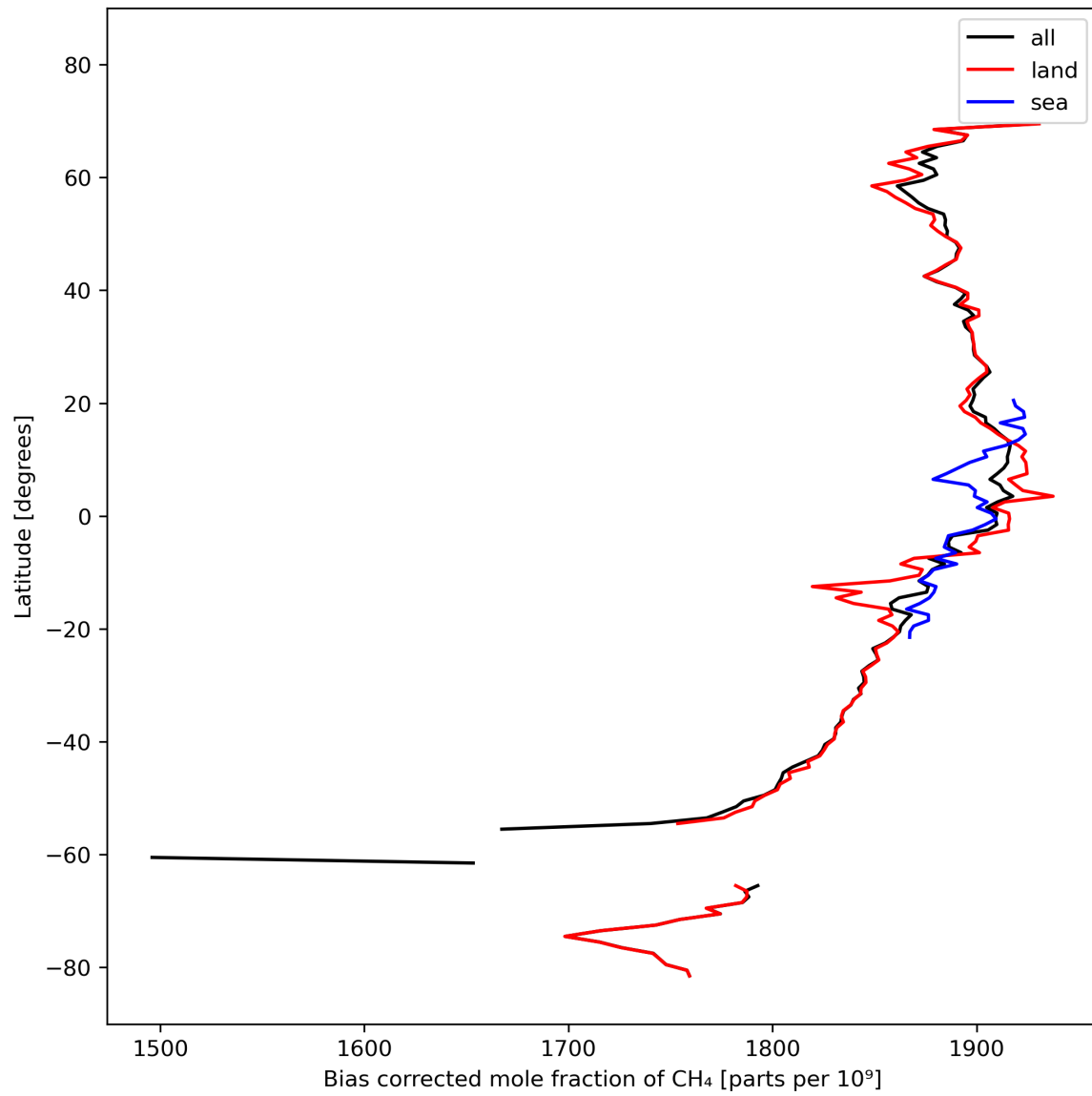
Figure 14: Zonal average of “Bias corrected mole fraction of CH 4 ” for 2024-03-04 to 2024-03-05.
