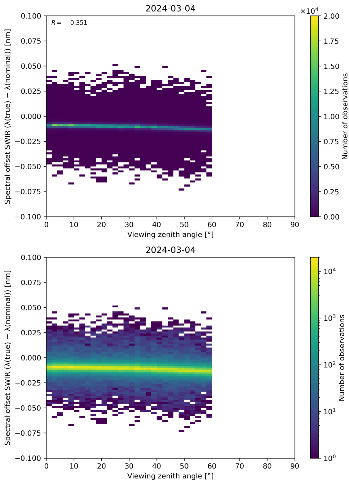
Figure 116: Scatter density plot of “Viewing zenith angle” against “Spectral offset SWIR ( \lambda(\text{true}) - \lambda(\text{nominal}) )” for 2024-03-04 to 2024-03-05.
