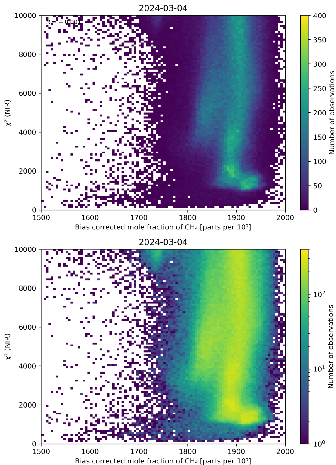
Figure 63: Scatter density plot of “Bias corrected mole fraction of CH 4 ” against “ \chi^2 (NIR)” for 2024-03-04 to 2024-03-05.
