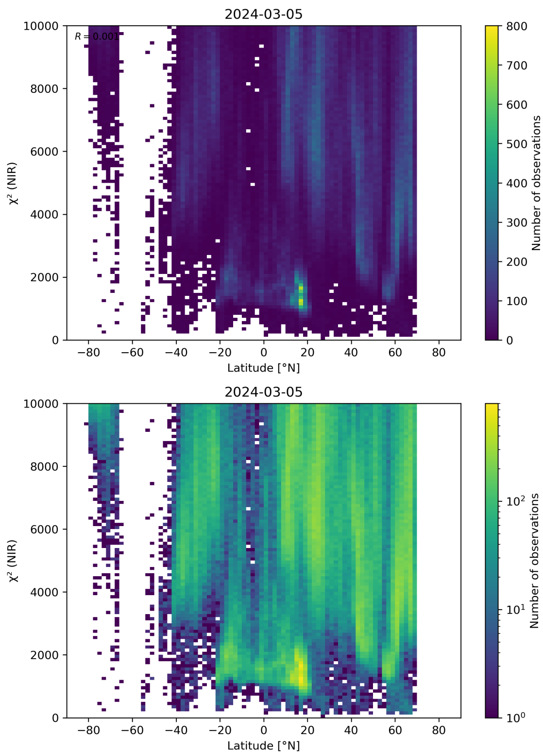
Figure 53: Scatter density plot of “Latitude” against “ \chi^2 (NIR)” for 2024-03-04 to 2024-03-06.
