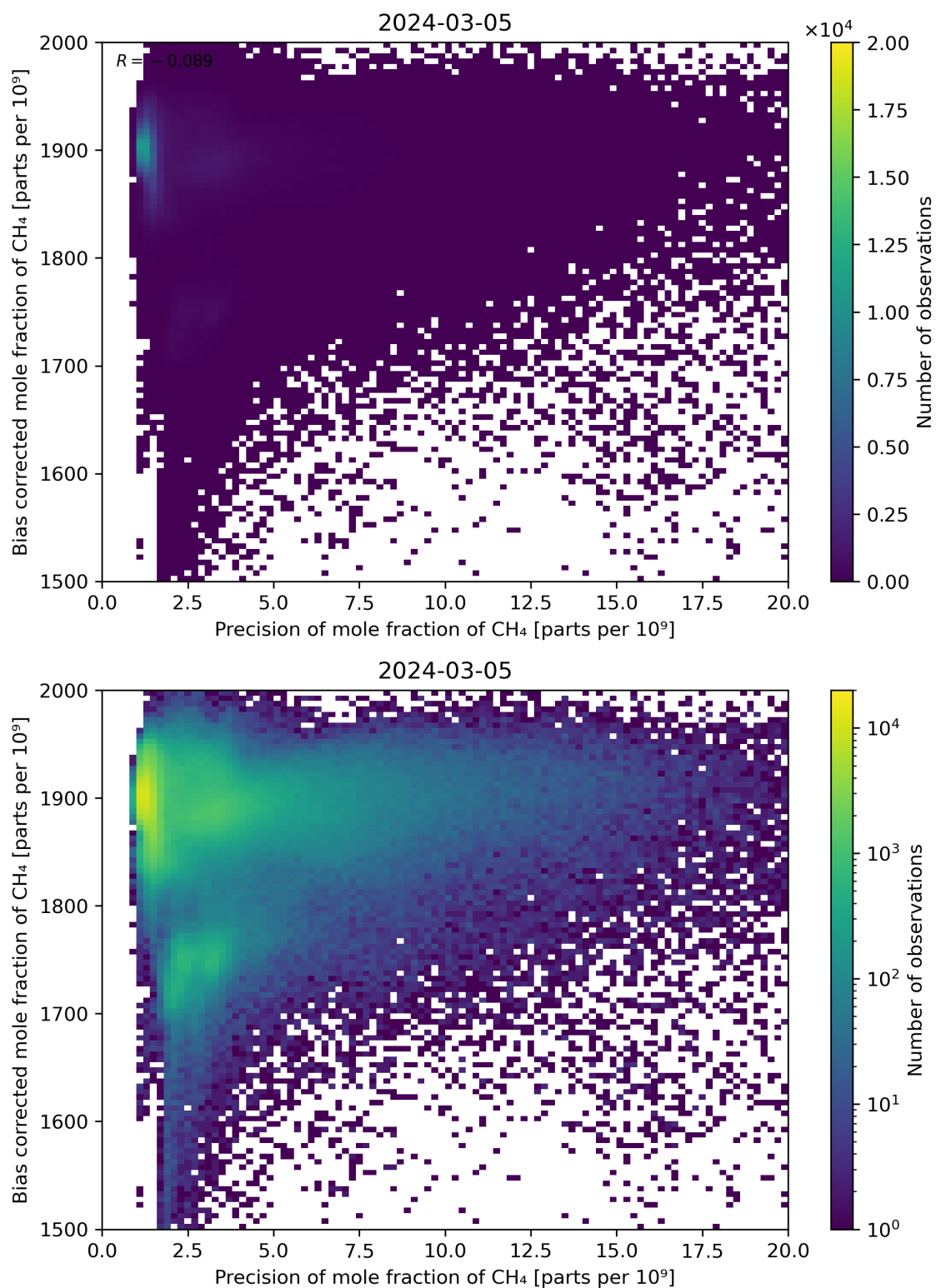
Figure 82: Scatter density plot of “Precision of mole fraction of CH 4 ” against “Bias corrected mole fraction of CH 4 ” for 2024-03-04 to 2024-03-06.
