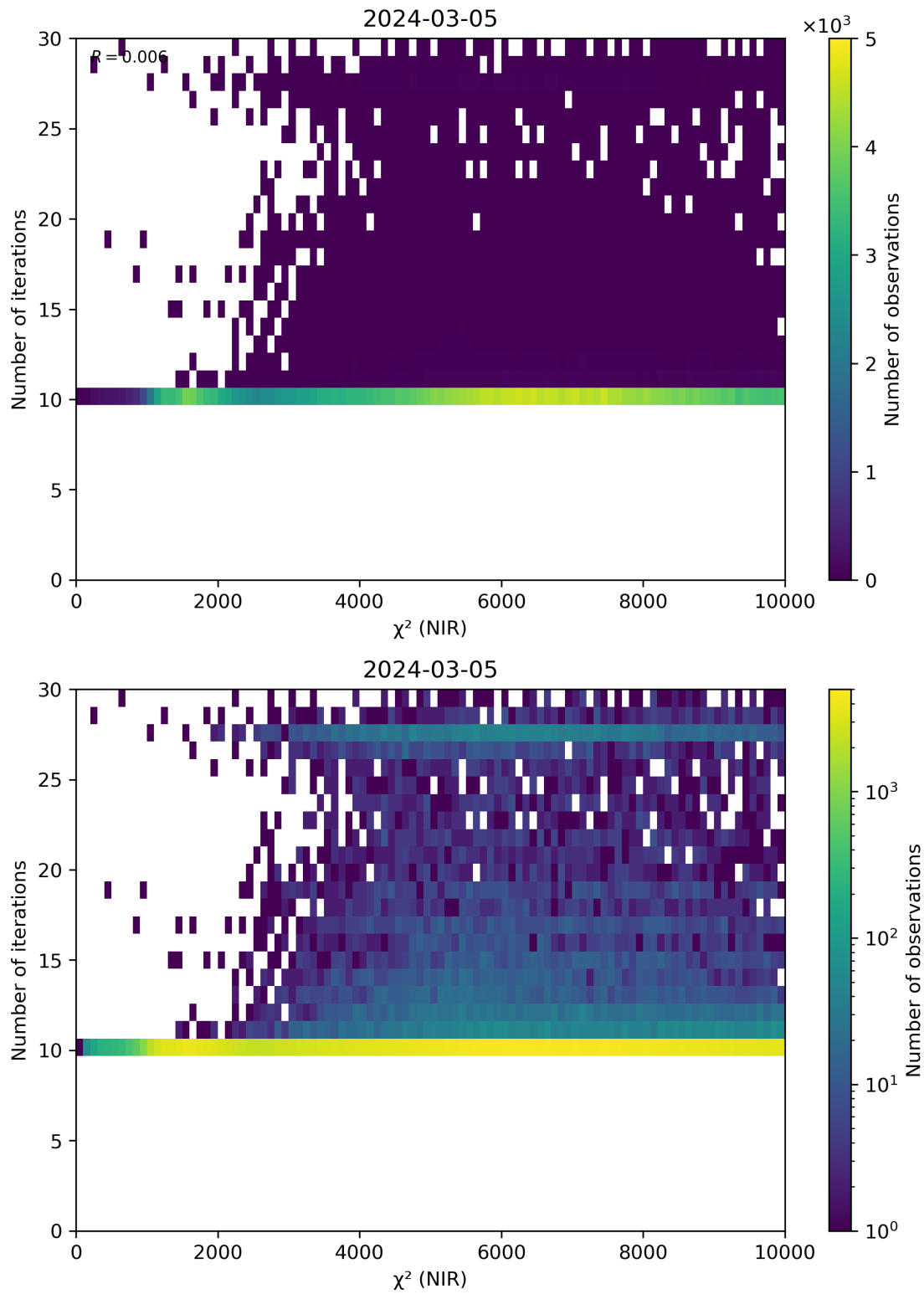
Figure 46: Scatter density plot of “ \chi^2 (NIR)” against “Number of iterations” for 2024-03-04 to 2024-03-06.
