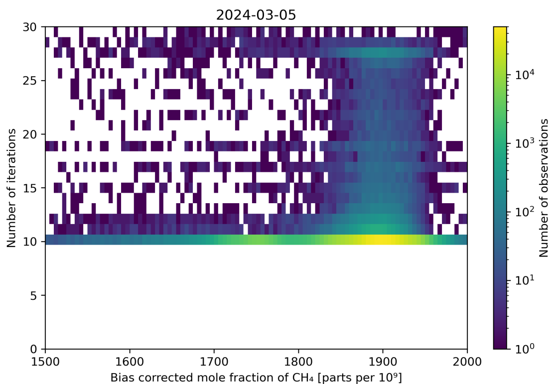
Figure 67: Scatter density plot of “Bias corrected mole fraction of CH 4 ” against “Number of iterations” for 2024-03-04 to 2024-03-06.
