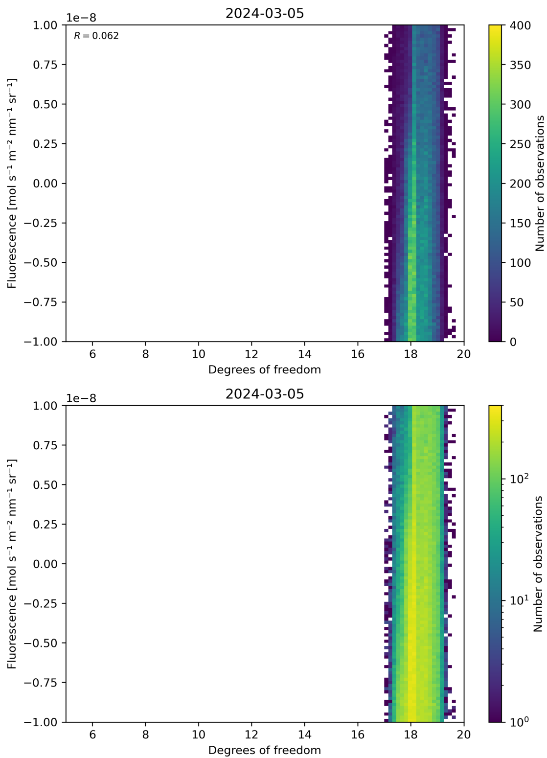
Figure 51: Scatter density plot of “Degrees of freedom” against “Fluorescence” for 2024-03-04 to 2024-03-06.
