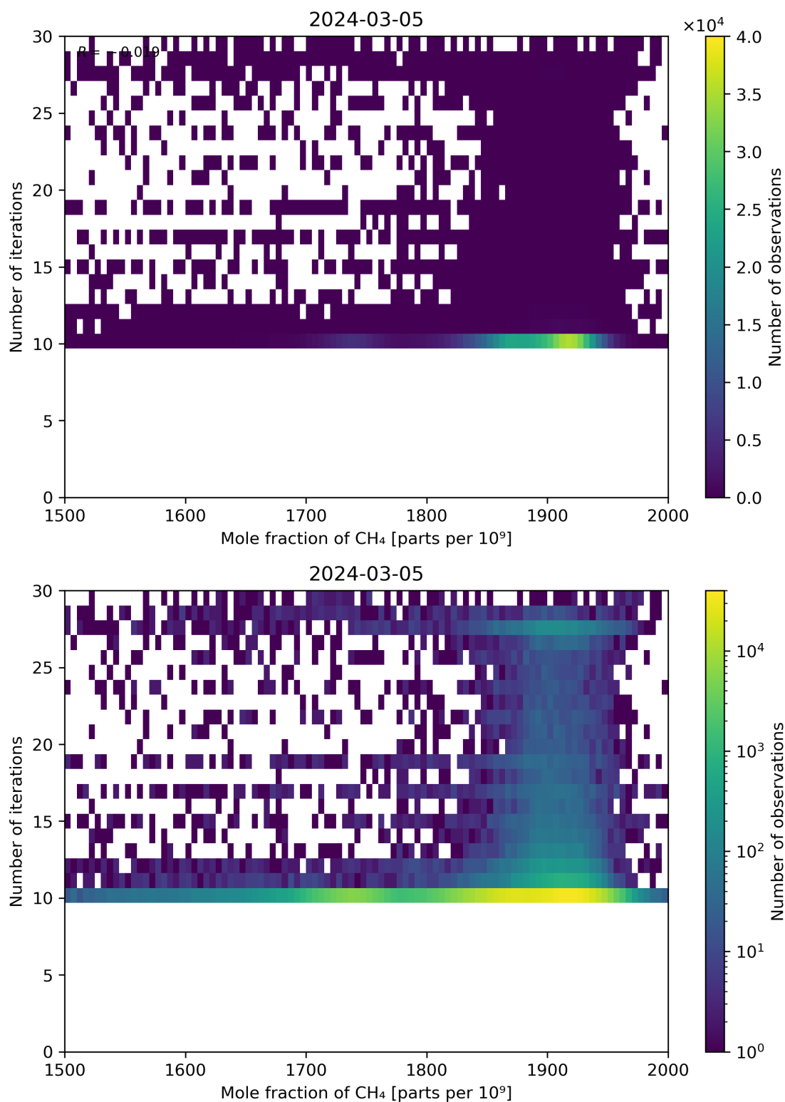
Figure 76: Scatter density plot of “Mole fraction of CH 4 ” against “Number of iterations” for 2024-03-04 to 2024-03-06.
