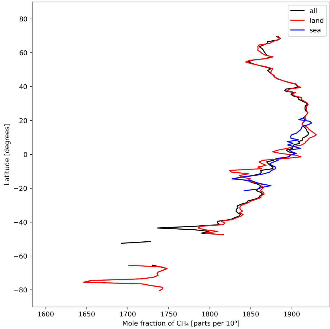
Figure 12: Zonal average of “Mole fraction of \text{CH}_4 ” for 2024-03-04 to 2024-03-06.
