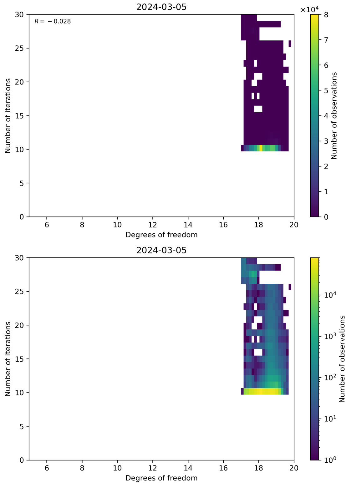
Figure 52: Scatter density plot of “Degrees of freedom” against “Number of iterations” for 2024-03-04 to 2024-03-06.
