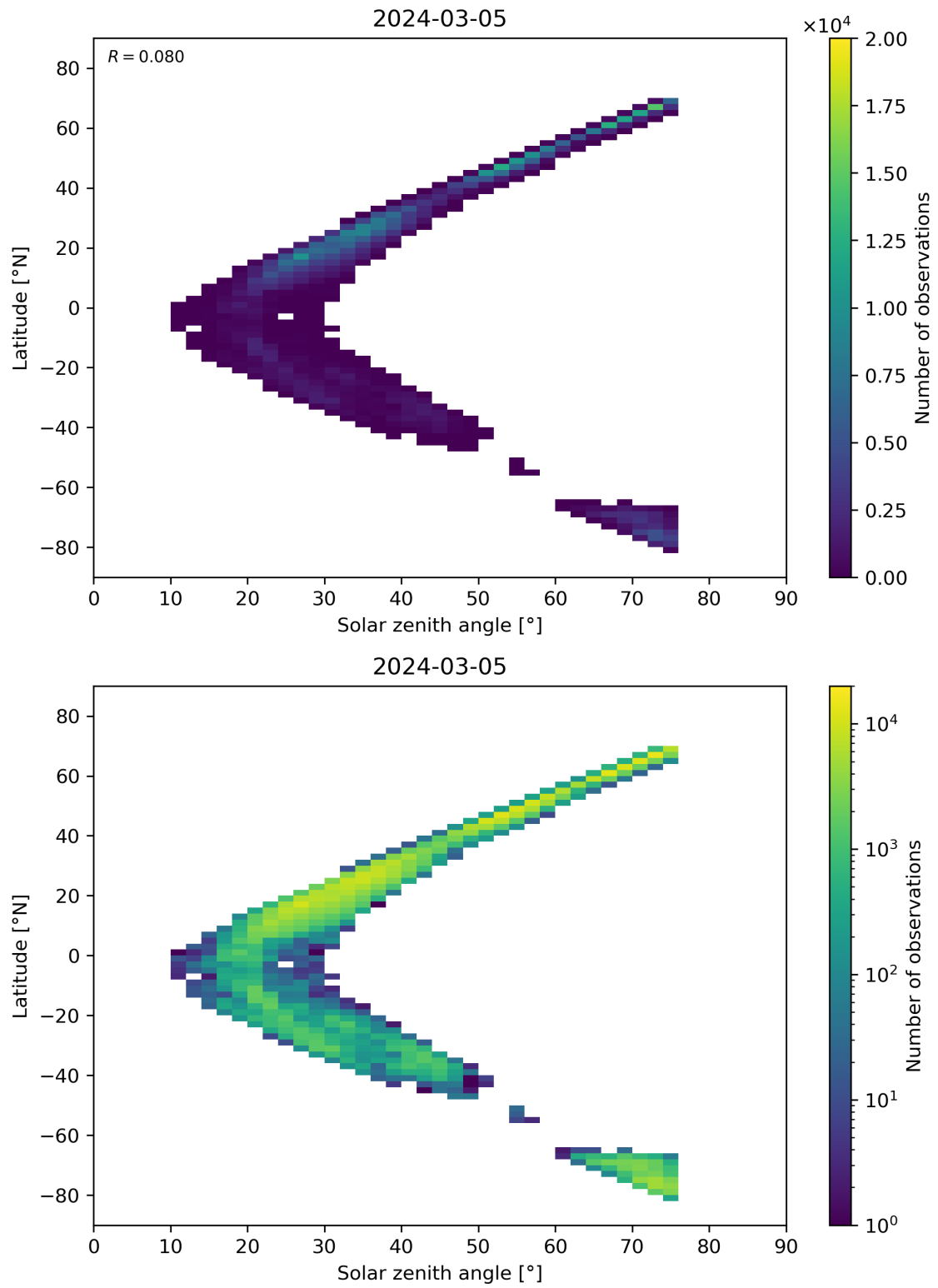
Figure 98: Scatter density plot of “Solar zenith angle” against “Latitude” for 2024-03-04 to 2024-03-06.
