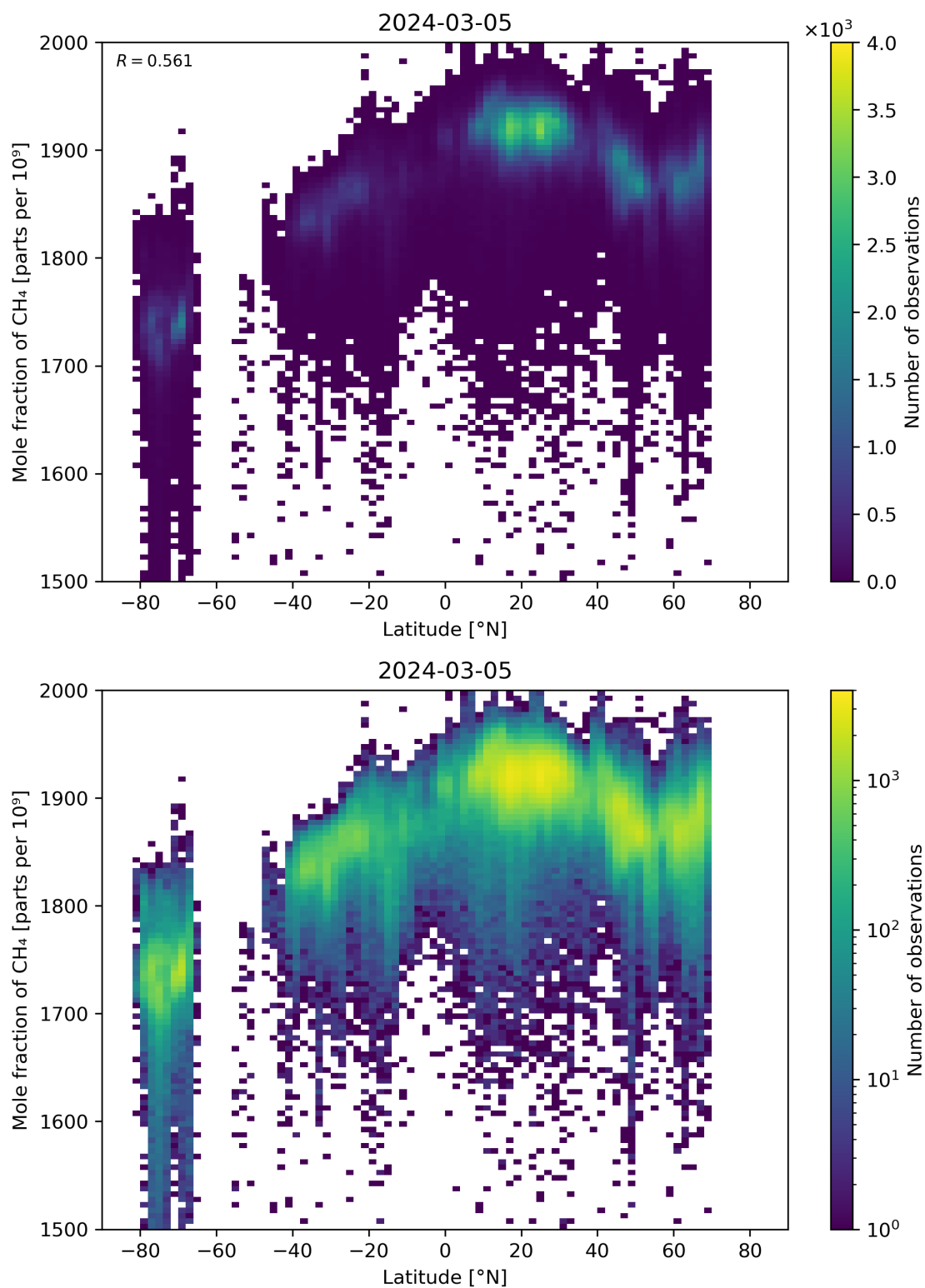
Figure 57: Scatter density plot of “Latitude” against “Mole fraction of \text{CH}_4 ” for 2024-03-04 to 2024-03-06.
