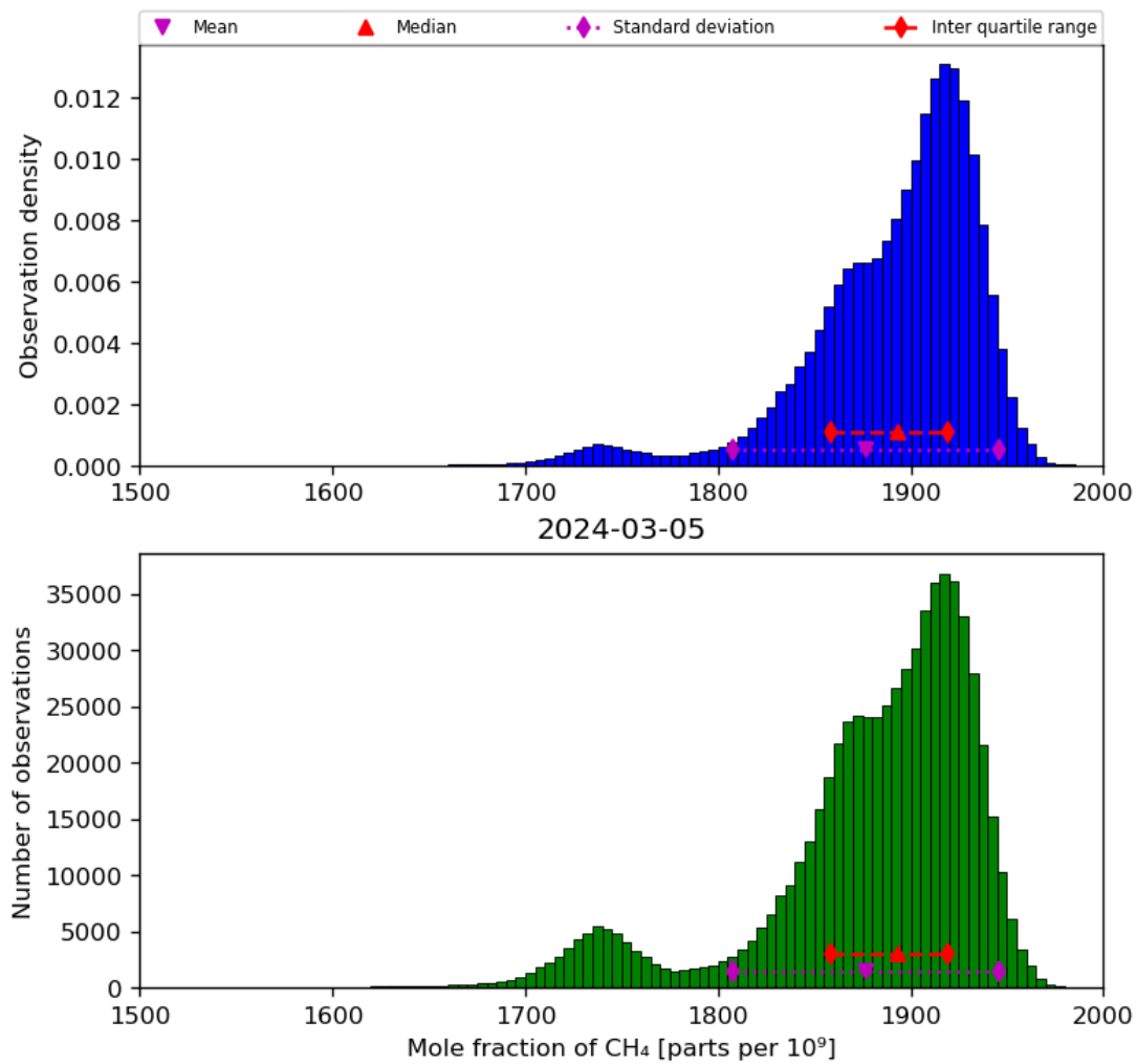
Figure 23: Histogram of "Mole fraction of CH 4 " for 2024-03-04 to 2024-03-06
