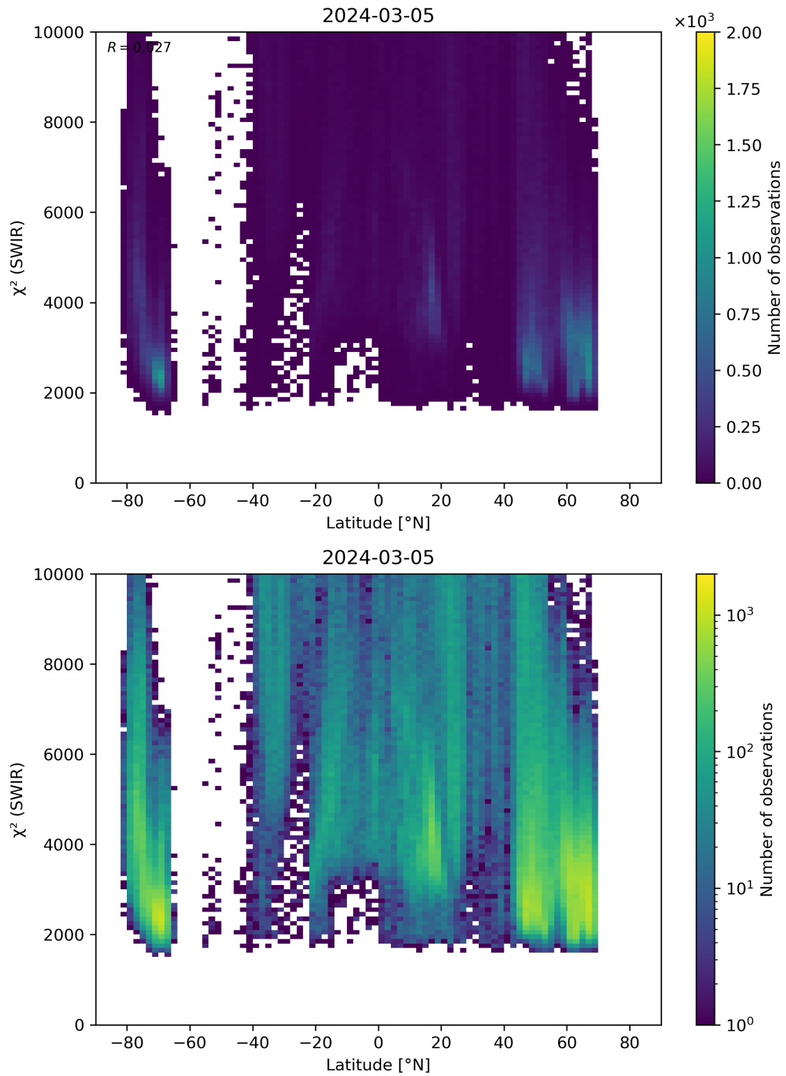
Figure 54: Scatter density plot of “Latitude” against “ \chi^2 (SWIR)” for 2024-03-04 to 2024-03-06.
