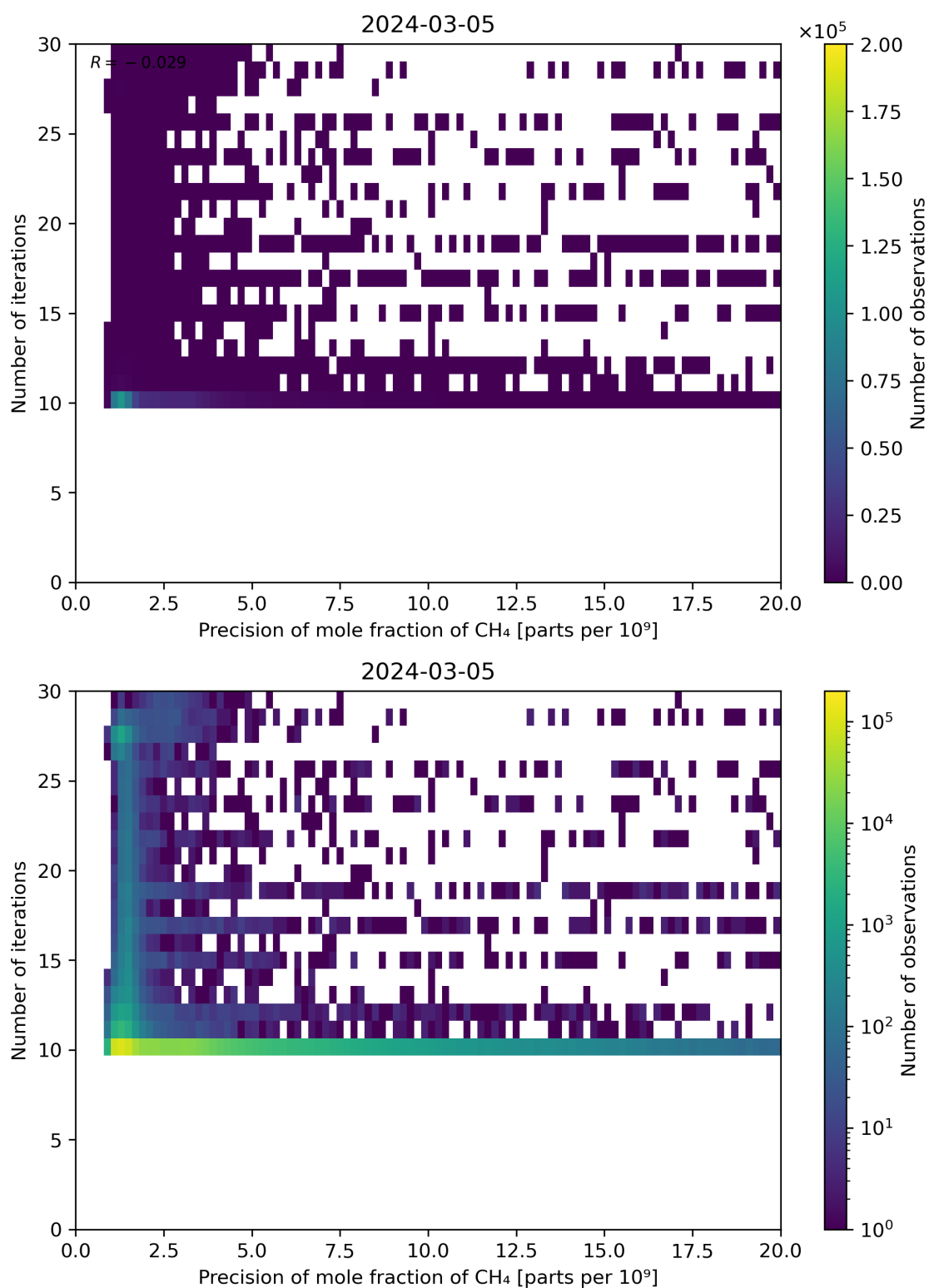
Figure 83: Scatter density plot of “Precision of mole fraction of CH 4 ” against “Number of iterations” for 2024-03-04 to 2024-03-06.
