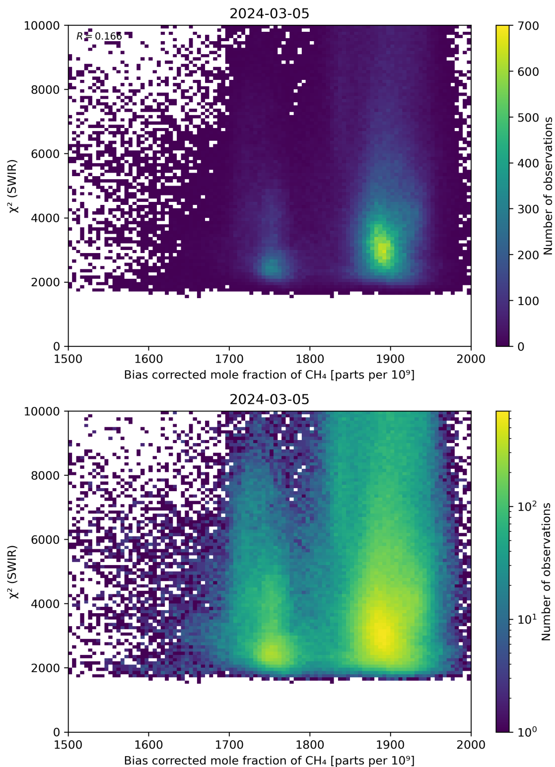
Figure 64: Scatter density plot of “Bias corrected mole fraction of CH 4 ” against “ \chi^2 (SWIR)” for 2024-03-04 to 2024-03-06.
