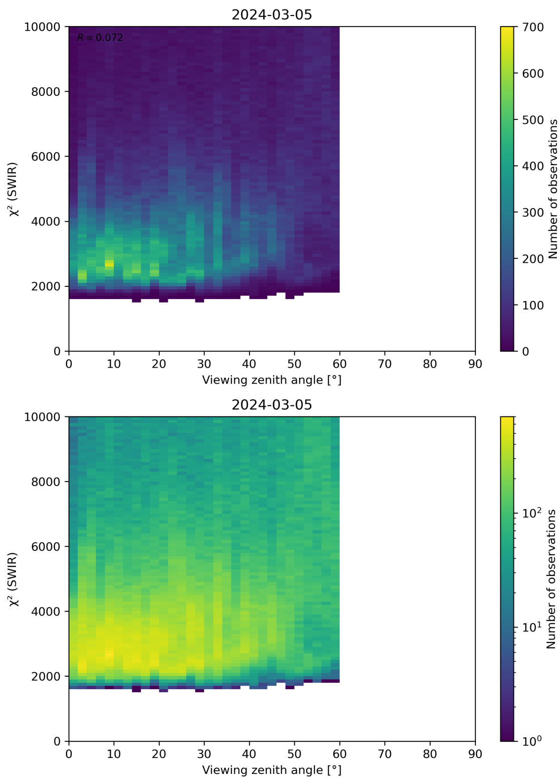
Figure 106: Scatter density plot of “Viewing zenith angle” against “ \chi^2 (SWIR)” for 2024-03-04 to 2024-03-06.
