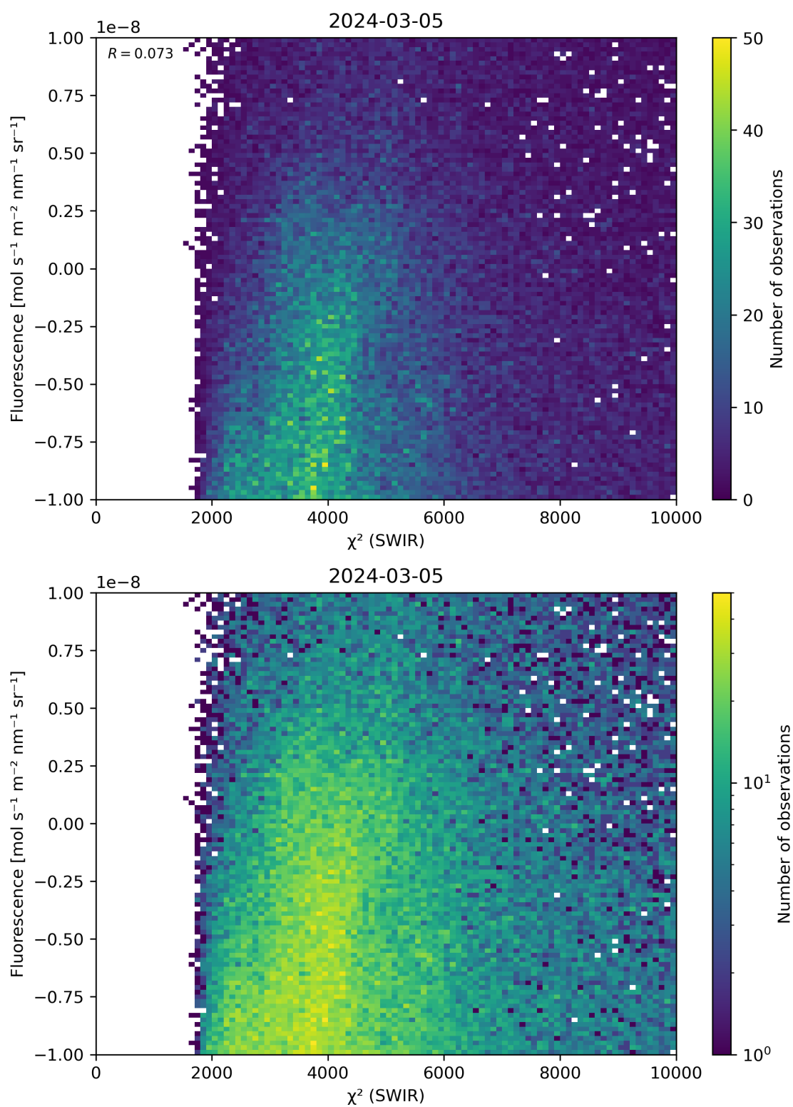
Figure 49: Scatter density plot of “ \chi^2 (SWIR)” against “Fluorescence” for 2024-03-04 to 2024-03-06.
