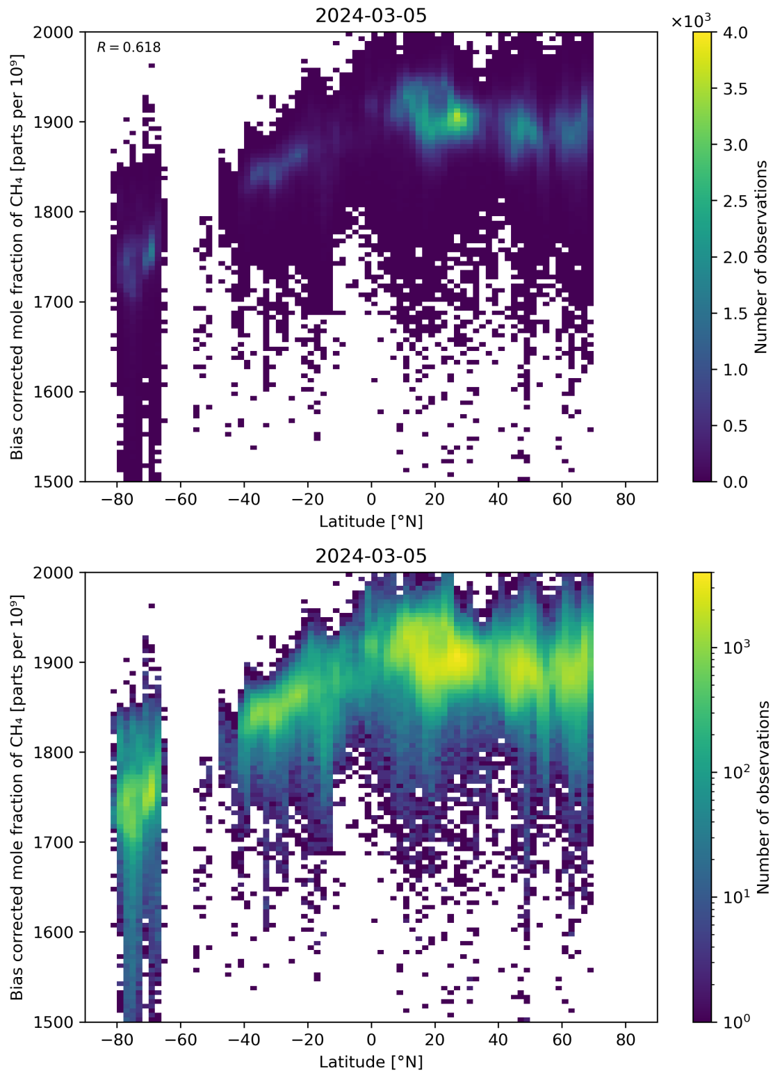
Figure 58: Scatter density plot of “Latitude” against “Bias corrected mole fraction of CH 4 ” for 2024-03-04 to 2024-03-06.
