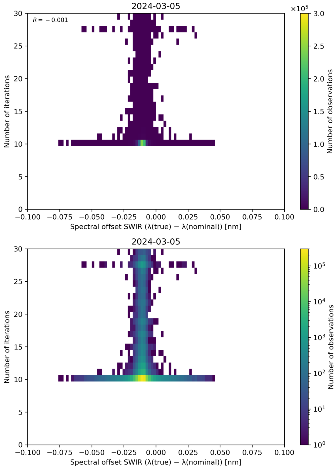
Figure 121: Scatter density plot of “Spectral offset SWIR ( \lambda(\text{true}) - \lambda(\text{nominal}) )” against “Number of iterations” for 2024-03-04 to 2024-03-06.
