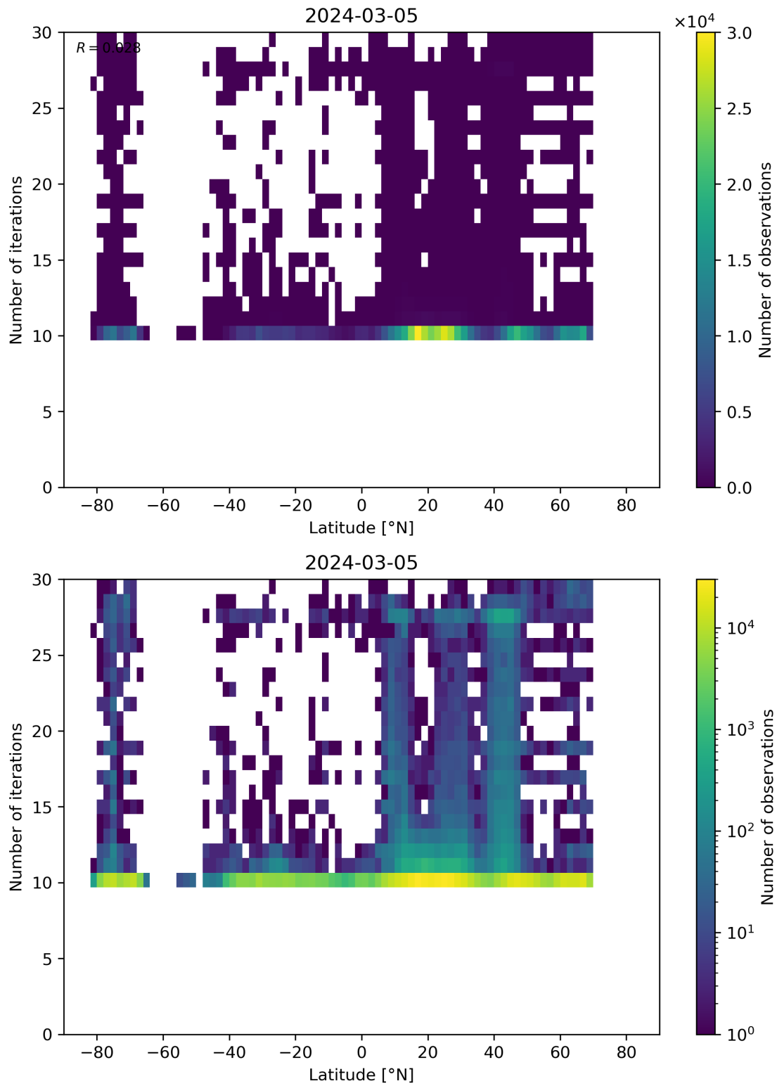
Figure 60: Scatter density plot of “Latitude” against “Number of iterations” for 2024-03-04 to 2024-03-06.
