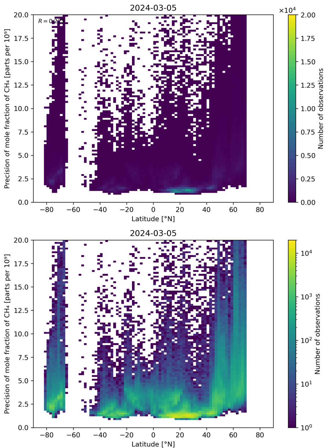
Figure 59: Scatter density plot of “Latitude” against “Precision of mole fraction of CH 4 ” for 2024-03-04 to 2024-03-06.
