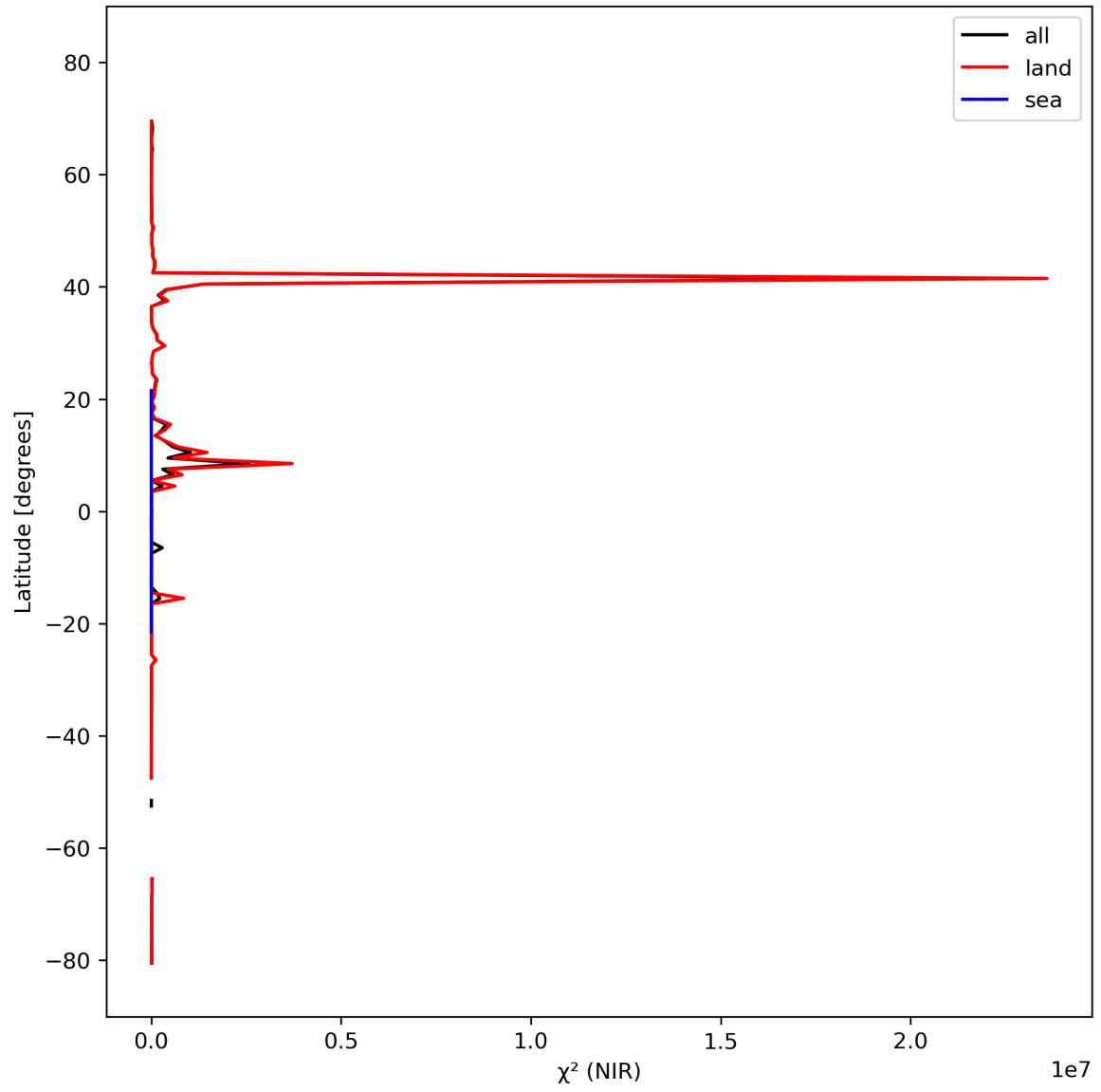
Figure 18: Zonal average of “ \chi^2 (NIR)” for 2024-03-04 to 2024-03-06.
