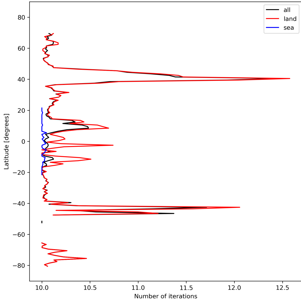
Figure 20: Zonal average of “Number of iterations” for 2024-03-04 to 2024-03-06.
