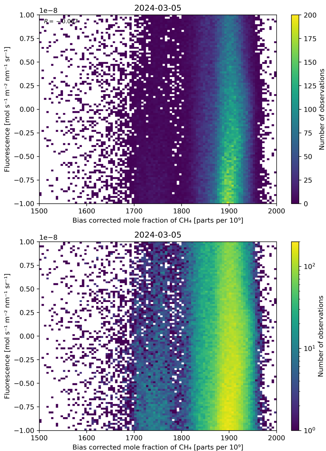
Figure 66: Scatter density plot of “Bias corrected mole fraction of \text{CH}_4 ” against “Fluorescence” for 2024-03-04 to 2024-03-06.
