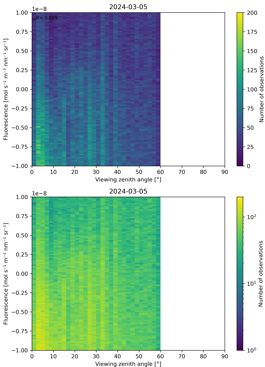
Figure 108: Scatter density plot of “Viewing zenith angle” against “Fluorescence” for 2024-03-04 to 2024-03-06.
