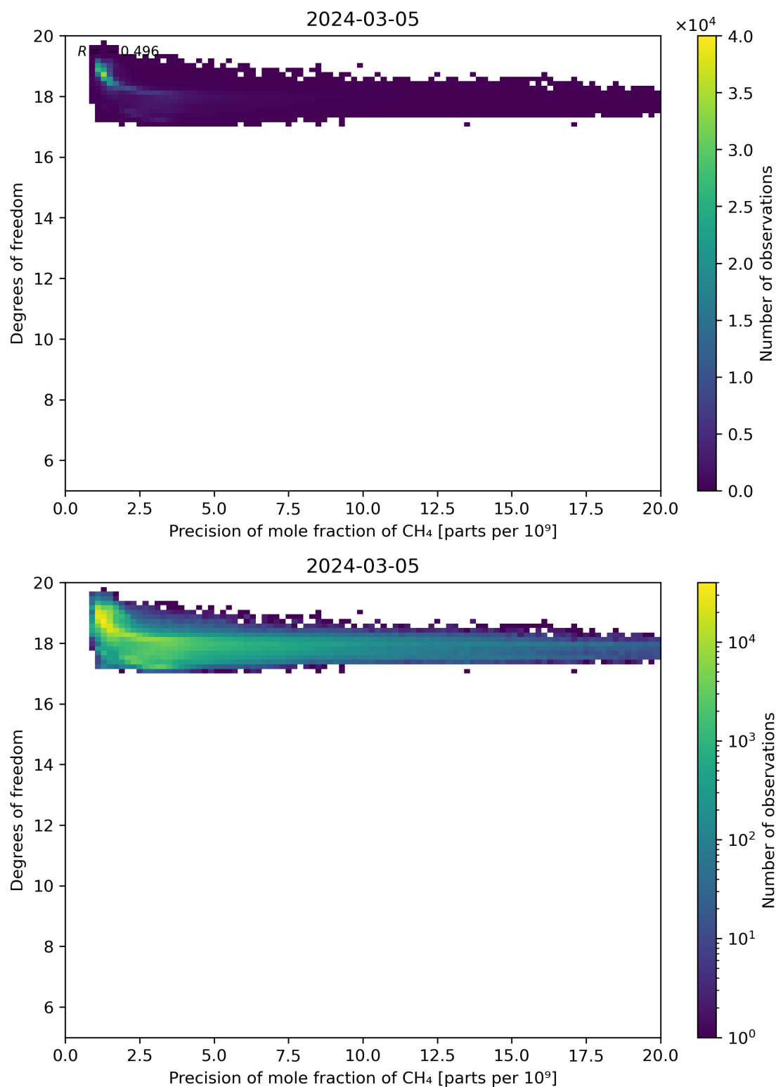
Figure 80: Scatter density plot of “Precision of mole fraction of CH 4 ” against “Degrees of freedom” for 2024-03-04 to 2024-03-06.
