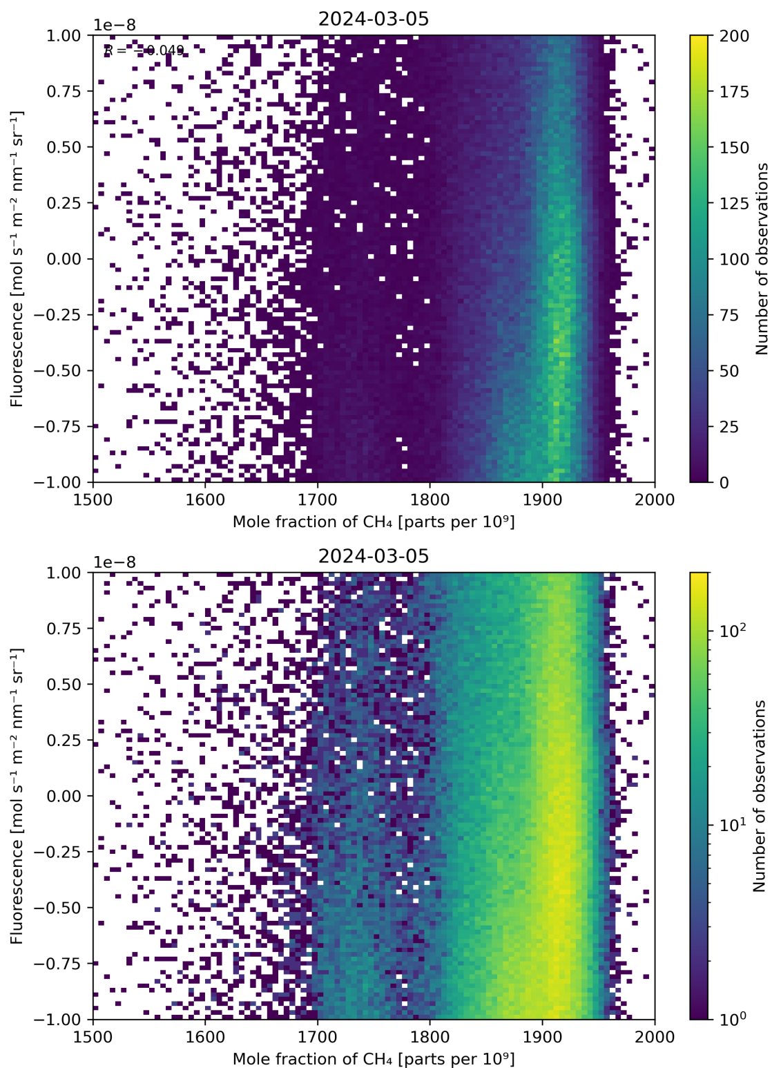
Figure 73: Scatter density plot of “Mole fraction of \text{CH}_4 ” against “Fluorescence” for 2024-03-04 to 2024-03-06.
