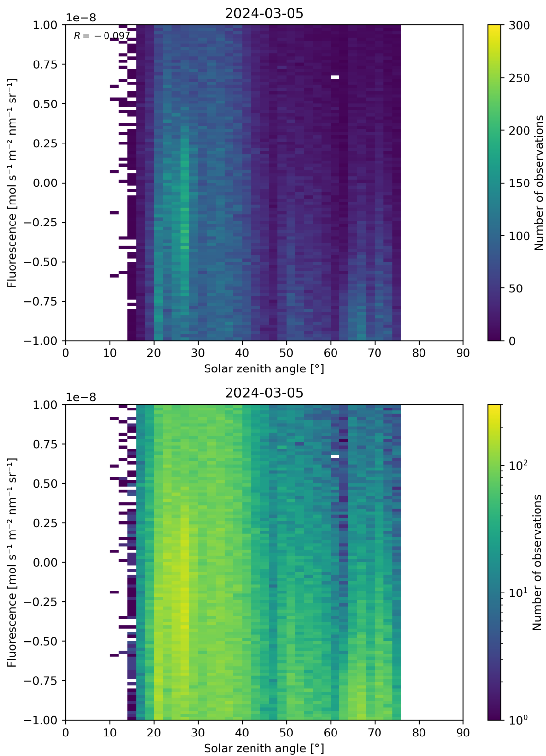
Figure 97: Scatter density plot of “Solar zenith angle” against “Fluorescence” for 2024-03-04 to 2024-03-06.
