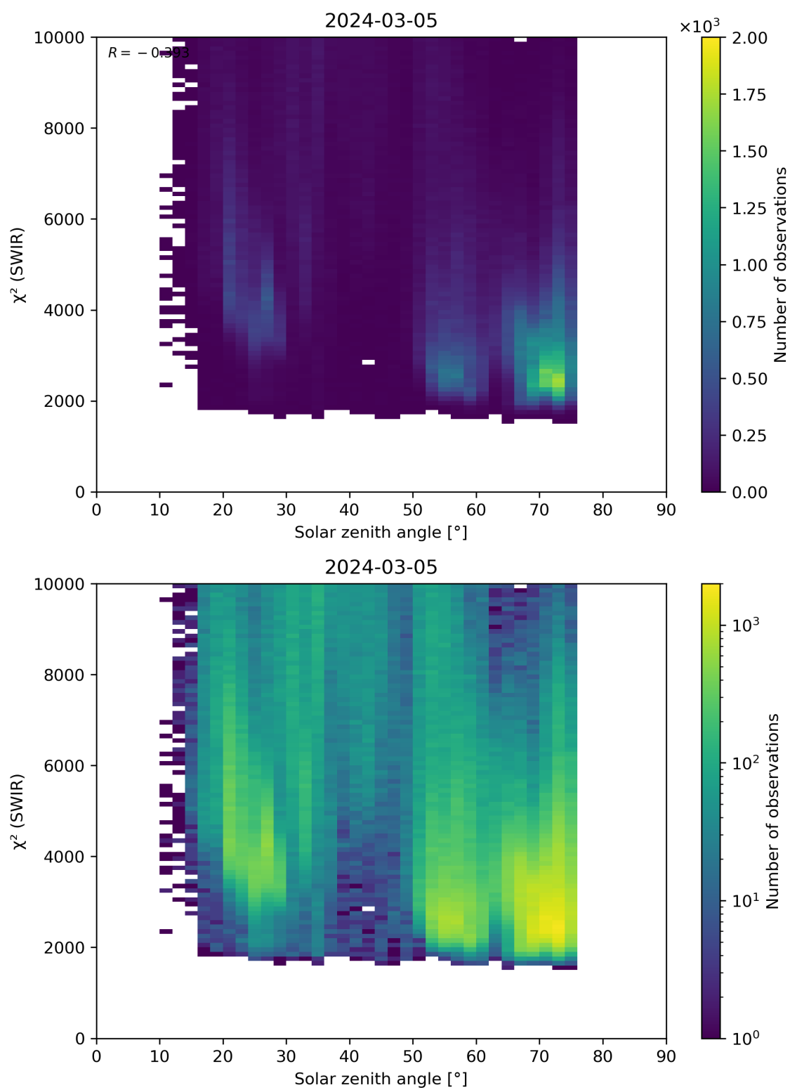
Figure 95: Scatter density plot of “Solar zenith angle” against “ \chi^2 (SWIR)” for 2024-03-04 to 2024-03-06.
