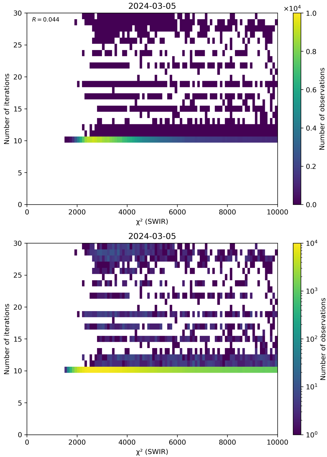
Figure 50: Scatter density plot of “ \chi^2 (SWIR)” against “Number of iterations” for 2024-03-04 to 2024-03-06.
