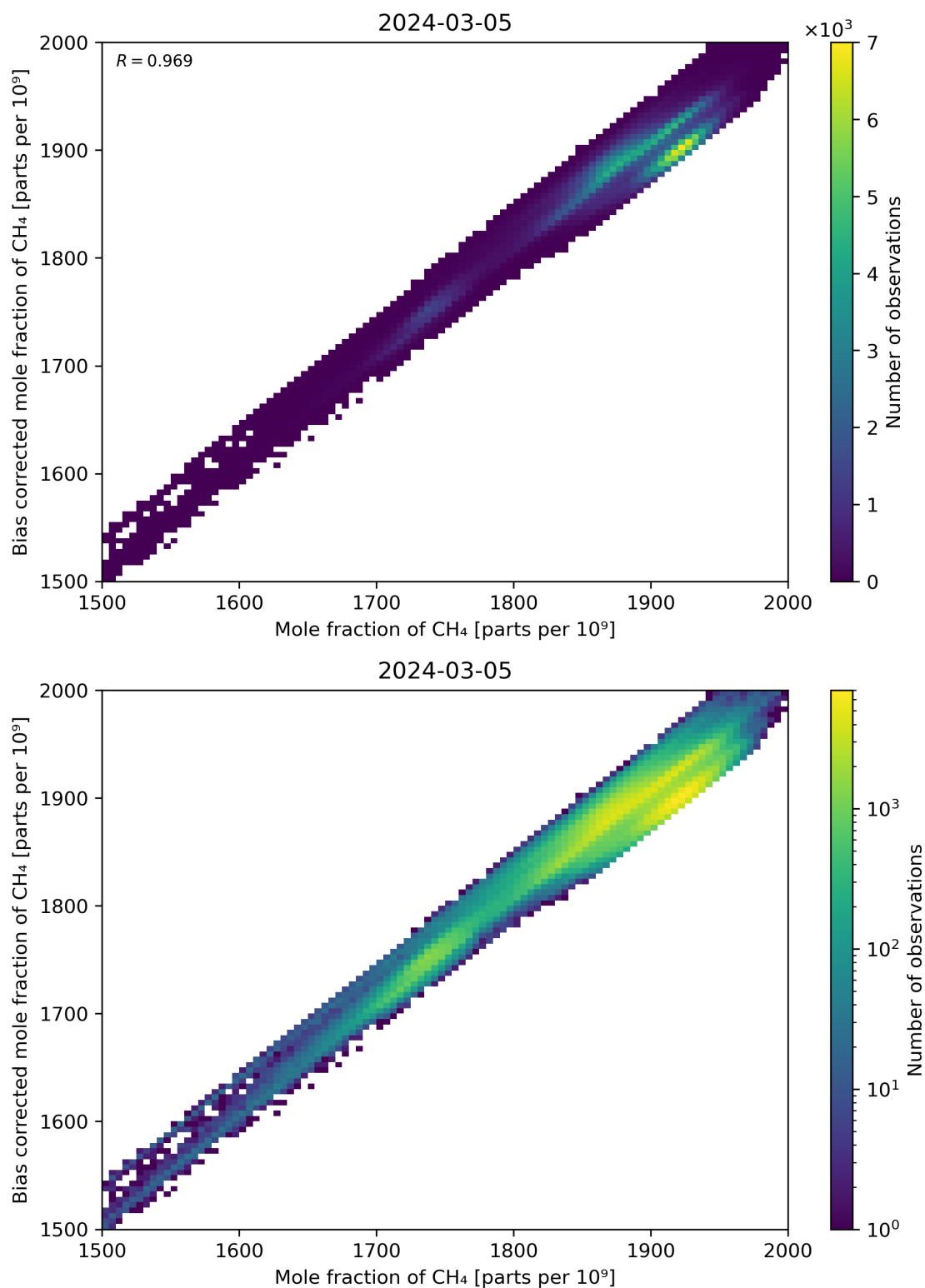
Figure 74: Scatter density plot of “Mole fraction of CH 4 ” against “Bias corrected mole fraction of CH 4 ” for 2024-03-04 to 2024-03-06.
