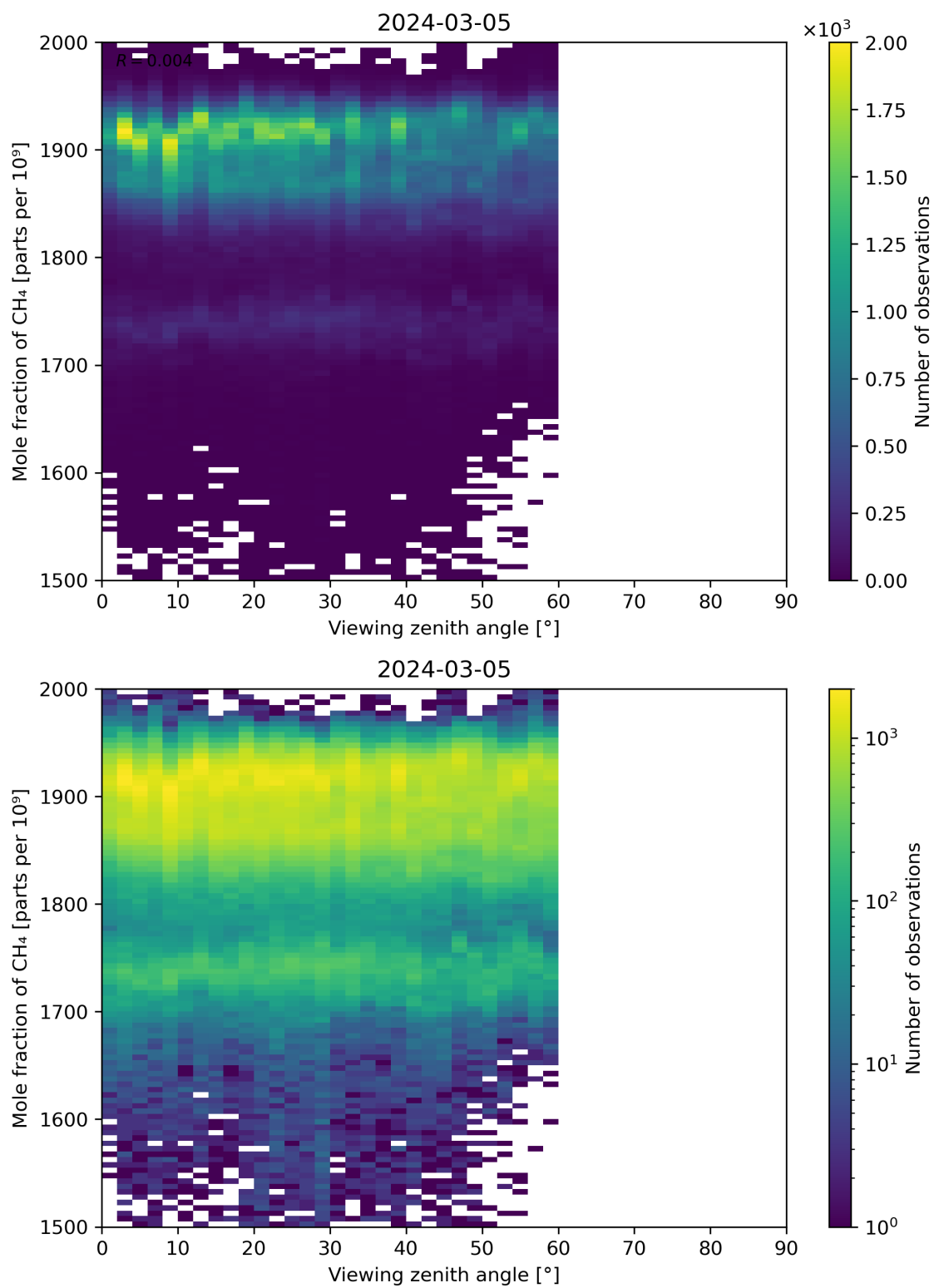
Figure 110: Scatter density plot of “Viewing zenith angle” against “Mole fraction of CH 4 ” for 2024-03-04 to 2024-03-06.
