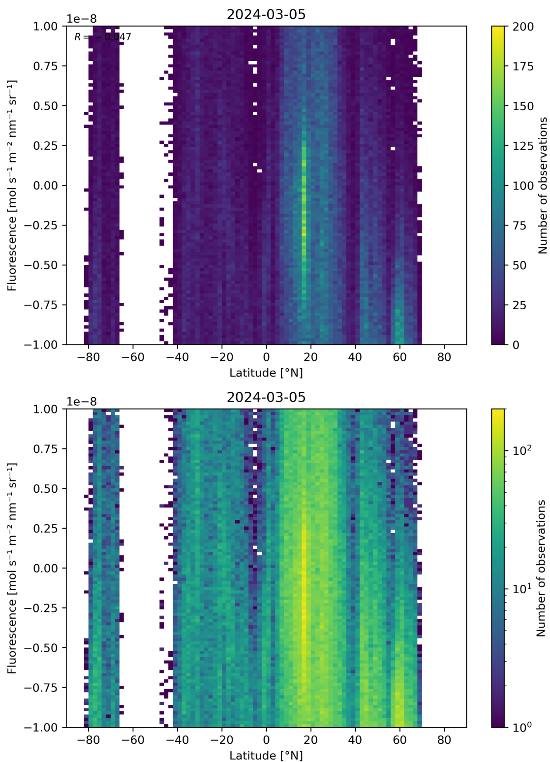
Figure 56: Scatter density plot of “Latitude” against “Fluorescence” for 2024-03-04 to 2024-03-06.
