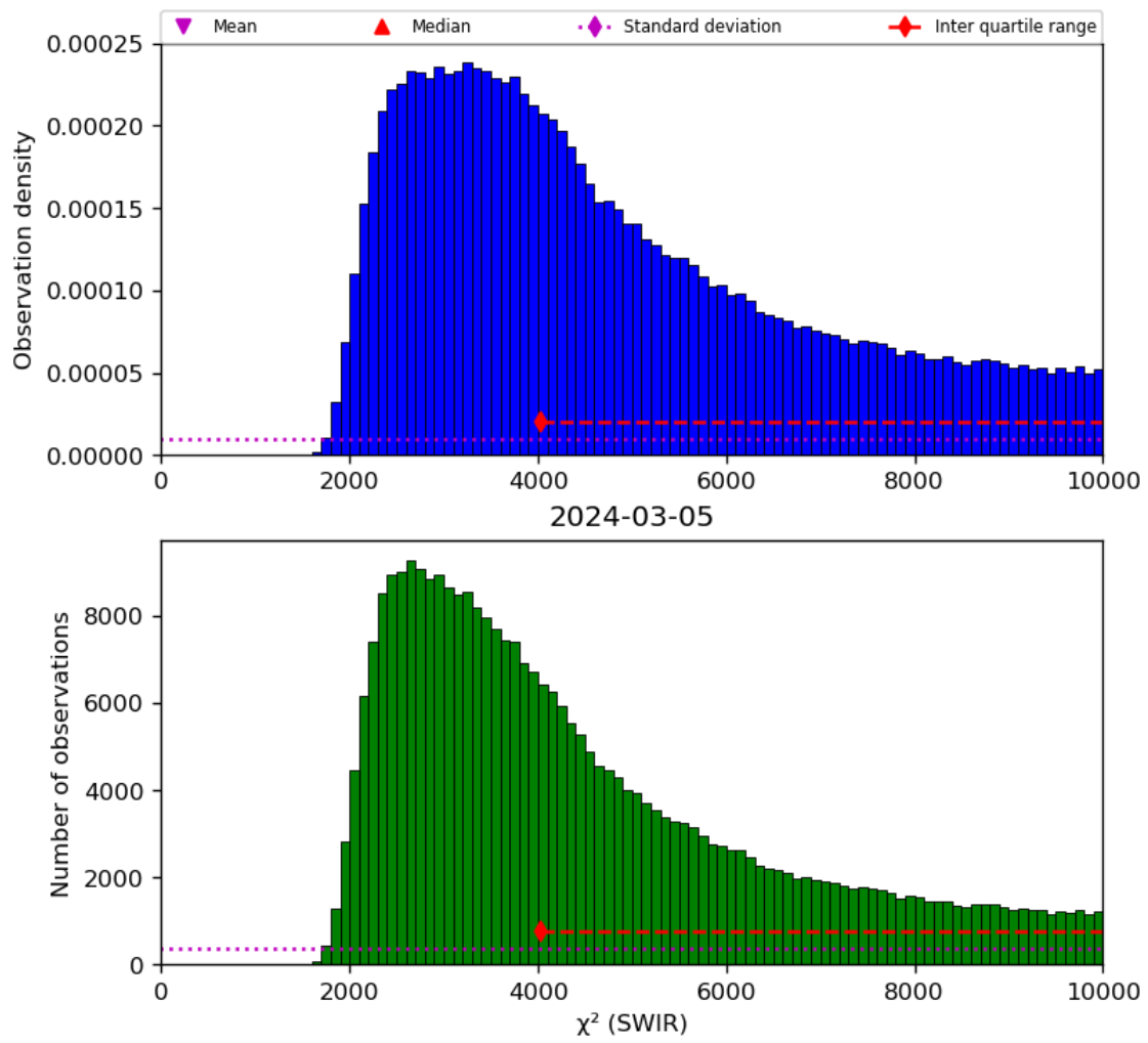
Figure 28: Histogram of “ \chi^2 (SWIR)” for 2024-03-04 to 2024-03-06
