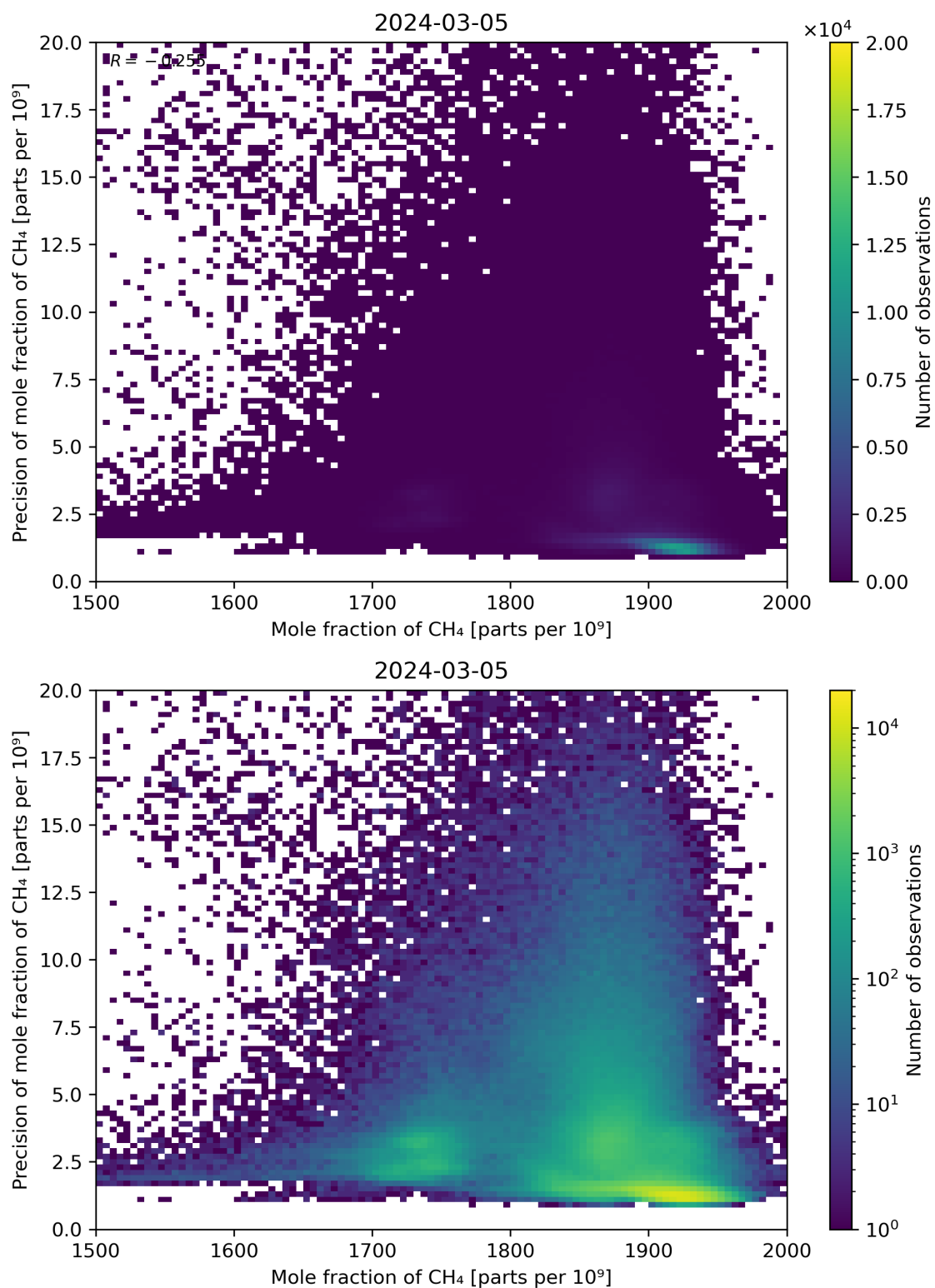
Figure 75: Scatter density plot of “Mole fraction of CH 4 ” against “Precision of mole fraction of CH 4 ” for 2024-03-04 to 2024-03-06.
