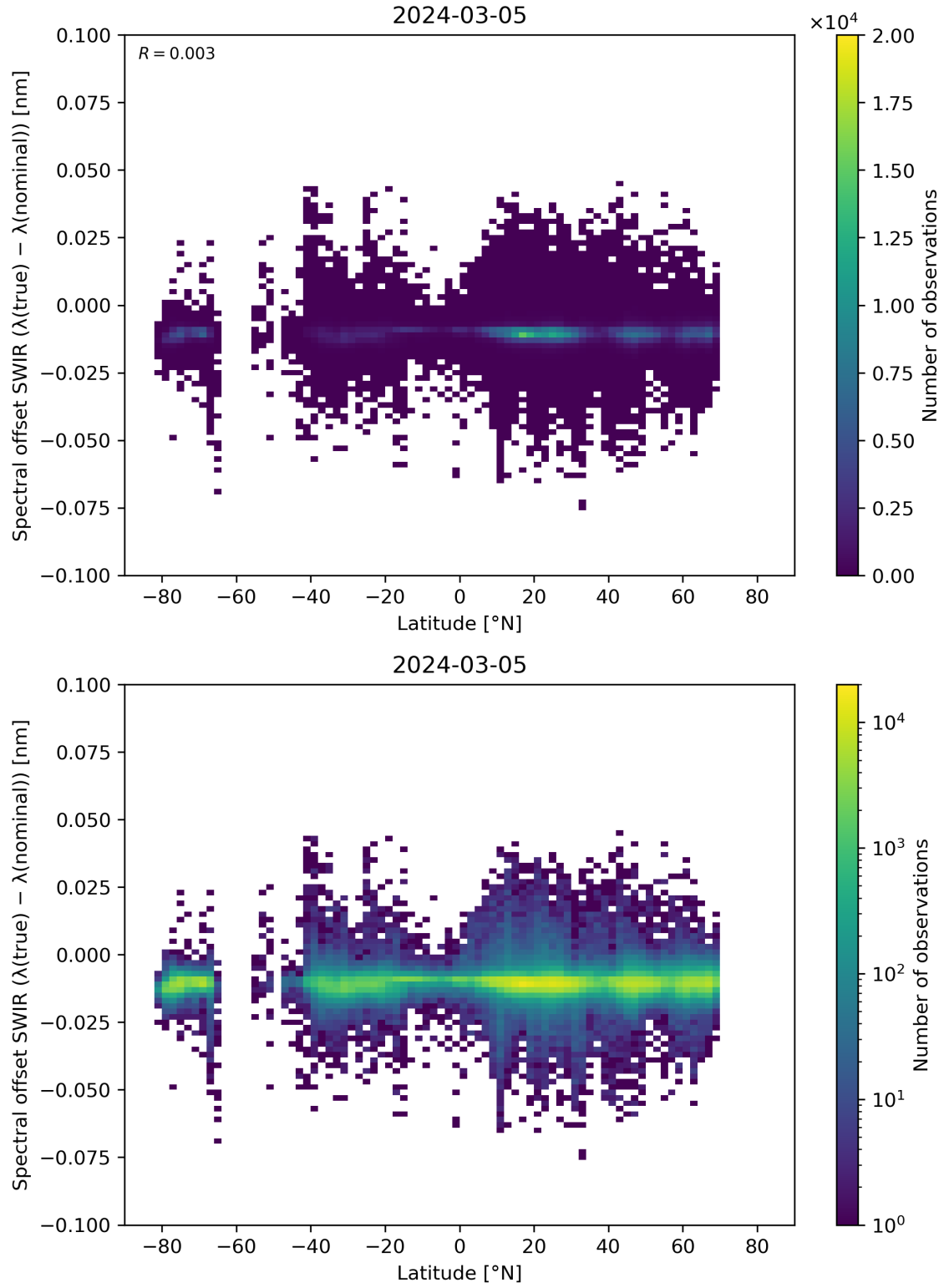
Figure 62: Scatter density plot of “Latitude” against “Spectral offset SWIR ( \lambda(\text{true}) - \lambda(\text{nominal}) )” for 2024-03-04 to 2024-03-06.
