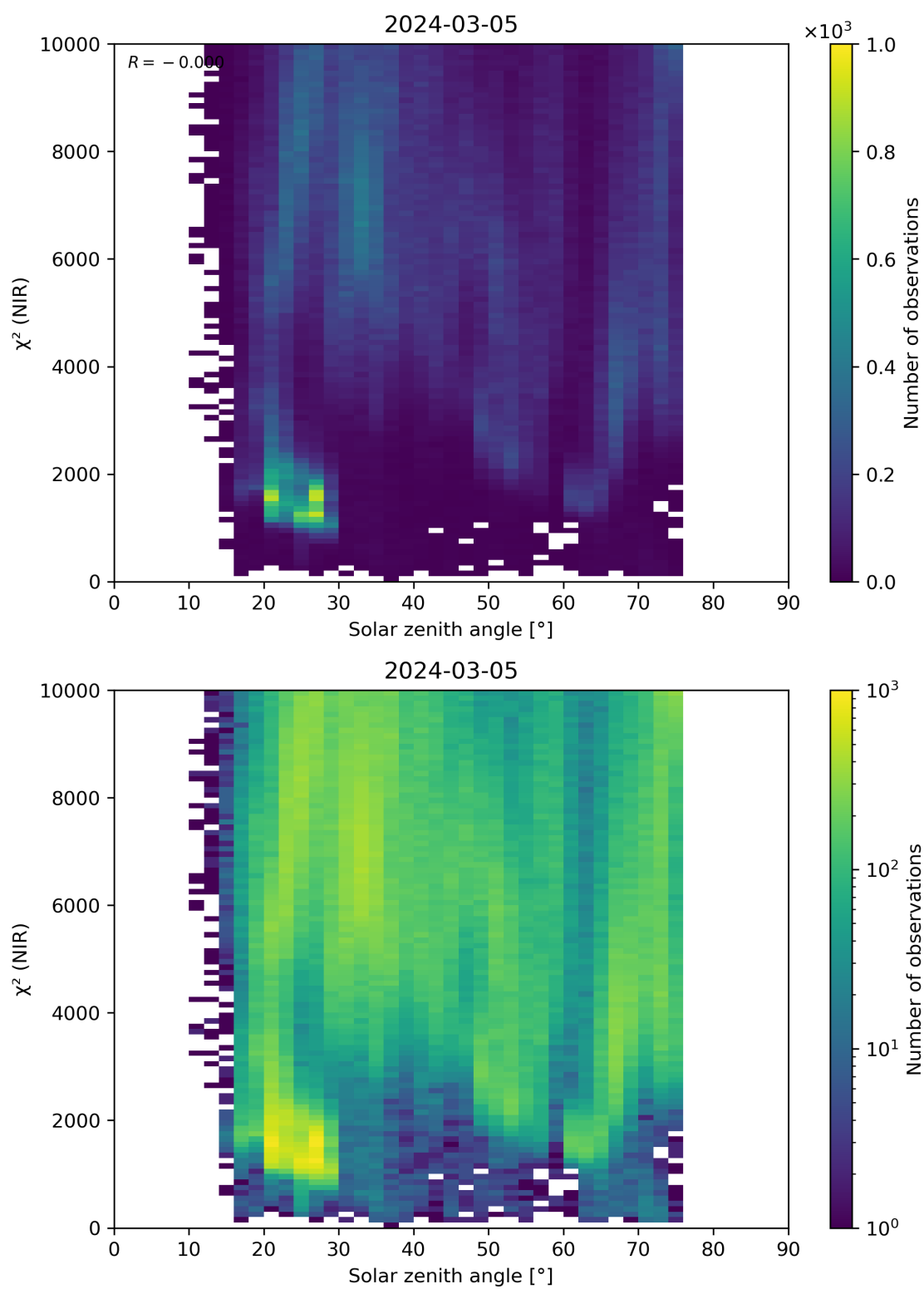
Figure 94: Scatter density plot of “Solar zenith angle” against “ \chi^2 (NIR)” for 2024-03-04 to 2024-03-06.
