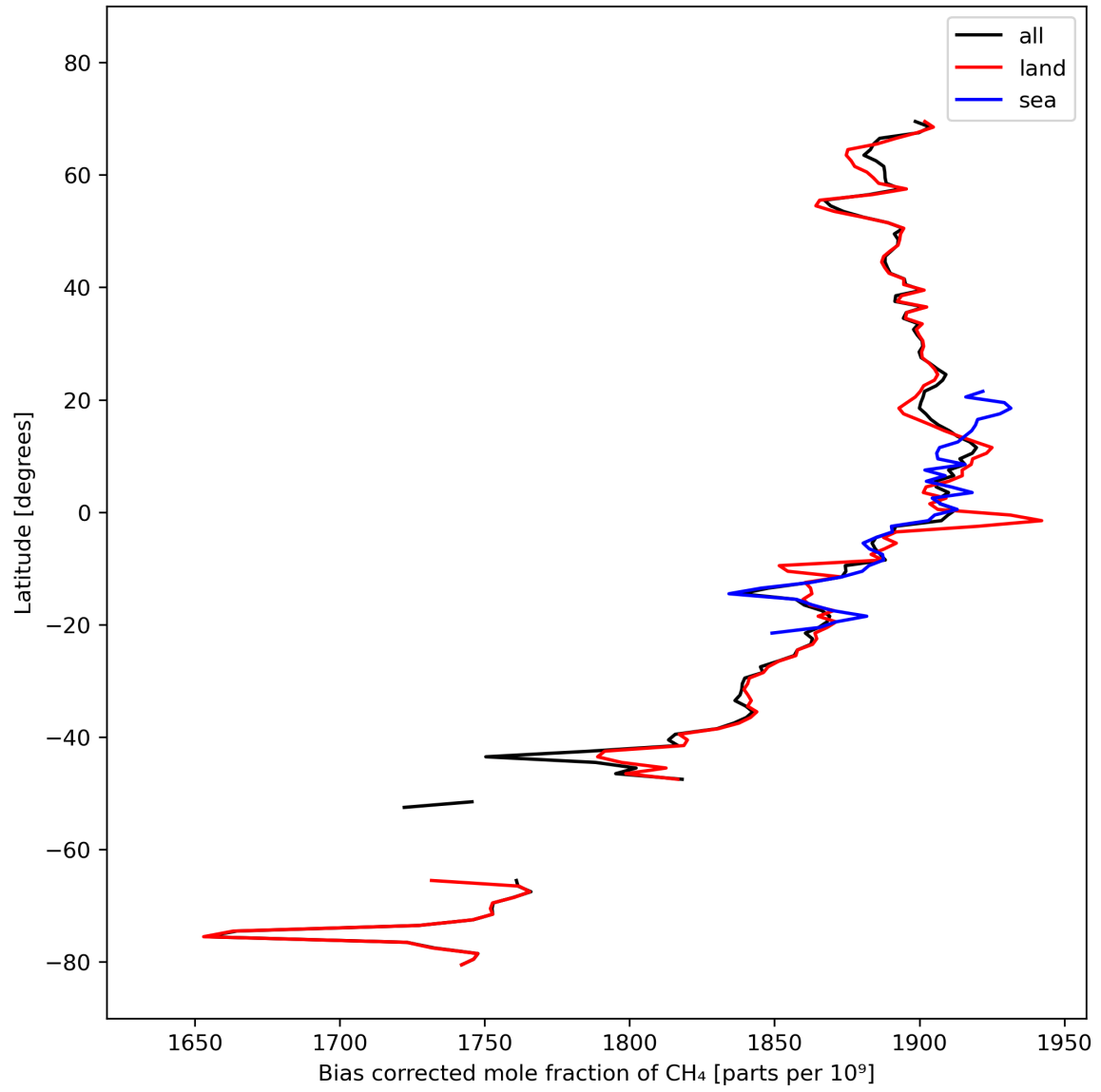
Figure 14: Zonal average of “Bias corrected mole fraction of \text{CH}_4 ” for 2024-03-04 to 2024-03-06.
