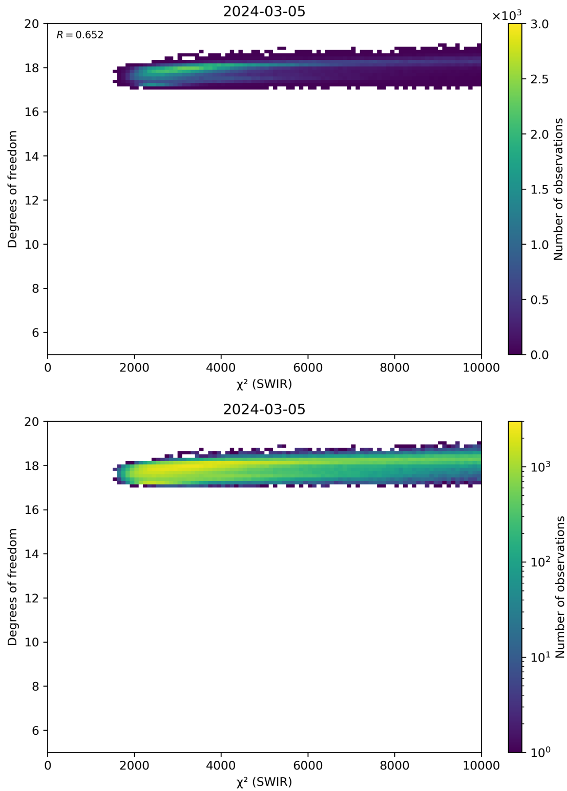
Figure 48: Scatter density plot of “ \chi^2 (SWIR)” against “Degrees of freedom” for 2024-03-04 to 2024-03-06.
