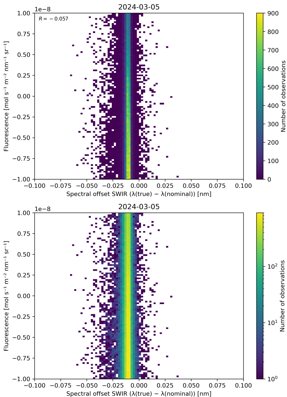
Figure 120: Scatter density plot of “Spectral offset SWIR ( \lambda(\text{true}) - \lambda(\text{nominal}) )” against “Fluorescence” for 2024-03-04 to 2024-03-06.
