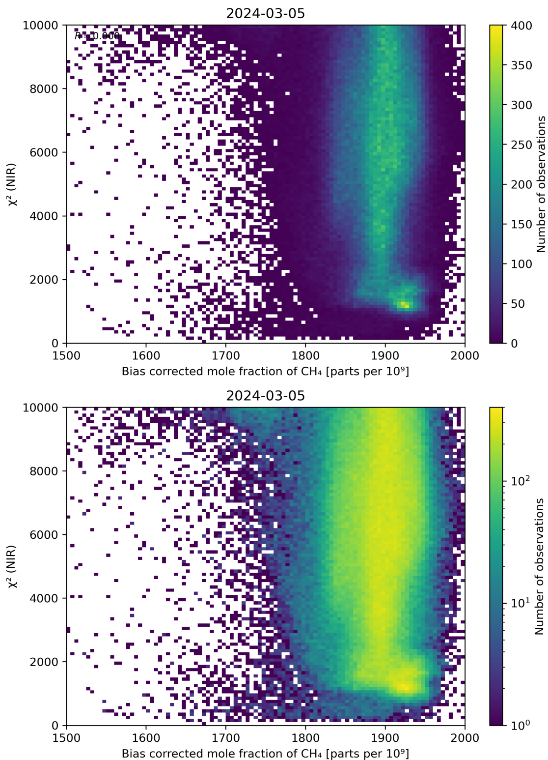
Figure 63: Scatter density plot of “Bias corrected mole fraction of CH 4 ” against “ \chi^2 (NIR)” for 2024-03-04 to 2024-03-06.
