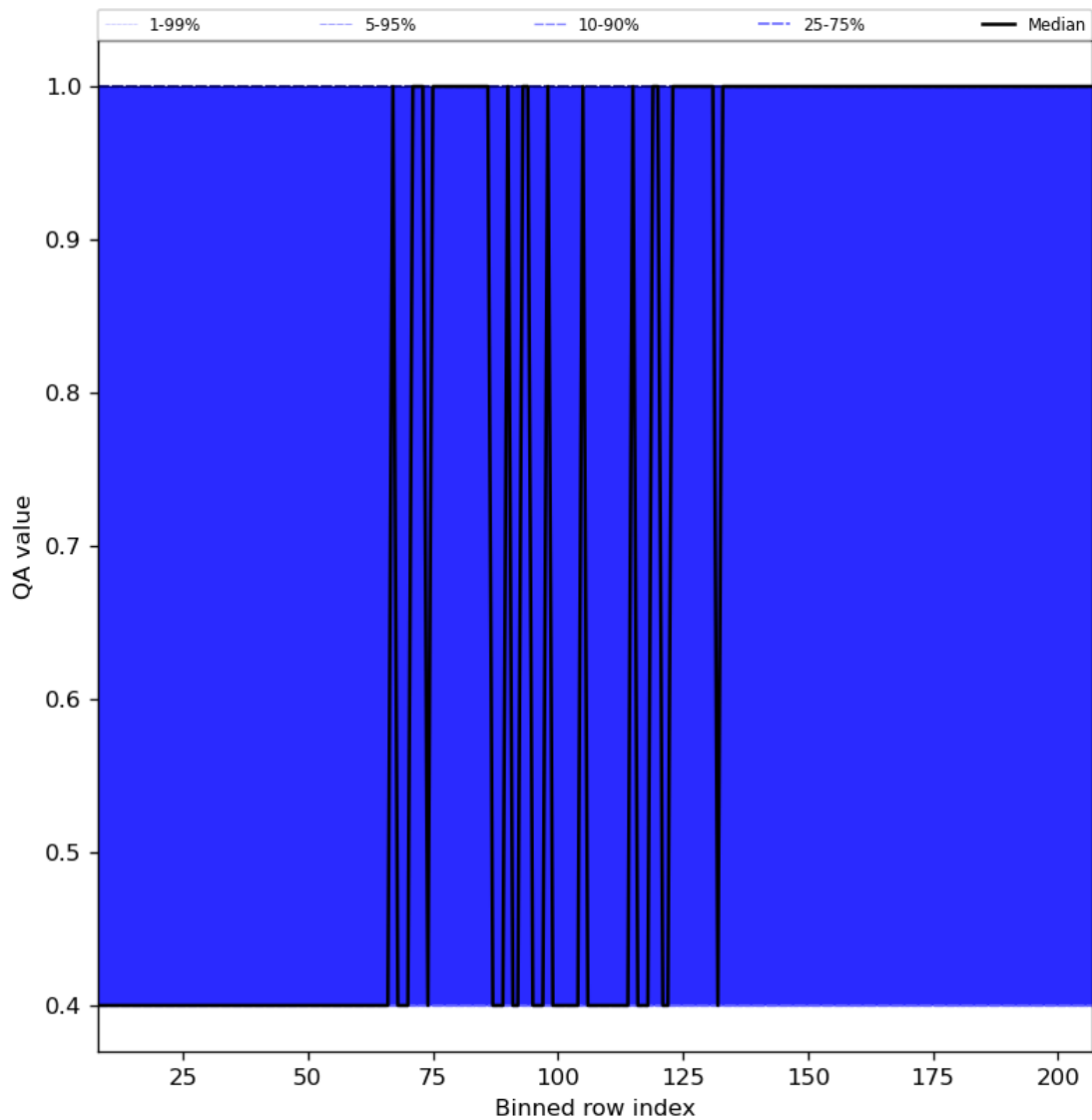
Figure 33: Along track statistics of “QA value” for 2024-03-04 to 2024-03-06
