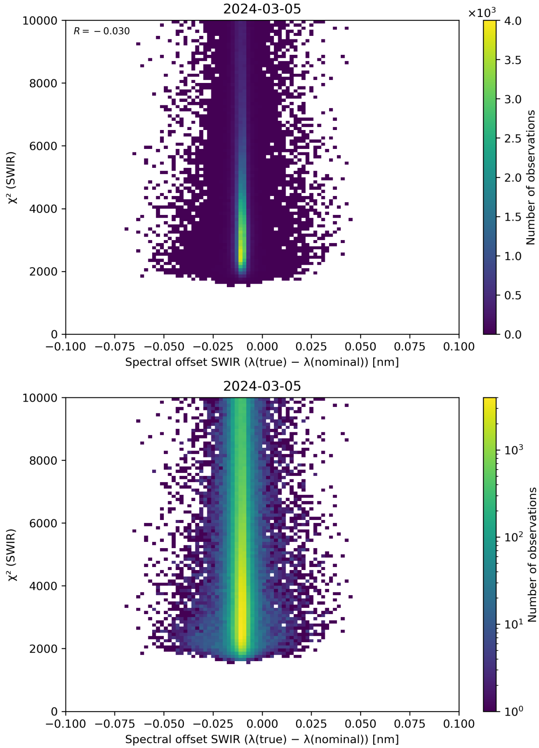
Figure 118: Scatter density plot of “Spectral offset SWIR ( \lambda(\text{true}) - \lambda(\text{nominal}) )” against “ \chi^2 (SWIR)” for 2024-03-04 to 2024-03-06.
