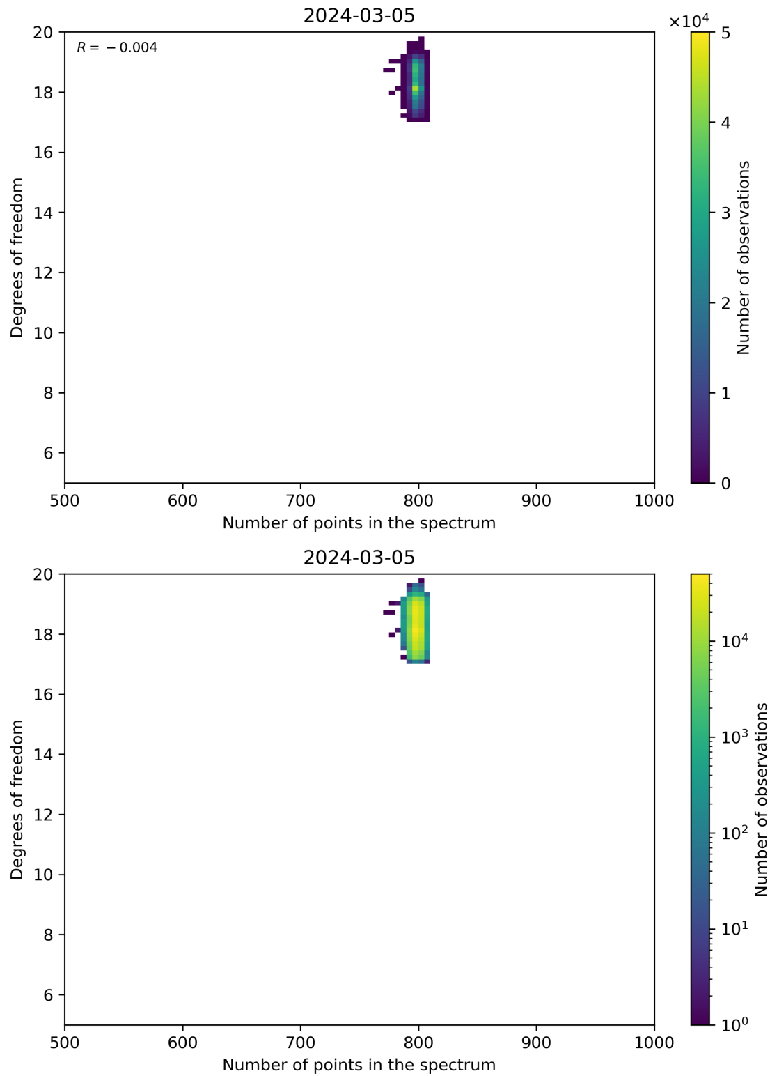
Figure 90: Scatter density plot of “Number of points in the spectrum” against “Degrees of freedom” for 2024-03-04 to 2024-03-06.
