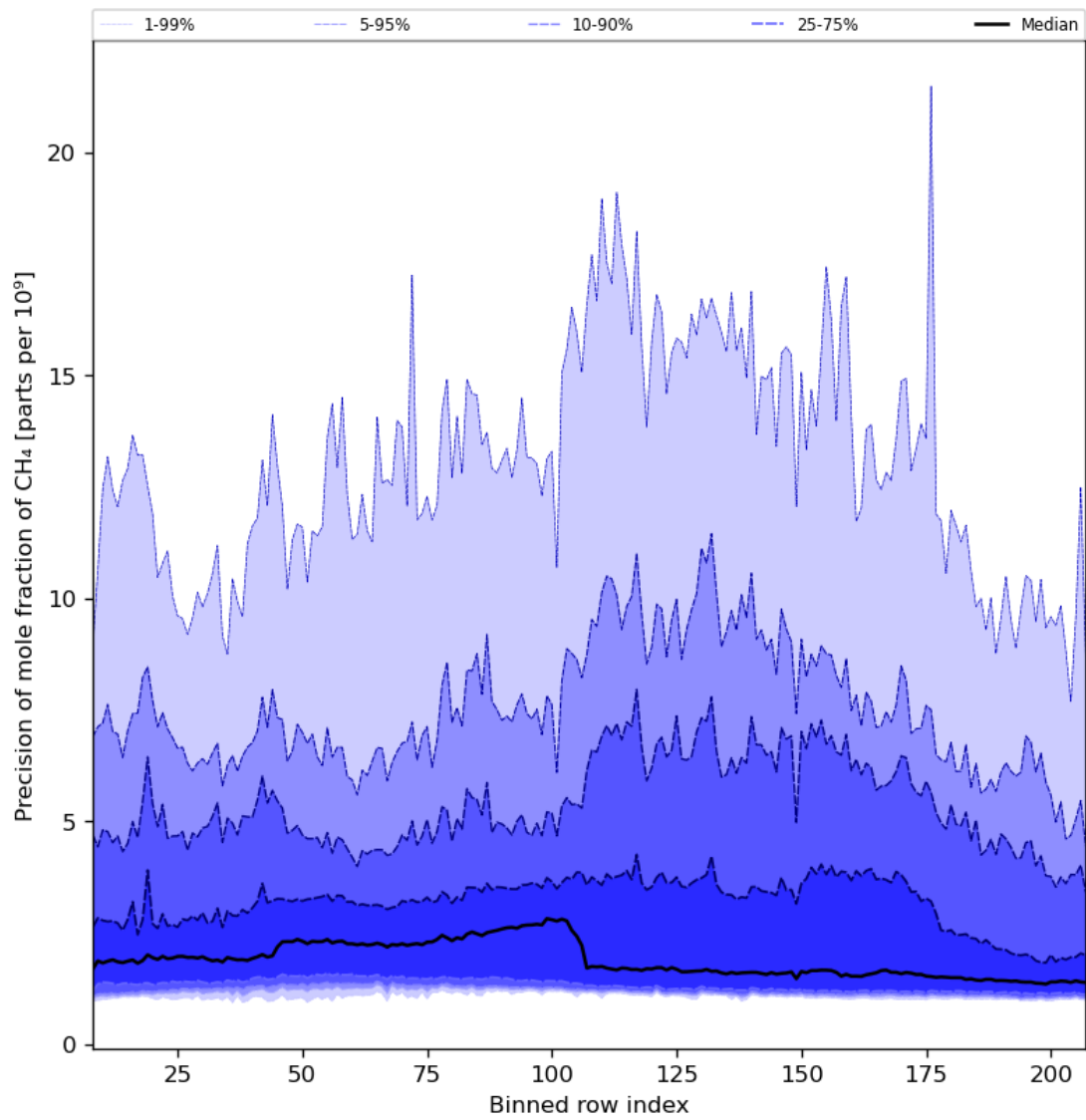
Figure 35: Along track statistics of “Precision of mole fraction of CH 4 ” for 2024-03-04 to 2024-03-06
