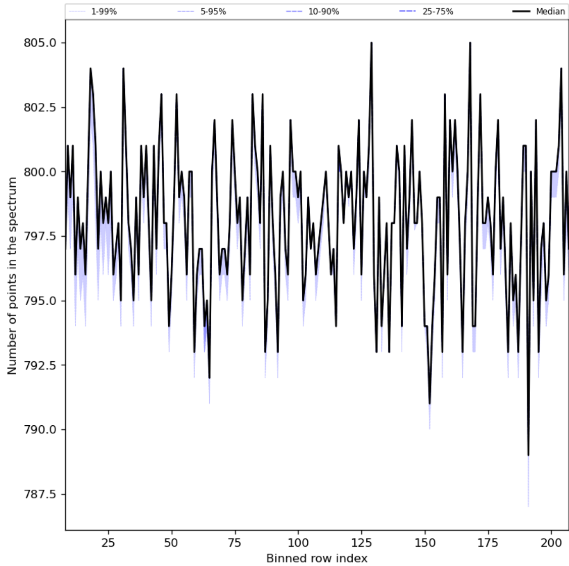
Figure 37: Along track statistics of “Number of points in the spectrum” for 2024-03-04 to 2024-03-06
