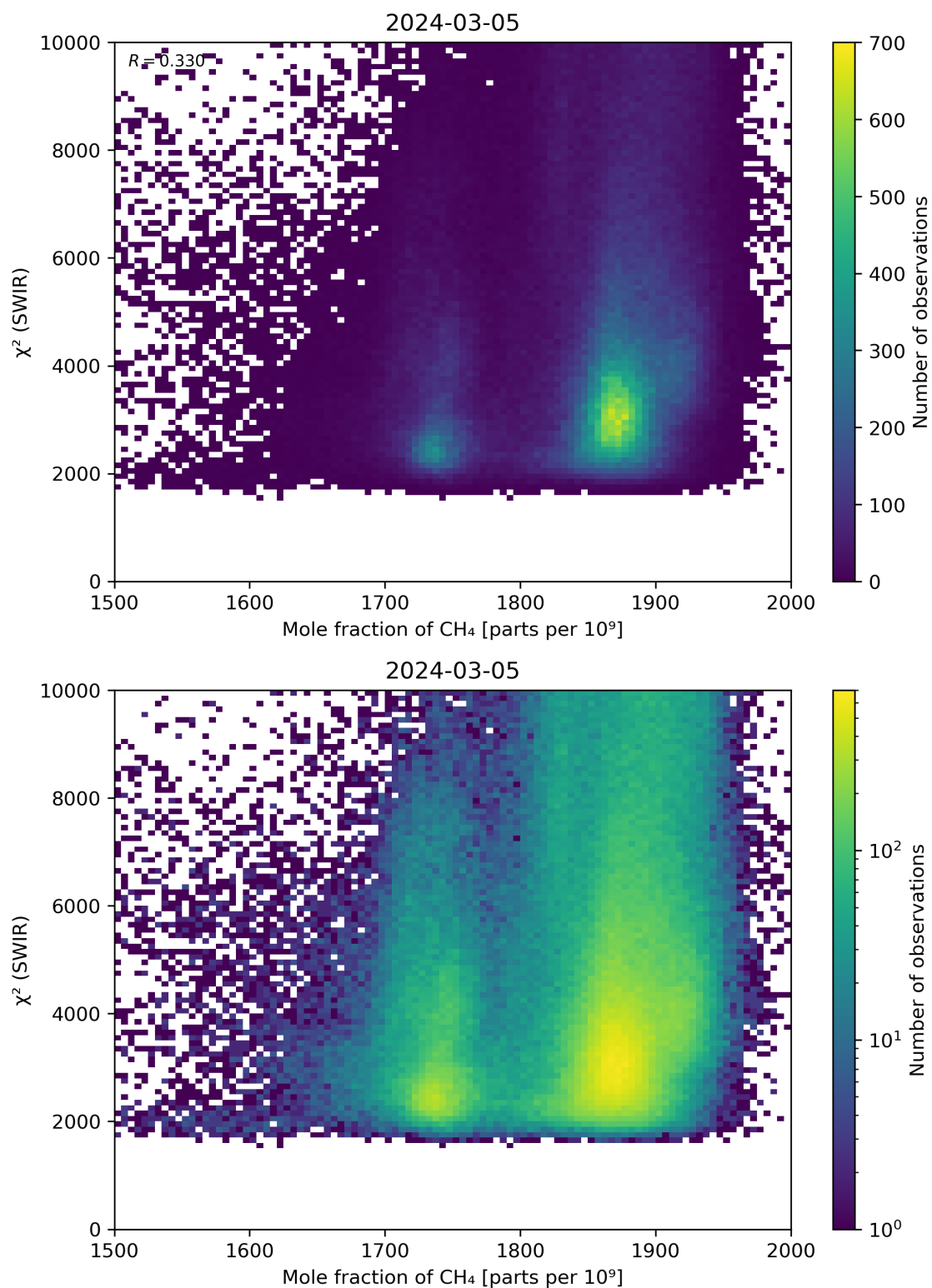
Figure 71: Scatter density plot of “Mole fraction of \text{CH}_4 ” against “ \chi^2 (SWIR)” for 2024-03-04 to 2024-03-06.
