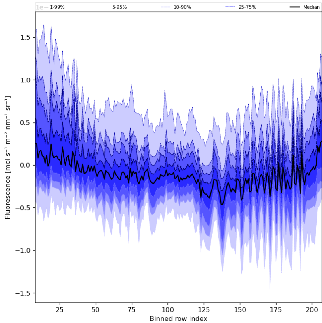
Figure 43: Along track statistics of “Fluorescence” for 2024-03-04 to 2024-03-06
