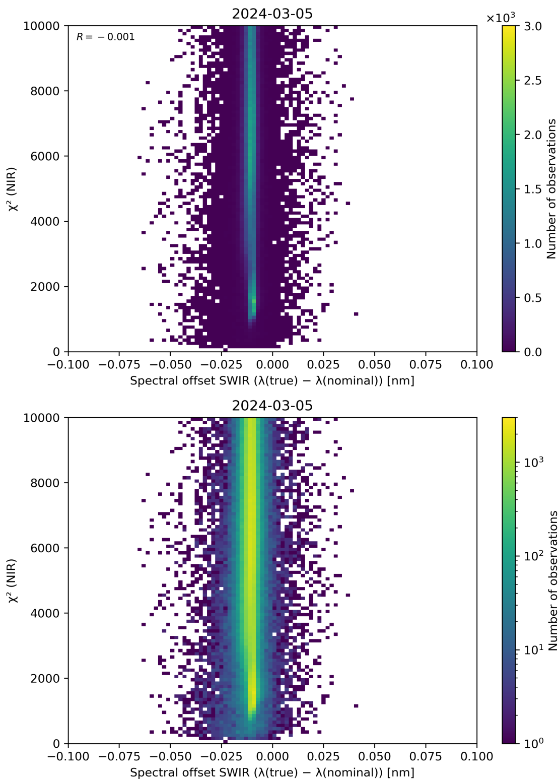
Figure 117: Scatter density plot of “Spectral offset SWIR ( \lambda(\text{true}) - \lambda(\text{nominal}) )” against “ \chi^2 (NIR)” for 2024-03-04 to 2024-03-06.
