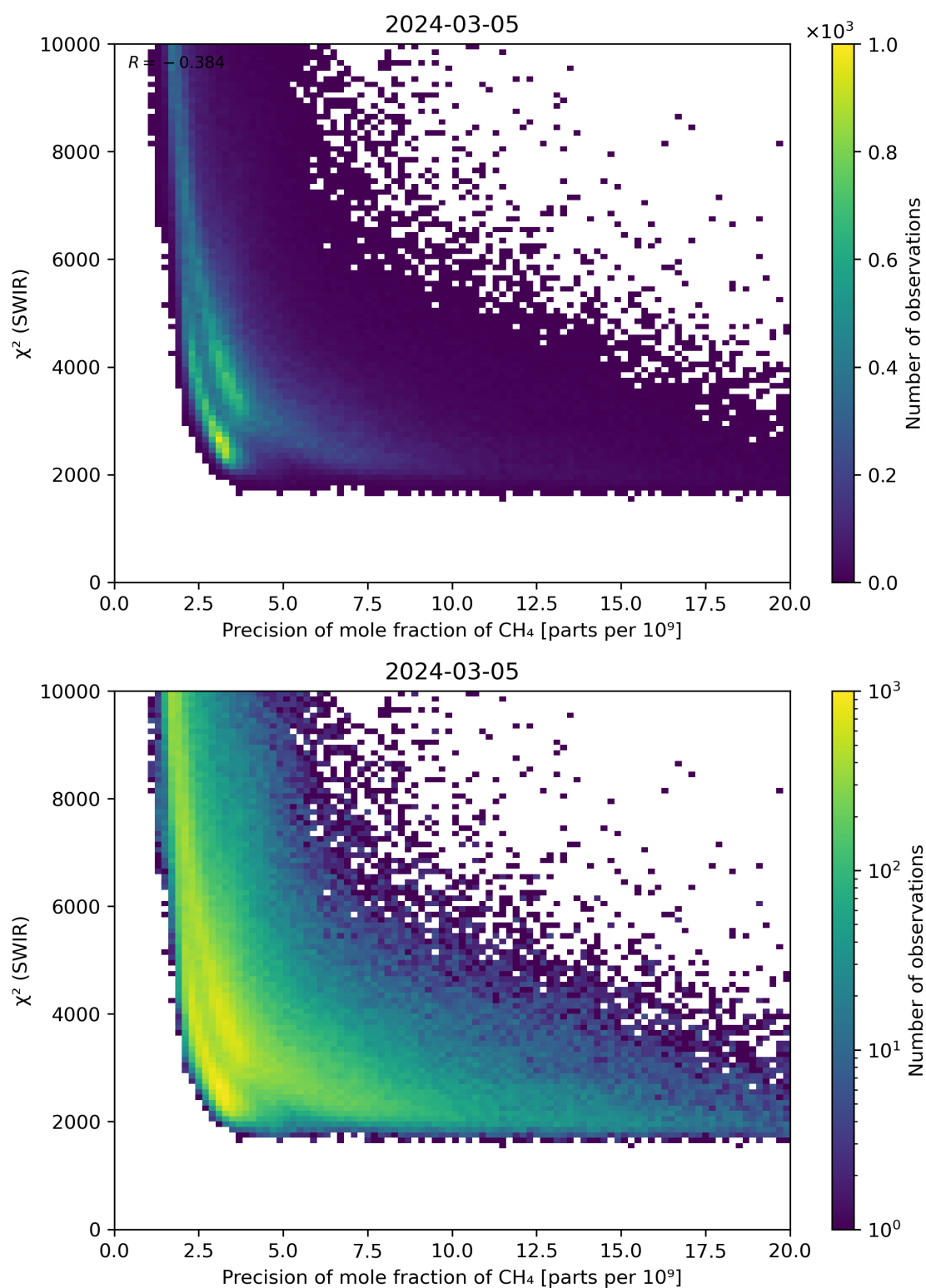
Figure 79: Scatter density plot of “Precision of mole fraction of CH 4 ” against “ \chi^2 (SWIR)” for 2024-03-04 to 2024-03-06.
