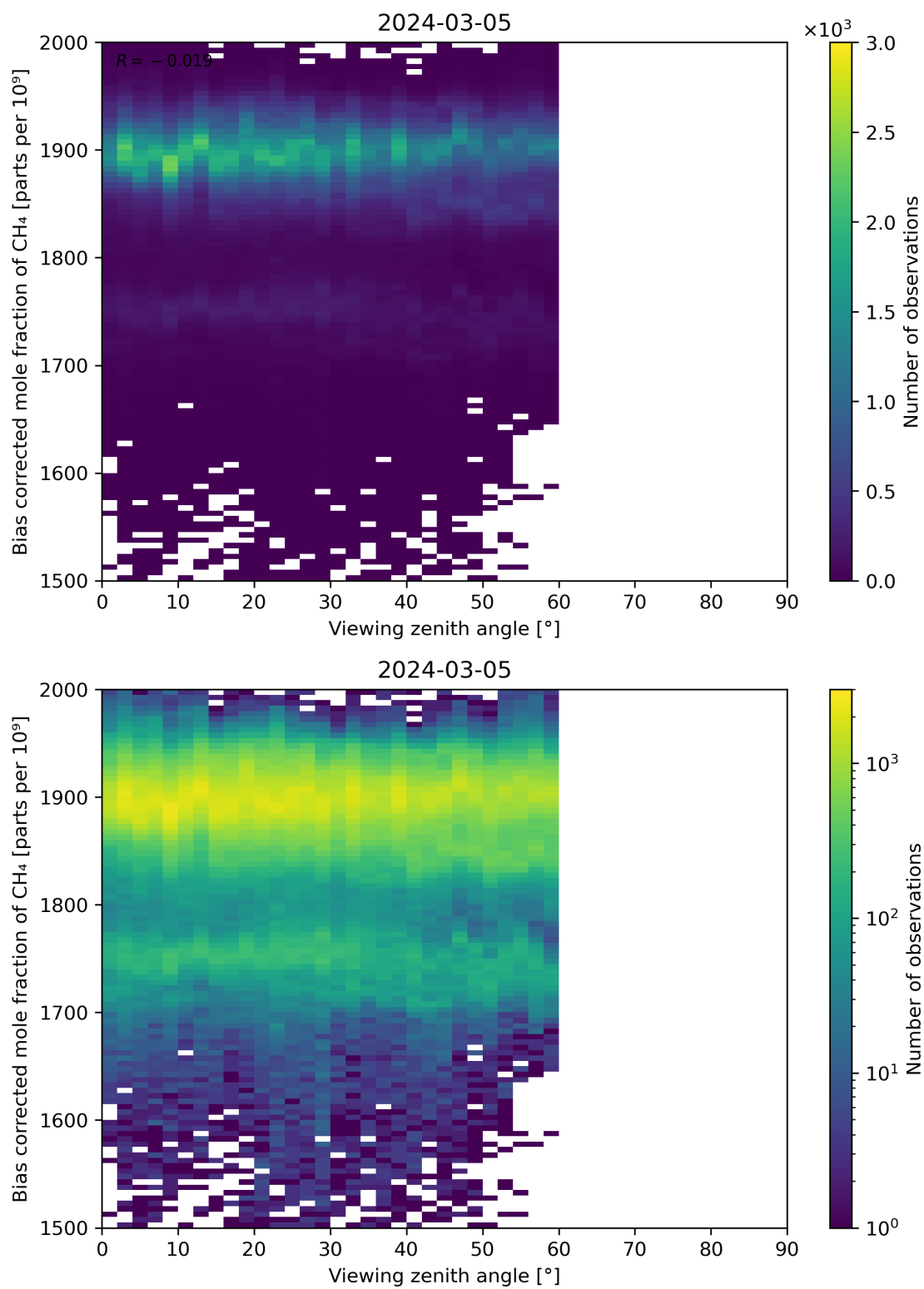
Figure 111: Scatter density plot of “Viewing zenith angle” against “Bias corrected mole fraction of CH 4 ” for 2024-03-04 to 2024-03-06.
