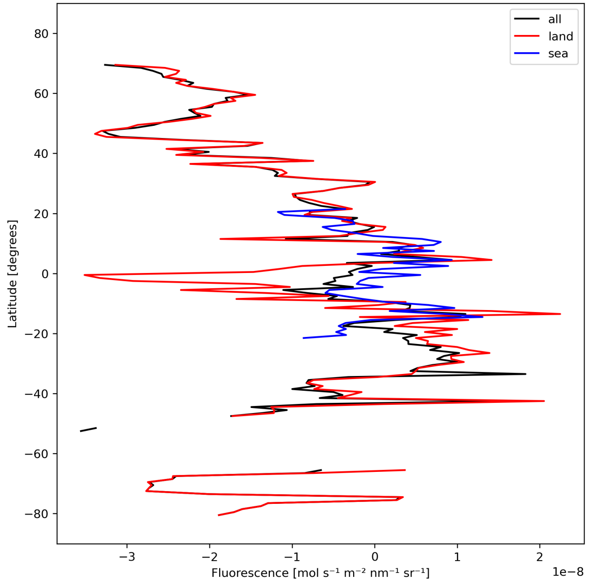
Figure 21: Zonal average of “Fluorescence” for 2024-03-04 to 2024-03-06.
