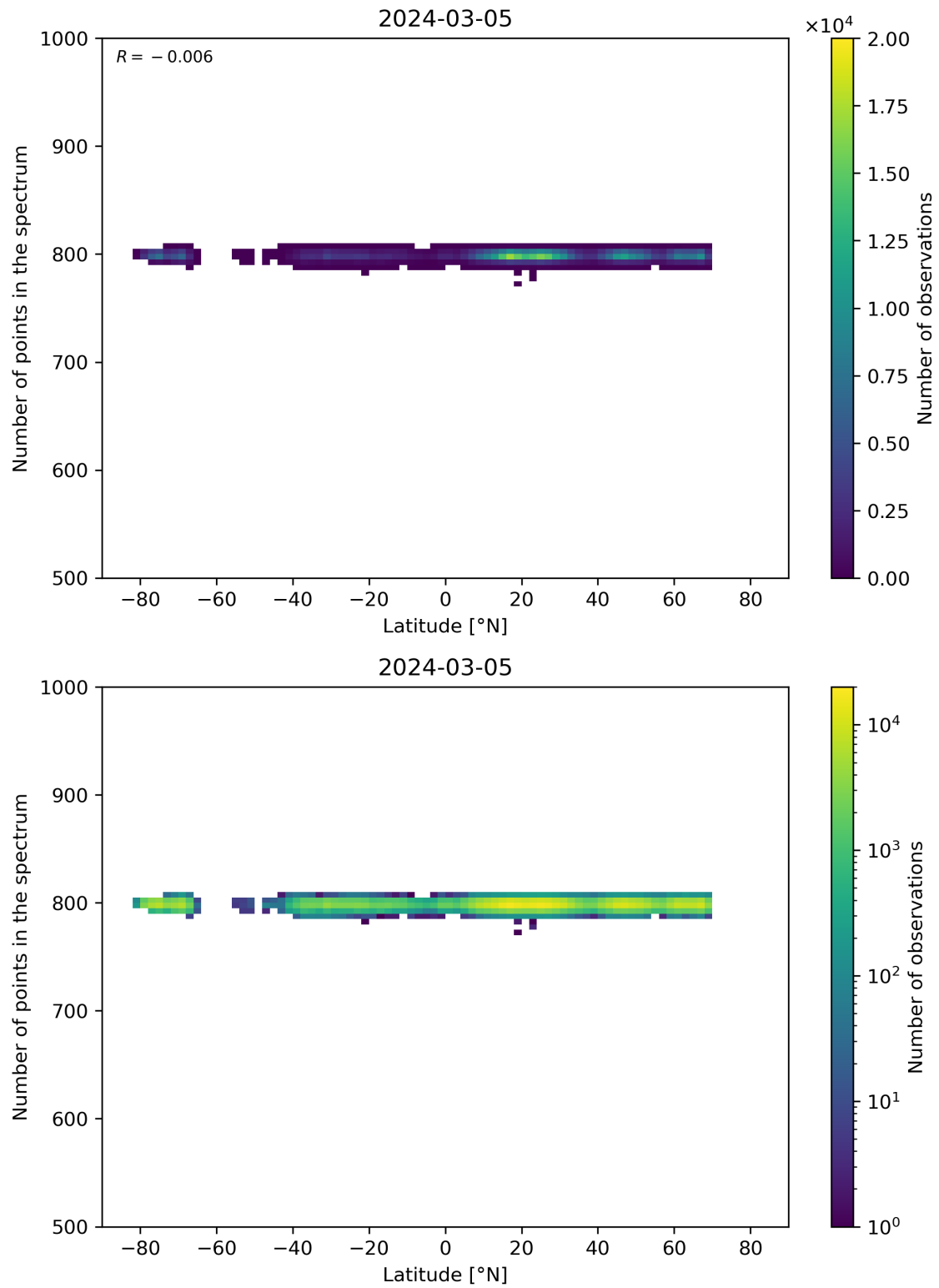
Figure 61: Scatter density plot of “Latitude” against “Number of points in the spectrum” for 2024-03-04 to 2024-03-06.
