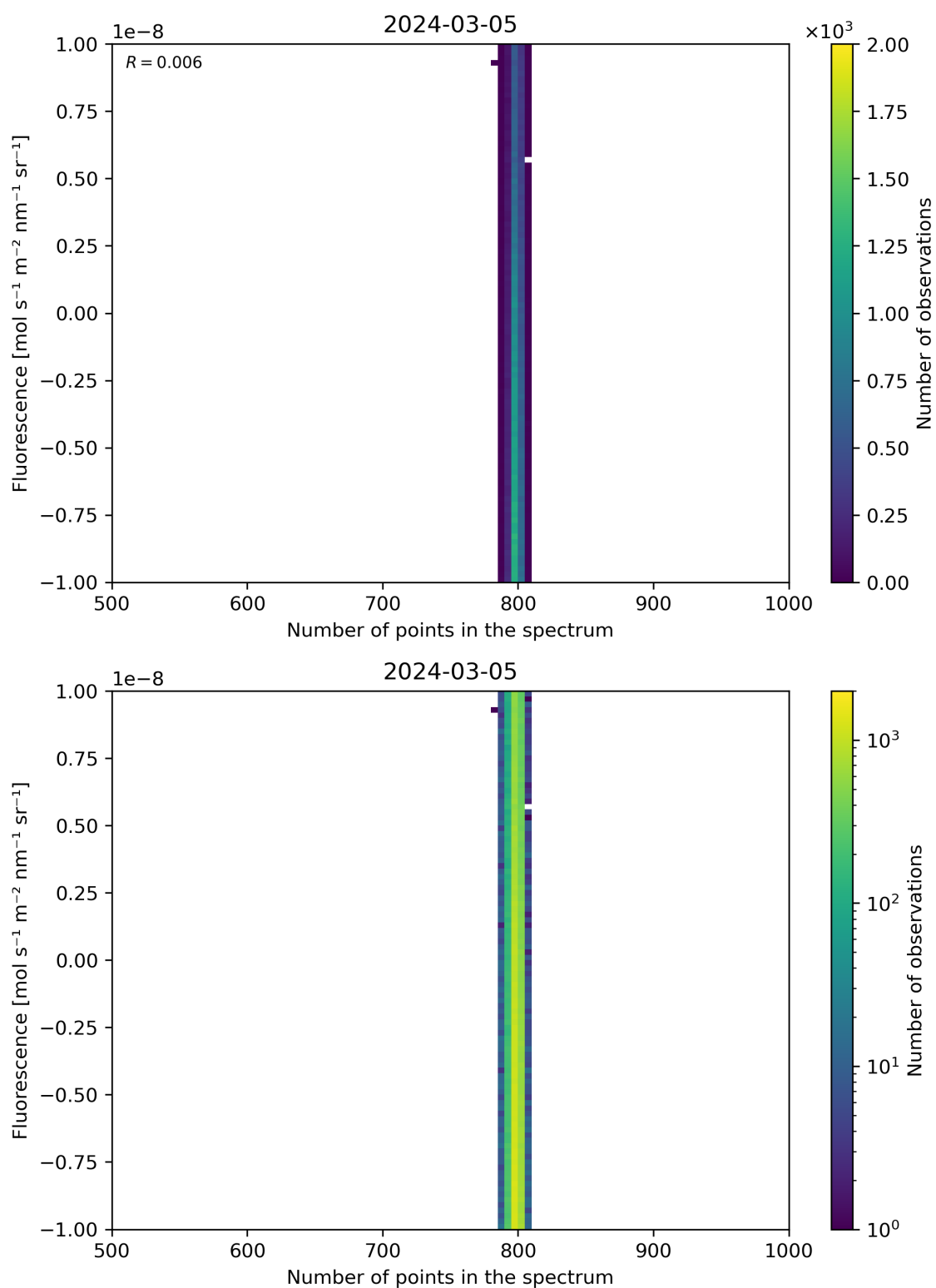
Figure 91: Scatter density plot of “Number of points in the spectrum” against “Fluorescence” for 2024-03-04 to 2024-03-06.
