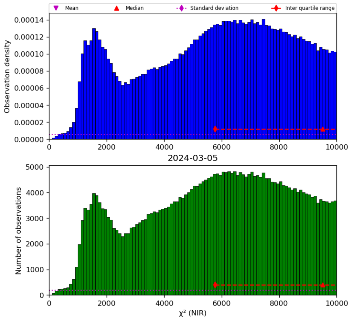
Figure 29: Histogram of “ \chi^2 (NIR)” for 2024-03-04 to 2024-03-06
