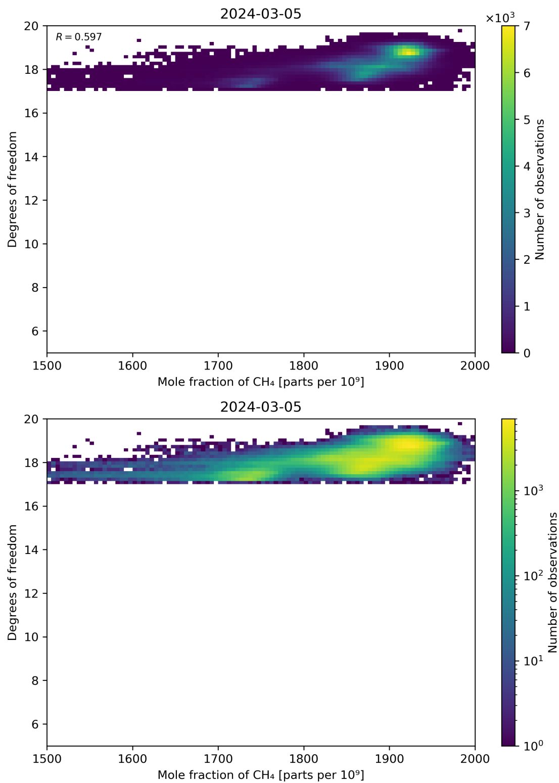
Figure 72: Scatter density plot of “Mole fraction of CH 4 ” against “Degrees of freedom” for 2024-03-04 to 2024-03-06.
