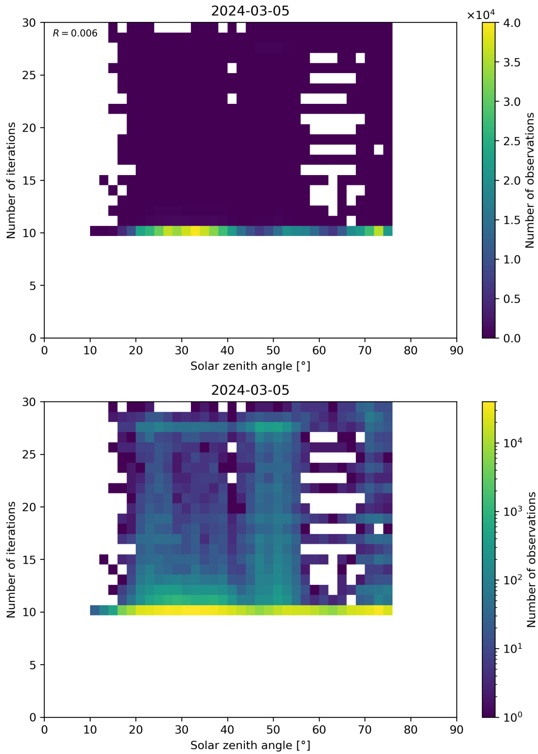
Figure 102: Scatter density plot of “Solar zenith angle” against “Number of iterations” for 2024-03-04 to 2024-03-06.
