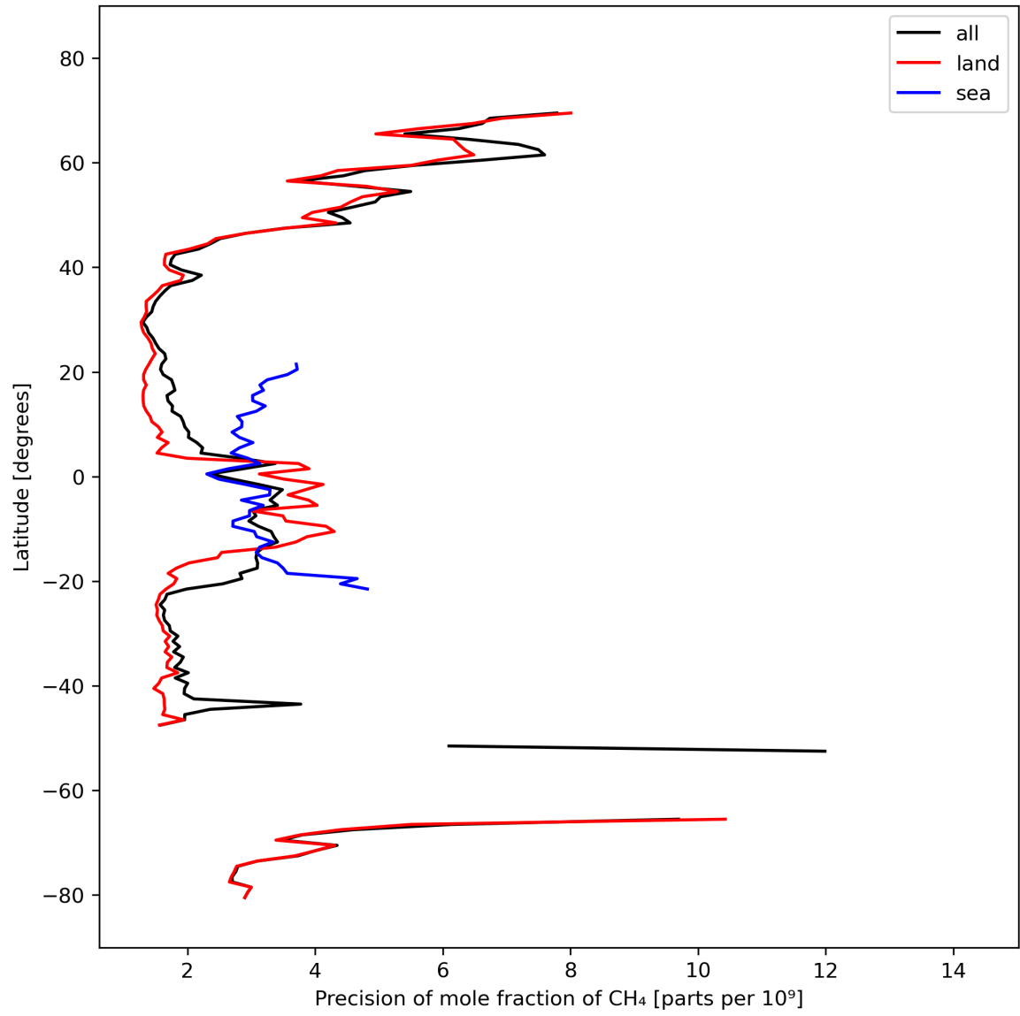
Figure 13: Zonal average of “Precision of mole fraction of CH 4 ” for 2024-03-04 to 2024-03-06.
