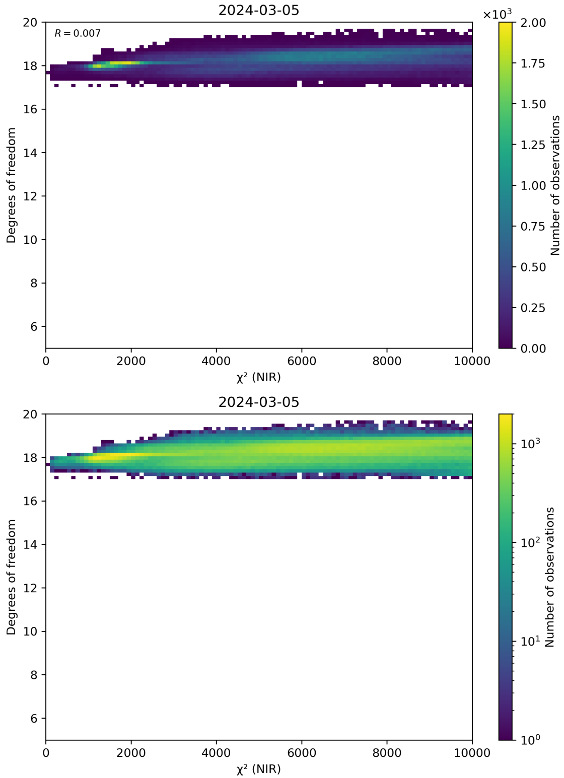
Figure 44: Scatter density plot of “ \chi^2 (NIR)” against “Degrees of freedom” for 2024-03-04 to 2024-03-06.
