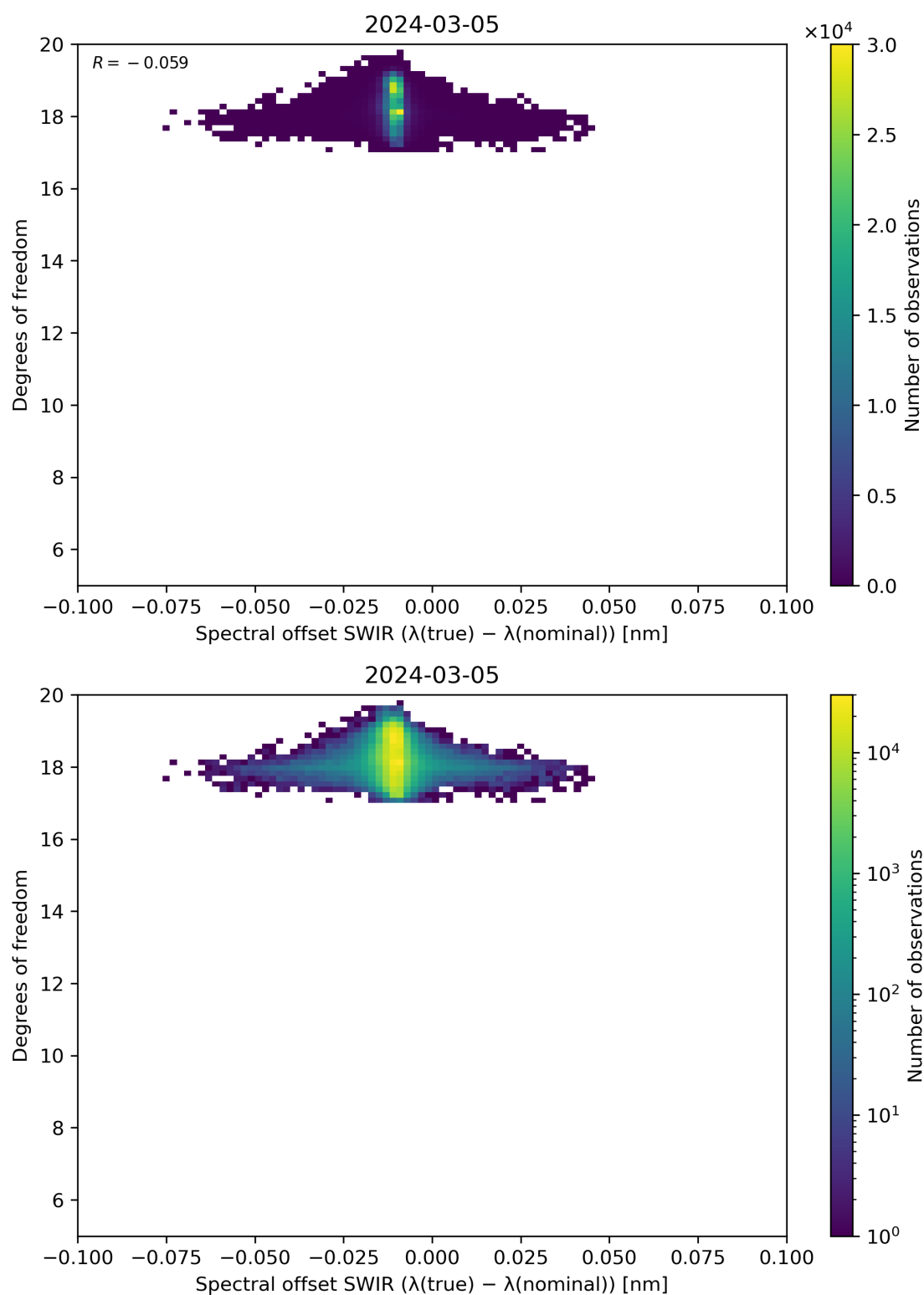
Figure 119: Scatter density plot of “Spectral offset SWIR ( \lambda(\text{true}) - \lambda(\text{nominal}) )” against “Degrees of freedom” for 2024-03-04 to 2024-03-06.
