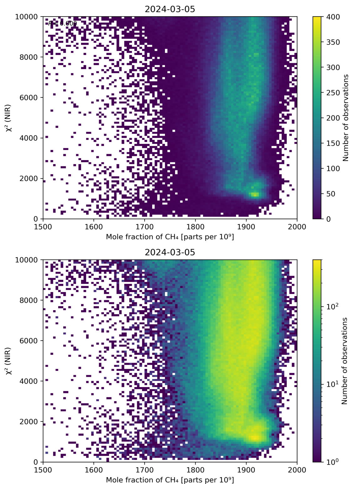
Figure 70: Scatter density plot of “Mole fraction of CH 4 ” against “ \chi^2 (NIR)” for 2024-03-04 to 2024-03-06.
