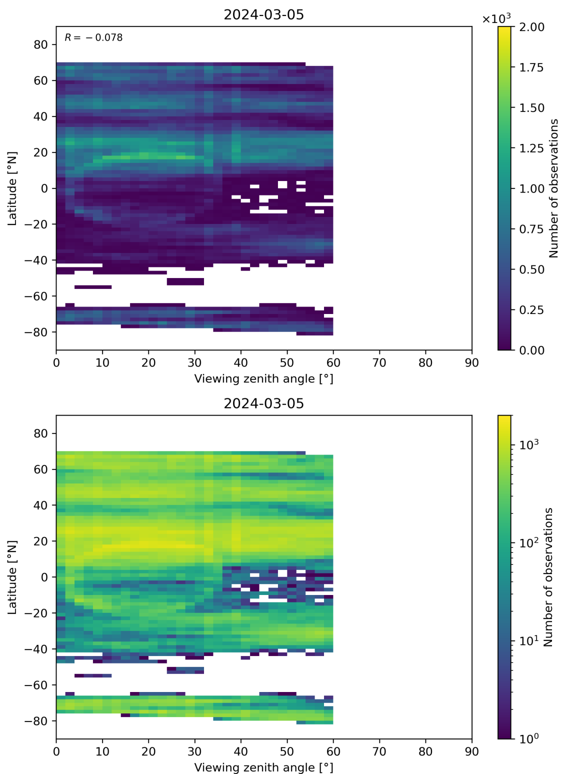
Figure 109: Scatter density plot of “Viewing zenith angle” against “Latitude” for 2024-03-04 to 2024-03-06.
