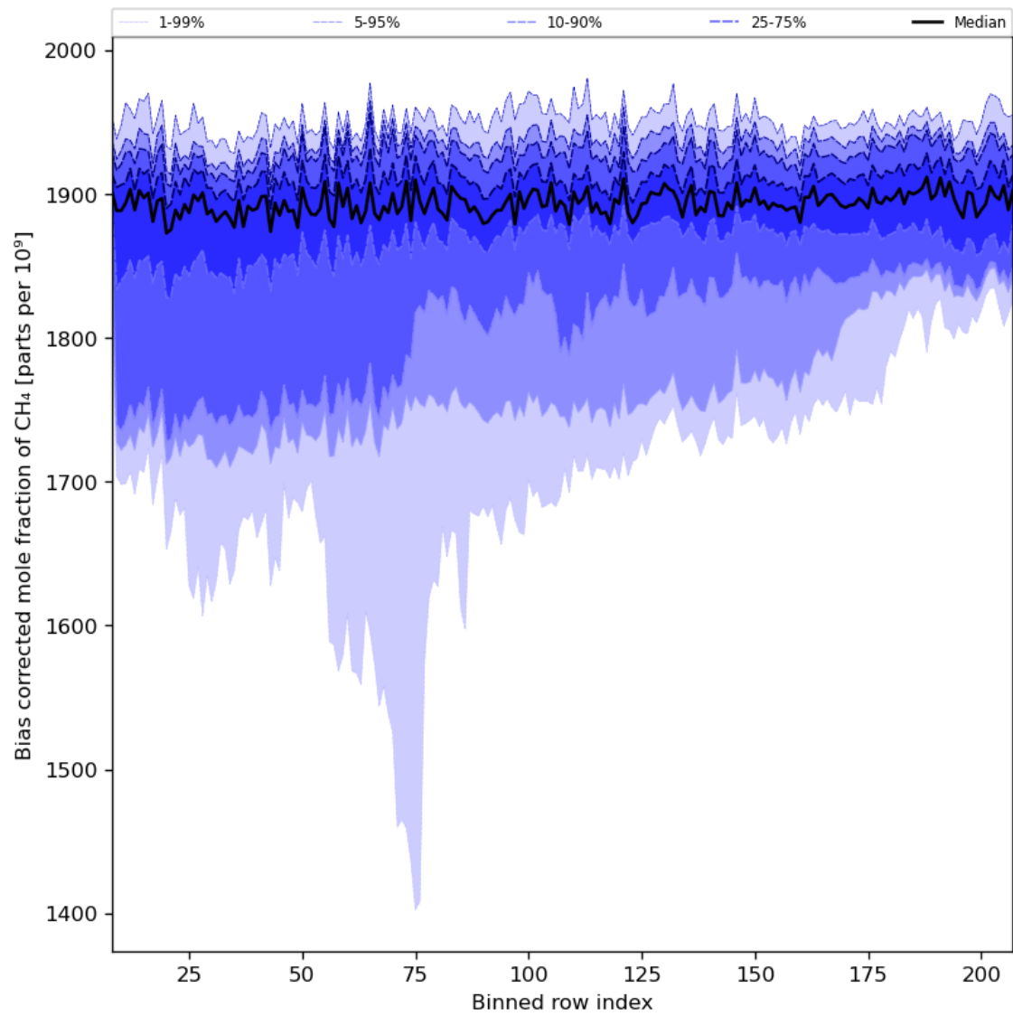
Figure 36: Along track statistics of “Bias corrected mole fraction of CH 4 ” for 2024-03-04 to 2024-03-06
