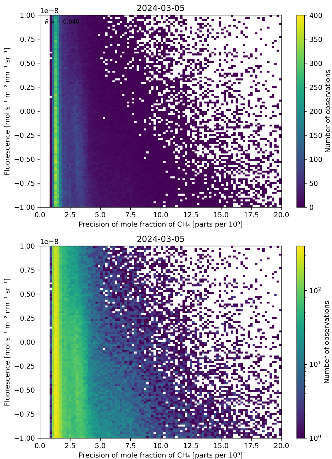
Figure 81: Scatter density plot of “Precision of mole fraction of \text{CH}_4 ” against “Fluorescence” for 2024-03-04 to 2024-03-06.
