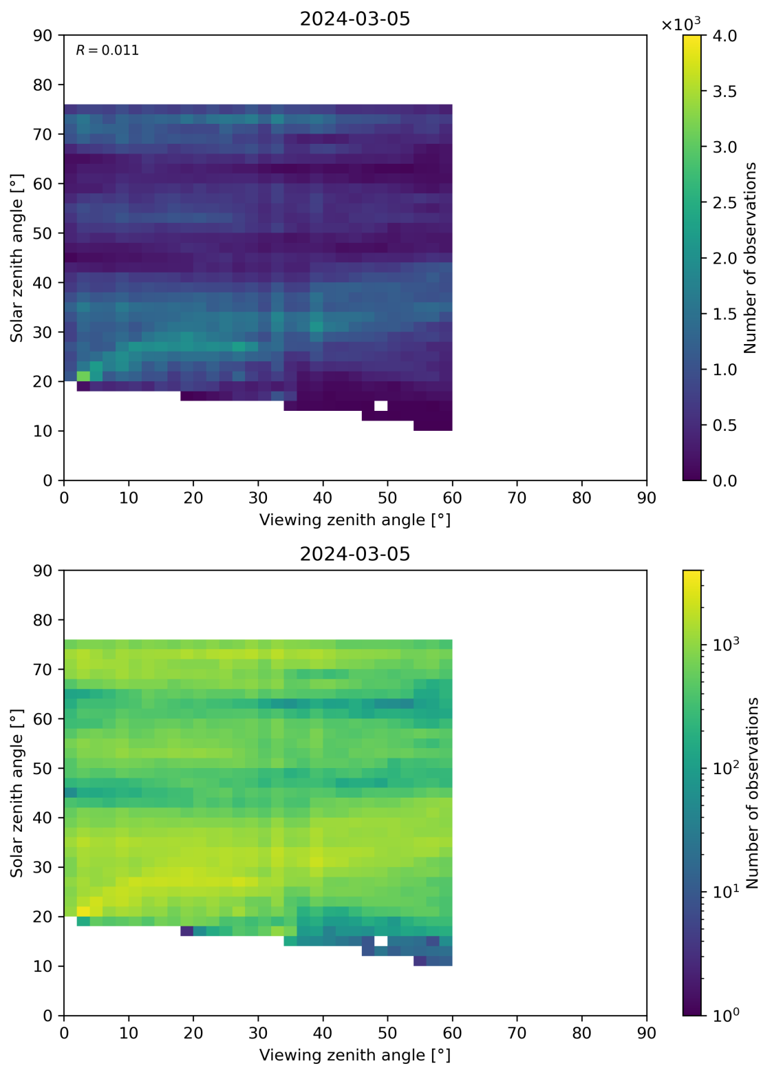
Figure 115: Scatter density plot of “Viewing zenith angle” against “Solar zenith angle” for 2024-03-04 to 2024-03-06.
