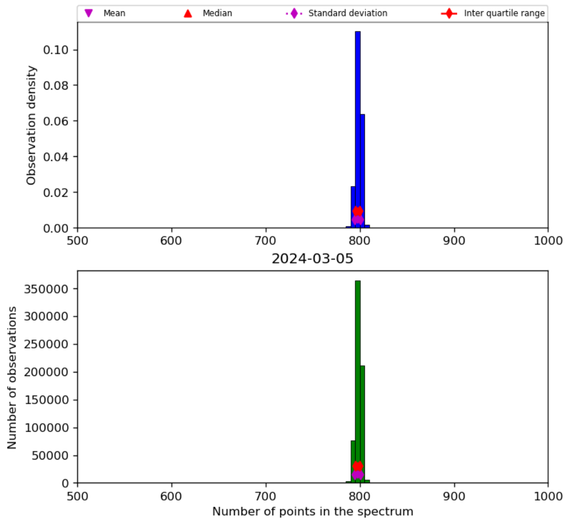
Figure 26: Histogram of “Number of points in the spectrum” for 2024-03-04 to 2024-03-06
