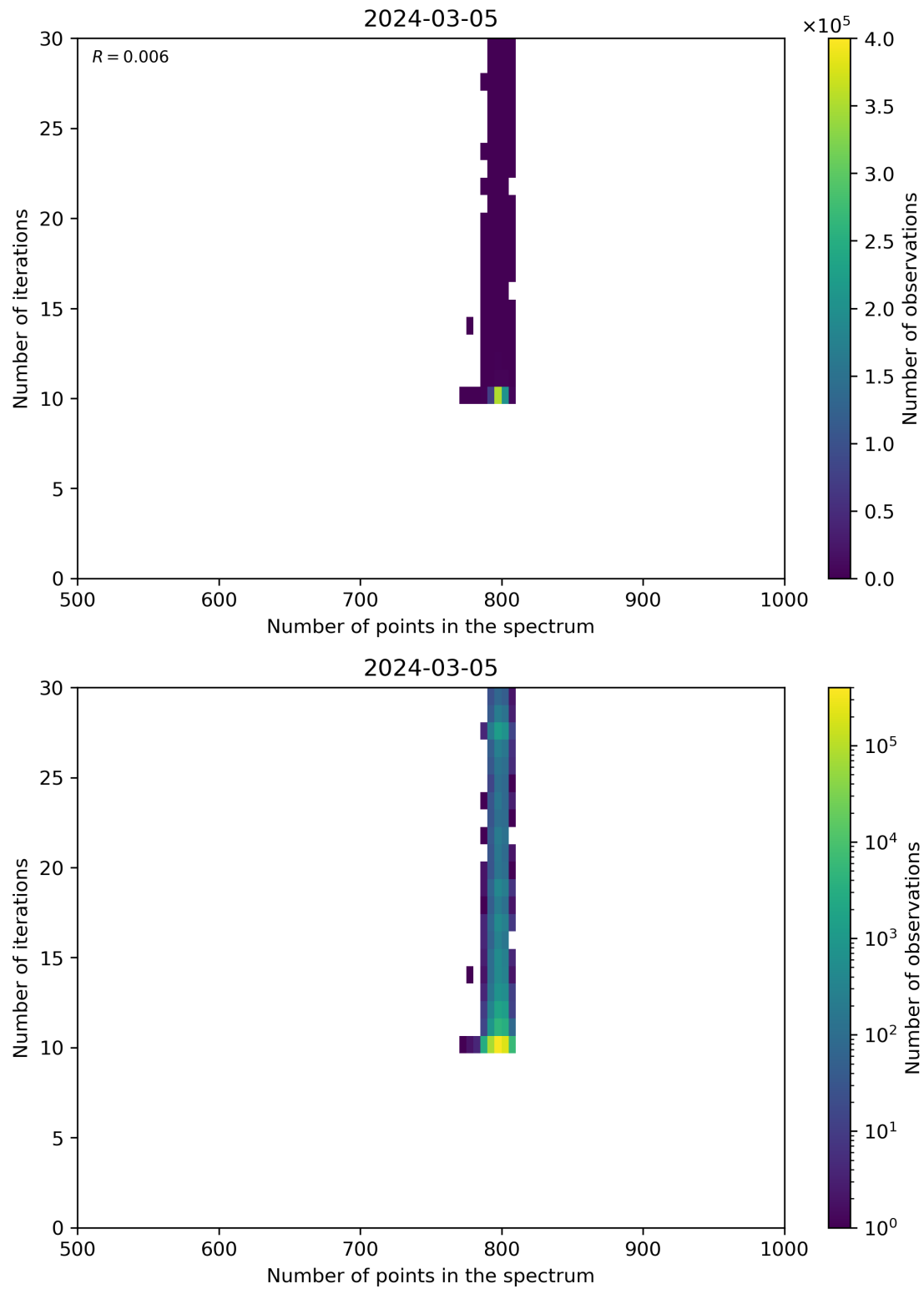
Figure 92: Scatter density plot of “Number of points in the spectrum” against “Number of iterations” for 2024-03-04 to 2024-03-06.
