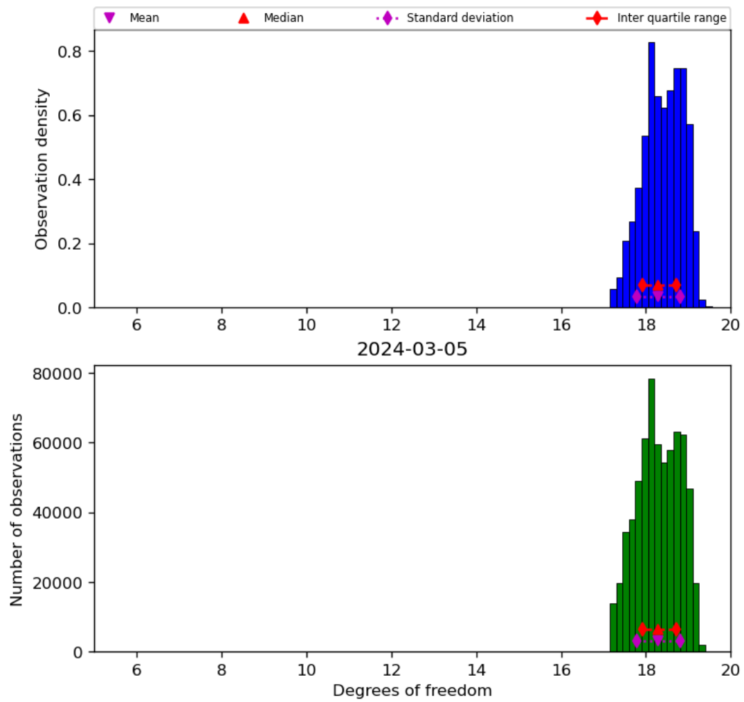
Figure 30: Histogram of “Degrees of freedom” for 2024-03-04 to 2024-03-06
