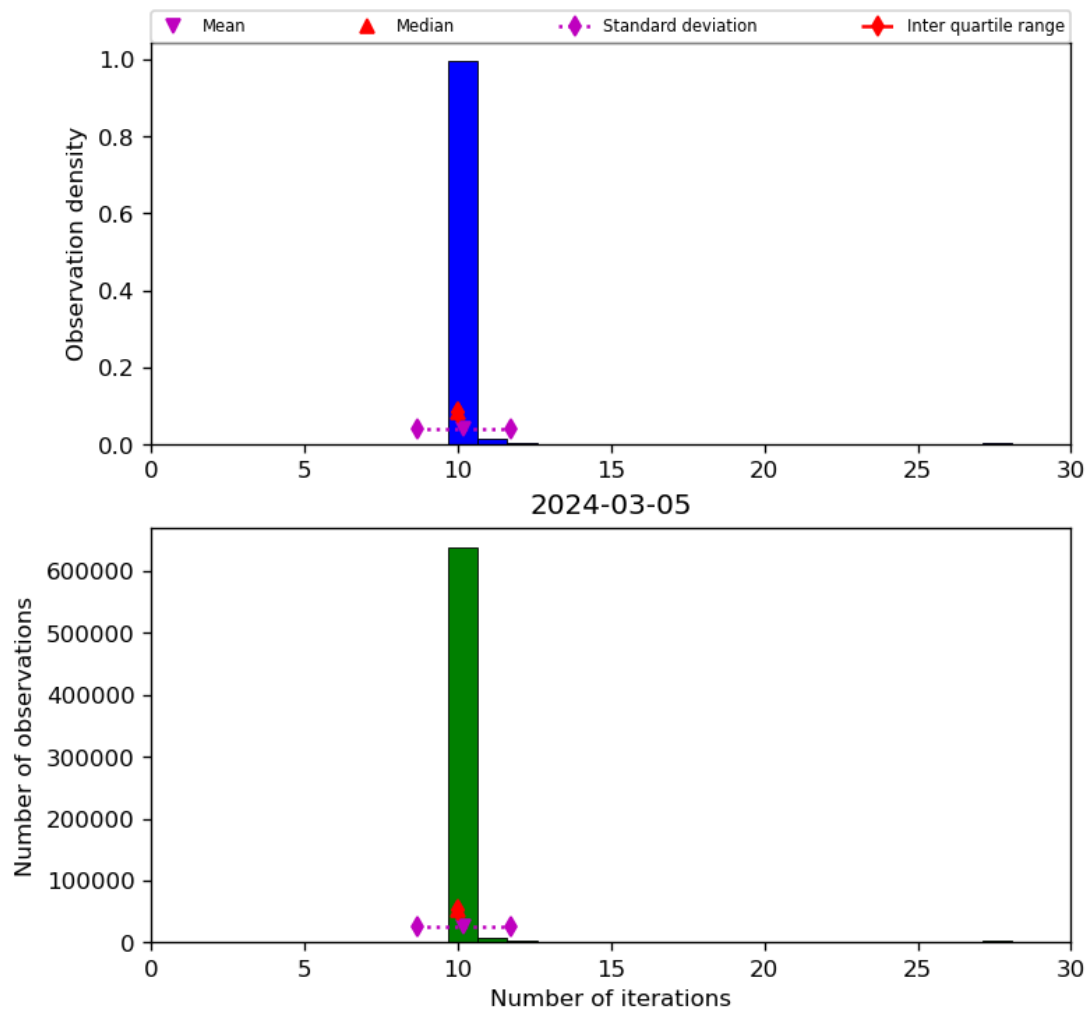
Figure 31: Histogram of “Number of iterations” for 2024-03-04 to 2024-03-06
