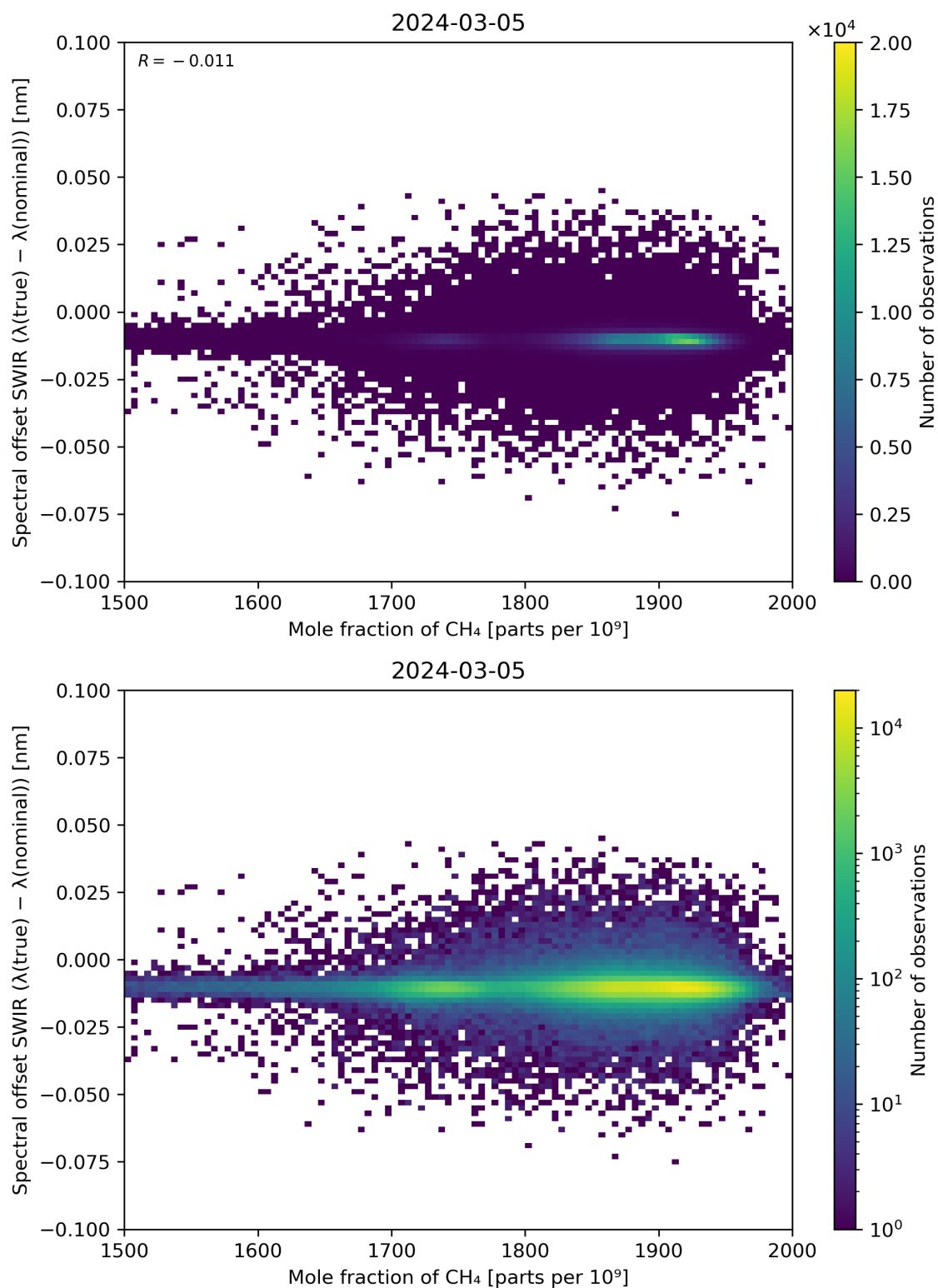
Figure 86: Scatter density plot of “Mole fraction of CH 4 ” against “Spectral offset SWIR ( \lambda(\text{true}) - \lambda(\text{nominal}) )” for 2024-03-04 to 2024-03-06.
