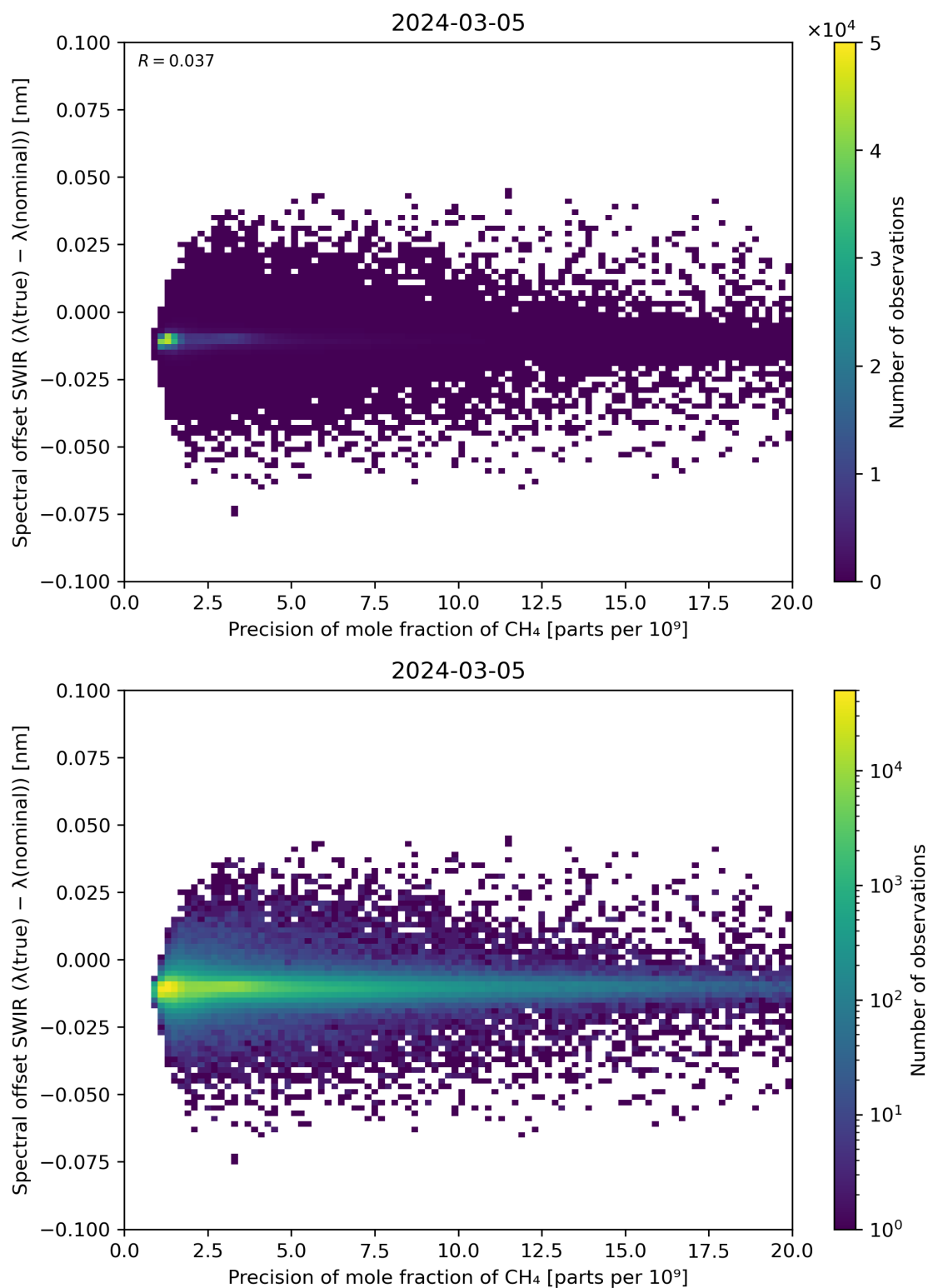
Figure 85: Scatter density plot of “Precision of mole fraction of CH 4 ” against “Spectral offset SWIR ( \lambda(\text{true}) - \lambda(\text{nominal}) )” for 2024-03-04 to 2024-03-06.
