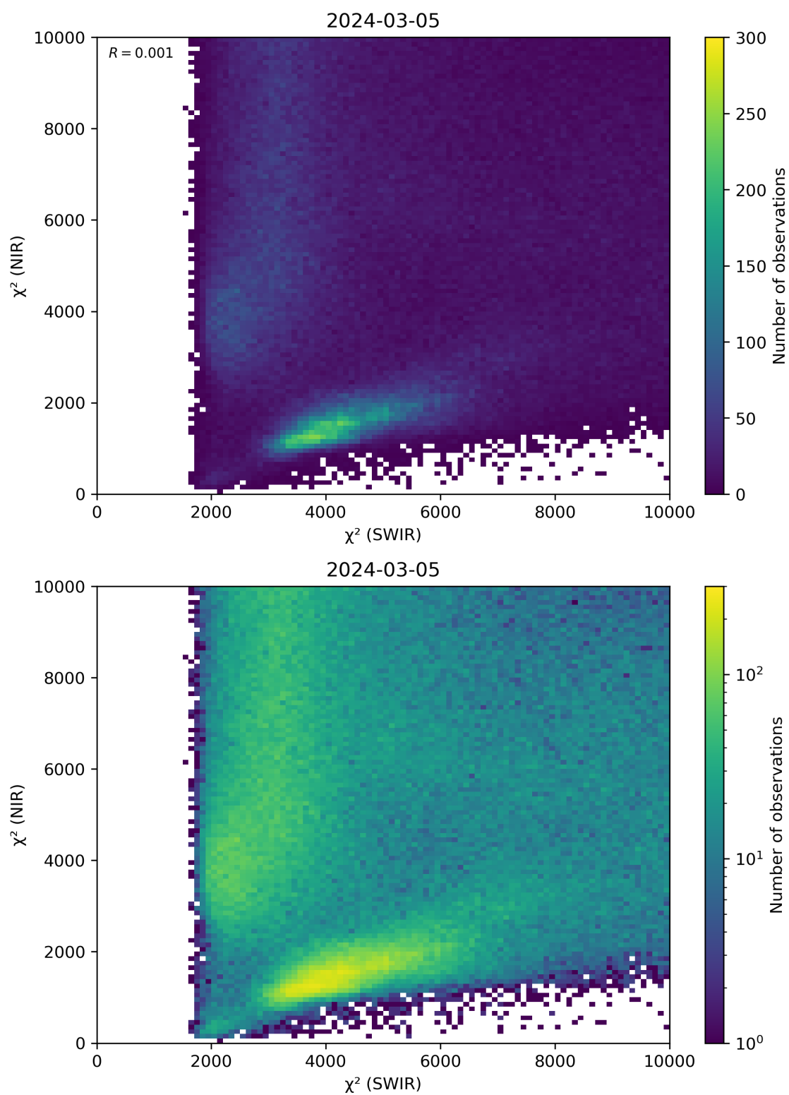
Figure 47: Scatter density plot of “ \chi^2 (SWIR)” against “ \chi^2 (NIR)” for 2024-03-04 to 2024-03-06.
