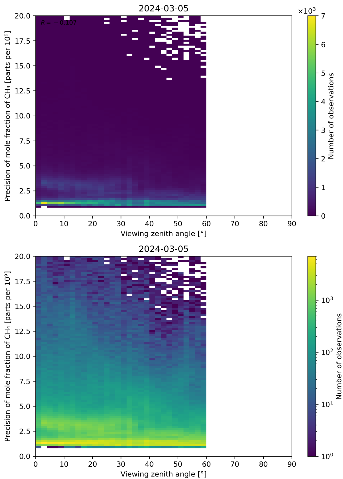
Figure 112: Scatter density plot of “Viewing zenith angle” against “Precision of mole fraction of CH 4 ” for 2024-03-04 to 2024-03-06.
