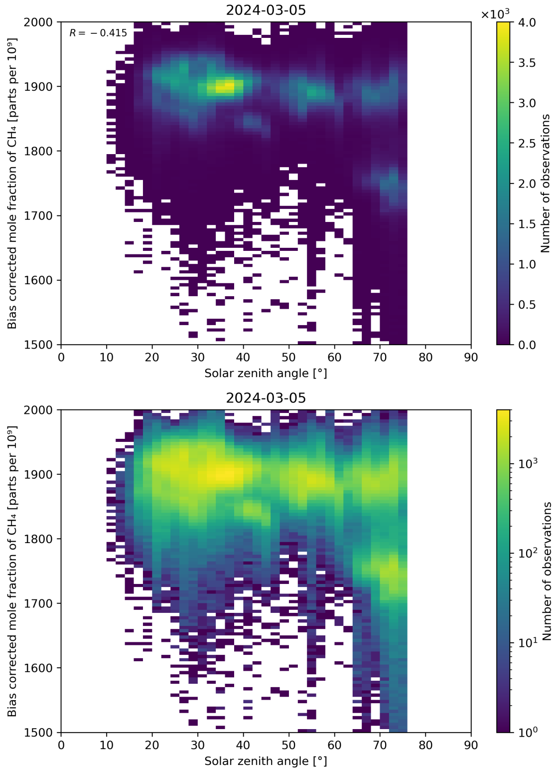
Figure 100: Scatter density plot of “Solar zenith angle” against “Bias corrected mole fraction of \text{CH}_4 ” for 2024-03-04 to 2024-03-06.
