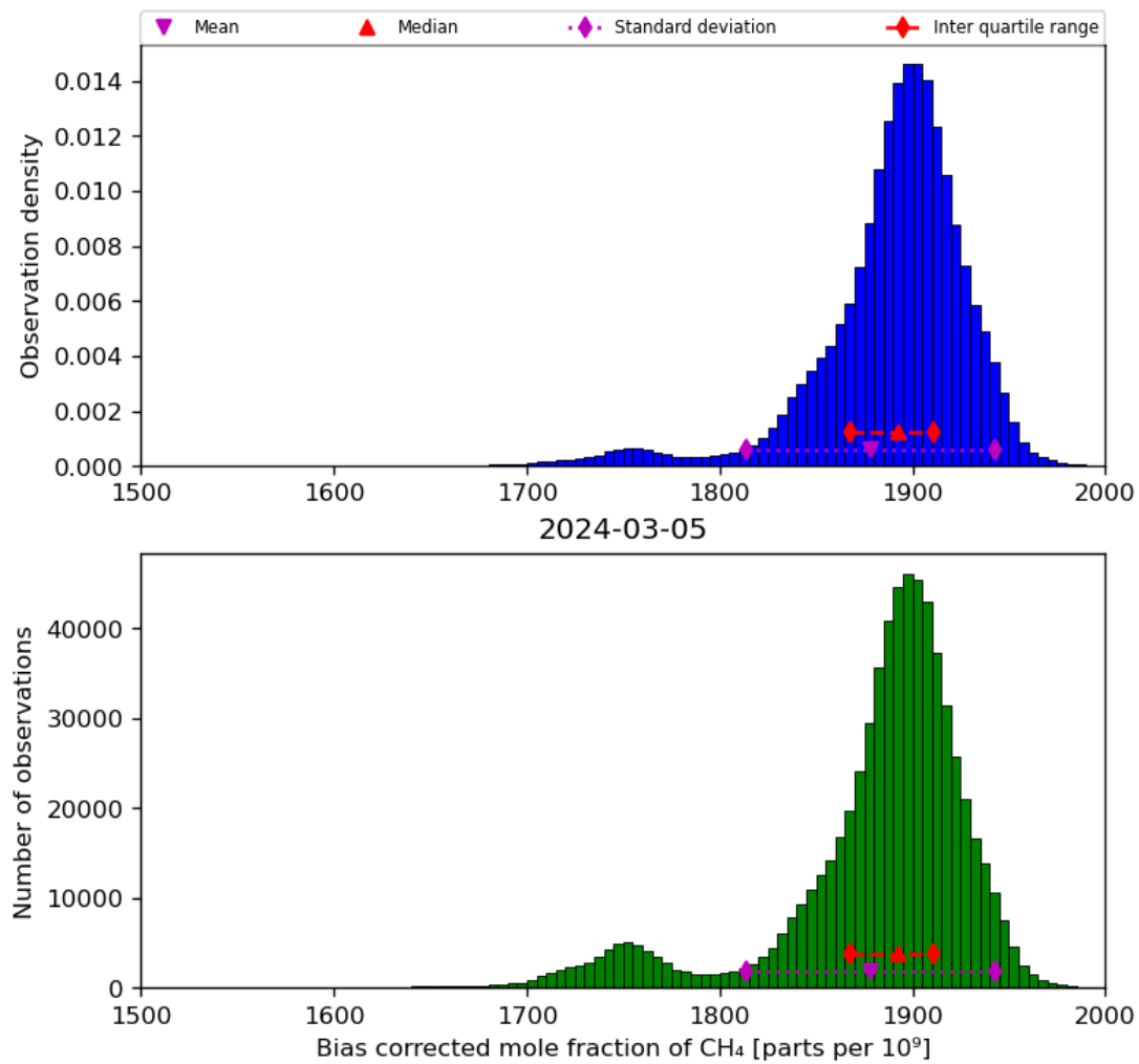
Figure 25: Histogram of “Bias corrected mole fraction of CH 4 ” for 2024-03-04 to 2024-03-06
