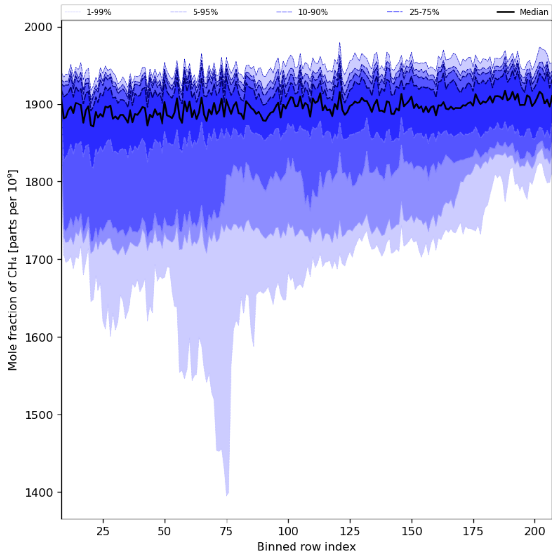
Figure 34: Along track statistics of “Mole fraction of CH 4 ” for 2024-03-04 to 2024-03-06
