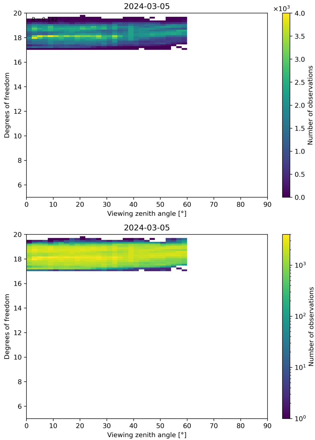
Figure 107: Scatter density plot of “Viewing zenith angle” against “Degrees of freedom” for 2024-03-04 to 2024-03-06.
