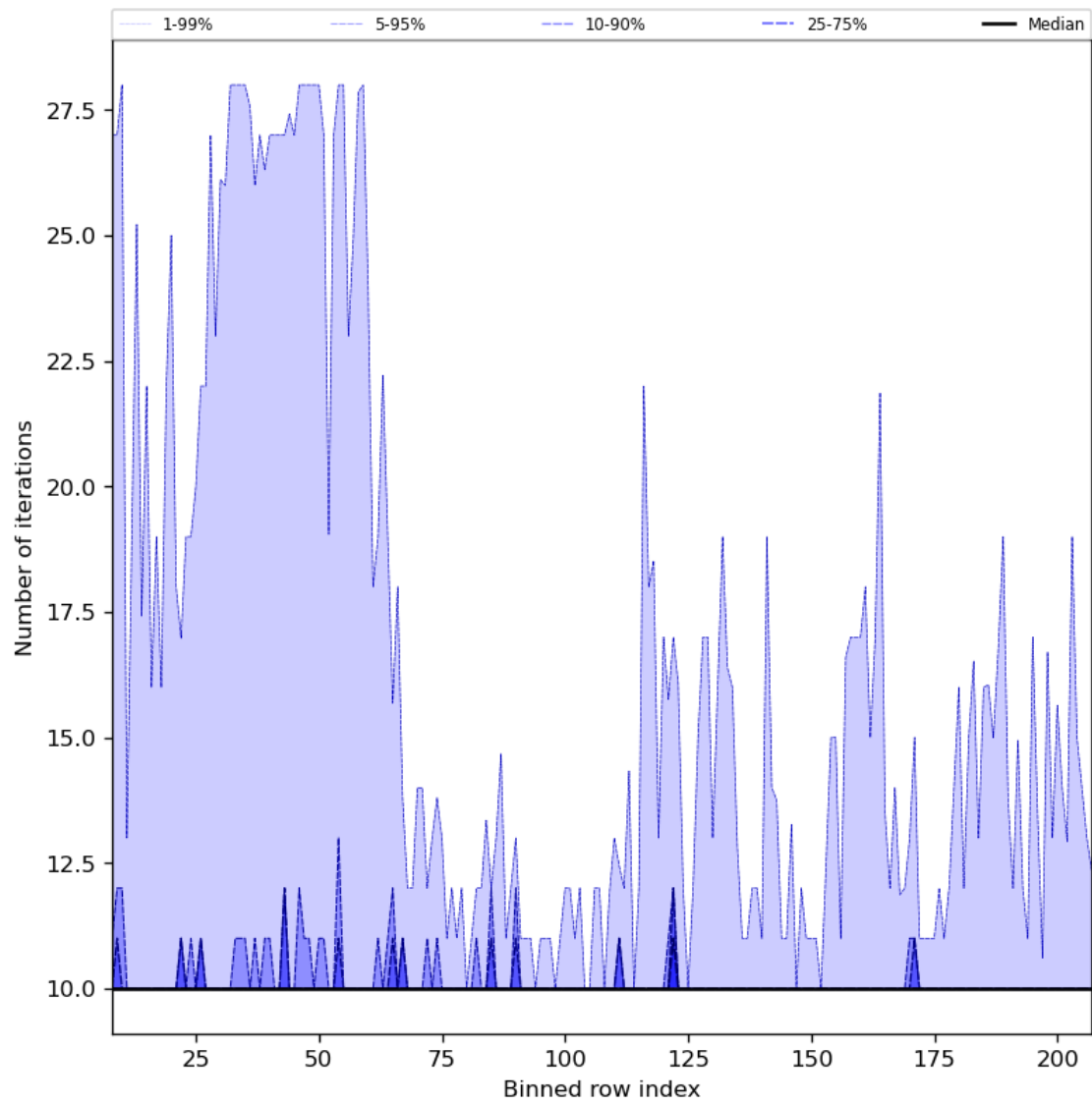
Figure 42: Along track statistics of “Number of iterations” for 2024-03-04 to 2024-03-06
