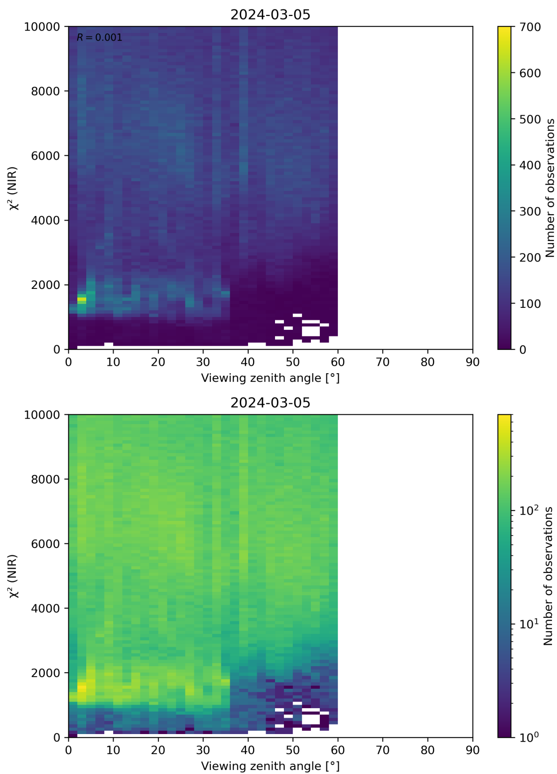
Figure 105: Scatter density plot of “Viewing zenith angle” against “ \chi^2 (NIR)” for 2024-03-04 to 2024-03-06.
