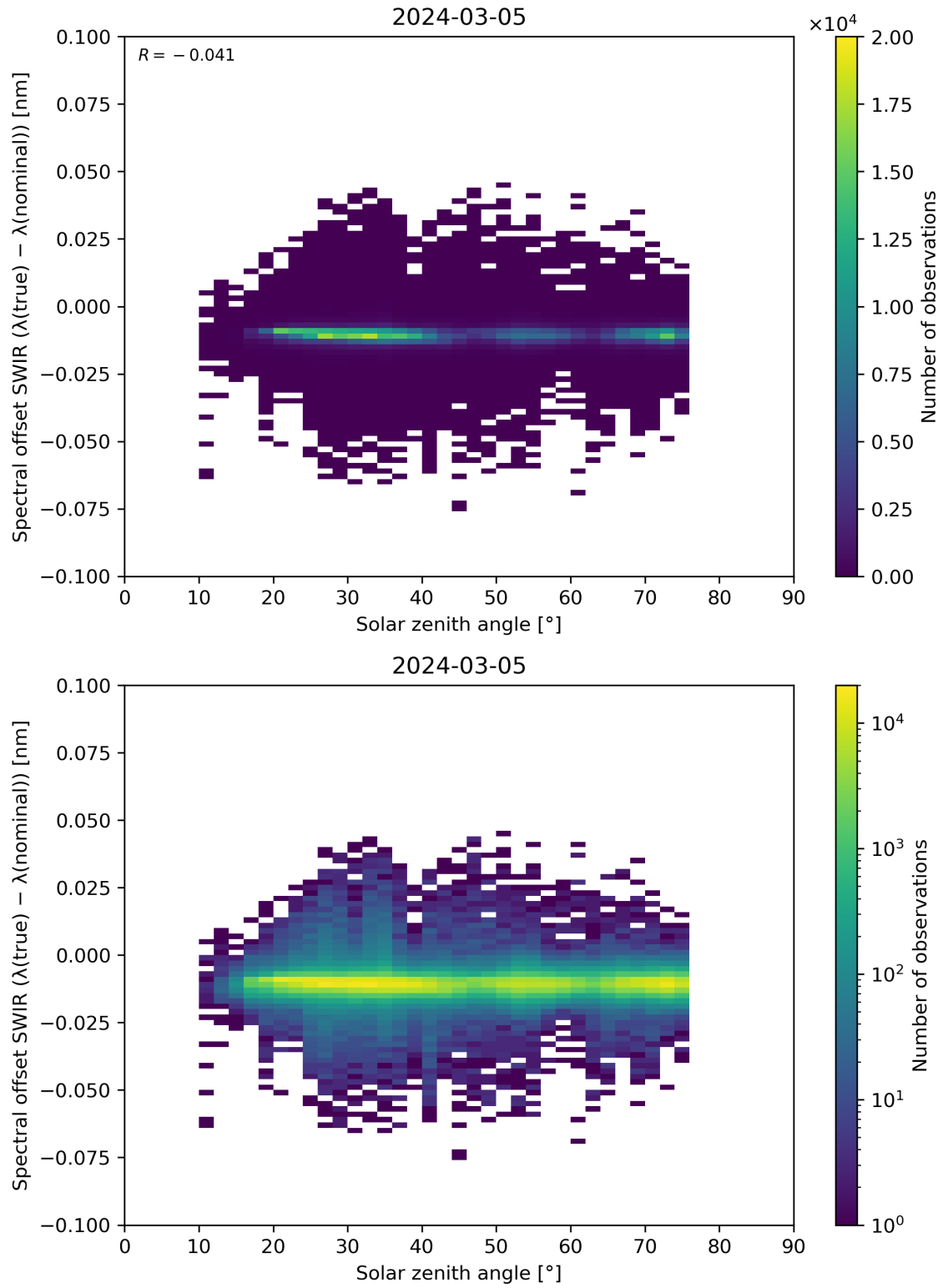
Figure 104: Scatter density plot of “Solar zenith angle” against “Spectral offset SWIR ( \lambda(\text{true}) - \lambda(\text{nominal}) )” for 2024-03-04 to 2024-03-06.
