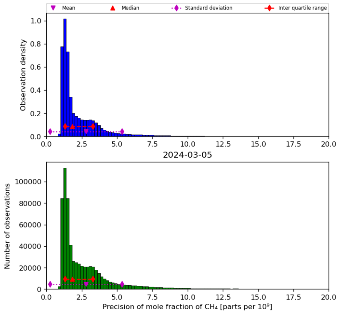
Figure 24: Histogram of “Precision of mole fraction of CH 4 ” for 2024-03-04 to 2024-03-06
