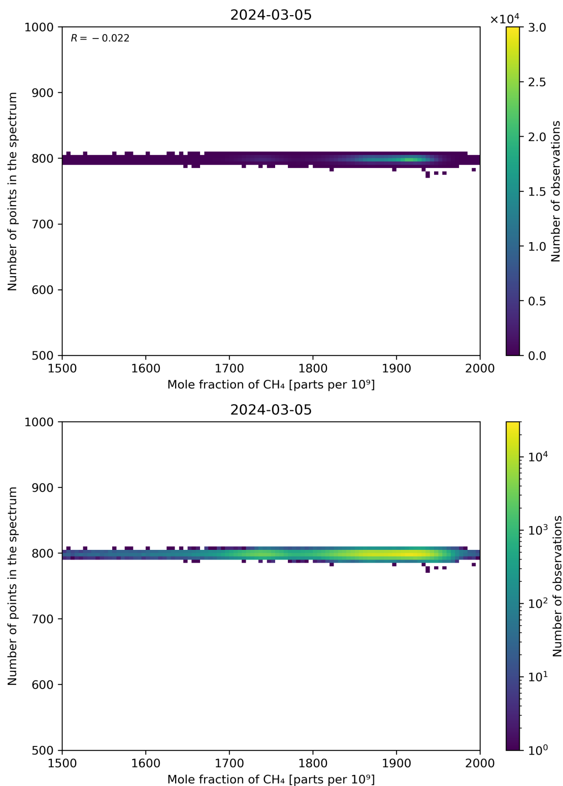
Figure 77: Scatter density plot of “Mole fraction of CH 4 ” against “Number of points in the spectrum” for 2024-03-04 to 2024-03-06.
