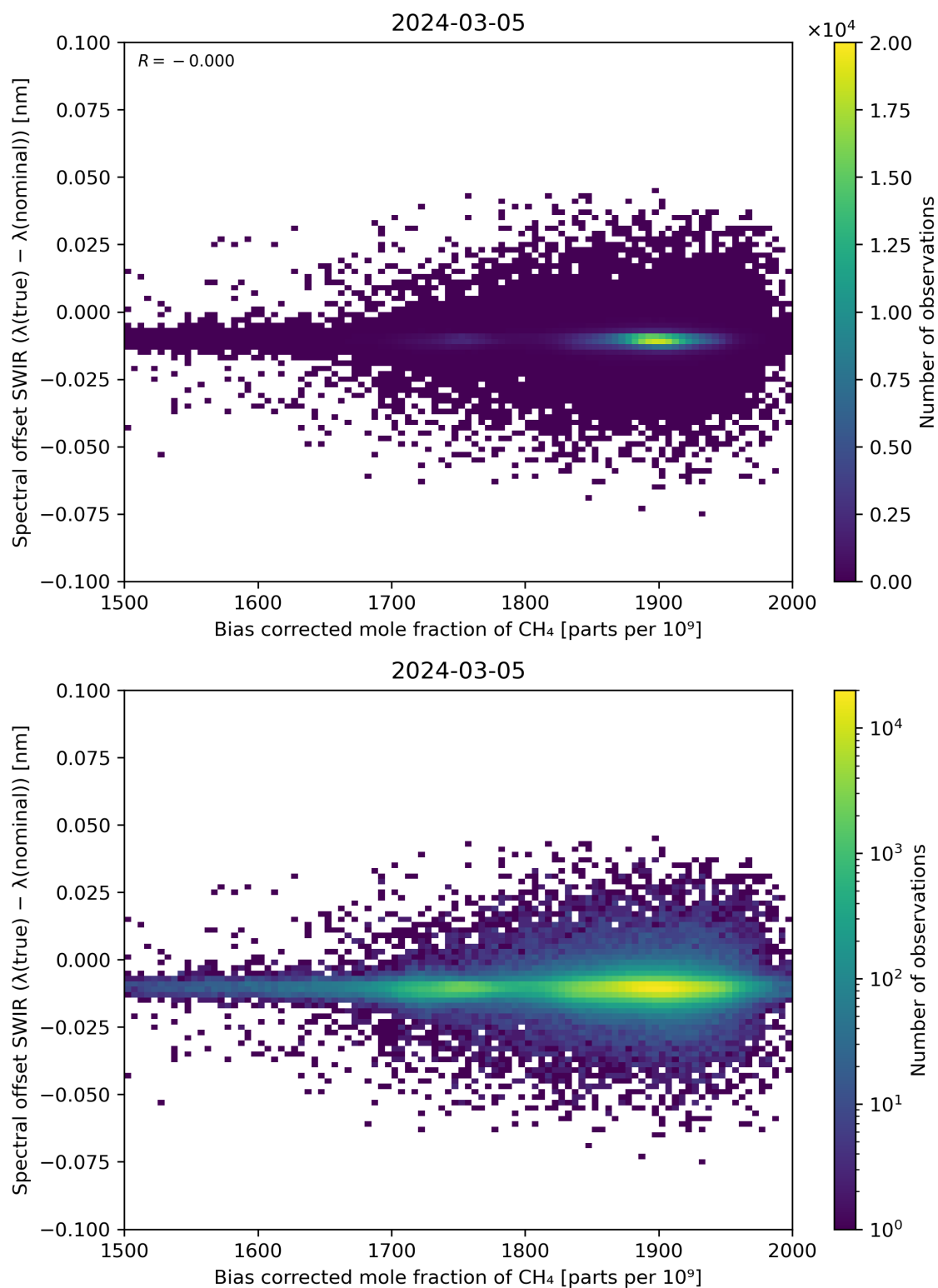
Figure 69: Scatter density plot of “Bias corrected mole fraction of \text{CH}_4 ” against “Spectral offset SWIR ( \lambda(\text{true}) - \lambda(\text{nominal}) )” for 2024-03-04 to 2024-03-06.
