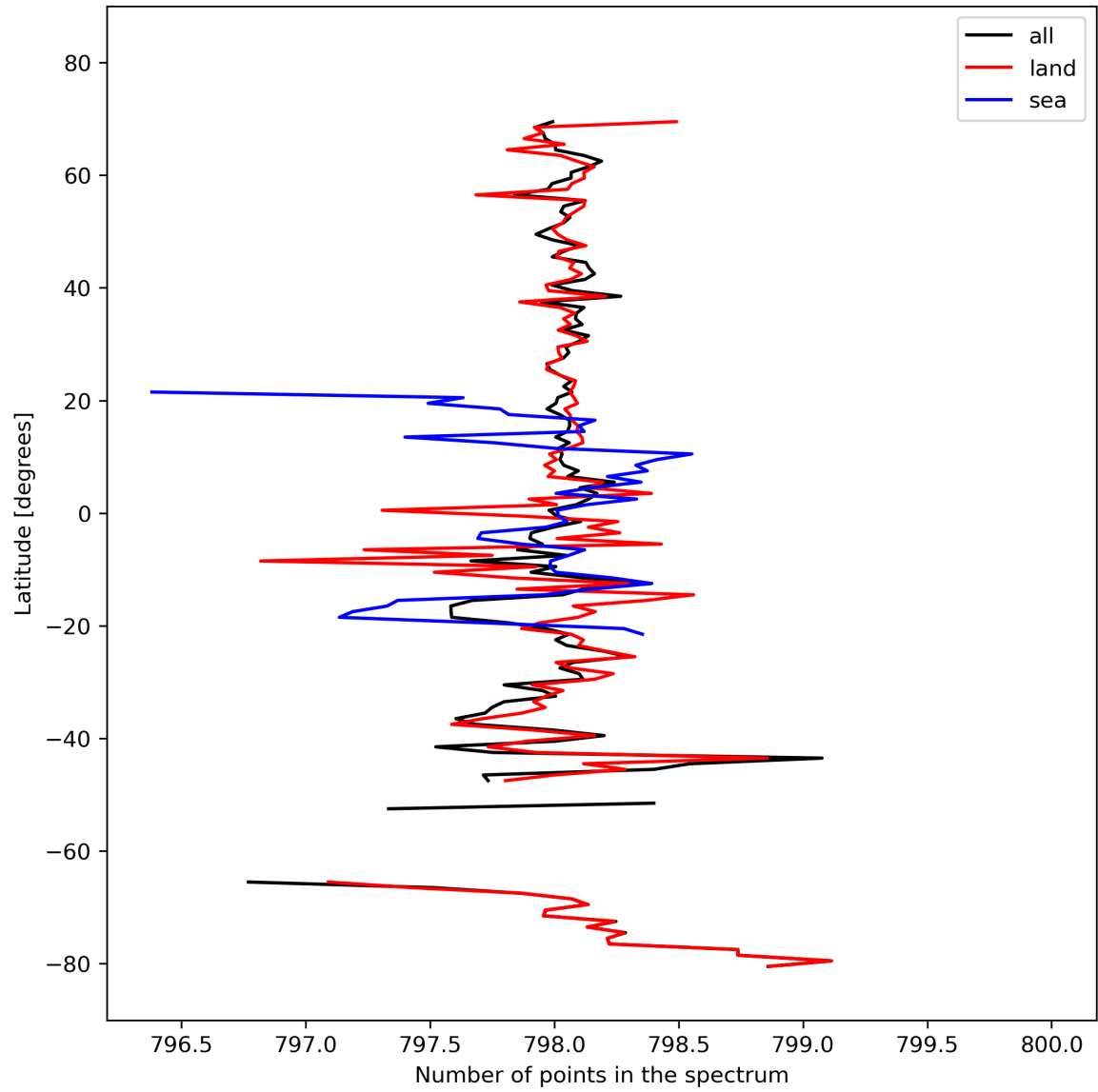
Figure 15: Zonal average of “Number of points in the spectrum” for 2024-03-04 to 2024-03-06.
