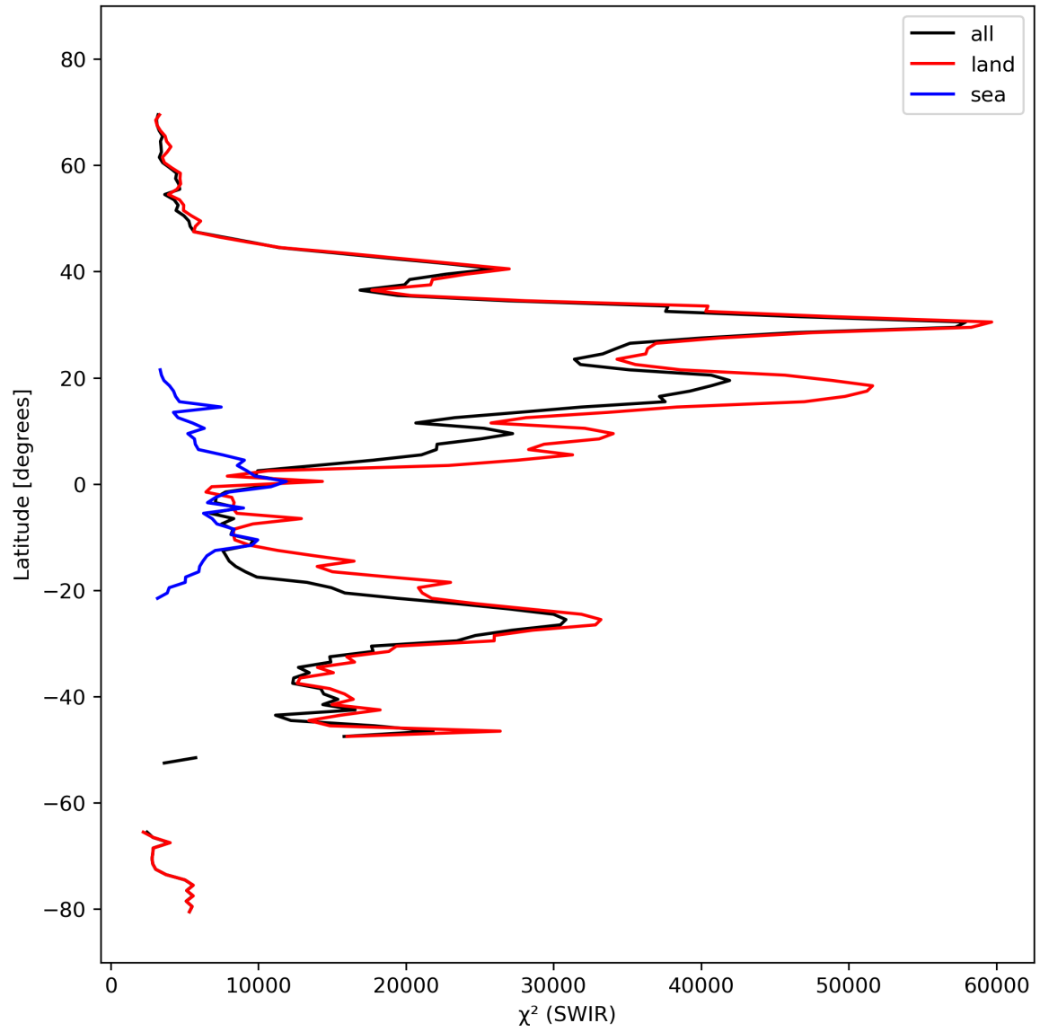
Figure 17: Zonal average of “ \chi^2 (SWIR)” for 2024-03-04 to 2024-03-06.
