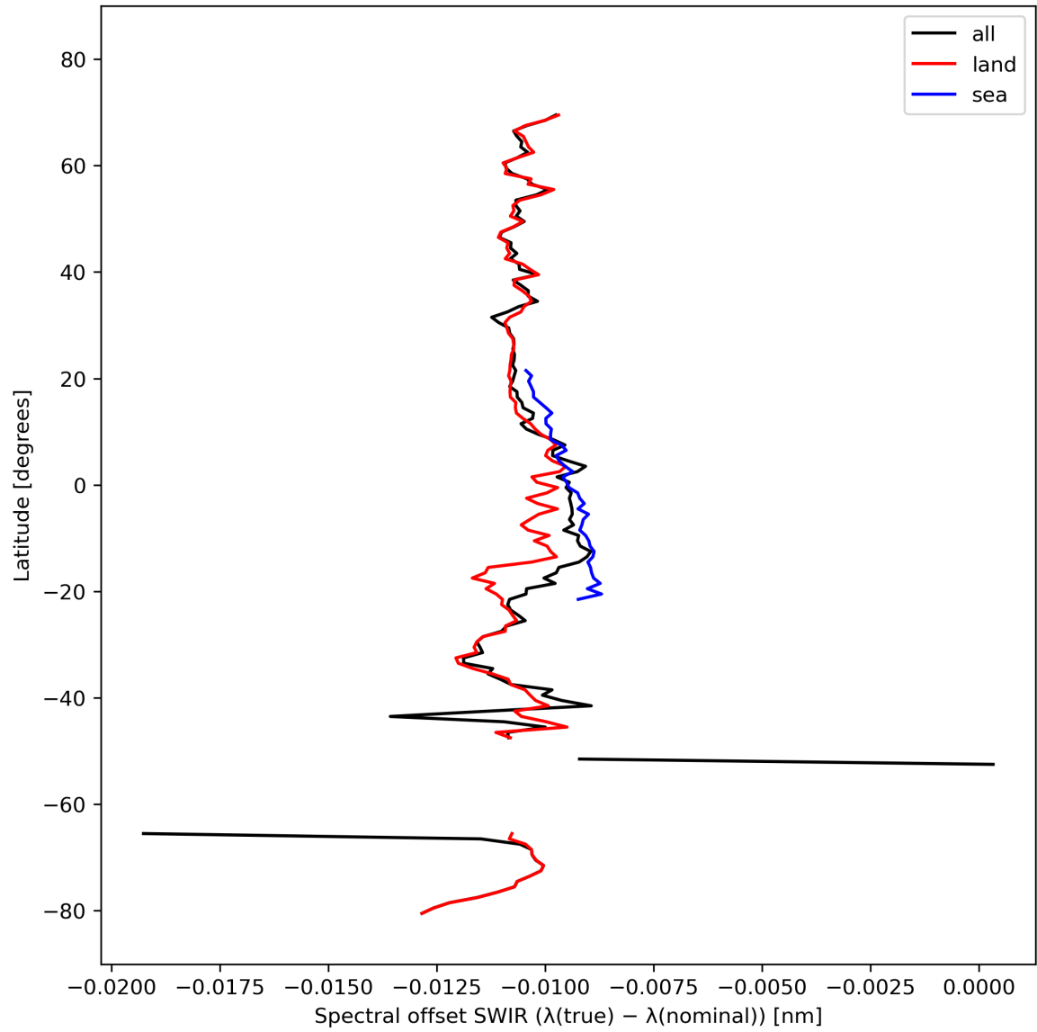
Figure 16: Zonal average of “Spectral offset SWIR ( \lambda(\text{true}) - \lambda(\text{nominal}) )” for 2024-03-04 to 2024-03-06.
