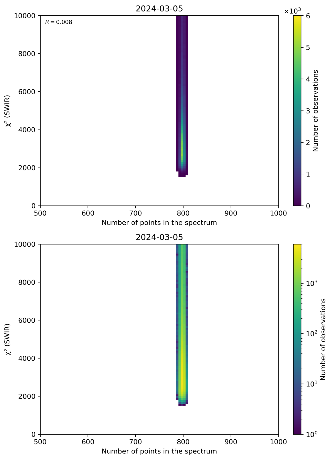
Figure 89: Scatter density plot of “Number of points in the spectrum” against “ \chi^2 (SWIR)” for 2024-03-04 to 2024-03-06.
