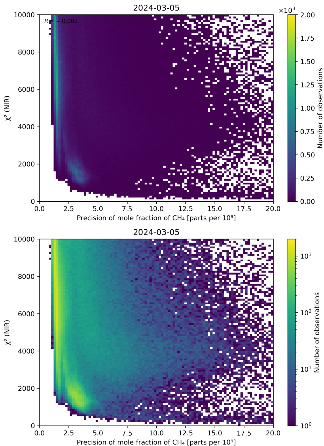
Figure 78: Scatter density plot of “Precision of mole fraction of CH 4 ” against “ \chi^2 (NIR)” for 2024-03-04 to 2024-03-06.
