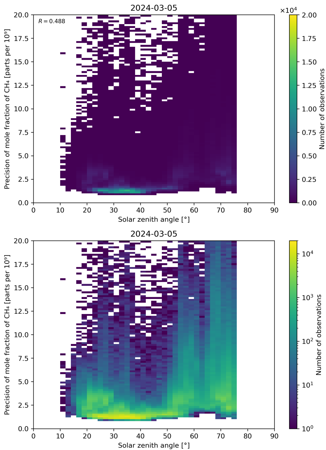
Figure 101: Scatter density plot of “Solar zenith angle” against “Precision of mole fraction of CH 4 ” for 2024-03-04 to 2024-03-06.
