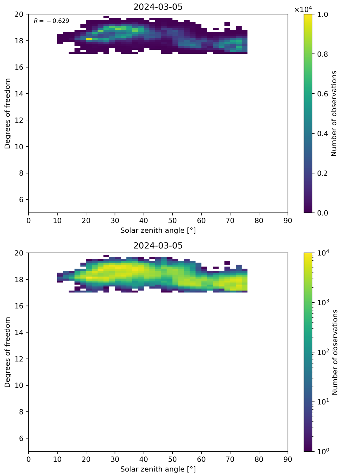
Figure 96: Scatter density plot of “Solar zenith angle” against “Degrees of freedom” for 2024-03-04 to 2024-03-06.
