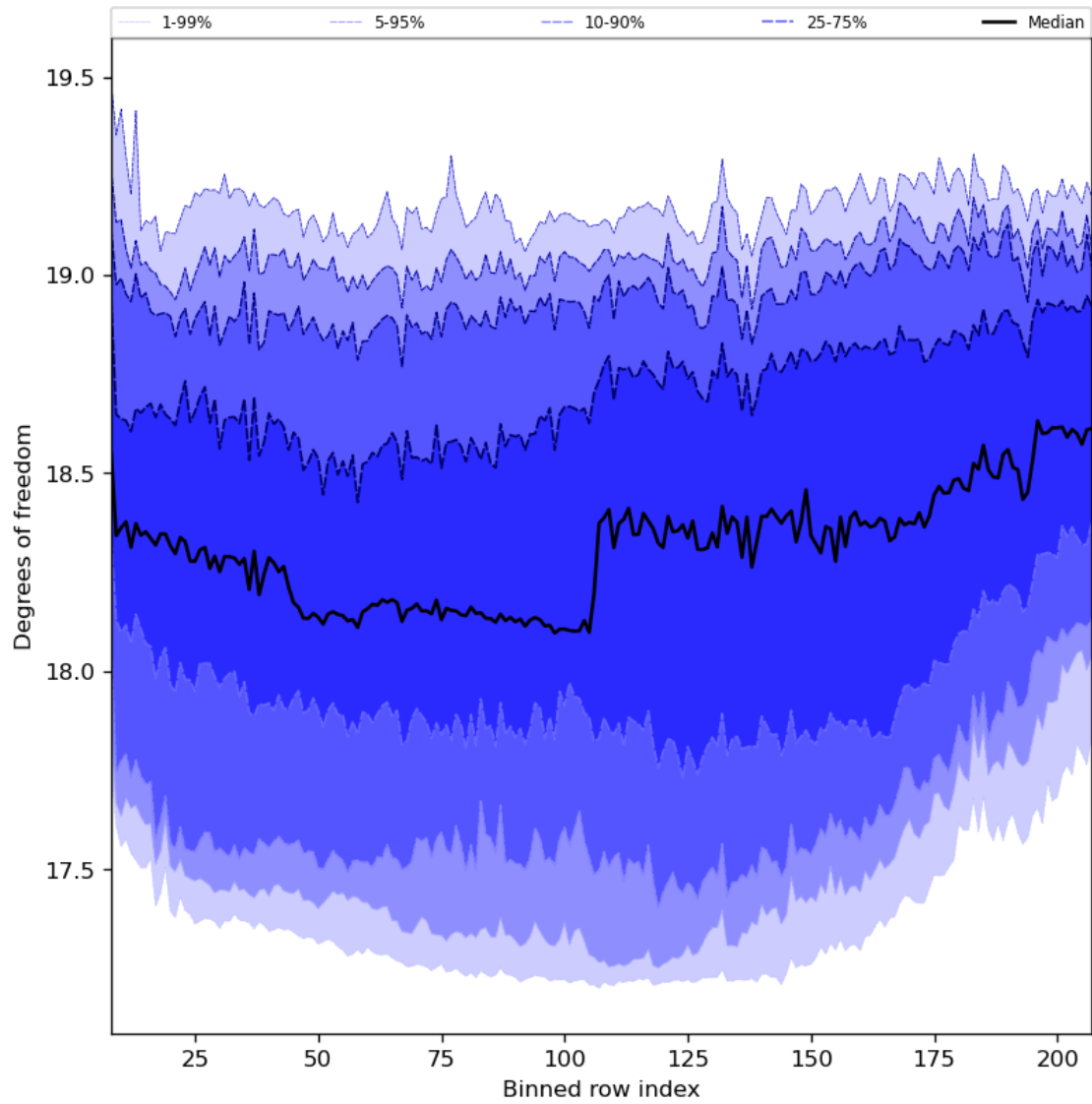
Figure 41: Along track statistics of “Degrees of freedom” for 2024-03-04 to 2024-03-06
