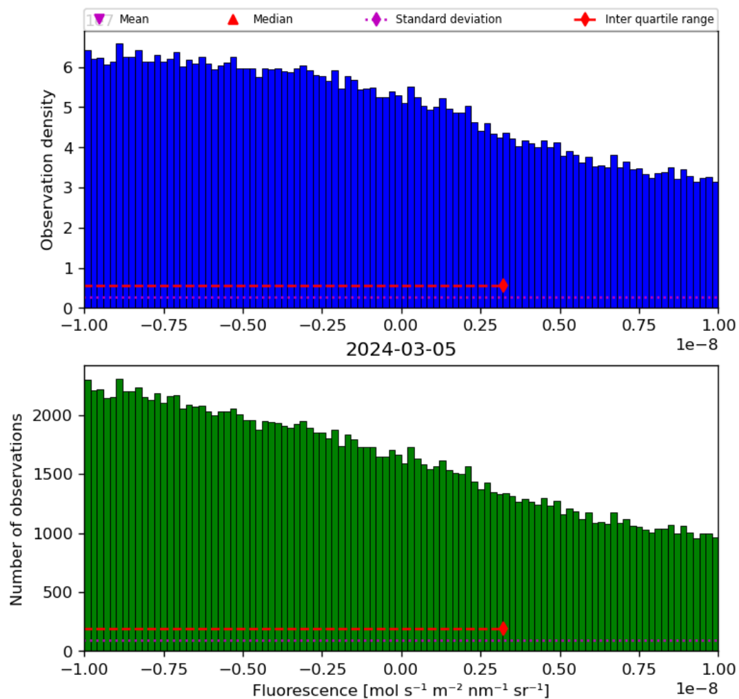
Figure 32: Histogram of “Fluorescence” for 2024-03-04 to 2024-03-06
