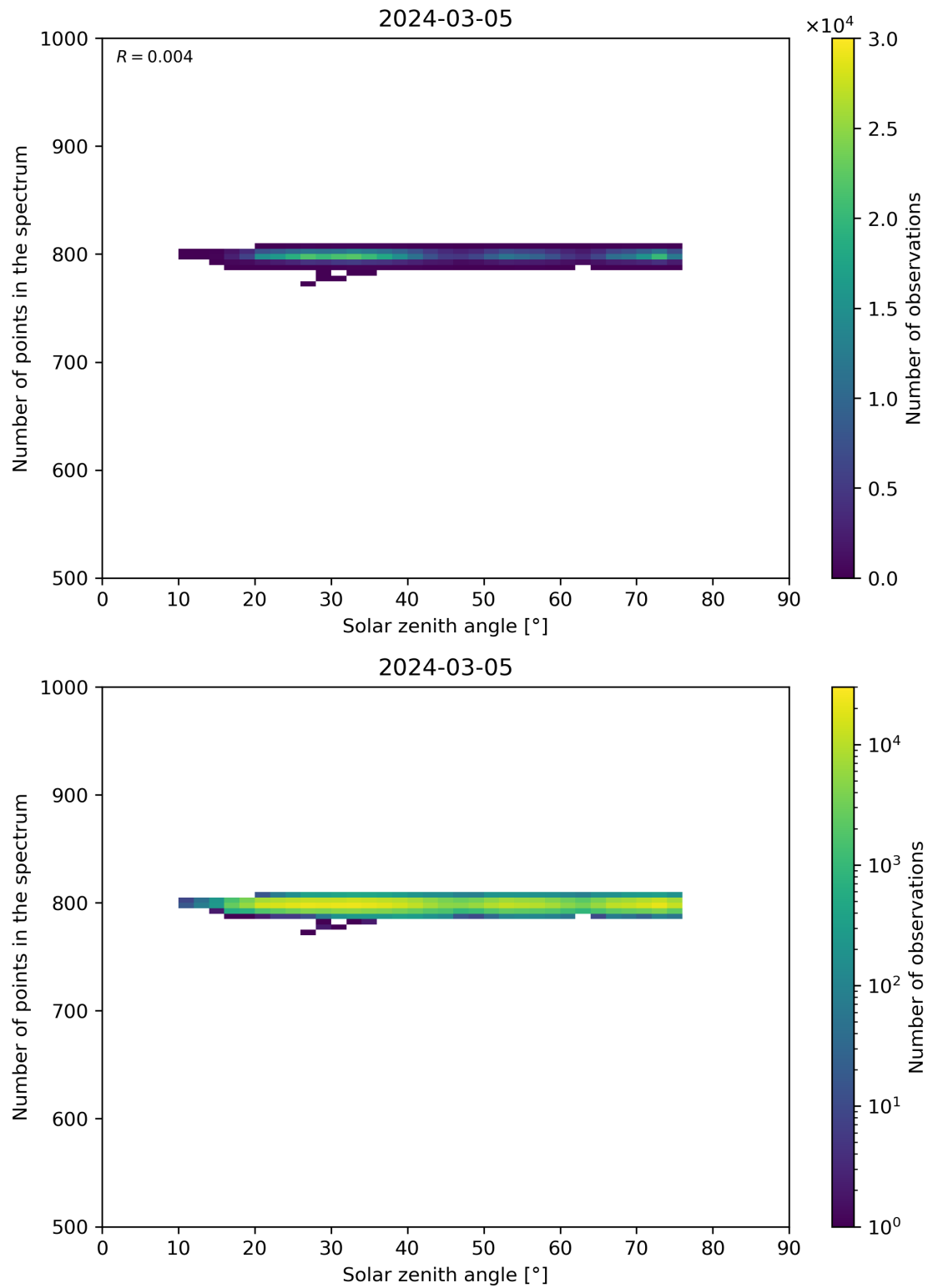
Figure 103: Scatter density plot of “Solar zenith angle” against “Number of points in the spectrum” for 2024-03-04 to 2024-03-06.
