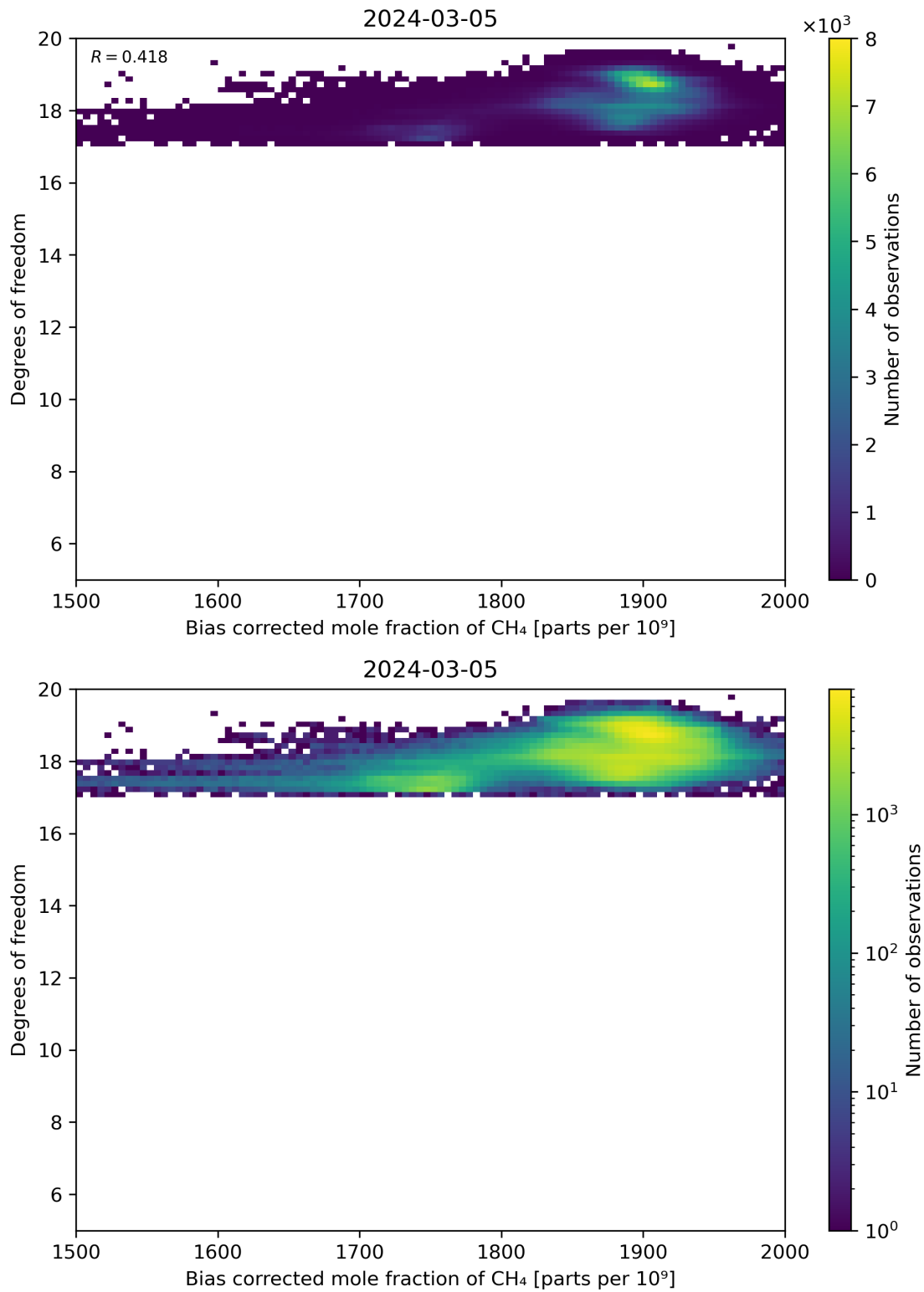
Figure 65: Scatter density plot of “Bias corrected mole fraction of CH 4 ” against “Degrees of freedom” for 2024-03-04 to 2024-03-06.
