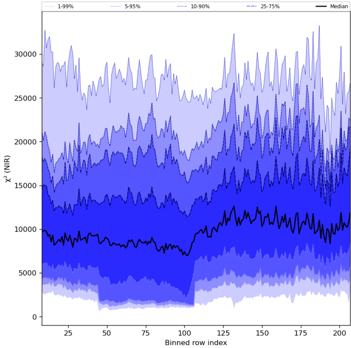
Figure 40: Along track statistics of “ \chi^2 (NIR)” for 2024-03-04 to 2024-03-06
