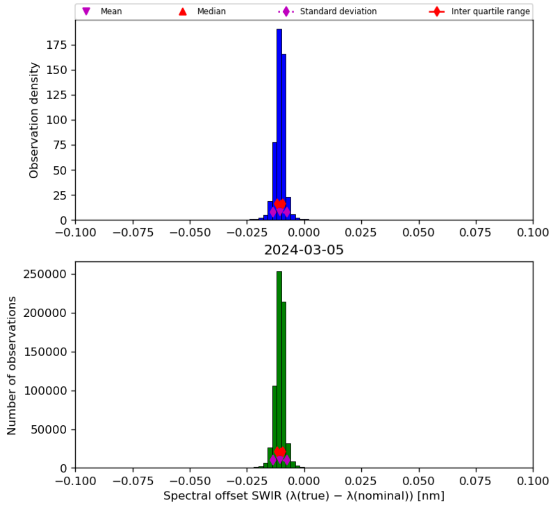
Figure 27: Histogram of “Spectral offset SWIR ( \lambda(\text{true}) - \lambda(\text{nominal}) )” for 2024-03-04 to 2024-03-06
