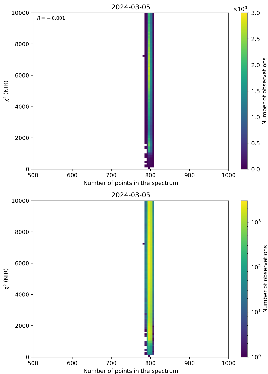
Figure 88: Scatter density plot of “Number of points in the spectrum” against “ \chi^2 (NIR)” for 2024-03-04 to 2024-03-06.
