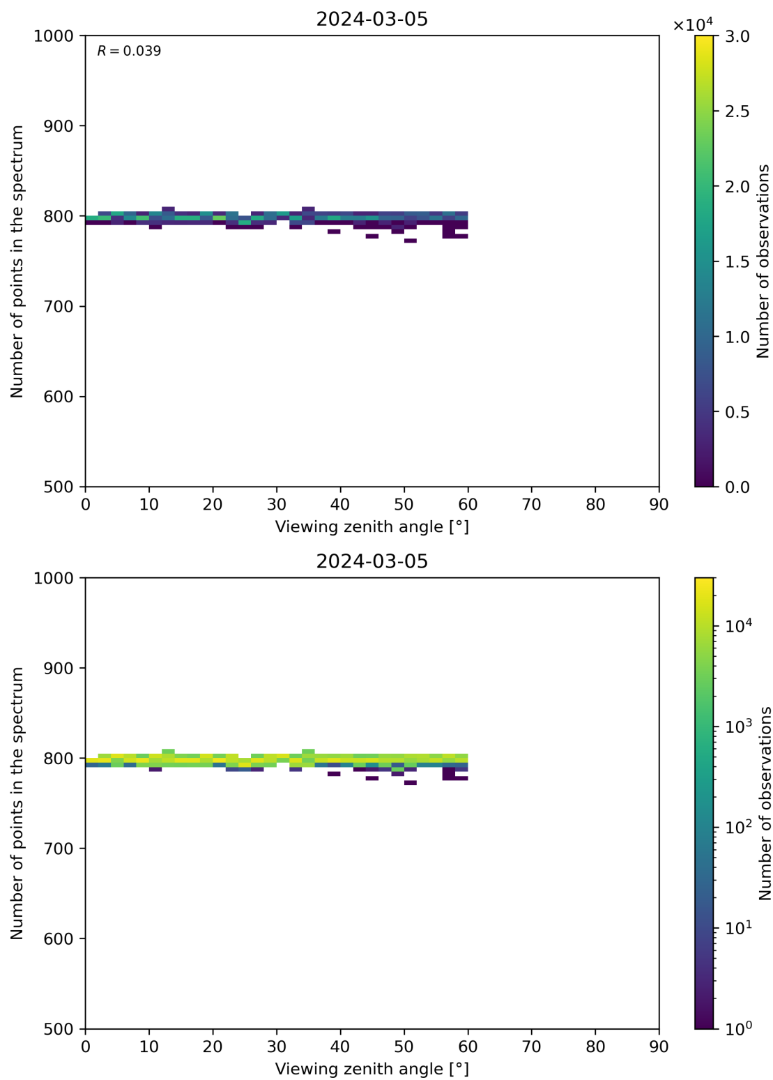
Figure 114: Scatter density plot of “Viewing zenith angle” against “Number of points in the spectrum” for 2024-03-04 to 2024-03-06.
