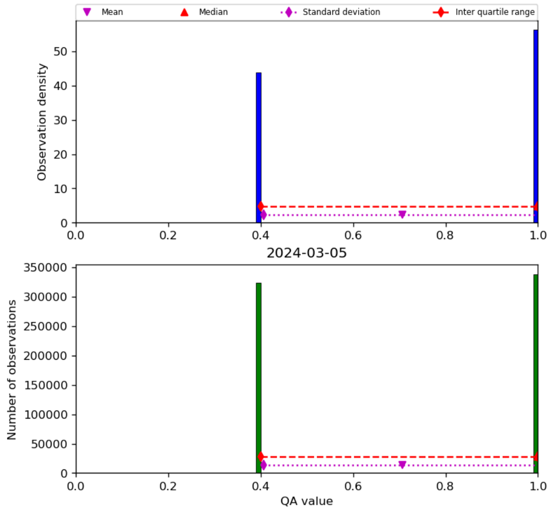
Figure 22: Histogram of “QA value” for 2024-03-04 to 2024-03-06
