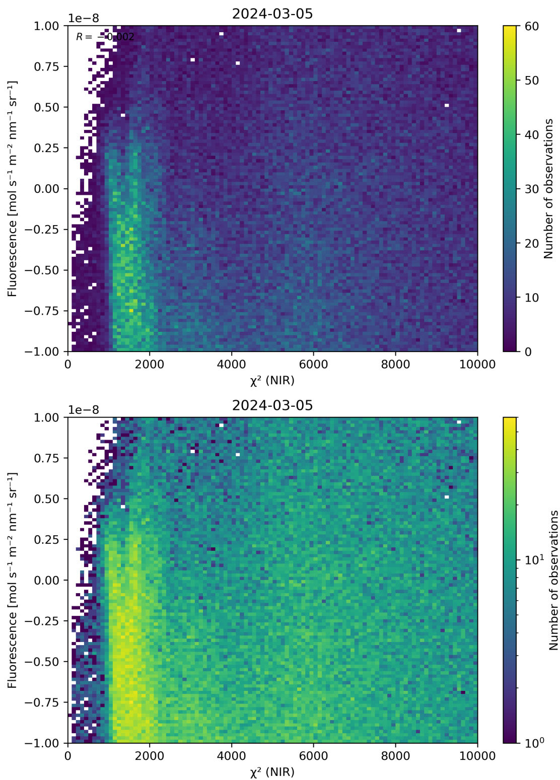
Figure 45: Scatter density plot of “ \chi^2 (NIR)” against “Fluorescence” for 2024-03-04 to 2024-03-06.
