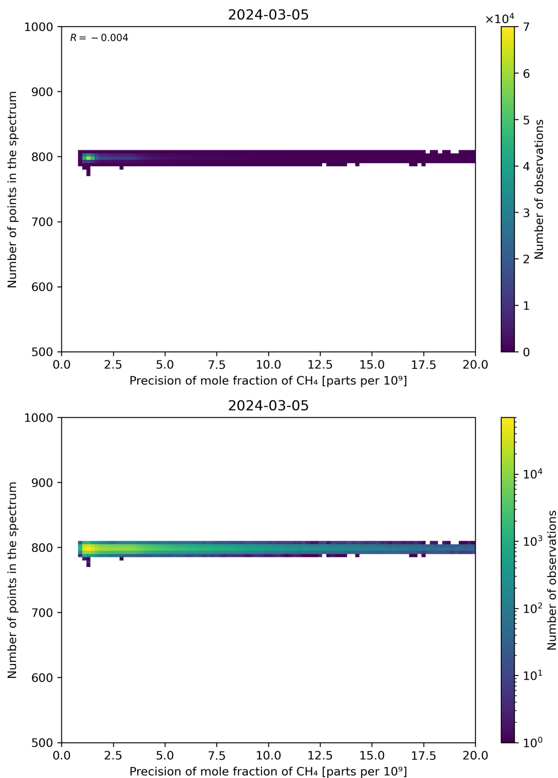
Figure 84: Scatter density plot of “Precision of mole fraction of CH 4 ” against “Number of points in the spectrum” for 2024-03-04 to 2024-03-06.
