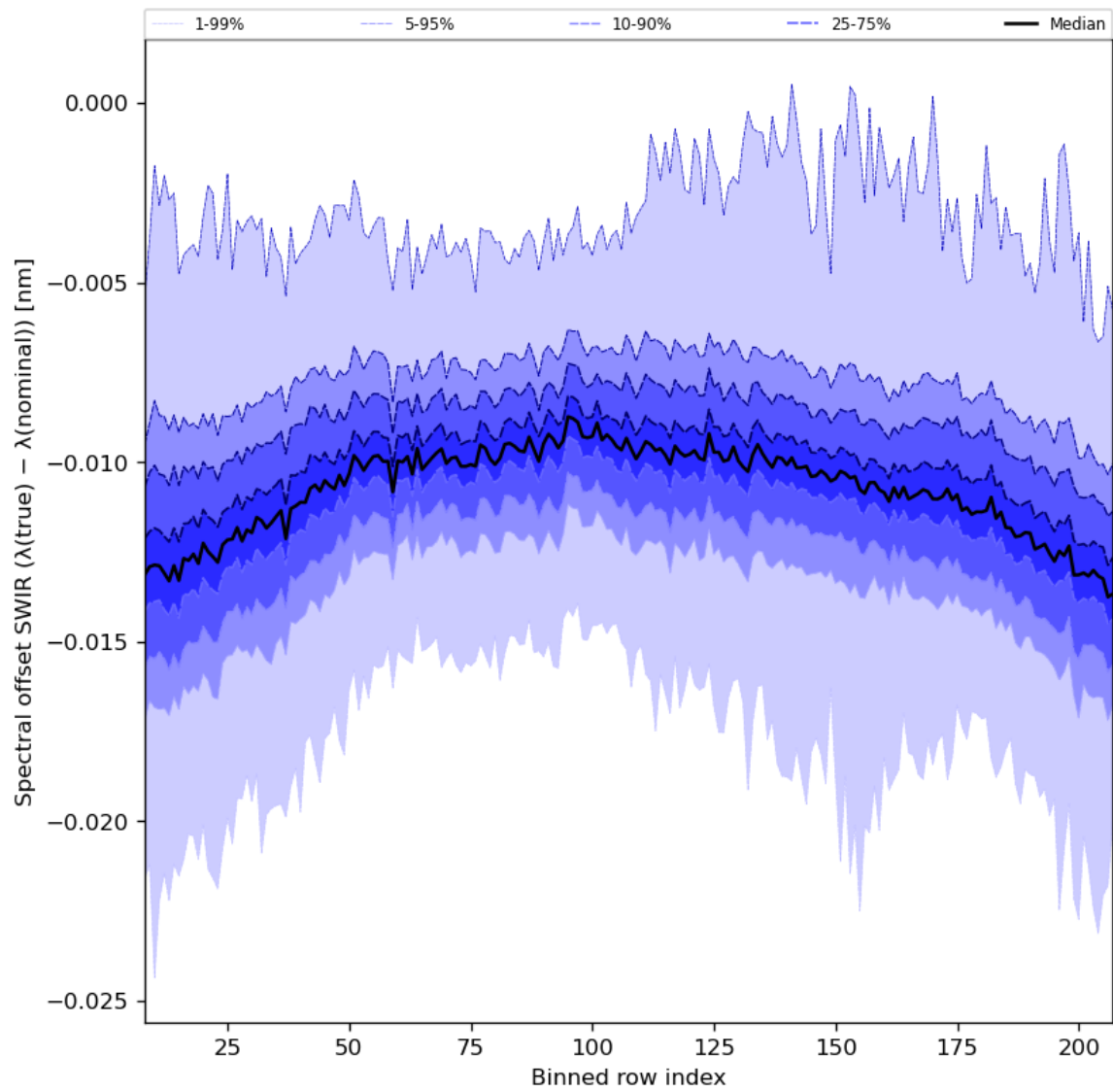
Figure 38: Along track statistics of “Spectral offset SWIR ( \lambda(\text{true}) - \lambda(\text{nominal}) )” for 2024-03-04 to 2024-03-06
