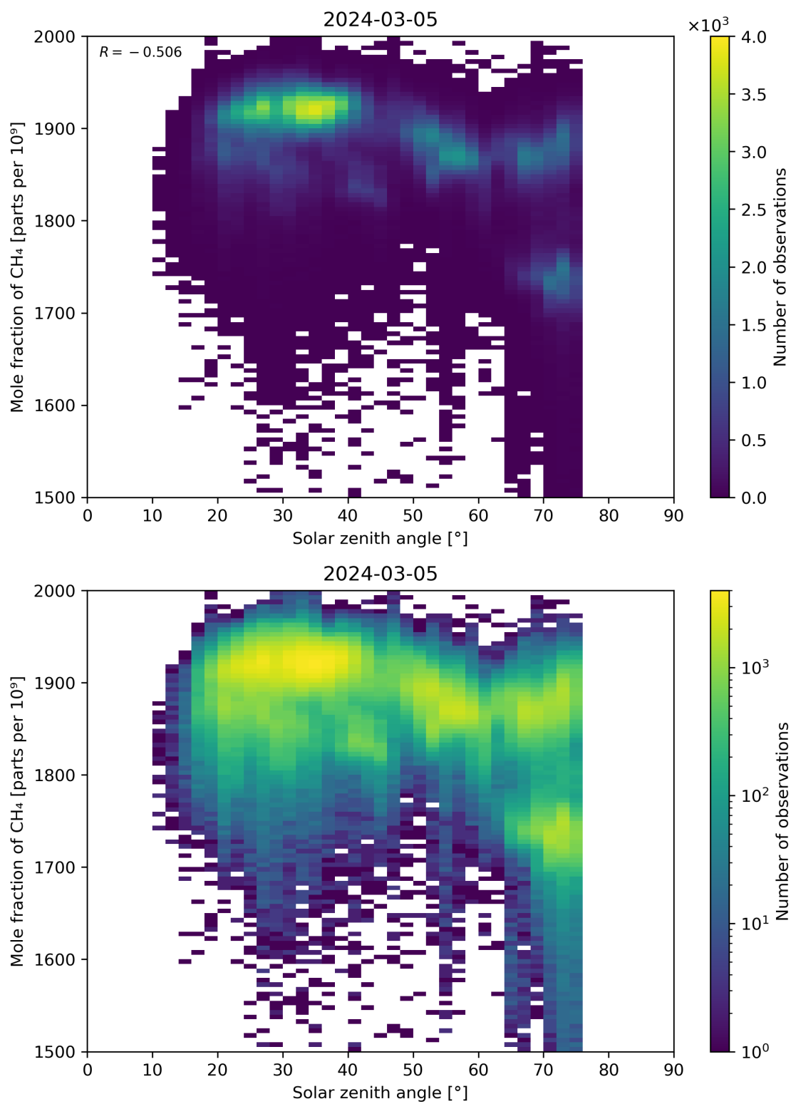
Figure 99: Scatter density plot of “Solar zenith angle” against “Mole fraction of \text{CH}_4 ” for 2024-03-04 to 2024-03-06.
