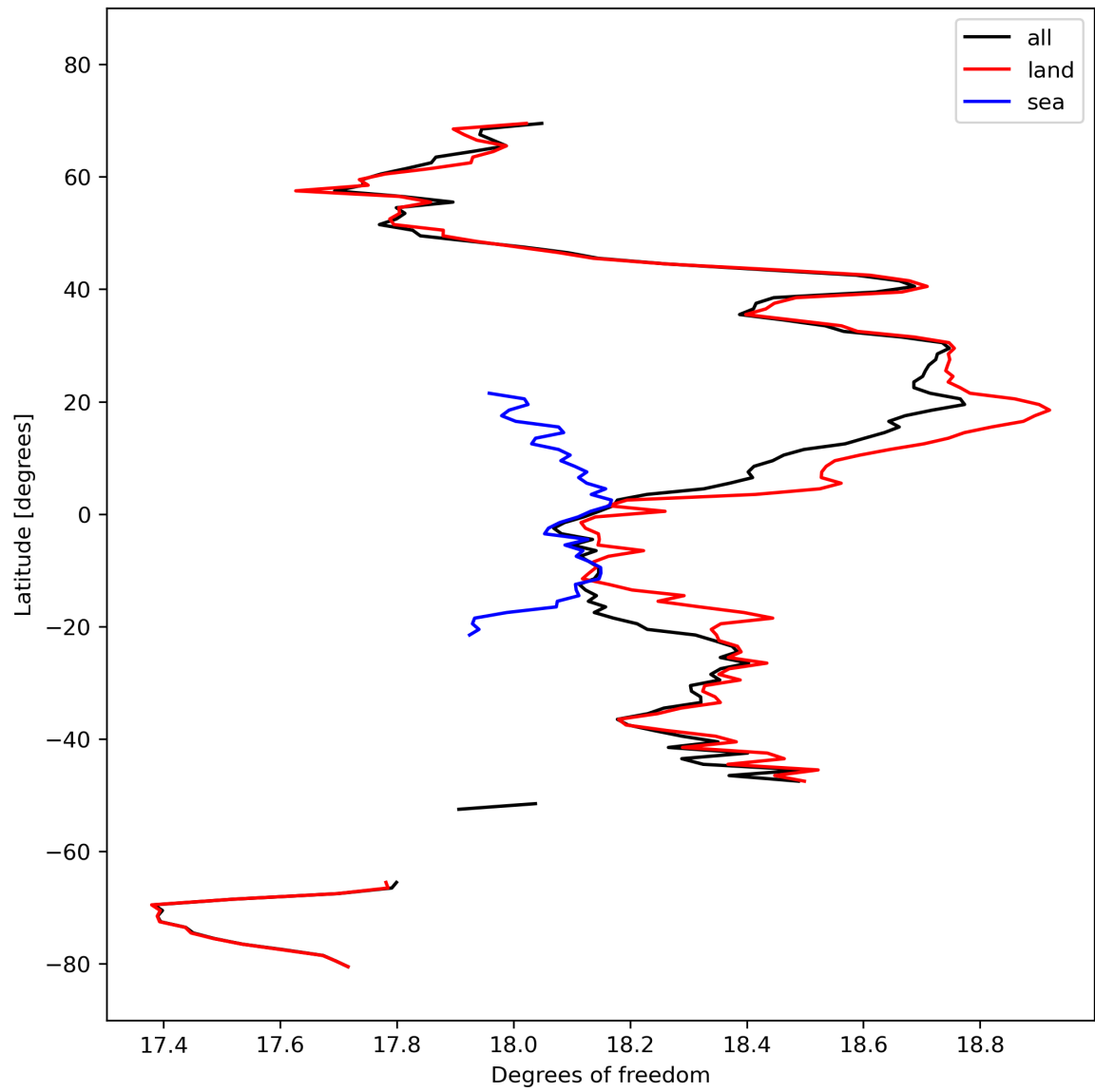
Figure 19: Zonal average of “Degrees of freedom” for 2024-03-04 to 2024-03-06.
