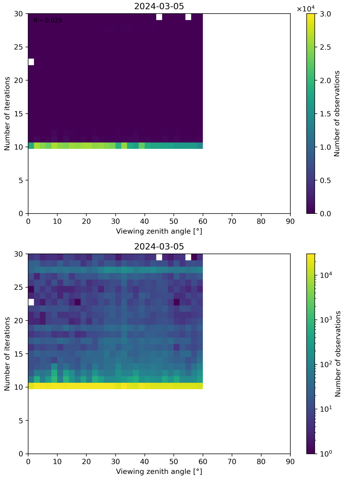
Figure 113: Scatter density plot of “Viewing zenith angle” against “Number of iterations” for 2024-03-04 to 2024-03-06.
