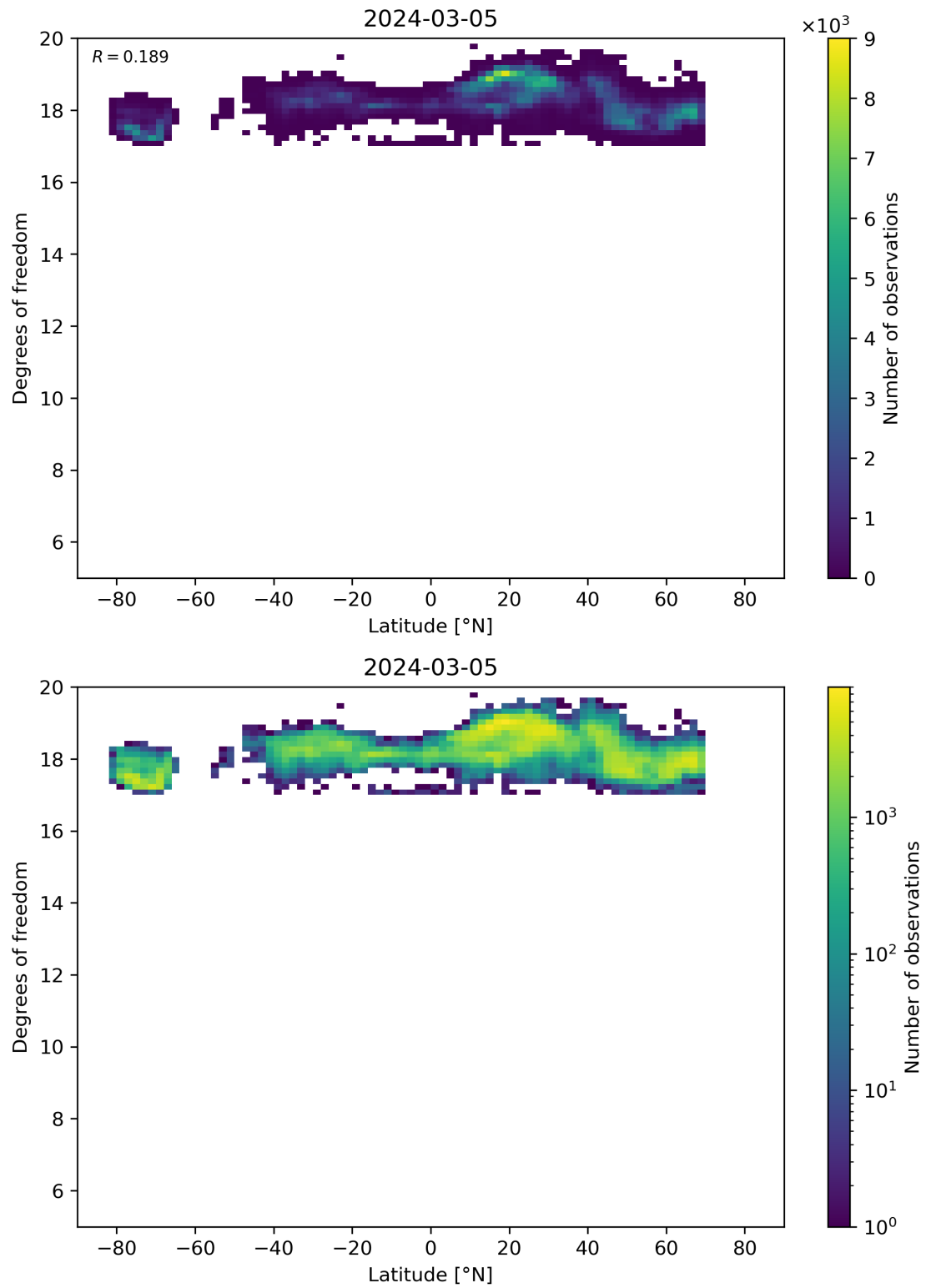
Figure 55: Scatter density plot of “Latitude” against “Degrees of freedom” for 2024-03-04 to 2024-03-06.
