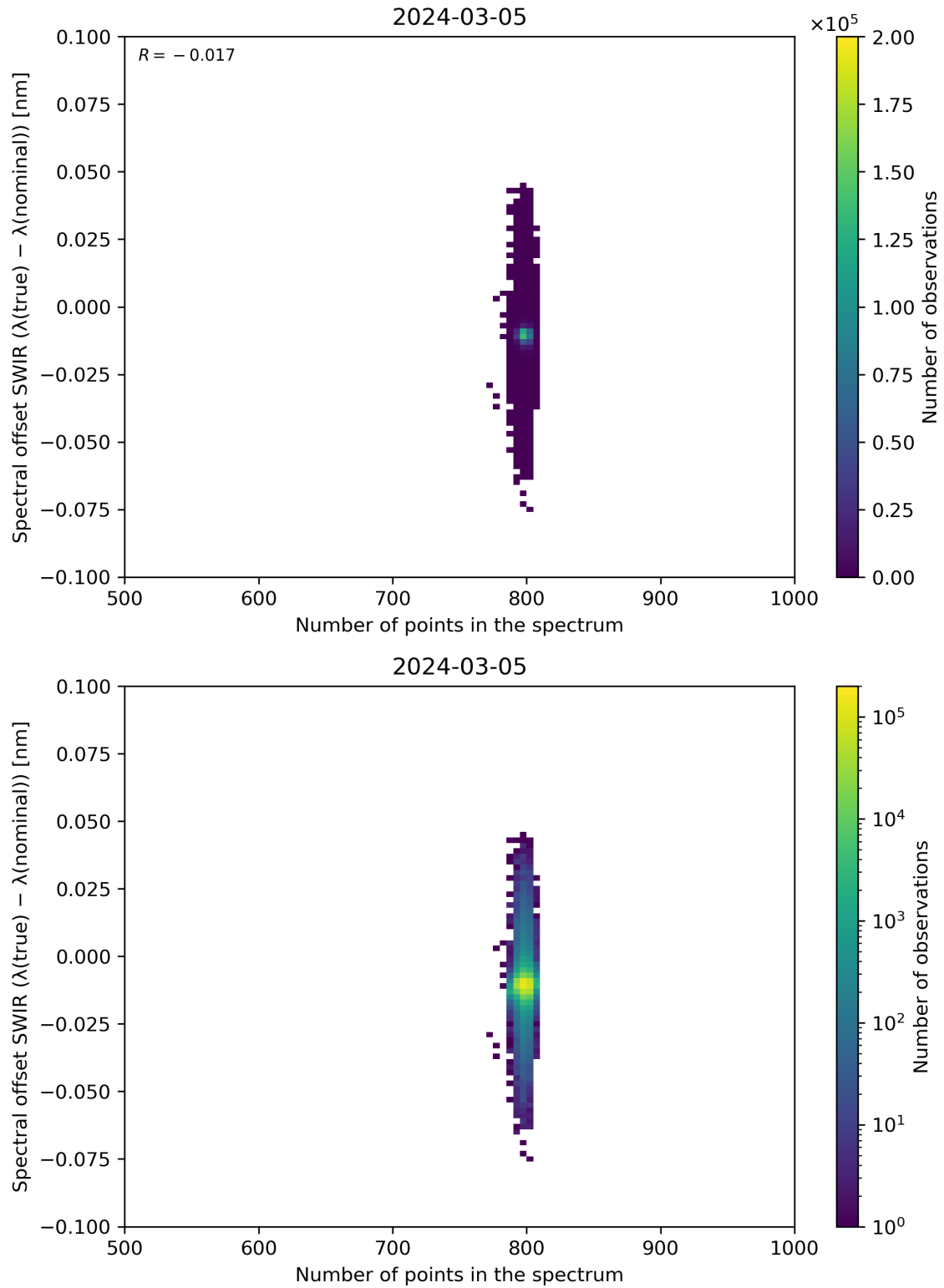
Figure 93: Scatter density plot of “Number of points in the spectrum” against “Spectral offset SWIR ( \lambda(\text{true}) - \lambda(\text{nominal}) )” for 2024-03-04 to 2024-03-06.
