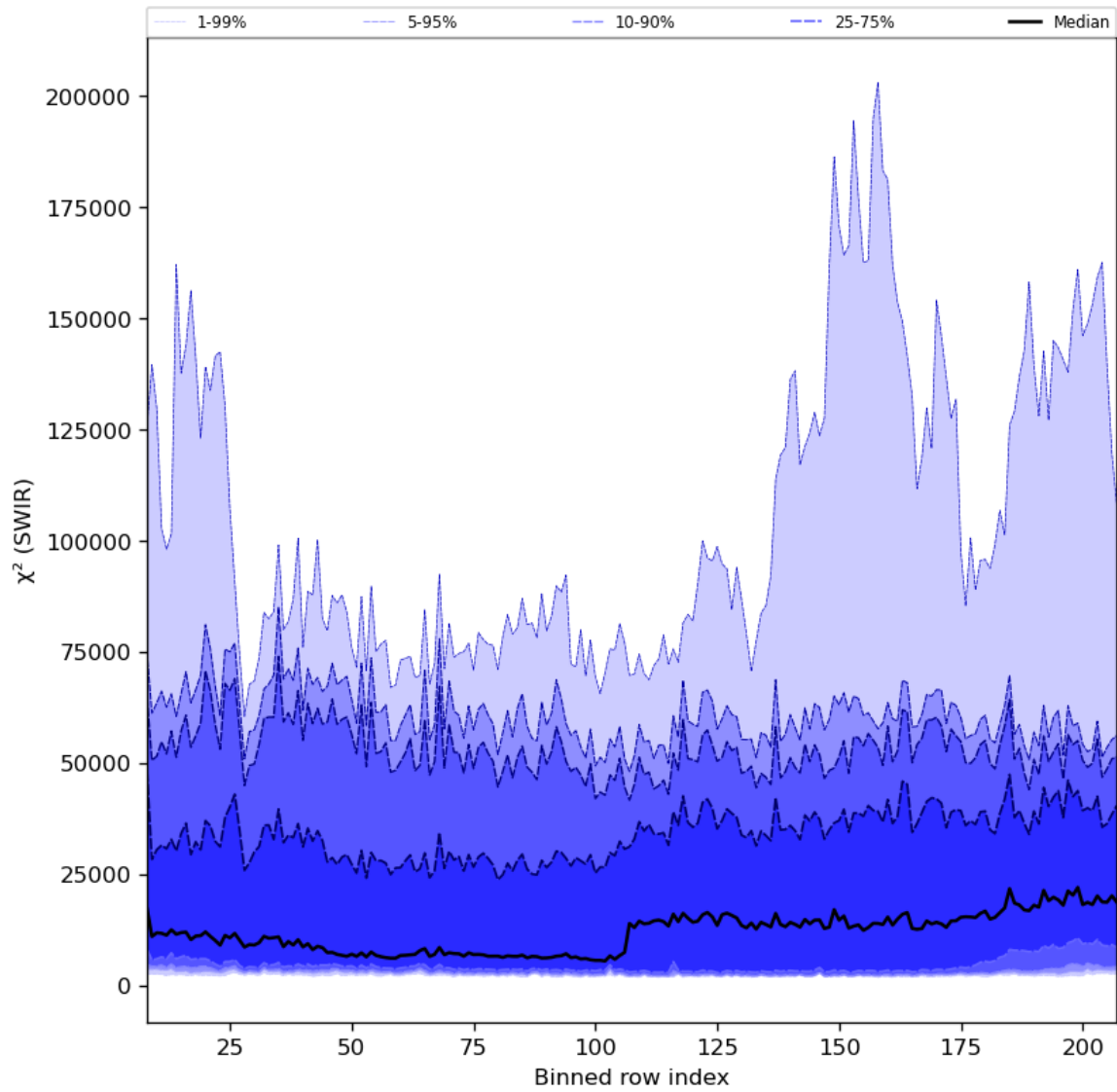
Figure 39: Along track statistics of “ \chi^2 (SWIR)” for 2024-03-04 to 2024-03-06
