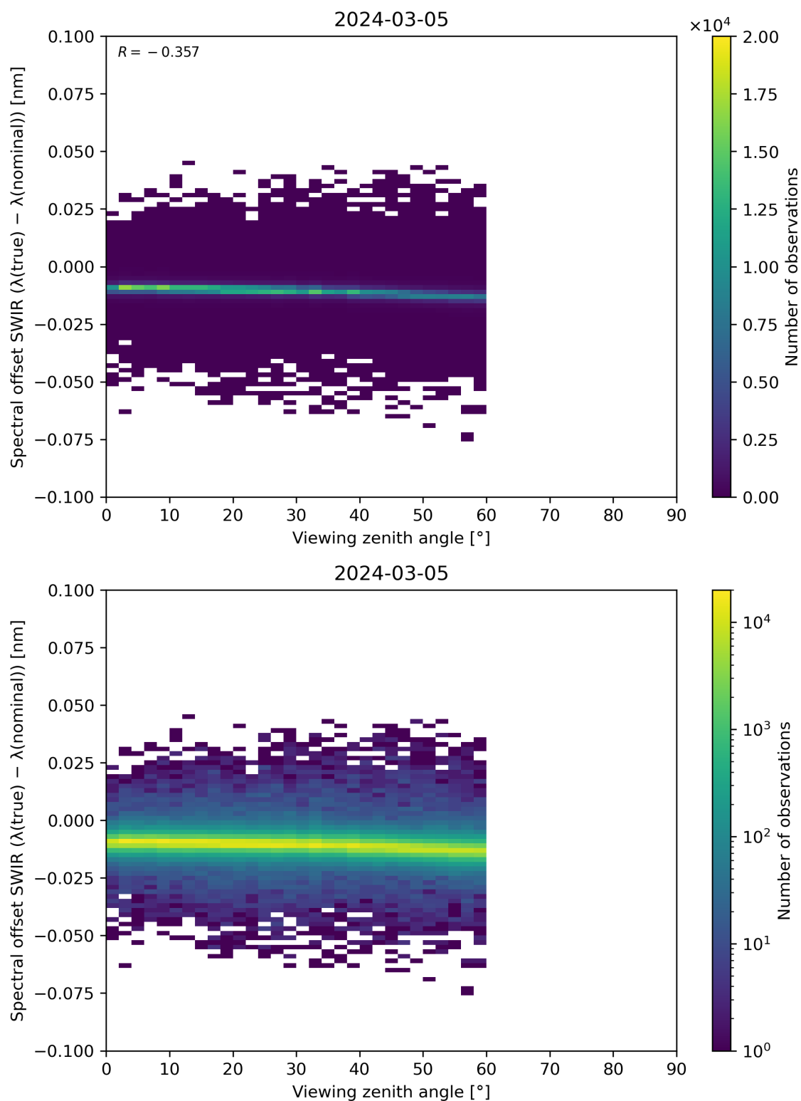
Figure 116: Scatter density plot of “Viewing zenith angle” against “Spectral offset SWIR ( \lambda(\text{true}) - \lambda(\text{nominal}) )” for 2024-03-04 to 2024-03-06.
