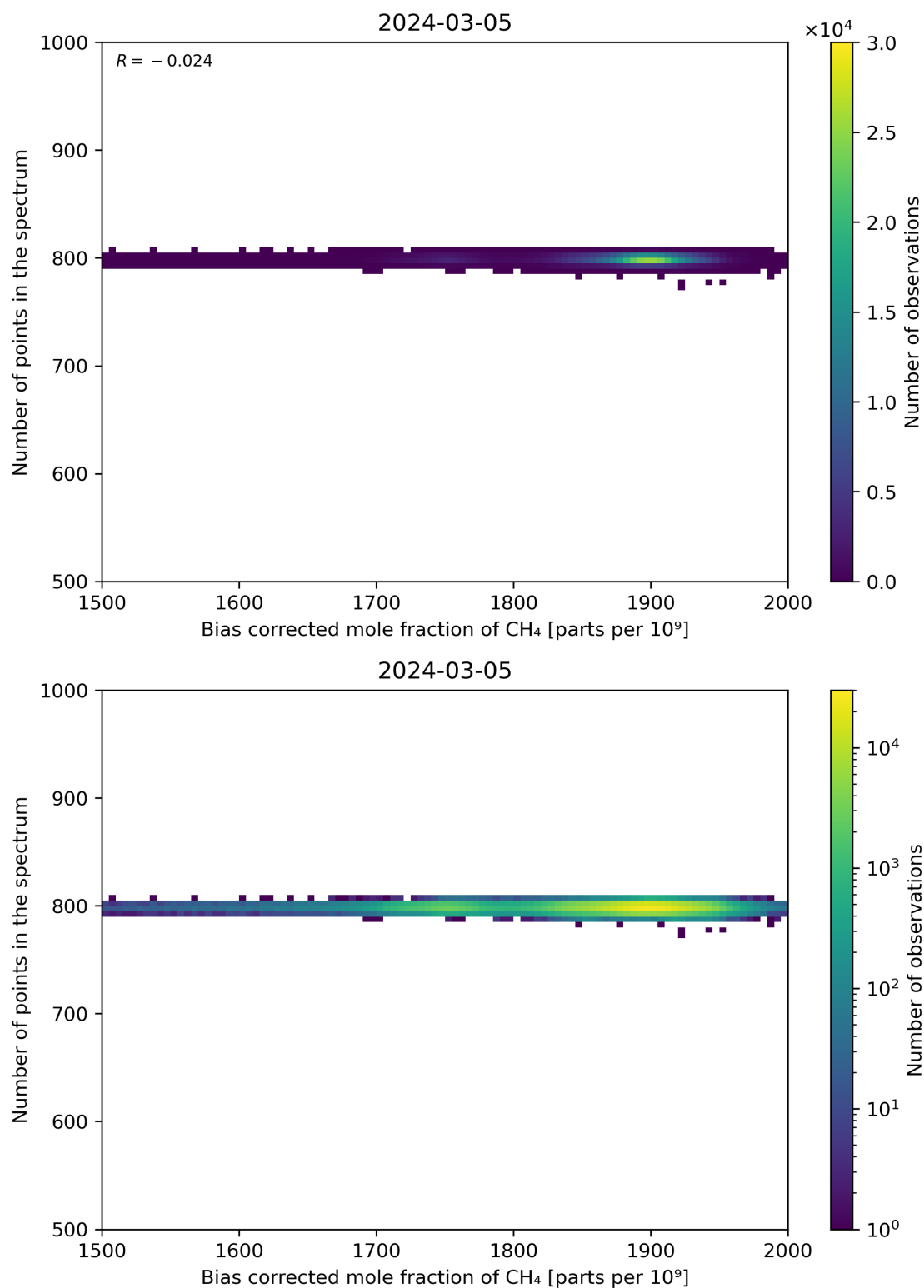
Figure 68: Scatter density plot of “Bias corrected mole fraction of CH 4 ” against “Number of points in the spectrum” for 2024-03-04 to 2024-03-06.
