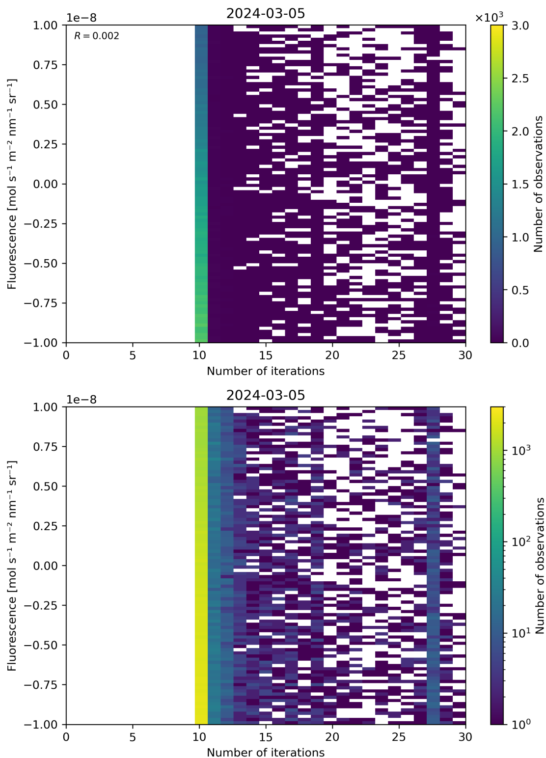
Figure 87: Scatter density plot of “Number of iterations” against “Fluorescence” for 2024-03-04 to 2024-03-06.
