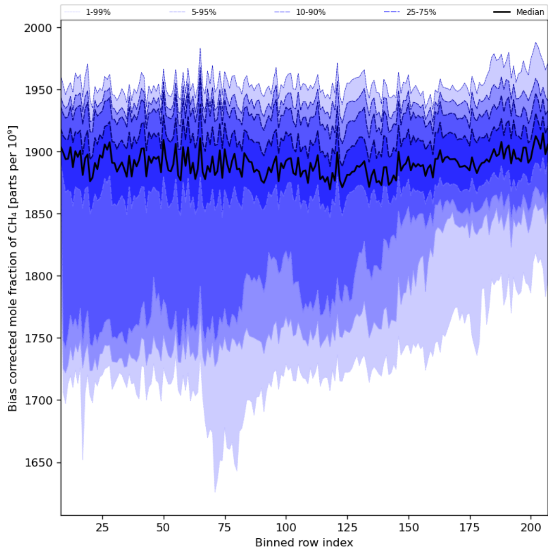
Figure 36: Along track statistics of “Bias corrected mole fraction of CH 4 ” for 2024-03-07 to 2024-03-09
