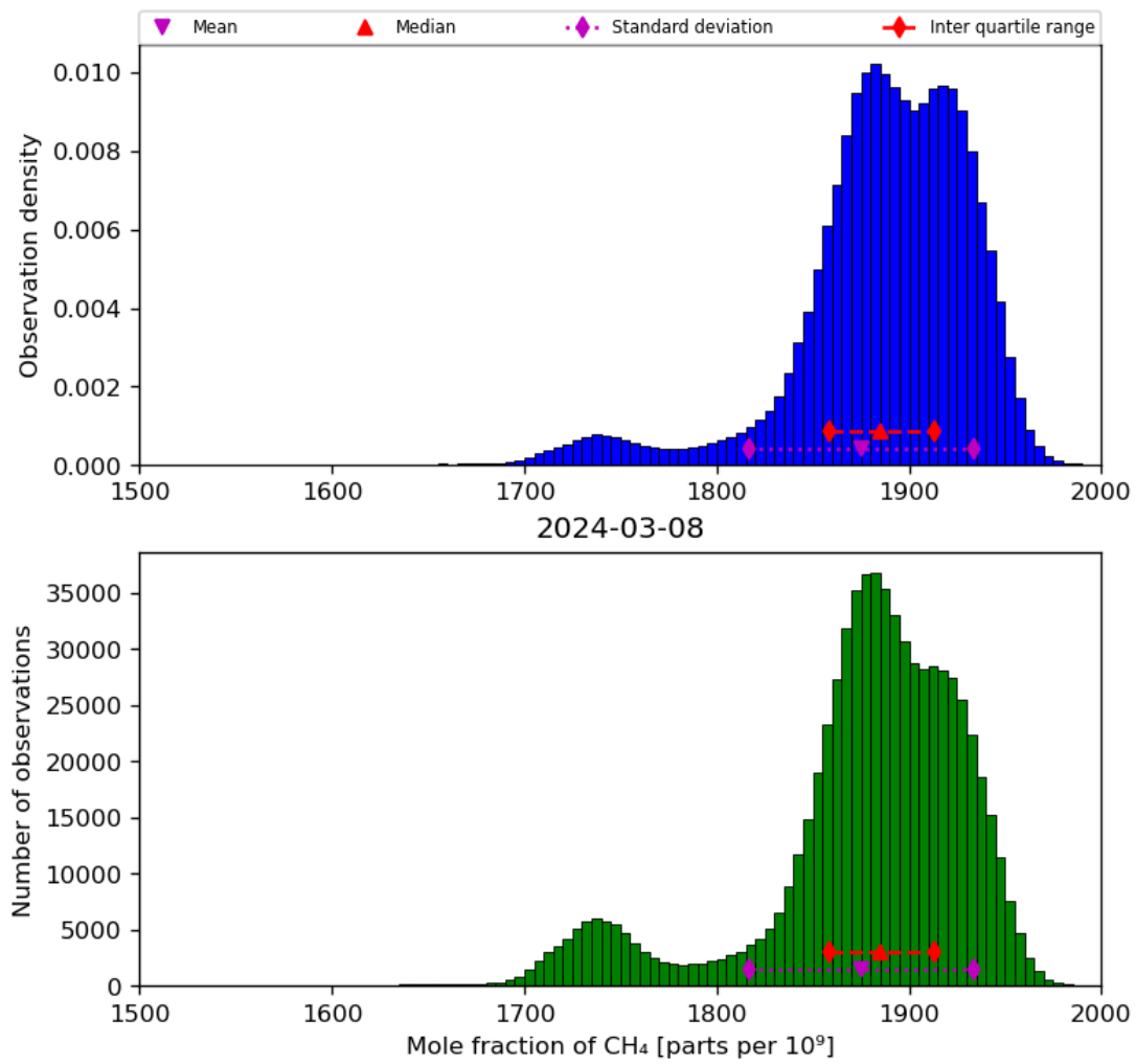
Figure 23: Histogram of “Mole fraction of CH 4 ” for 2024-03-07 to 2024-03-09
