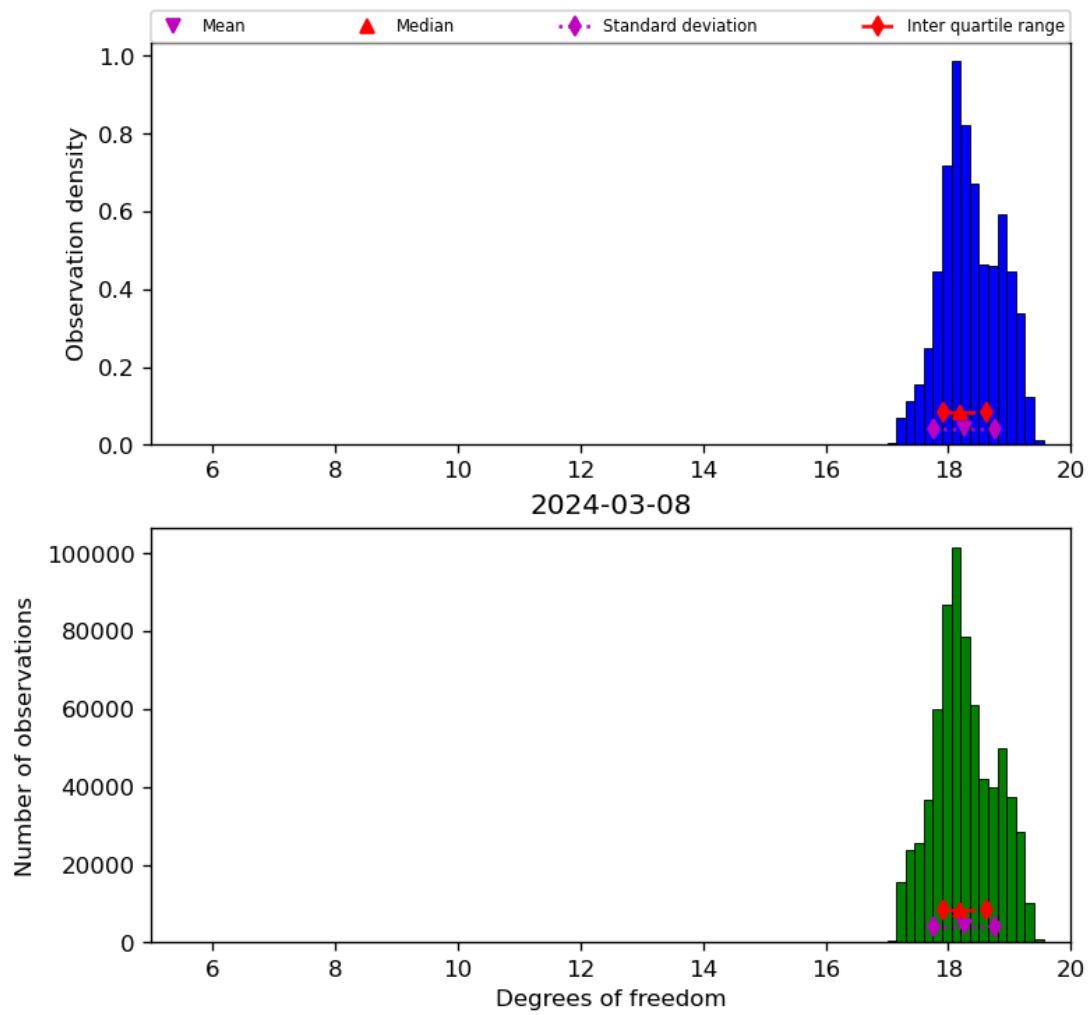
Figure 30: Histogram of “Degrees of freedom” for 2024-03-07 to 2024-03-09
