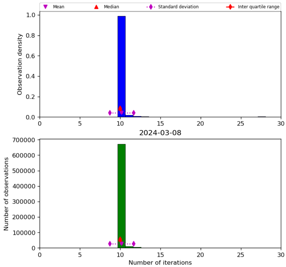
Figure 31: Histogram of “Number of iterations” for 2024-03-07 to 2024-03-09
