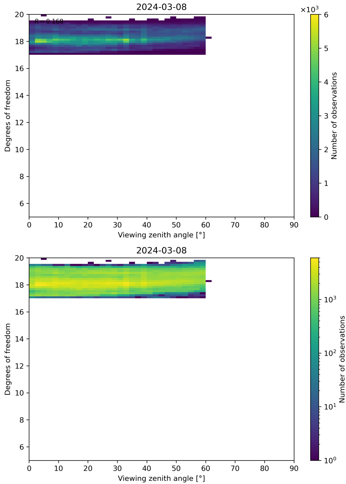
Figure 107: Scatter density plot of “Viewing zenith angle” against “Degrees of freedom” for 2024-03-07 to 2024-03-09.
