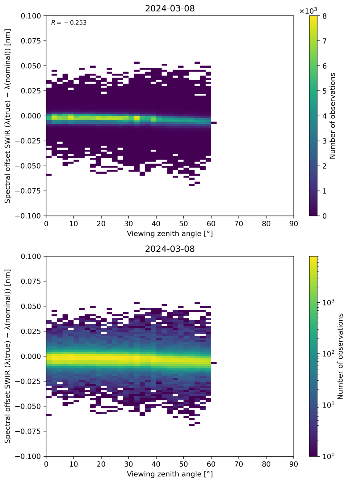
Figure 116: Scatter density plot of “Viewing zenith angle” against “Spectral offset SWIR ( \lambda(\text{true}) - \lambda(\text{nominal}) )” for 2024-03-07 to 2024-03-09.
