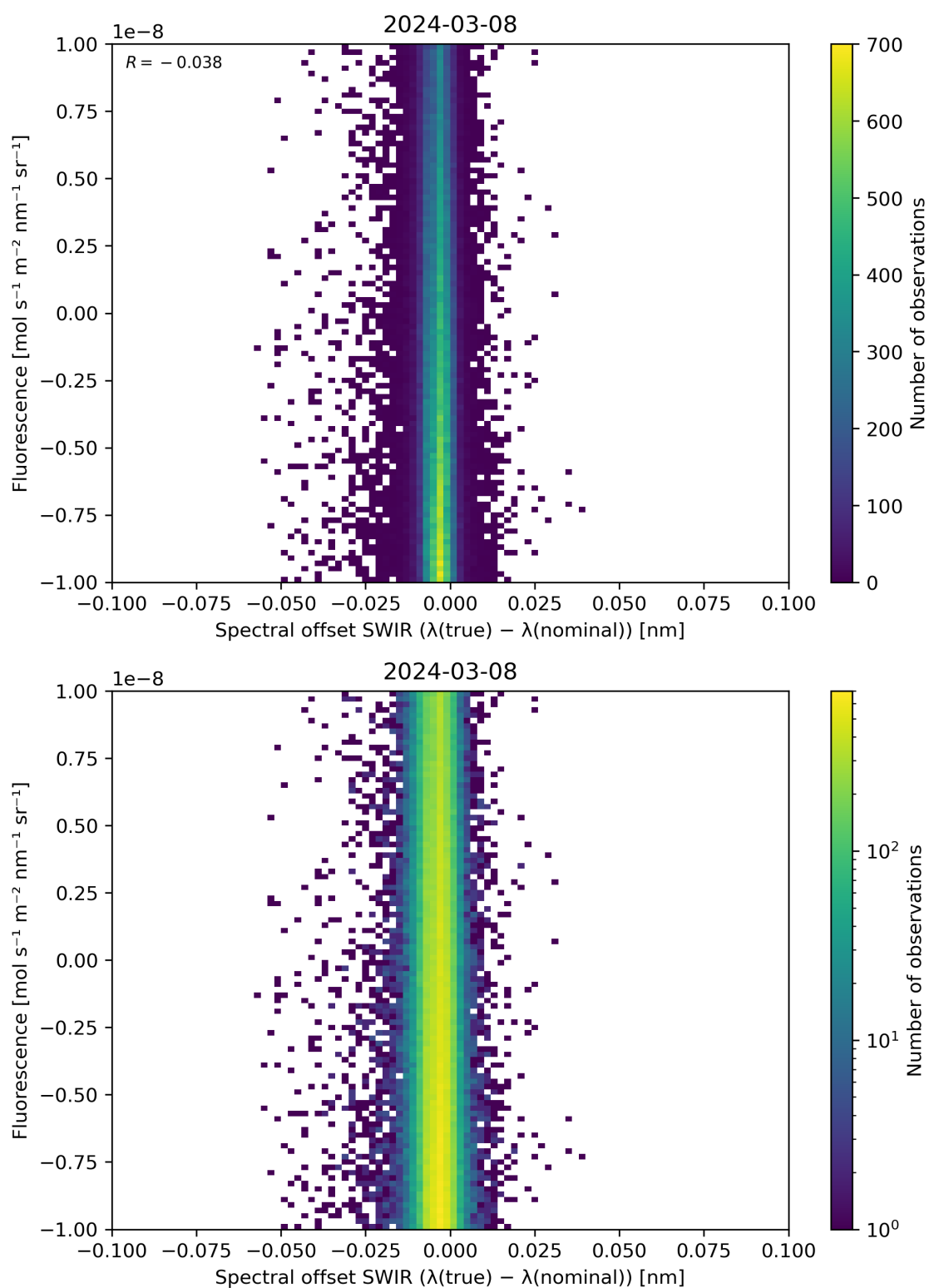
Figure 120: Scatter density plot of “Spectral offset SWIR ( \lambda(\text{true}) - \lambda(\text{nominal}) )” against “Fluorescence” for 2024-03-07 to 2024-03-09.
