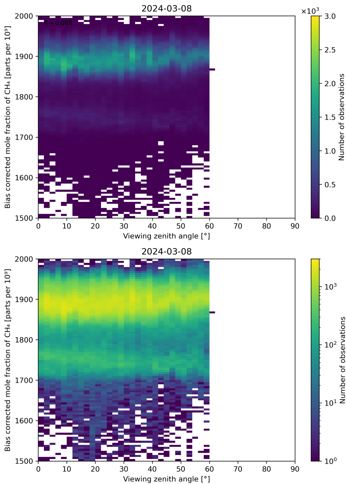
Figure 111: Scatter density plot of “Viewing zenith angle” against “Bias corrected mole fraction of \text{CH}_4 ” for 2024-03-07 to 2024-03-09.
