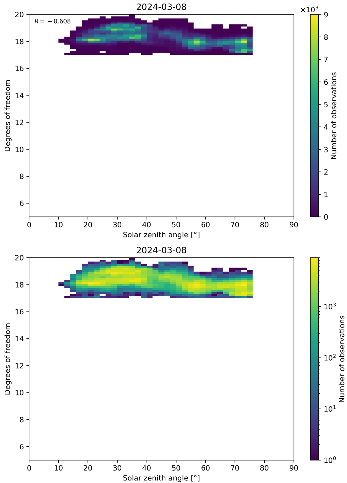
Figure 96: Scatter density plot of “Solar zenith angle” against “Degrees of freedom” for 2024-03-07 to 2024-03-09.
