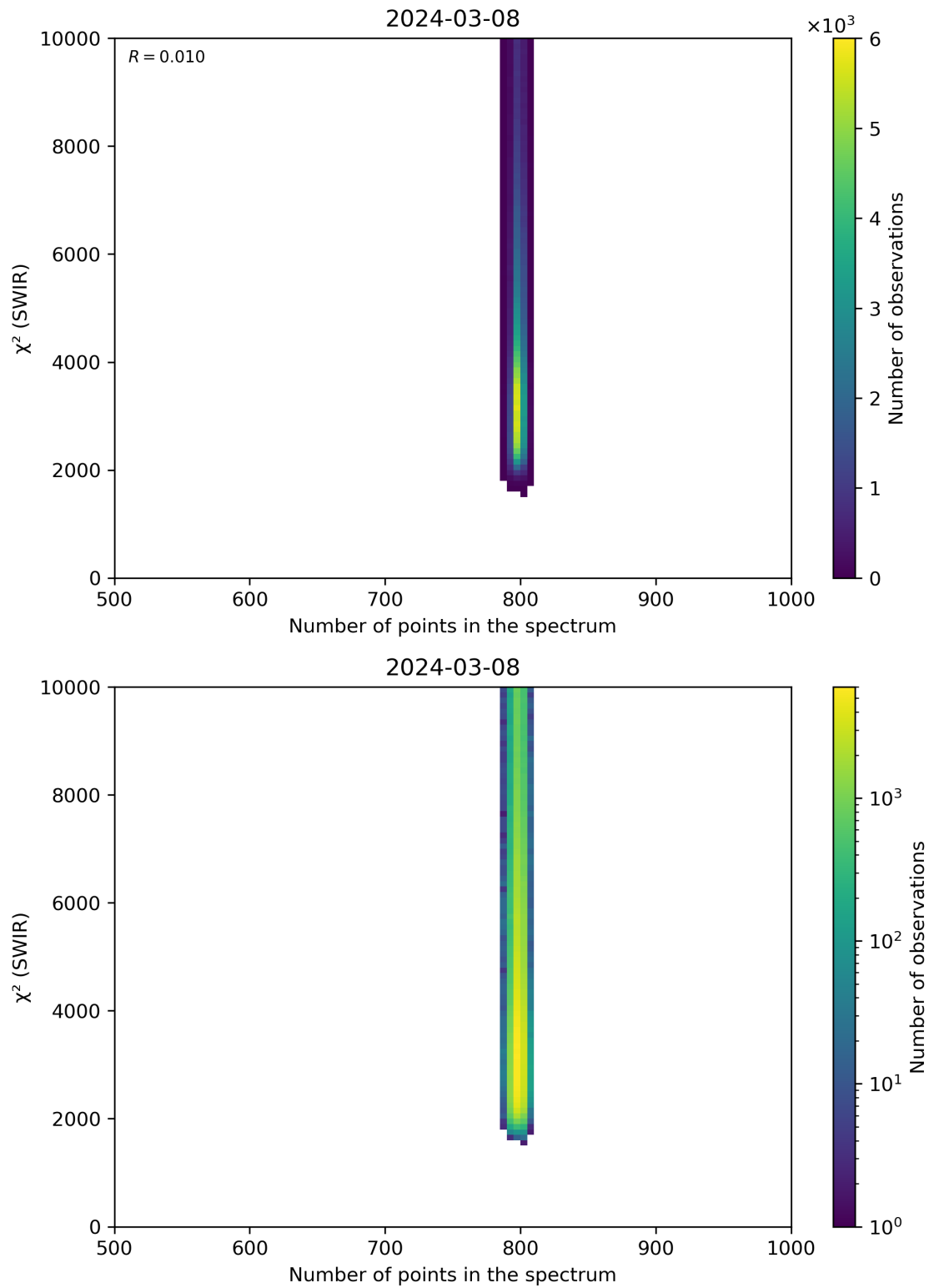
Figure 89: Scatter density plot of “Number of points in the spectrum” against “ \chi^2 (SWIR)” for 2024-03-07 to 2024-03-09.
