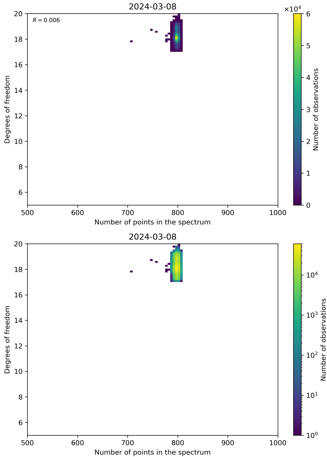
Figure 90: Scatter density plot of “Number of points in the spectrum” against “Degrees of freedom” for 2024-03-07 to 2024-03-09.
