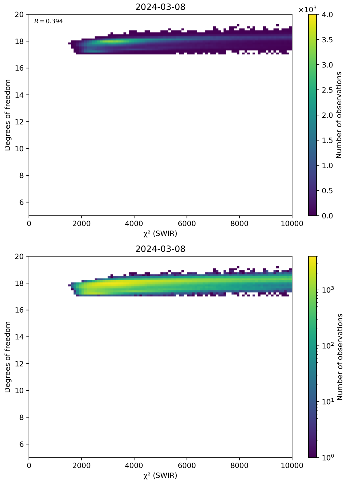
Figure 48: Scatter density plot of “ \chi^2 (SWIR)” against “Degrees of freedom” for 2024-03-07 to 2024-03-09.
