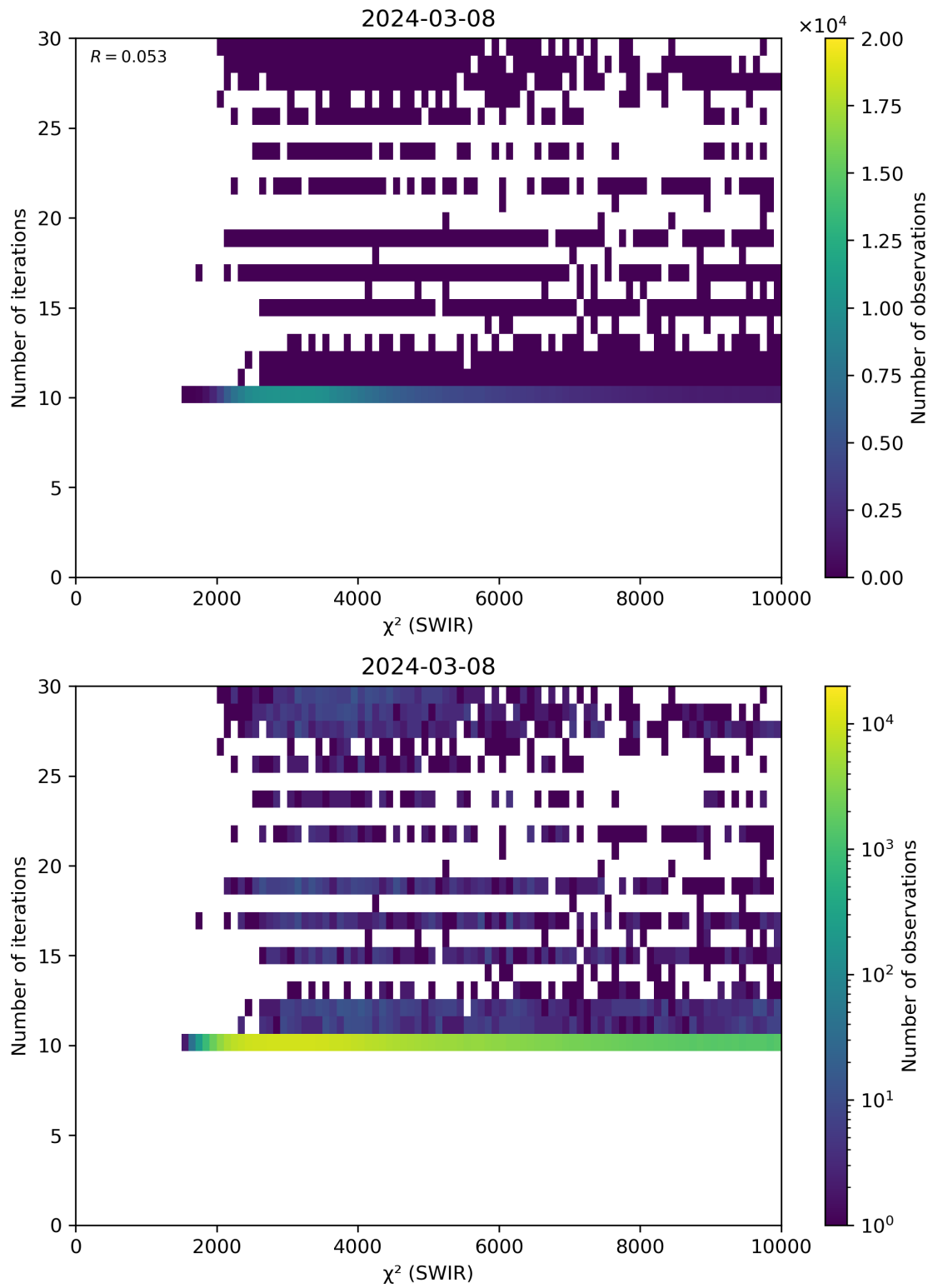
Figure 50: Scatter density plot of “ \chi^2 (SWIR)” against “Number of iterations” for 2024-03-07 to 2024-03-09.
