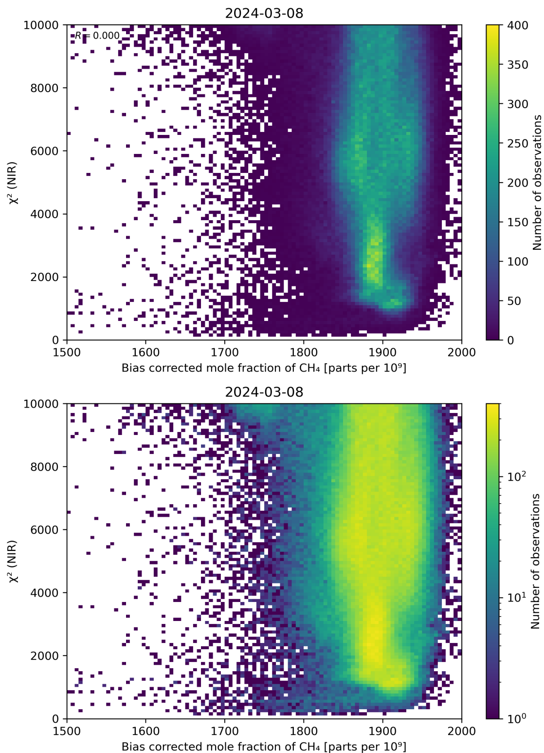
Figure 63: Scatter density plot of “Bias corrected mole fraction of CH 4 ” against “ \chi^2 (NIR)” for 2024-03-07 to 2024-03-09.
