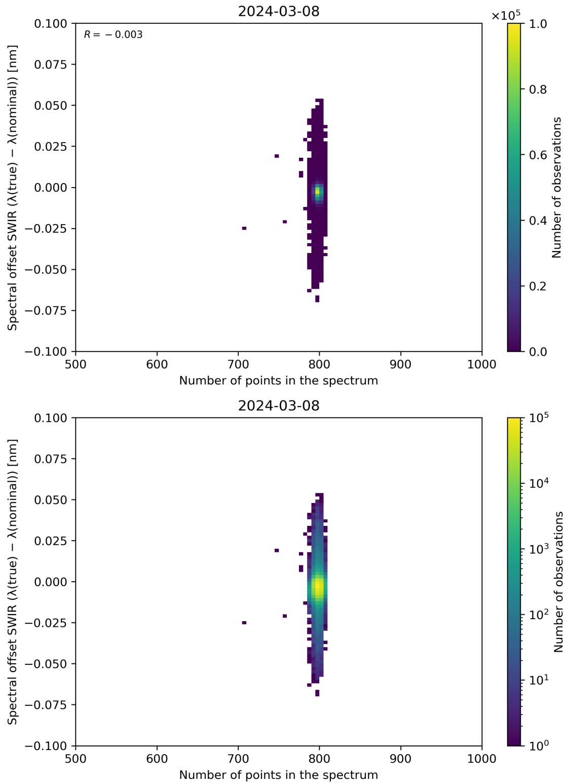
Figure 93: Scatter density plot of “Number of points in the spectrum” against “Spectral offset SWIR ( \lambda(\text{true}) - \lambda(\text{nominal}) )” for 2024-03-07 to 2024-03-09.
