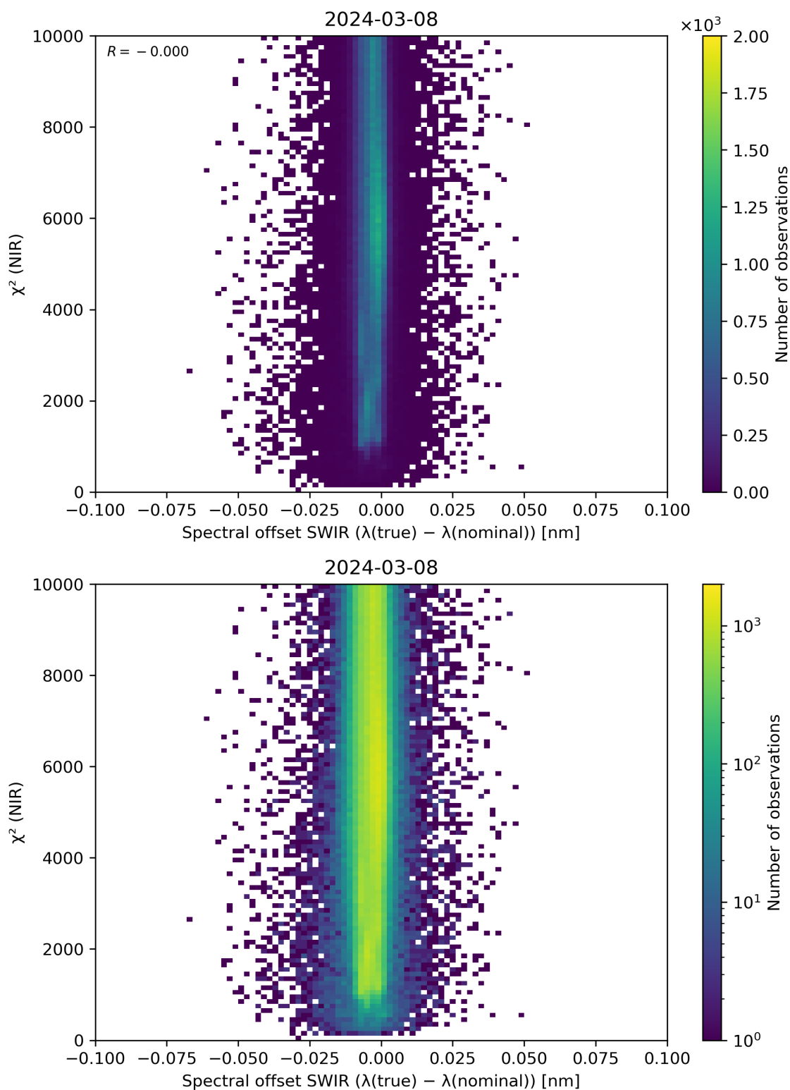
Figure 117: Scatter density plot of “Spectral offset SWIR ( \lambda(\text{true}) - \lambda(\text{nominal}) )” against “ \chi^2 (NIR)” for 2024-03-07 to 2024-03-09.
