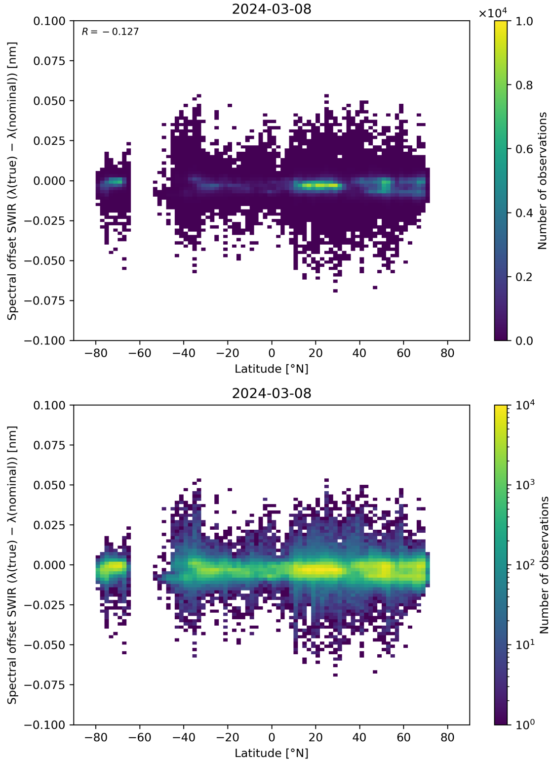
Figure 62: Scatter density plot of “Latitude” against “Spectral offset SWIR ( \lambda(\text{true}) - \lambda(\text{nominal}) )” for 2024-03-07 to 2024-03-09.
