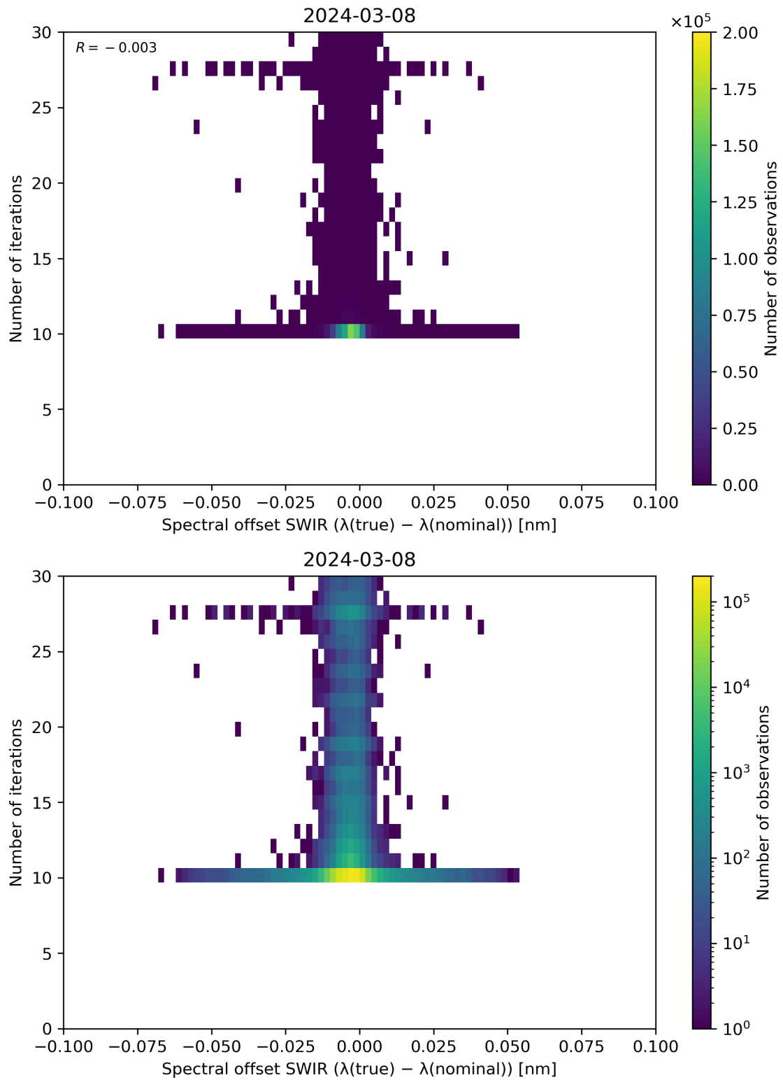
Figure 121: Scatter density plot of “Spectral offset SWIR ( \lambda(\text{true}) - \lambda(\text{nominal}) )” against “Number of iterations” for 2024-03-07 to 2024-03-09.
