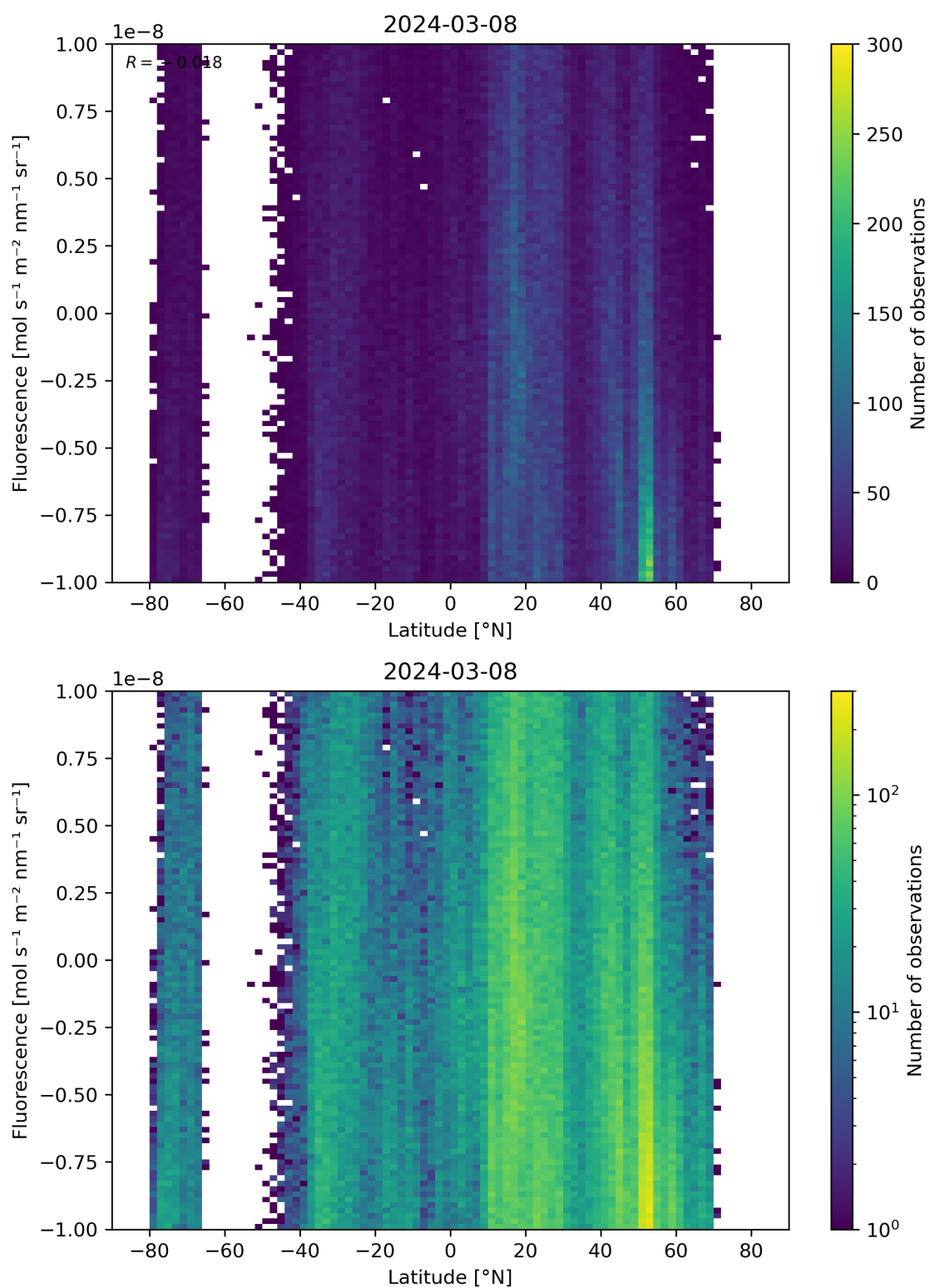
Figure 56: Scatter density plot of “Latitude” against “Fluorescence” for 2024-03-07 to 2024-03-09.
