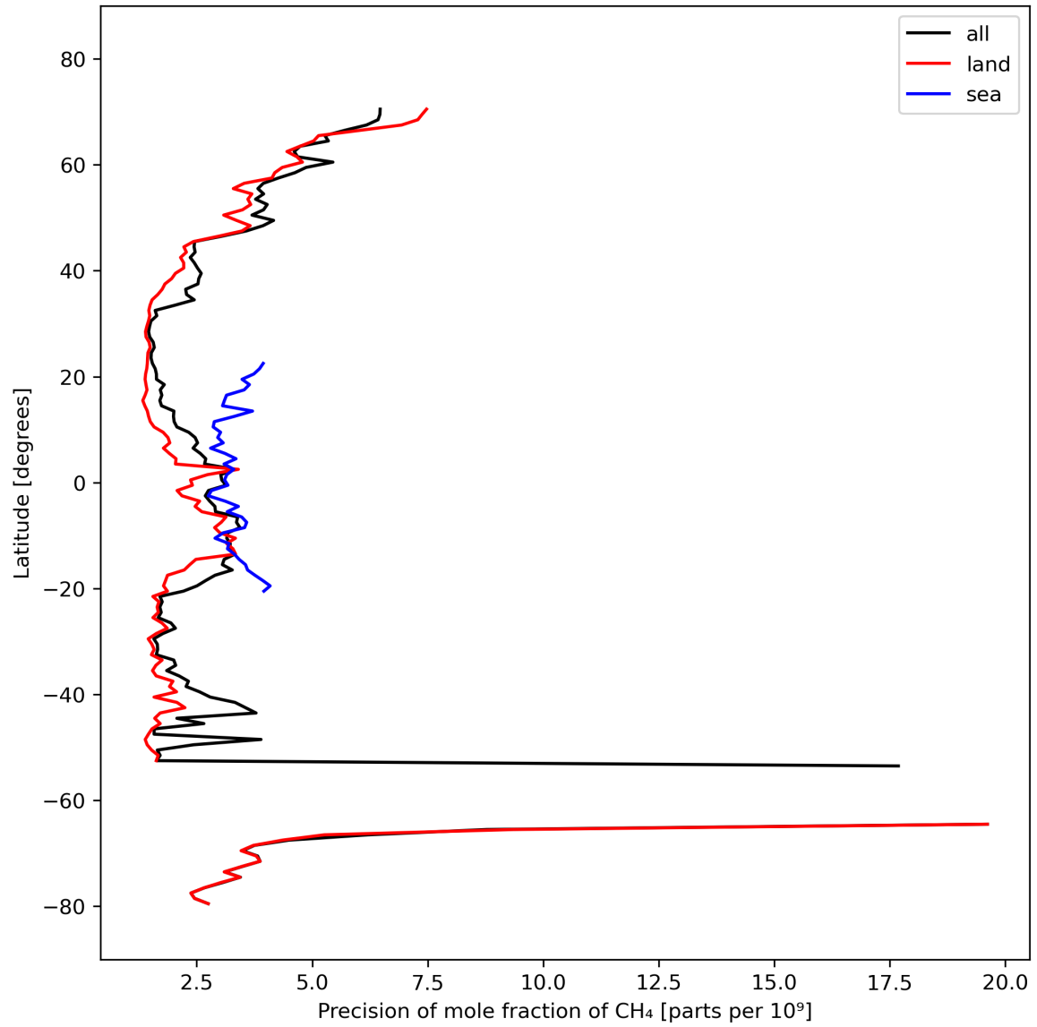
Figure 13: Zonal average of “Precision of mole fraction of CH 4 ” for 2024-03-07 to 2024-03-09.
