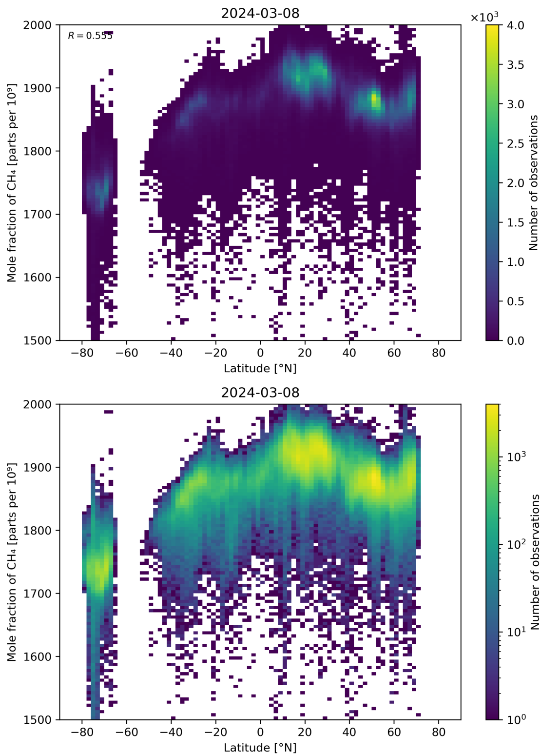
Figure 57: Scatter density plot of “Latitude” against “Mole fraction of \text{CH}_4 ” for 2024-03-07 to 2024-03-09.
