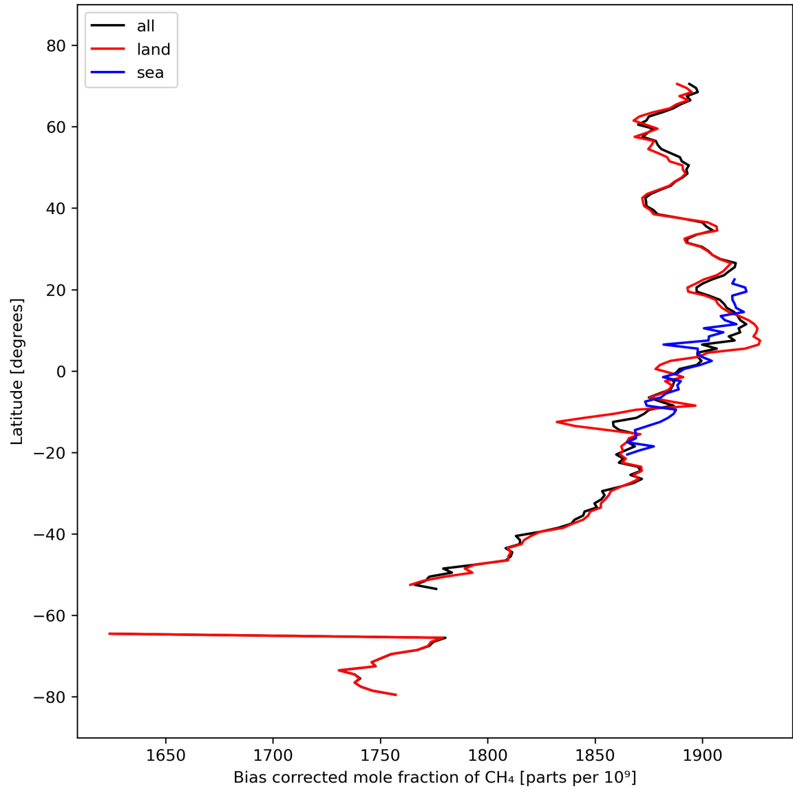
Figure 14: Zonal average of “Bias corrected mole fraction of CH 4 ” for 2024-03-07 to 2024-03-09.
