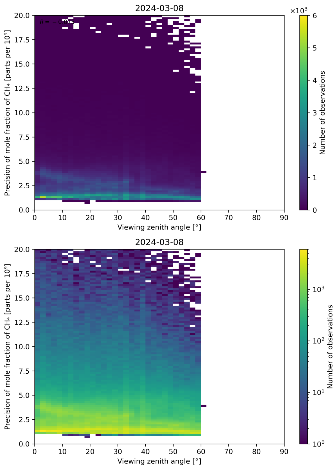
Figure 112: Scatter density plot of “Viewing zenith angle” against “Precision of mole fraction of CH 4 ” for 2024-03-07 to 2024-03-09.
