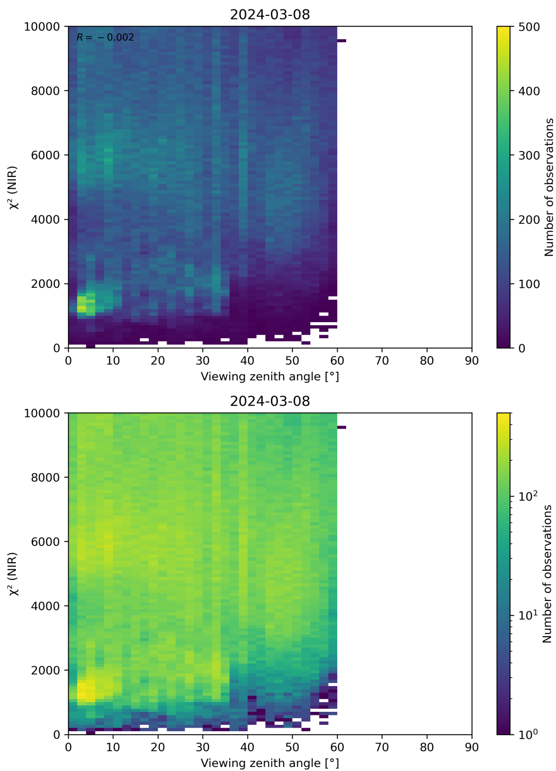
Figure 105: Scatter density plot of “Viewing zenith angle” against “ \chi^2 (NIR)” for 2024-03-07 to 2024-03-09.
