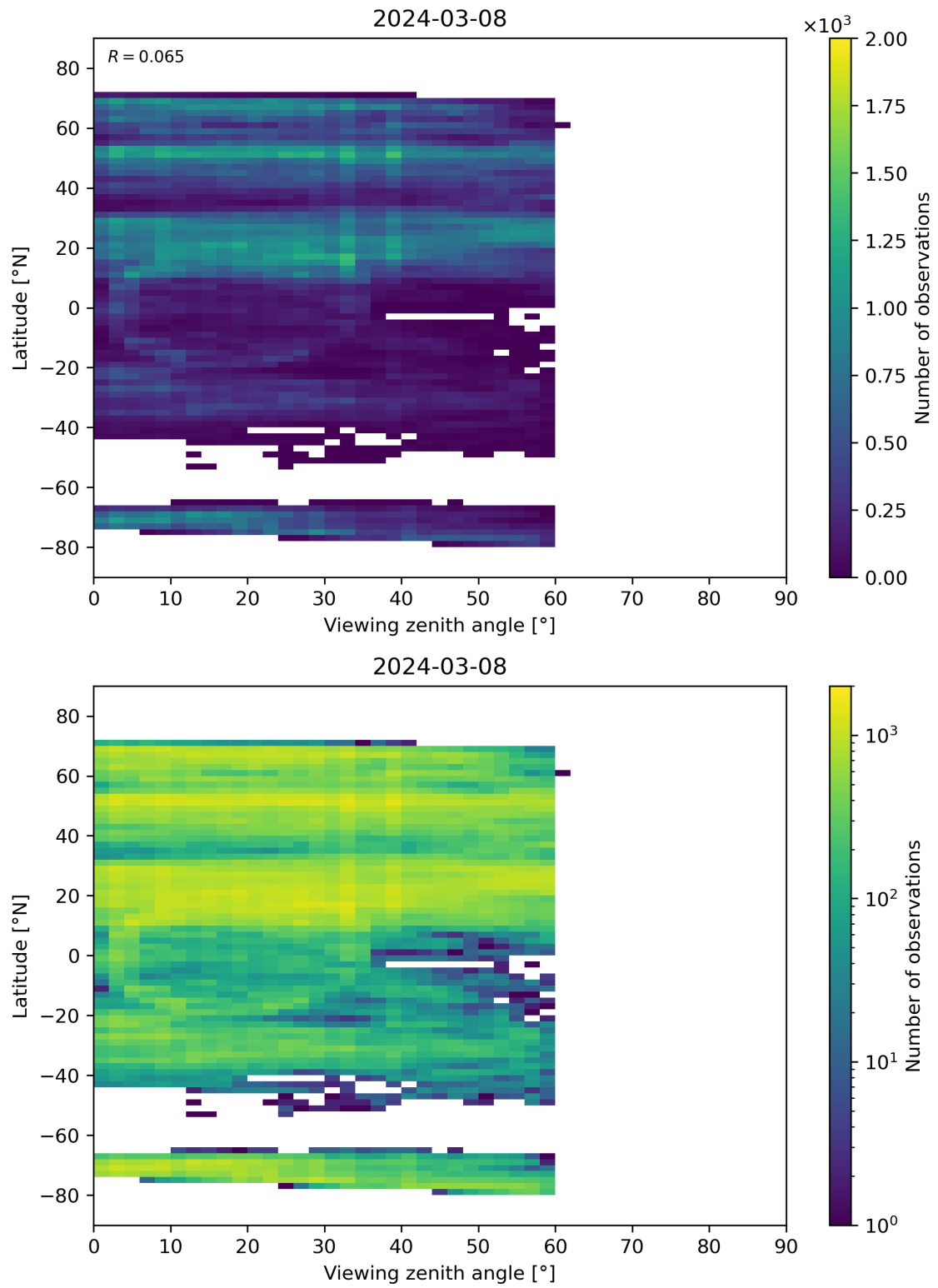
Figure 109: Scatter density plot of “Viewing zenith angle” against “Latitude” for 2024-03-07 to 2024-03-09.
