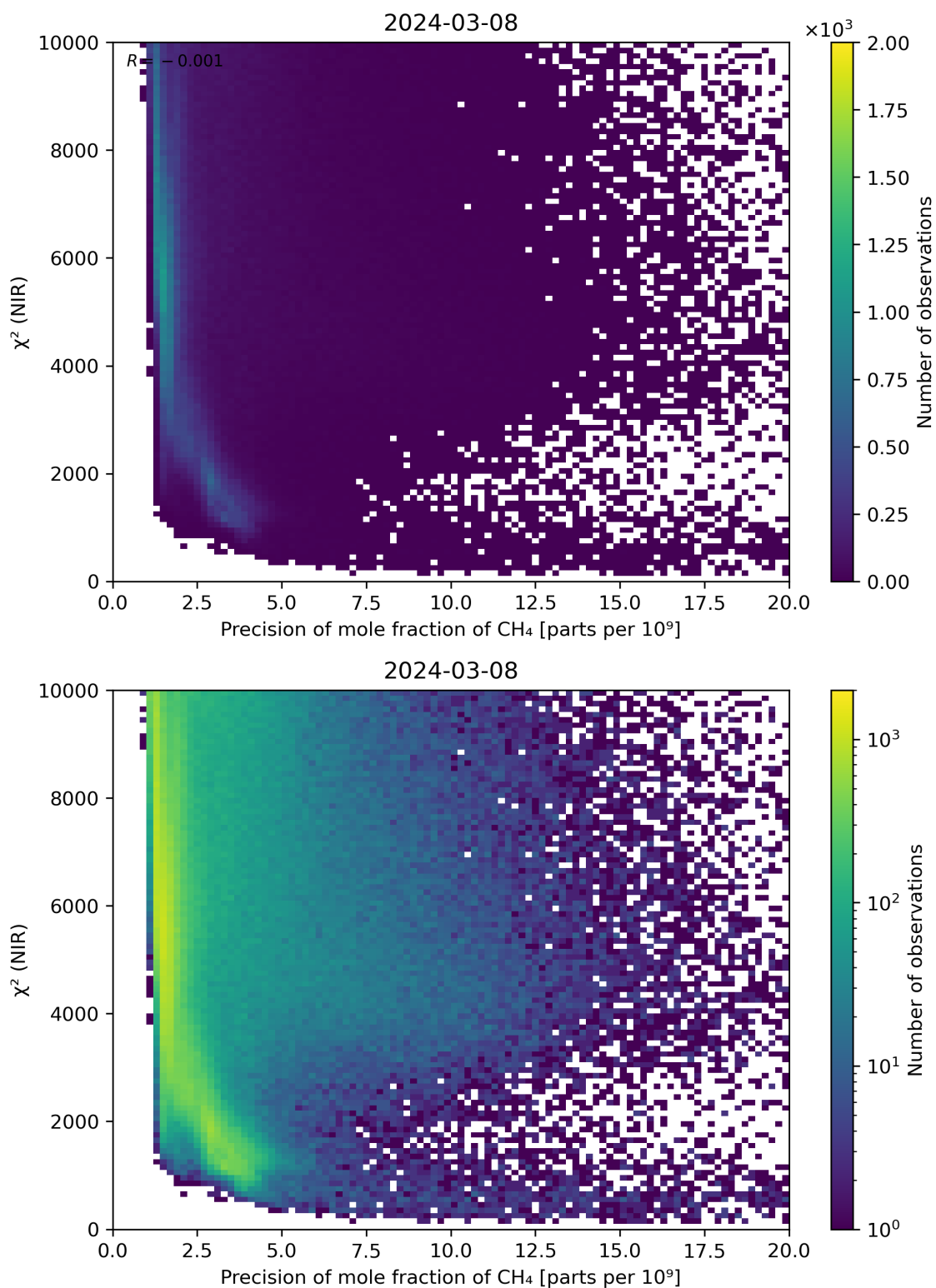
Figure 78: Scatter density plot of “Precision of mole fraction of \text{CH}_4 ” against “ \chi^2 (NIR)” for 2024-03-07 to 2024-03-09.
