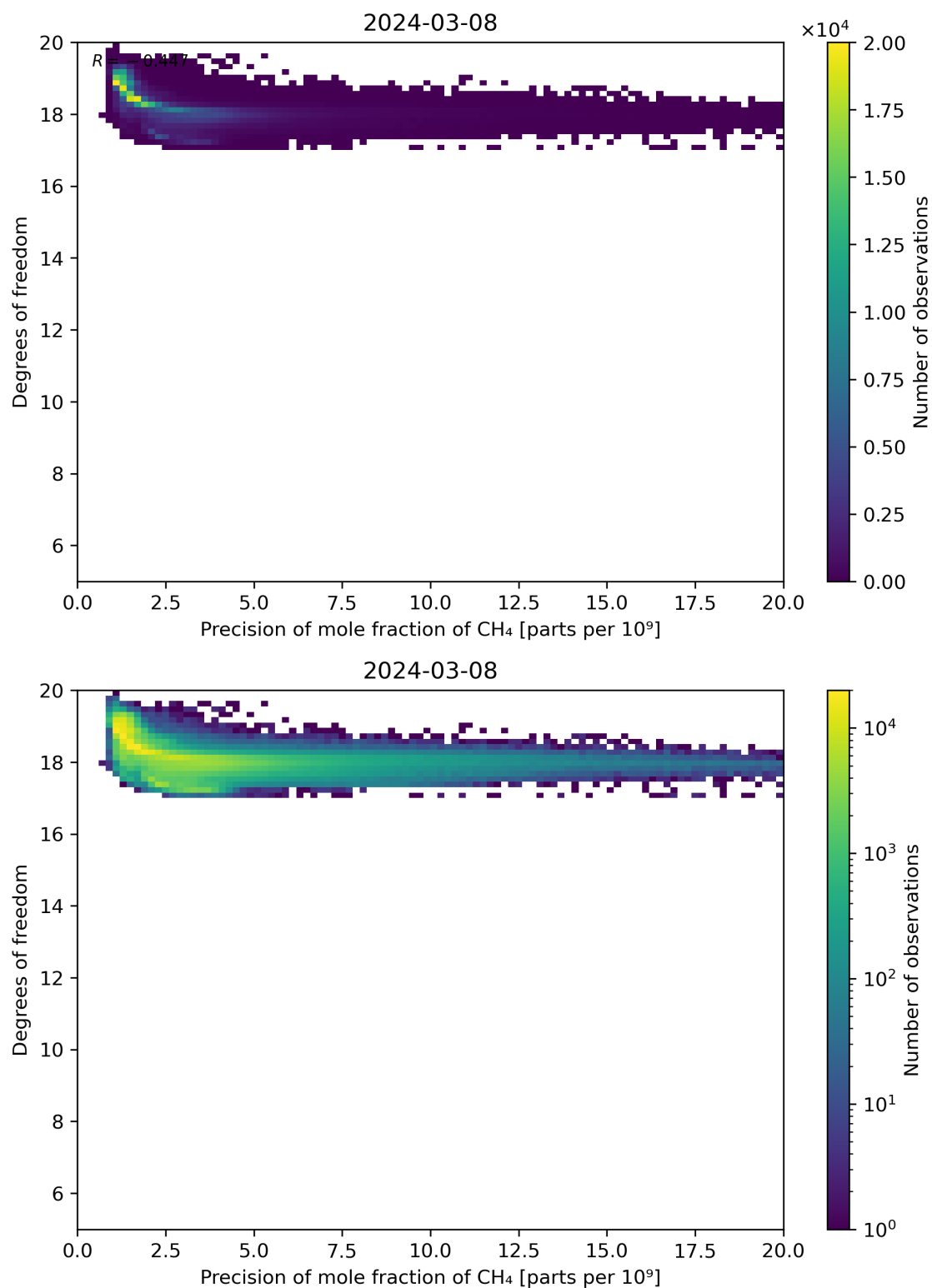
Figure 80: Scatter density plot of “Precision of mole fraction of CH 4 ” against “Degrees of freedom” for 2024-03-07 to 2024-03-09.
