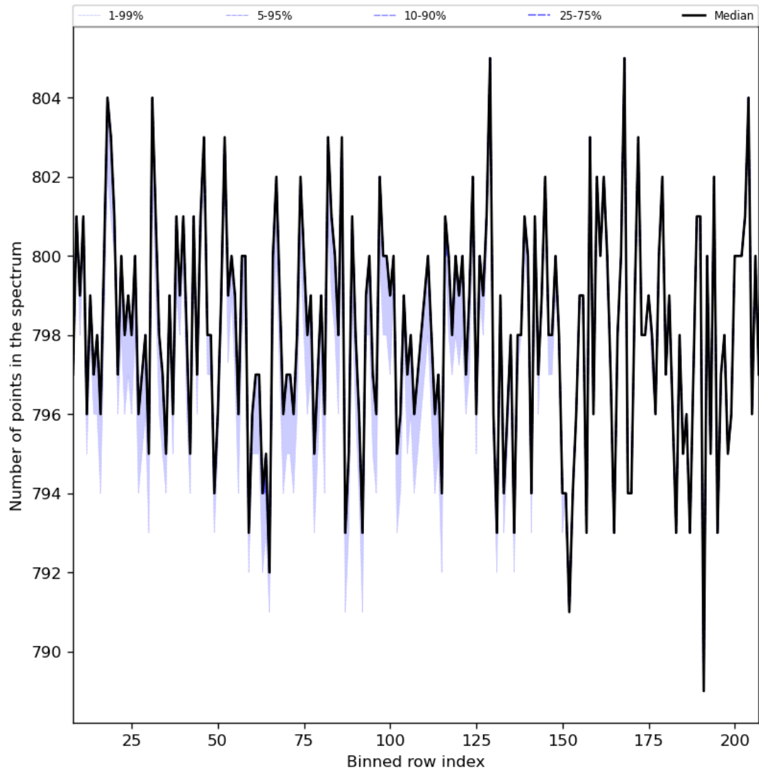
Figure 37: Along track statistics of “Number of points in the spectrum” for 2024-03-07 to 2024-03-09
