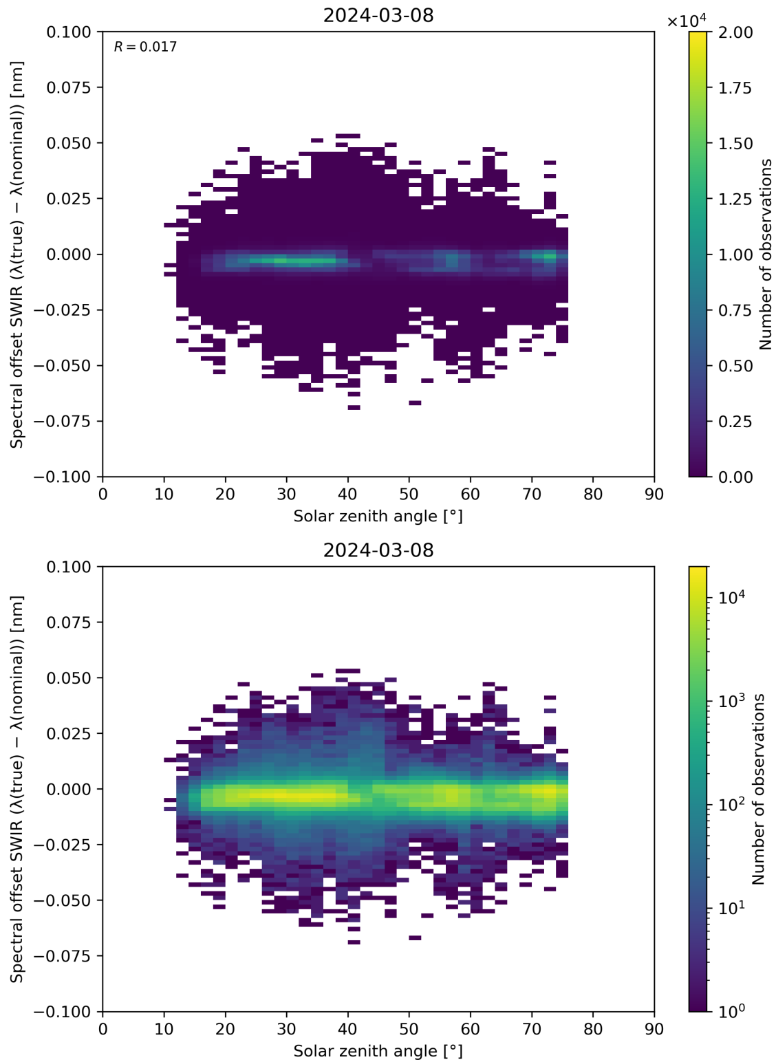
Figure 104: Scatter density plot of “Solar zenith angle” against “Spectral offset SWIR ( \lambda(\text{true}) - \lambda(\text{nominal}) )” for 2024-03-07 to 2024-03-09.
