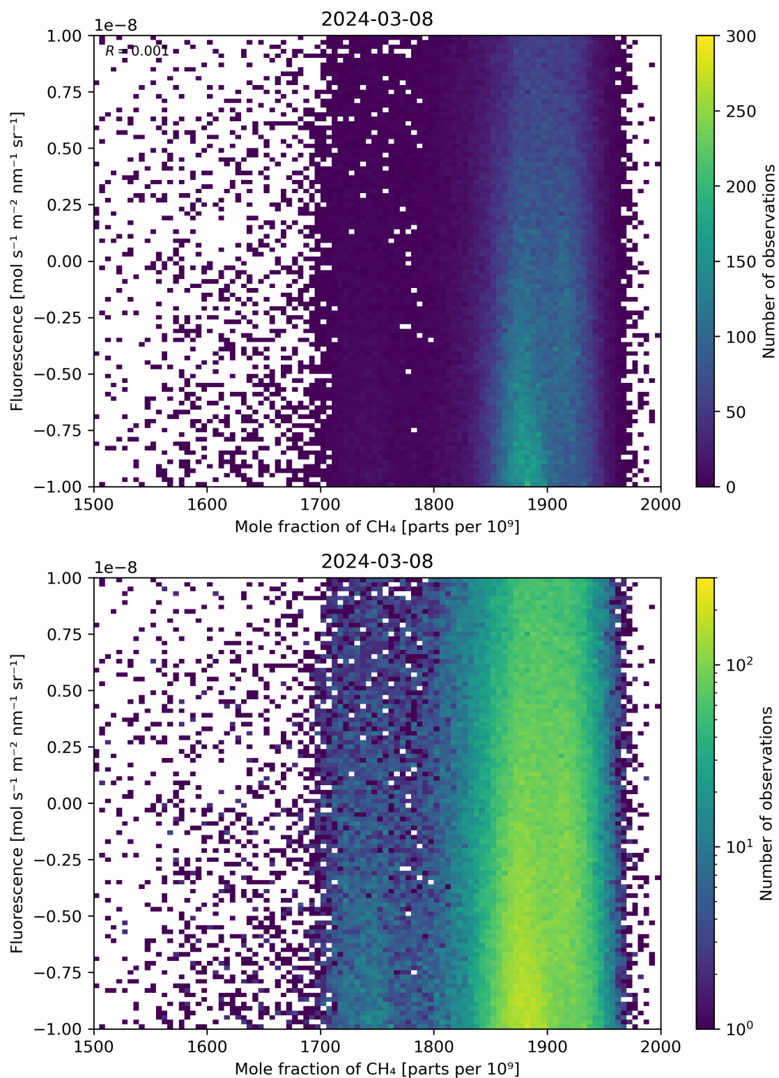
Figure 73: Scatter density plot of “Mole fraction of \text{CH}_4 ” against “Fluorescence” for 2024-03-07 to 2024-03-09.
