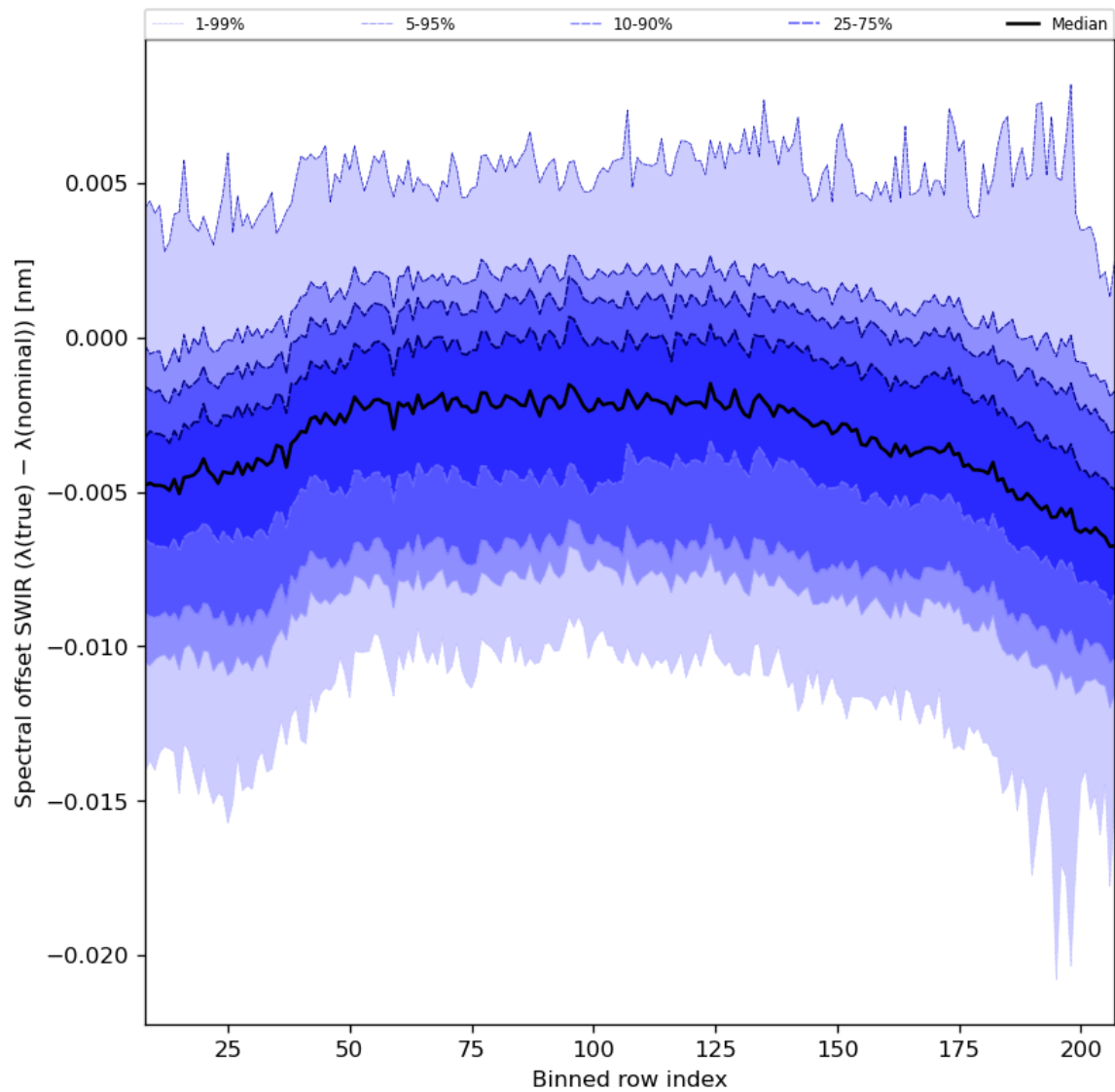
Figure 38: Along track statistics of “Spectral offset SWIR ( \lambda(\text{true}) - \lambda(\text{nominal}) )” for 2024-03-07 to 2024-03-09
