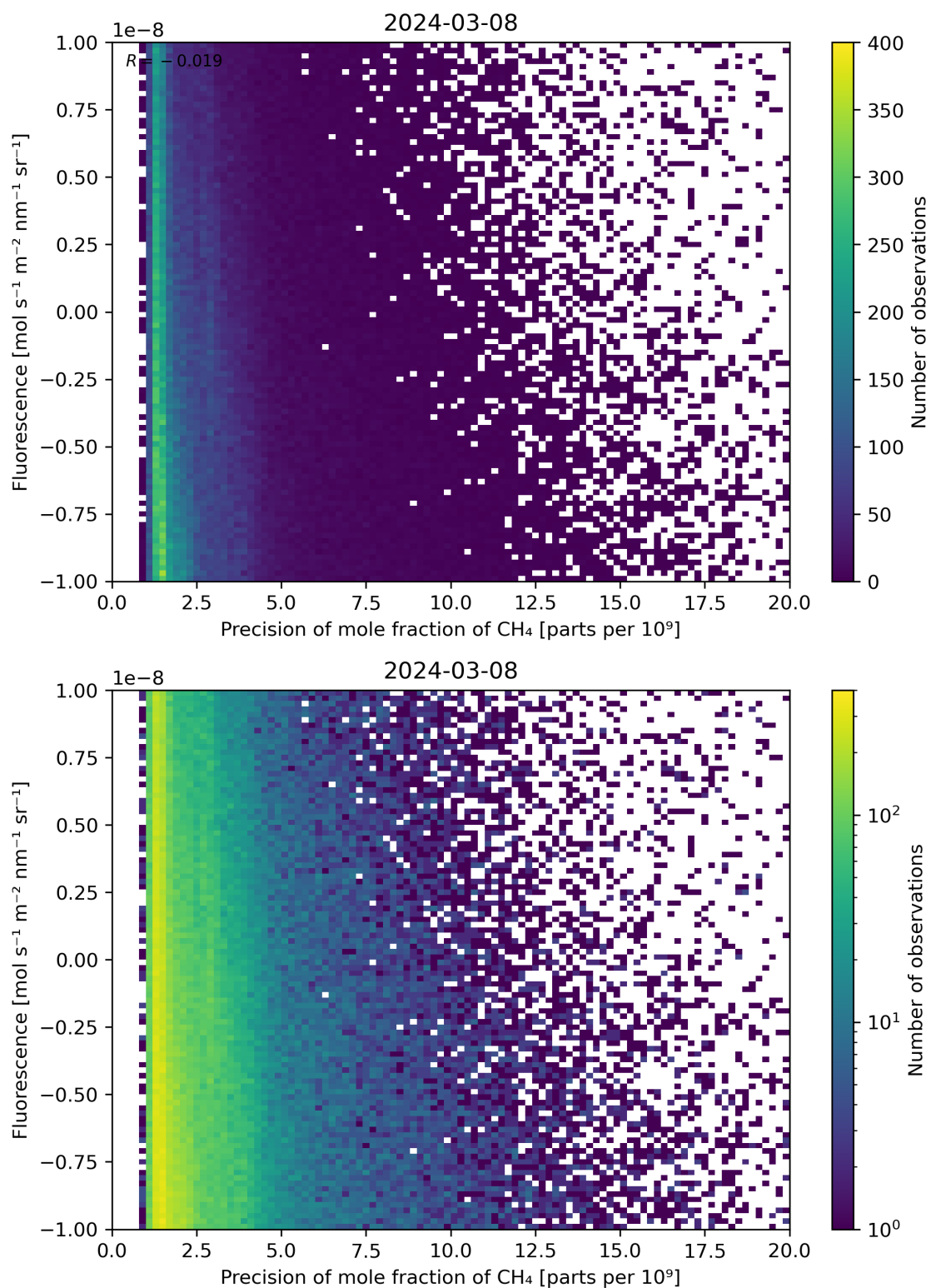
Figure 81: Scatter density plot of “Precision of mole fraction of \text{CH}_4 ” against “Fluorescence” for 2024-03-07 to 2024-03-09.
