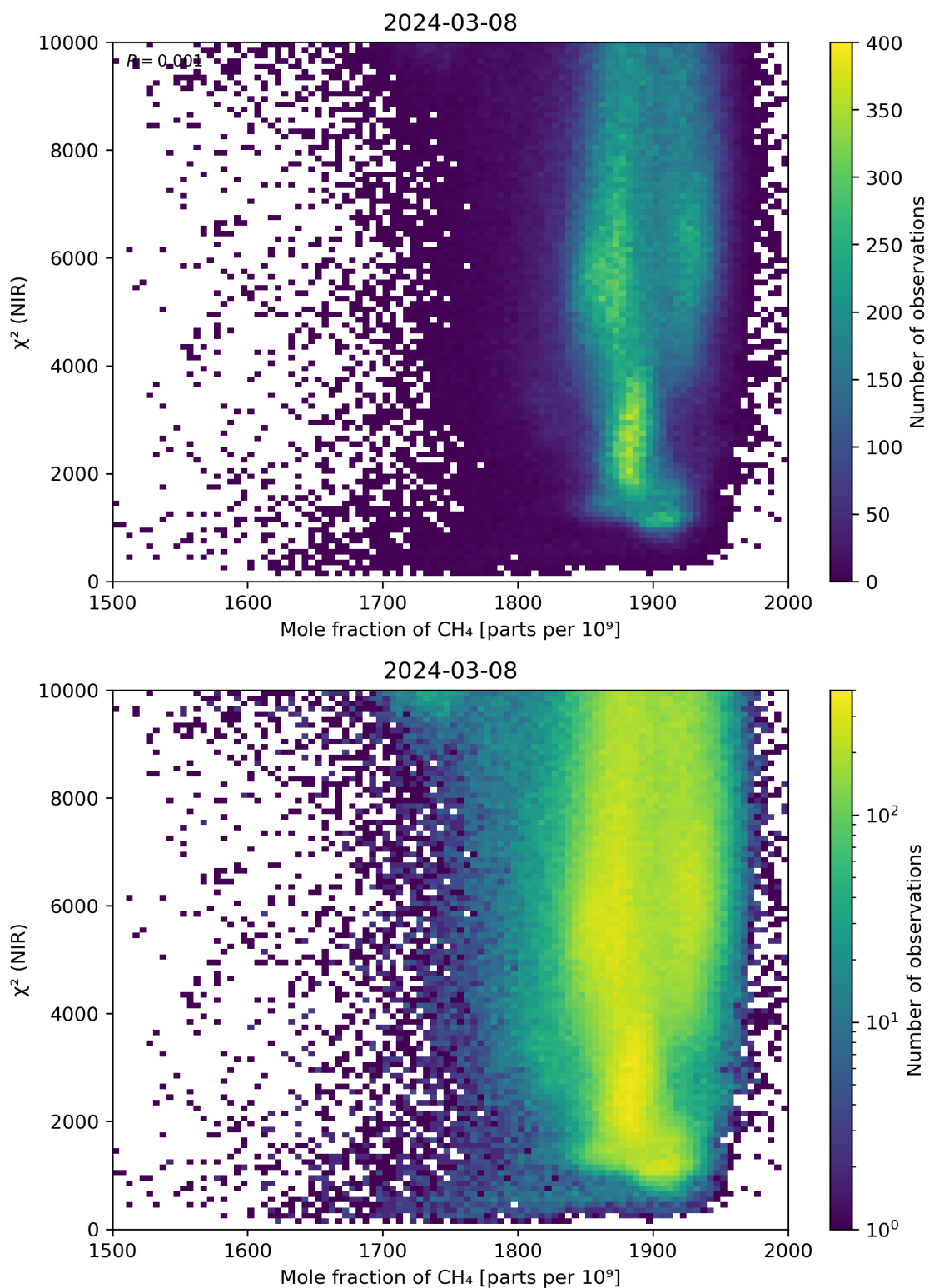
Figure 70: Scatter density plot of “Mole fraction of \text{CH}_4 ” against “ \chi^2 (NIR)” for 2024-03-07 to 2024-03-09.
