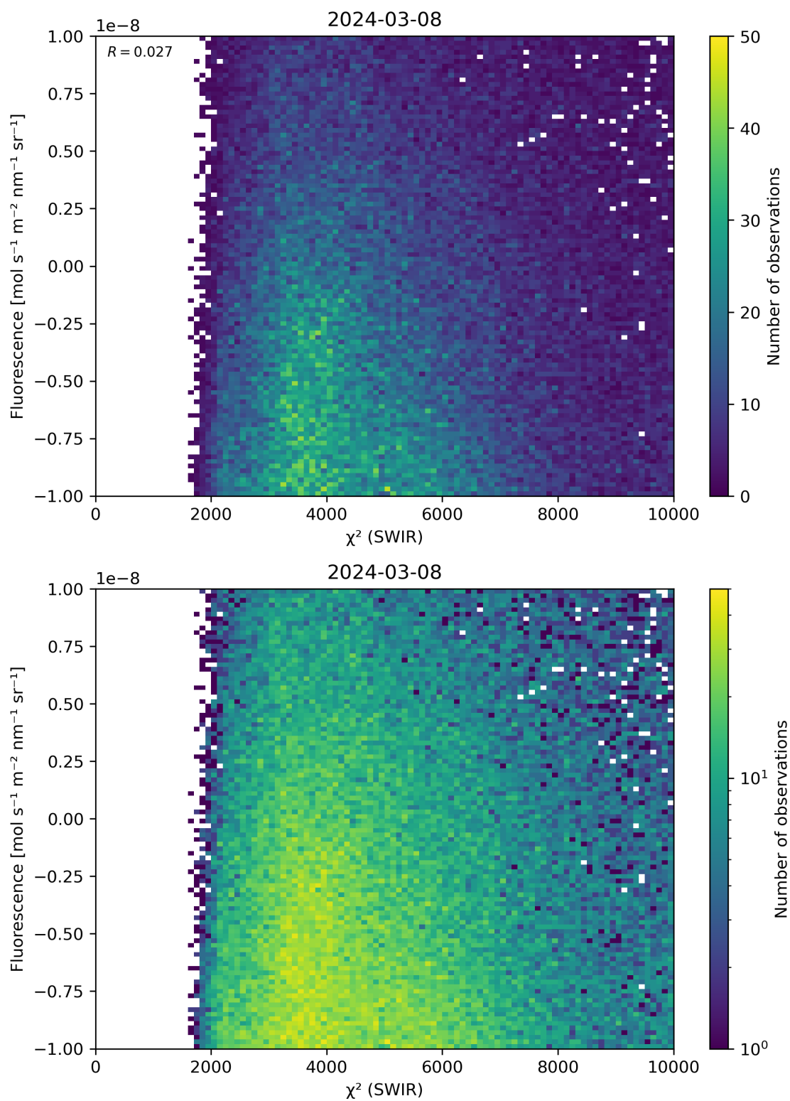
Figure 49: Scatter density plot of “ \chi^2 (SWIR)” against “Fluorescence” for 2024-03-07 to 2024-03-09.
