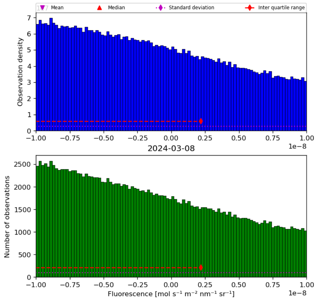
Figure 32: Histogram of “Fluorescence” for 2024-03-07 to 2024-03-09
