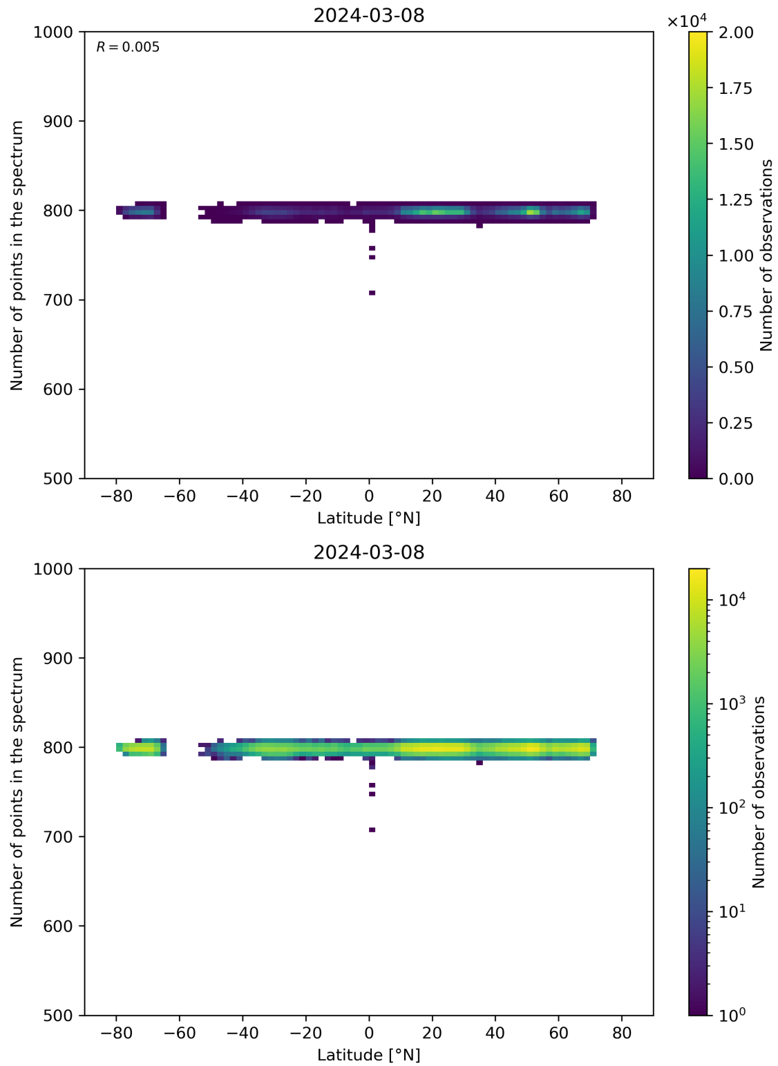
Figure 61: Scatter density plot of “Latitude” against “Number of points in the spectrum” for 2024-03-07 to 2024-03-09.
