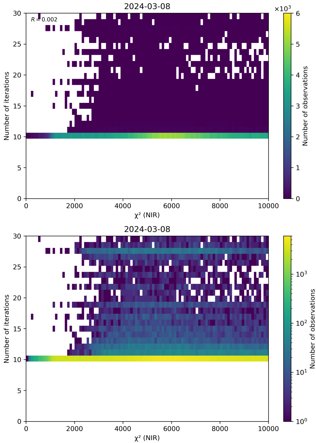
Figure 46: Scatter density plot of “ \chi^2 (NIR)” against “Number of iterations” for 2024-03-07 to 2024-03-09.
