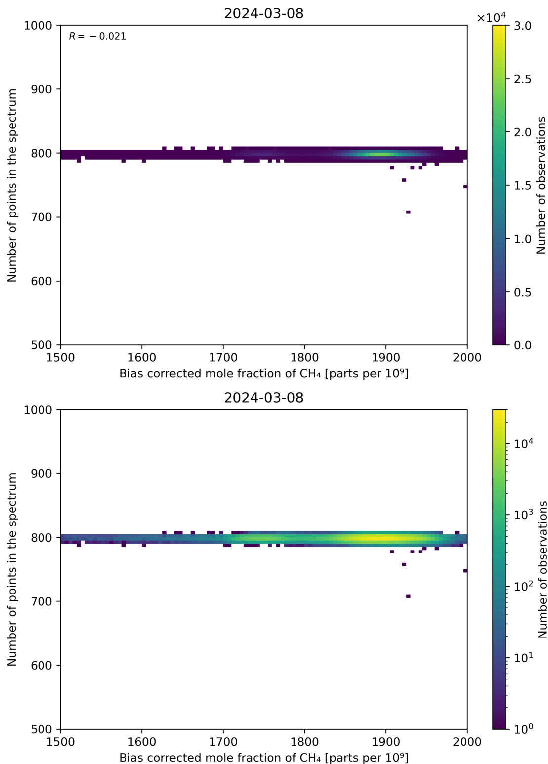
Figure 68: Scatter density plot of “Bias corrected mole fraction of CH 4 ” against “Number of points in the spectrum” for 2024-03-07 to 2024-03-09.
