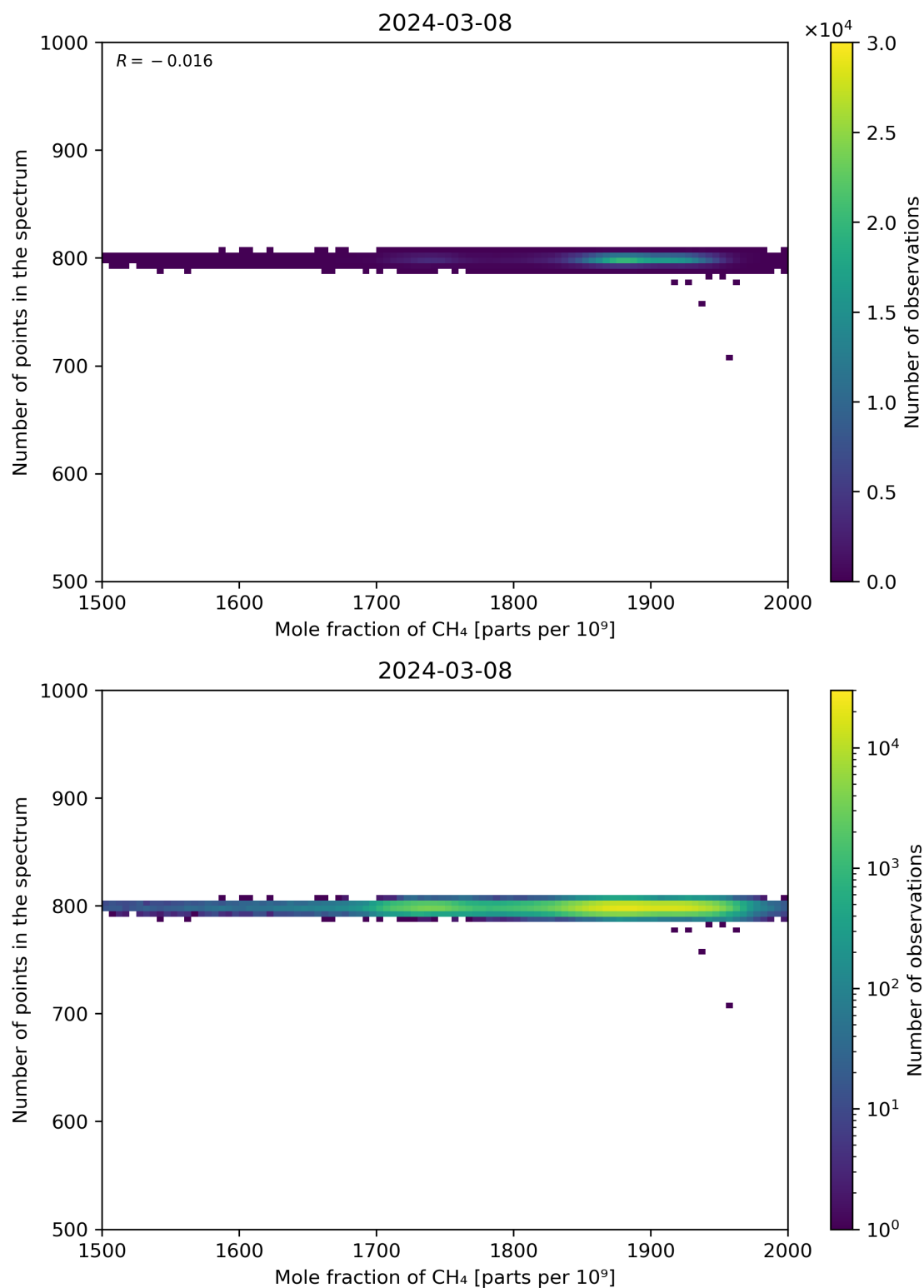
Figure 77: Scatter density plot of “Mole fraction of CH 4 ” against “Number of points in the spectrum” for 2024-03-07 to 2024-03-09.
