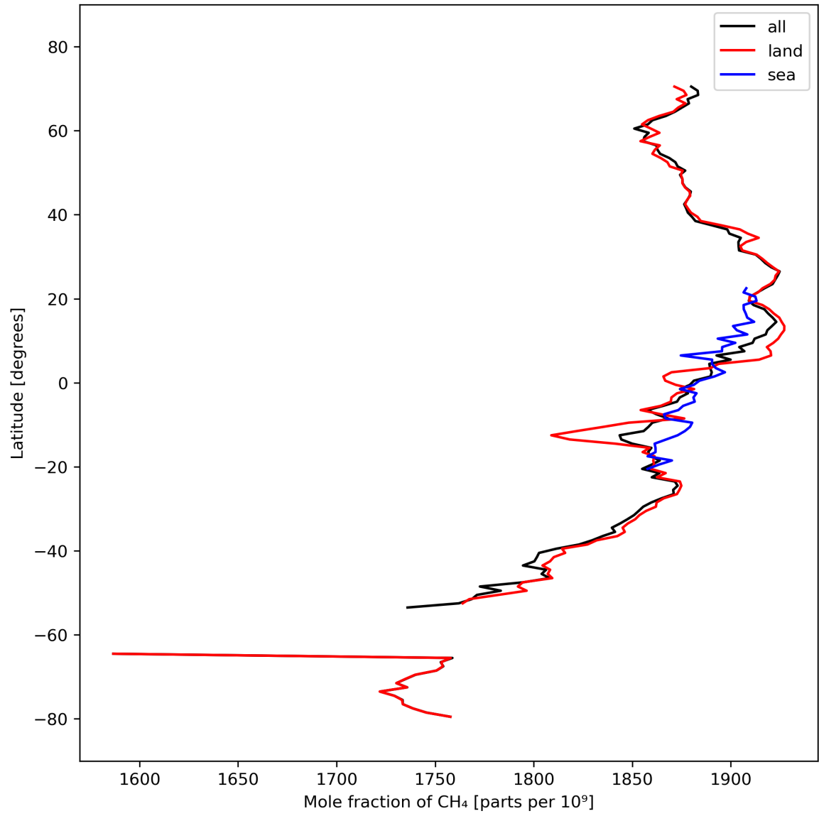
Figure 12: Zonal average of “Mole fraction of \text{CH}_4 ” for 2024-03-07 to 2024-03-09.
