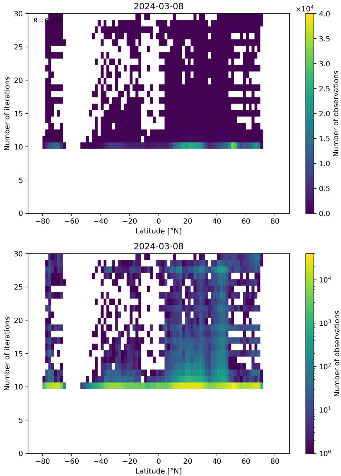
Figure 60: Scatter density plot of “Latitude” against “Number of iterations” for 2024-03-07 to 2024-03-09.
