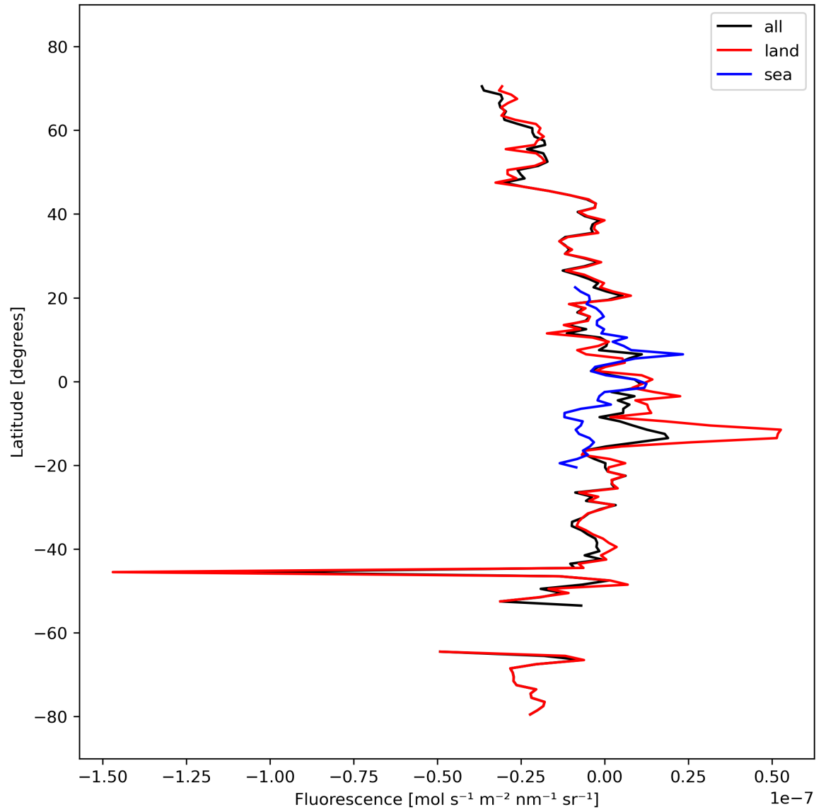
Figure 21: Zonal average of “Fluorescence” for 2024-03-07 to 2024-03-09.
