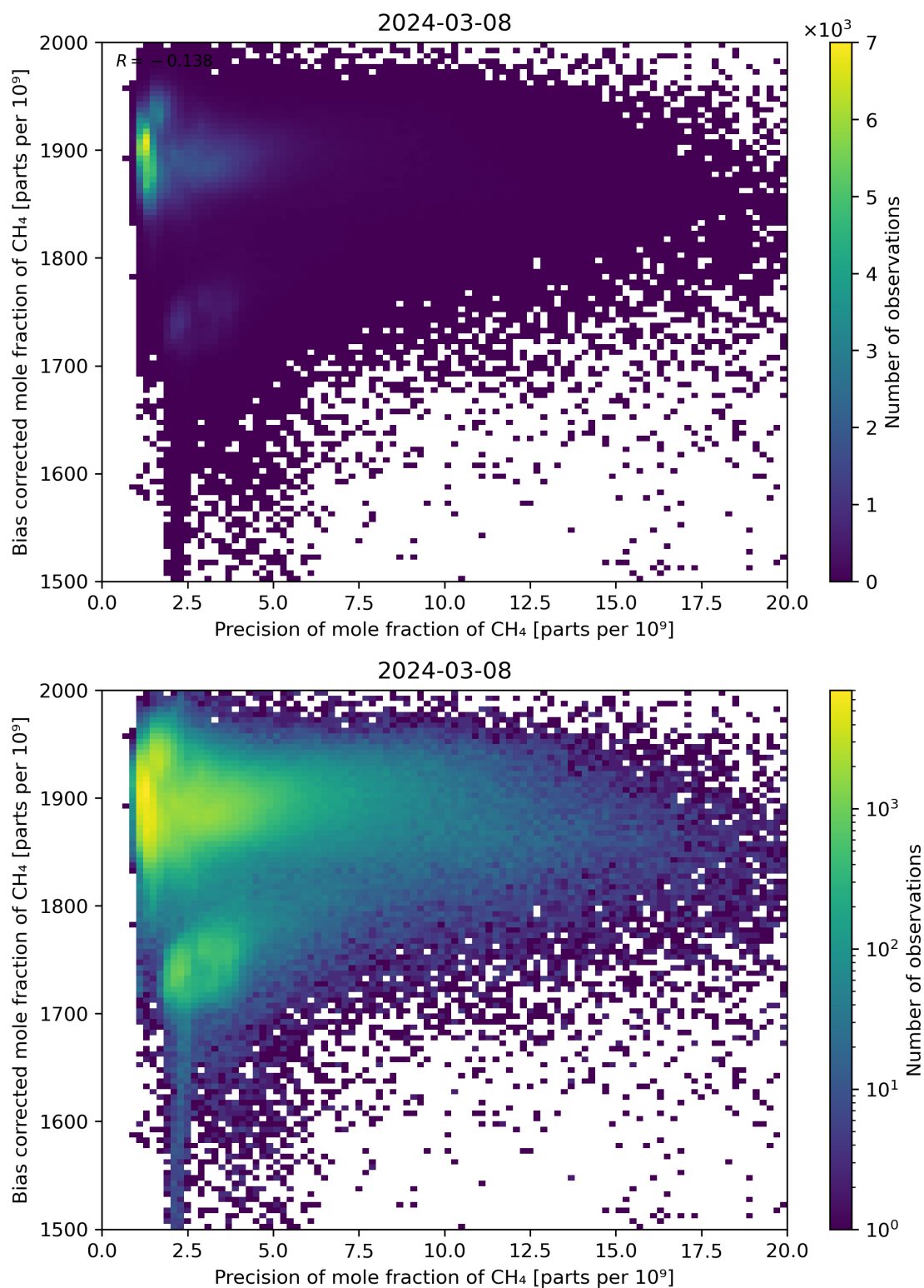
Figure 82: Scatter density plot of “Precision of mole fraction of CH 4 ” against “Bias corrected mole fraction of CH 4 ” for 2024-03-07 to 2024-03-09.
