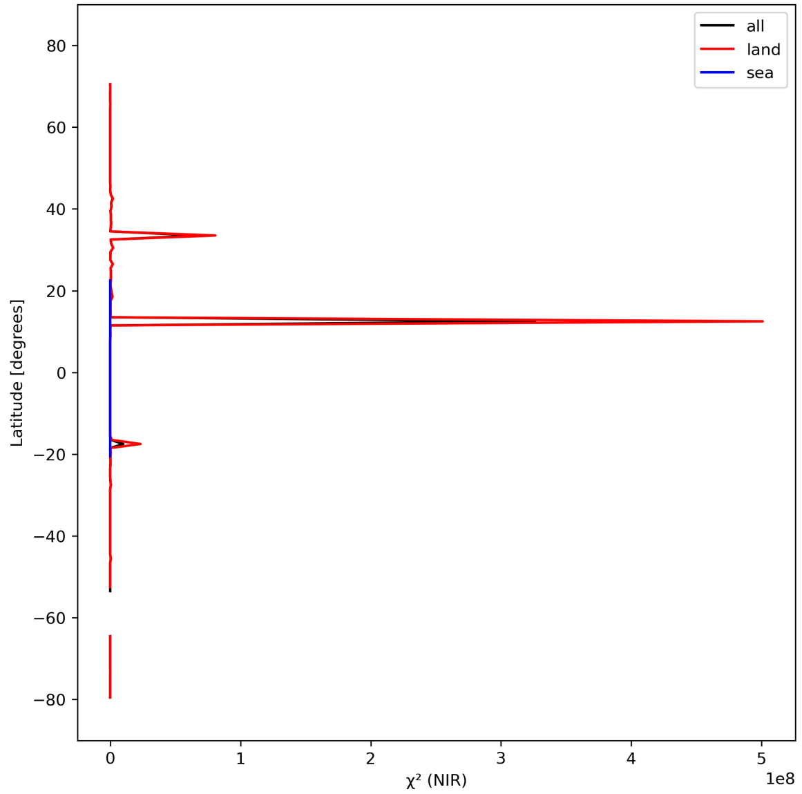
Figure 18: Zonal average of “ \chi^2 (NIR)” for 2024-03-07 to 2024-03-09.
