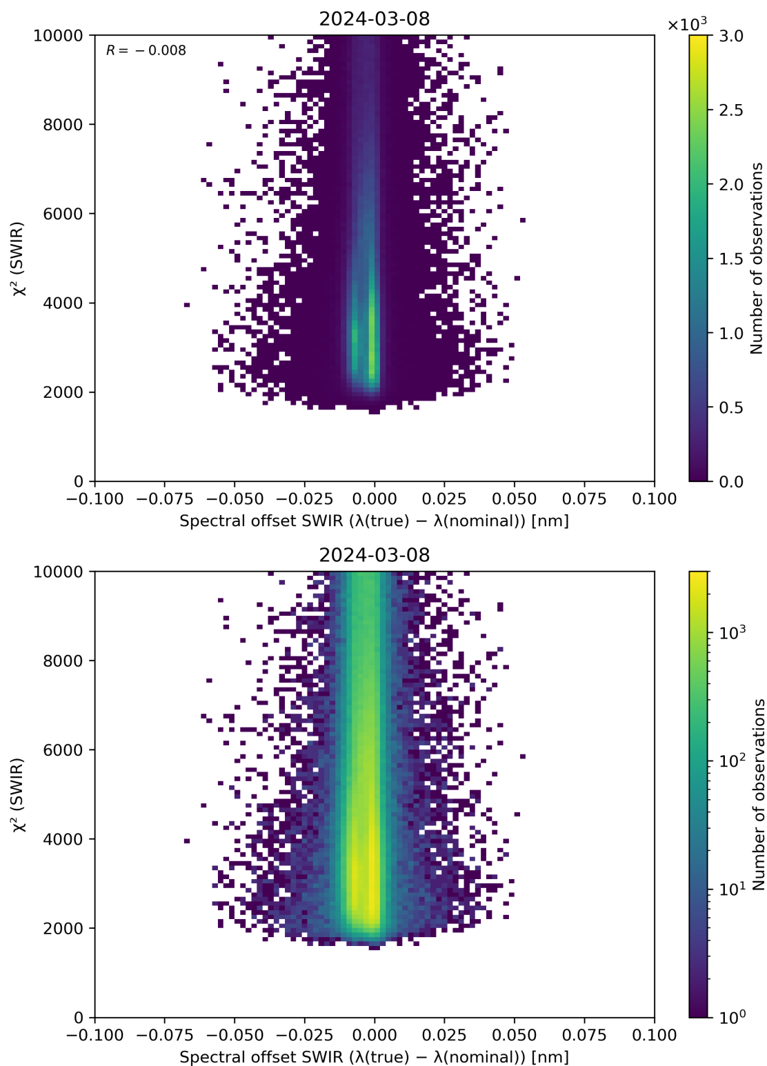
Figure 118: Scatter density plot of “Spectral offset SWIR ( \lambda(\text{true}) - \lambda(\text{nominal}) )” against “ \chi^2 (SWIR)” for 2024-03-07 to 2024-03-09.
