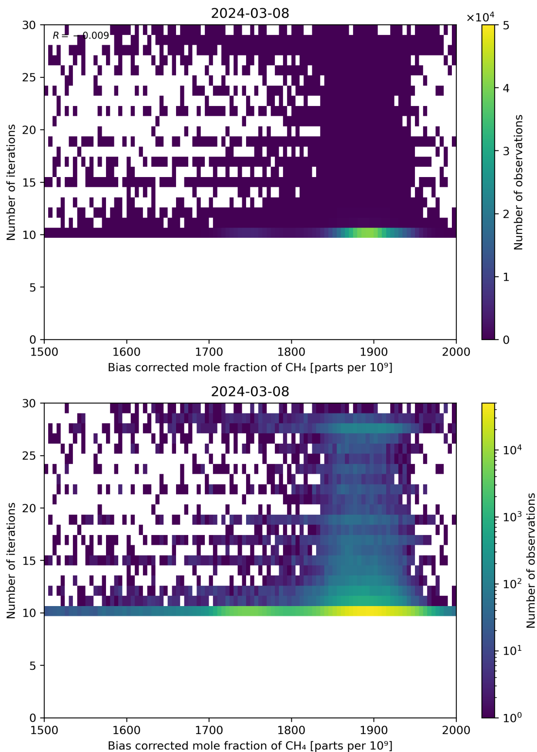
Figure 67: Scatter density plot of “Bias corrected mole fraction of CH 4 ” against “Number of iterations” for 2024-03-07 to 2024-03-09.
