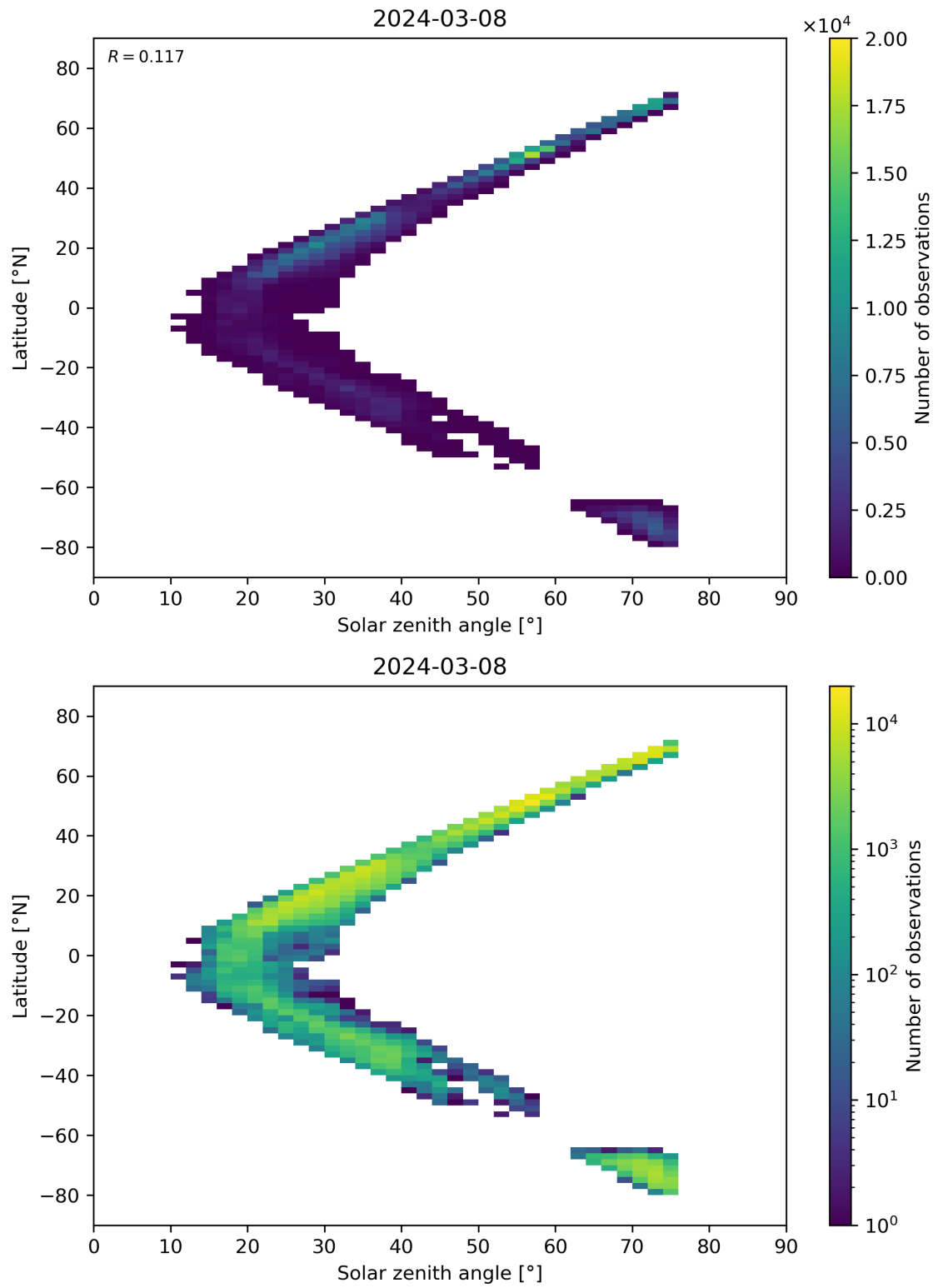
Figure 98: Scatter density plot of “Solar zenith angle” against “Latitude” for 2024-03-07 to 2024-03-09.
