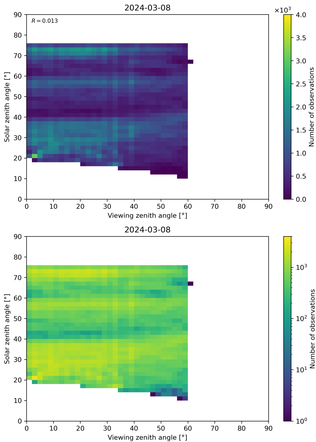
Figure 115: Scatter density plot of “Viewing zenith angle” against “Solar zenith angle” for 2024-03-07 to 2024-03-09.
