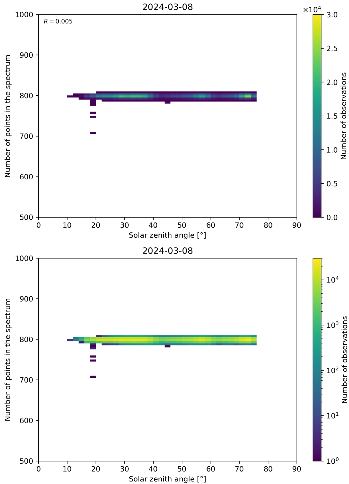
Figure 103: Scatter density plot of “Solar zenith angle” against “Number of points in the spectrum” for 2024-03-07 to 2024-03-09.
