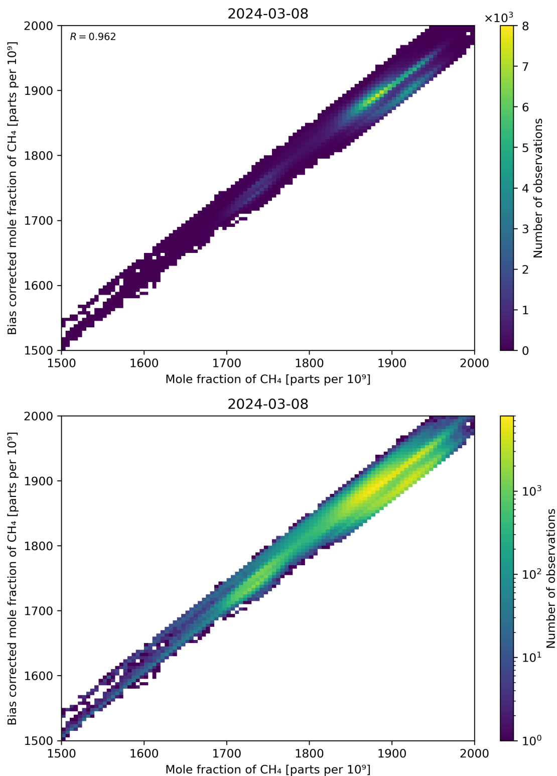
Figure 74: Scatter density plot of “Mole fraction of CH 4 ” against “Bias corrected mole fraction of CH 4 ” for 2024-03-07 to 2024-03-09.
