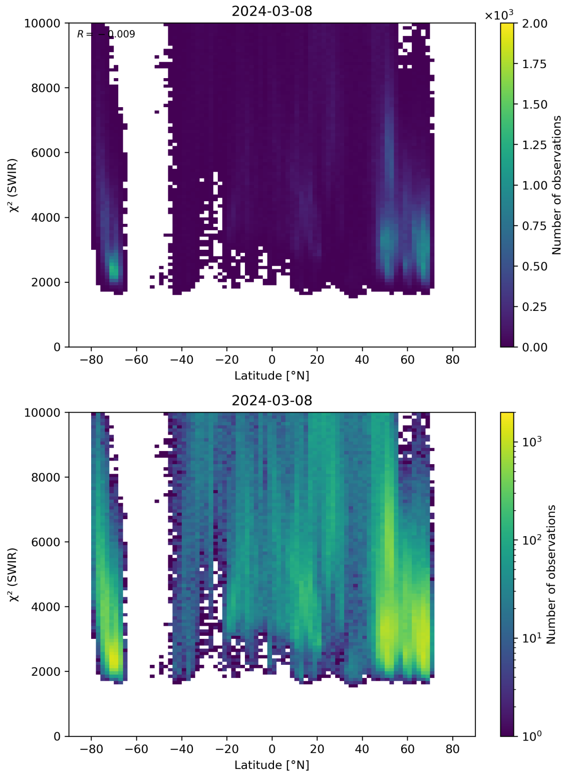
Figure 54: Scatter density plot of “Latitude” against “ \chi^2 (SWIR)” for 2024-03-07 to 2024-03-09.
