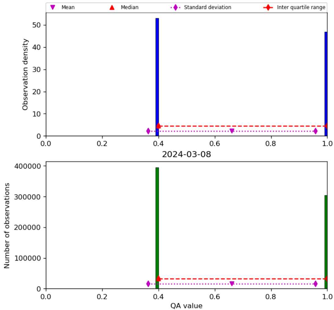
Figure 22: Histogram of “QA value” for 2024-03-07 to 2024-03-09
