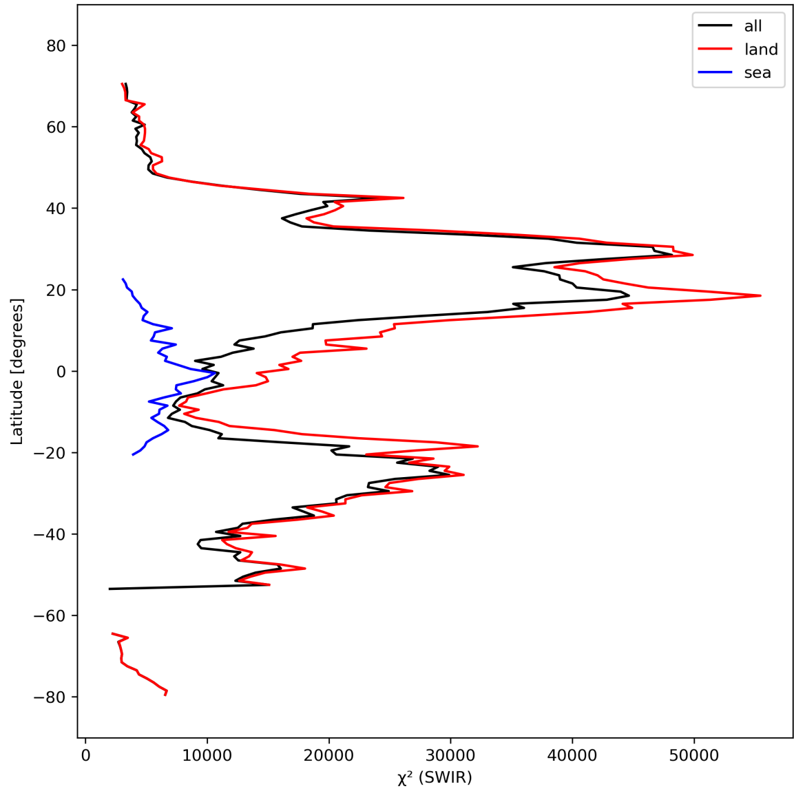
Figure 17: Zonal average of “ \chi^2 (SWIR)” for 2024-03-07 to 2024-03-09.
