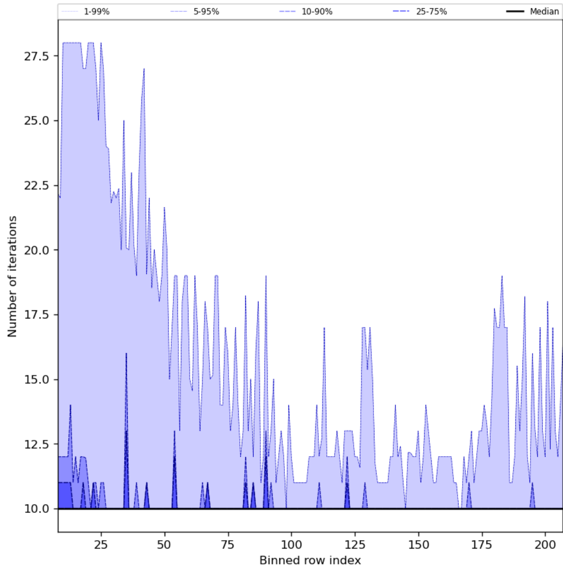
Figure 42: Along track statistics of “Number of iterations” for 2024-03-07 to 2024-03-09
