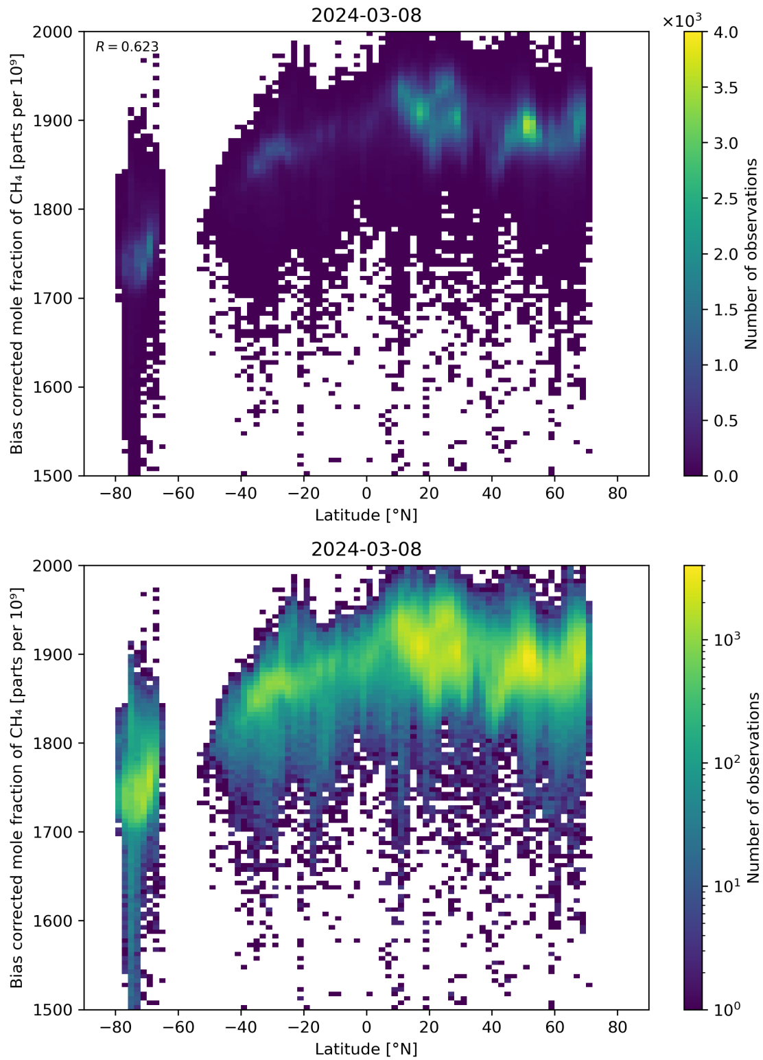
Figure 58: Scatter density plot of “Latitude” against “Bias corrected mole fraction of CH 4 ” for 2024-03-07 to 2024-03-09.
