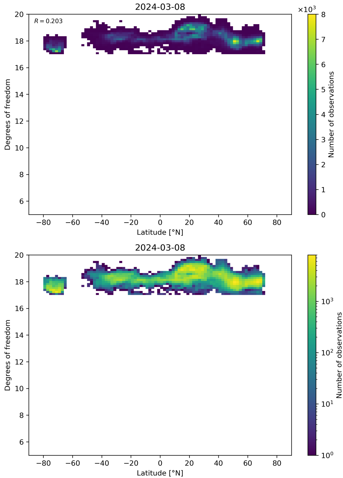
Figure 55: Scatter density plot of “Latitude” against “Degrees of freedom” for 2024-03-07 to 2024-03-09.
