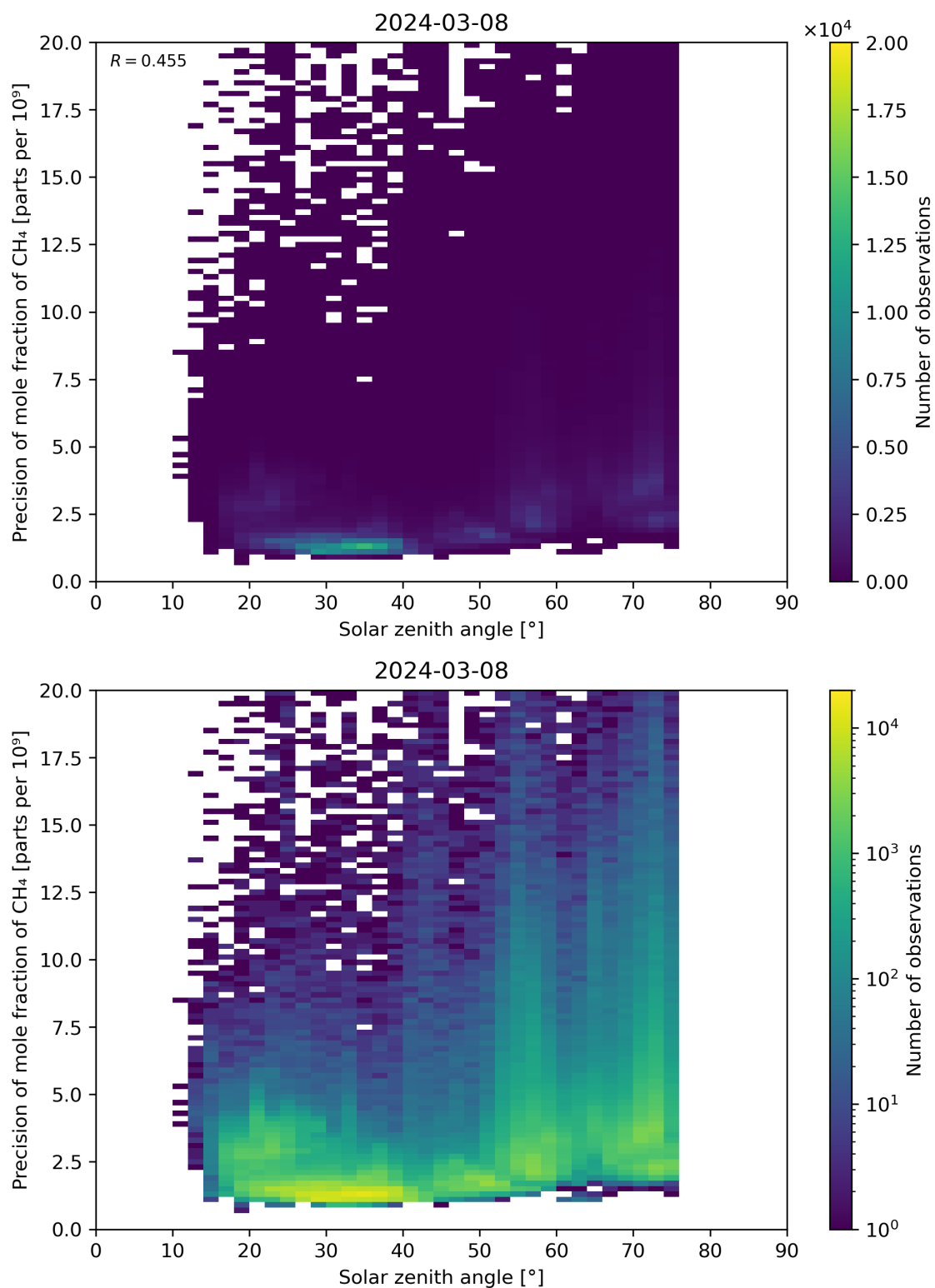
Figure 101: Scatter density plot of “Solar zenith angle” against “Precision of mole fraction of CH 4 ” for 2024-03-07 to 2024-03-09.
