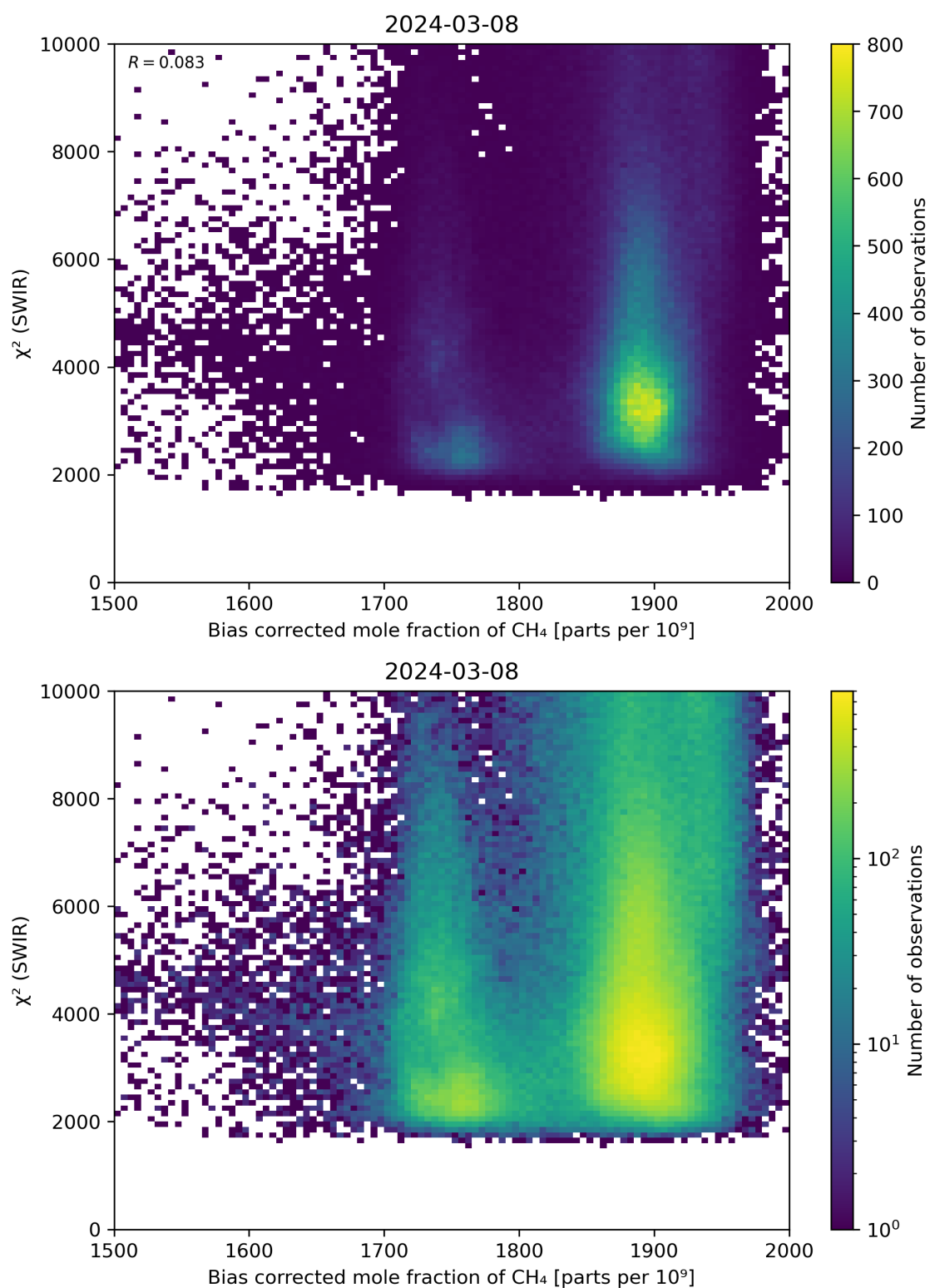
Figure 64: Scatter density plot of “Bias corrected mole fraction of CH 4 ” against “ \chi^2 (SWIR)” for 2024-03-07 to 2024-03-09.
