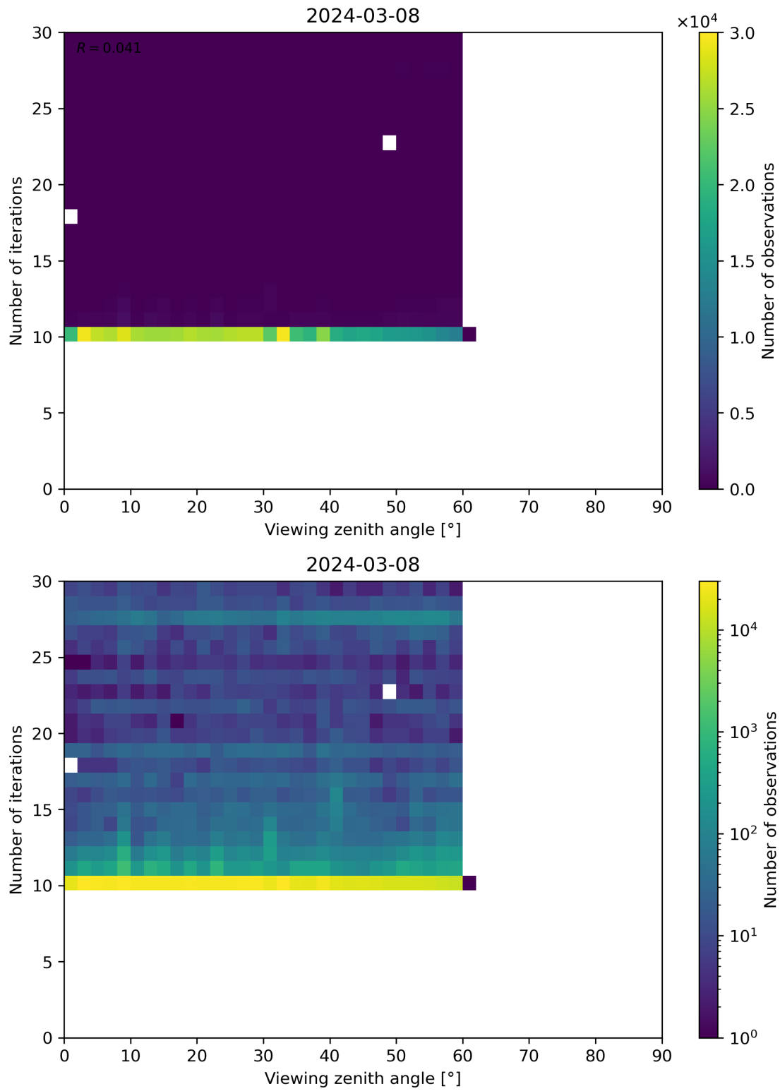
Figure 113: Scatter density plot of “Viewing zenith angle” against “Number of iterations” for 2024-03-07 to 2024-03-09.
