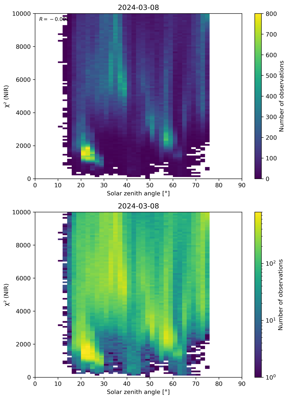
Figure 94: Scatter density plot of “Solar zenith angle” against “ \chi^2 (NIR)” for 2024-03-07 to 2024-03-09.
