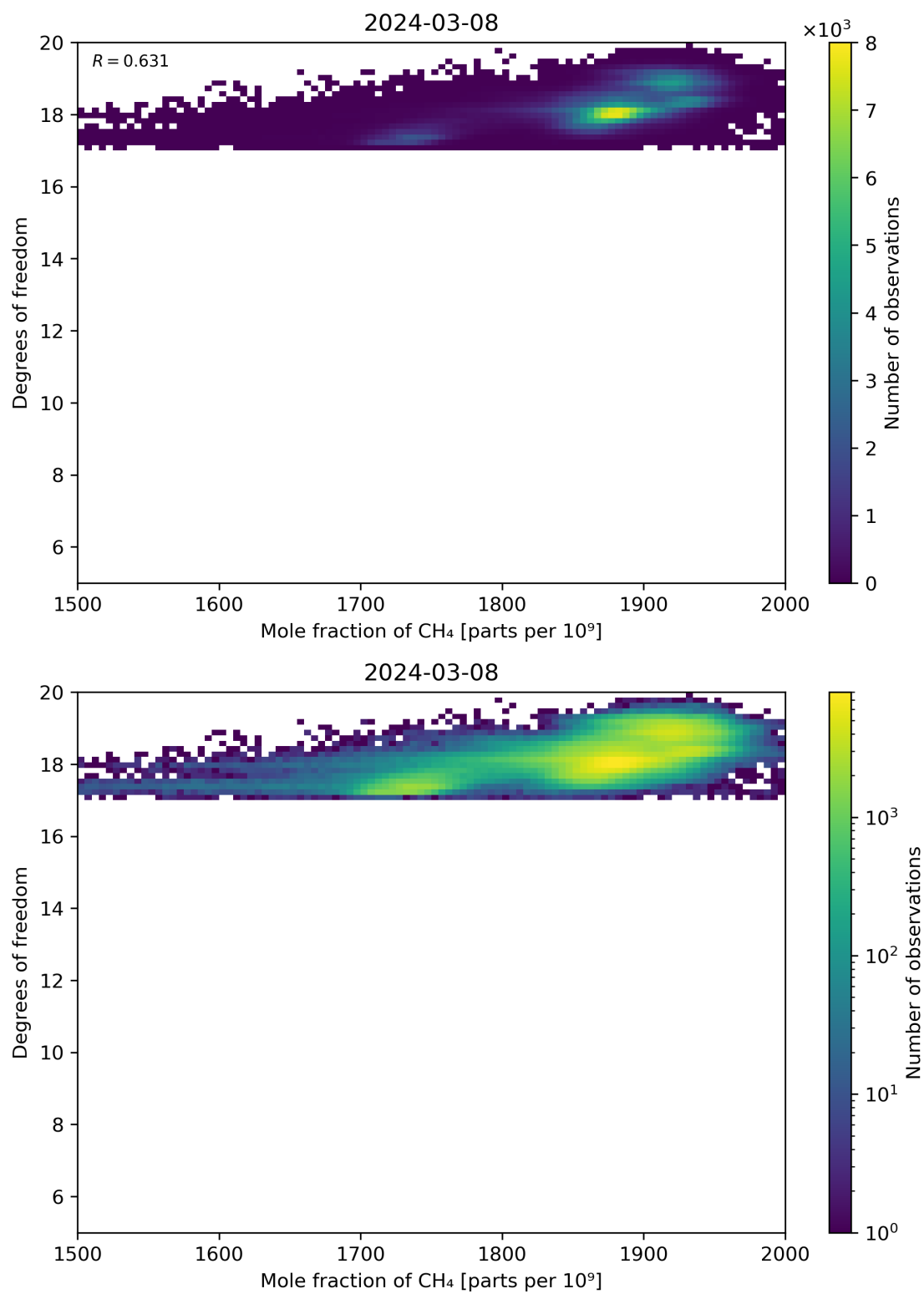
Figure 72: Scatter density plot of “Mole fraction of CH 4 ” against “Degrees of freedom” for 2024-03-07 to 2024-03-09.
