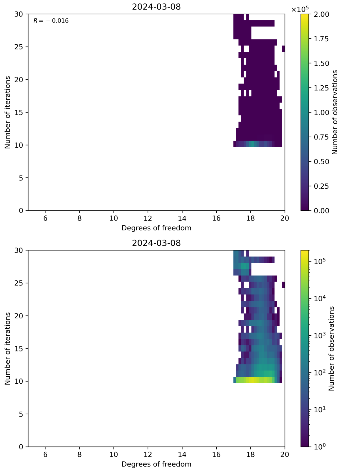
Figure 52: Scatter density plot of “Degrees of freedom” against “Number of iterations” for 2024-03-07 to 2024-03-09.
