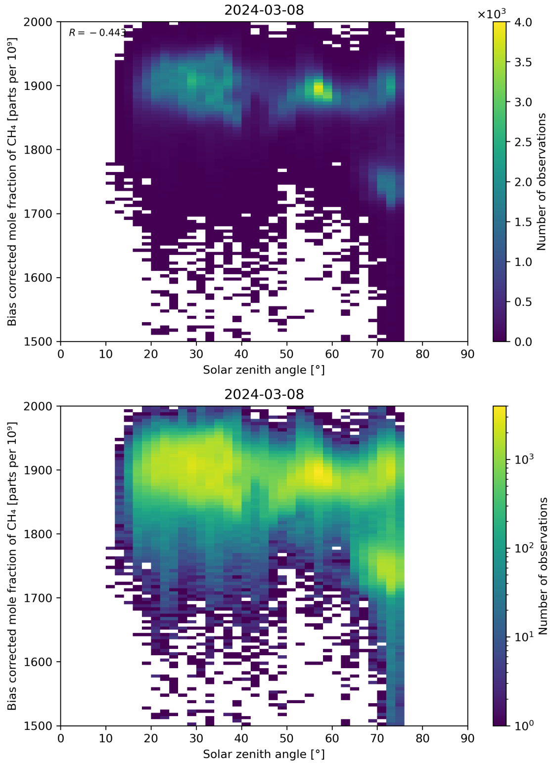
Figure 100: Scatter density plot of “Solar zenith angle” against “Bias corrected mole fraction of \text{CH}_4 ” for 2024-03-07 to 2024-03-09.
