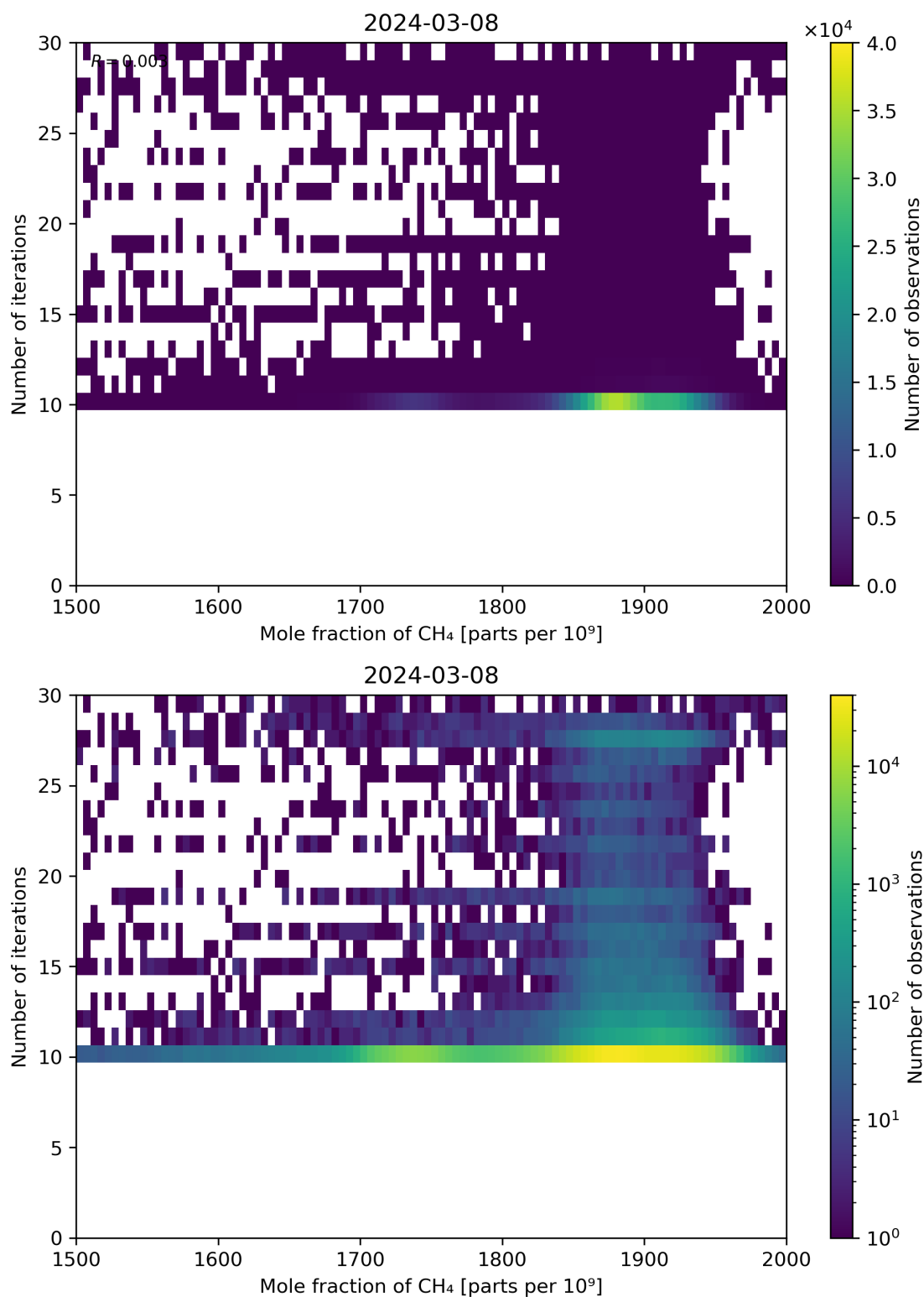
Figure 76: Scatter density plot of “Mole fraction of CH 4 ” against “Number of iterations” for 2024-03-07 to 2024-03-09.
