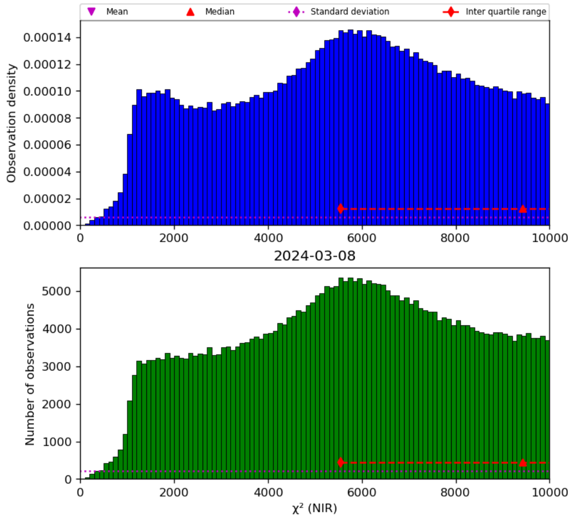
Figure 29: Histogram of “ \chi^2 (NIR)” for 2024-03-07 to 2024-03-09
