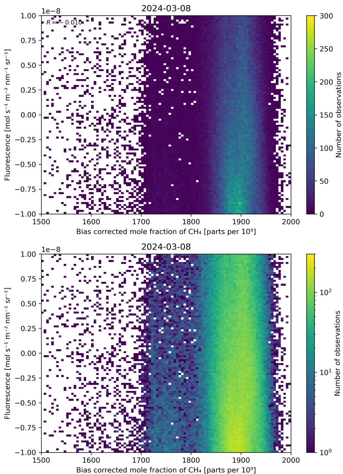
Figure 66: Scatter density plot of “Bias corrected mole fraction of \text{CH}_4 ” against “Fluorescence” for 2024-03-07 to 2024-03-09.
