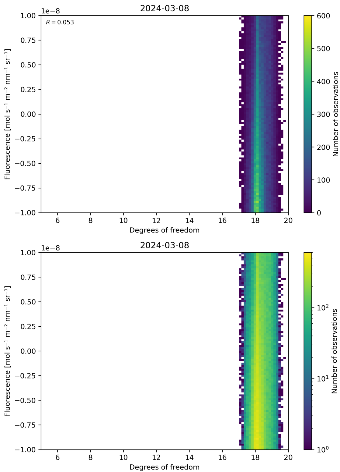
Figure 51: Scatter density plot of “Degrees of freedom” against “Fluorescence” for 2024-03-07 to 2024-03-09.
