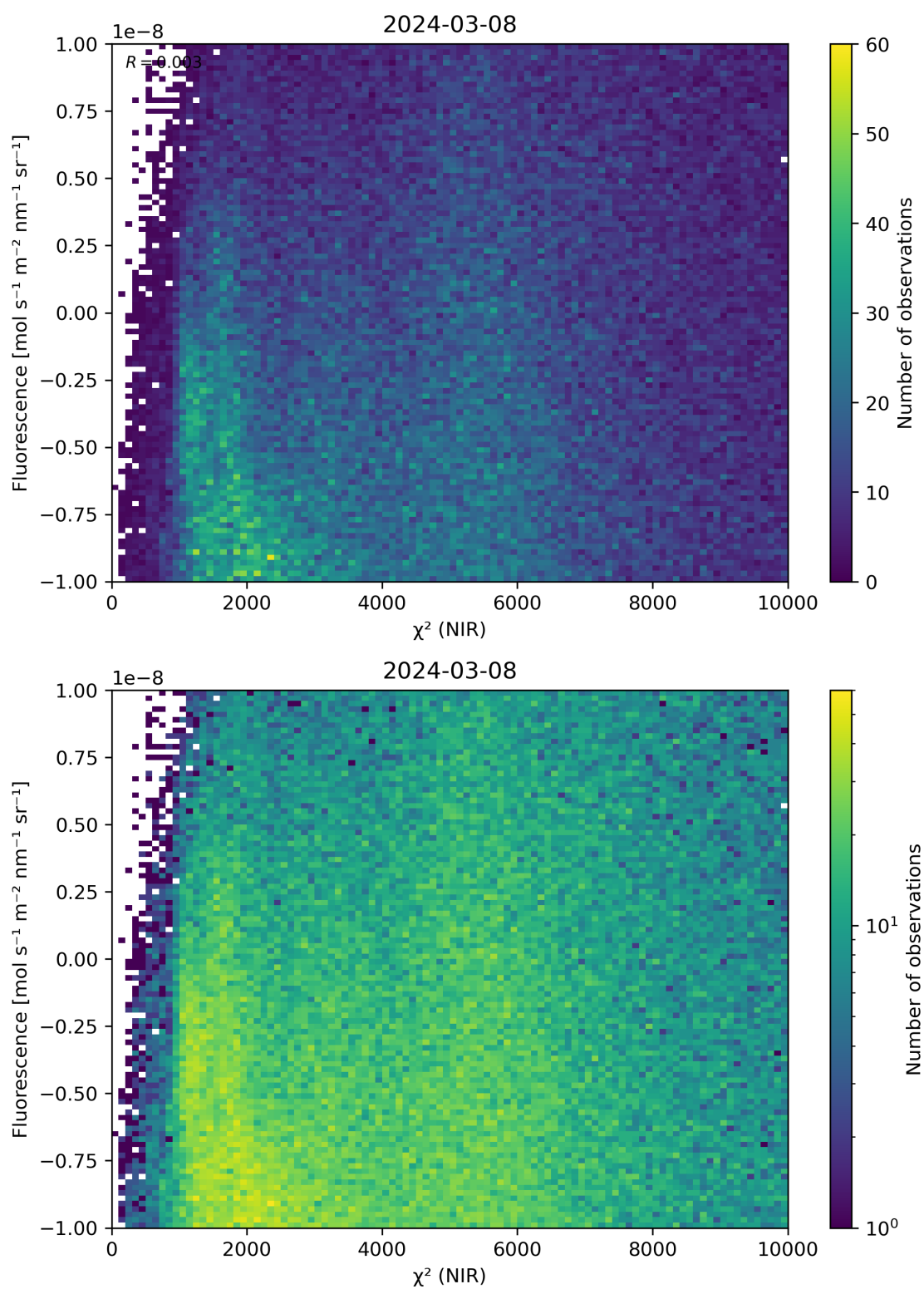
Figure 45: Scatter density plot of “ \chi^2 (NIR)” against “Fluorescence” for 2024-03-07 to 2024-03-09.
