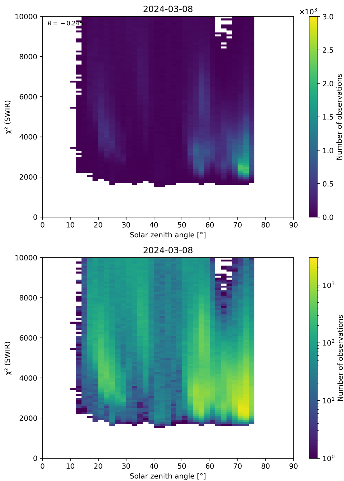
Figure 95: Scatter density plot of “Solar zenith angle” against “ \chi^2 (SWIR)” for 2024-03-07 to 2024-03-09.
