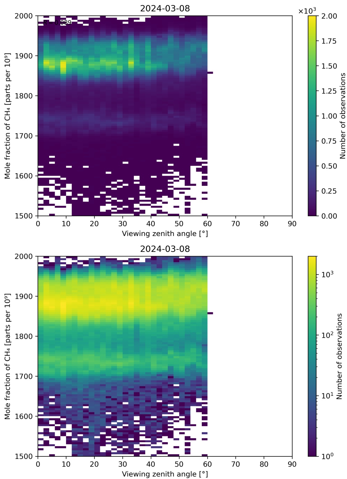
Figure 110: Scatter density plot of “Viewing zenith angle” against “Mole fraction of CH 4 ” for 2024-03-07 to 2024-03-09.
