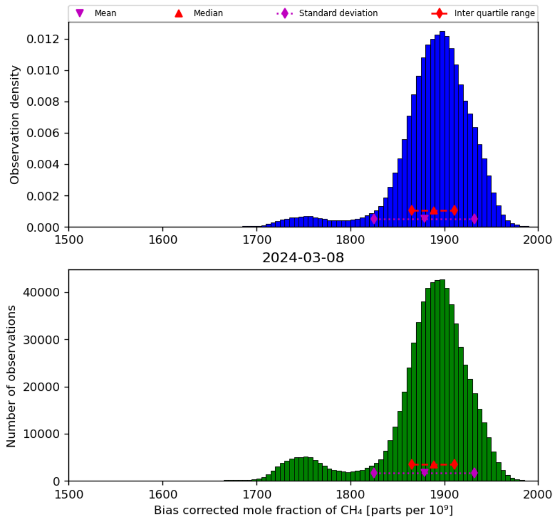
Figure 25: Histogram of “Bias corrected mole fraction of CH 4 ” for 2024-03-07 to 2024-03-09
