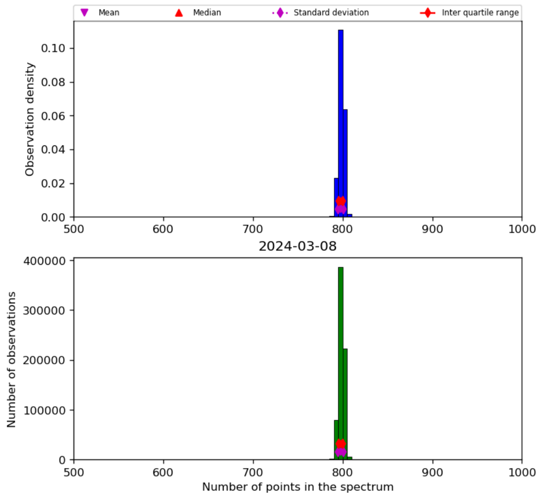
Figure 26: Histogram of “Number of points in the spectrum” for 2024-03-07 to 2024-03-09
