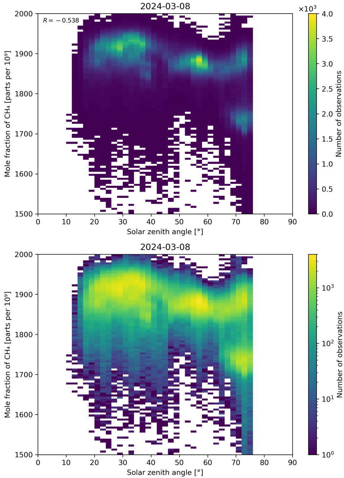
Figure 99: Scatter density plot of “Solar zenith angle” against “Mole fraction of \text{CH}_4 ” for 2024-03-07 to 2024-03-09.
