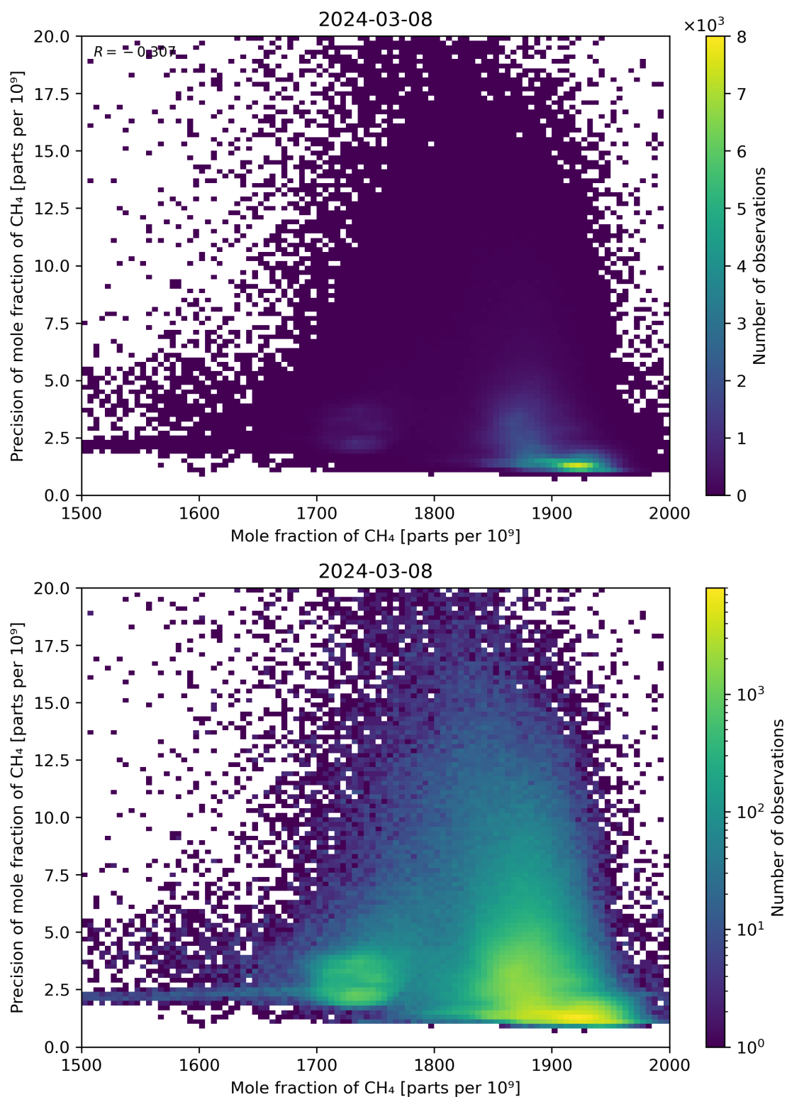
Figure 75: Scatter density plot of “Mole fraction of CH 4 ” against “Precision of mole fraction of CH 4 ” for 2024-03-07 to 2024-03-09.
