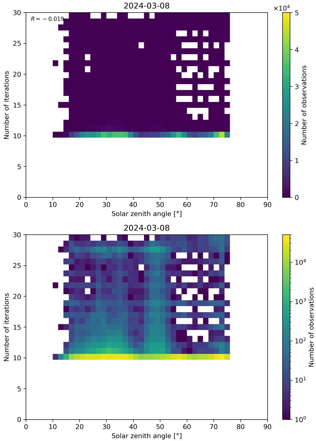
Figure 102: Scatter density plot of “Solar zenith angle” against “Number of iterations” for 2024-03-07 to 2024-03-09.
