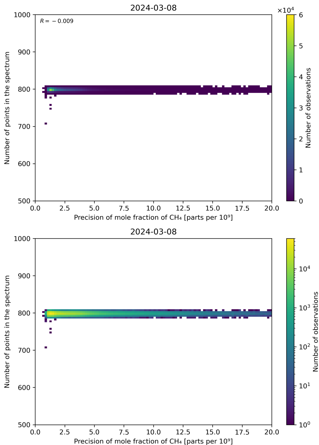
Figure 84: Scatter density plot of “Precision of mole fraction of CH 4 ” against “Number of points in the spectrum” for 2024-03-07 to 2024-03-09.
