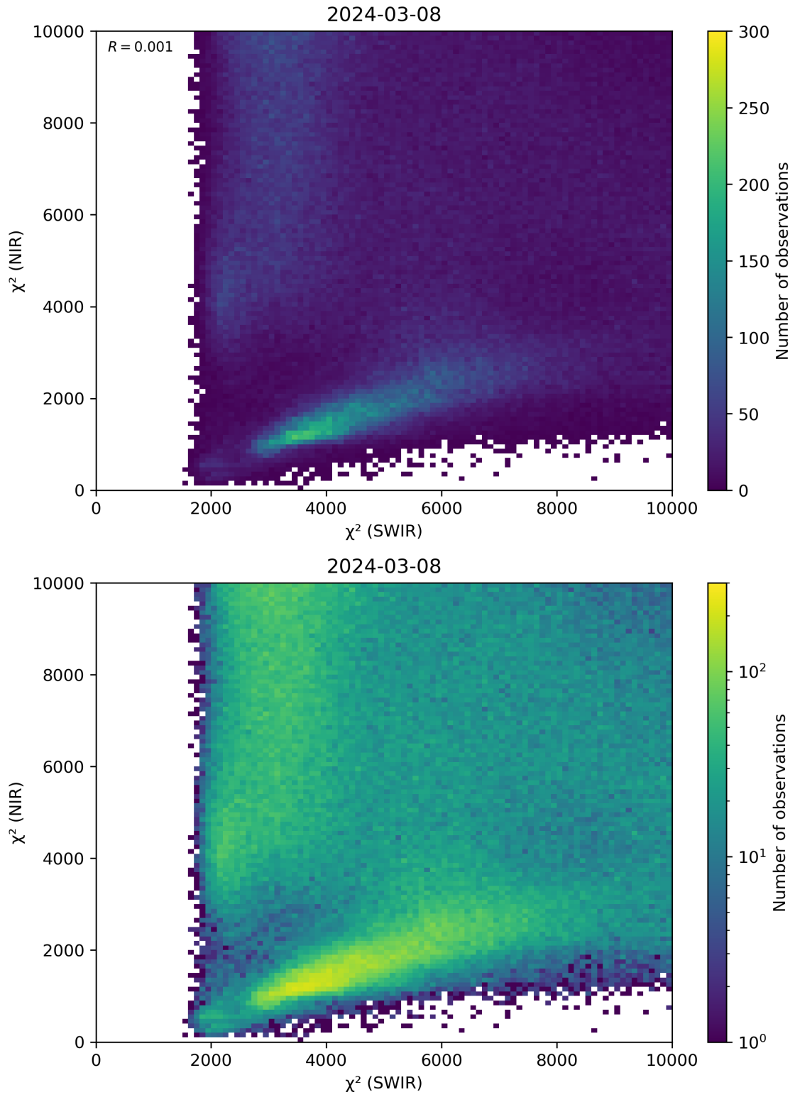
Figure 47: Scatter density plot of “ \chi^2 (SWIR)” against “ \chi^2 (NIR)” for 2024-03-07 to 2024-03-09.
