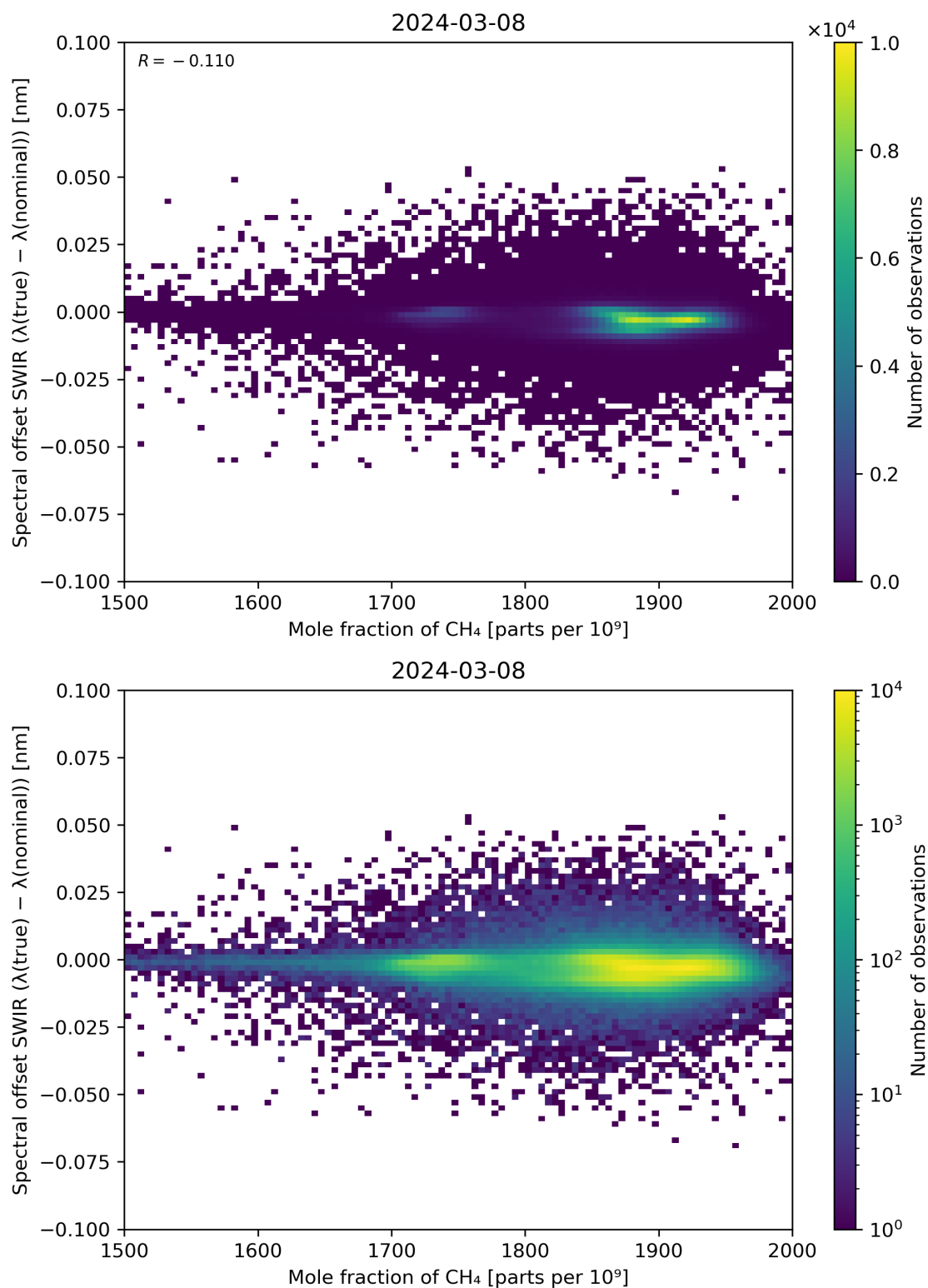
Figure 86: Scatter density plot of “Mole fraction of CH 4 ” against “Spectral offset SWIR ( \lambda(\text{true}) - \lambda(\text{nominal}) )” for 2024-03-07 to 2024-03-09.
