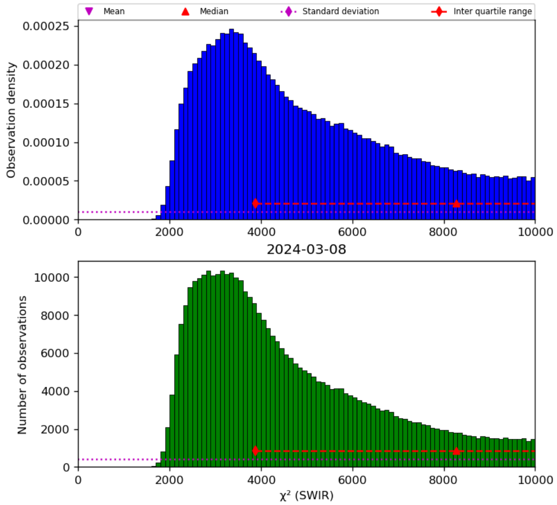
Figure 28: Histogram of “ \chi^2 (SWIR)” for 2024-03-07 to 2024-03-09
