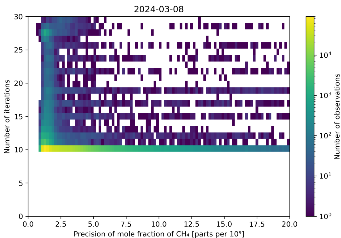
Figure 83: Scatter density plot of “Precision of mole fraction of CH 4 ” against “Number of iterations” for 2024-03-07 to 2024-03-09.
