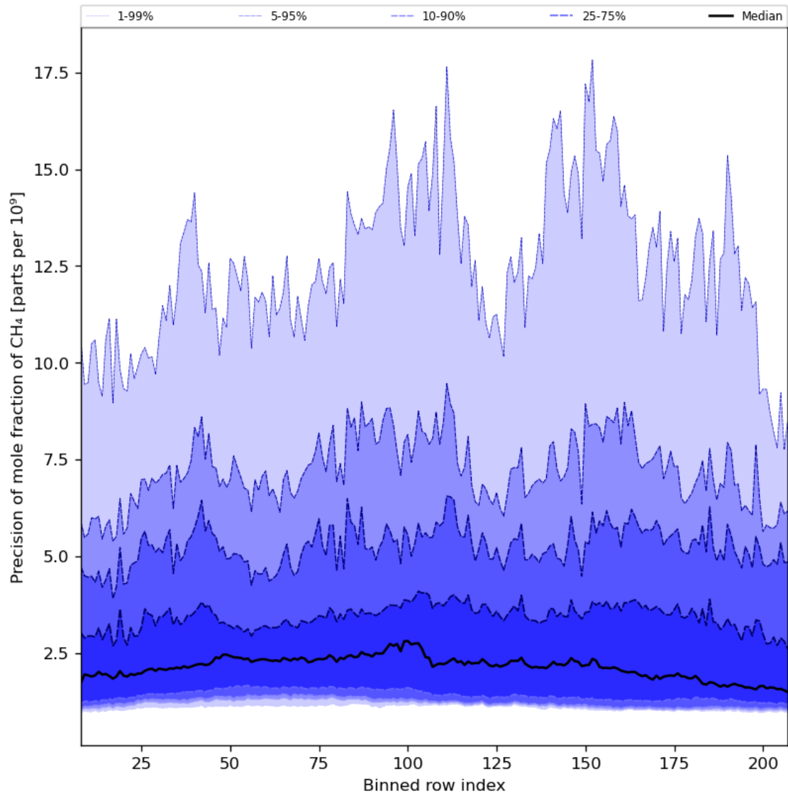
Figure 35: Along track statistics of “Precision of mole fraction of CH 4 ” for 2024-03-07 to 2024-03-09
