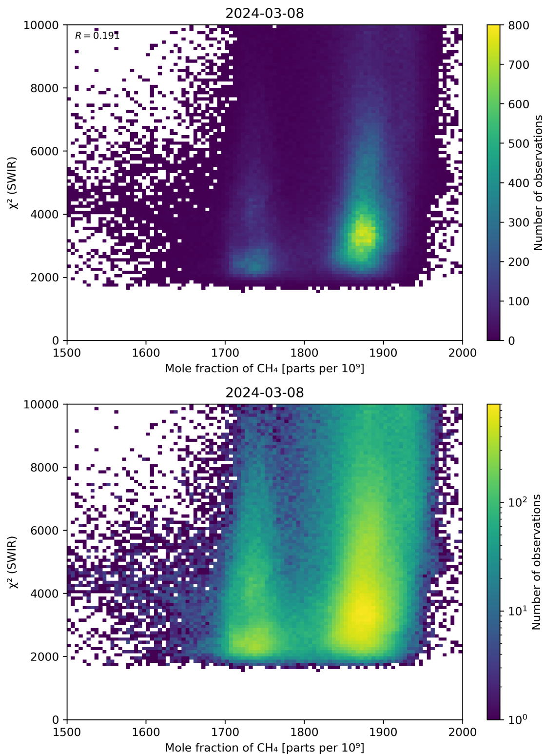
Figure 71: Scatter density plot of “Mole fraction of \text{CH}_4 ” against “ \chi^2 (SWIR)” for 2024-03-07 to 2024-03-09.
