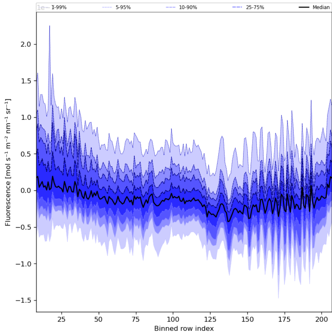
Figure 43: Along track statistics of “Fluorescence” for 2024-03-07 to 2024-03-09
