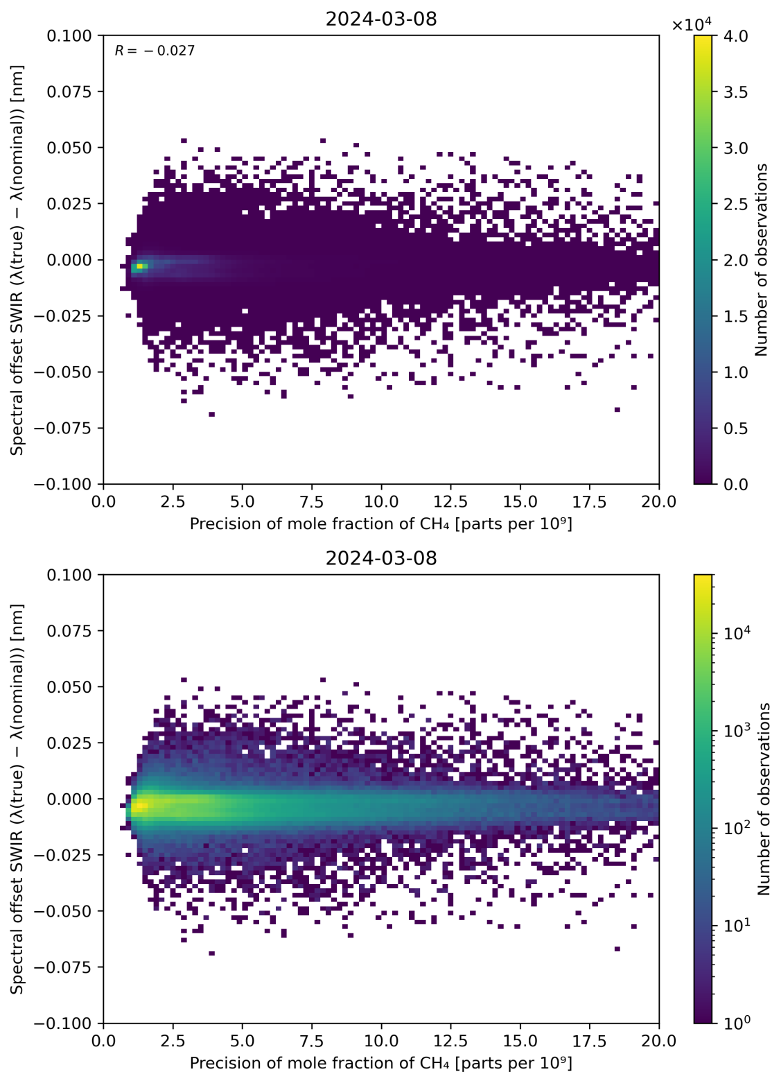
Figure 85: Scatter density plot of “Precision of mole fraction of \text{CH}_4 ” against “Spectral offset SWIR ( \lambda(\text{true}) - \lambda(\text{nominal}) )” for 2024-03-07 to 2024-03-09.
