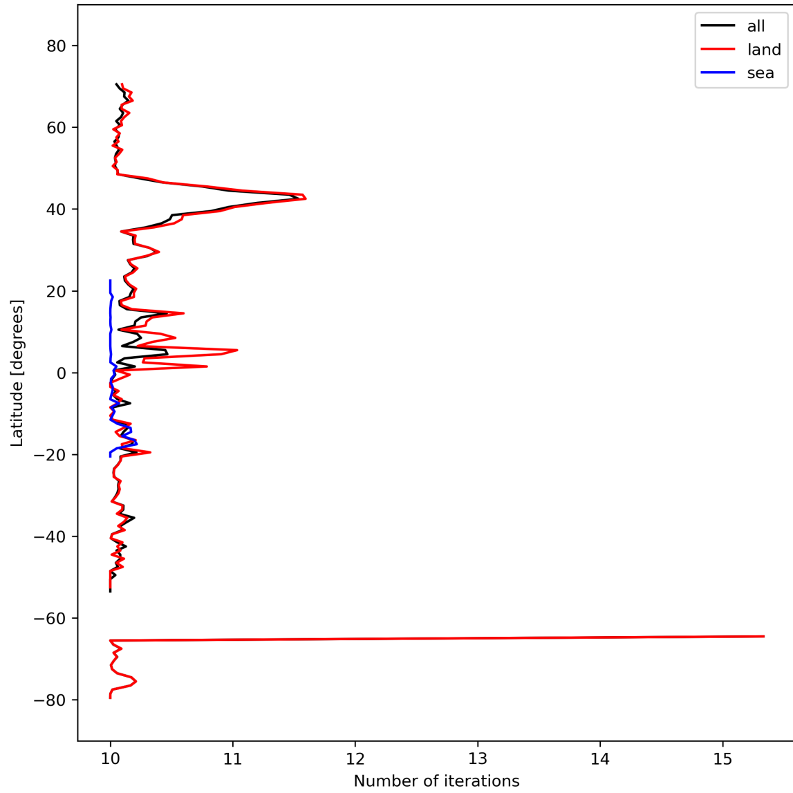
Figure 20: Zonal average of “Number of iterations” for 2024-03-07 to 2024-03-09.
