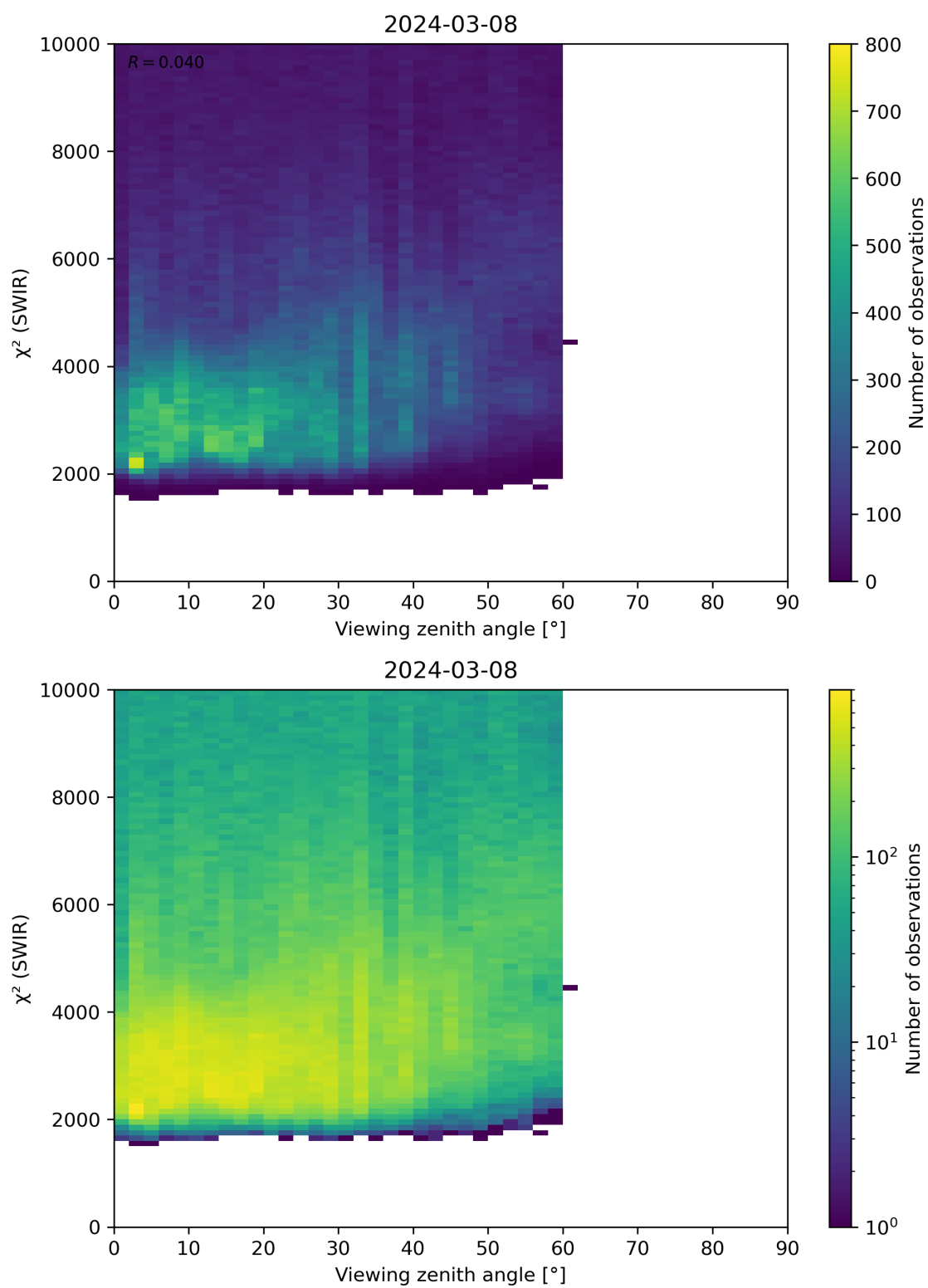
Figure 106: Scatter density plot of “Viewing zenith angle” against “ \chi^2 (SWIR)” for 2024-03-07 to 2024-03-09.
