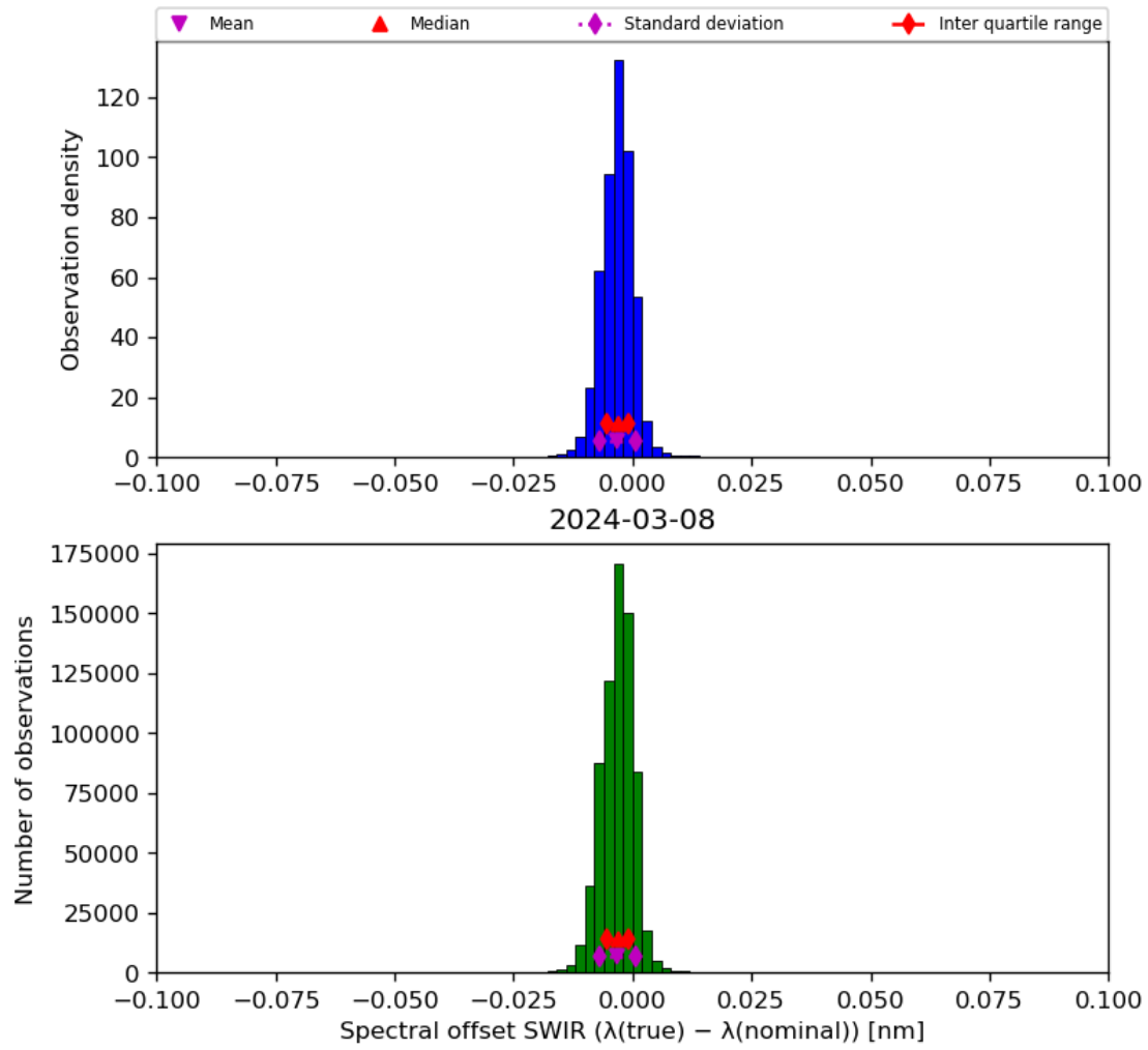
Figure 27: Histogram of “Spectral offset SWIR ( \lambda(\text{true}) - \lambda(\text{nominal}) )” for 2024-03-07 to 2024-03-09
