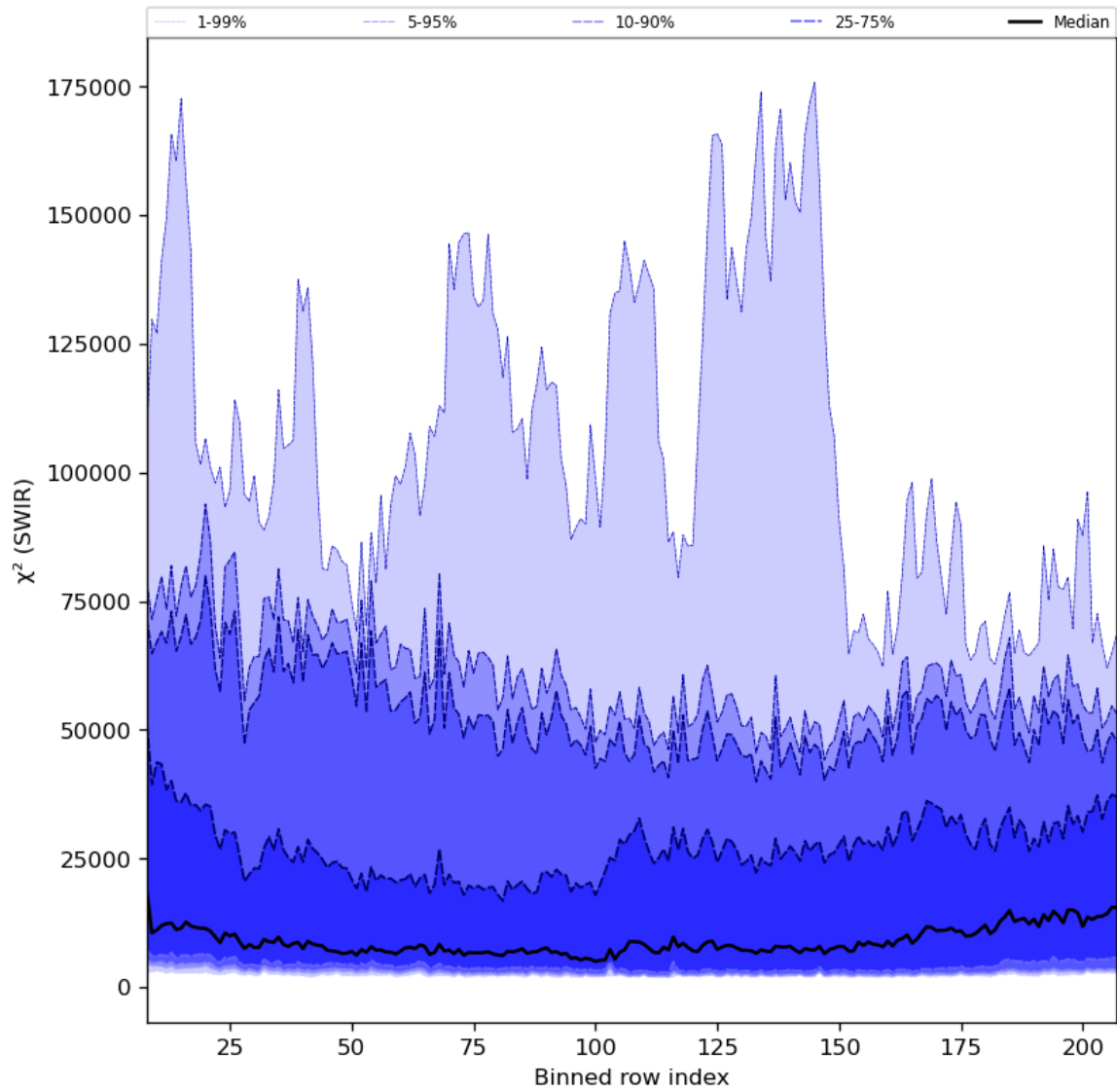
Figure 39: Along track statistics of " \chi^2 (SWIR)" for 2024-03-07 to 2024-03-09
