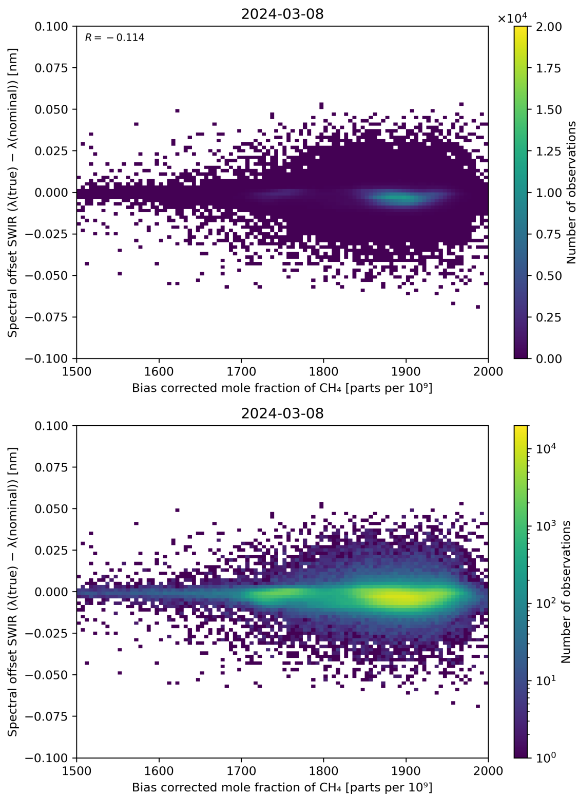
Figure 69: Scatter density plot of “Bias corrected mole fraction of \text{CH}_4 ” against “Spectral offset SWIR ( \lambda(\text{true}) - \lambda(\text{nominal}) )” for 2024-03-07 to 2024-03-09.
