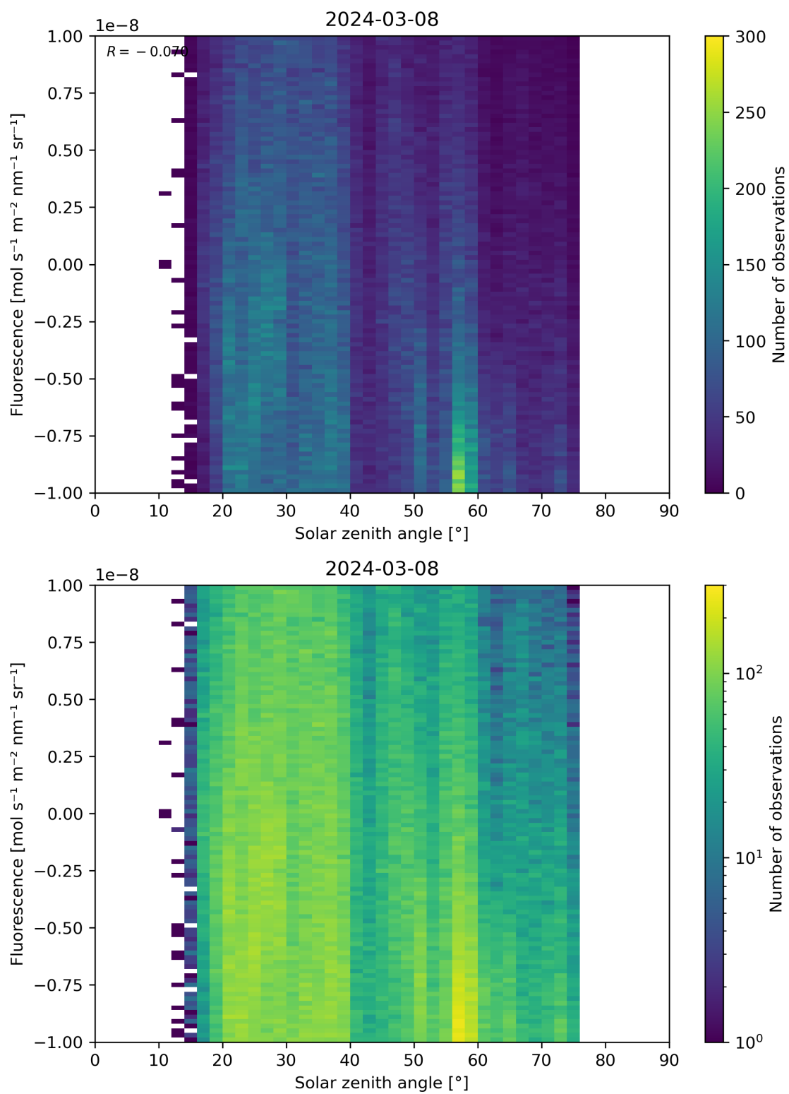
Figure 97: Scatter density plot of “Solar zenith angle” against “Fluorescence” for 2024-03-07 to 2024-03-09.
