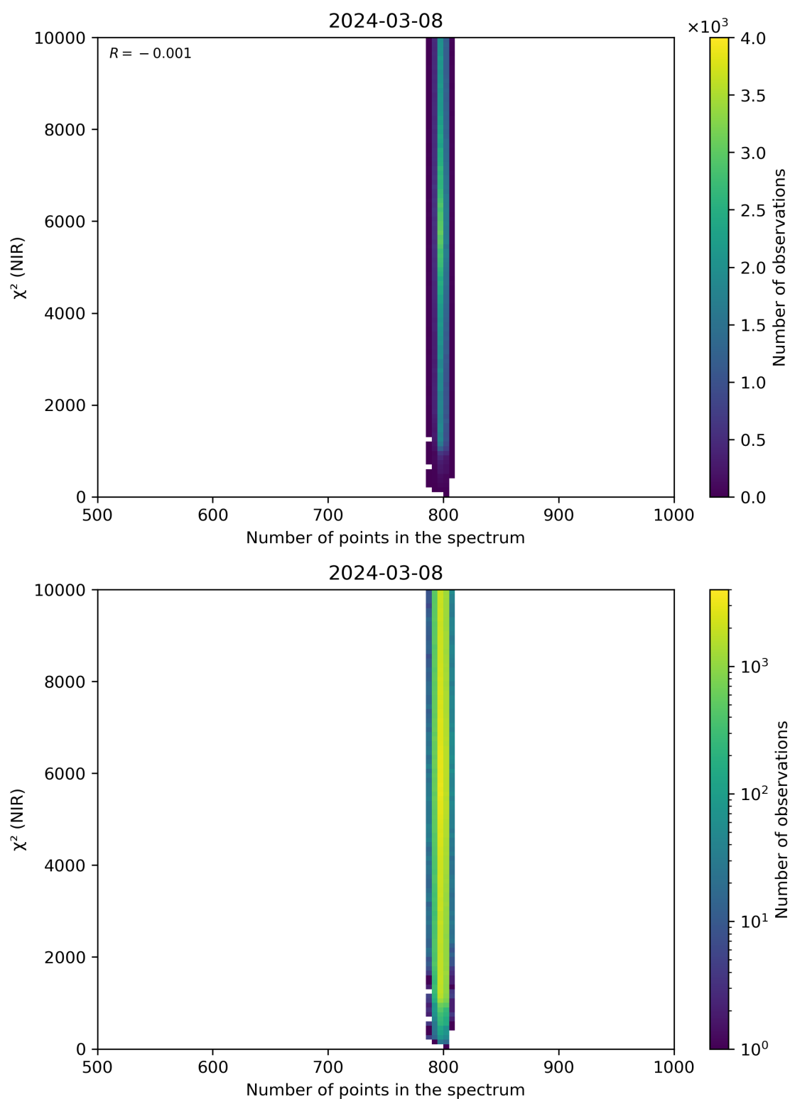
Figure 88: Scatter density plot of “Number of points in the spectrum” against “ \chi^2 (NIR)” for 2024-03-07 to 2024-03-09.
