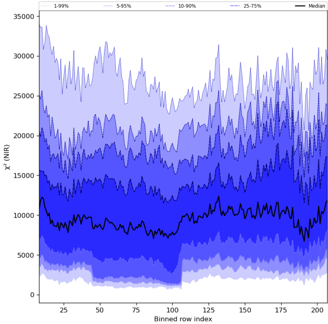
Figure 40: Along track statistics of “ \chi^2 (NIR)” for 2024-03-07 to 2024-03-09
