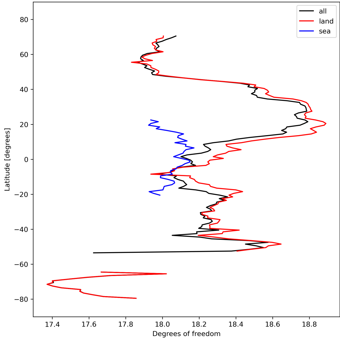
Figure 19: Zonal average of “Degrees of freedom” for 2024-03-07 to 2024-03-09.
