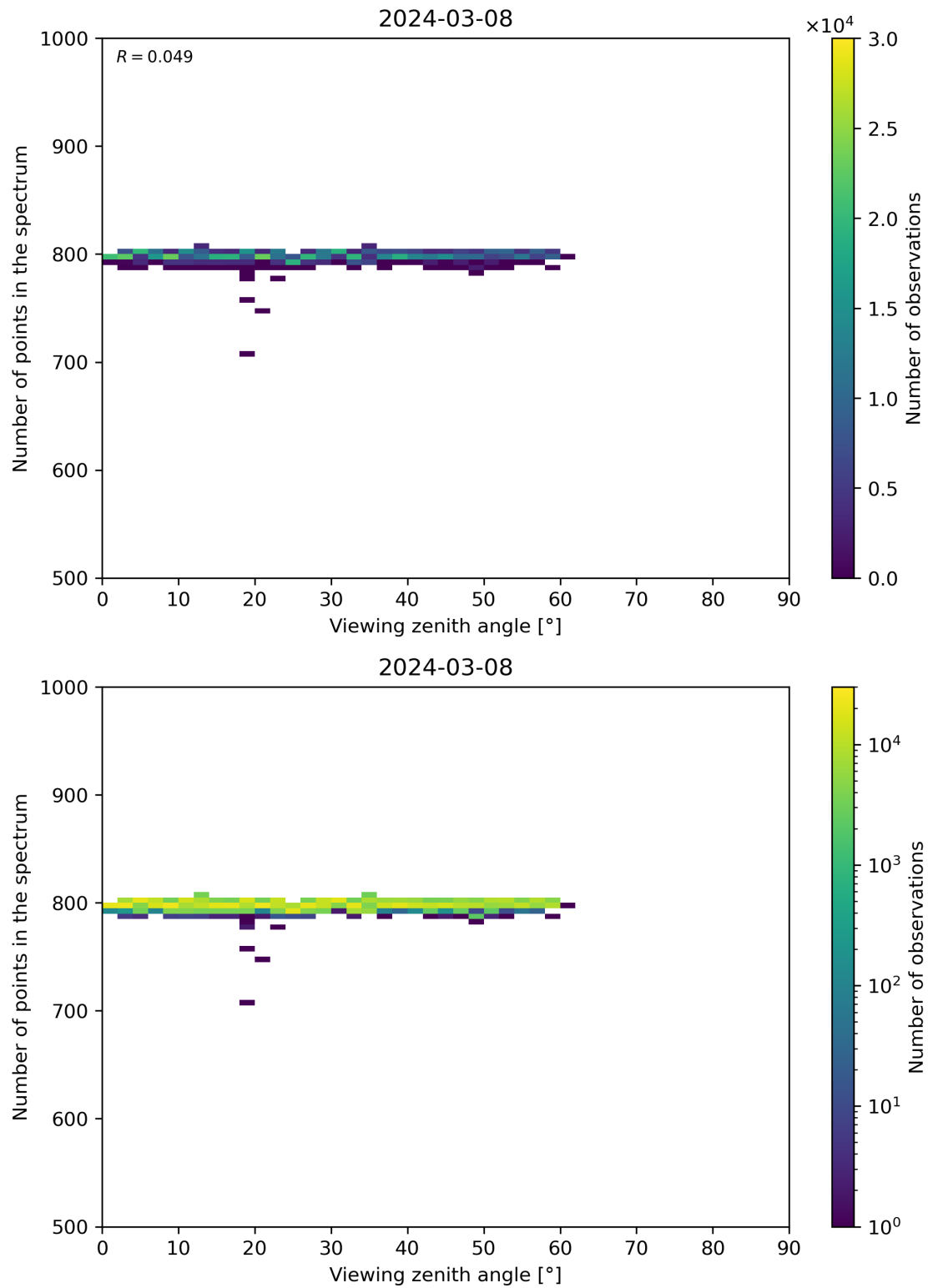
Figure 114: Scatter density plot of “Viewing zenith angle” against “Number of points in the spectrum” for 2024-03-07 to 2024-03-09.
