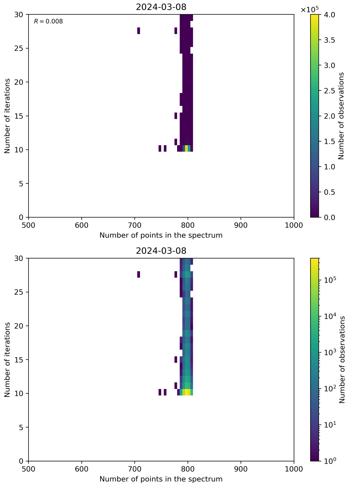
Figure 92: Scatter density plot of “Number of points in the spectrum” against “Number of iterations” for 2024-03-07 to 2024-03-09.
