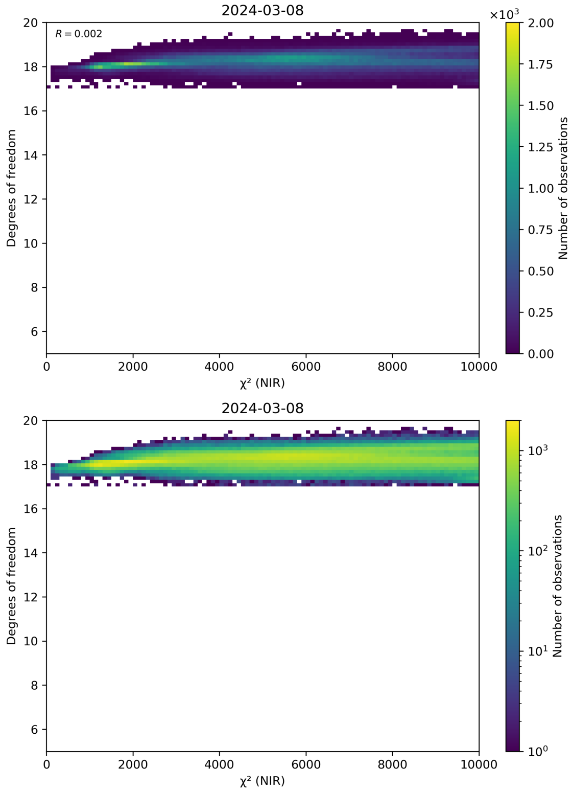
Figure 44: Scatter density plot of “ \chi^2 (NIR)” against “Degrees of freedom” for 2024-03-07 to 2024-03-09.
