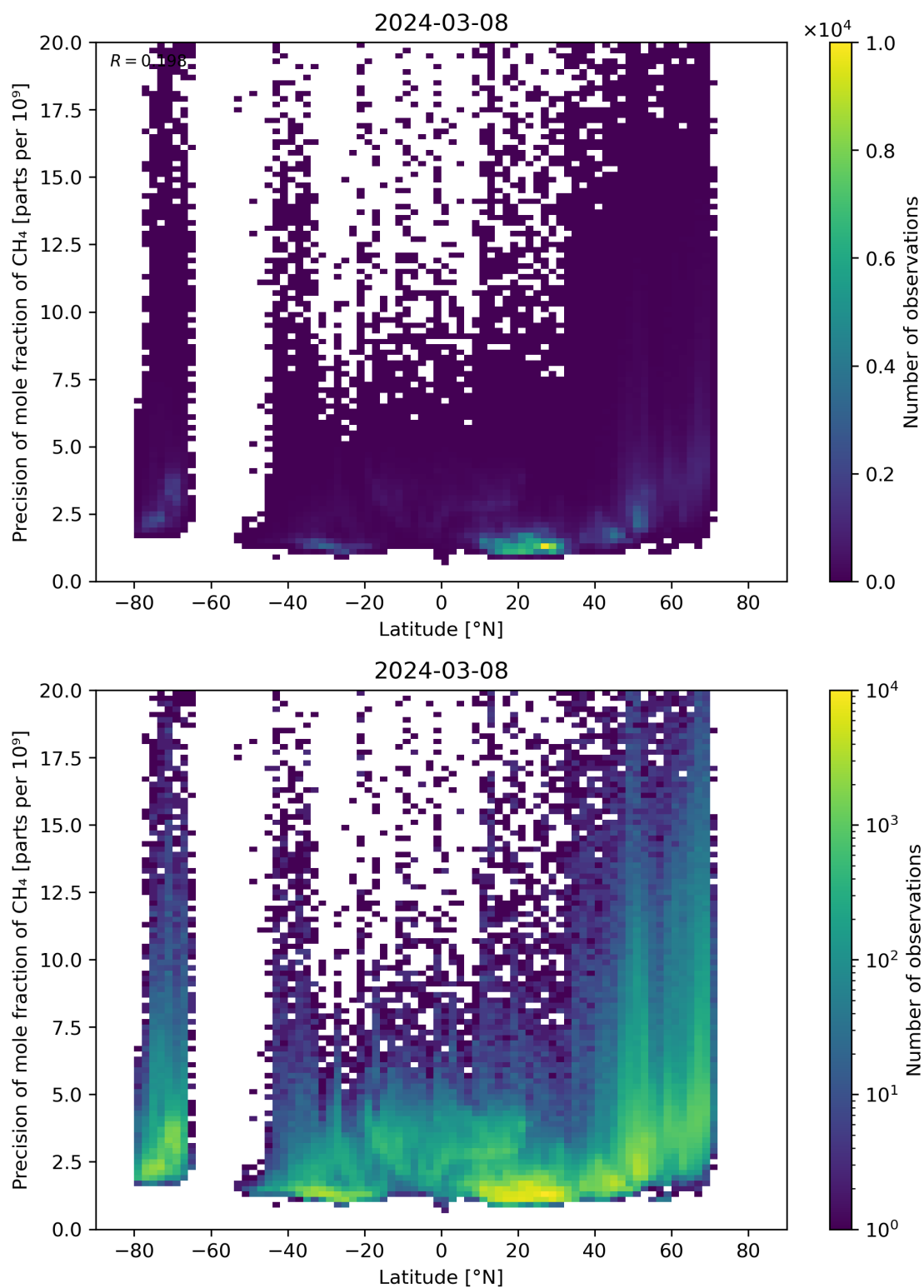
Figure 59: Scatter density plot of “Latitude” against “Precision of mole fraction of \text{CH}_4 ” for 2024-03-07 to 2024-03-09.
