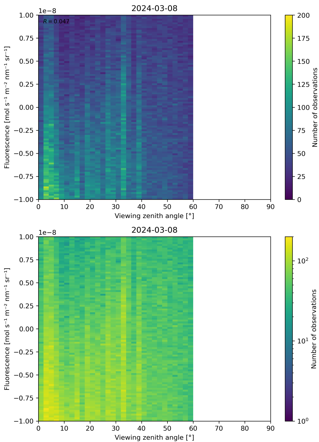
Figure 108: Scatter density plot of “Viewing zenith angle” against “Fluorescence” for 2024-03-07 to 2024-03-09.
