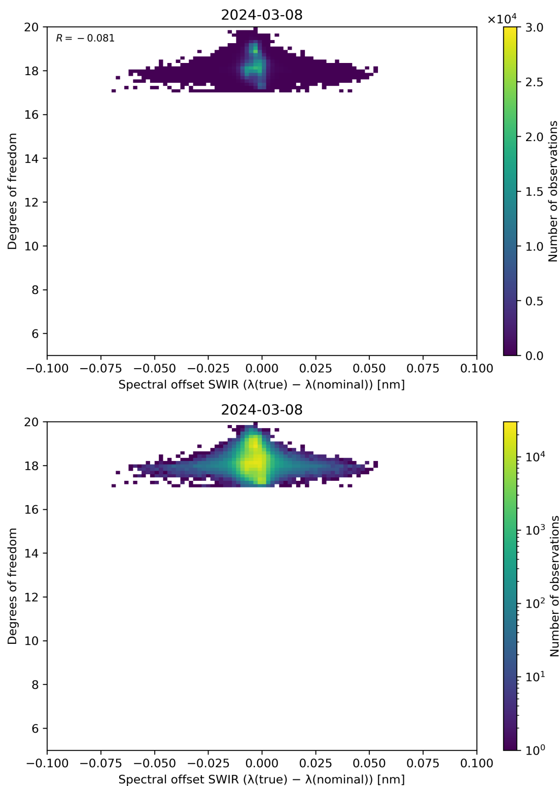
Figure 119: Scatter density plot of “Spectral offset SWIR ( \lambda(\text{true}) - \lambda(\text{nominal}) )” against “Degrees of freedom” for 2024-03-07 to 2024-03-09.
