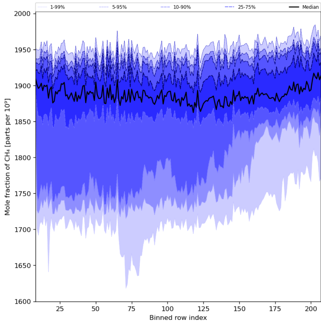
Figure 34: Along track statistics of “Mole fraction of CH 4 ” for 2024-03-07 to 2024-03-09
