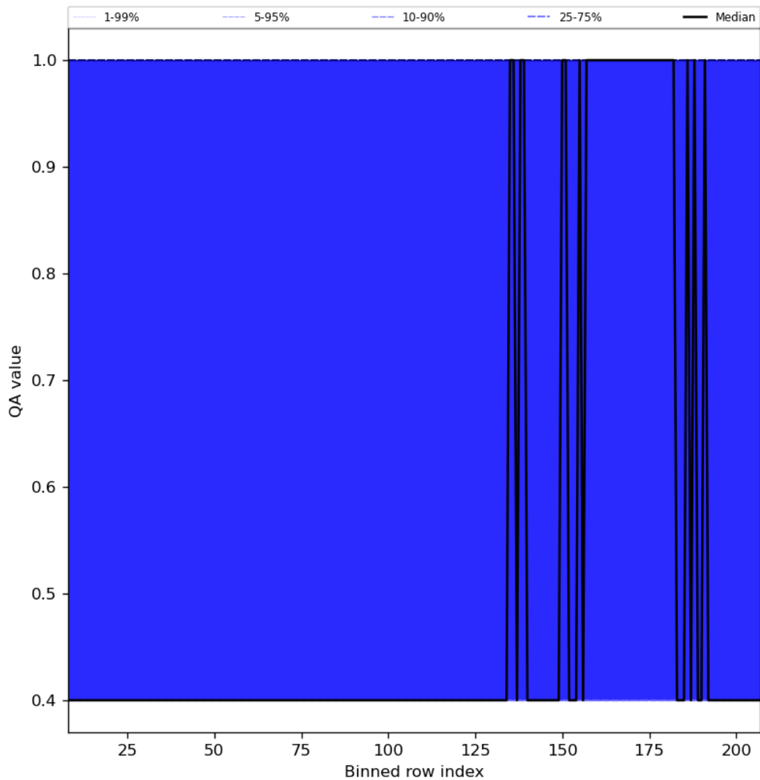
Figure 33: Along track statistics of “QA value” for 2024-03-07 to 2024-03-09
