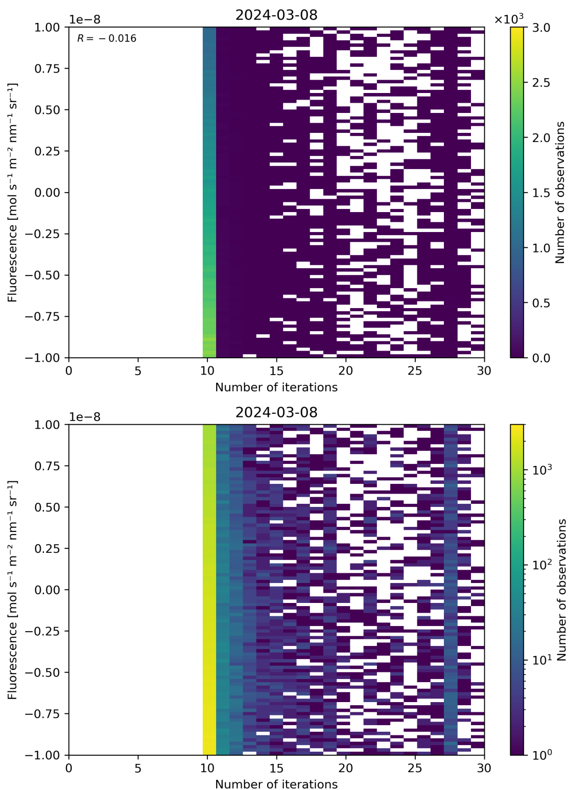
Figure 87: Scatter density plot of “Number of iterations” against “Fluorescence” for 2024-03-07 to 2024-03-09.
