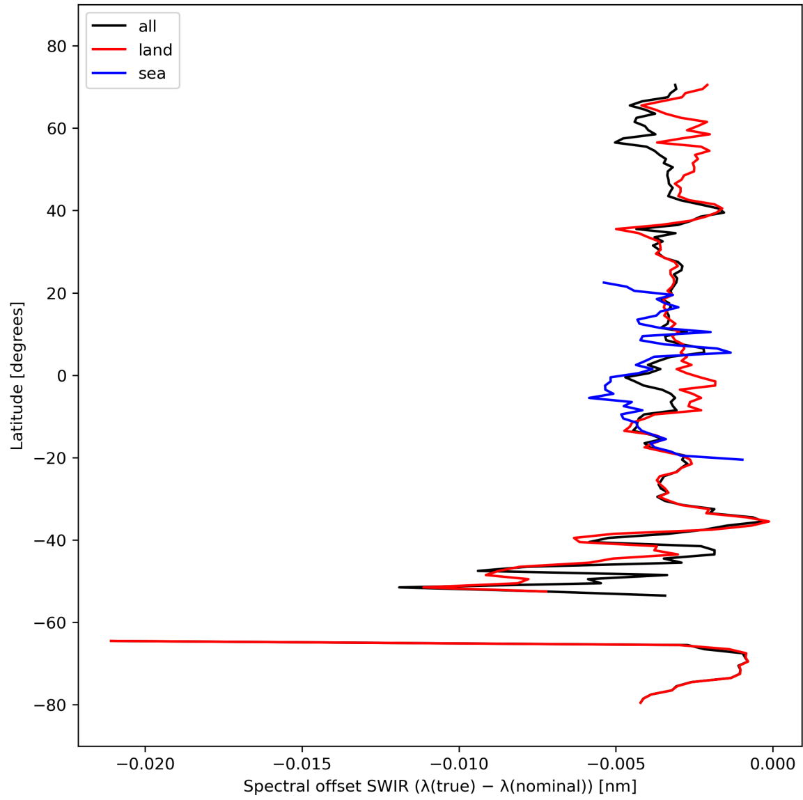
Figure 16: Zonal average of “Spectral offset SWIR ( \lambda(\text{true}) - \lambda(\text{nominal}) )” for 2024-03-07 to 2024-03-09.
