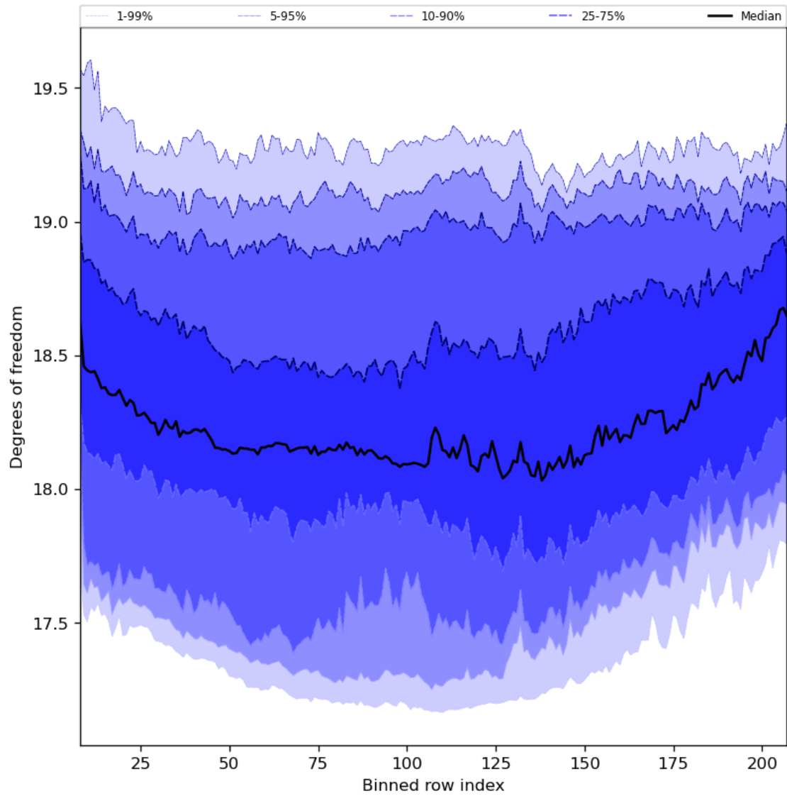
Figure 41: Along track statistics of “Degrees of freedom” for 2024-03-07 to 2024-03-09
