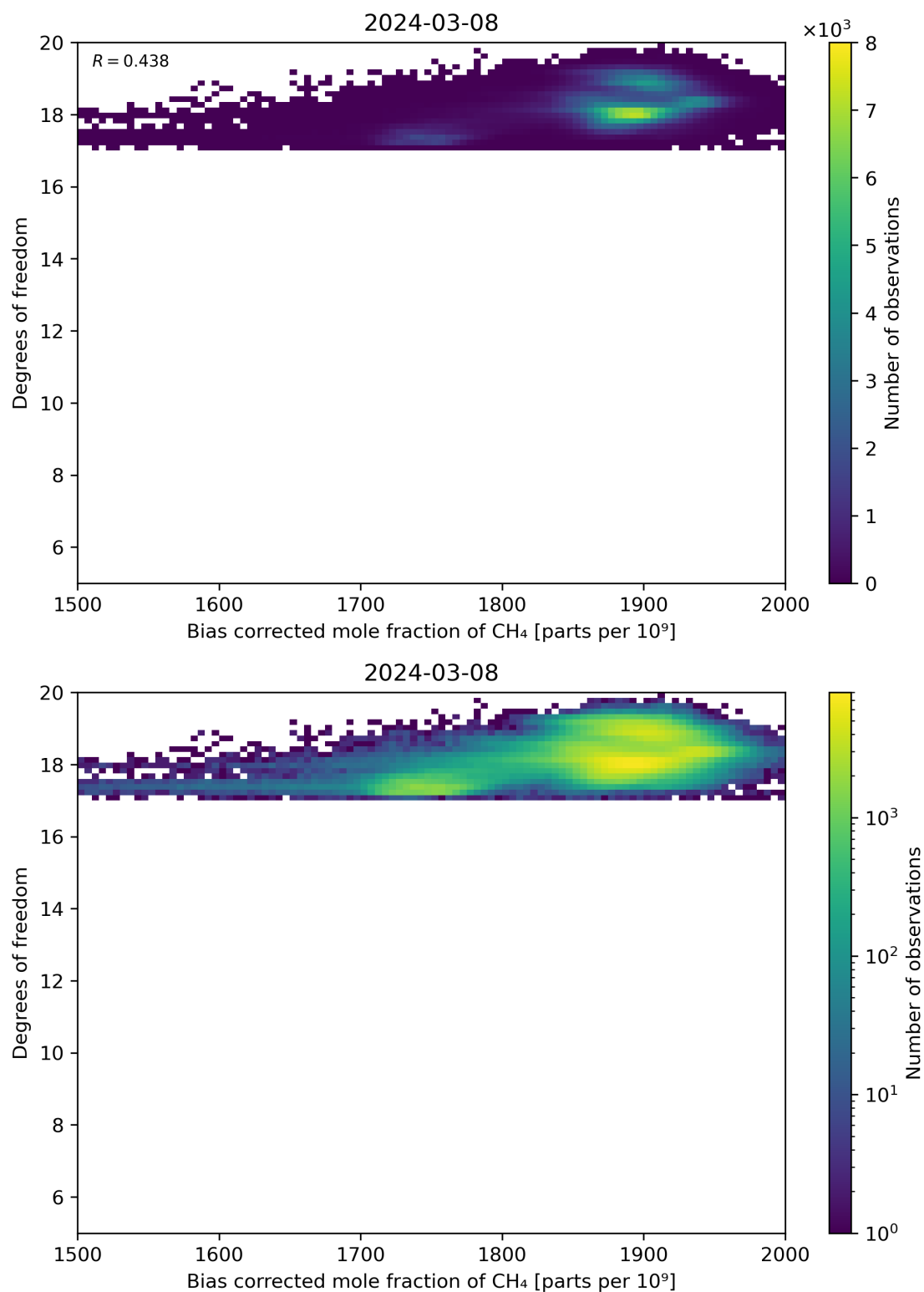
Figure 65: Scatter density plot of “Bias corrected mole fraction of CH 4 ” against “Degrees of freedom” for 2024-03-07 to 2024-03-09.
