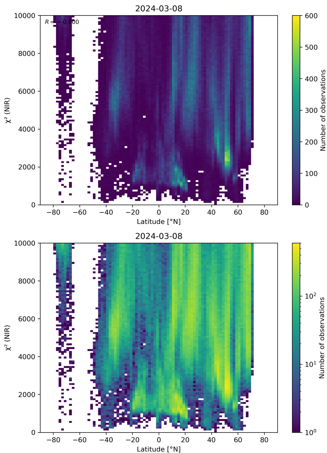
Figure 53: Scatter density plot of “Latitude” against “ \chi^2 (NIR)” for 2024-03-07 to 2024-03-09.
