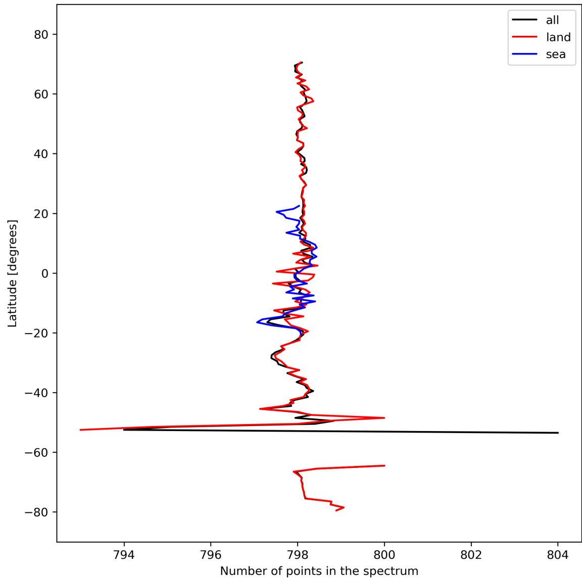
Figure 15: Zonal average of “Number of points in the spectrum” for 2024-03-07 to 2024-03-09.
