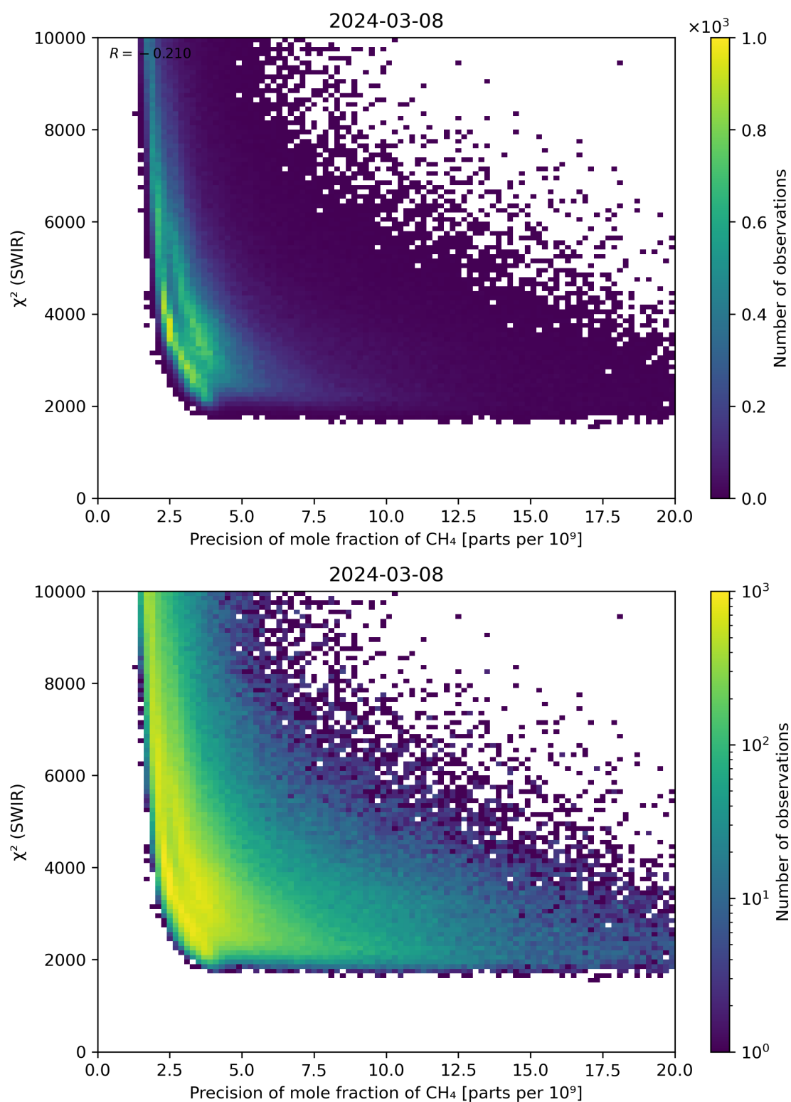
Figure 79: Scatter density plot of “Precision of mole fraction of \text{CH}_4 ” against “ \chi^2 (SWIR)” for 2024-03-07 to 2024-03-09.
