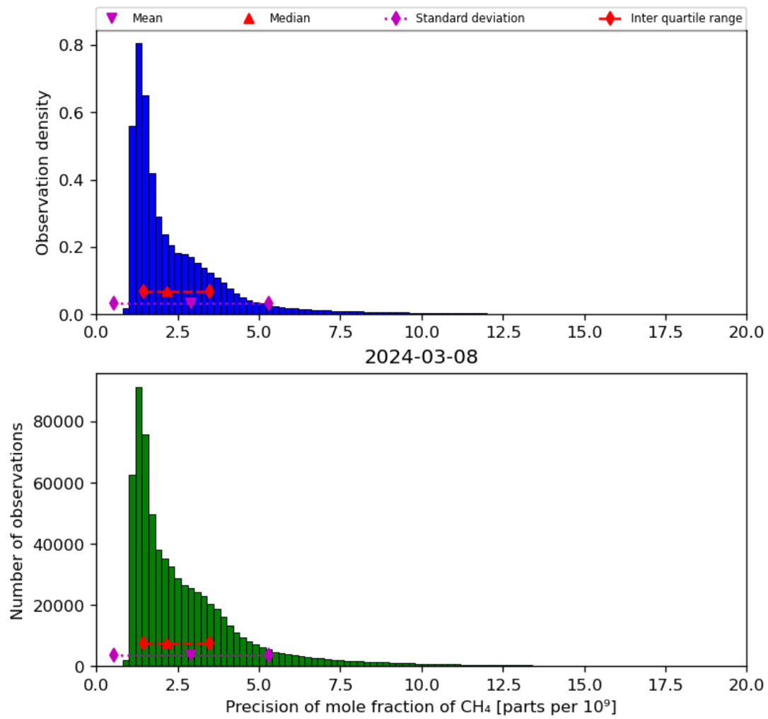
Figure 24: Histogram of “Precision of mole fraction of CH 4 ” for 2024-03-07 to 2024-03-09
