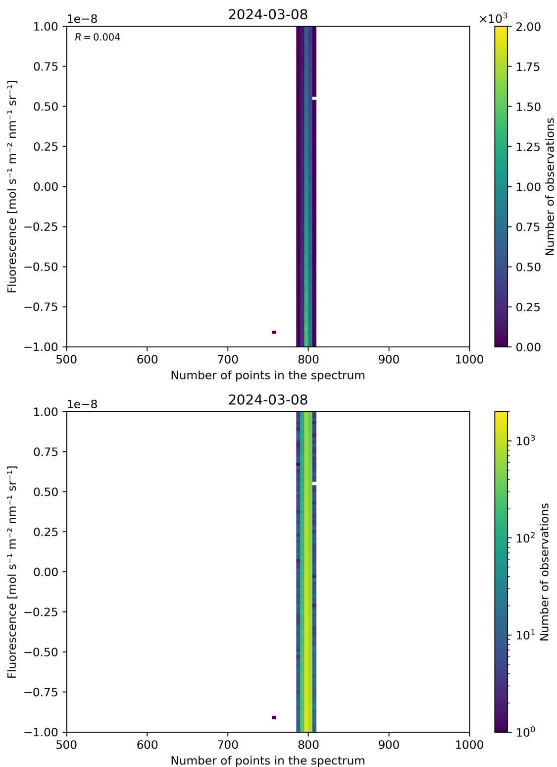
Figure 91: Scatter density plot of “Number of points in the spectrum” against “Fluorescence” for 2024-03-07 to 2024-03-09.
