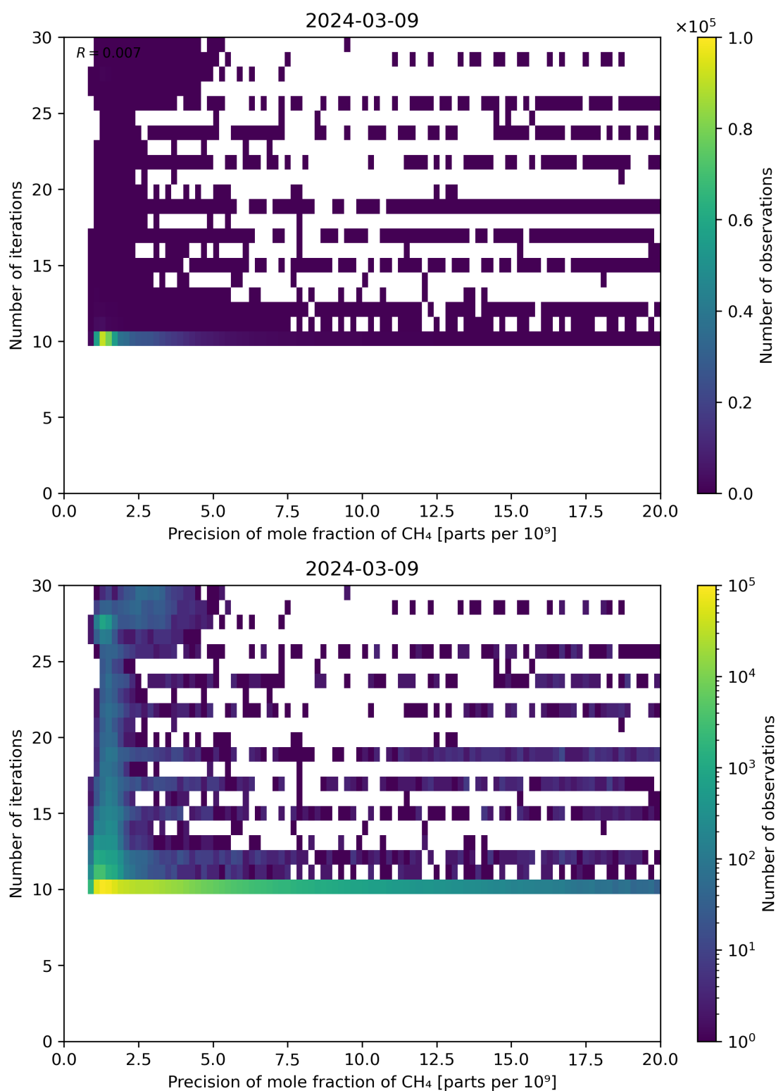
Figure 83: Scatter density plot of “Precision of mole fraction of \text{CH}_4 ” against “Number of iterations” for 2024-03-09 to 2024-03-10.
