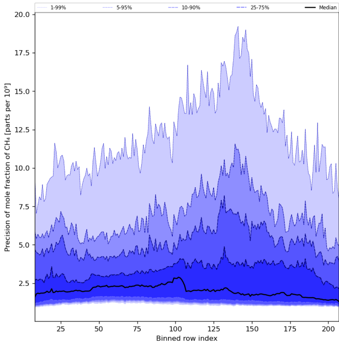
Figure 35: Along track statistics of “Precision of mole fraction of CH 4 ” for 2024-03-09 to 2024-03-10
