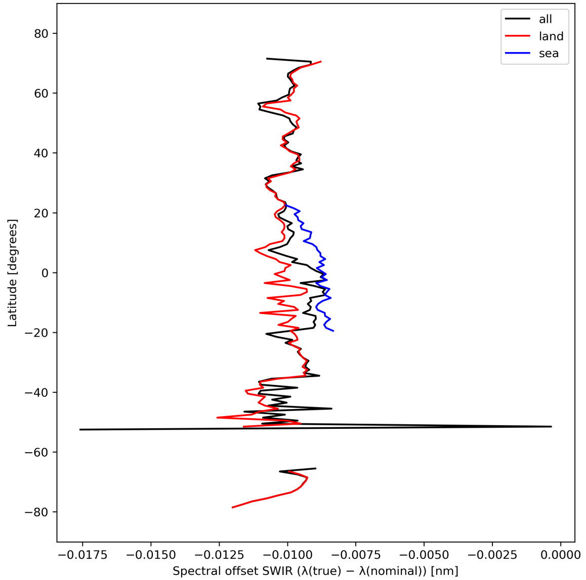
Figure 16: Zonal average of “Spectral offset SWIR ( \lambda(\text{true}) - \lambda(\text{nominal}) )” for 2024-03-09 to 2024-03-10.
