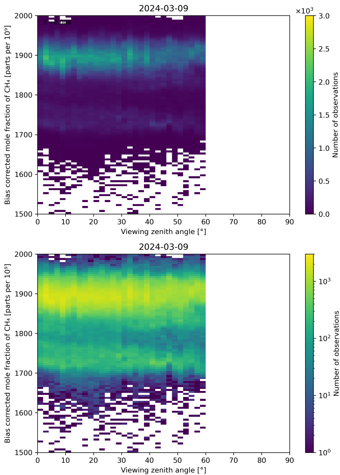
Figure 111: Scatter density plot of “Viewing zenith angle” against “Bias corrected mole fraction of CH 4 ” for 2024-03-09 to 2024-03-10.
