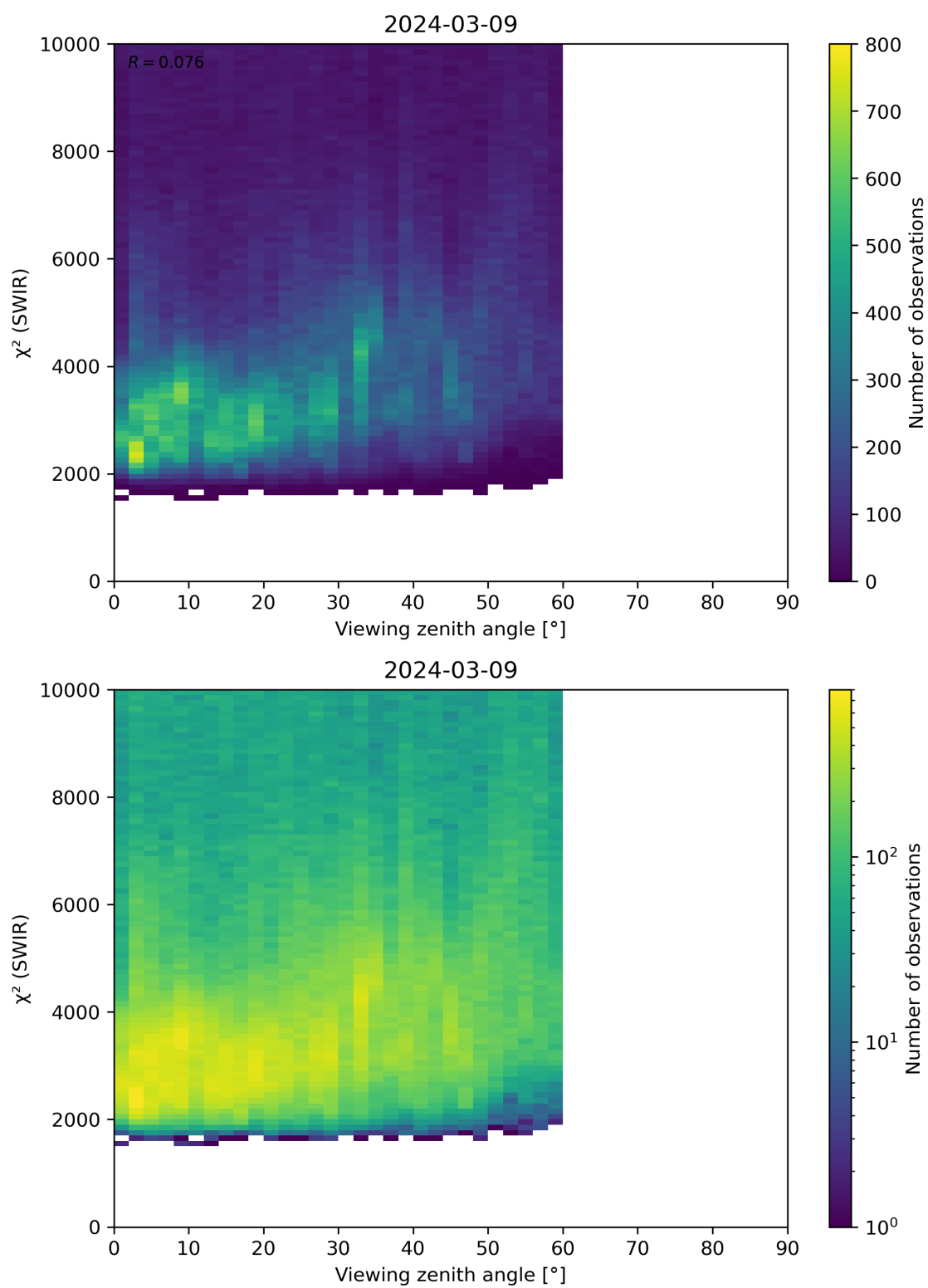
Figure 106: Scatter density plot of “Viewing zenith angle” against “ \chi^2 (SWIR)” for 2024-03-09 to 2024-03-10.
