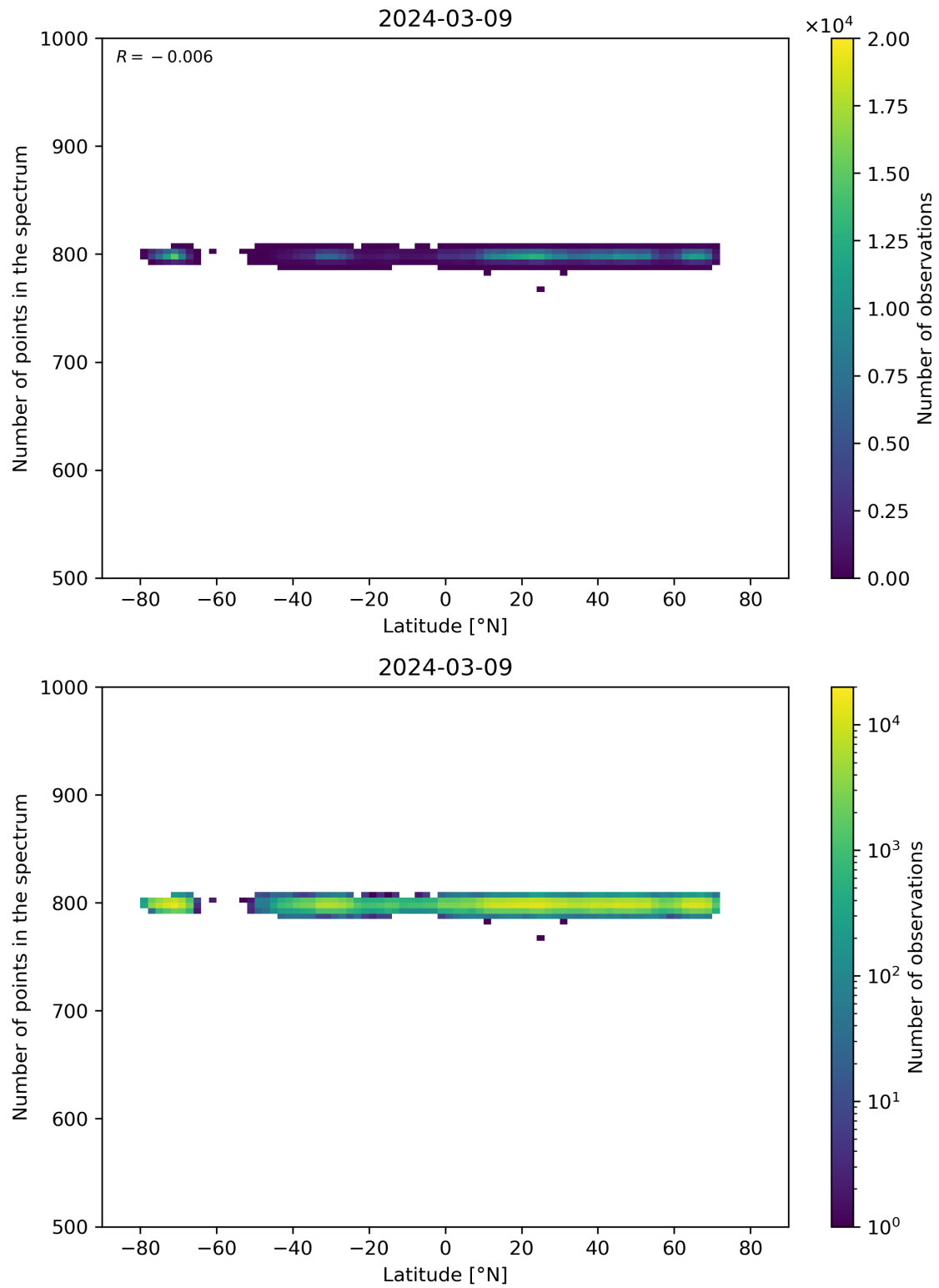
Figure 61: Scatter density plot of “Latitude” against “Number of points in the spectrum” for 2024-03-09 to 2024-03-10.
