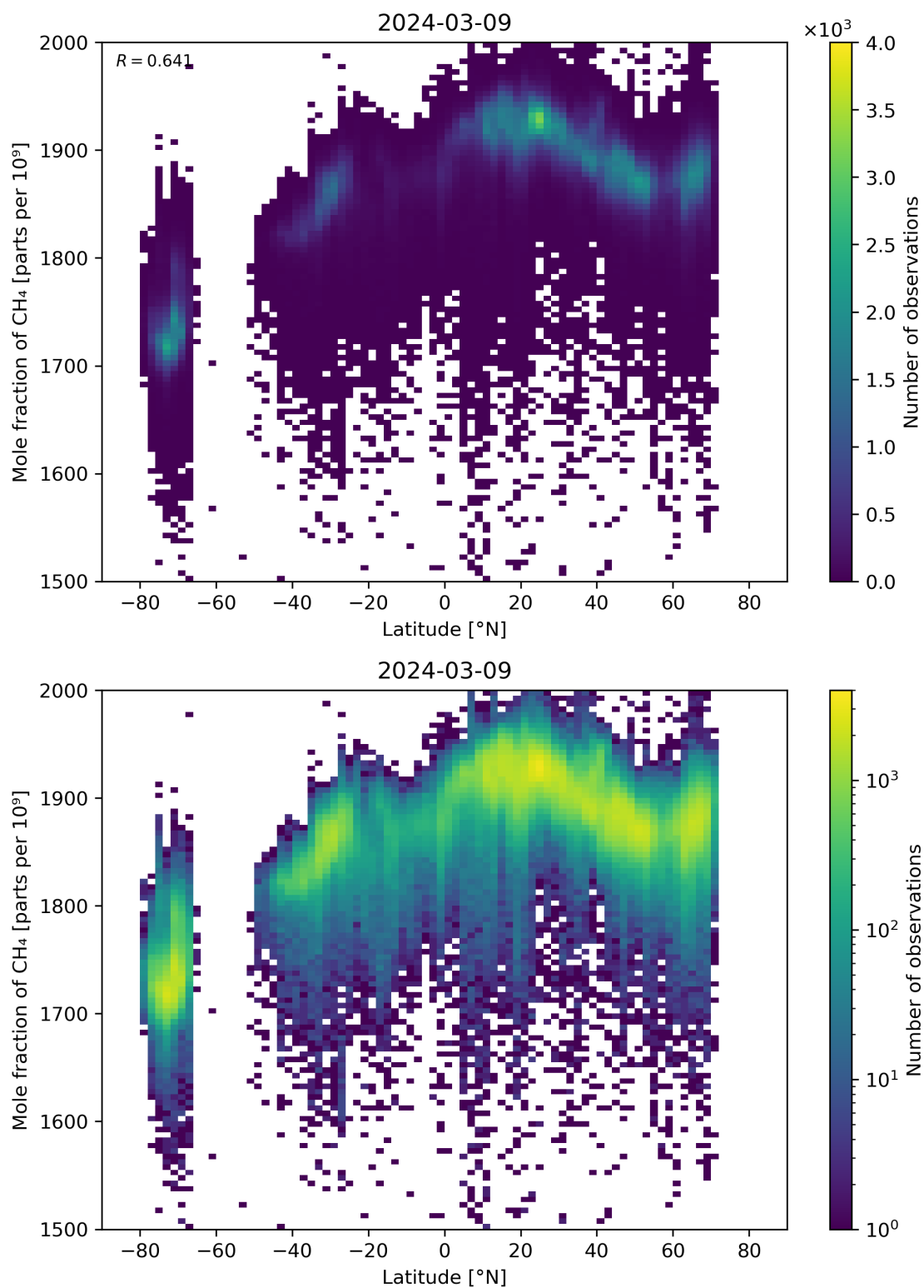
Figure 57: Scatter density plot of “Latitude” against “Mole fraction of CH 4 ” for 2024-03-09 to 2024-03-10.
