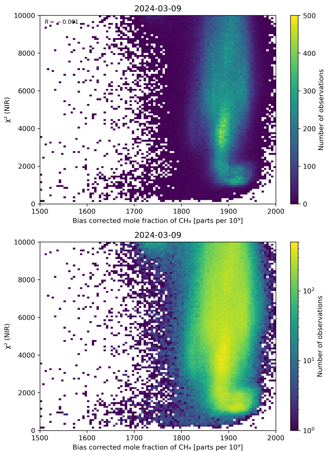
Figure 63: Scatter density plot of “Bias corrected mole fraction of CH 4 ” against “ \chi^2 (NIR)” for 2024-03-09 to 2024-03-10.
