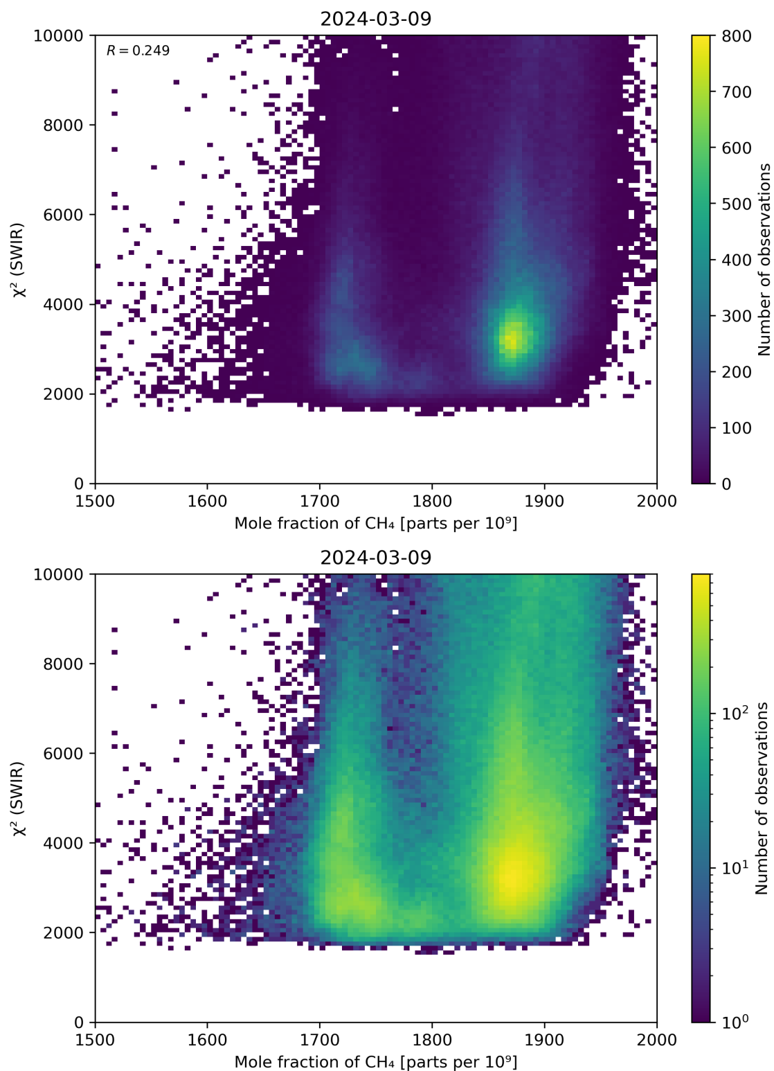
Figure 71: Scatter density plot of “Mole fraction of \text{CH}_4 ” against “ \chi^2 (SWIR)” for 2024-03-09 to 2024-03-10.
