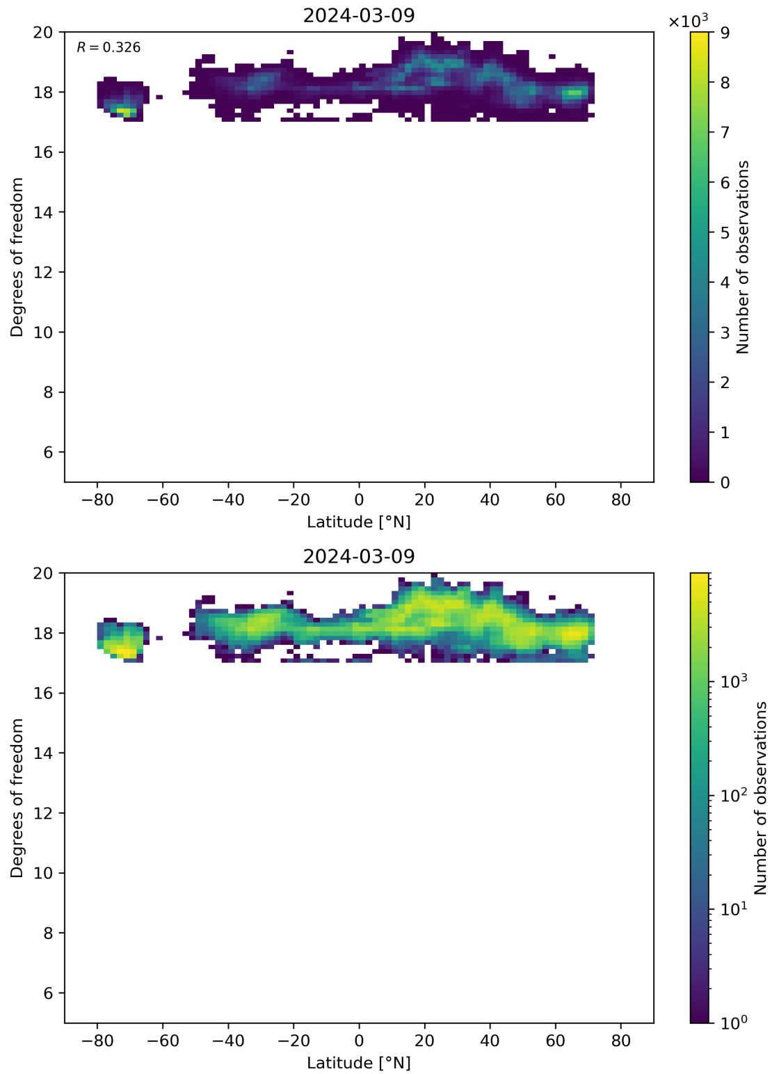
Figure 55: Scatter density plot of “Latitude” against “Degrees of freedom” for 2024-03-09 to 2024-03-10.
