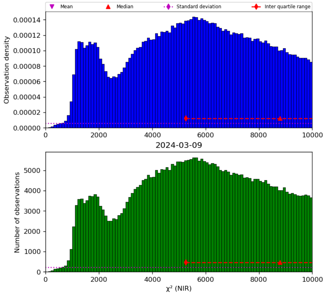
Figure 29: Histogram of “ \chi^2 (NIR)” for 2024-03-09 to 2024-03-10
