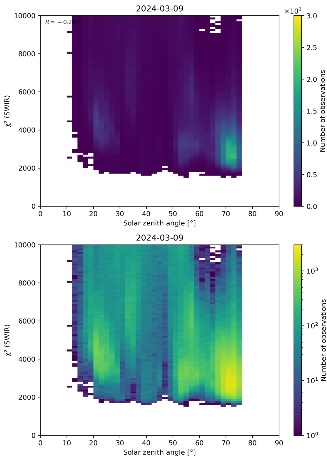
Figure 95: Scatter density plot of “Solar zenith angle” against “ \chi^2 (SWIR)” for 2024-03-09 to 2024-03-10.
