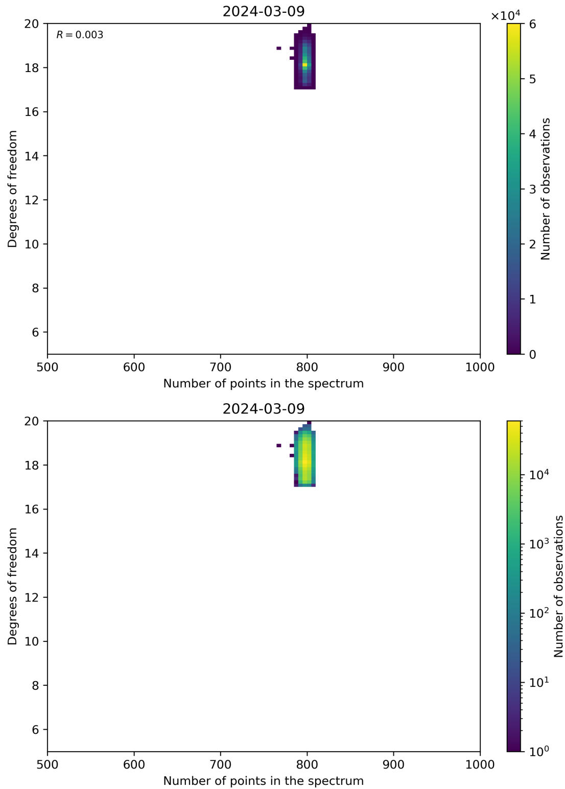
Figure 90: Scatter density plot of “Number of points in the spectrum” against “Degrees of freedom” for 2024-03-09 to 2024-03-10.
