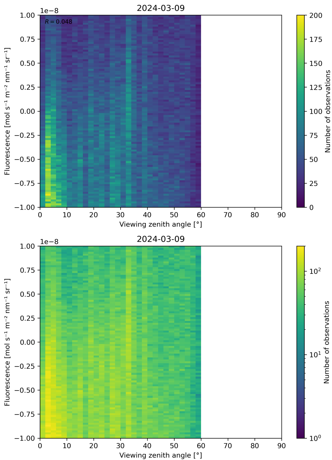
Figure 108: Scatter density plot of “Viewing zenith angle” against “Fluorescence” for 2024-03-09 to 2024-03-10.
