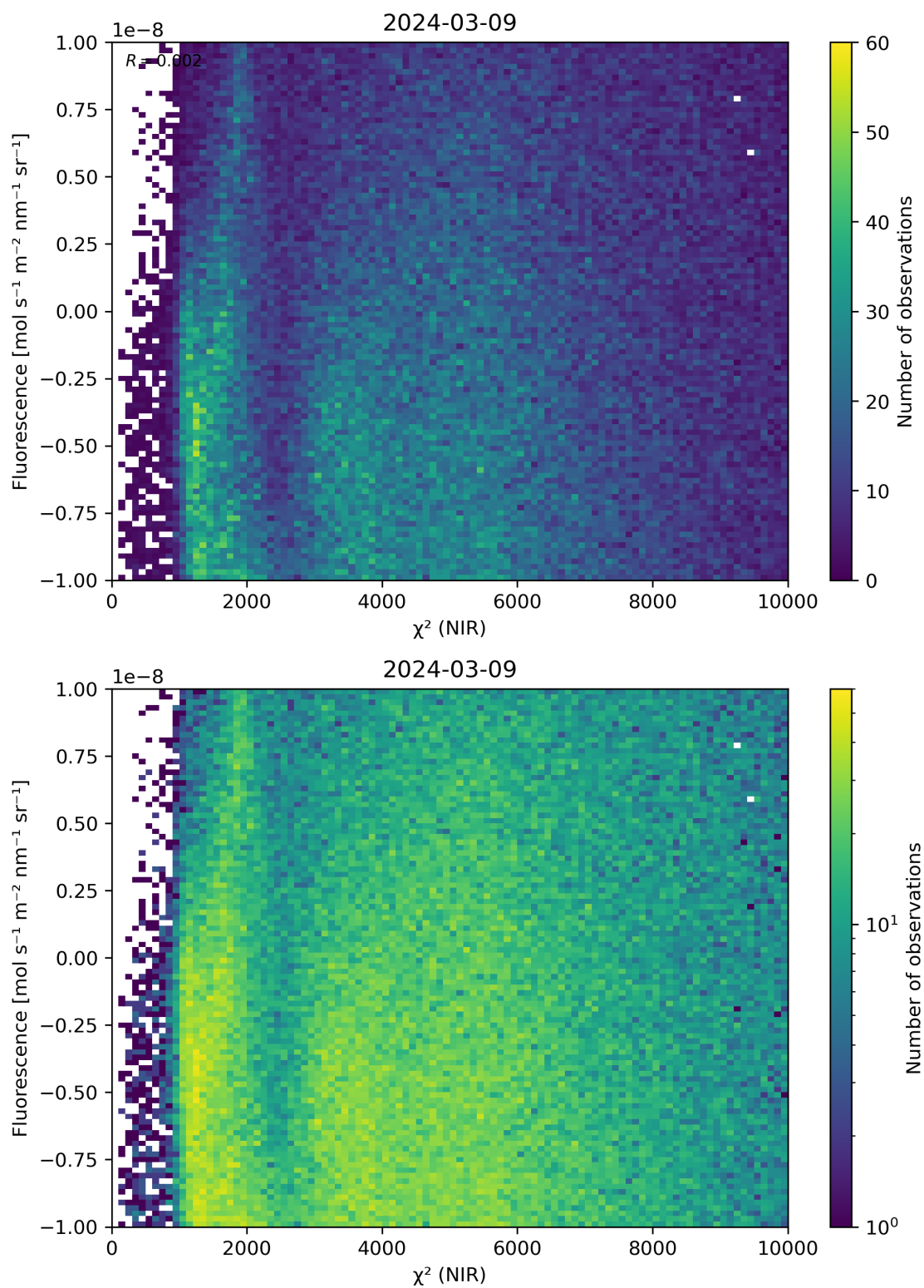
Figure 45: Scatter density plot of “ \chi^2 (NIR)” against “Fluorescence” for 2024-03-09 to 2024-03-10.
