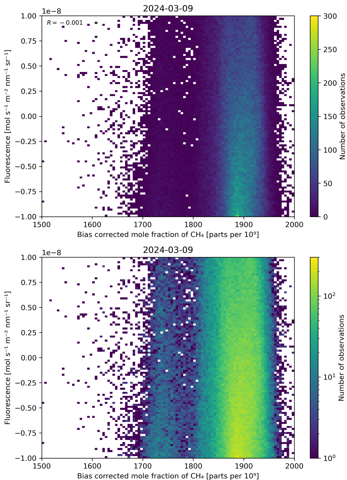
Figure 66: Scatter density plot of “Bias corrected mole fraction of \text{CH}_4 ” against “Fluorescence” for 2024-03-09 to 2024-03-10.
