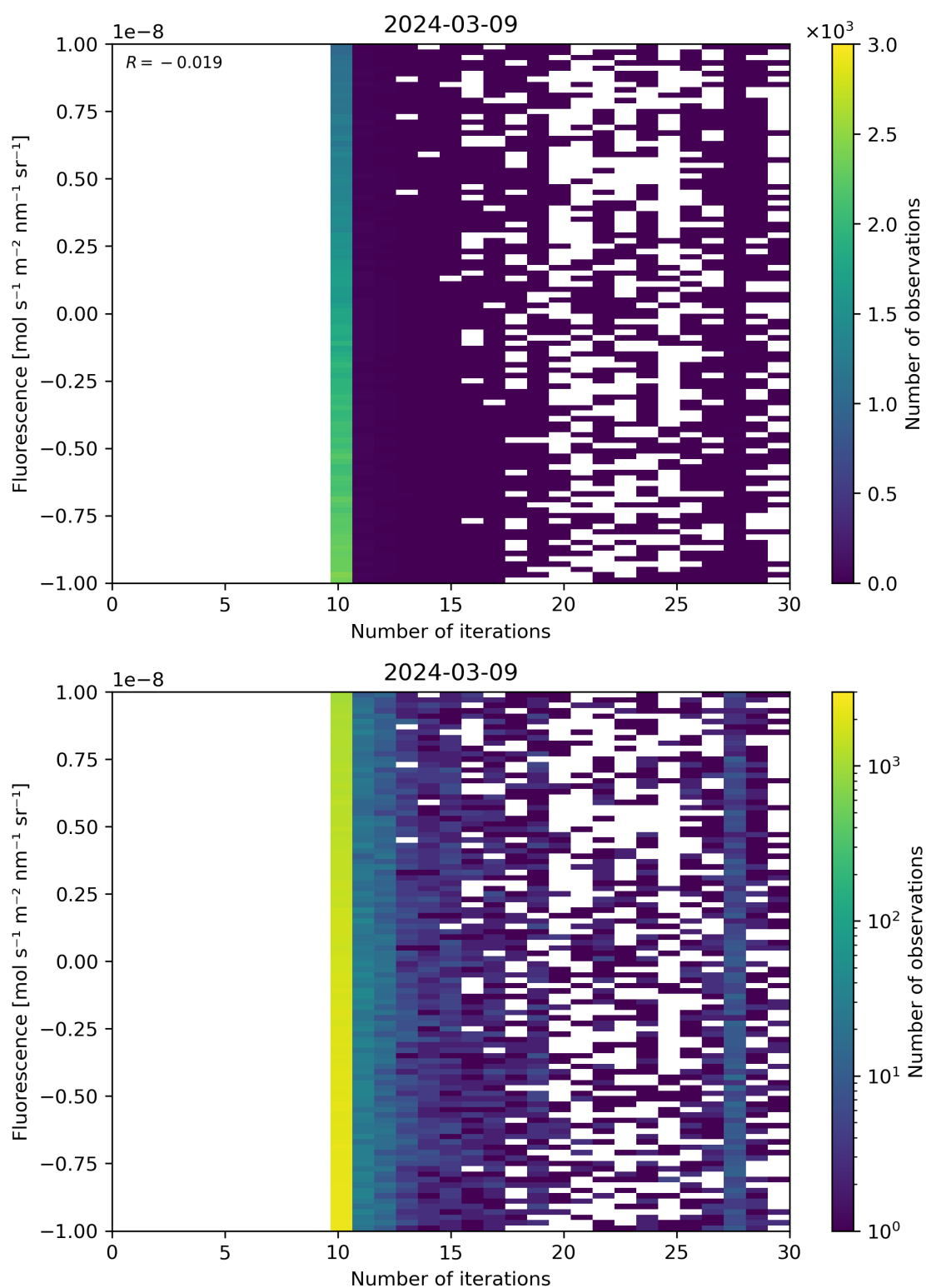
Figure 87: Scatter density plot of “Number of iterations” against “Fluorescence” for 2024-03-09 to 2024-03-10.
