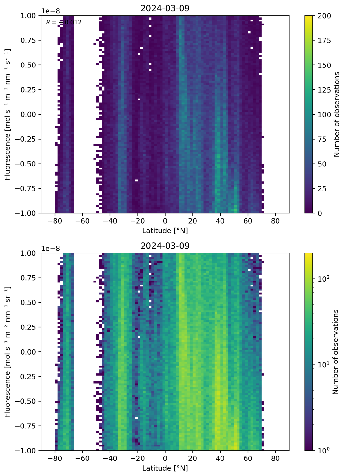
Figure 56: Scatter density plot of “Latitude” against “Fluorescence” for 2024-03-09 to 2024-03-10.
