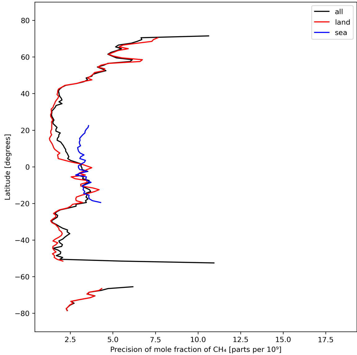
Figure 13: Zonal average of “Precision of mole fraction of CH 4 ” for 2024-03-09 to 2024-03-10.
