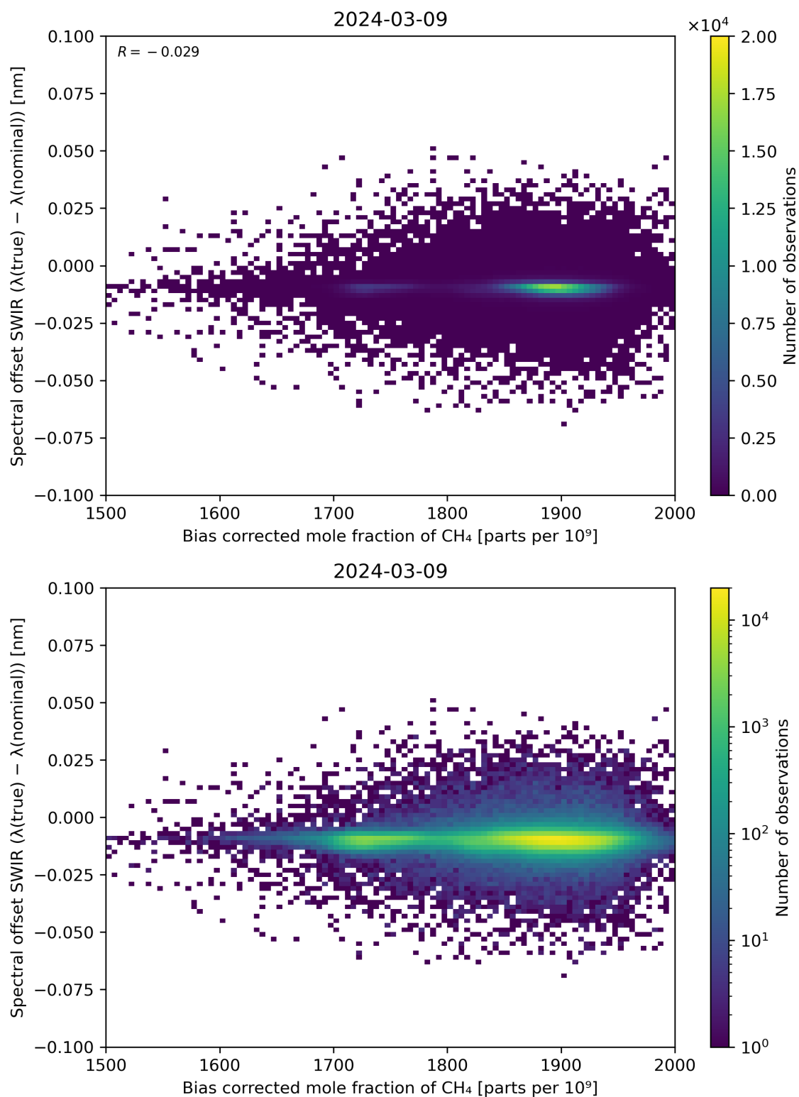
Figure 69: Scatter density plot of “Bias corrected mole fraction of \text{CH}_4 ” against “Spectral offset SWIR ( \lambda(\text{true}) - \lambda(\text{nominal}) )” for 2024-03-09 to 2024-03-10.
