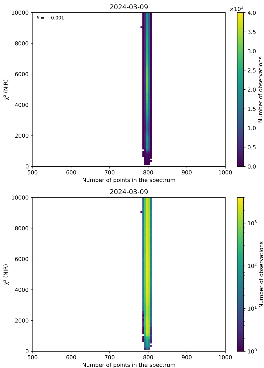
Figure 88: Scatter density plot of “Number of points in the spectrum” against “ \chi^2 (NIR)” for 2024-03-09 to 2024-03-10.
