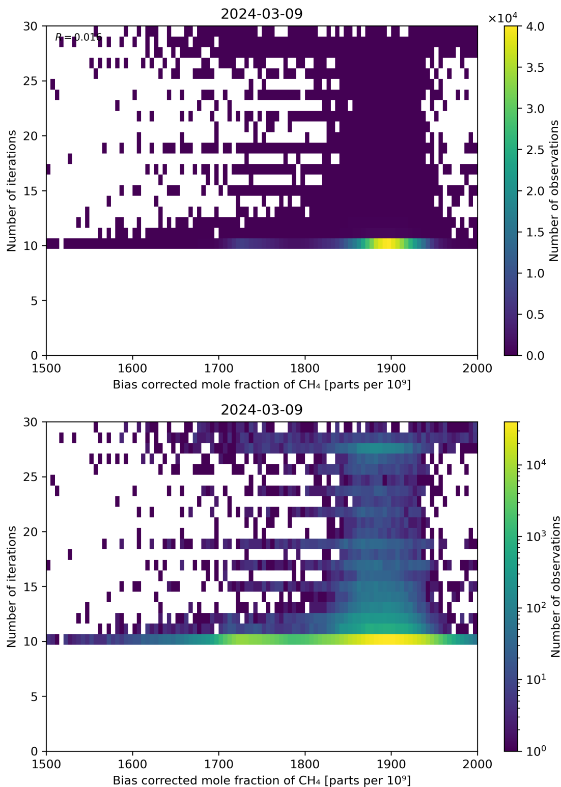
Figure 67: Scatter density plot of “Bias corrected mole fraction of CH 4 ” against “Number of iterations” for 2024-03-09 to 2024-03-10.
