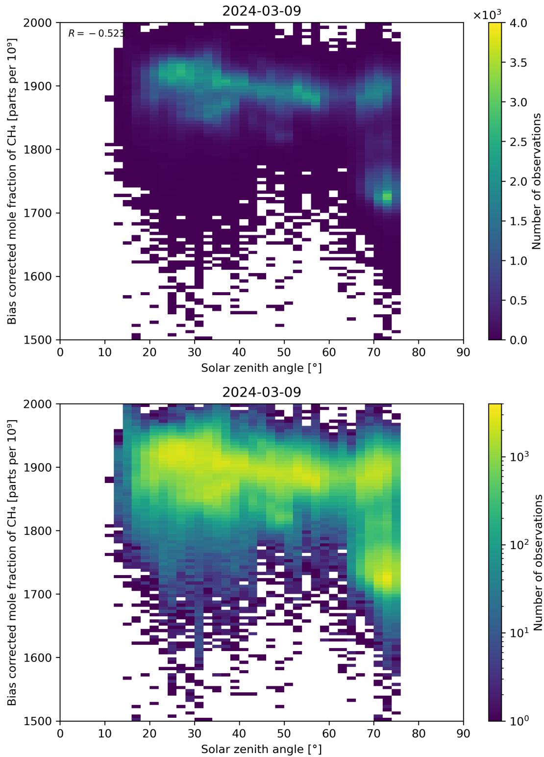
Figure 100: Scatter density plot of “Solar zenith angle” against “Bias corrected mole fraction of CH 4 ” for 2024-03-09 to 2024-03-10.
