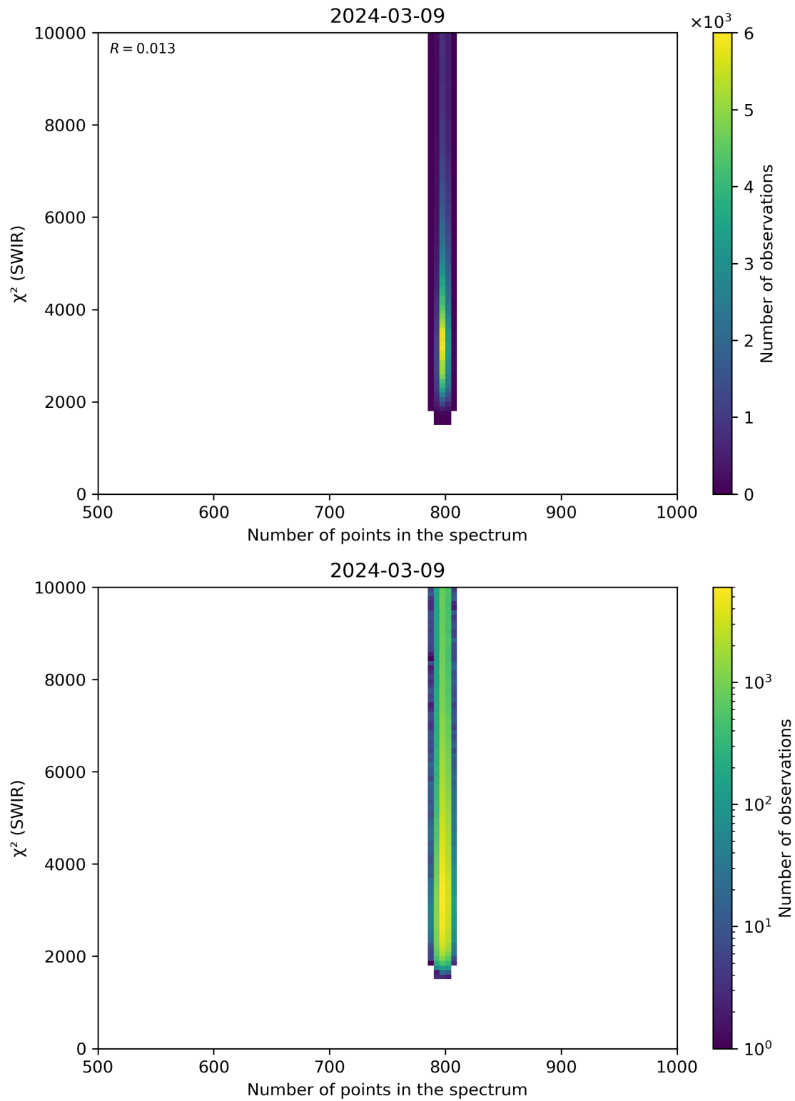
Figure 89: Scatter density plot of “Number of points in the spectrum” against “ \chi^2 (SWIR)” for 2024-03-09 to 2024-03-10.
