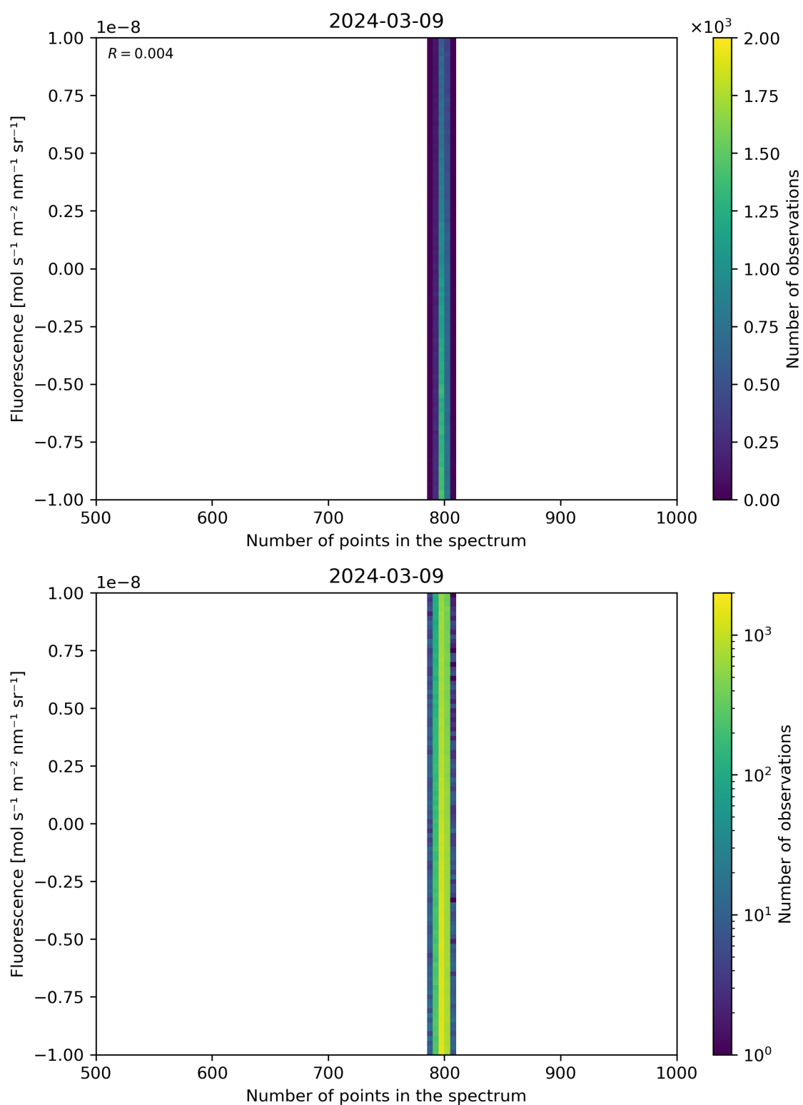
Figure 91: Scatter density plot of “Number of points in the spectrum” against “Fluorescence” for 2024-03-09 to 2024-03-10.
