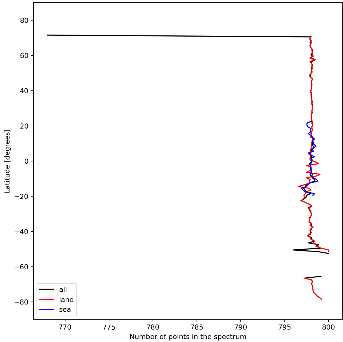
Figure 15: Zonal average of “Number of points in the spectrum” for 2024-03-09 to 2024-03-10.
