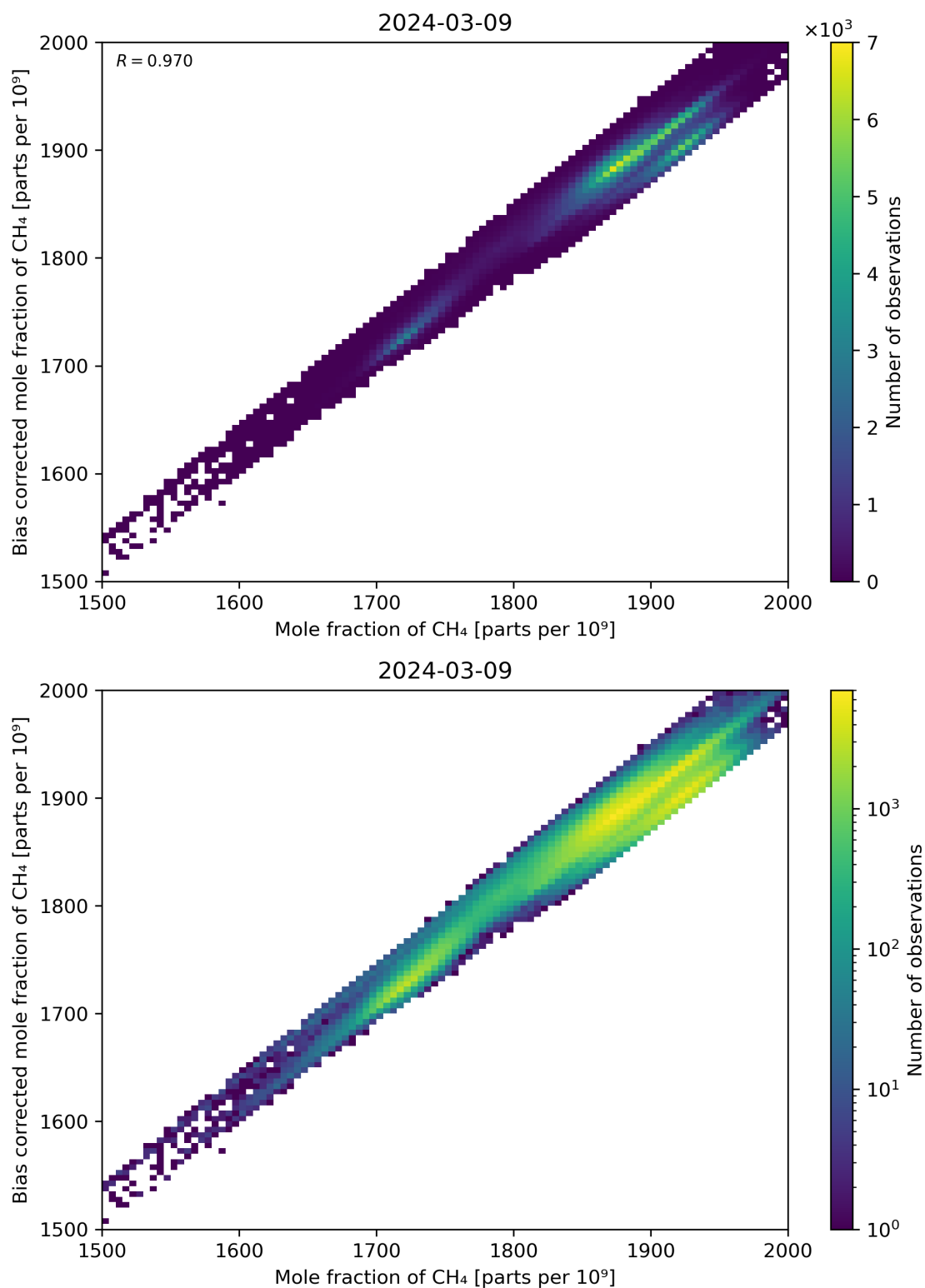
Figure 74: Scatter density plot of “Mole fraction of CH 4 ” against “Bias corrected mole fraction of CH 4 ” for 2024-03-09 to 2024-03-10.
