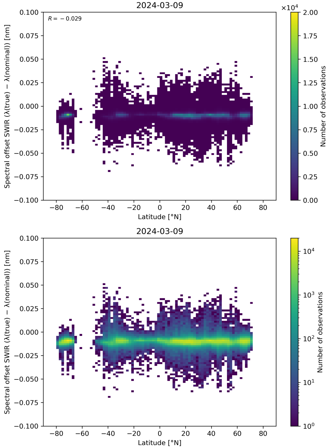
Figure 62: Scatter density plot of “Latitude” against “Spectral offset SWIR ( \lambda(\text{true}) - \lambda(\text{nominal}) )” for 2024-03-09 to 2024-03-10.
