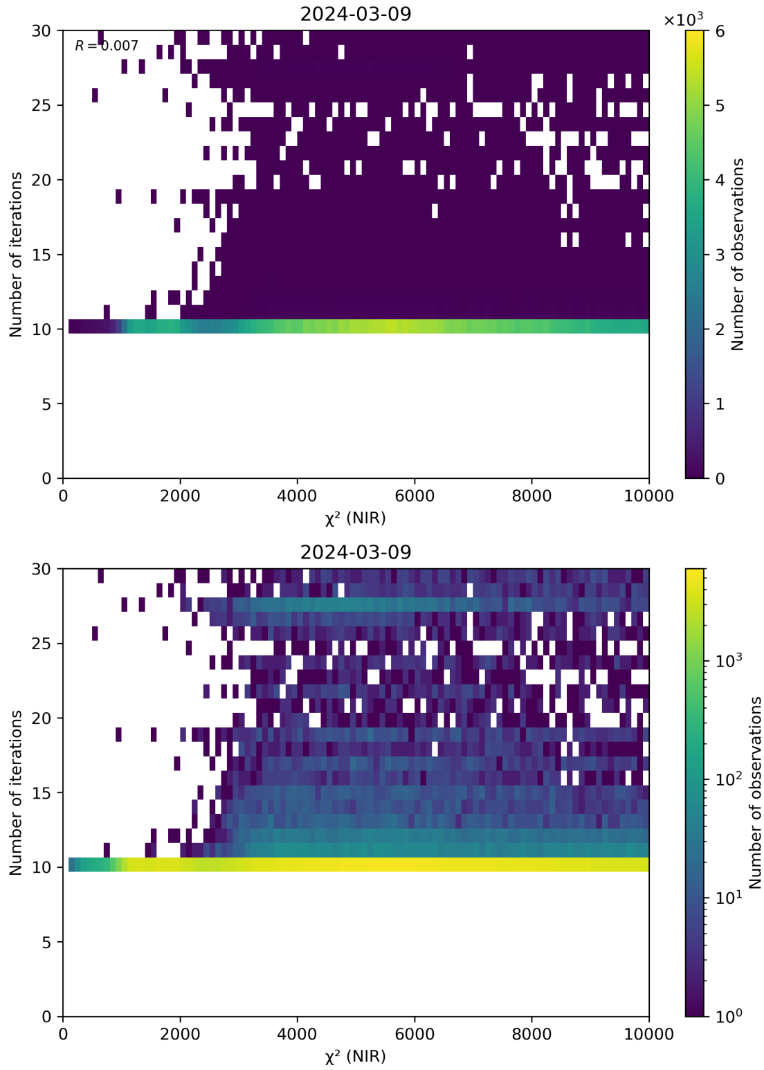
Figure 46: Scatter density plot of “ \chi^2 (NIR)” against “Number of iterations” for 2024-03-09 to 2024-03-10.
