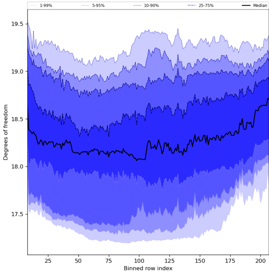
Figure 41: Along track statistics of “Degrees of freedom” for 2024-03-09 to 2024-03-10
