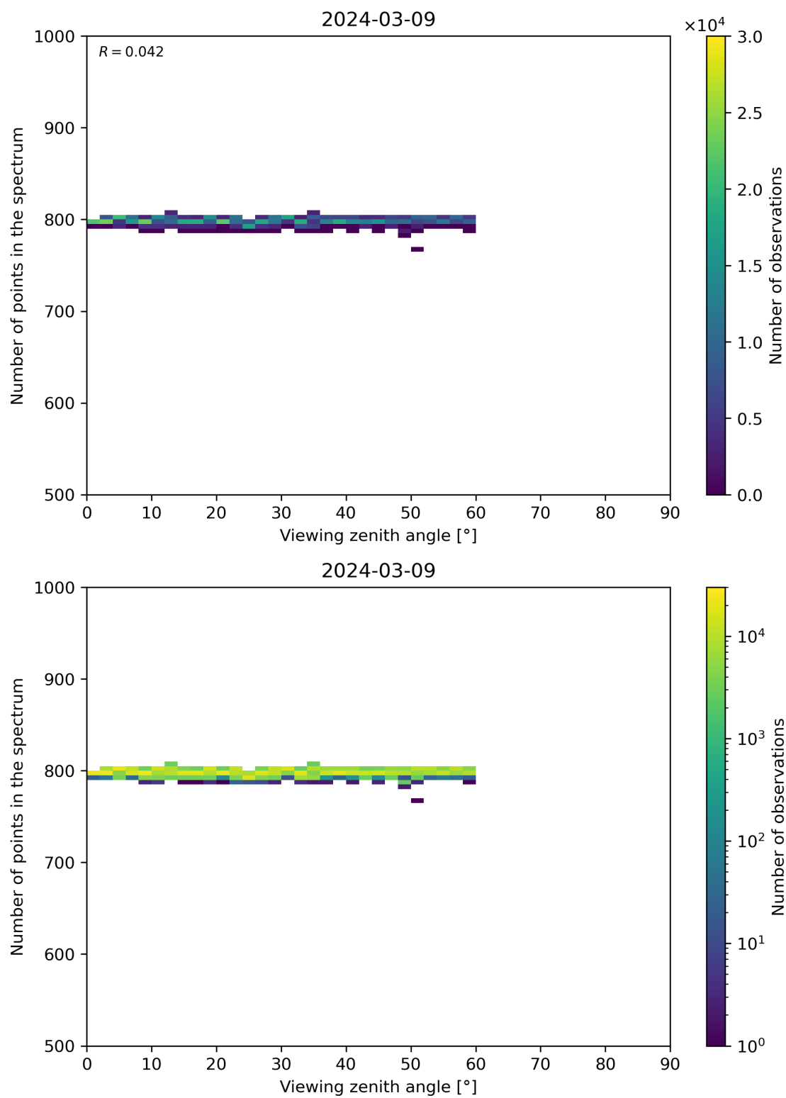
Figure 114: Scatter density plot of “Viewing zenith angle” against “Number of points in the spectrum” for 2024-03-09 to 2024-03-10.
