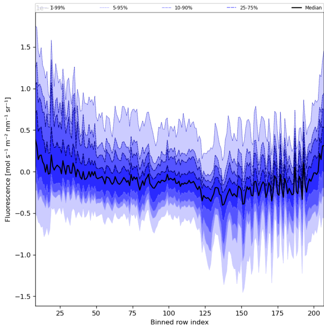
Figure 43: Along track statistics of “Fluorescence” for 2024-03-09 to 2024-03-10
