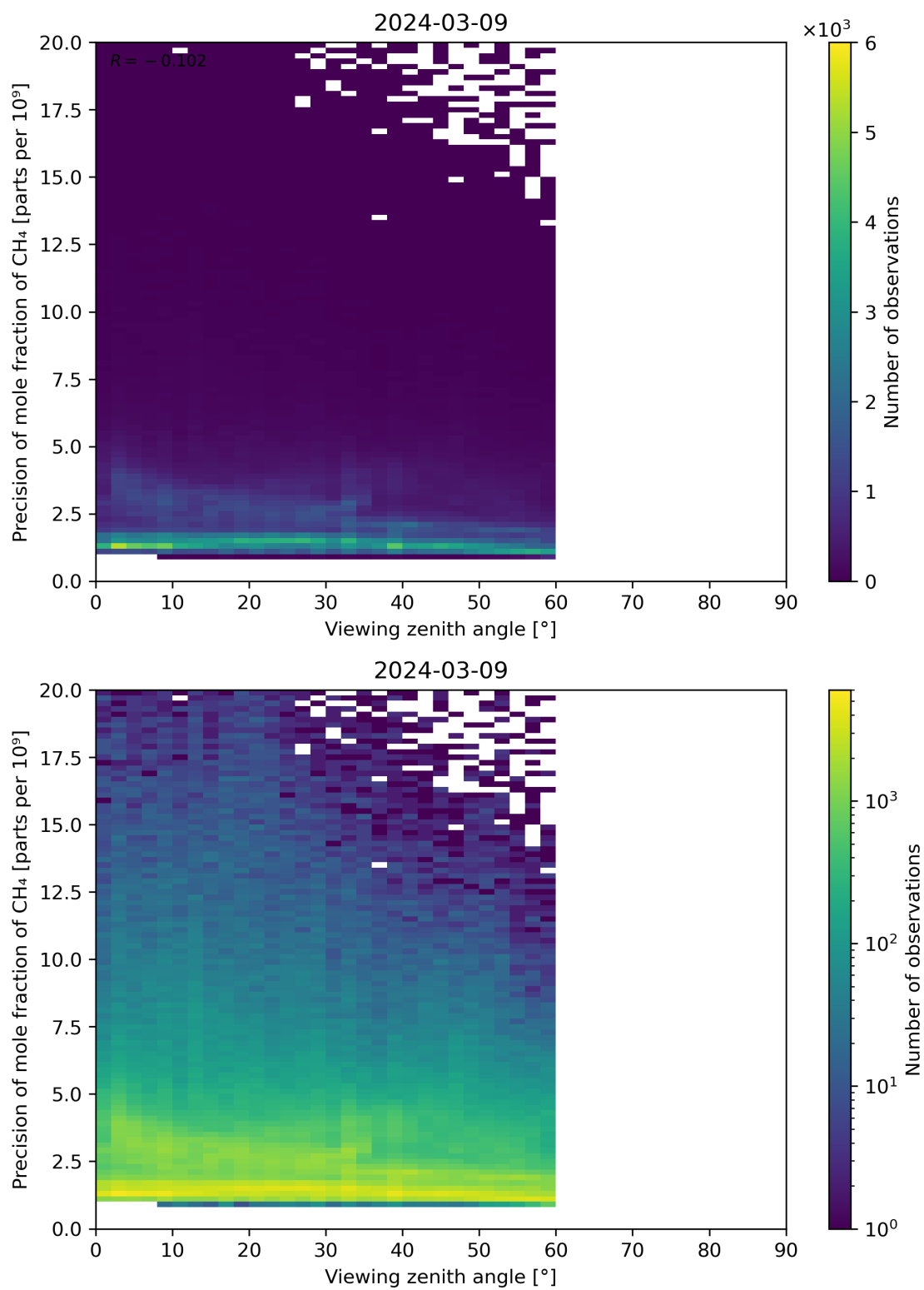
Figure 112: Scatter density plot of “Viewing zenith angle” against “Precision of mole fraction of CH 4 ” for 2024-03-09 to 2024-03-10.
