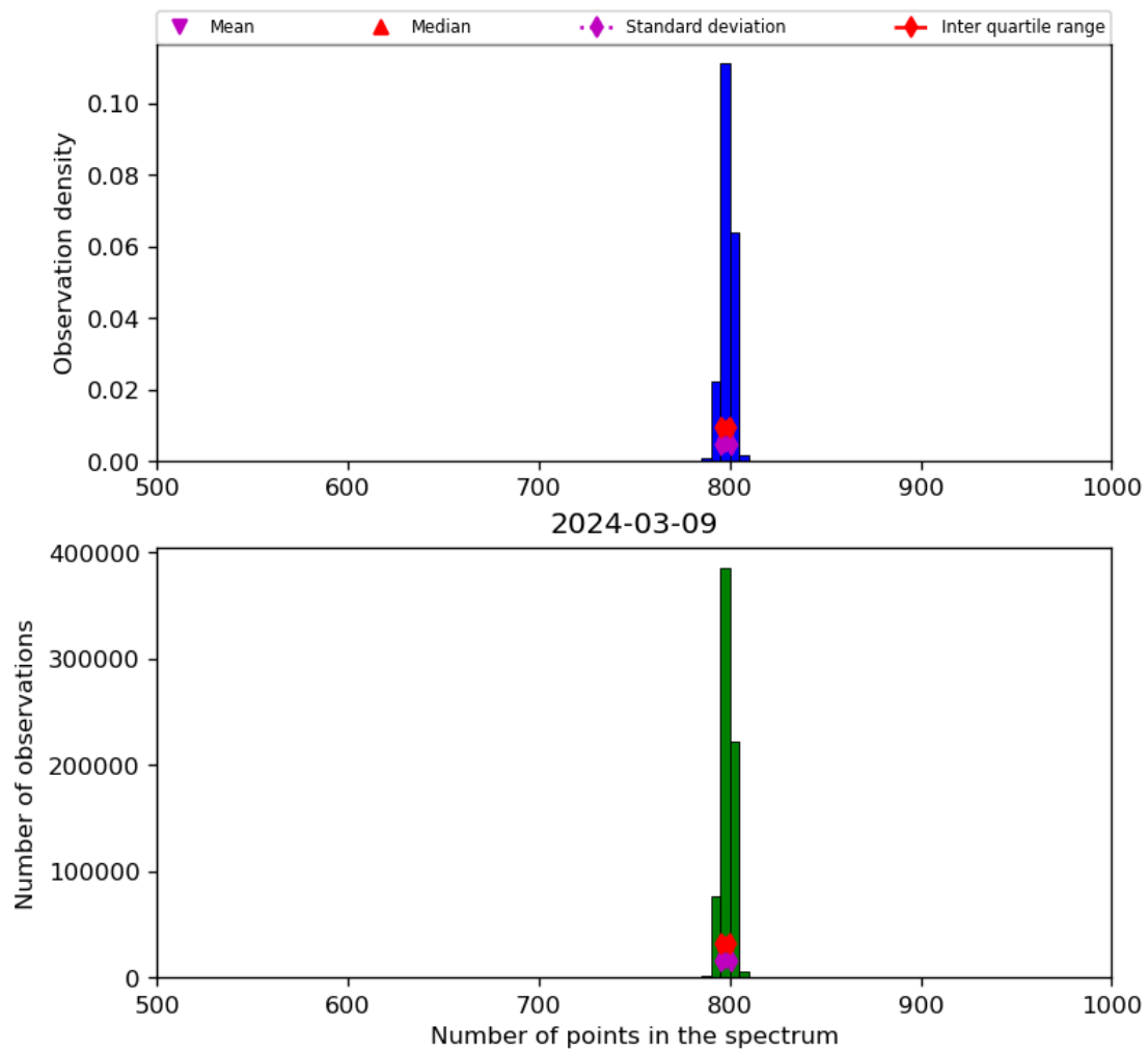
Figure 26: Histogram of “Number of points in the spectrum” for 2024-03-09 to 2024-03-10
