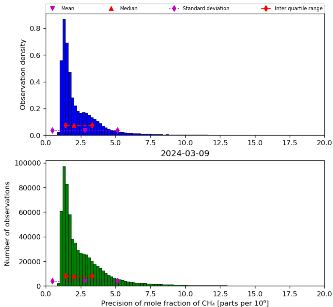
Figure 24: Histogram of “Precision of mole fraction of CH 4 ” for 2024-03-09 to 2024-03-10
