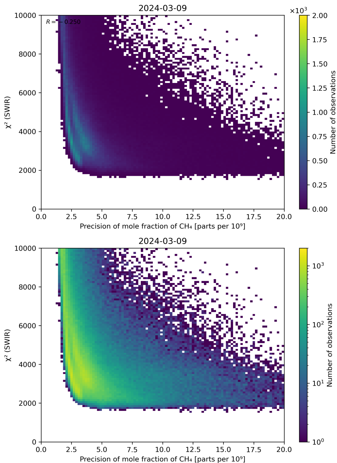
Figure 79: Scatter density plot of “Precision of mole fraction of \text{CH}_4 ” against “ \chi^2 (SWIR)” for 2024-03-09 to 2024-03-10.
