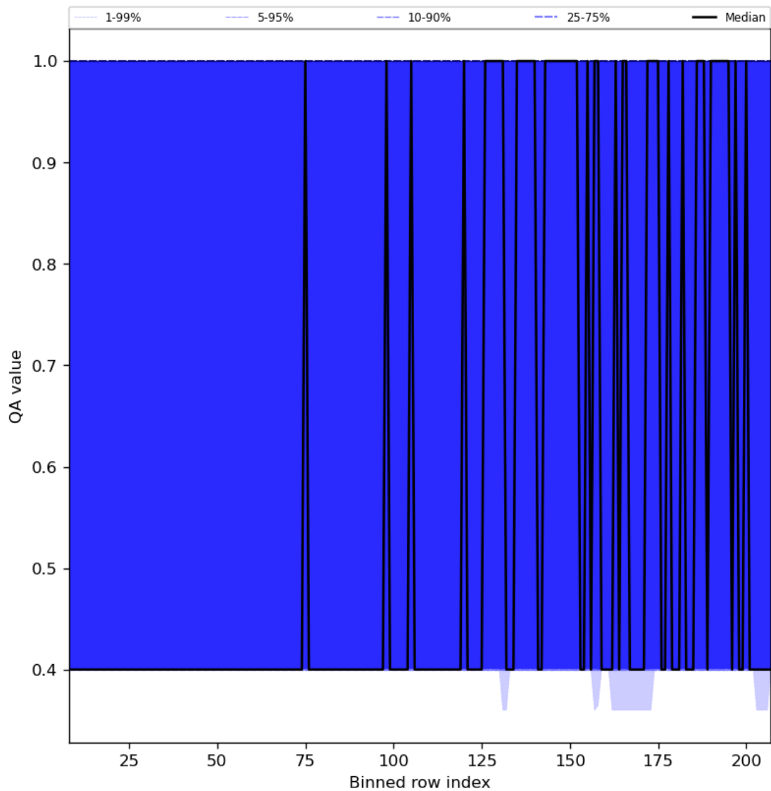
Figure 33: Along track statistics of “QA value” for 2024-03-09 to 2024-03-10
