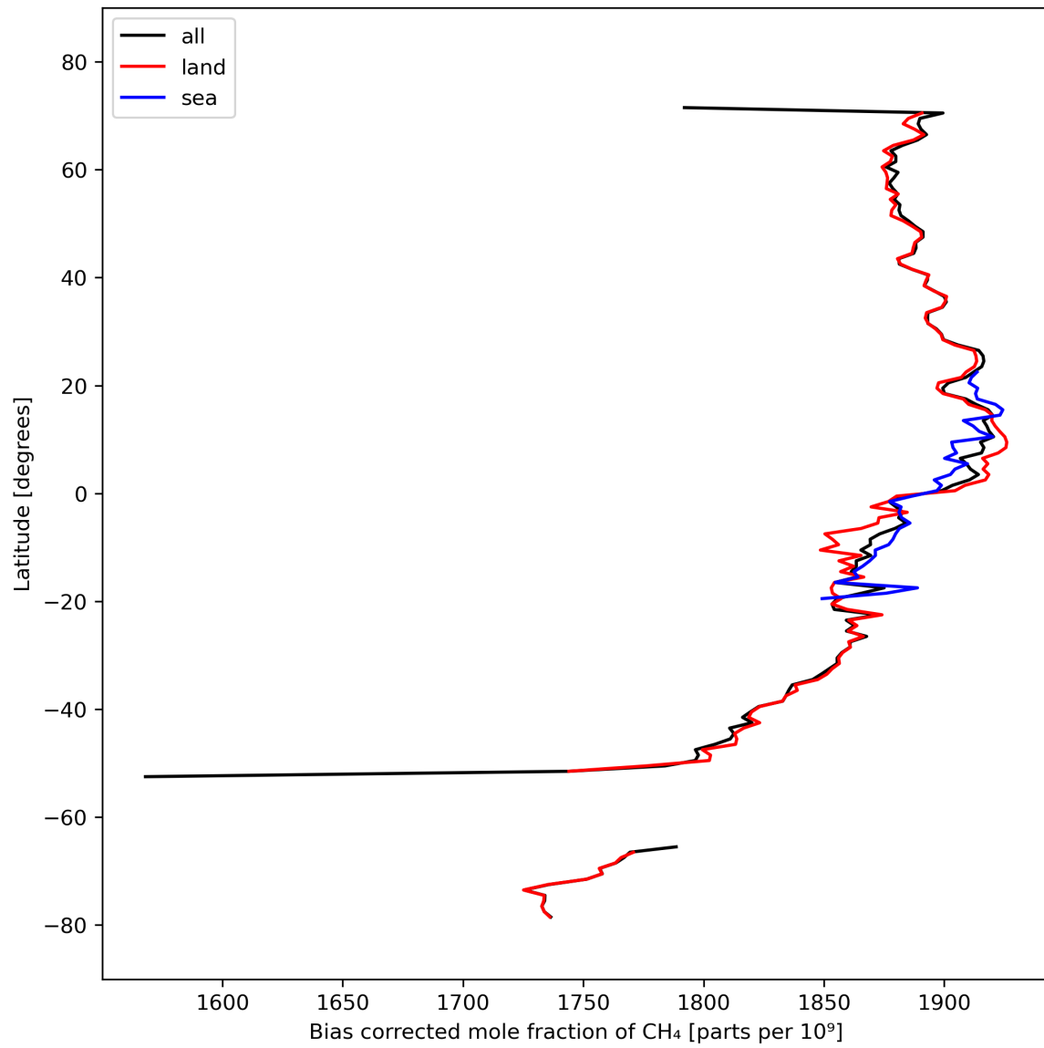
Figure 14: Zonal average of “Bias corrected mole fraction of CH 4 ” for 2024-03-09 to 2024-03-10.
