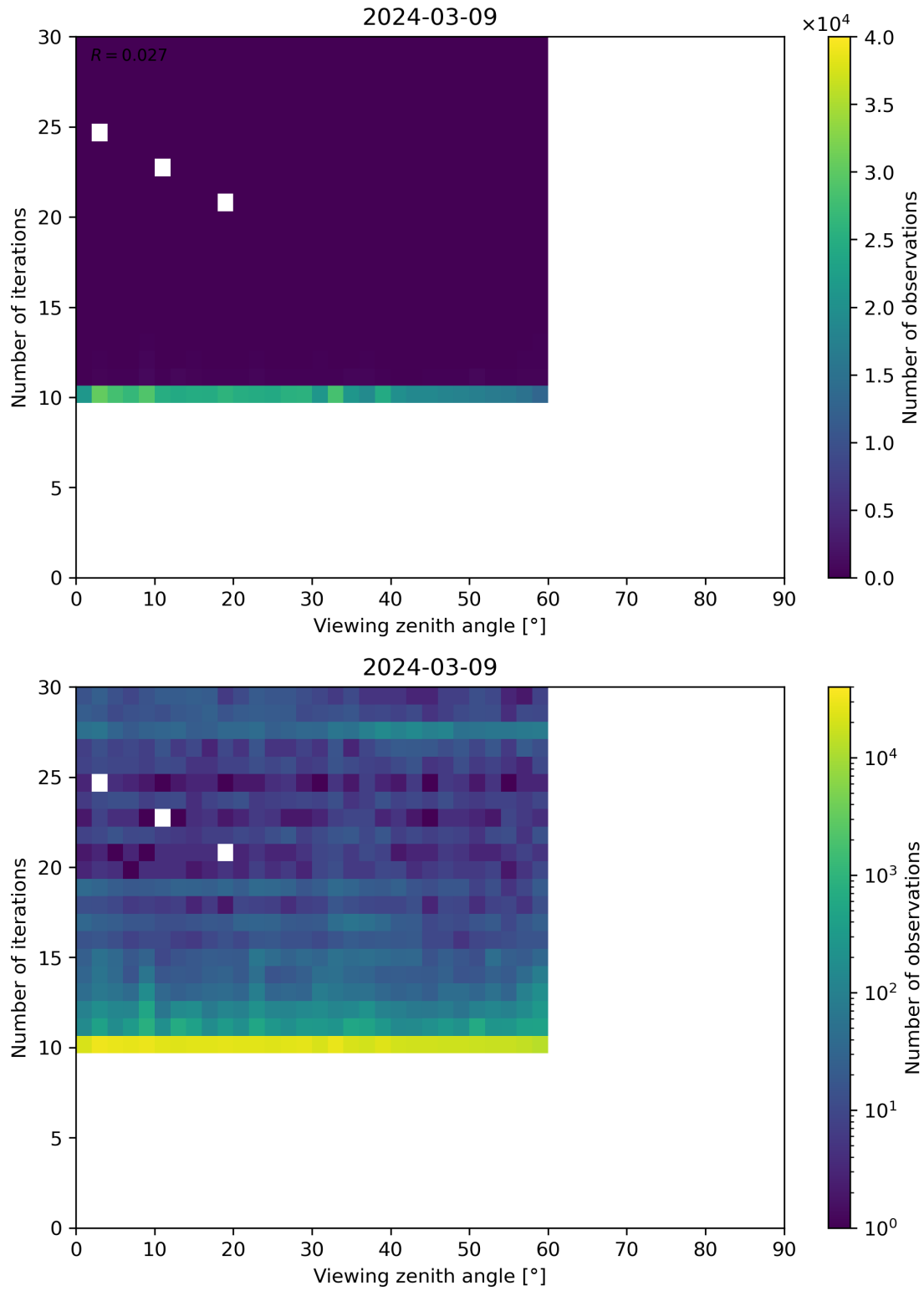
Figure 113: Scatter density plot of “Viewing zenith angle” against “Number of iterations” for 2024-03-09 to 2024-03-10.
