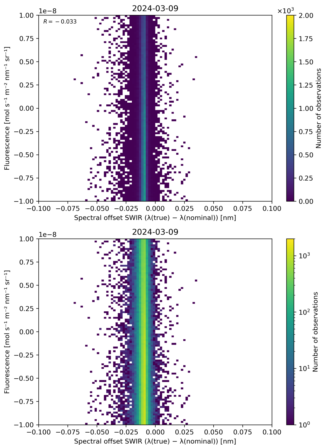
Figure 120: Scatter density plot of “Spectral offset SWIR ( \lambda(\text{true}) - \lambda(\text{nominal}) )” against “Fluorescence” for 2024-03-09 to 2024-03-10.
