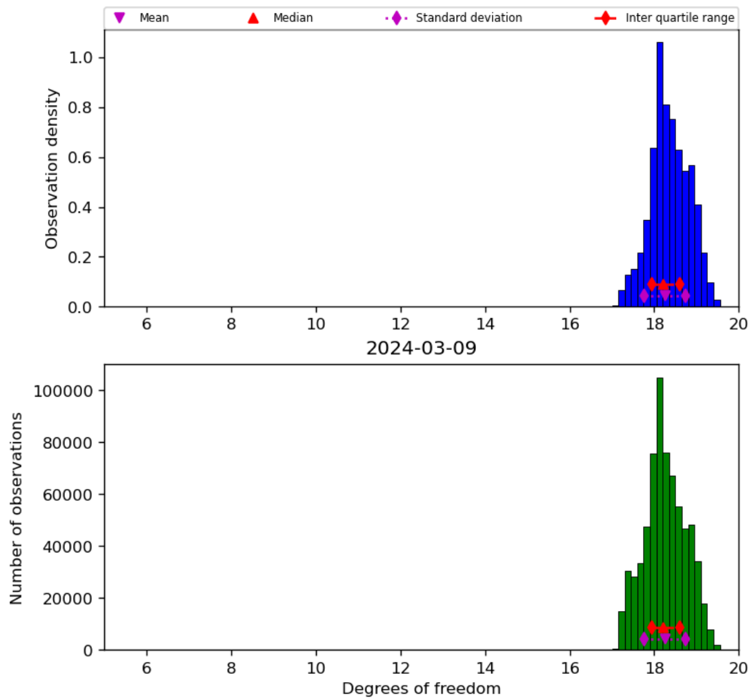
Figure 30: Histogram of “Degrees of freedom” for 2024-03-09 to 2024-03-10
