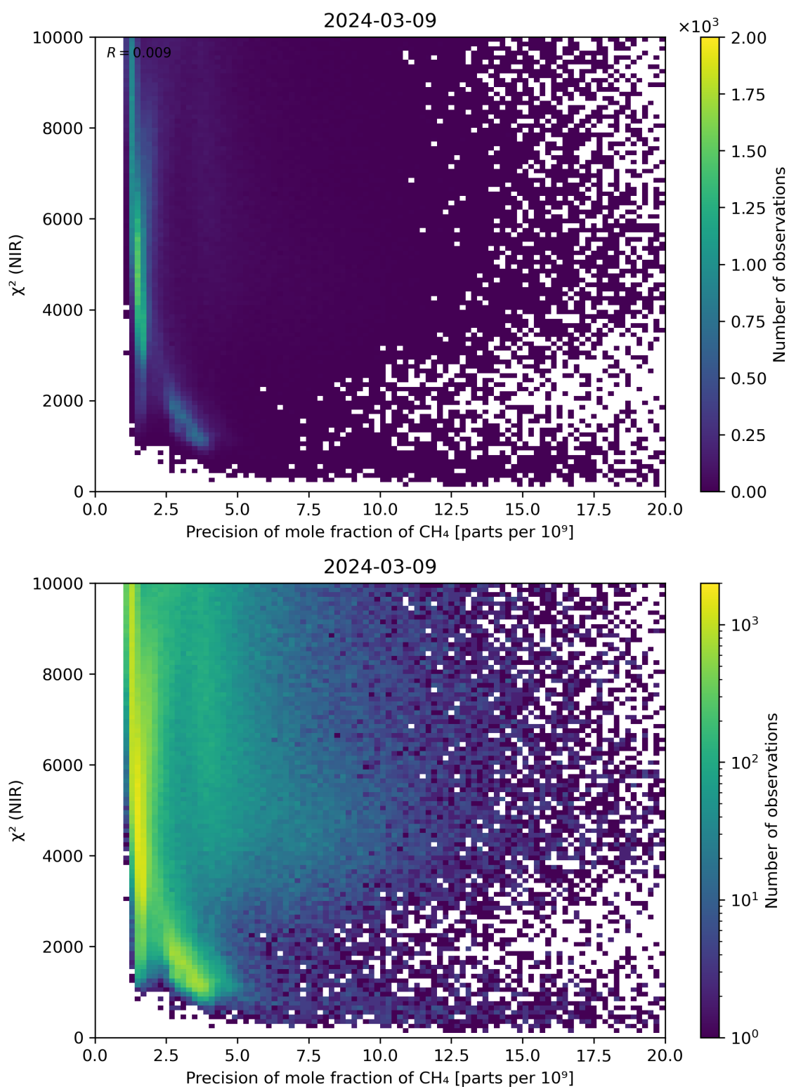
Figure 78: Scatter density plot of “Precision of mole fraction of CH 4 ” against “ \chi^2 (NIR)” for 2024-03-09 to 2024-03-10.
