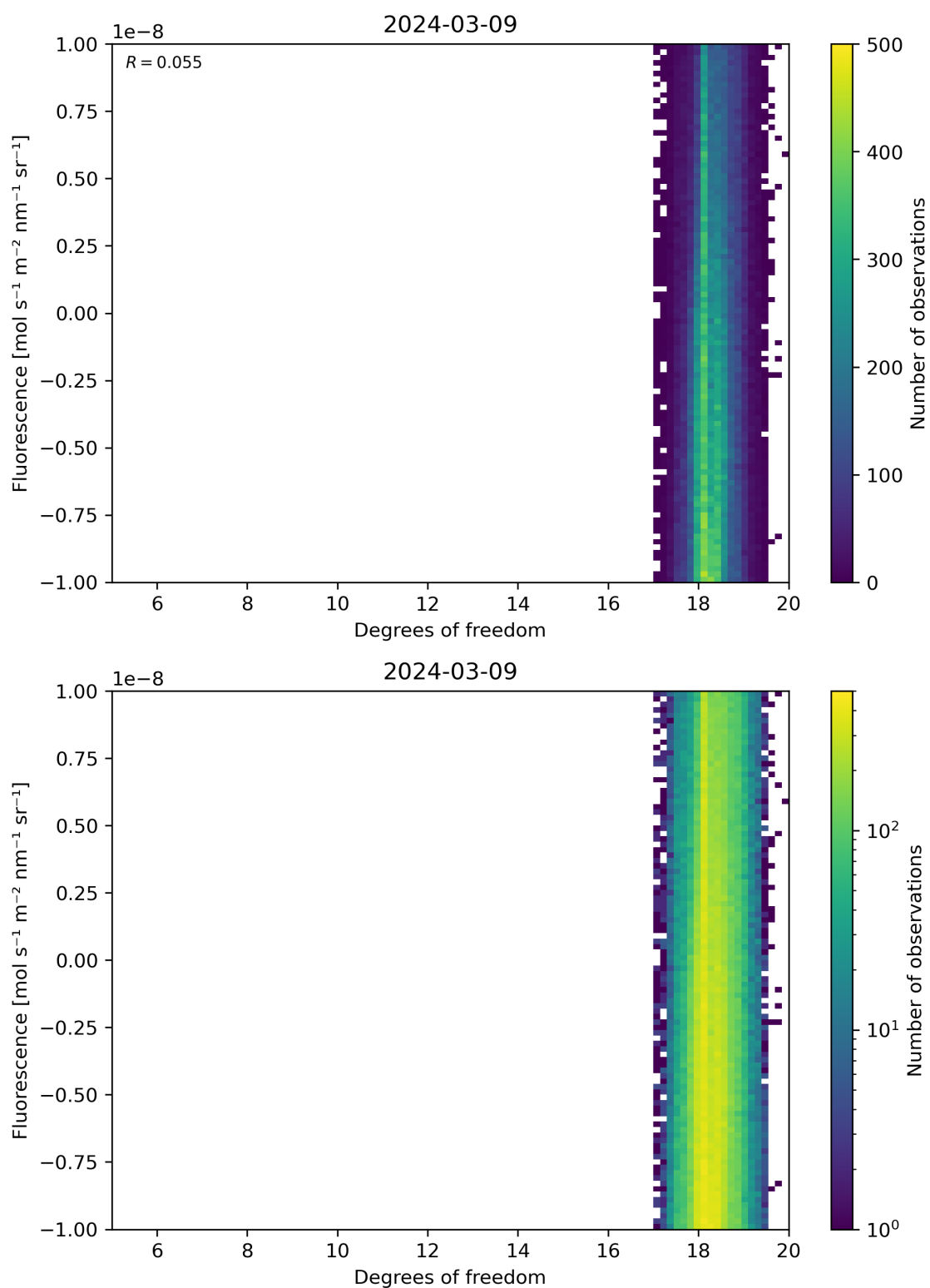
Figure 51: Scatter density plot of “Degrees of freedom” against “Fluorescence” for 2024-03-09 to 2024-03-10.
