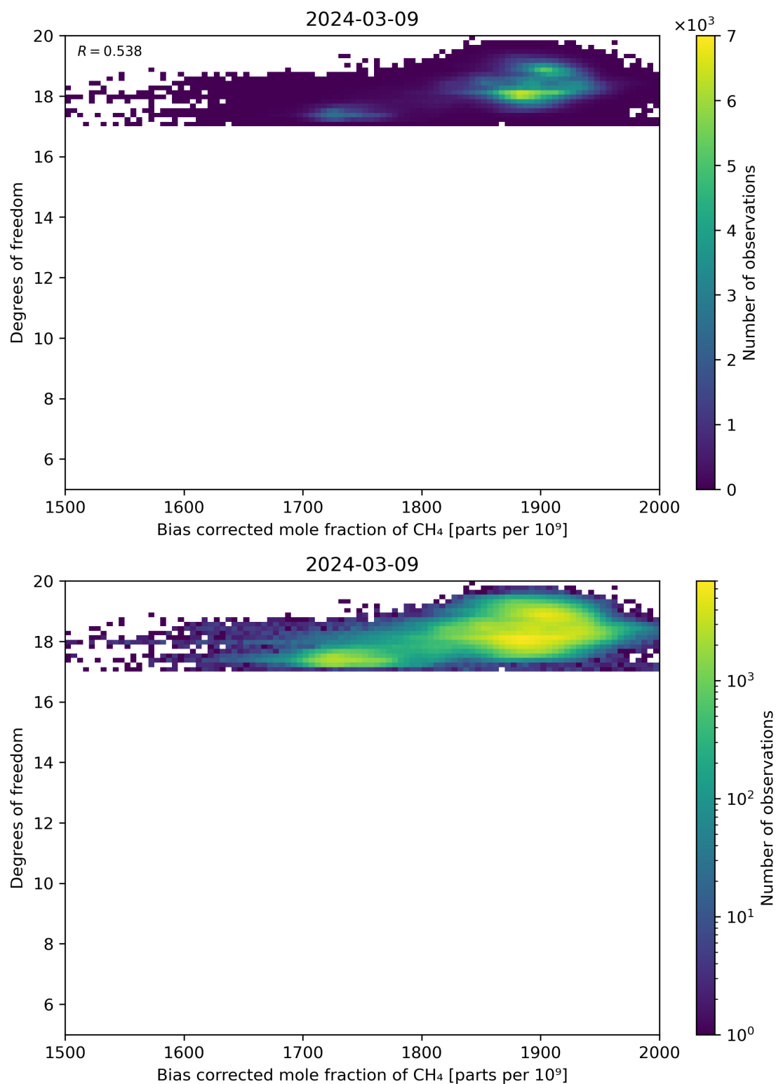
Figure 65: Scatter density plot of “Bias corrected mole fraction of CH 4 ” against “Degrees of freedom” for 2024-03-09 to 2024-03-10.
