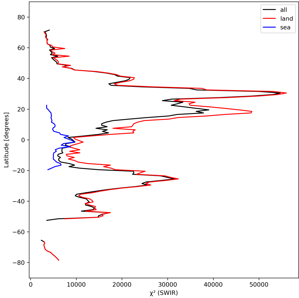
Figure 17: Zonal average of “ \chi^2 (SWIR)” for 2024-03-09 to 2024-03-10.
