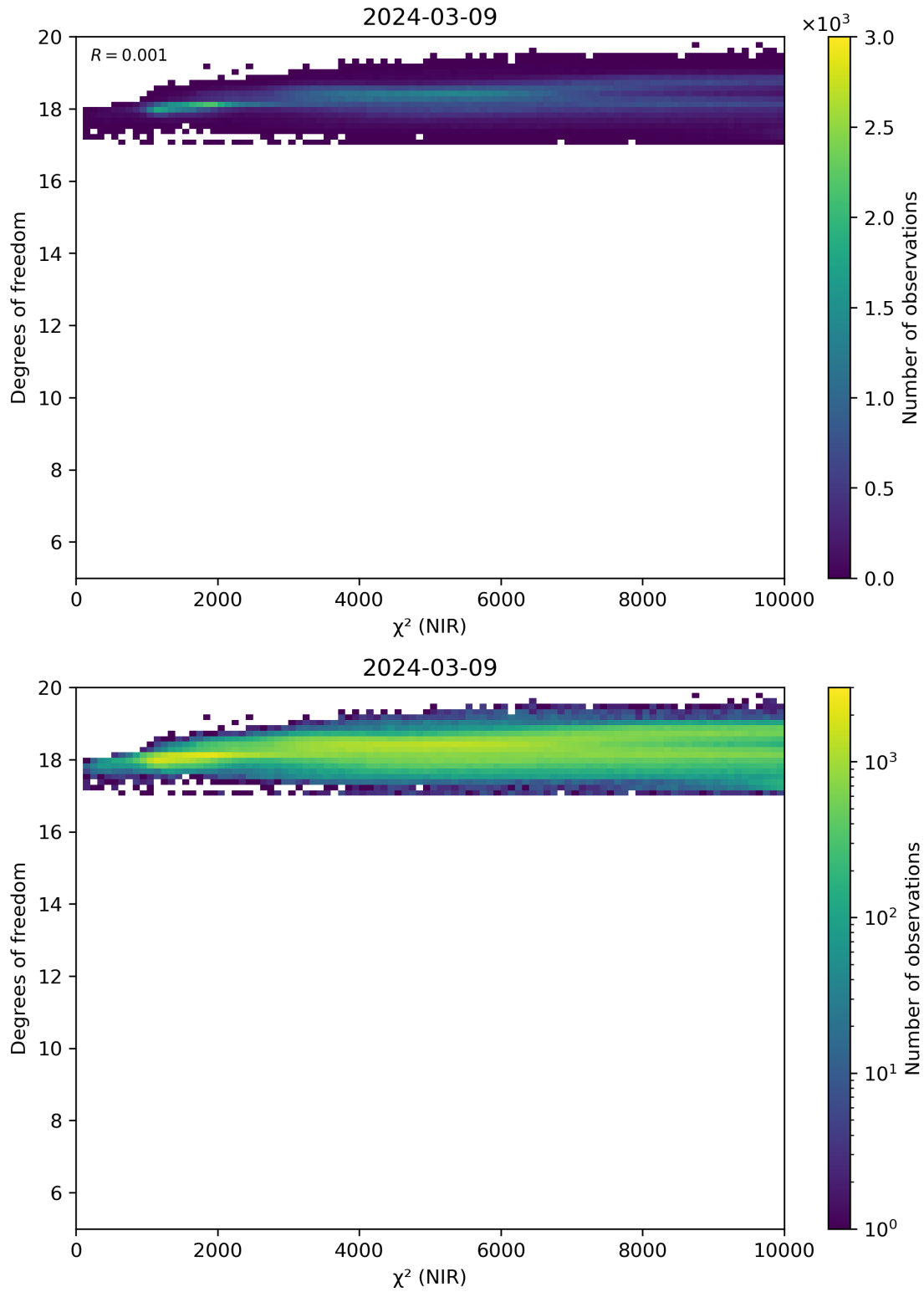
Figure 44: Scatter density plot of “ \chi^2 (NIR)” against “Degrees of freedom” for 2024-03-09 to 2024-03-10.
