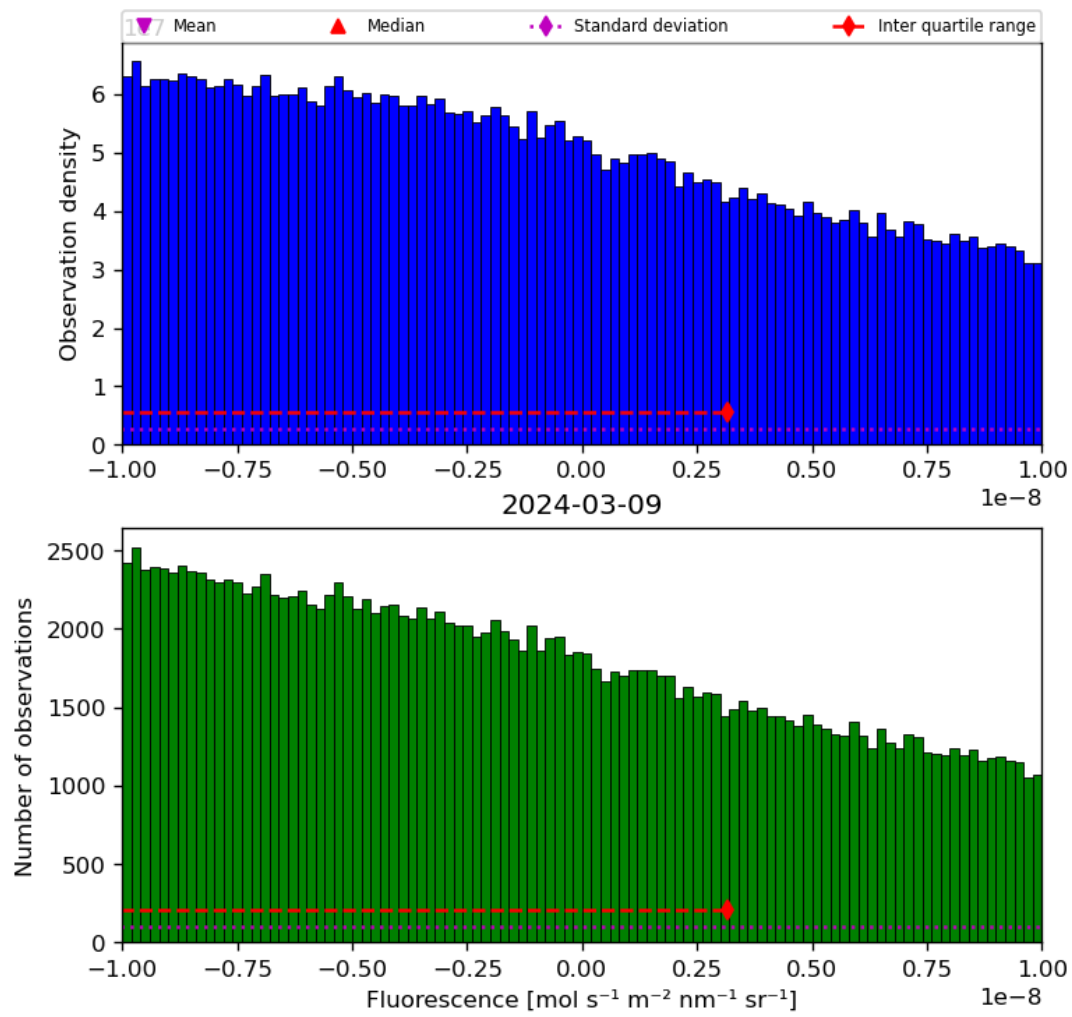
Figure 32: Histogram of “Fluorescence” for 2024-03-09 to 2024-03-10
