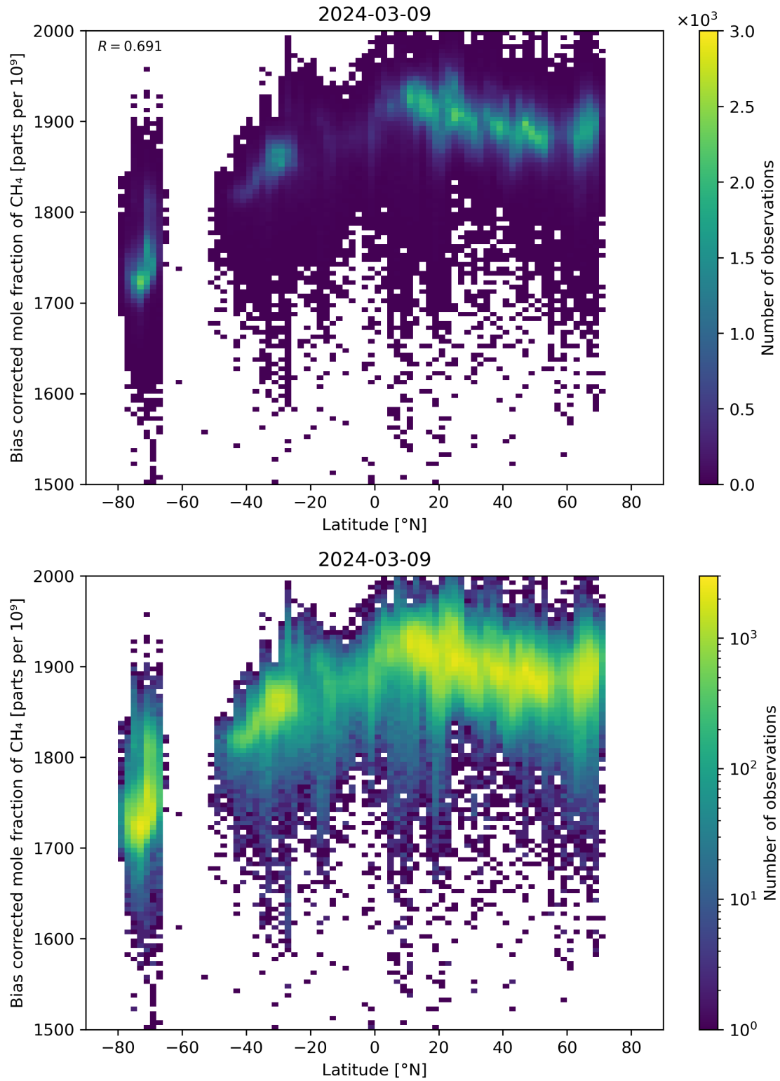
Figure 58: Scatter density plot of “Latitude” against “Bias corrected mole fraction of CH 4 ” for 2024-03-09 to 2024-03-10.
