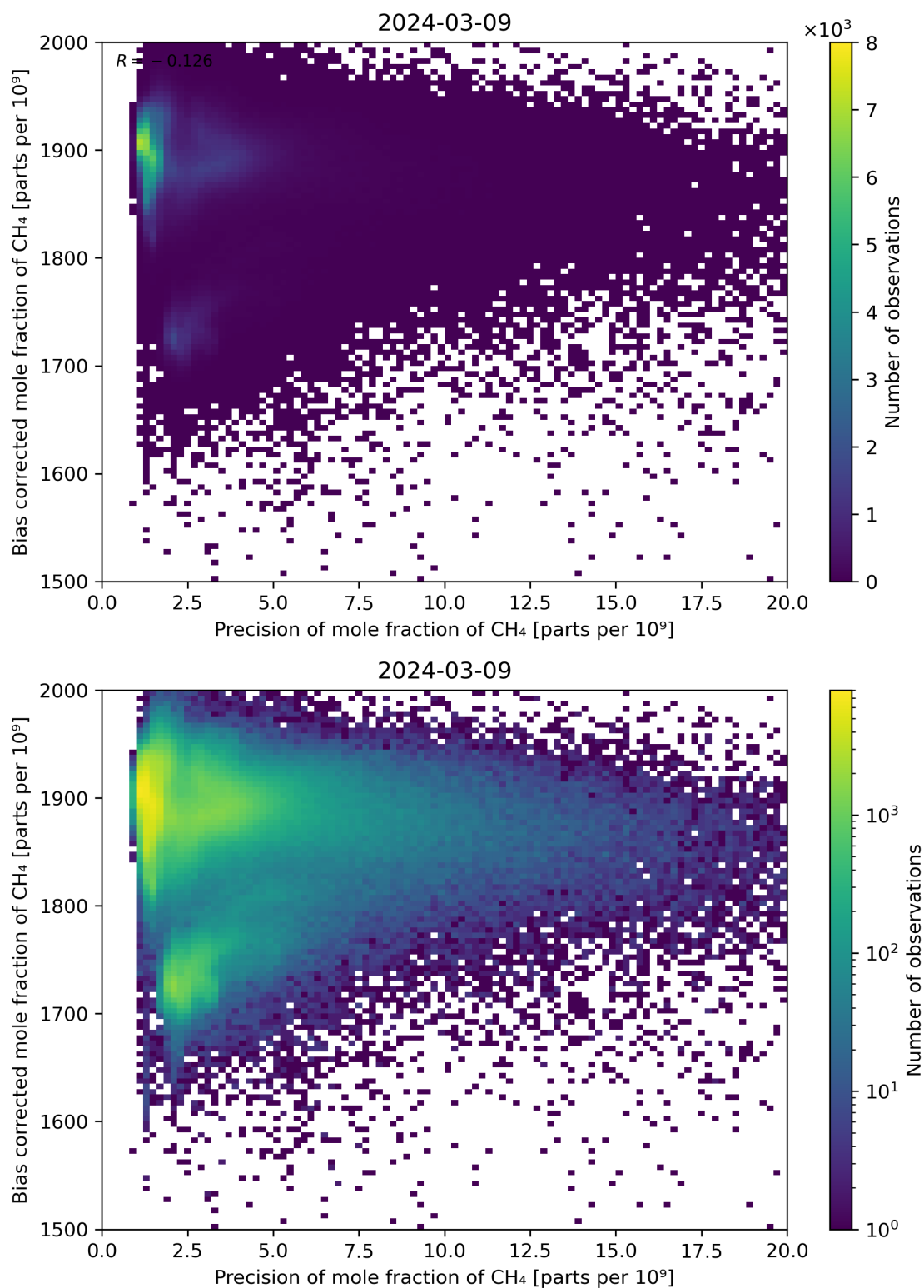
Figure 82: Scatter density plot of “Precision of mole fraction of CH 4 ” against “Bias corrected mole fraction of CH 4 ” for 2024-03-09 to 2024-03-10.
