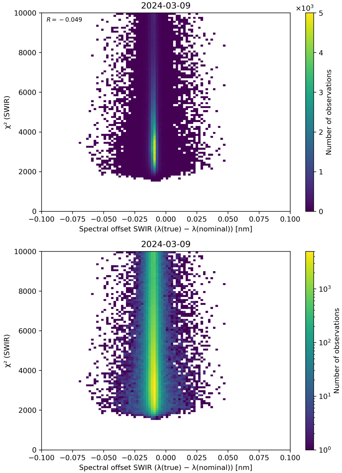
Figure 118: Scatter density plot of “Spectral offset SWIR ( \lambda(\text{true}) - \lambda(\text{nominal}) )” against “ \chi^2 (SWIR)” for 2024-03-09 to 2024-03-10.
