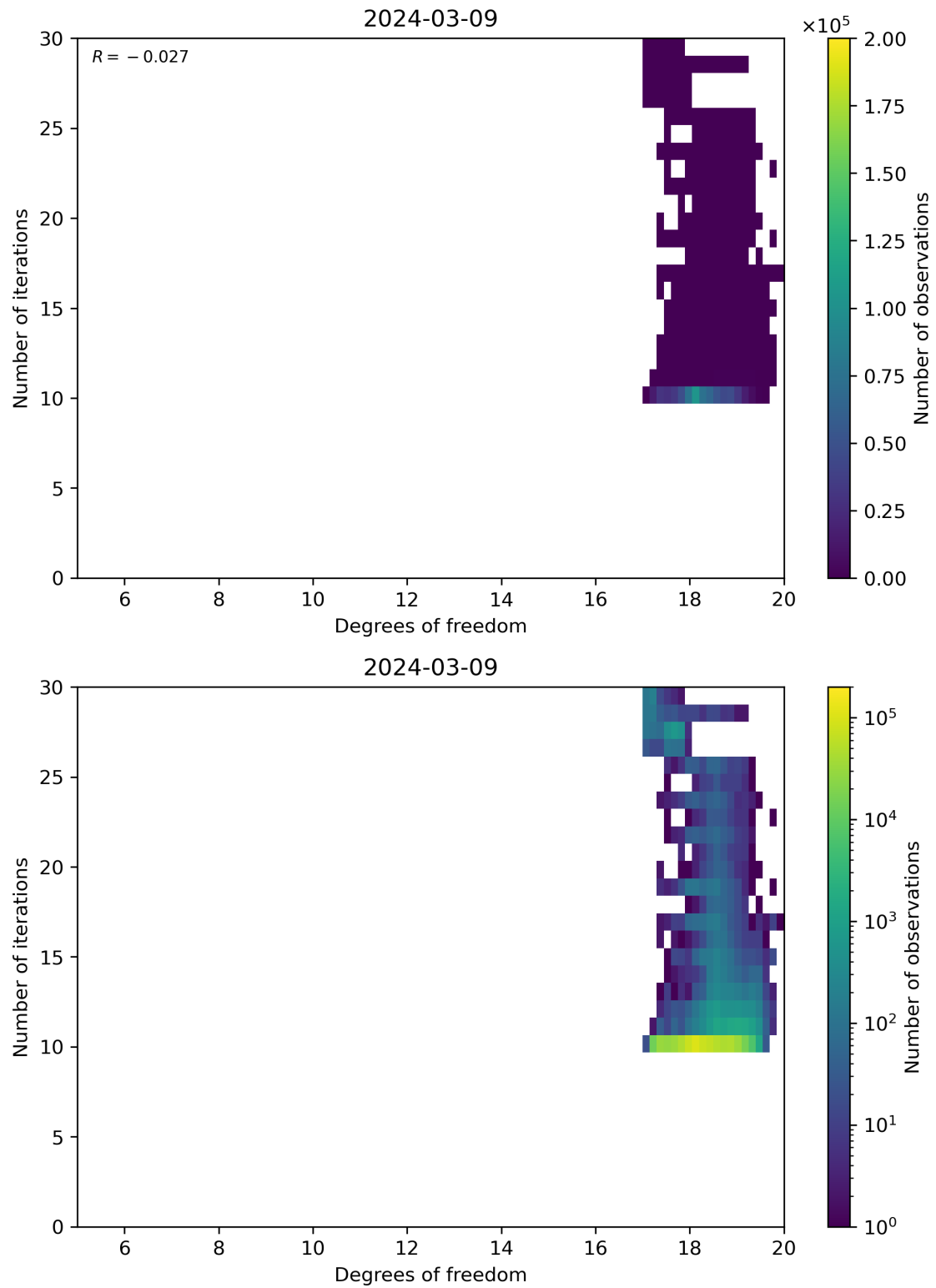
Figure 52: Scatter density plot of “Degrees of freedom” against “Number of iterations” for 2024-03-09 to 2024-03-10.
