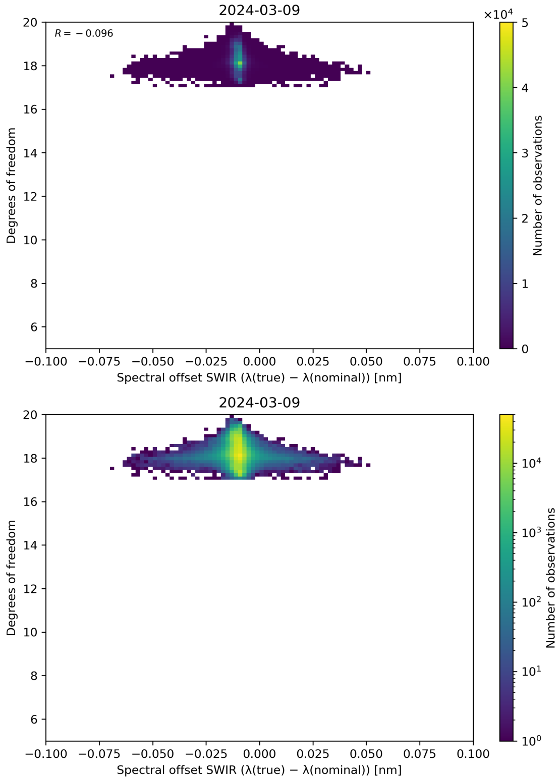
Figure 119: Scatter density plot of “Spectral offset SWIR ( \lambda(\text{true}) - \lambda(\text{nominal}) )” against “Degrees of freedom” for 2024-03-09 to 2024-03-10.
