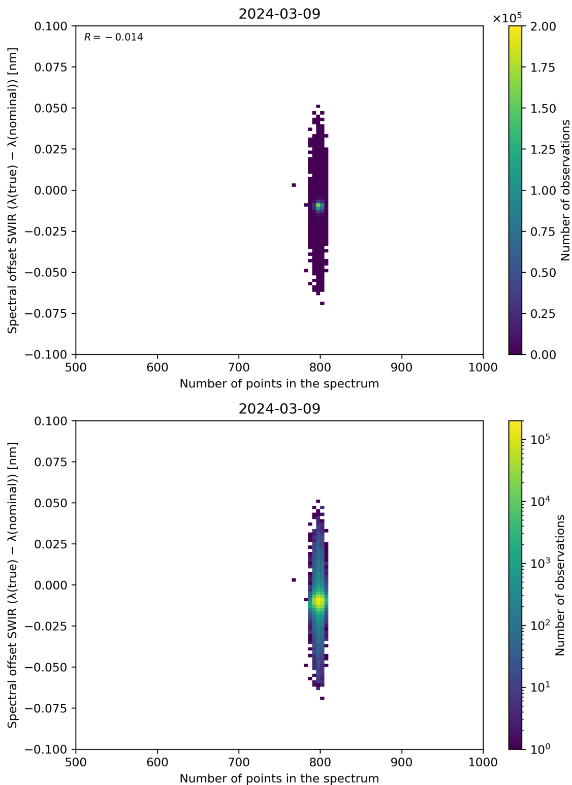
Figure 93: Scatter density plot of “Number of points in the spectrum” against “Spectral offset SWIR ( \lambda(\text{true}) - \lambda(\text{nominal}) )” for 2024-03-09 to 2024-03-10.
