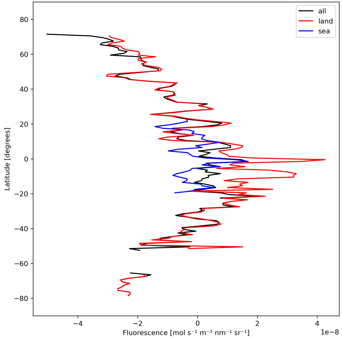
Figure 21: Zonal average of “Fluorescence” for 2024-03-09 to 2024-03-10.
