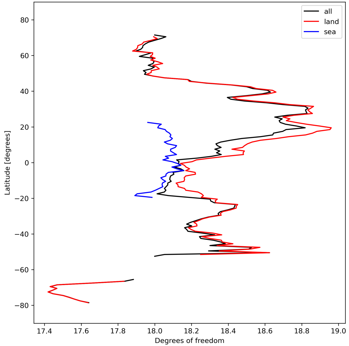
Figure 19: Zonal average of “Degrees of freedom” for 2024-03-09 to 2024-03-10.
