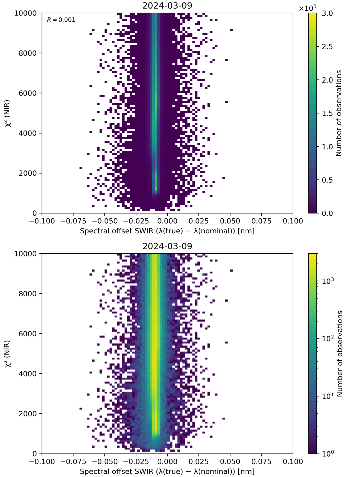
Figure 117: Scatter density plot of “Spectral offset SWIR ( \lambda(\text{true}) - \lambda(\text{nominal}) )” against “ \chi^2 (NIR)” for 2024-03-09 to 2024-03-10.
