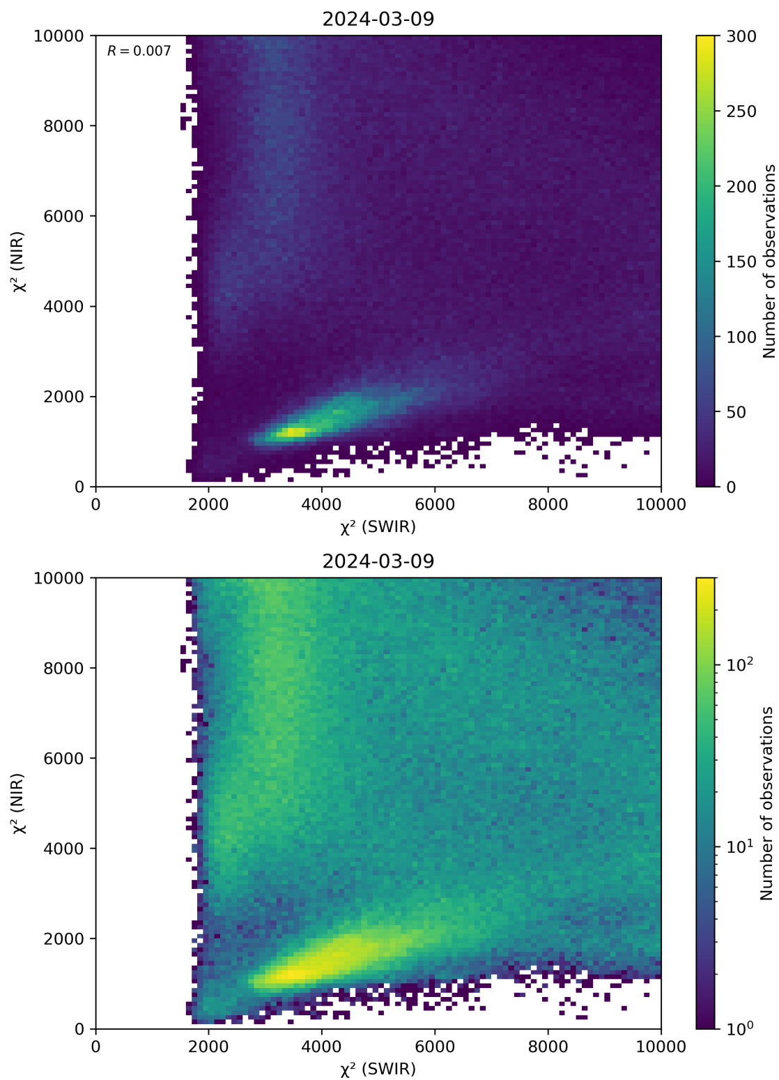
Figure 47: Scatter density plot of “ \chi^2 (SWIR)” against “ \chi^2 (NIR)” for 2024-03-09 to 2024-03-10.
