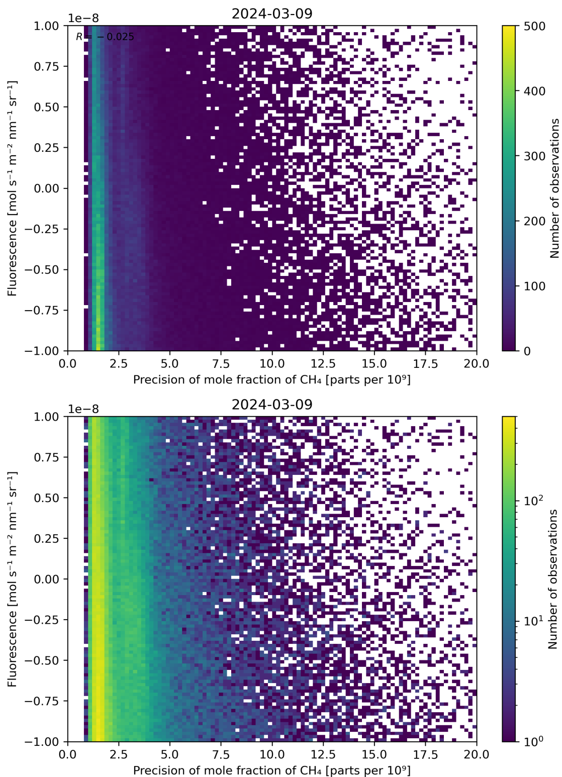
Figure 81: Scatter density plot of “Precision of mole fraction of \text{CH}_4 ” against “Fluorescence” for 2024-03-09 to 2024-03-10.
