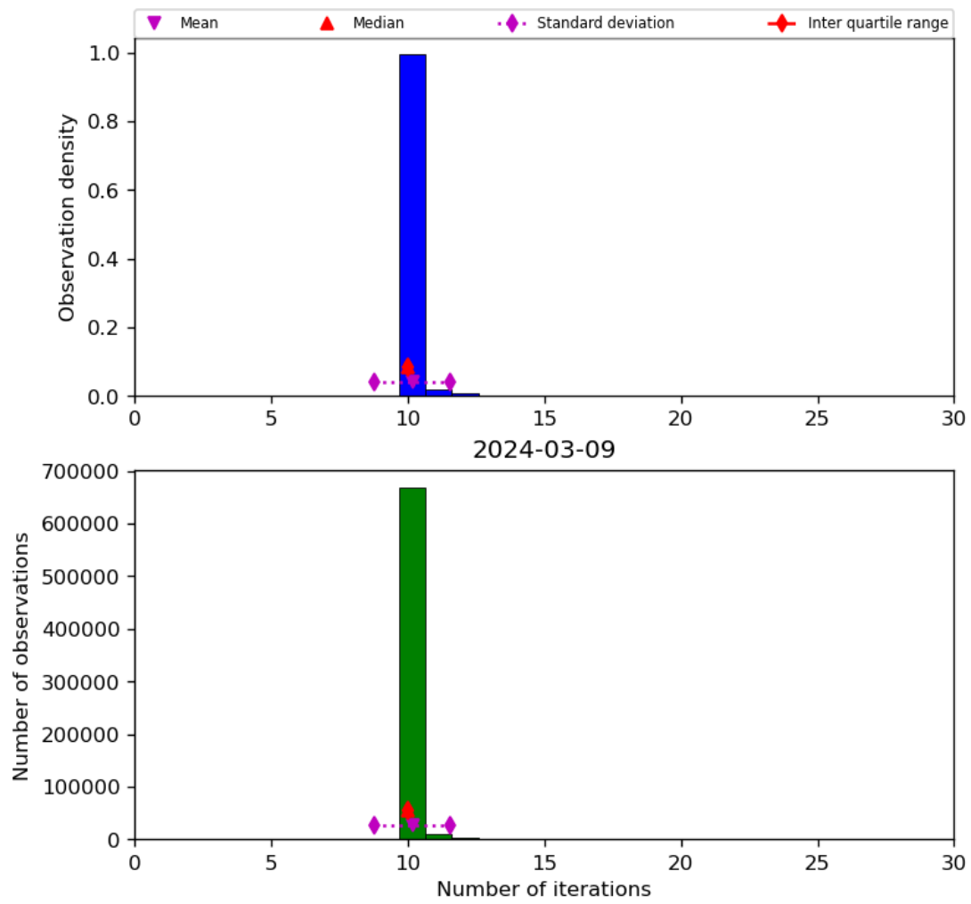
Figure 31: Histogram of “Number of iterations” for 2024-03-09 to 2024-03-10
