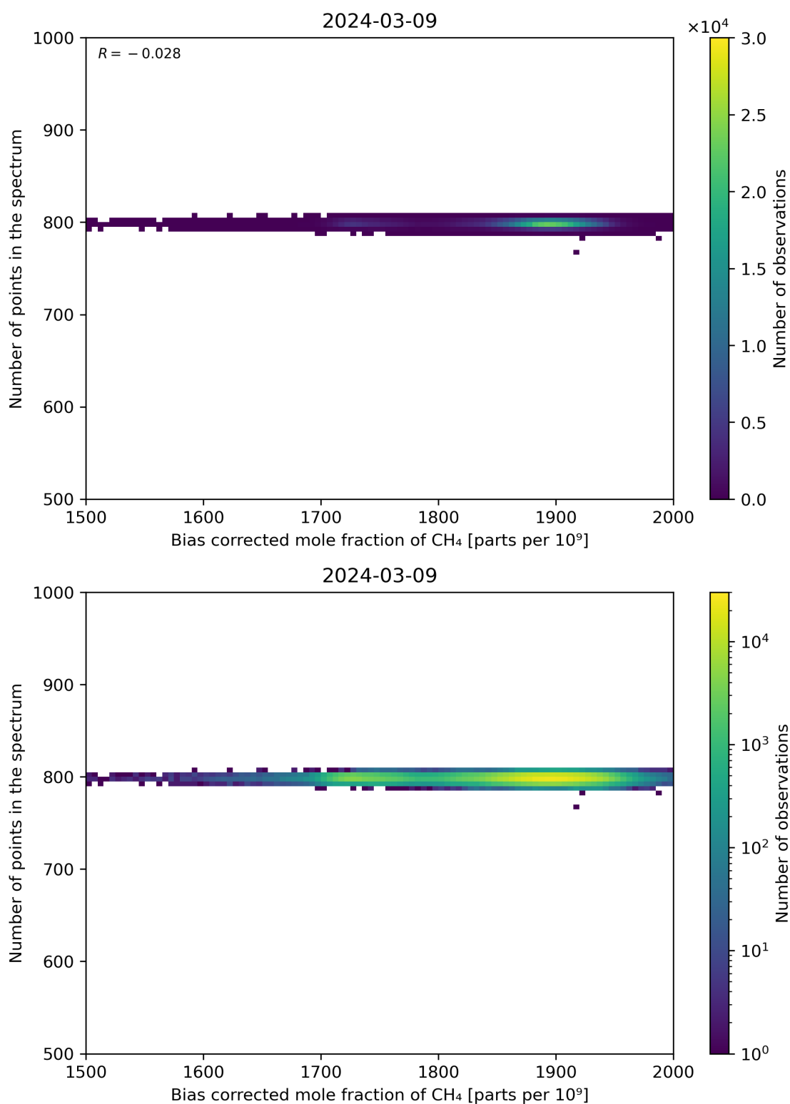
Figure 68: Scatter density plot of “Bias corrected mole fraction of CH 4 ” against “Number of points in the spectrum” for 2024-03-09 to 2024-03-10.
