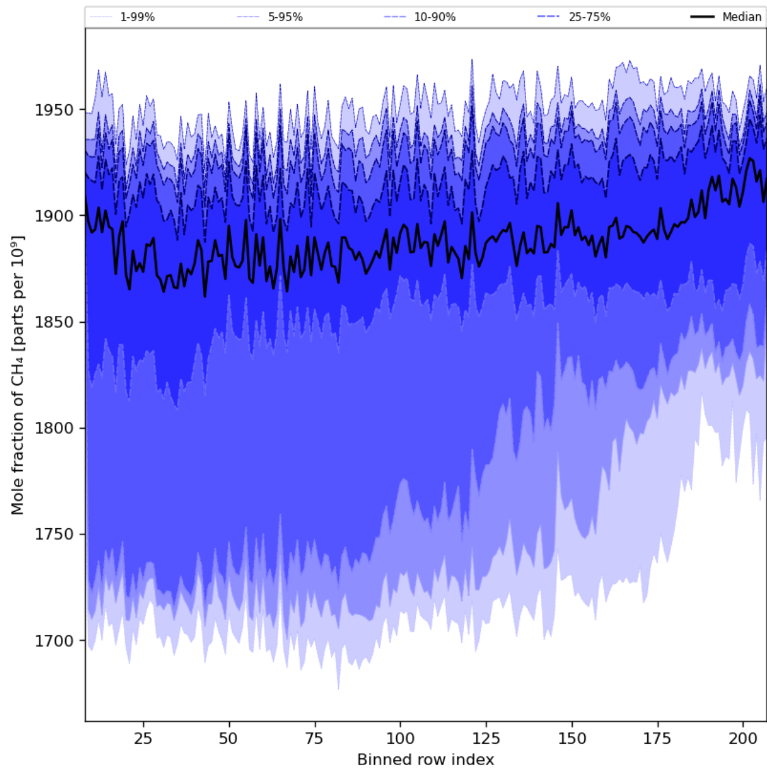
Figure 34: Along track statistics of “Mole fraction of CH 4 ” for 2024-03-09 to 2024-03-10
