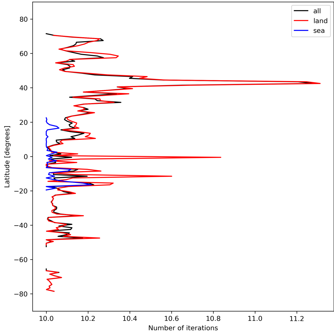
Figure 20: Zonal average of “Number of iterations” for 2024-03-09 to 2024-03-10.
