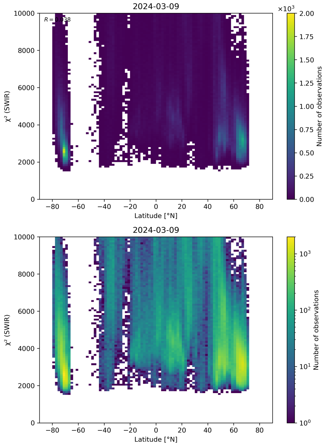
Figure 54: Scatter density plot of “Latitude” against “ \chi^2 (SWIR)” for 2024-03-09 to 2024-03-10.
