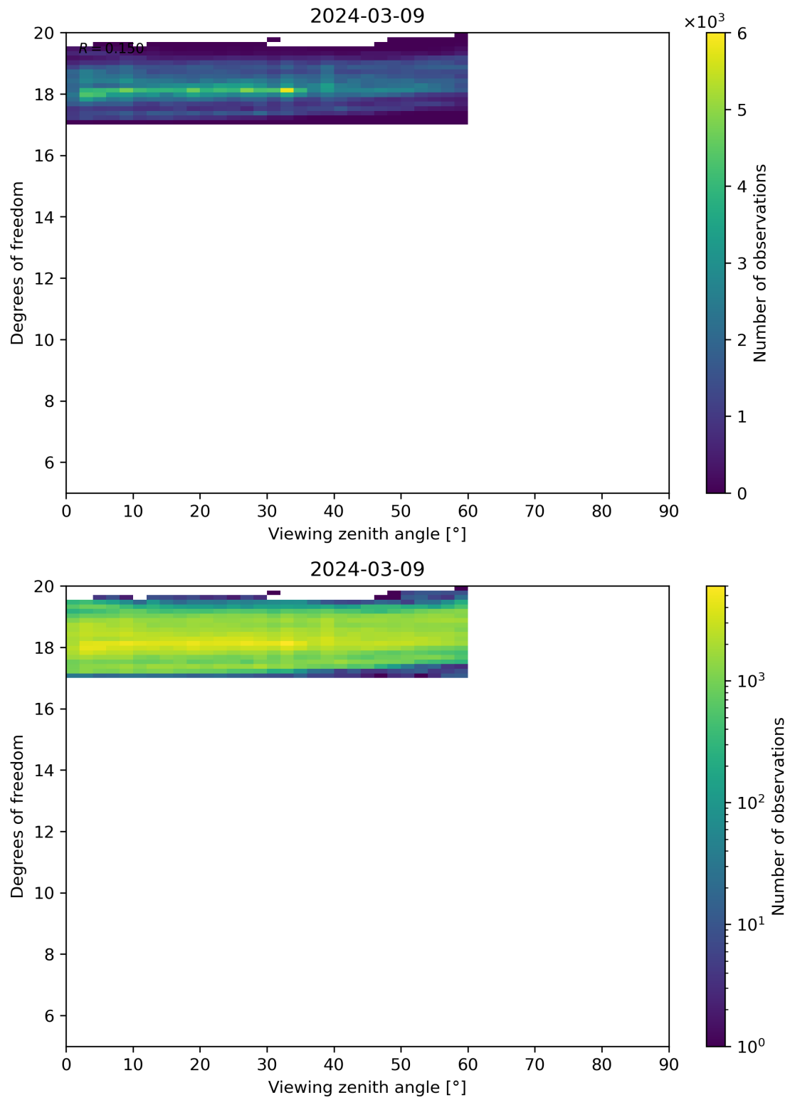
Figure 107: Scatter density plot of “Viewing zenith angle” against “Degrees of freedom” for 2024-03-09 to 2024-03-10.
