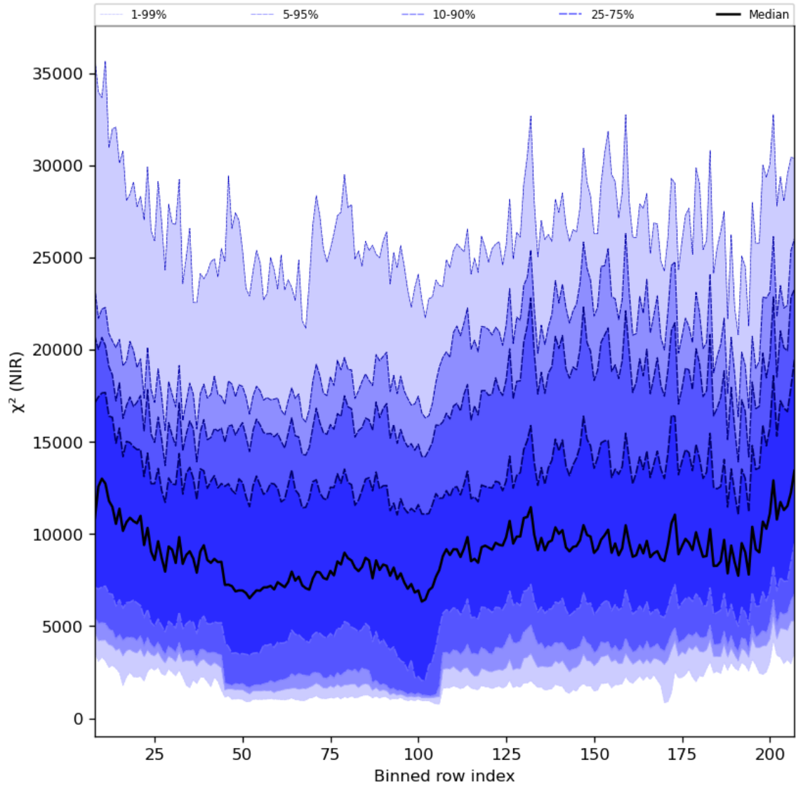
Figure 40: Along track statistics of “ \chi^2 (NIR)” for 2024-03-09 to 2024-03-10
