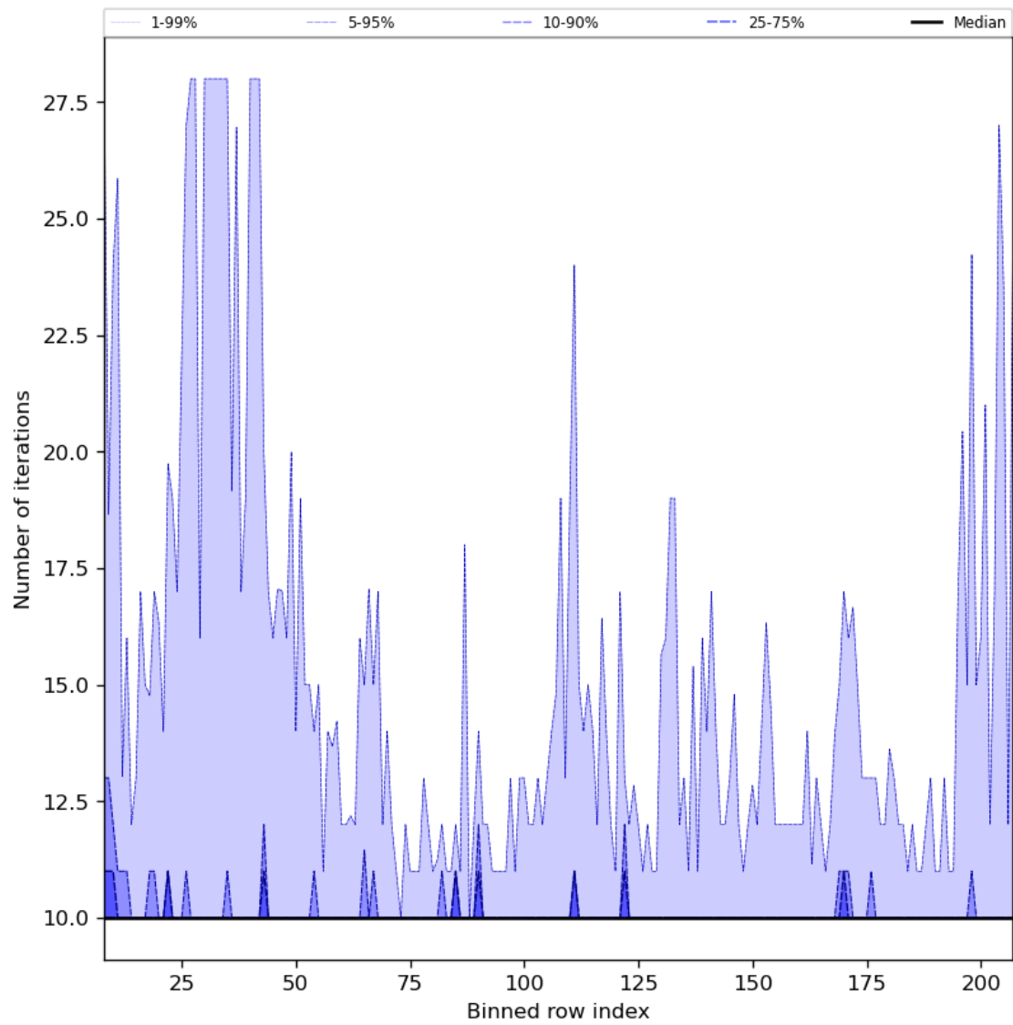
Figure 42: Along track statistics of “Number of iterations” for 2024-03-09 to 2024-03-10
