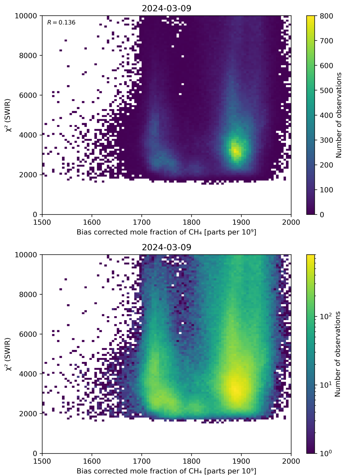
Figure 64: Scatter density plot of “Bias corrected mole fraction of CH 4 ” against “ \chi^2 (SWIR)” for 2024-03-09 to 2024-03-10.
