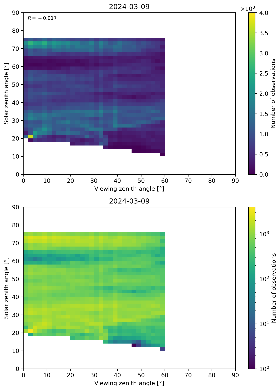
Figure 115: Scatter density plot of “Viewing zenith angle” against “Solar zenith angle” for 2024-03-09 to 2024-03-10.
