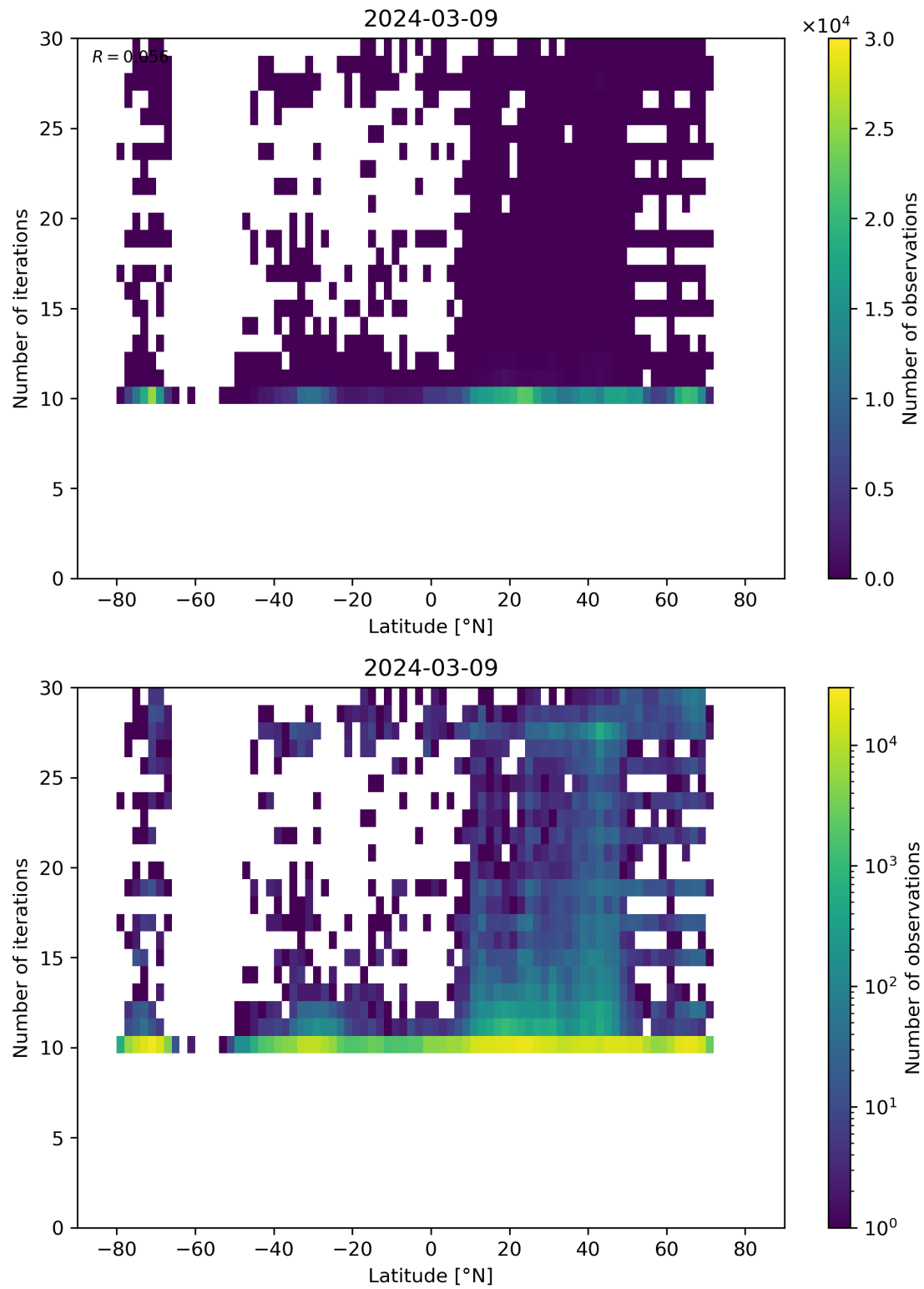
Figure 60: Scatter density plot of “Latitude” against “Number of iterations” for 2024-03-09 to 2024-03-10.
