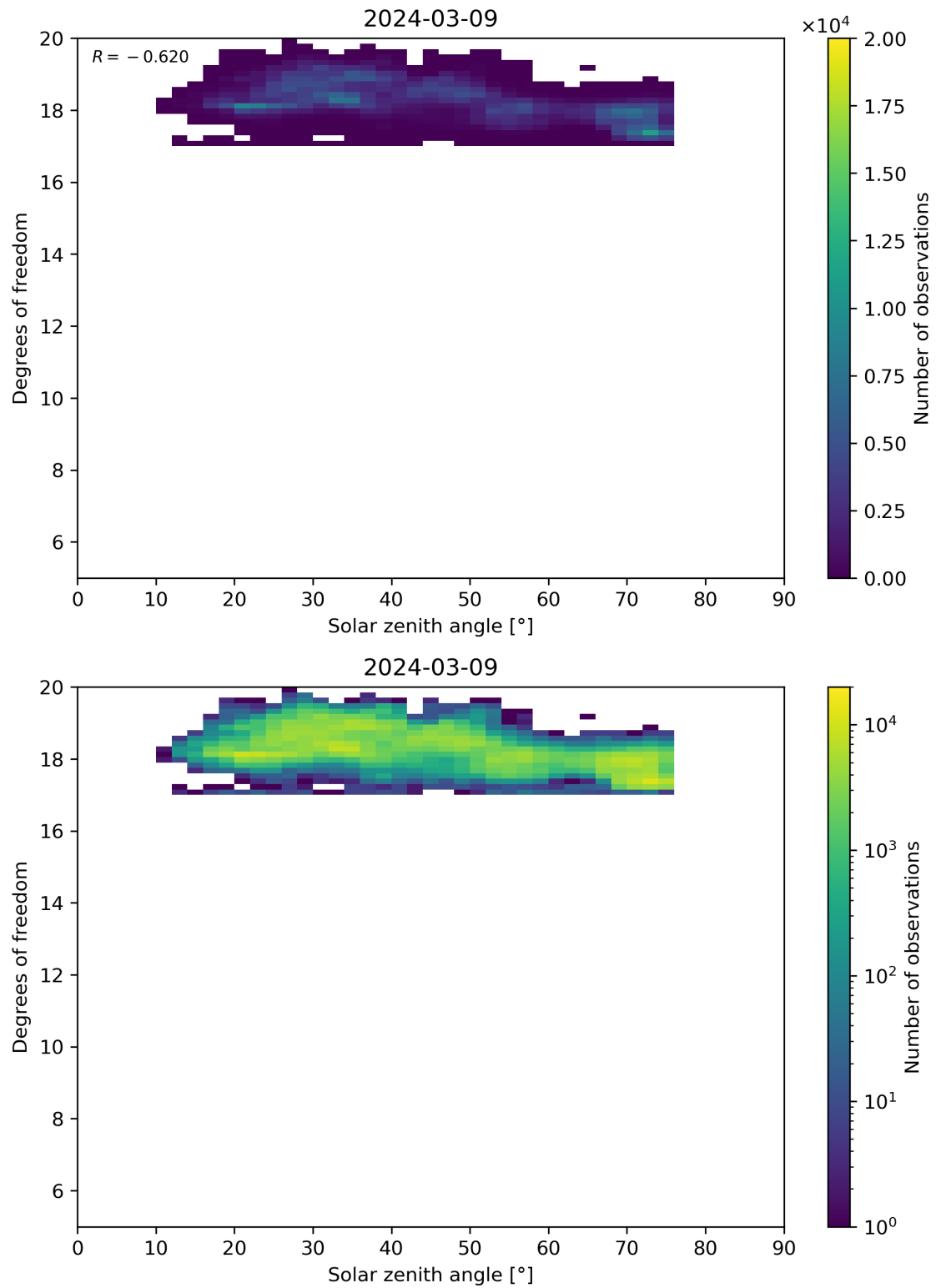
Figure 96: Scatter density plot of “Solar zenith angle” against “Degrees of freedom” for 2024-03-09 to 2024-03-10.
