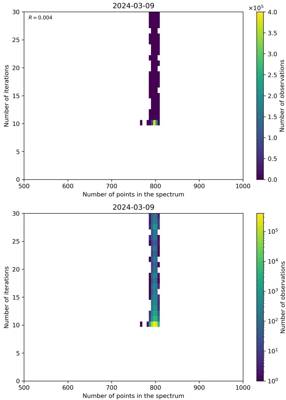
Figure 92: Scatter density plot of “Number of points in the spectrum” against “Number of iterations” for 2024-03-09 to 2024-03-10.
