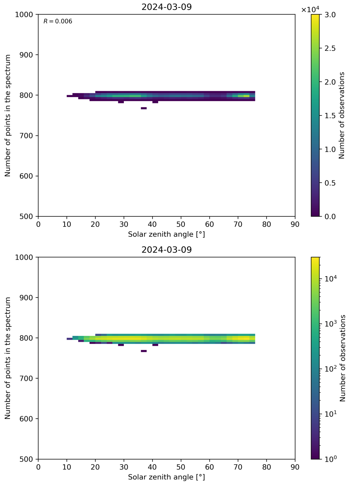
Figure 103: Scatter density plot of “Solar zenith angle” against “Number of points in the spectrum” for 2024-03-09 to 2024-03-10.
