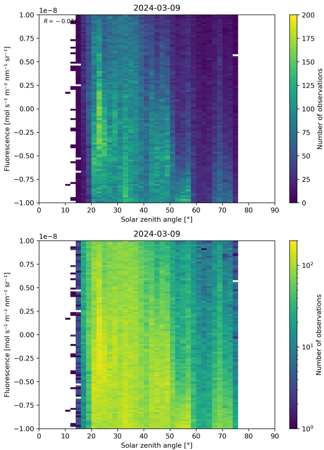
Figure 97: Scatter density plot of “Solar zenith angle” against “Fluorescence” for 2024-03-09 to 2024-03-10.
