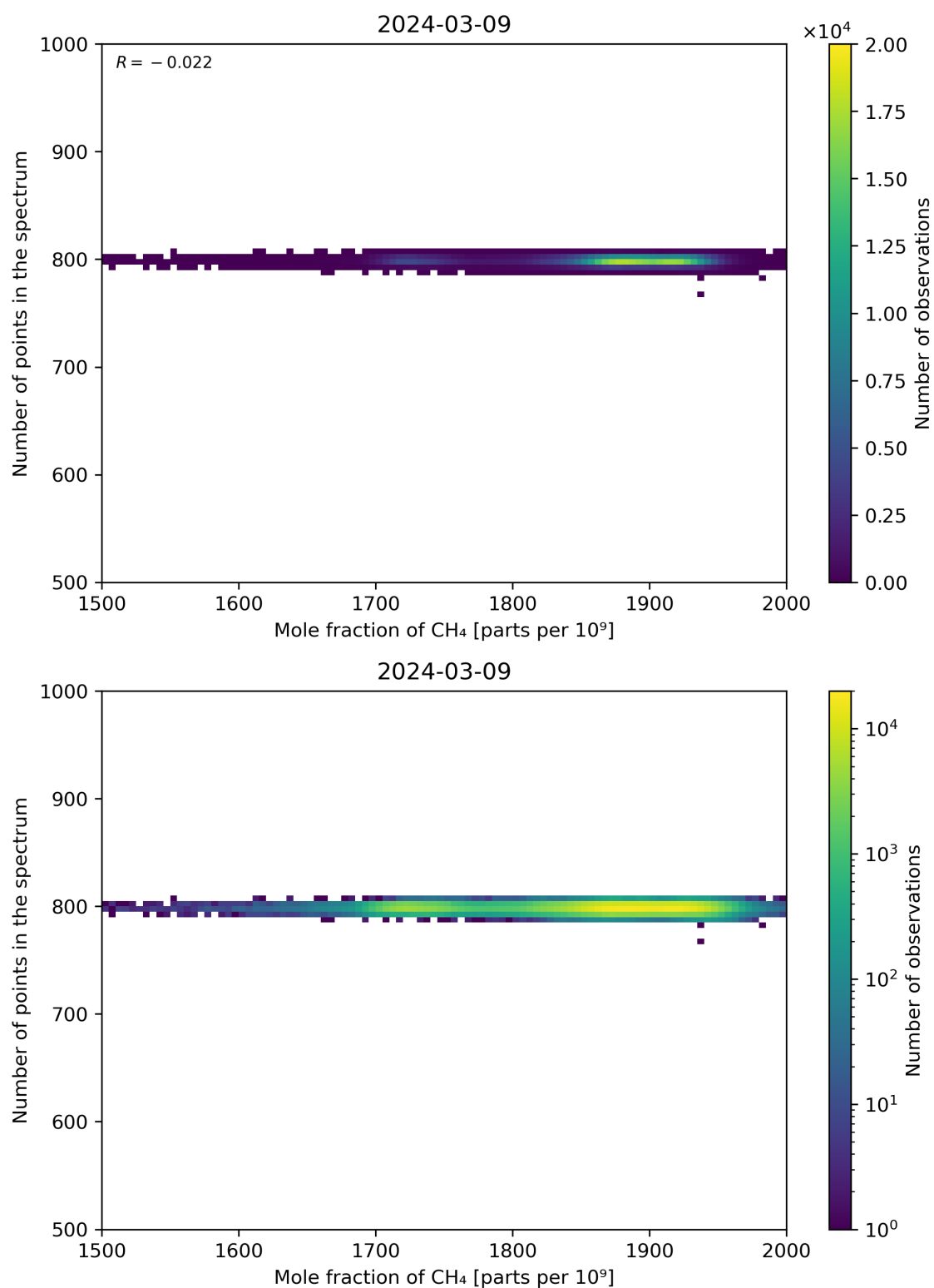
Figure 77: Scatter density plot of “Mole fraction of CH 4 ” against “Number of points in the spectrum” for 2024-03-09 to 2024-03-10.
