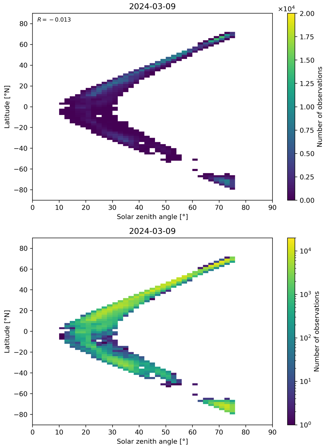
Figure 98: Scatter density plot of “Solar zenith angle” against “Latitude” for 2024-03-09 to 2024-03-10.
