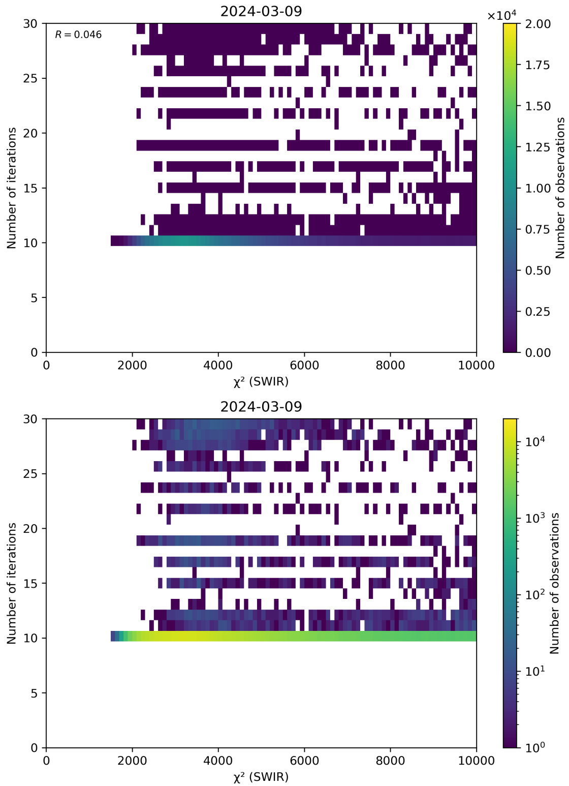
Figure 50: Scatter density plot of “ \chi^2 (SWIR)” against “Number of iterations” for 2024-03-09 to 2024-03-10.
