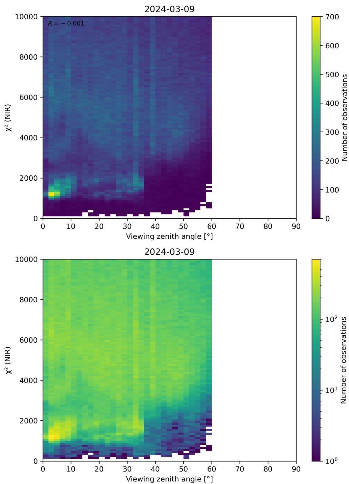
Figure 105: Scatter density plot of “Viewing zenith angle” against “ \chi^2 (NIR)” for 2024-03-09 to 2024-03-10.
