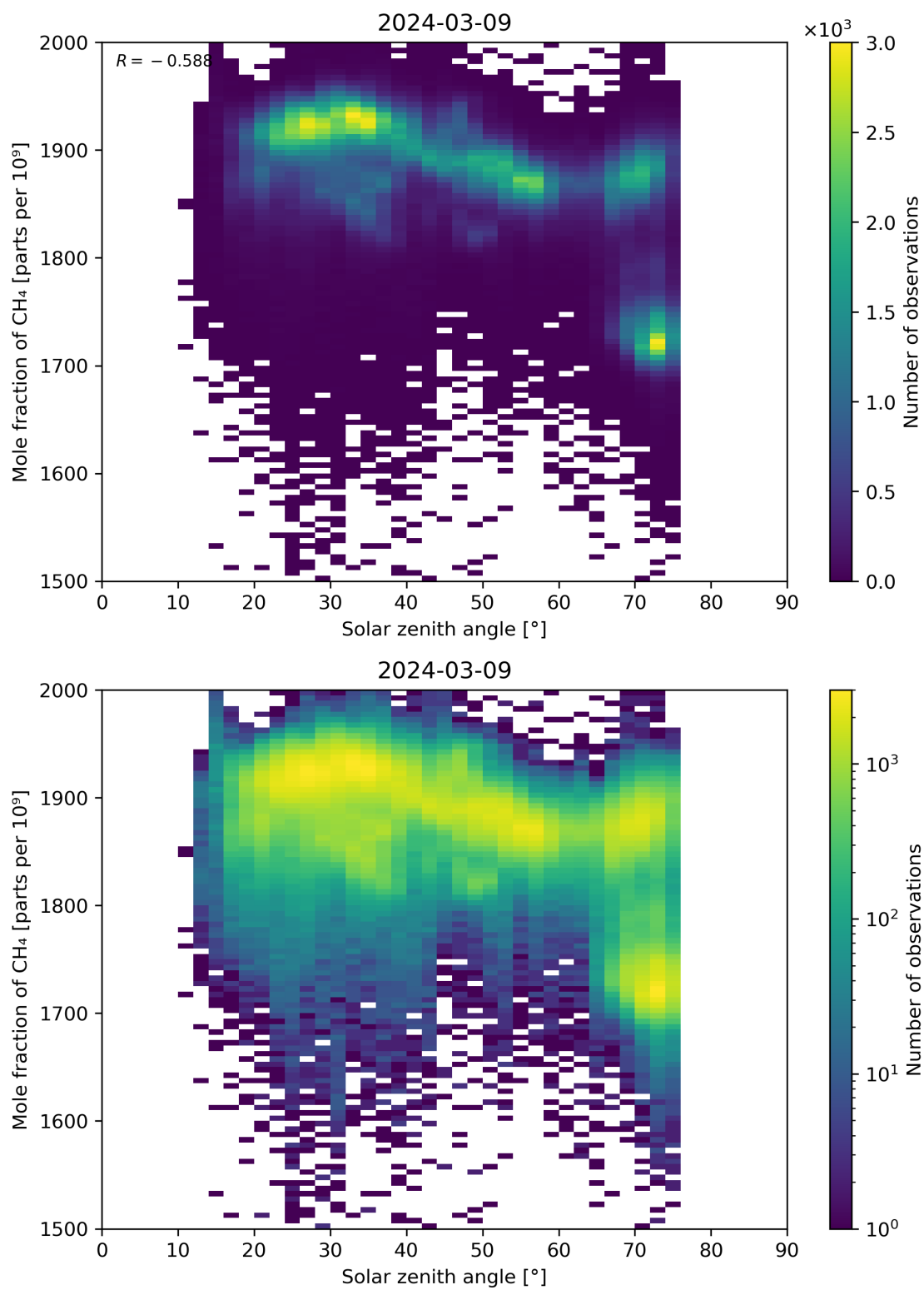
Figure 99: Scatter density plot of “Solar zenith angle” against “Mole fraction of \text{CH}_4 ” for 2024-03-09 to 2024-03-10.
