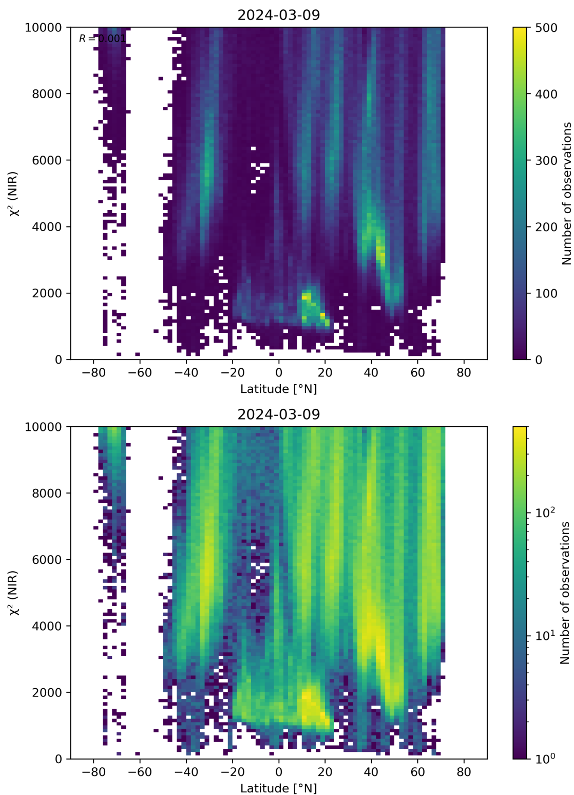
Figure 53: Scatter density plot of “Latitude” against “ \chi^2 (NIR)” for 2024-03-09 to 2024-03-10.
