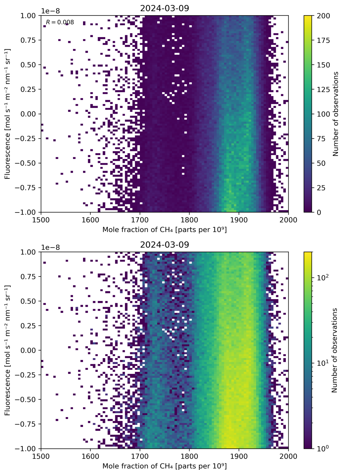
Figure 73: Scatter density plot of “Mole fraction of \text{CH}_4 ” against “Fluorescence” for 2024-03-09 to 2024-03-10.
