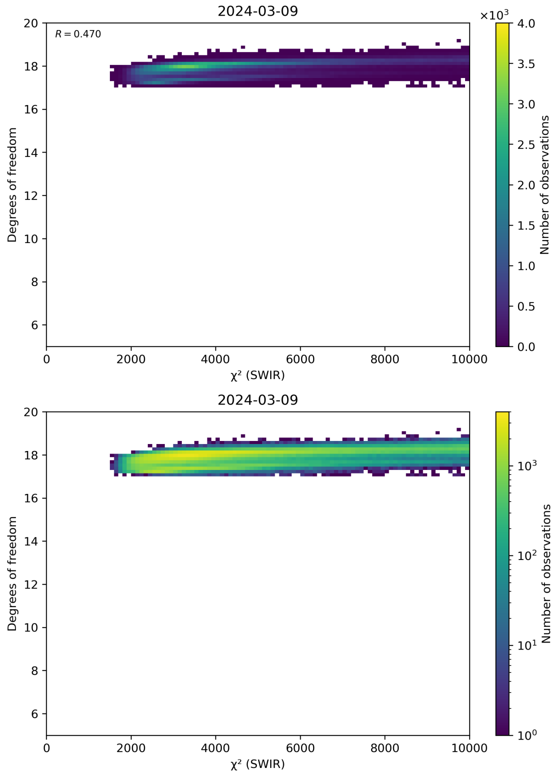
Figure 48: Scatter density plot of “ \chi^2 (SWIR)” against “Degrees of freedom” for 2024-03-09 to 2024-03-10.
