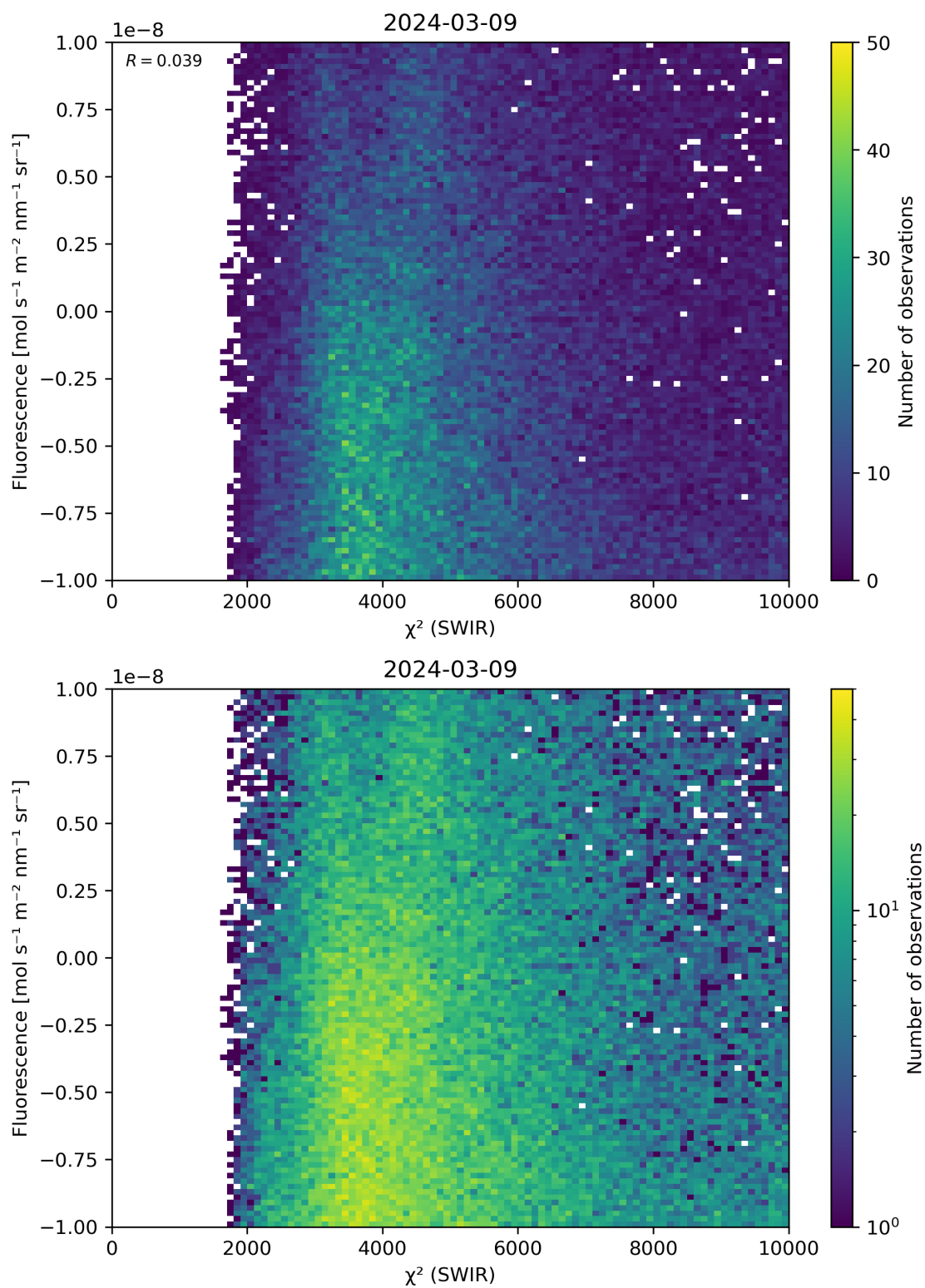
Figure 49: Scatter density plot of “ \chi^2 (SWIR)” against “Fluorescence” for 2024-03-09 to 2024-03-10.
