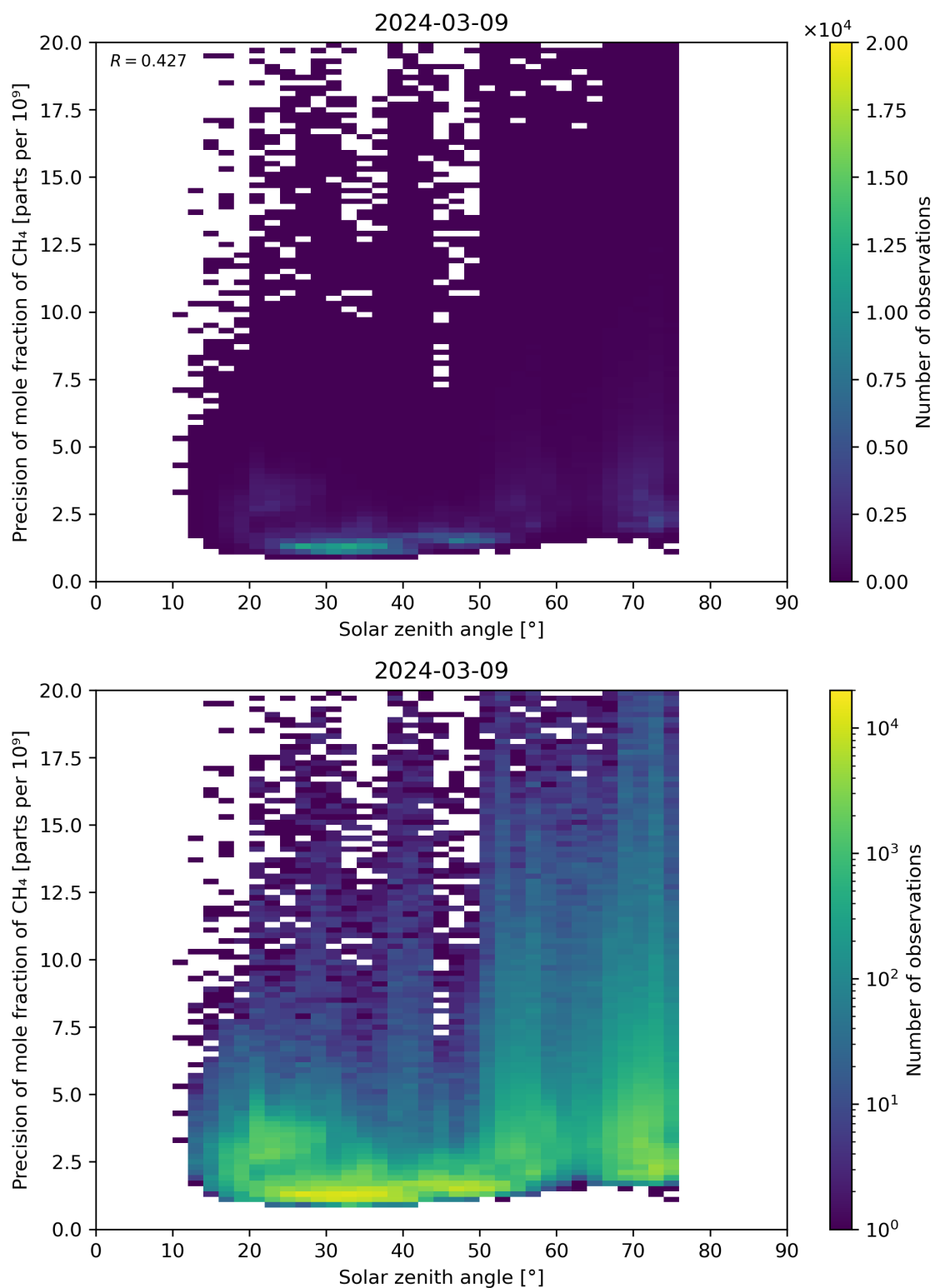
Figure 101: Scatter density plot of “Solar zenith angle” against “Precision of mole fraction of CH 4 ” for 2024-03-09 to 2024-03-10.
