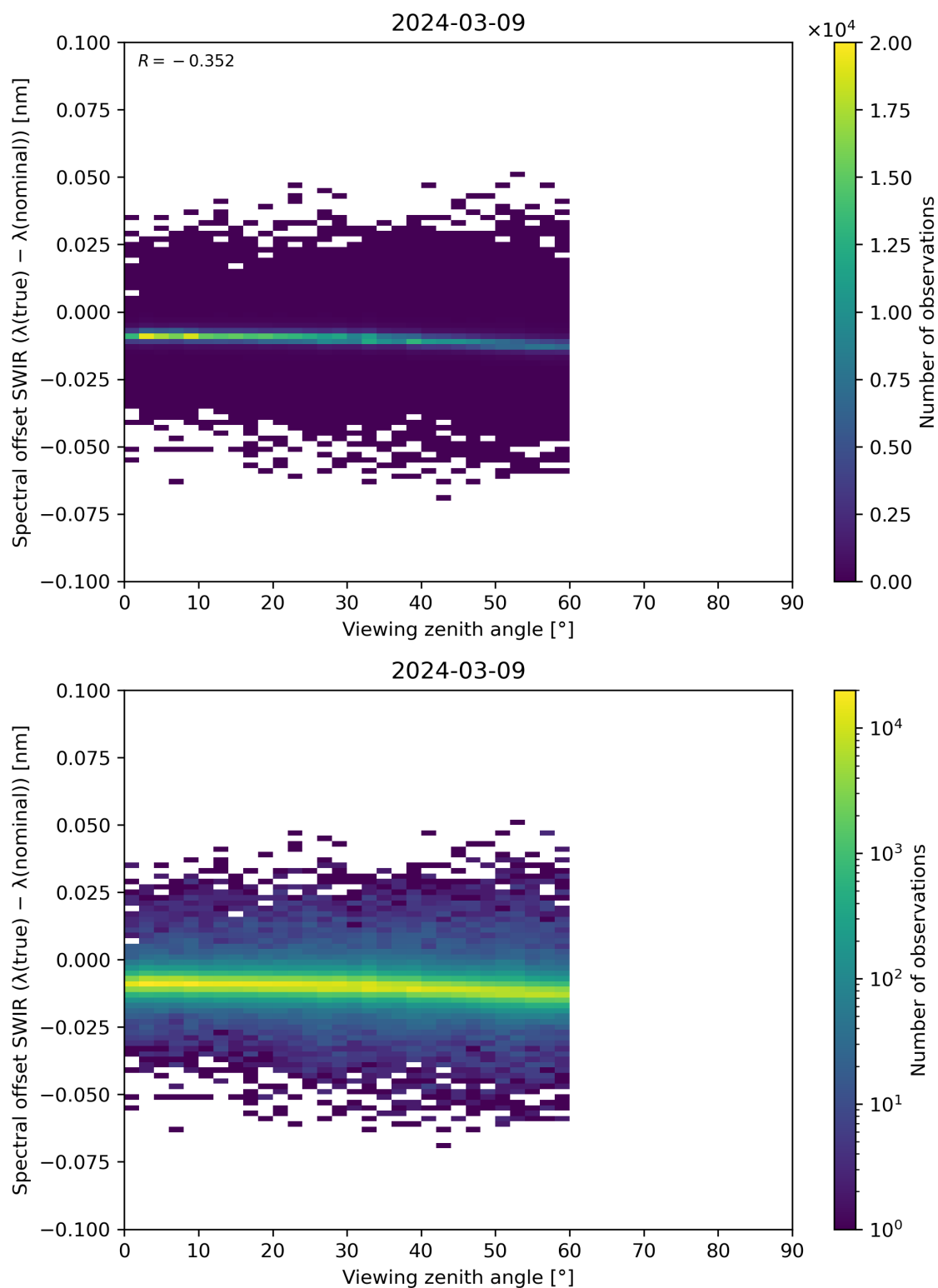
Figure 116: Scatter density plot of “Viewing zenith angle” against “Spectral offset SWIR ( \lambda(\text{true}) - \lambda(\text{nominal}) )” for 2024-03-09 to 2024-03-10.
