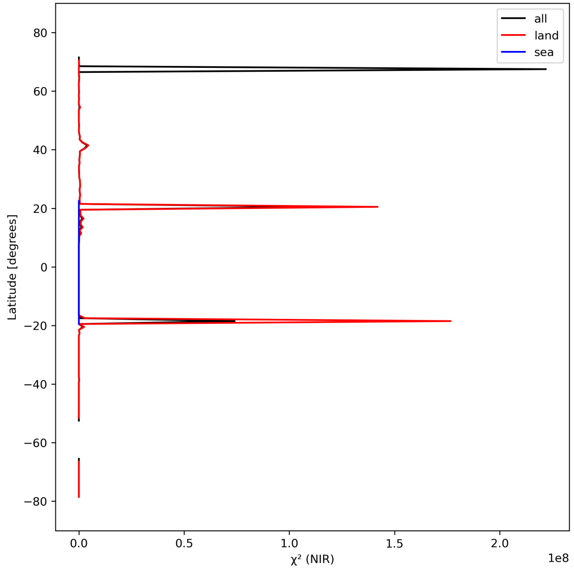
Figure 18: Zonal average of “ \chi^2 (NIR)” for 2024-03-09 to 2024-03-10.
