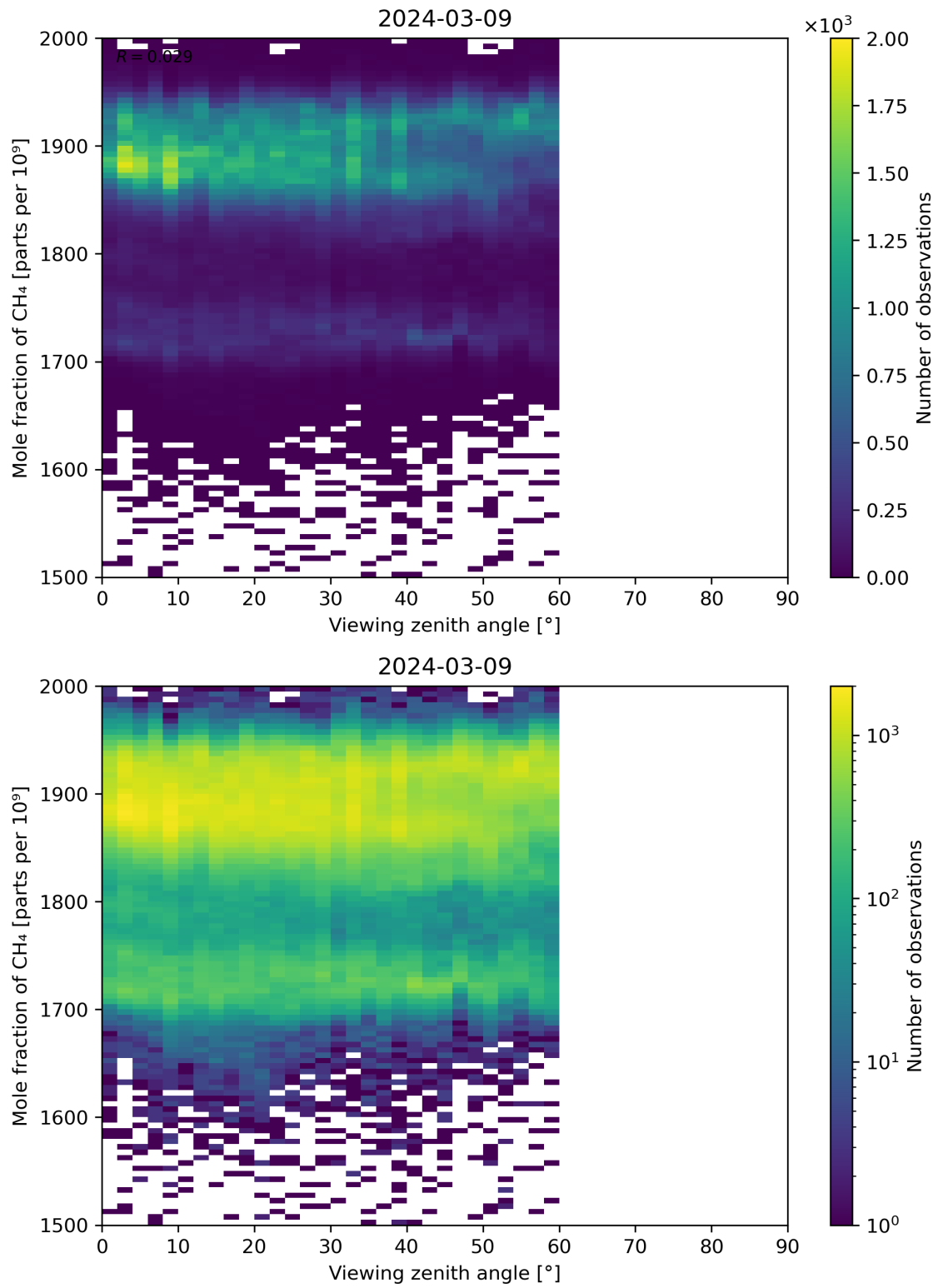
Figure 110: Scatter density plot of “Viewing zenith angle” against “Mole fraction of CH 4 ” for 2024-03-09 to 2024-03-10.
