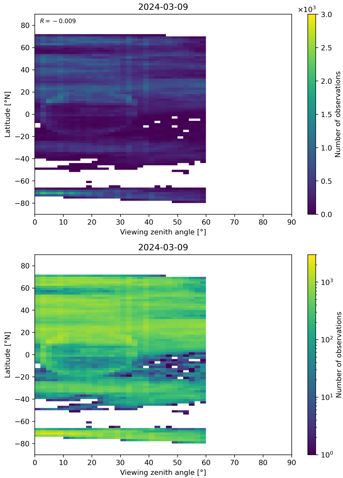
Figure 109: Scatter density plot of “Viewing zenith angle” against “Latitude” for 2024-03-09 to 2024-03-10.
