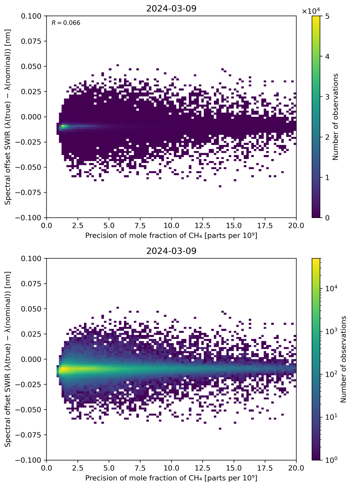
Figure 85: Scatter density plot of “Precision of mole fraction of \text{CH}_4 ” against “Spectral offset SWIR ( \lambda(\text{true}) - \lambda(\text{nominal}) )” for 2024-03-09 to 2024-03-10.
