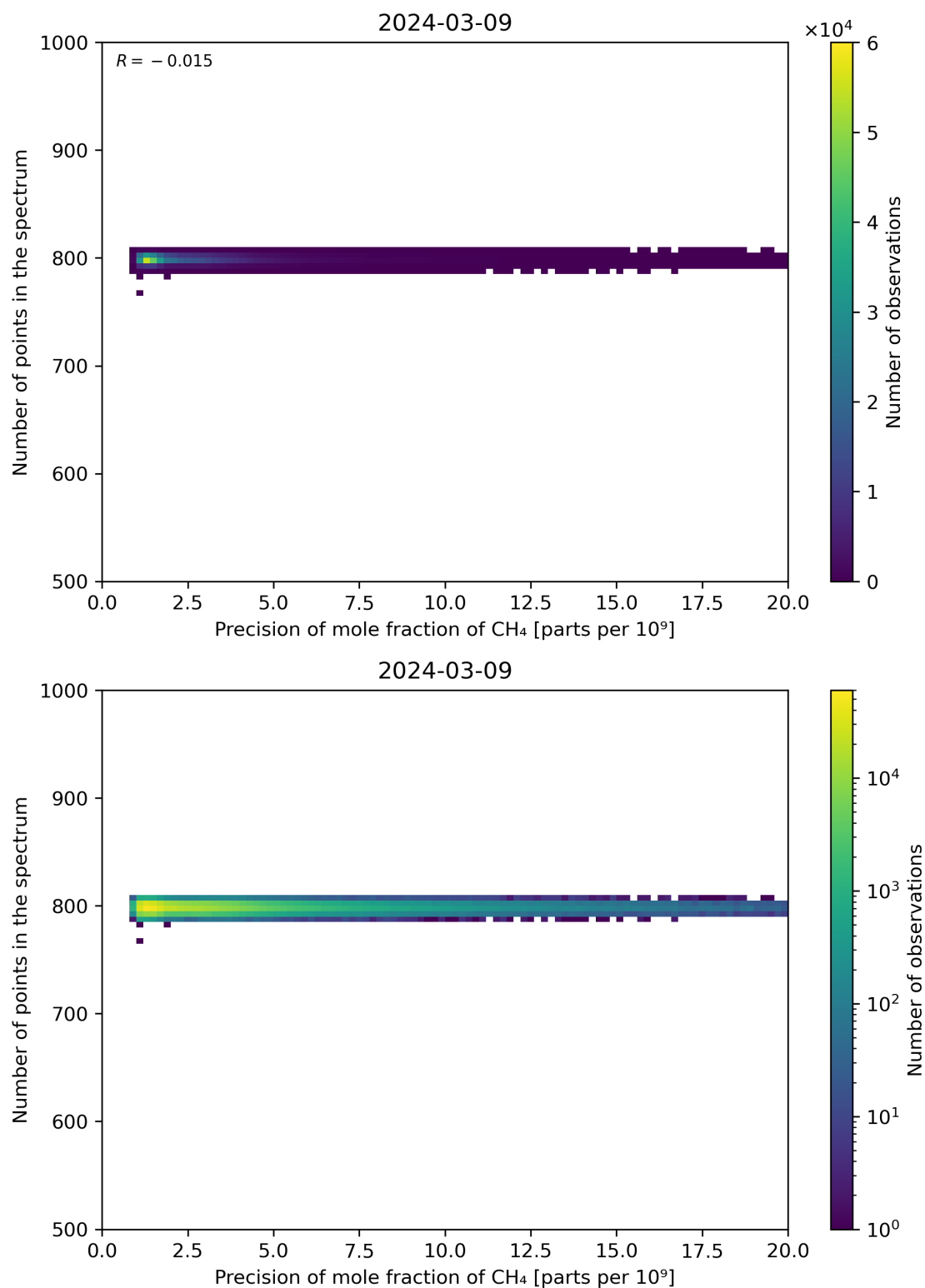
Figure 84: Scatter density plot of “Precision of mole fraction of CH 4 ” against “Number of points in the spectrum” for 2024-03-09 to 2024-03-10.
