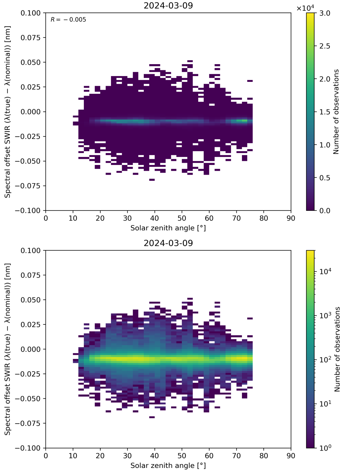
Figure 104: Scatter density plot of “Solar zenith angle” against “Spectral offset SWIR ( \lambda(\text{true}) - \lambda(\text{nominal}) )” for 2024-03-09 to 2024-03-10.
