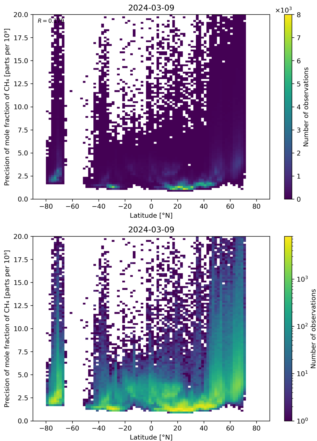
Figure 59: Scatter density plot of “Latitude” against “Precision of mole fraction of CH 4 ” for 2024-03-09 to 2024-03-10.
