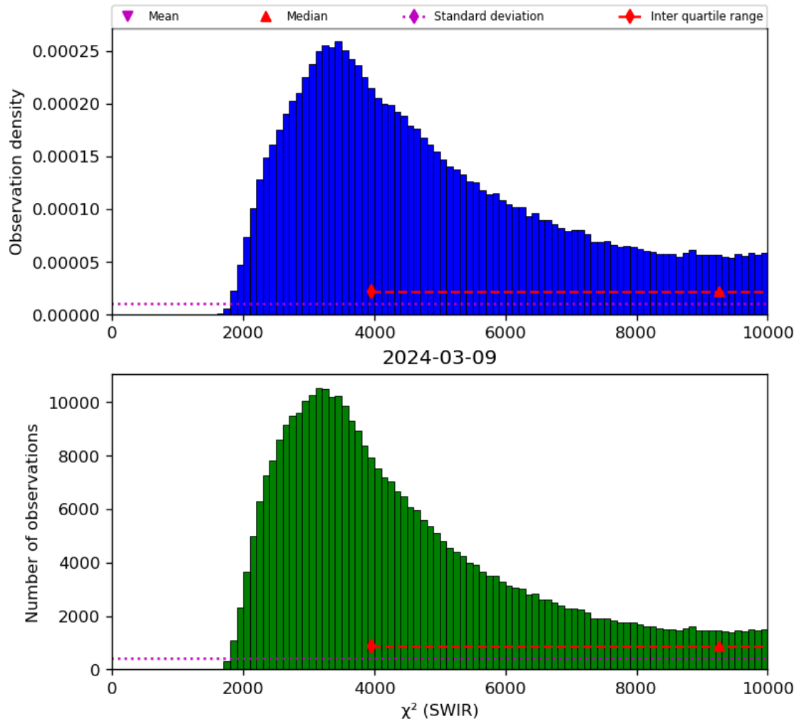
Figure 28: Histogram of “ \chi^2 (SWIR)” for 2024-03-09 to 2024-03-10
