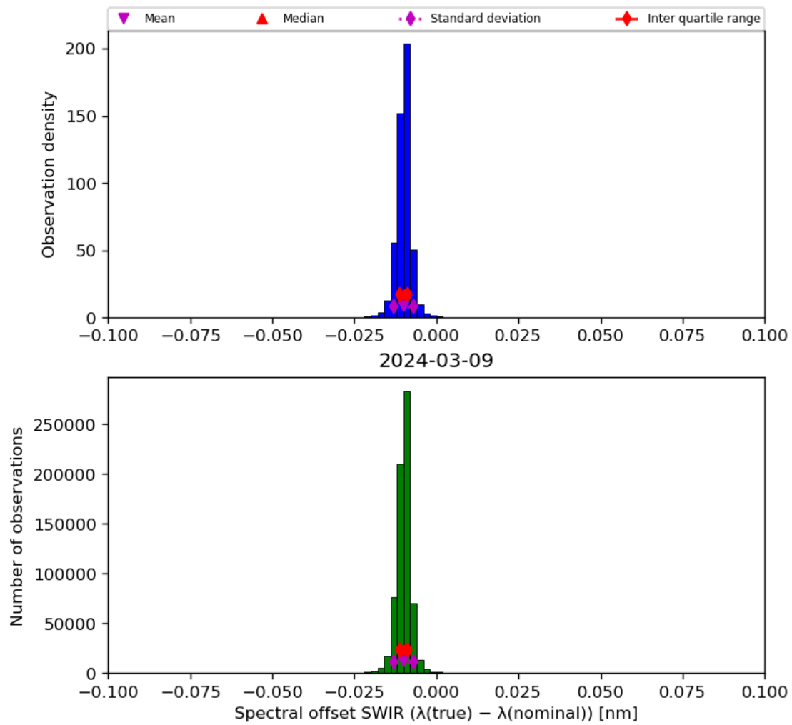
Figure 27: Histogram of “Spectral offset SWIR ( \lambda(\text{true}) - \lambda(\text{nominal}) )” for 2024-03-09 to 2024-03-10
