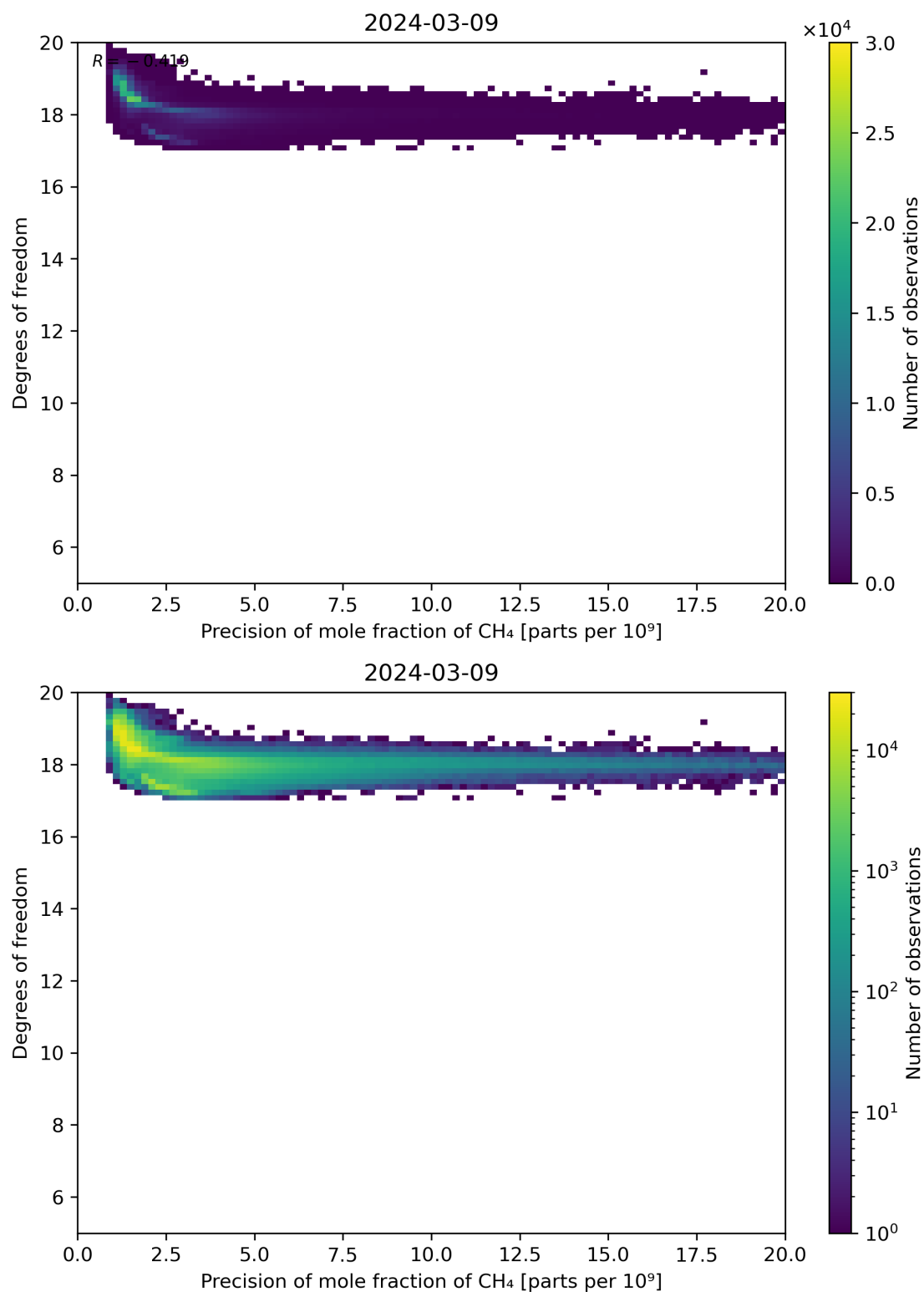
Figure 80: Scatter density plot of “Precision of mole fraction of CH 4 ” against “Degrees of freedom” for 2024-03-09 to 2024-03-10.
