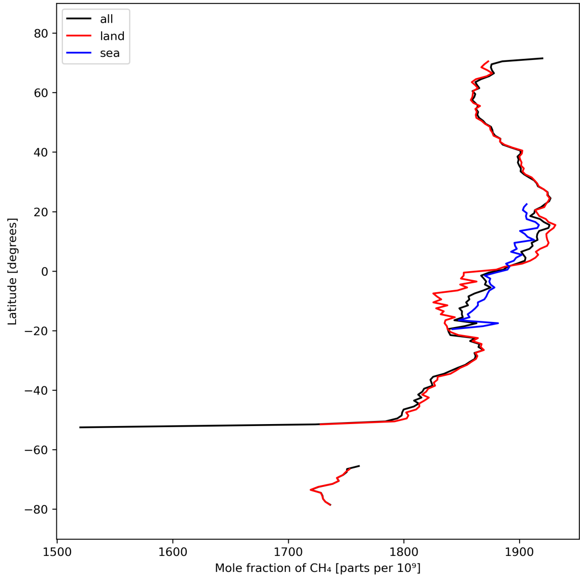
Figure 12: Zonal average of “Mole fraction of \text{CH}_4 ” for 2024-03-09 to 2024-03-10.
