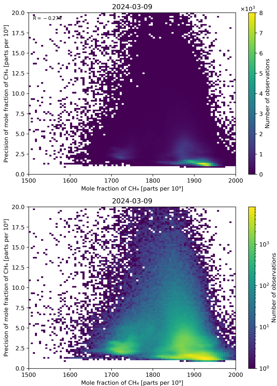
Figure 75: Scatter density plot of “Mole fraction of CH 4 ” against “Precision of mole fraction of CH 4 ” for 2024-03-09 to 2024-03-10.
