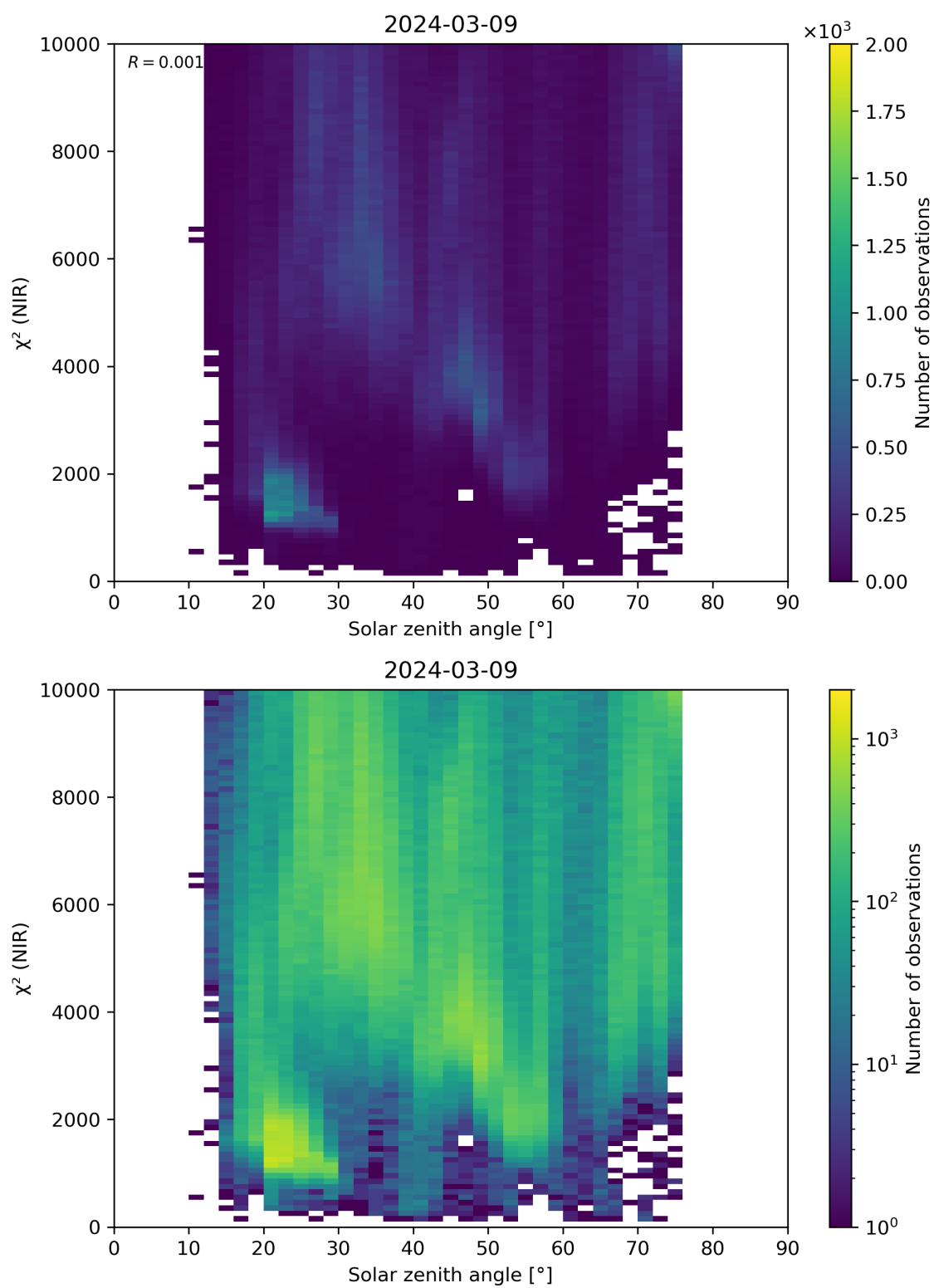
Figure 94: Scatter density plot of “Solar zenith angle” against “ \chi^2 (NIR)” for 2024-03-09 to 2024-03-10.
