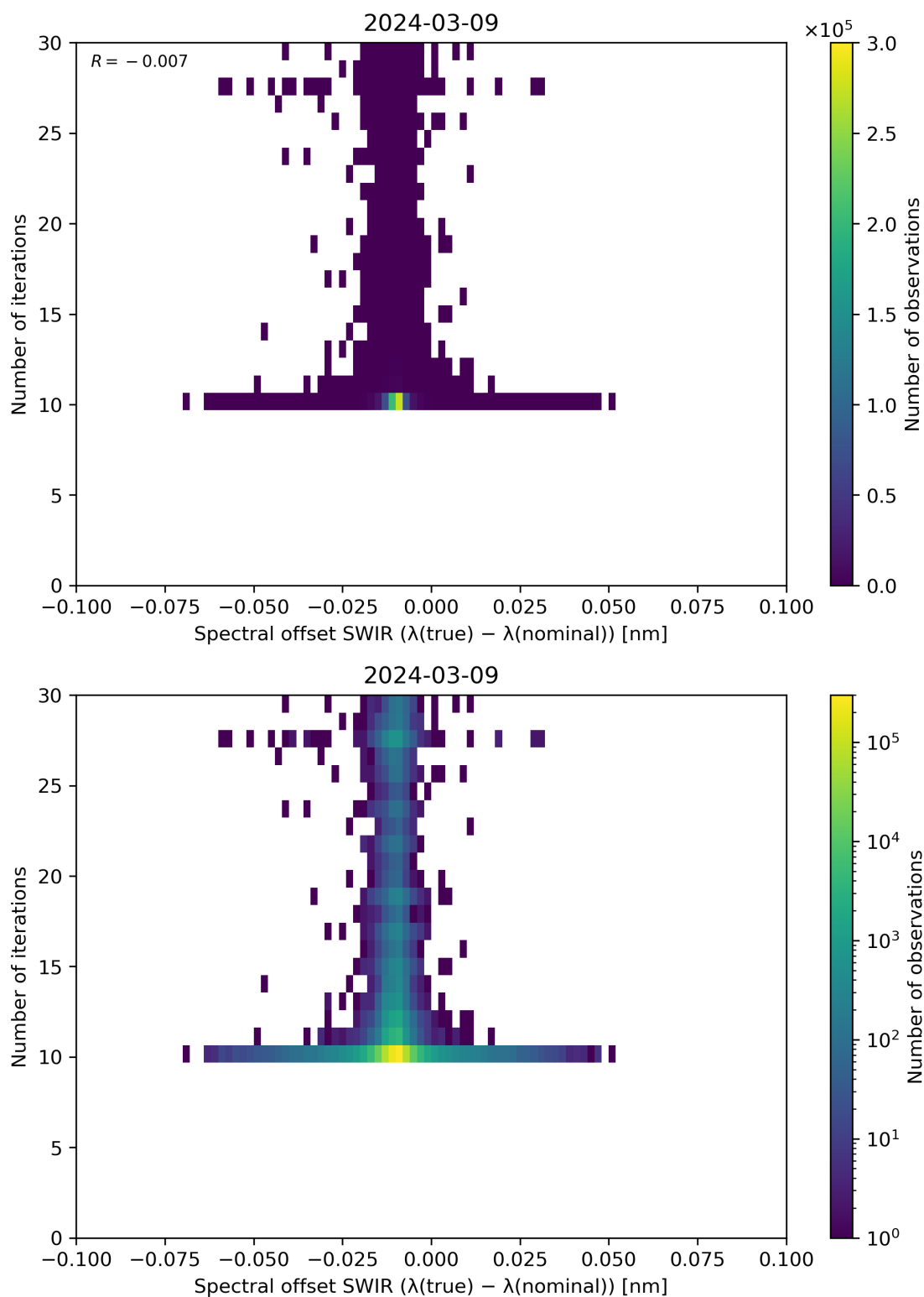
Figure 121: Scatter density plot of “Spectral offset SWIR ( \lambda(\text{true}) - \lambda(\text{nominal}) )” against “Number of iterations” for 2024-03-09 to 2024-03-10.
