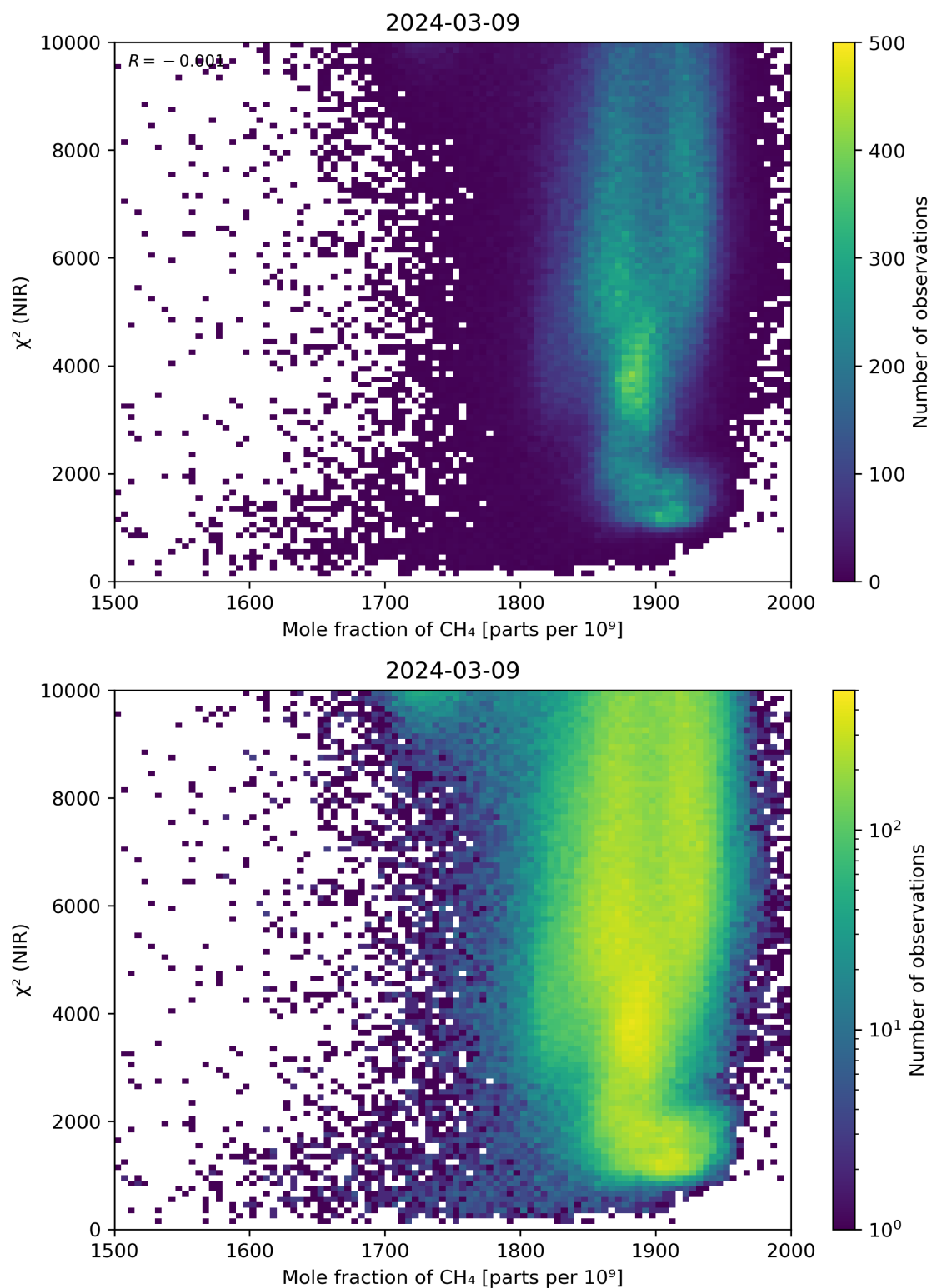
Figure 70: Scatter density plot of “Mole fraction of CH 4 ” against “ \chi^2 (NIR)” for 2024-03-09 to 2024-03-10.
