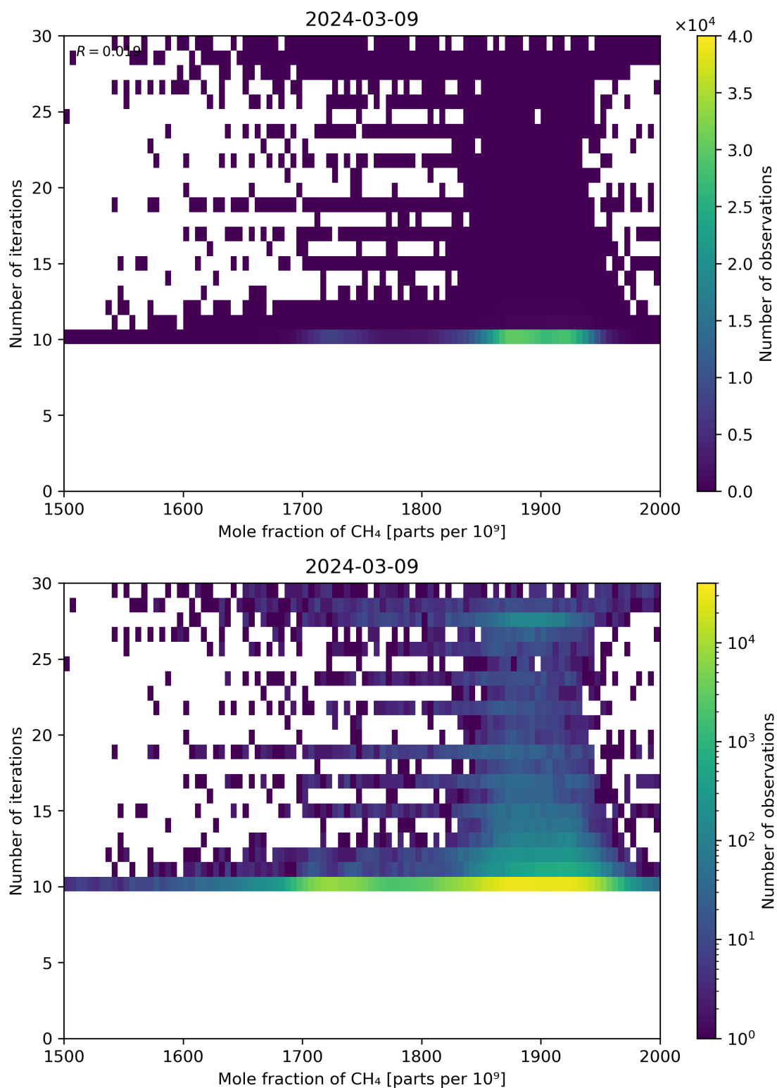
Figure 76: Scatter density plot of “Mole fraction of CH 4 ” against “Number of iterations” for 2024-03-09 to 2024-03-10.
