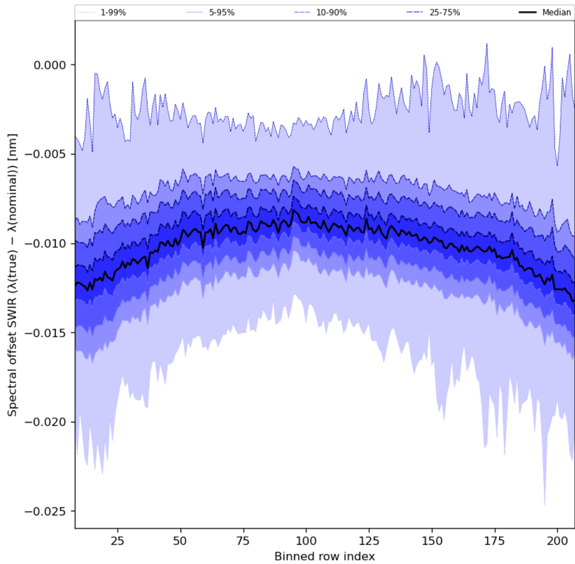
Figure 38: Along track statistics of “Spectral offset SWIR ( \lambda(\text{true}) - \lambda(\text{nominal}) )” for 2024-03-09 to 2024-03-10
