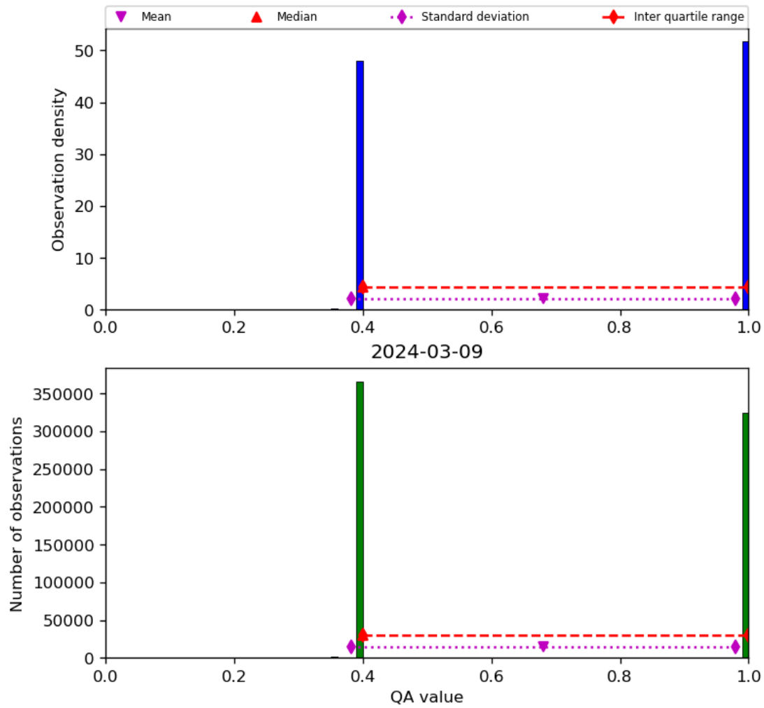
Figure 22: Histogram of “QA value” for 2024-03-09 to 2024-03-10
