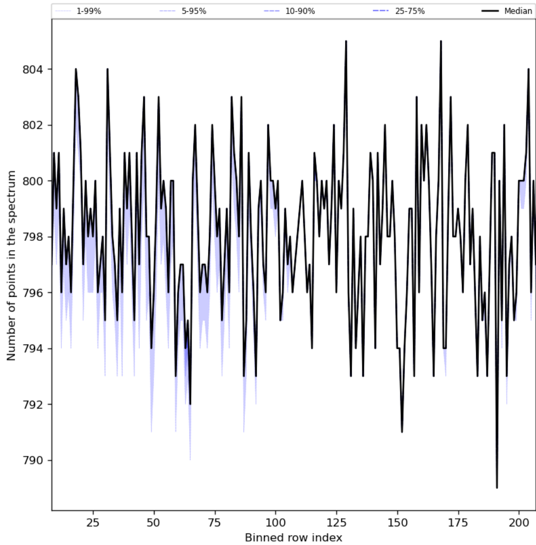
Figure 37: Along track statistics of “Number of points in the spectrum” for 2024-03-09 to 2024-03-10
