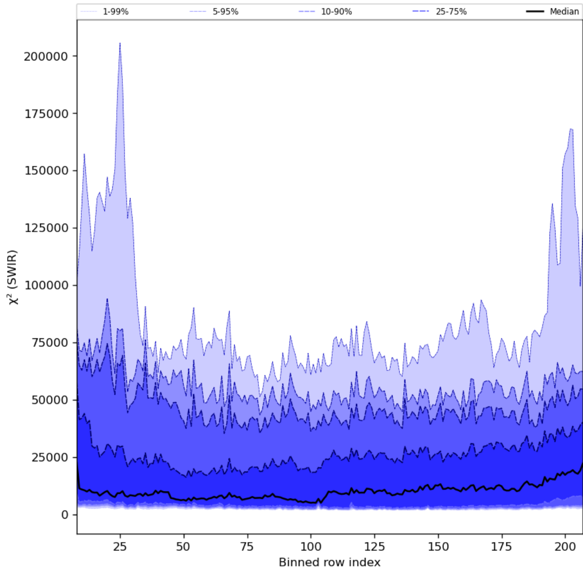
Figure 39: Along track statistics of “ \chi^2 (SWIR)” for 2024-03-09 to 2024-03-10
