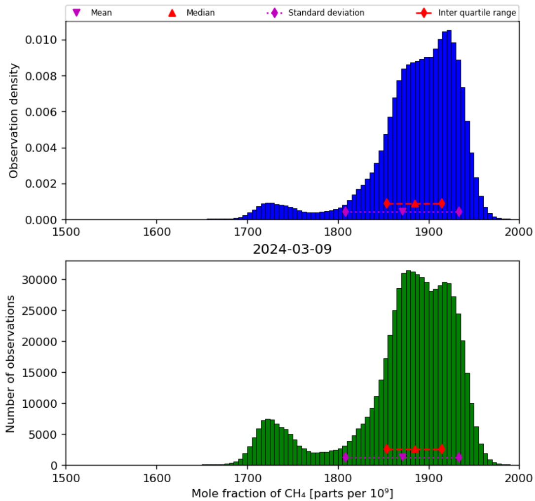
Figure 23: Histogram of “Mole fraction of CH 4 ” for 2024-03-09 to 2024-03-10
