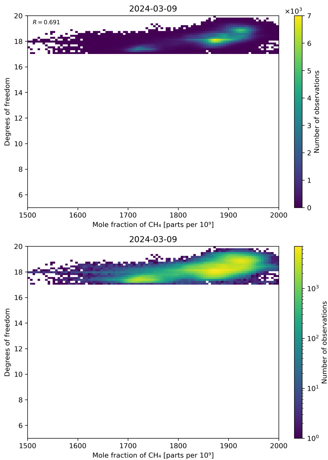
Figure 72: Scatter density plot of “Mole fraction of CH 4 ” against “Degrees of freedom” for 2024-03-09 to 2024-03-10.
