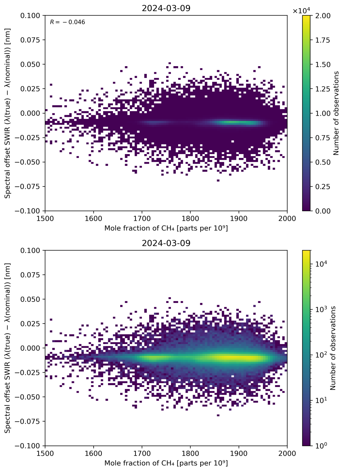
Figure 86: Scatter density plot of “Mole fraction of CH 4 ” against “Spectral offset SWIR ( \lambda(\text{true}) - \lambda(\text{nominal}) )” for 2024-03-09 to 2024-03-10.
