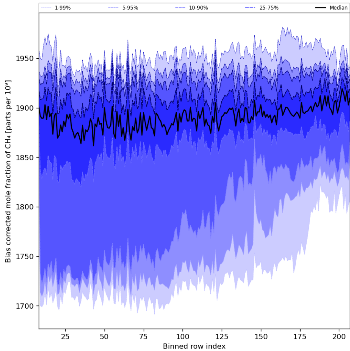
Figure 36: Along track statistics of “Bias corrected mole fraction of CH 4 ” for 2024-03-09 to 2024-03-10
