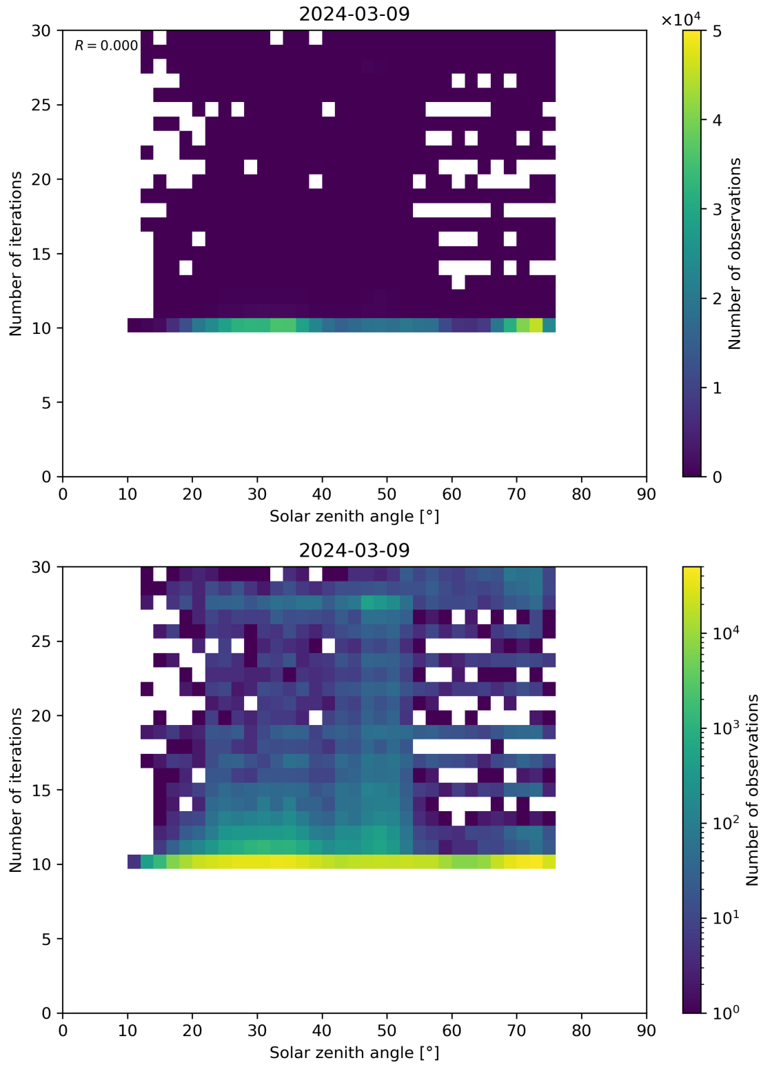
Figure 102: Scatter density plot of “Solar zenith angle” against “Number of iterations” for 2024-03-09 to 2024-03-10.
