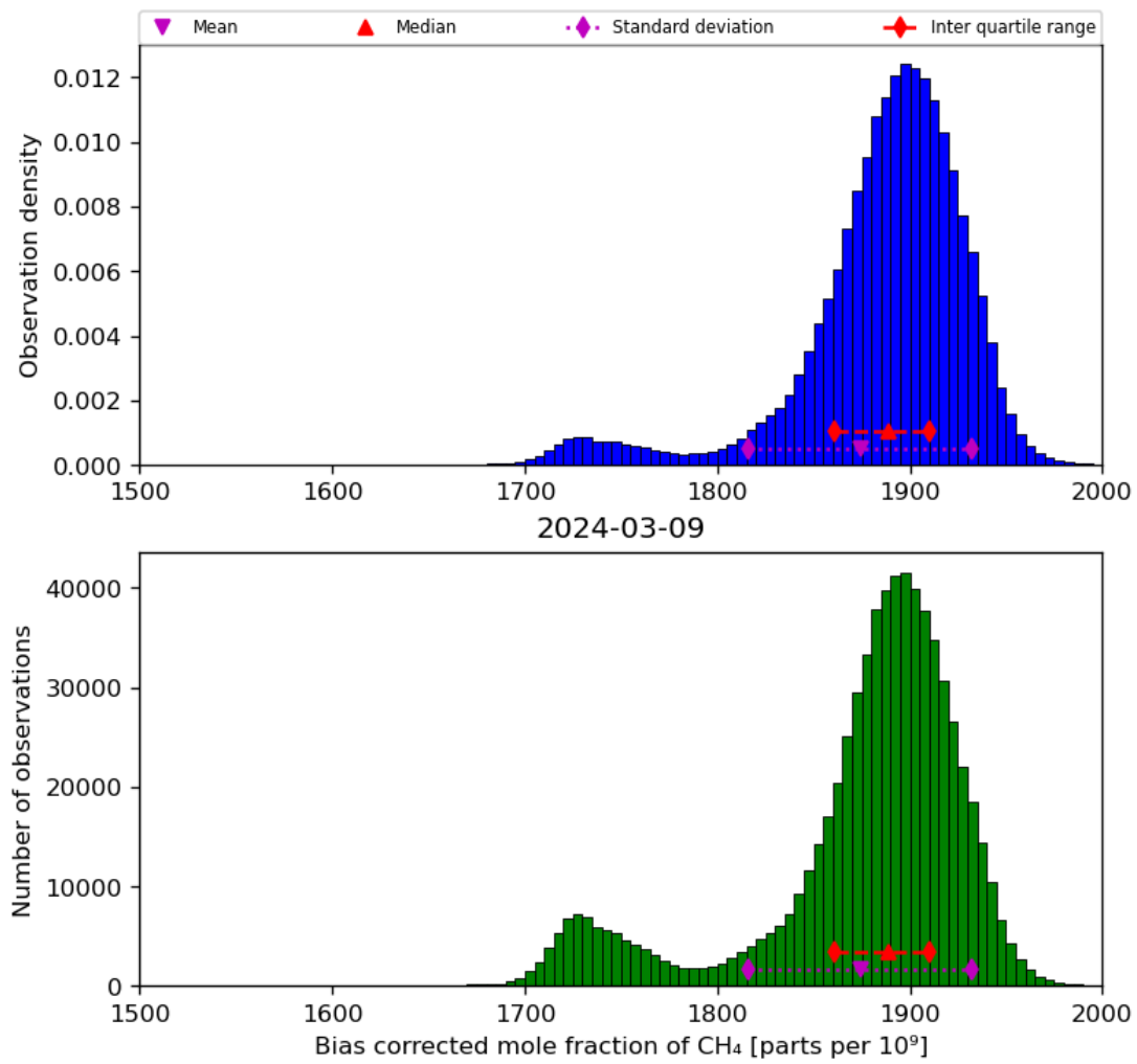
Figure 25: Histogram of “Bias corrected mole fraction of CH 4 ” for 2024-03-09 to 2024-03-10
