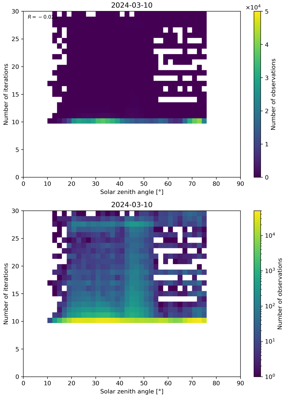
Figure 102: Scatter density plot of “Solar zenith angle” against “Number of iterations” for 2024-03-09 to 2024-03-11.
