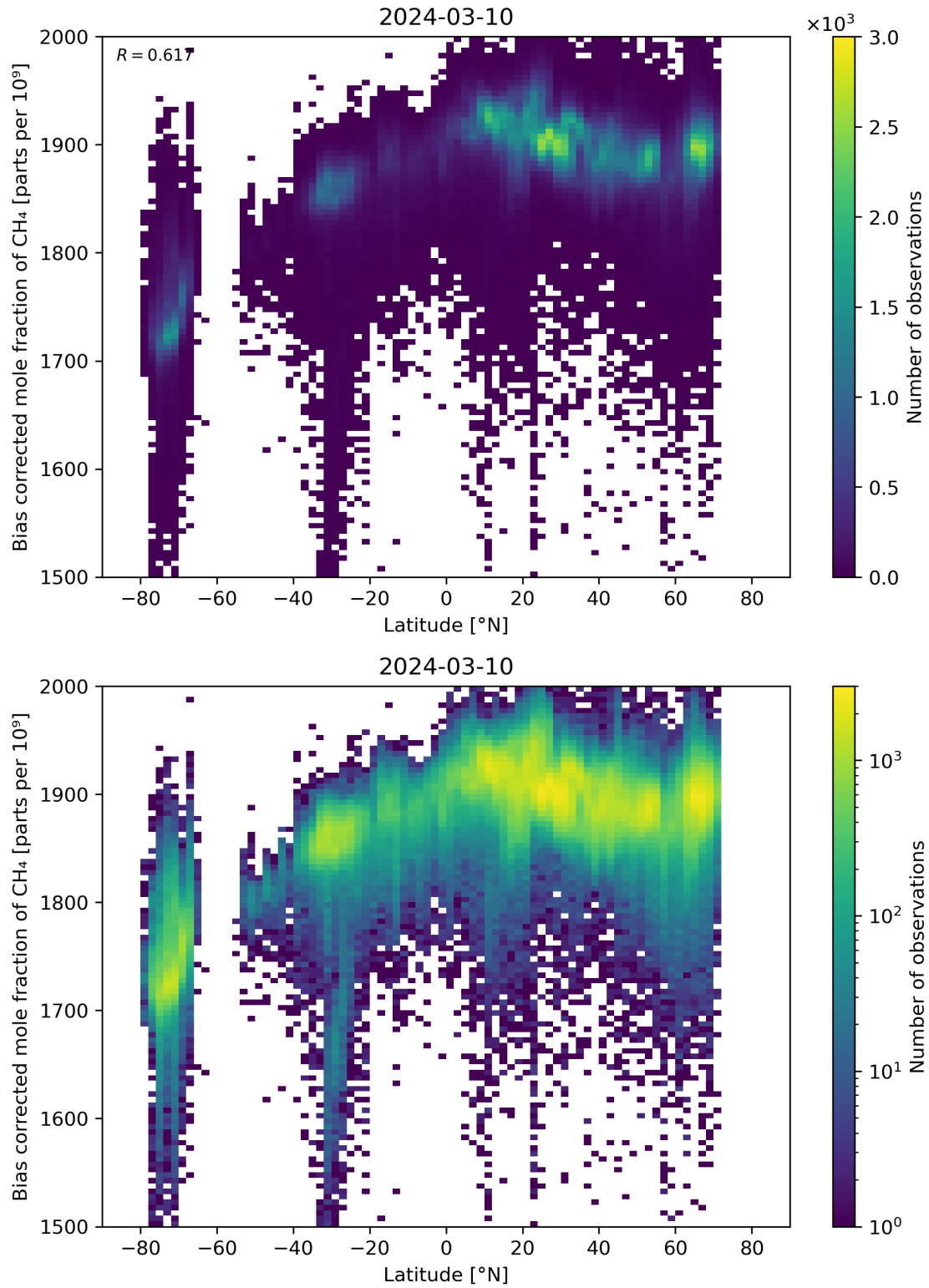
Figure 58: Scatter density plot of “Latitude” against “Bias corrected mole fraction of \text{CH}_4 ” for 2024-03-09 to 2024-03-11.
