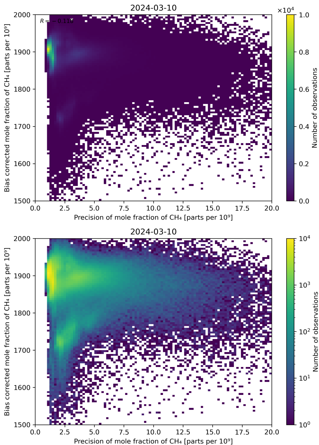
Figure 82: Scatter density plot of “Precision of mole fraction of CH 4 ” against “Bias corrected mole fraction of CH 4 ” for 2024-03-09 to 2024-03-11.
