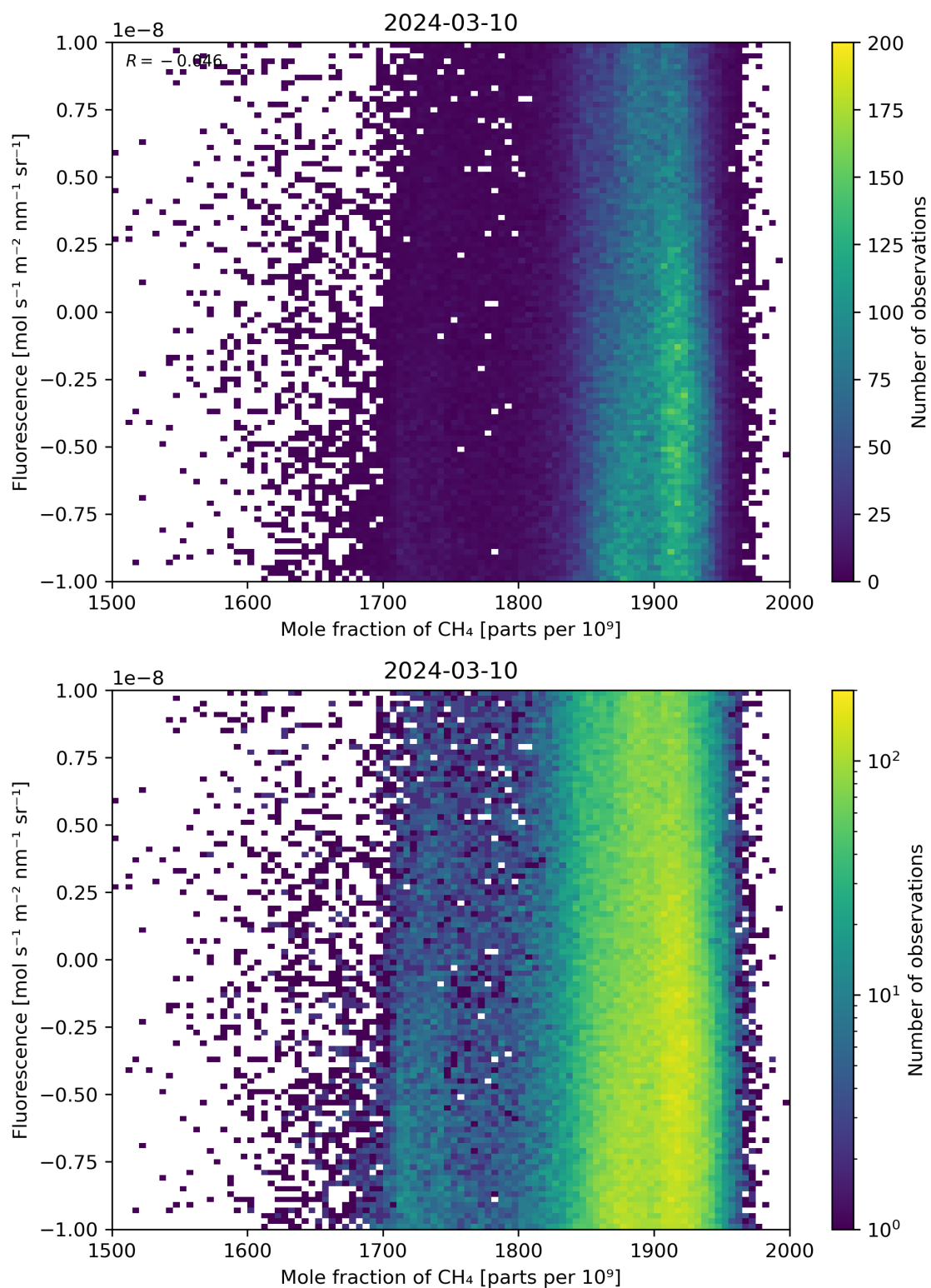
Figure 73: Scatter density plot of “Mole fraction of \text{CH}_4 ” against “Fluorescence” for 2024-03-09 to 2024-03-11.
