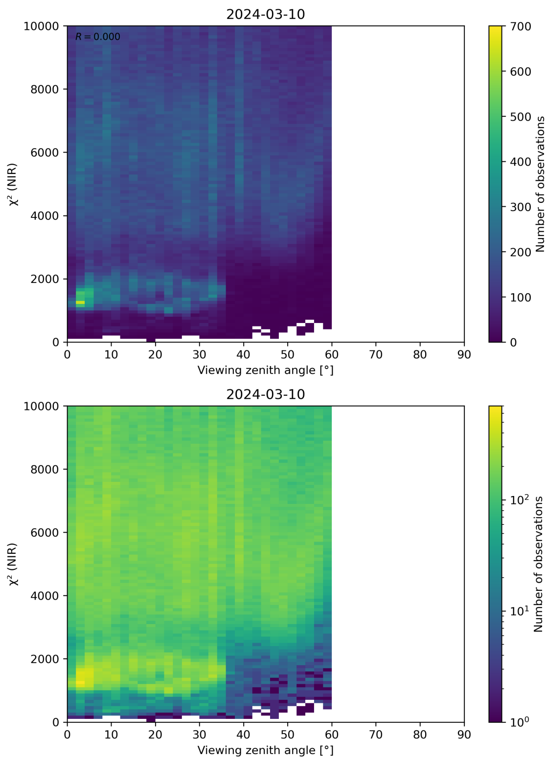
Figure 105: Scatter density plot of “Viewing zenith angle” against “ \chi^2 (NIR)” for 2024-03-09 to 2024-03-11.
