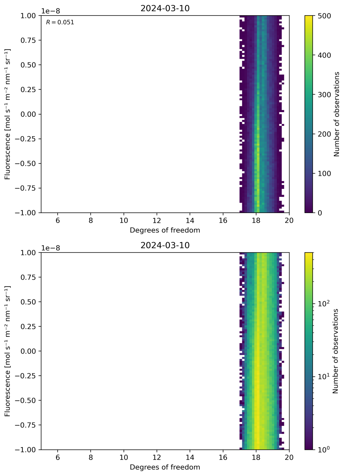
Figure 51: Scatter density plot of “Degrees of freedom” against “Fluorescence” for 2024-03-09 to 2024-03-11.
