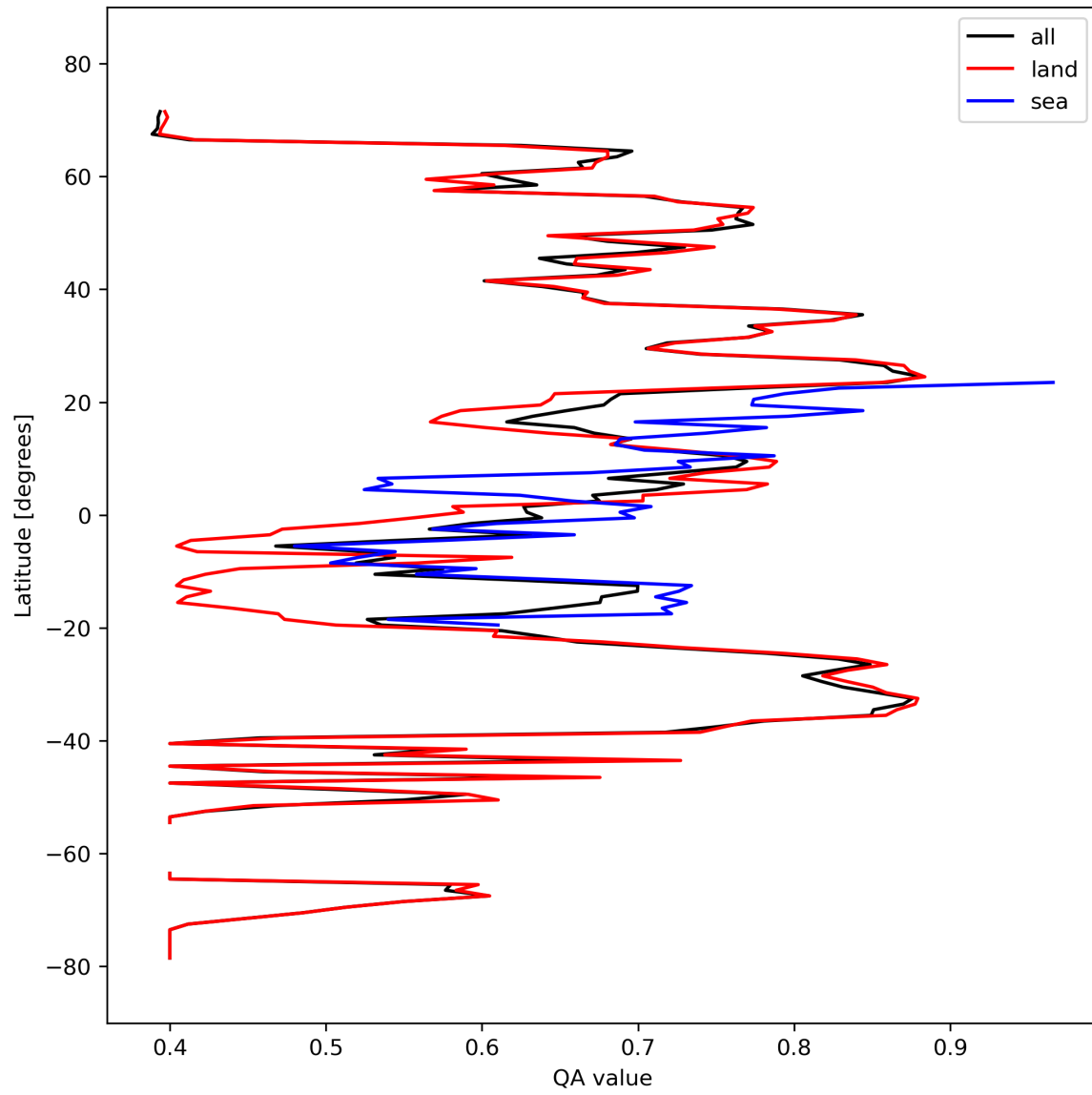
Figure 11: Zonal average of “QA value” for 2024-03-09 to 2024-03-11.
