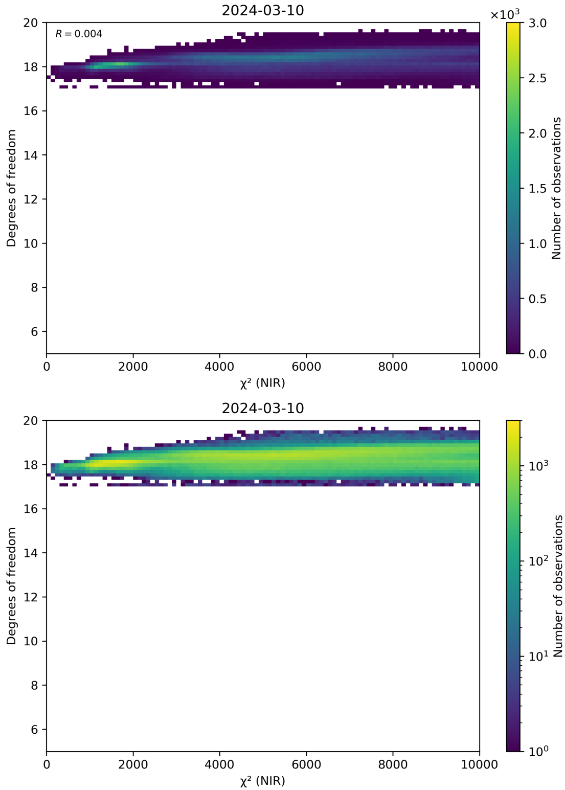
Figure 44: Scatter density plot of “ \chi^2 (NIR)” against “Degrees of freedom” for 2024-03-09 to 2024-03-11.
