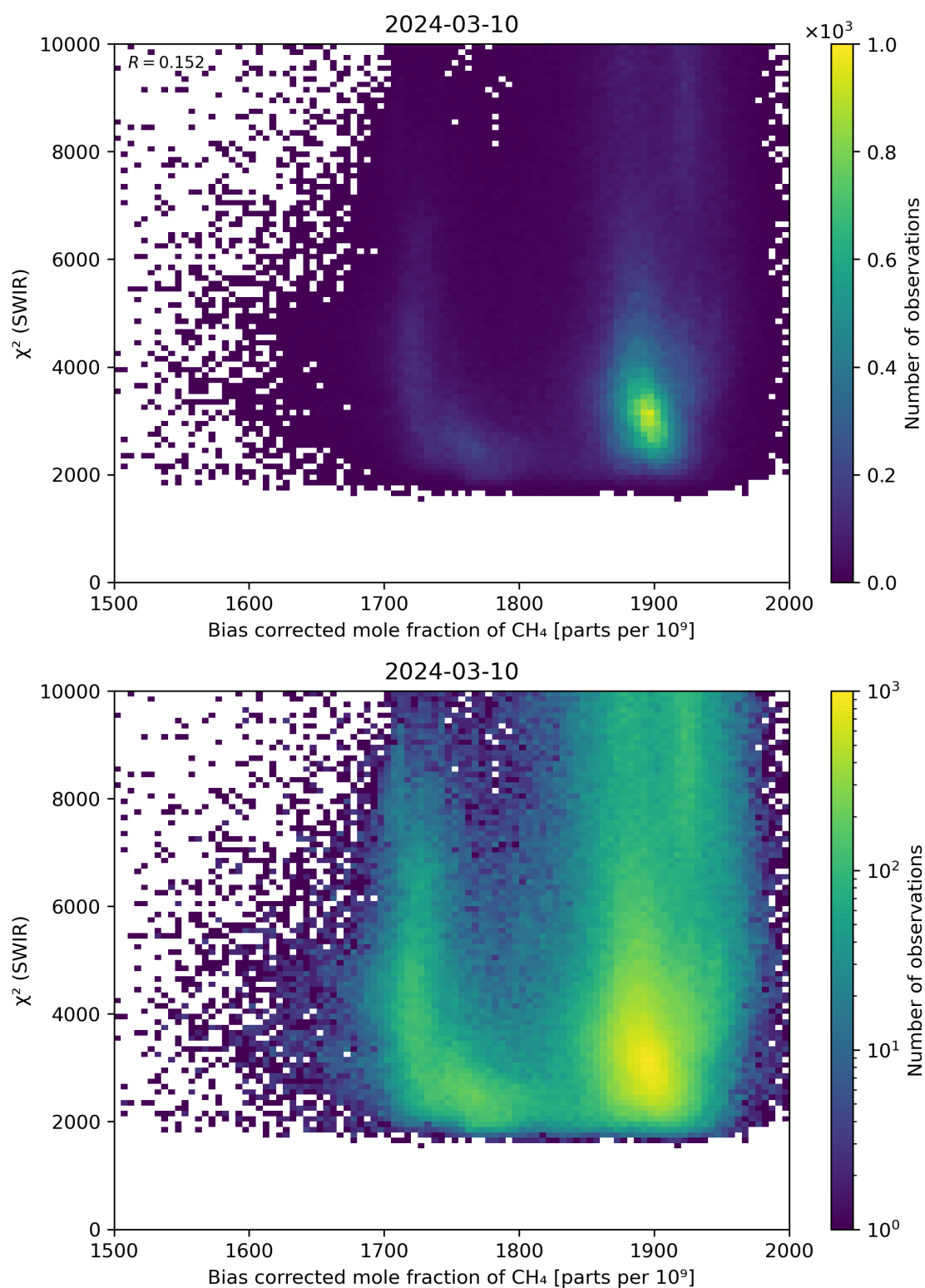
Figure 64: Scatter density plot of “Bias corrected mole fraction of CH 4 ” against “ \chi^2 (SWIR)” for 2024-03-09 to 2024-03-11.
