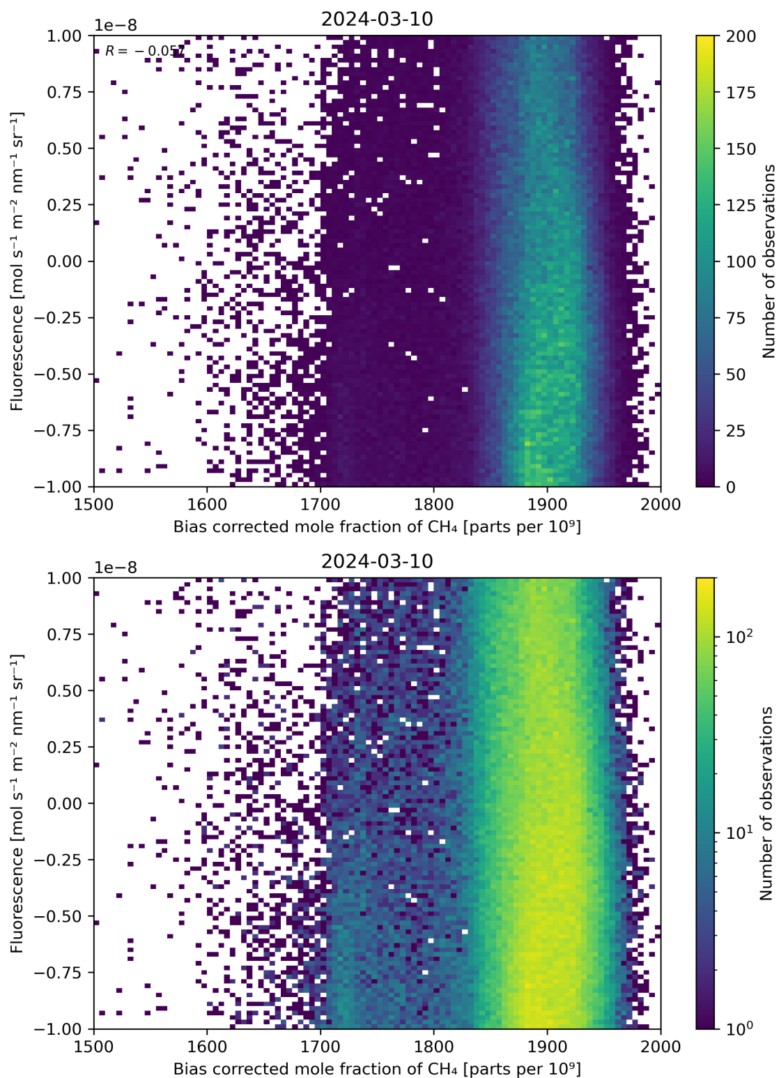
Figure 66: Scatter density plot of “Bias corrected mole fraction of \text{CH}_4 ” against “Fluorescence” for 2024-03-09 to 2024-03-11.
