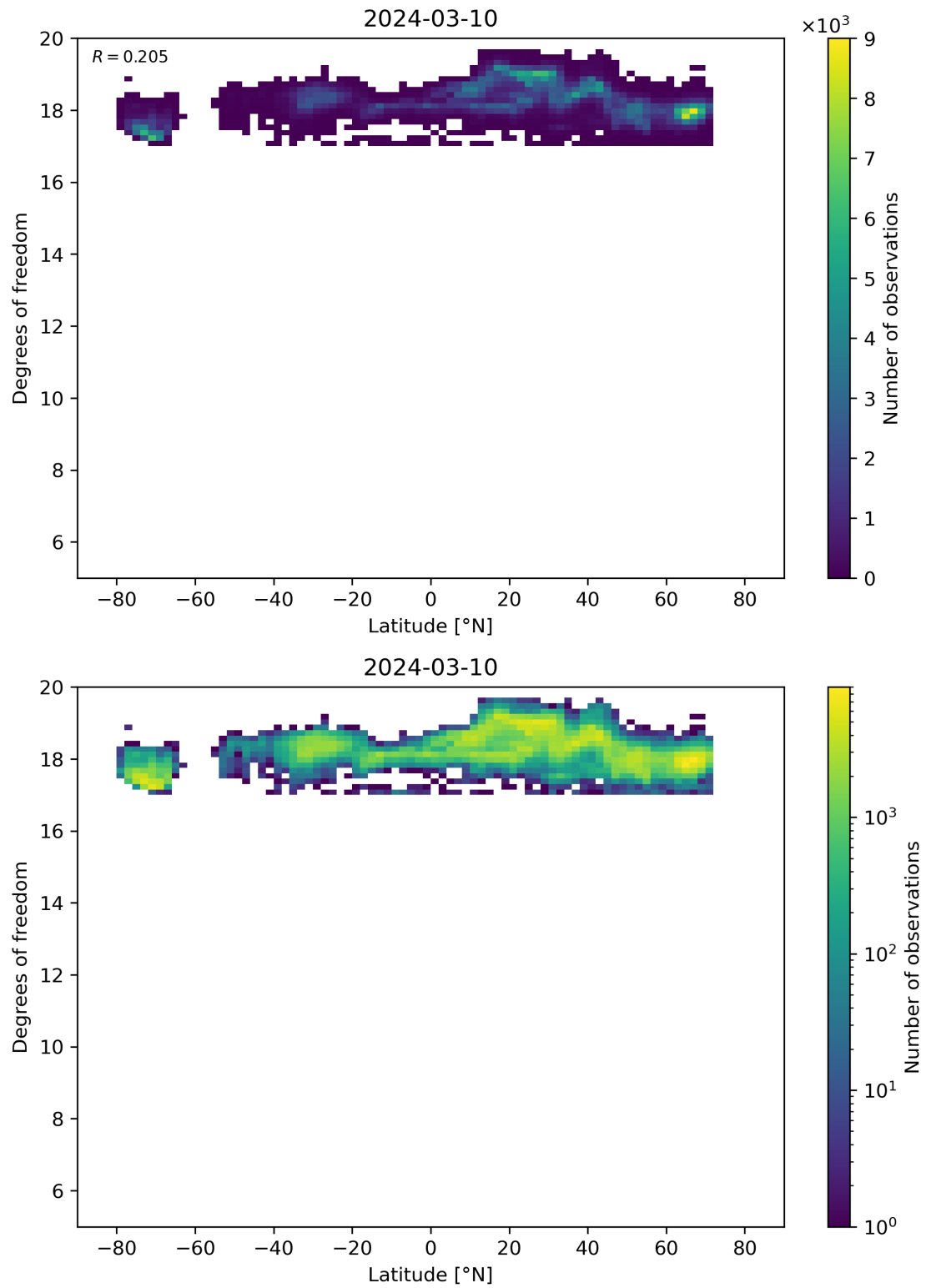
Figure 55: Scatter density plot of “Latitude” against “Degrees of freedom” for 2024-03-09 to 2024-03-11.
