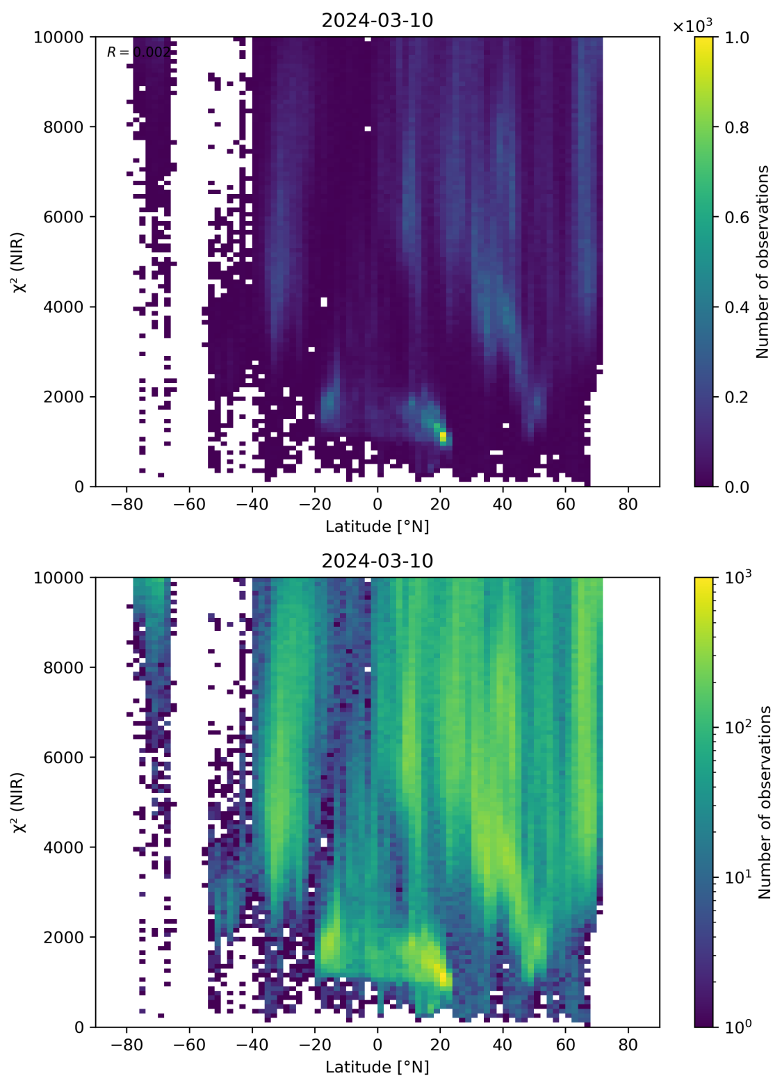
Figure 53: Scatter density plot of “Latitude” against “ \chi^2 (NIR)” for 2024-03-09 to 2024-03-11.
