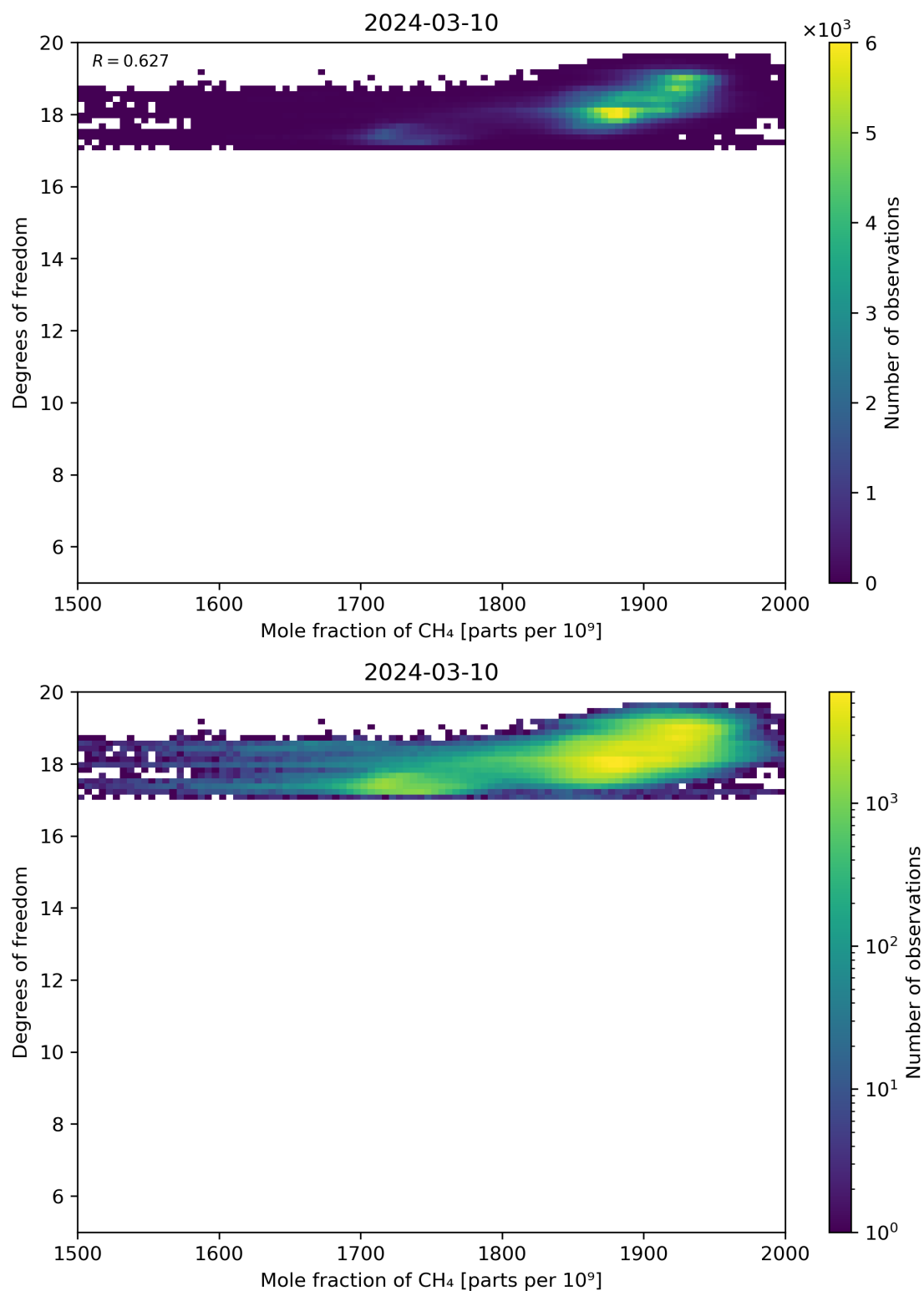
Figure 72: Scatter density plot of “Mole fraction of CH 4 ” against “Degrees of freedom” for 2024-03-09 to 2024-03-11.
