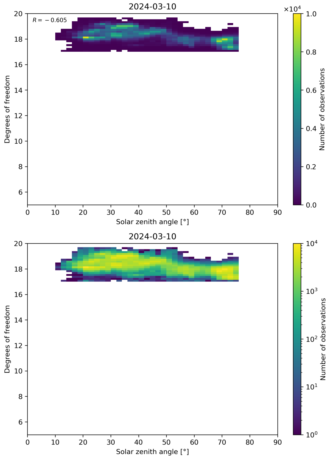
Figure 96: Scatter density plot of “Solar zenith angle” against “Degrees of freedom” for 2024-03-09 to 2024-03-11.
