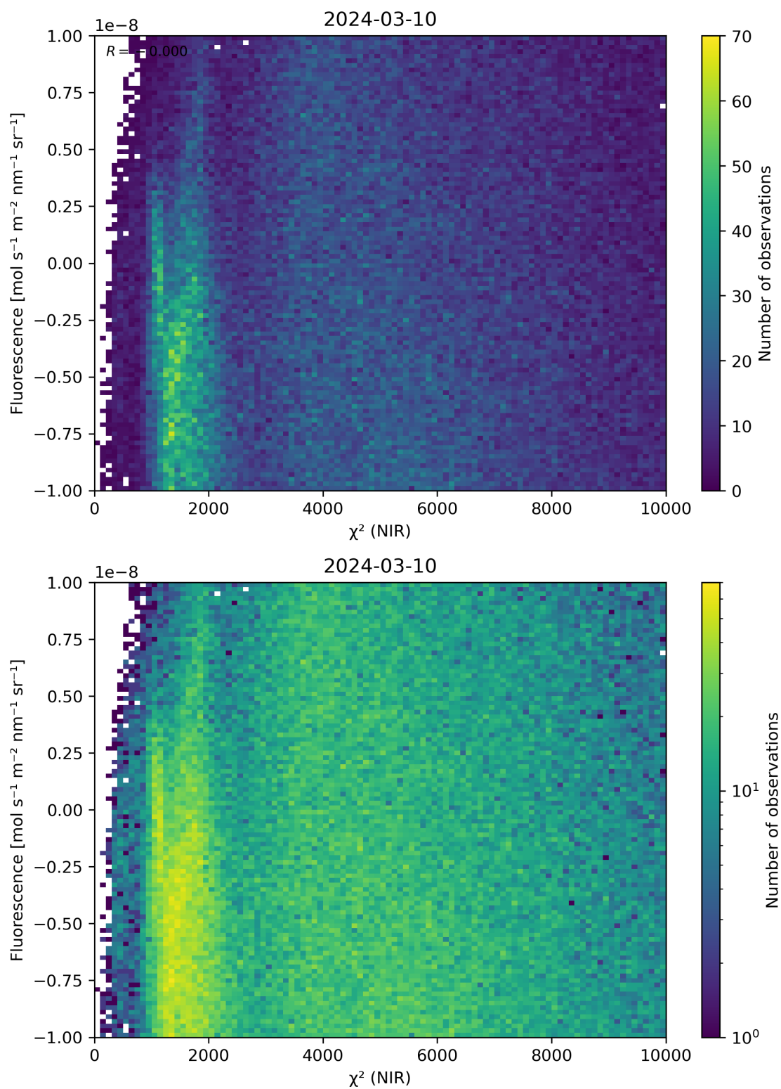
Figure 45: Scatter density plot of “ \chi^2 (NIR)” against “Fluorescence” for 2024-03-09 to 2024-03-11.
