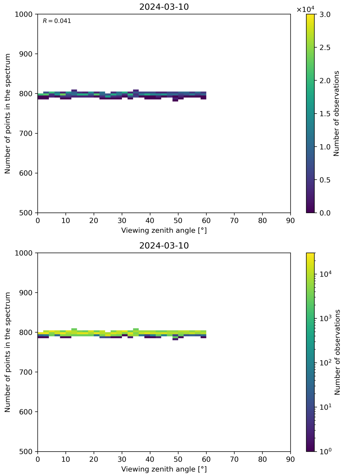
Figure 114: Scatter density plot of “Viewing zenith angle” against “Number of points in the spectrum” for 2024-03-09 to 2024-03-11.
