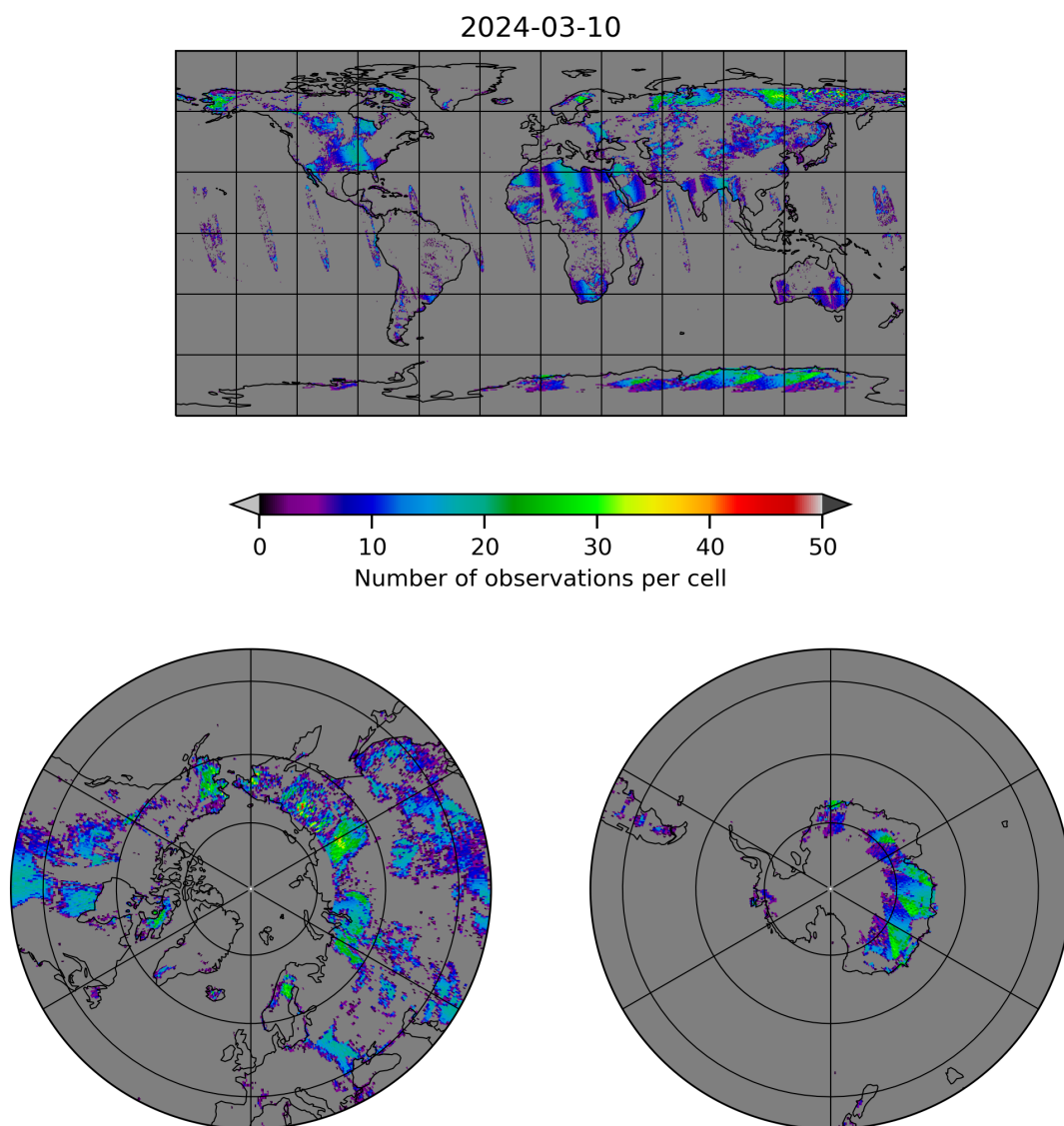
Figure 10: Map of the number of observations for 2024-03-09 to 2024-03-11
