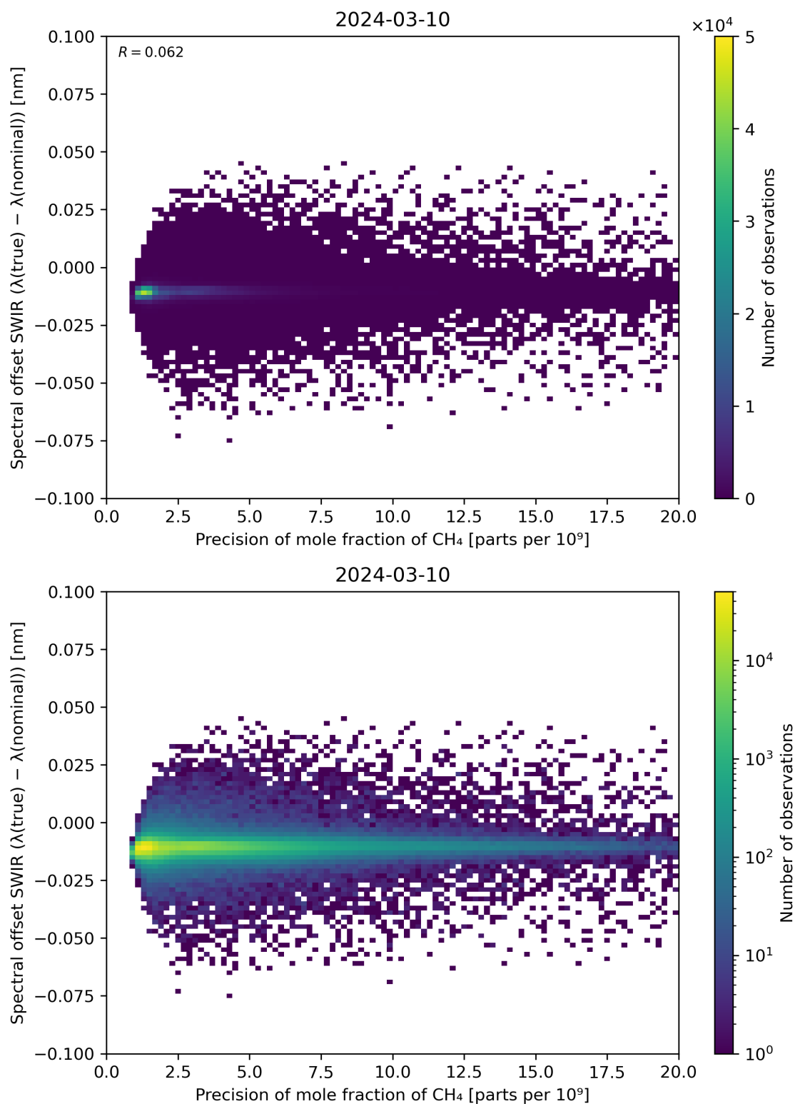
Figure 85: Scatter density plot of “Precision of mole fraction of CH 4 ” against “Spectral offset SWIR ( \lambda(\text{true}) - \lambda(\text{nominal}) )” for 2024-03-09 to 2024-03-11.
