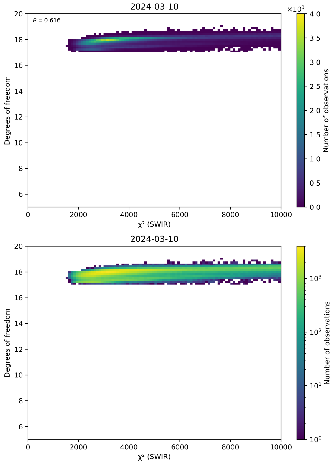
Figure 48: Scatter density plot of “ \chi^2 (SWIR)” against “Degrees of freedom” for 2024-03-09 to 2024-03-11.
