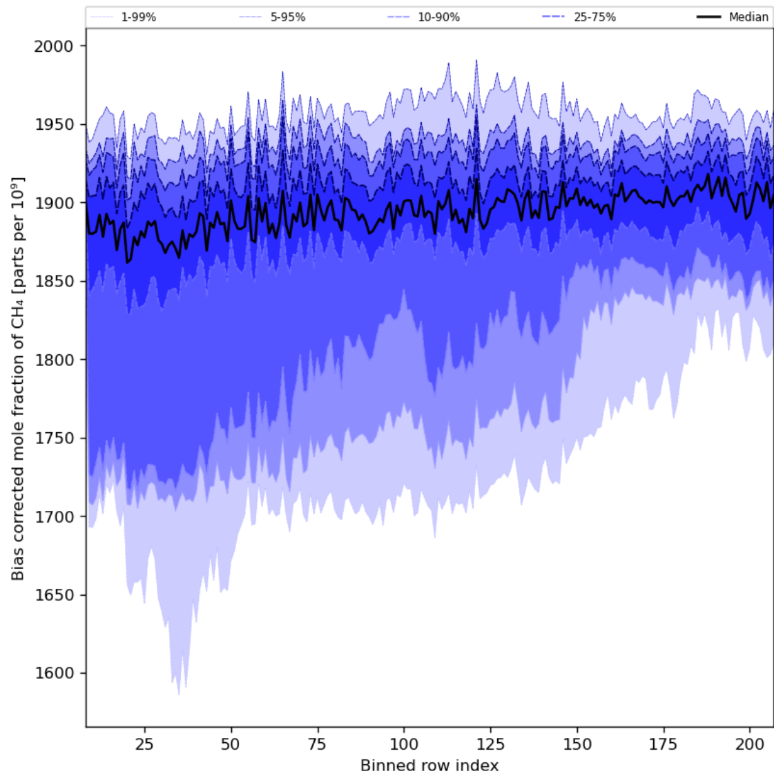
Figure 36: Along track statistics of “Bias corrected mole fraction of CH 4 ” for 2024-03-09 to 2024-03-11
