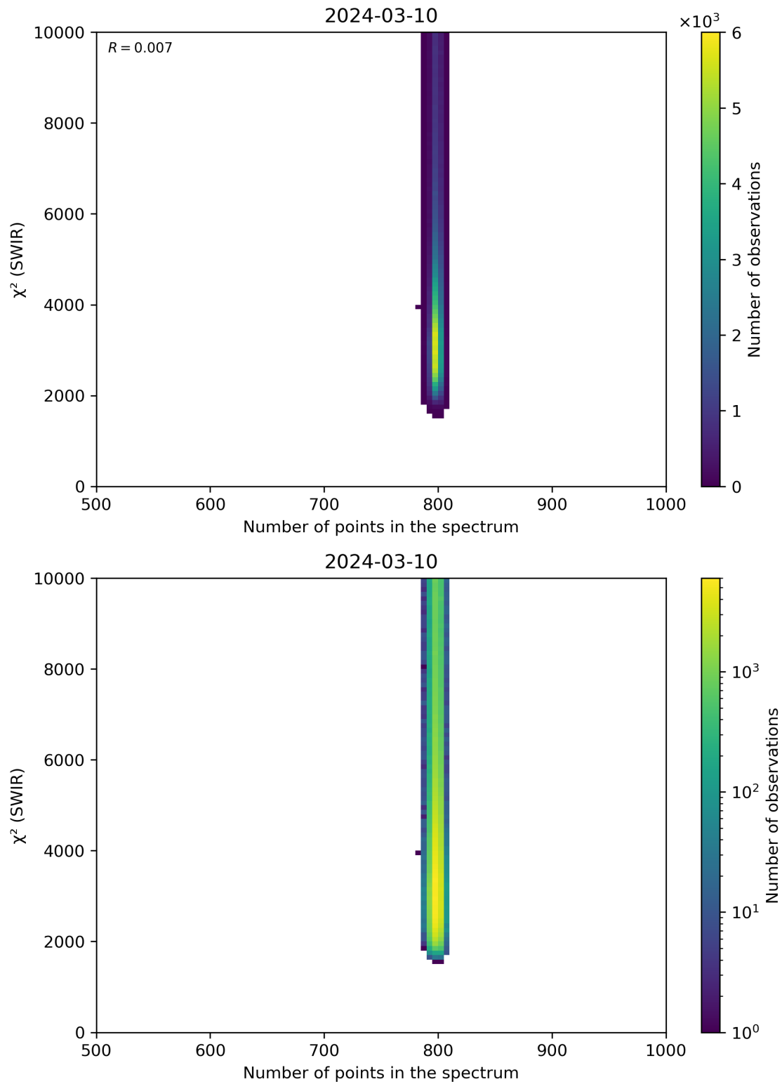
Figure 89: Scatter density plot of “Number of points in the spectrum” against “ \chi^2 (SWIR)” for 2024-03-09 to 2024-03-11.
