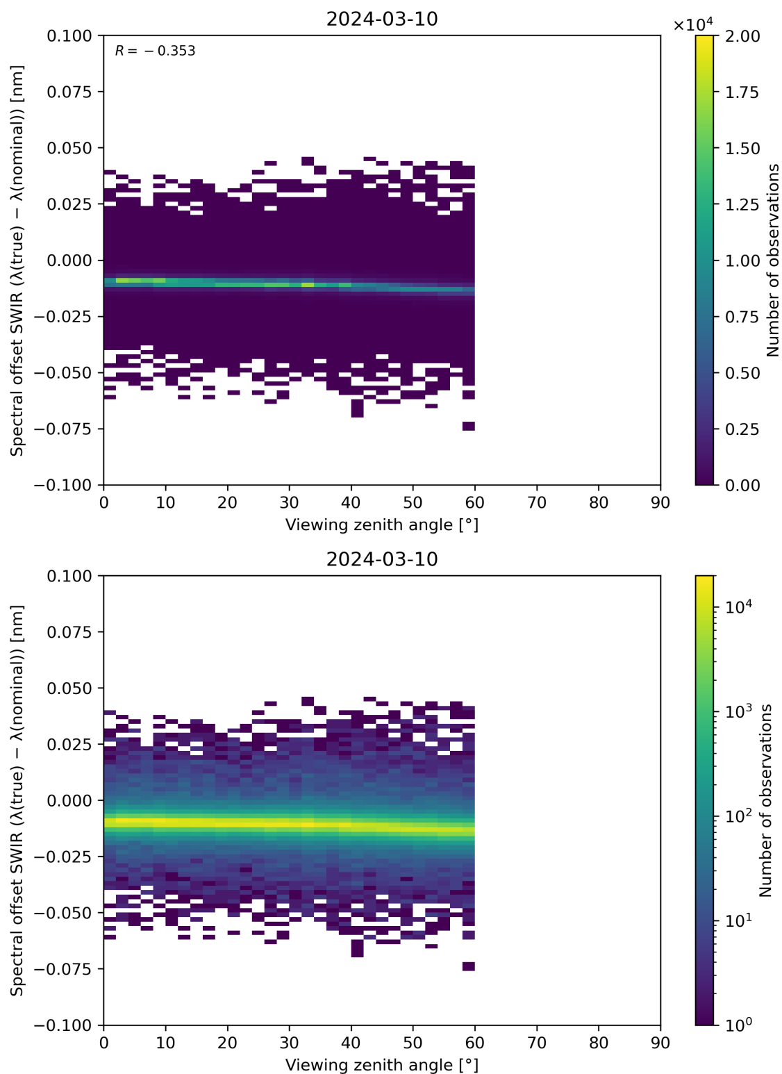
Figure 116: Scatter density plot of “Viewing zenith angle” against “Spectral offset SWIR ( \lambda(\text{true}) - \lambda(\text{nominal}) )” for 2024-03-09 to 2024-03-11.
