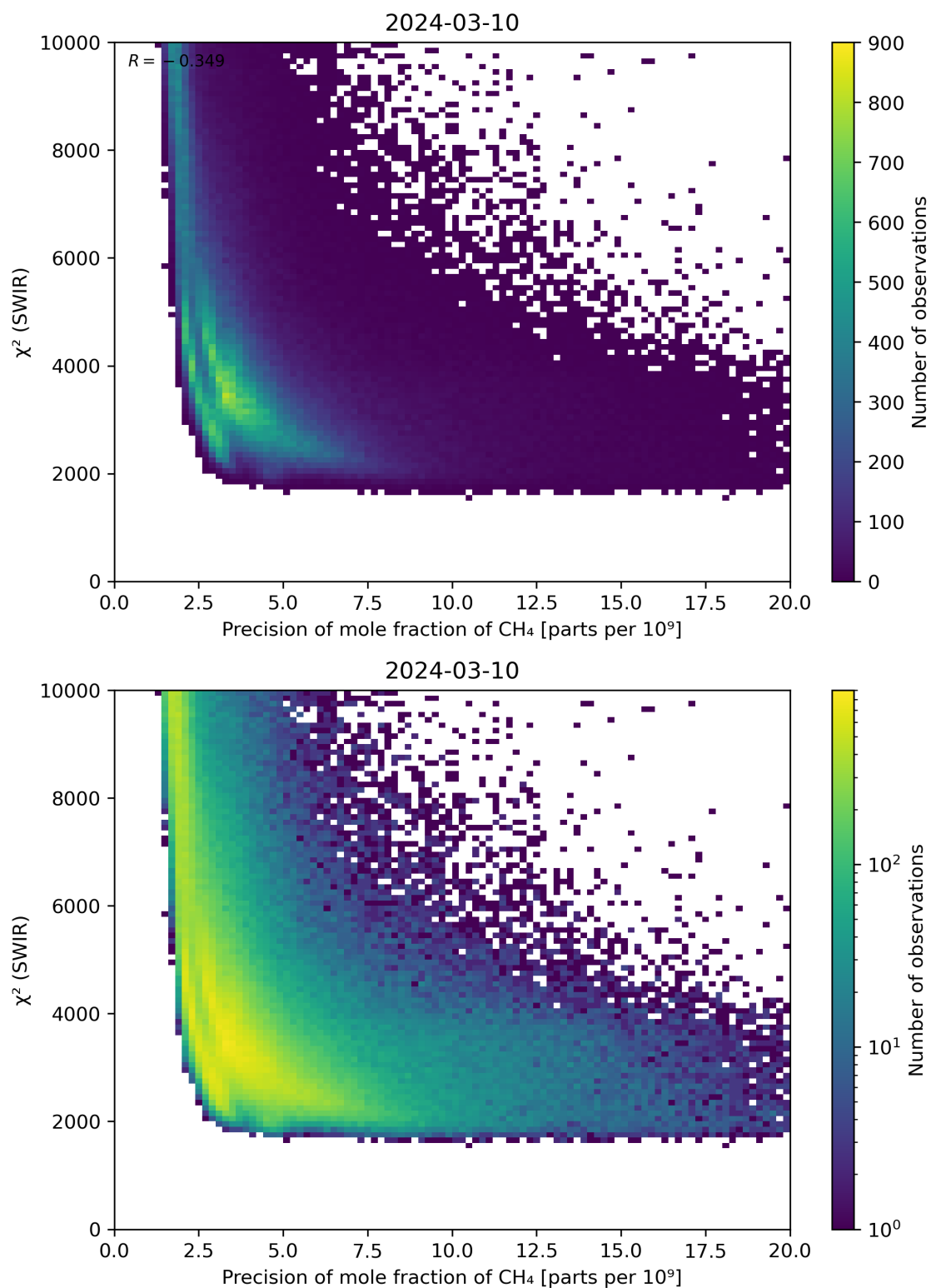
Figure 79: Scatter density plot of “Precision of mole fraction of \text{CH}_4 ” against “ \chi^2 (SWIR)” for 2024-03-09 to 2024-03-11.
