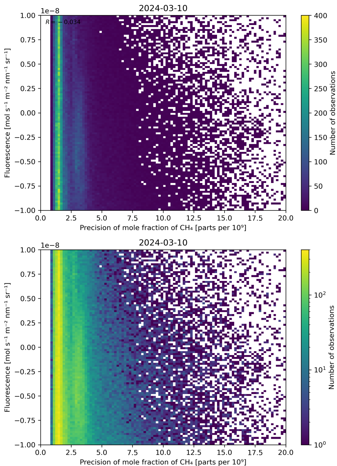
Figure 81: Scatter density plot of “Precision of mole fraction of CH 4 ” against “Fluorescence” for 2024-03-09 to 2024-03-11.
