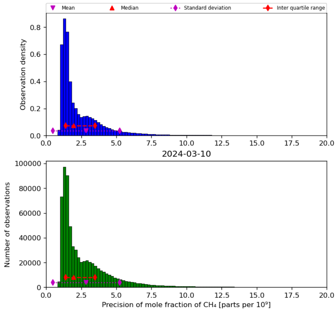
Figure 24: Histogram of “Precision of mole fraction of CH 4 ” for 2024-03-09 to 2024-03-11
