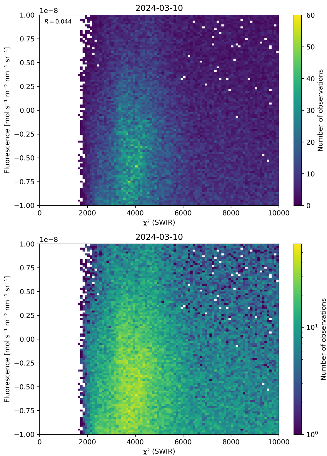
Figure 49: Scatter density plot of “ \chi^2 (SWIR)” against “Fluorescence” for 2024-03-09 to 2024-03-11.
