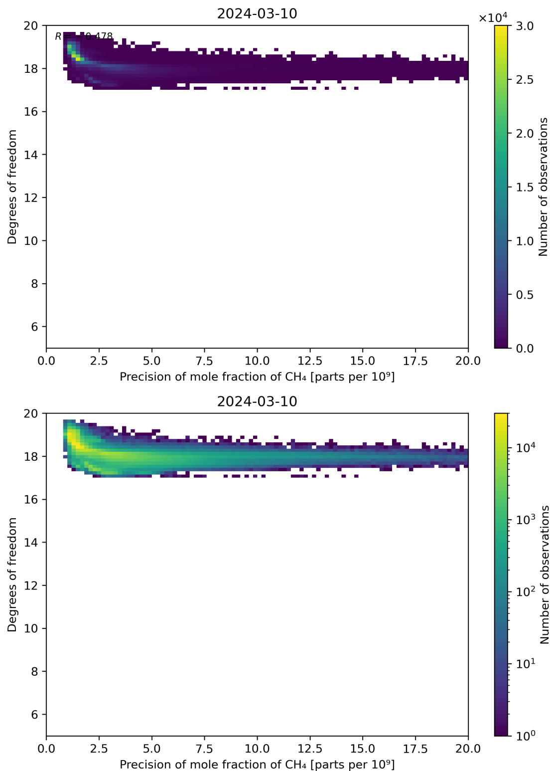
Figure 80: Scatter density plot of “Precision of mole fraction of CH 4 ” against “Degrees of freedom” for 2024-03-09 to 2024-03-11.
