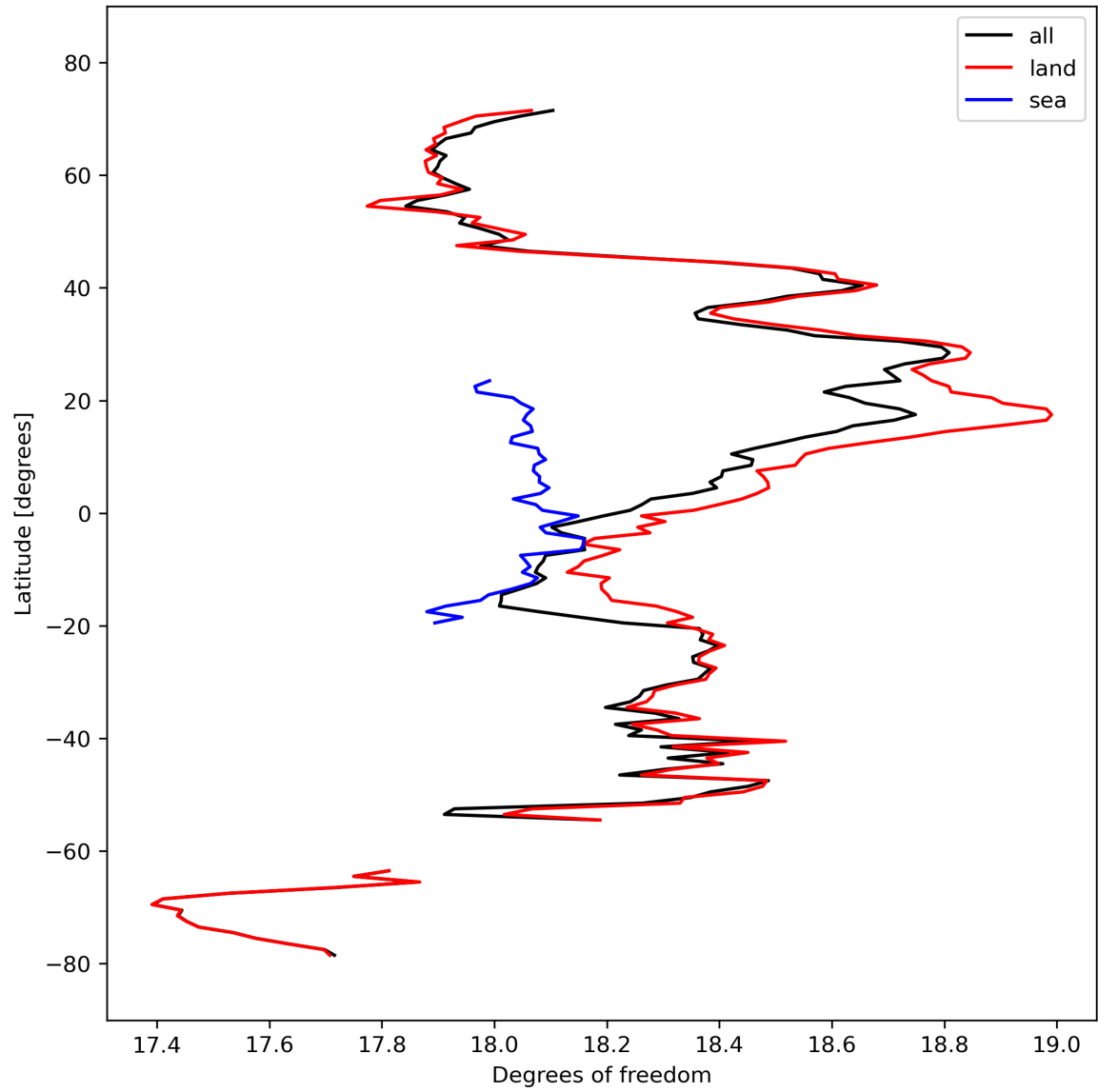
Figure 19: Zonal average of “Degrees of freedom” for 2024-03-09 to 2024-03-11.
