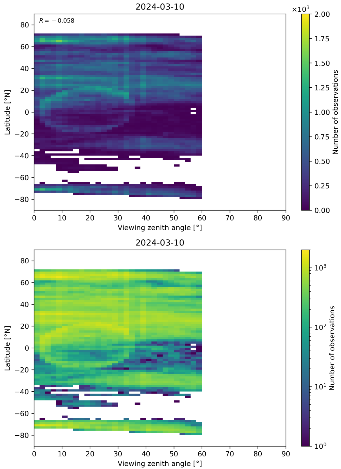
Figure 109: Scatter density plot of “Viewing zenith angle” against “Latitude” for 2024-03-09 to 2024-03-11.
