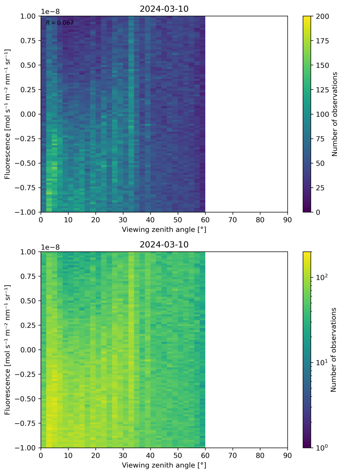
Figure 108: Scatter density plot of “Viewing zenith angle” against “Fluorescence” for 2024-03-09 to 2024-03-11.
