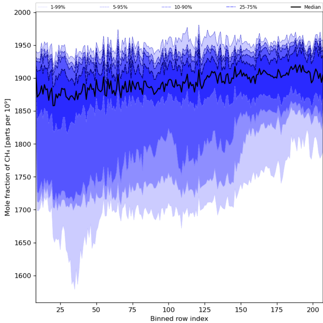
Figure 34: Along track statistics of “Mole fraction of CH 4 ” for 2024-03-09 to 2024-03-11
