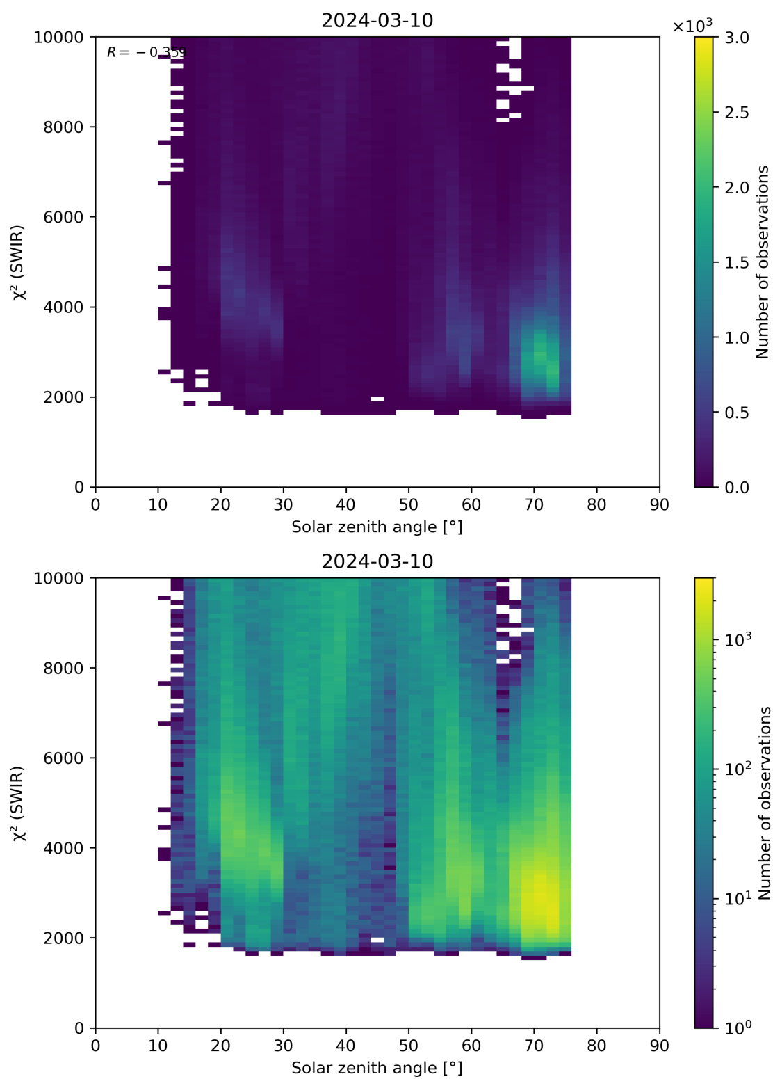
Figure 95: Scatter density plot of “Solar zenith angle” against “ \chi^2 (SWIR)” for 2024-03-09 to 2024-03-11.
