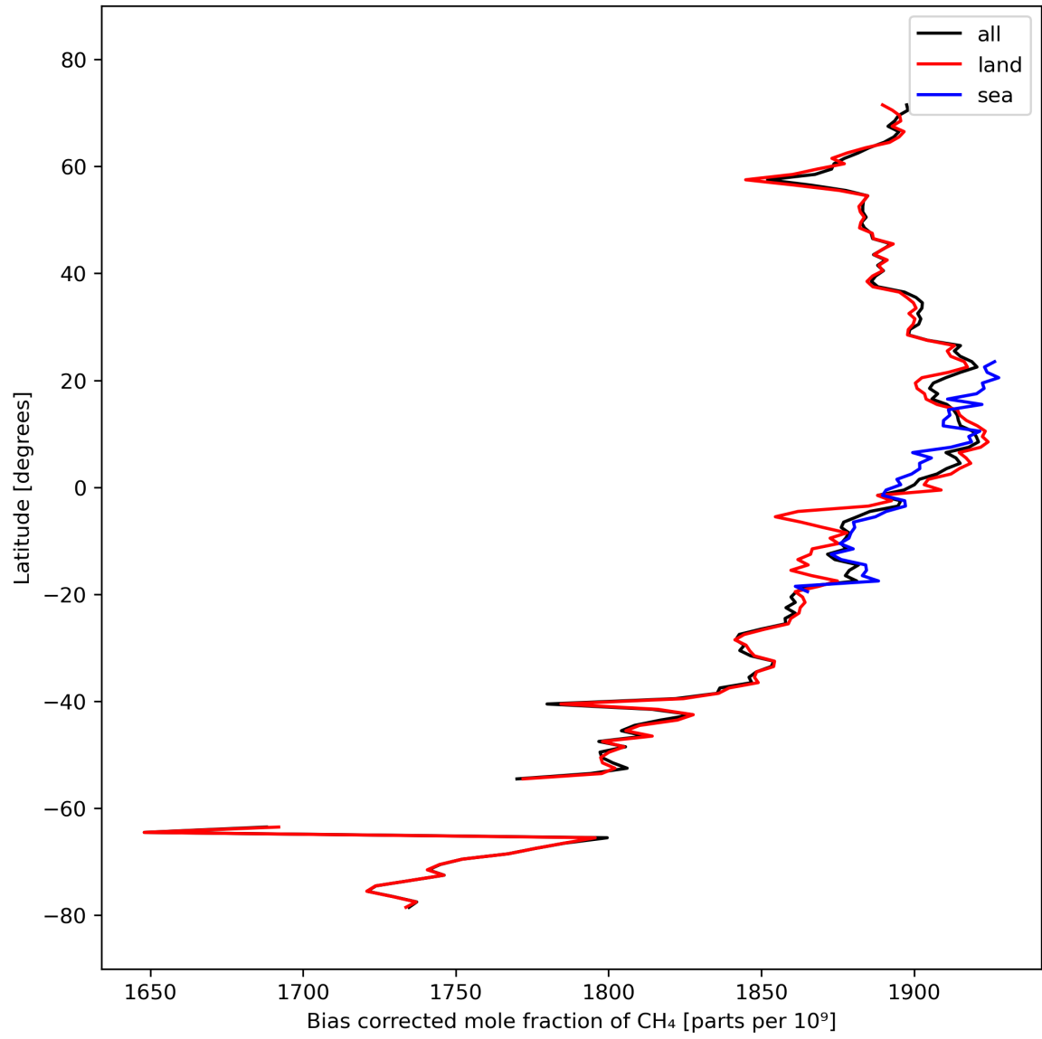
Figure 14: Zonal average of “Bias corrected mole fraction of CH 4 ” for 2024-03-09 to 2024-03-11.
