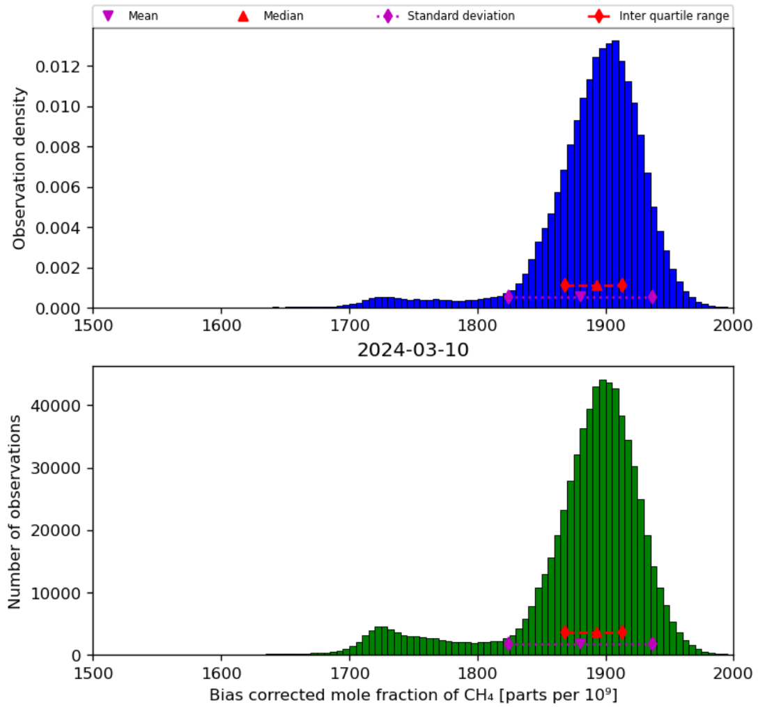
Figure 25: Histogram of “Bias corrected mole fraction of CH 4 ” for 2024-03-09 to 2024-03-11
