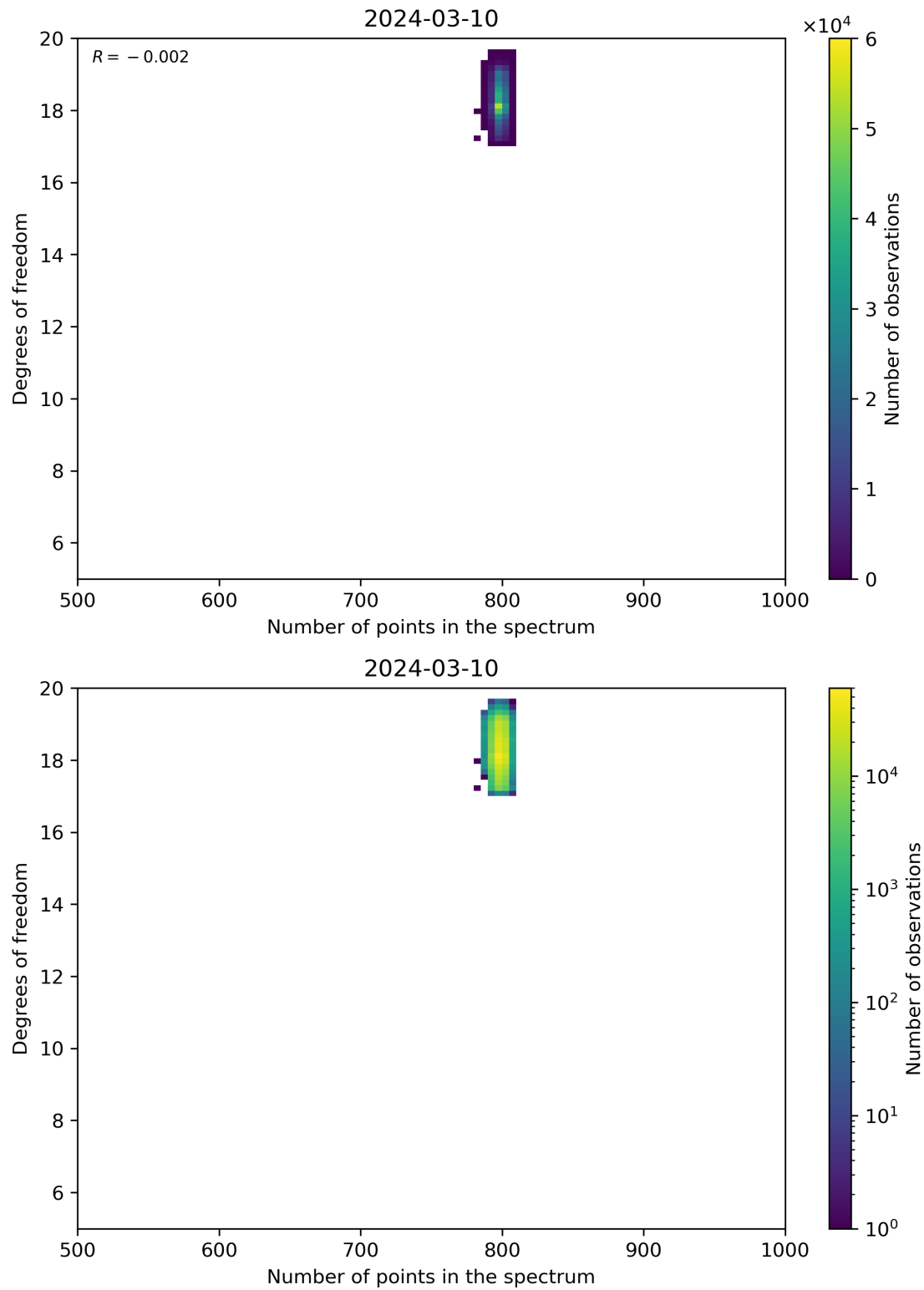
Figure 90: Scatter density plot of “Number of points in the spectrum” against “Degrees of freedom” for 2024-03-09 to 2024-03-11.
