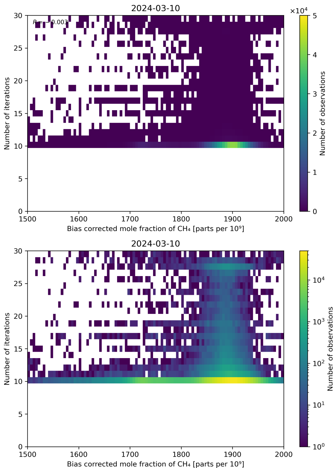
Figure 67: Scatter density plot of “Bias corrected mole fraction of CH 4 ” against “Number of iterations” for 2024-03-09 to 2024-03-11.
