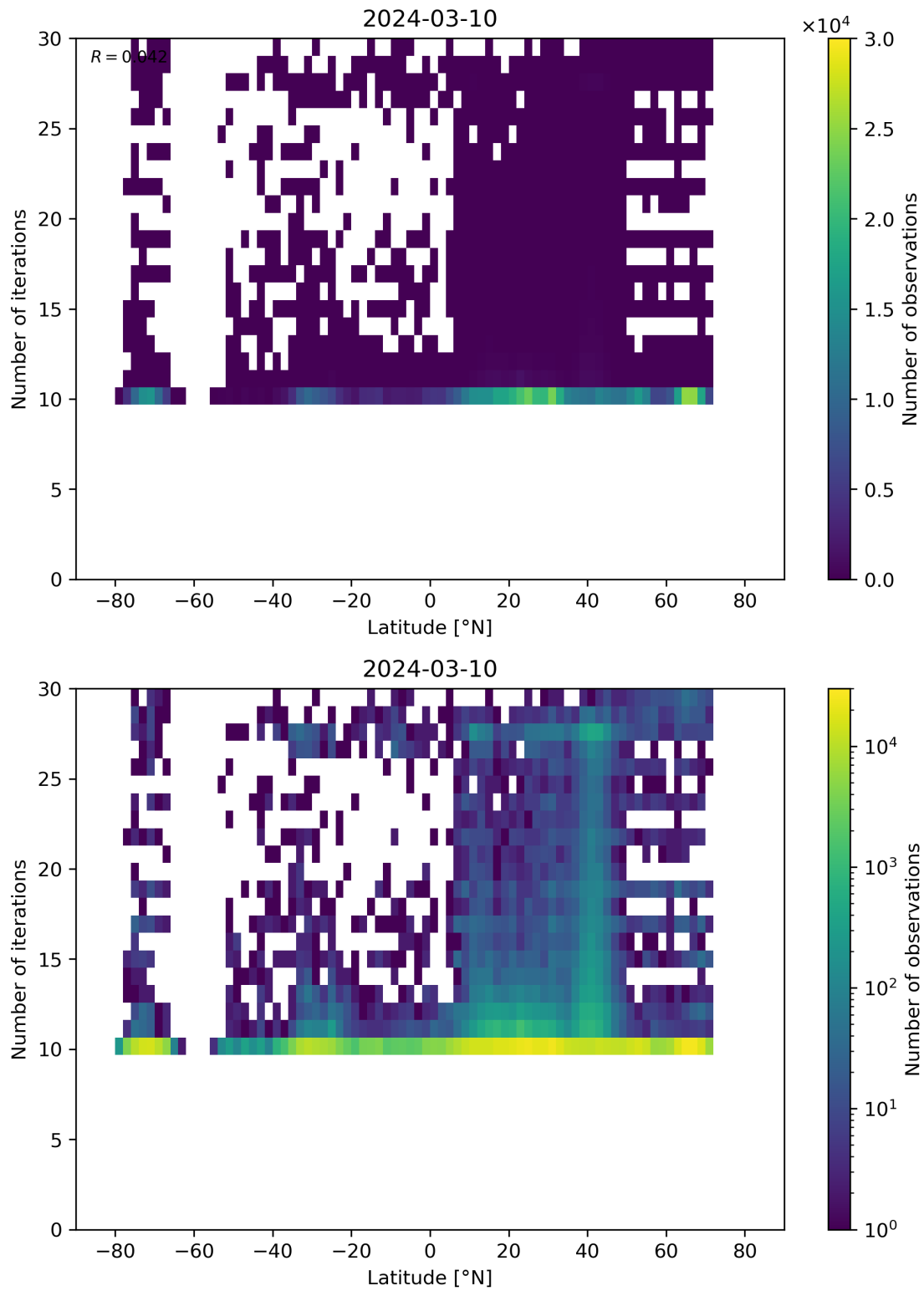
Figure 60: Scatter density plot of “Latitude” against “Number of iterations” for 2024-03-09 to 2024-03-11.
