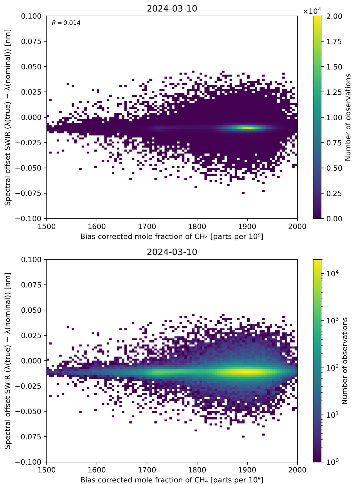
Figure 69: Scatter density plot of “Bias corrected mole fraction of \text{CH}_4 ” against “Spectral offset SWIR ( \lambda(\text{true}) - \lambda(\text{nominal}) )” for 2024-03-09 to 2024-03-11.
