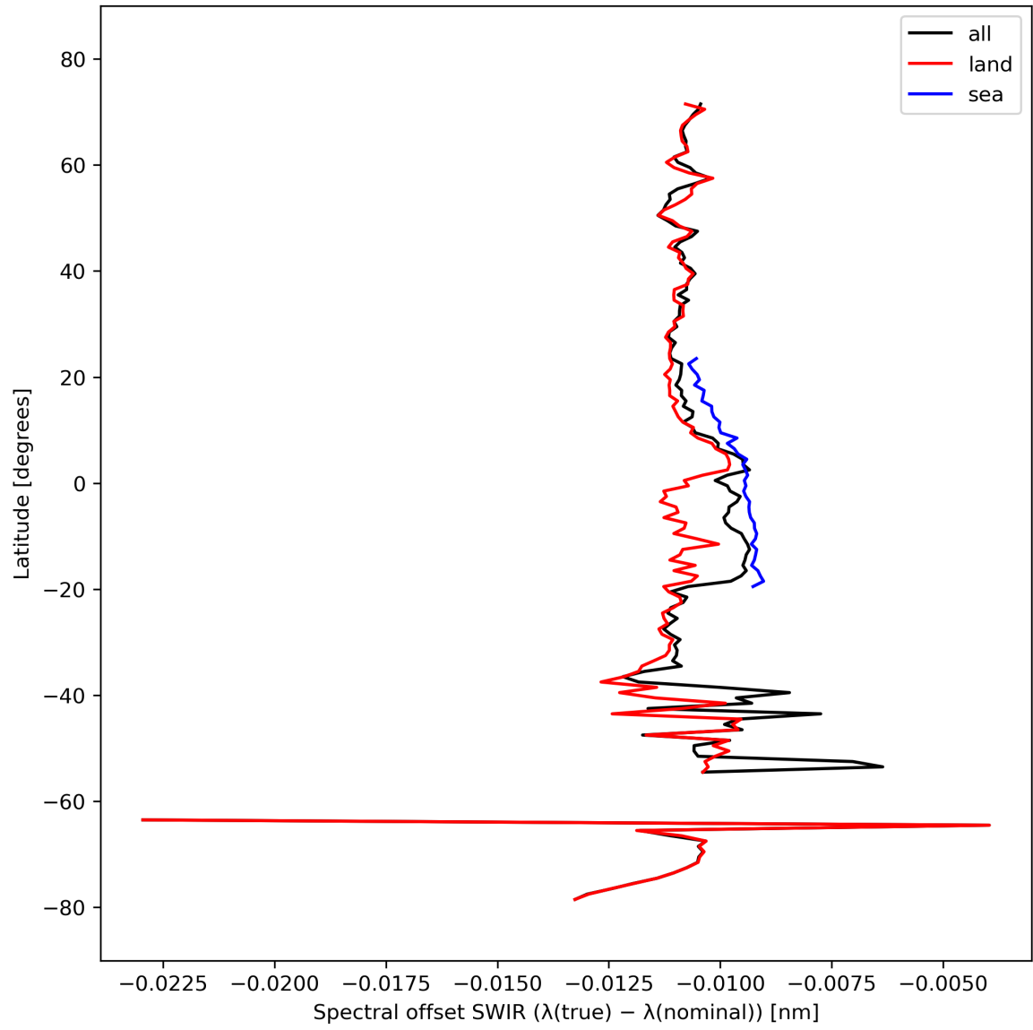
Figure 16: Zonal average of “Spectral offset SWIR ( \lambda(\text{true}) - \lambda(\text{nominal}) )” for 2024-03-09 to 2024-03-11.
