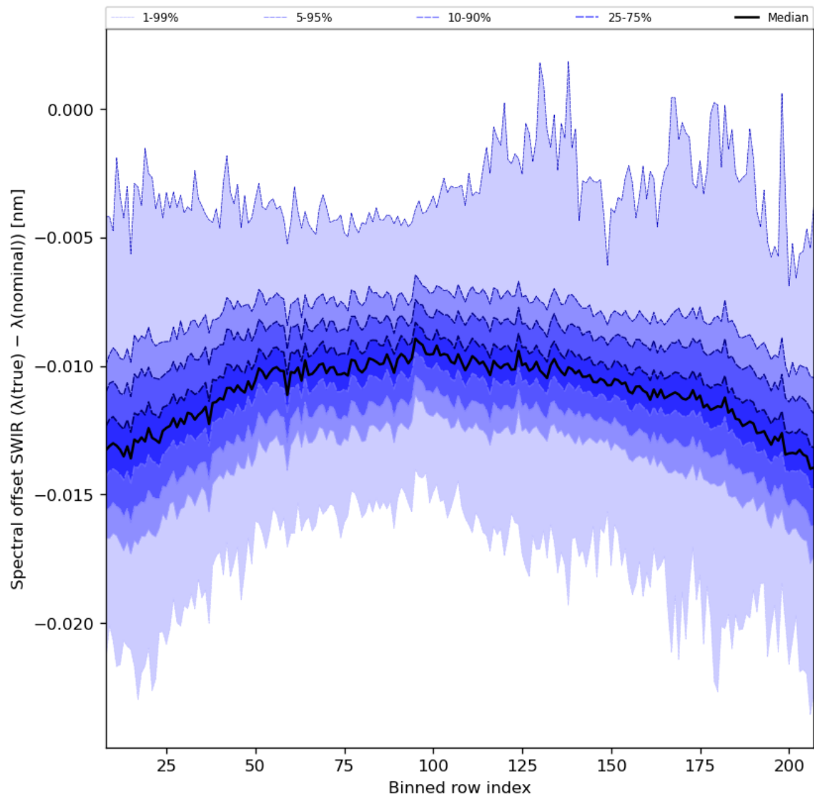
Figure 38: Along track statistics of “Spectral offset SWIR ( \lambda(\text{true}) - \lambda(\text{nominal}) )” for 2024-03-09 to 2024-03-11
