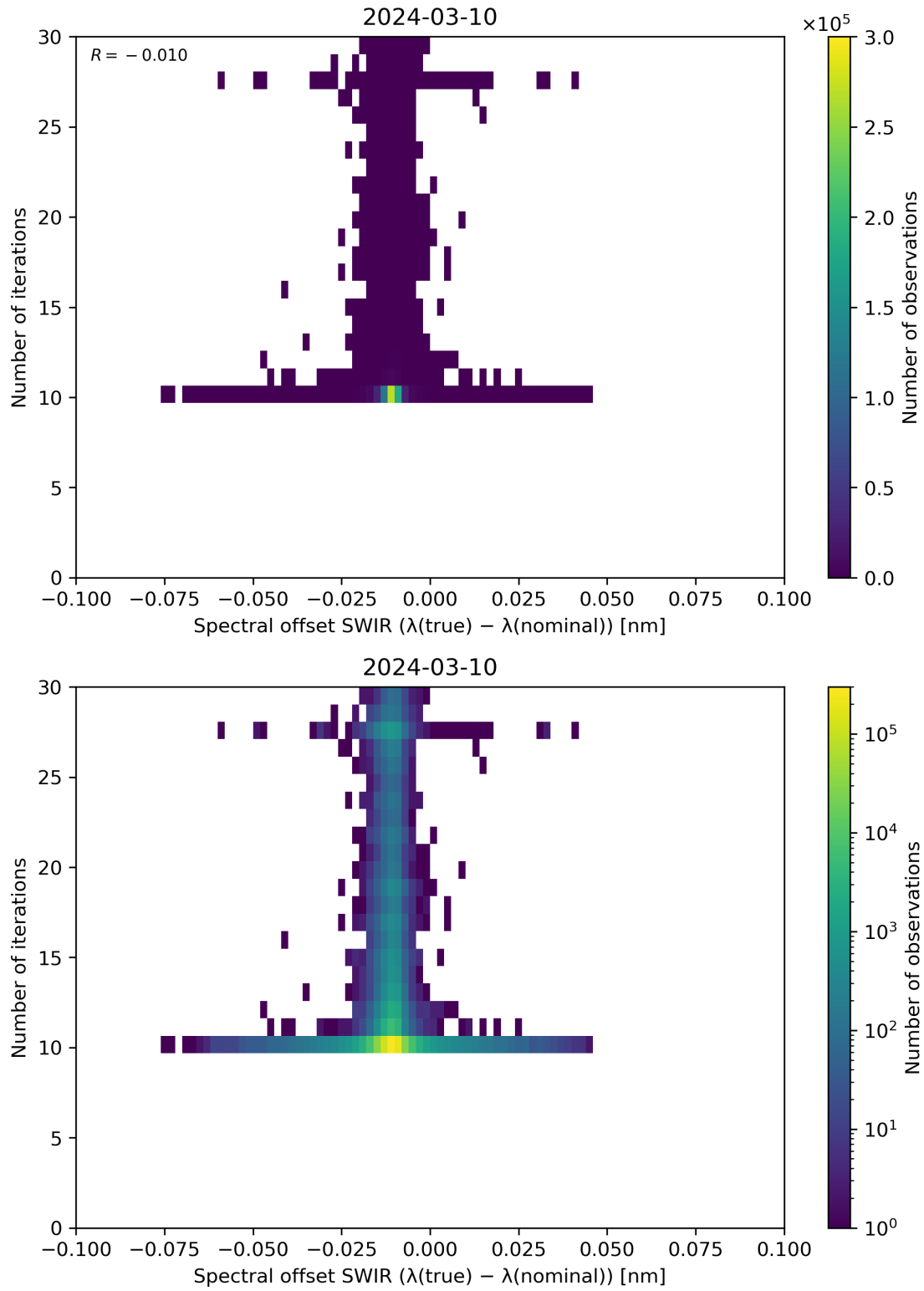
Figure 121: Scatter density plot of “Spectral offset SWIR ( \lambda(\text{true}) - \lambda(\text{nominal}) )” against “Number of iterations” for 2024-03-09 to 2024-03-11.
