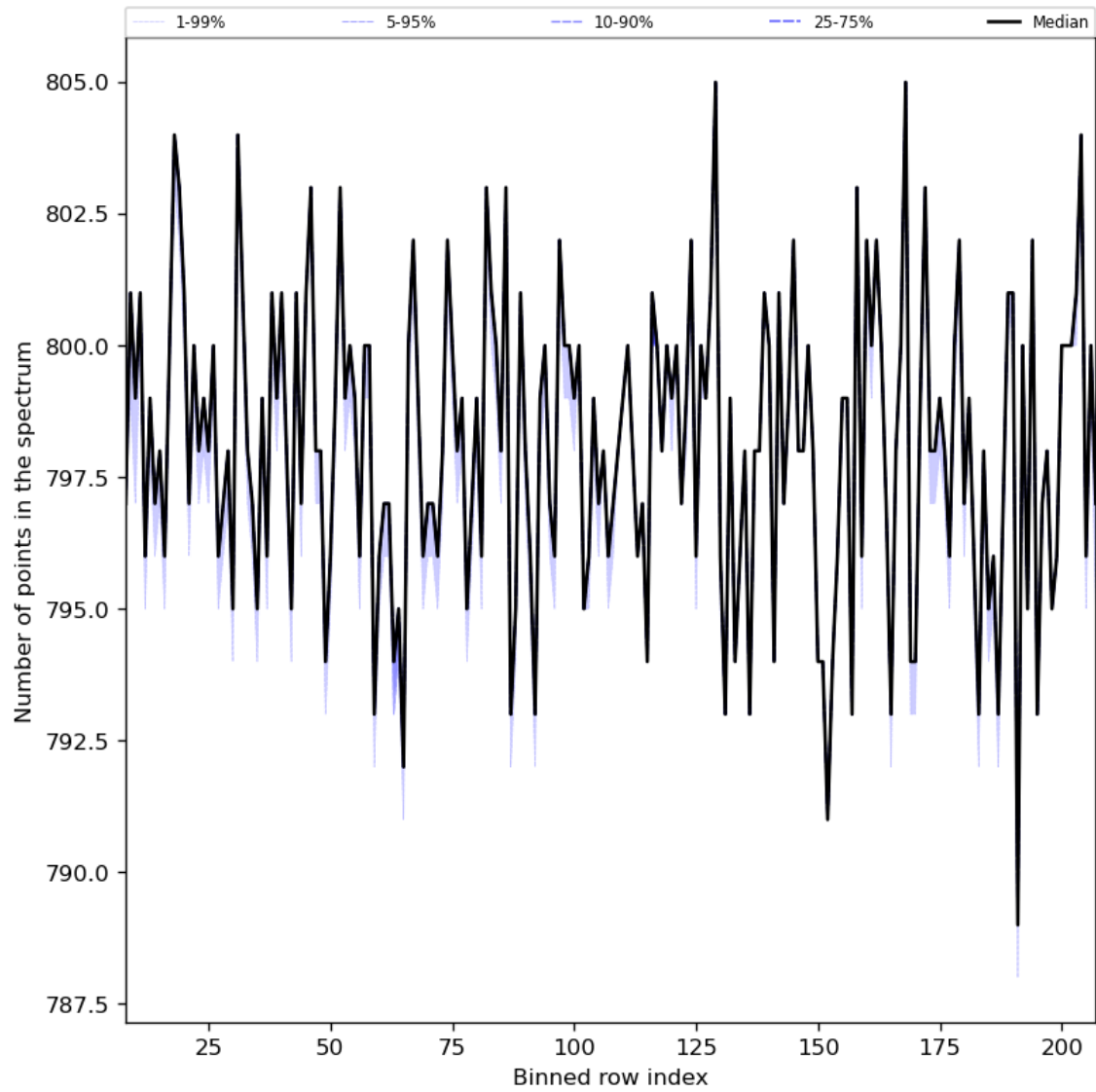
Figure 37: Along track statistics of “Number of points in the spectrum” for 2024-03-09 to 2024-03-11
