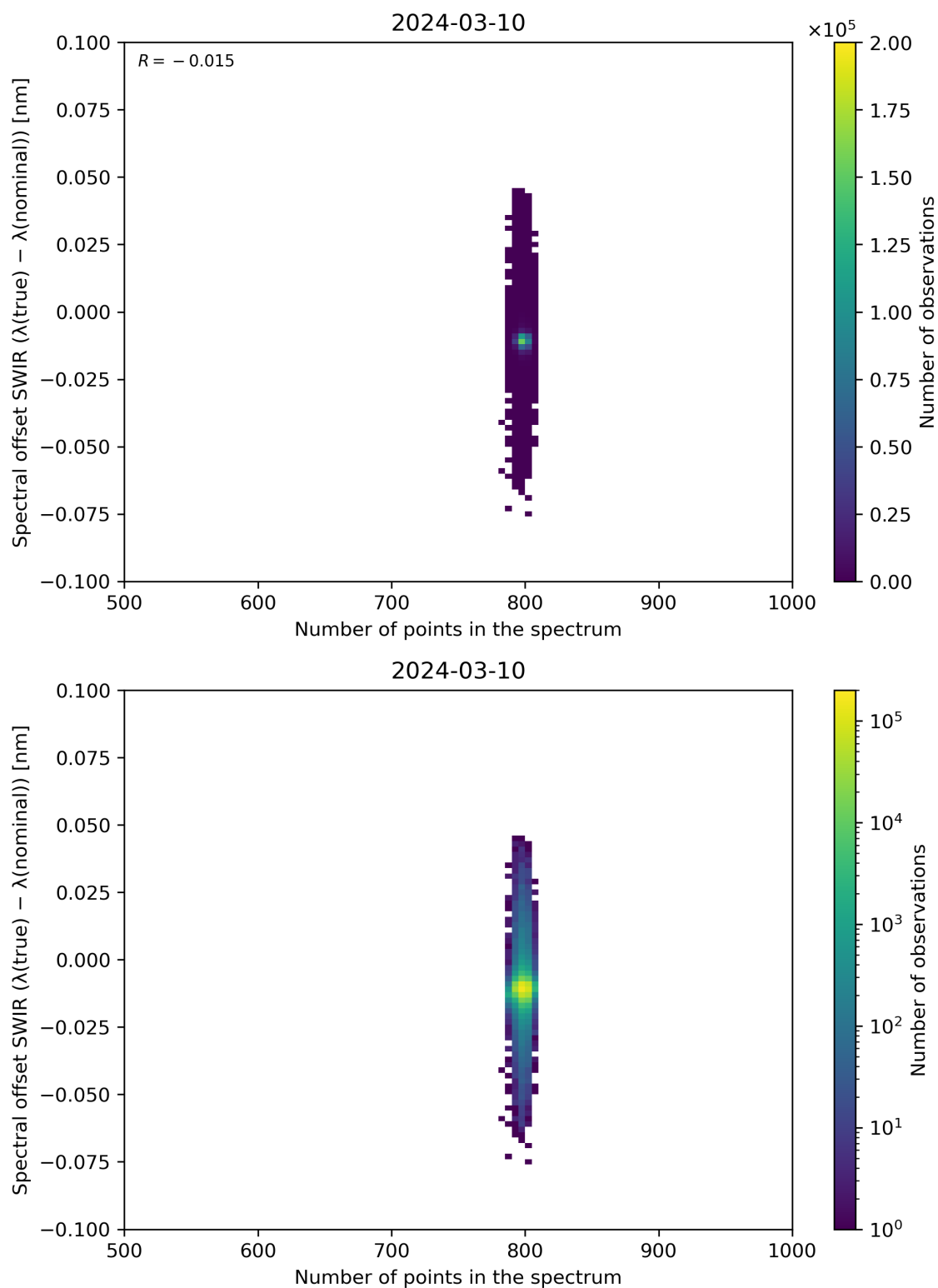
Figure 93: Scatter density plot of “Number of points in the spectrum” against “Spectral offset SWIR ( \lambda(\text{true}) - \lambda(\text{nominal}) )” for 2024-03-09 to 2024-03-11.
