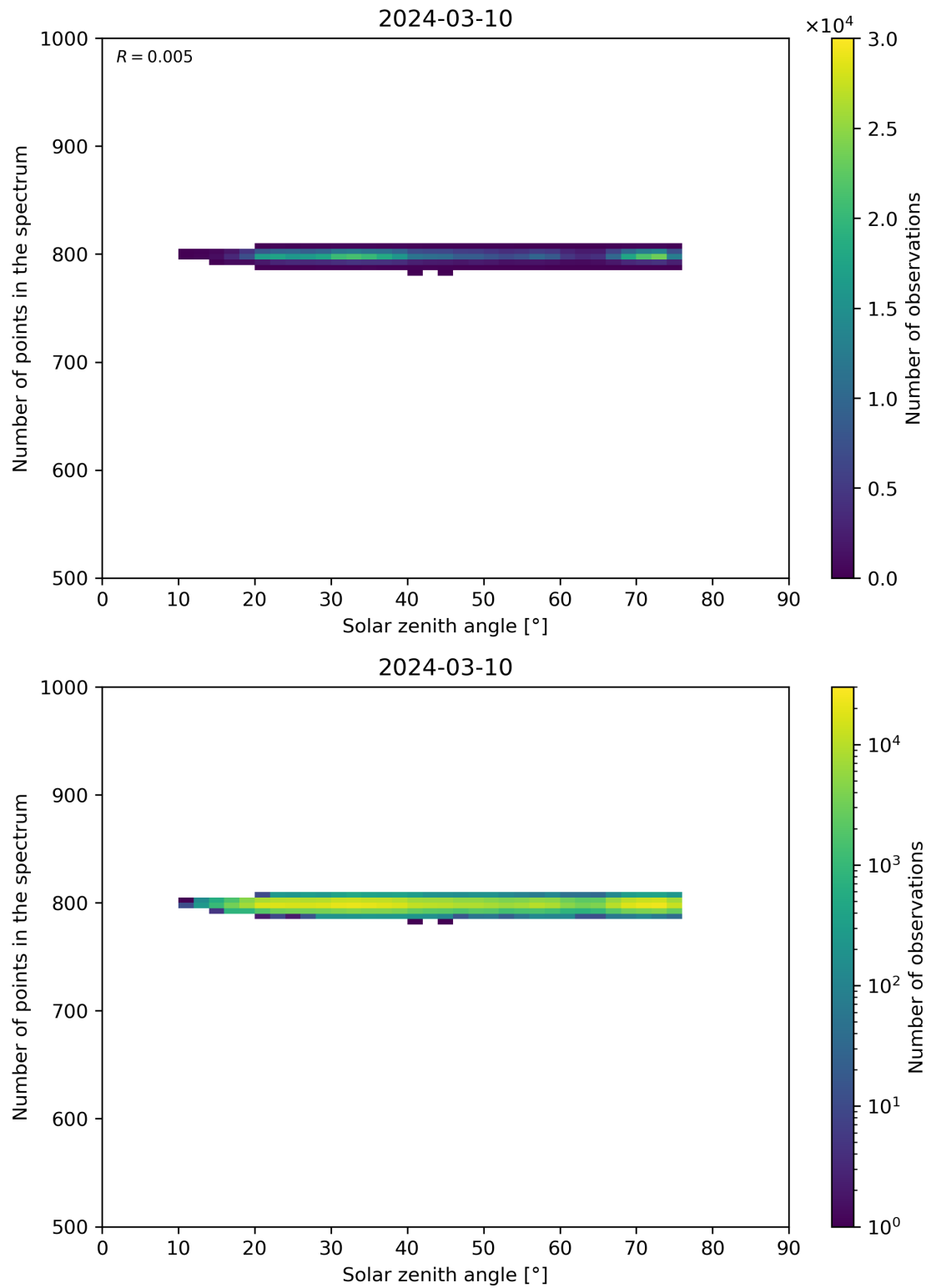
Figure 103: Scatter density plot of “Solar zenith angle” against “Number of points in the spectrum” for 2024-03-09 to 2024-03-11.
