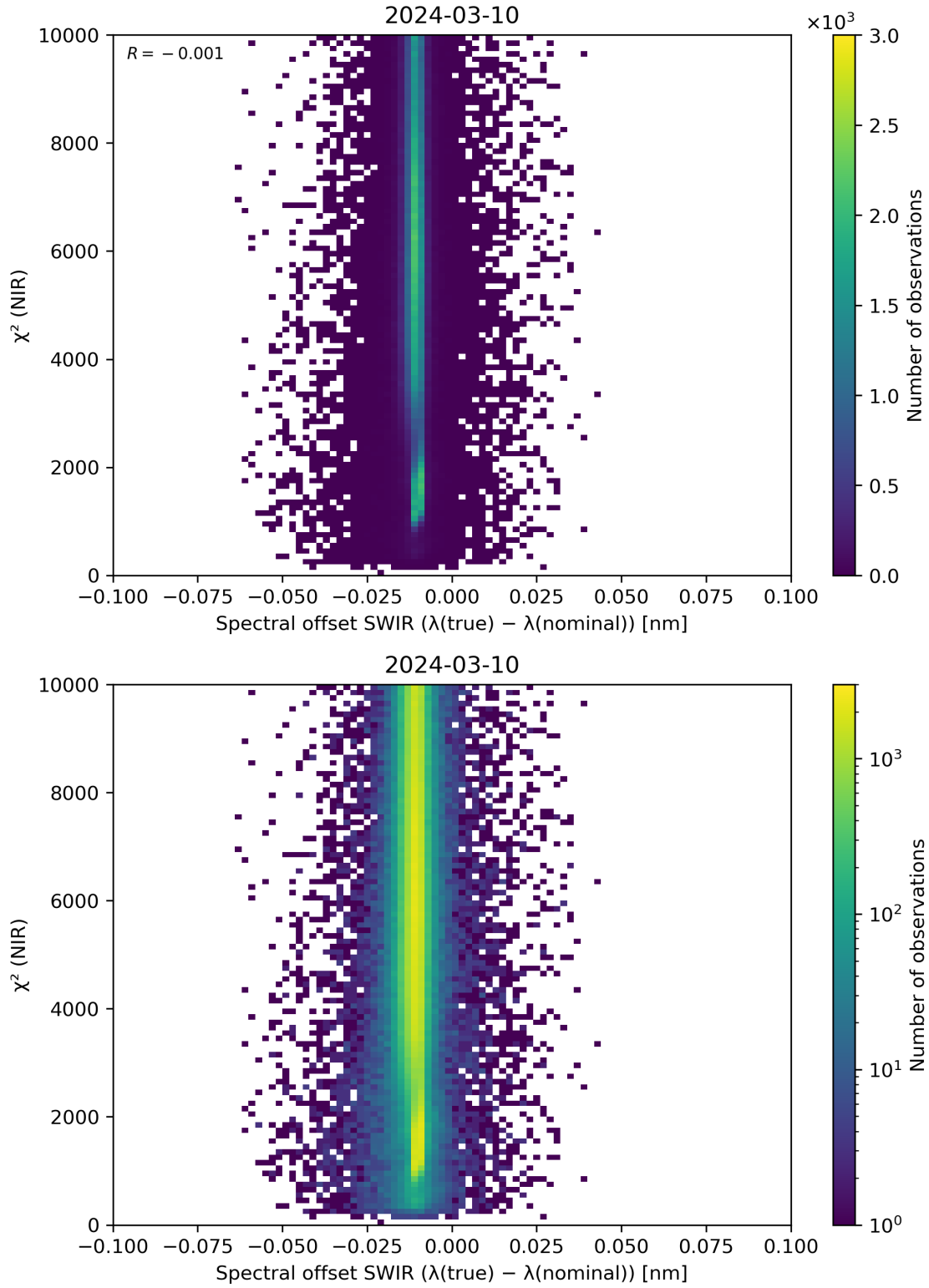
Figure 117: Scatter density plot of “Spectral offset SWIR ( \lambda(\text{true}) - \lambda(\text{nominal}) )” against “ \chi^2 (NIR)” for 2024-03-09 to 2024-03-11.
