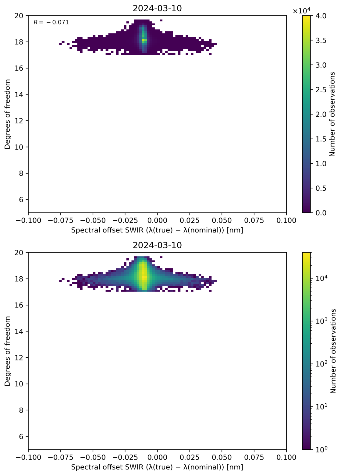
Figure 119: Scatter density plot of “Spectral offset SWIR ( \lambda(\text{true}) - \lambda(\text{nominal}) )” against “Degrees of freedom” for 2024-03-09 to 2024-03-11.
