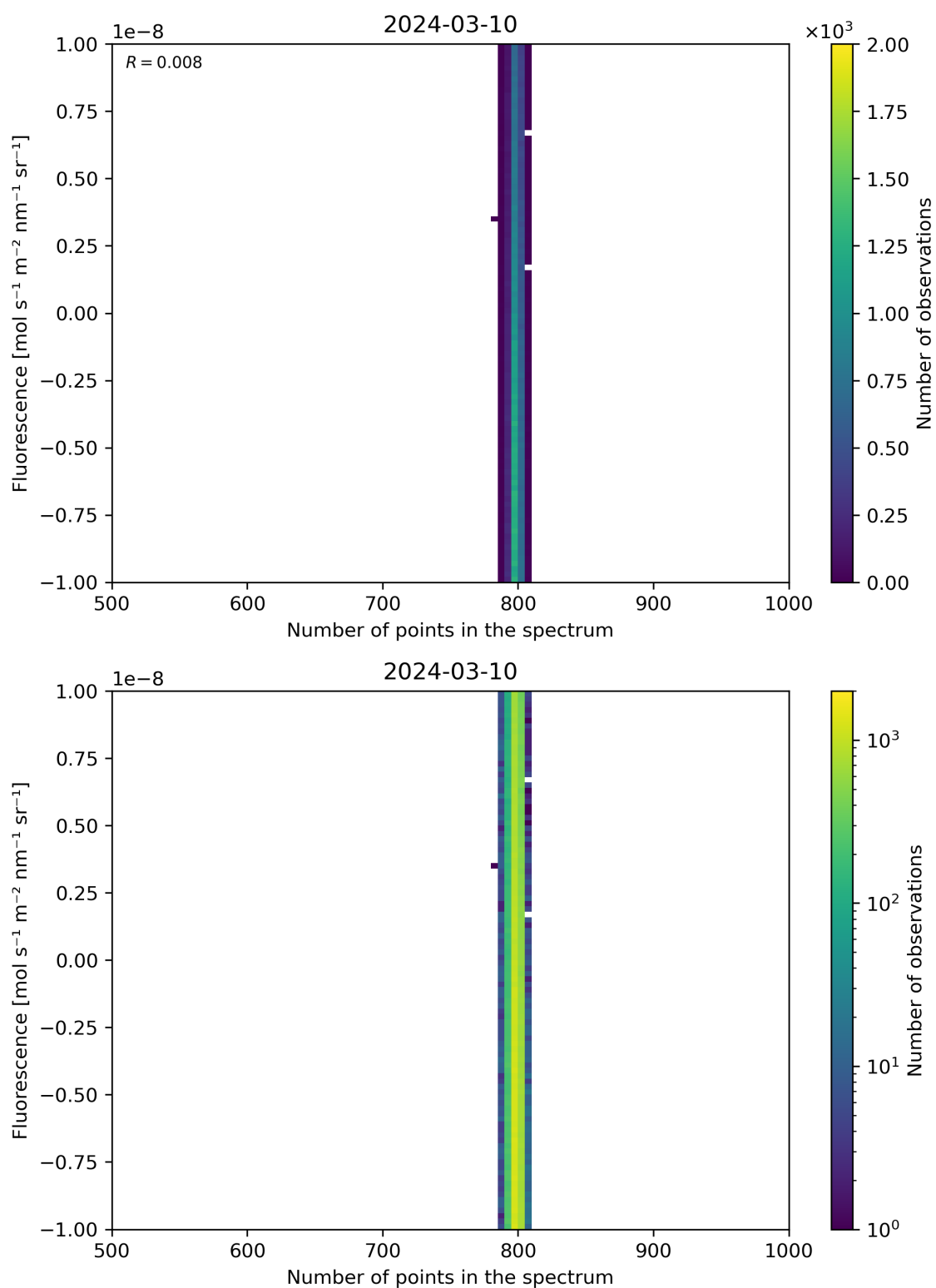
Figure 91: Scatter density plot of “Number of points in the spectrum” against “Fluorescence” for 2024-03-09 to 2024-03-11.
