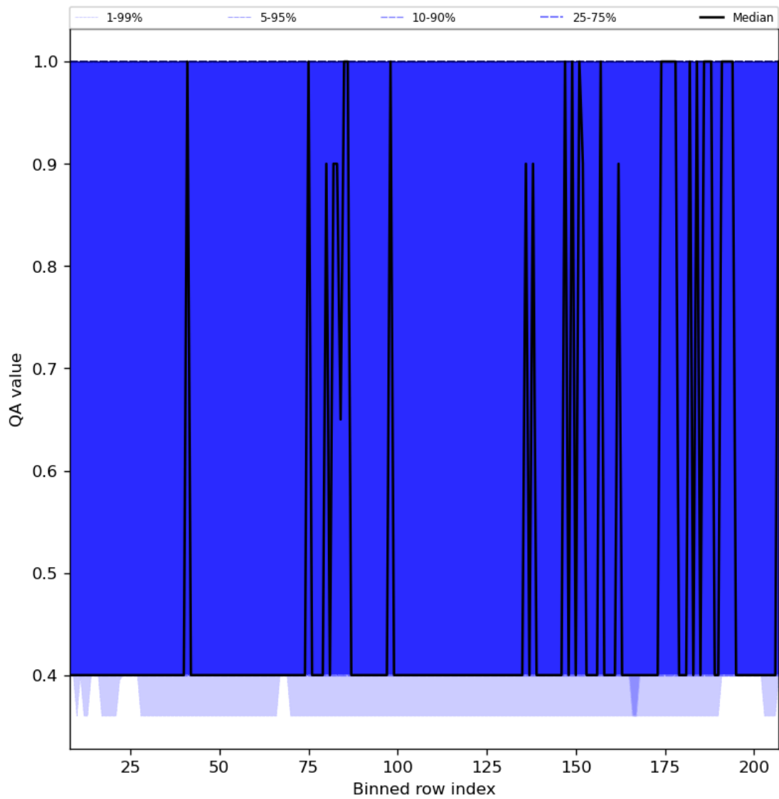
Figure 33: Along track statistics of "QA value" for 2024-03-09 to 2024-03-11
