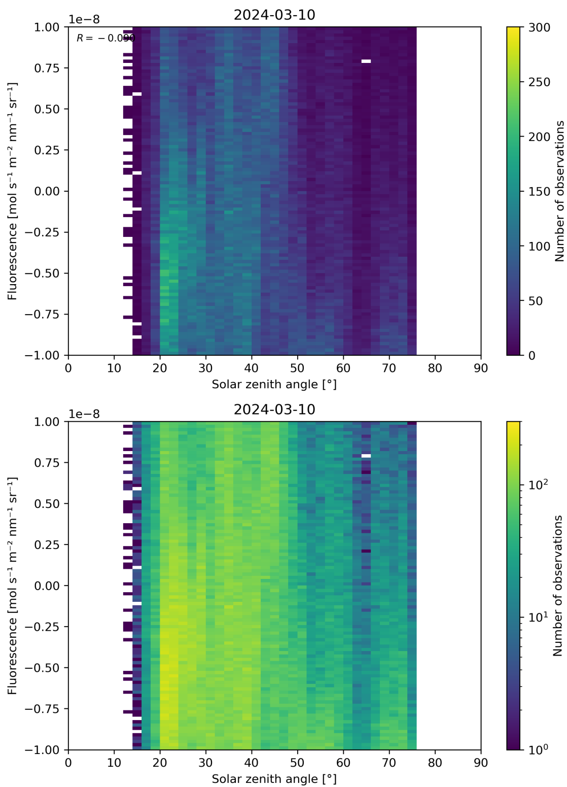
Figure 97: Scatter density plot of “Solar zenith angle” against “Fluorescence” for 2024-03-09 to 2024-03-11.
