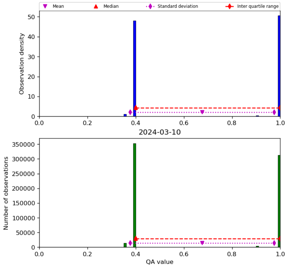
Figure 22: Histogram of “QA value” for 2024-03-09 to 2024-03-11
