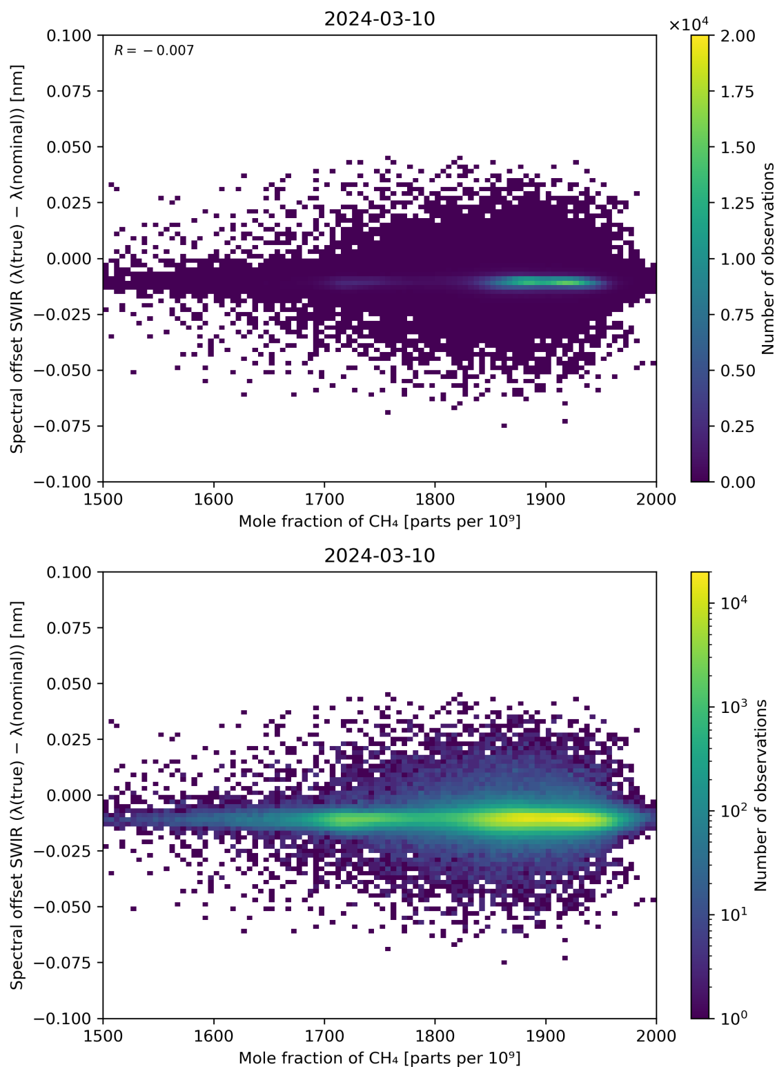
Figure 86: Scatter density plot of “Mole fraction of CH 4 ” against “Spectral offset SWIR ( \lambda(\text{true}) - \lambda(\text{nominal}) )” for 2024-03-09 to 2024-03-11.
