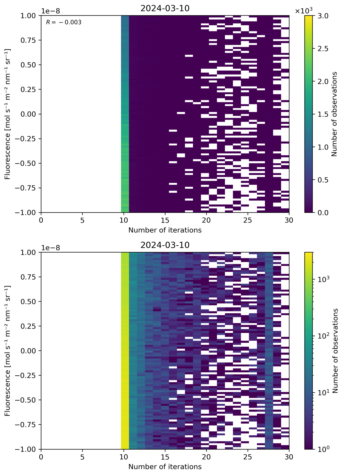
Figure 87: Scatter density plot of “Number of iterations” against “Fluorescence” for 2024-03-09 to 2024-03-11.
