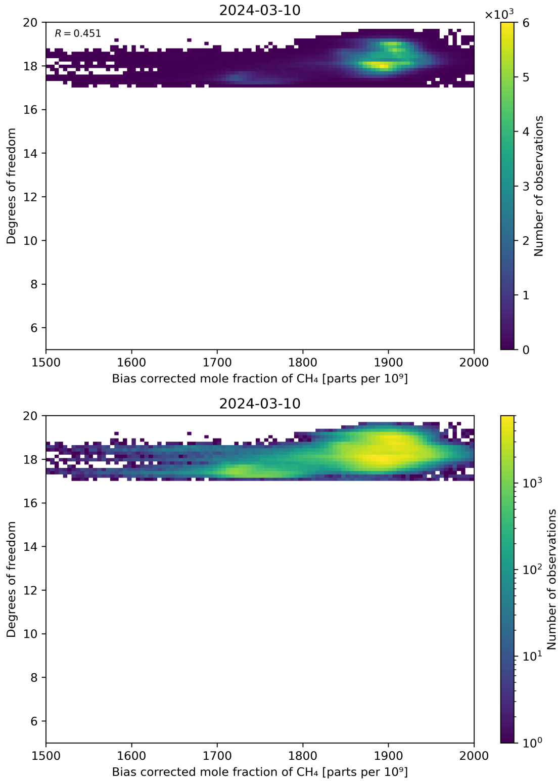
Figure 65: Scatter density plot of “Bias corrected mole fraction of CH 4 ” against “Degrees of freedom” for 2024-03-09 to 2024-03-11.
