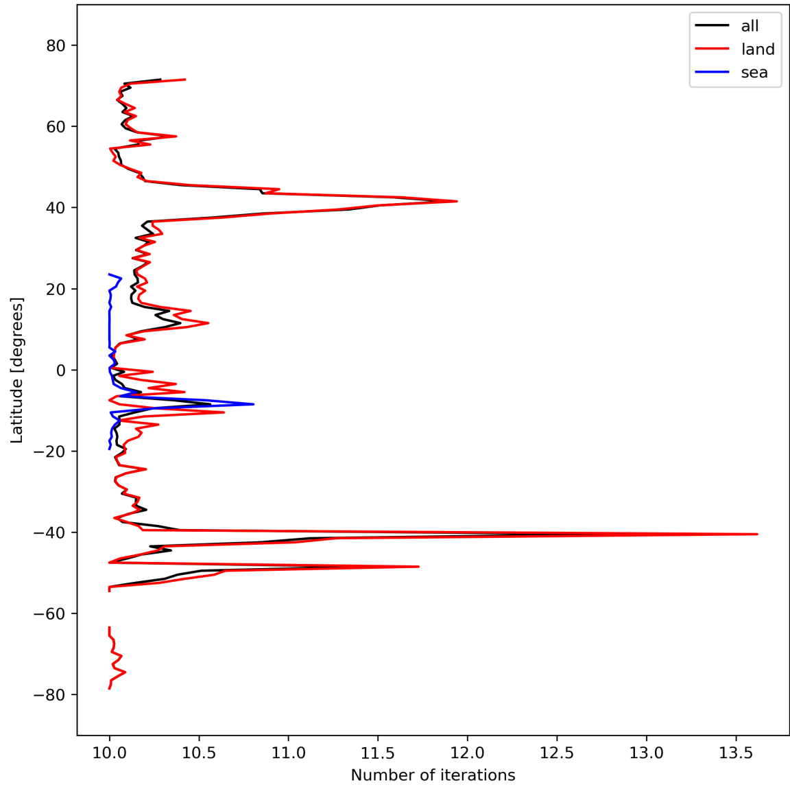
Figure 20: Zonal average of “Number of iterations” for 2024-03-09 to 2024-03-11.
