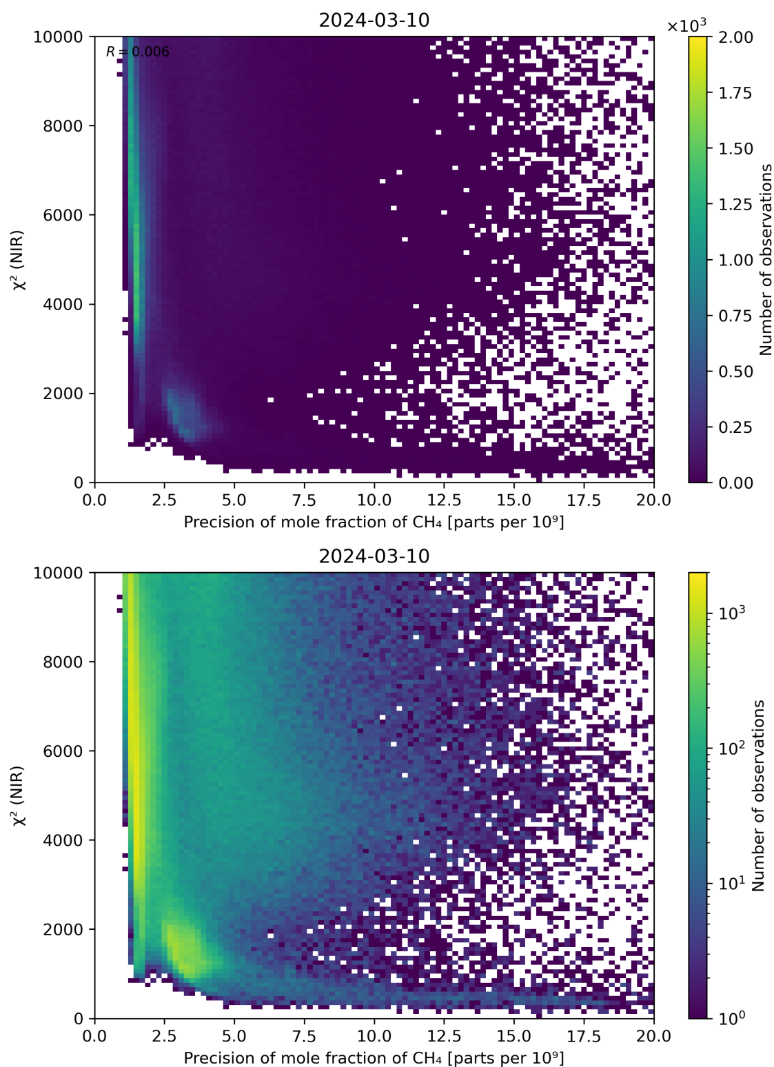
Figure 78: Scatter density plot of “Precision of mole fraction of CH 4 ” against “ \chi^2 (NIR)” for 2024-03-09 to 2024-03-11.
