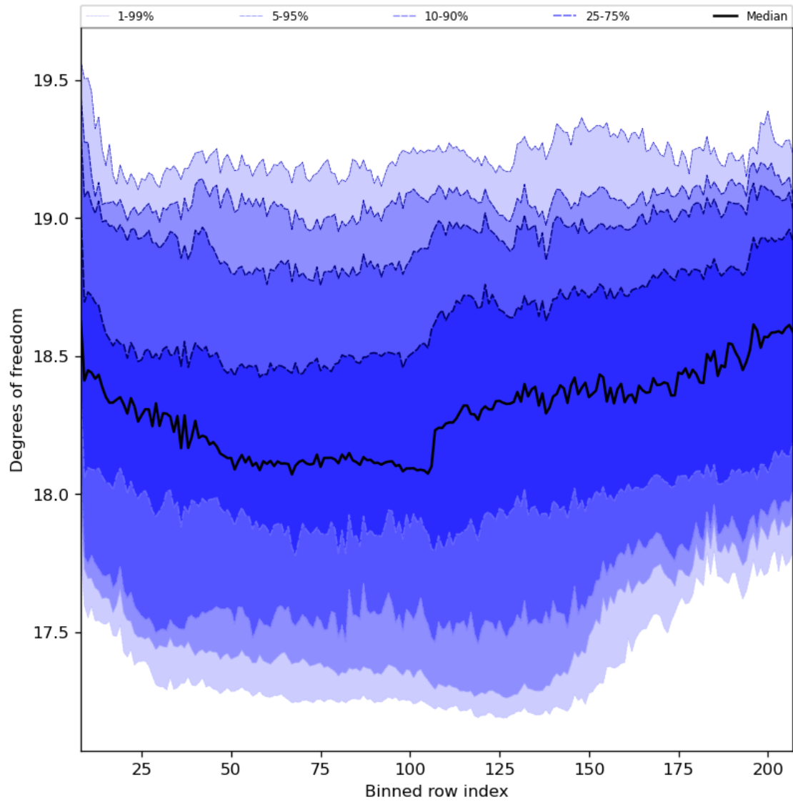
Figure 41: Along track statistics of “Degrees of freedom” for 2024-03-09 to 2024-03-11
