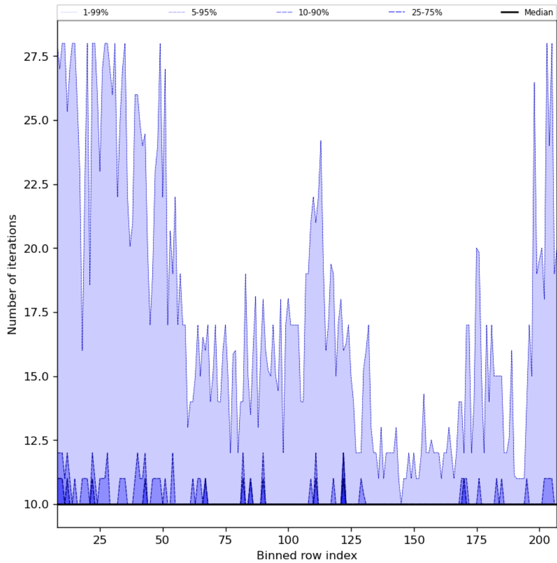
Figure 42: Along track statistics of “Number of iterations” for 2024-03-09 to 2024-03-11
