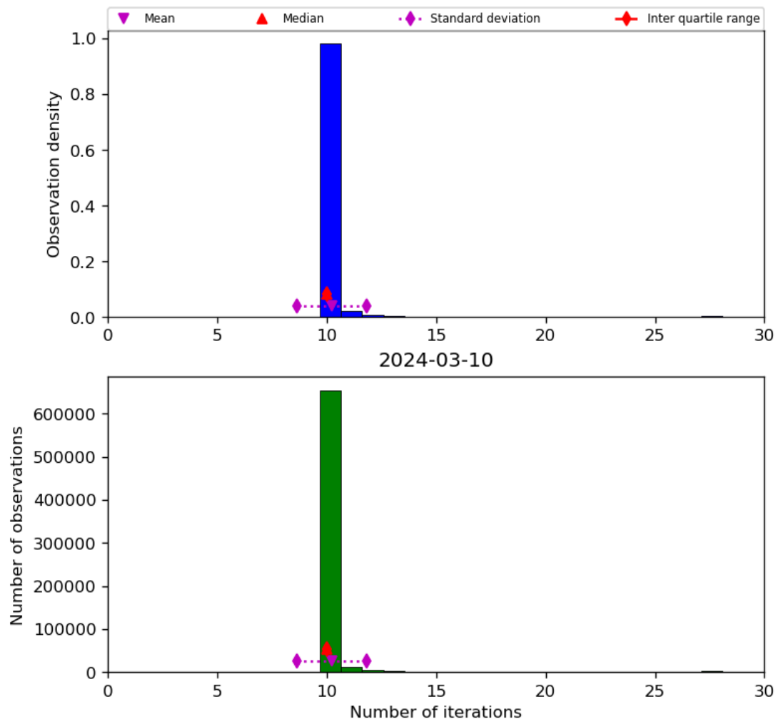
Figure 31: Histogram of “Number of iterations” for 2024-03-09 to 2024-03-11
