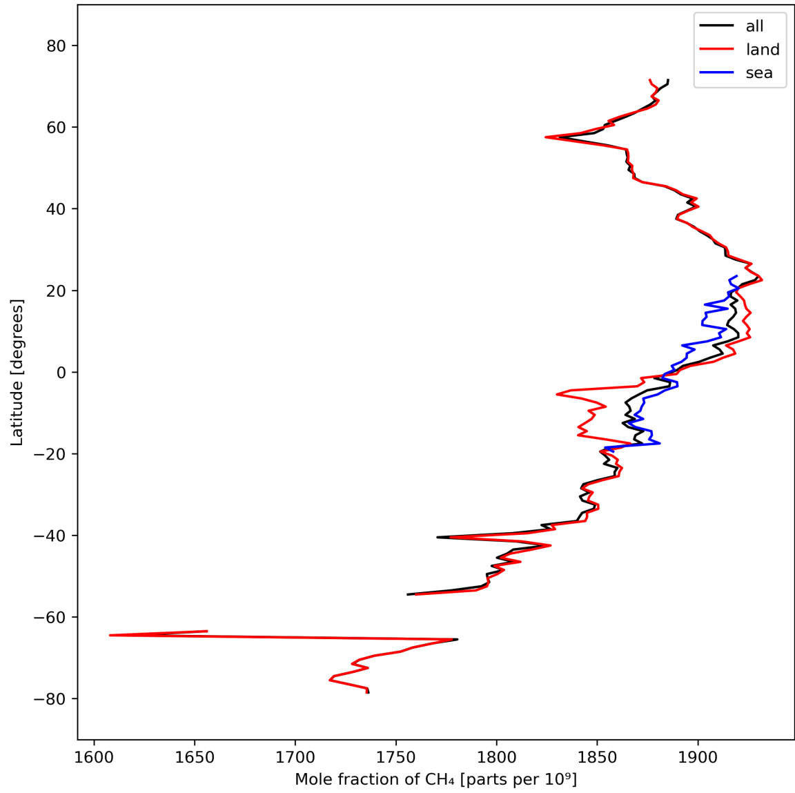
Figure 12: Zonal average of “Mole fraction of \text{CH}_4 ” for 2024-03-09 to 2024-03-11.
