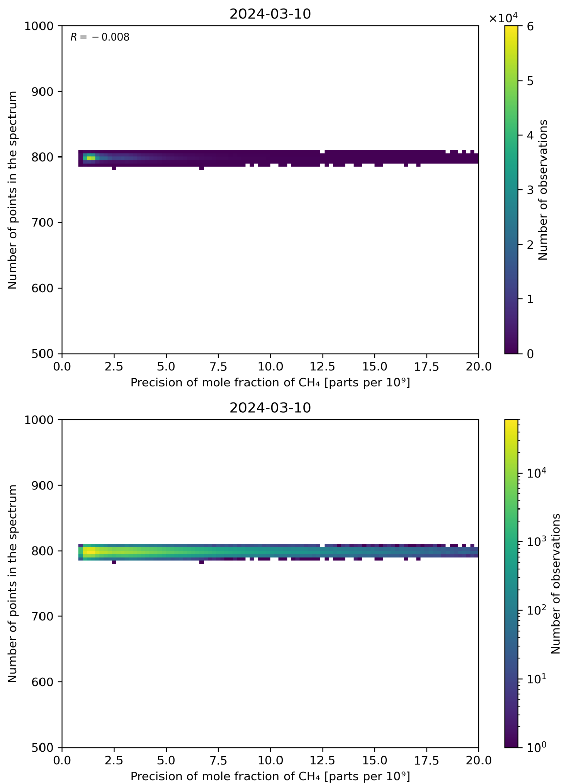
Figure 84: Scatter density plot of “Precision of mole fraction of CH 4 ” against “Number of points in the spectrum” for 2024-03-09 to 2024-03-11.
