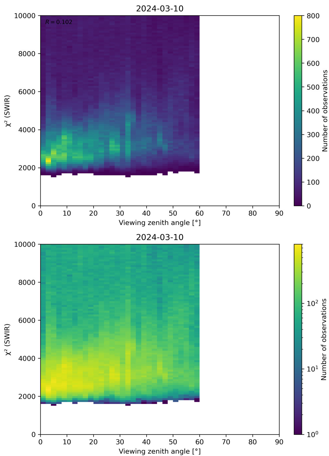
Figure 106: Scatter density plot of “Viewing zenith angle” against “ \chi^2 (SWIR)” for 2024-03-09 to 2024-03-11.
