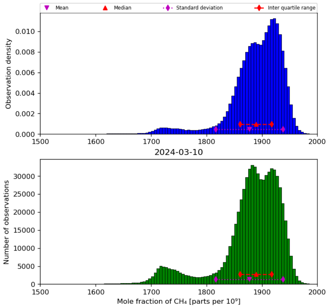
Figure 23: Histogram of “Mole fraction of CH 4 ” for 2024-03-09 to 2024-03-11
