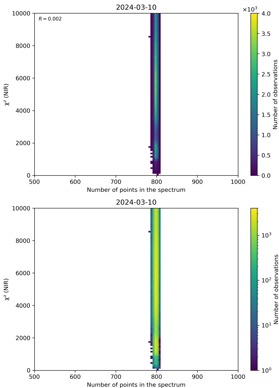
Figure 88: Scatter density plot of “Number of points in the spectrum” against “ \chi^2 (NIR)” for 2024-03-09 to 2024-03-11.
