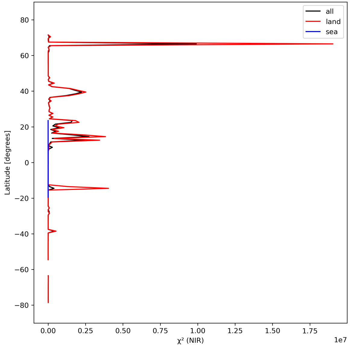
Figure 18: Zonal average of “ \chi^2 (NIR)” for 2024-03-09 to 2024-03-11.
