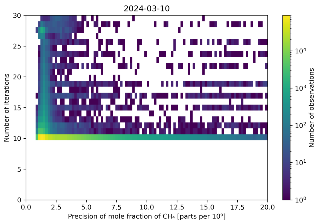
Figure 83: Scatter density plot of “Precision of mole fraction of CH 4 ” against “Number of iterations” for 2024-03-09 to 2024-03-11.
