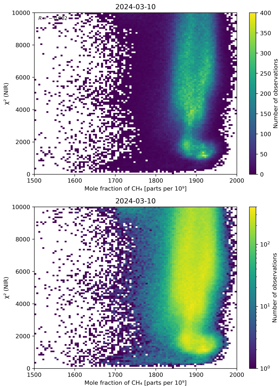
Figure 70: Scatter density plot of “Mole fraction of \text{CH}_4 ” against “ \chi^2 (NIR)” for 2024-03-09 to 2024-03-11.
