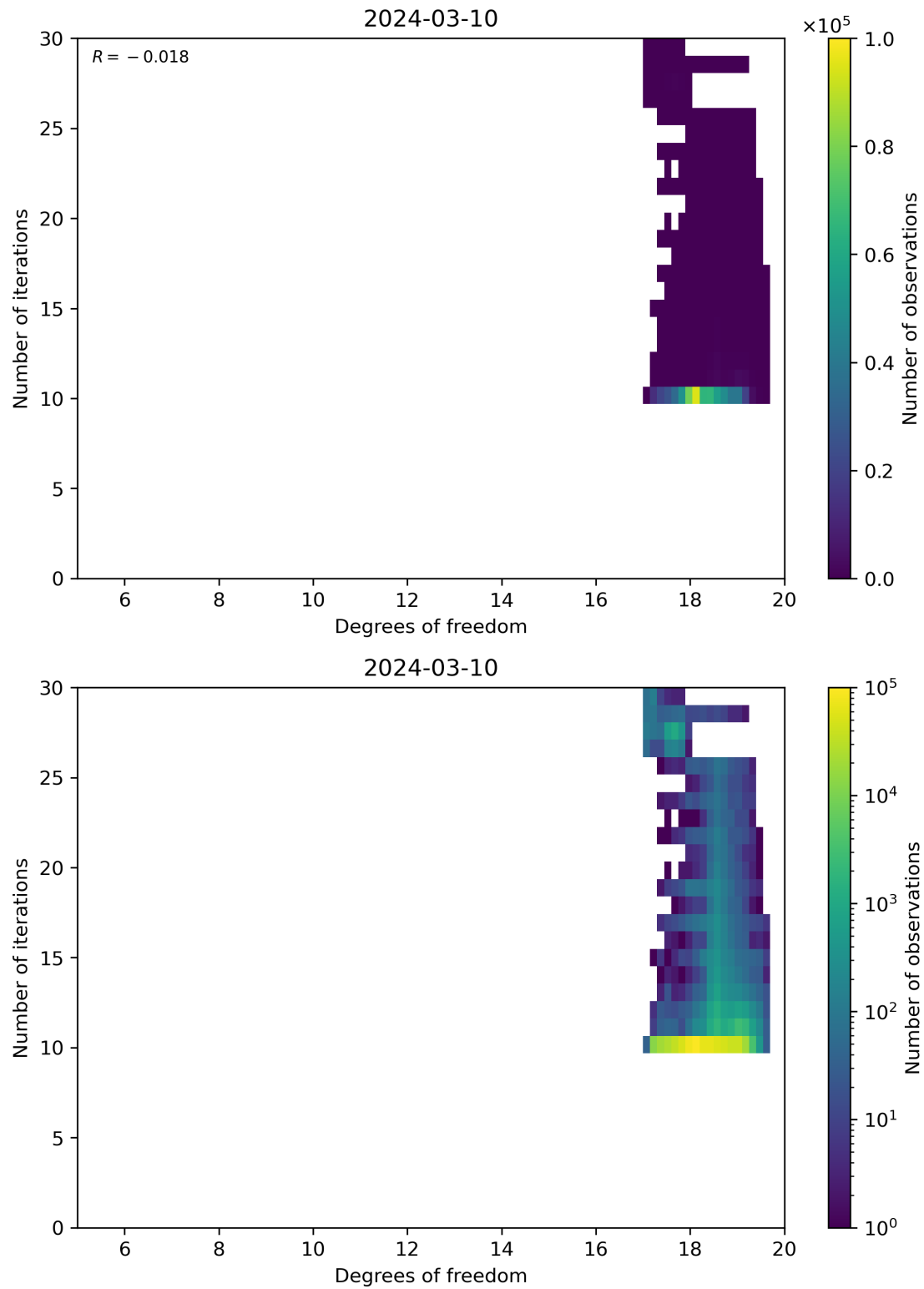
Figure 52: Scatter density plot of “Degrees of freedom” against “Number of iterations” for 2024-03-09 to 2024-03-11.
