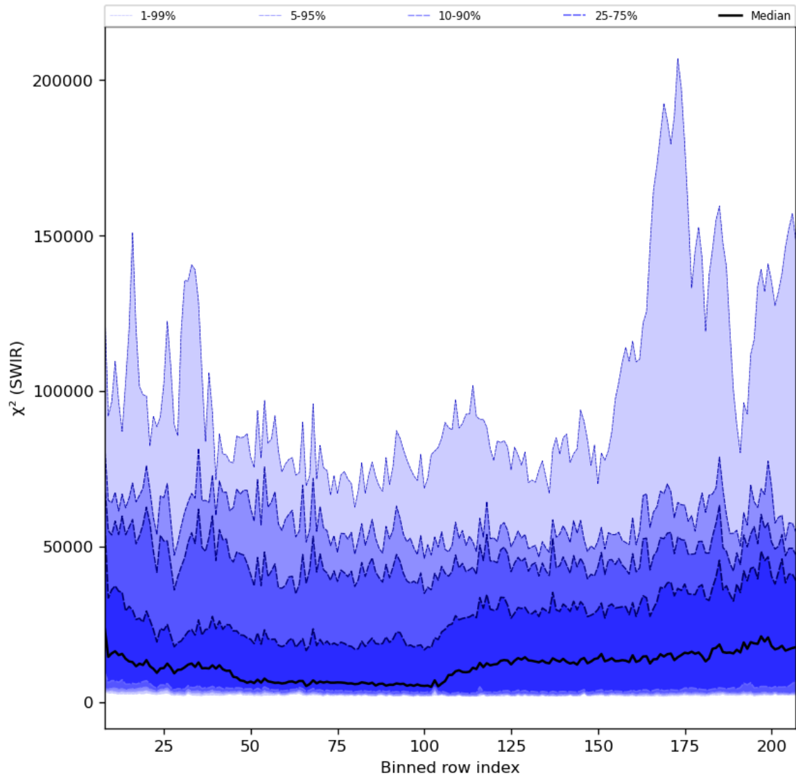
Figure 39: Along track statistics of " \chi^2 (SWIR)" for 2024-03-09 to 2024-03-11
