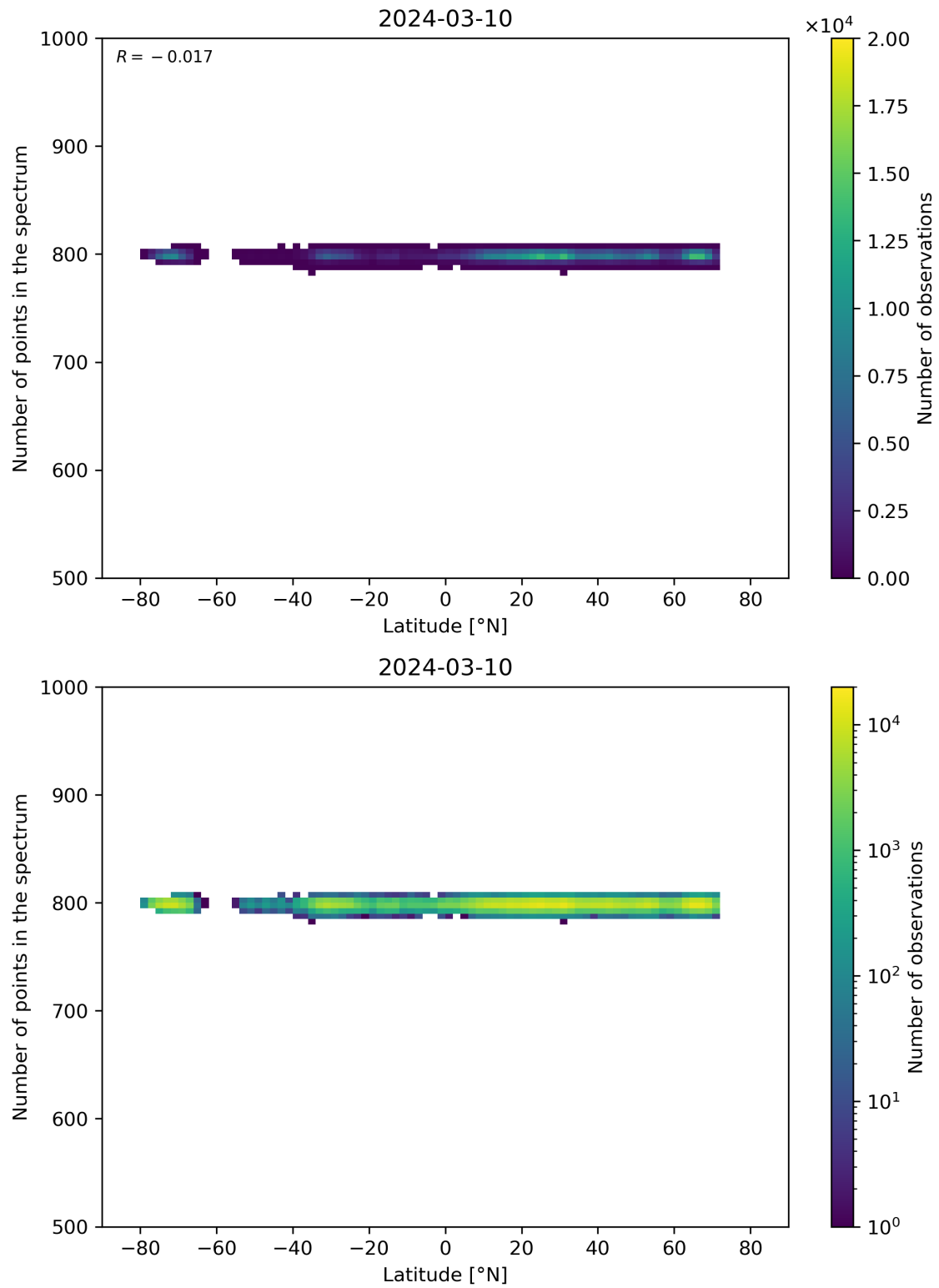
Figure 61: Scatter density plot of “Latitude” against “Number of points in the spectrum” for 2024-03-09 to 2024-03-11.
