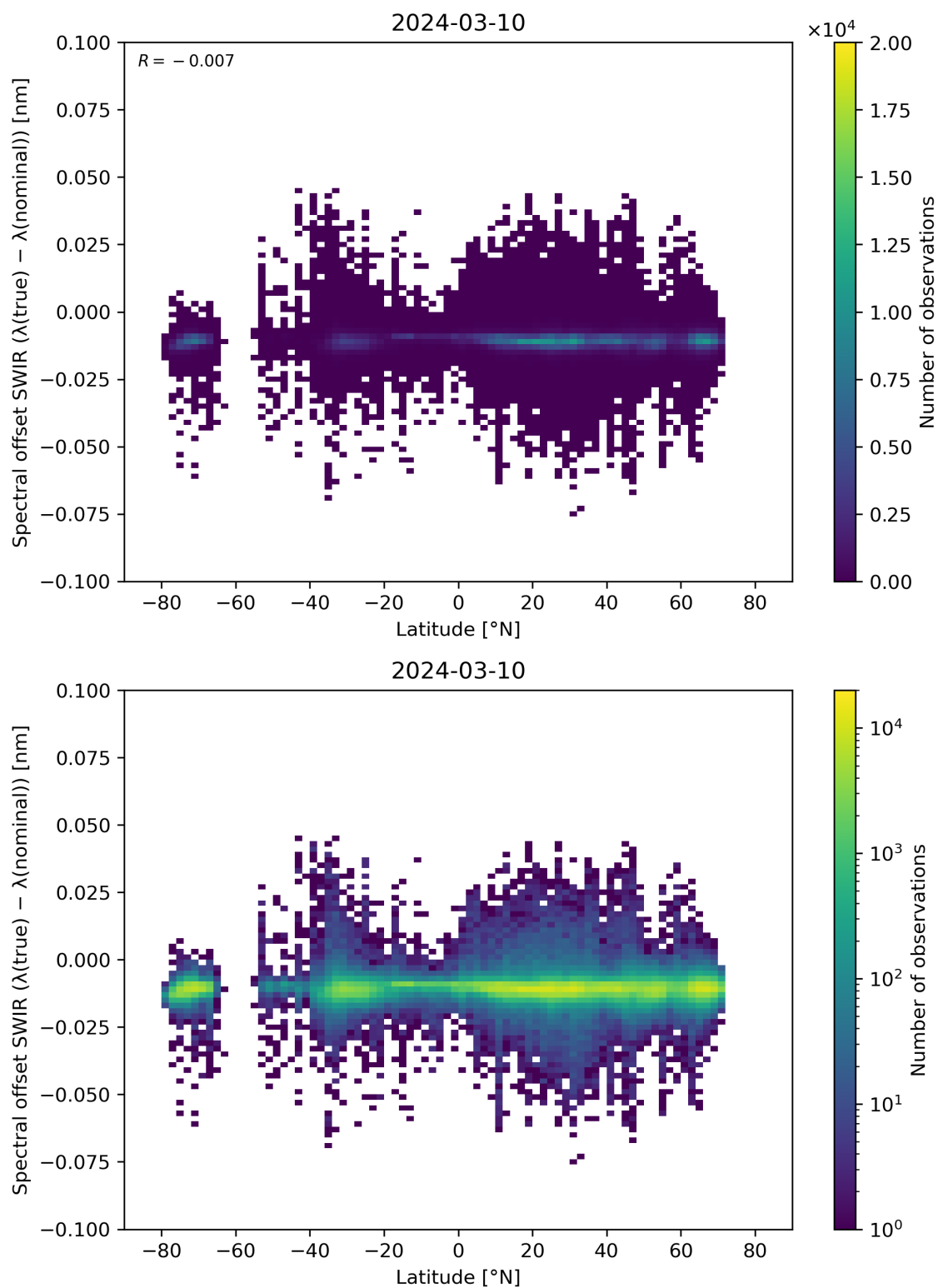
Figure 62: Scatter density plot of “Latitude” against “Spectral offset SWIR ( \lambda(\text{true}) - \lambda(\text{nominal}) )” for 2024-03-09 to 2024-03-11.
