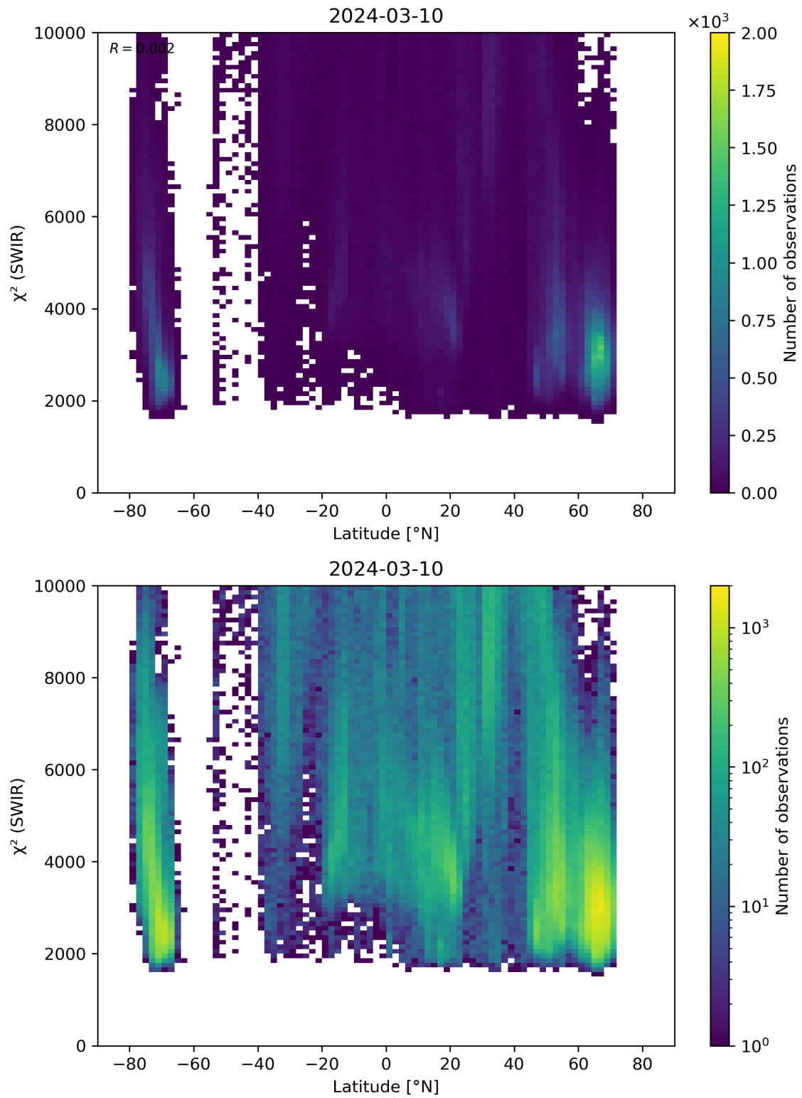
Figure 54: Scatter density plot of “Latitude” against “ \chi^2 (SWIR)” for 2024-03-09 to 2024-03-11.
