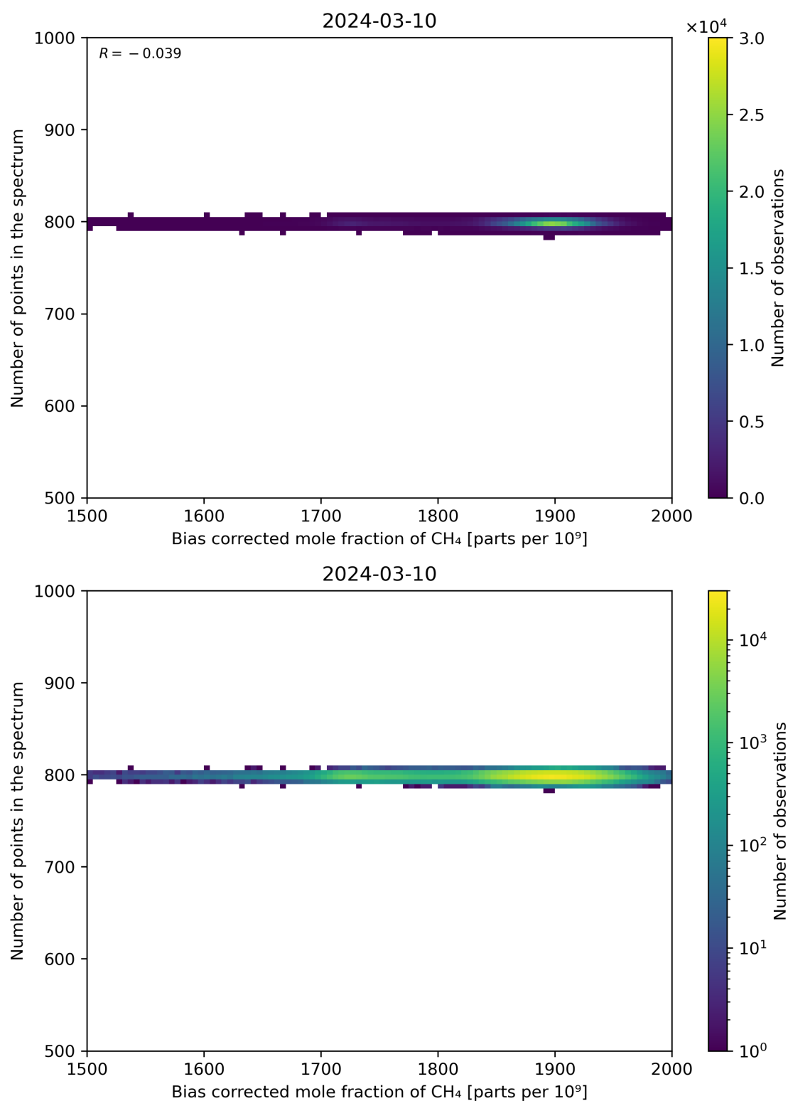
Figure 68: Scatter density plot of “Bias corrected mole fraction of CH 4 ” against “Number of points in the spectrum” for 2024-03-09 to 2024-03-11.
