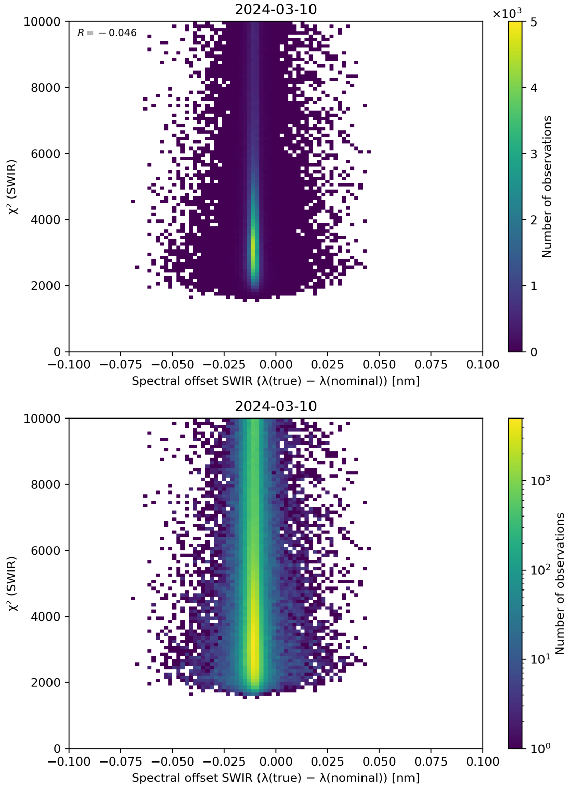
Figure 118: Scatter density plot of “Spectral offset SWIR ( \lambda(\text{true}) - \lambda(\text{nominal}) )” against “ \chi^2 (SWIR)” for 2024-03-09 to 2024-03-11.
