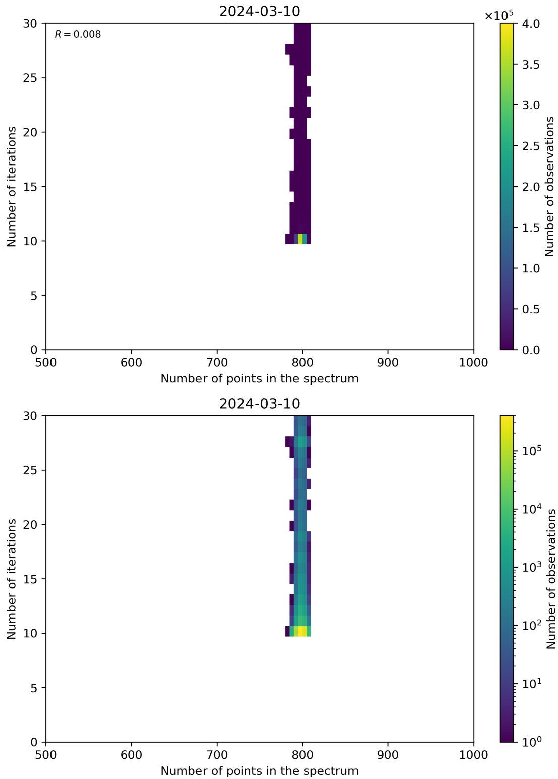
Figure 92: Scatter density plot of “Number of points in the spectrum” against “Number of iterations” for 2024-03-09 to 2024-03-11.
