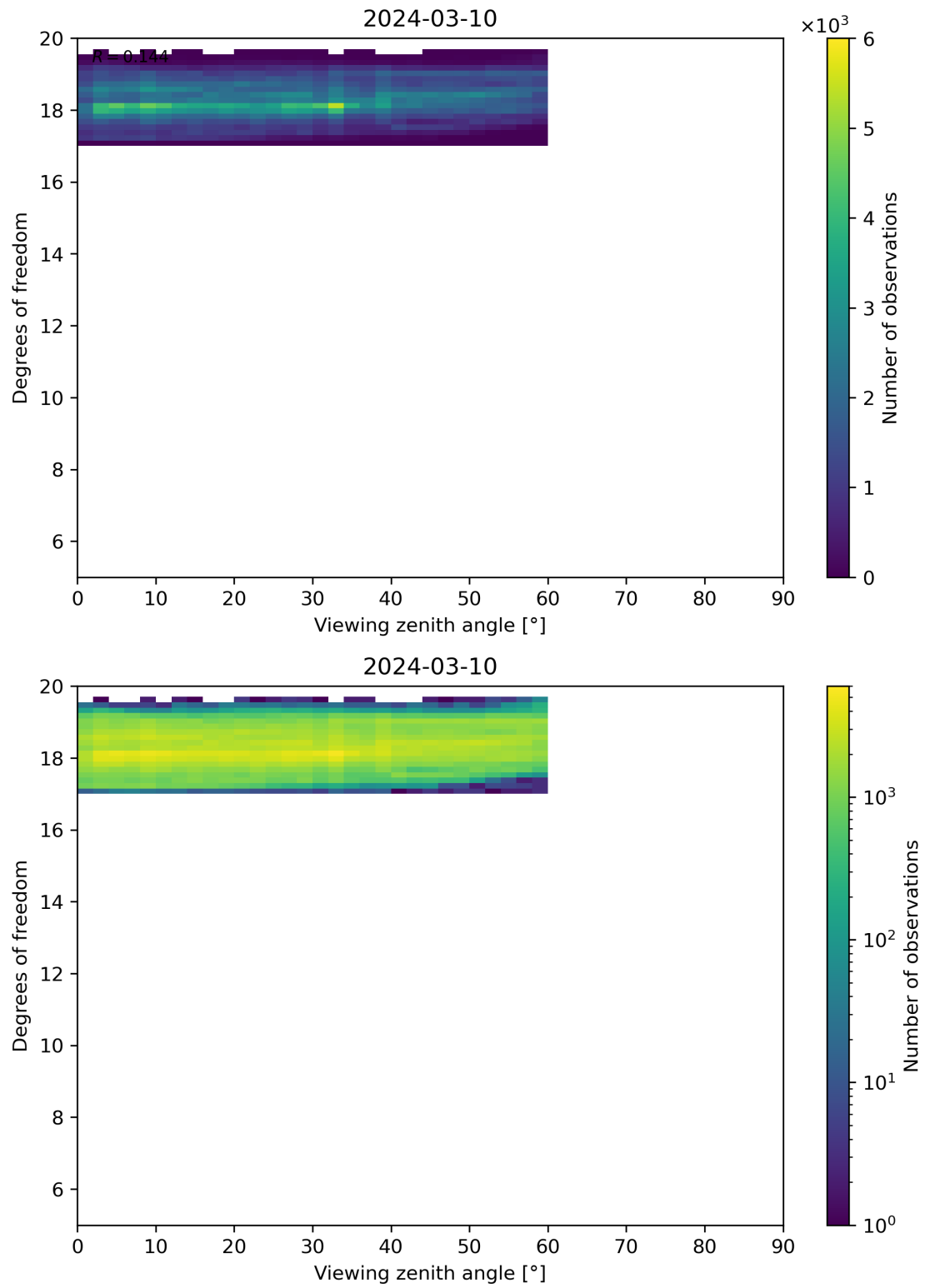
Figure 107: Scatter density plot of “Viewing zenith angle” against “Degrees of freedom” for 2024-03-09 to 2024-03-11.
