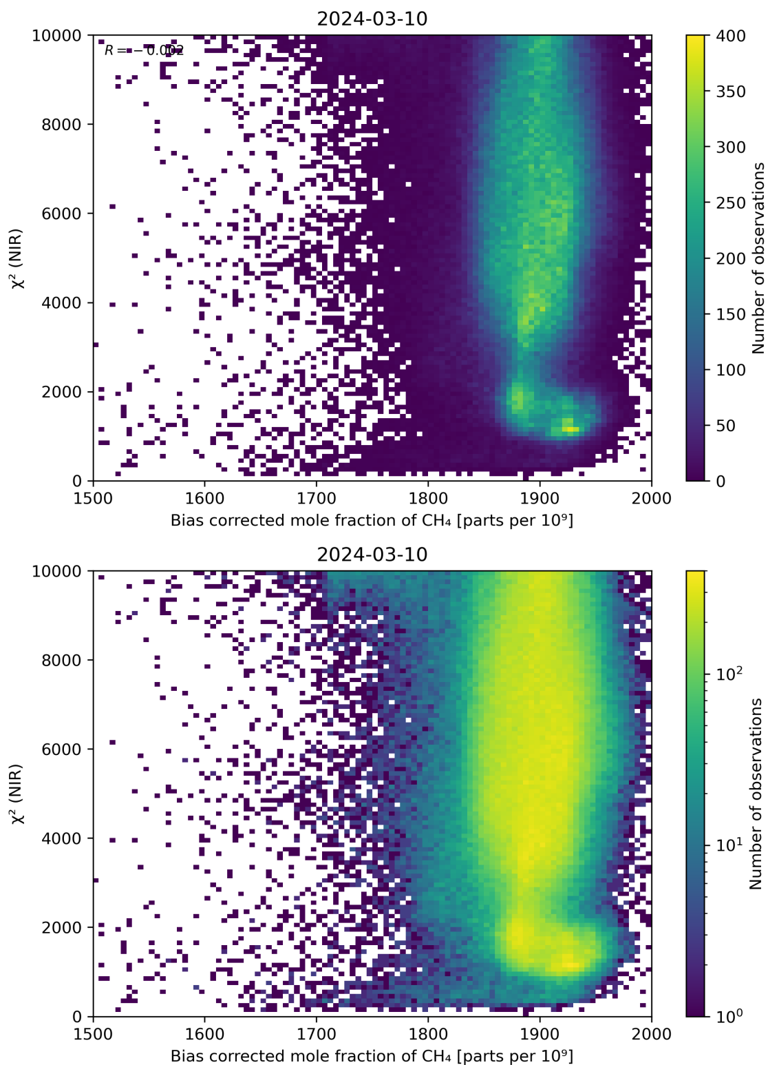
Figure 63: Scatter density plot of “Bias corrected mole fraction of \text{CH}_4 ” against “ \chi^2 (NIR)” for 2024-03-09 to 2024-03-11.
