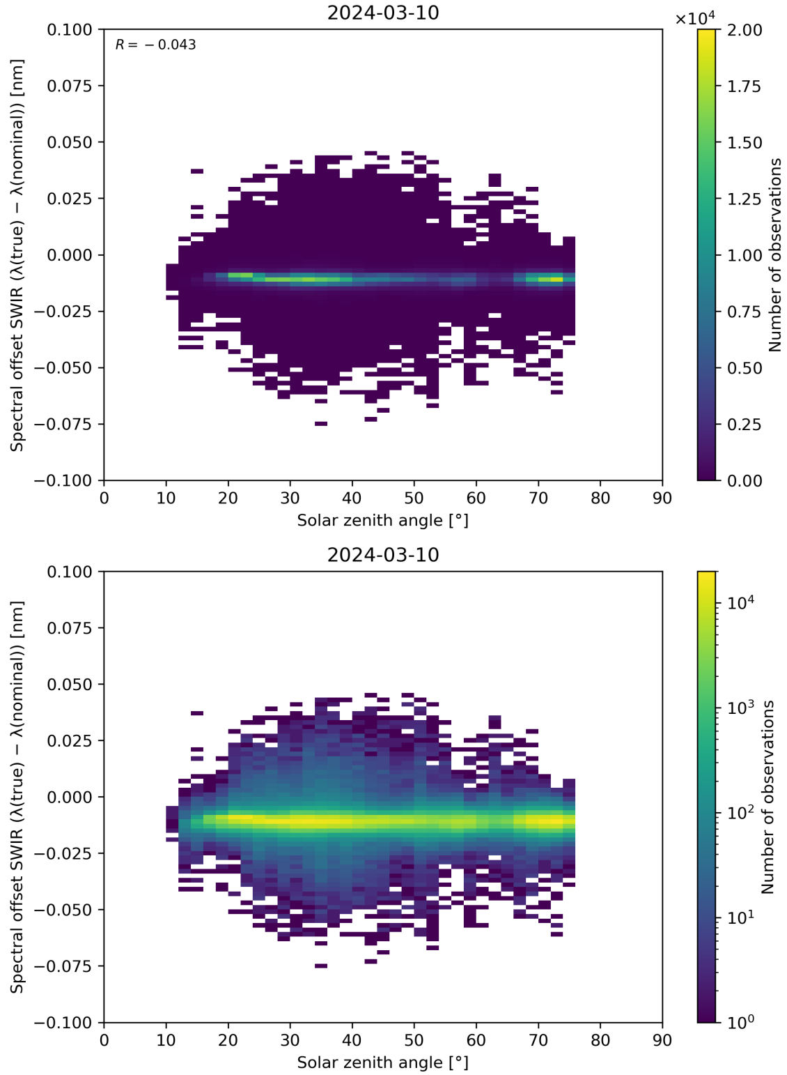
Figure 104: Scatter density plot of “Solar zenith angle” against “Spectral offset SWIR ( \lambda(\text{true}) - \lambda(\text{nominal}) )” for 2024-03-09 to 2024-03-11.
