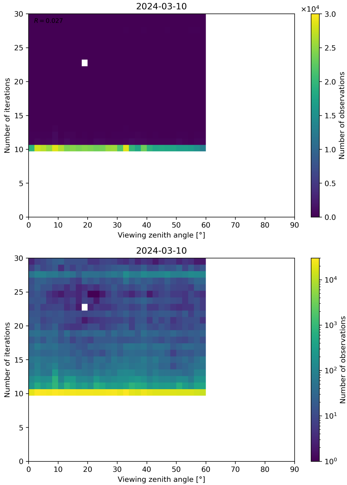
Figure 113: Scatter density plot of “Viewing zenith angle” against “Number of iterations” for 2024-03-09 to 2024-03-11.
