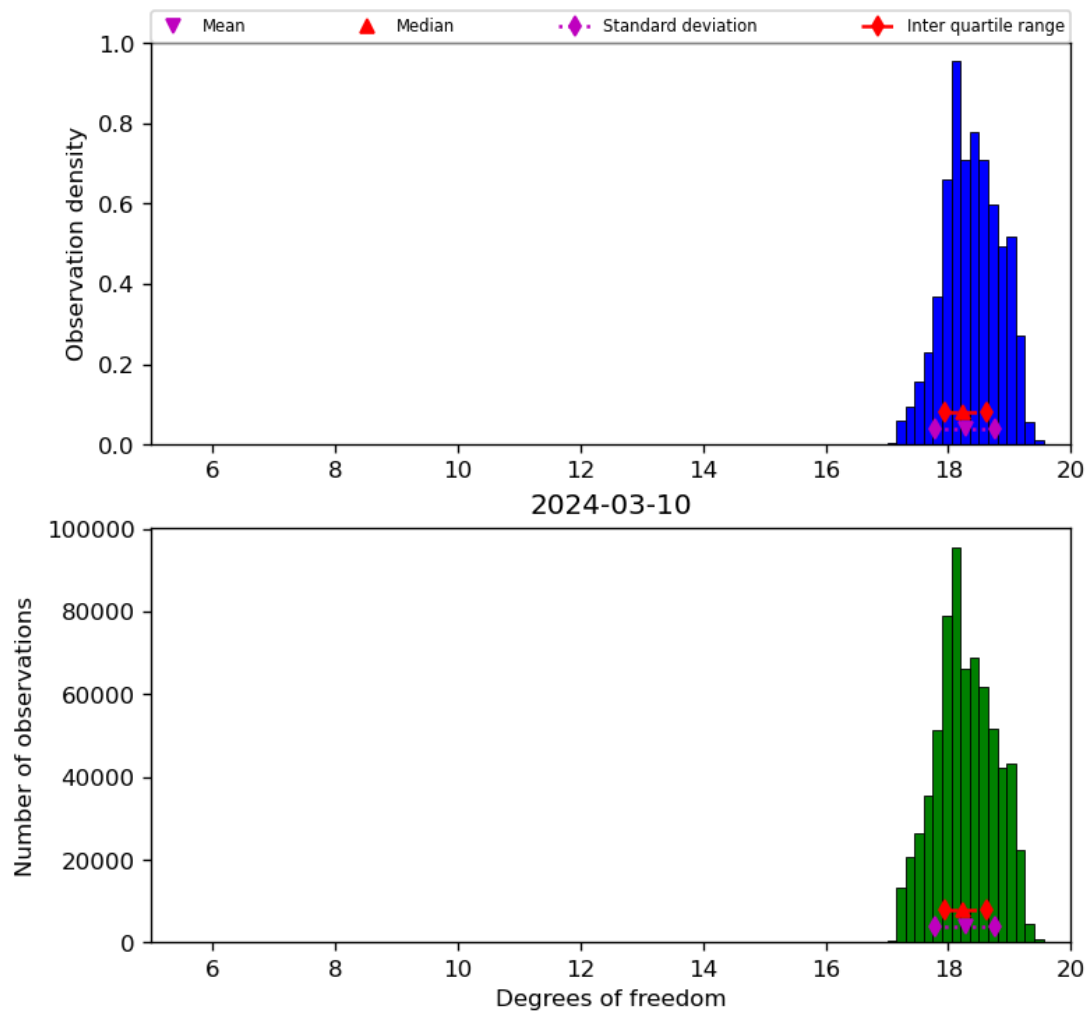
Figure 30: Histogram of “Degrees of freedom” for 2024-03-09 to 2024-03-11
