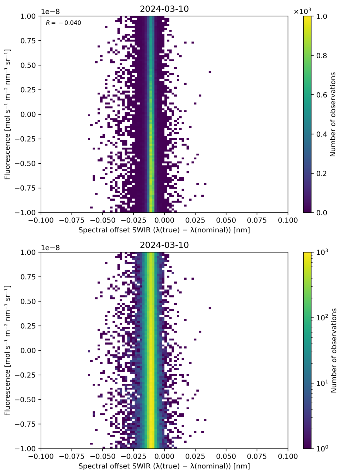
Figure 120: Scatter density plot of “Spectral offset SWIR ( \lambda(\text{true}) - \lambda(\text{nominal}) )” against “Fluorescence” for 2024-03-09 to 2024-03-11.
