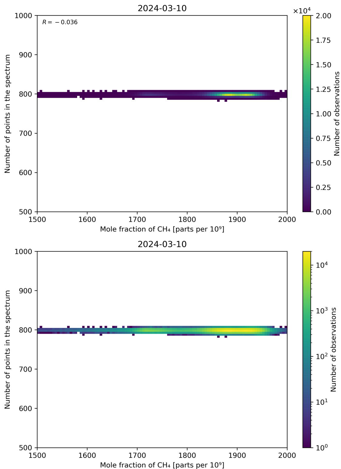
Figure 77: Scatter density plot of “Mole fraction of CH 4 ” against “Number of points in the spectrum” for 2024-03-09 to 2024-03-11.
