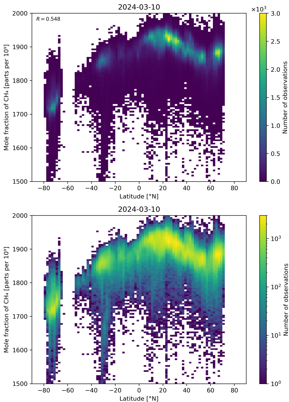
Figure 57: Scatter density plot of “Latitude” against “Mole fraction of CH 4 ” for 2024-03-09 to 2024-03-11.
