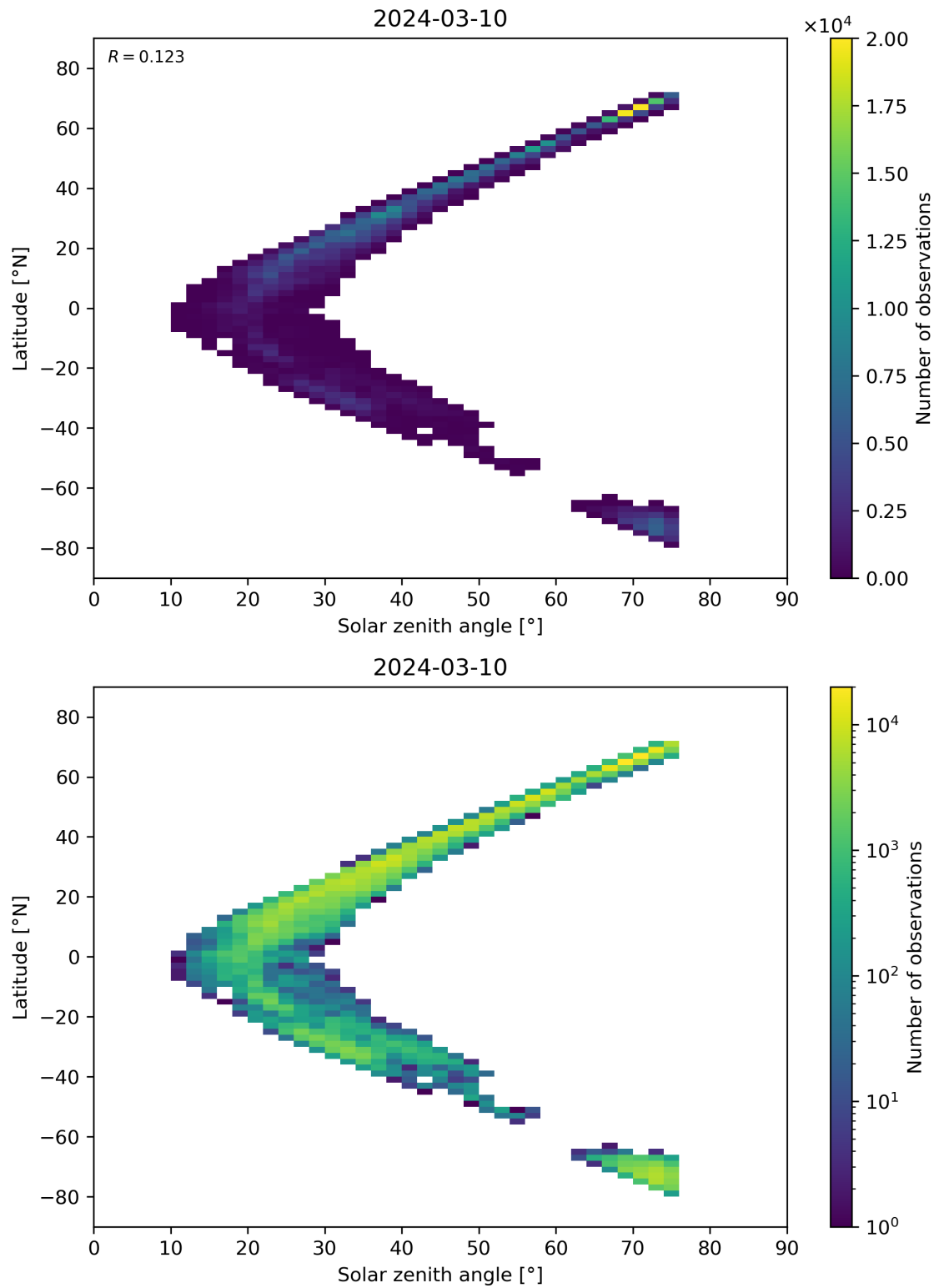
Figure 98: Scatter density plot of “Solar zenith angle” against “Latitude” for 2024-03-09 to 2024-03-11.
