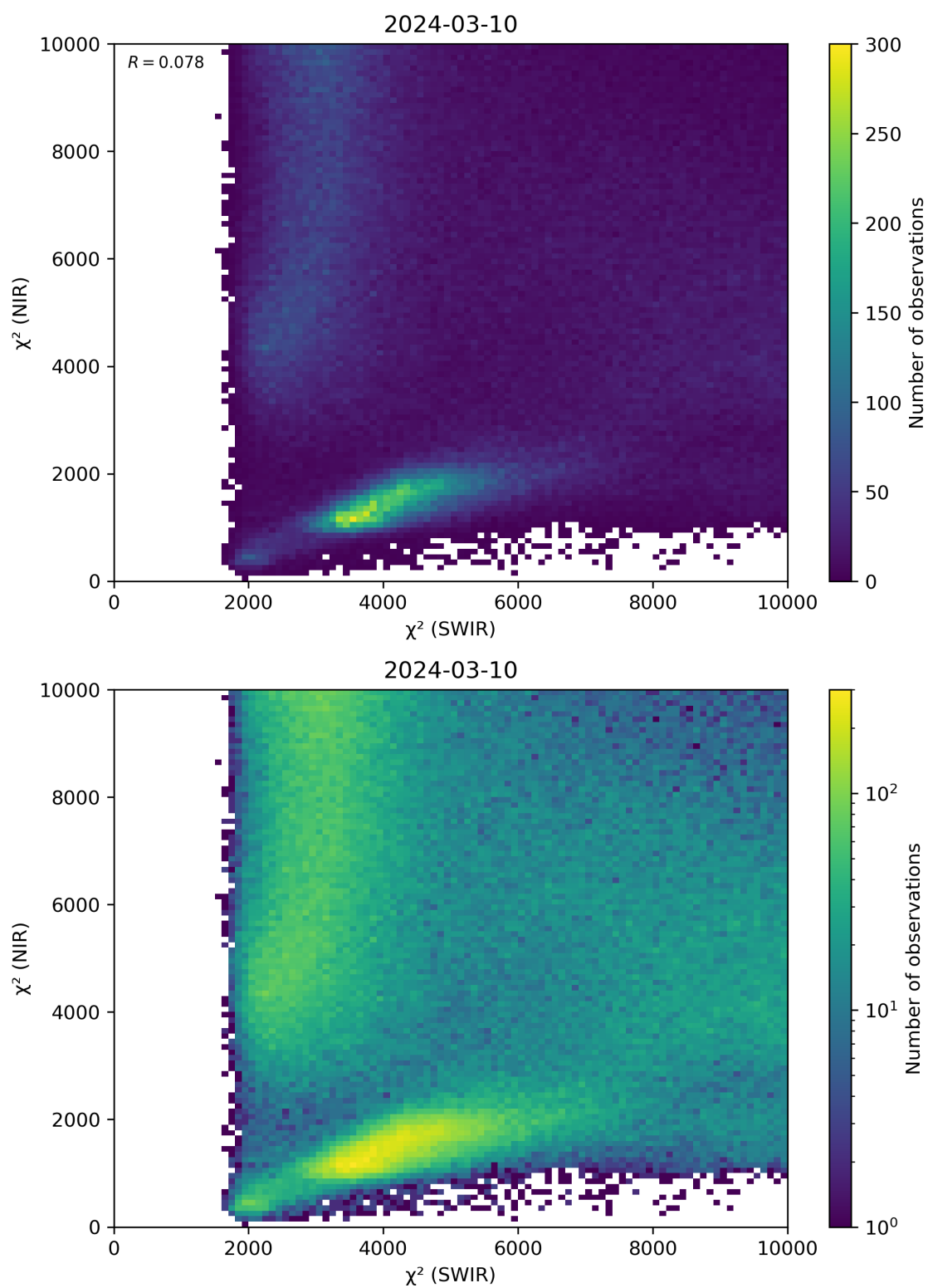
Figure 47: Scatter density plot of “ \chi^2 (SWIR)” against “ \chi^2 (NIR)” for 2024-03-09 to 2024-03-11.
