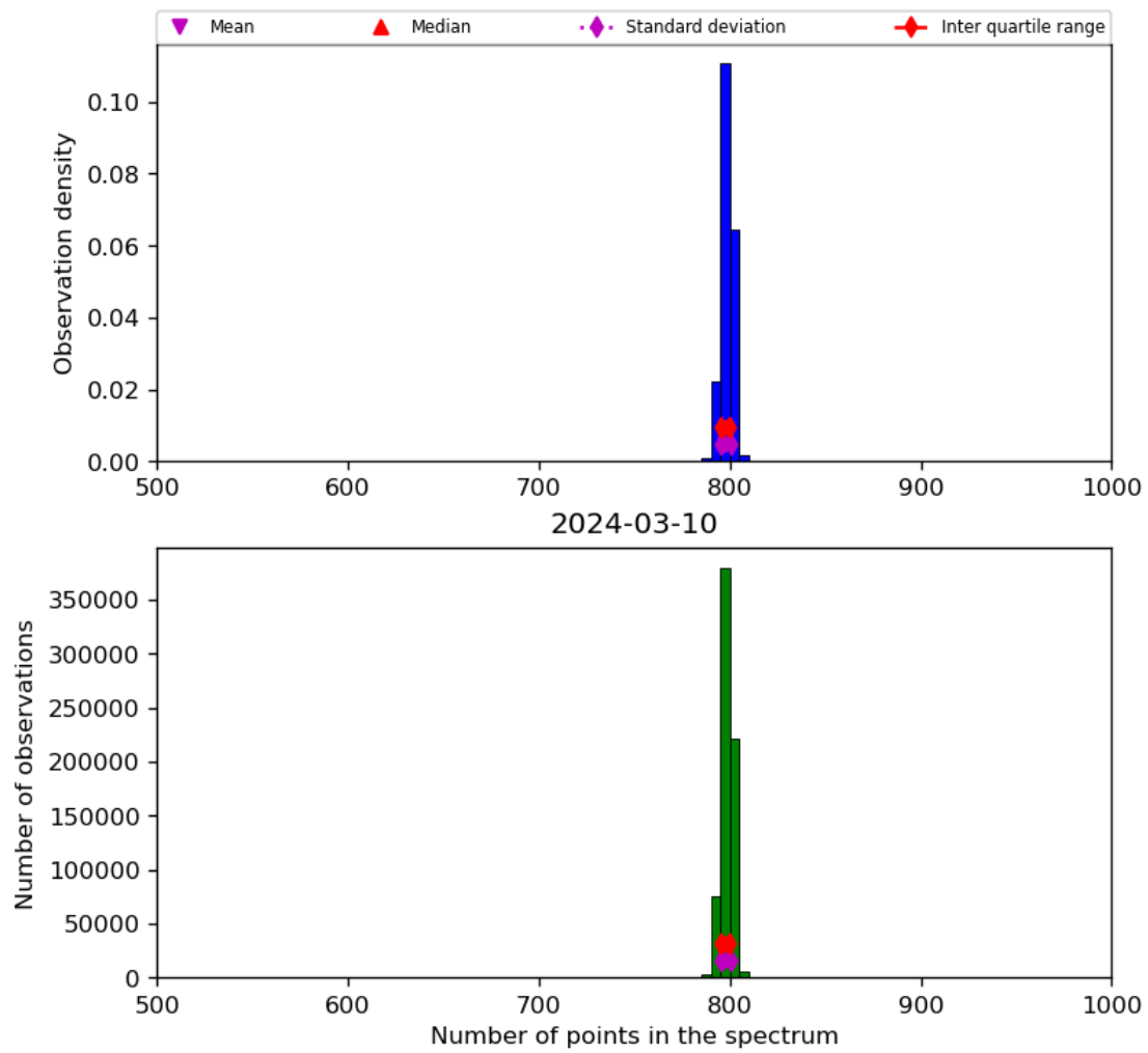
Figure 26: Histogram of “Number of points in the spectrum” for 2024-03-09 to 2024-03-11
