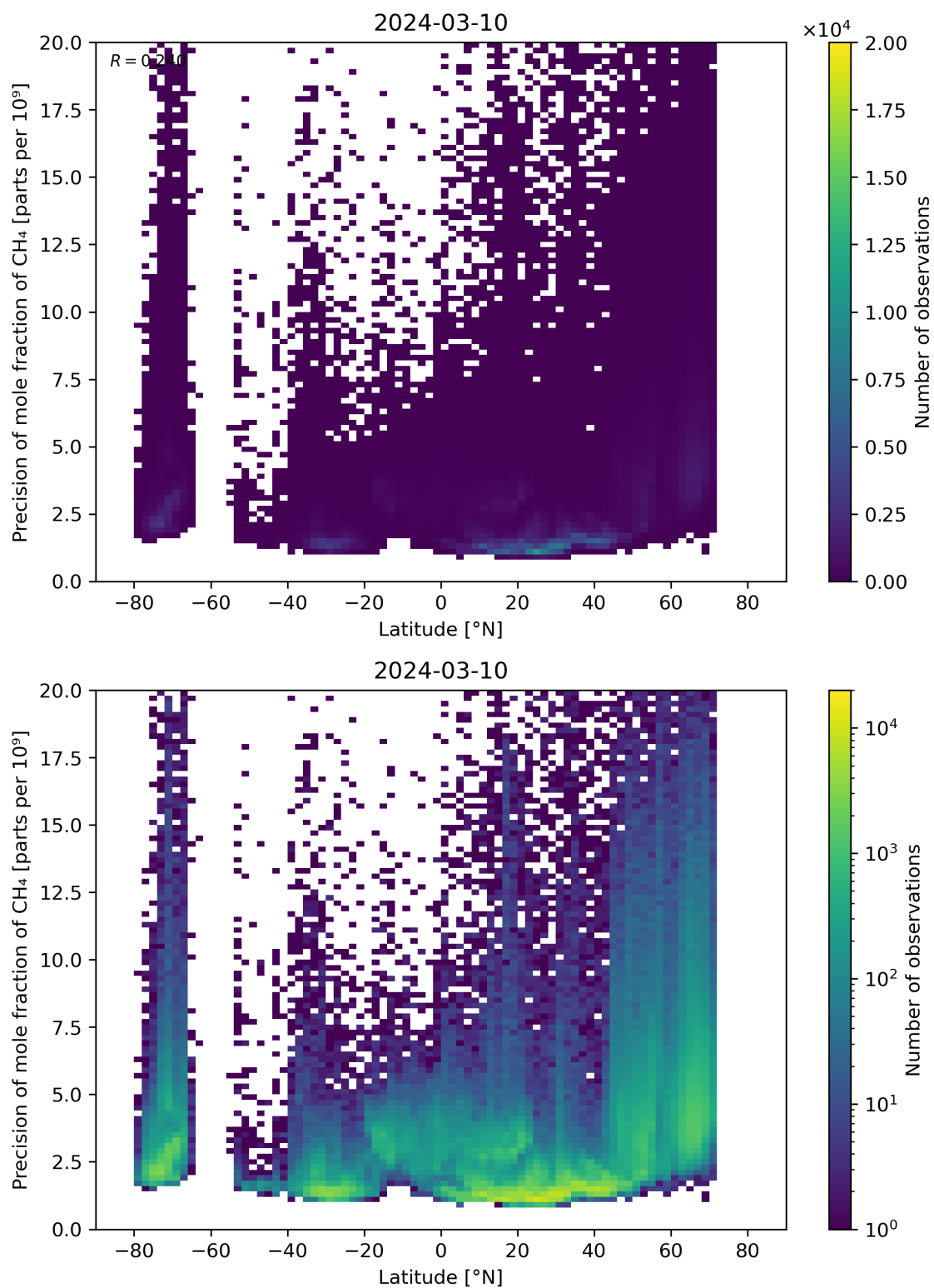
Figure 59: Scatter density plot of “Latitude” against “Precision of mole fraction of CH 4 ” for 2024-03-09 to 2024-03-11.
