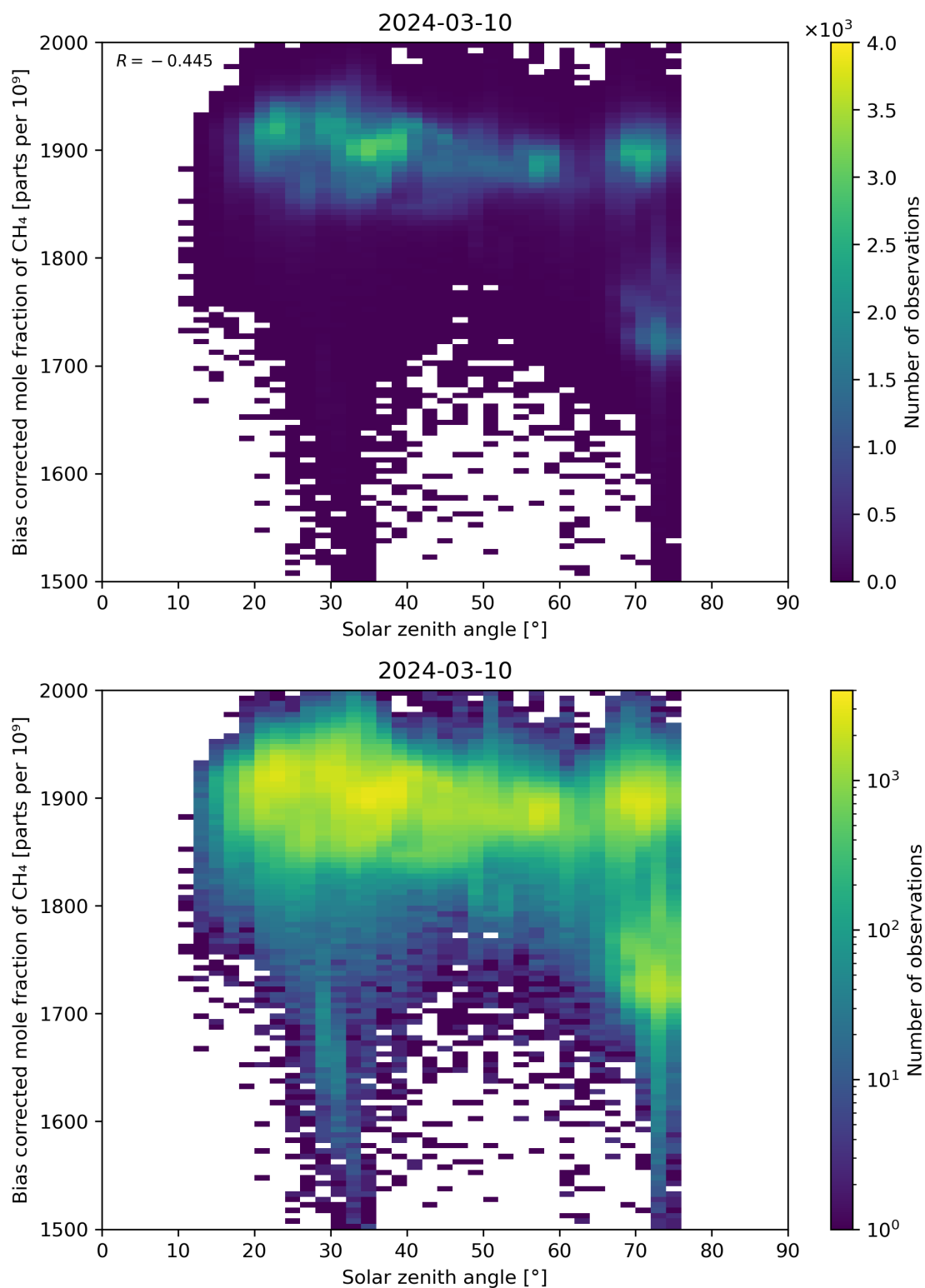
Figure 100: Scatter density plot of “Solar zenith angle” against “Bias corrected mole fraction of \text{CH}_4 ” for 2024-03-09 to 2024-03-11.
