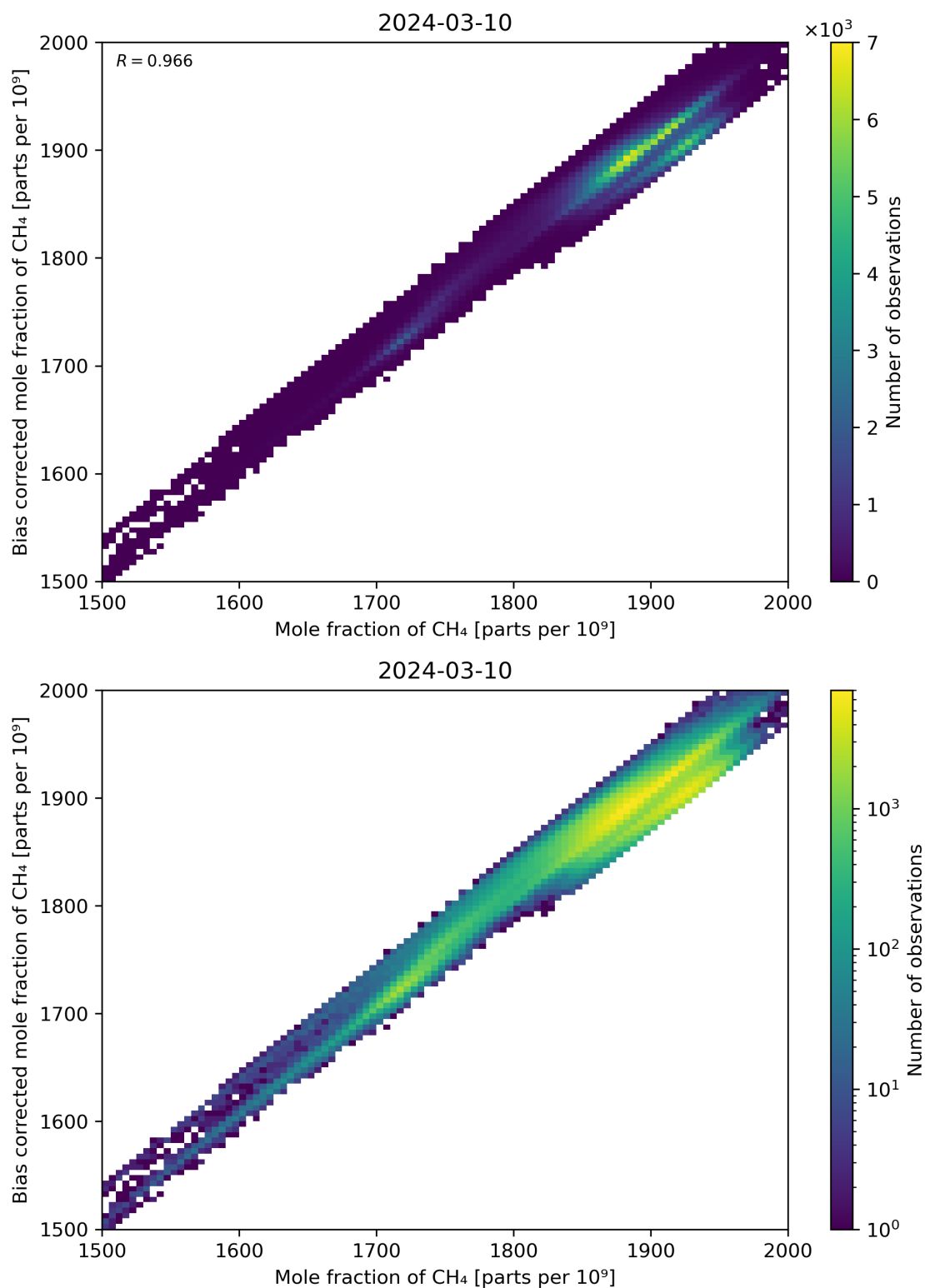
Figure 74: Scatter density plot of “Mole fraction of CH 4 ” against “Bias corrected mole fraction of CH 4 ” for 2024-03-09 to 2024-03-11.
