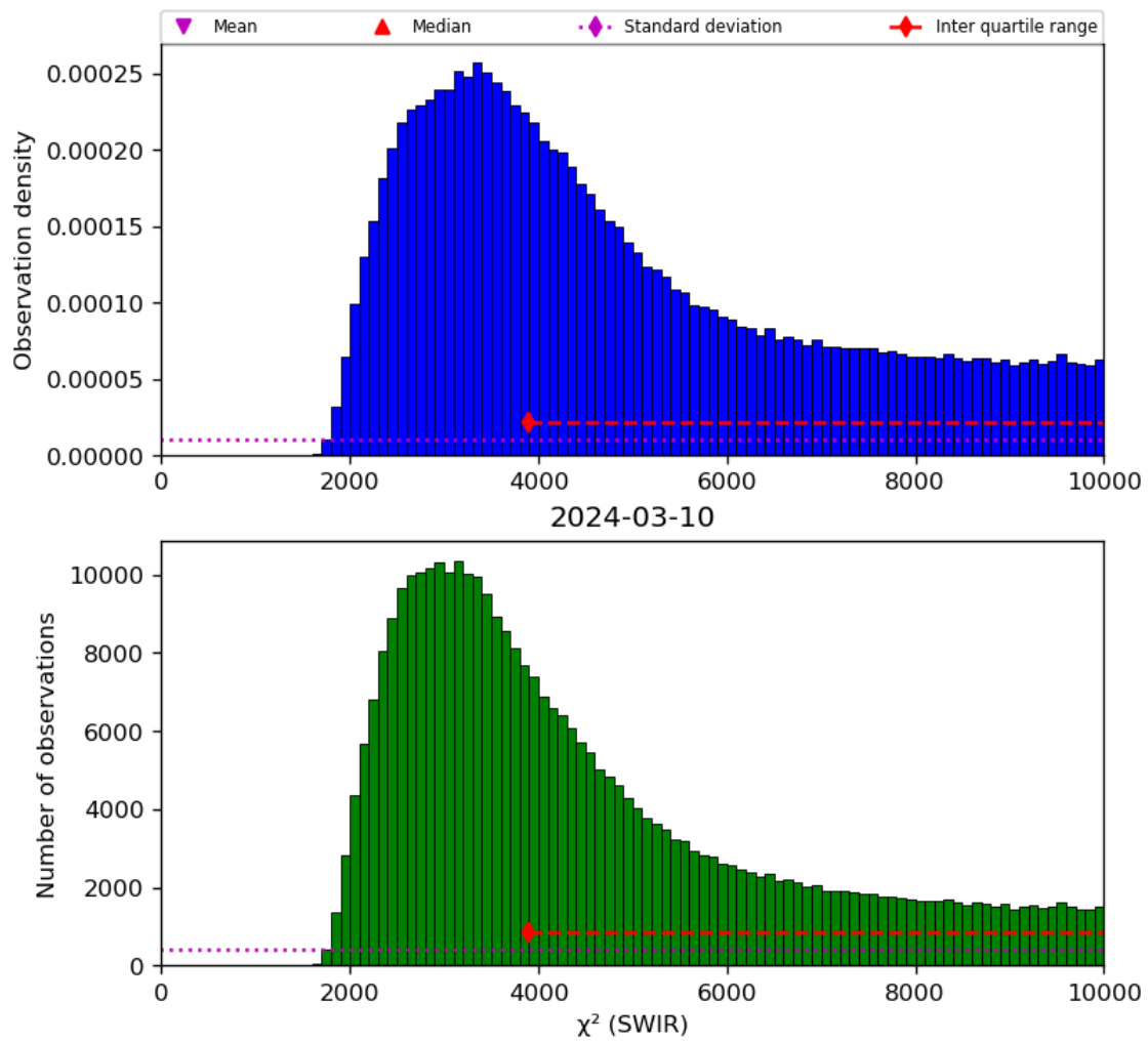
Figure 28: Histogram of “ \chi^2 (SWIR)” for 2024-03-09 to 2024-03-11
