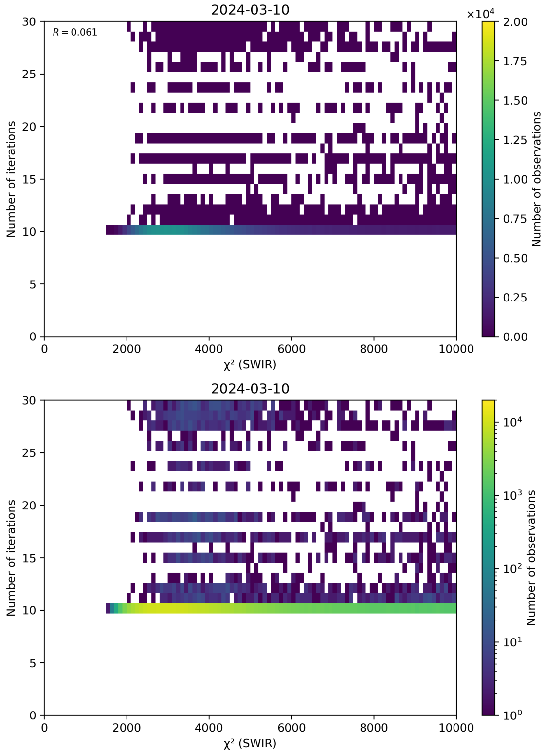
Figure 50: Scatter density plot of “ \chi^2 (SWIR)” against “Number of iterations” for 2024-03-09 to 2024-03-11.
