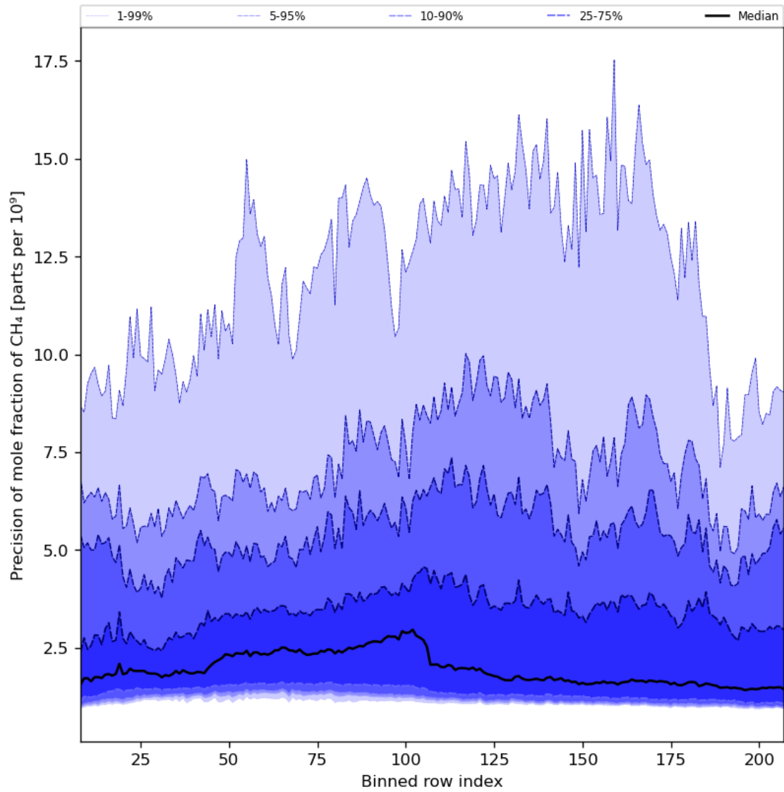
Figure 35: Along track statistics of “Precision of mole fraction of CH 4 ” for 2024-03-09 to 2024-03-11
