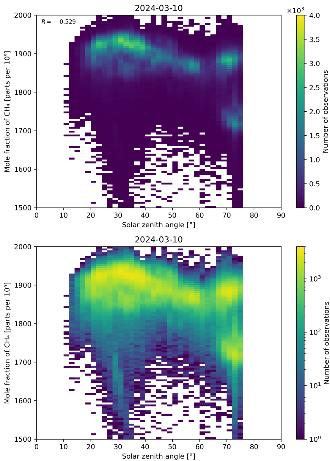
Figure 99: Scatter density plot of “Solar zenith angle” against “Mole fraction of CH 4 ” for 2024-03-09 to 2024-03-11.
