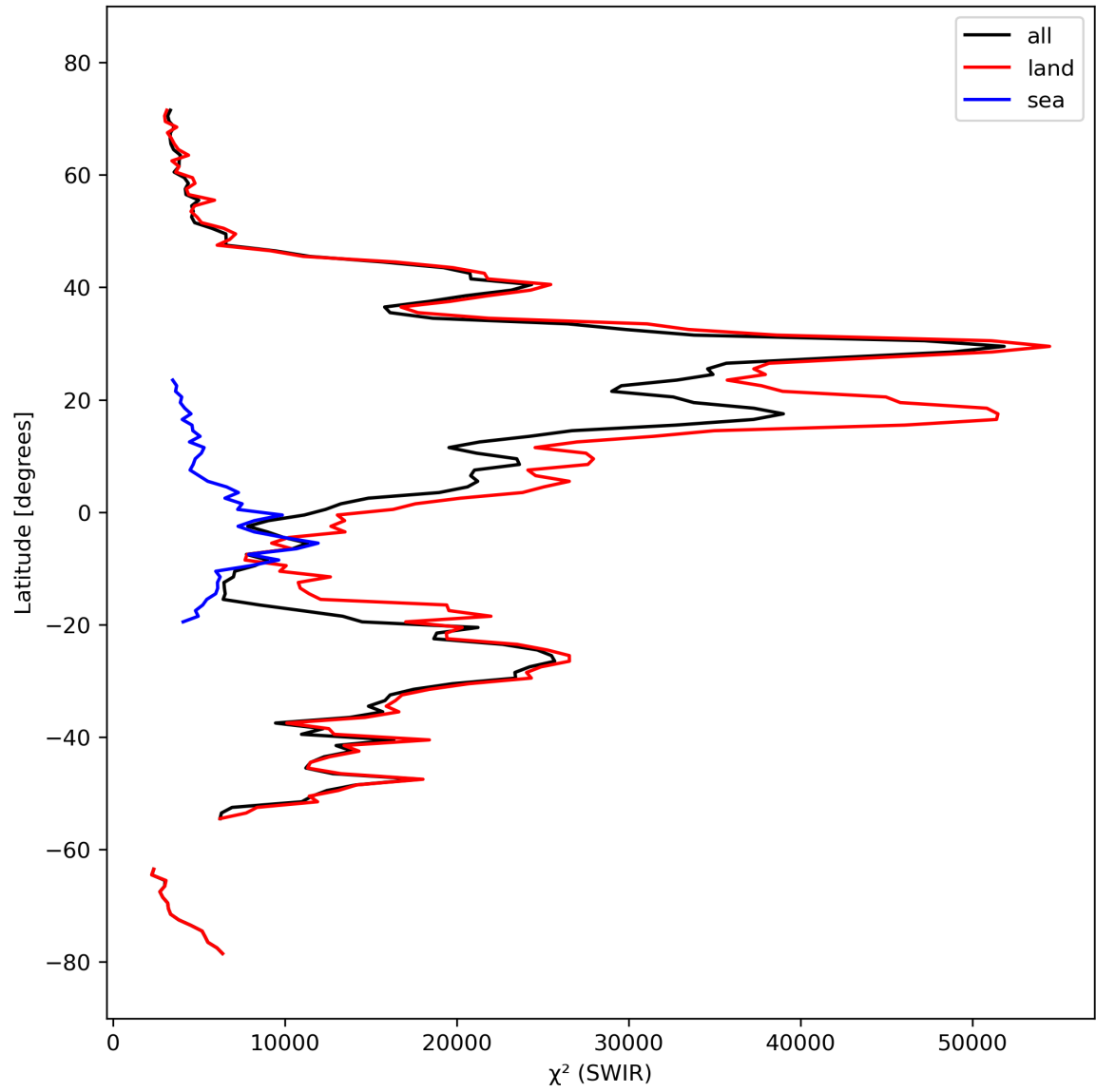
Figure 17: Zonal average of “ \chi^2 (SWIR)” for 2024-03-09 to 2024-03-11.
