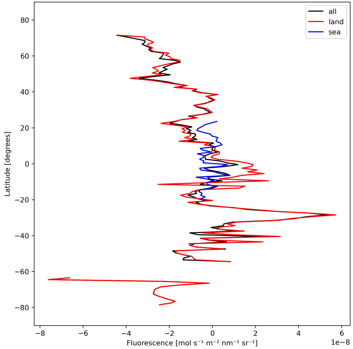
Figure 21: Zonal average of “Fluorescence” for 2024-03-09 to 2024-03-11.
