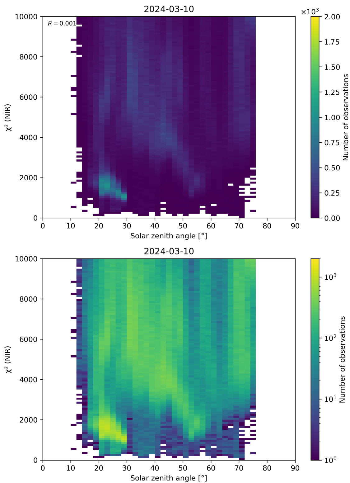
Figure 94: Scatter density plot of “Solar zenith angle” against “ \chi^2 (NIR)” for 2024-03-09 to 2024-03-11.
