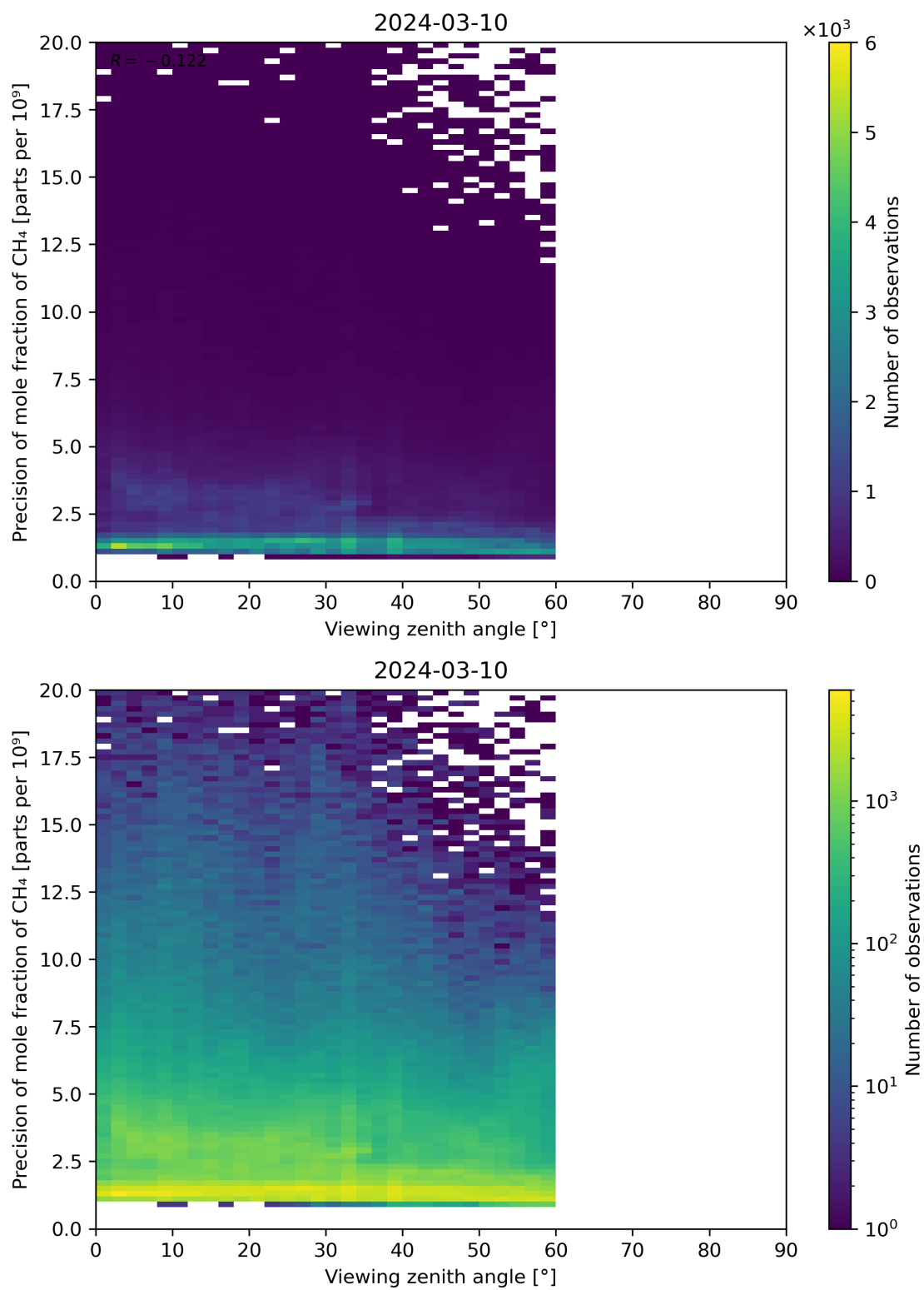
Figure 112: Scatter density plot of “Viewing zenith angle” against “Precision of mole fraction of CH 4 ” for 2024-03-09 to 2024-03-11.
