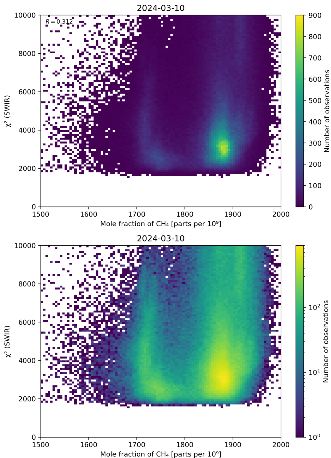
Figure 71: Scatter density plot of “Mole fraction of CH 4 ” against “ \chi^2 (SWIR)” for 2024-03-09 to 2024-03-11.
