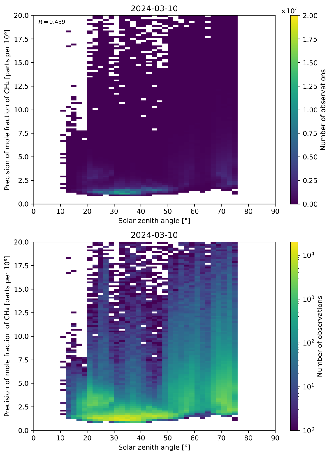
Figure 101: Scatter density plot of “Solar zenith angle” against “Precision of mole fraction of CH 4 ” for 2024-03-09 to 2024-03-11.
