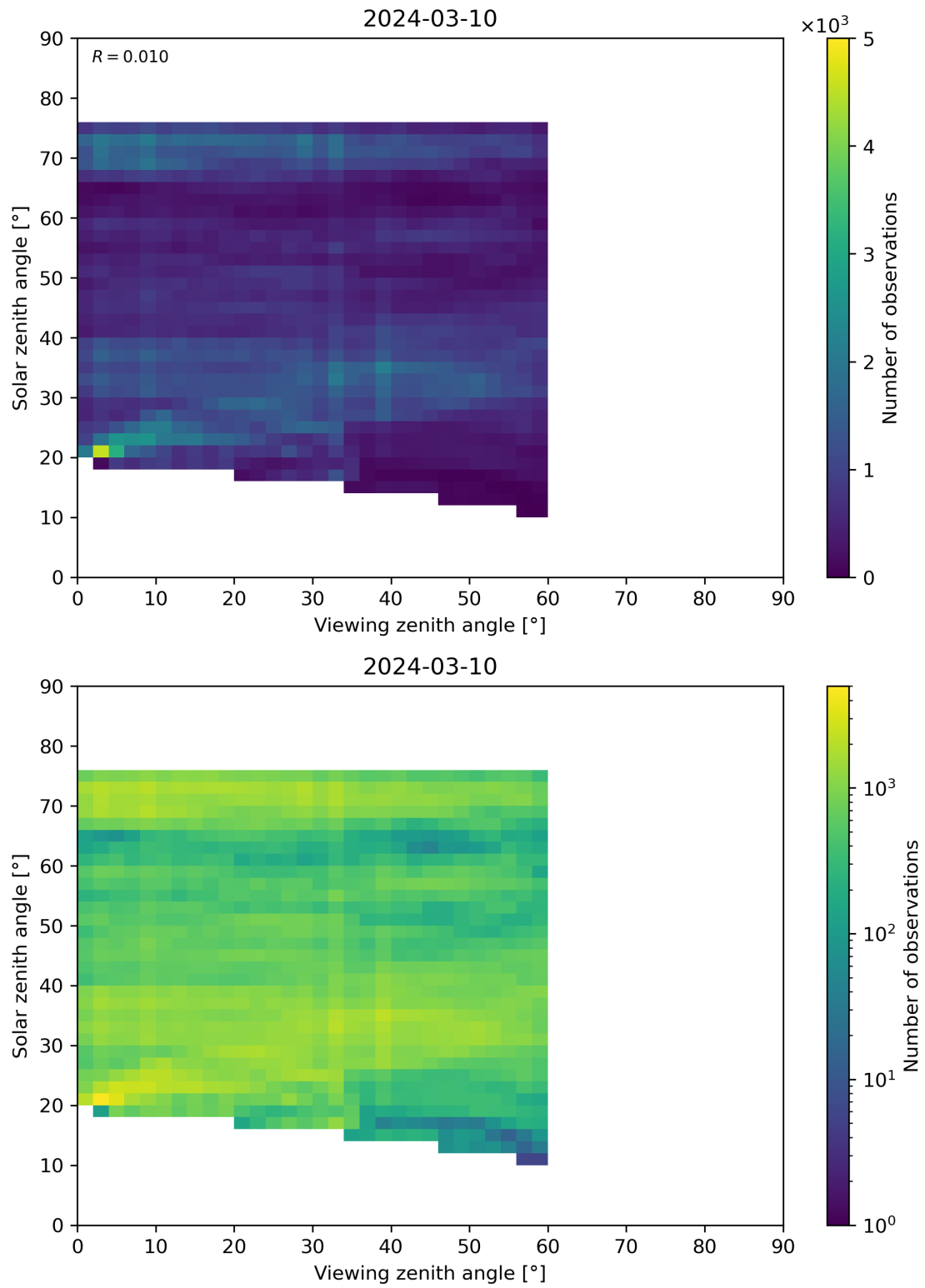
Figure 115: Scatter density plot of “Viewing zenith angle” against “Solar zenith angle” for 2024-03-09 to 2024-03-11.
