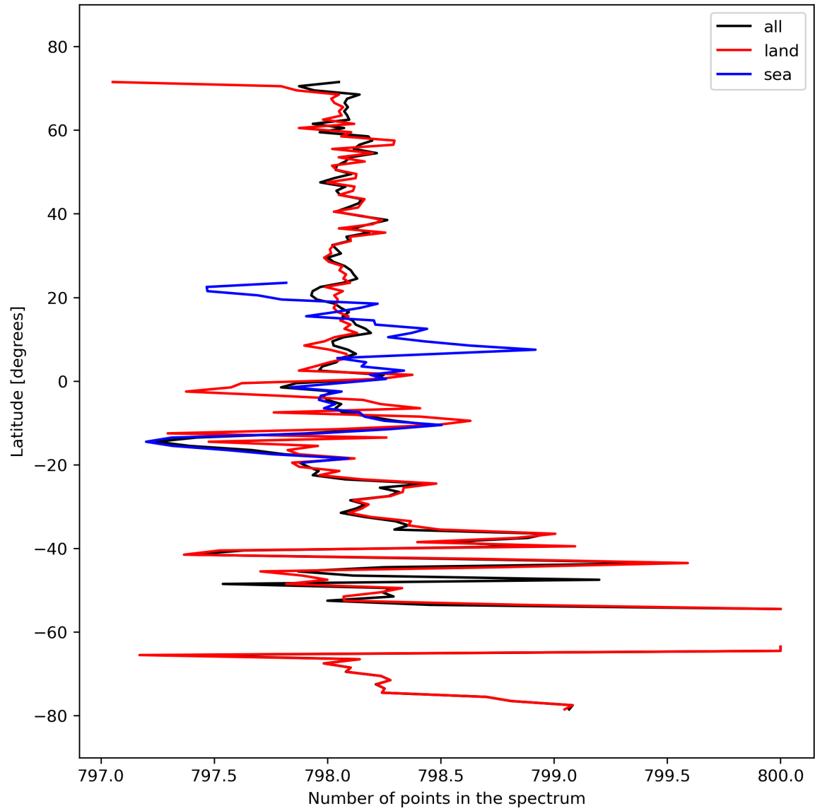
Figure 15: Zonal average of “Number of points in the spectrum” for 2024-03-09 to 2024-03-11.
