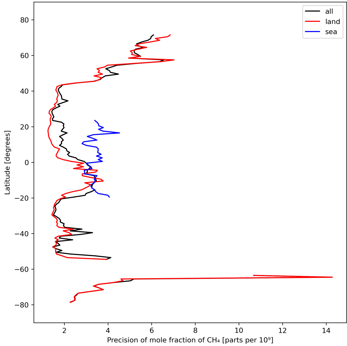
Figure 13: Zonal average of “Precision of mole fraction of CH 4 ” for 2024-03-09 to 2024-03-11.
