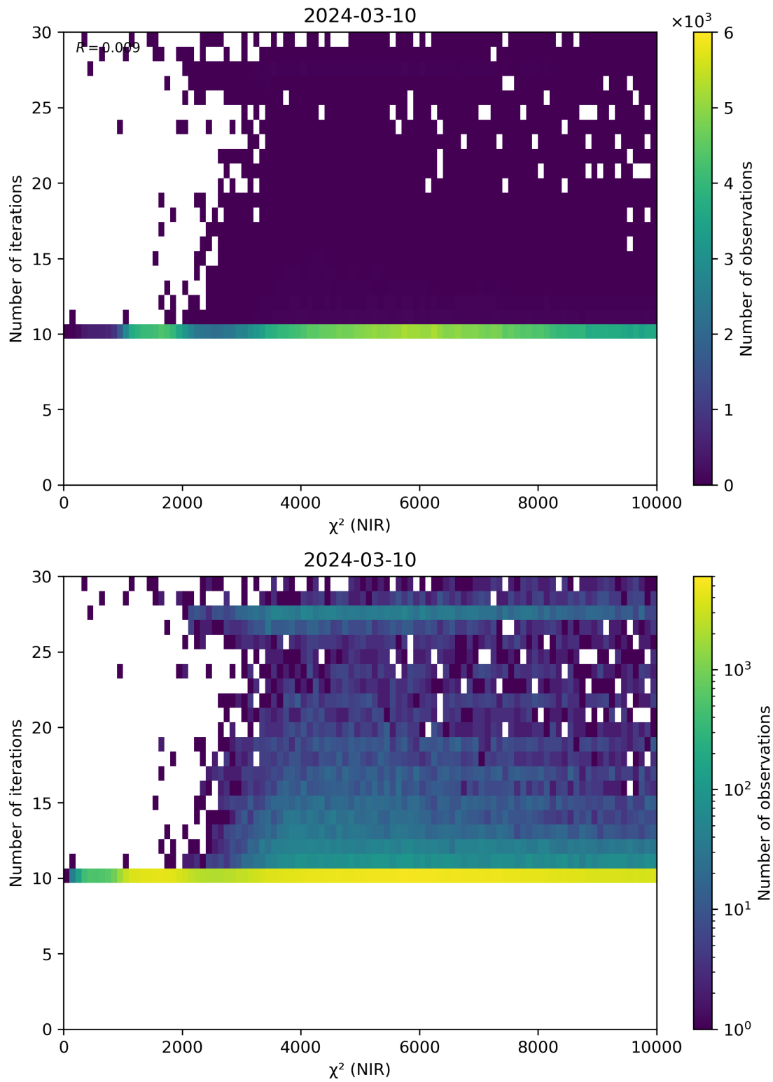
Figure 46: Scatter density plot of “ \chi^2 (NIR)” against “Number of iterations” for 2024-03-09 to 2024-03-11.
