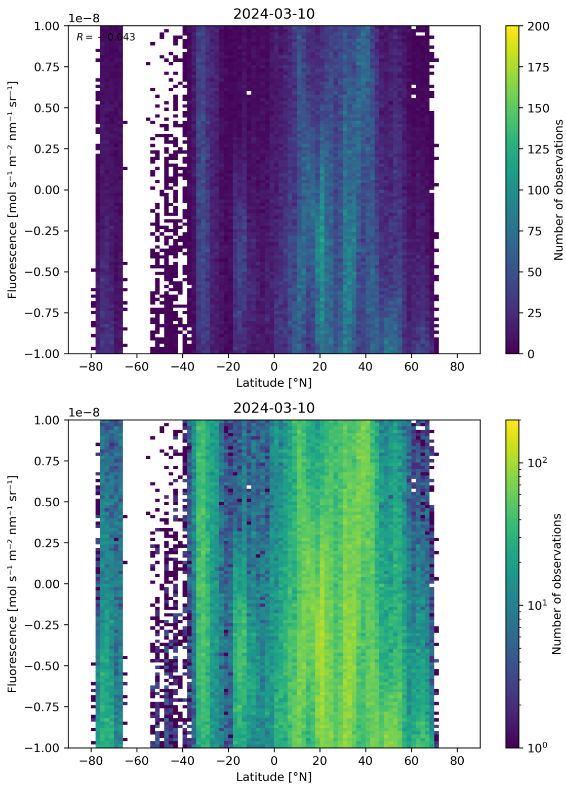
Figure 56: Scatter density plot of “Latitude” against “Fluorescence” for 2024-03-09 to 2024-03-11.
