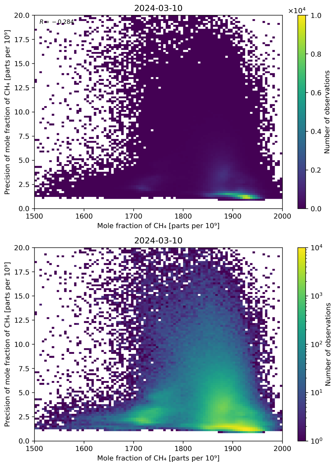
Figure 75: Scatter density plot of “Mole fraction of CH 4 ” against “Precision of mole fraction of CH 4 ” for 2024-03-09 to 2024-03-11.
