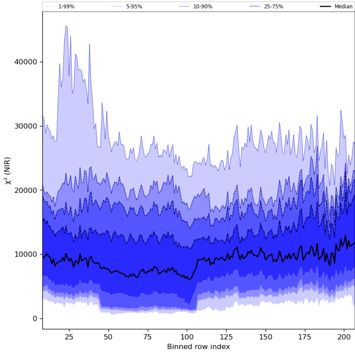
Figure 40: Along track statistics of “ \chi^2 (NIR)” for 2024-03-09 to 2024-03-11
