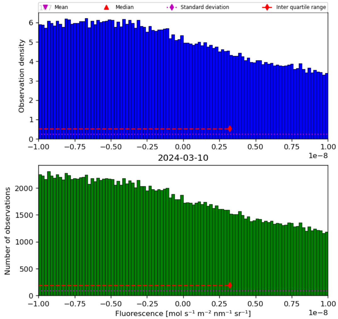
Figure 32: Histogram of “Fluorescence” for 2024-03-09 to 2024-03-11
