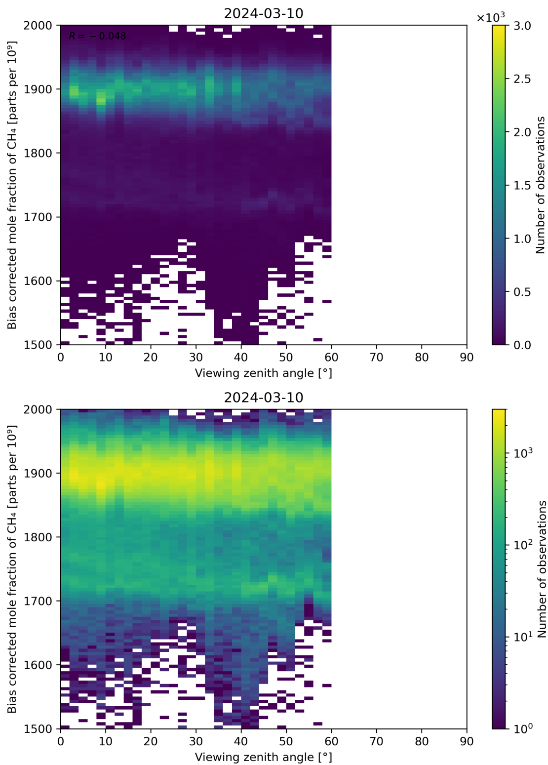
Figure 111: Scatter density plot of “Viewing zenith angle” against “Bias corrected mole fraction of CH 4 ” for 2024-03-09 to 2024-03-11.
