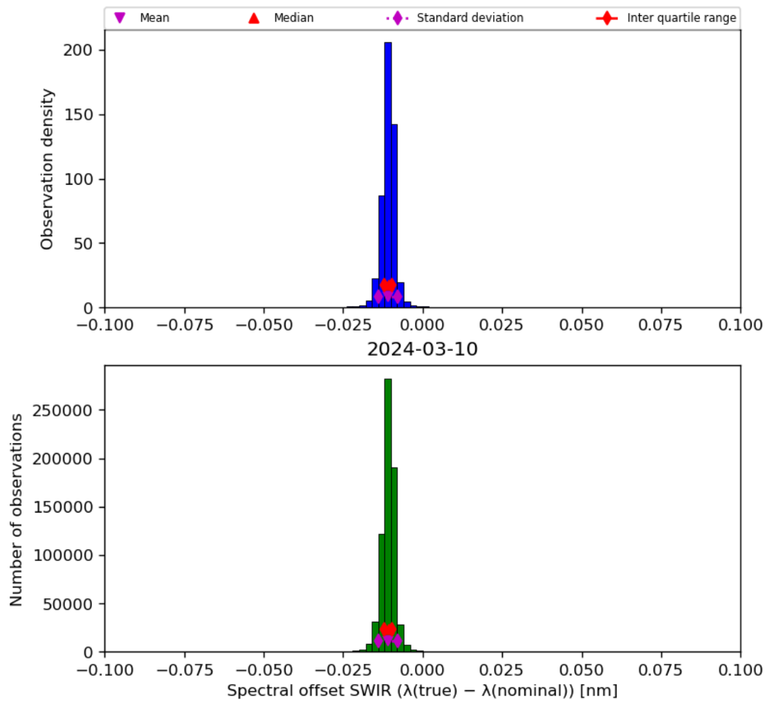
Figure 27: Histogram of “Spectral offset SWIR ( \lambda(\text{true}) - \lambda(\text{nominal}) )” for 2024-03-09 to 2024-03-11
