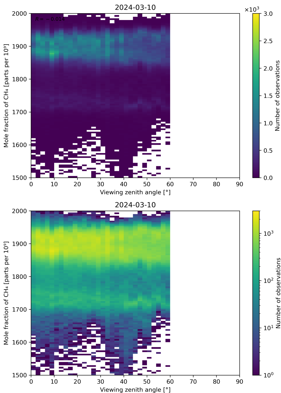
Figure 110: Scatter density plot of “Viewing zenith angle” against “Mole fraction of CH 4 ” for 2024-03-09 to 2024-03-11.
