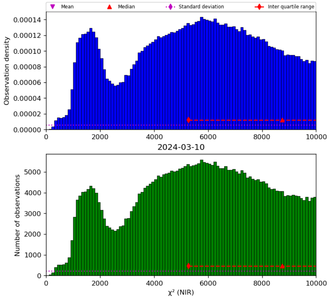
Figure 29: Histogram of “ \chi^2 (NIR)” for 2024-03-09 to 2024-03-11
