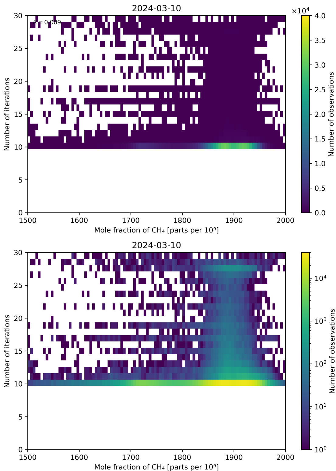
Figure 76: Scatter density plot of “Mole fraction of CH 4 ” against “Number of iterations” for 2024-03-09 to 2024-03-11.
