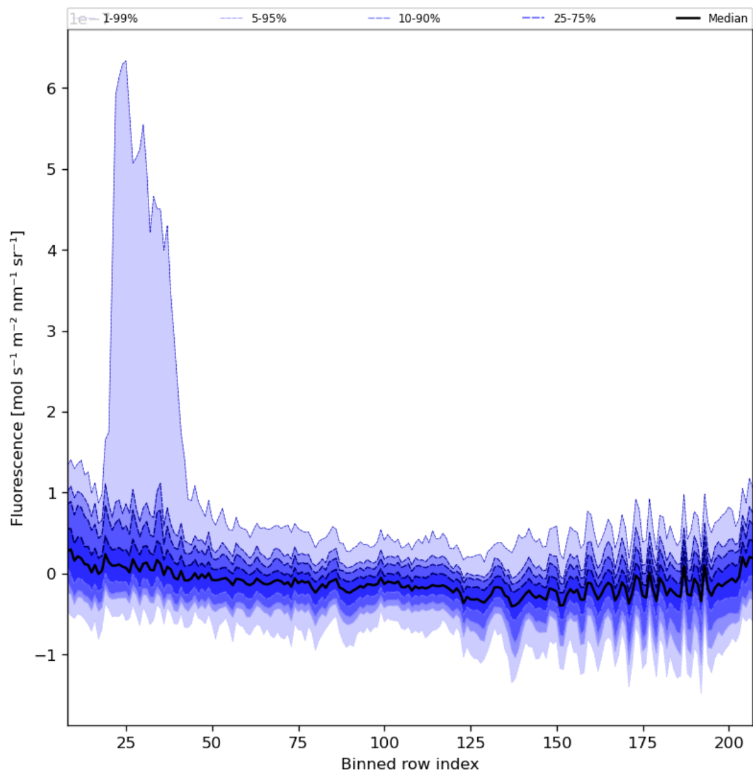
Figure 43: Along track statistics of “Fluorescence” for 2024-03-09 to 2024-03-11
