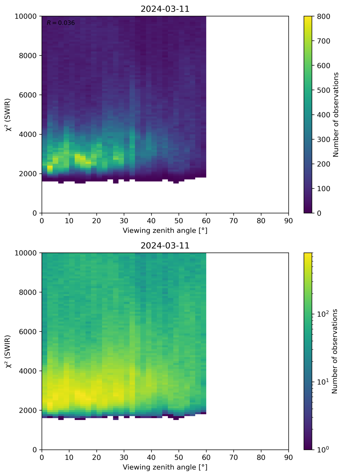
Figure 106: Scatter density plot of “Viewing zenith angle” against “ \chi^2 (SWIR)” for 2024-03-10 to 2024-03-12.
