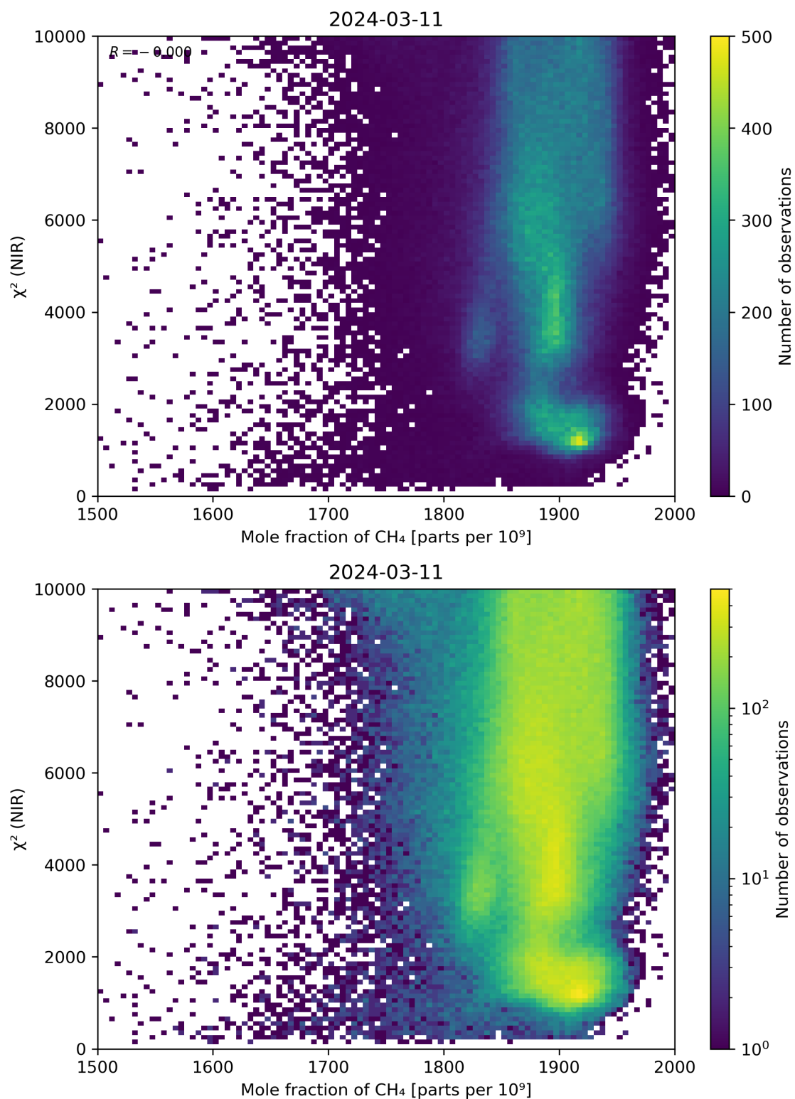
Figure 70: Scatter density plot of “Mole fraction of CH 4 ” against “ \chi^2 (NIR)” for 2024-03-10 to 2024-03-12.
