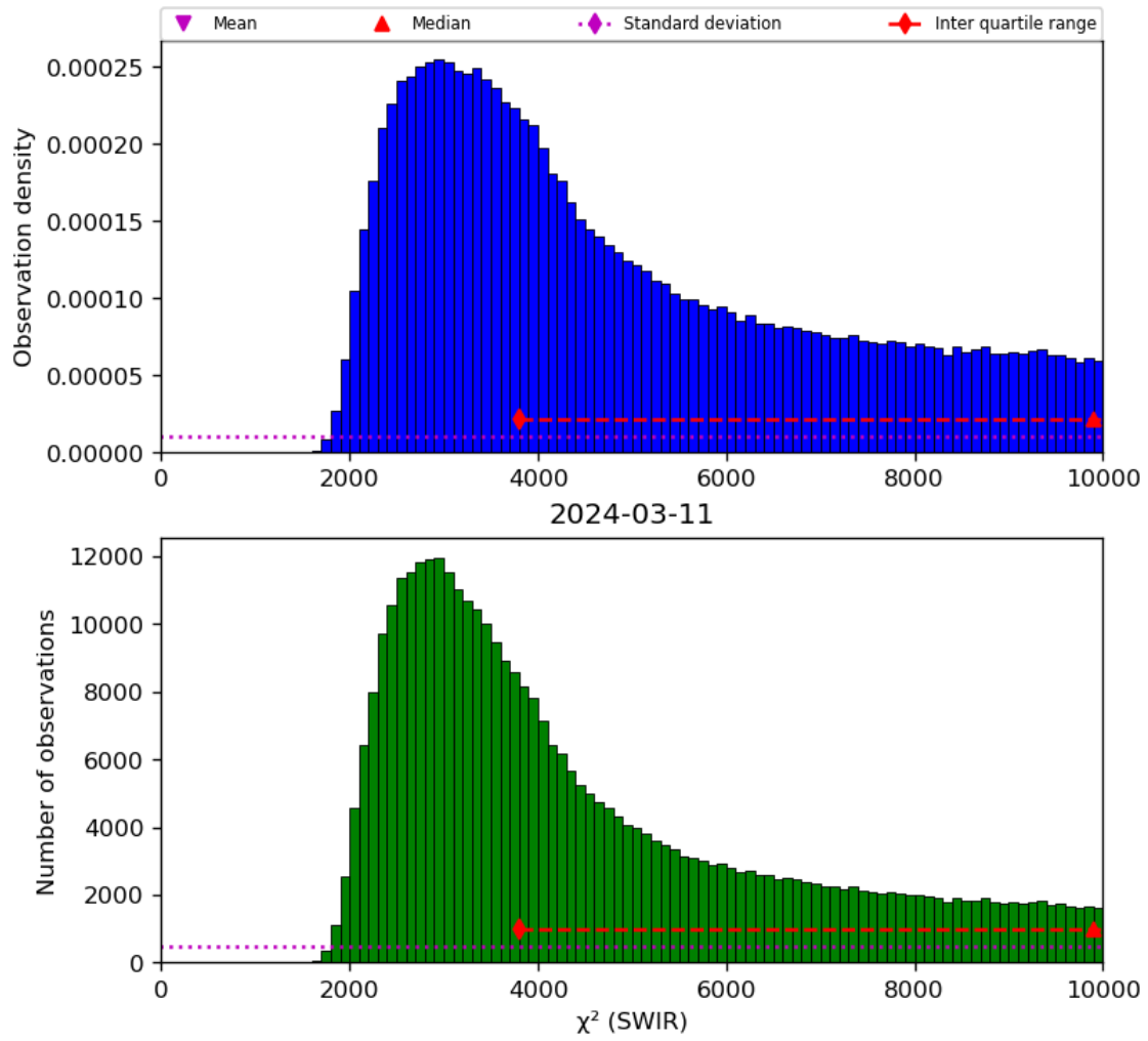
Figure 28: Histogram of “ \chi^2 (SWIR)” for 2024-03-10 to 2024-03-12
