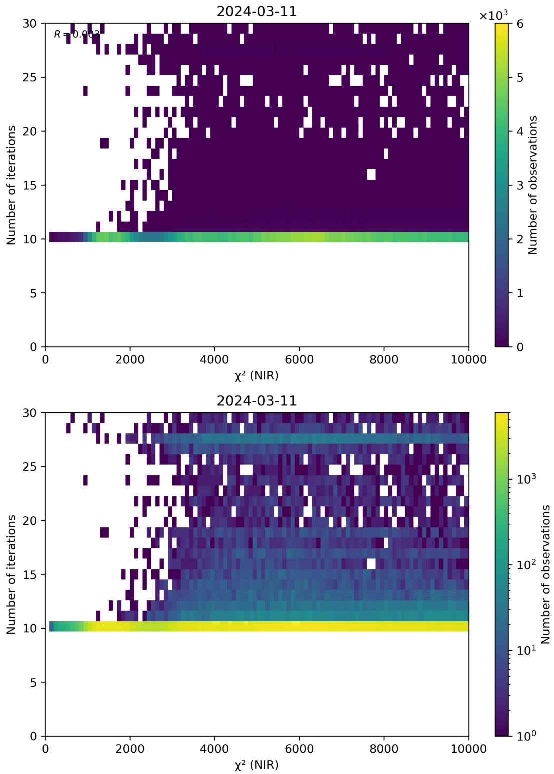
Figure 46: Scatter density plot of “ \chi^2 (NIR)” against “Number of iterations” for 2024-03-10 to 2024-03-12.
