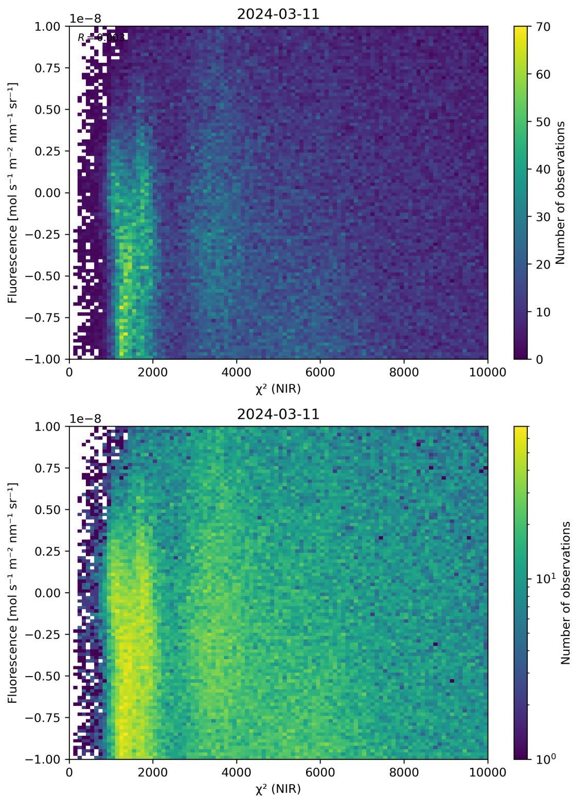
Figure 45: Scatter density plot of “ \chi^2 (NIR)” against “Fluorescence” for 2024-03-10 to 2024-03-12.
