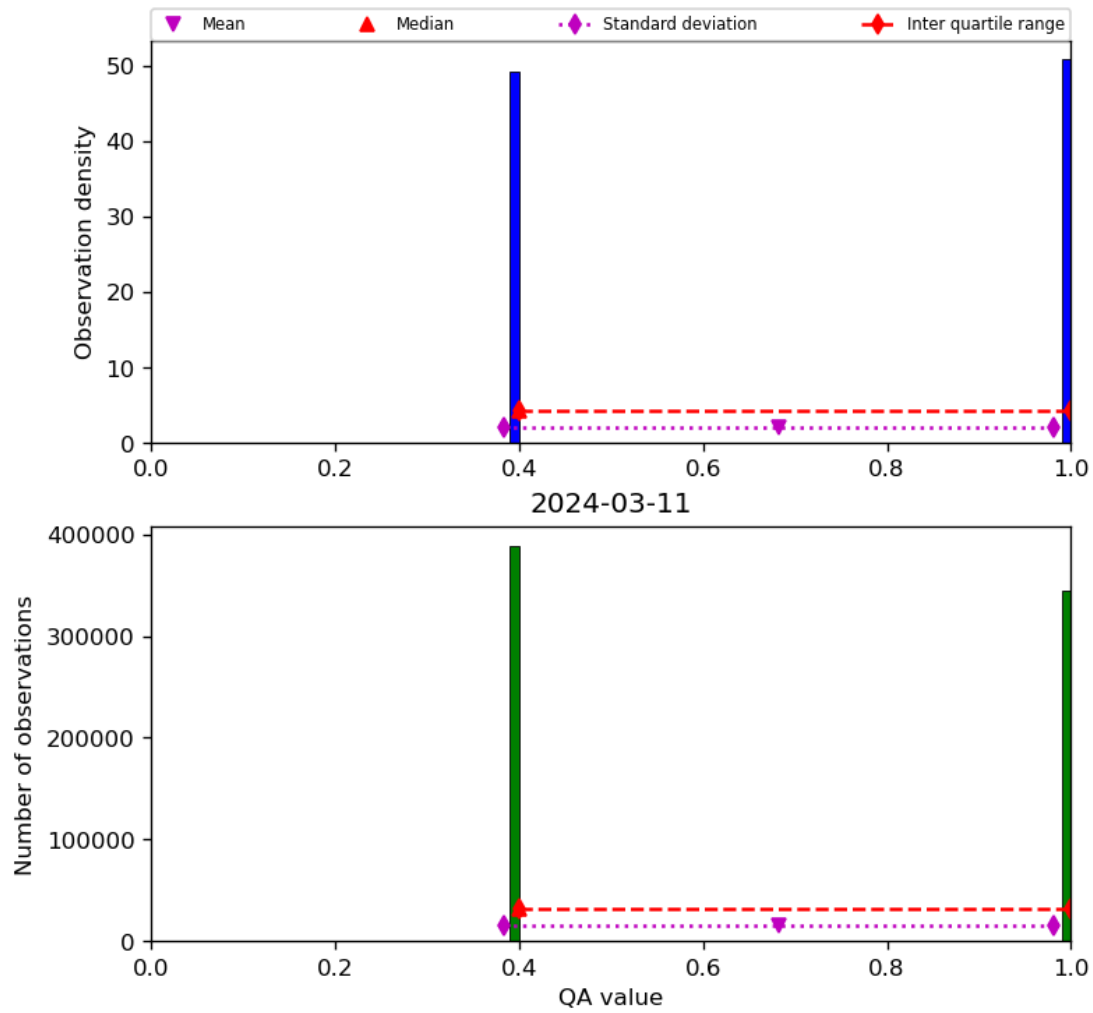
Figure 22: Histogram of “QA value” for 2024-03-10 to 2024-03-12
