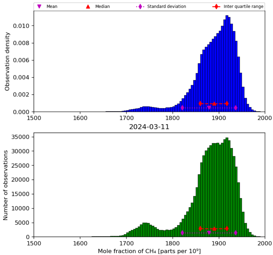
Figure 23: Histogram of “Mole fraction of CH 4 ” for 2024-03-10 to 2024-03-12
