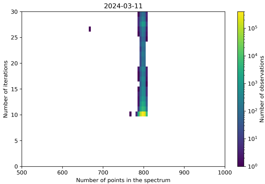
Figure 92: Scatter density plot of “Number of points in the spectrum” against “Number of iterations” for 2024-03-10 to 2024-03-12.
