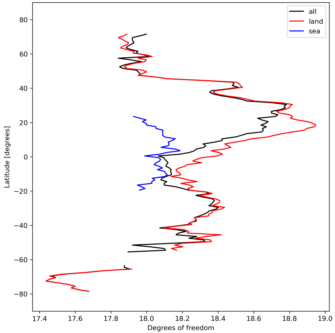
Figure 19: Zonal average of “Degrees of freedom” for 2024-03-10 to 2024-03-12.
