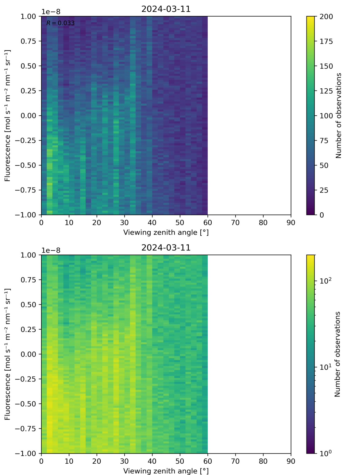
Figure 108: Scatter density plot of “Viewing zenith angle” against “Fluorescence” for 2024-03-10 to 2024-03-12.
