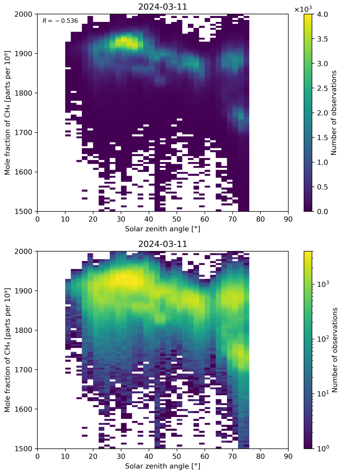
Figure 99: Scatter density plot of “Solar zenith angle” against “Mole fraction of CH 4 ” for 2024-03-10 to 2024-03-12.
