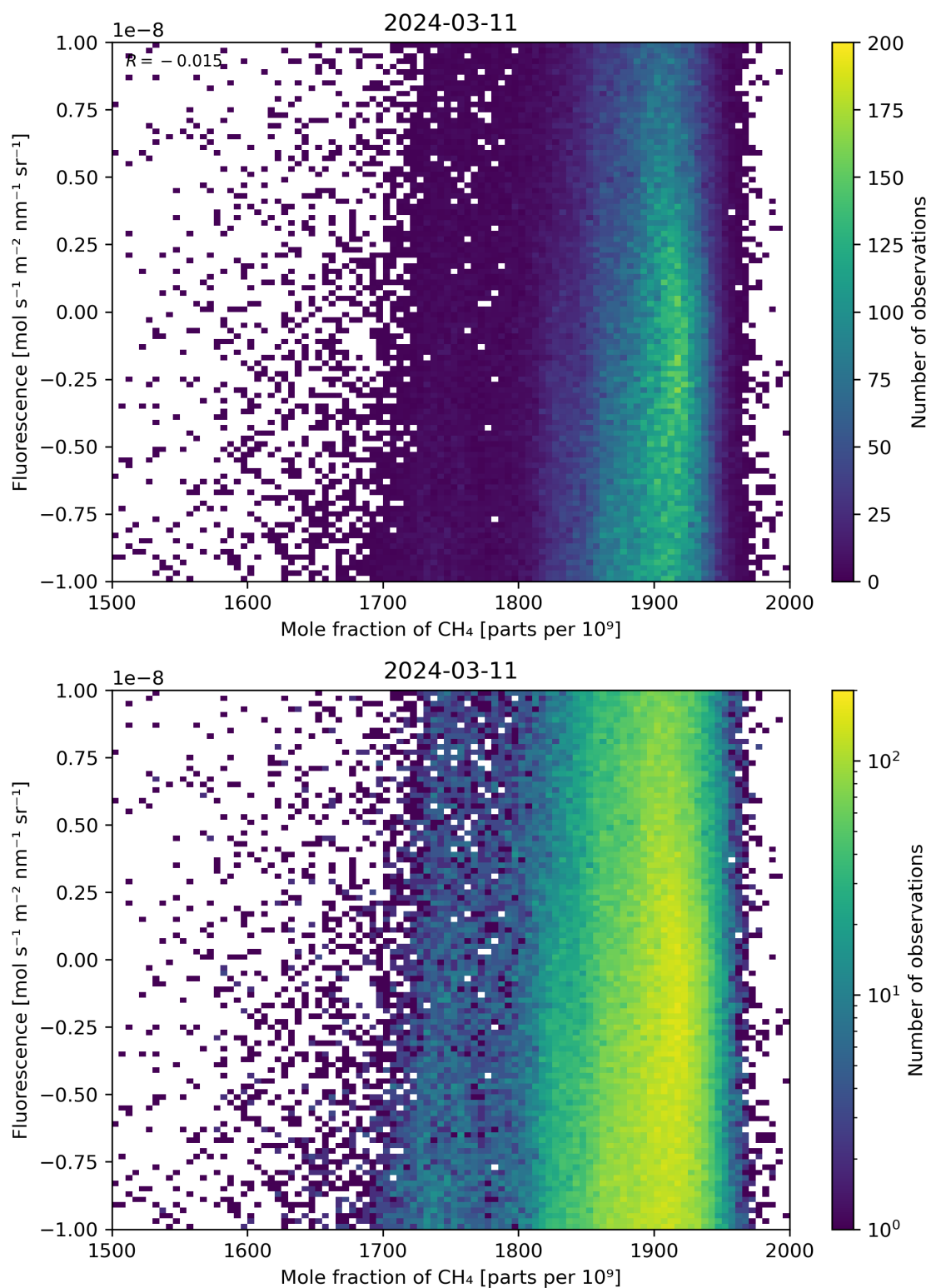
Figure 73: Scatter density plot of “Mole fraction of \text{CH}_4 ” against “Fluorescence” for 2024-03-10 to 2024-03-12.
