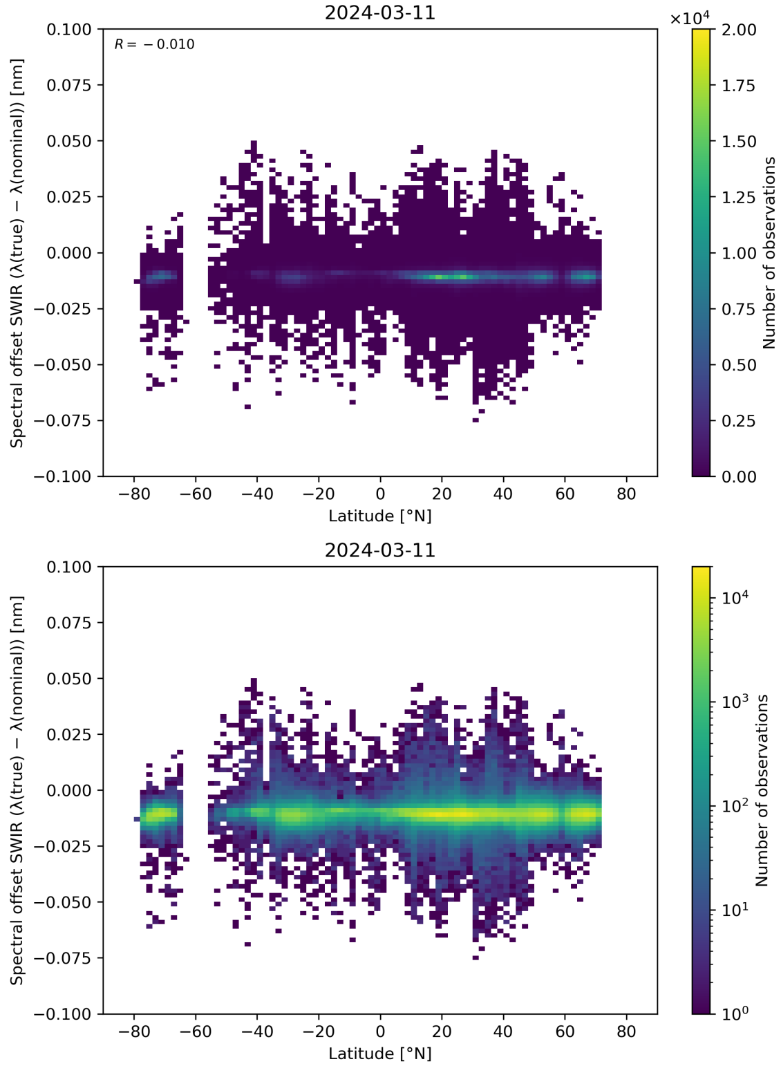
Figure 62: Scatter density plot of “Latitude” against “Spectral offset SWIR ( \lambda(\text{true}) - \lambda(\text{nominal}) )” for 2024-03-10 to 2024-03-12.
