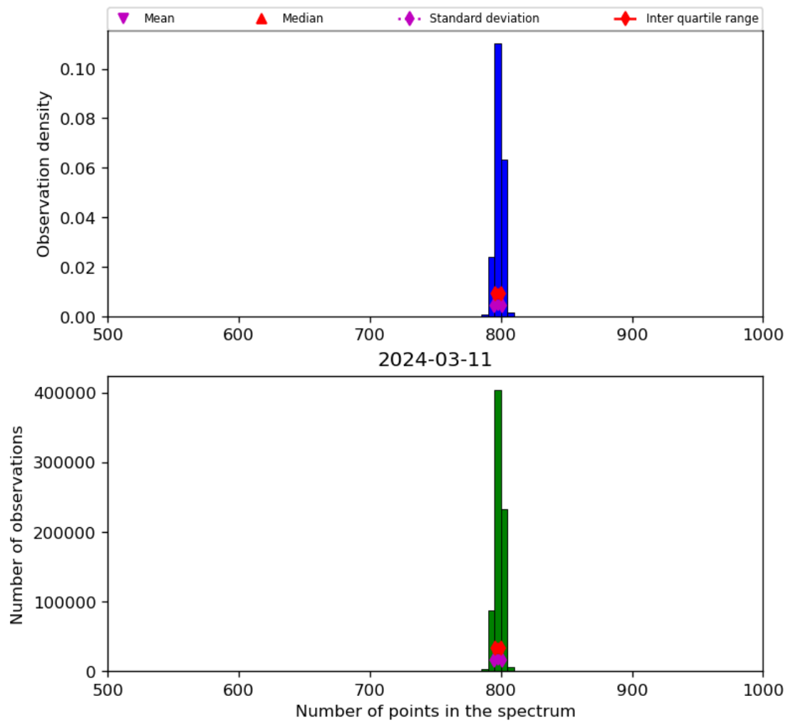
Figure 26: Histogram of “Number of points in the spectrum” for 2024-03-10 to 2024-03-12
