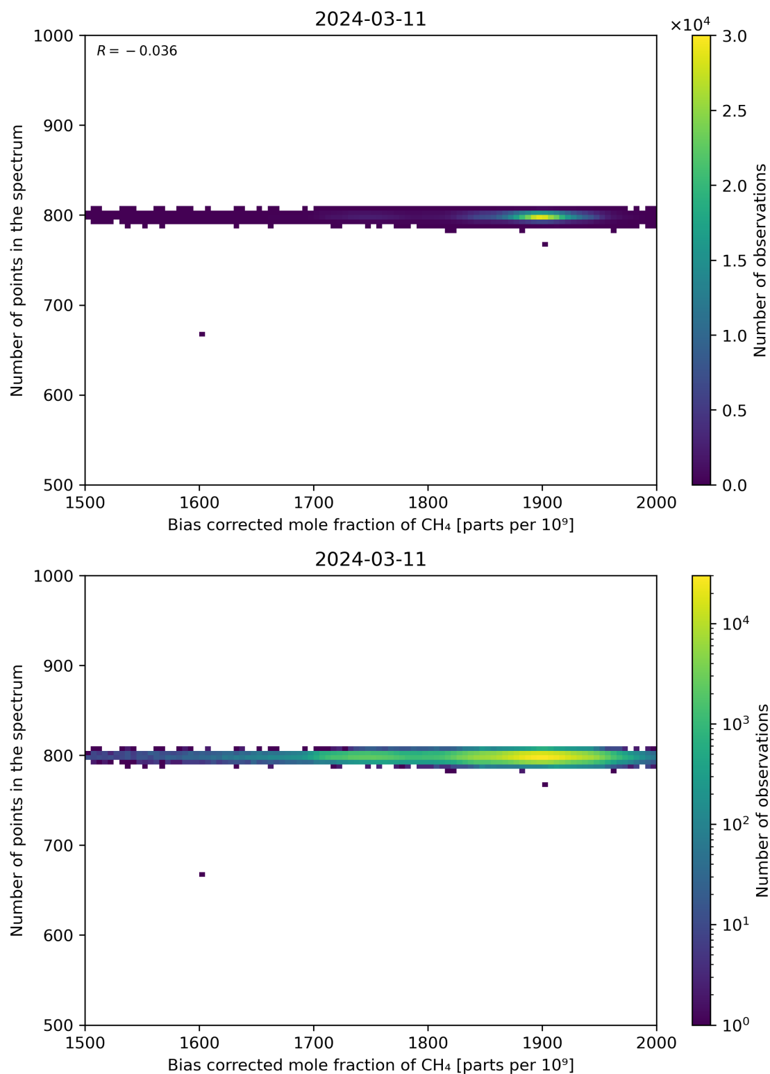
Figure 68: Scatter density plot of “Bias corrected mole fraction of CH 4 ” against “Number of points in the spectrum” for 2024-03-10 to 2024-03-12.
