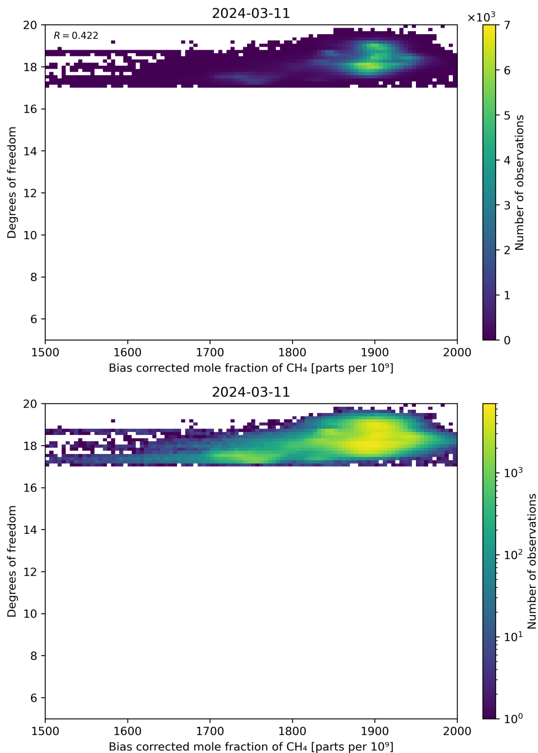
Figure 65: Scatter density plot of “Bias corrected mole fraction of CH 4 ” against “Degrees of freedom” for 2024-03-10 to 2024-03-12.
