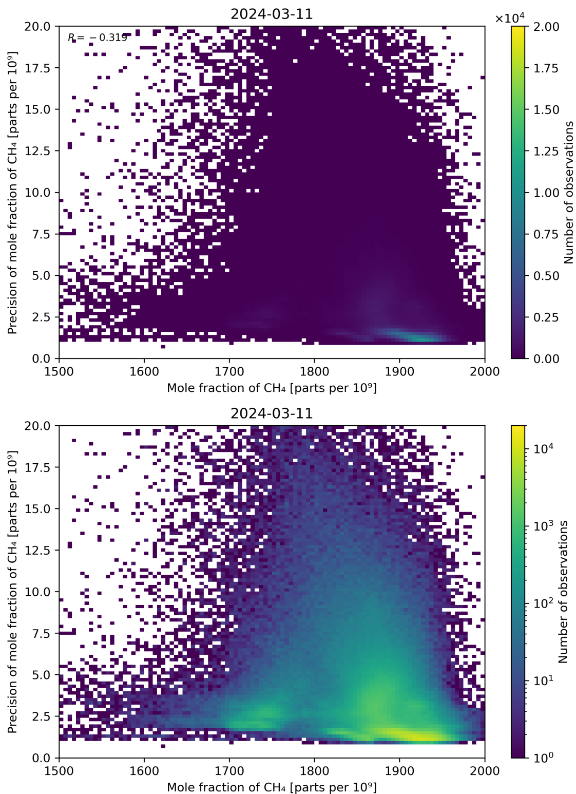
Figure 75: Scatter density plot of “Mole fraction of CH 4 ” against “Precision of mole fraction of CH 4 ” for 2024-03-10 to 2024-03-12.
