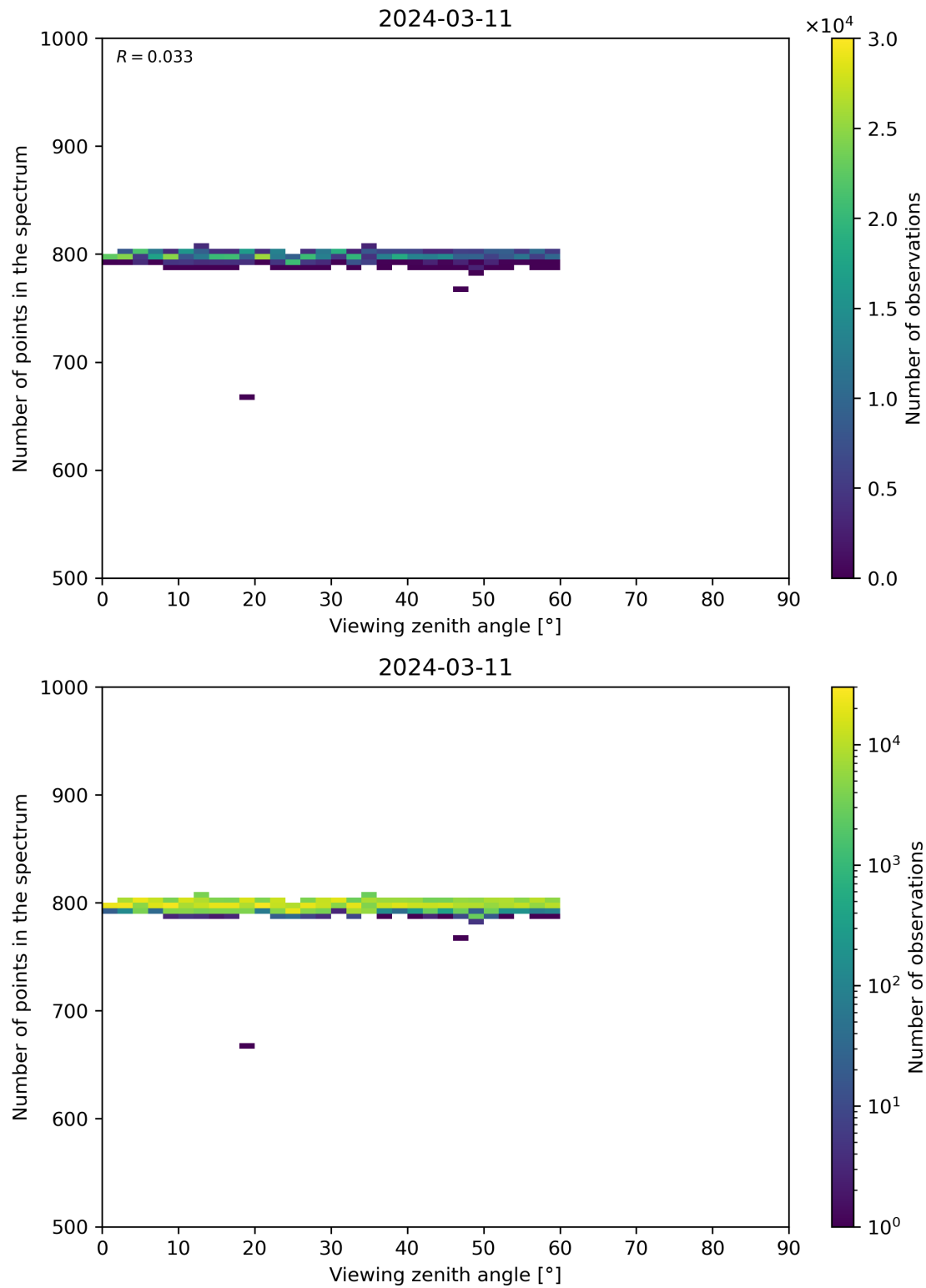
Figure 114: Scatter density plot of “Viewing zenith angle” against “Number of points in the spectrum” for 2024-03-10 to 2024-03-12.
