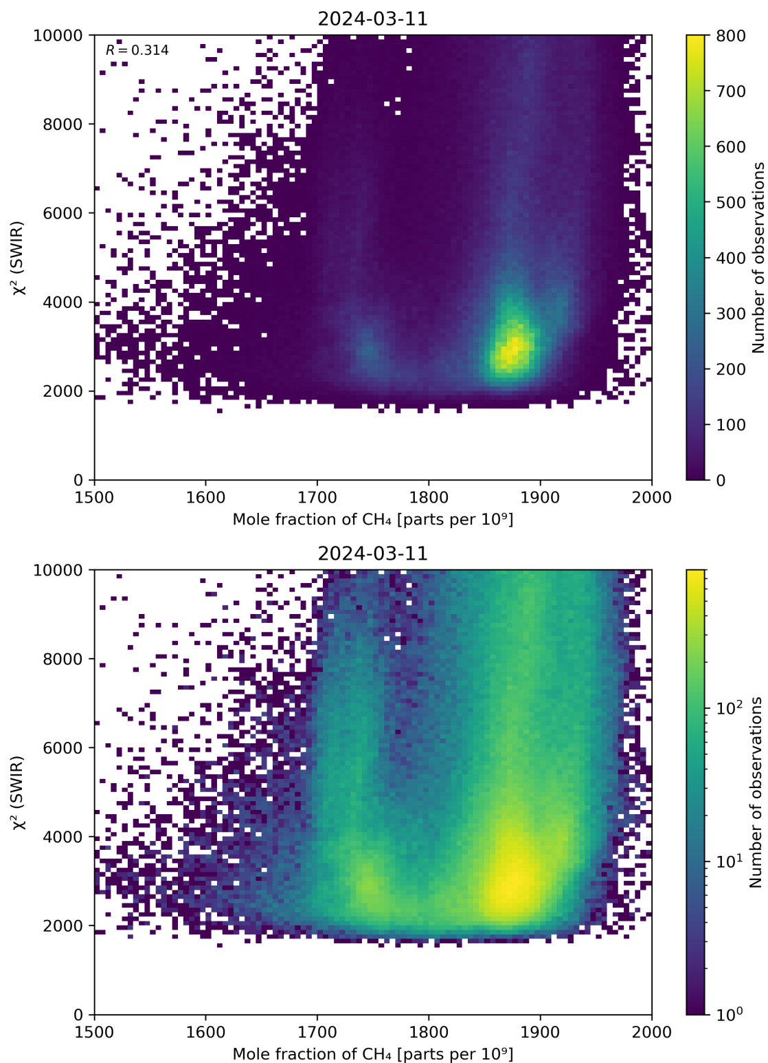
Figure 71: Scatter density plot of “Mole fraction of \text{CH}_4 ” against “ \chi^2 (SWIR)” for 2024-03-10 to 2024-03-12.
