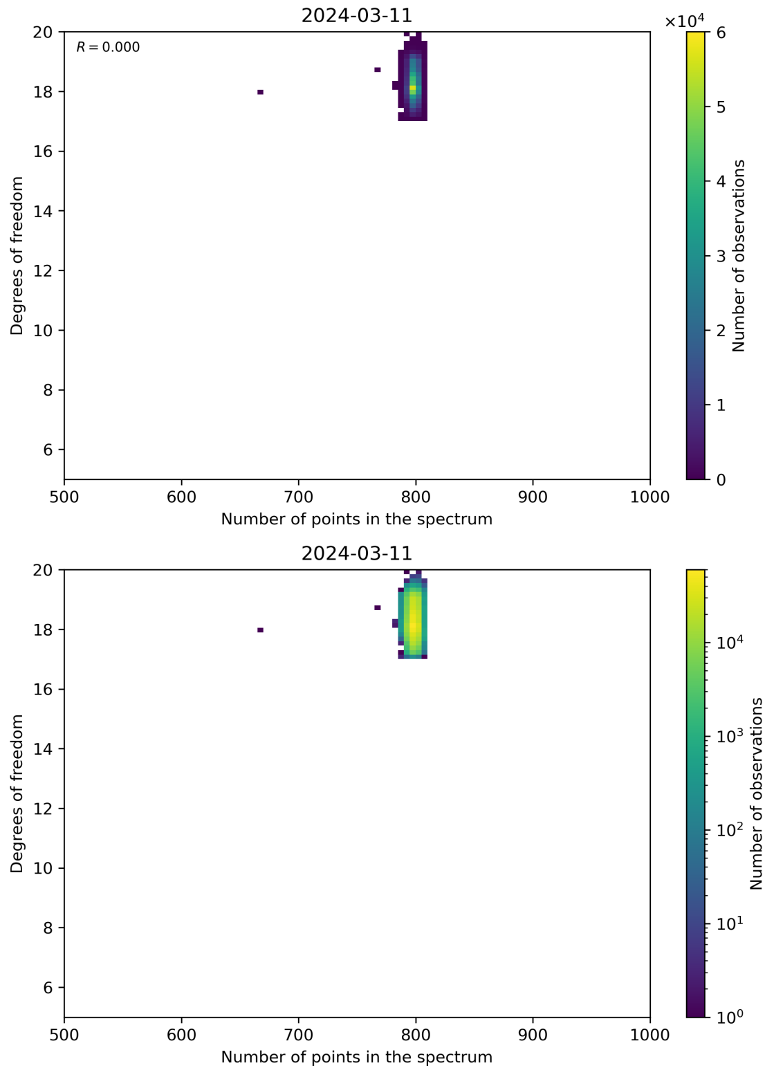
Figure 90: Scatter density plot of “Number of points in the spectrum” against “Degrees of freedom” for 2024-03-10 to 2024-03-12.
