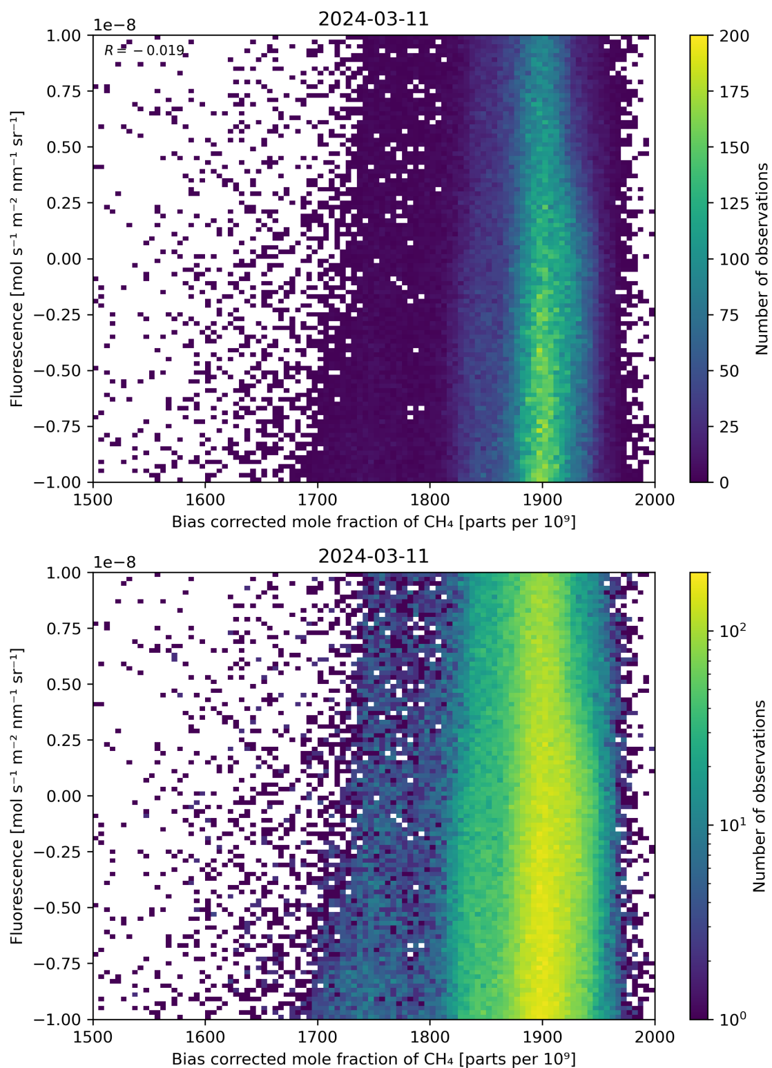
Figure 66: Scatter density plot of “Bias corrected mole fraction of \text{CH}_4 ” against “Fluorescence” for 2024-03-10 to 2024-03-12.
