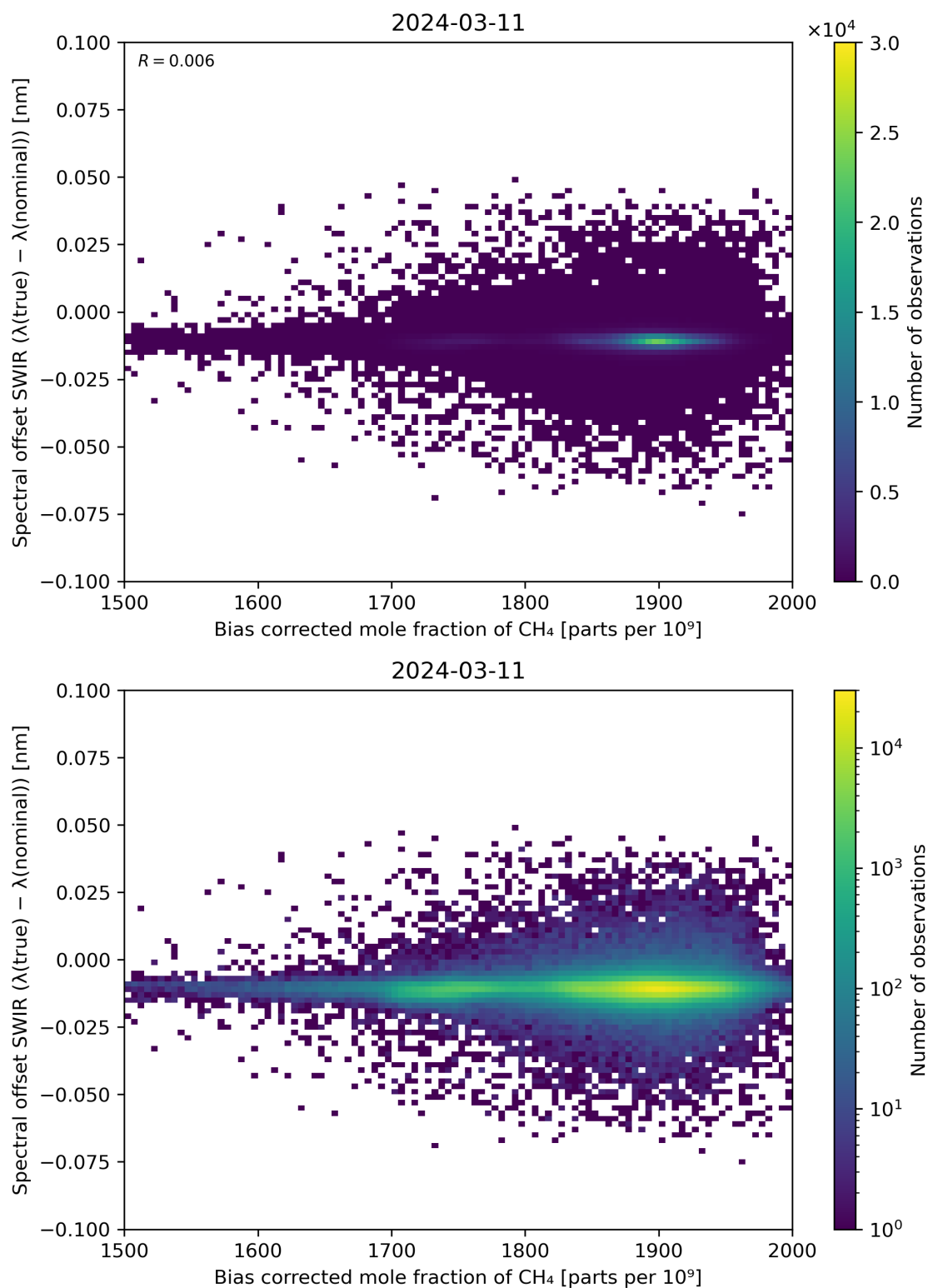
Figure 69: Scatter density plot of “Bias corrected mole fraction of \text{CH}_4 ” against “Spectral offset SWIR ( \lambda(\text{true}) - \lambda(\text{nominal}) )” for 2024-03-10 to 2024-03-12.
