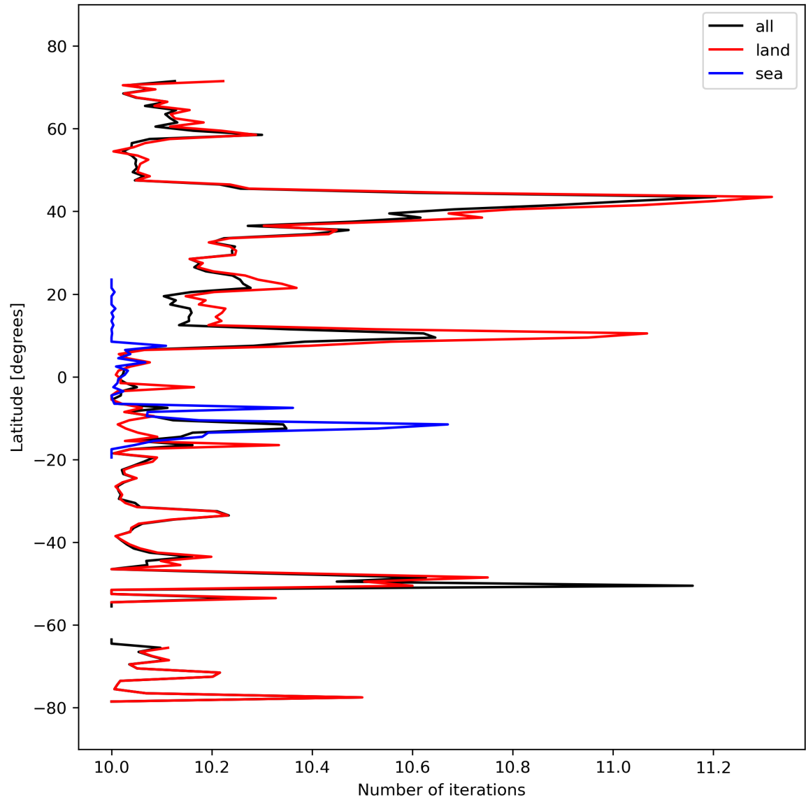
Figure 20: Zonal average of “Number of iterations” for 2024-03-10 to 2024-03-12.
