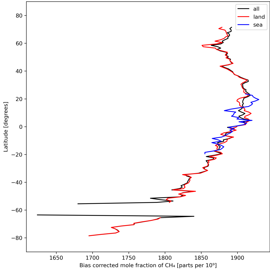
Figure 14: Zonal average of “Bias corrected mole fraction of CH 4 ” for 2024-03-10 to 2024-03-12.
