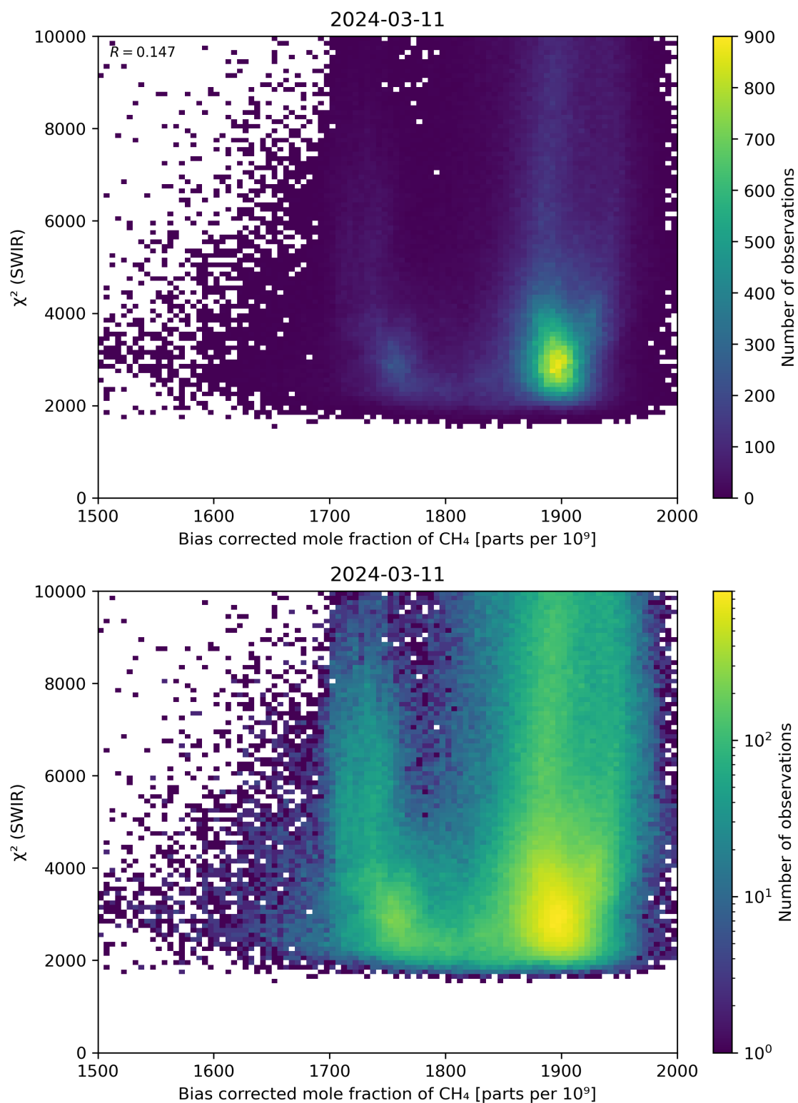
Figure 64: Scatter density plot of “Bias corrected mole fraction of \text{CH}_4 ” against “ \chi^2 (SWIR)” for 2024-03-10 to 2024-03-12.
