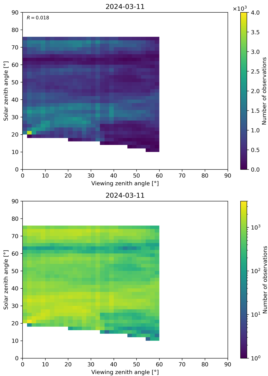
Figure 115: Scatter density plot of “Viewing zenith angle” against “Solar zenith angle” for 2024-03-10 to 2024-03-12.
