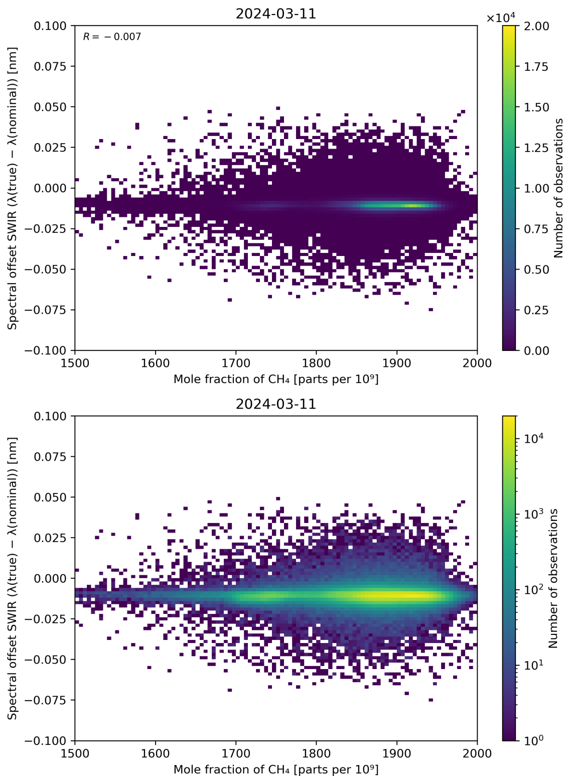
Figure 86: Scatter density plot of “Mole fraction of CH 4 ” against “Spectral offset SWIR ( \lambda(\text{true}) - \lambda(\text{nominal}) )” for 2024-03-10 to 2024-03-12.
