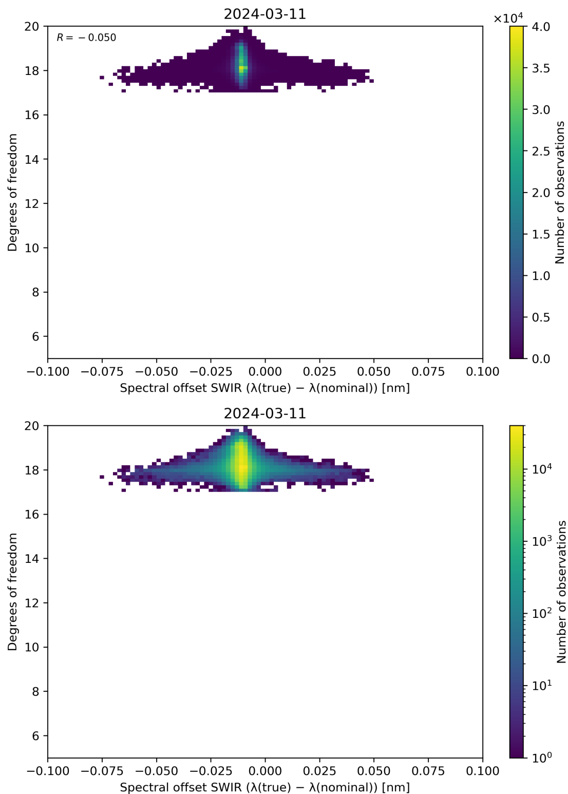
Figure 119: Scatter density plot of “Spectral offset SWIR ( \lambda(\text{true}) - \lambda(\text{nominal}) )” against “Degrees of freedom” for 2024-03-10 to 2024-03-12.
