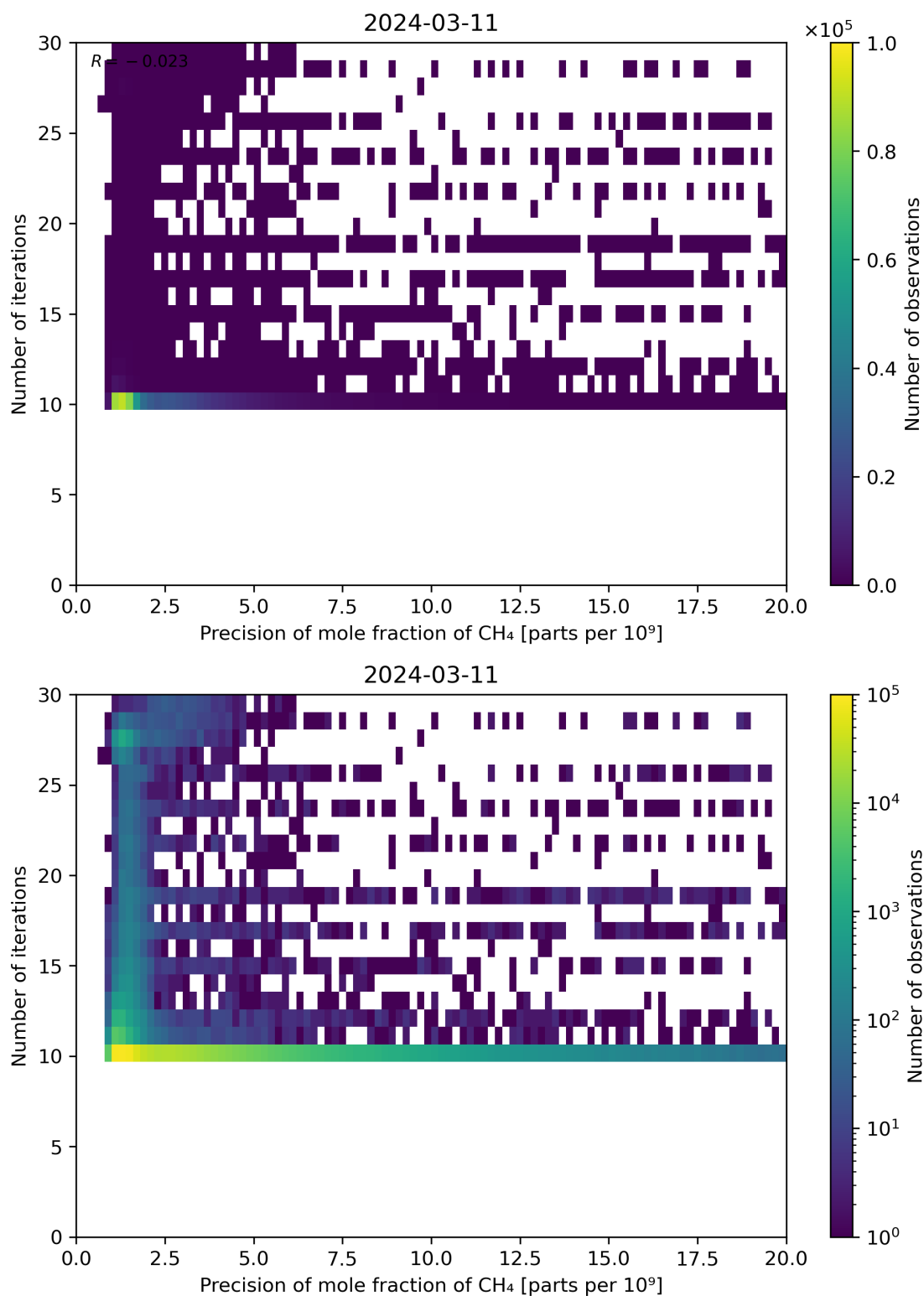
Figure 83: Scatter density plot of “Precision of mole fraction of CH 4 ” against “Number of iterations” for 2024-03-10 to 2024-03-12.
