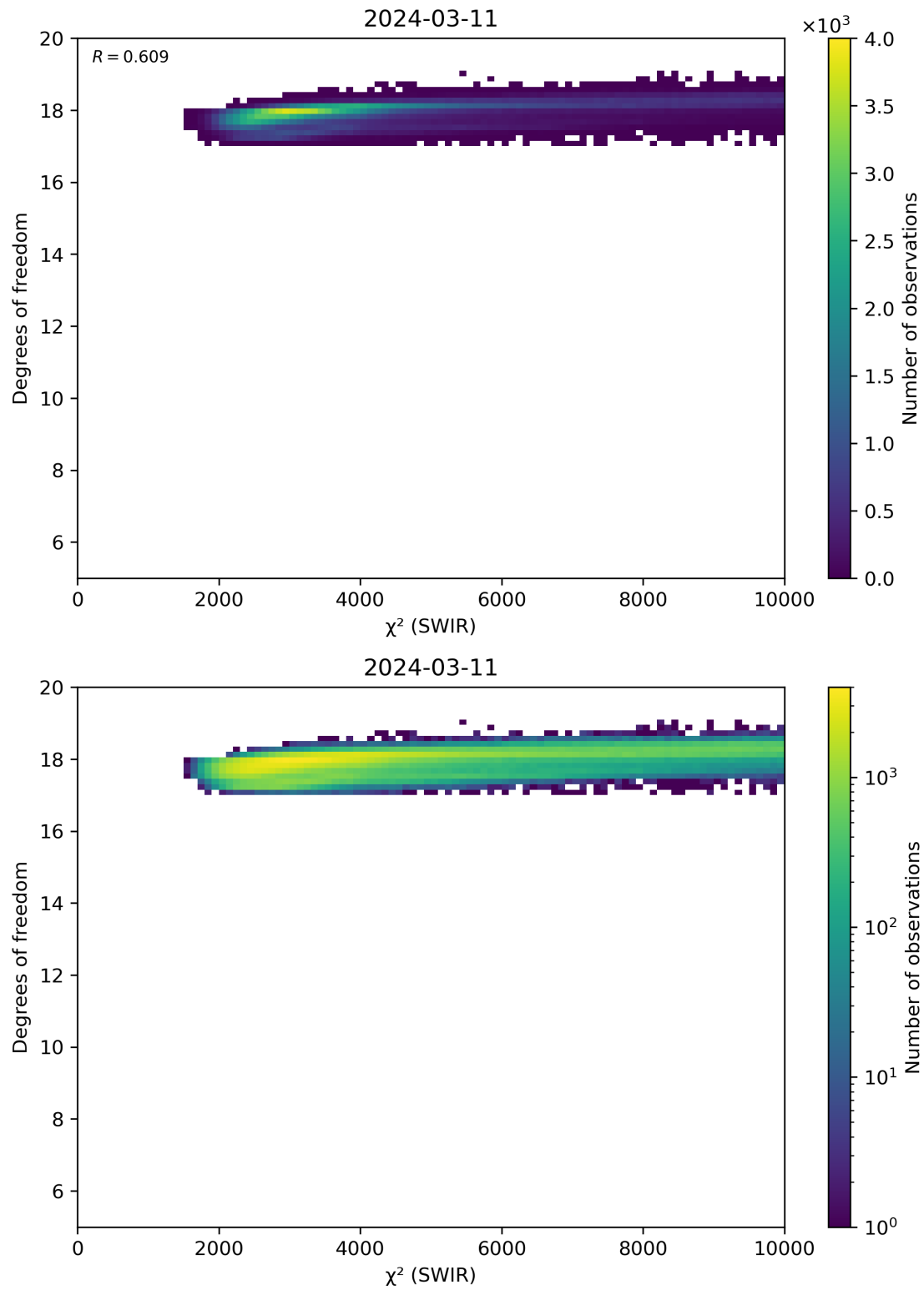
Figure 48: Scatter density plot of “ \chi^2 (SWIR)” against “Degrees of freedom” for 2024-03-10 to 2024-03-12.
