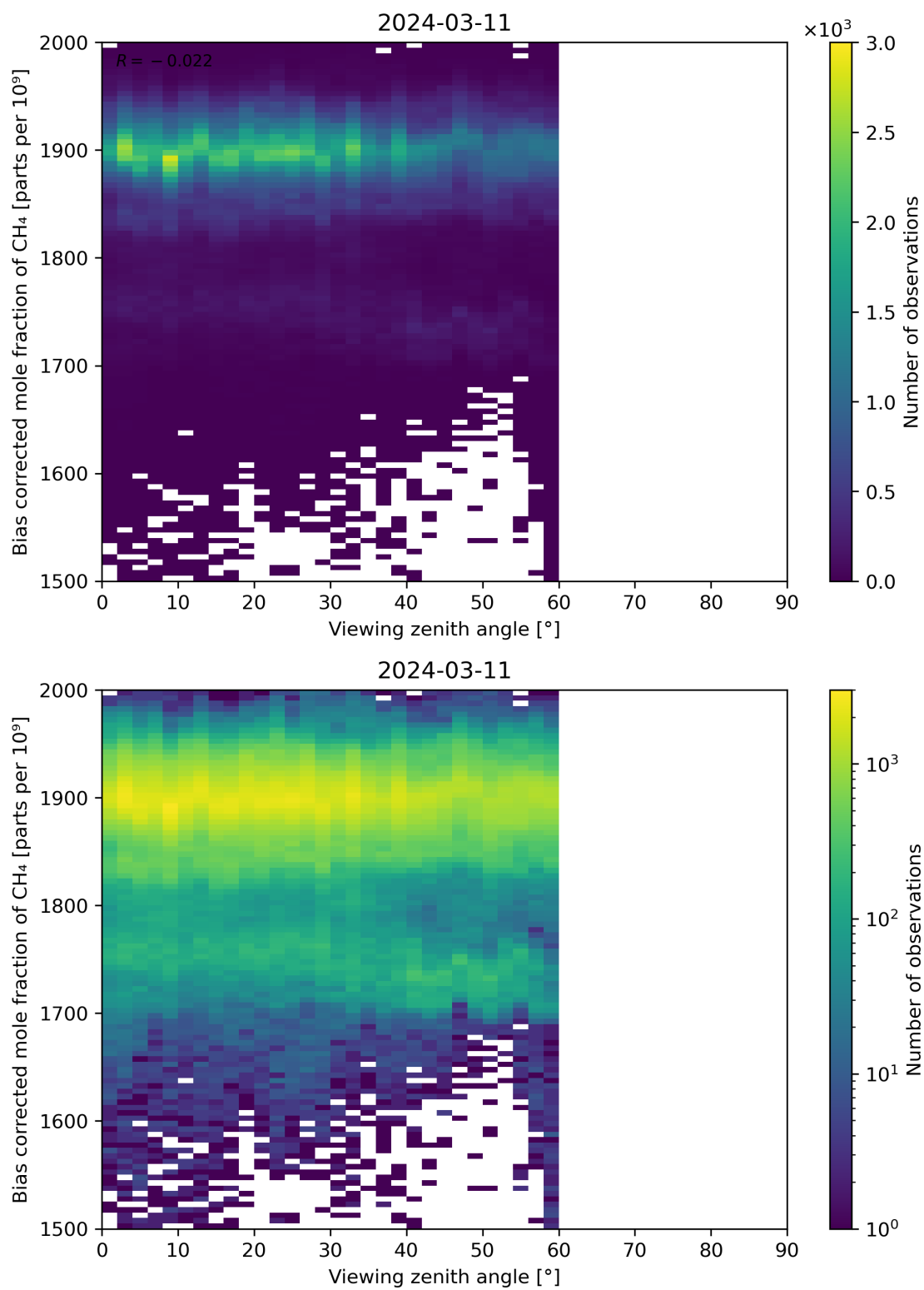
Figure 111: Scatter density plot of “Viewing zenith angle” against “Bias corrected mole fraction of CH 4 ” for 2024-03-10 to 2024-03-12.
