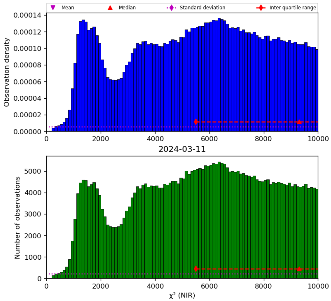
Figure 29: Histogram of “ \chi^2 (NIR)” for 2024-03-10 to 2024-03-12
