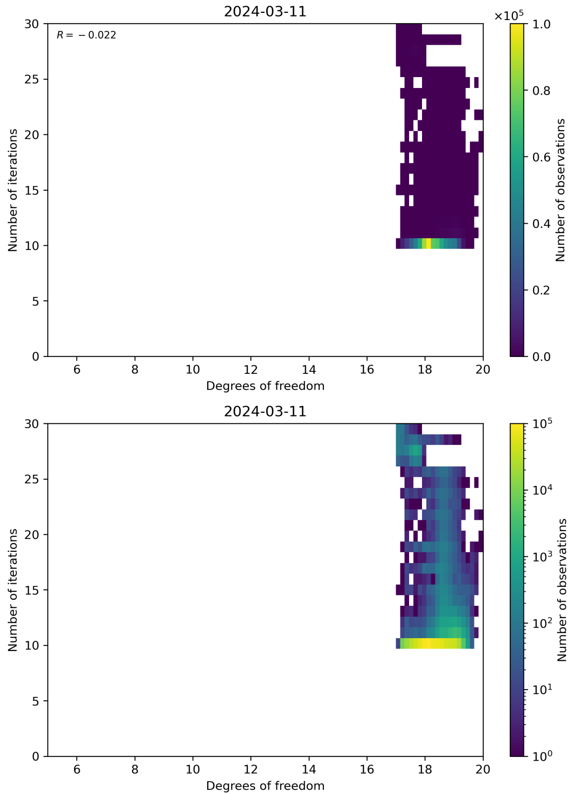
Figure 52: Scatter density plot of “Degrees of freedom” against “Number of iterations” for 2024-03-10 to 2024-03-12.
