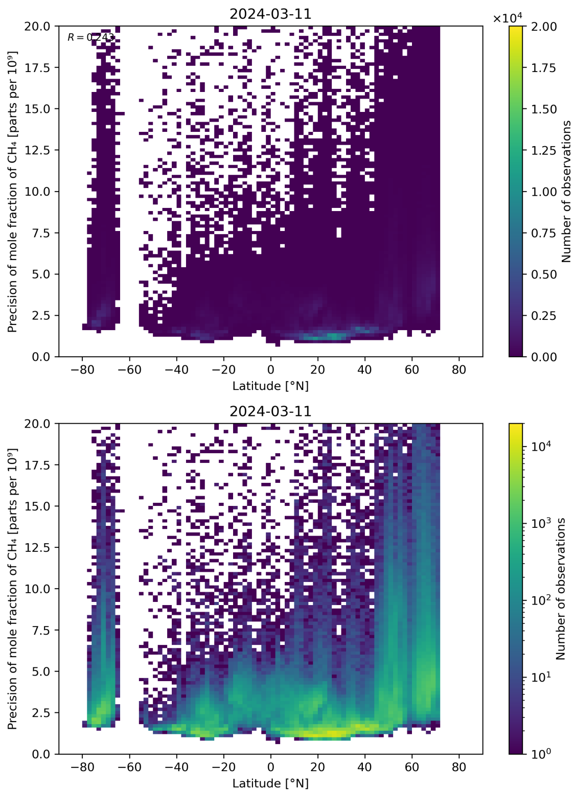
Figure 59: Scatter density plot of “Latitude” against “Precision of mole fraction of CH 4 ” for 2024-03-10 to 2024-03-12.
