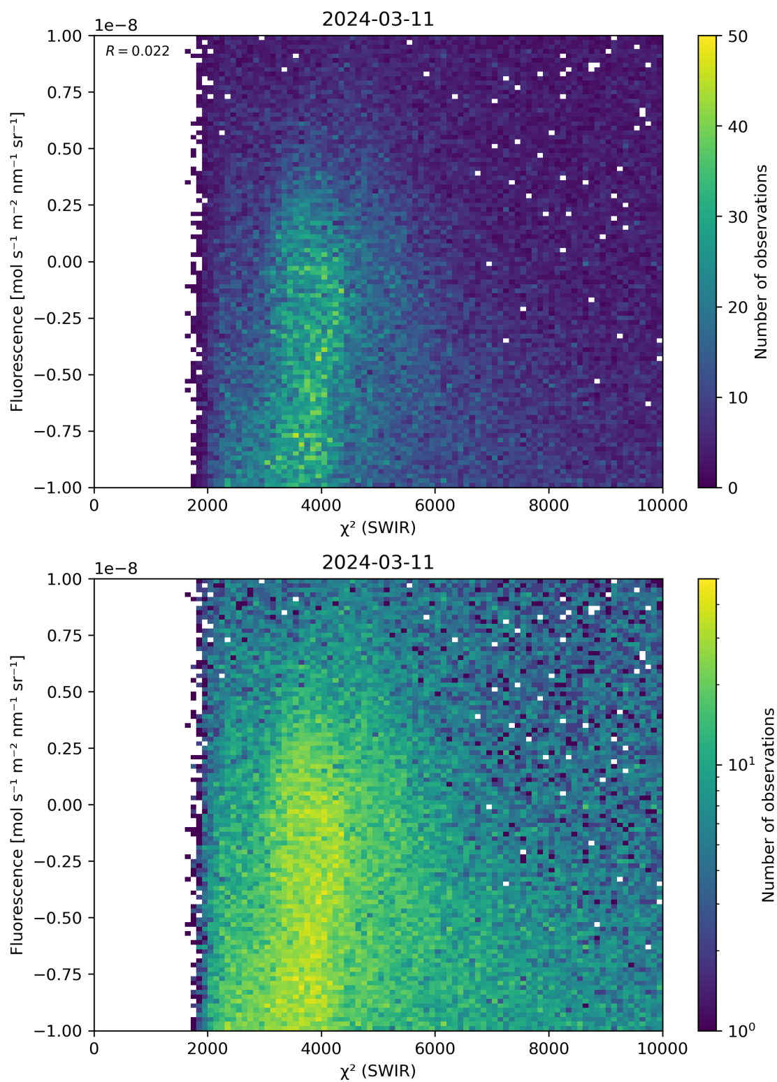
Figure 49: Scatter density plot of “ \chi^2 (SWIR)” against “Fluorescence” for 2024-03-10 to 2024-03-12.
