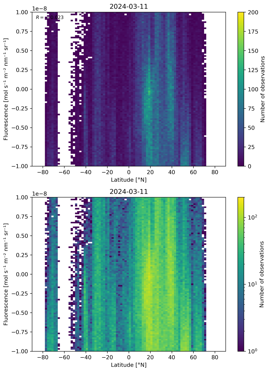
Figure 56: Scatter density plot of “Latitude” against “Fluorescence” for 2024-03-10 to 2024-03-12.
