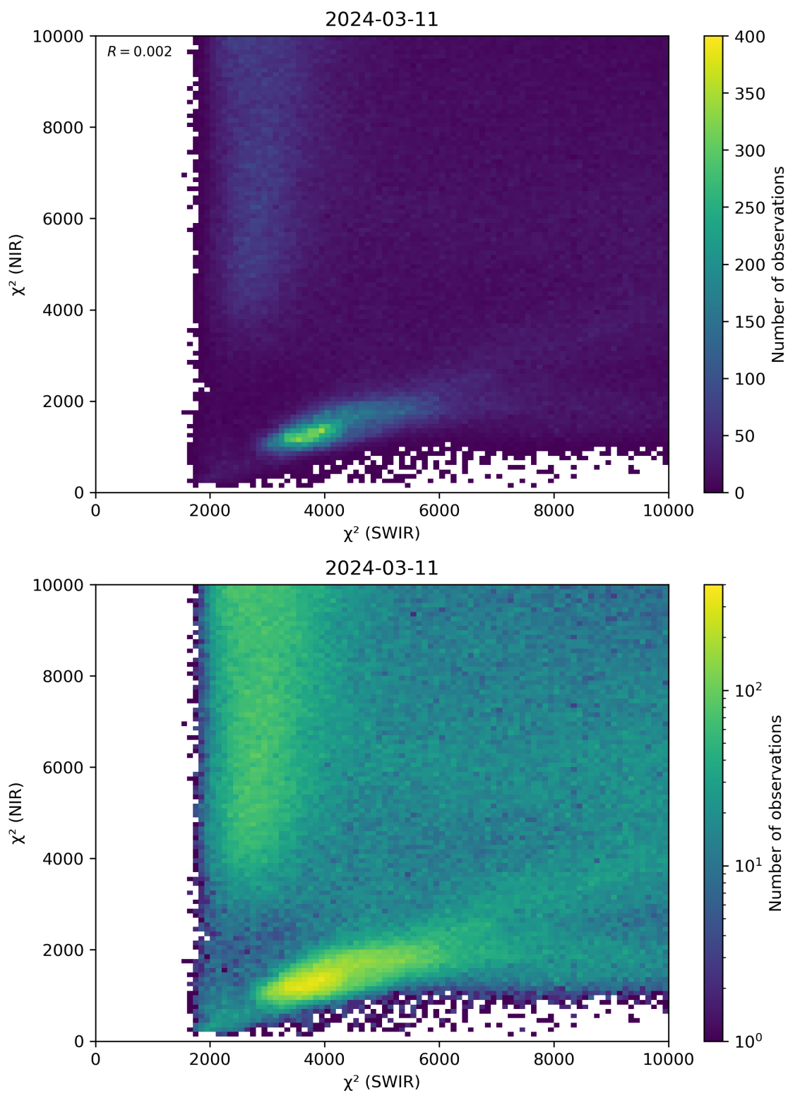
Figure 47: Scatter density plot of “ \chi^2 (SWIR)” against “ \chi^2 (NIR)” for 2024-03-10 to 2024-03-12.
