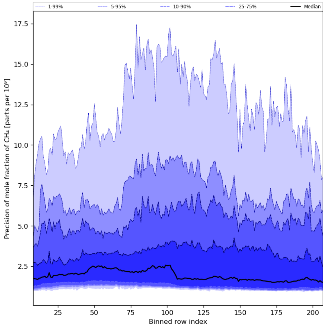
Figure 35: Along track statistics of “Precision of mole fraction of CH 4 ” for 2024-03-10 to 2024-03-12
