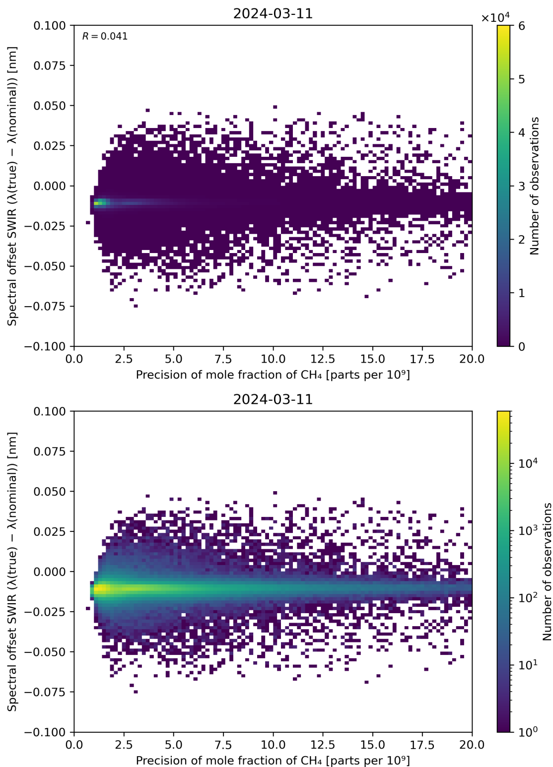
Figure 85: Scatter density plot of “Precision of mole fraction of \text{CH}_4 ” against “Spectral offset SWIR ( \lambda(\text{true}) - \lambda(\text{nominal}) )” for 2024-03-10 to 2024-03-12.
