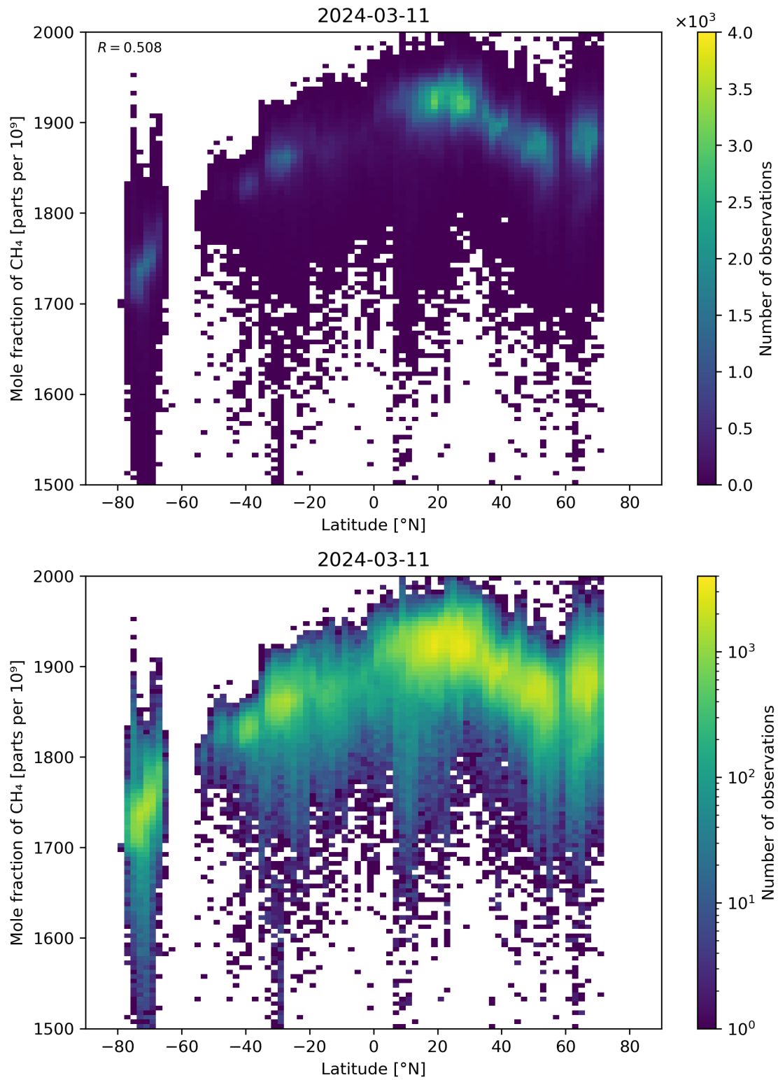
Figure 57: Scatter density plot of “Latitude” against “Mole fraction of CH 4 ” for 2024-03-10 to 2024-03-12.
