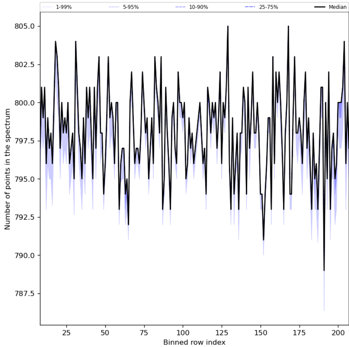
Figure 37: Along track statistics of “Number of points in the spectrum” for 2024-03-10 to 2024-03-12
