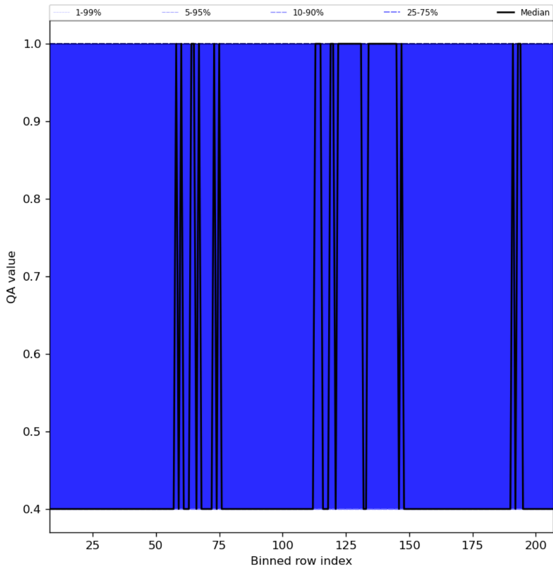
Figure 33: Along track statistics of “QA value” for 2024-03-10 to 2024-03-12
