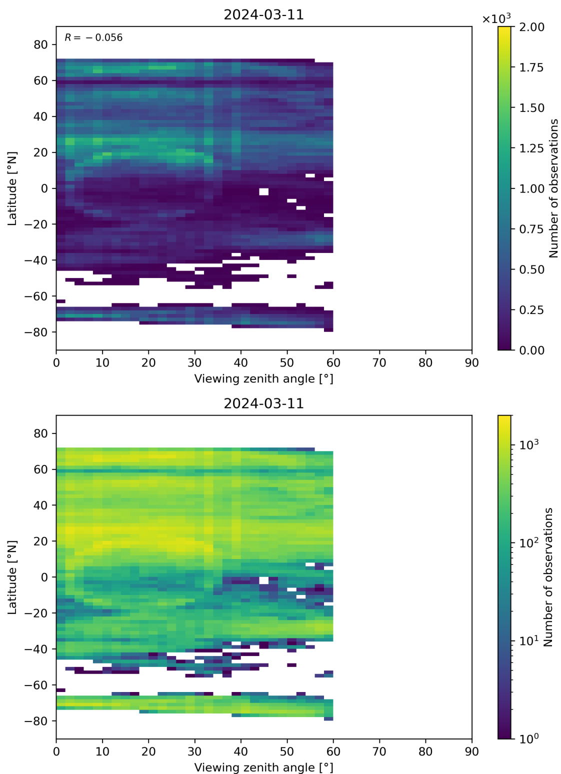
Figure 109: Scatter density plot of “Viewing zenith angle” against “Latitude” for 2024-03-10 to 2024-03-12.
