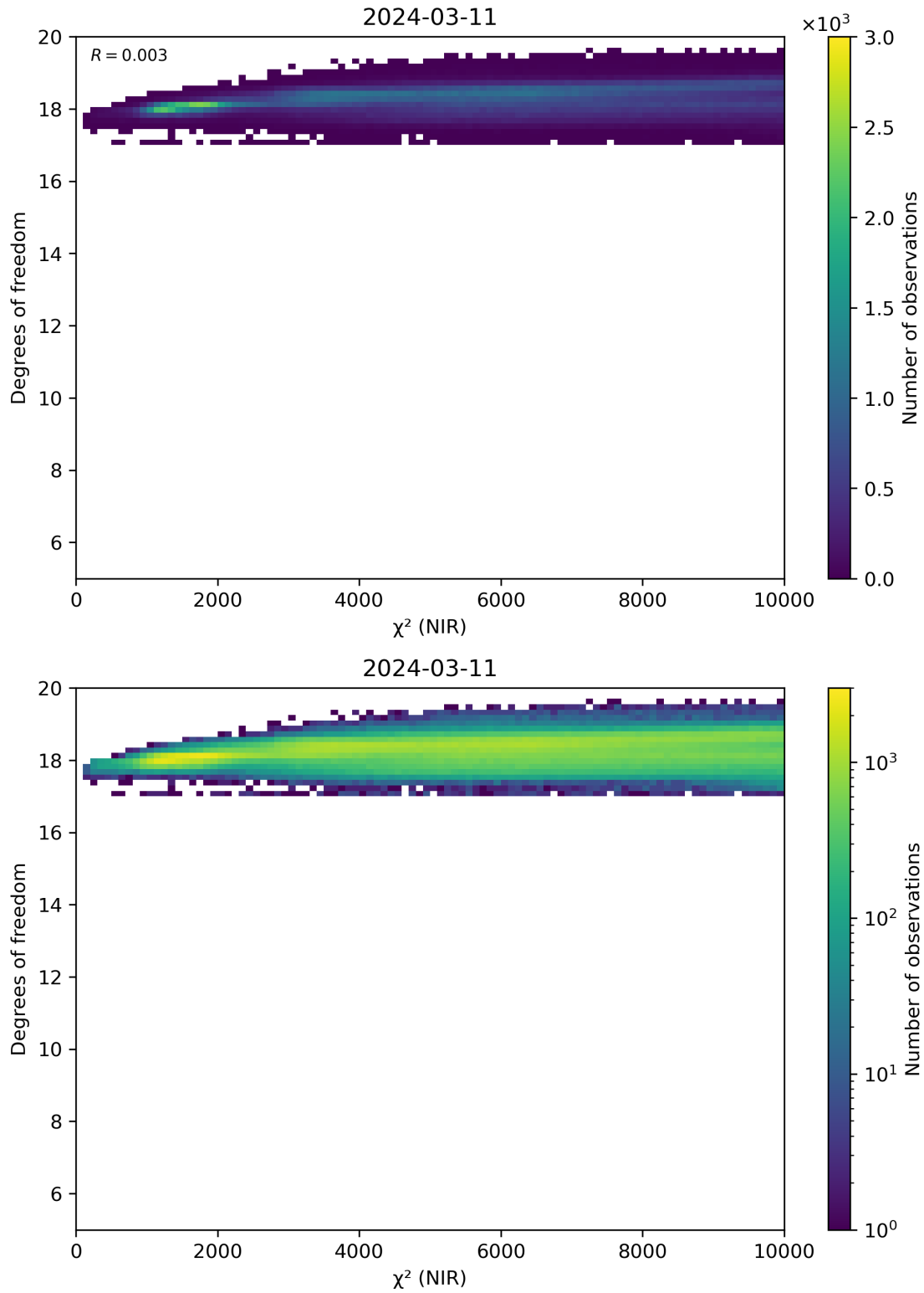
Figure 44: Scatter density plot of “ \chi^2 (NIR)” against “Degrees of freedom” for 2024-03-10 to 2024-03-12.
