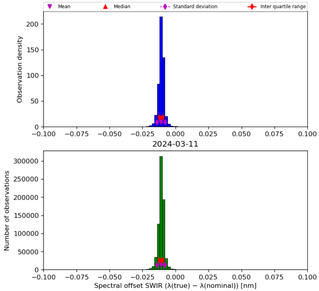
Figure 27: Histogram of “Spectral offset SWIR ( \lambda(\text{true}) - \lambda(\text{nominal}) )” for 2024-03-10 to 2024-03-12
