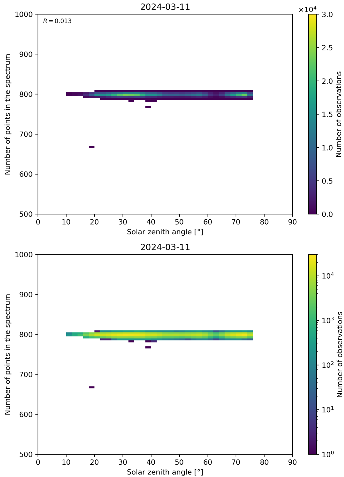
Figure 103: Scatter density plot of “Solar zenith angle” against “Number of points in the spectrum” for 2024-03-10 to 2024-03-12.
