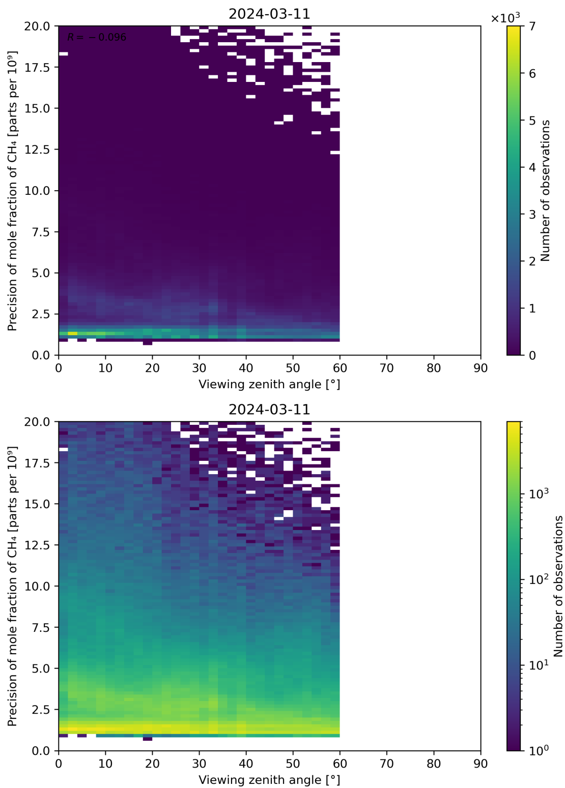
Figure 112: Scatter density plot of “Viewing zenith angle” against “Precision of mole fraction of CH 4 ” for 2024-03-10 to 2024-03-12.
