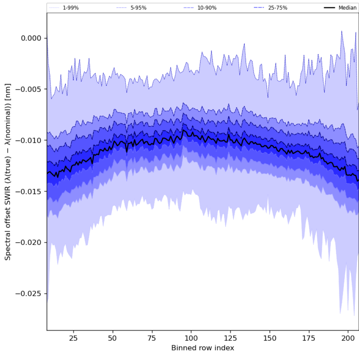
Figure 38: Along track statistics of “Spectral offset SWIR ( \lambda(\text{true}) - \lambda(\text{nominal}) )” for 2024-03-10 to 2024-03-12
