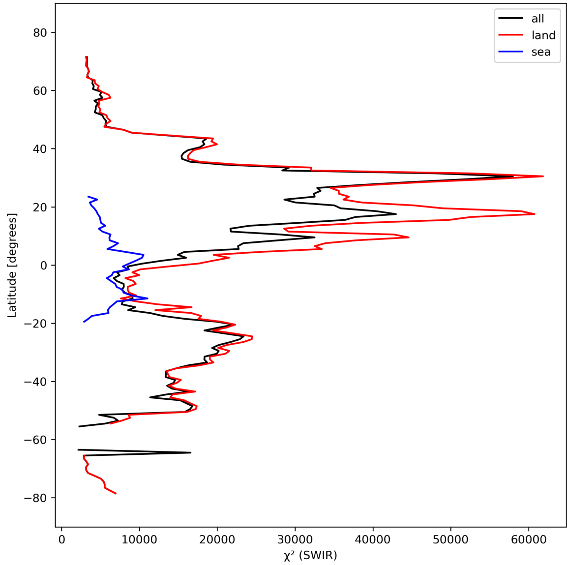
Figure 17: Zonal average of “ \chi^2 (SWIR)” for 2024-03-10 to 2024-03-12.
