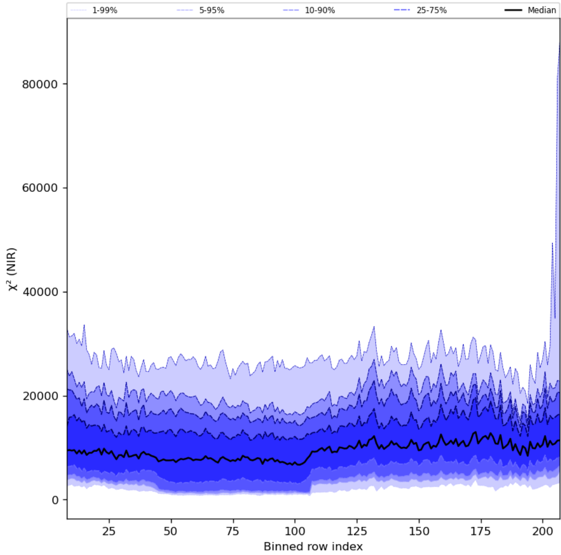
Figure 40: Along track statistics of “ \chi^2 (NIR)” for 2024-03-10 to 2024-03-12
