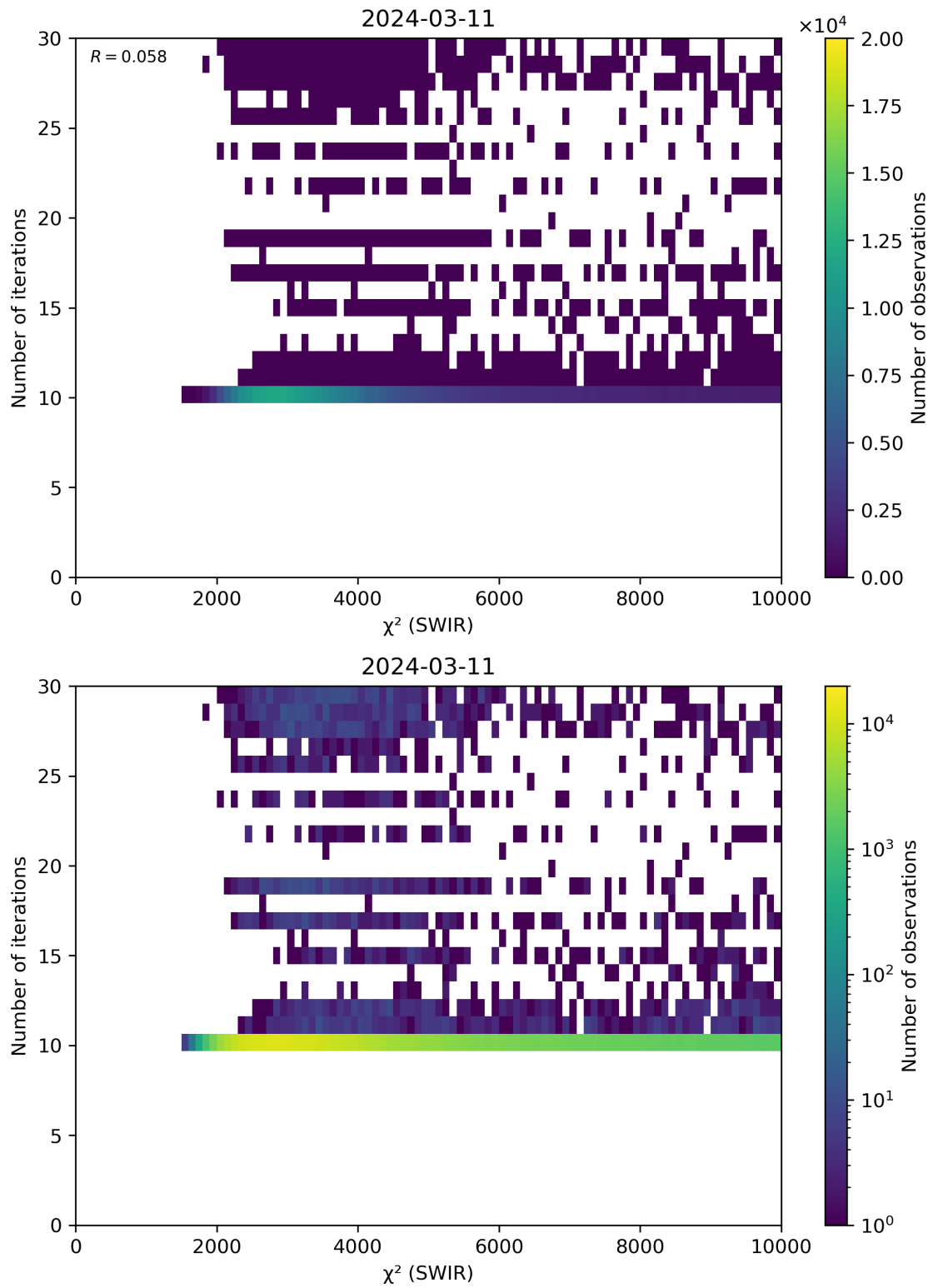
Figure 50: Scatter density plot of “ \chi^2 (SWIR)” against “Number of iterations” for 2024-03-10 to 2024-03-12.
