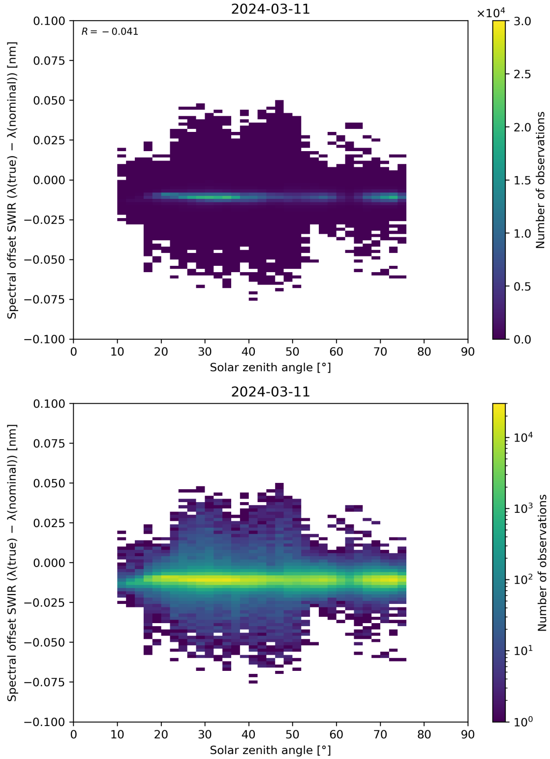
Figure 104: Scatter density plot of “Solar zenith angle” against “Spectral offset SWIR ( \lambda(\text{true}) - \lambda(\text{nominal}) )” for 2024-03-10 to 2024-03-12.
