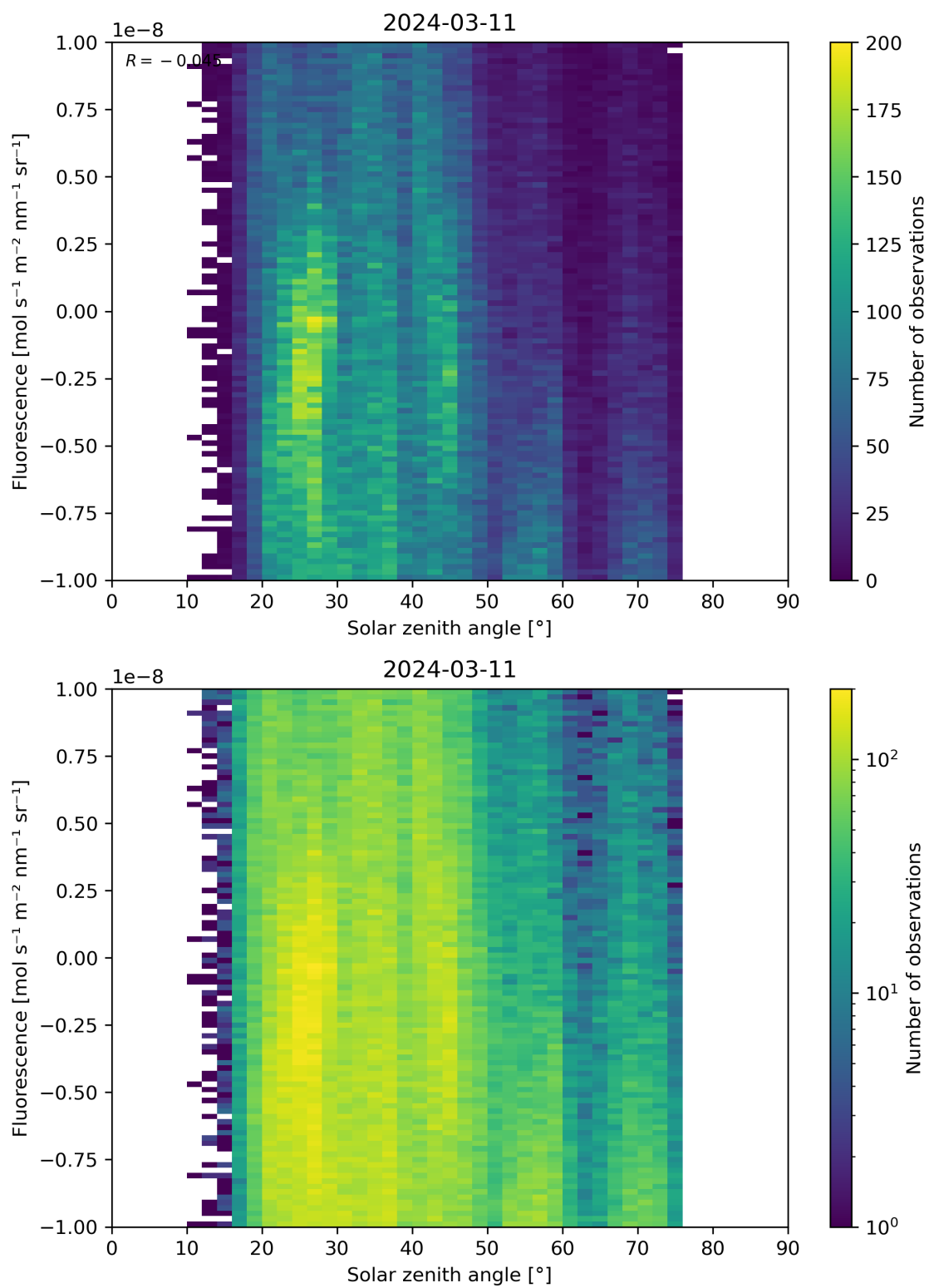
Figure 97: Scatter density plot of “Solar zenith angle” against “Fluorescence” for 2024-03-10 to 2024-03-12.
