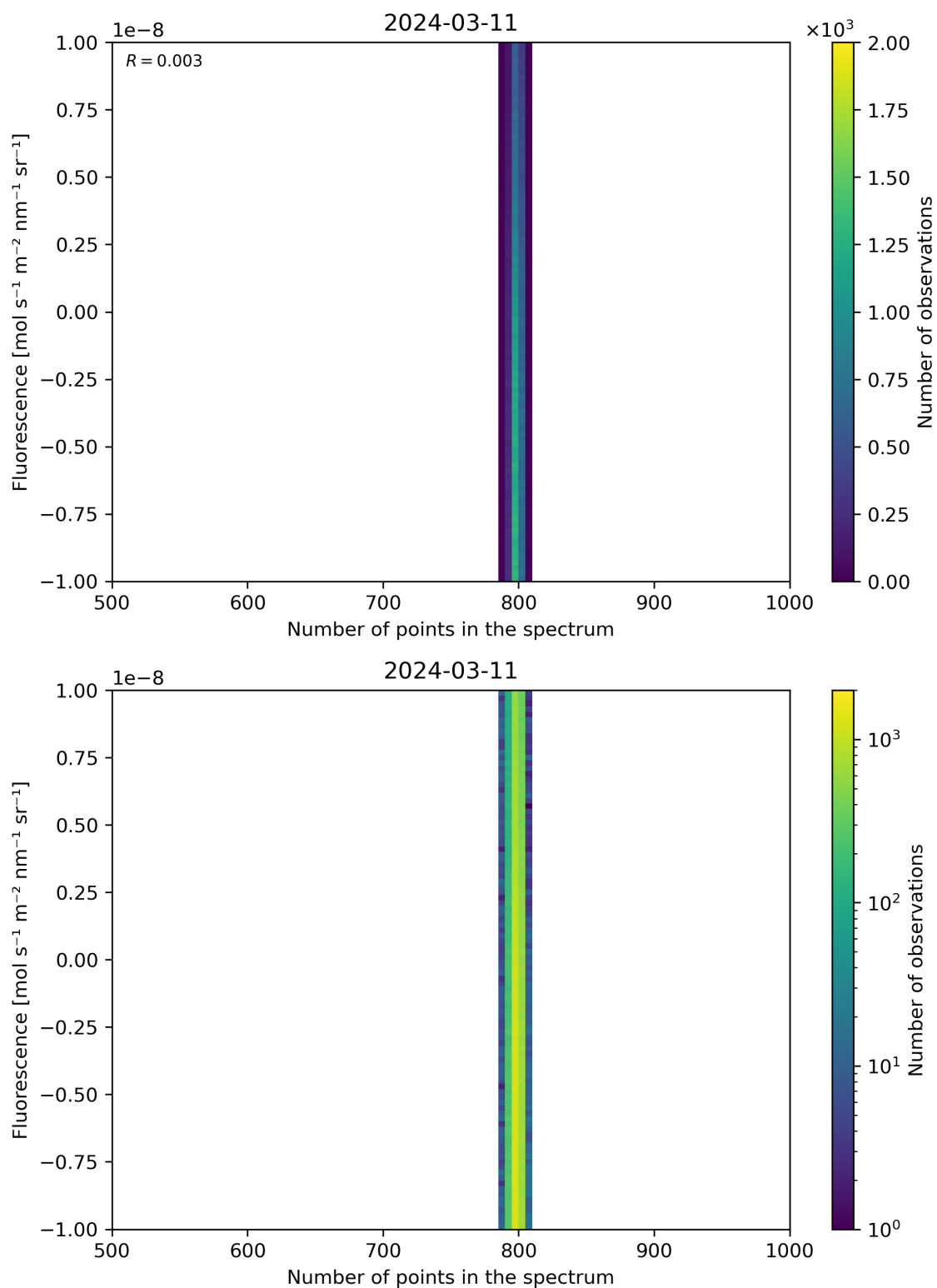
Figure 91: Scatter density plot of “Number of points in the spectrum” against “Fluorescence” for 2024-03-10 to 2024-03-12.
