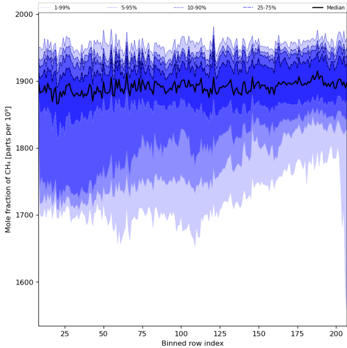
Figure 34: Along track statistics of “Mole fraction of CH 4 ” for 2024-03-10 to 2024-03-12
