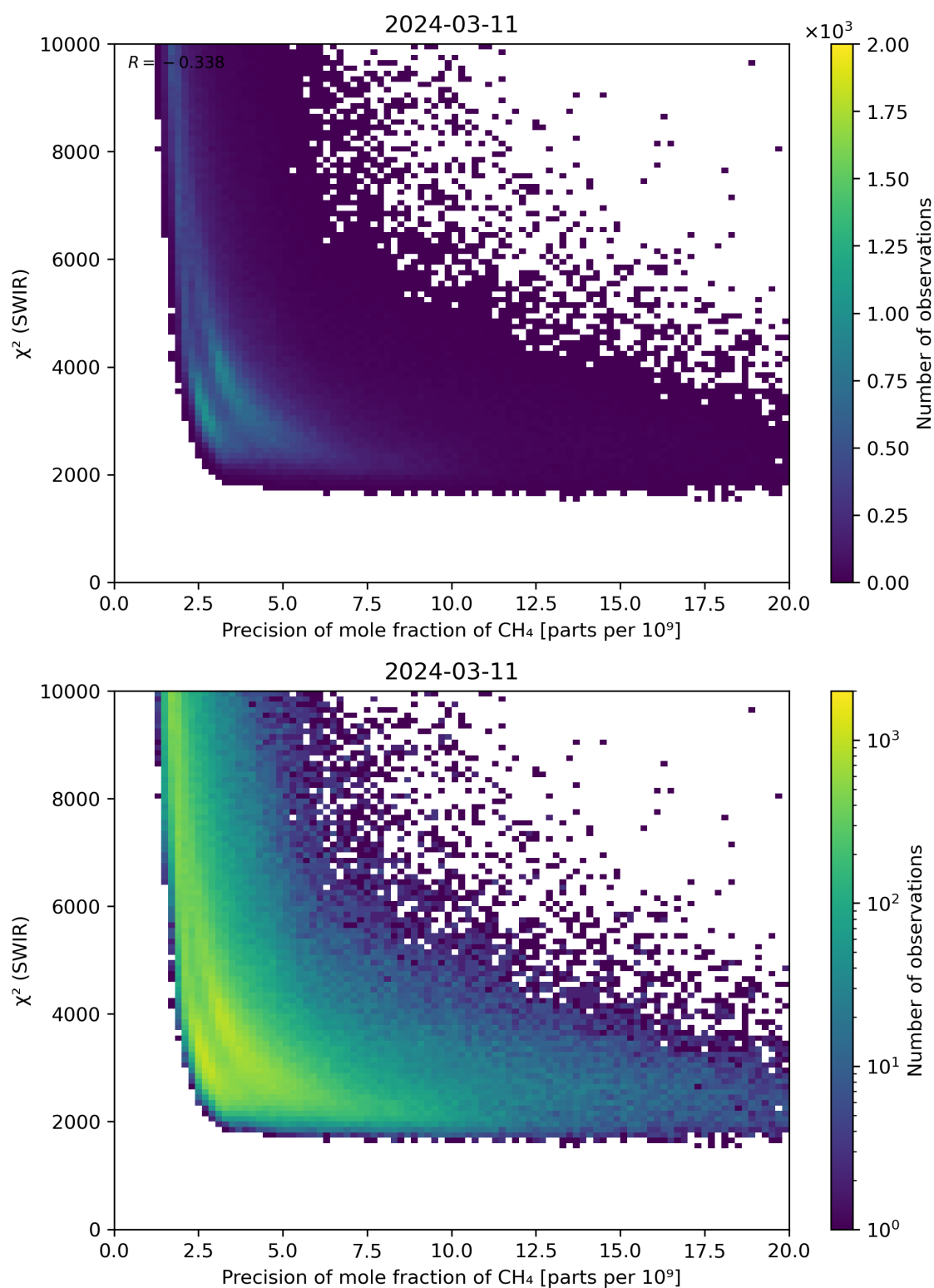
Figure 79: Scatter density plot of “Precision of mole fraction of CH 4 ” against “ \chi^2 (SWIR)” for 2024-03-10 to 2024-03-12.
