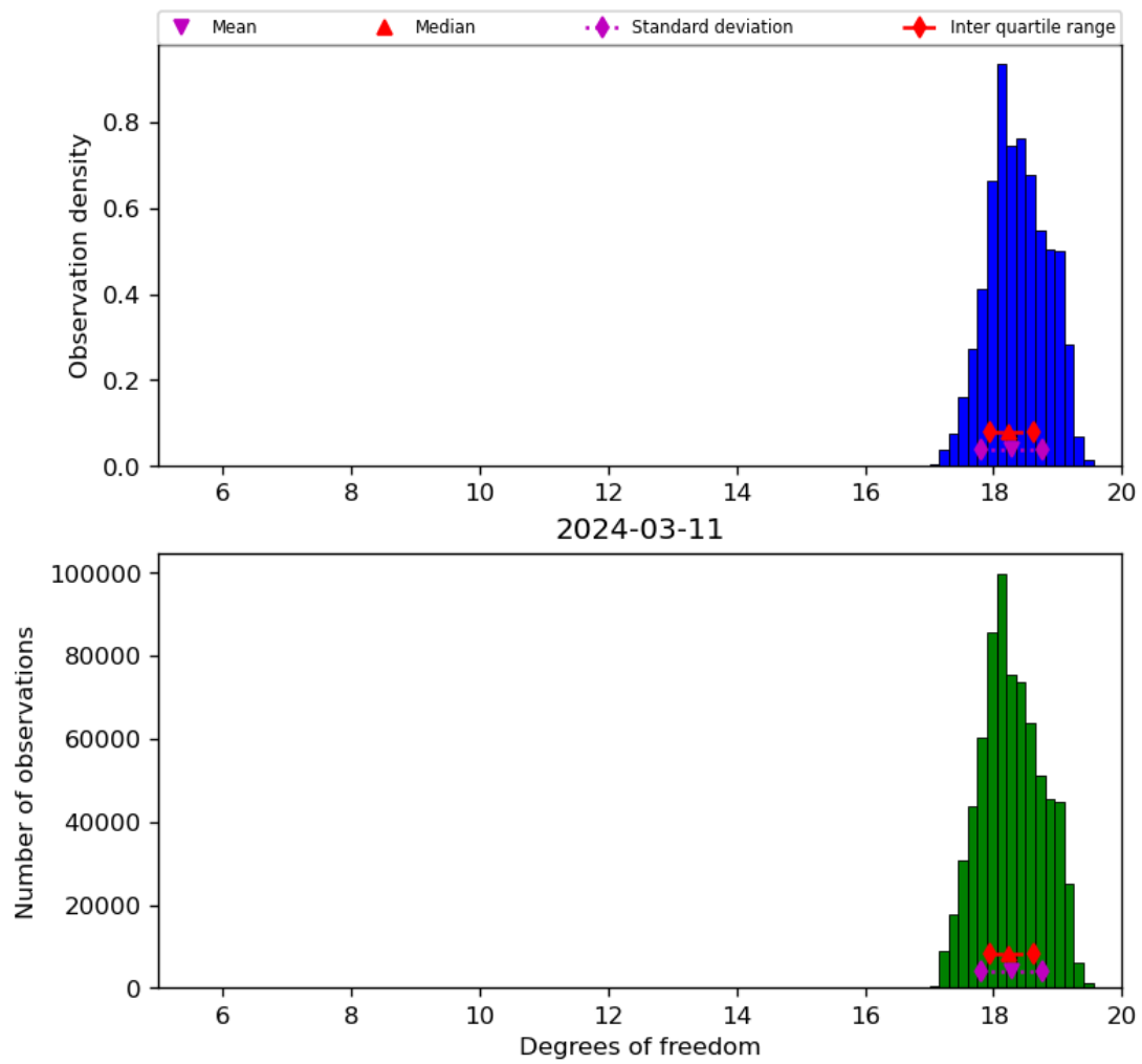
Figure 30: Histogram of “Degrees of freedom” for 2024-03-10 to 2024-03-12
