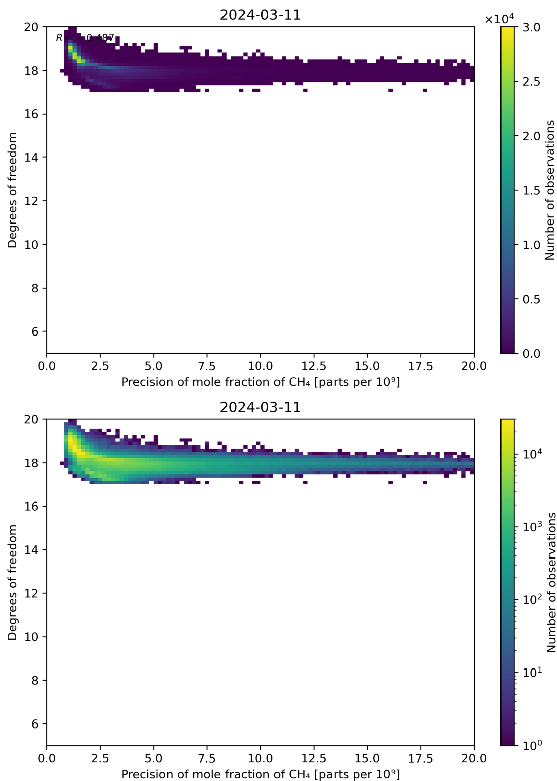
Figure 80: Scatter density plot of “Precision of mole fraction of CH 4 ” against “Degrees of freedom” for 2024-03-10 to 2024-03-12.
