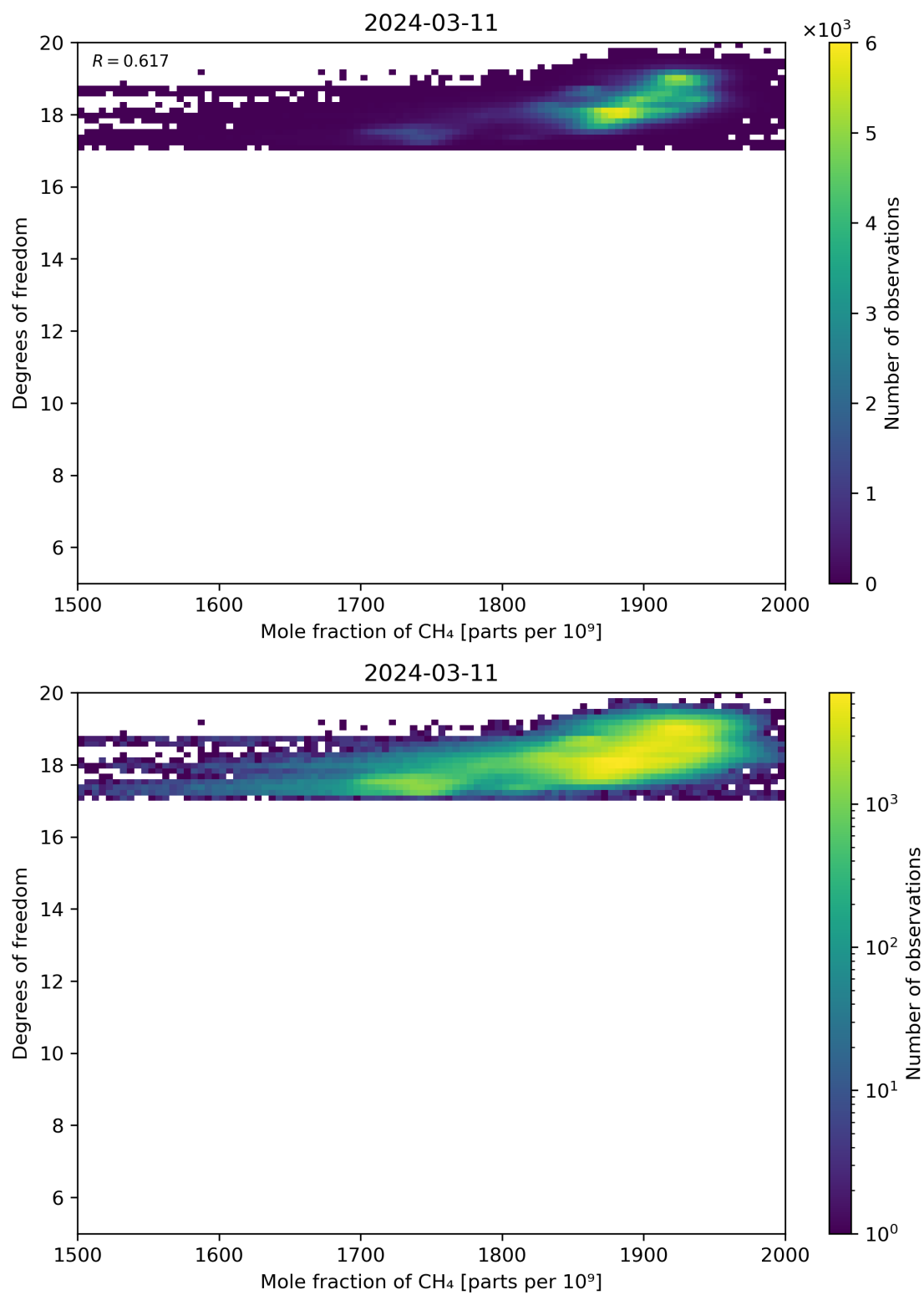
Figure 72: Scatter density plot of “Mole fraction of CH 4 ” against “Degrees of freedom” for 2024-03-10 to 2024-03-12.
