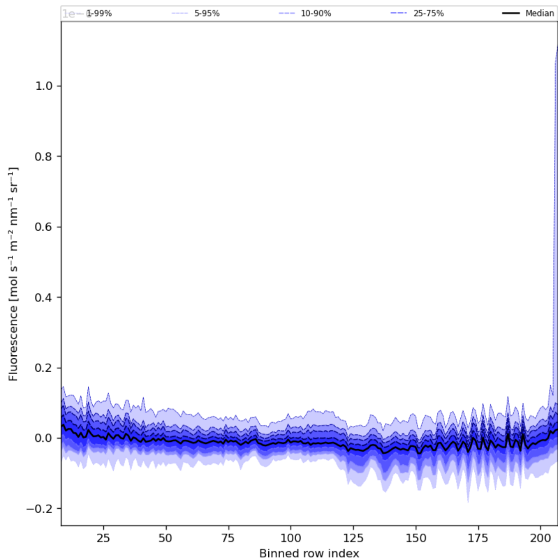
Figure 43: Along track statistics of “Fluorescence” for 2024-03-10 to 2024-03-12
