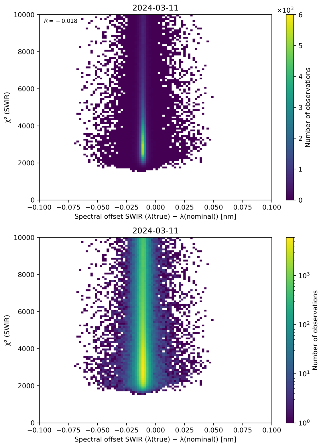
Figure 118: Scatter density plot of “Spectral offset SWIR ( \lambda(\text{true}) - \lambda(\text{nominal}) )” against “ \chi^2 (SWIR)” for 2024-03-10 to 2024-03-12.
