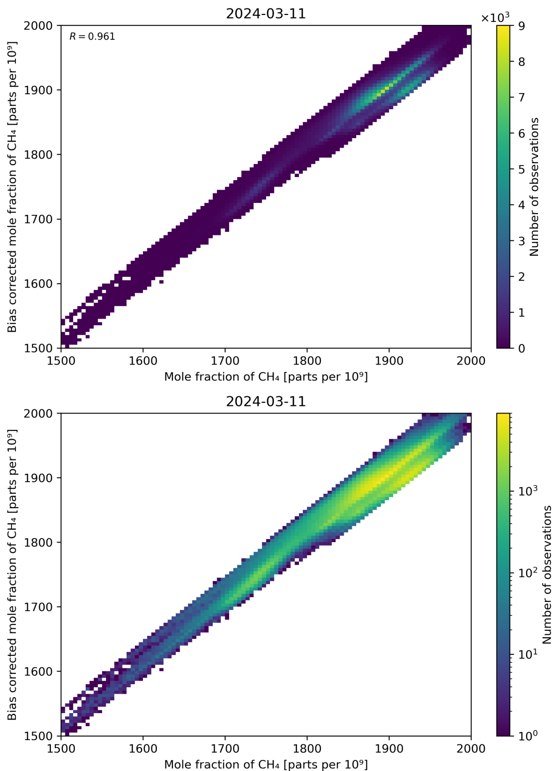
Figure 74: Scatter density plot of “Mole fraction of CH 4 ” against “Bias corrected mole fraction of CH 4 ” for 2024-03-10 to 2024-03-12.
