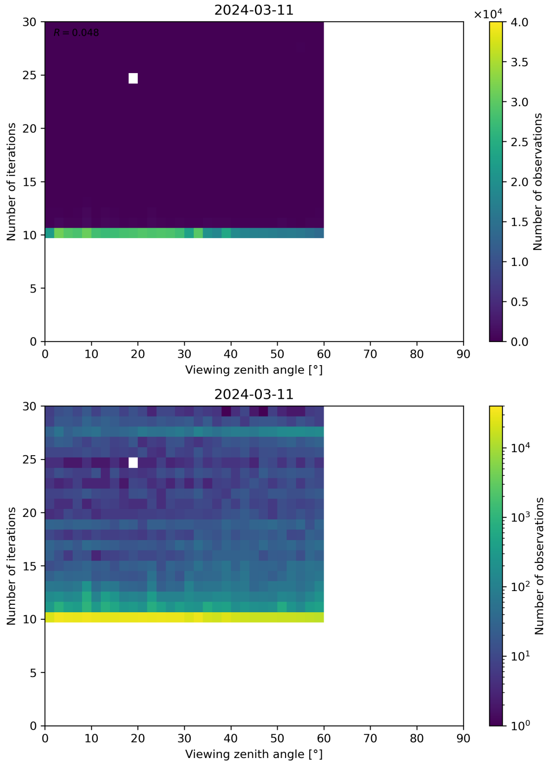
Figure 113: Scatter density plot of “Viewing zenith angle” against “Number of iterations” for 2024-03-10 to 2024-03-12.
