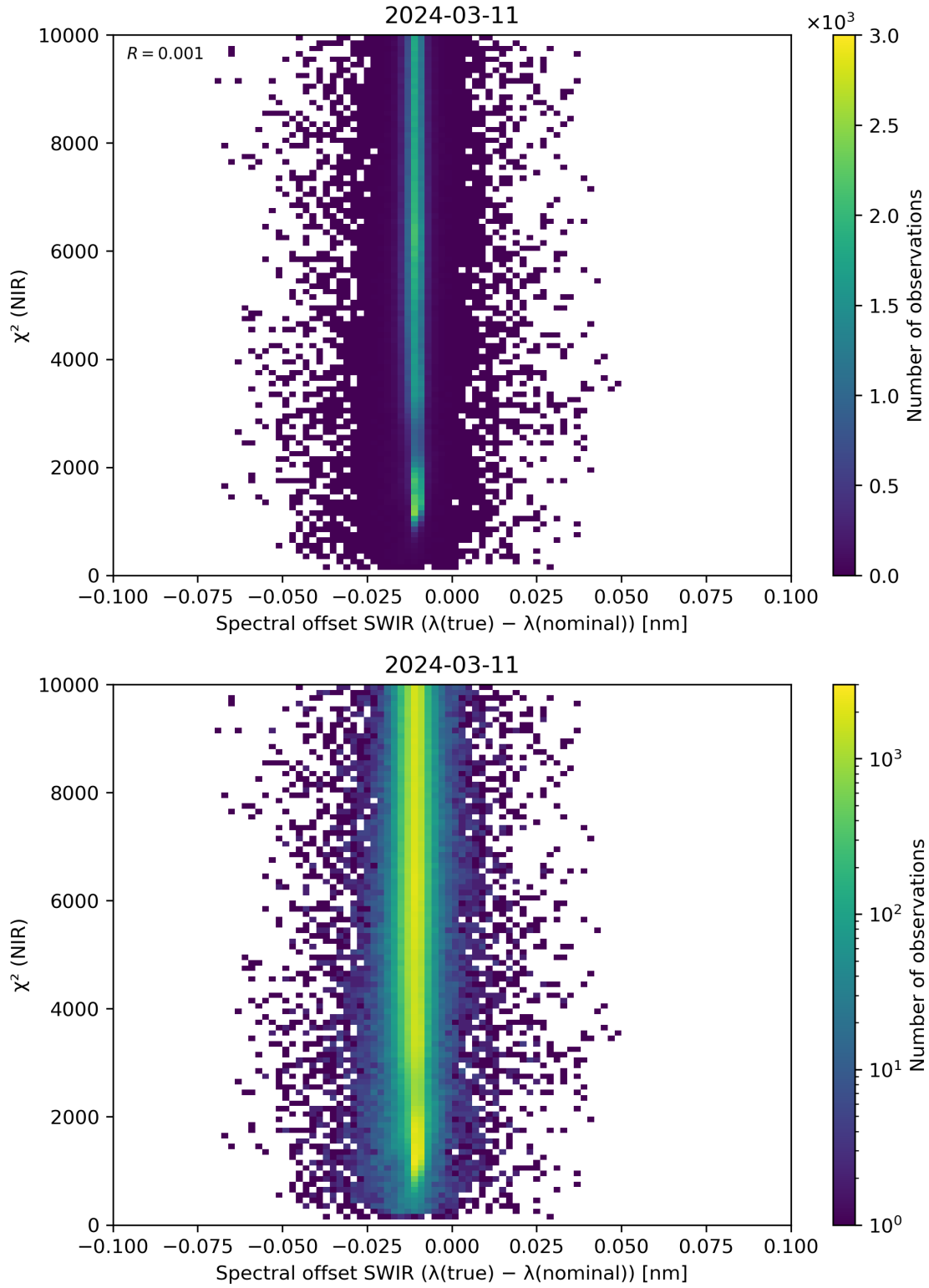
Figure 117: Scatter density plot of “Spectral offset SWIR ( \lambda(\text{true}) - \lambda(\text{nominal}) )” against “ \chi^2 (NIR)” for 2024-03-10 to 2024-03-12.
