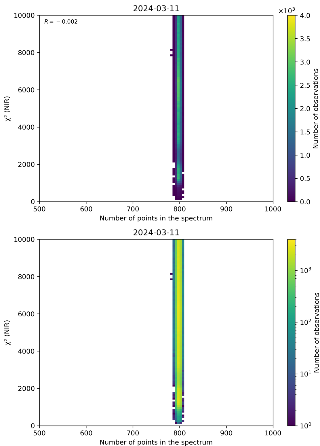
Figure 88: Scatter density plot of “Number of points in the spectrum” against “ \chi^2 (NIR)” for 2024-03-10 to 2024-03-12.
