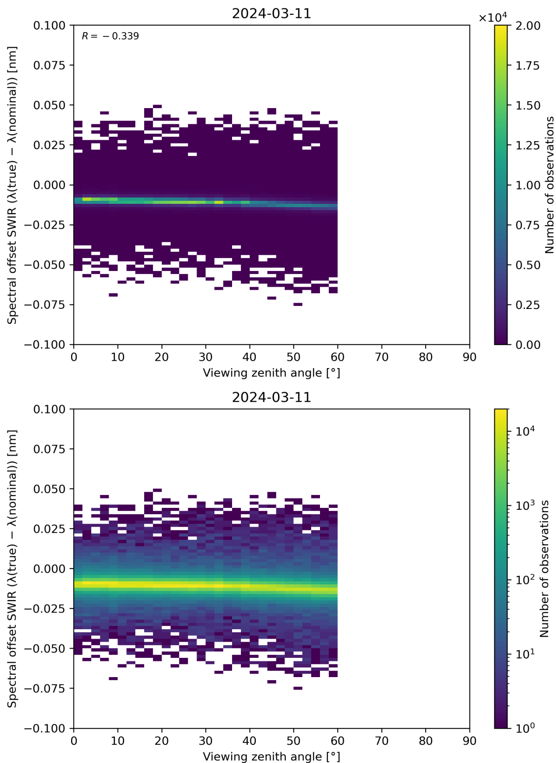
Figure 116: Scatter density plot of “Viewing zenith angle” against “Spectral offset SWIR ( \lambda(\text{true}) - \lambda(\text{nominal}) )” for 2024-03-10 to 2024-03-12.
