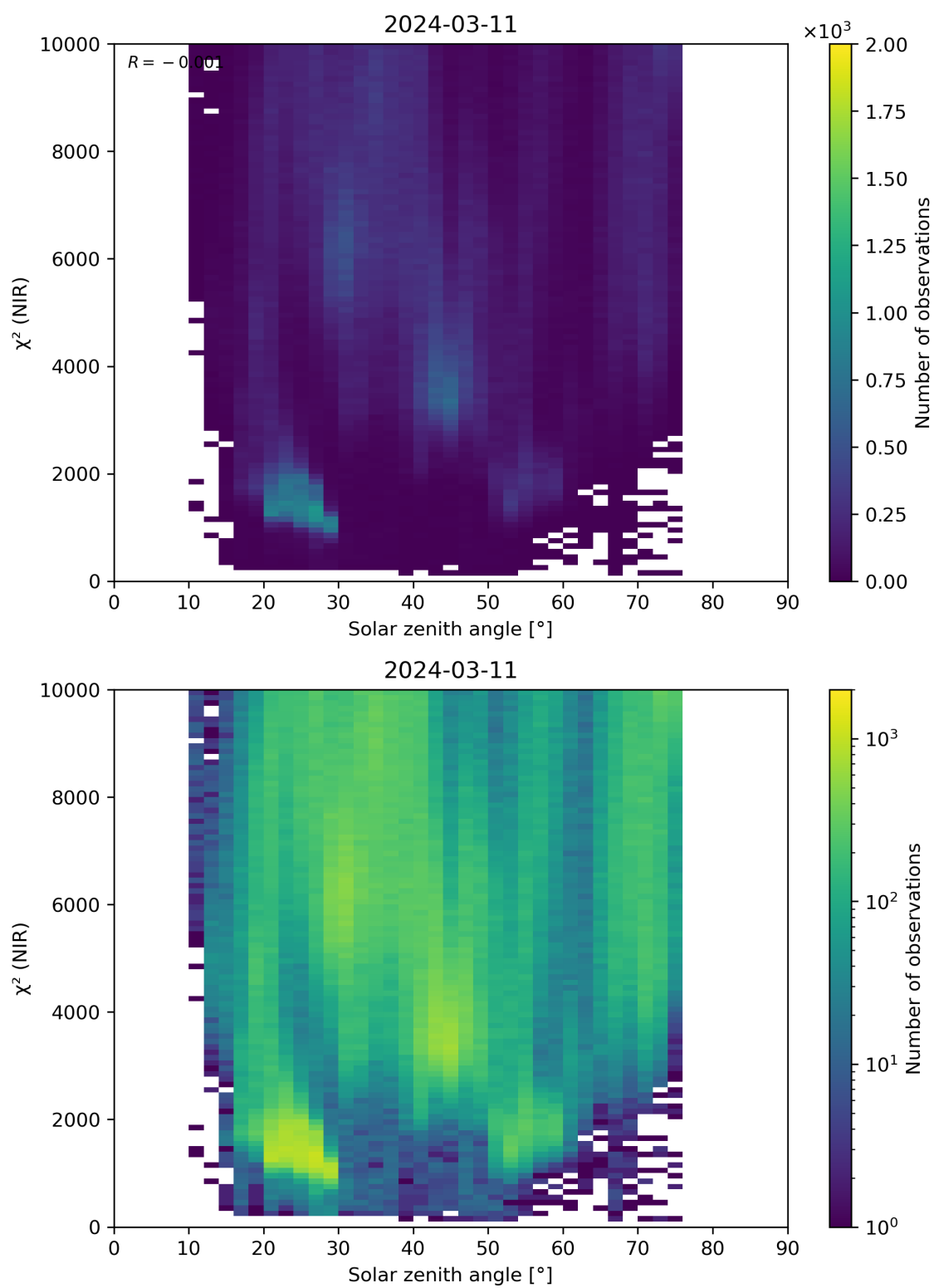
Figure 94: Scatter density plot of “Solar zenith angle” against “ \chi^2 (NIR)” for 2024-03-10 to 2024-03-12.
