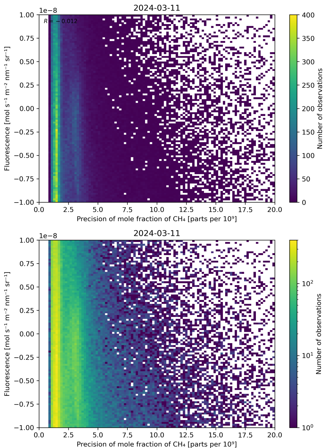
Figure 81: Scatter density plot of “Precision of mole fraction of CH 4 ” against “Fluorescence” for 2024-03-10 to 2024-03-12.
