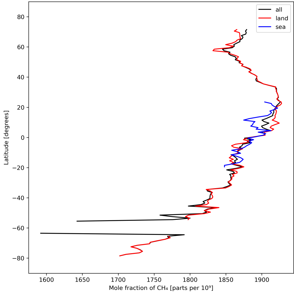
Figure 12: Zonal average of “Mole fraction of \text{CH}_4 ” for 2024-03-10 to 2024-03-12.
