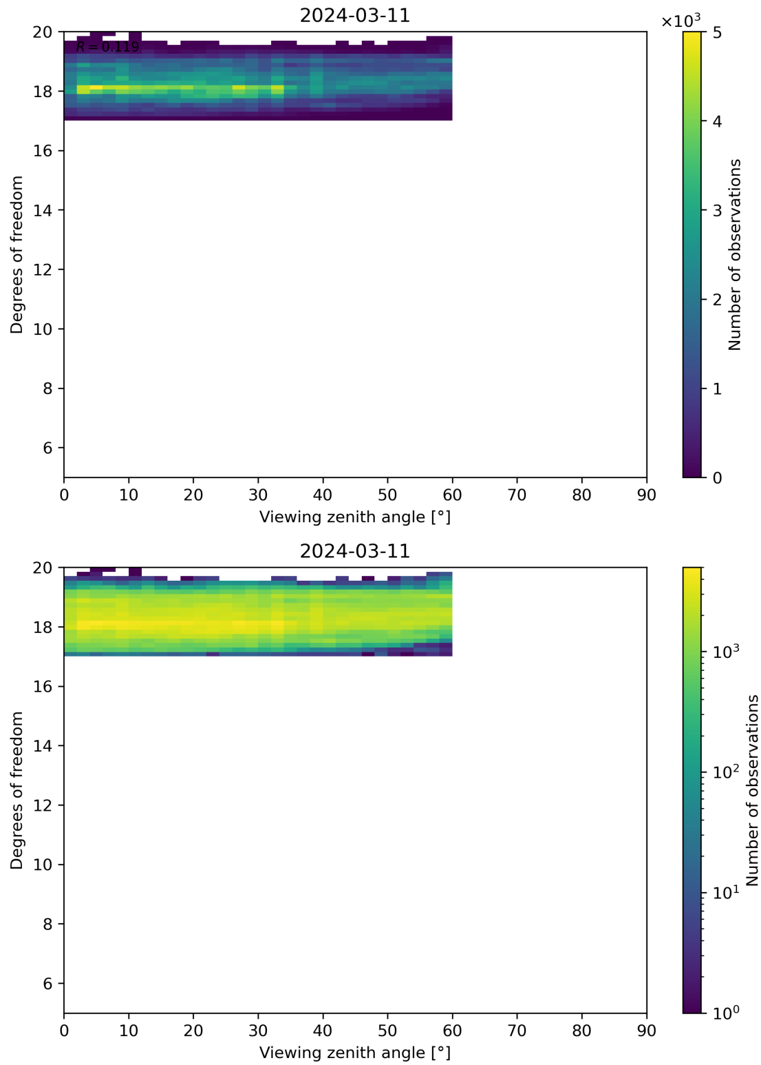
Figure 107: Scatter density plot of “Viewing zenith angle” against “Degrees of freedom” for 2024-03-10 to 2024-03-12.
