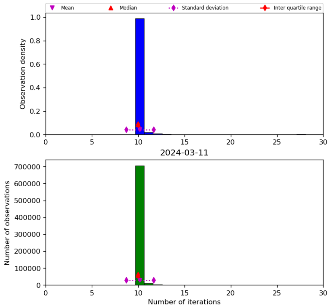
Figure 31: Histogram of “Number of iterations” for 2024-03-10 to 2024-03-12
