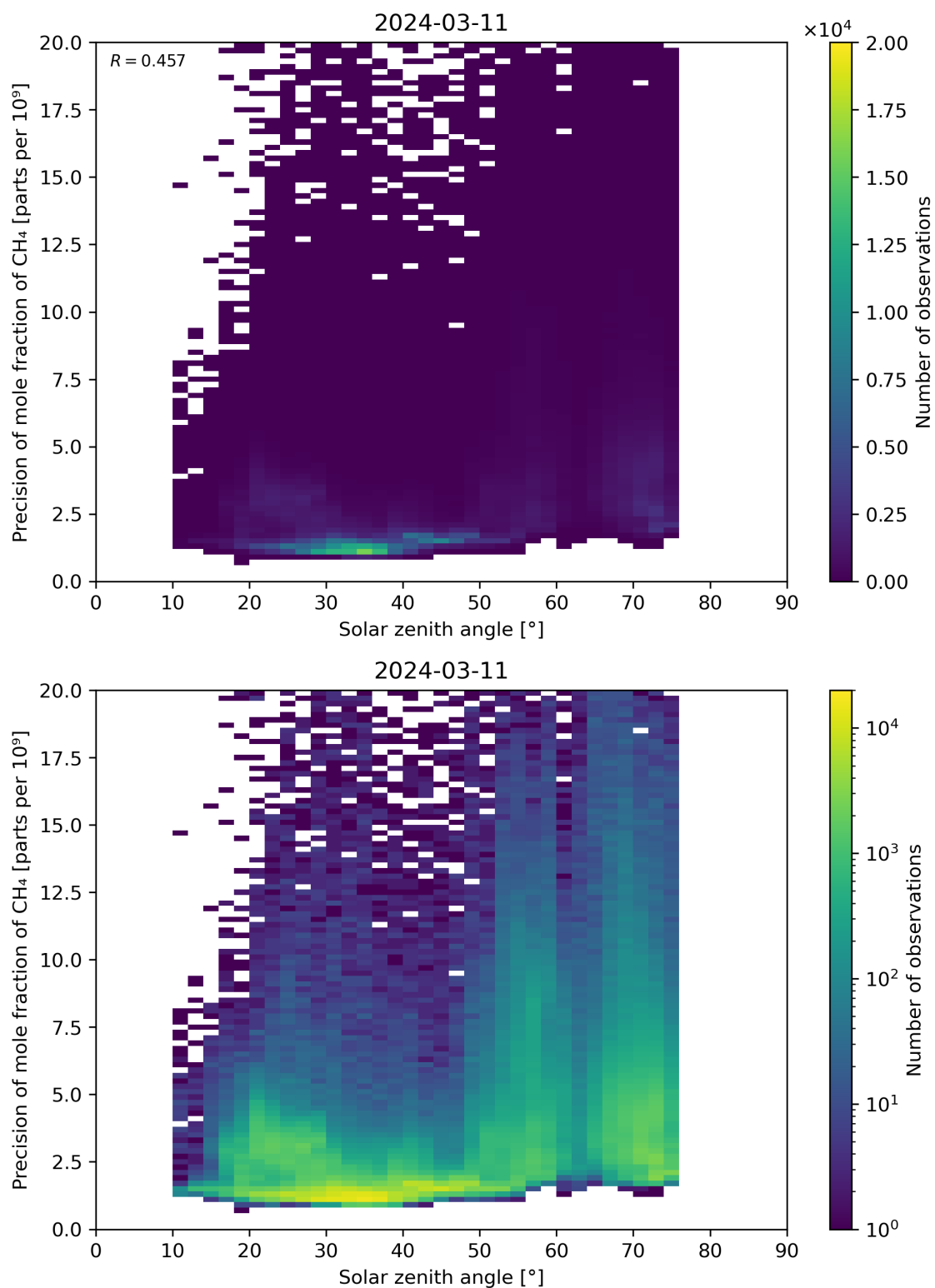
Figure 101: Scatter density plot of “Solar zenith angle” against “Precision of mole fraction of CH 4 ” for 2024-03-10 to 2024-03-12.
