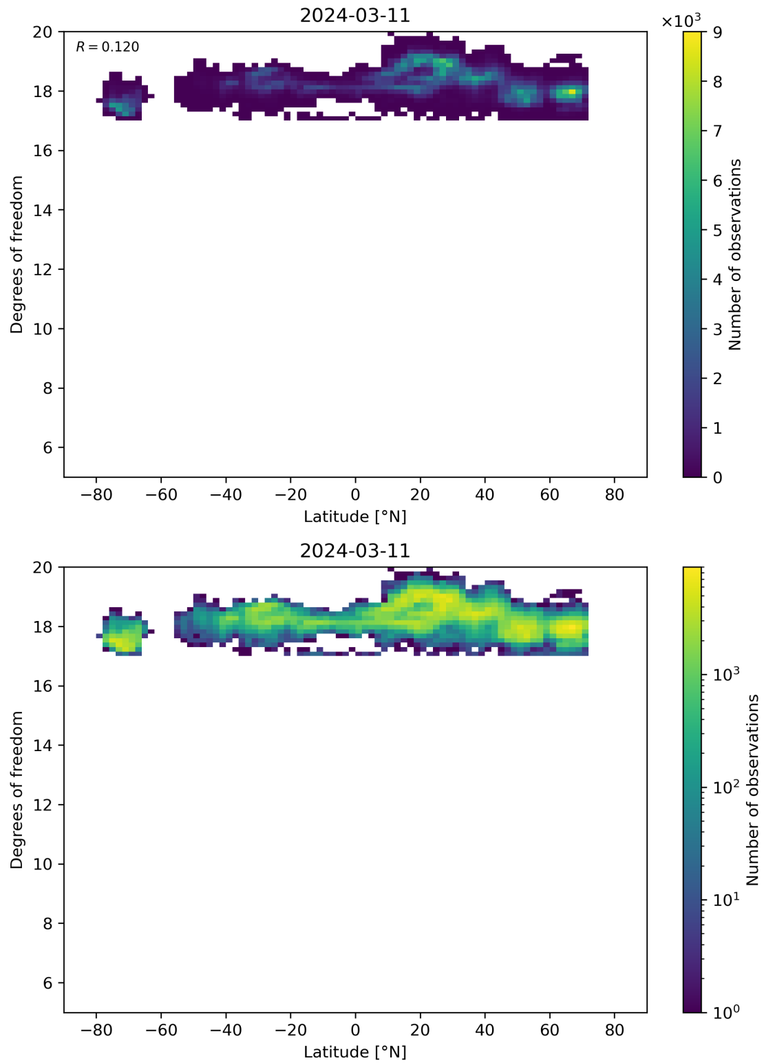
Figure 55: Scatter density plot of “Latitude” against “Degrees of freedom” for 2024-03-10 to 2024-03-12.
