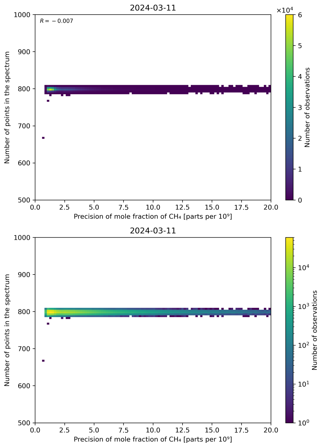
Figure 84: Scatter density plot of “Precision of mole fraction of CH 4 ” against “Number of points in the spectrum” for 2024-03-10 to 2024-03-12.
