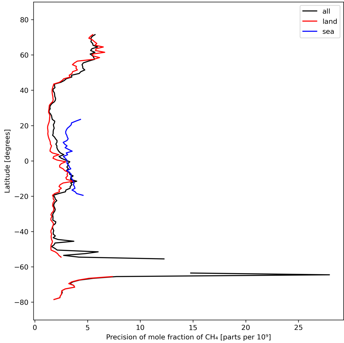
Figure 13: Zonal average of “Precision of mole fraction of CH 4 ” for 2024-03-10 to 2024-03-12.
