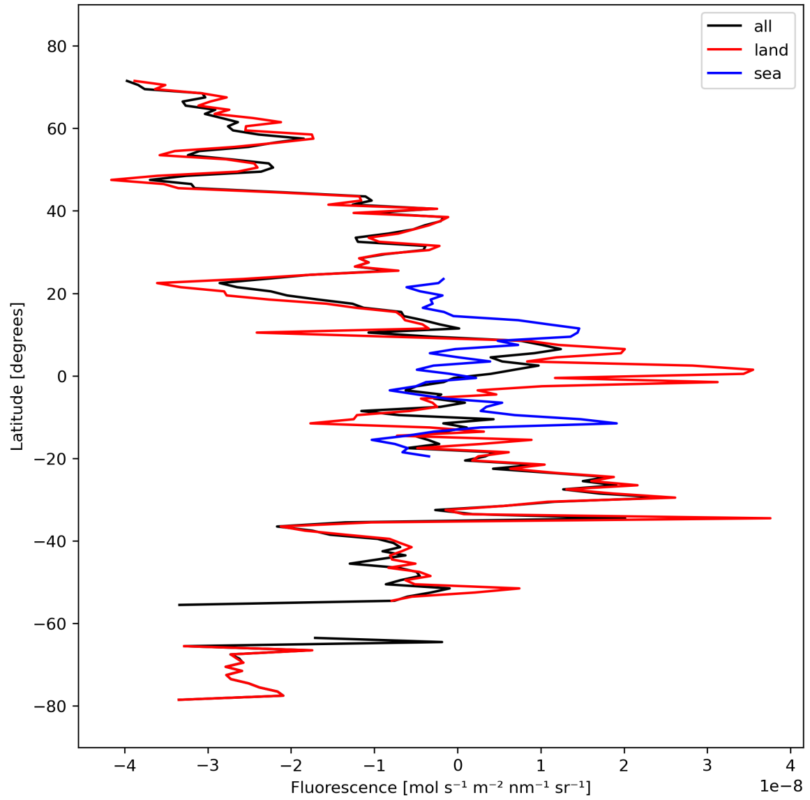
Figure 21: Zonal average of “Fluorescence” for 2024-03-10 to 2024-03-12.
