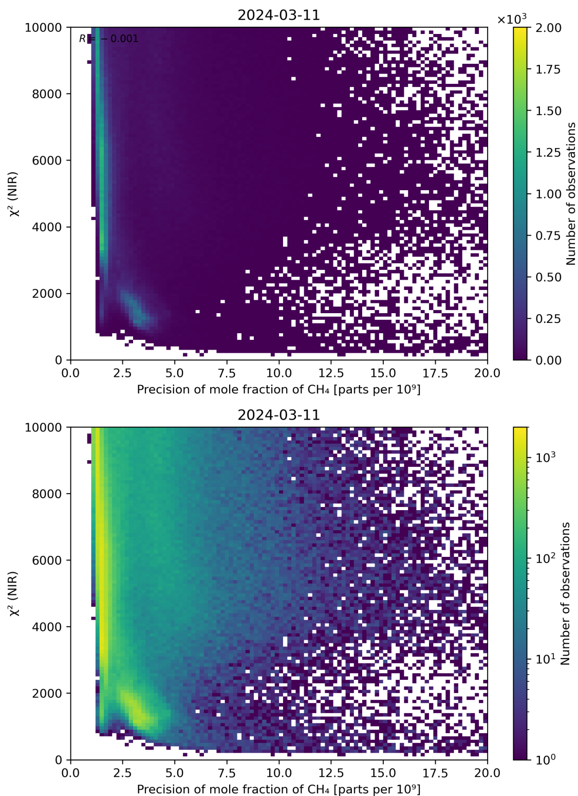
Figure 78: Scatter density plot of “Precision of mole fraction of CH 4 ” against “ \chi^2 (NIR)” for 2024-03-10 to 2024-03-12.
