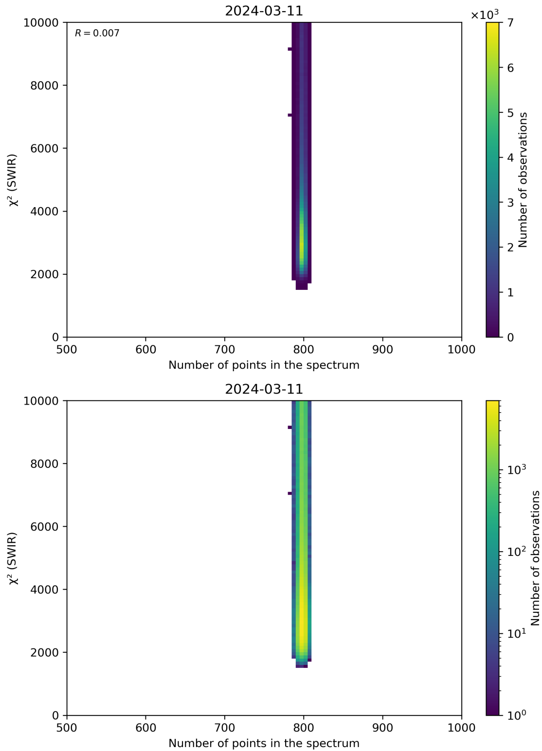
Figure 89: Scatter density plot of “Number of points in the spectrum” against “ \chi^2 (SWIR)” for 2024-03-10 to 2024-03-12.
