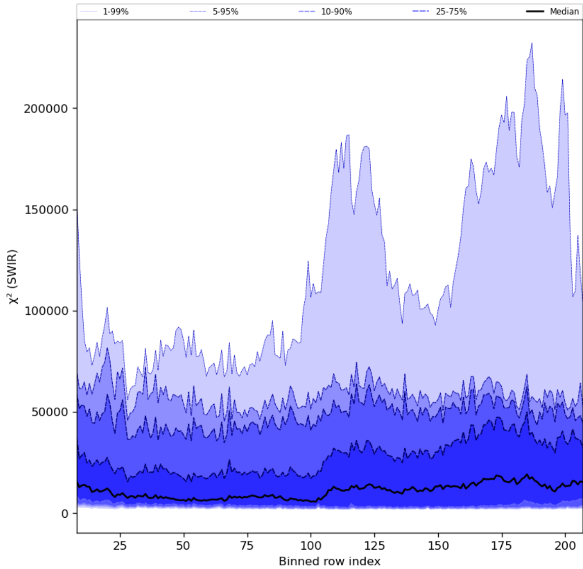
Figure 39: Along track statistics of “ \chi^2 (SWIR)” for 2024-03-10 to 2024-03-12
