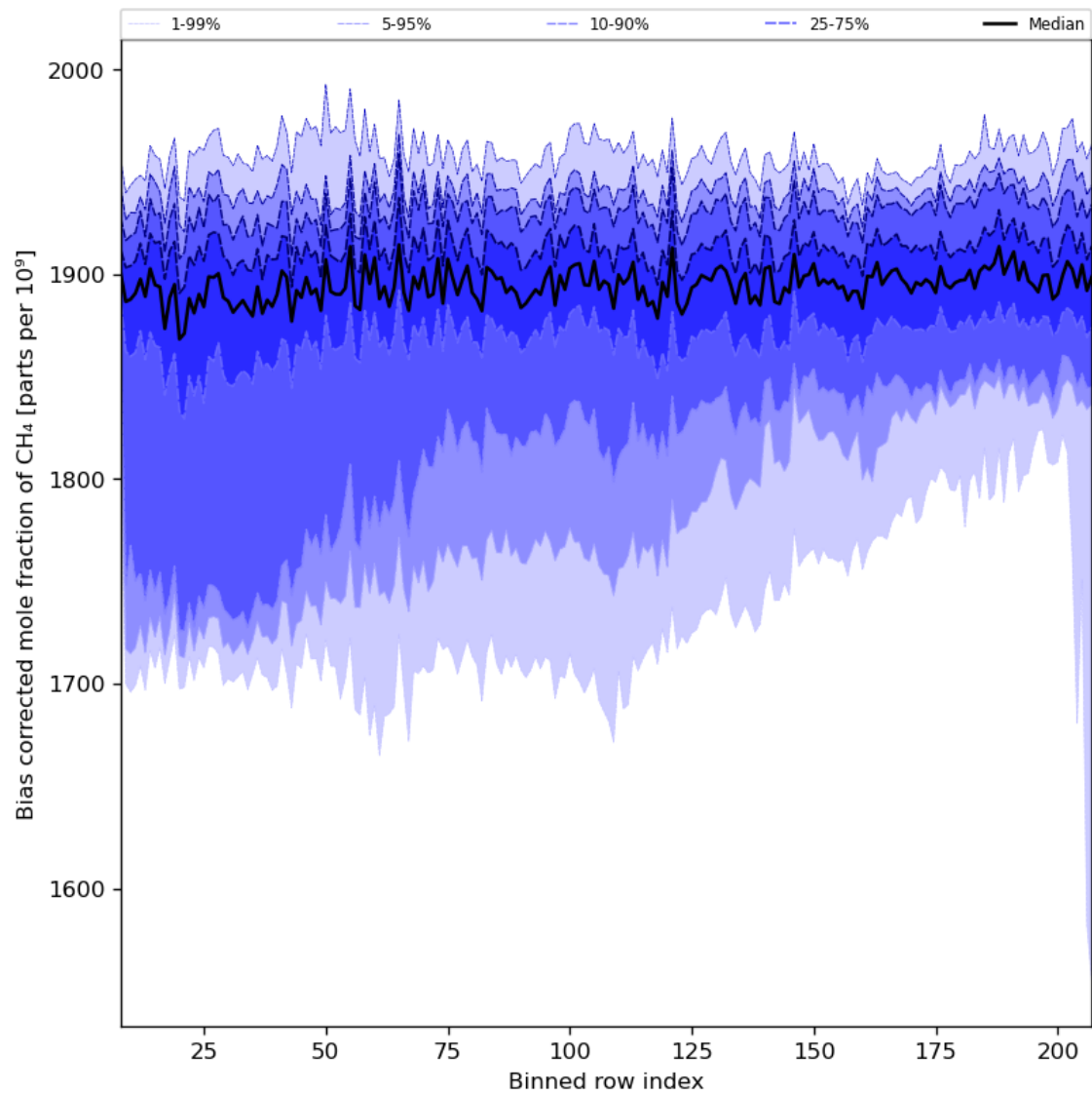
Figure 36: Along track statistics of “Bias corrected mole fraction of CH 4 ” for 2024-03-10 to 2024-03-12
