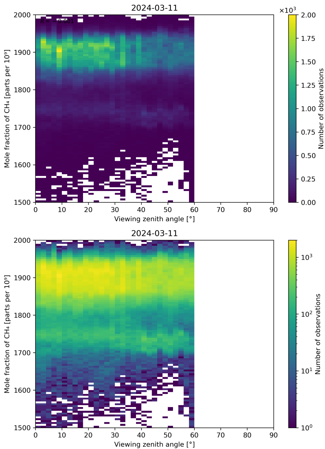
Figure 110: Scatter density plot of “Viewing zenith angle” against “Mole fraction of CH 4 ” for 2024-03-10 to 2024-03-12.
