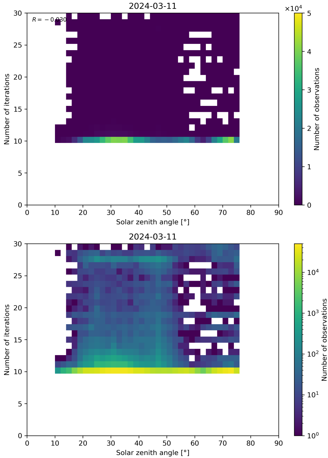
Figure 102: Scatter density plot of “Solar zenith angle” against “Number of iterations” for 2024-03-10 to 2024-03-12.
