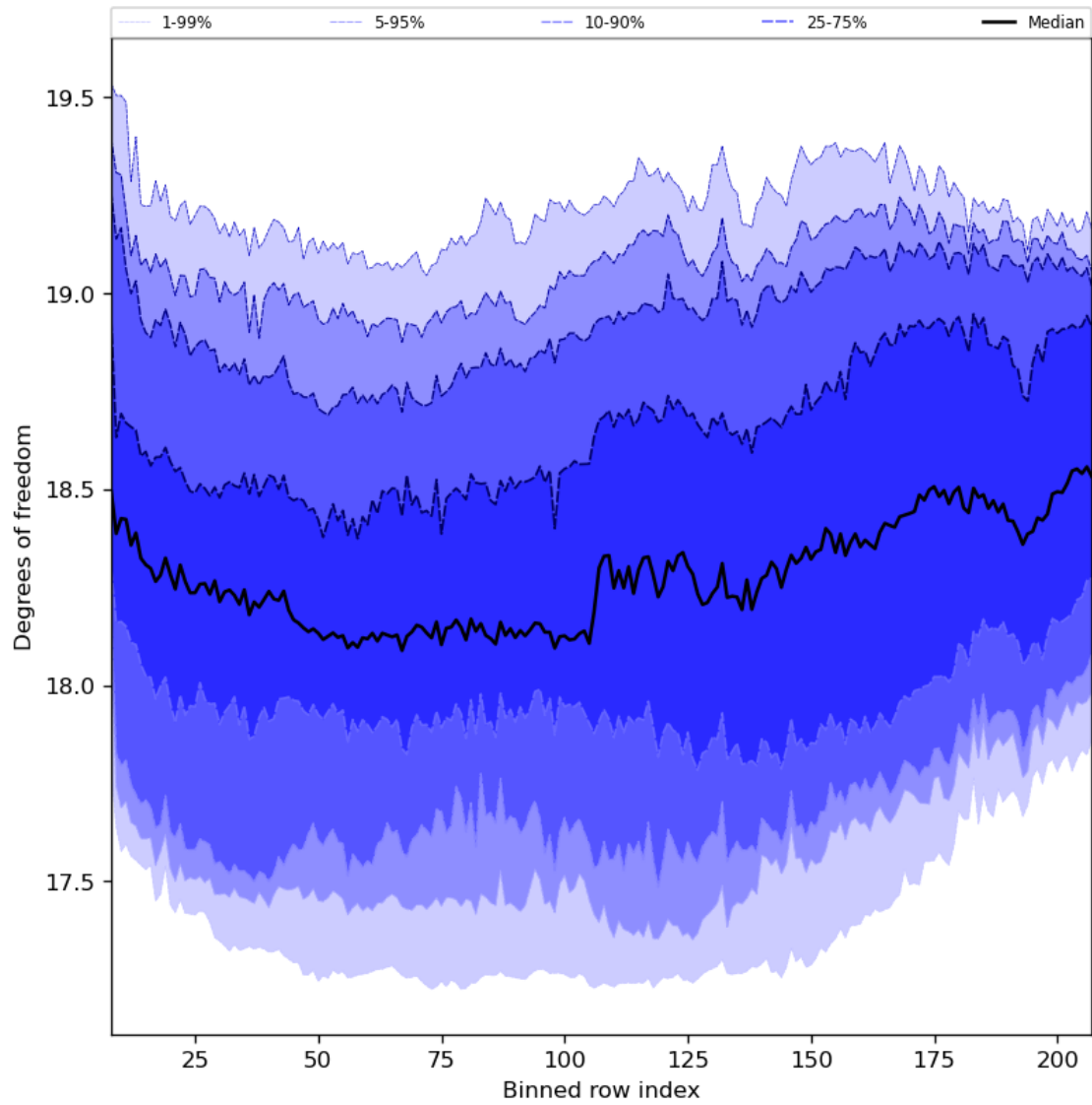
Figure 41: Along track statistics of “Degrees of freedom” for 2024-03-10 to 2024-03-12
