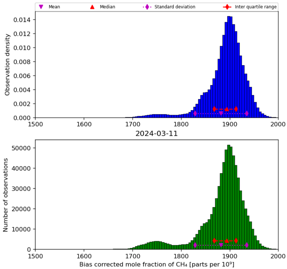
Figure 25: Histogram of “Bias corrected mole fraction of CH 4 ” for 2024-03-10 to 2024-03-12
