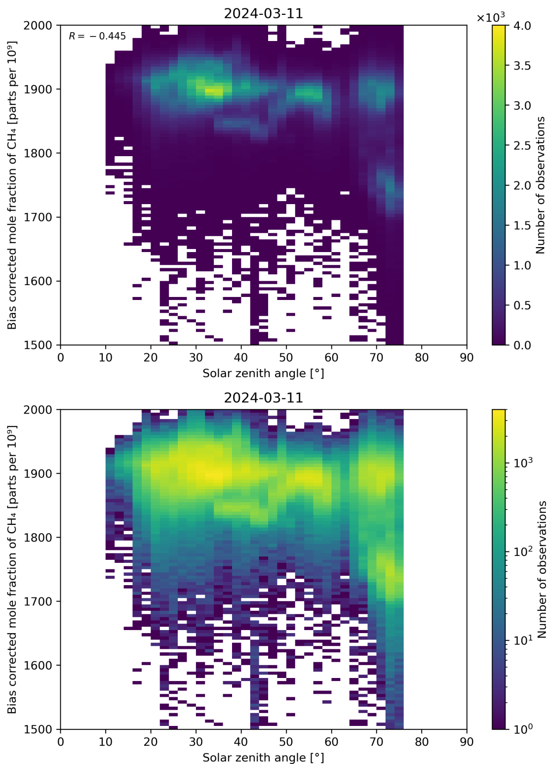
Figure 100: Scatter density plot of “Solar zenith angle” against “Bias corrected mole fraction of CH 4 ” for 2024-03-10 to 2024-03-12.
