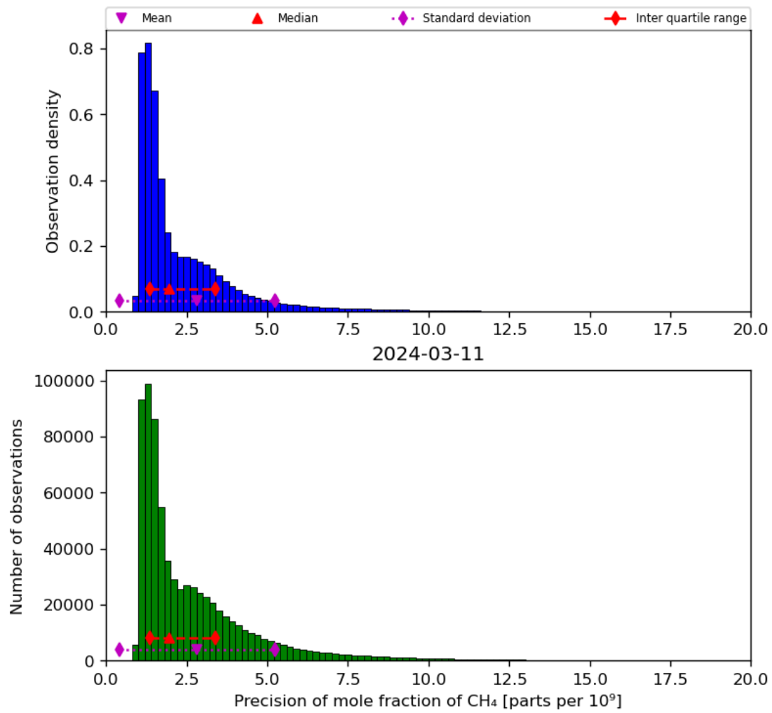
Figure 24: Histogram of “Precision of mole fraction of CH 4 ” for 2024-03-10 to 2024-03-12
