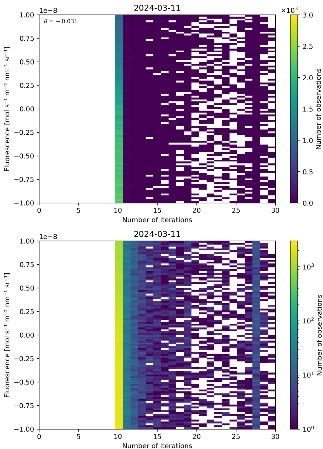
Figure 87: Scatter density plot of “Number of iterations” against “Fluorescence” for 2024-03-10 to 2024-03-12.
