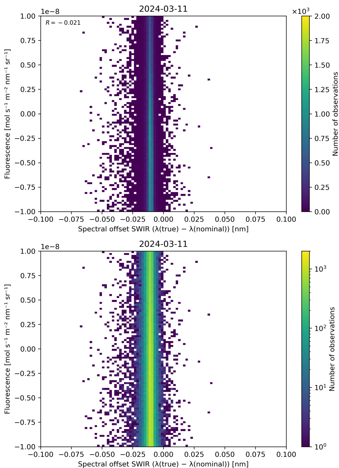
Figure 120: Scatter density plot of “Spectral offset SWIR ( \lambda(\text{true}) - \lambda(\text{nominal}) )” against “Fluorescence” for 2024-03-10 to 2024-03-12.
