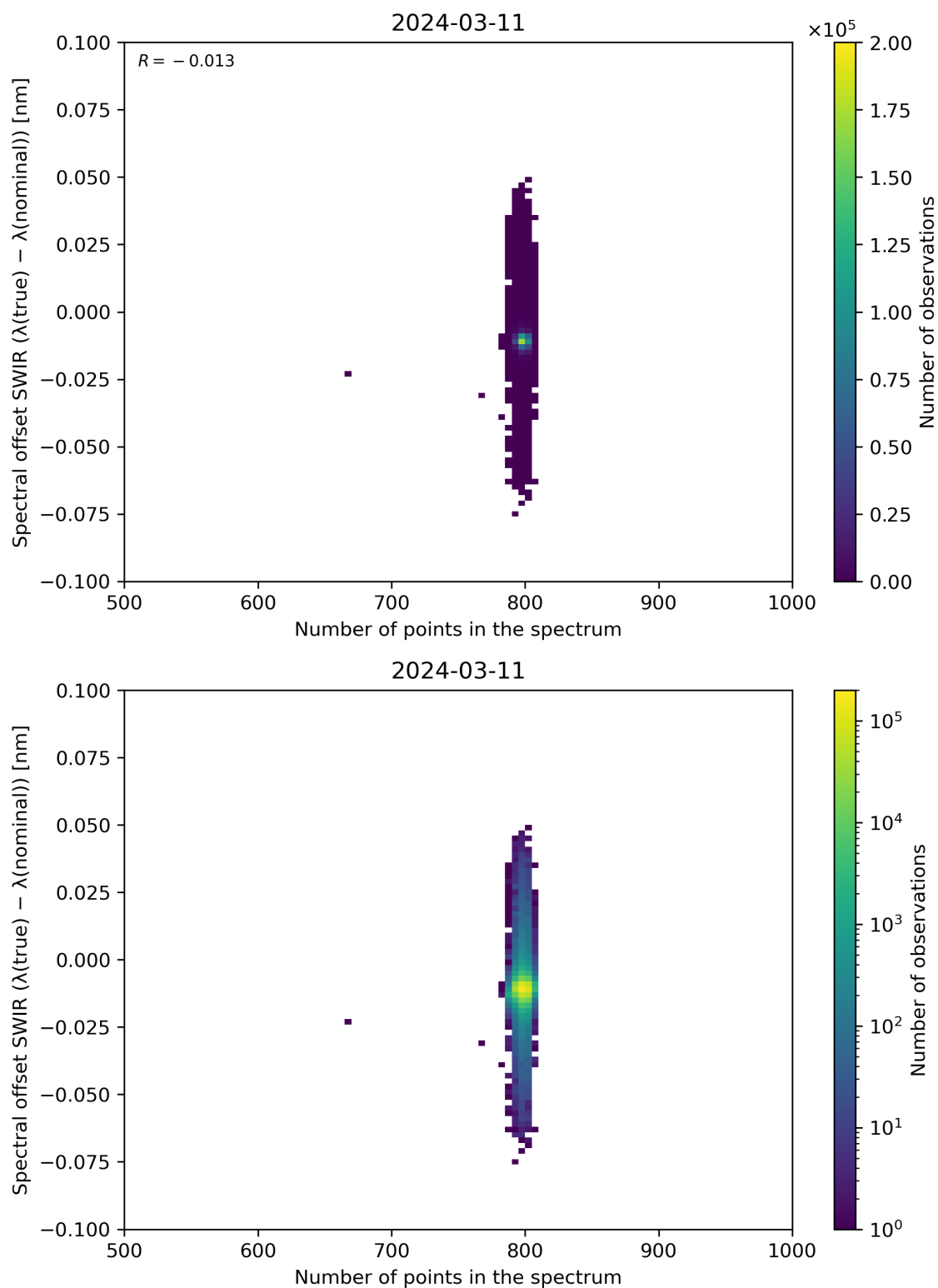
Figure 93: Scatter density plot of “Number of points in the spectrum” against “Spectral offset SWIR ( \lambda(\text{true}) - \lambda(\text{nominal}) )” for 2024-03-10 to 2024-03-12.
