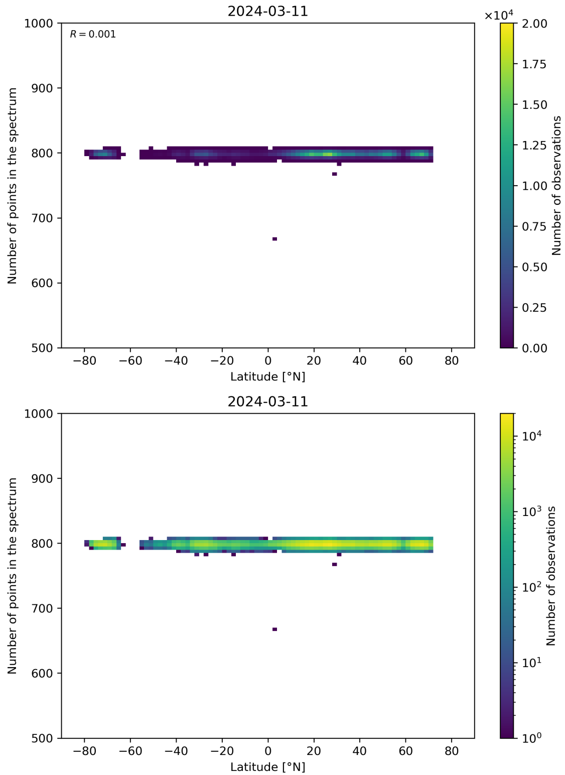
Figure 61: Scatter density plot of “Latitude” against “Number of points in the spectrum” for 2024-03-10 to 2024-03-12.
