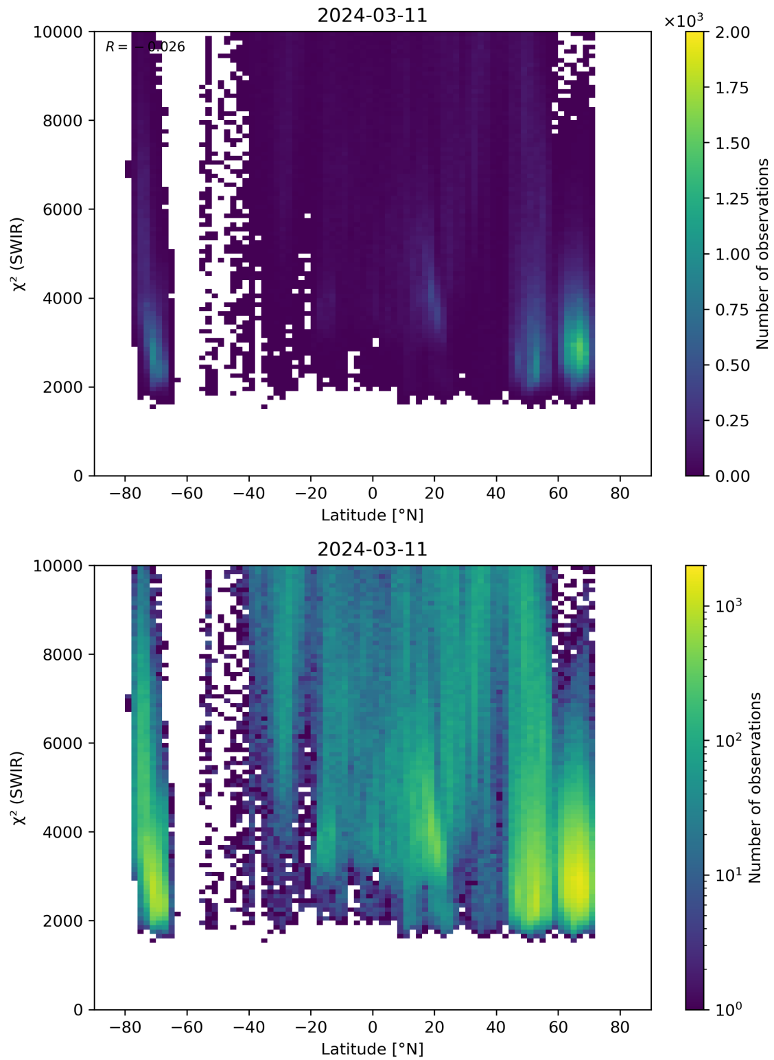
Figure 54: Scatter density plot of “Latitude” against “ \chi^2 (SWIR)” for 2024-03-10 to 2024-03-12.
