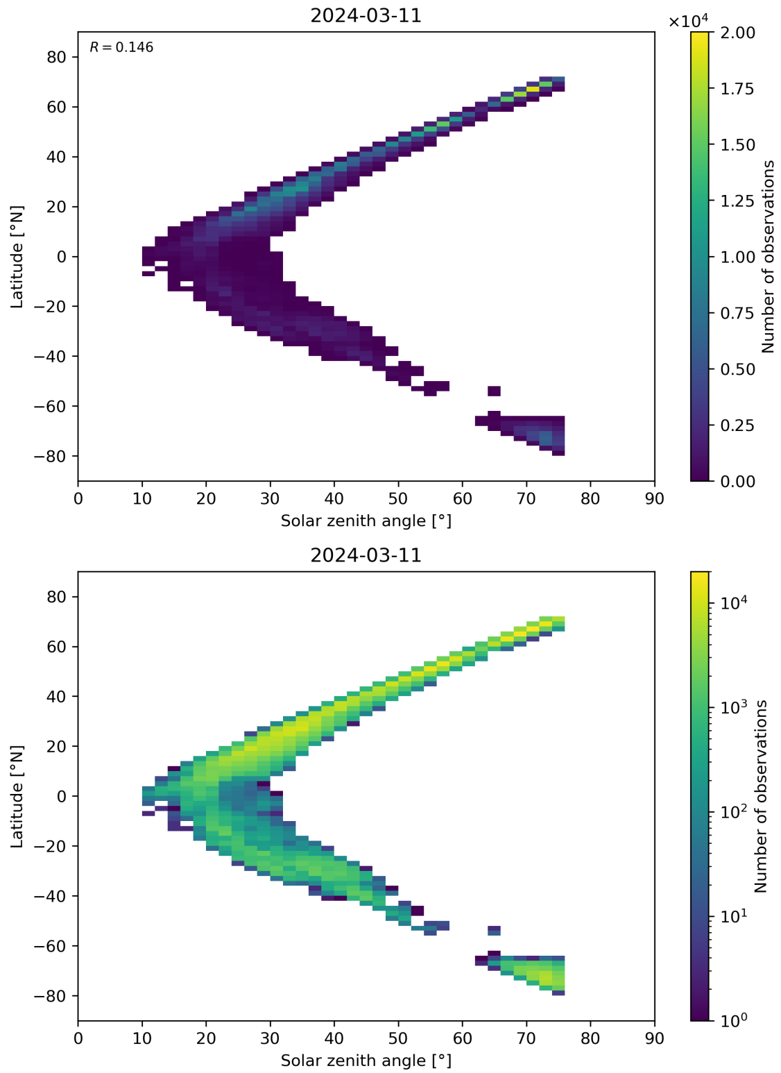
Figure 98: Scatter density plot of “Solar zenith angle” against “Latitude” for 2024-03-10 to 2024-03-12.
