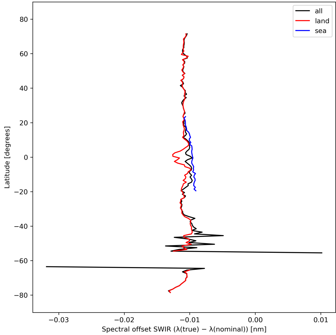
Figure 16: Zonal average of “Spectral offset SWIR ( \lambda(\text{true}) - \lambda(\text{nominal}) )” for 2024-03-10 to 2024-03-12.
