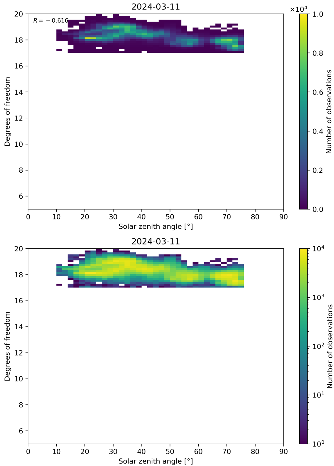
Figure 96: Scatter density plot of “Solar zenith angle” against “Degrees of freedom” for 2024-03-10 to 2024-03-12.
