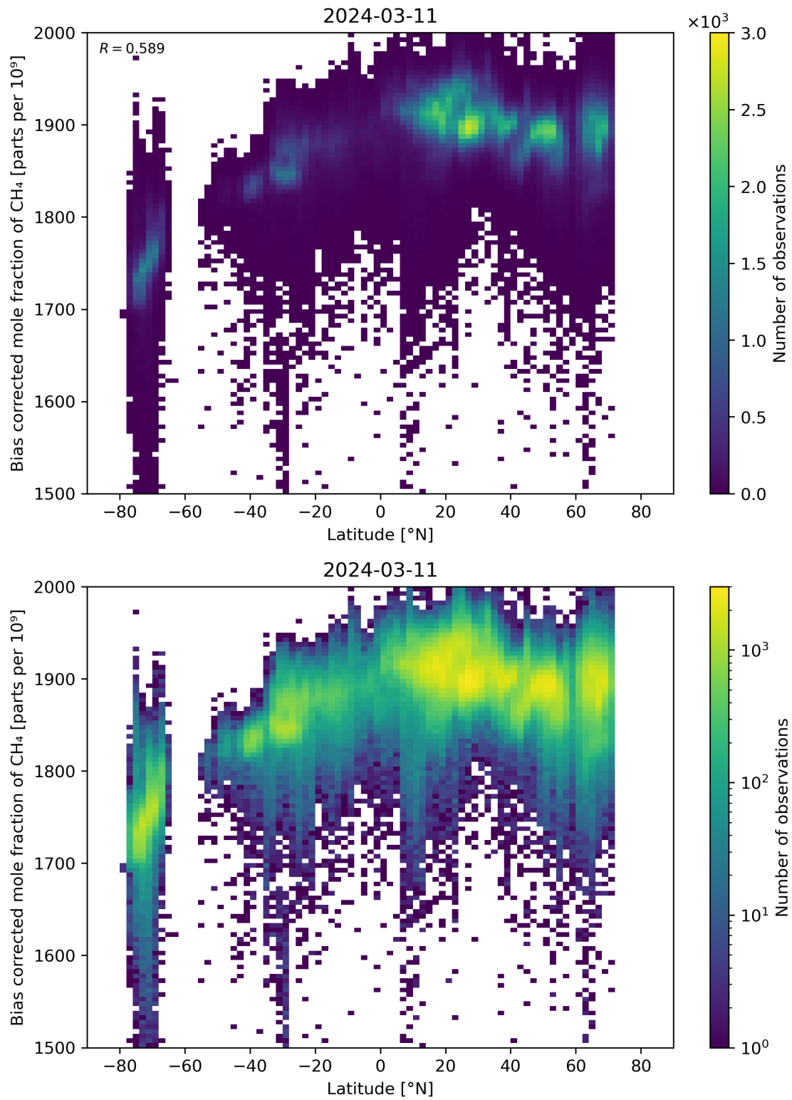
Figure 58: Scatter density plot of “Latitude” against “Bias corrected mole fraction of CH 4 ” for 2024-03-10 to 2024-03-12.
