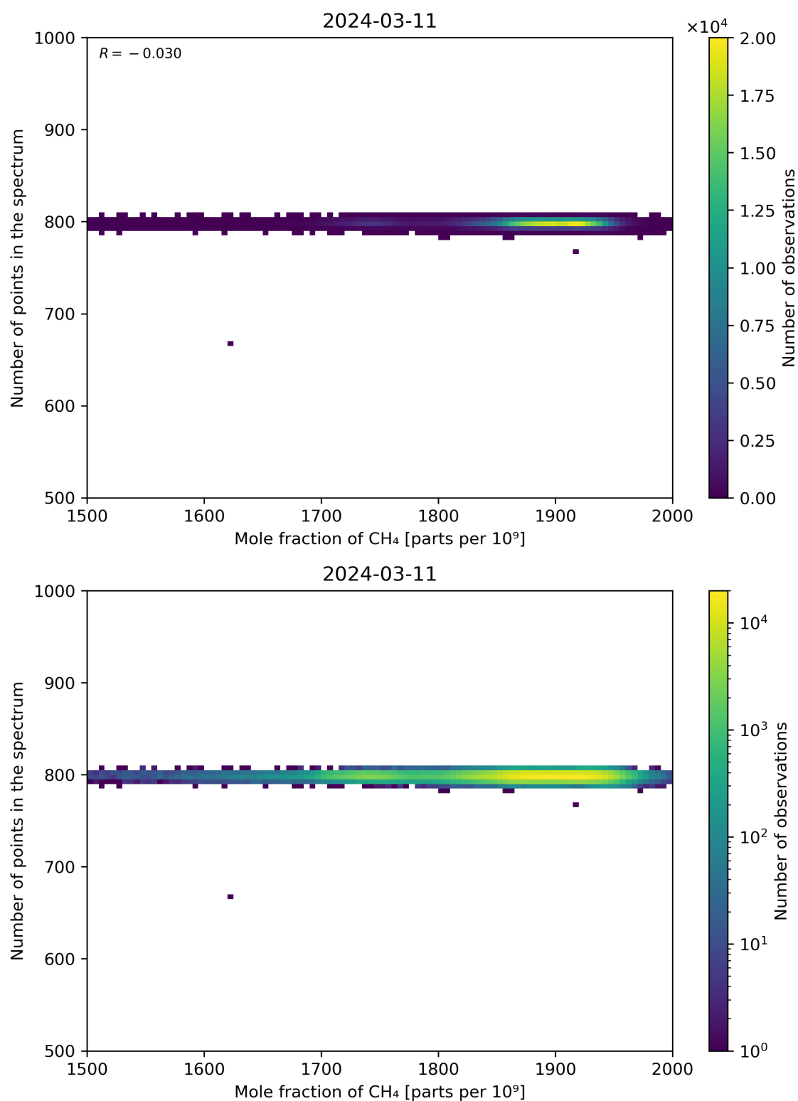
Figure 77: Scatter density plot of “Mole fraction of CH 4 ” against “Number of points in the spectrum” for 2024-03-10 to 2024-03-12.
