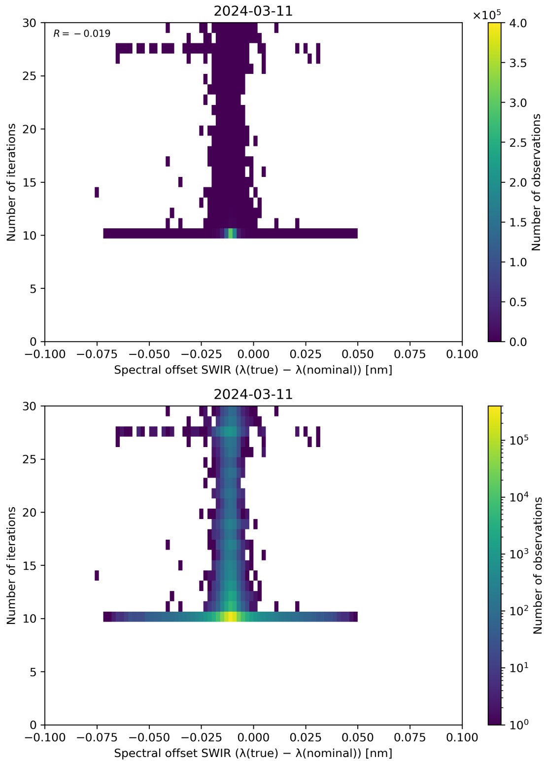
Figure 121: Scatter density plot of “Spectral offset SWIR ( \lambda(\text{true}) - \lambda(\text{nominal}) )” against “Number of iterations” for 2024-03-10 to 2024-03-12.
