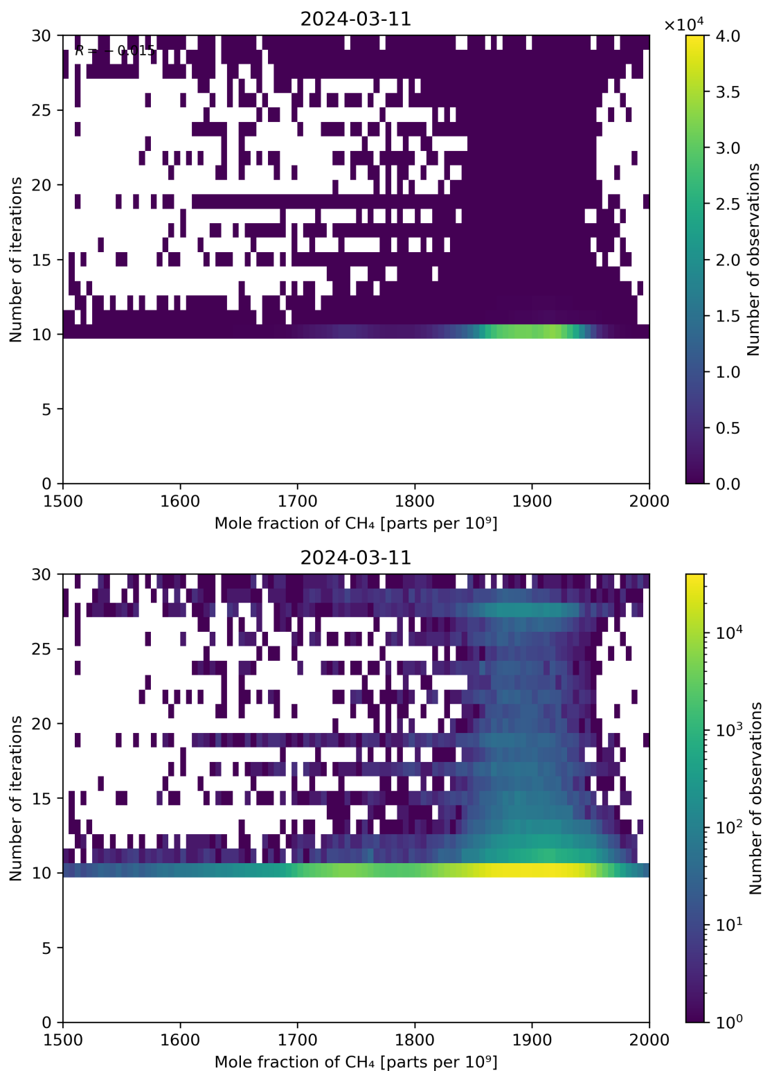
Figure 76: Scatter density plot of “Mole fraction of CH 4 ” against “Number of iterations” for 2024-03-10 to 2024-03-12.
