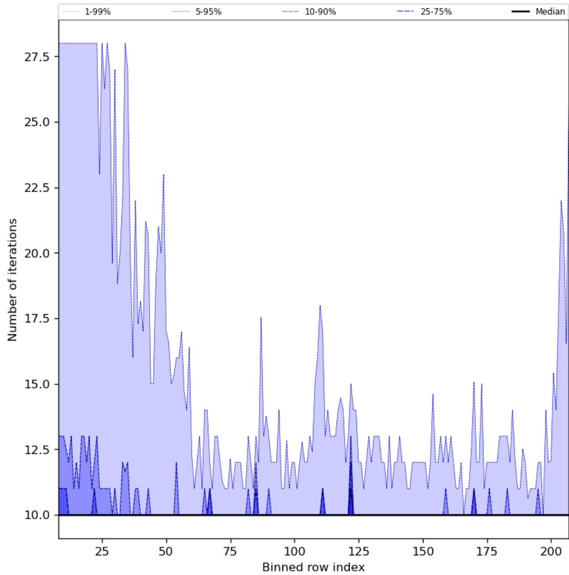
Figure 42: Along track statistics of “Number of iterations” for 2024-03-10 to 2024-03-12
