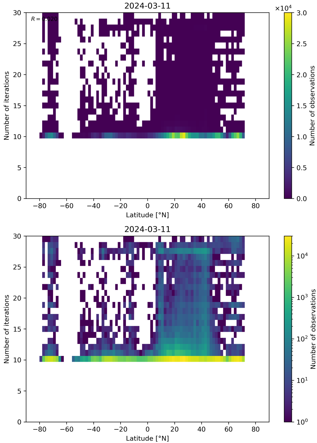
Figure 60: Scatter density plot of “Latitude” against “Number of iterations” for 2024-03-10 to 2024-03-12.
