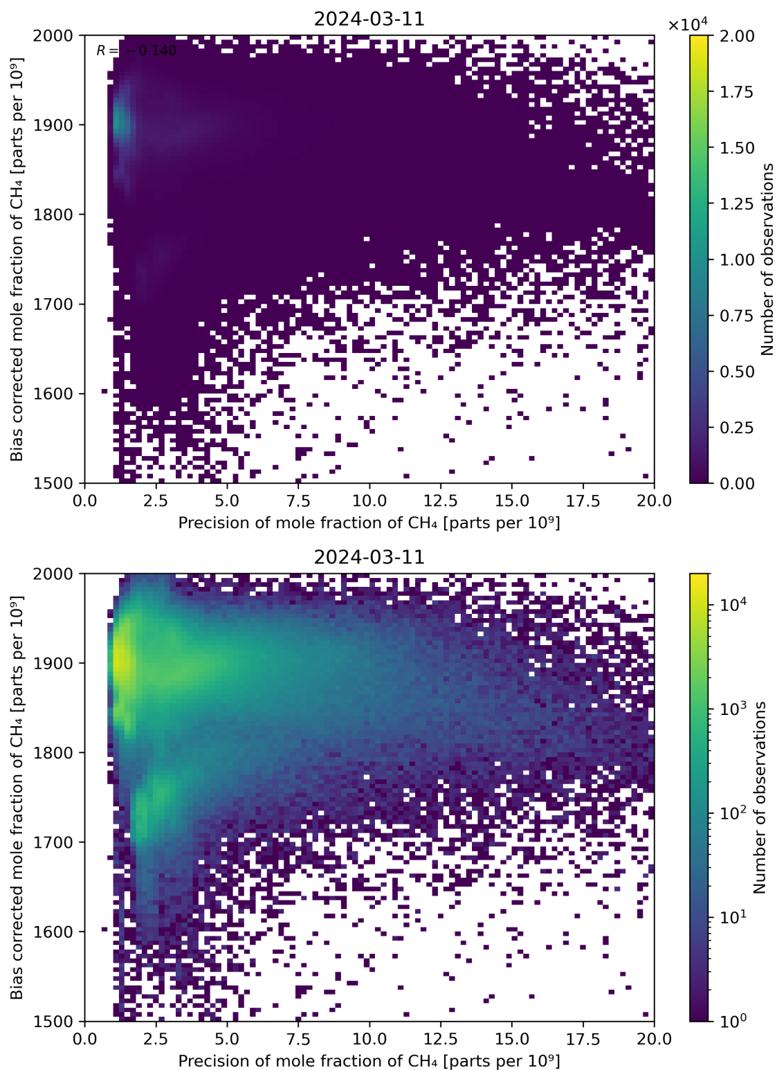
Figure 82: Scatter density plot of “Precision of mole fraction of CH 4 ” against “Bias corrected mole fraction of CH 4 ” for 2024-03-10 to 2024-03-12.
