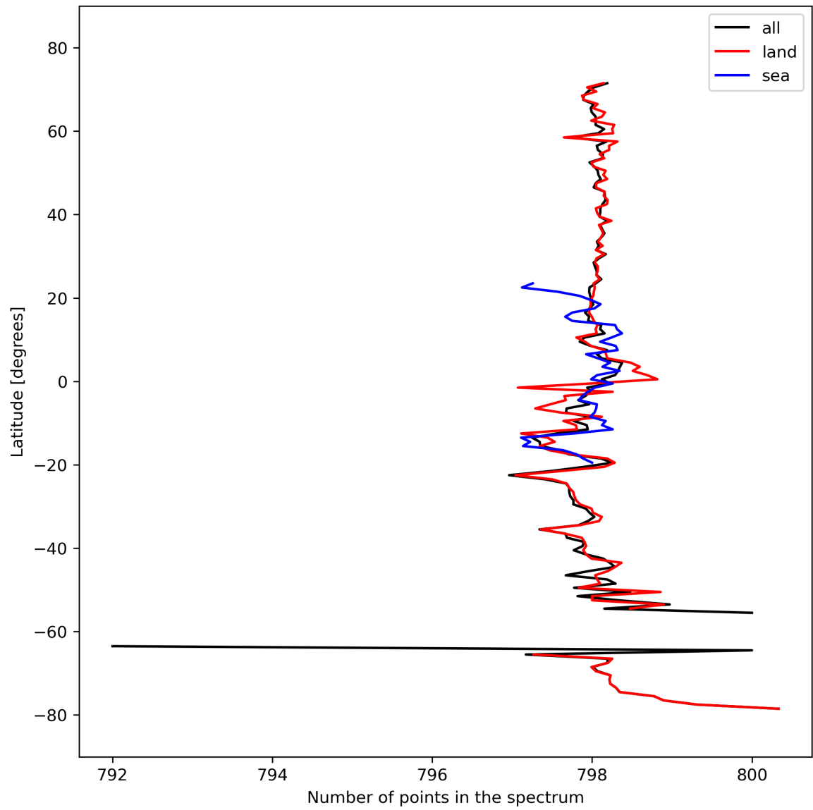
Figure 15: Zonal average of “Number of points in the spectrum” for 2024-03-10 to 2024-03-12.
