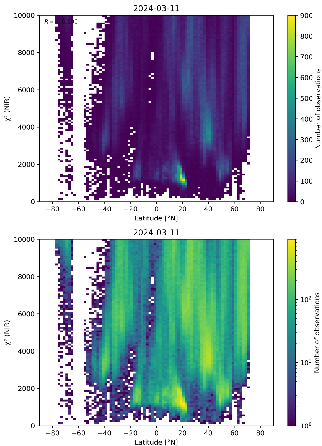
Figure 53: Scatter density plot of “Latitude” against “ \chi^2 (NIR)” for 2024-03-10 to 2024-03-12.
