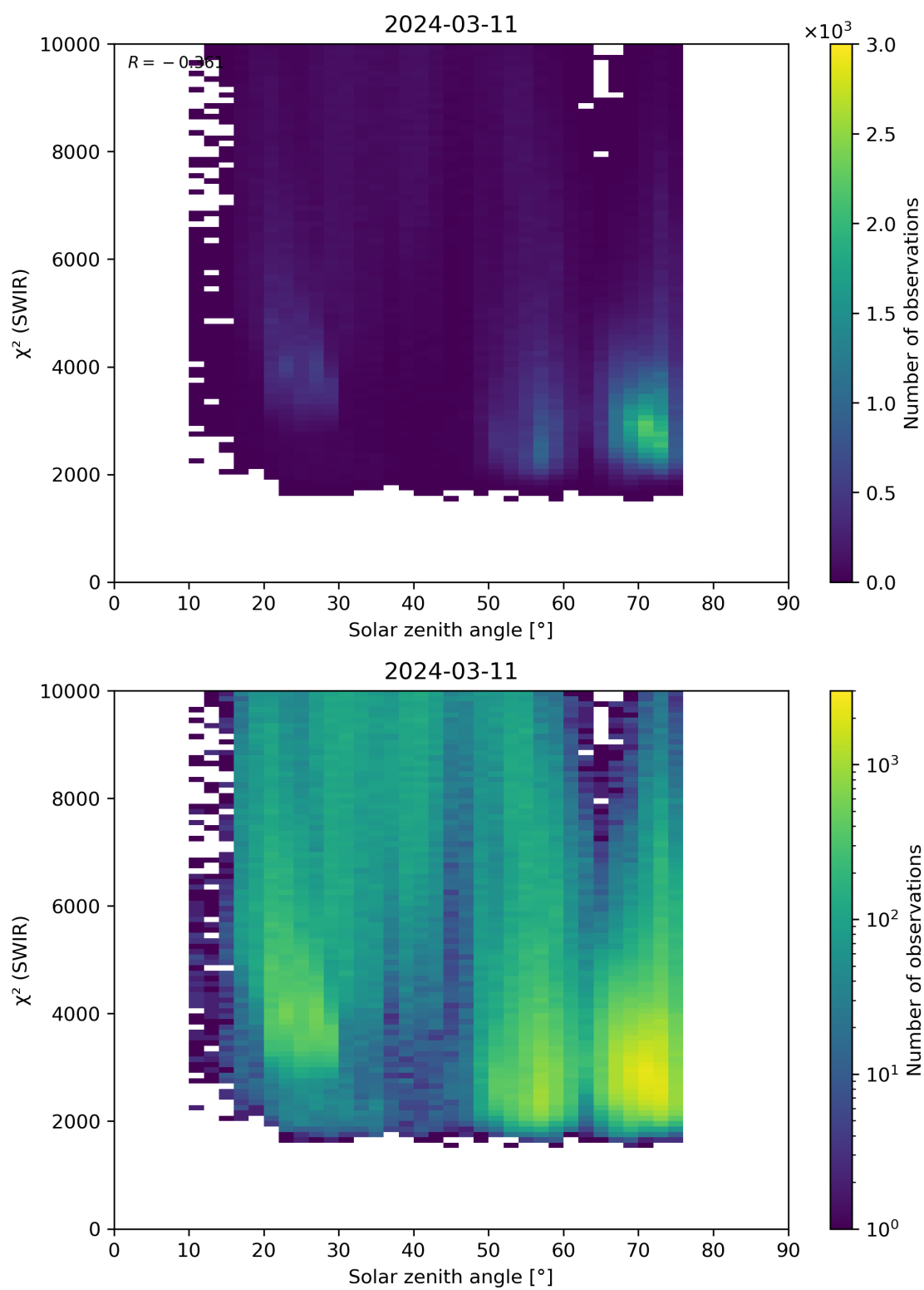
Figure 95: Scatter density plot of “Solar zenith angle” against “ \chi^2 (SWIR)” for 2024-03-10 to 2024-03-12.
