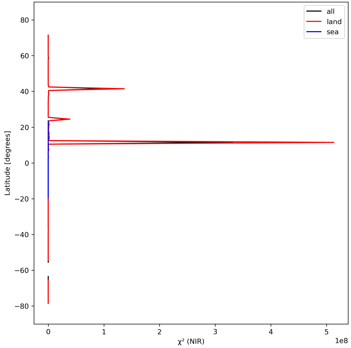
Figure 18: Zonal average of “ \chi^2 (NIR)” for 2024-03-10 to 2024-03-12.
