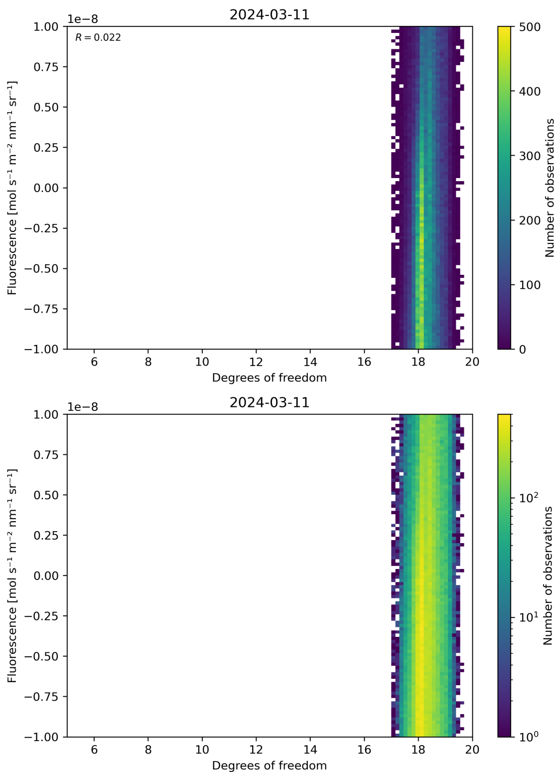
Figure 51: Scatter density plot of “Degrees of freedom” against “Fluorescence” for 2024-03-10 to 2024-03-12.
