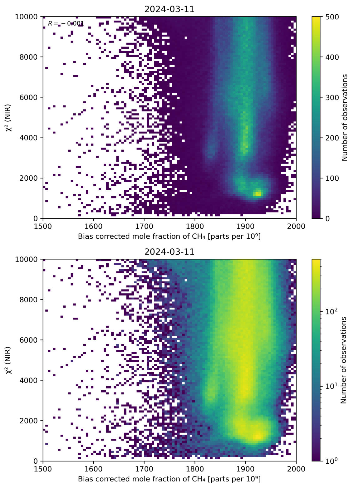
Figure 63: Scatter density plot of “Bias corrected mole fraction of CH 4 ” against “ \chi^2 (NIR)” for 2024-03-10 to 2024-03-12.
