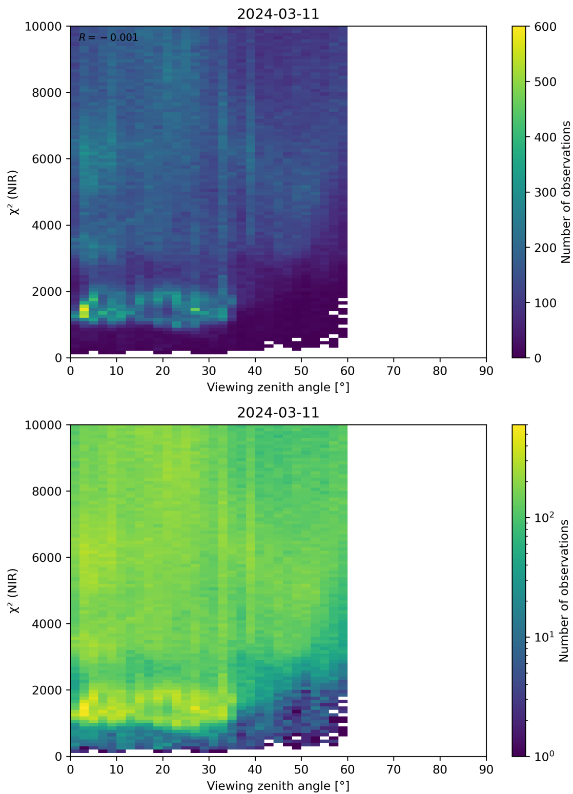
Figure 105: Scatter density plot of “Viewing zenith angle” against “ \chi^2 (NIR)” for 2024-03-10 to 2024-03-12.
