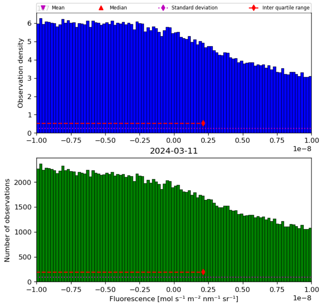
Figure 32: Histogram of “Fluorescence” for 2024-03-10 to 2024-03-12
