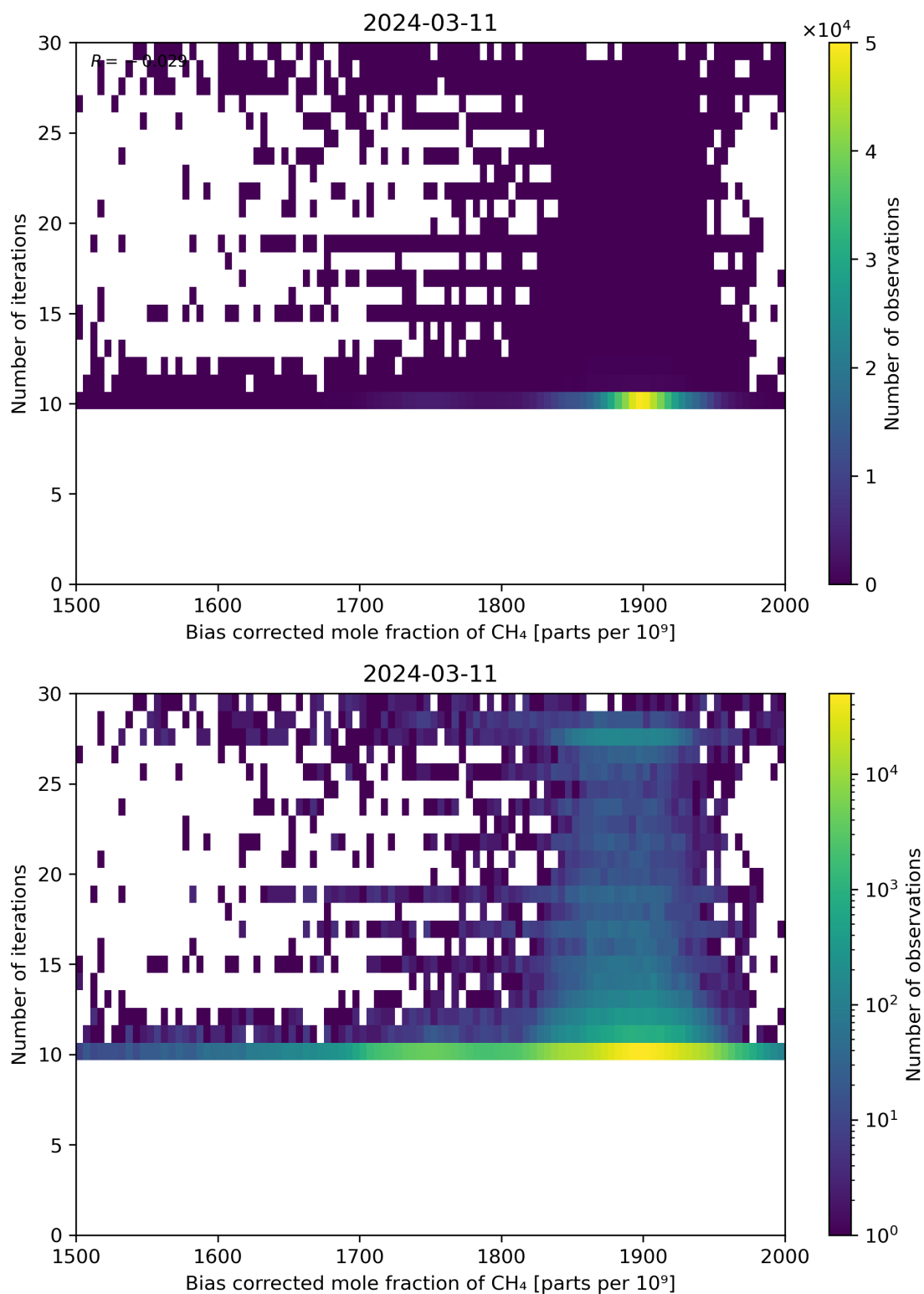
Figure 67: Scatter density plot of “Bias corrected mole fraction of CH 4 ” against “Number of iterations” for 2024-03-10 to 2024-03-12.
