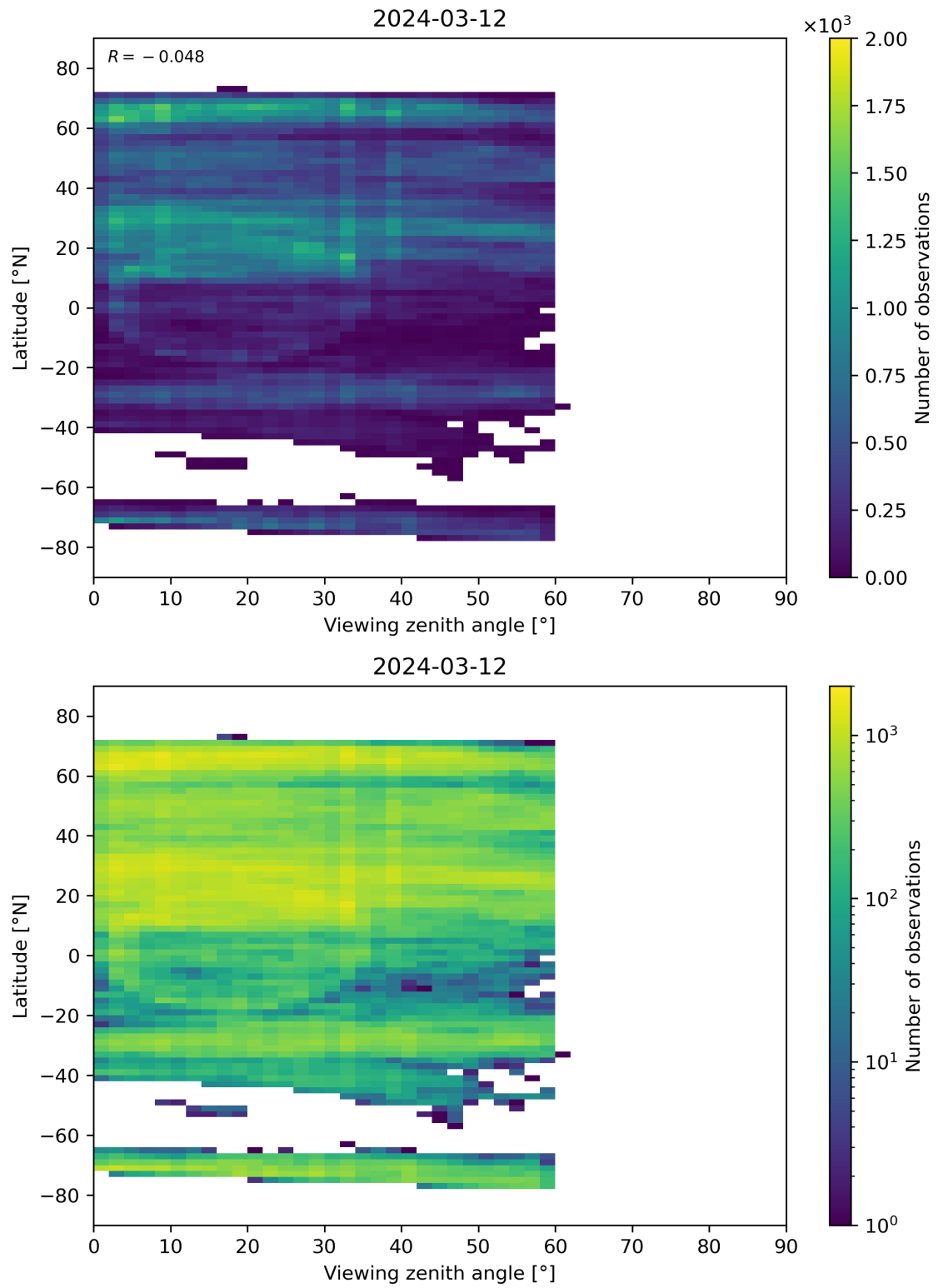
Figure 109: Scatter density plot of “Viewing zenith angle” against “Latitude” for 2024-03-11 to 2024-03-13.
