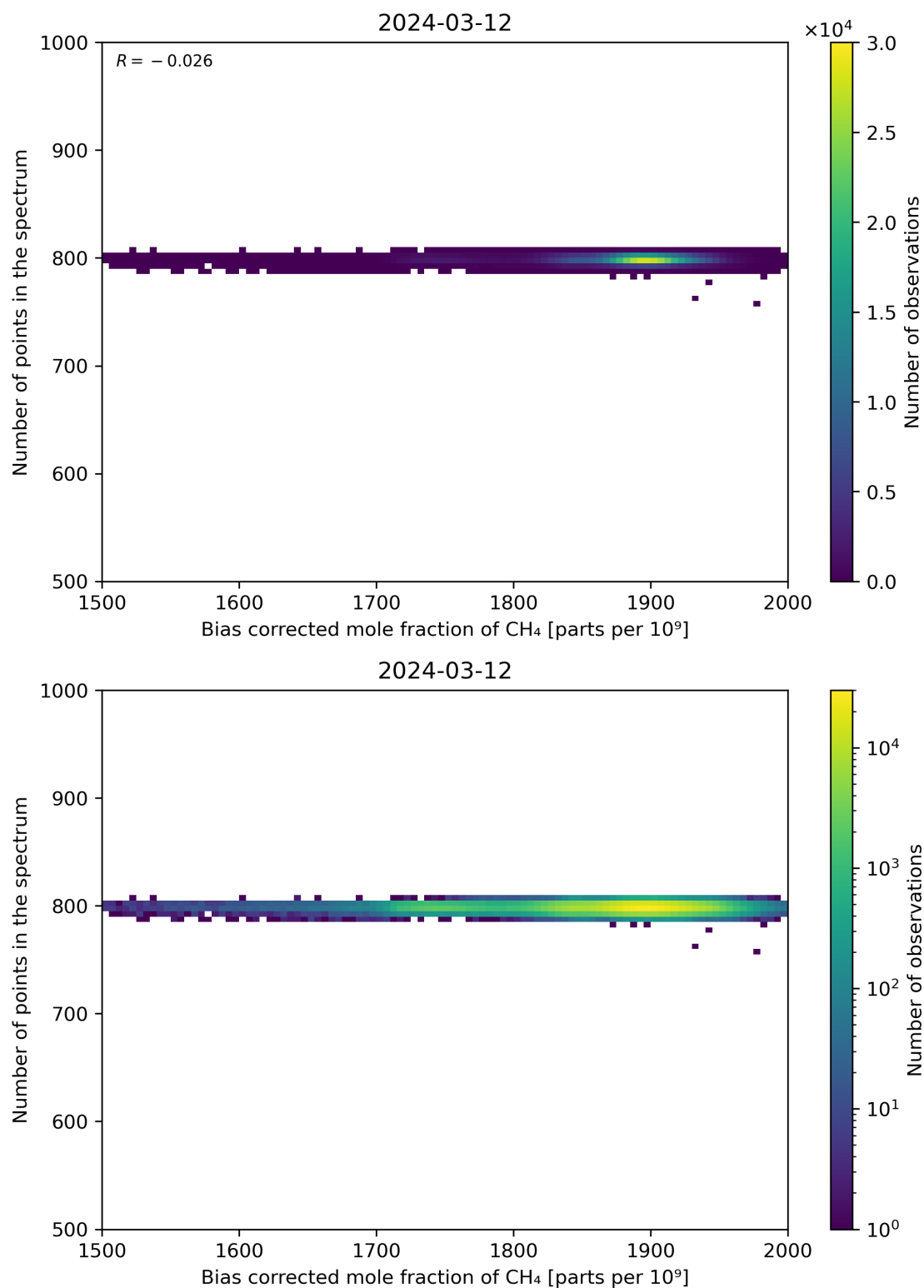
Figure 68: Scatter density plot of “Bias corrected mole fraction of CH 4 ” against “Number of points in the spectrum” for 2024-03-11 to 2024-03-13.
