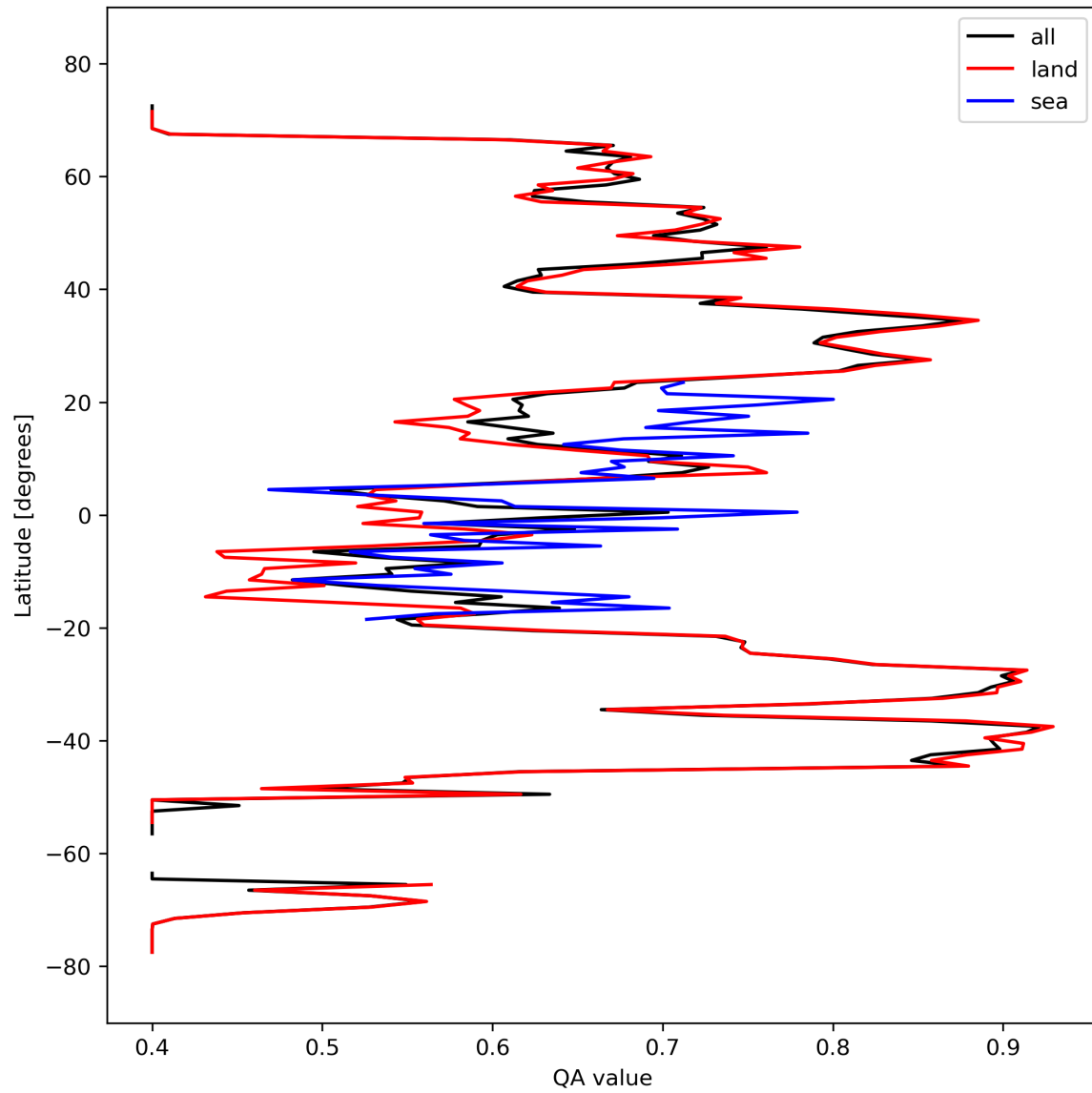
Figure 11: Zonal average of “QA value” for 2024-03-11 to 2024-03-13.
