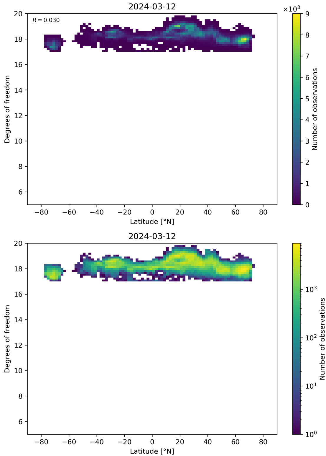
Figure 55: Scatter density plot of “Latitude” against “Degrees of freedom” for 2024-03-11 to 2024-03-13.
