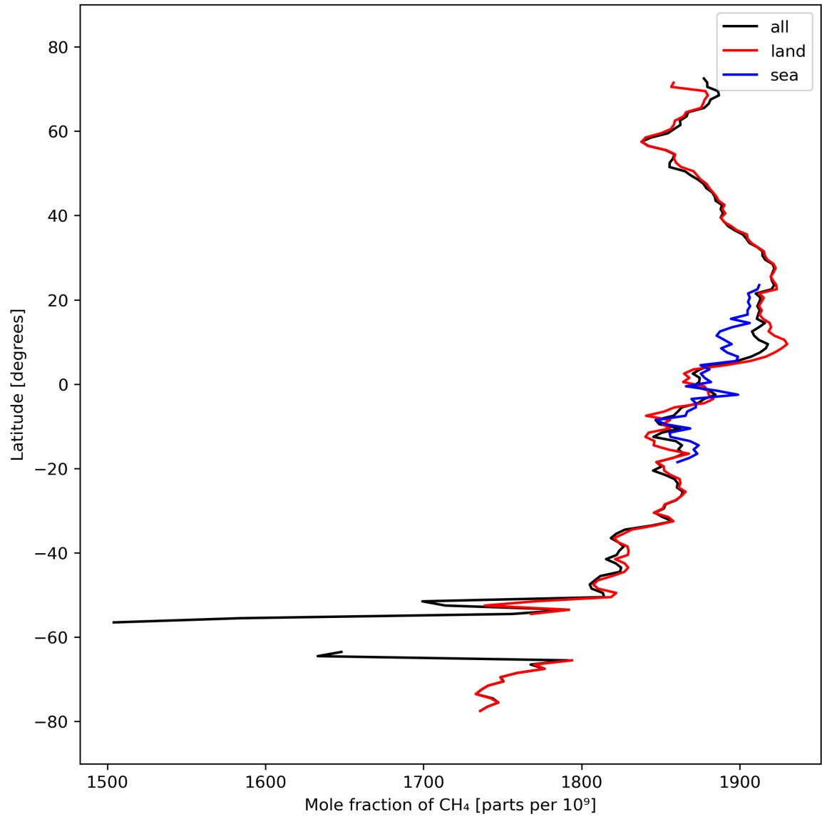
Figure 12: Zonal average of “Mole fraction of \text{CH}_4 ” for 2024-03-11 to 2024-03-13.
