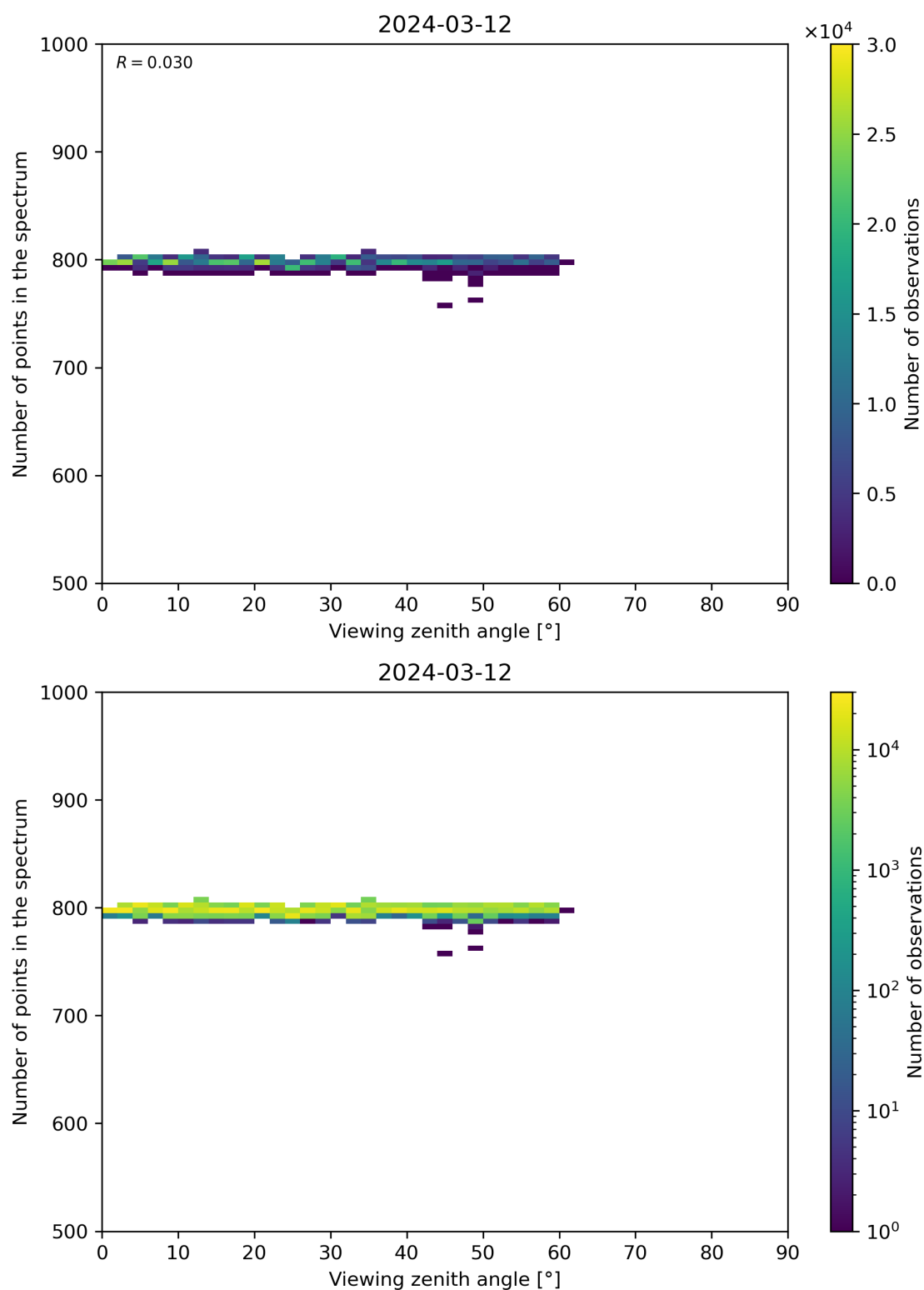
Figure 114: Scatter density plot of “Viewing zenith angle” against “Number of points in the spectrum” for 2024-03-11 to 2024-03-13.
