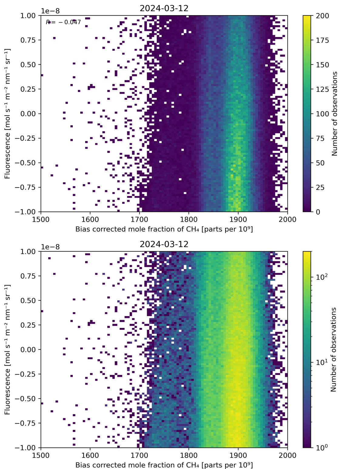
Figure 66: Scatter density plot of “Bias corrected mole fraction of \text{CH}_4 ” against “Fluorescence” for 2024-03-11 to 2024-03-13.
