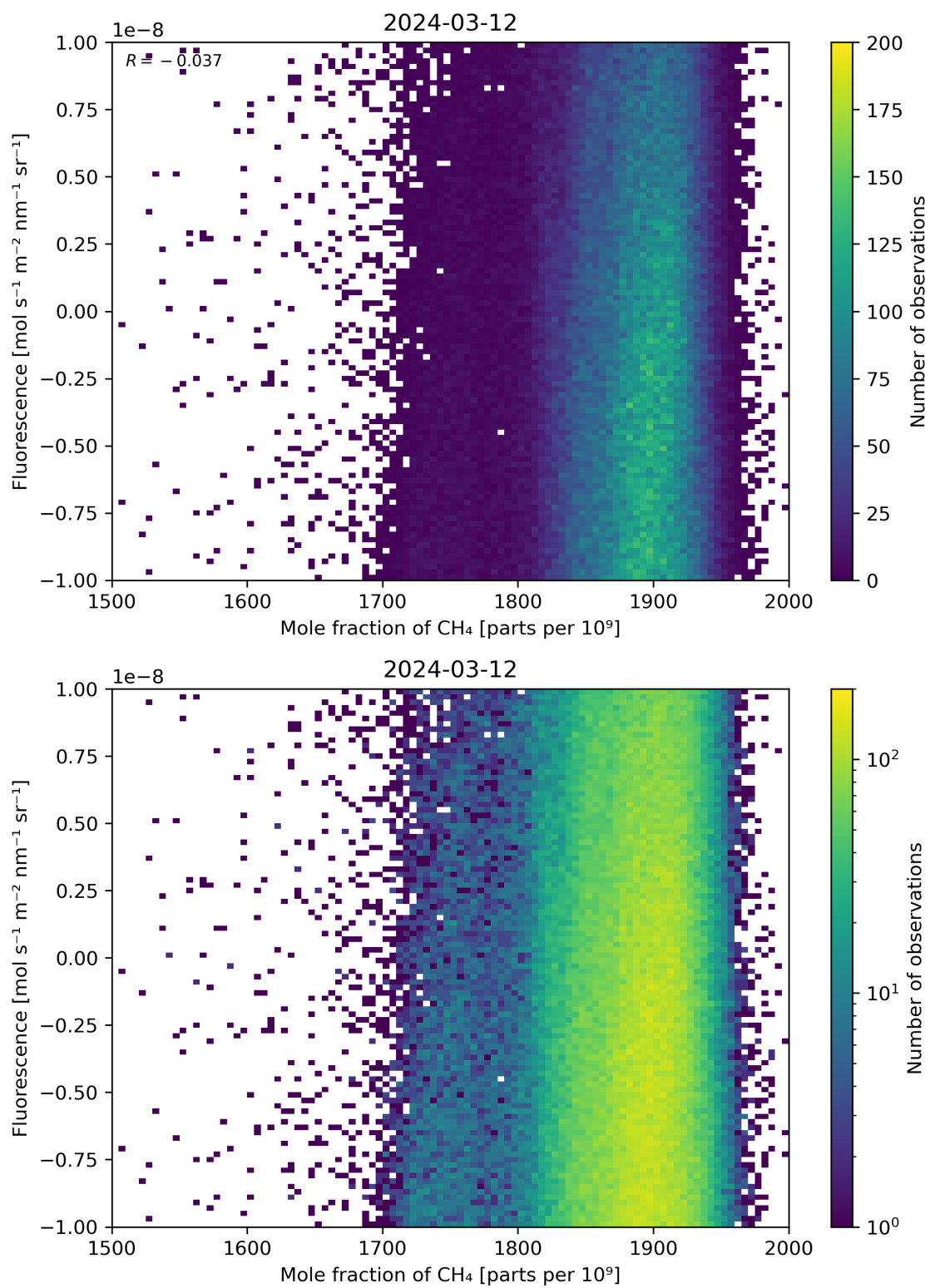
Figure 73: Scatter density plot of “Mole fraction of \text{CH}_4 ” against “Fluorescence” for 2024-03-11 to 2024-03-13.
