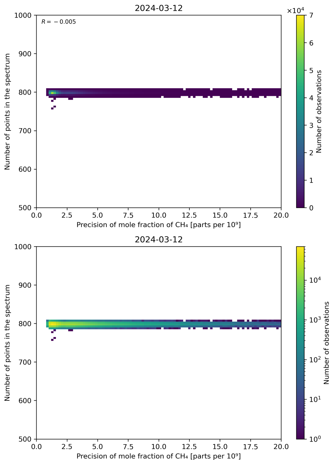
Figure 84: Scatter density plot of “Precision of mole fraction of CH 4 ” against “Number of points in the spectrum” for 2024-03-11 to 2024-03-13.
