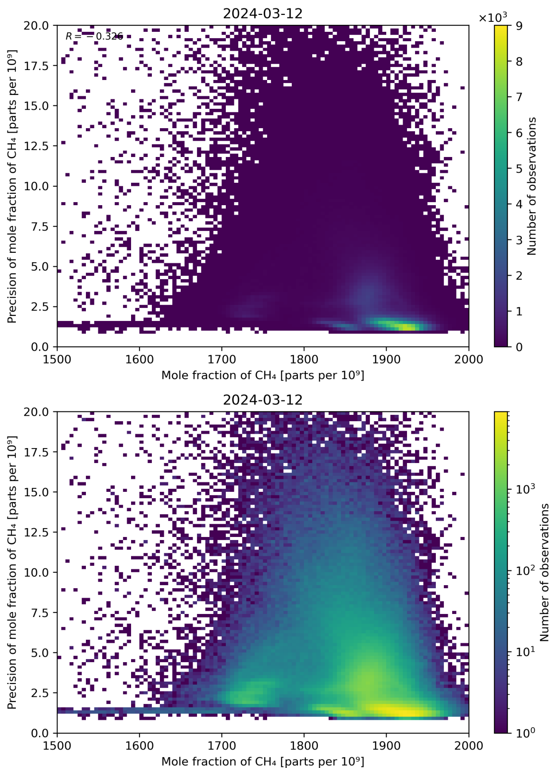
Figure 75: Scatter density plot of “Mole fraction of CH 4 ” against “Precision of mole fraction of CH 4 ” for 2024-03-11 to 2024-03-13.
