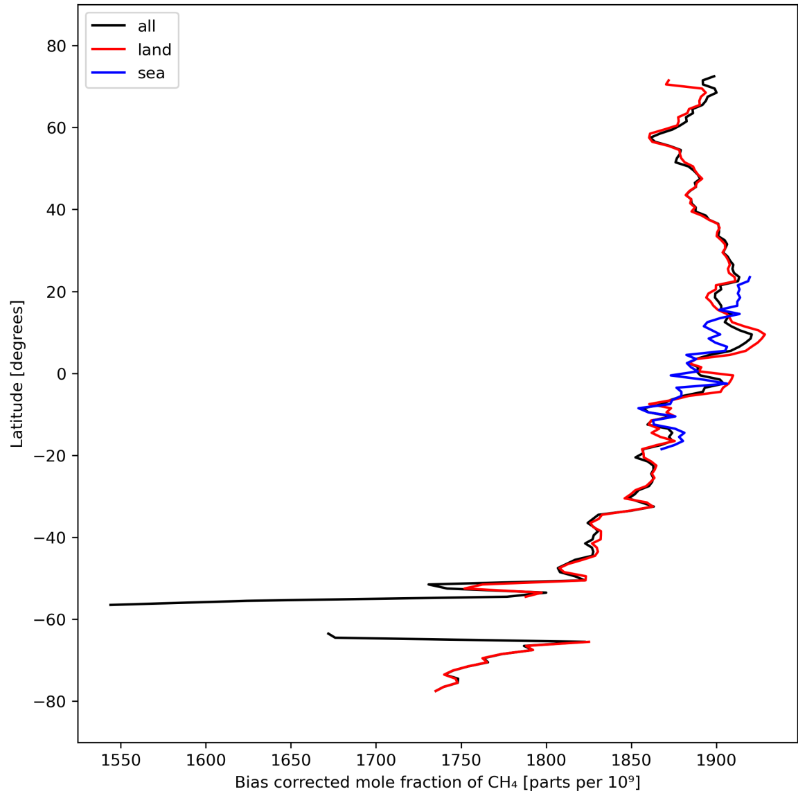
Figure 14: Zonal average of “Bias corrected mole fraction of CH 4 ” for 2024-03-11 to 2024-03-13.
