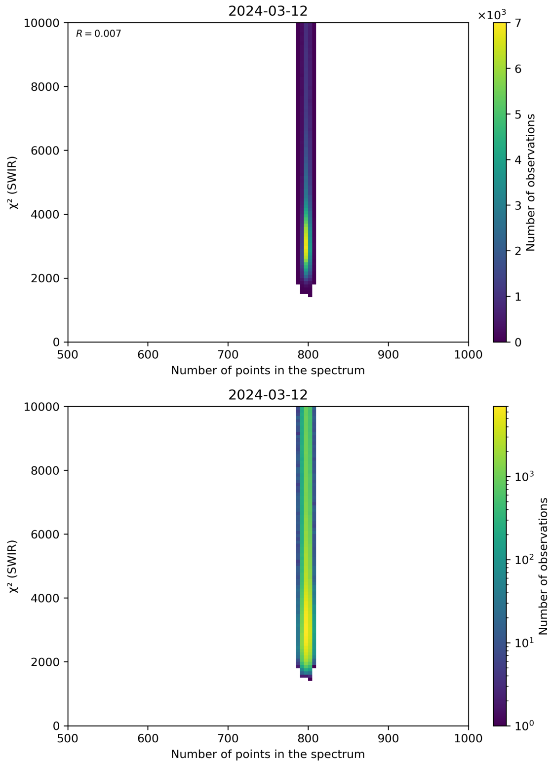
Figure 89: Scatter density plot of “Number of points in the spectrum” against “ \chi^2 (SWIR)” for 2024-03-11 to 2024-03-13.
