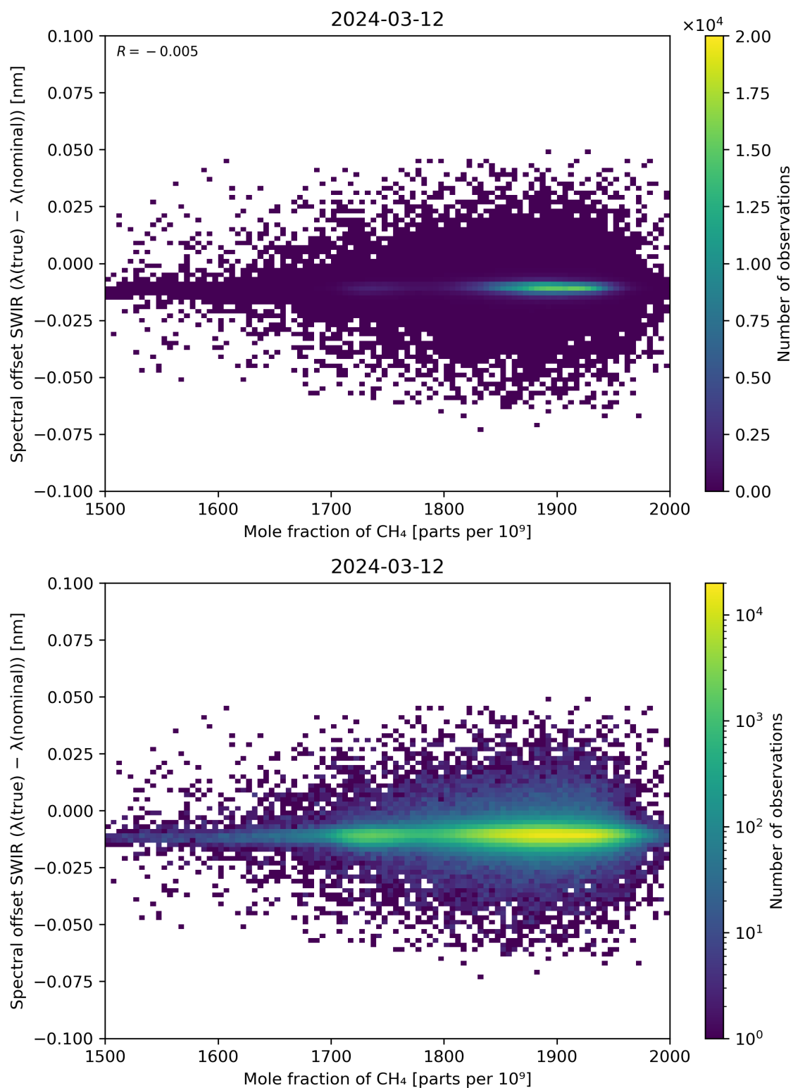
Figure 86: Scatter density plot of “Mole fraction of CH 4 ” against “Spectral offset SWIR ( \lambda(\text{true}) - \lambda(\text{nominal}) )” for 2024-03-11 to 2024-03-13.
