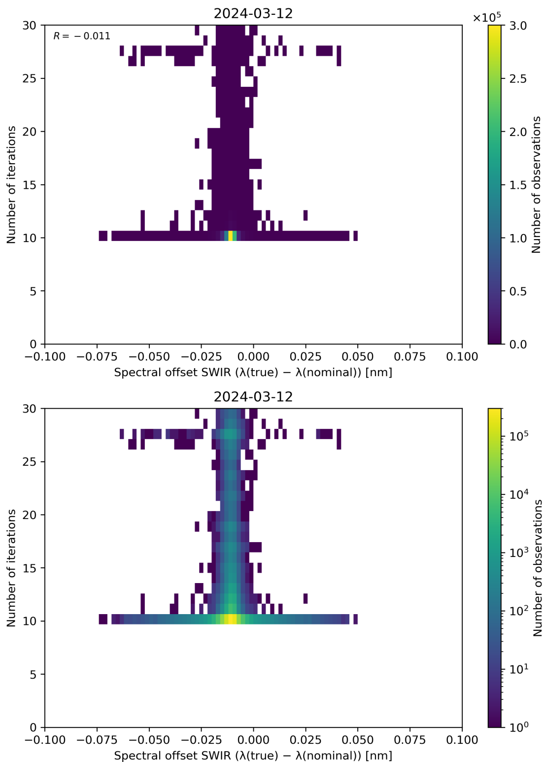
Figure 121: Scatter density plot of “Spectral offset SWIR ( \lambda(\text{true}) - \lambda(\text{nominal}) )” against “Number of iterations” for 2024-03-11 to 2024-03-13.
