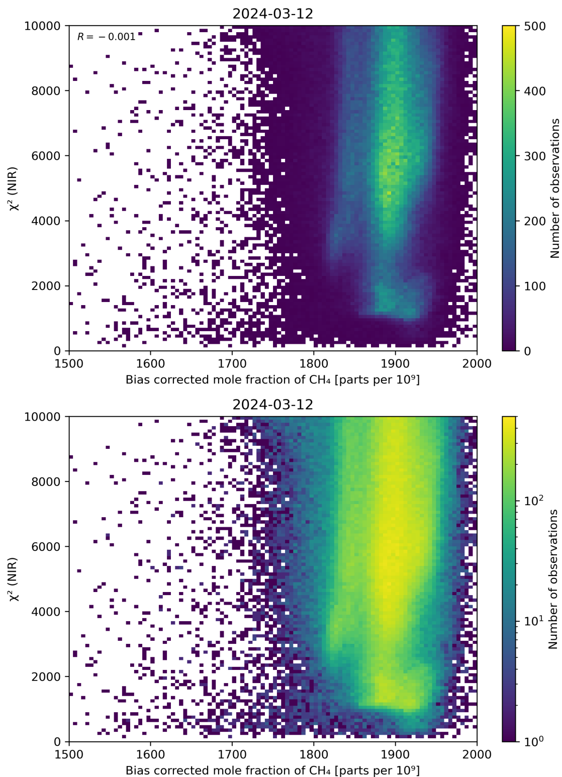
Figure 63: Scatter density plot of “Bias corrected mole fraction of CH 4 ” against “ \chi^2 (NIR)” for 2024-03-11 to 2024-03-13.
