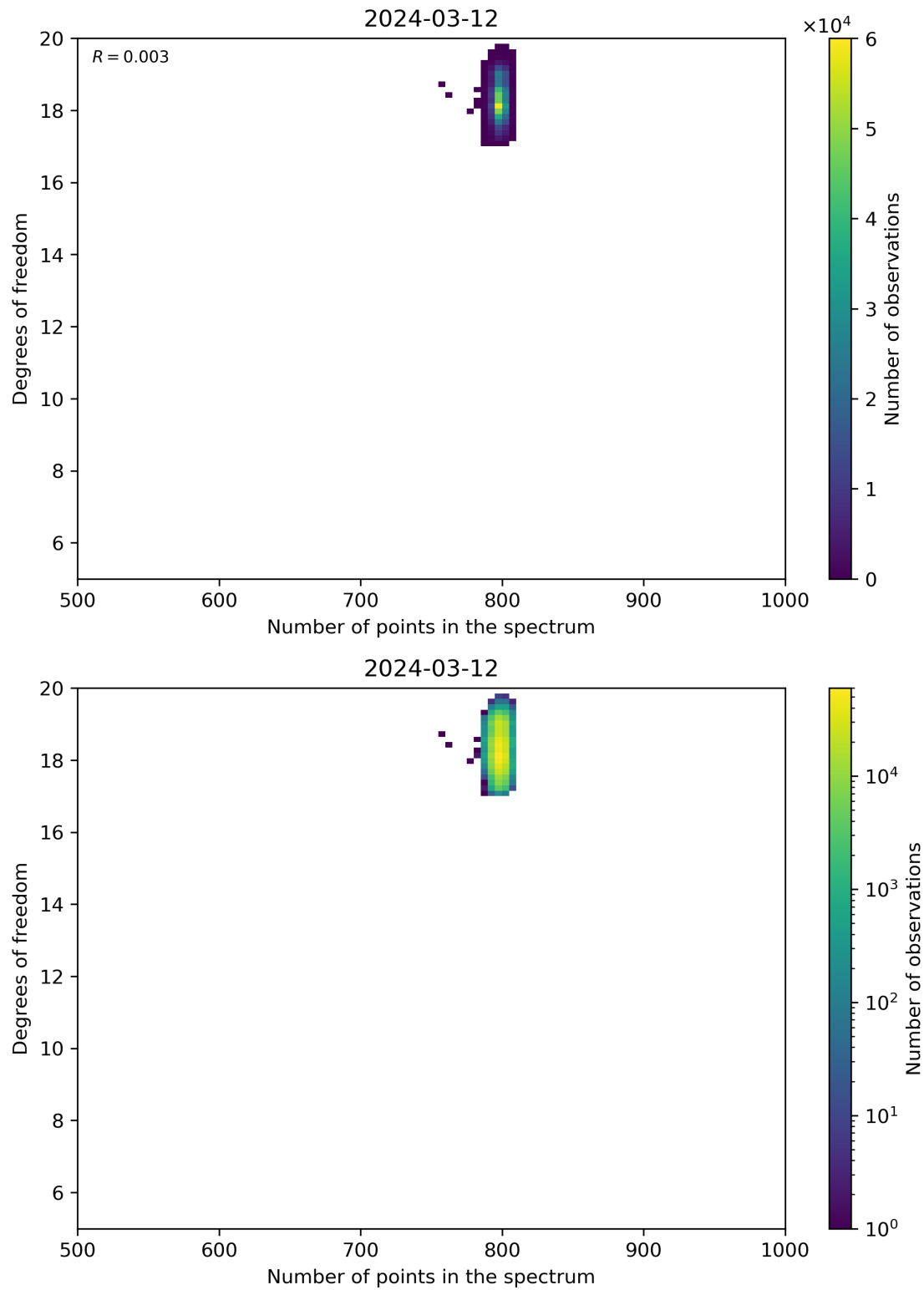
Figure 90: Scatter density plot of “Number of points in the spectrum” against “Degrees of freedom” for 2024-03-11 to 2024-03-13.
