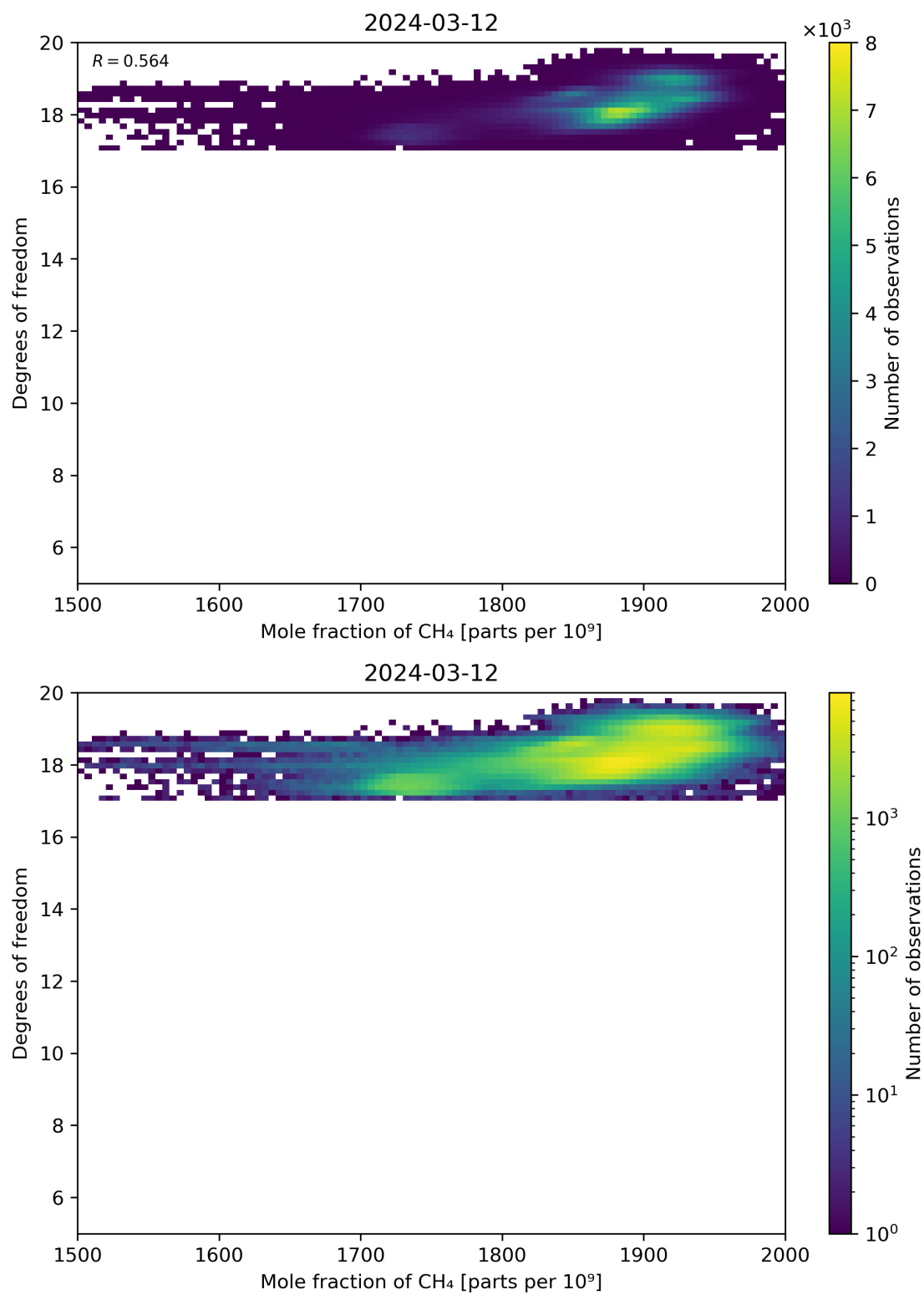
Figure 72: Scatter density plot of “Mole fraction of CH 4 ” against “Degrees of freedom” for 2024-03-11 to 2024-03-13.
