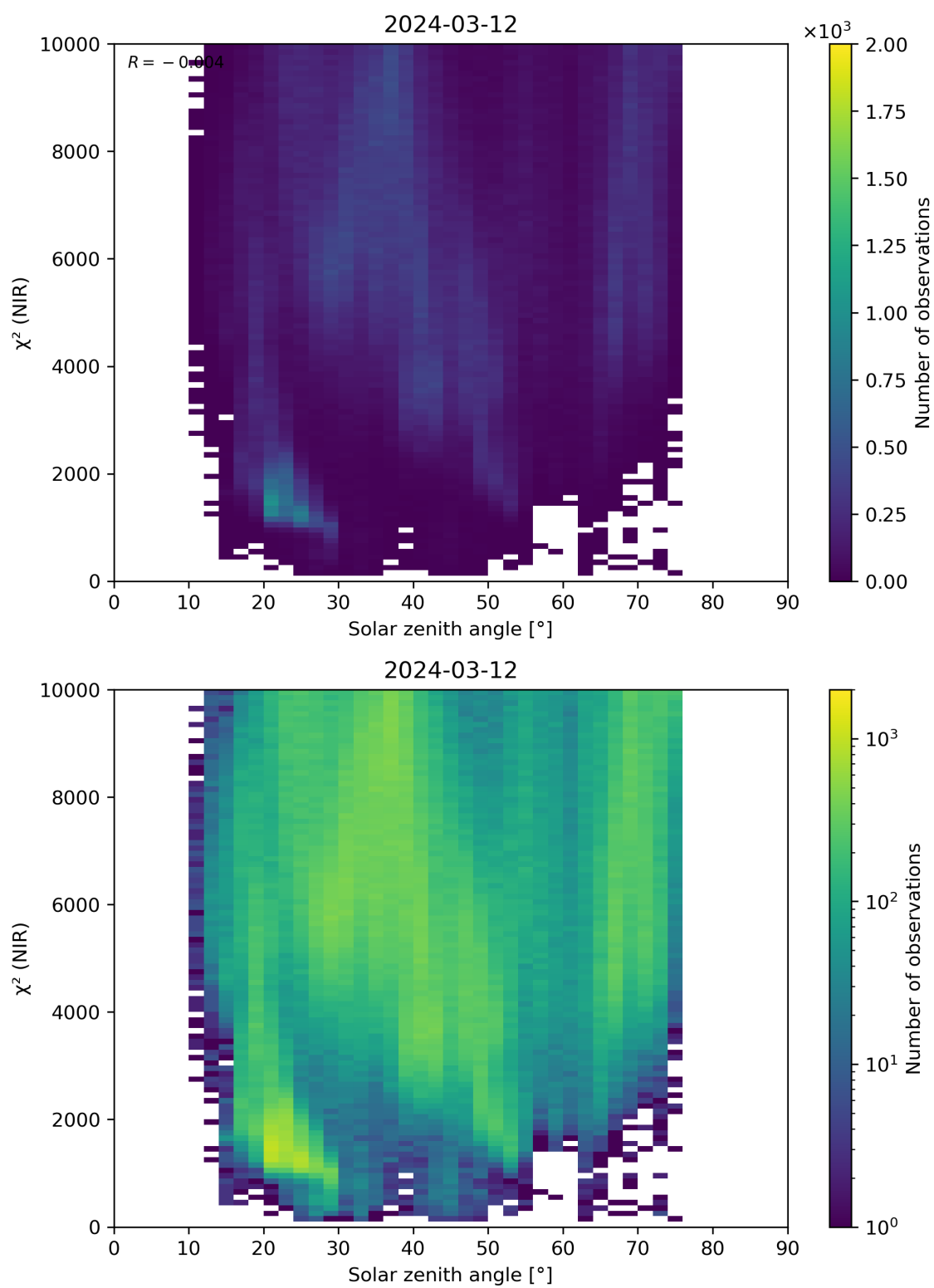
Figure 94: Scatter density plot of “Solar zenith angle” against “ \chi^2 (NIR)” for 2024-03-11 to 2024-03-13.
