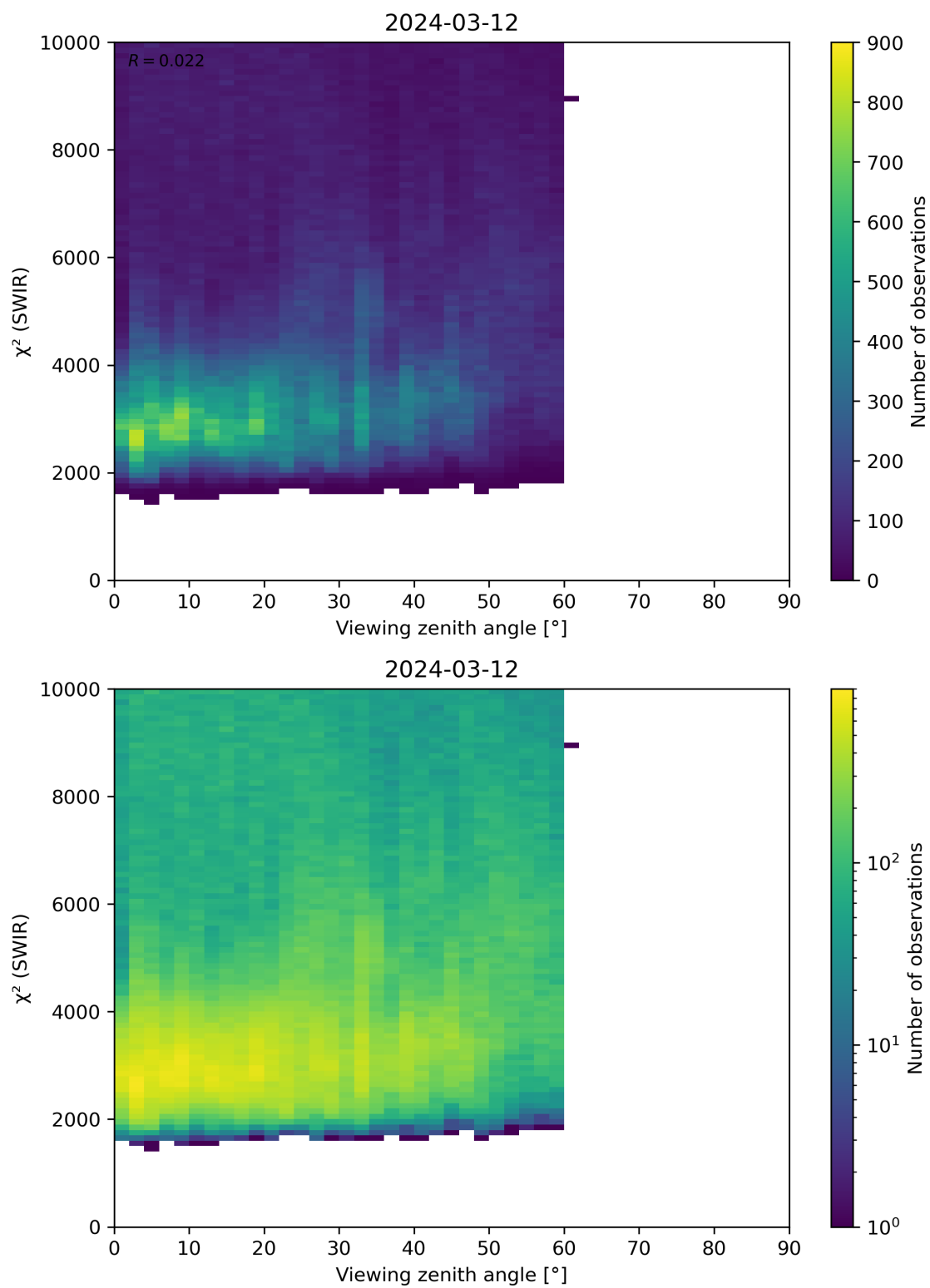
Figure 106: Scatter density plot of “Viewing zenith angle” against “ \chi^2 (SWIR)” for 2024-03-11 to 2024-03-13.
