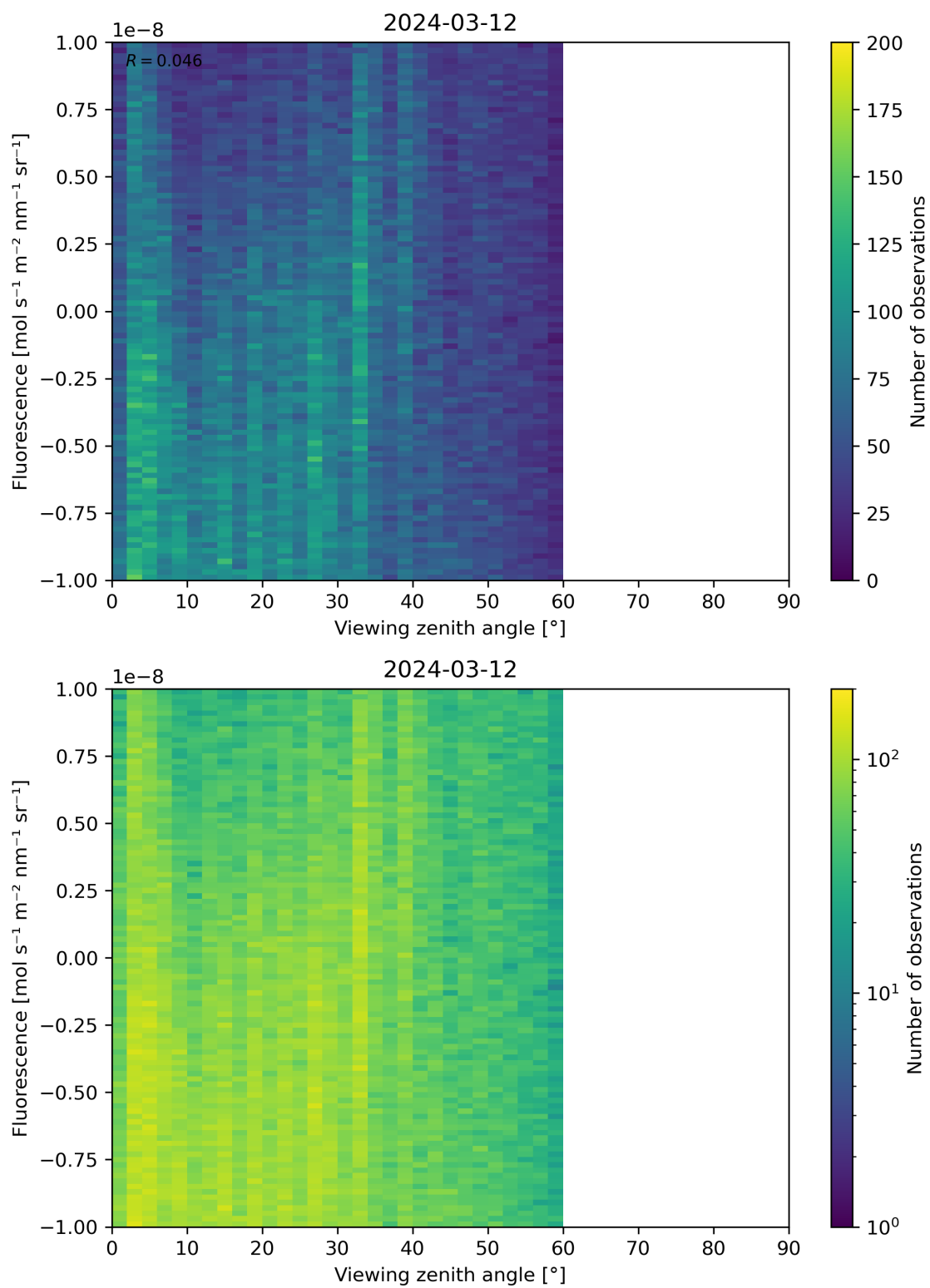
Figure 108: Scatter density plot of “Viewing zenith angle” against “Fluorescence” for 2024-03-11 to 2024-03-13.
