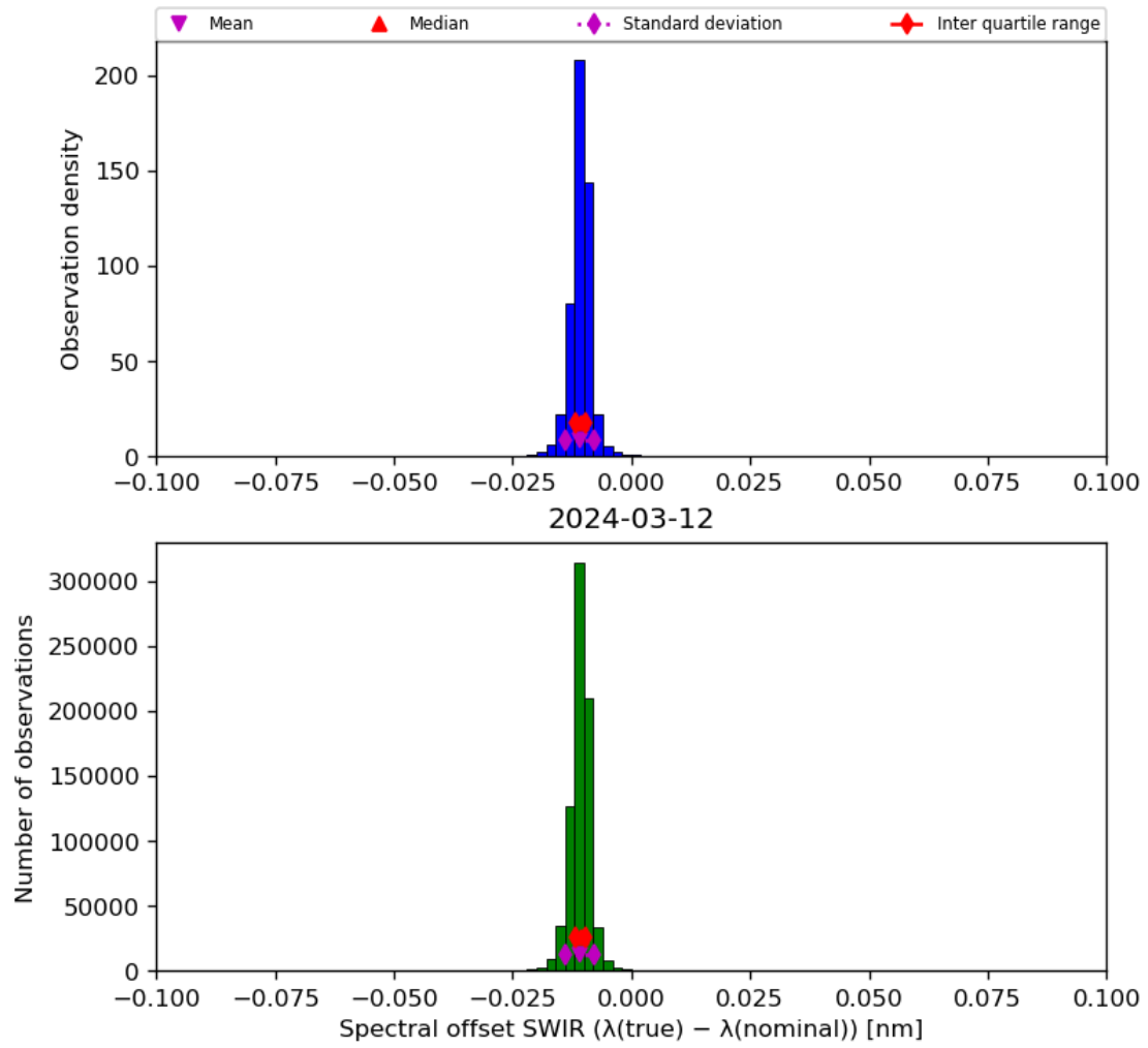
Figure 27: Histogram of “Spectral offset SWIR ( \lambda(\text{true}) - \lambda(\text{nominal}) )” for 2024-03-11 to 2024-03-13
