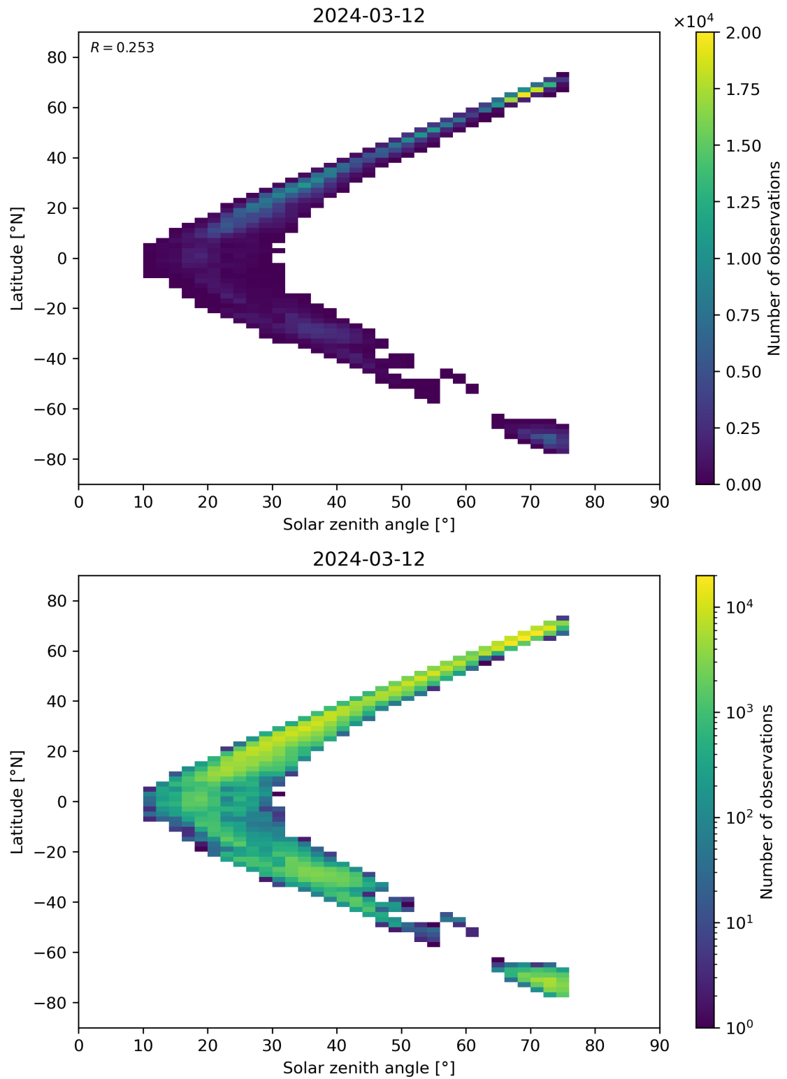
Figure 98: Scatter density plot of “Solar zenith angle” against “Latitude” for 2024-03-11 to 2024-03-13.
