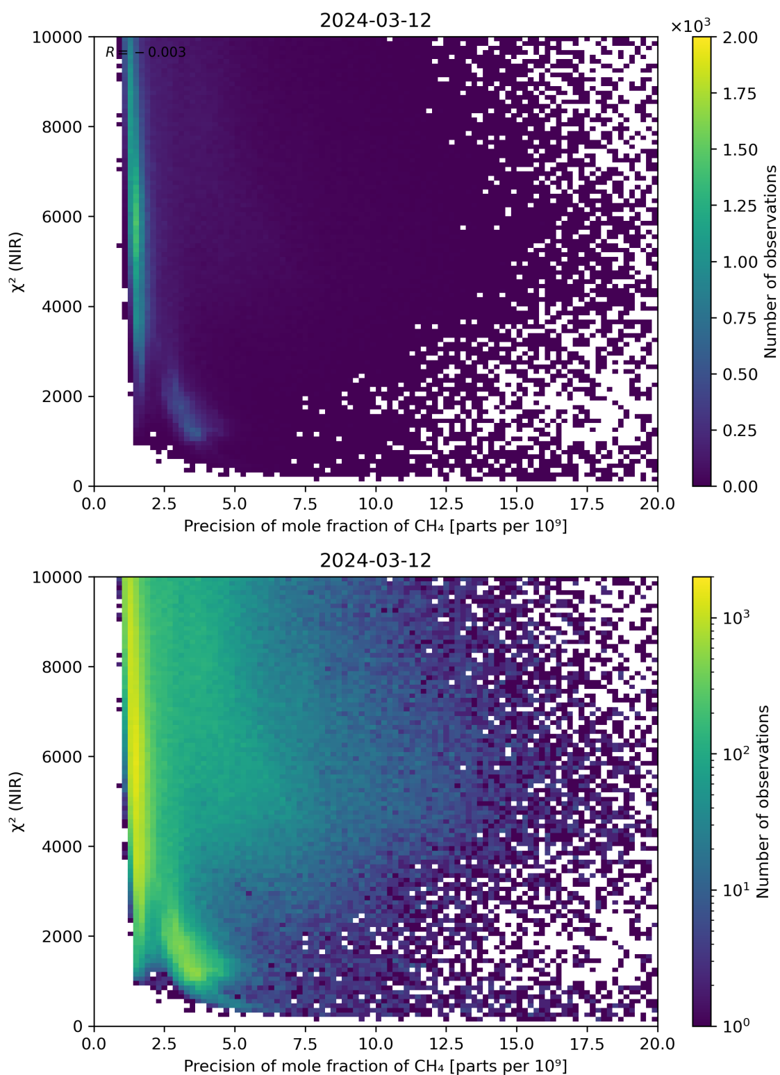
Figure 78: Scatter density plot of “Precision of mole fraction of CH 4 ” against “ \chi^2 (NIR)” for 2024-03-11 to 2024-03-13.
