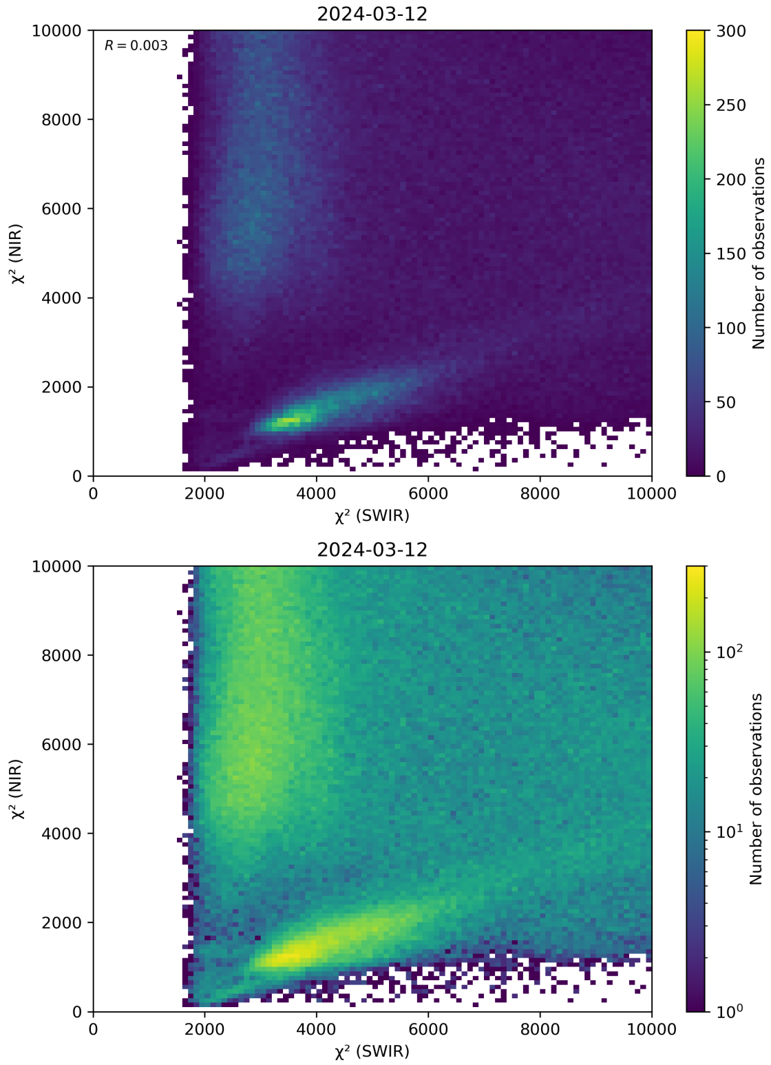
Figure 47: Scatter density plot of “ \chi^2 (SWIR)” against “ \chi^2 (NIR)” for 2024-03-11 to 2024-03-13.
