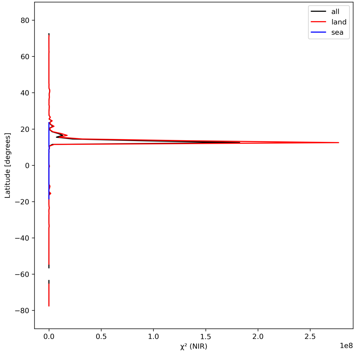
Figure 18: Zonal average of “ \chi^2 (NIR)” for 2024-03-11 to 2024-03-13.
