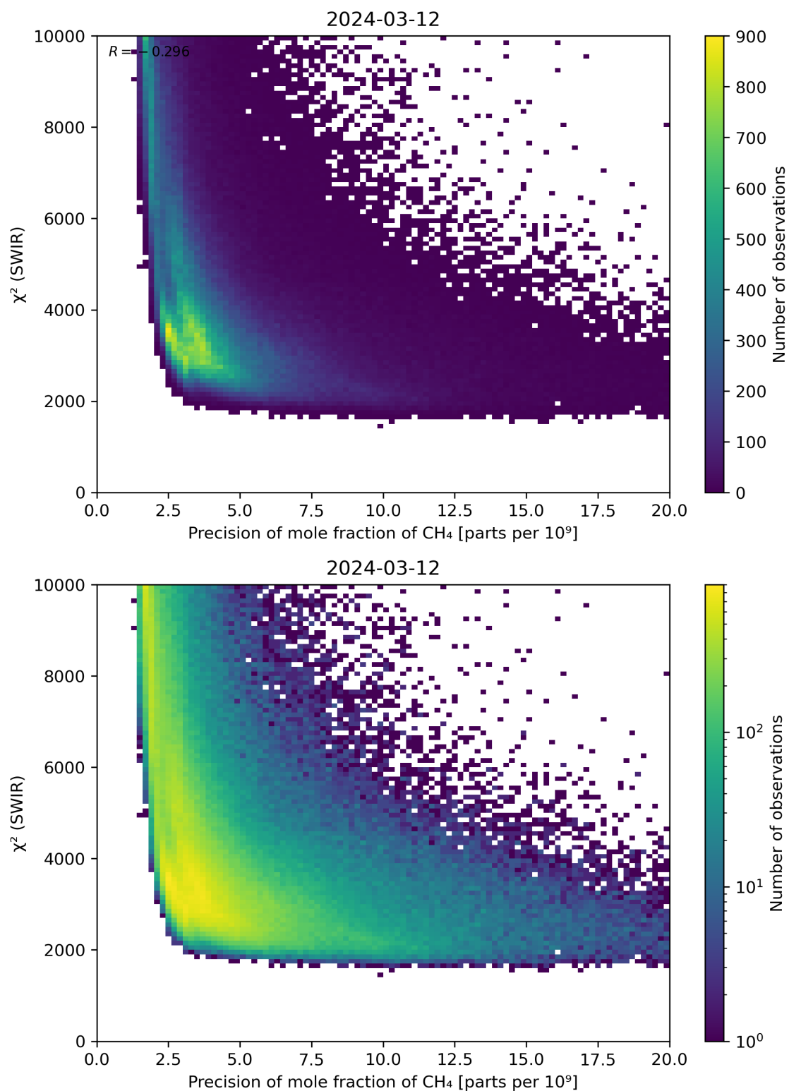
Figure 79: Scatter density plot of “Precision of mole fraction of \text{CH}_4 ” against “ \chi^2 (SWIR)” for 2024-03-11 to 2024-03-13.
