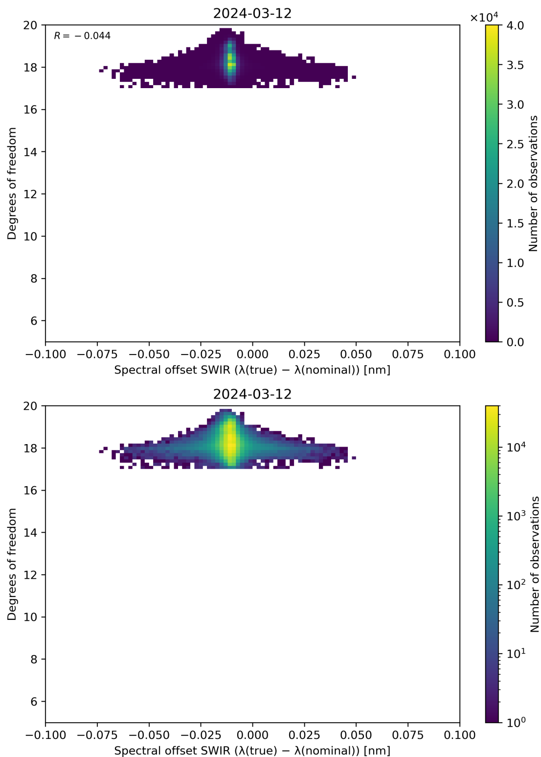
Figure 119: Scatter density plot of “Spectral offset SWIR ( \lambda(\text{true}) - \lambda(\text{nominal}) )” against “Degrees of freedom” for 2024-03-11 to 2024-03-13.
