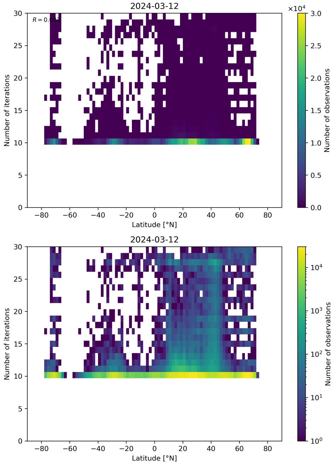
Figure 60: Scatter density plot of “Latitude” against “Number of iterations” for 2024-03-11 to 2024-03-13.
