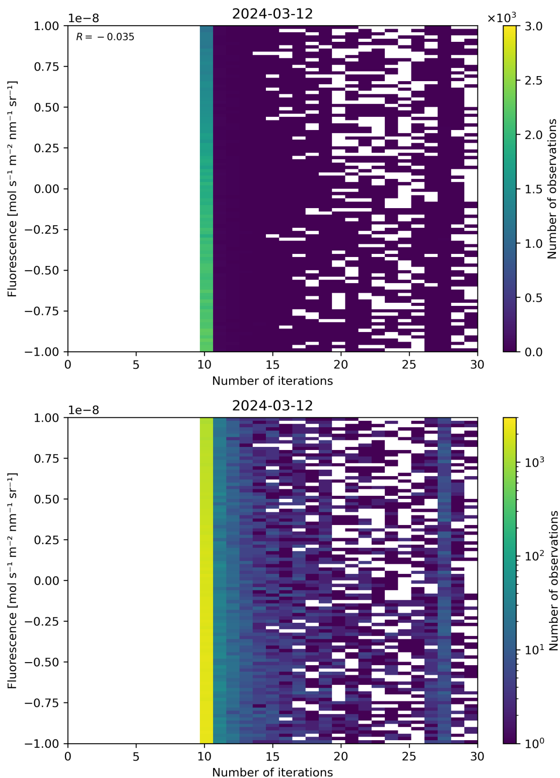
Figure 87: Scatter density plot of “Number of iterations” against “Fluorescence” for 2024-03-11 to 2024-03-13.
