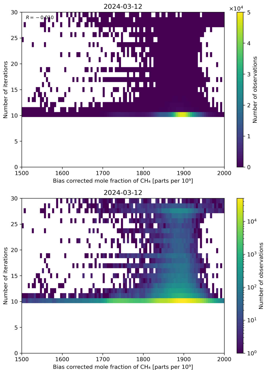
Figure 67: Scatter density plot of “Bias corrected mole fraction of CH 4 ” against “Number of iterations” for 2024-03-11 to 2024-03-13.
