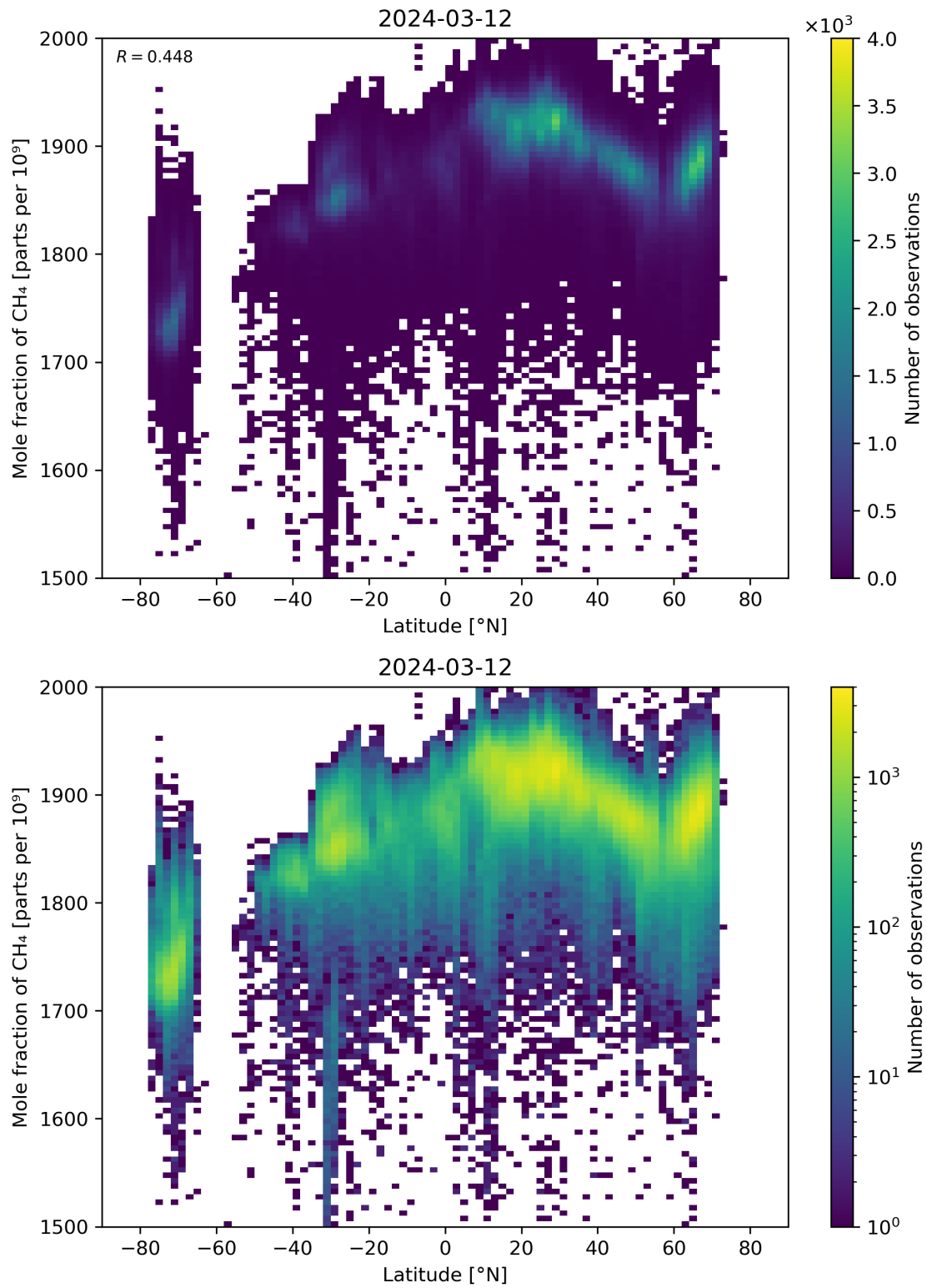
Figure 57: Scatter density plot of “Latitude” against “Mole fraction of CH 4 ” for 2024-03-11 to 2024-03-13.
