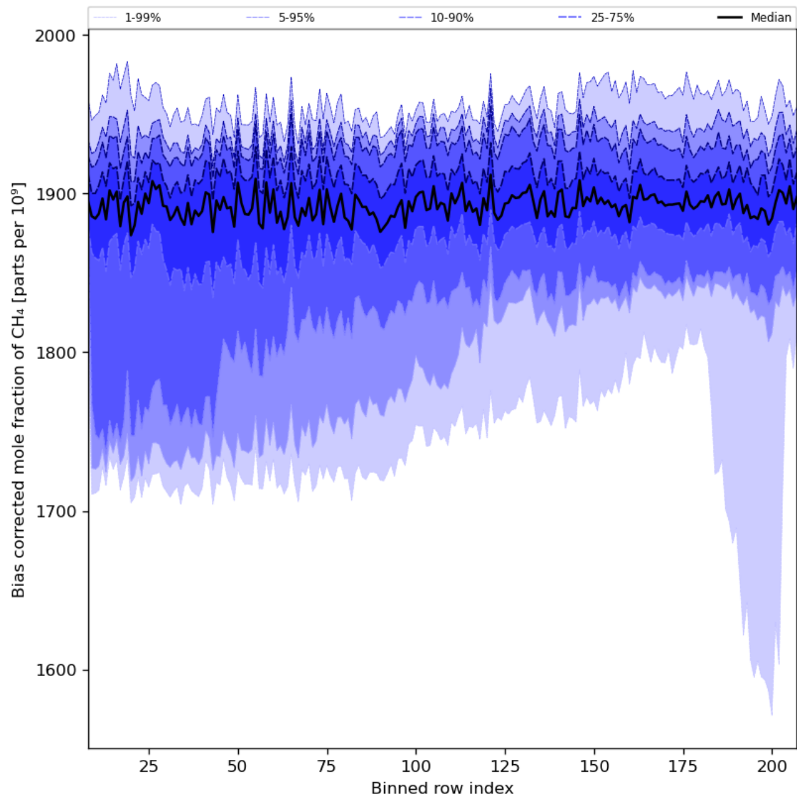
Figure 36: Along track statistics of “Bias corrected mole fraction of CH 4 ” for 2024-03-11 to 2024-03-13
