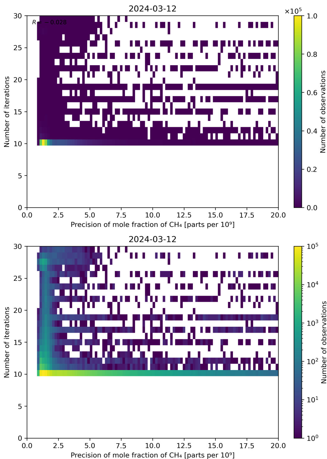
Figure 83: Scatter density plot of “Precision of mole fraction of CH 4 ” against “Number of iterations” for 2024-03-11 to 2024-03-13.
