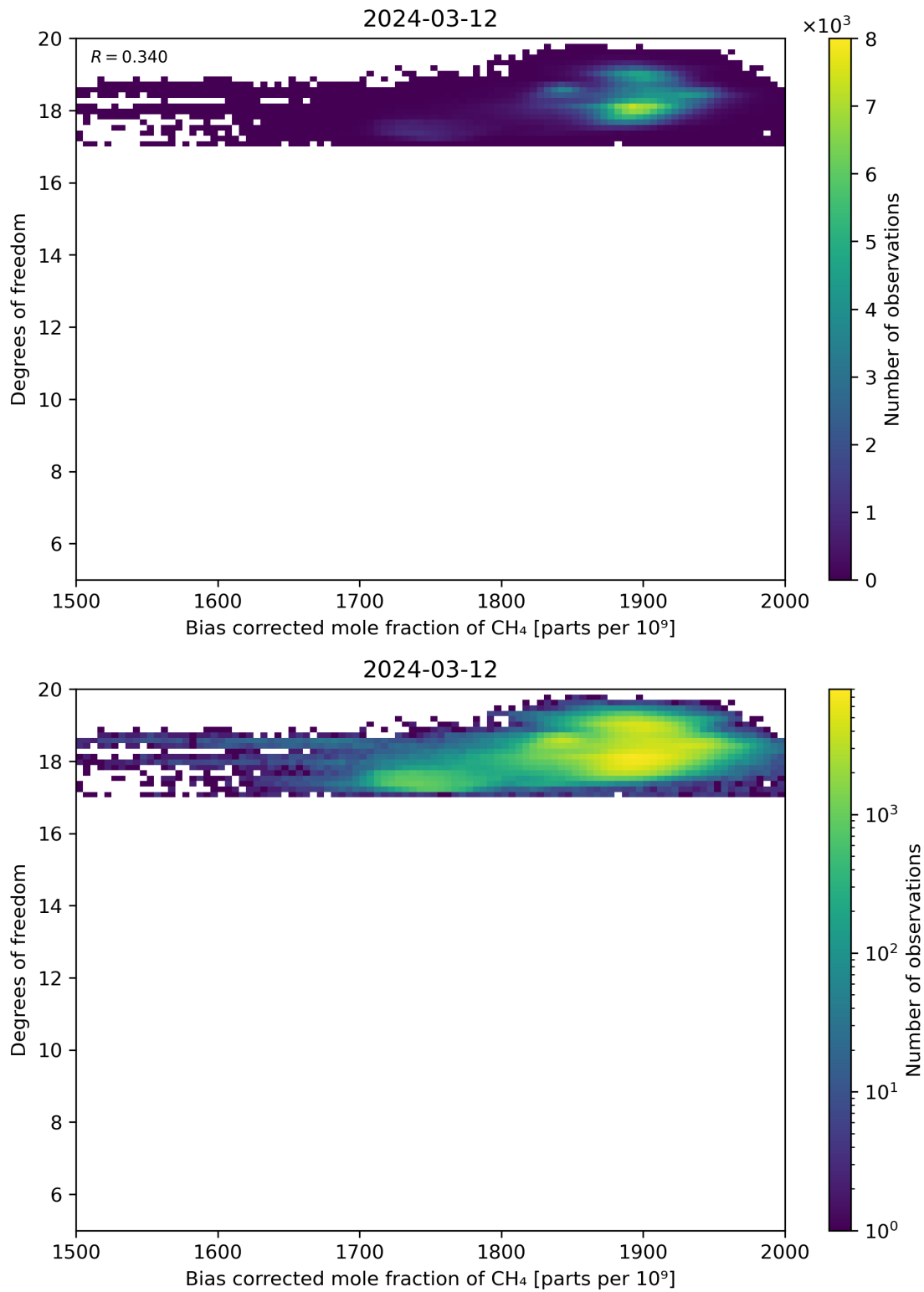
Figure 65: Scatter density plot of “Bias corrected mole fraction of CH 4 ” against “Degrees of freedom” for 2024-03-11 to 2024-03-13.
