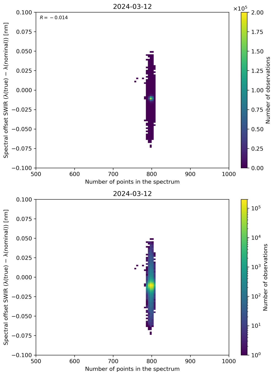
Figure 93: Scatter density plot of “Number of points in the spectrum” against “Spectral offset SWIR ( \lambda(\text{true}) - \lambda(\text{nominal}) )” for 2024-03-11 to 2024-03-13.
