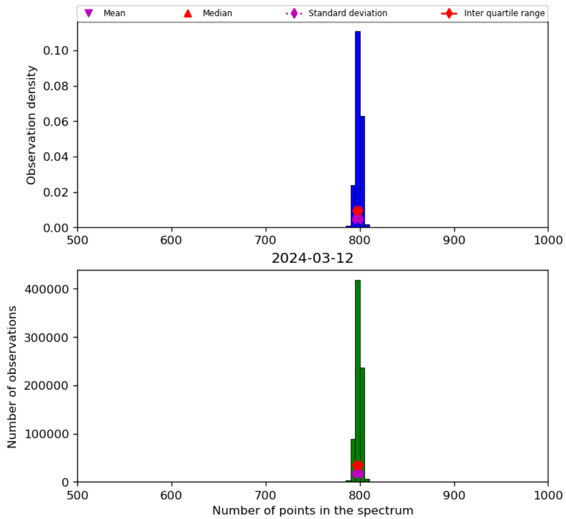
Figure 26: Histogram of “Number of points in the spectrum” for 2024-03-11 to 2024-03-13
