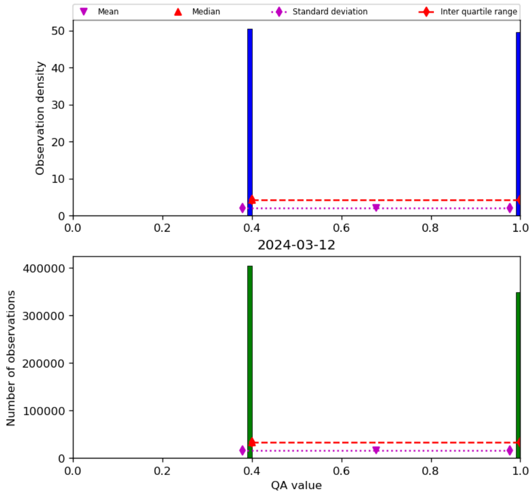
Figure 22: Histogram of “QA value” for 2024-03-11 to 2024-03-13
