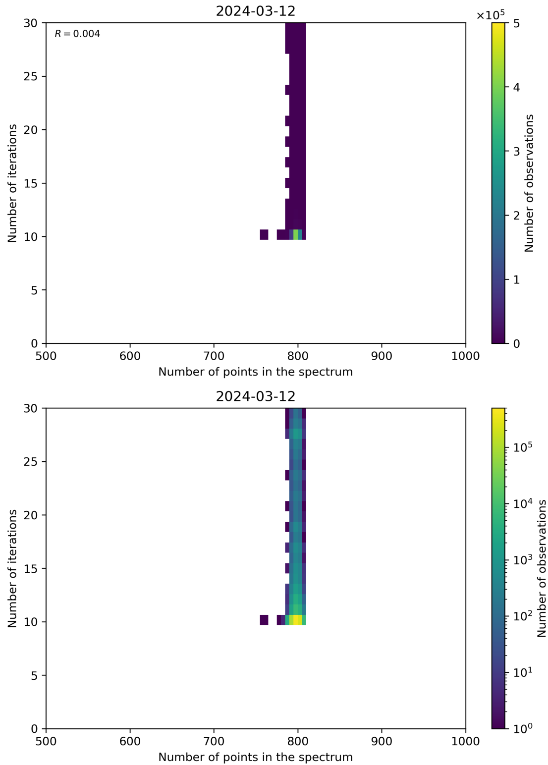
Figure 92: Scatter density plot of “Number of points in the spectrum” against “Number of iterations” for 2024-03-11 to 2024-03-13.
