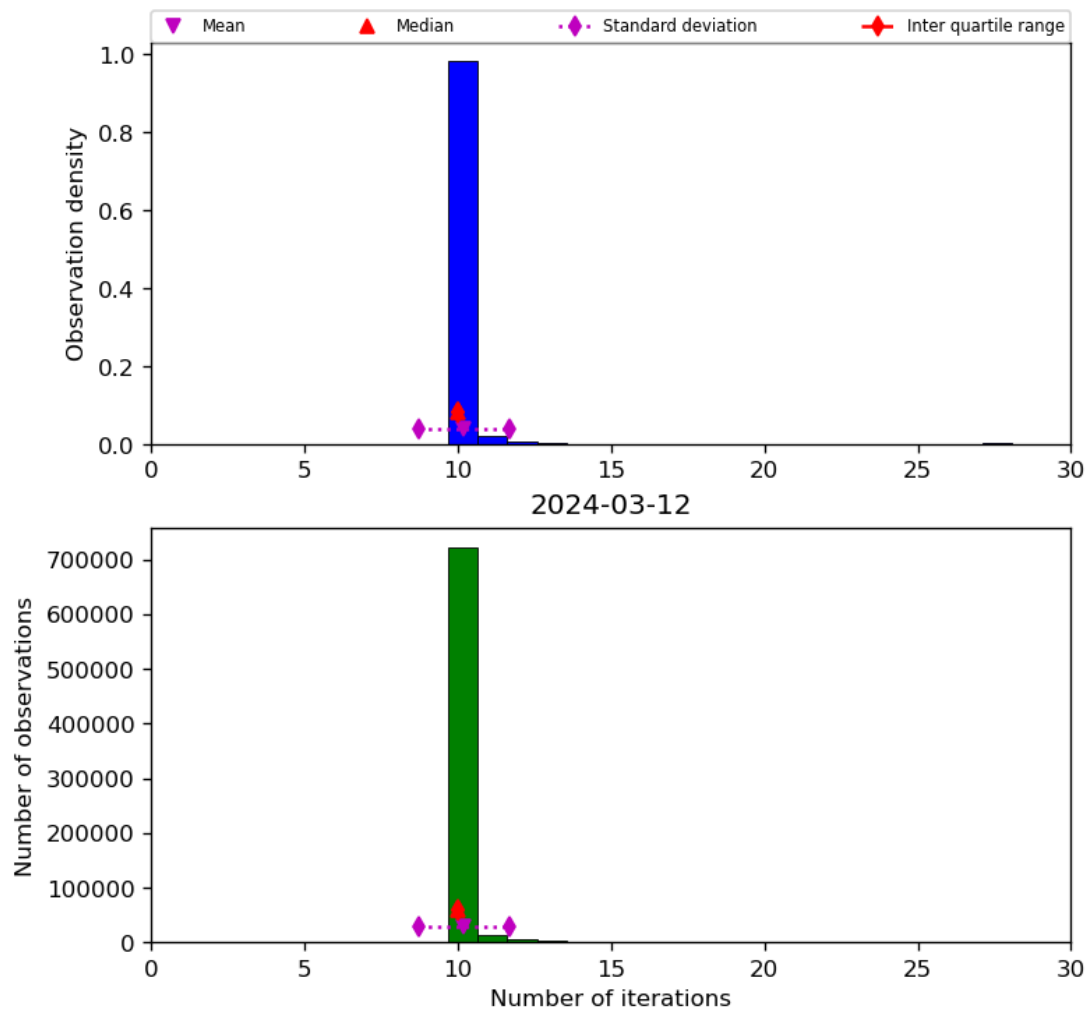
Figure 31: Histogram of “Number of iterations” for 2024-03-11 to 2024-03-13
