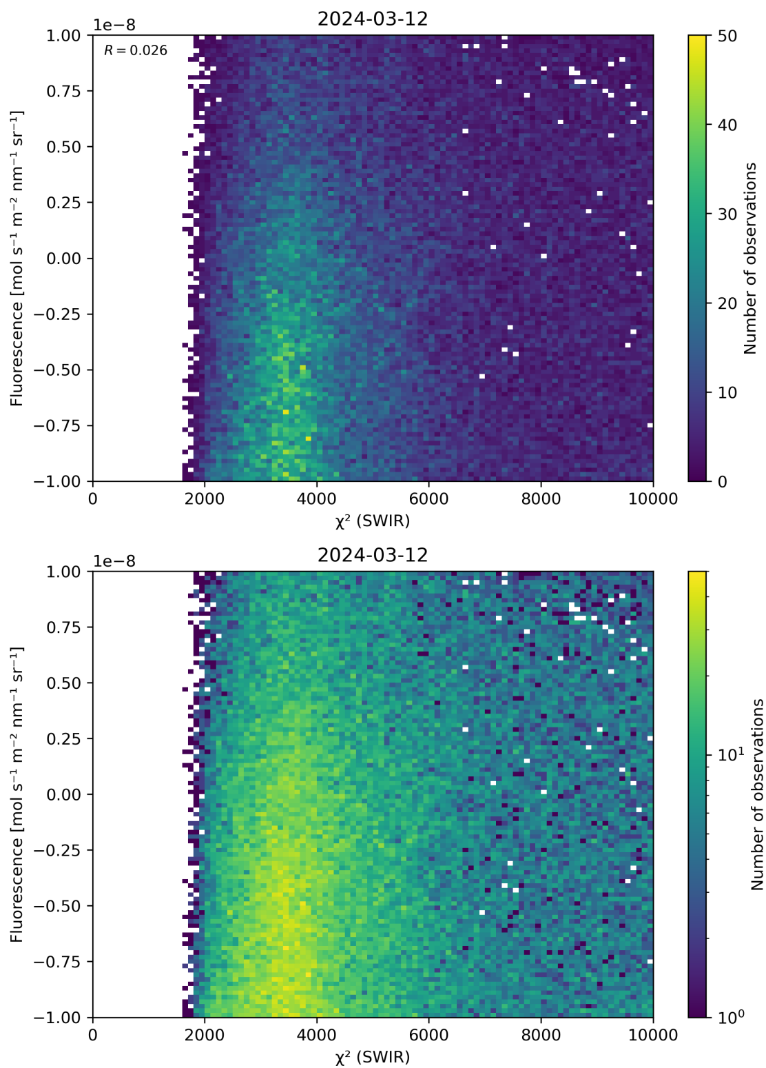
Figure 49: Scatter density plot of “ \chi^2 (SWIR)” against “Fluorescence” for 2024-03-11 to 2024-03-13.
