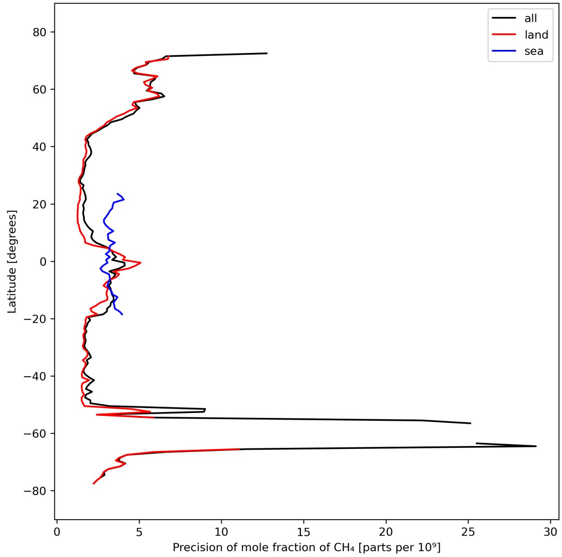
Figure 13: Zonal average of “Precision of mole fraction of CH 4 ” for 2024-03-11 to 2024-03-13.
