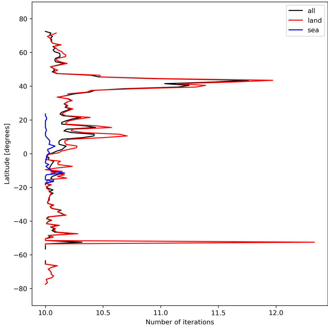
Figure 20: Zonal average of “Number of iterations” for 2024-03-11 to 2024-03-13.
