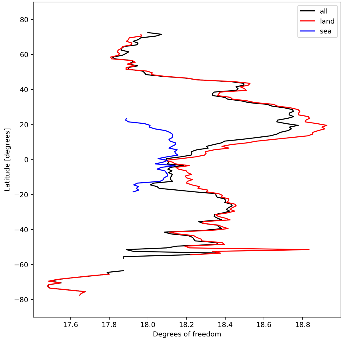
Figure 19: Zonal average of “Degrees of freedom” for 2024-03-11 to 2024-03-13.
