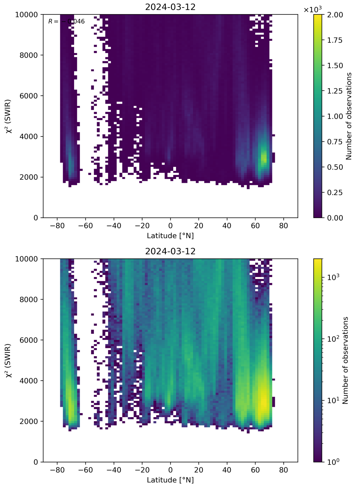
Figure 54: Scatter density plot of “Latitude” against “ \chi^2 (SWIR)” for 2024-03-11 to 2024-03-13.
