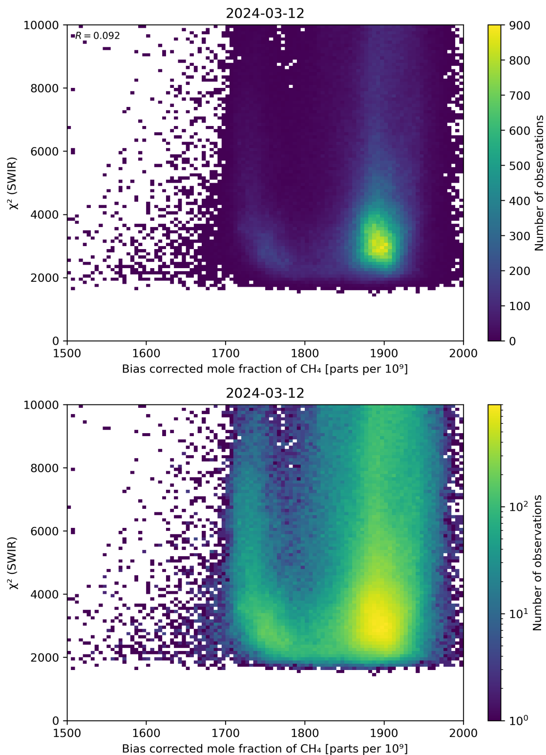
Figure 64: Scatter density plot of “Bias corrected mole fraction of CH 4 ” against “ \chi^2 (SWIR)” for 2024-03-11 to 2024-03-13.
