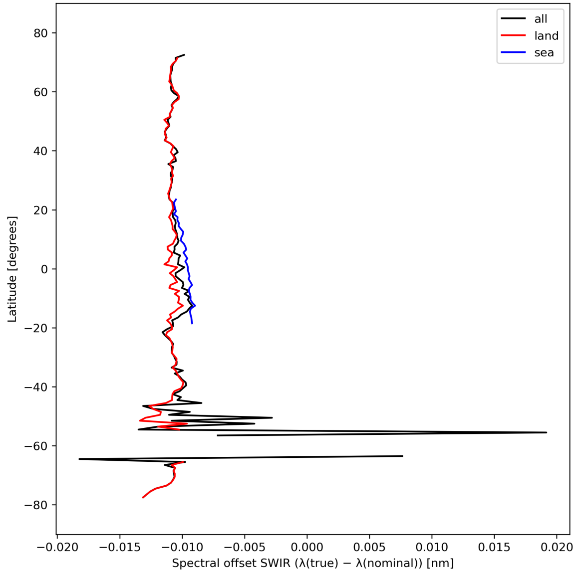
Figure 16: Zonal average of “Spectral offset SWIR ( \lambda(\text{true}) - \lambda(\text{nominal}) )” for 2024-03-11 to 2024-03-13.
