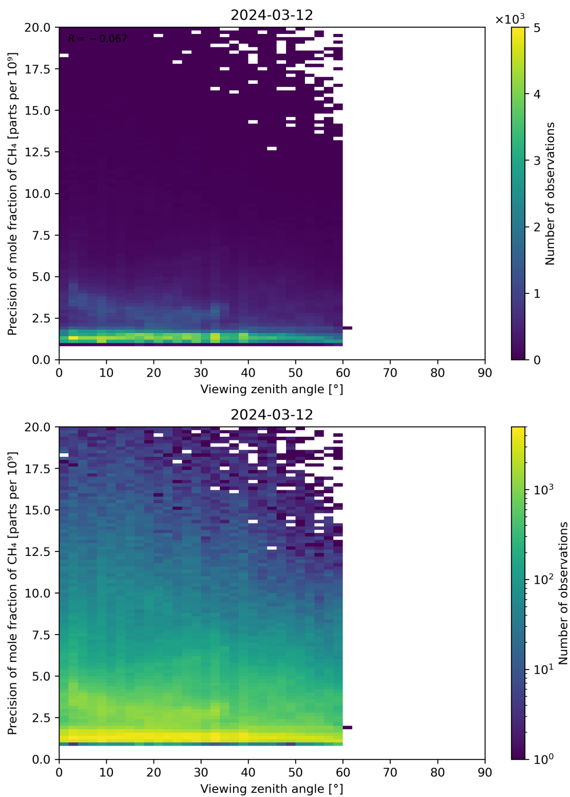
Figure 112: Scatter density plot of “Viewing zenith angle” against “Precision of mole fraction of CH 4 ” for 2024-03-11 to 2024-03-13.
