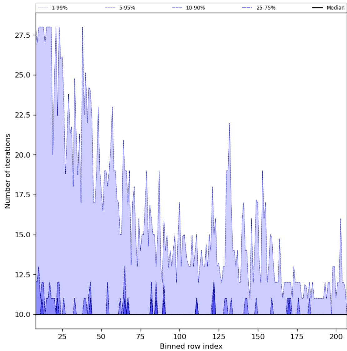
Figure 42: Along track statistics of “Number of iterations” for 2024-03-11 to 2024-03-13
