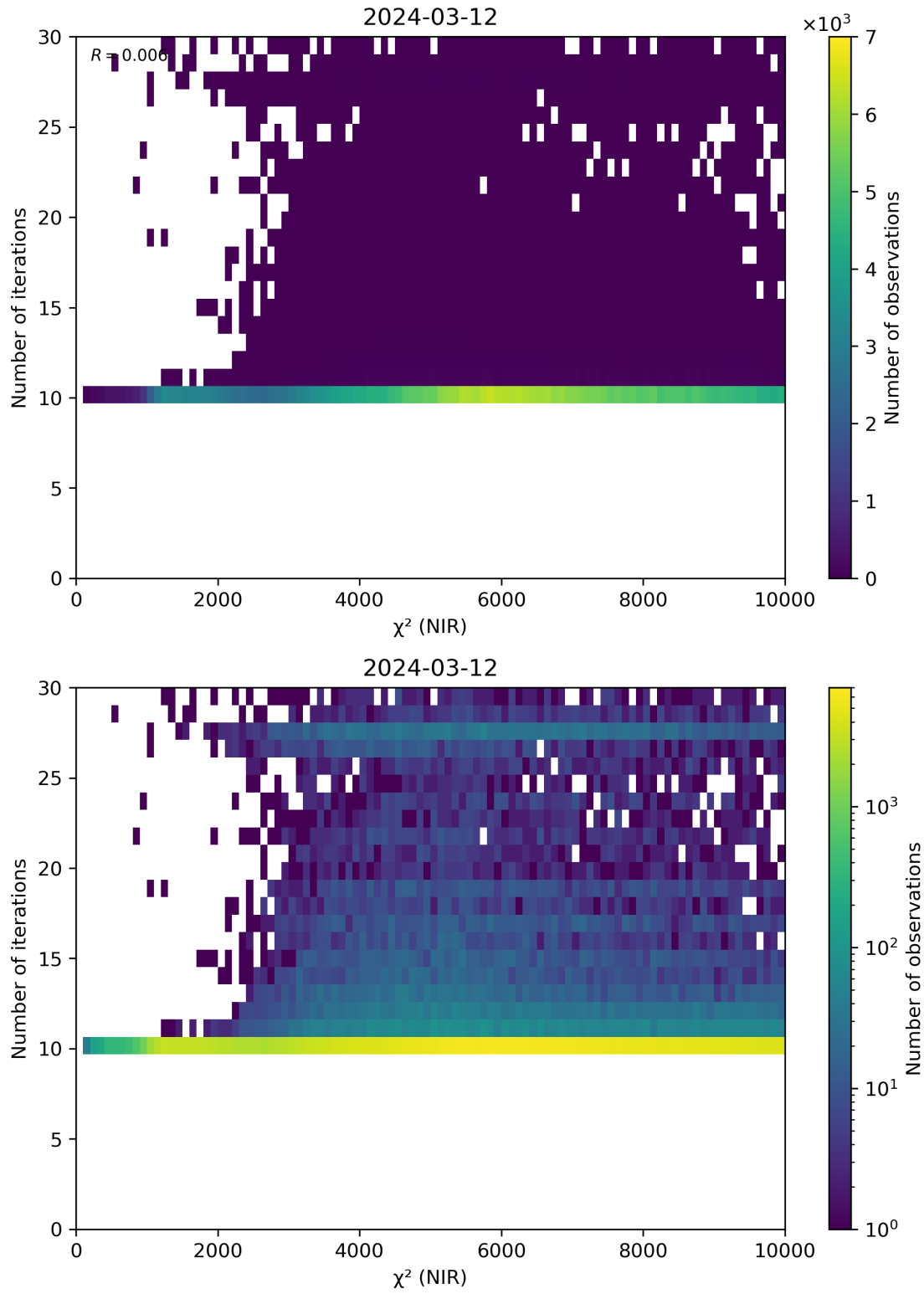
Figure 46: Scatter density plot of “ \chi^2 (NIR)” against “Number of iterations” for 2024-03-11 to 2024-03-13.
