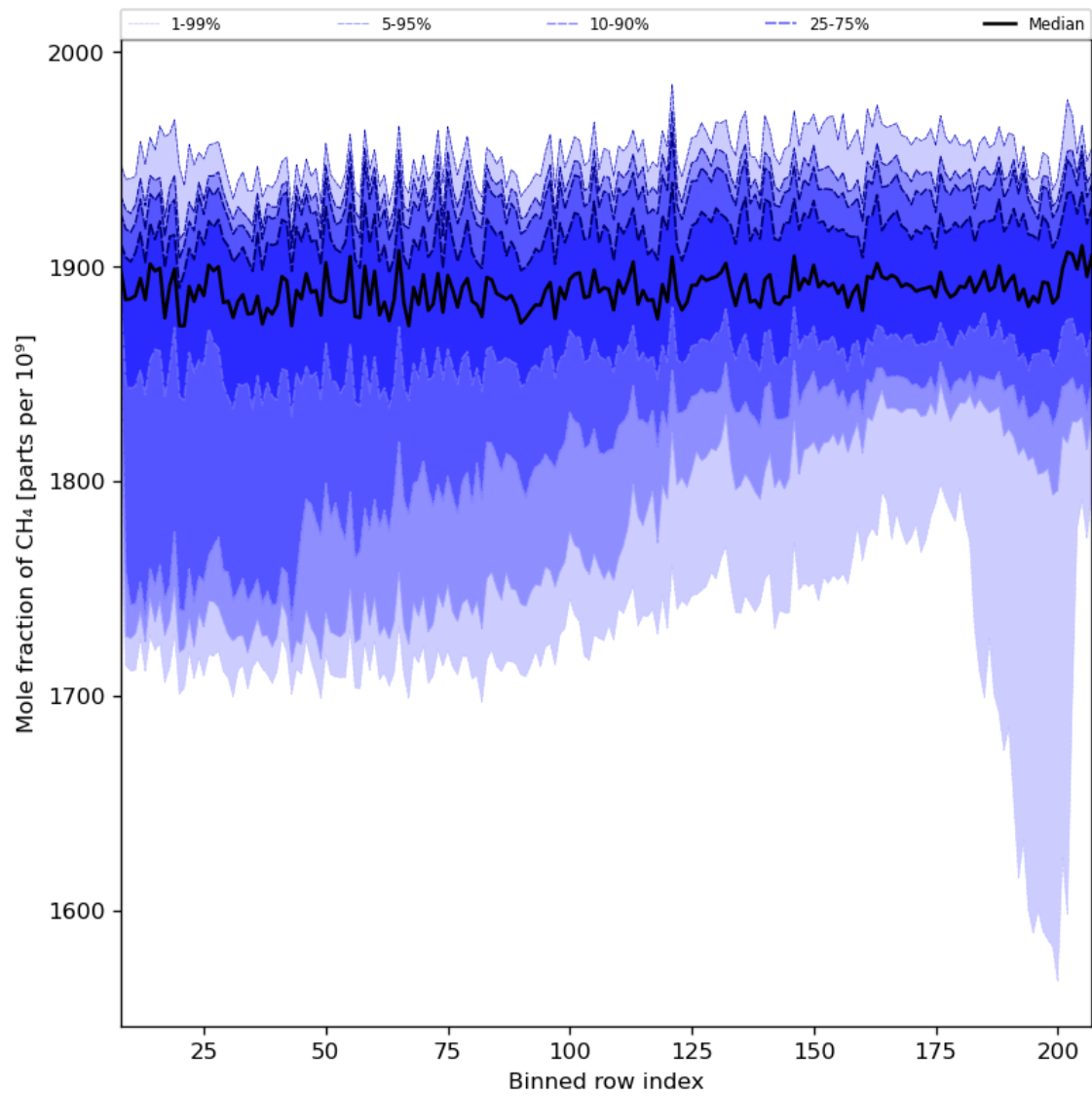
Figure 34: Along track statistics of “Mole fraction of CH 4 ” for 2024-03-11 to 2024-03-13
