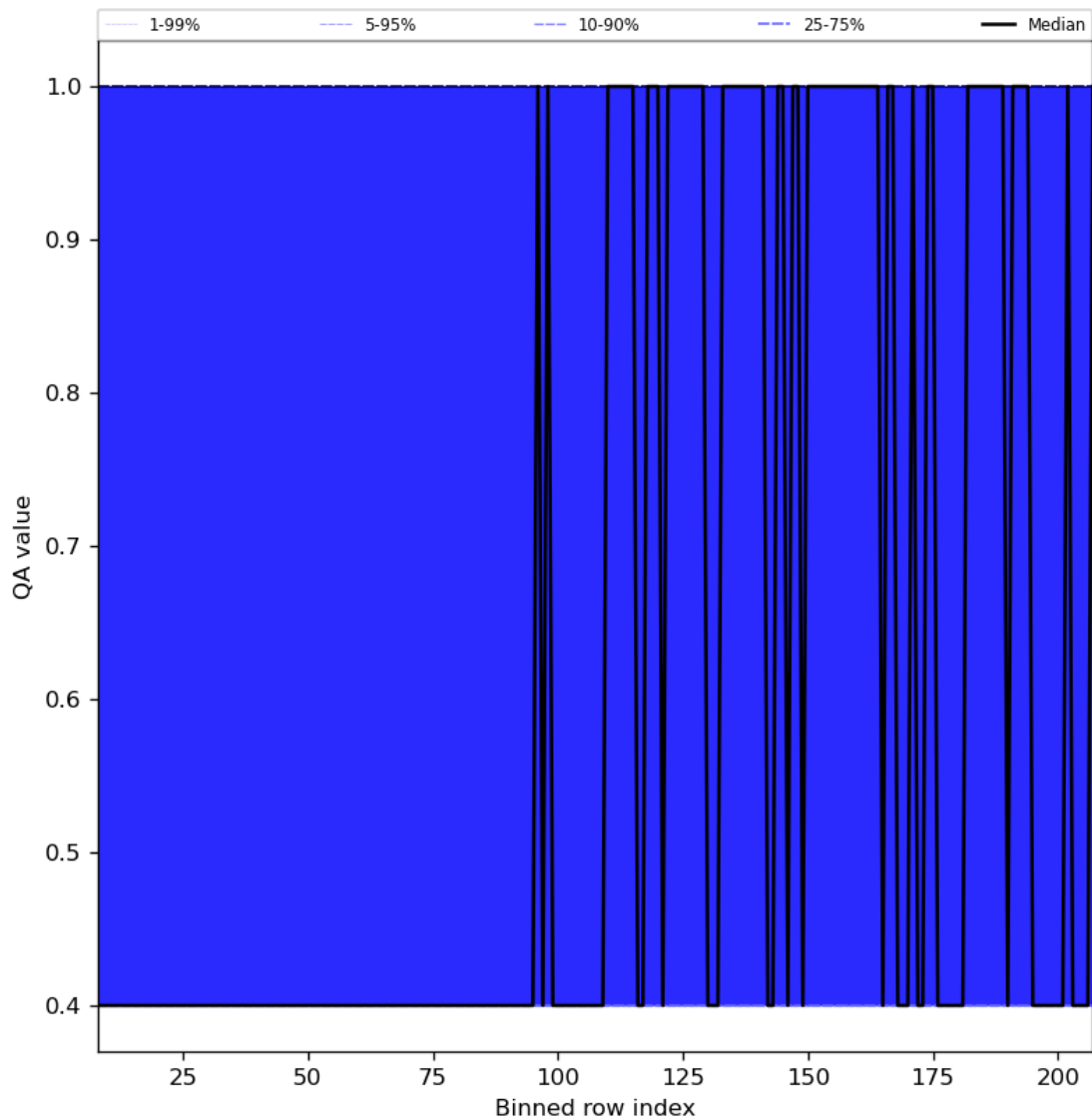
Figure 33: Along track statistics of “QA value” for 2024-03-11 to 2024-03-13
