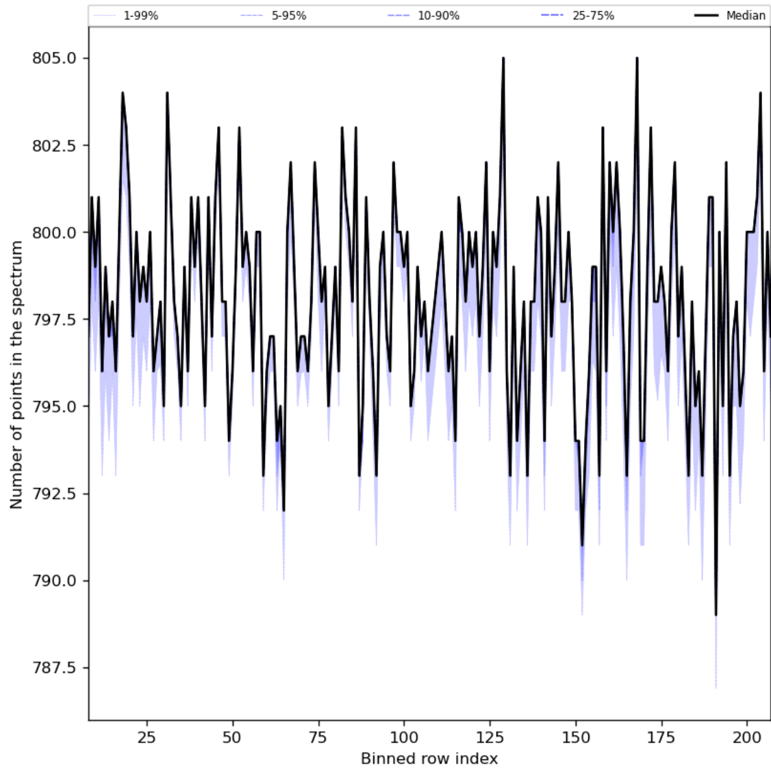
Figure 37: Along track statistics of “Number of points in the spectrum” for 2024-03-11 to 2024-03-13
