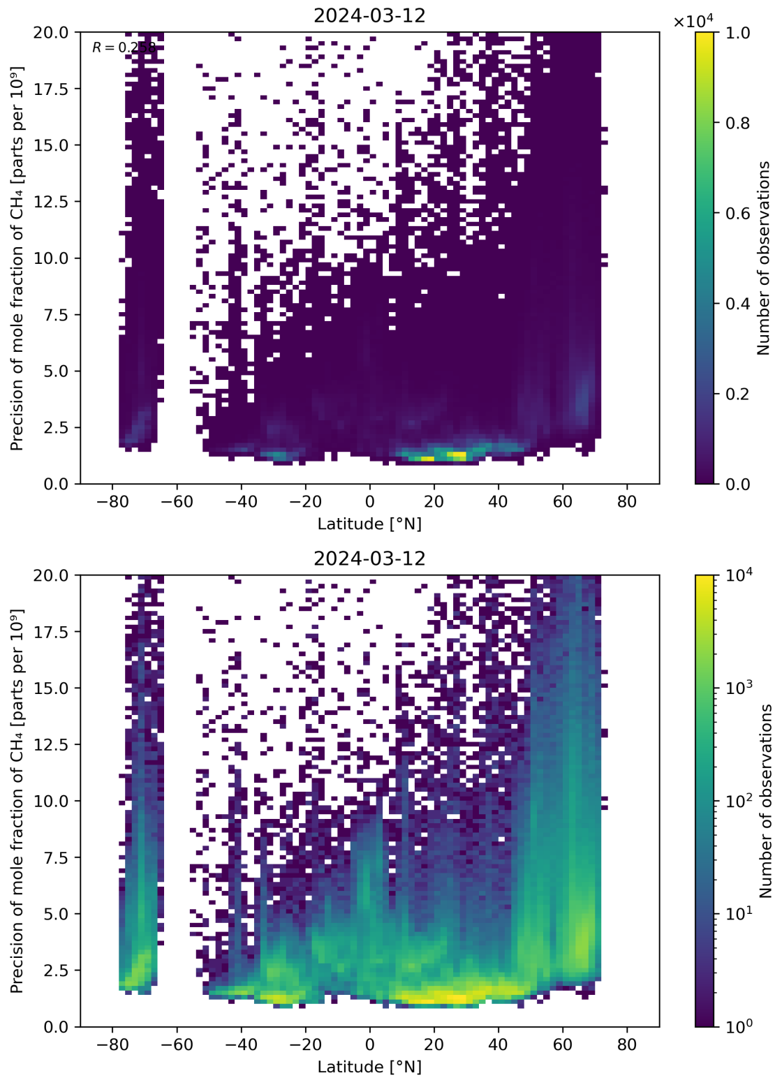
Figure 59: Scatter density plot of “Latitude” against “Precision of mole fraction of CH 4 ” for 2024-03-11 to 2024-03-13.
