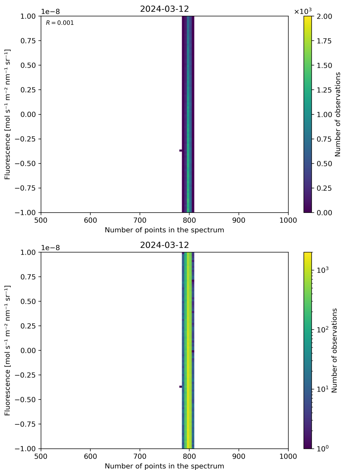
Figure 91: Scatter density plot of “Number of points in the spectrum” against “Fluorescence” for 2024-03-11 to 2024-03-13.
