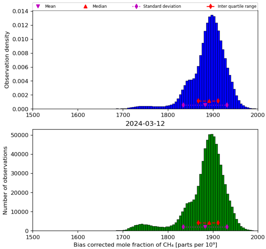
Figure 25: Histogram of “Bias corrected mole fraction of CH 4 ” for 2024-03-11 to 2024-03-13
