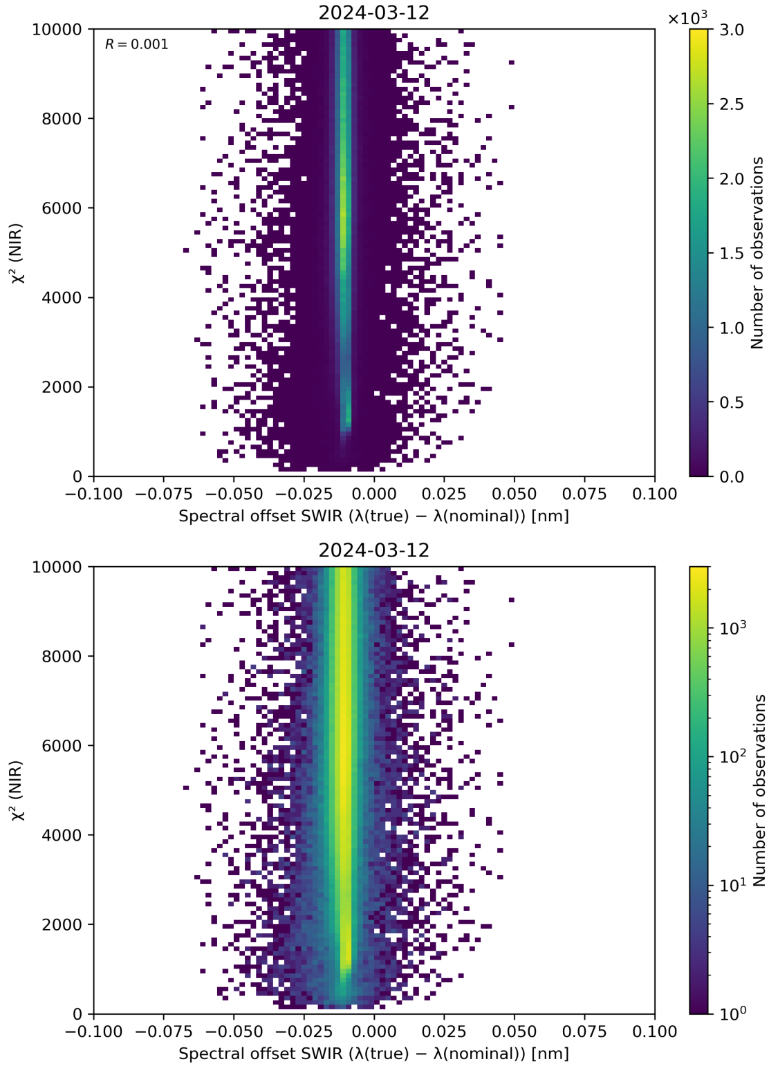
Figure 117: Scatter density plot of “Spectral offset SWIR ( \lambda(\text{true}) - \lambda(\text{nominal}) )” against “ \chi^2 (NIR)” for 2024-03-11 to 2024-03-13.
