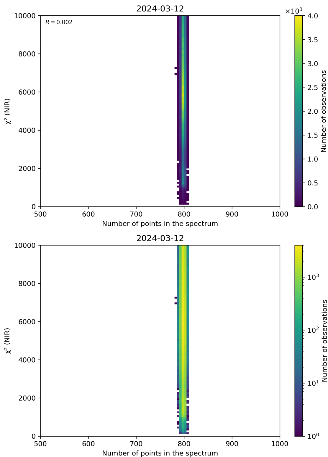
Figure 88: Scatter density plot of “Number of points in the spectrum” against “ \chi^2 (NIR)” for 2024-03-11 to 2024-03-13.
