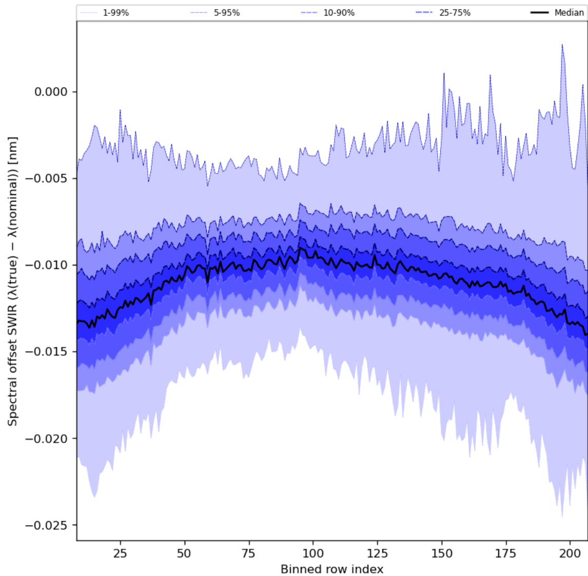
Figure 38: Along track statistics of “Spectral offset SWIR ( \lambda(\text{true}) - \lambda(\text{nominal}) )” for 2024-03-11 to 2024-03-13
