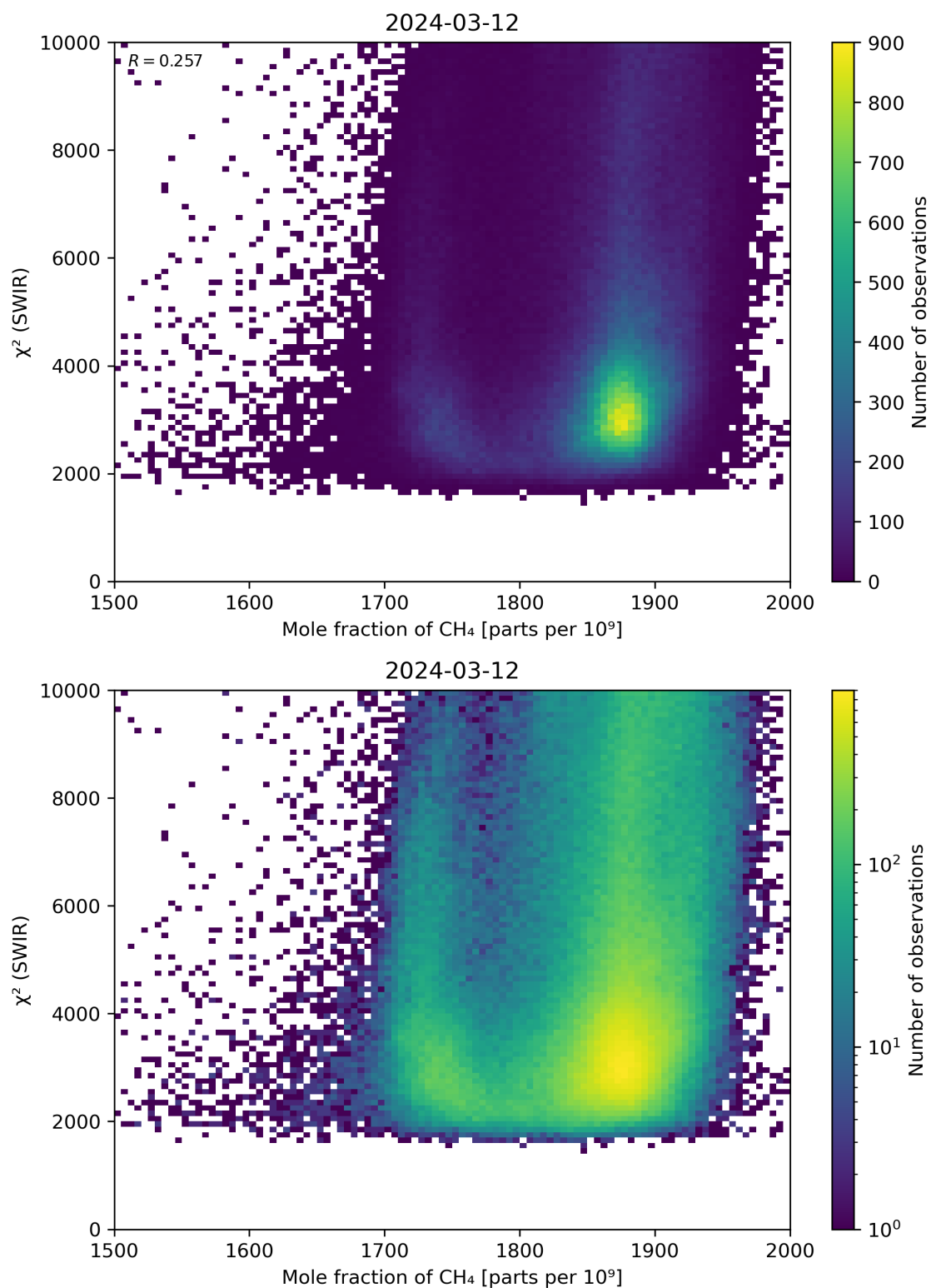
Figure 71: Scatter density plot of “Mole fraction of \text{CH}_4 ” against “ \chi^2 (SWIR)” for 2024-03-11 to 2024-03-13.
