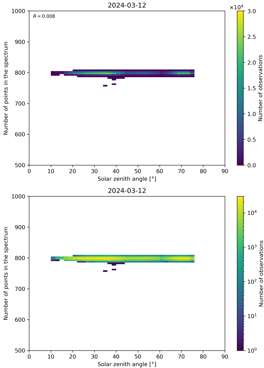
Figure 103: Scatter density plot of “Solar zenith angle” against “Number of points in the spectrum” for 2024-03-11 to 2024-03-13.
