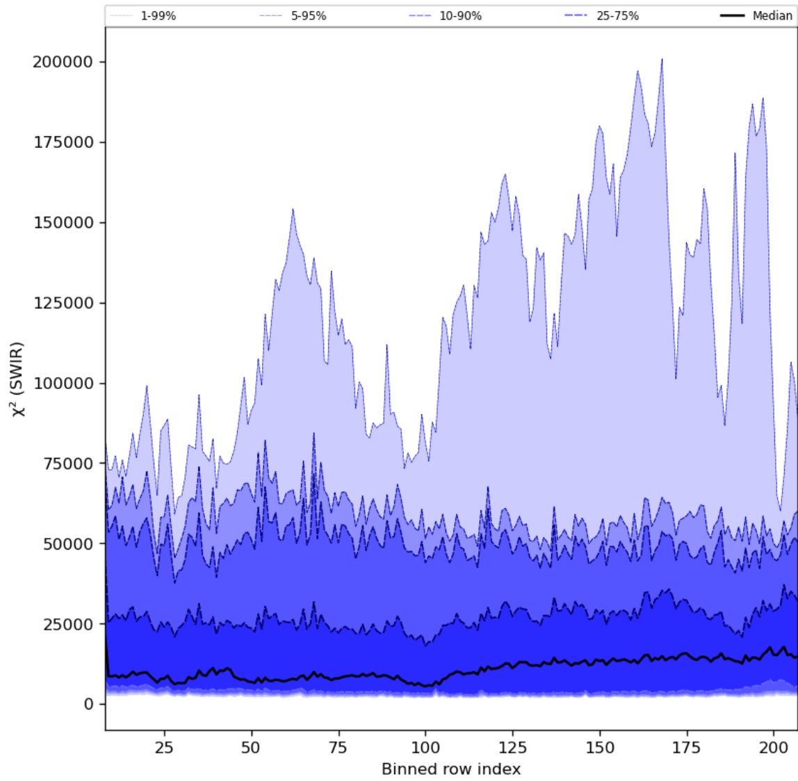
Figure 39: Along track statistics of “ \chi^2 (SWIR)” for 2024-03-11 to 2024-03-13
