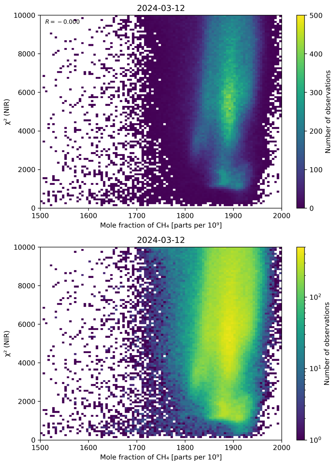
Figure 70: Scatter density plot of “Mole fraction of CH 4 ” against “ \chi^2 (NIR)” for 2024-03-11 to 2024-03-13.
