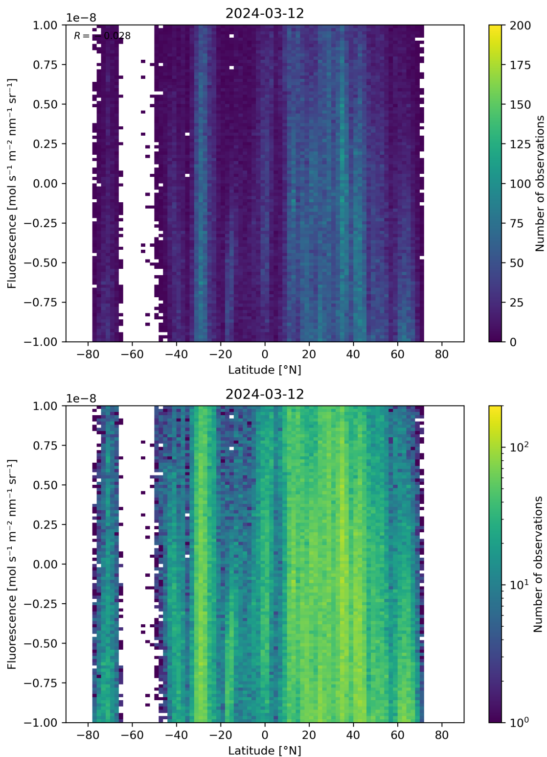
Figure 56: Scatter density plot of “Latitude” against “Fluorescence” for 2024-03-11 to 2024-03-13.
