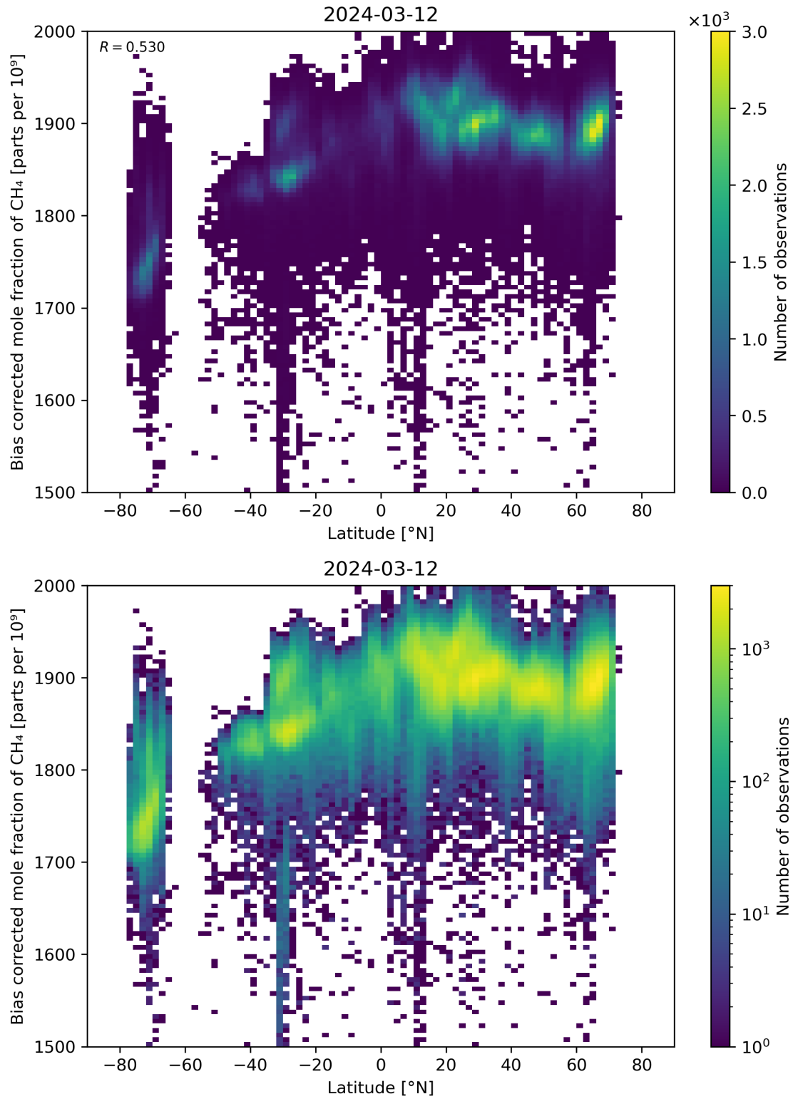
Figure 58: Scatter density plot of “Latitude” against “Bias corrected mole fraction of \text{CH}_4 ” for 2024-03-11 to 2024-03-13.
