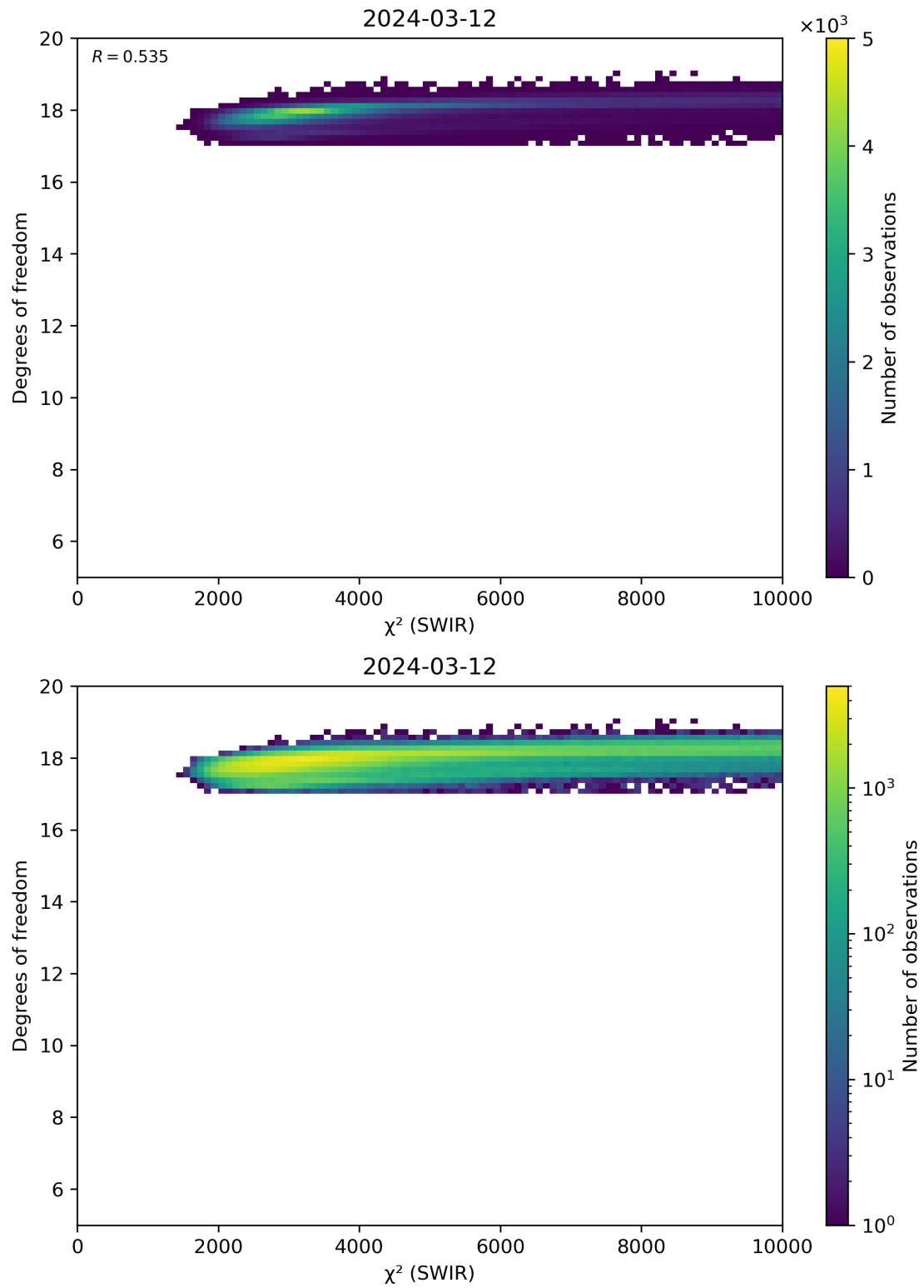
Figure 48: Scatter density plot of “ \chi^2 (SWIR)” against “Degrees of freedom” for 2024-03-11 to 2024-03-13.
