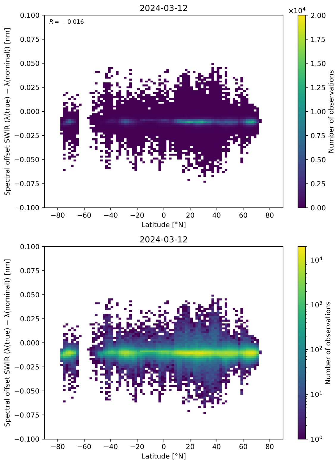
Figure 62: Scatter density plot of “Latitude” against “Spectral offset SWIR ( \lambda(\text{true}) - \lambda(\text{nominal}) )” for 2024-03-11 to 2024-03-13.
