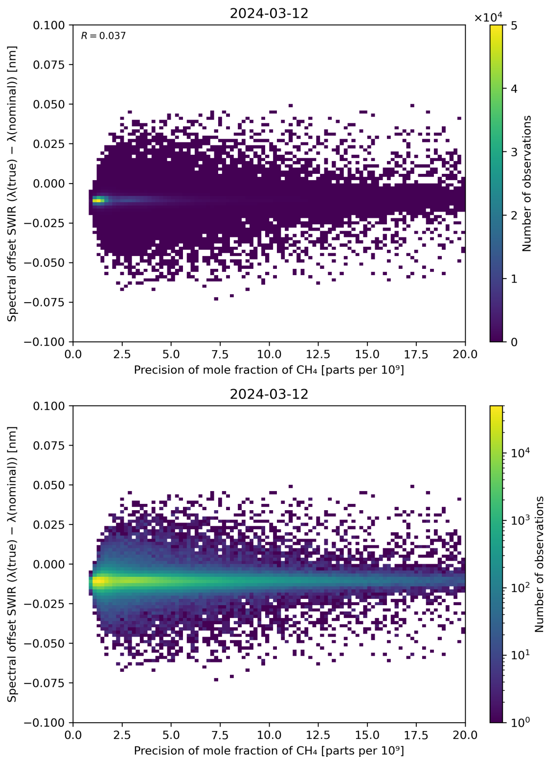
Figure 85: Scatter density plot of “Precision of mole fraction of \text{CH}_4 ” against “Spectral offset SWIR ( \lambda(\text{true}) - \lambda(\text{nominal}) )” for 2024-03-11 to 2024-03-13.
