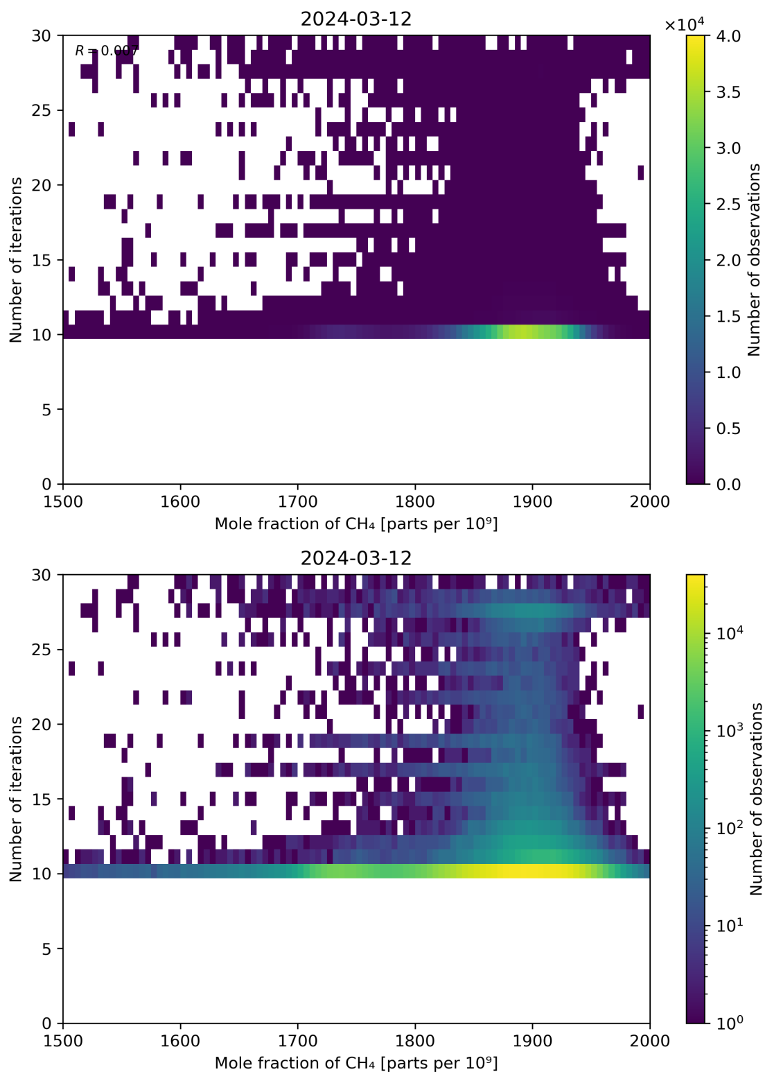
Figure 76: Scatter density plot of “Mole fraction of CH 4 ” against “Number of iterations” for 2024-03-11 to 2024-03-13.
