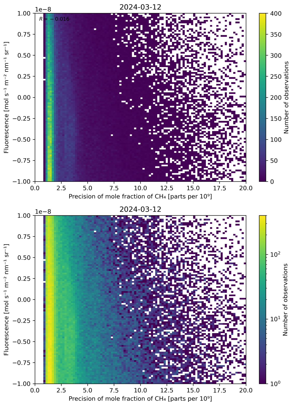
Figure 81: Scatter density plot of “Precision of mole fraction of CH 4 ” against “Fluorescence” for 2024-03-11 to 2024-03-13.
