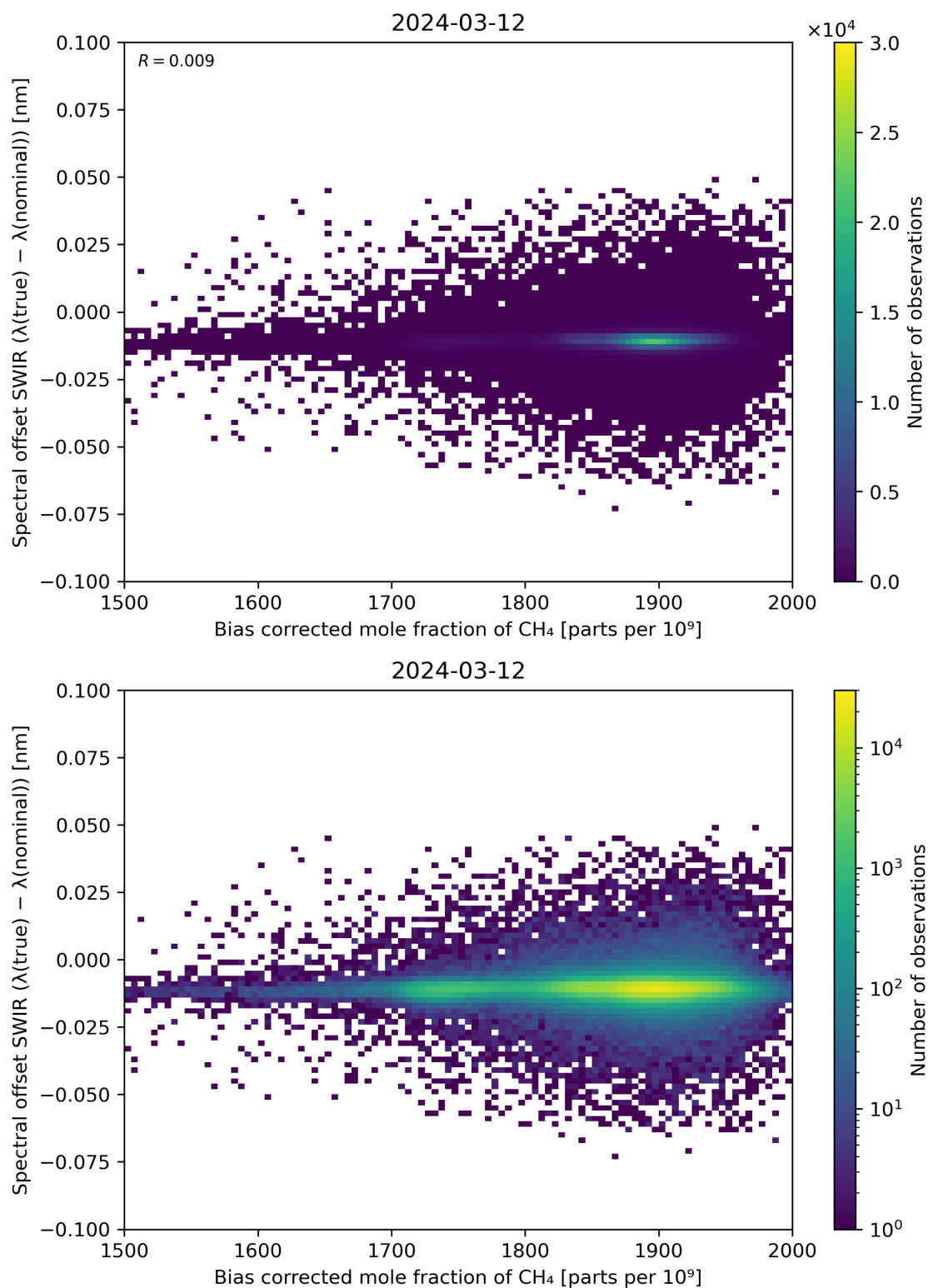
Figure 69: Scatter density plot of “Bias corrected mole fraction of \text{CH}_4 ” against “Spectral offset SWIR ( \lambda(\text{true}) - \lambda(\text{nominal}) )” for 2024-03-11 to 2024-03-13.
