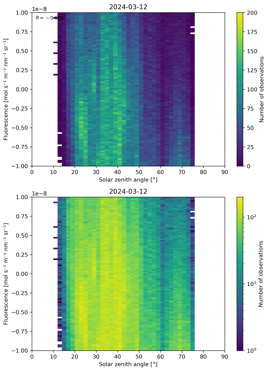
Figure 97: Scatter density plot of “Solar zenith angle” against “Fluorescence” for 2024-03-11 to 2024-03-13.
