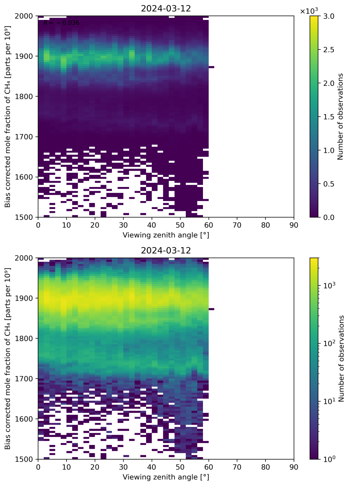
Figure 111: Scatter density plot of “Viewing zenith angle” against “Bias corrected mole fraction of CH 4 ” for 2024-03-11 to 2024-03-13.
