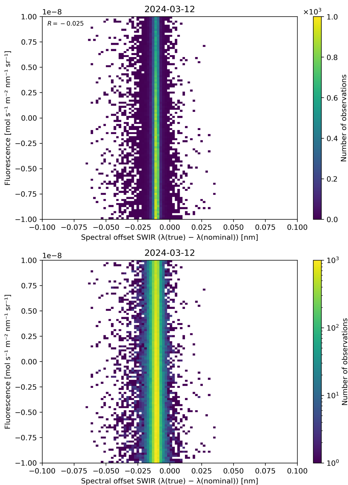
Figure 120: Scatter density plot of “Spectral offset SWIR ( \lambda(\text{true}) - \lambda(\text{nominal}) )” against “Fluorescence” for 2024-03-11 to 2024-03-13.
