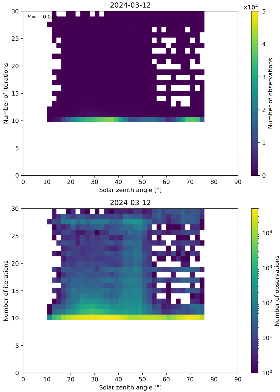
Figure 102: Scatter density plot of “Solar zenith angle” against “Number of iterations” for 2024-03-11 to 2024-03-13.
