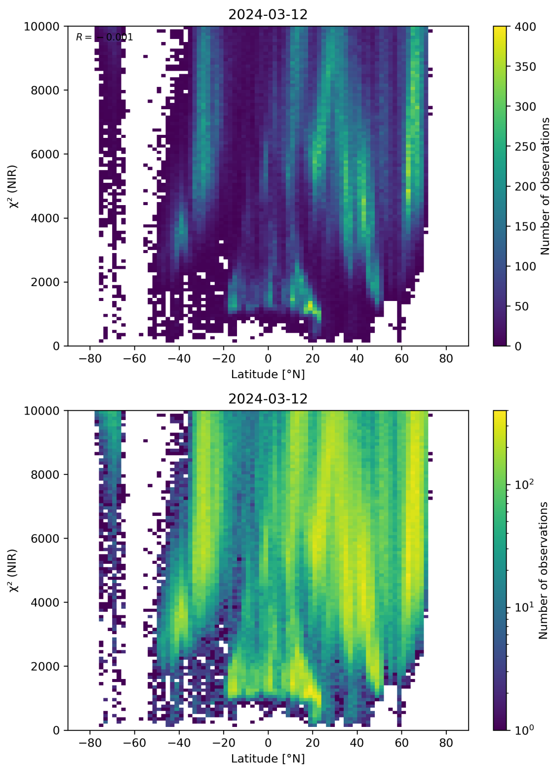
Figure 53: Scatter density plot of “Latitude” against “ \chi^2 (NIR)” for 2024-03-11 to 2024-03-13.
