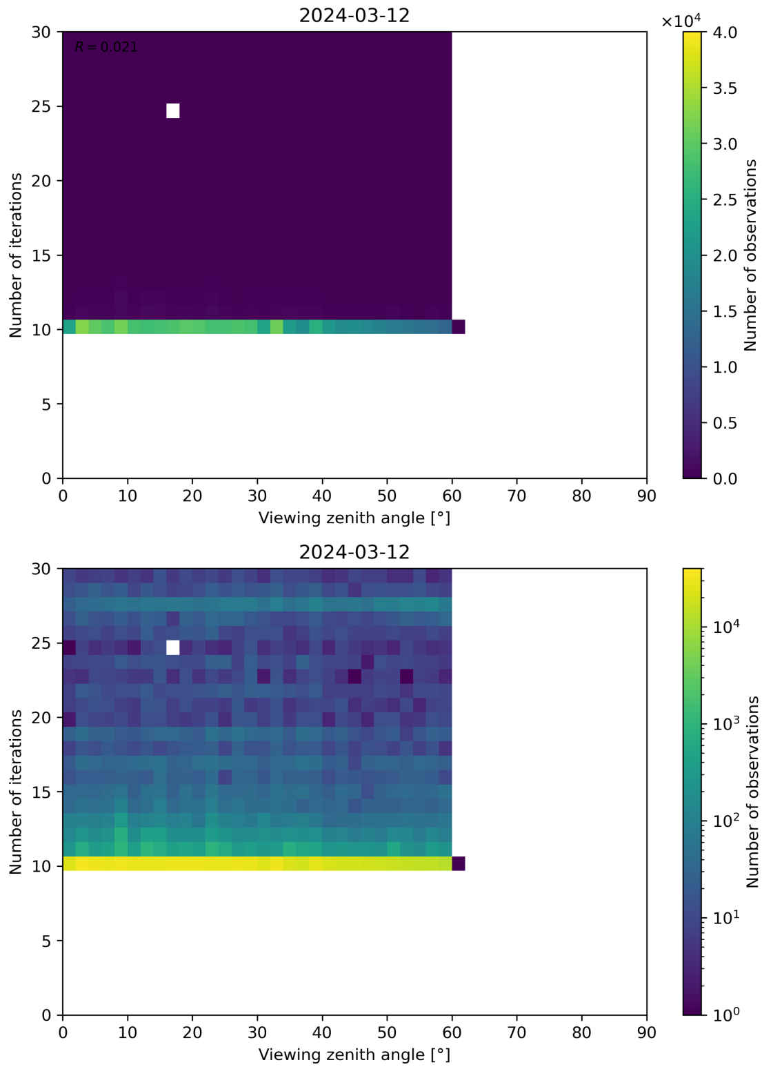
Figure 113: Scatter density plot of “Viewing zenith angle” against “Number of iterations” for 2024-03-11 to 2024-03-13.
