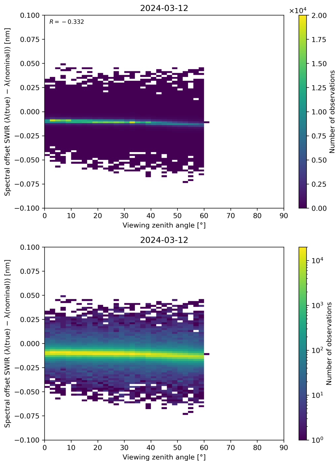
Figure 116: Scatter density plot of “Viewing zenith angle” against “Spectral offset SWIR ( \lambda(\text{true}) - \lambda(\text{nominal}) )” for 2024-03-11 to 2024-03-13.
