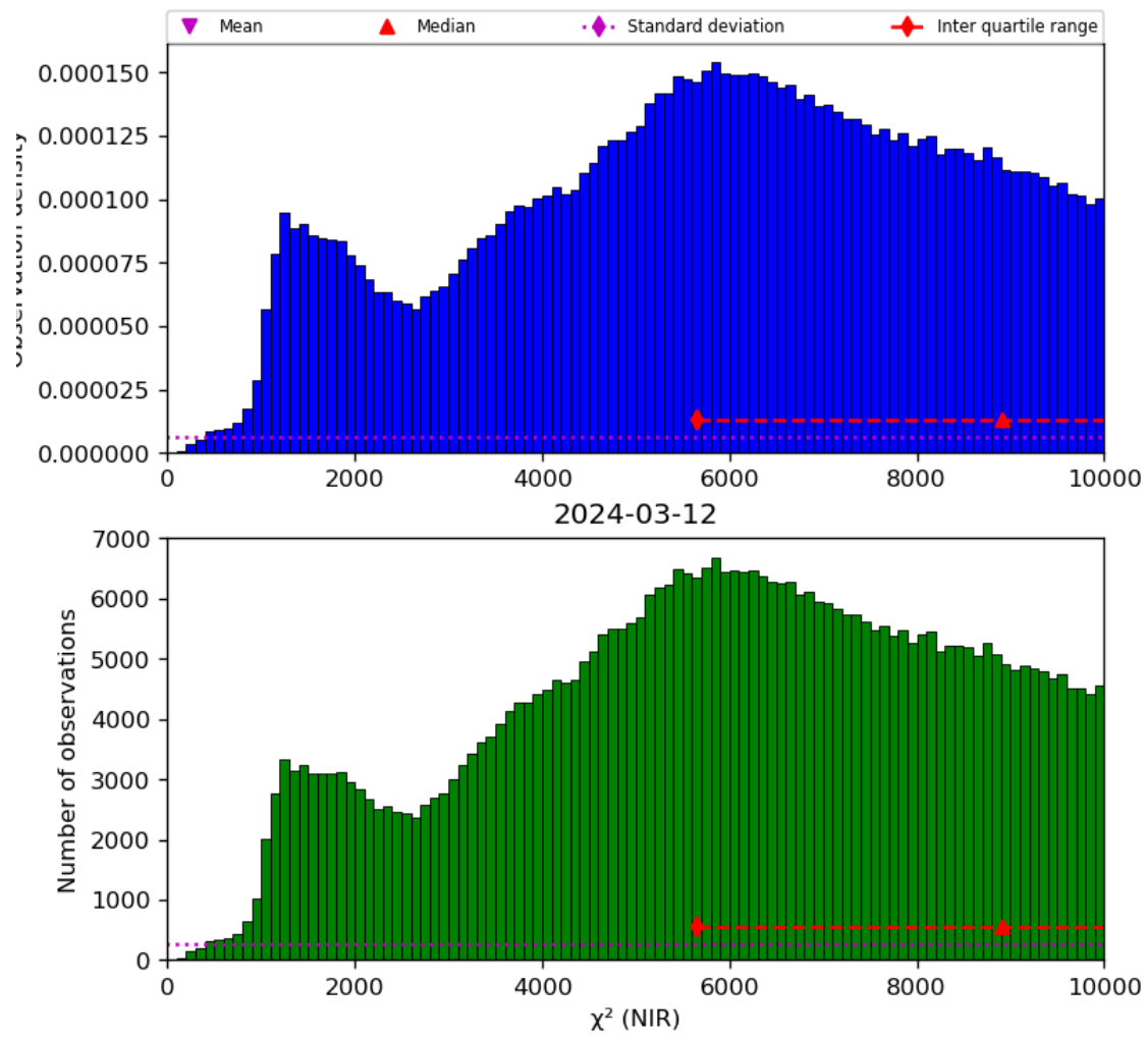
Figure 29: Histogram of “ \chi^2 (NIR)” for 2024-03-11 to 2024-03-13
