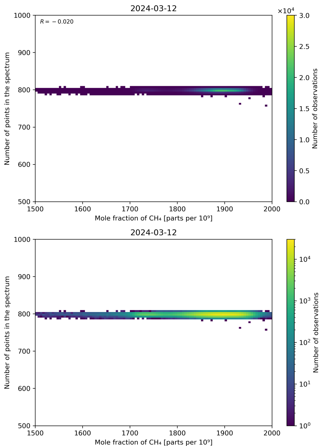
Figure 77: Scatter density plot of “Mole fraction of CH 4 ” against “Number of points in the spectrum” for 2024-03-11 to 2024-03-13.
