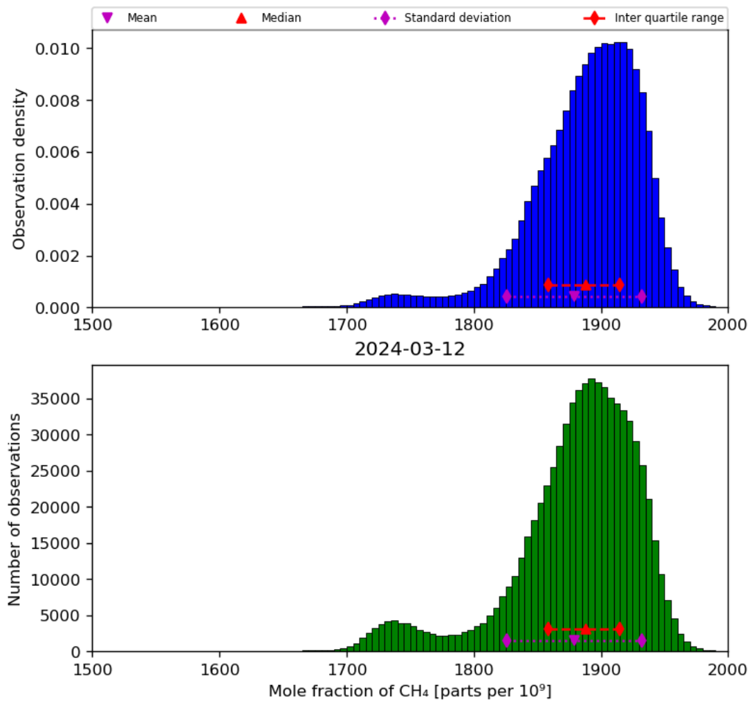
Figure 23: Histogram of “Mole fraction of CH 4 ” for 2024-03-11 to 2024-03-13
