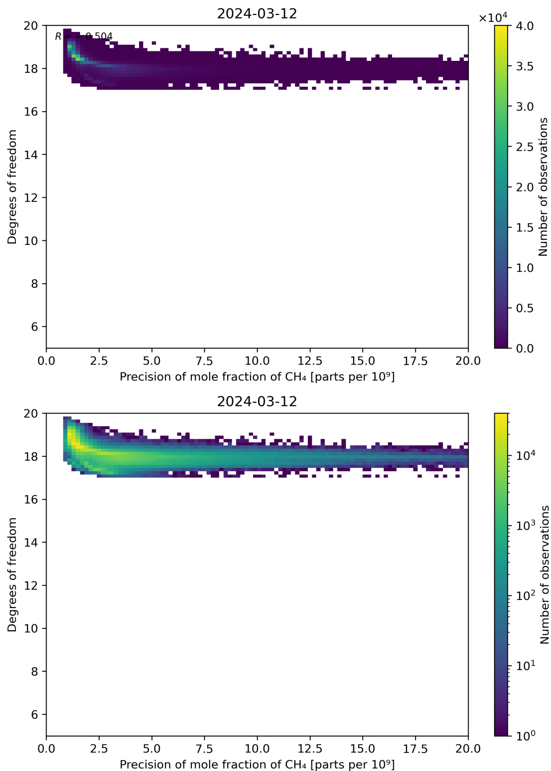
Figure 80: Scatter density plot of “Precision of mole fraction of CH 4 ” against “Degrees of freedom” for 2024-03-11 to 2024-03-13.
