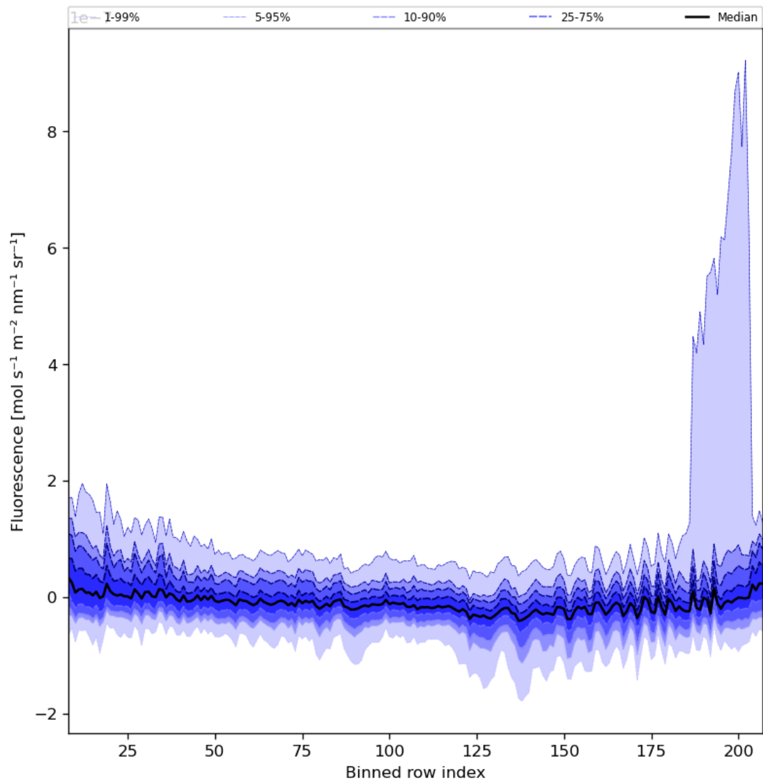
Figure 43: Along track statistics of “Fluorescence” for 2024-03-11 to 2024-03-13
