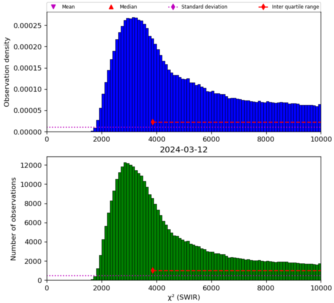
Figure 28: Histogram of “ \chi^2 (SWIR)” for 2024-03-11 to 2024-03-13
