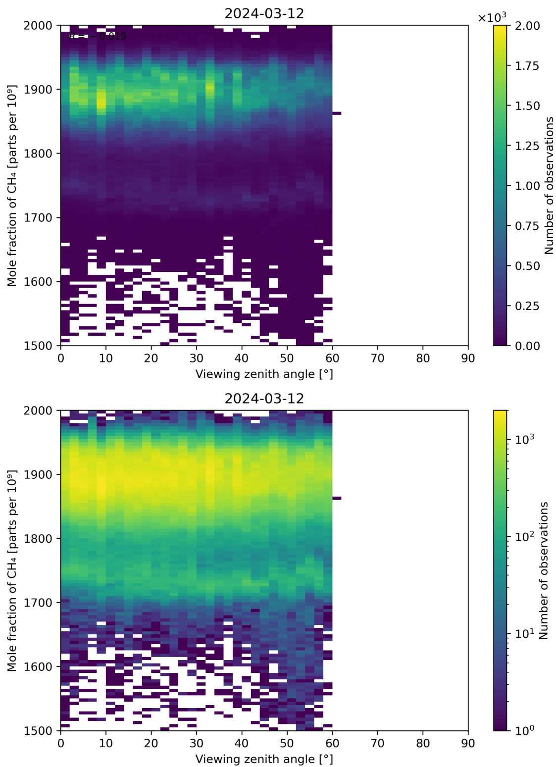
Figure 110: Scatter density plot of “Viewing zenith angle” against “Mole fraction of CH 4 ” for 2024-03-11 to 2024-03-13.
