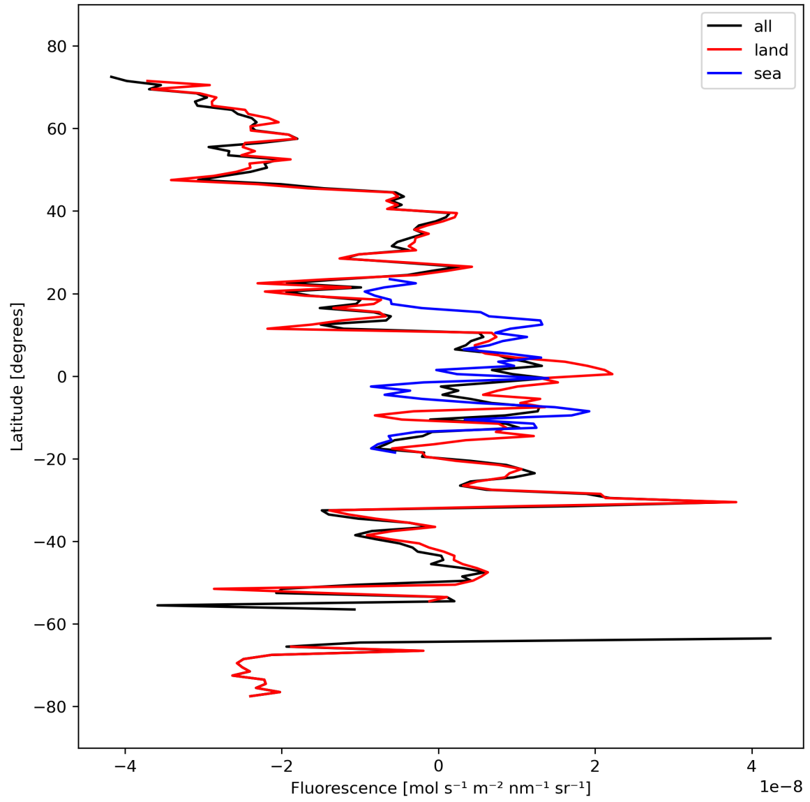
Figure 21: Zonal average of “Fluorescence” for 2024-03-11 to 2024-03-13.
