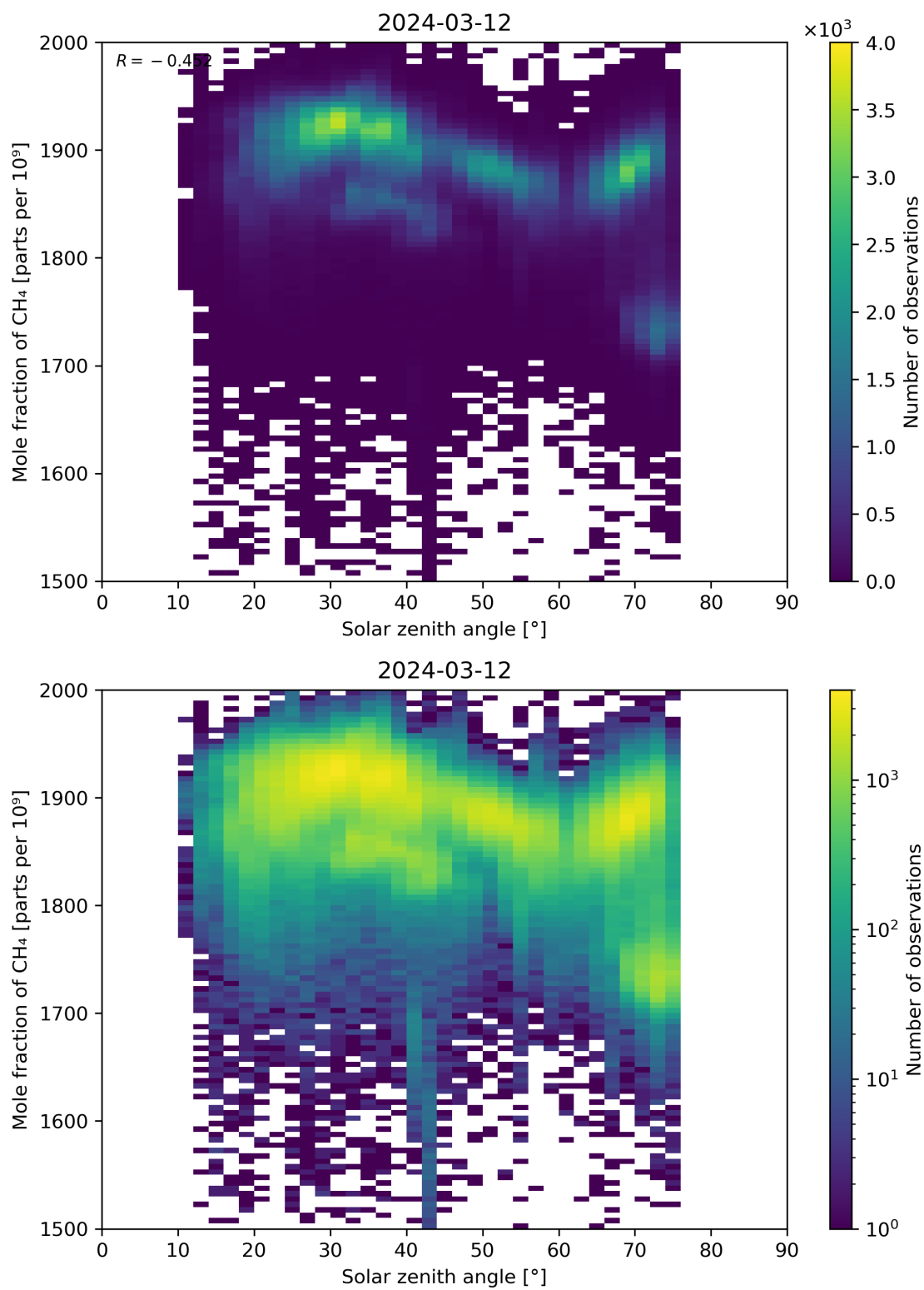
Figure 99: Scatter density plot of “Solar zenith angle” against “Mole fraction of CH 4 ” for 2024-03-11 to 2024-03-13.
