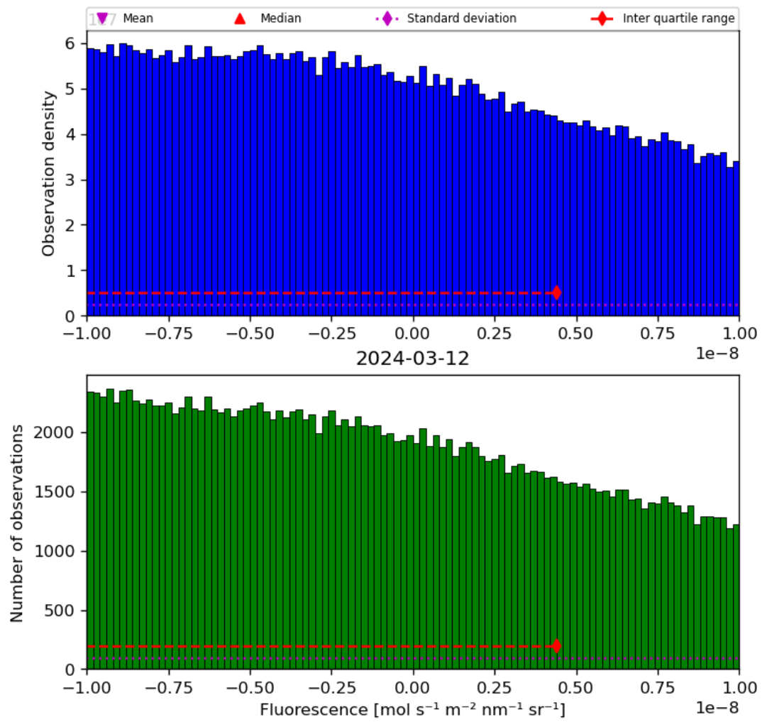
Figure 32: Histogram of “Fluorescence” for 2024-03-11 to 2024-03-13
