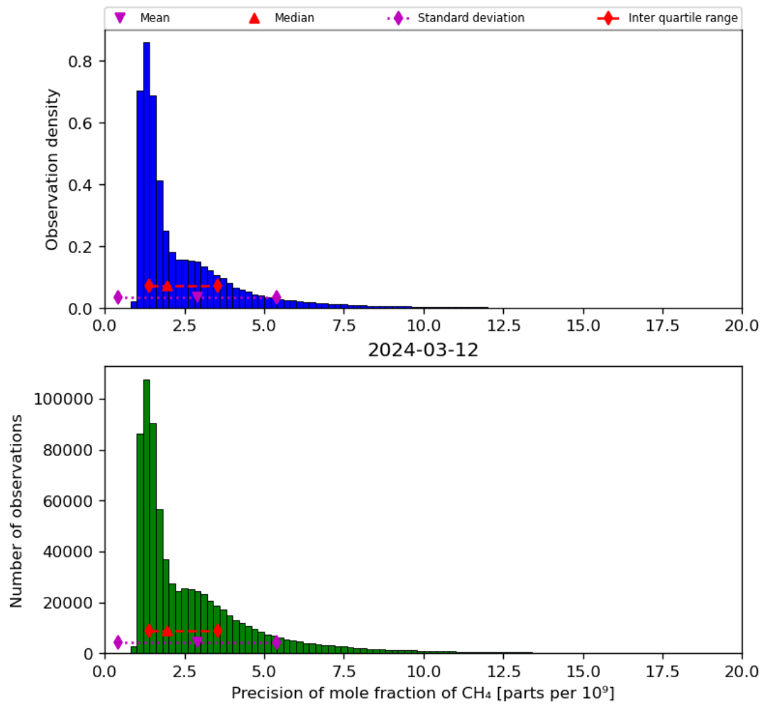
Figure 24: Histogram of “Precision of mole fraction of CH 4 ” for 2024-03-11 to 2024-03-13
