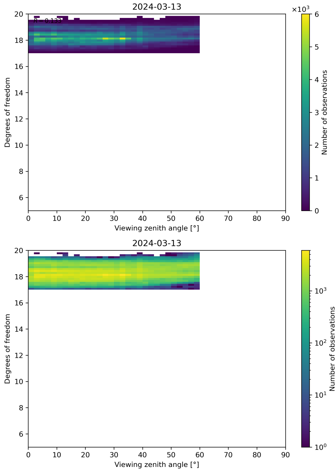
Figure 107: Scatter density plot of “Viewing zenith angle” against “Degrees of freedom” for 2024-03-12 to 2024-03-14.
