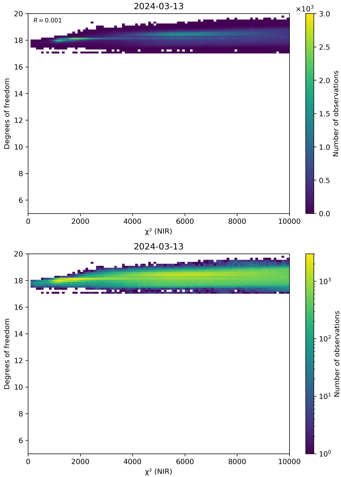
Figure 44: Scatter density plot of “ \chi^2 (NIR)” against “Degrees of freedom” for 2024-03-12 to 2024-03-14.
