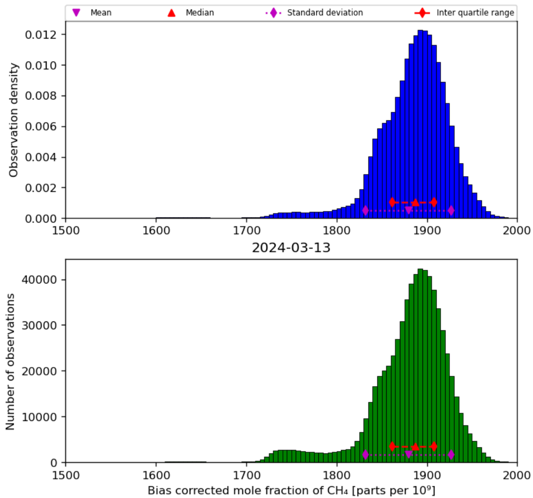
Figure 25: Histogram of “Bias corrected mole fraction of CH 4 ” for 2024-03-12 to 2024-03-14
