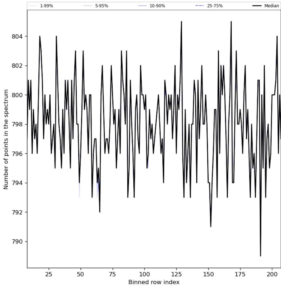
Figure 37: Along track statistics of “Number of points in the spectrum” for 2024-03-12 to 2024-03-14
