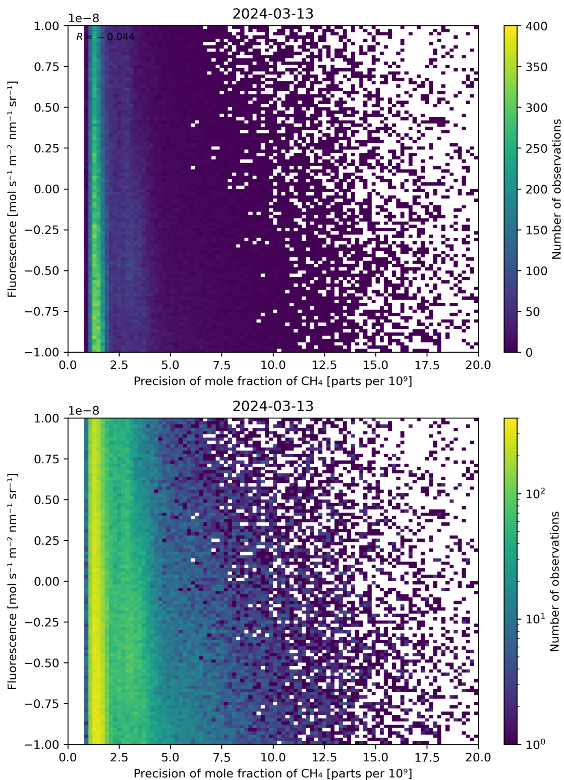
Figure 81: Scatter density plot of “Precision of mole fraction of \text{CH}_4 ” against “Fluorescence” for 2024-03-12 to 2024-03-14.
