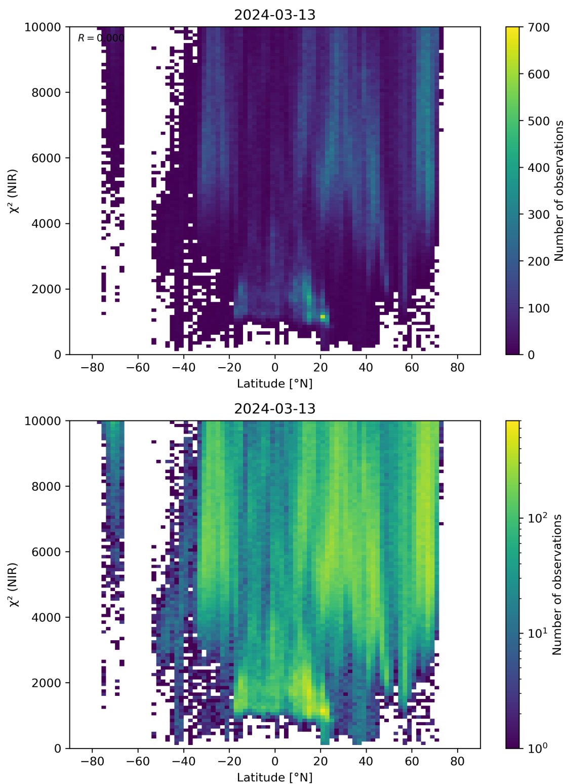
Figure 53: Scatter density plot of “Latitude” against “ \chi^2 (NIR)” for 2024-03-12 to 2024-03-14.
