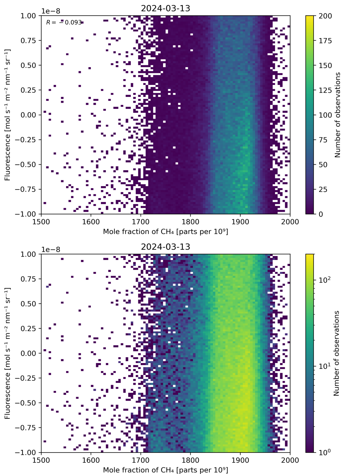
Figure 73: Scatter density plot of “Mole fraction of \text{CH}_4 ” against “Fluorescence” for 2024-03-12 to 2024-03-14.
