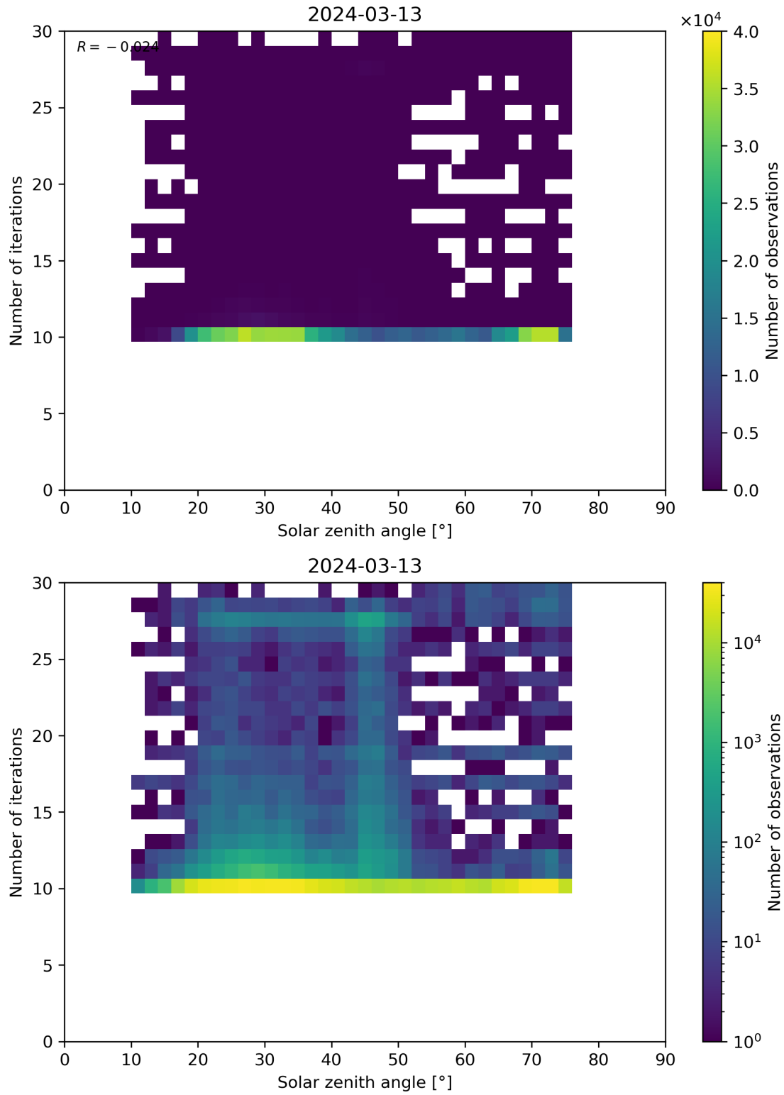
Figure 102: Scatter density plot of “Solar zenith angle” against “Number of iterations” for 2024-03-12 to 2024-03-14.
