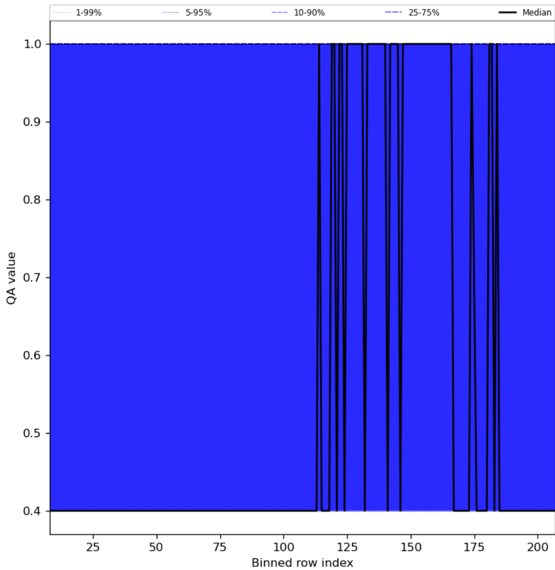
Figure 33: Along track statistics of “QA value” for 2024-03-12 to 2024-03-14
