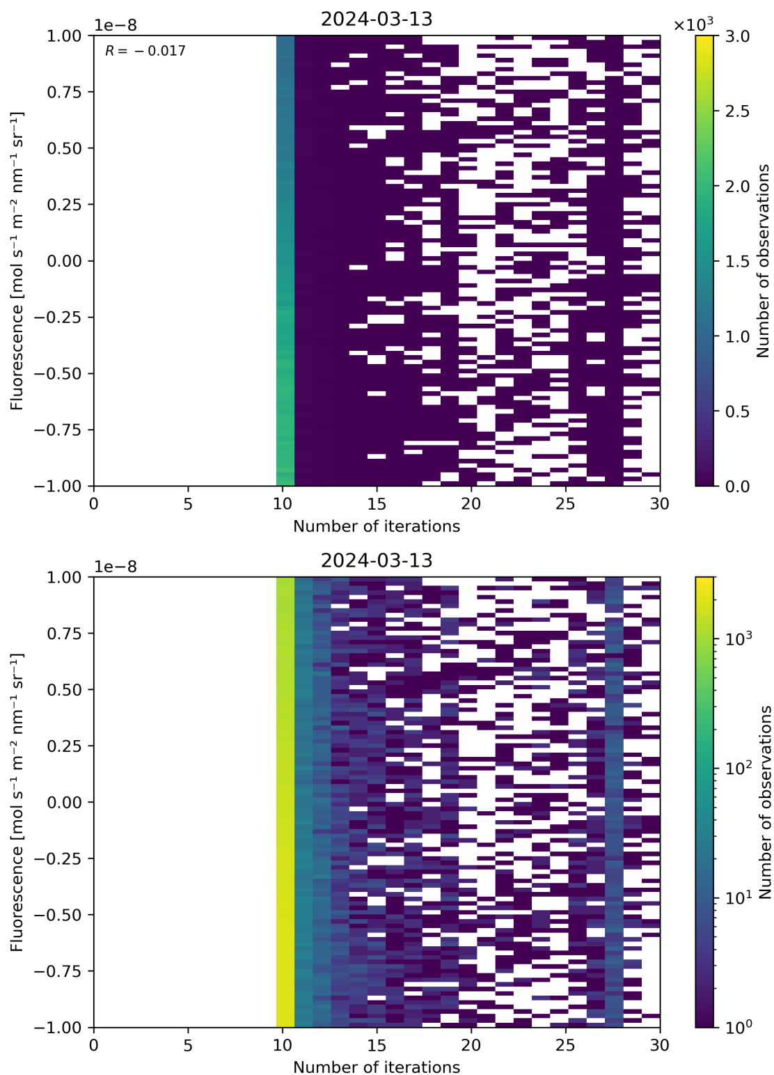
Figure 87: Scatter density plot of “Number of iterations” against “Fluorescence” for 2024-03-12 to 2024-03-14.
