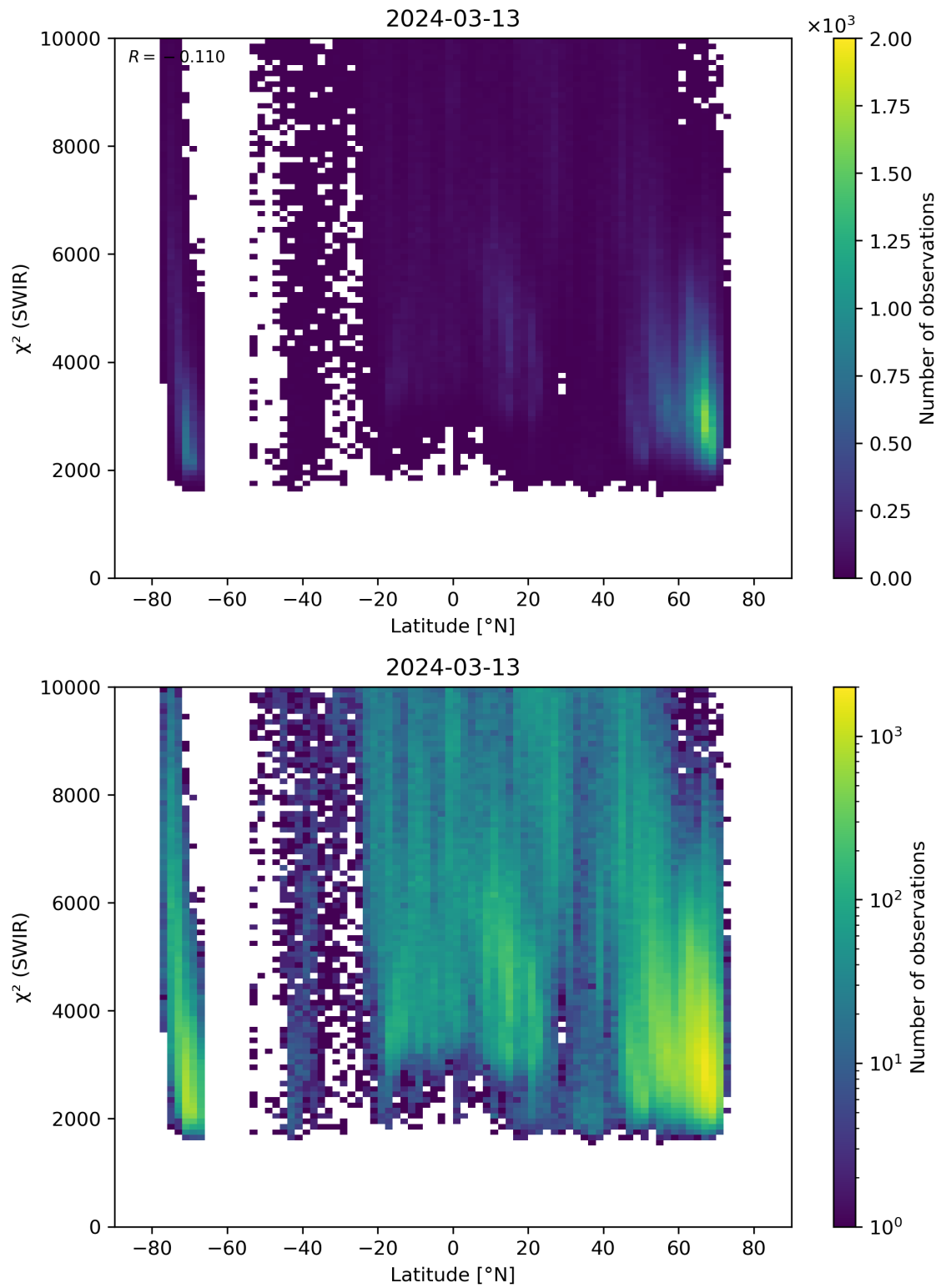
Figure 54: Scatter density plot of “Latitude” against “ \chi^2 (SWIR)” for 2024-03-12 to 2024-03-14.
