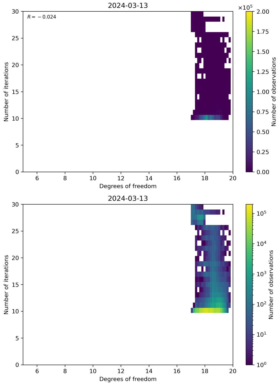
Figure 52: Scatter density plot of “Degrees of freedom” against “Number of iterations” for 2024-03-12 to 2024-03-14.
