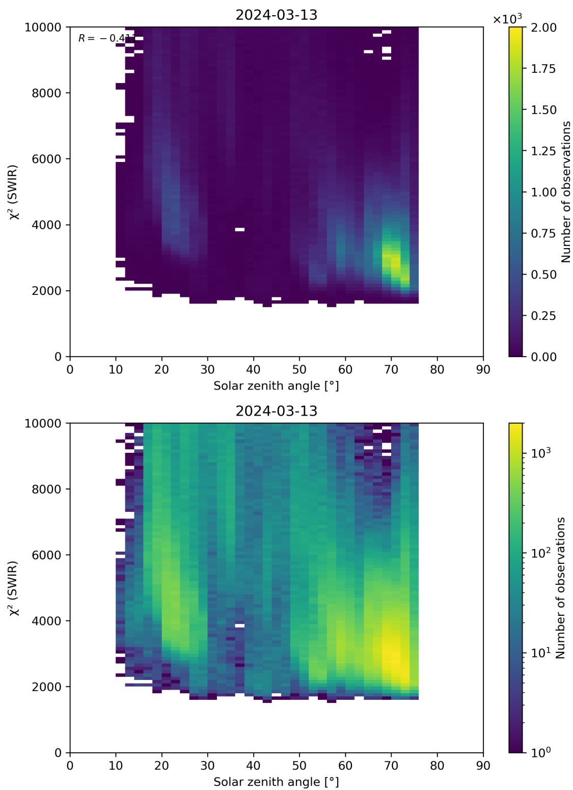
Figure 95: Scatter density plot of “Solar zenith angle” against “ \chi^2 (SWIR)” for 2024-03-12 to 2024-03-14.
