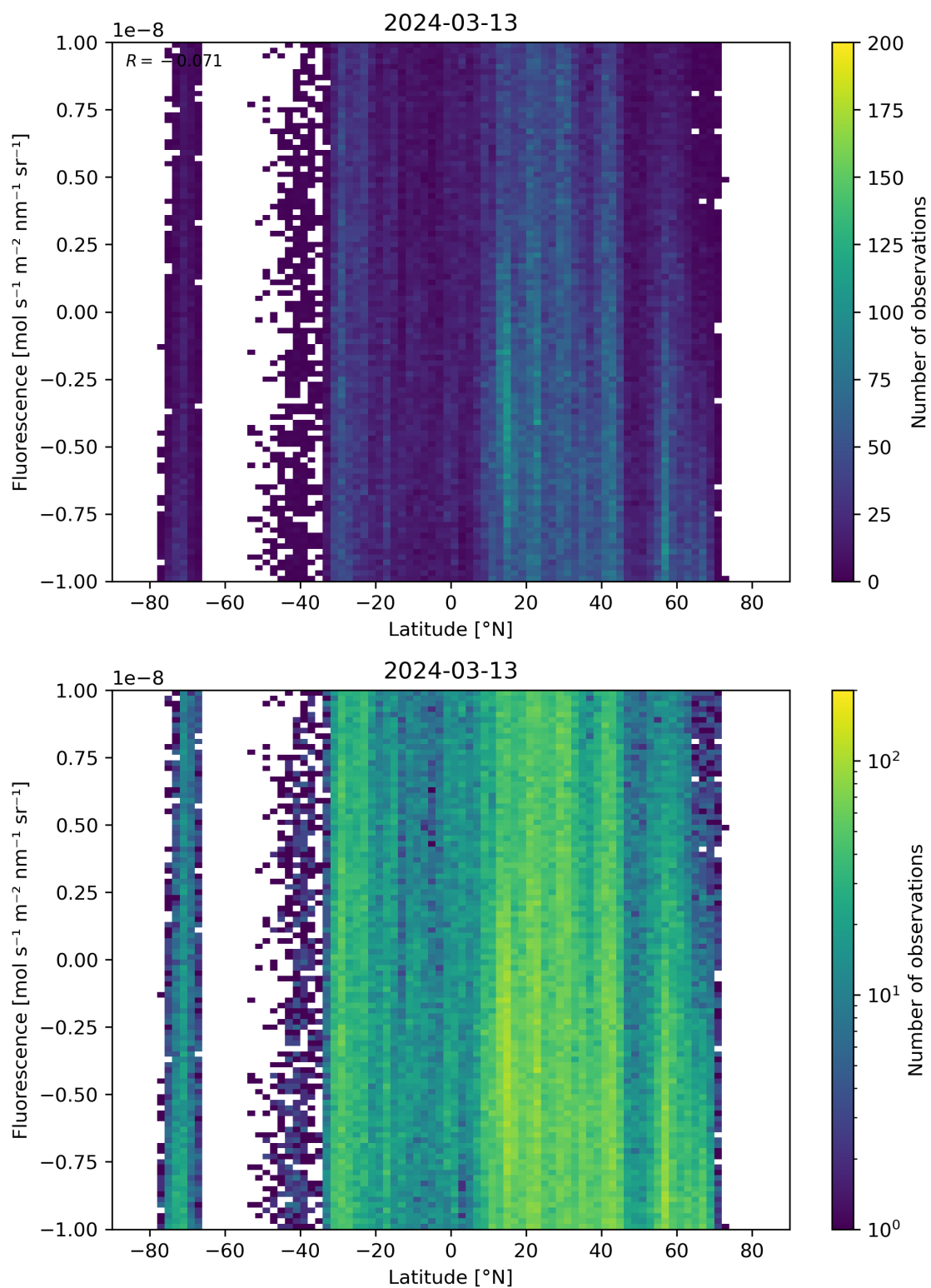
Figure 56: Scatter density plot of “Latitude” against “Fluorescence” for 2024-03-12 to 2024-03-14.
