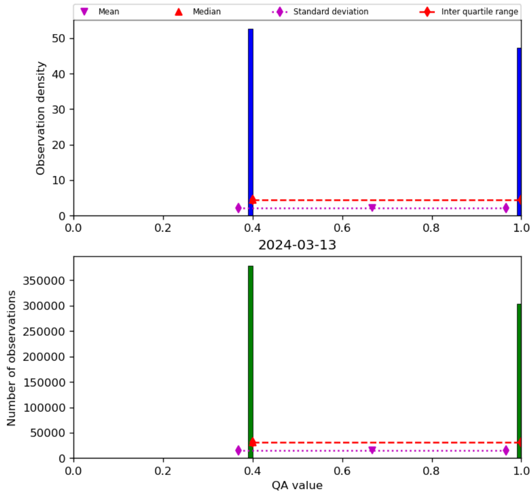
Figure 22: Histogram of “QA value” for 2024-03-12 to 2024-03-14
