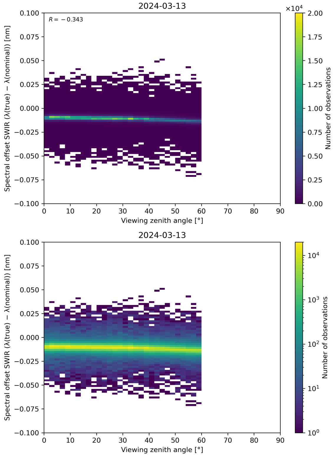
Figure 116: Scatter density plot of “Viewing zenith angle” against “Spectral offset SWIR ( \lambda(\text{true}) - \lambda(\text{nominal}) )” for 2024-03-12 to 2024-03-14.
