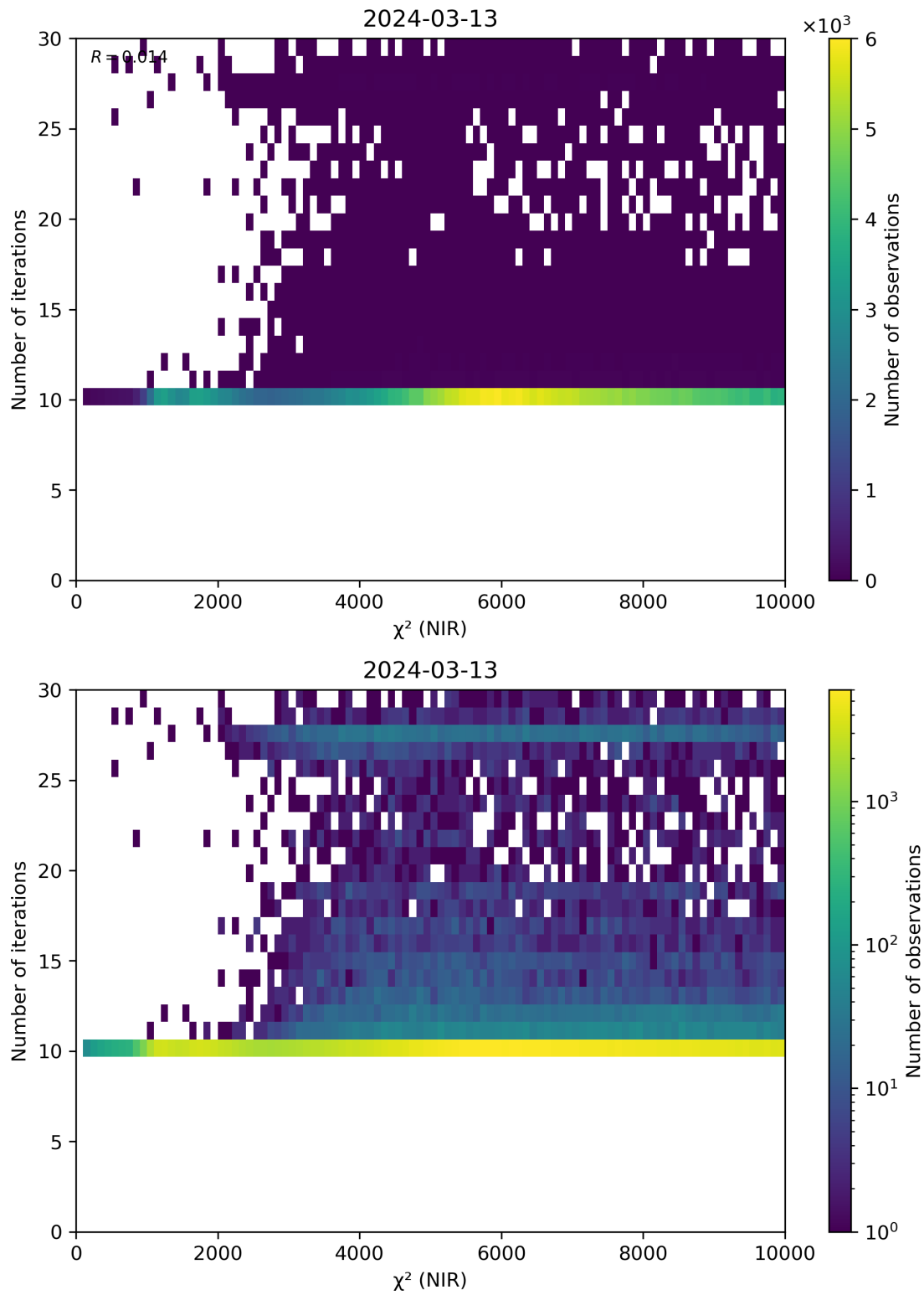
Figure 46: Scatter density plot of “ \chi^2 (NIR)” against “Number of iterations” for 2024-03-12 to 2024-03-14.
