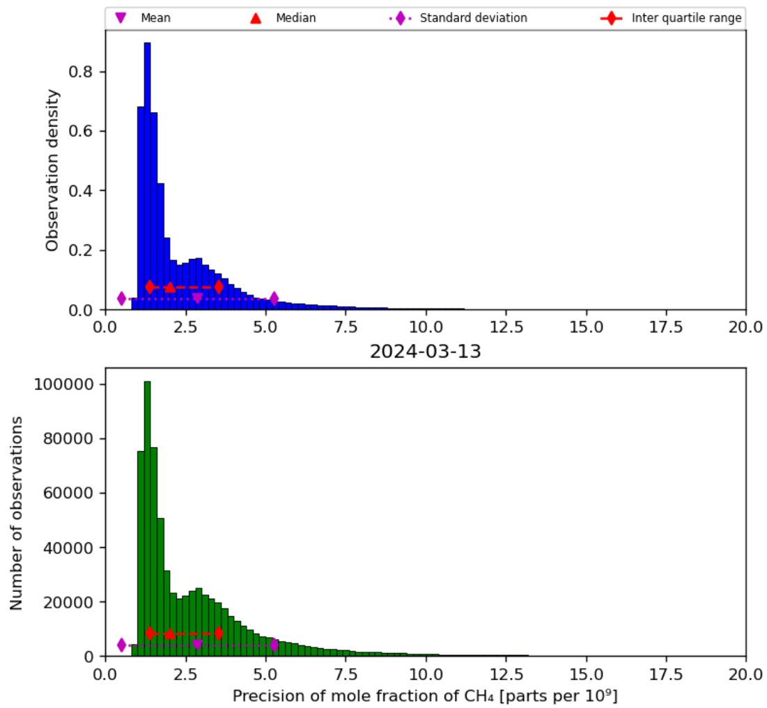
Figure 24: Histogram of “Precision of mole fraction of CH 4 ” for 2024-03-12 to 2024-03-14
