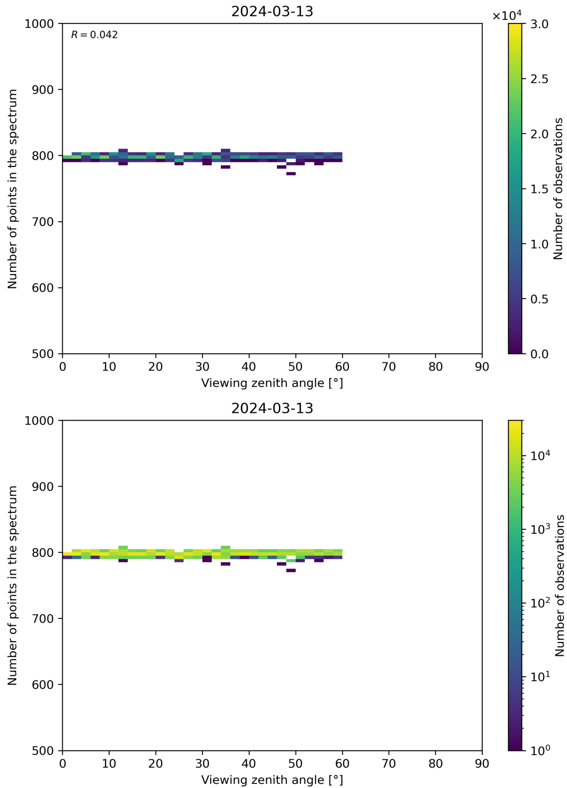
Figure 114: Scatter density plot of “Viewing zenith angle” against “Number of points in the spectrum” for 2024-03-12 to 2024-03-14.
