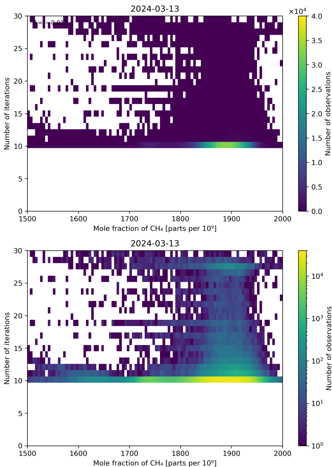
Figure 76: Scatter density plot of “Mole fraction of CH 4 ” against “Number of iterations” for 2024-03-12 to 2024-03-14.
