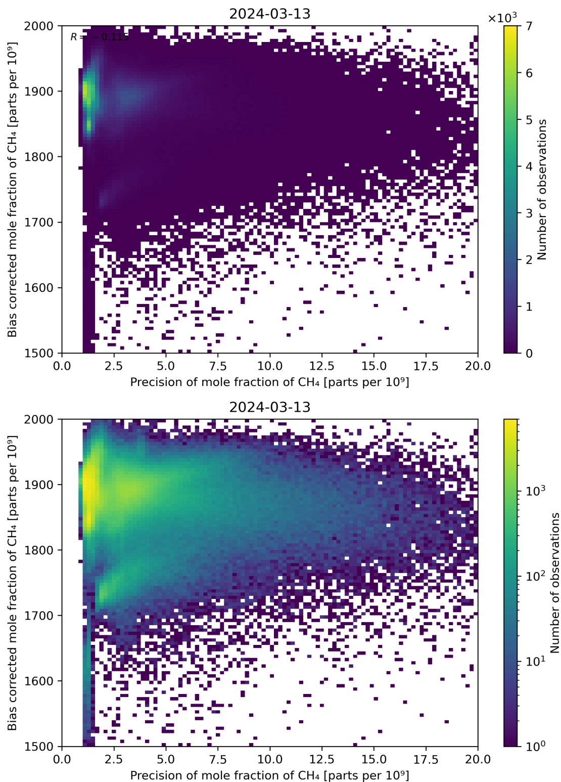
Figure 82: Scatter density plot of “Precision of mole fraction of CH 4 ” against “Bias corrected mole fraction of CH 4 ” for 2024-03-12 to 2024-03-14.
