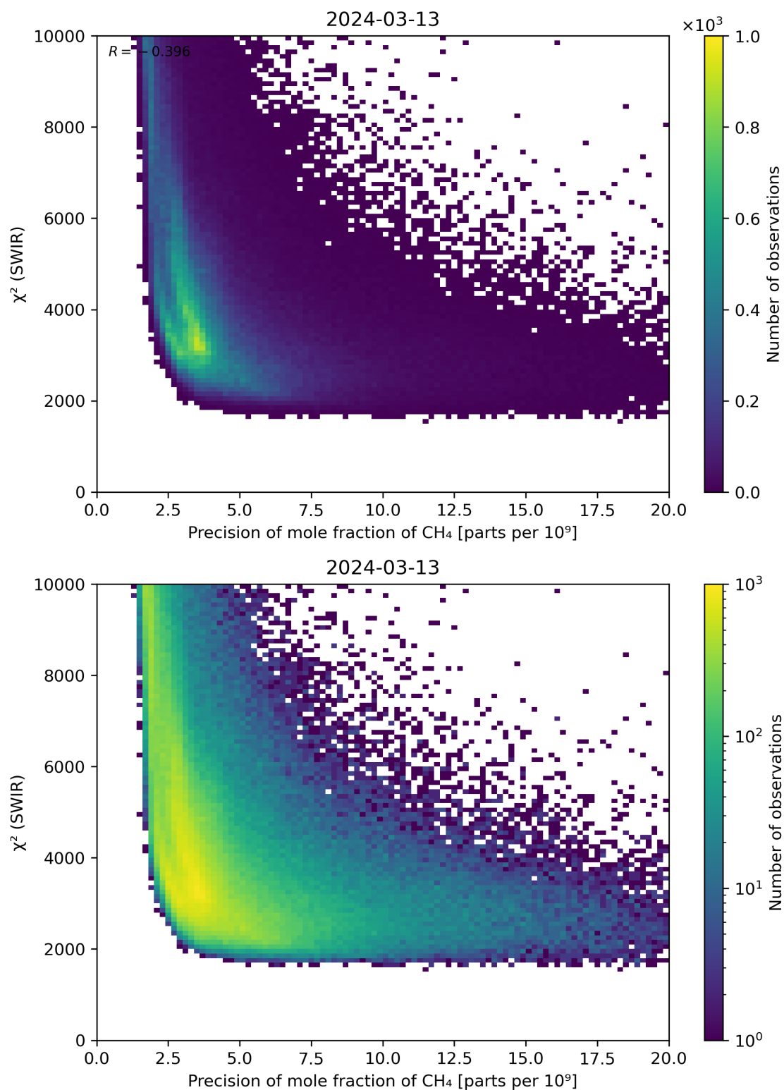
Figure 79: Scatter density plot of “Precision of mole fraction of \text{CH}_4 ” against “ \chi^2 (SWIR)” for 2024-03-12 to 2024-03-14.
