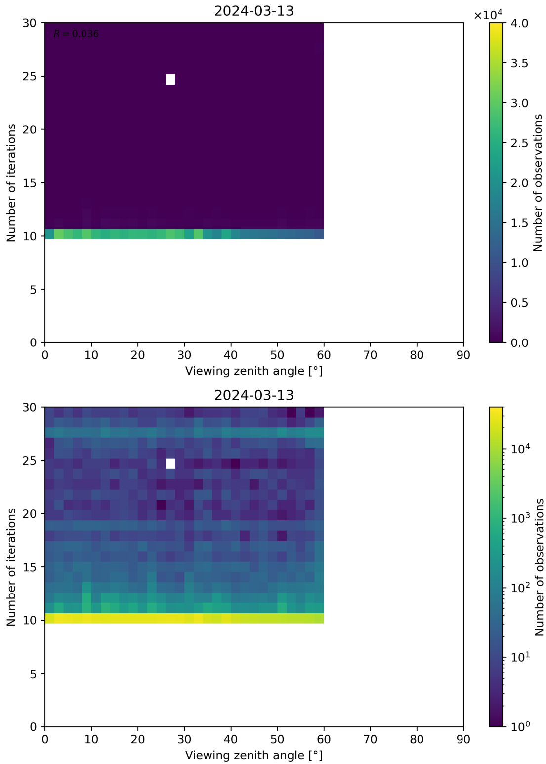
Figure 113: Scatter density plot of “Viewing zenith angle” against “Number of iterations” for 2024-03-12 to 2024-03-14.
