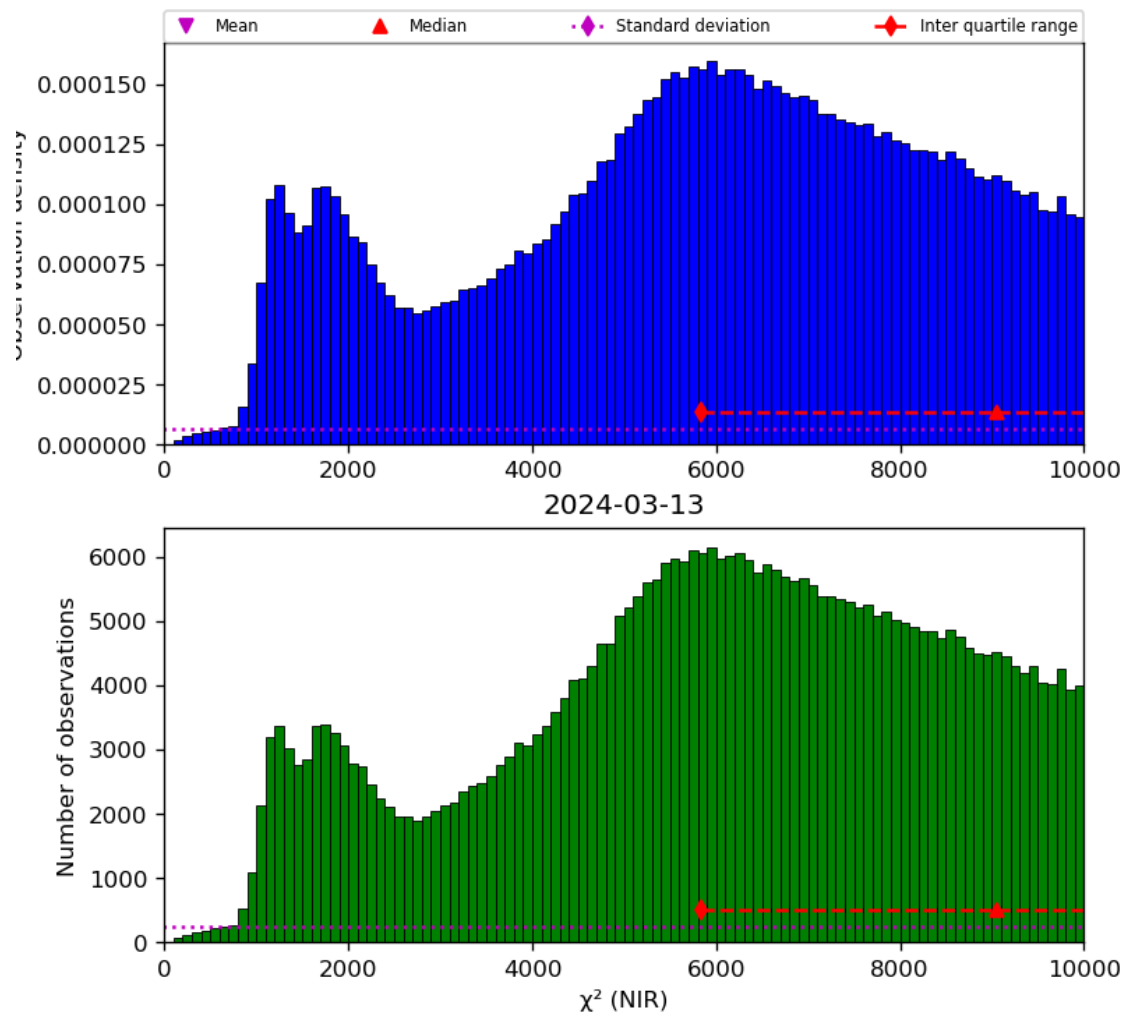
Figure 29: Histogram of “ \chi^2 (NIR)” for 2024-03-12 to 2024-03-14
