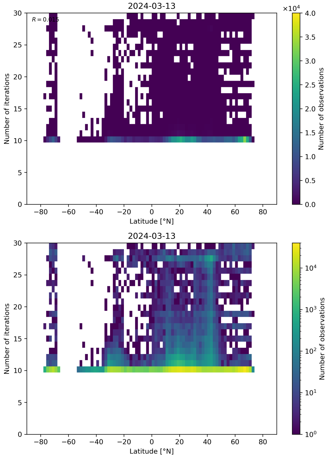
Figure 60: Scatter density plot of “Latitude” against “Number of iterations” for 2024-03-12 to 2024-03-14.
