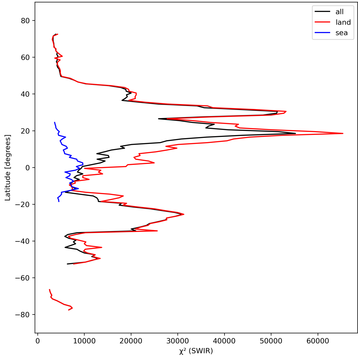
Figure 17: Zonal average of “ \chi^2 (SWIR)” for 2024-03-12 to 2024-03-14.
