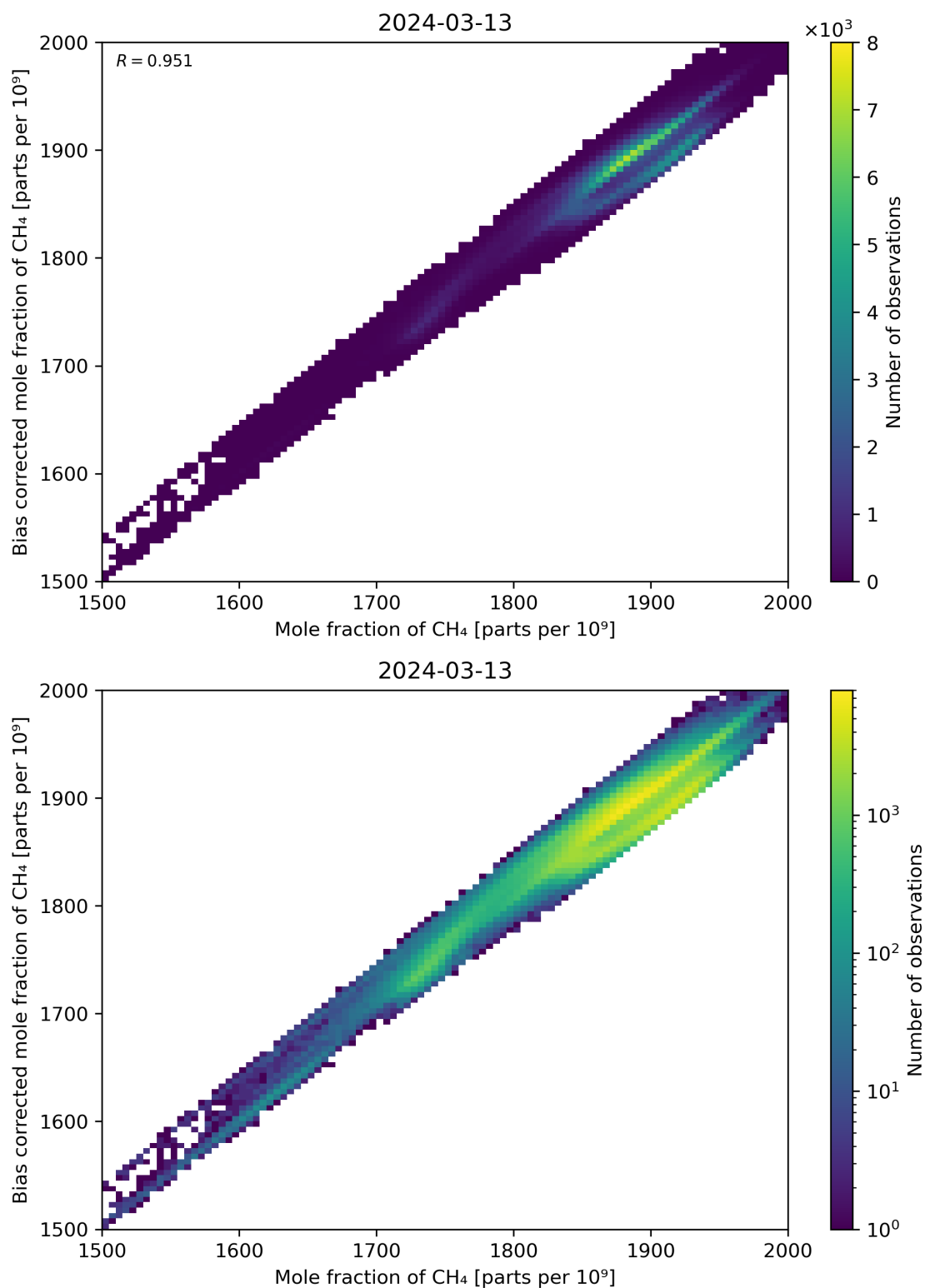
Figure 74: Scatter density plot of “Mole fraction of CH 4 ” against “Bias corrected mole fraction of CH 4 ” for 2024-03-12 to 2024-03-14.
