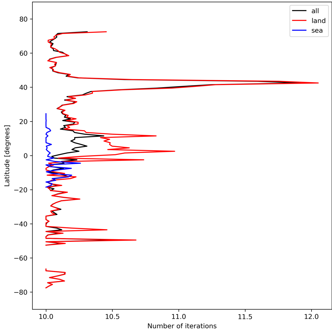
Figure 20: Zonal average of “Number of iterations” for 2024-03-12 to 2024-03-14.
