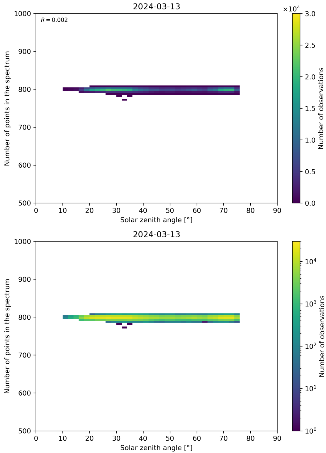
Figure 103: Scatter density plot of “Solar zenith angle” against “Number of points in the spectrum” for 2024-03-12 to 2024-03-14.
