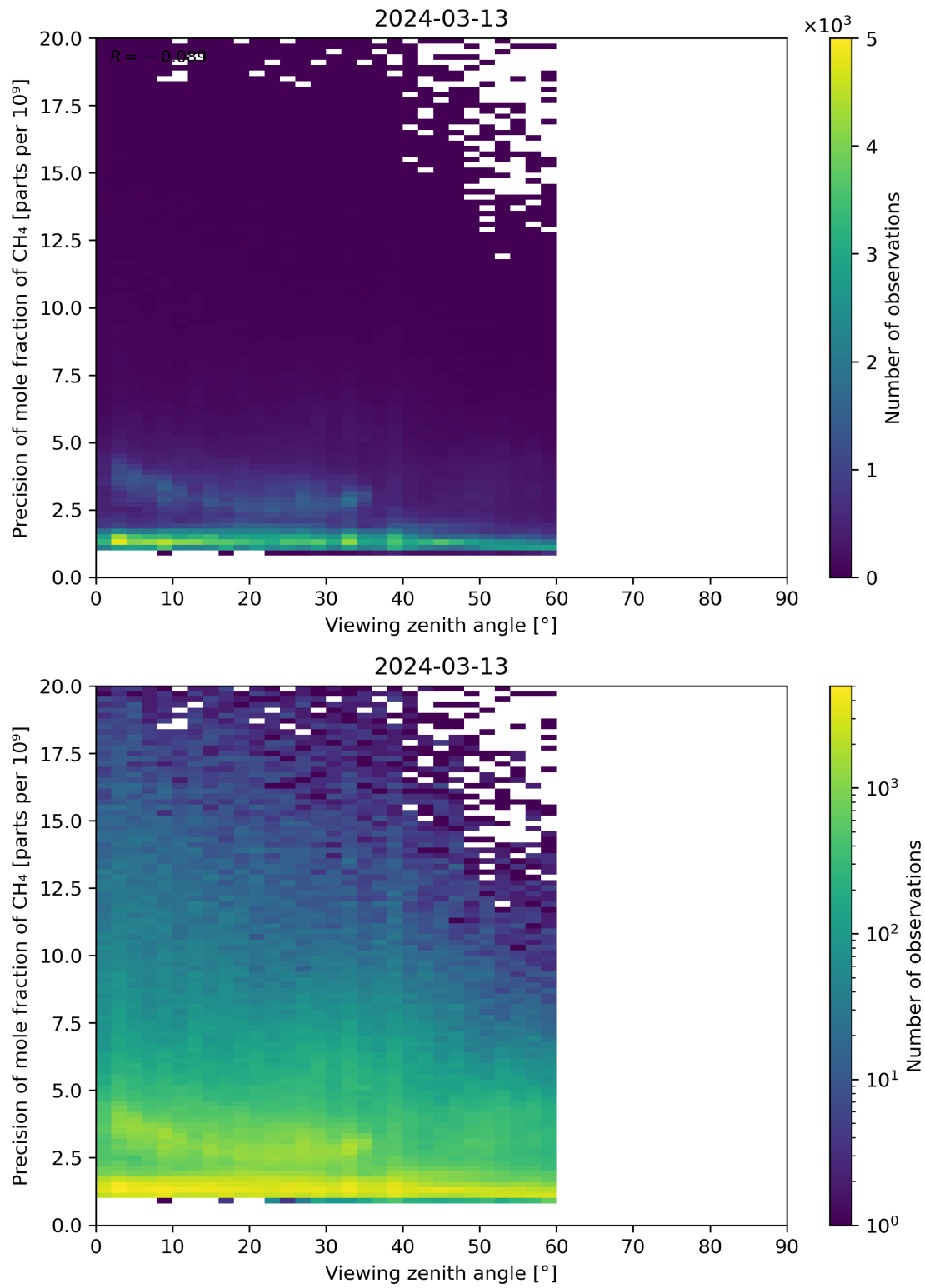
Figure 112: Scatter density plot of “Viewing zenith angle” against “Precision of mole fraction of CH 4 ” for 2024-03-12 to 2024-03-14.
