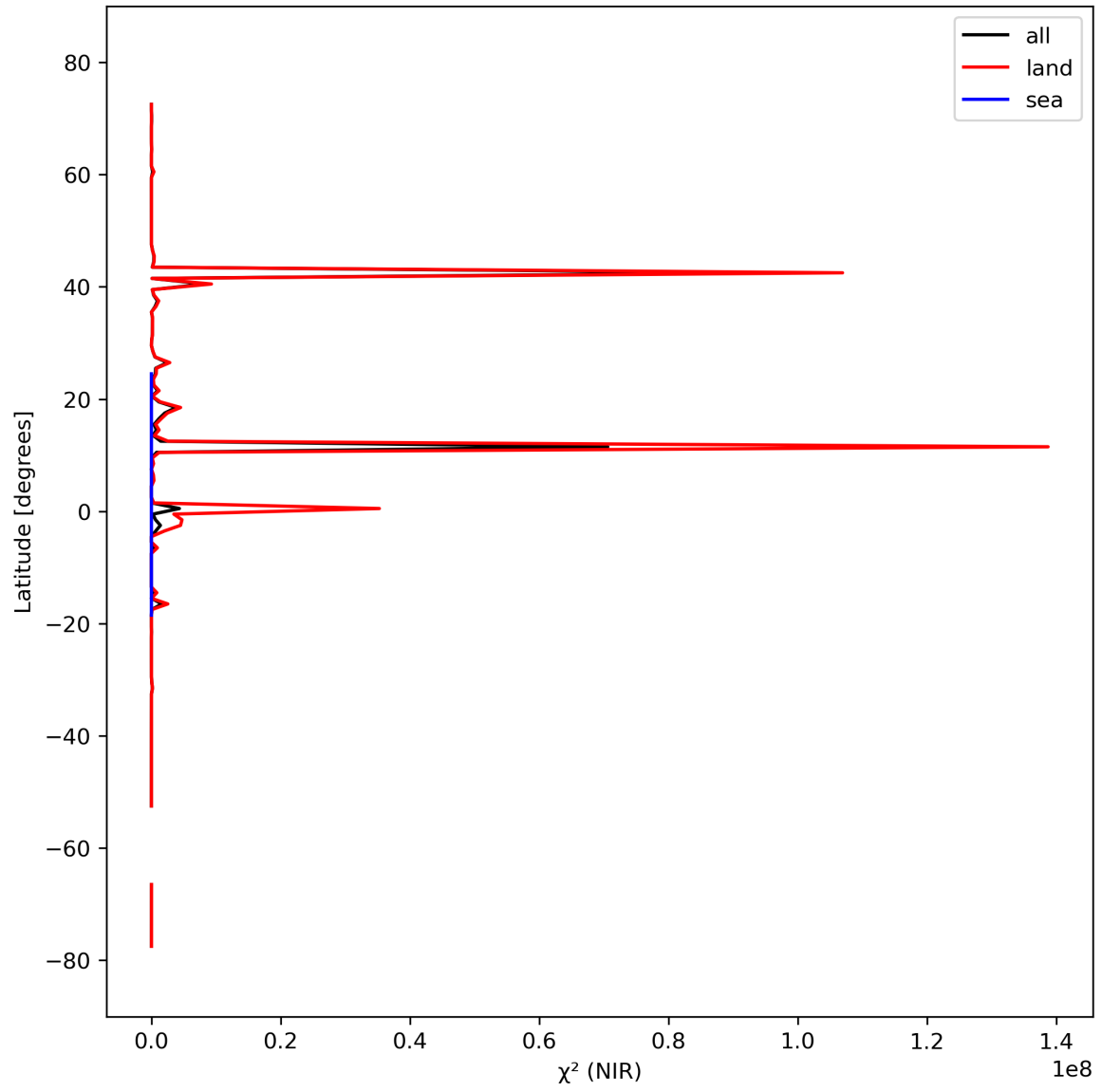
Figure 18: Zonal average of “ \chi^2 (NIR)” for 2024-03-12 to 2024-03-14.
