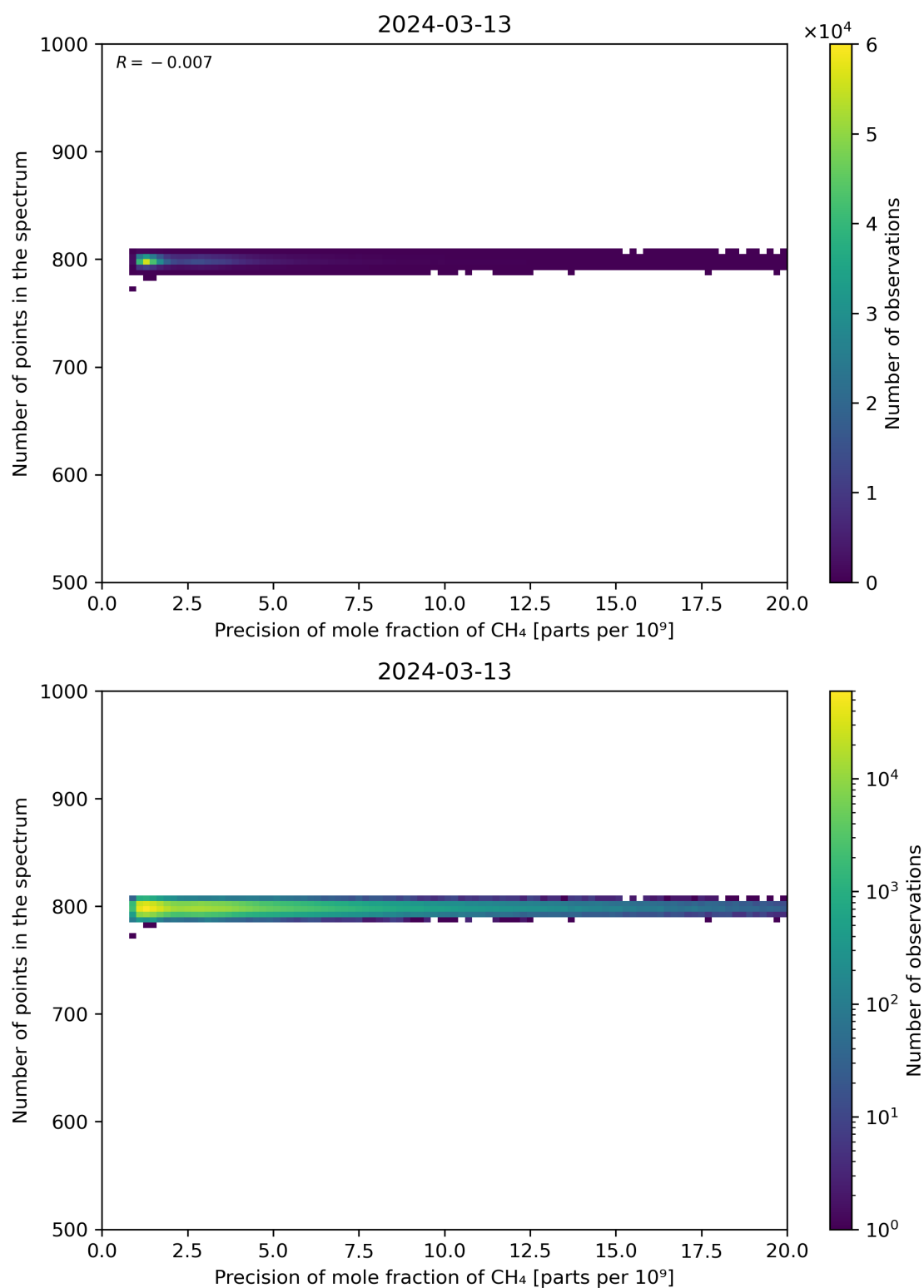
Figure 84: Scatter density plot of “Precision of mole fraction of CH 4 ” against “Number of points in the spectrum” for 2024-03-12 to 2024-03-14.
