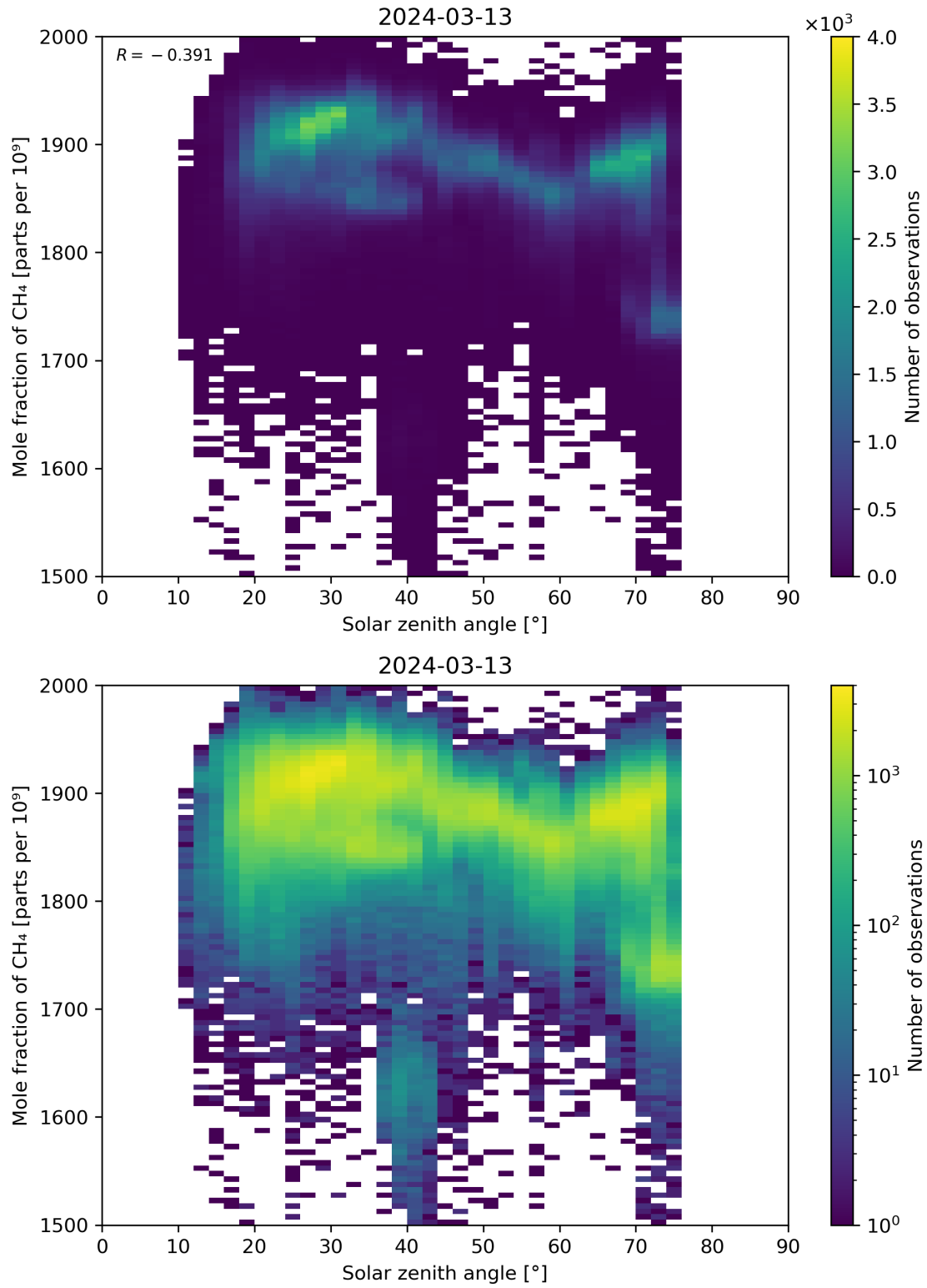
Figure 99: Scatter density plot of “Solar zenith angle” against “Mole fraction of \text{CH}_4 ” for 2024-03-12 to 2024-03-14.
