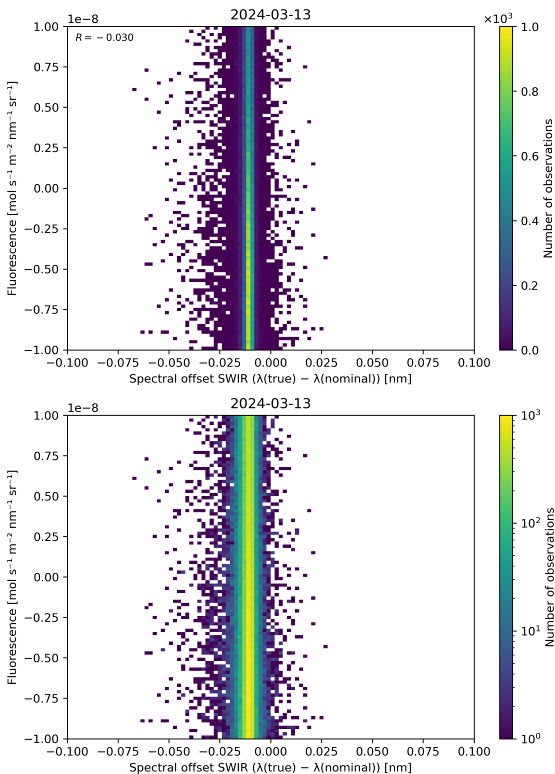
Figure 120: Scatter density plot of “Spectral offset SWIR ( \lambda(\text{true}) - \lambda(\text{nominal}) )” against “Fluorescence” for 2024-03-12 to 2024-03-14.
