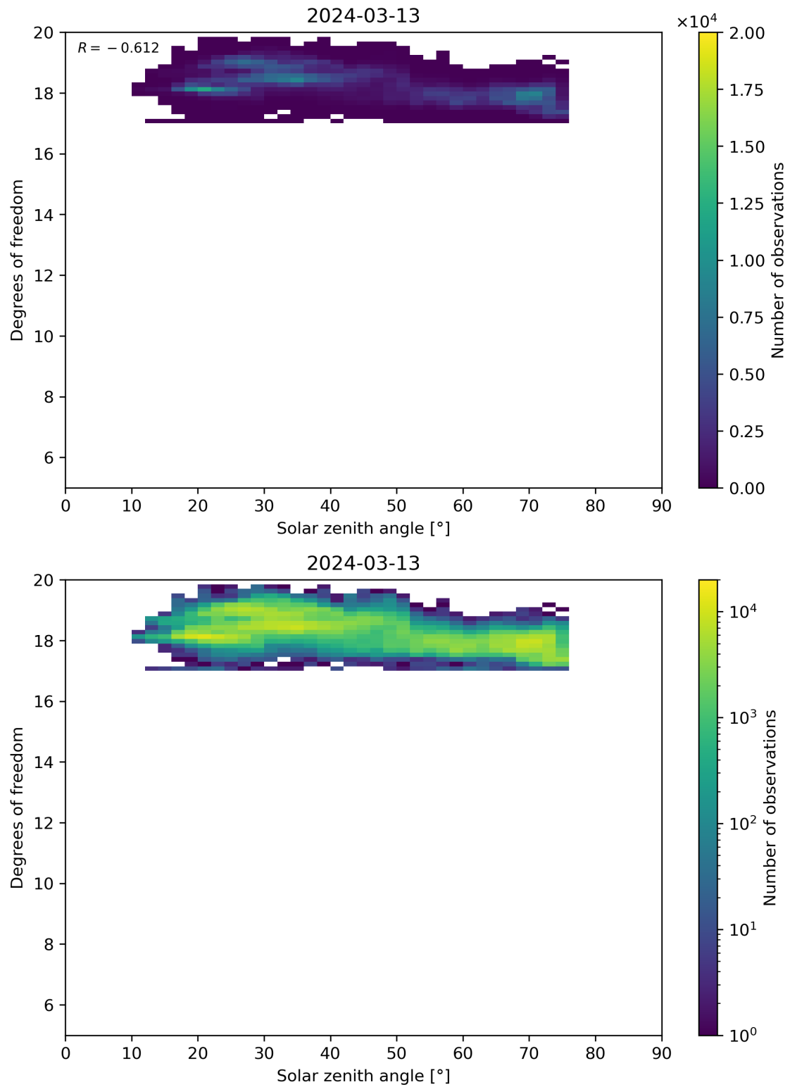
Figure 96: Scatter density plot of “Solar zenith angle” against “Degrees of freedom” for 2024-03-12 to 2024-03-14.
