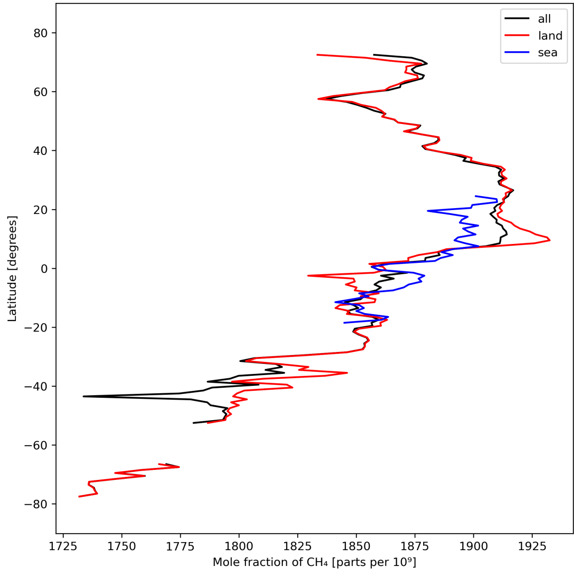
Figure 12: Zonal average of “Mole fraction of \text{CH}_4 ” for 2024-03-12 to 2024-03-14.
