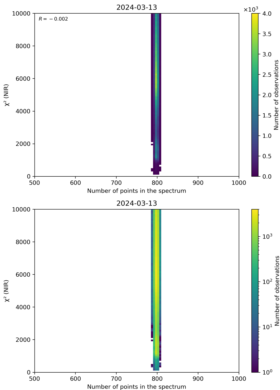
Figure 88: Scatter density plot of “Number of points in the spectrum” against “ \chi^2 (NIR)” for 2024-03-12 to 2024-03-14.
