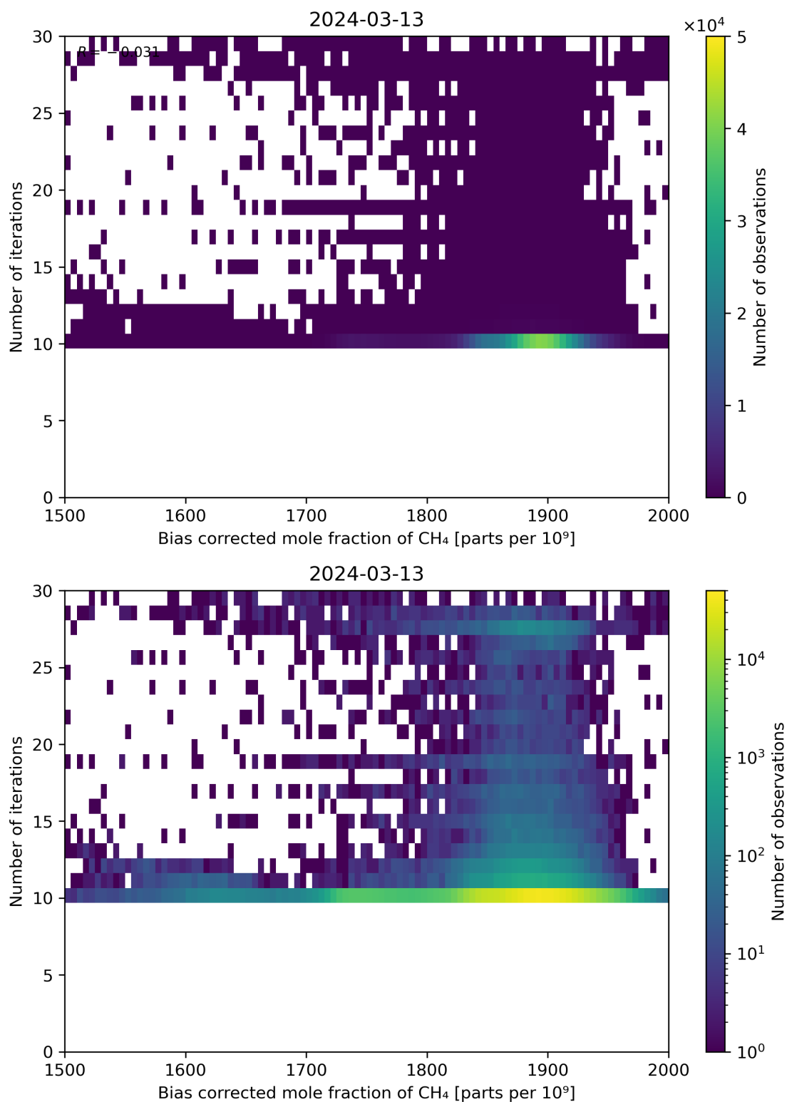
Figure 67: Scatter density plot of “Bias corrected mole fraction of \text{CH}_4 ” against “Number of iterations” for 2024-03-12 to 2024-03-14.
