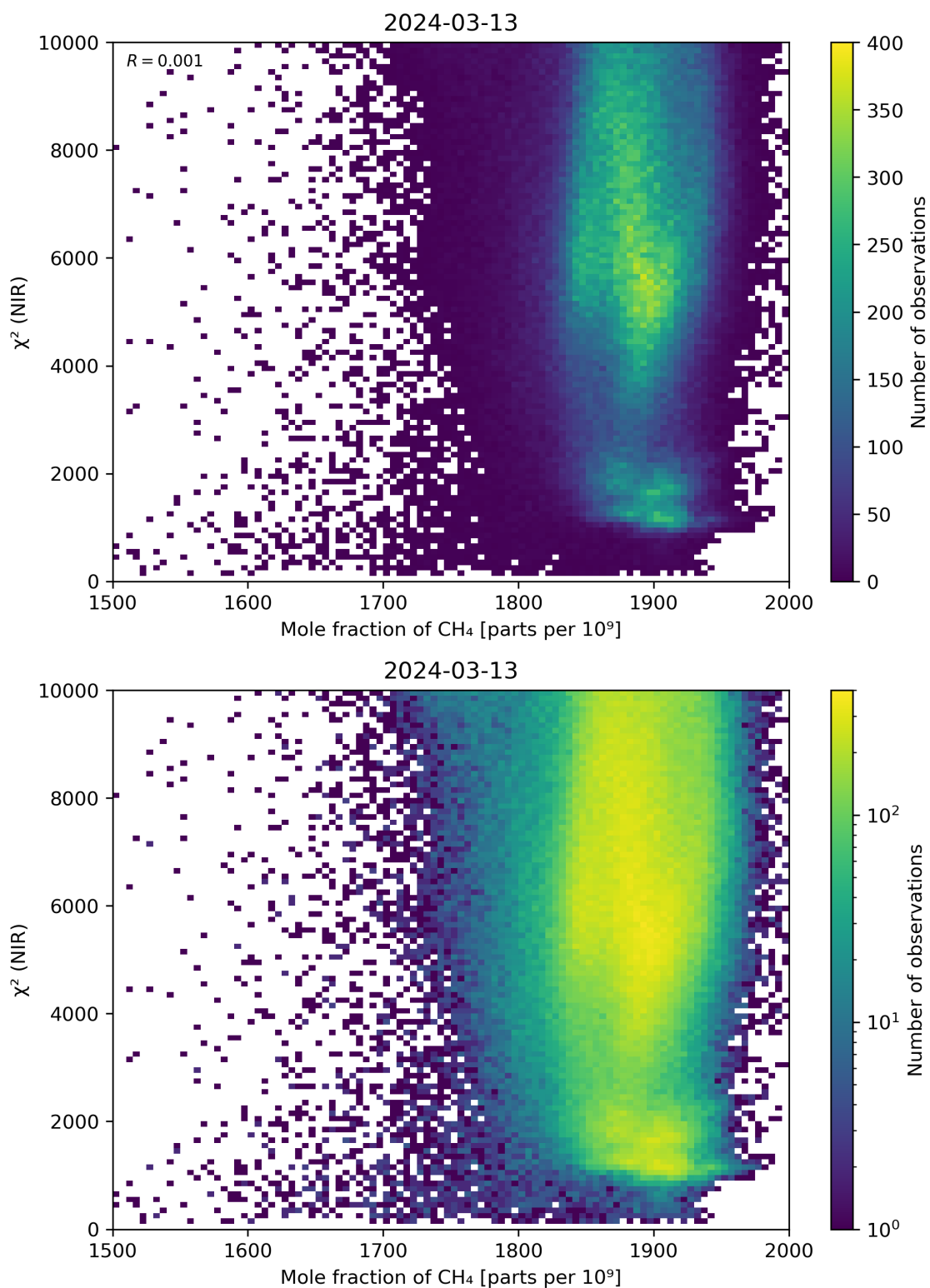
Figure 70: Scatter density plot of “Mole fraction of CH 4 ” against “ \chi^2 (NIR)” for 2024-03-12 to 2024-03-14.
