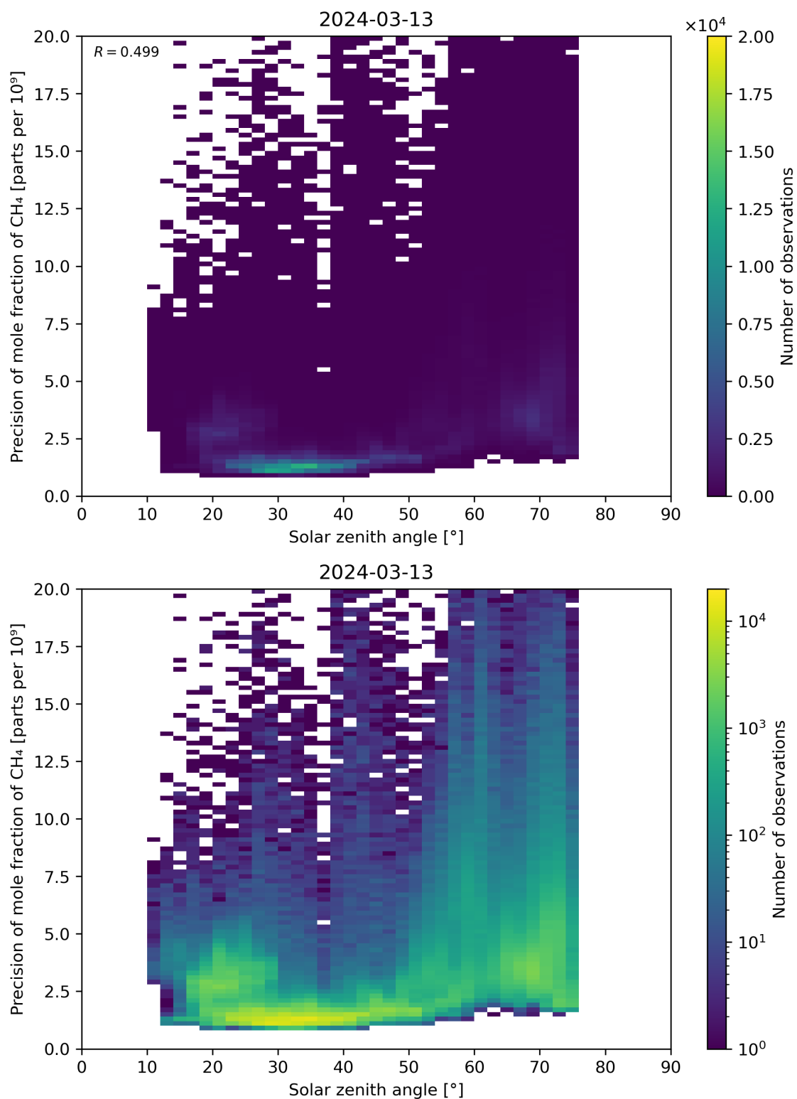
Figure 101: Scatter density plot of “Solar zenith angle” against “Precision of mole fraction of CH 4 ” for 2024-03-12 to 2024-03-14.
