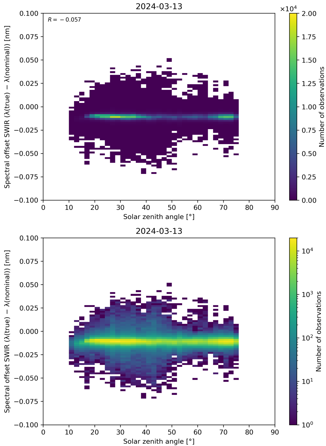
Figure 104: Scatter density plot of “Solar zenith angle” against “Spectral offset SWIR ( \lambda(\text{true}) - \lambda(\text{nominal}) )” for 2024-03-12 to 2024-03-14.
