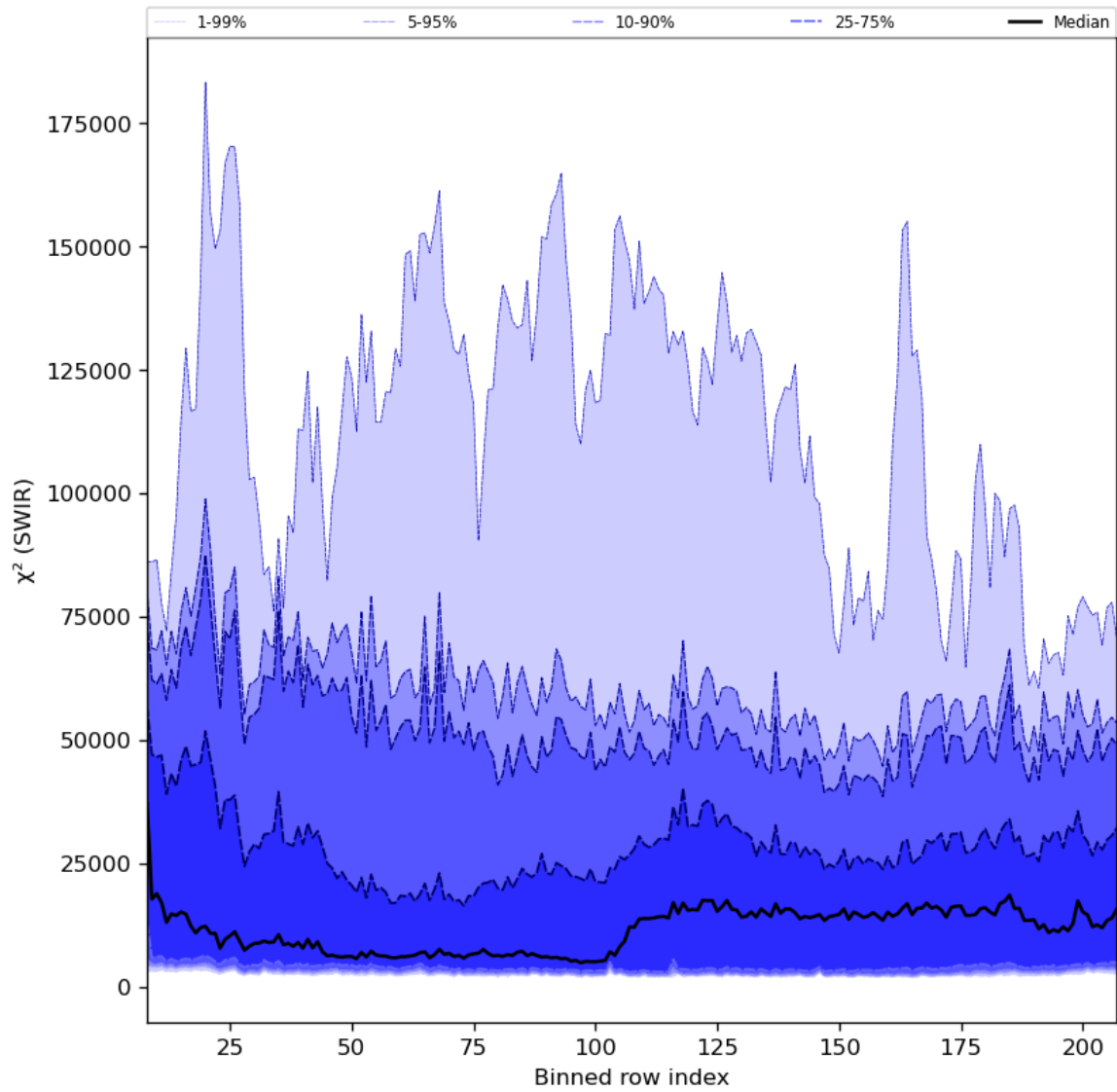
Figure 39: Along track statistics of “ \chi^2 (SWIR)” for 2024-03-12 to 2024-03-14
