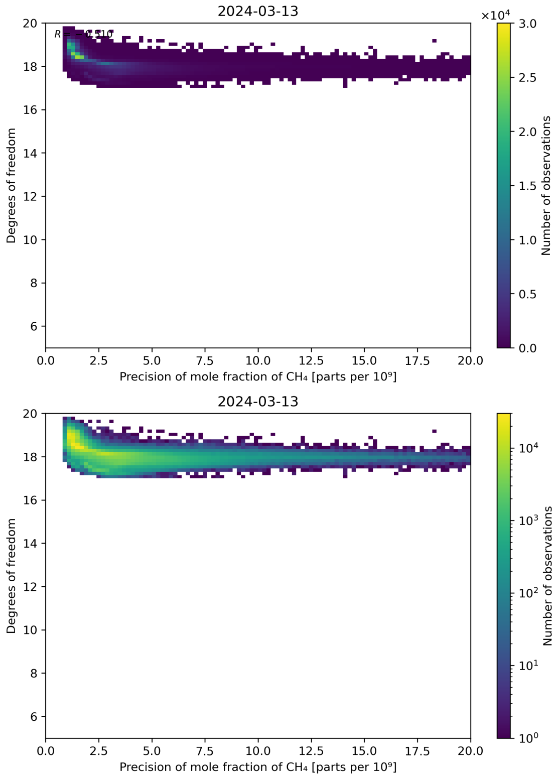
Figure 80: Scatter density plot of “Precision of mole fraction of CH 4 ” against “Degrees of freedom” for 2024-03-12 to 2024-03-14.
