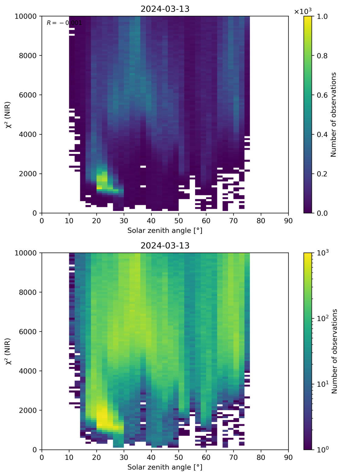
Figure 94: Scatter density plot of “Solar zenith angle” against “ \chi^2 (NIR)” for 2024-03-12 to 2024-03-14.
