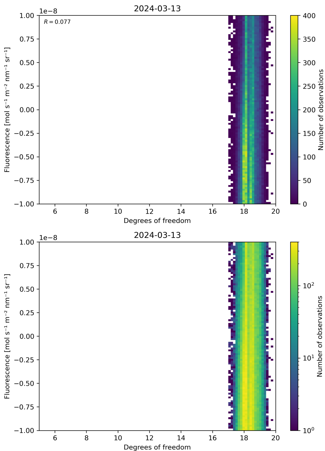
Figure 51: Scatter density plot of “Degrees of freedom” against “Fluorescence” for 2024-03-12 to 2024-03-14.
