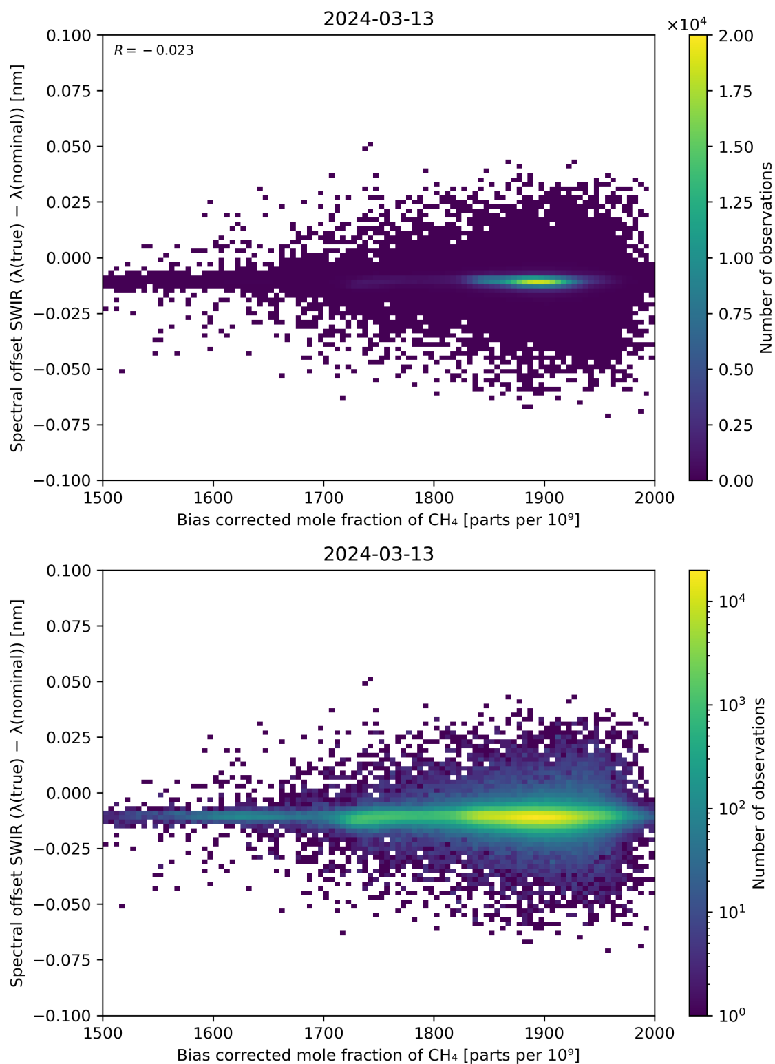
Figure 69: Scatter density plot of “Bias corrected mole fraction of \text{CH}_4 ” against “Spectral offset SWIR ( \lambda(\text{true}) - \lambda(\text{nominal}) )” for 2024-03-12 to 2024-03-14.
