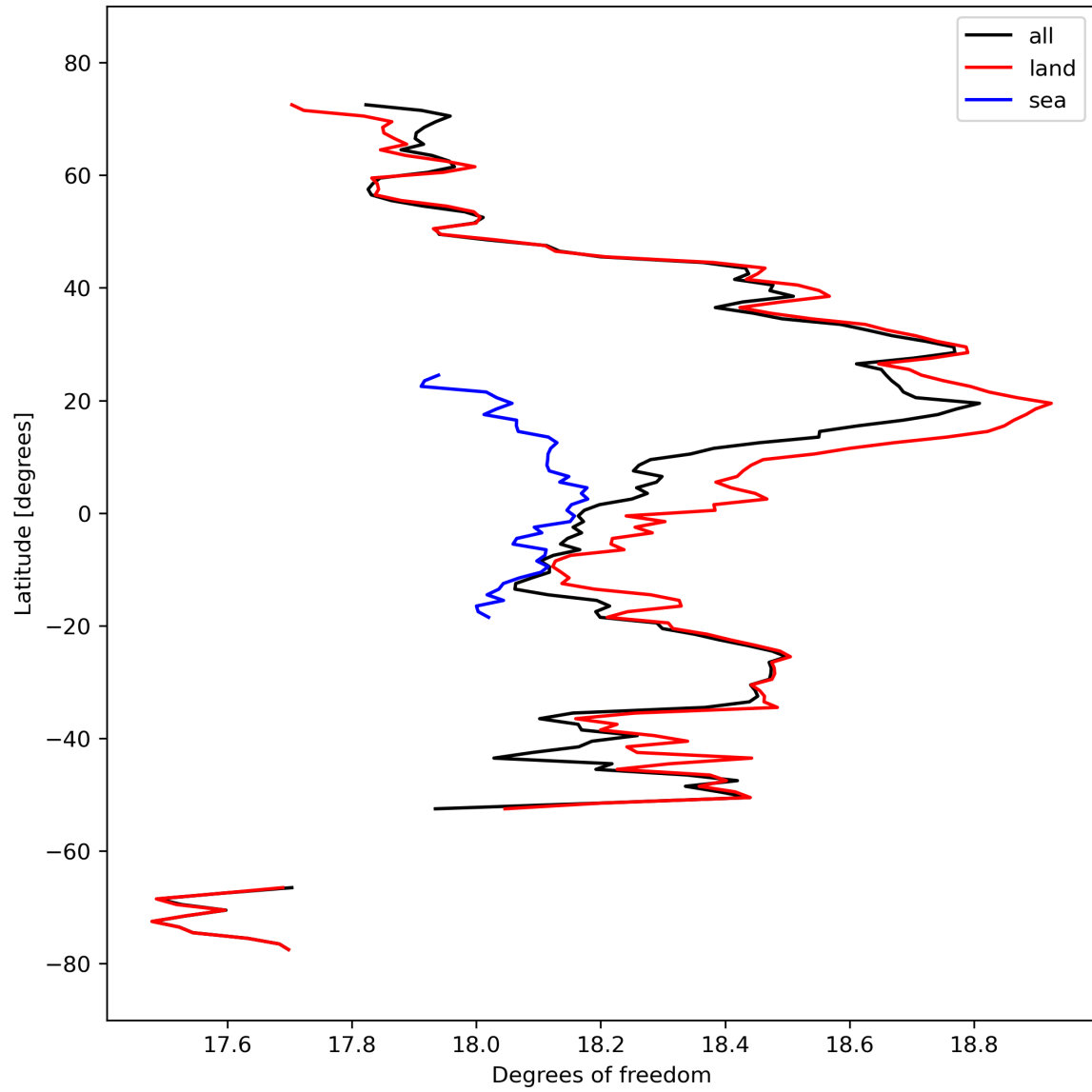
Figure 19: Zonal average of “Degrees of freedom” for 2024-03-12 to 2024-03-14.
