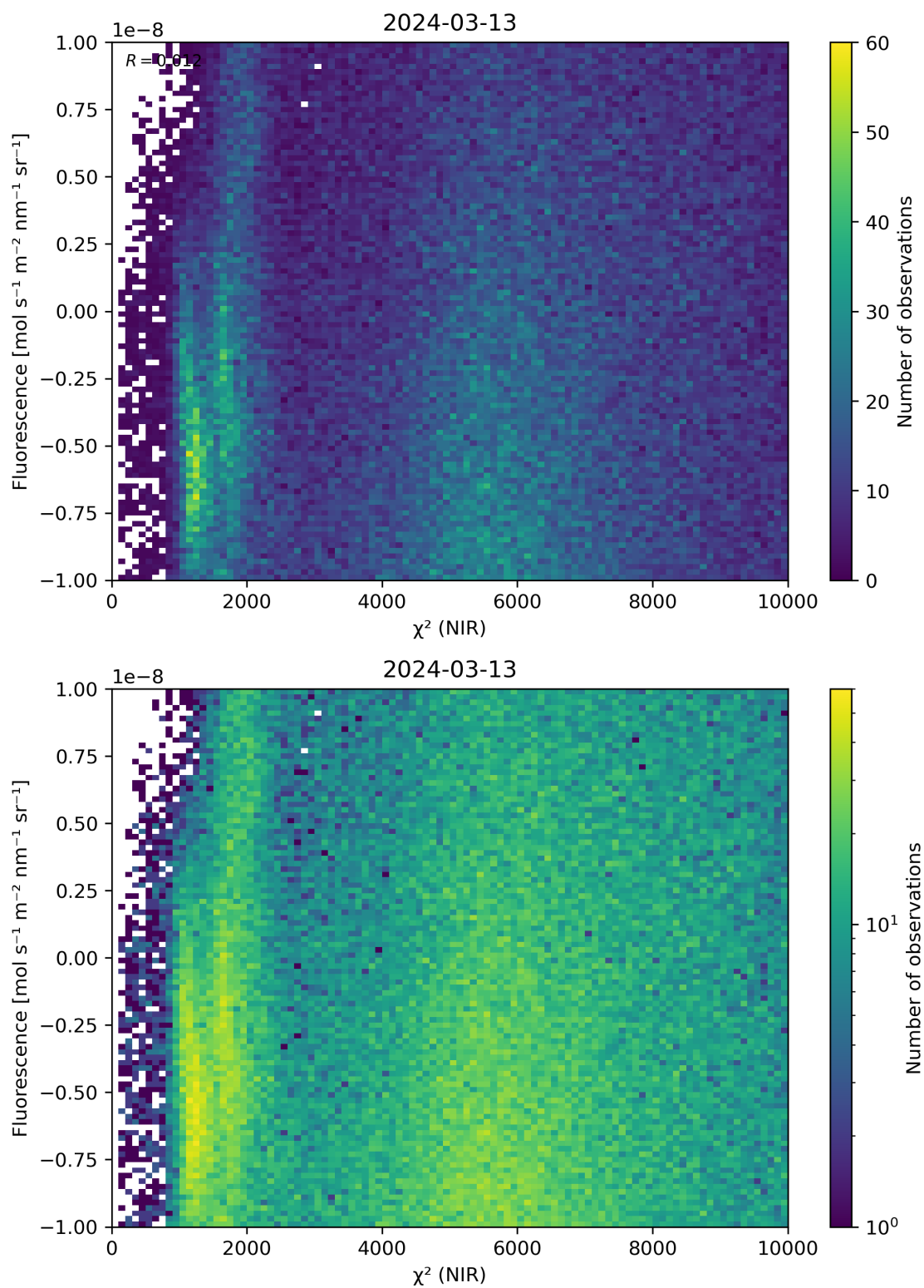
Figure 45: Scatter density plot of “ \chi^2 (NIR)” against “Fluorescence” for 2024-03-12 to 2024-03-14.
