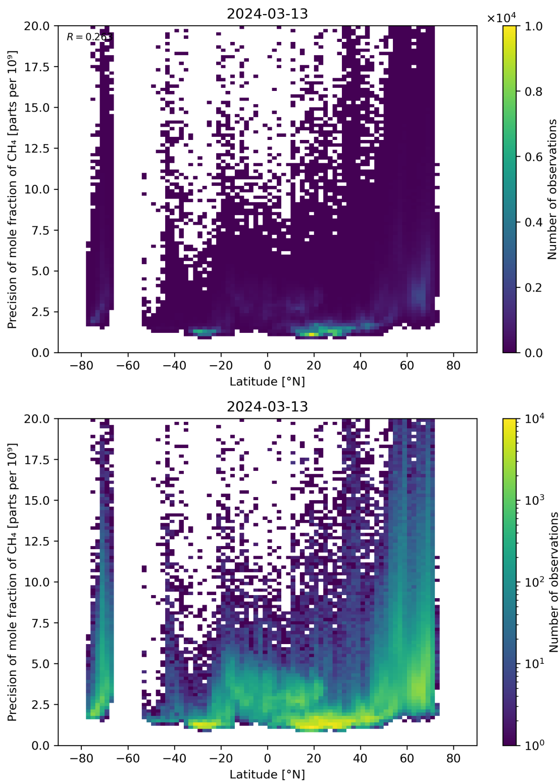
Figure 59: Scatter density plot of “Latitude” against “Precision of mole fraction of \text{CH}_4 ” for 2024-03-12 to 2024-03-14.
