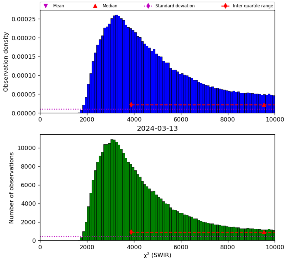
Figure 28: Histogram of “ \chi^2 (SWIR)” for 2024-03-12 to 2024-03-14
