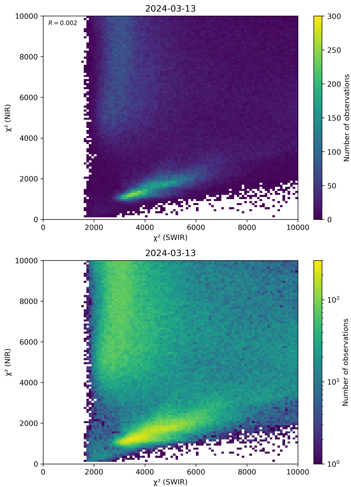
Figure 47: Scatter density plot of “ \chi^2 (SWIR)” against “ \chi^2 (NIR)” for 2024-03-12 to 2024-03-14.
