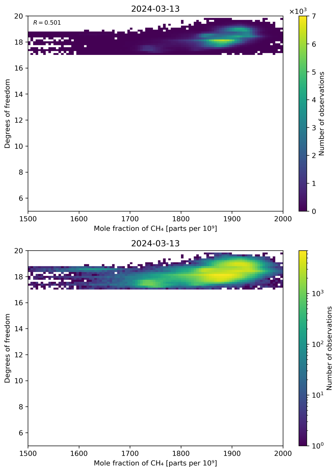
Figure 72: Scatter density plot of "Mole fraction of CH 4 " against "Degrees of freedom" for 2024-03-12 to 2024-03-14.
