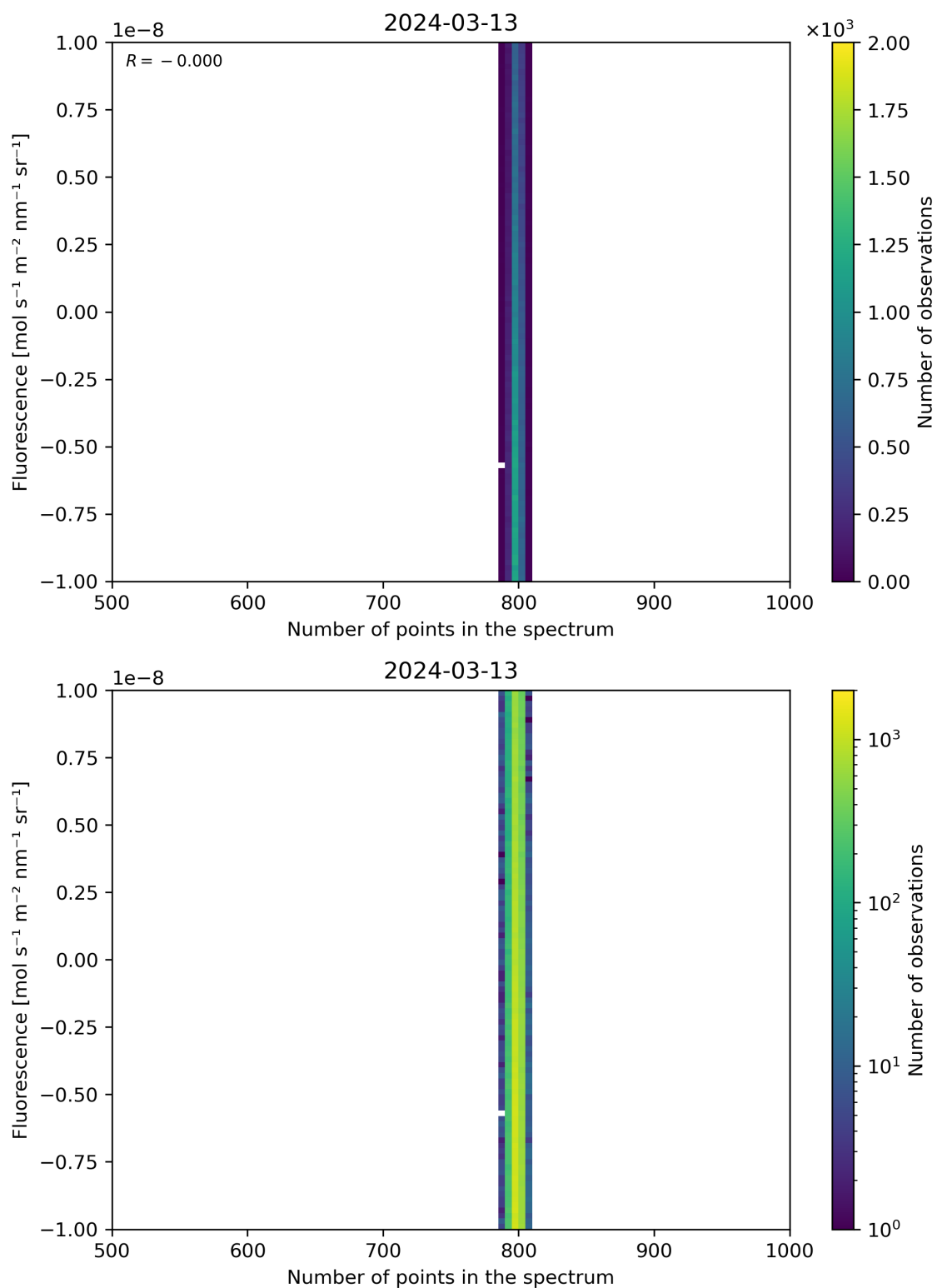
Figure 91: Scatter density plot of “Number of points in the spectrum” against “Fluorescence” for 2024-03-12 to 2024-03-14.
