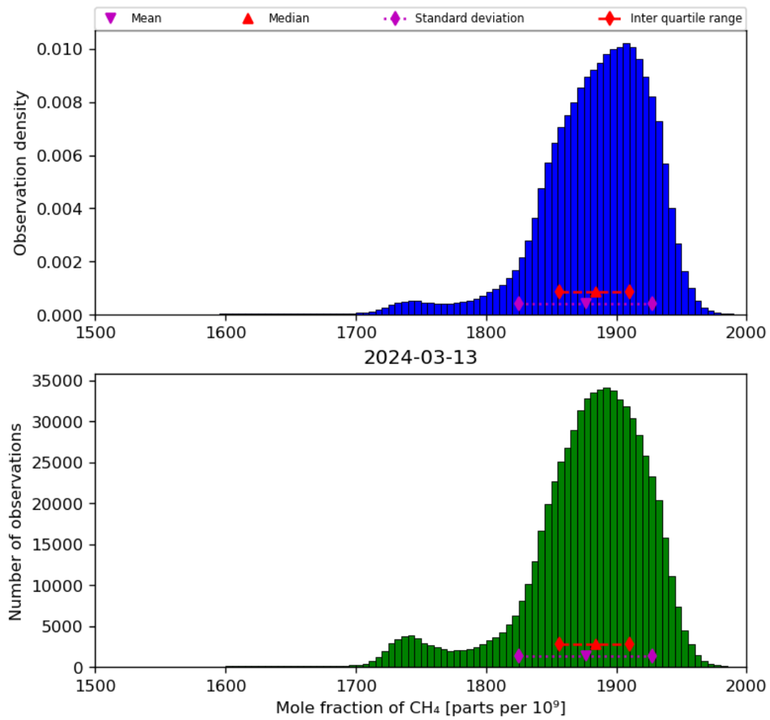
Figure 23: Histogram of “Mole fraction of CH 4 ” for 2024-03-12 to 2024-03-14
