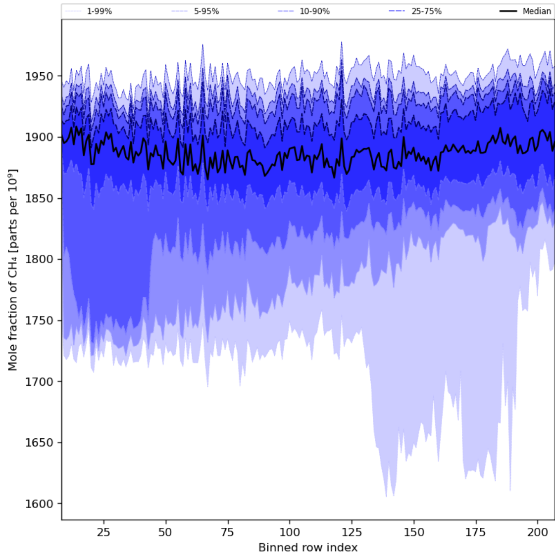
Figure 34: Along track statistics of “Mole fraction of CH 4 ” for 2024-03-12 to 2024-03-14
