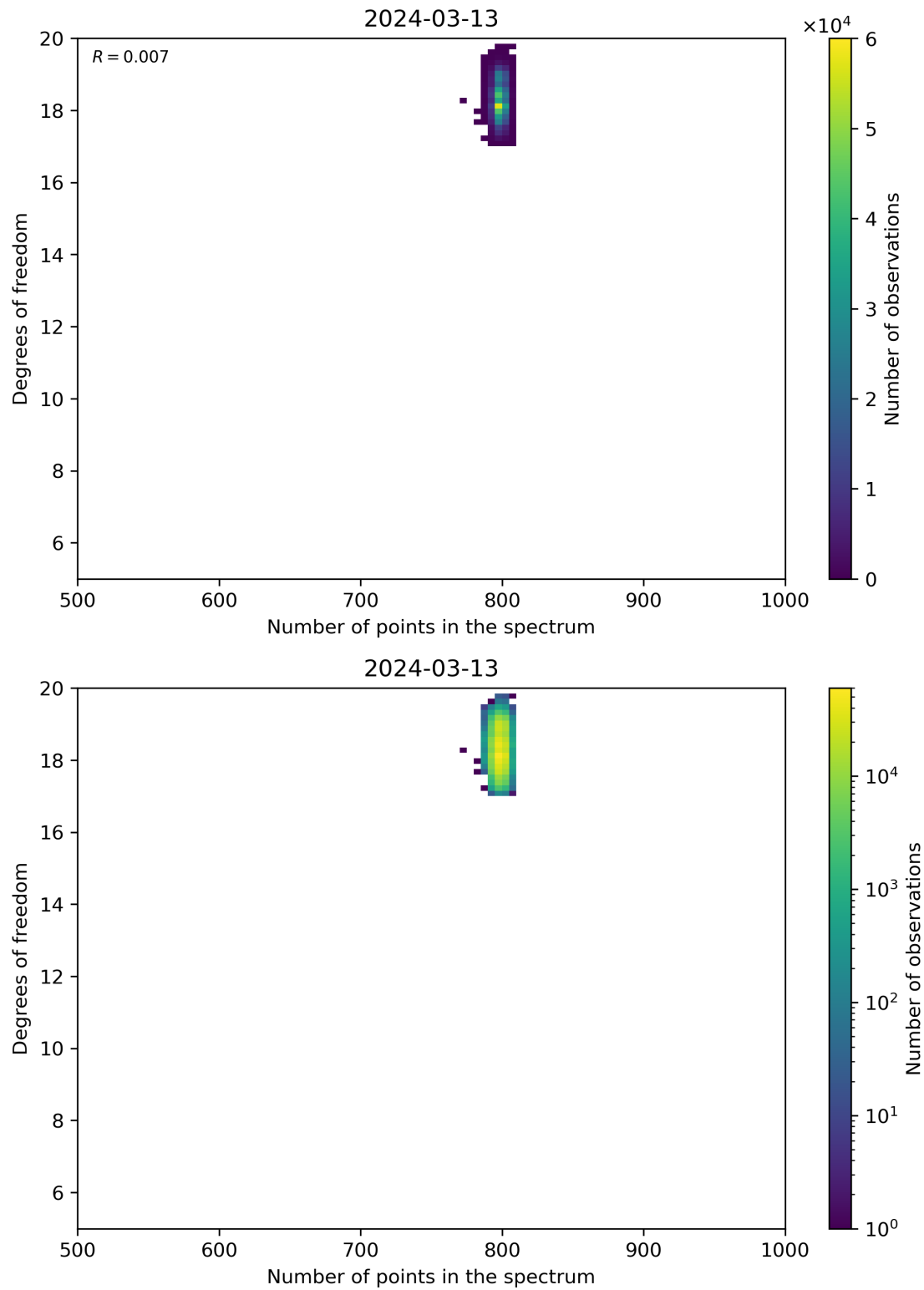
Figure 90: Scatter density plot of “Number of points in the spectrum” against “Degrees of freedom” for 2024-03-12 to 2024-03-14.
