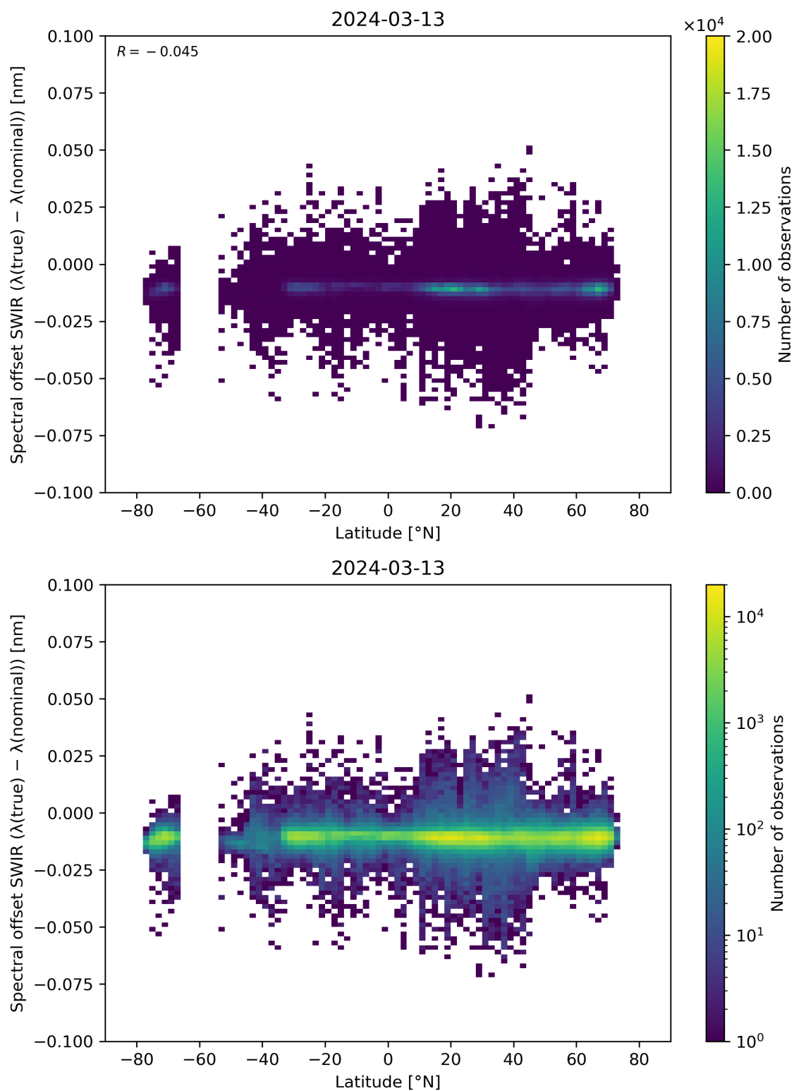
Figure 62: Scatter density plot of “Latitude” against “Spectral offset SWIR ( \lambda(\text{true}) - \lambda(\text{nominal}) )” for 2024-03-12 to 2024-03-14.
