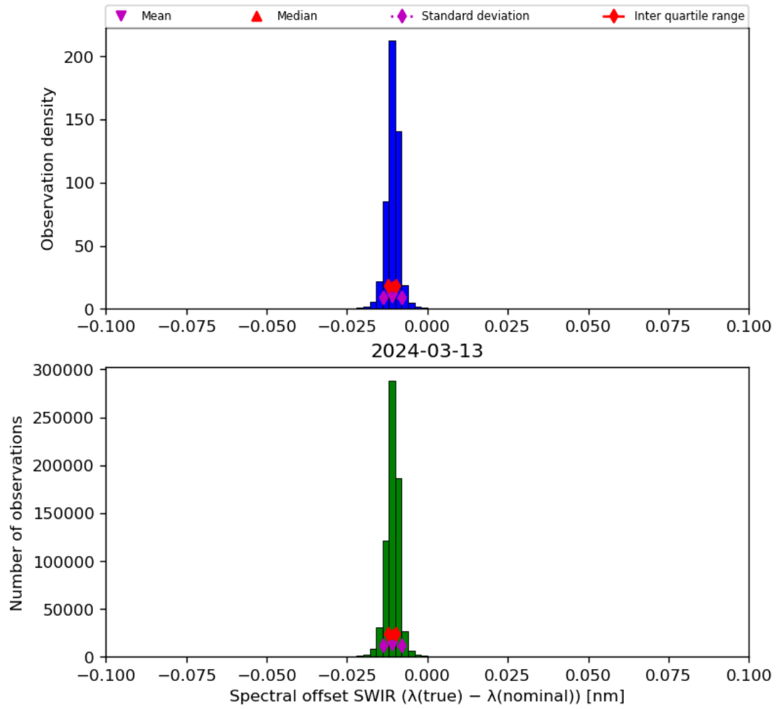
Figure 27: Histogram of “Spectral offset SWIR ( \lambda(\text{true}) - \lambda(\text{nominal}) )” for 2024-03-12 to 2024-03-14
