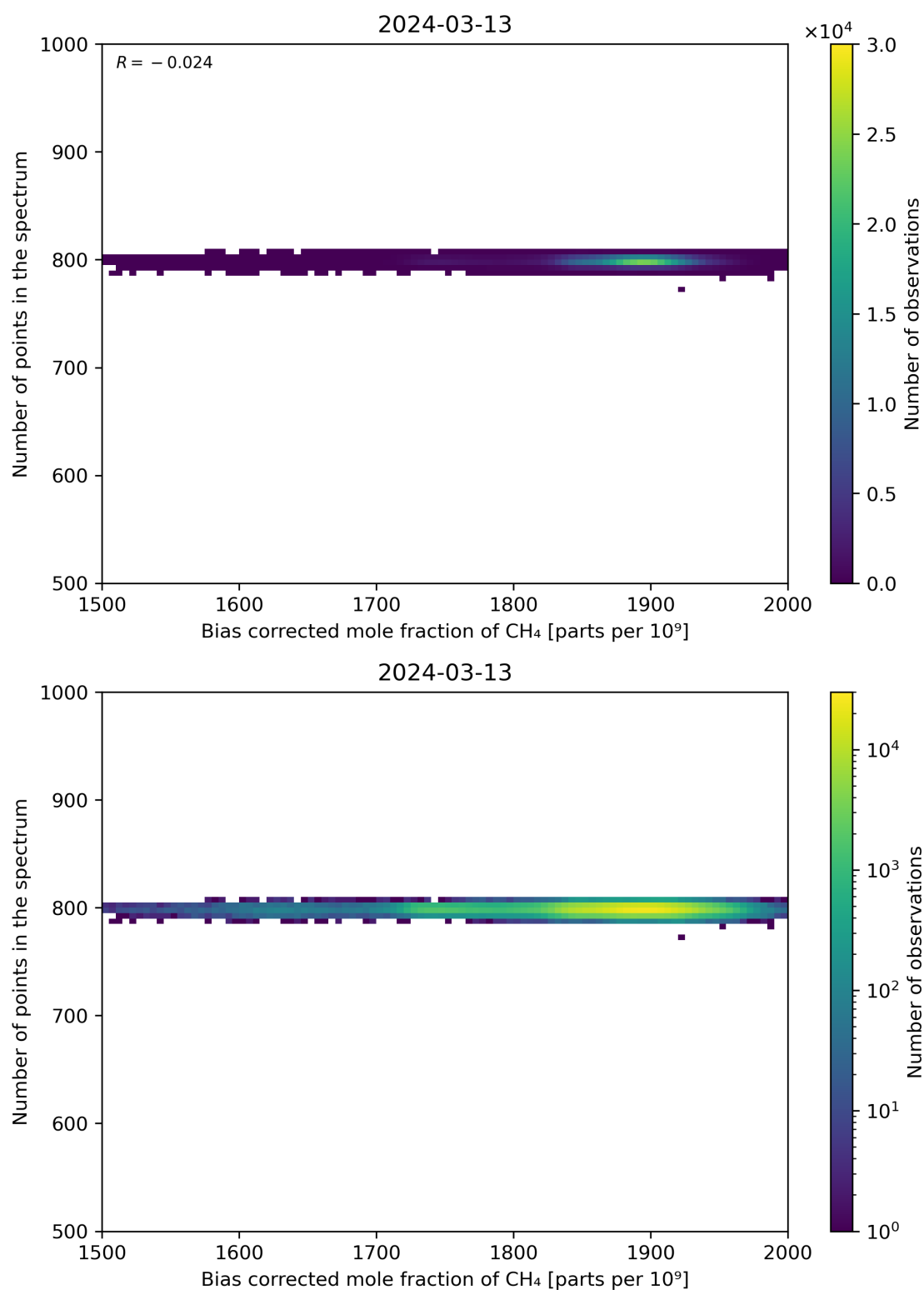
Figure 68: Scatter density plot of “Bias corrected mole fraction of CH 4 ” against “Number of points in the spectrum” for 2024-03-12 to 2024-03-14.
