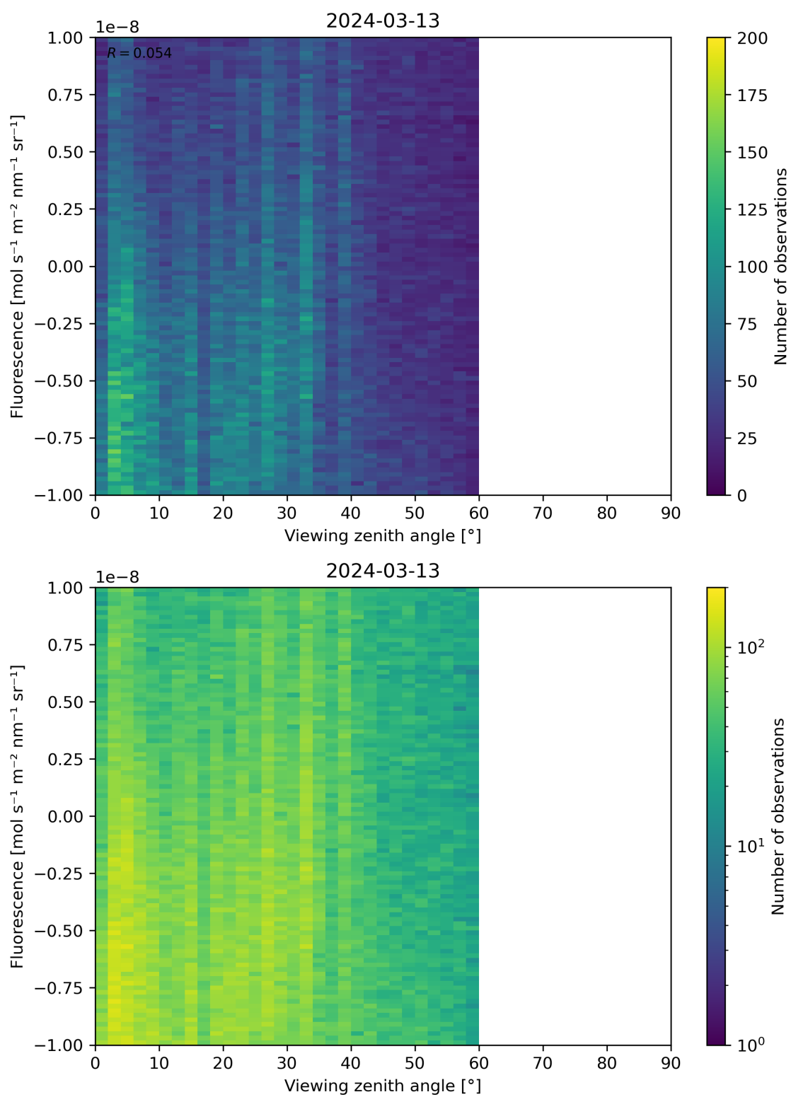
Figure 108: Scatter density plot of “Viewing zenith angle” against “Fluorescence” for 2024-03-12 to 2024-03-14.
