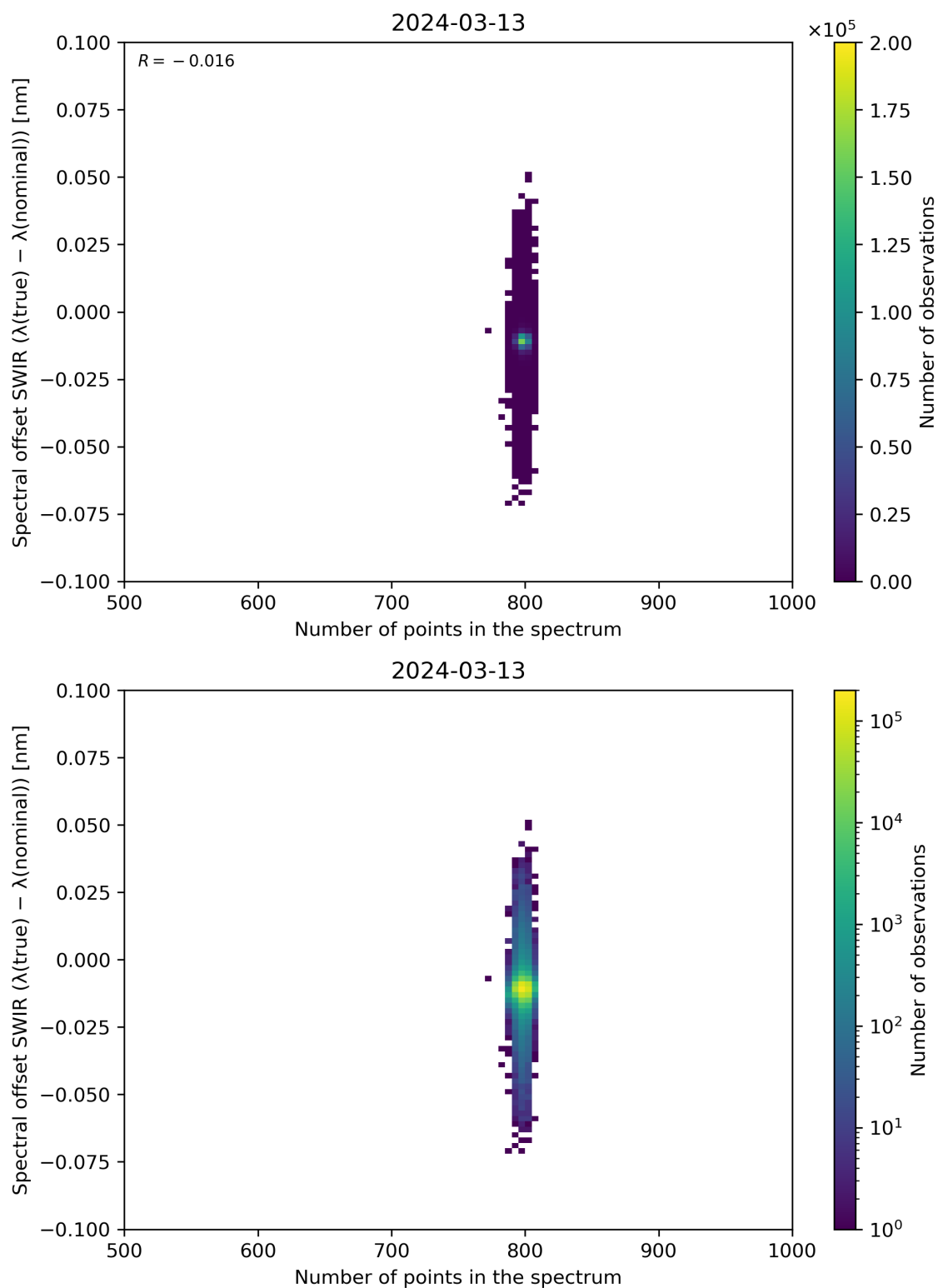
Figure 93: Scatter density plot of “Number of points in the spectrum” against “Spectral offset SWIR ( \lambda(\text{true}) - \lambda(\text{nominal}) )” for 2024-03-12 to 2024-03-14.
