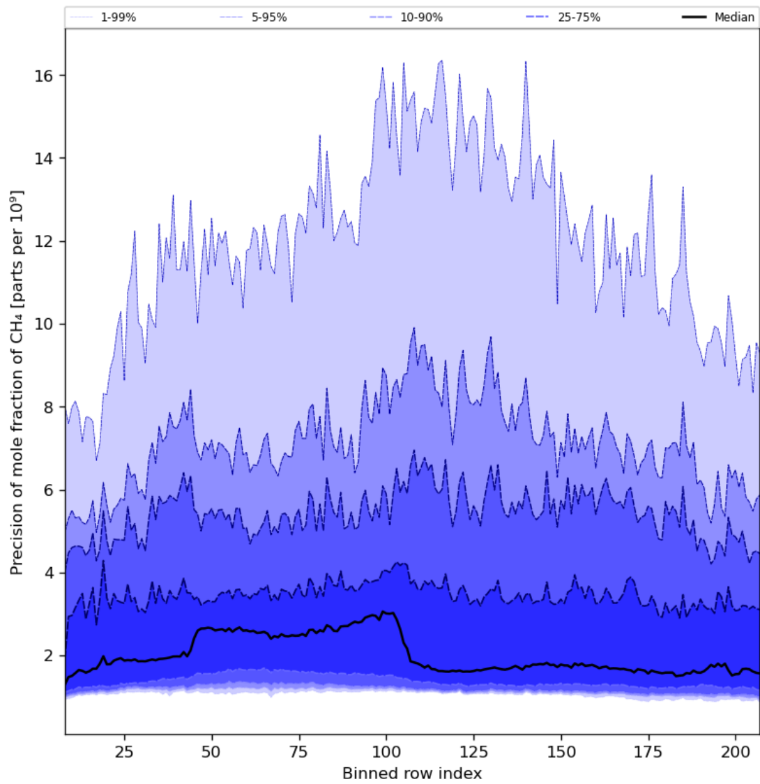
Figure 35: Along track statistics of “Precision of mole fraction of CH 4 ” for 2024-03-12 to 2024-03-14
