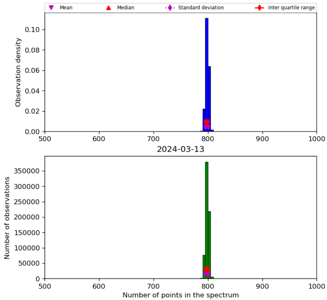
Figure 26: Histogram of “Number of points in the spectrum” for 2024-03-12 to 2024-03-14
