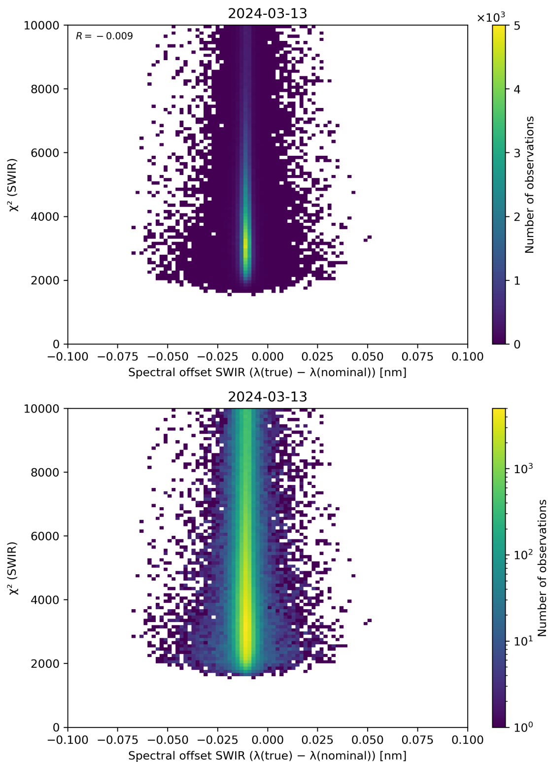
Figure 118: Scatter density plot of “Spectral offset SWIR ( \lambda(\text{true}) - \lambda(\text{nominal}) )” against “ \chi^2 (SWIR)” for 2024-03-12 to 2024-03-14.
