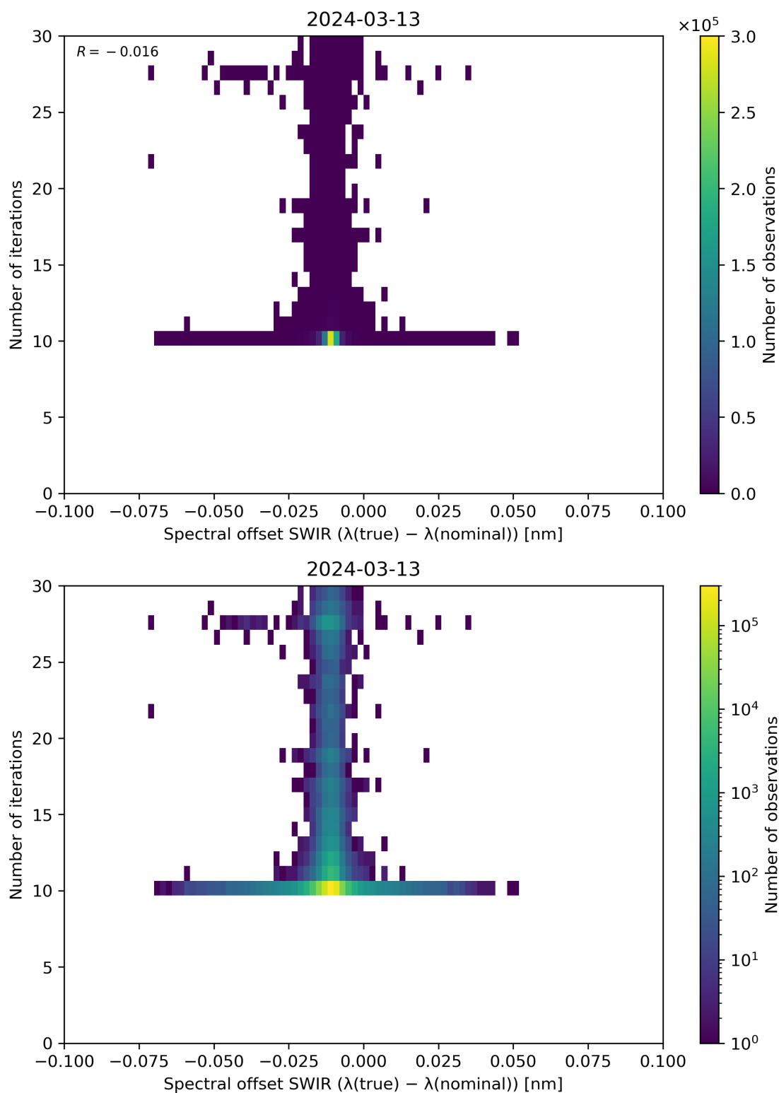
Figure 121: Scatter density plot of “Spectral offset SWIR ( \lambda(\text{true}) - \lambda(\text{nominal}) )” against “Number of iterations” for 2024-03-12 to 2024-03-14.
