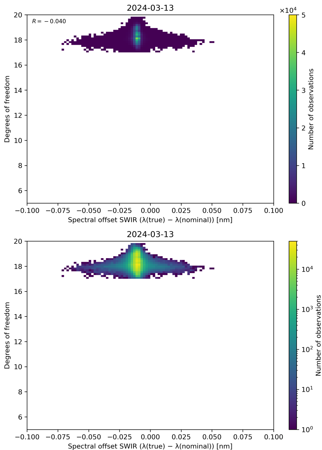
Figure 119: Scatter density plot of “Spectral offset SWIR ( \lambda(\text{true}) - \lambda(\text{nominal}) )” against “Degrees of freedom” for 2024-03-12 to 2024-03-14.
