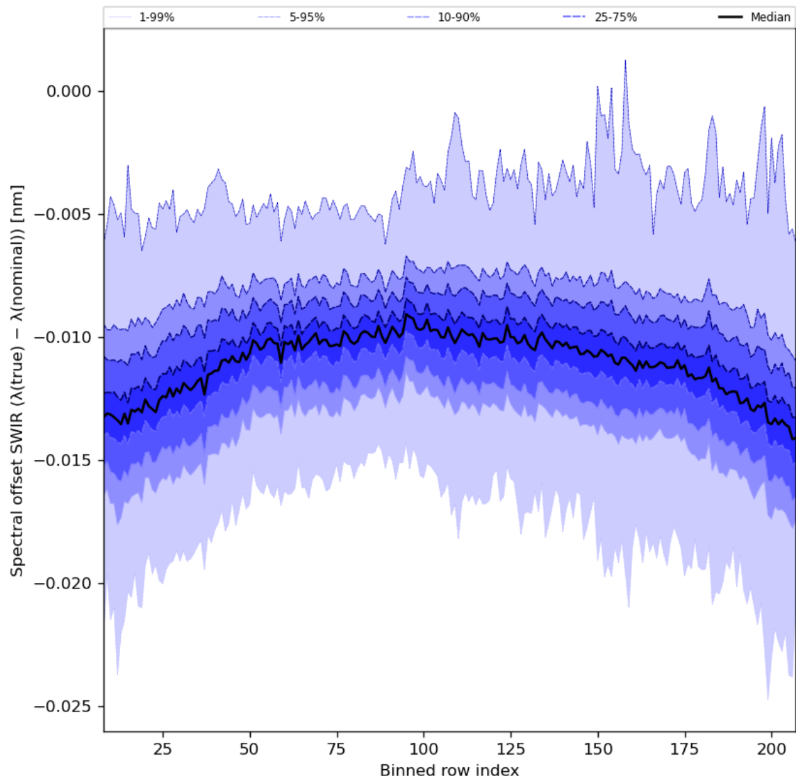
Figure 38: Along track statistics of “Spectral offset SWIR ( \lambda(\text{true}) - \lambda(\text{nominal}) )” for 2024-03-12 to 2024-03-14
