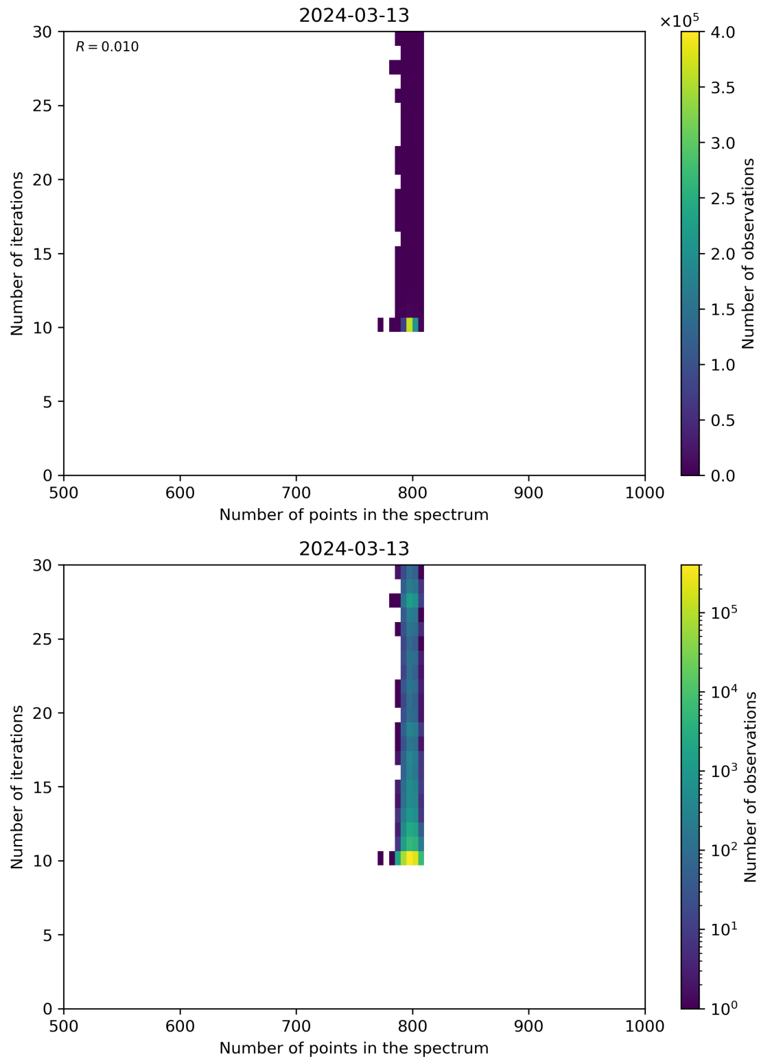
Figure 92: Scatter density plot of “Number of points in the spectrum” against “Number of iterations” for 2024-03-12 to 2024-03-14.
