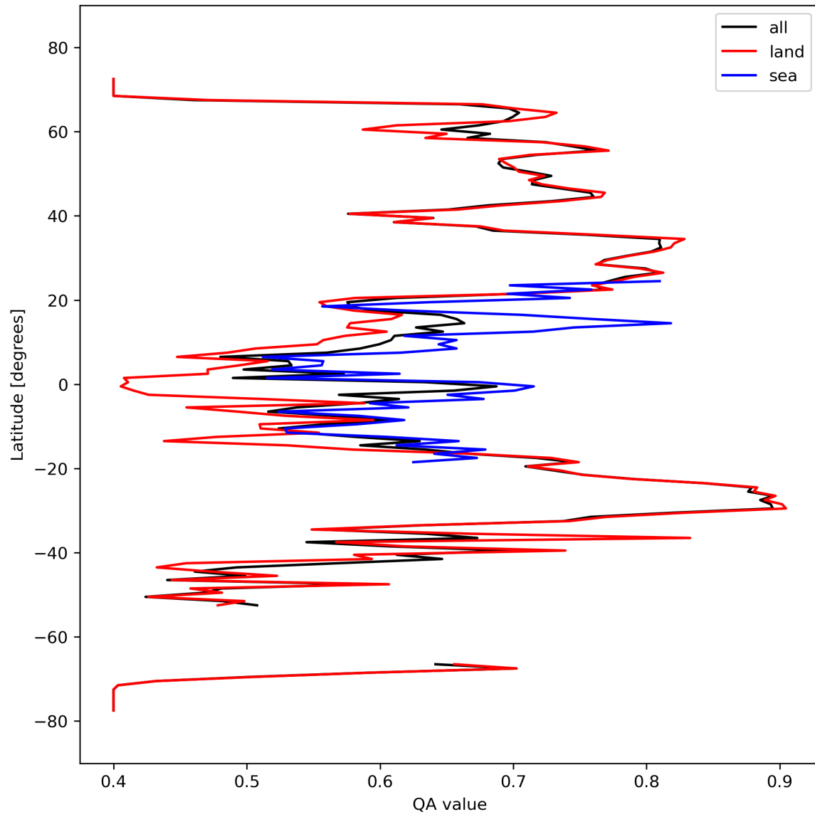
Figure 11: Zonal average of “QA value” for 2024-03-12 to 2024-03-14.
