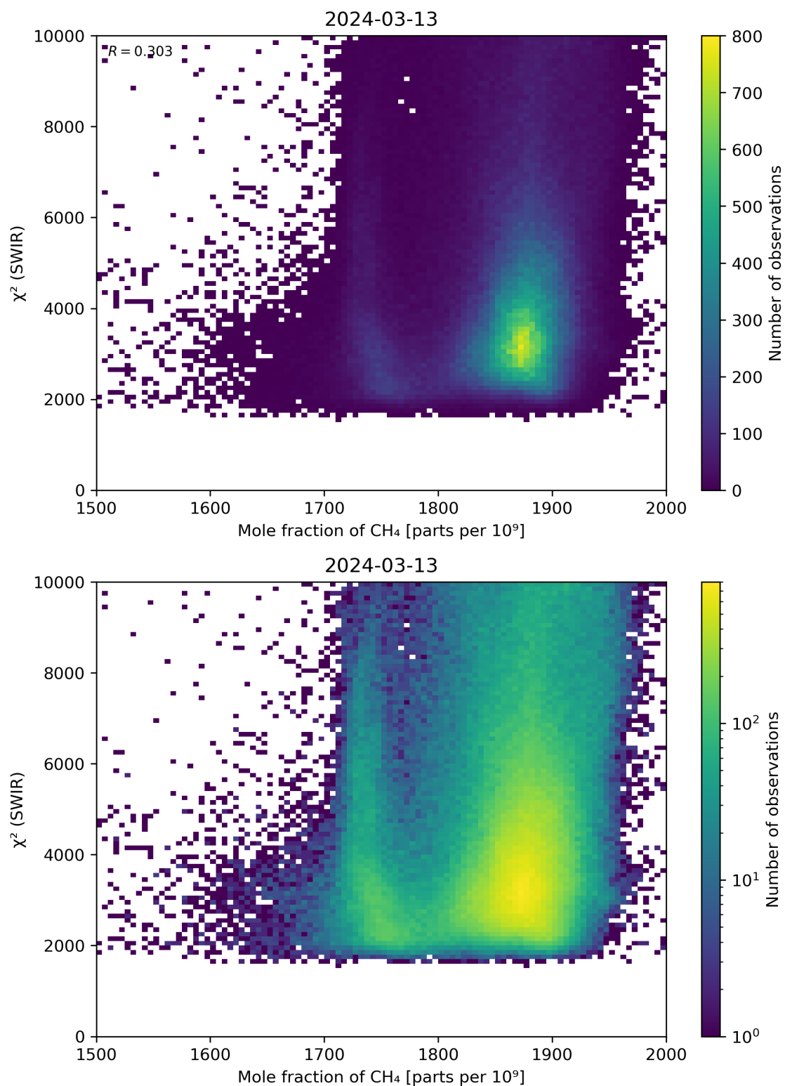
Figure 71: Scatter density plot of “Mole fraction of \text{CH}_4 ” against “ \chi^2 (SWIR)” for 2024-03-12 to 2024-03-14.
