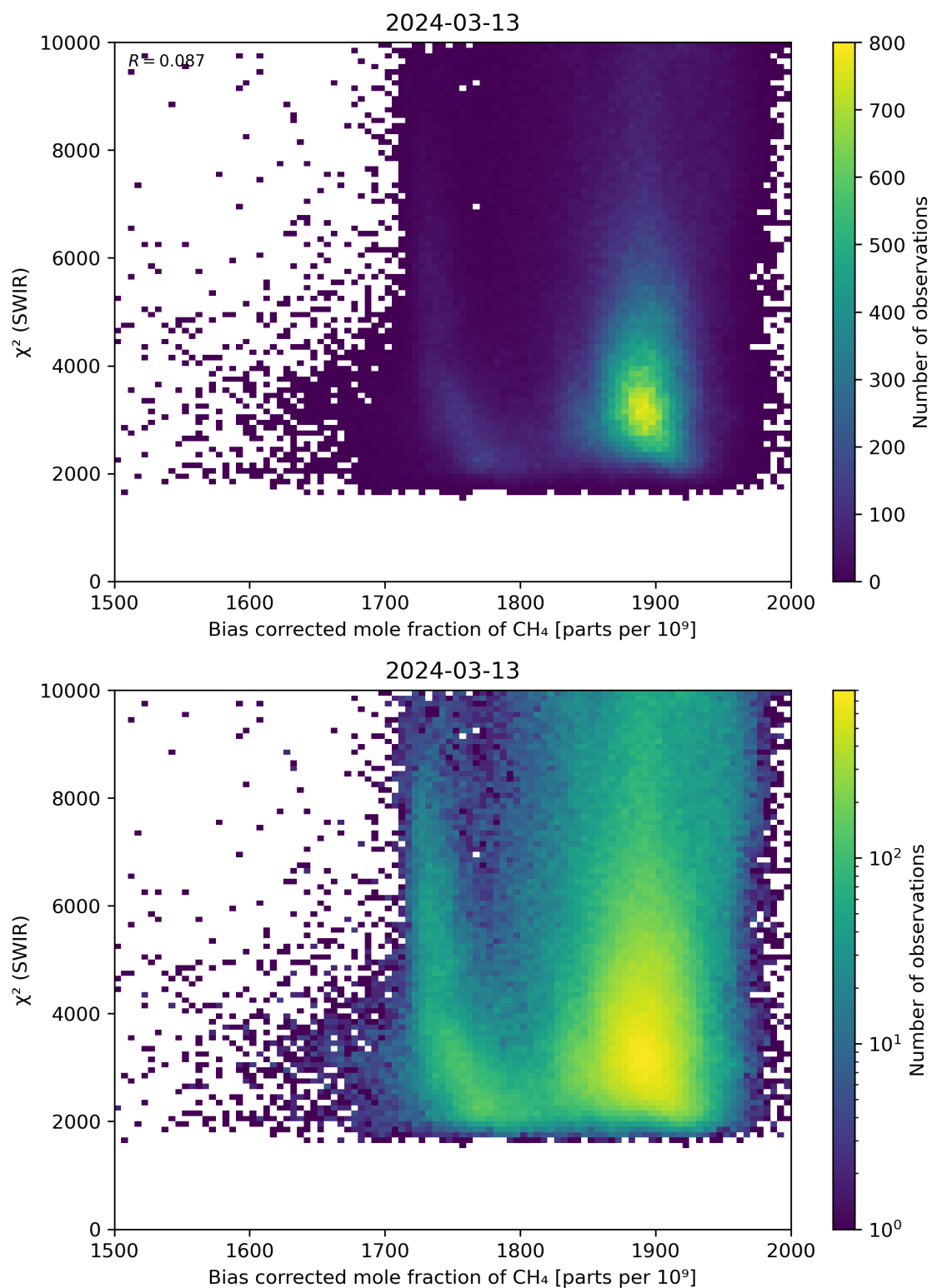
Figure 64: Scatter density plot of “Bias corrected mole fraction of CH 4 ” against “ \chi^2 (SWIR)” for 2024-03-12 to 2024-03-14.
