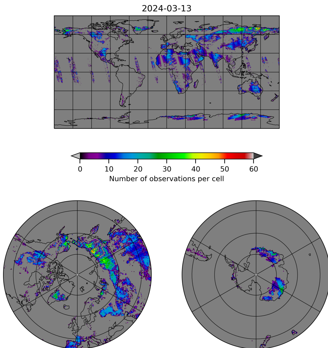
Figure 10: Map of the number of observations for 2024-03-12 to 2024-03-14
