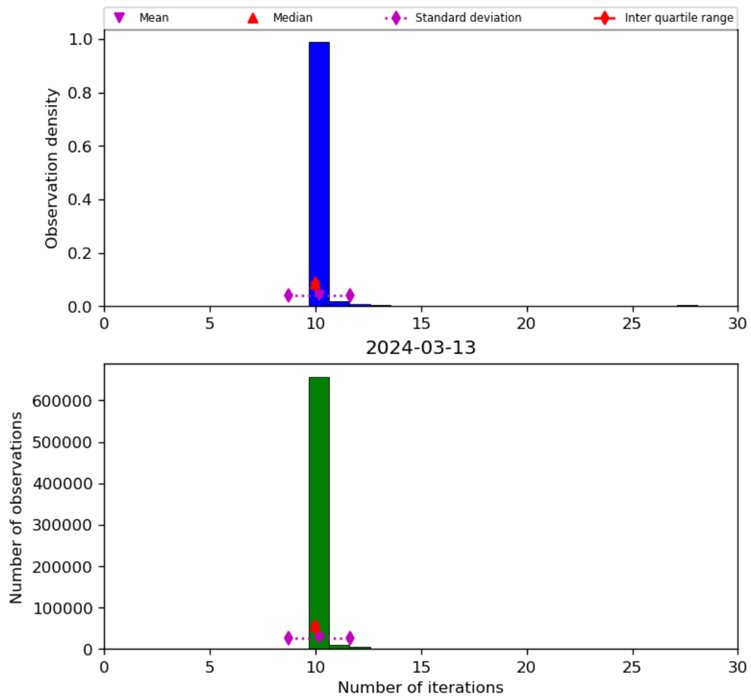
Figure 31: Histogram of “Number of iterations” for 2024-03-12 to 2024-03-14
