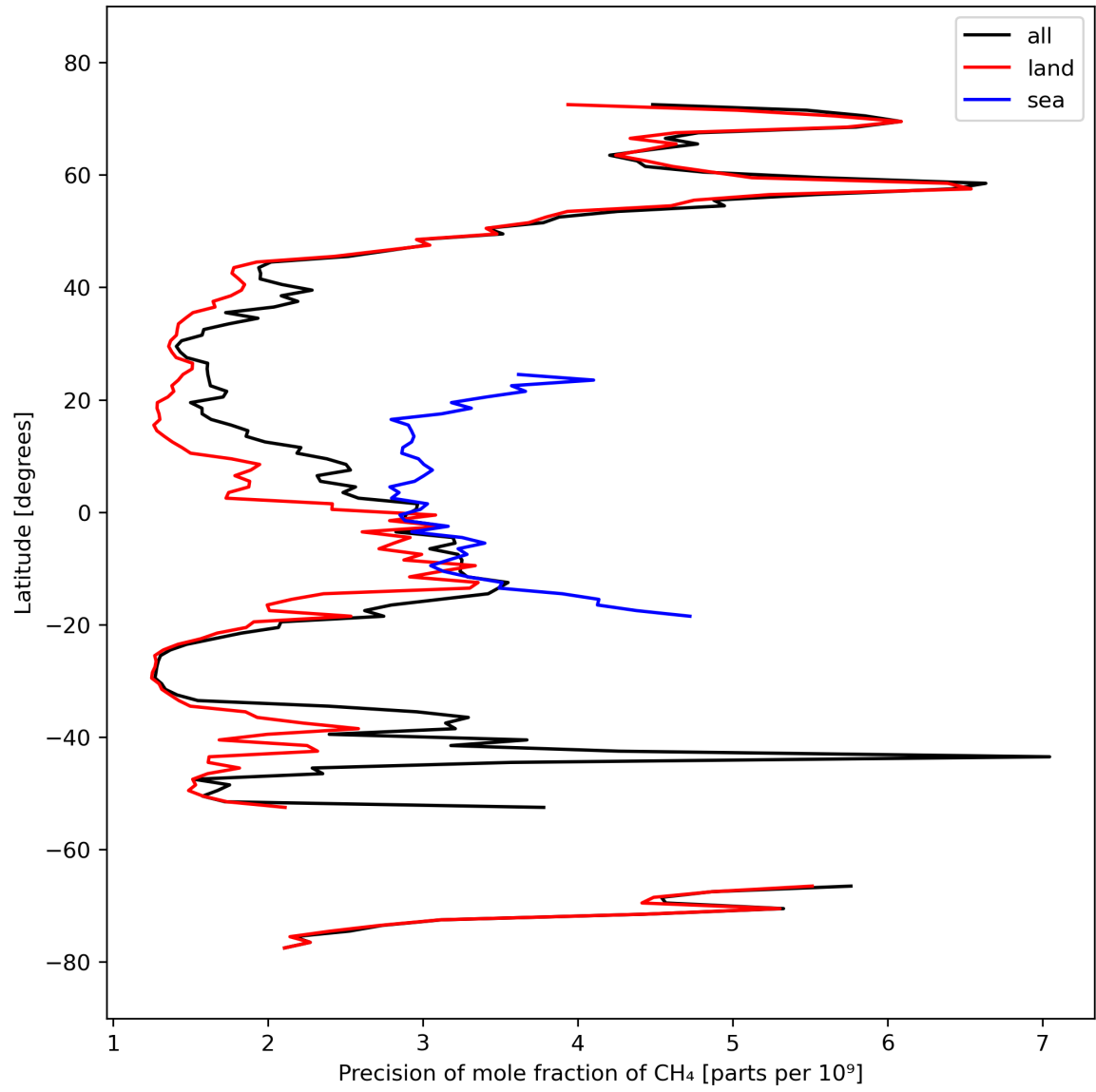
Figure 13: Zonal average of “Precision of mole fraction of CH 4 ” for 2024-03-12 to 2024-03-14.
