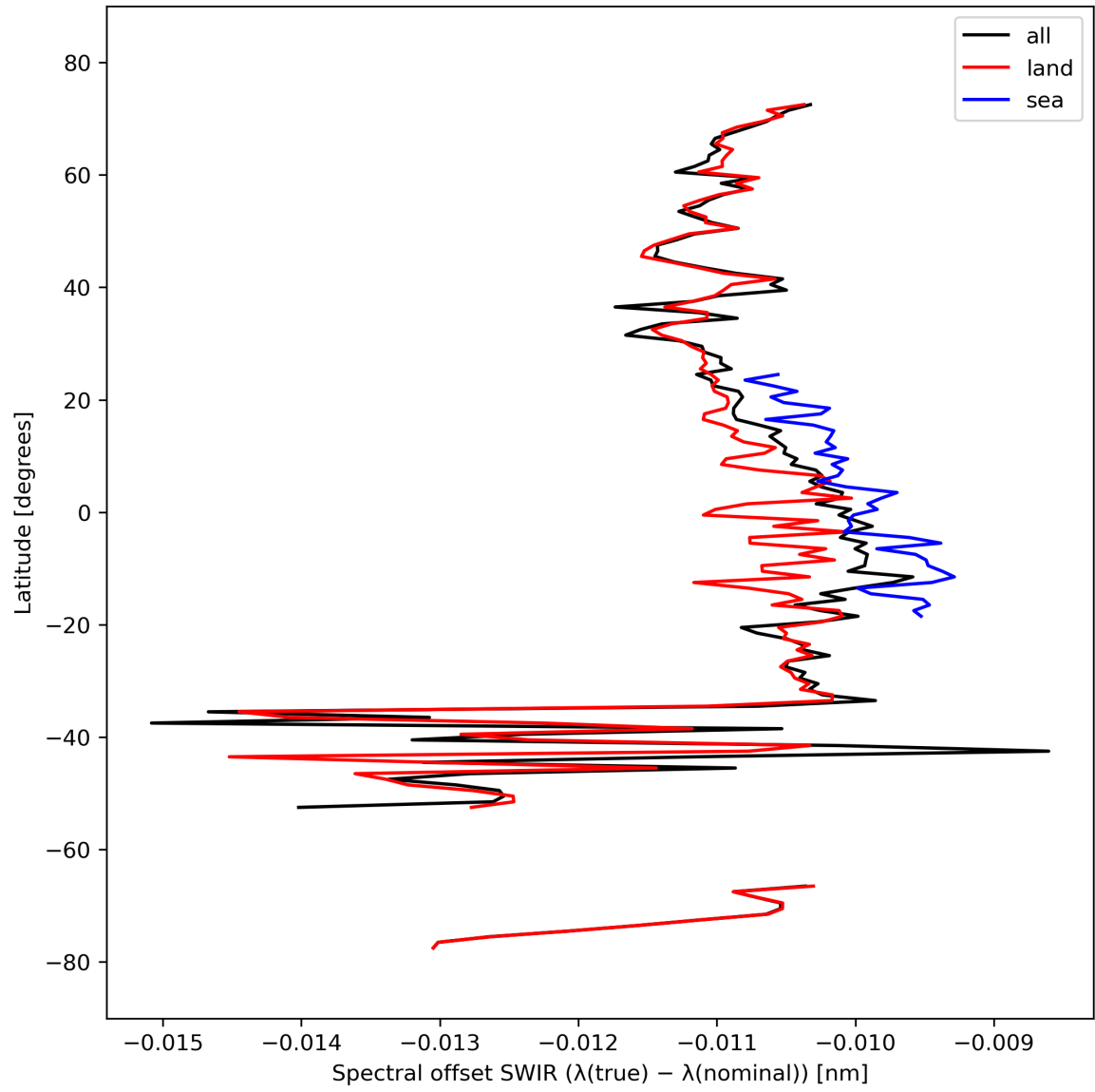
Figure 16: Zonal average of “Spectral offset SWIR ( \lambda(\text{true}) - \lambda(\text{nominal}) )” for 2024-03-12 to 2024-03-14.
