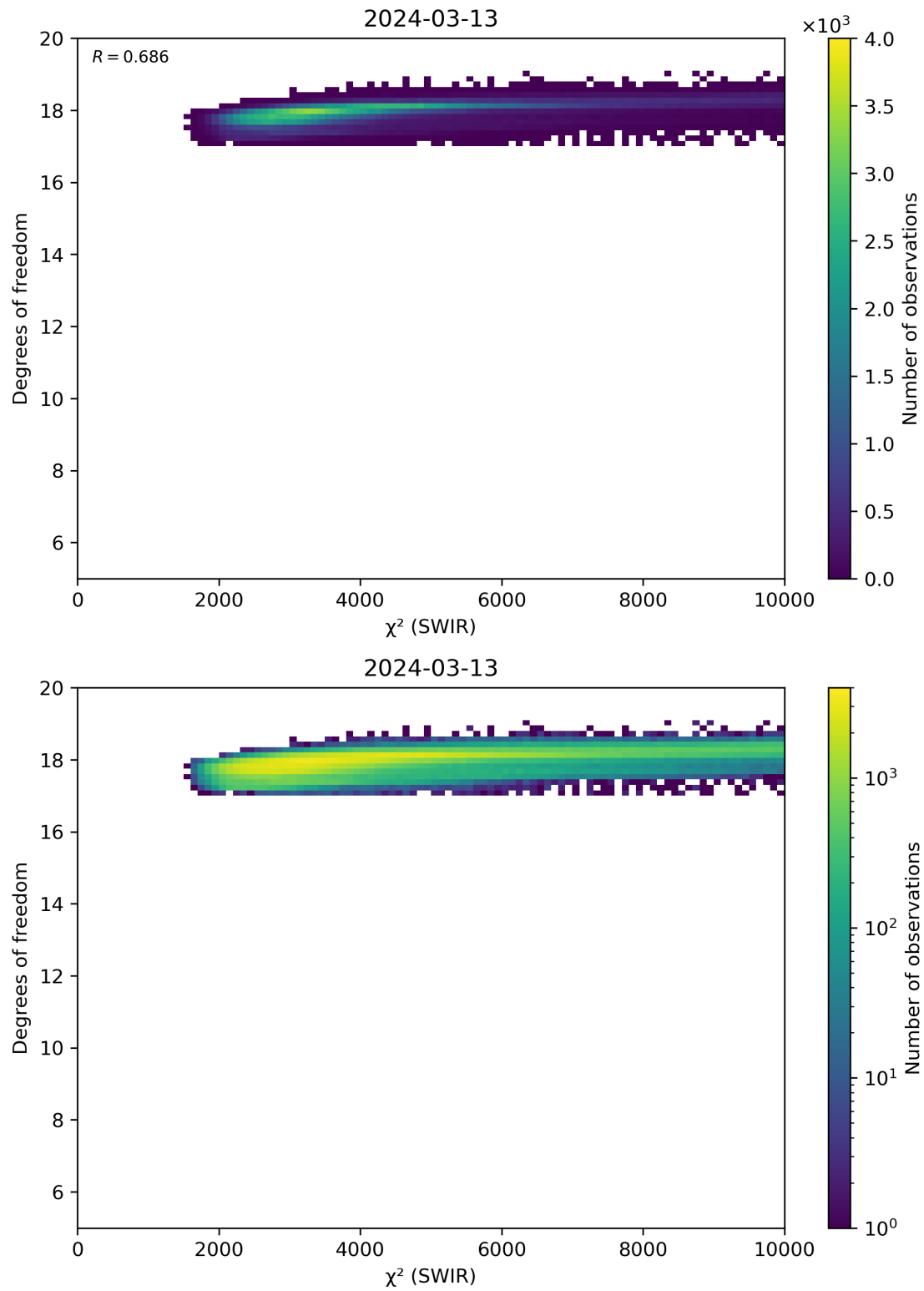
Figure 48: Scatter density plot of “ \chi^2 (SWIR)” against “Degrees of freedom” for 2024-03-12 to 2024-03-14.
