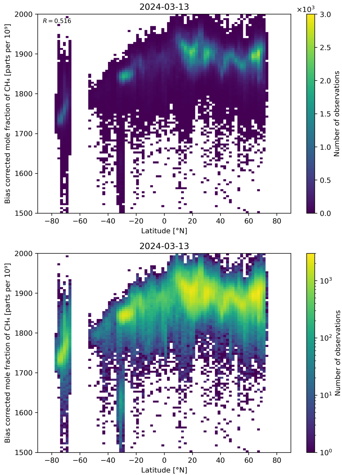
Figure 58: Scatter density plot of “Latitude” against “Bias corrected mole fraction of \text{CH}_4 ” for 2024-03-12 to 2024-03-14.
