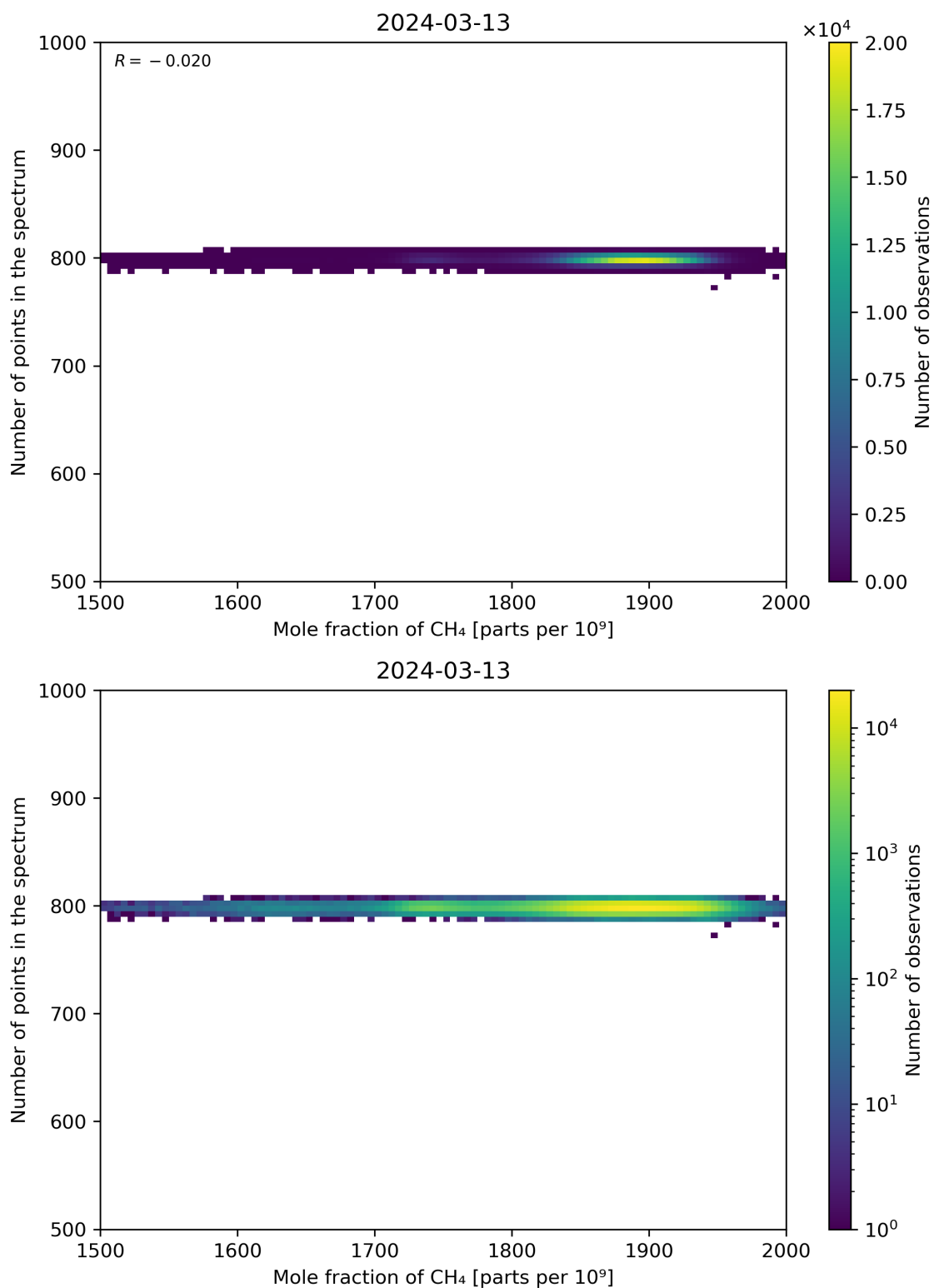
Figure 77: Scatter density plot of “Mole fraction of CH 4 ” against “Number of points in the spectrum” for 2024-03-12 to 2024-03-14.
