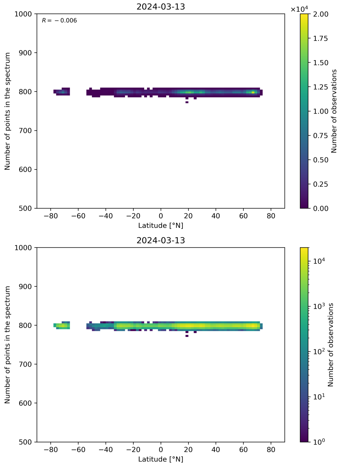
Figure 61: Scatter density plot of “Latitude” against “Number of points in the spectrum” for 2024-03-12 to 2024-03-14.
