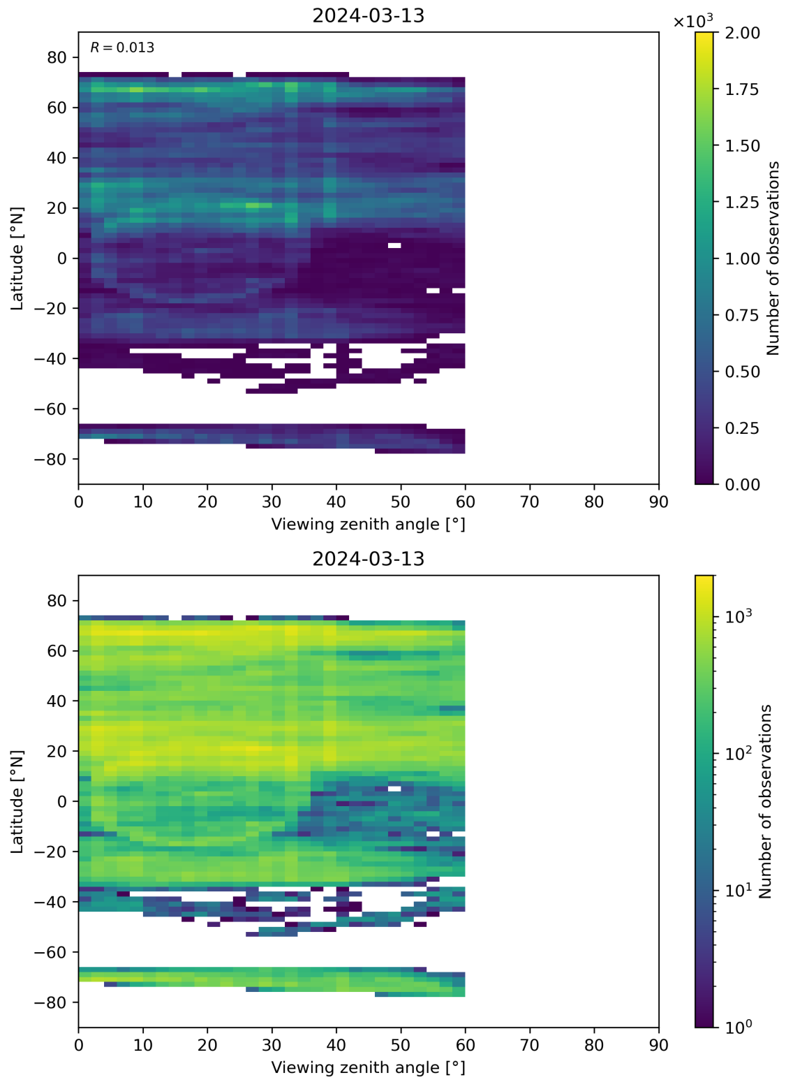
Figure 109: Scatter density plot of “Viewing zenith angle” against “Latitude” for 2024-03-12 to 2024-03-14.
