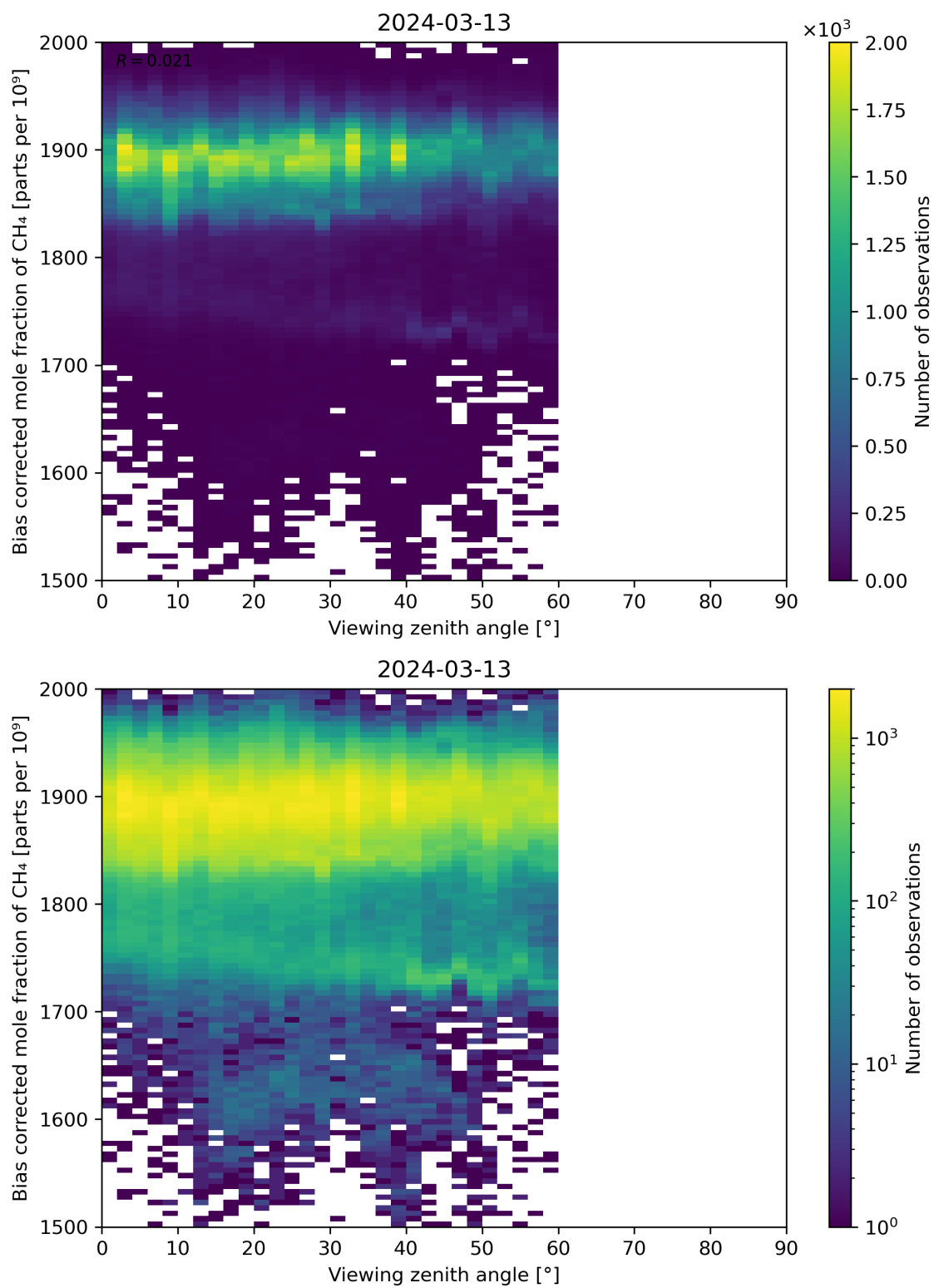
Figure 111: Scatter density plot of “Viewing zenith angle” against “Bias corrected mole fraction of CH 4 ” for 2024-03-12 to 2024-03-14.
