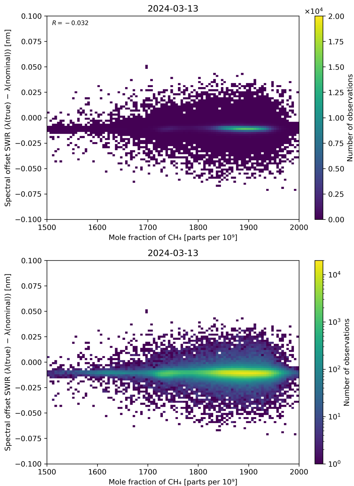
Figure 86: Scatter density plot of “Mole fraction of CH 4 ” against “Spectral offset SWIR ( \lambda(\text{true}) - \lambda(\text{nominal}) )” for 2024-03-12 to 2024-03-14.
