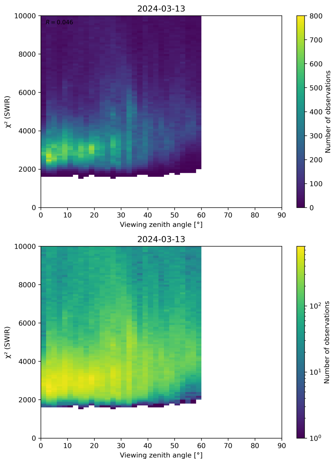
Figure 106: Scatter density plot of “Viewing zenith angle” against “ \chi^2 (SWIR)” for 2024-03-12 to 2024-03-14.
