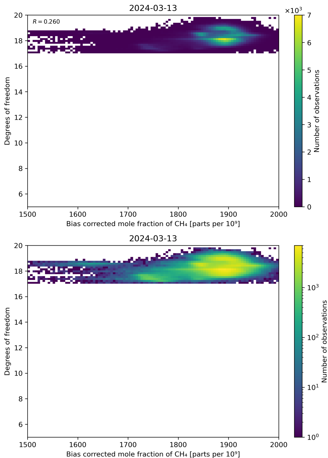
Figure 65: Scatter density plot of “Bias corrected mole fraction of CH 4 ” against “Degrees of freedom” for 2024-03-12 to 2024-03-14.
