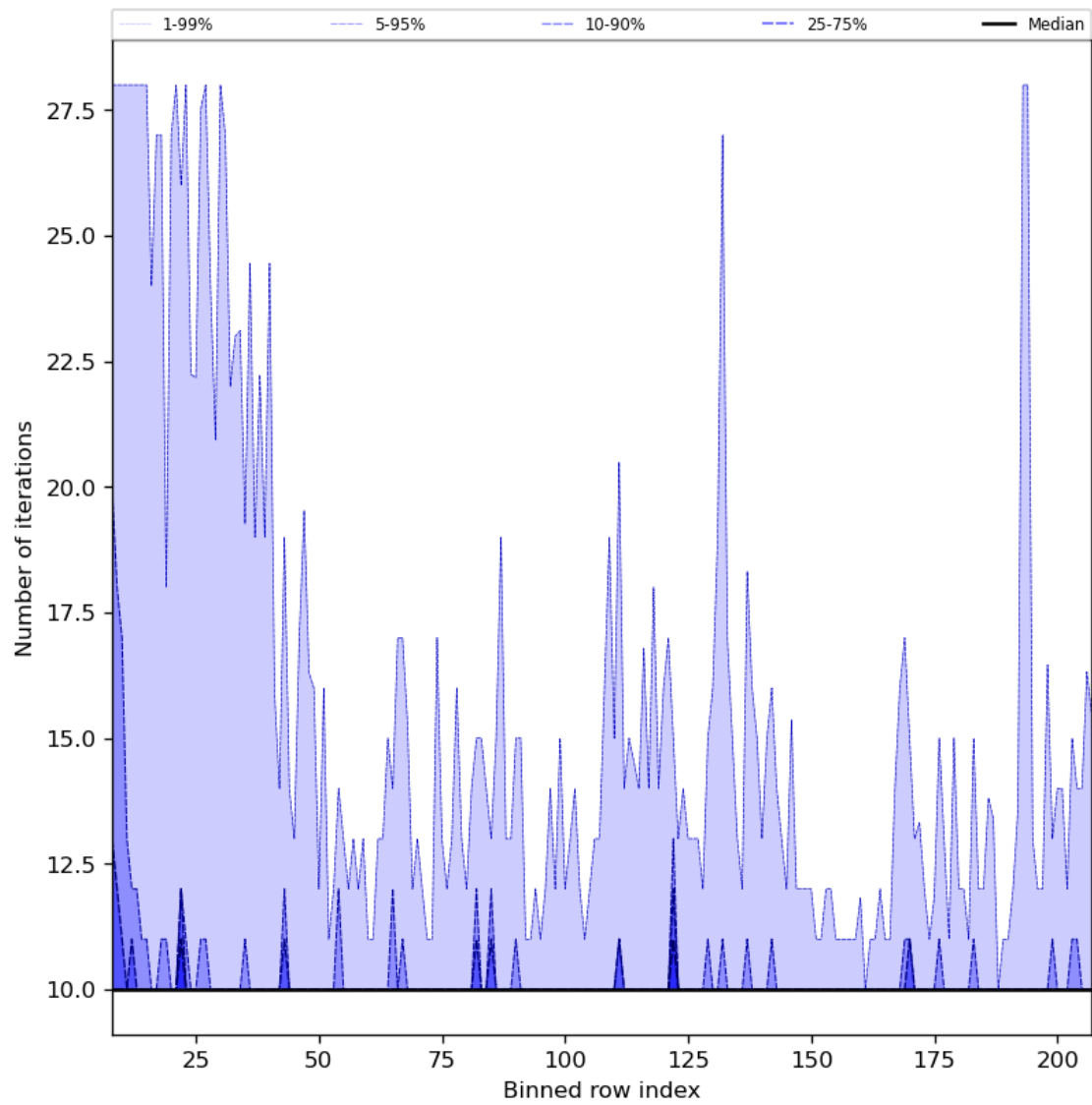
Figure 42: Along track statistics of “Number of iterations” for 2024-03-12 to 2024-03-14
