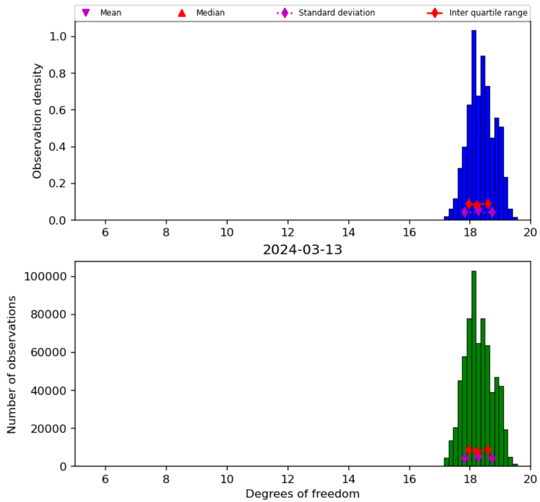
Figure 30: Histogram of “Degrees of freedom” for 2024-03-12 to 2024-03-14
