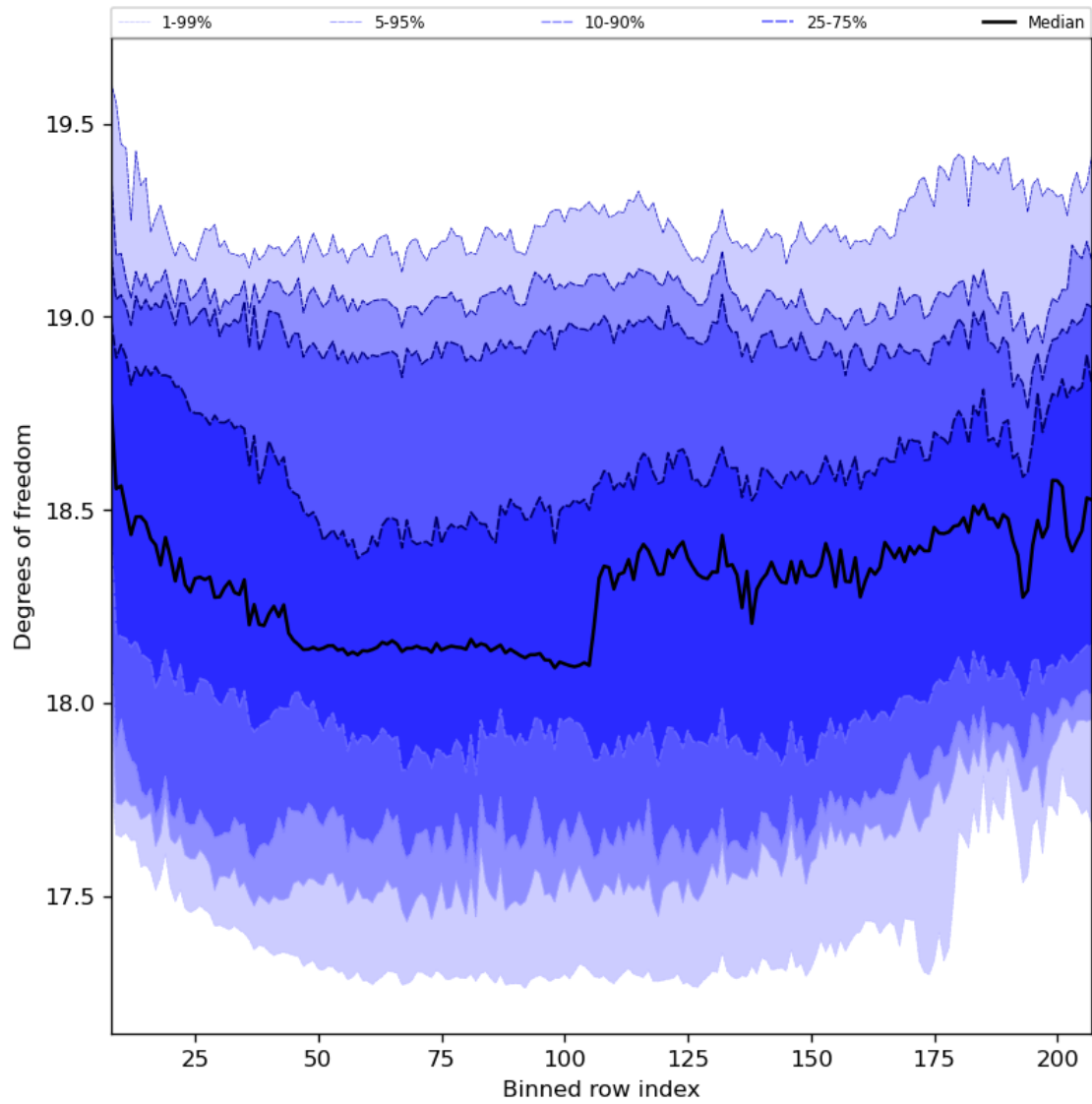
Figure 41: Along track statistics of “Degrees of freedom” for 2024-03-12 to 2024-03-14
