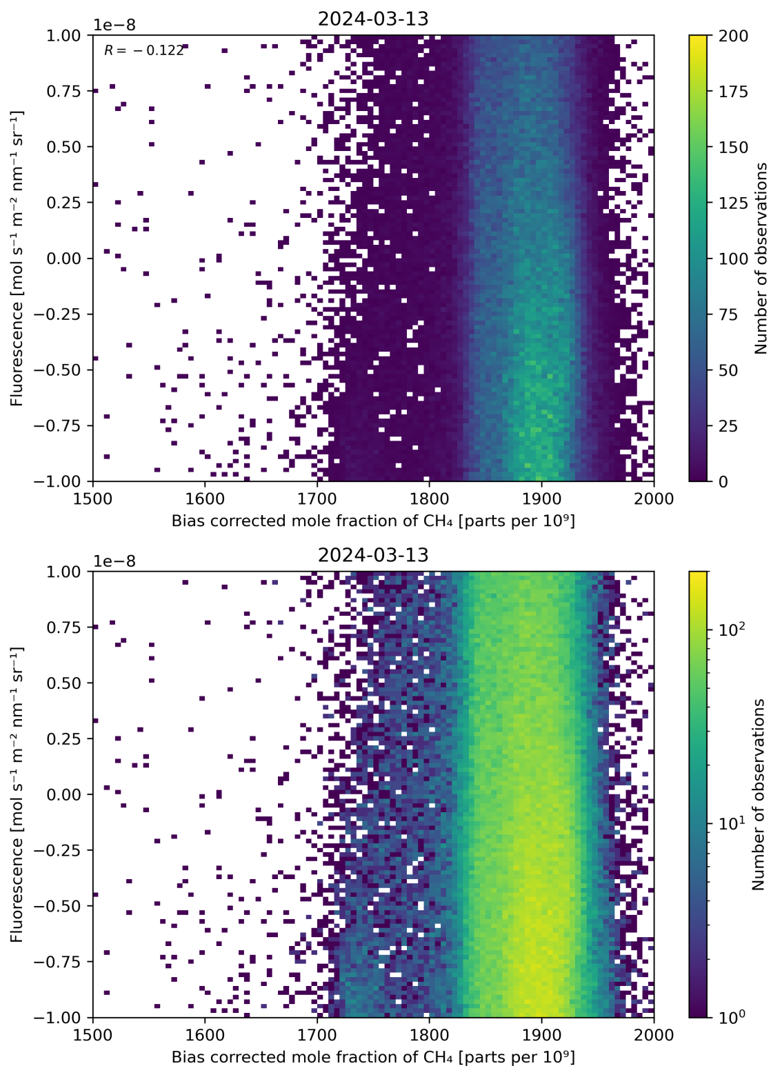
Figure 66: Scatter density plot of “Bias corrected mole fraction of \text{CH}_4 ” against “Fluorescence” for 2024-03-12 to 2024-03-14.
