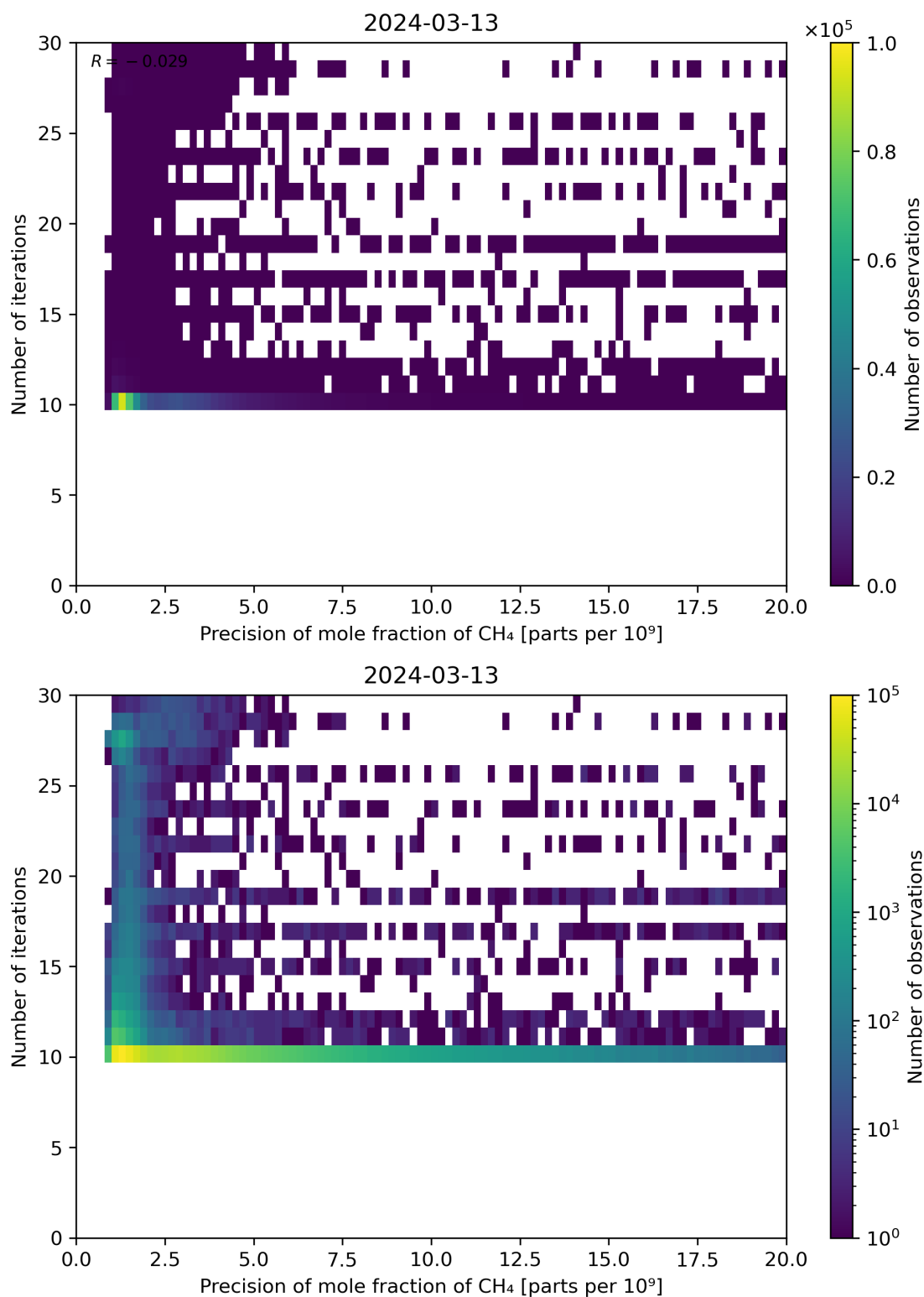
Figure 83: Scatter density plot of “Precision of mole fraction of CH 4 ” against “Number of iterations” for 2024-03-12 to 2024-03-14.
