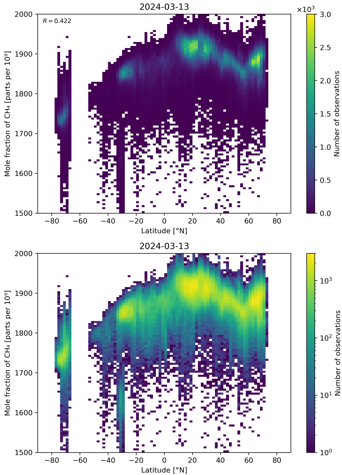
Figure 57: Scatter density plot of “Latitude” against “Mole fraction of \text{CH}_4 ” for 2024-03-12 to 2024-03-14.
