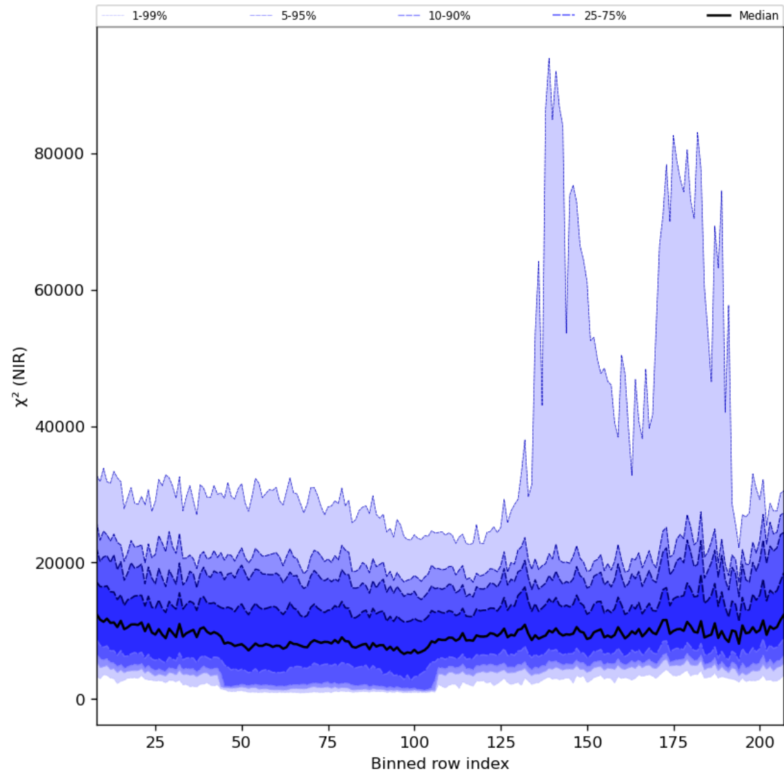
Figure 40: Along track statistics of “ \chi^2 (NIR)” for 2024-03-12 to 2024-03-14
