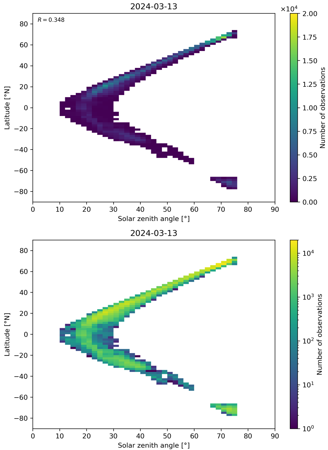
Figure 98: Scatter density plot of “Solar zenith angle” against “Latitude” for 2024-03-12 to 2024-03-14.
