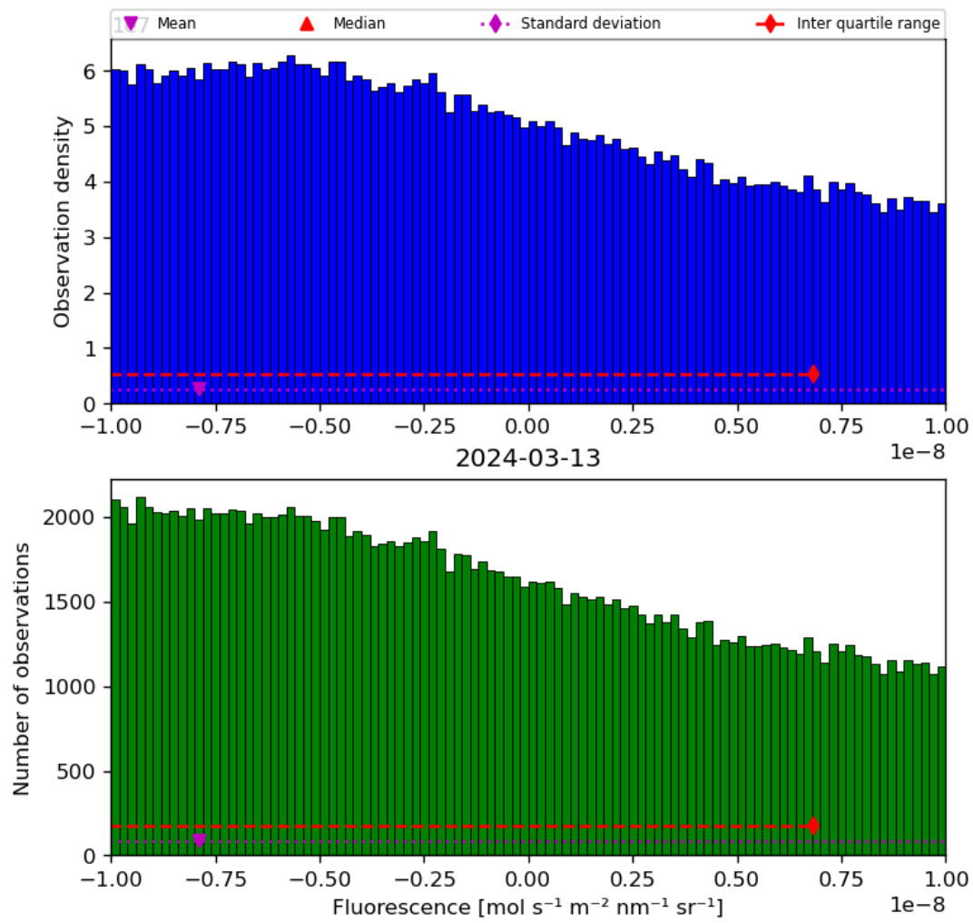
Figure 32: Histogram of “Fluorescence” for 2024-03-12 to 2024-03-14
