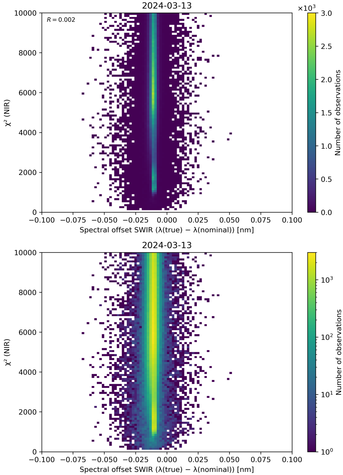
Figure 117: Scatter density plot of “Spectral offset SWIR ( \lambda(\text{true}) - \lambda(\text{nominal}) )” against “ \chi^2 (NIR)” for 2024-03-12 to 2024-03-14.
