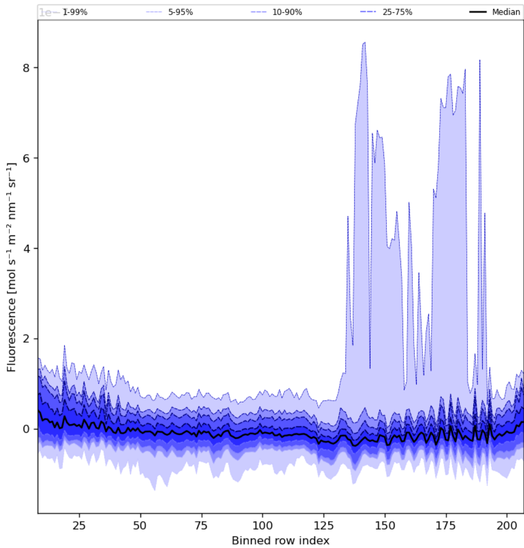
Figure 43: Along track statistics of “Fluorescence” for 2024-03-12 to 2024-03-14
