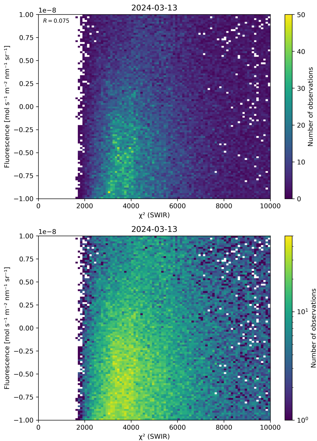
Figure 49: Scatter density plot of “ \chi^2 (SWIR)” against “Fluorescence” for 2024-03-12 to 2024-03-14.
