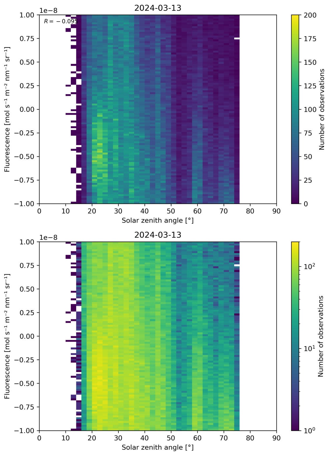
Figure 97: Scatter density plot of “Solar zenith angle” against “Fluorescence” for 2024-03-12 to 2024-03-14.
