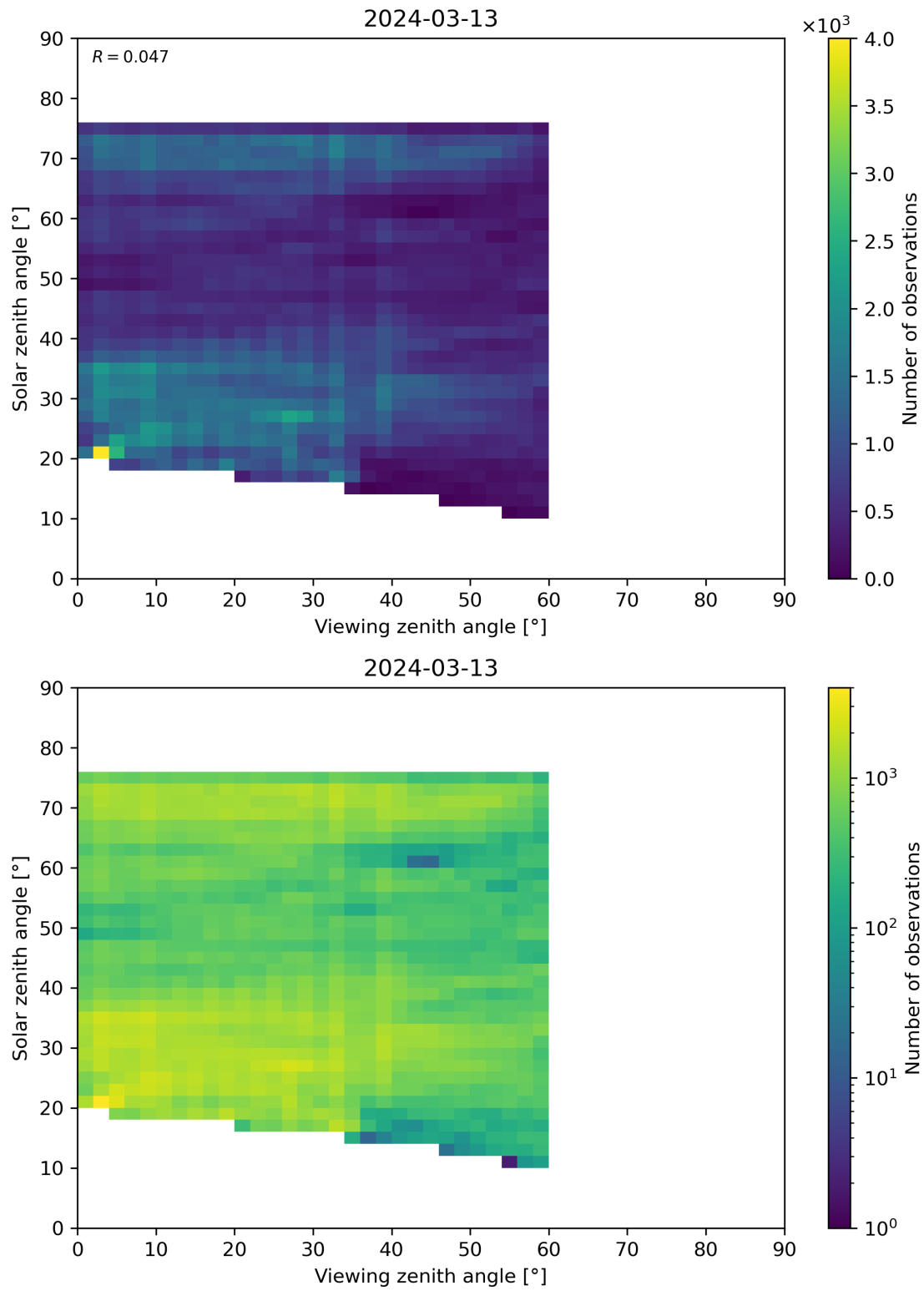
Figure 115: Scatter density plot of “Viewing zenith angle” against “Solar zenith angle” for 2024-03-12 to 2024-03-14.
