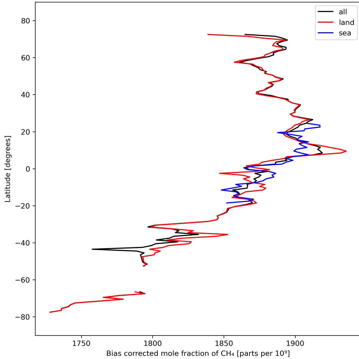
Figure 14: Zonal average of “Bias corrected mole fraction of CH 4 ” for 2024-03-12 to 2024-03-14.
