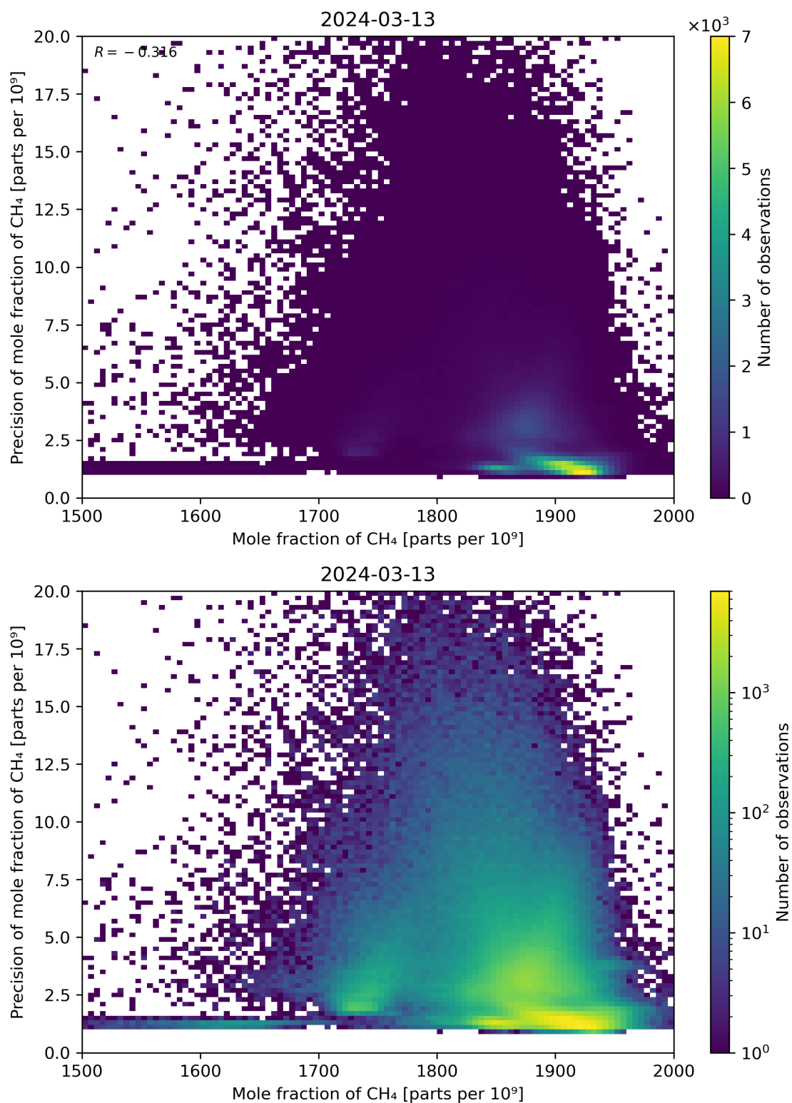
Figure 75: Scatter density plot of “Mole fraction of CH 4 ” against “Precision of mole fraction of CH 4 ” for 2024-03-12 to 2024-03-14.
