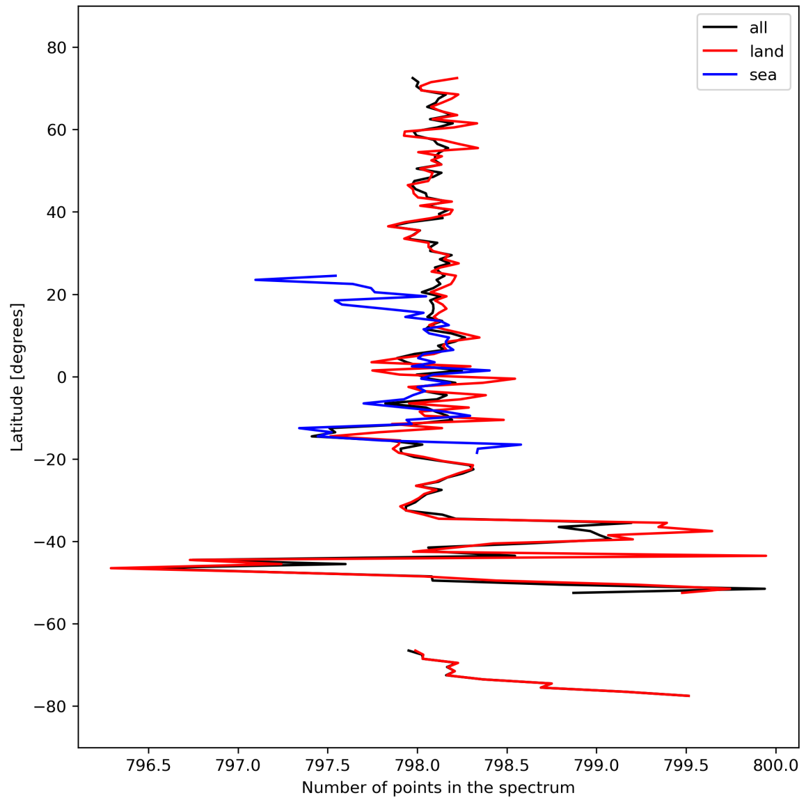
Figure 15: Zonal average of “Number of points in the spectrum” for 2024-03-12 to 2024-03-14.
