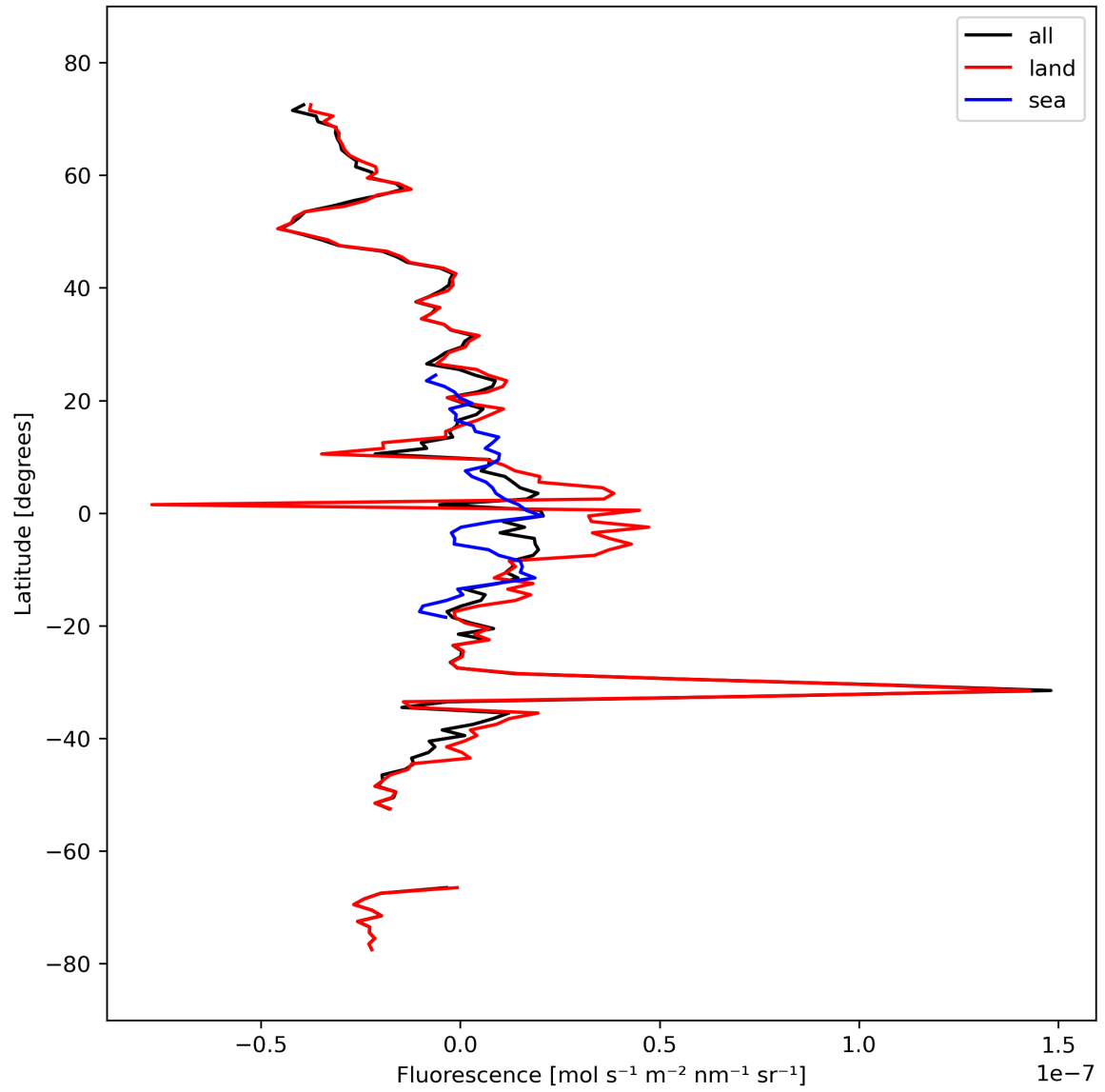
Figure 21: Zonal average of “Fluorescence” for 2024-03-12 to 2024-03-14.
