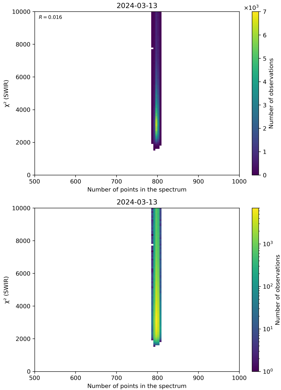
Figure 89: Scatter density plot of “Number of points in the spectrum” against “ \chi^2 (SWIR)” for 2024-03-12 to 2024-03-14.
