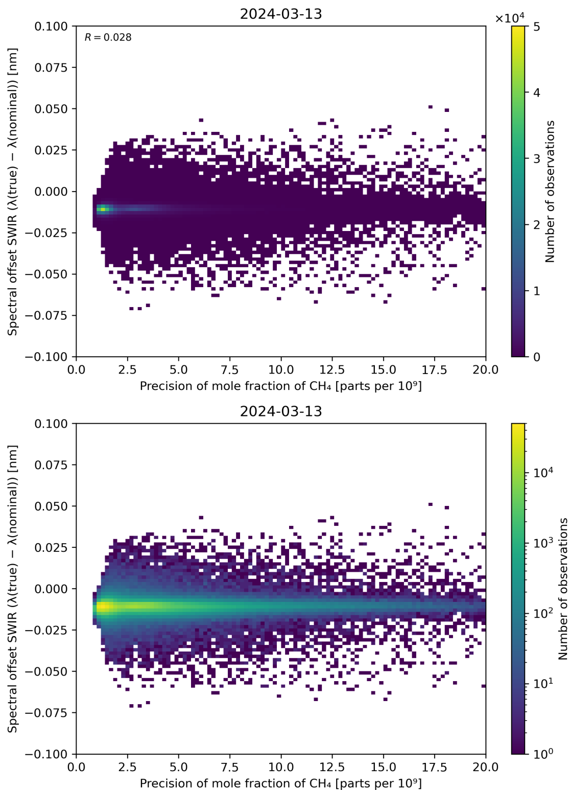
Figure 85: Scatter density plot of “Precision of mole fraction of CH 4 ” against “Spectral offset SWIR ( \lambda(\text{true}) - \lambda(\text{nominal}) )” for 2024-03-12 to 2024-03-14.
