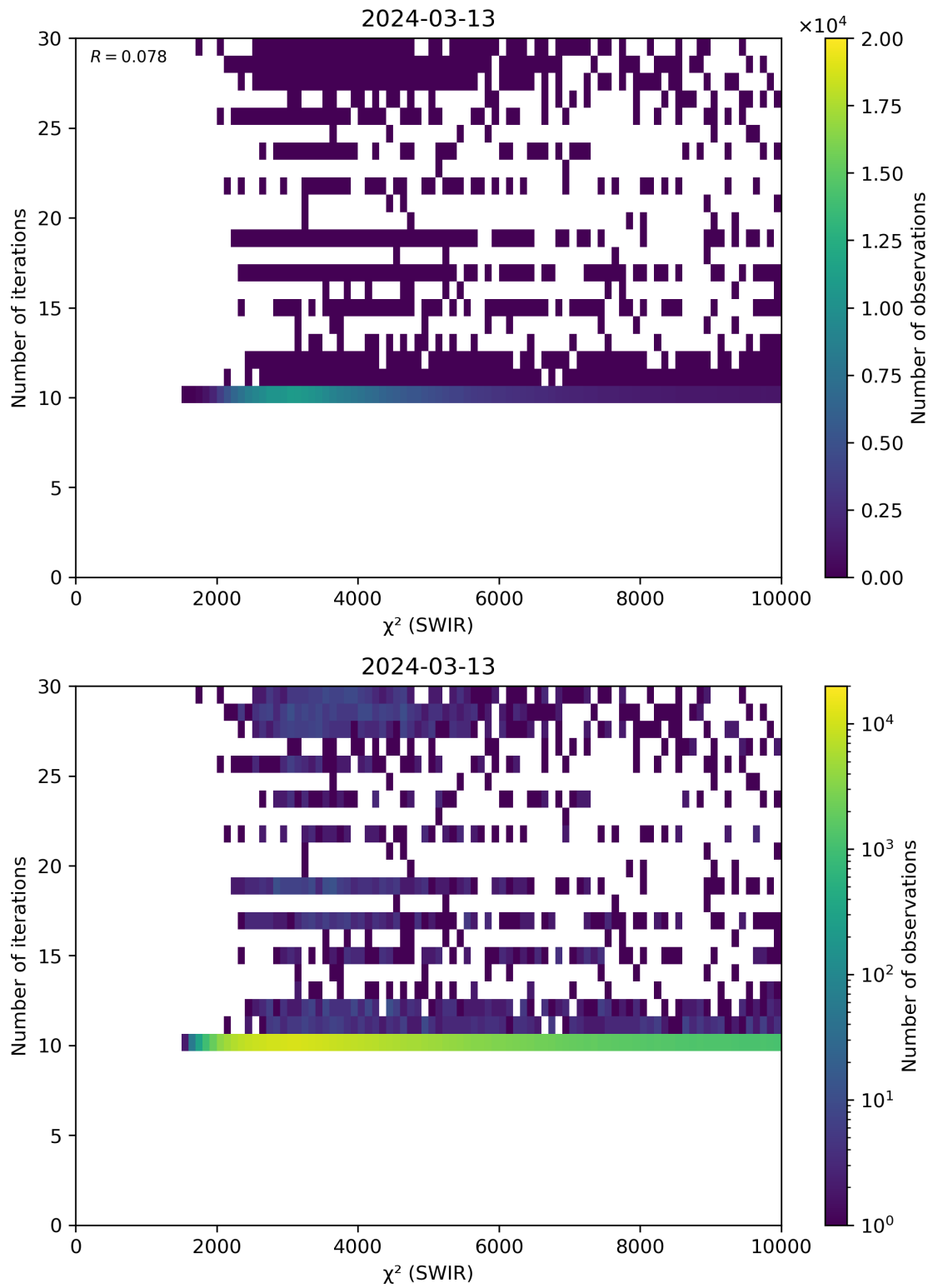
Figure 50: Scatter density plot of “ \chi^2 (SWIR)” against “Number of iterations” for 2024-03-12 to 2024-03-14.
