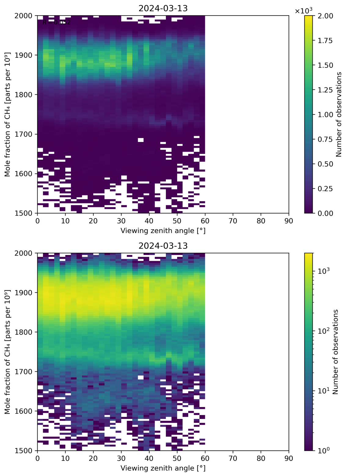
Figure 110: Scatter density plot of “Viewing zenith angle” against “Mole fraction of CH 4 ” for 2024-03-12 to 2024-03-14.
