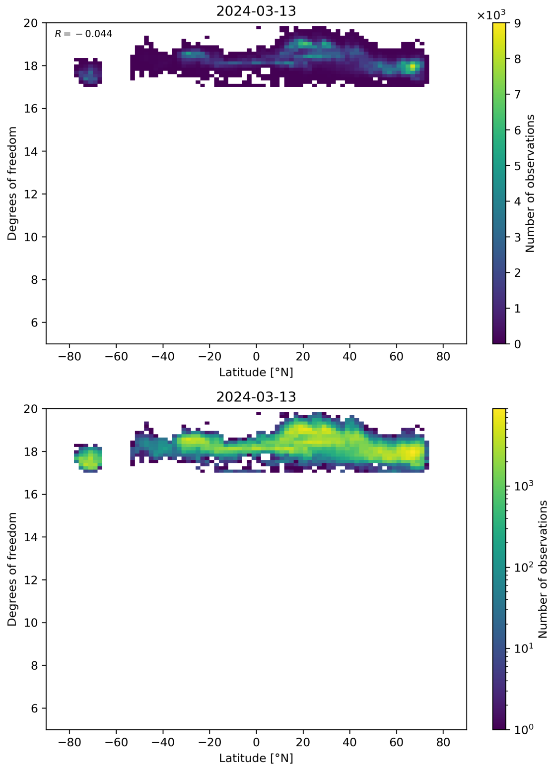
Figure 55: Scatter density plot of “Latitude” against “Degrees of freedom” for 2024-03-12 to 2024-03-14.
