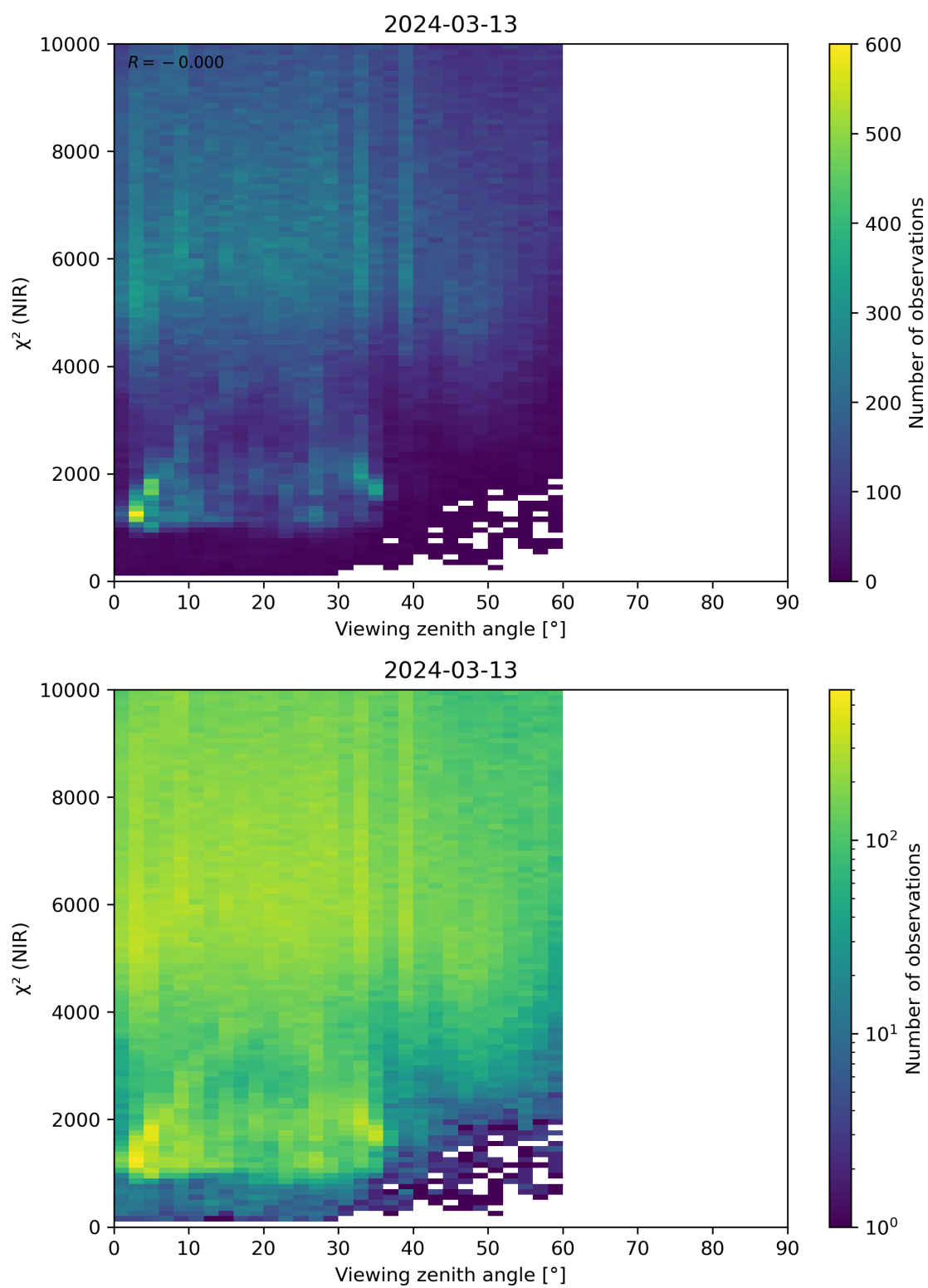
Figure 105: Scatter density plot of “Viewing zenith angle” against “ \chi^2 (NIR)” for 2024-03-12 to 2024-03-14.
