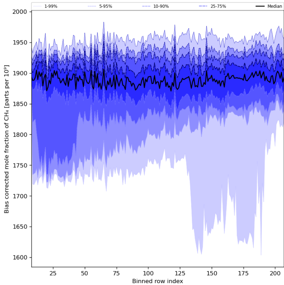
Figure 36: Along track statistics of “Bias corrected mole fraction of CH 4 ” for 2024-03-12 to 2024-03-14
