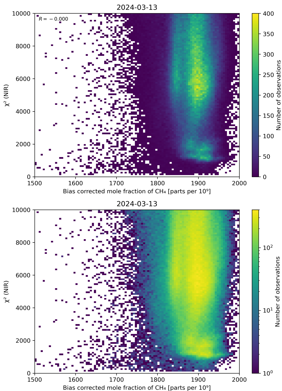
Figure 63: Scatter density plot of “Bias corrected mole fraction of \text{CH}_4 ” against “ \chi^2 (NIR)” for 2024-03-12 to 2024-03-14.
