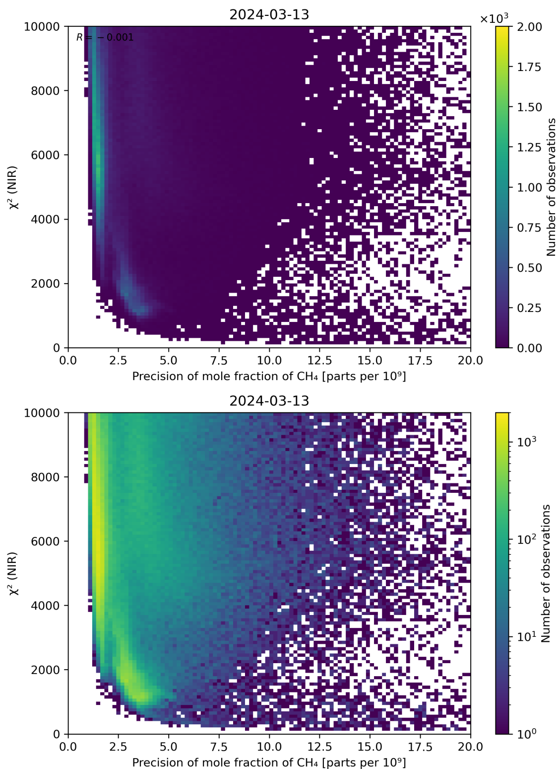
Figure 78: Scatter density plot of “Precision of mole fraction of CH 4 ” against “ \chi^2 (NIR)” for 2024-03-12 to 2024-03-14.
