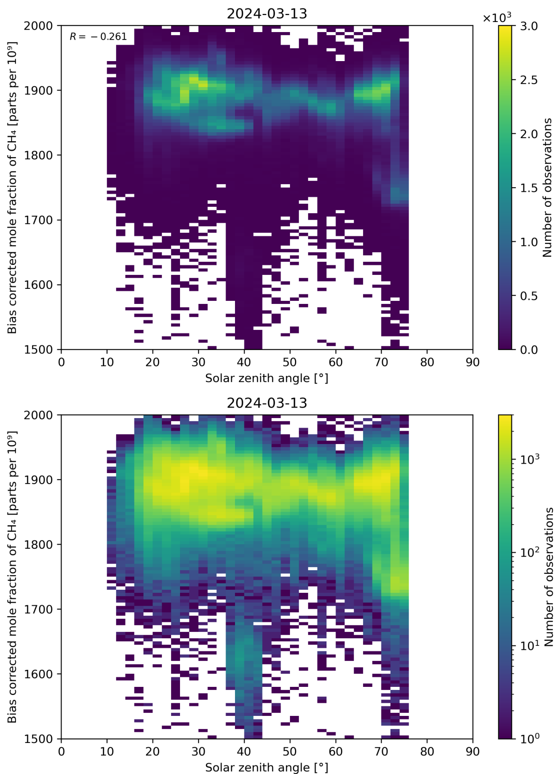
Figure 100: Scatter density plot of “Solar zenith angle” against “Bias corrected mole fraction of \text{CH}_4 ” for 2024-03-12 to 2024-03-14.
