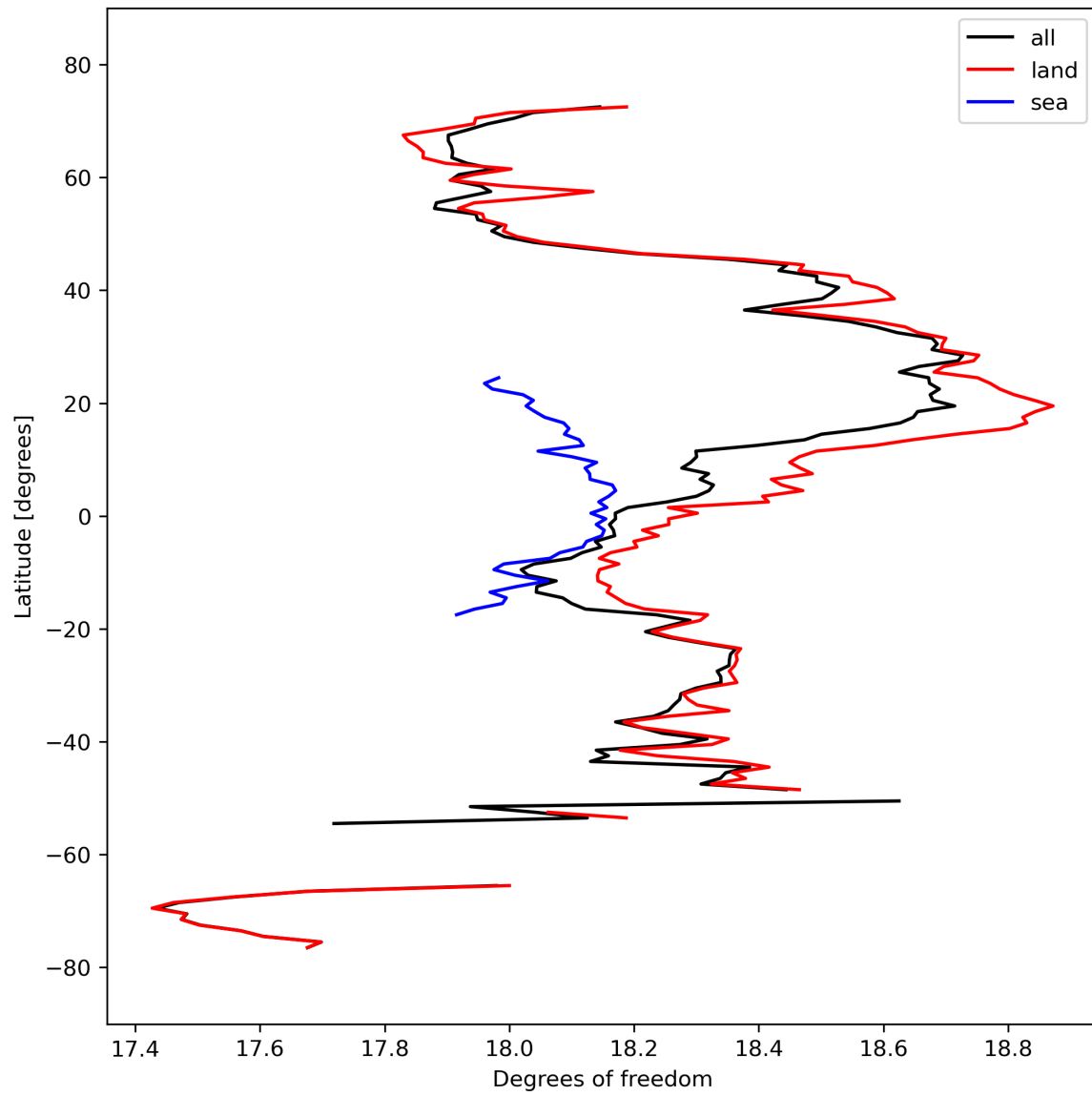
Figure 19: Zonal average of “Degrees of freedom” for 2024-03-14 to 2024-03-15.
