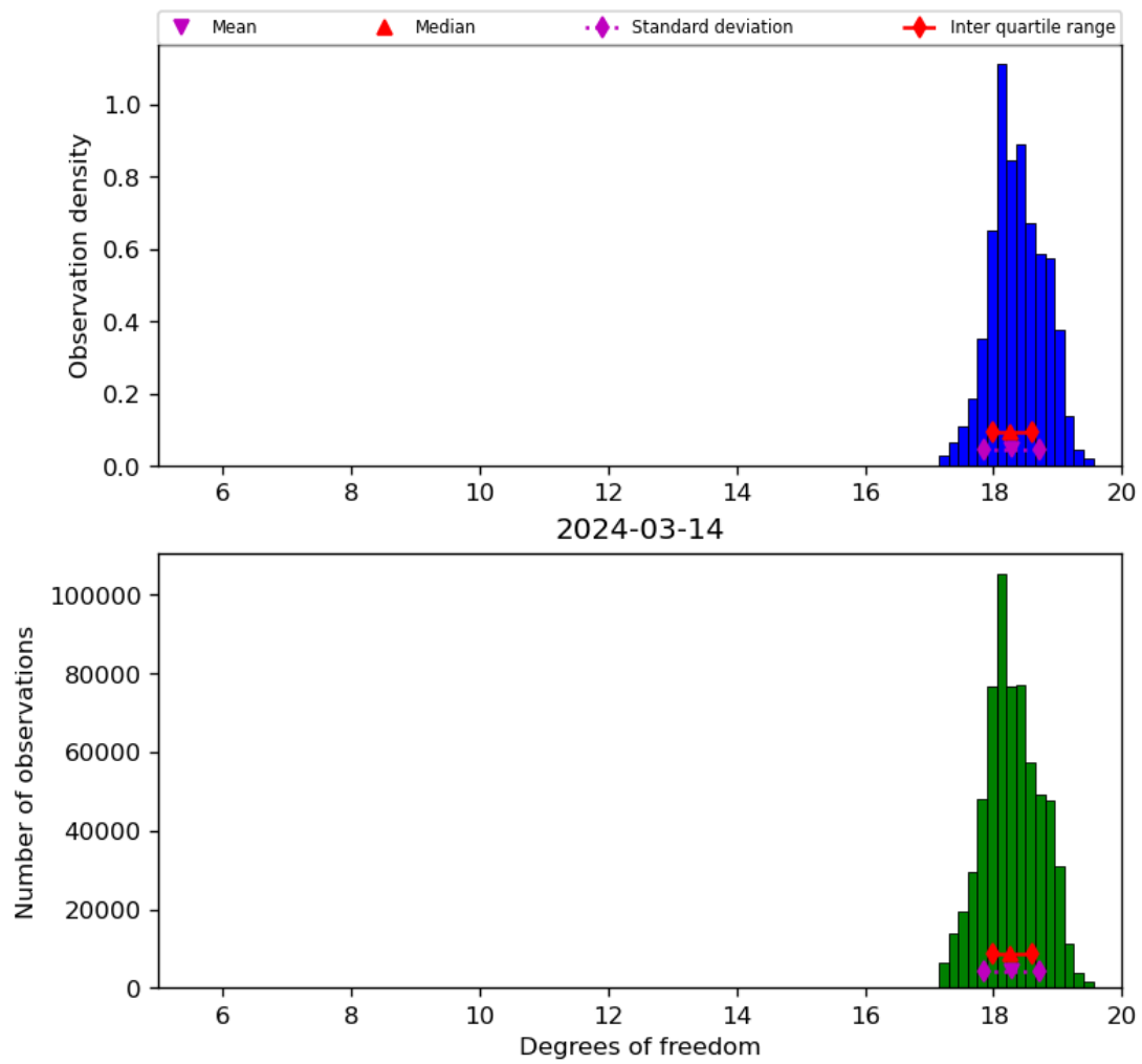
Figure 30: Histogram of “Degrees of freedom” for 2024-03-14 to 2024-03-15
