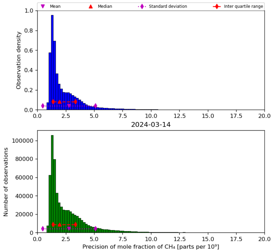
Figure 24: Histogram of “Precision of mole fraction of CH 4 ” for 2024-03-14 to 2024-03-15
