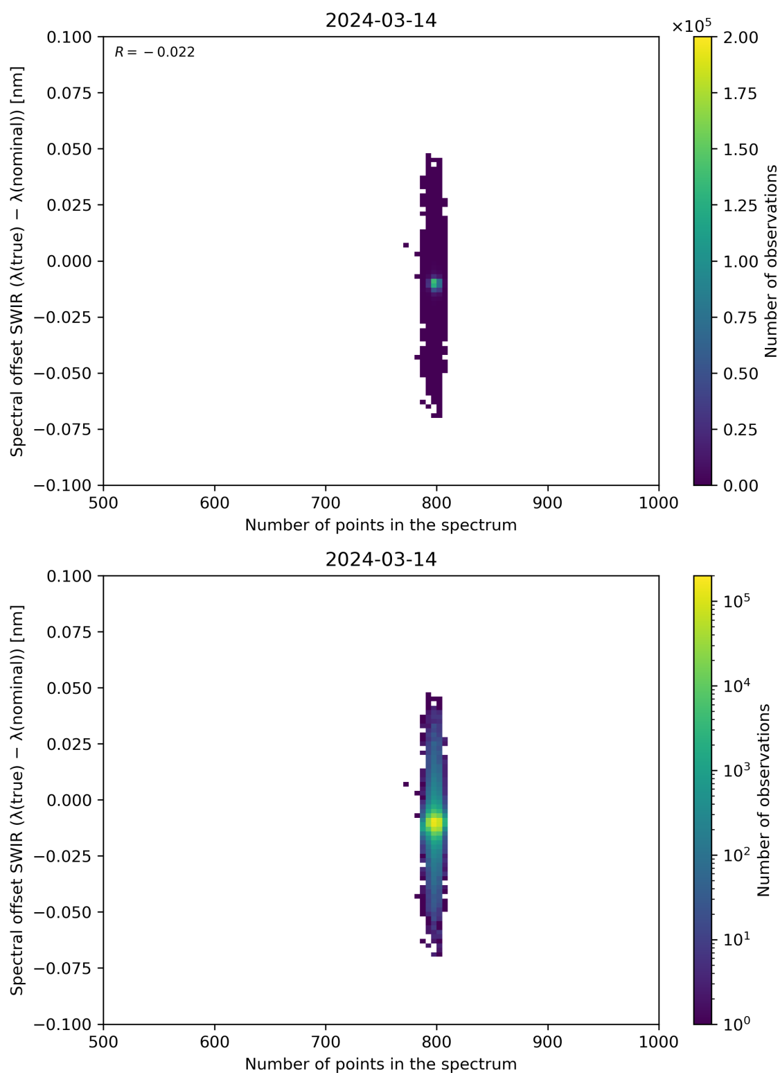
Figure 93: Scatter density plot of “Number of points in the spectrum” against “Spectral offset SWIR ( \lambda(\text{true}) - \lambda(\text{nominal}) )” for 2024-03-14 to 2024-03-15.
