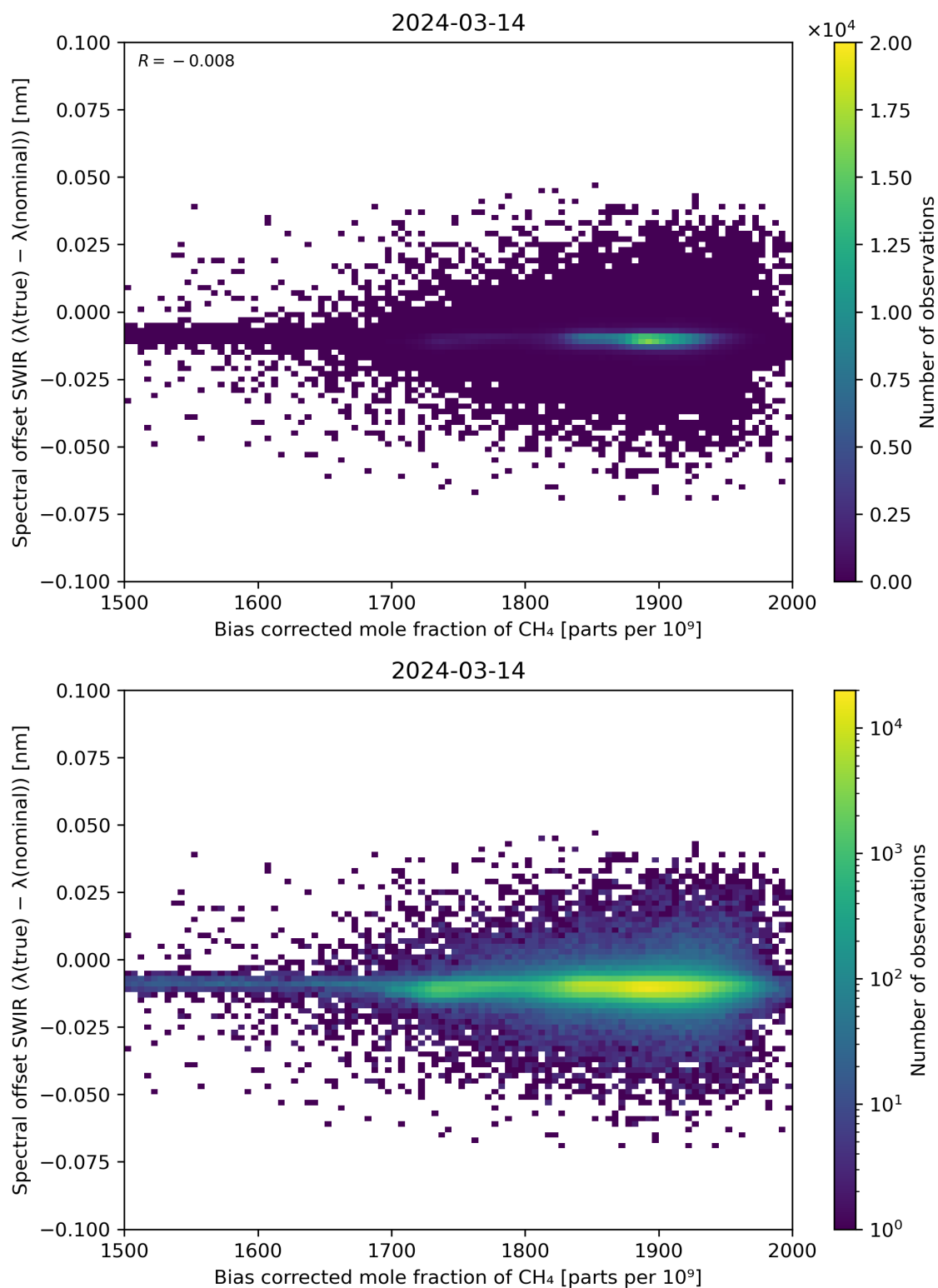
Figure 69: Scatter density plot of “Bias corrected mole fraction of \text{CH}_4 ” against “Spectral offset SWIR ( \lambda(\text{true}) - \lambda(\text{nominal}) )” for 2024-03-14 to 2024-03-15.
