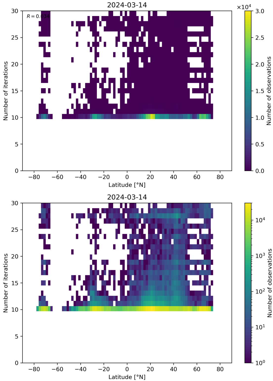
Figure 60: Scatter density plot of “Latitude” against “Number of iterations” for 2024-03-14 to 2024-03-15.
