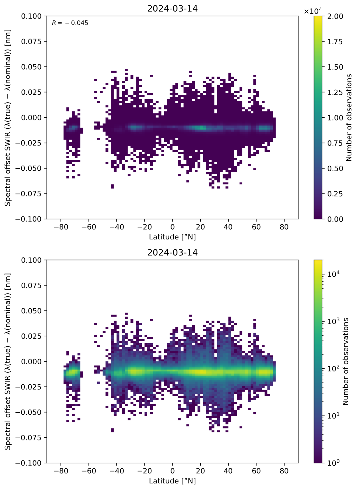
Figure 62: Scatter density plot of “Latitude” against “Spectral offset SWIR ( \lambda(\text{true}) - \lambda(\text{nominal}) )” for 2024-03-14 to 2024-03-15.
