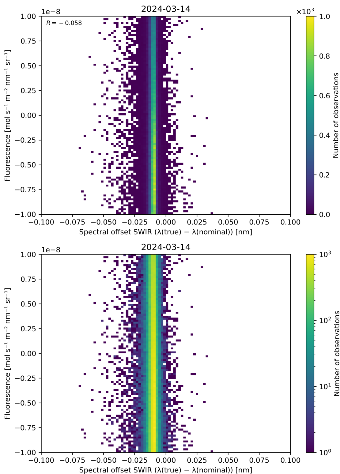
Figure 120: Scatter density plot of “Spectral offset SWIR ( \lambda(\text{true}) - \lambda(\text{nominal}) )” against “Fluorescence” for 2024-03-14 to 2024-03-15.
