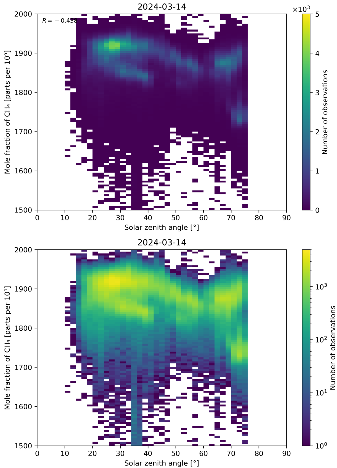
Figure 99: Scatter density plot of “Solar zenith angle” against “Mole fraction of CH 4 ” for 2024-03-14 to 2024-03-15.
