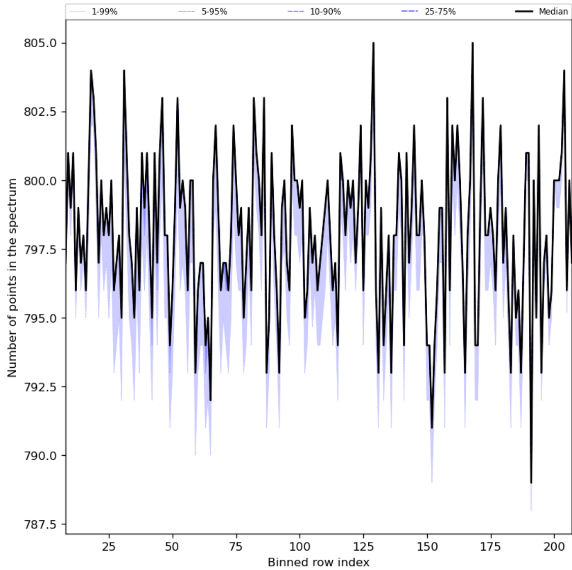
Figure 37: Along track statistics of “Number of points in the spectrum” for 2024-03-14 to 2024-03-15
