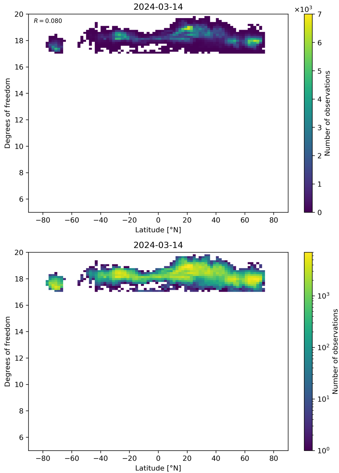
Figure 55: Scatter density plot of “Latitude” against “Degrees of freedom” for 2024-03-14 to 2024-03-15.
