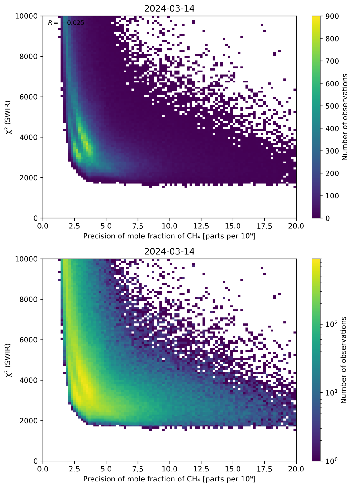
Figure 79: Scatter density plot of “Precision of mole fraction of \text{CH}_4 ” against “ \chi^2 (SWIR)” for 2024-03-14 to 2024-03-15.
