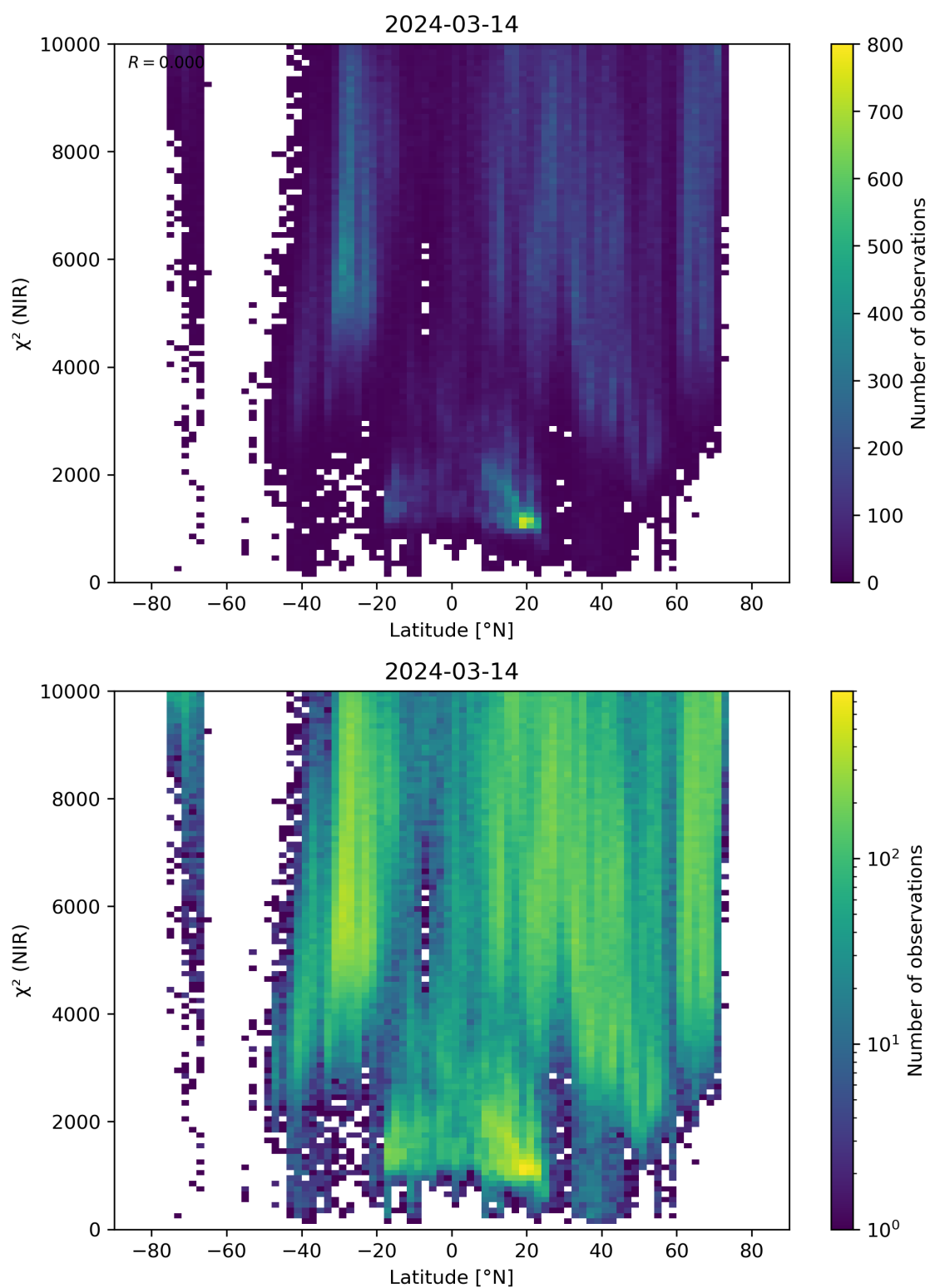
Figure 53: Scatter density plot of “Latitude” against “ \chi^2 (NIR)” for 2024-03-14 to 2024-03-15.
