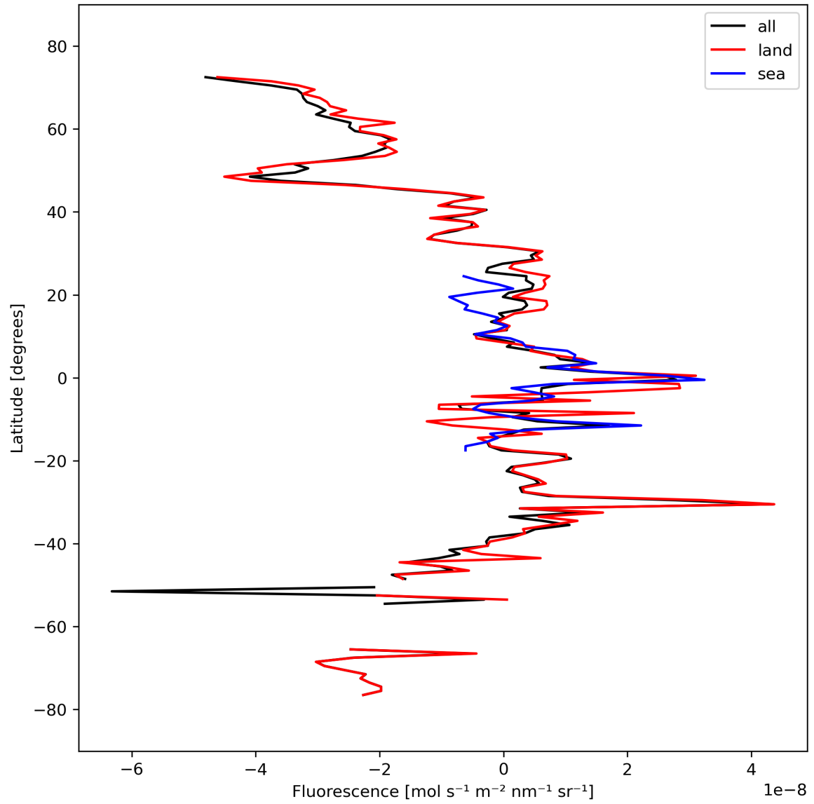
Figure 21: Zonal average of “Fluorescence” for 2024-03-14 to 2024-03-15.
