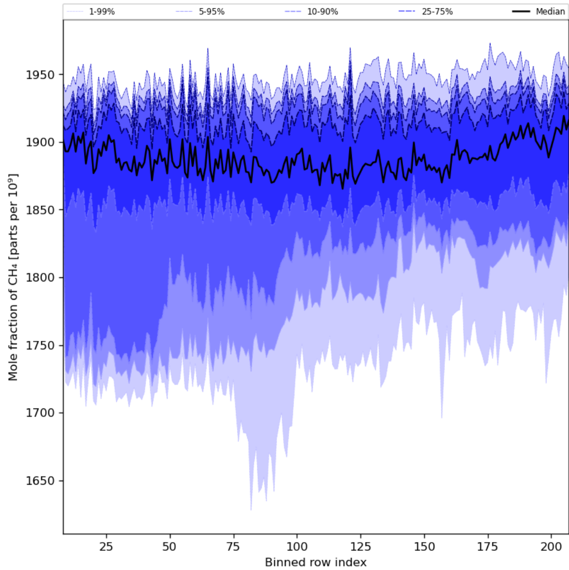
Figure 34: Along track statistics of “Mole fraction of CH 4 ” for 2024-03-14 to 2024-03-15
