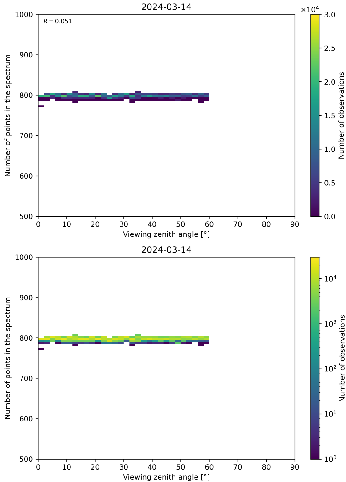
Figure 114: Scatter density plot of “Viewing zenith angle” against “Number of points in the spectrum” for 2024-03-14 to 2024-03-15.
