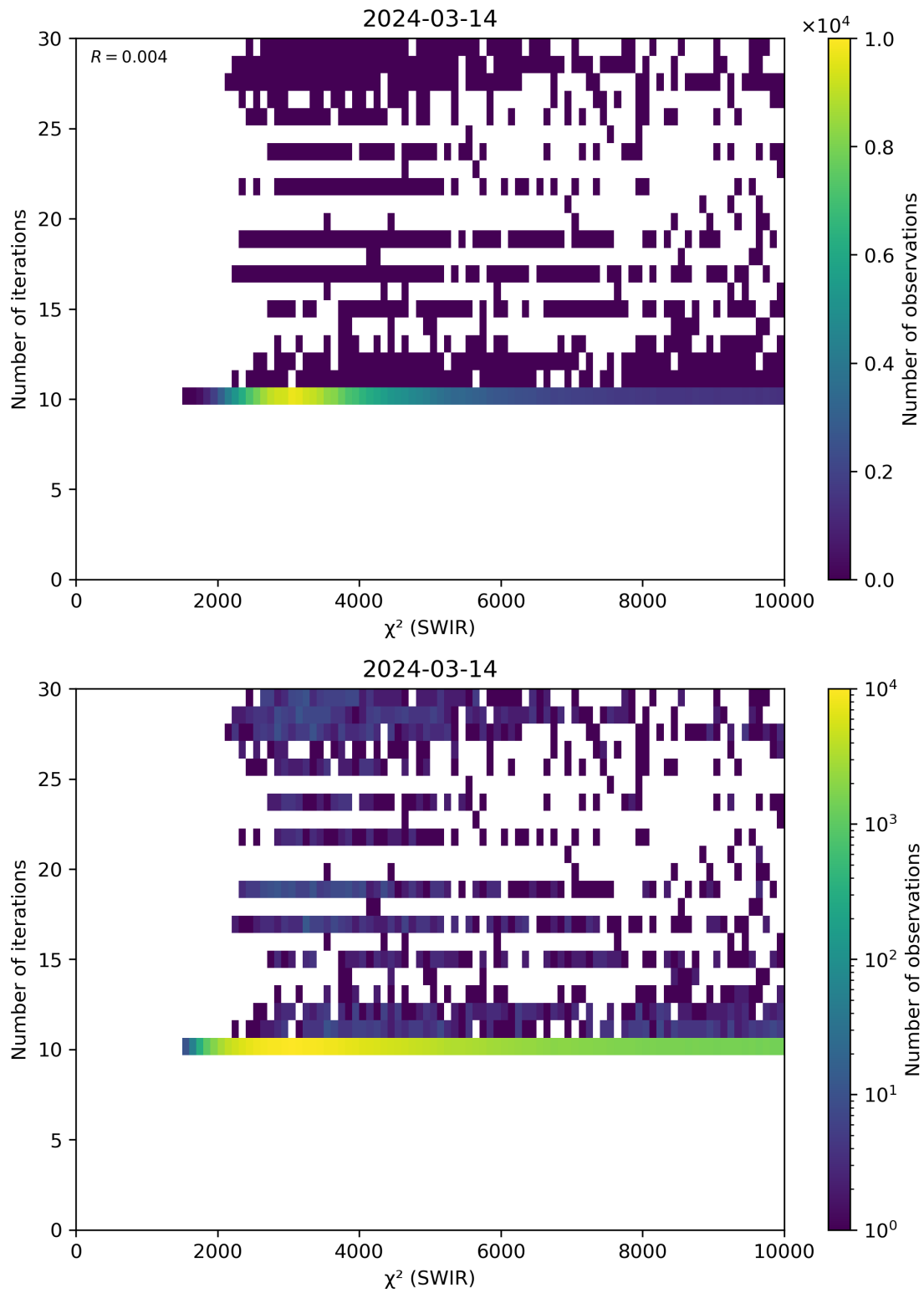
Figure 50: Scatter density plot of “ \chi^2 (SWIR)” against “Number of iterations” for 2024-03-14 to 2024-03-15.
