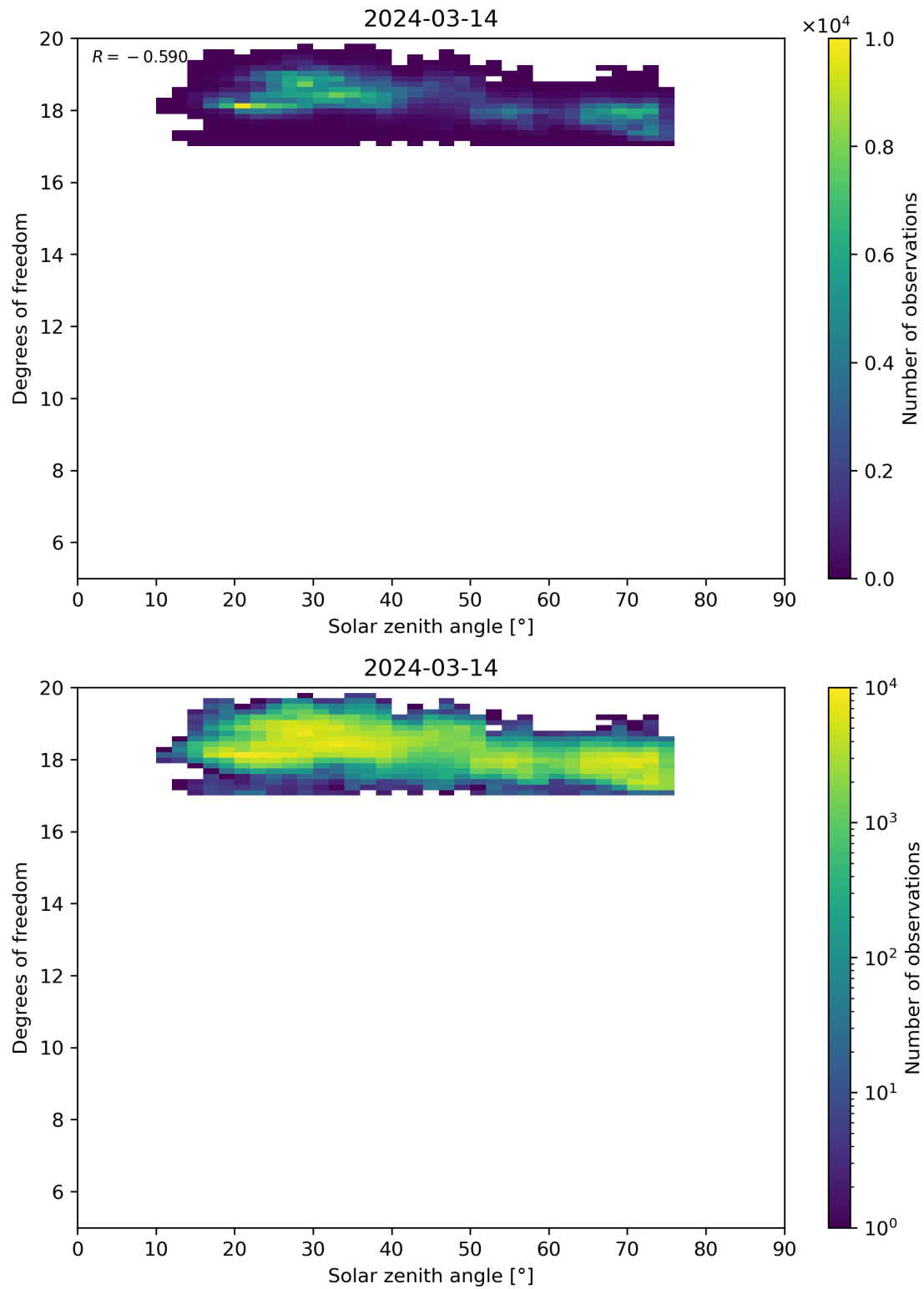
Figure 96: Scatter density plot of “Solar zenith angle” against “Degrees of freedom” for 2024-03-14 to 2024-03-15.
