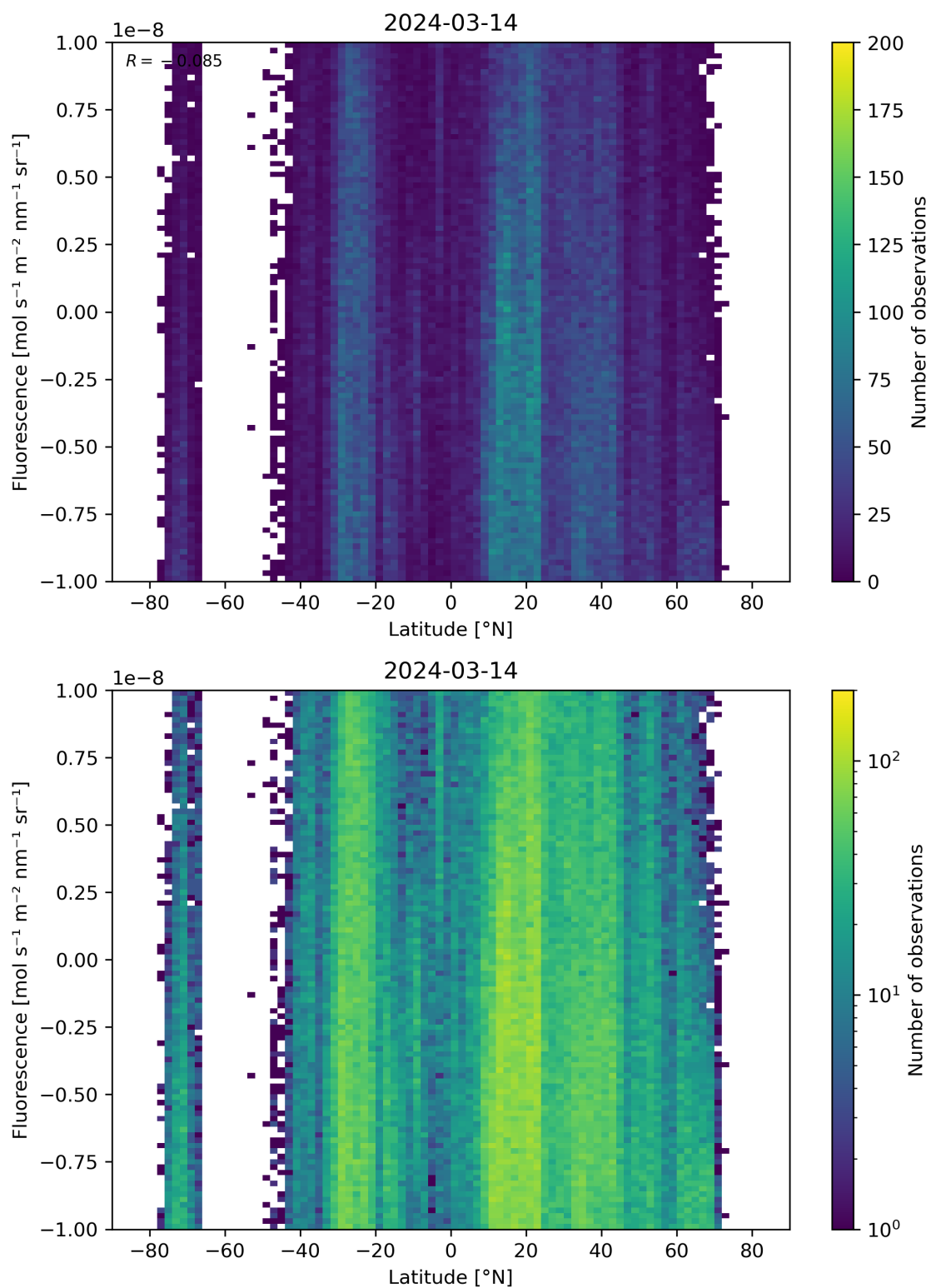
Figure 56: Scatter density plot of “Latitude” against “Fluorescence” for 2024-03-14 to 2024-03-15.
