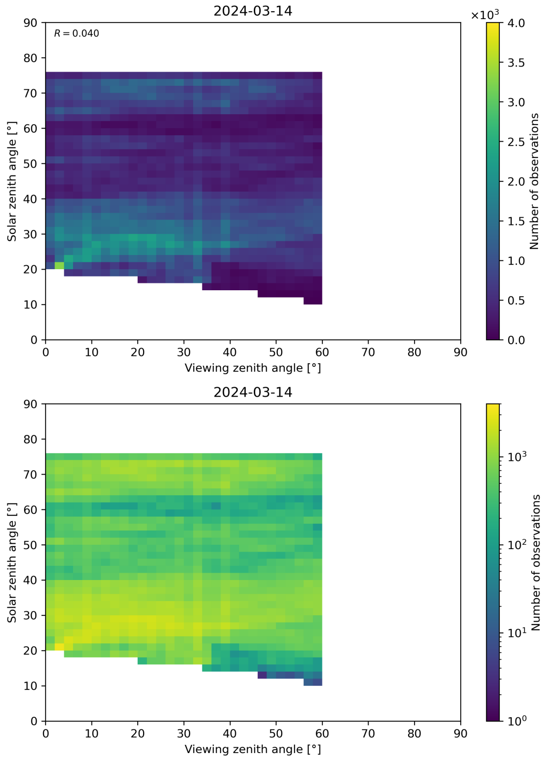
Figure 115: Scatter density plot of “Viewing zenith angle” against “Solar zenith angle” for 2024-03-14 to 2024-03-15.
