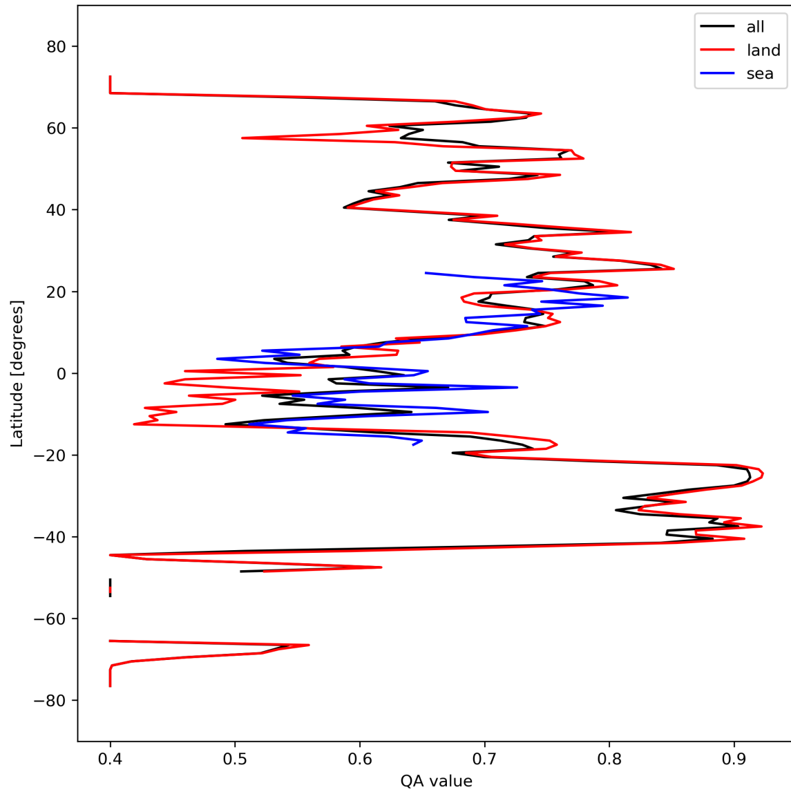
Figure 11: Zonal average of “QA value” for 2024-03-14 to 2024-03-15.
