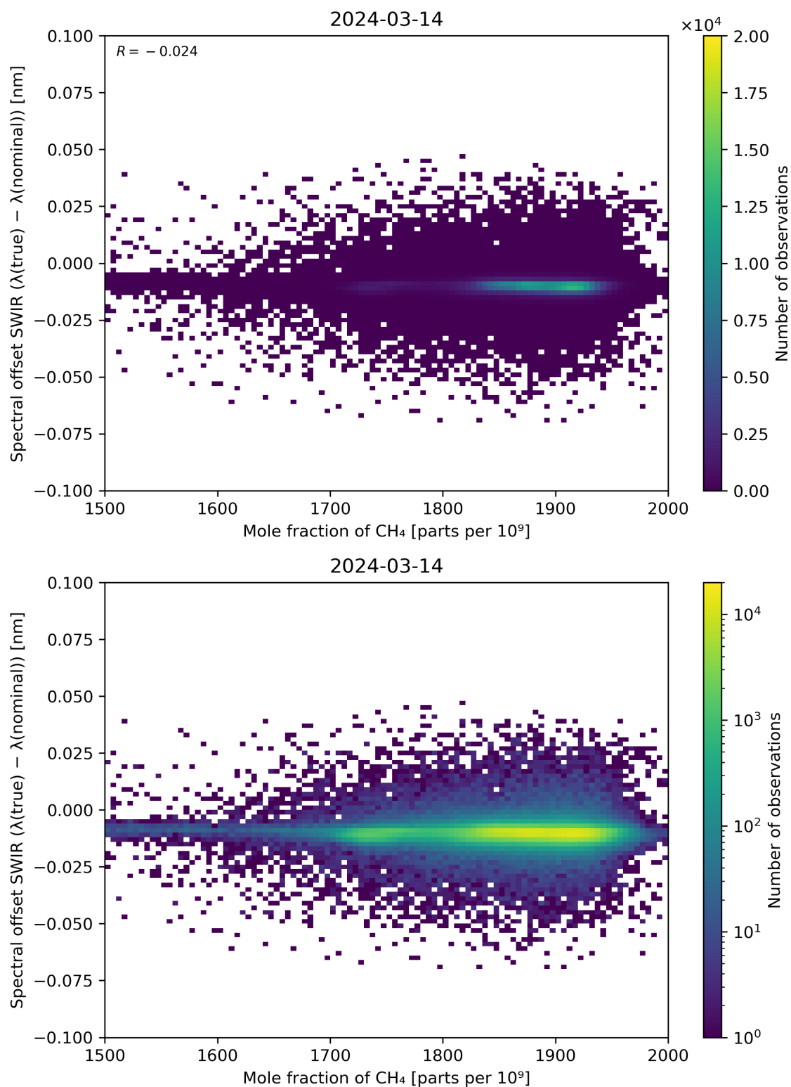
Figure 86: Scatter density plot of “Mole fraction of CH 4 ” against “Spectral offset SWIR ( \lambda(\text{true}) - \lambda(\text{nominal}) )” for 2024-03-14 to 2024-03-15.
