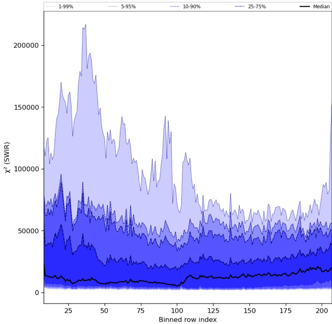
Figure 39: Along track statistics of “ \chi^2 (SWIR)” for 2024-03-14 to 2024-03-15
