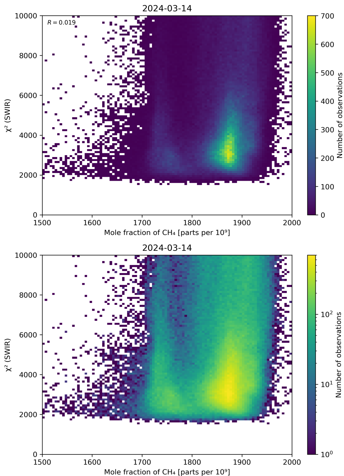
Figure 71: Scatter density plot of “Mole fraction of CH 4 ” against “ \chi^2 (SWIR)” for 2024-03-14 to 2024-03-15.
