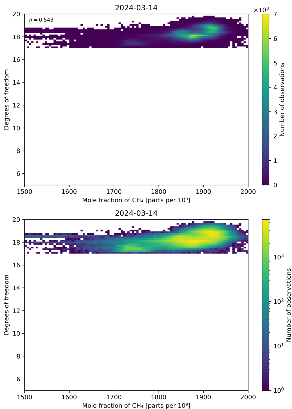
Figure 72: Scatter density plot of “Mole fraction of CH 4 ” against “Degrees of freedom” for 2024-03-14 to 2024-03-15.
