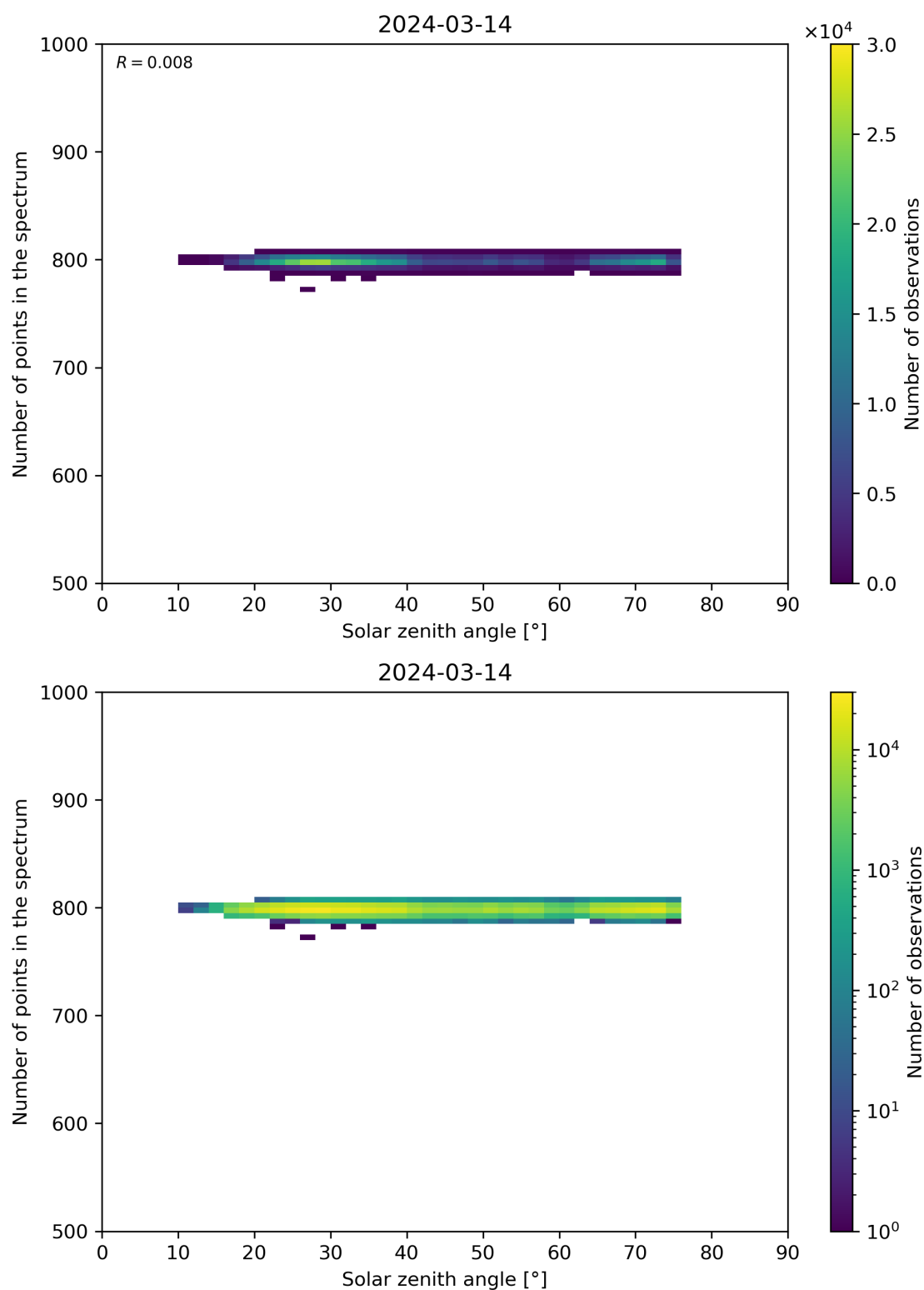
Figure 103: Scatter density plot of “Solar zenith angle” against “Number of points in the spectrum” for 2024-03-14 to 2024-03-15.
