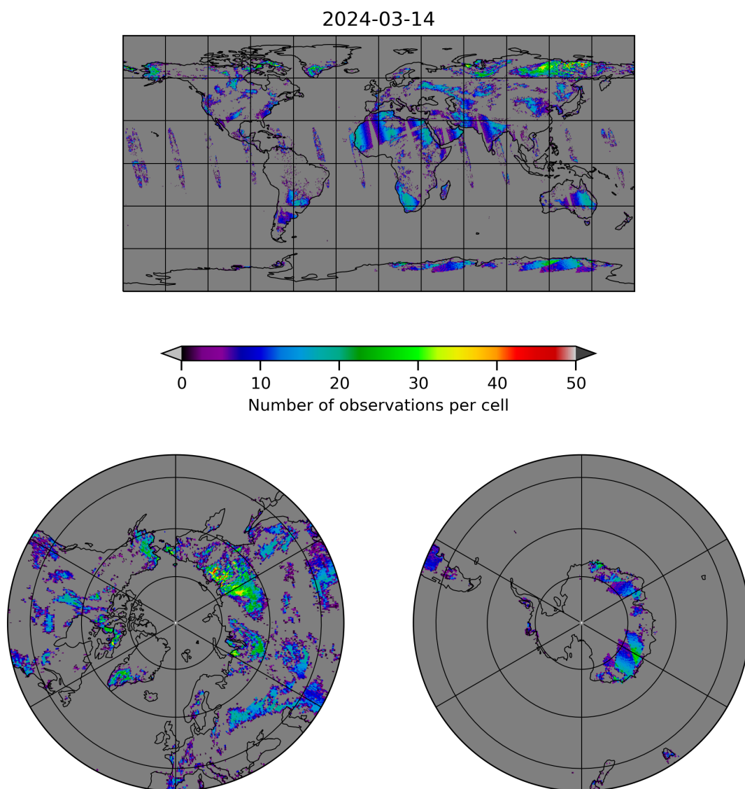
Figure 10: Map of the number of observations for 2024-03-14 to 2024-03-15
