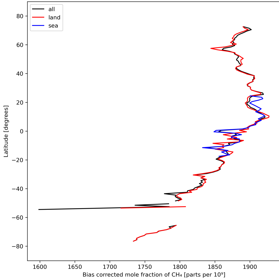
Figure 14: Zonal average of “Bias corrected mole fraction of CH 4 ” for 2024-03-14 to 2024-03-15.
