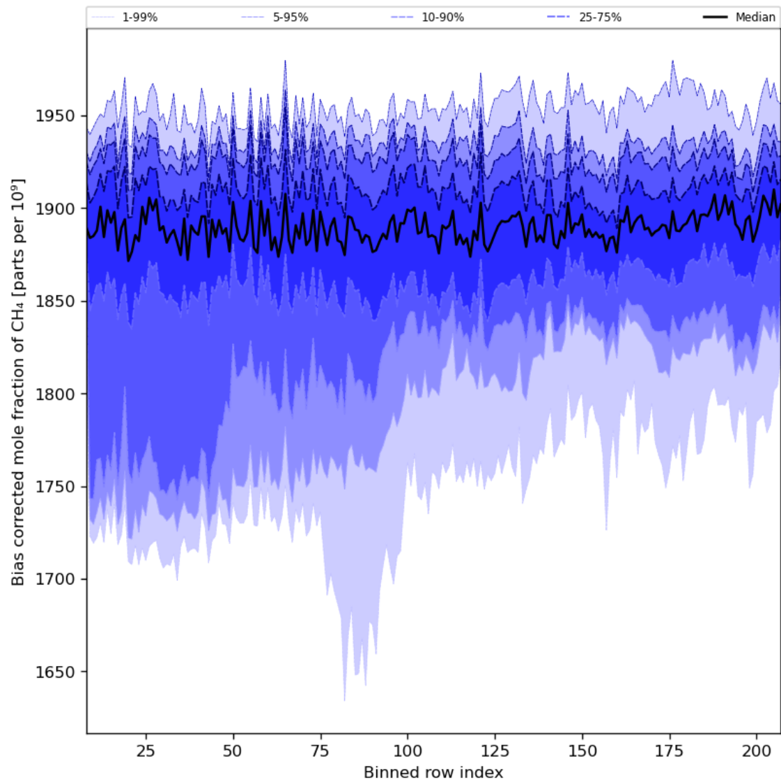
Figure 36: Along track statistics of “Bias corrected mole fraction of CH 4 ” for 2024-03-14 to 2024-03-15
