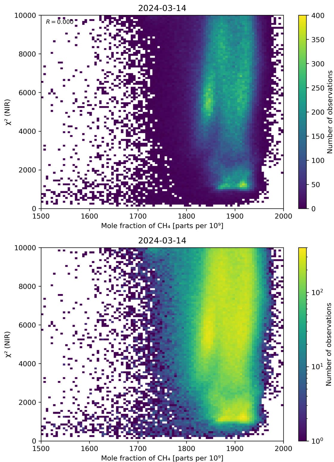
Figure 70: Scatter density plot of “Mole fraction of \text{CH}_4 ” against “ \chi^2 (NIR)” for 2024-03-14 to 2024-03-15.
