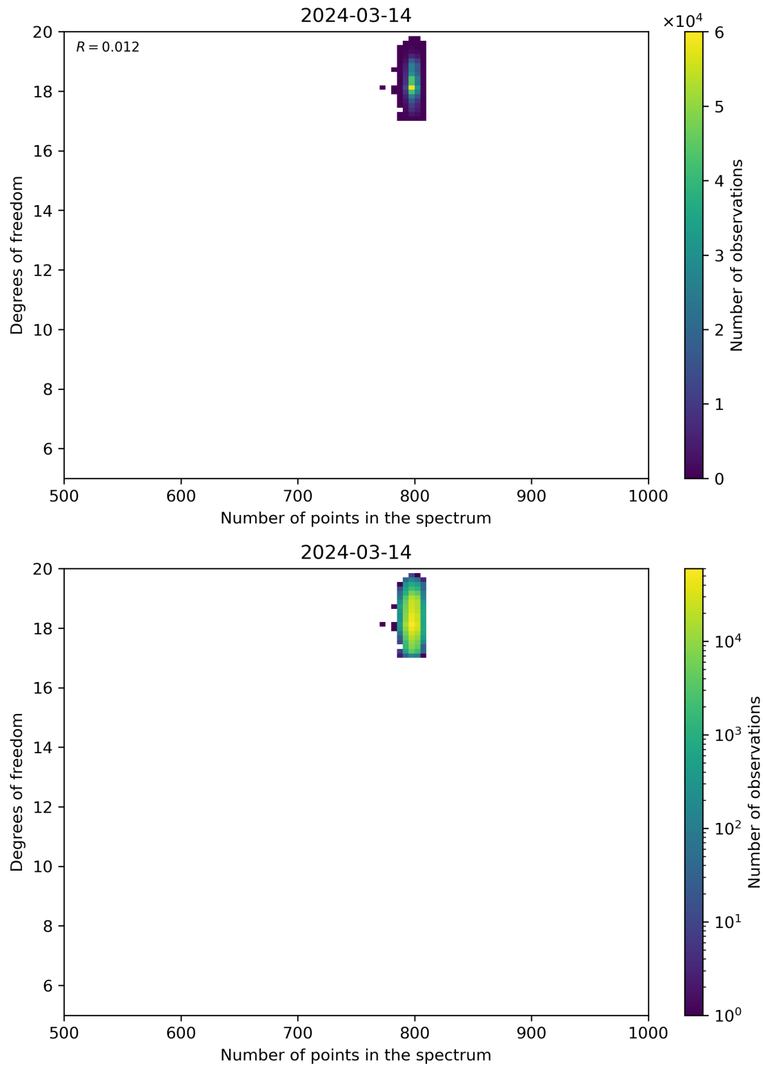
Figure 90: Scatter density plot of “Number of points in the spectrum” against “Degrees of freedom” for 2024-03-14 to 2024-03-15.
