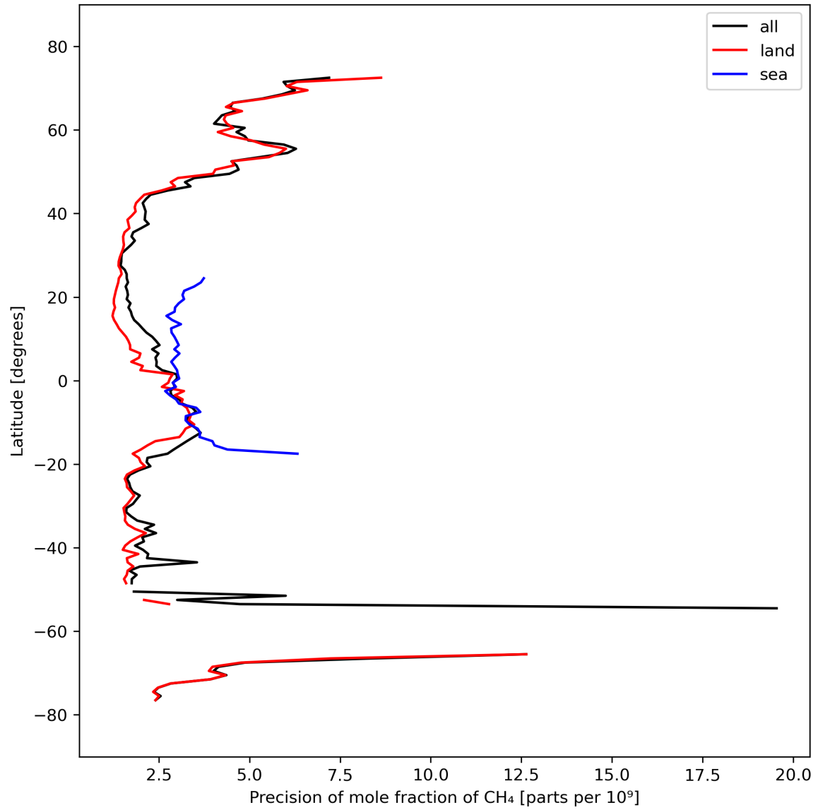
Figure 13: Zonal average of “Precision of mole fraction of CH 4 ” for 2024-03-14 to 2024-03-15.
