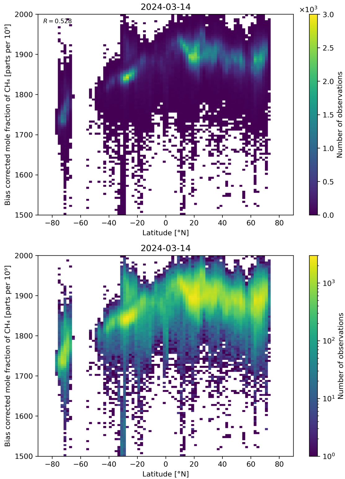
Figure 58: Scatter density plot of “Latitude” against “Bias corrected mole fraction of CH 4 ” for 2024-03-14 to 2024-03-15.
