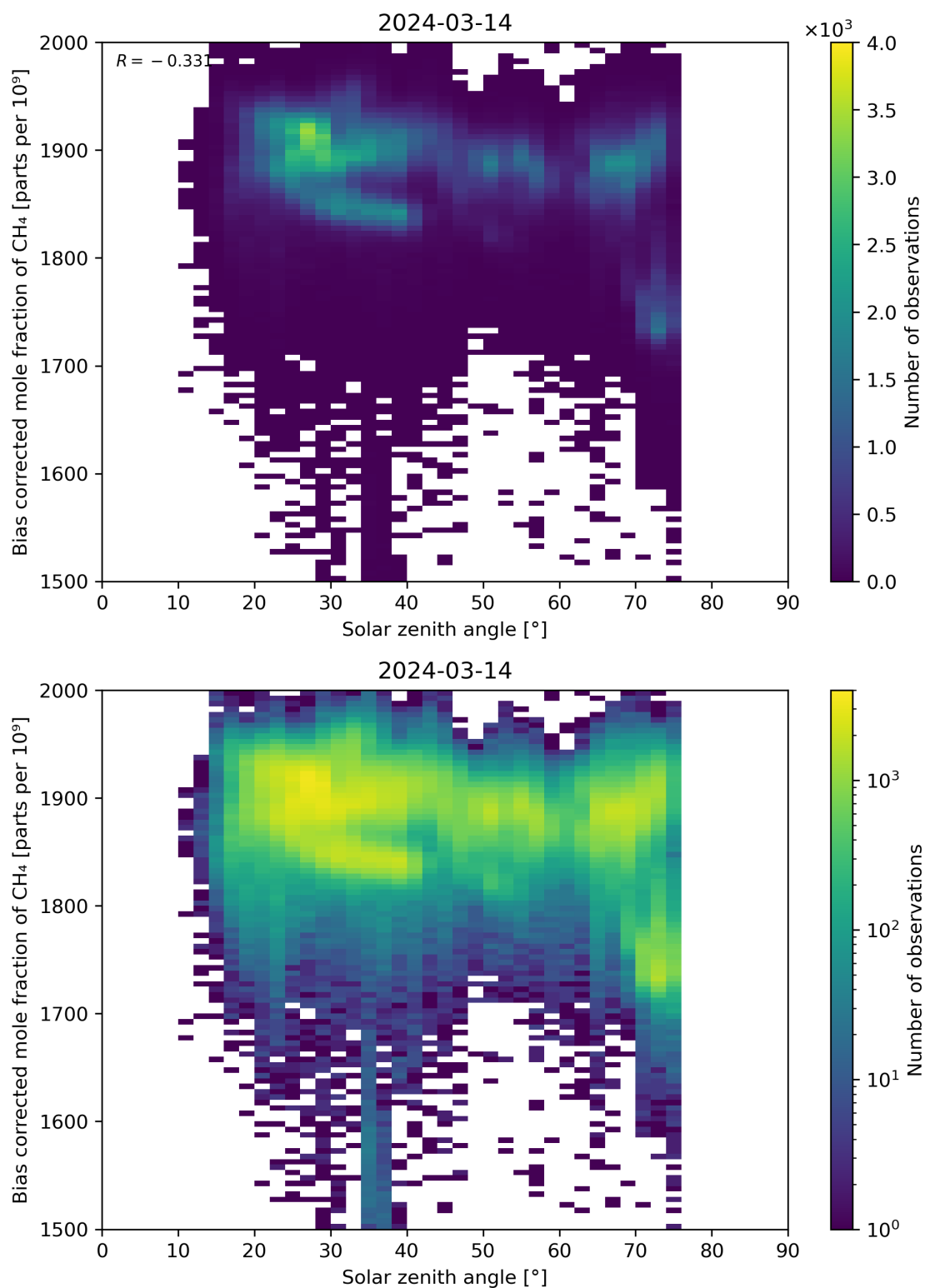
Figure 100: Scatter density plot of “Solar zenith angle” against “Bias corrected mole fraction of \text{CH}_4 ” for 2024-03-14 to 2024-03-15.
