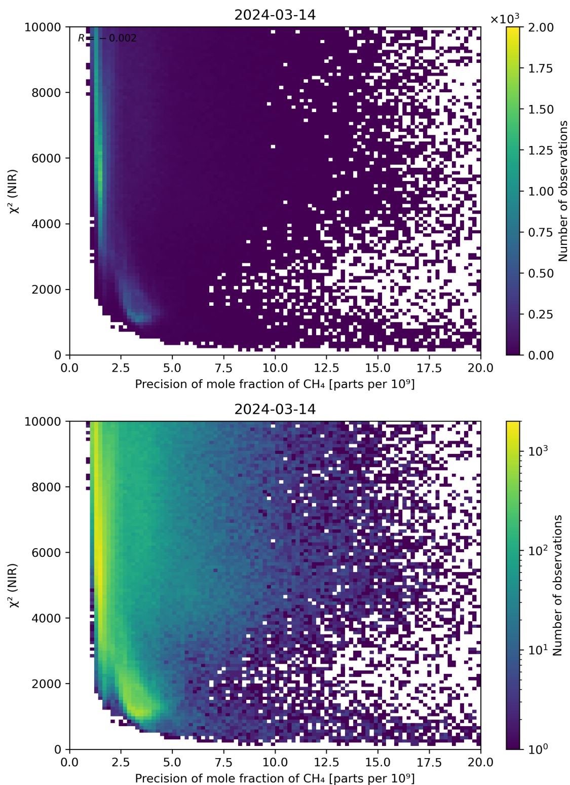
Figure 78: Scatter density plot of “Precision of mole fraction of CH 4 ” against “ \chi^2 (NIR)” for 2024-03-14 to 2024-03-15.
