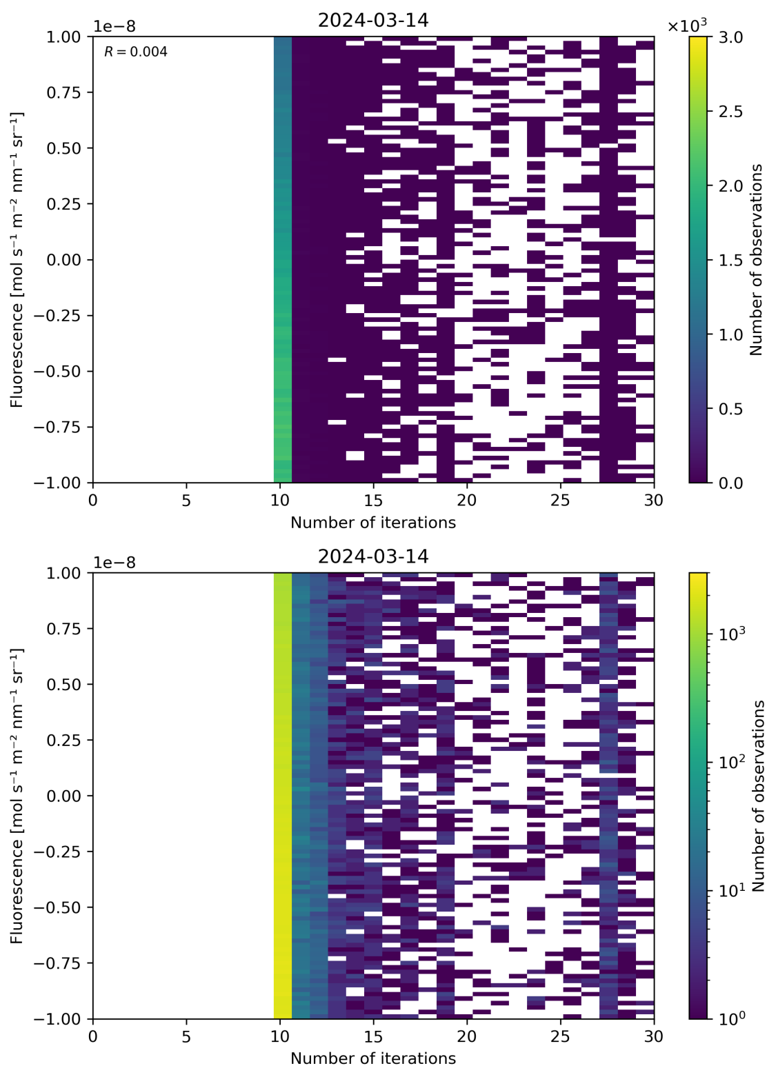
Figure 87: Scatter density plot of “Number of iterations” against “Fluorescence” for 2024-03-14 to 2024-03-15.
