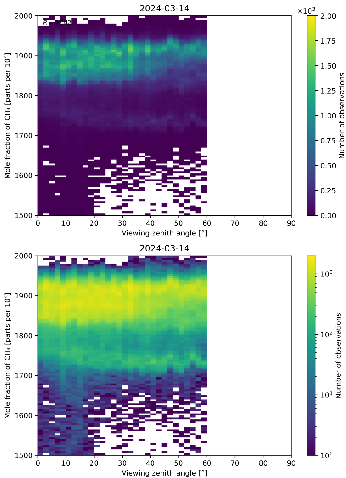
Figure 110: Scatter density plot of “Viewing zenith angle” against “Mole fraction of CH 4 ” for 2024-03-14 to 2024-03-15.
