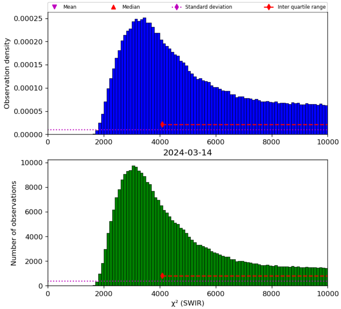
Figure 28: Histogram of “ \chi^2 (SWIR)” for 2024-03-14 to 2024-03-15
