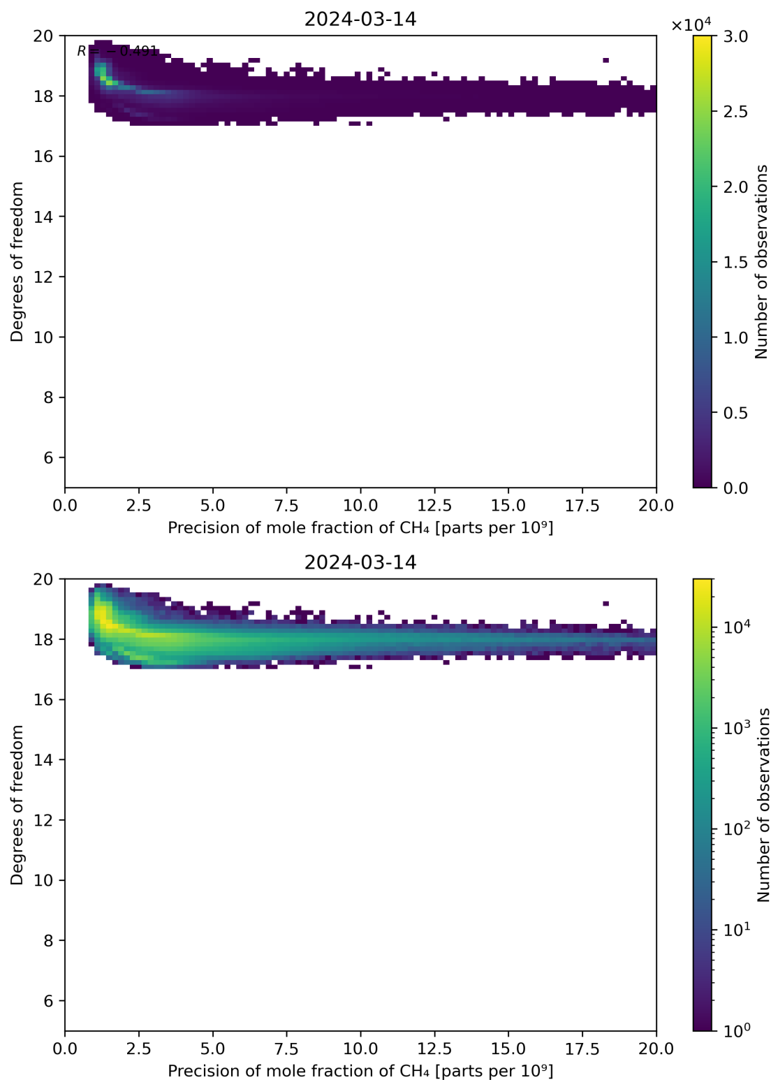
Figure 80: Scatter density plot of “Precision of mole fraction of CH 4 ” against “Degrees of freedom” for 2024-03-14 to 2024-03-15.
