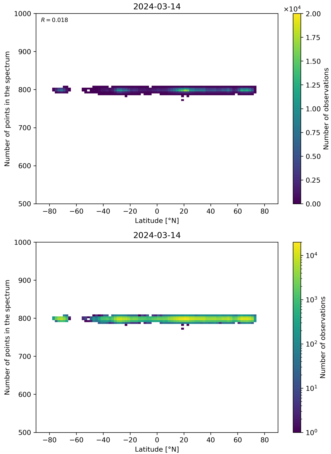
Figure 61: Scatter density plot of “Latitude” against “Number of points in the spectrum” for 2024-03-14 to 2024-03-15.
