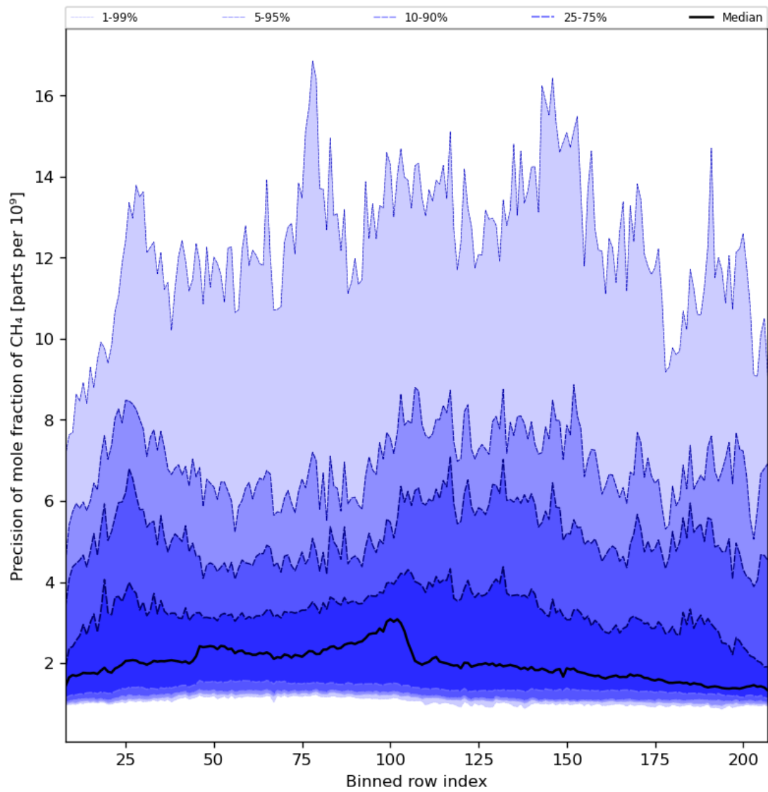
Figure 35: Along track statistics of “Precision of mole fraction of CH 4 ” for 2024-03-14 to 2024-03-15
