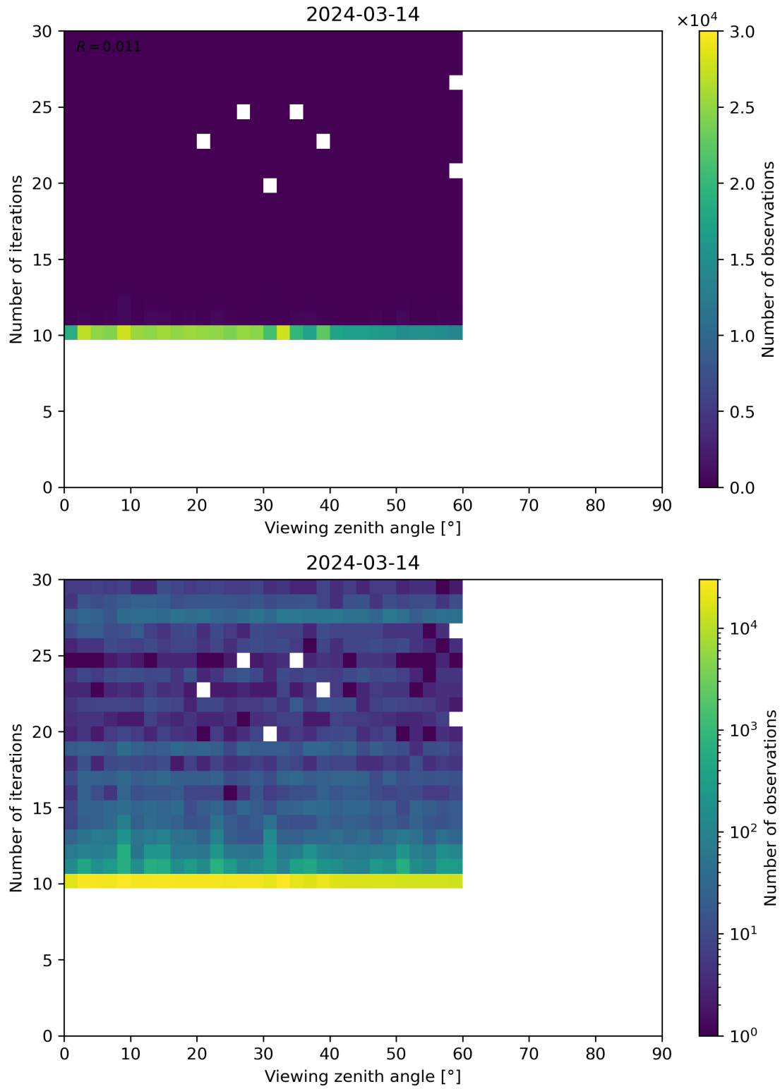
Figure 113: Scatter density plot of “Viewing zenith angle” against “Number of iterations” for 2024-03-14 to 2024-03-15.
