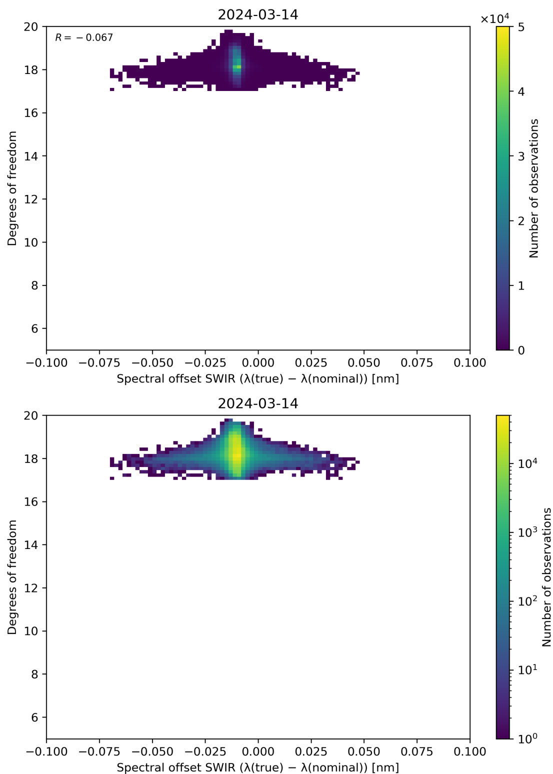
Figure 119: Scatter density plot of “Spectral offset SWIR ( \lambda(\text{true}) - \lambda(\text{nominal}) )” against “Degrees of freedom” for 2024-03-14 to 2024-03-15.
