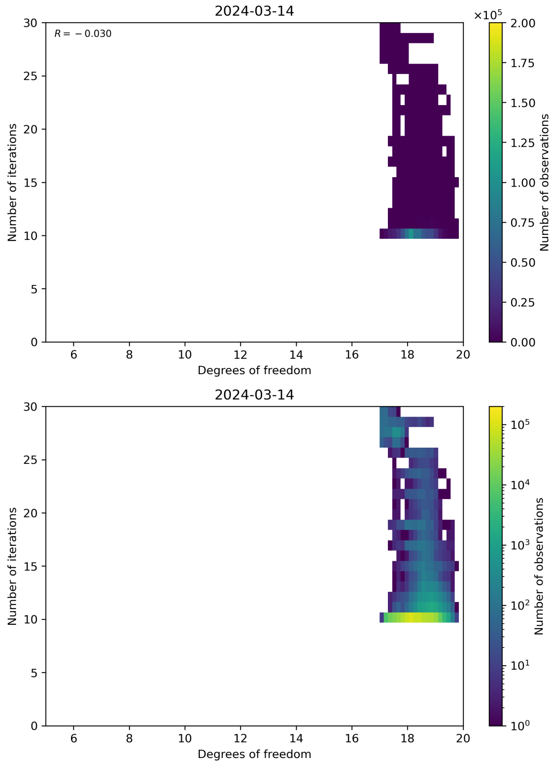
Figure 52: Scatter density plot of “Degrees of freedom” against “Number of iterations” for 2024-03-14 to 2024-03-15.
