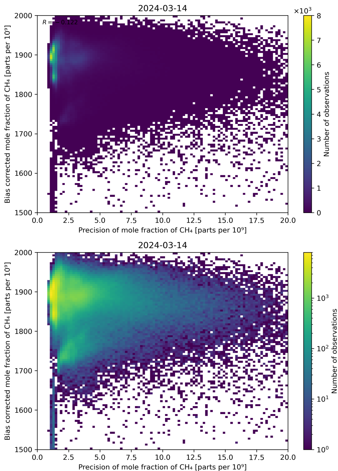
Figure 82: Scatter density plot of “Precision of mole fraction of CH 4 ” against “Bias corrected mole fraction of CH 4 ” for 2024-03-14 to 2024-03-15.
