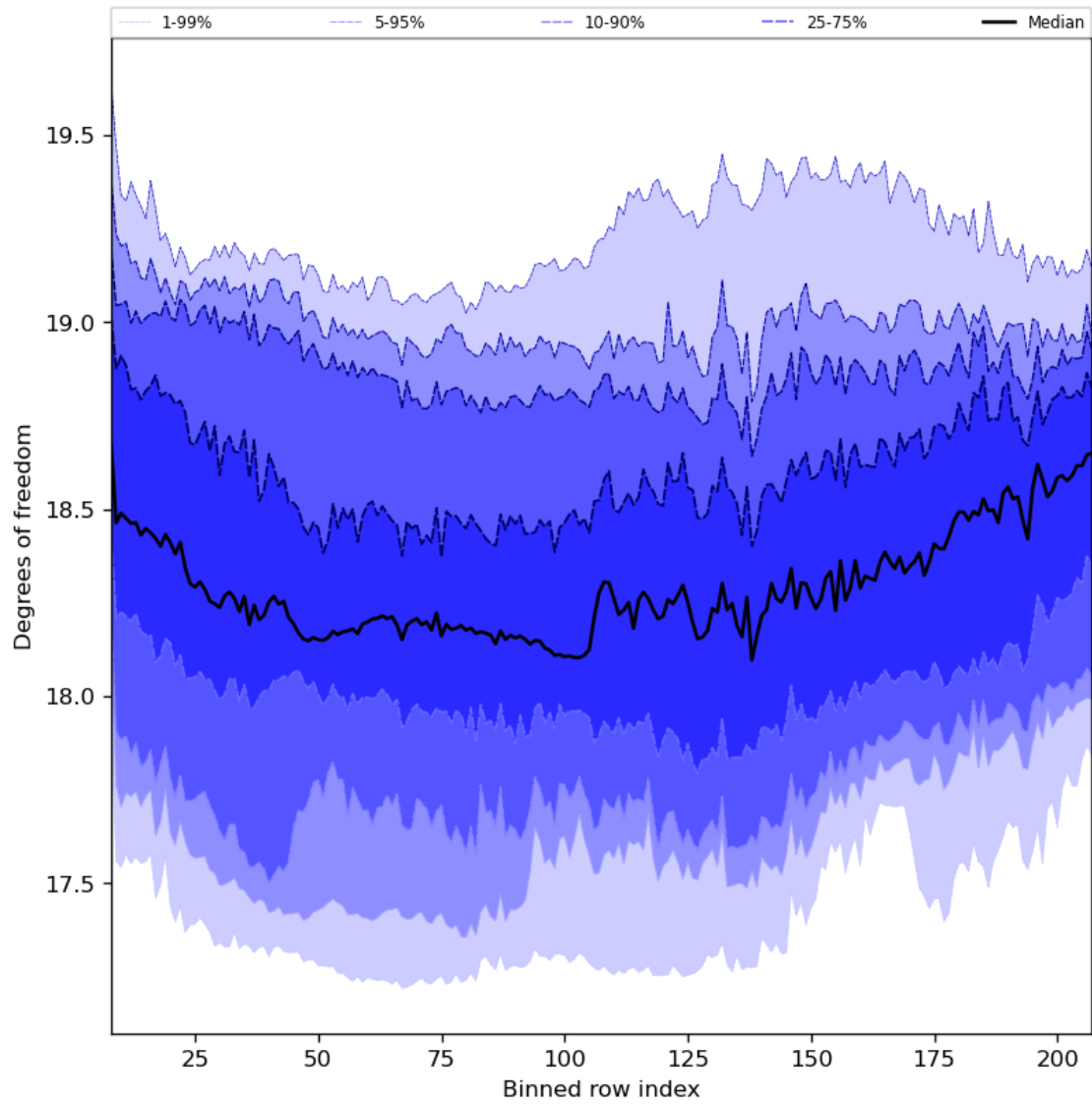
Figure 41: Along track statistics of “Degrees of freedom” for 2024-03-14 to 2024-03-15
