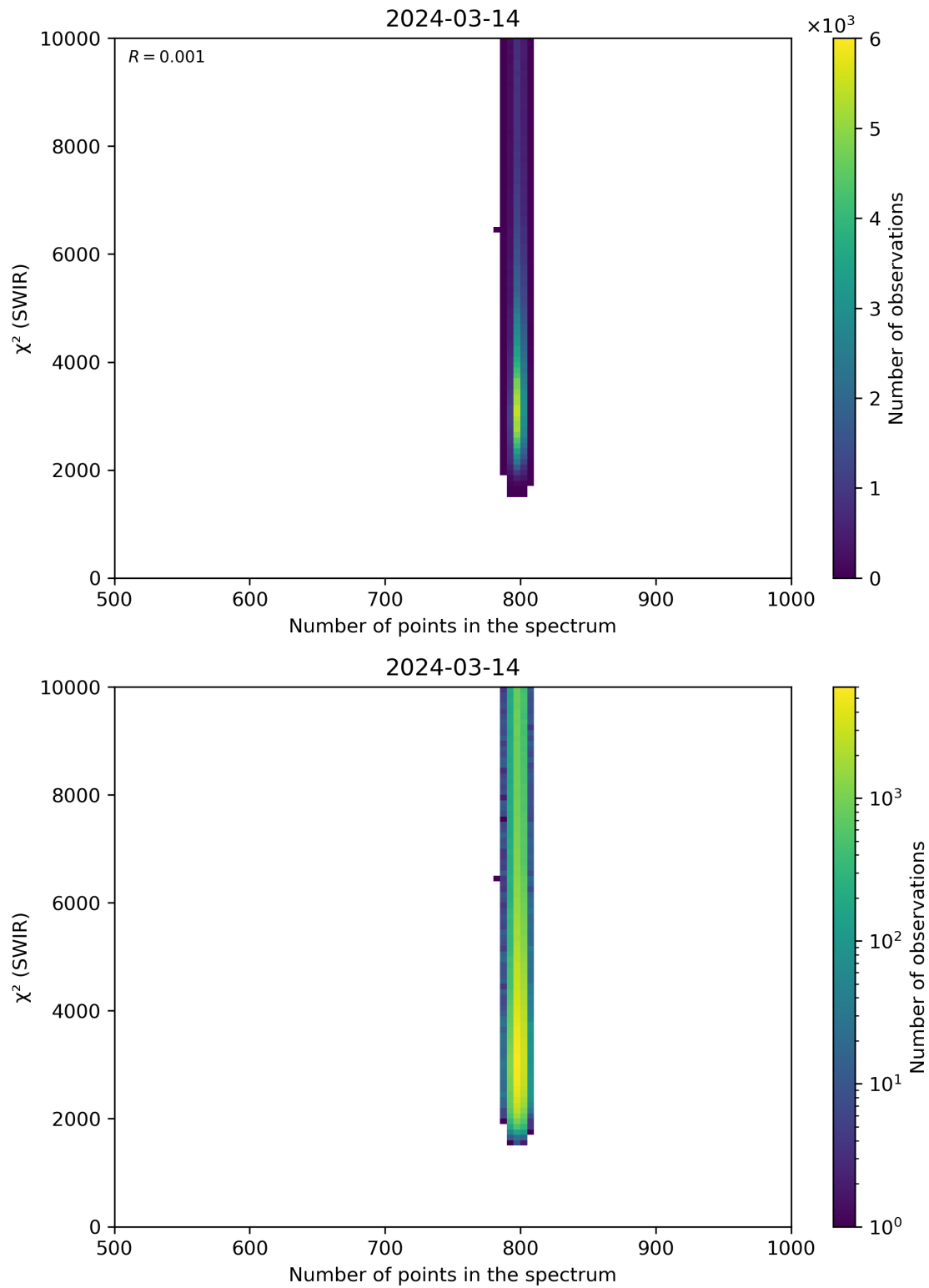
Figure 89: Scatter density plot of “Number of points in the spectrum” against “ \chi^2 (SWIR)” for 2024-03-14 to 2024-03-15.
