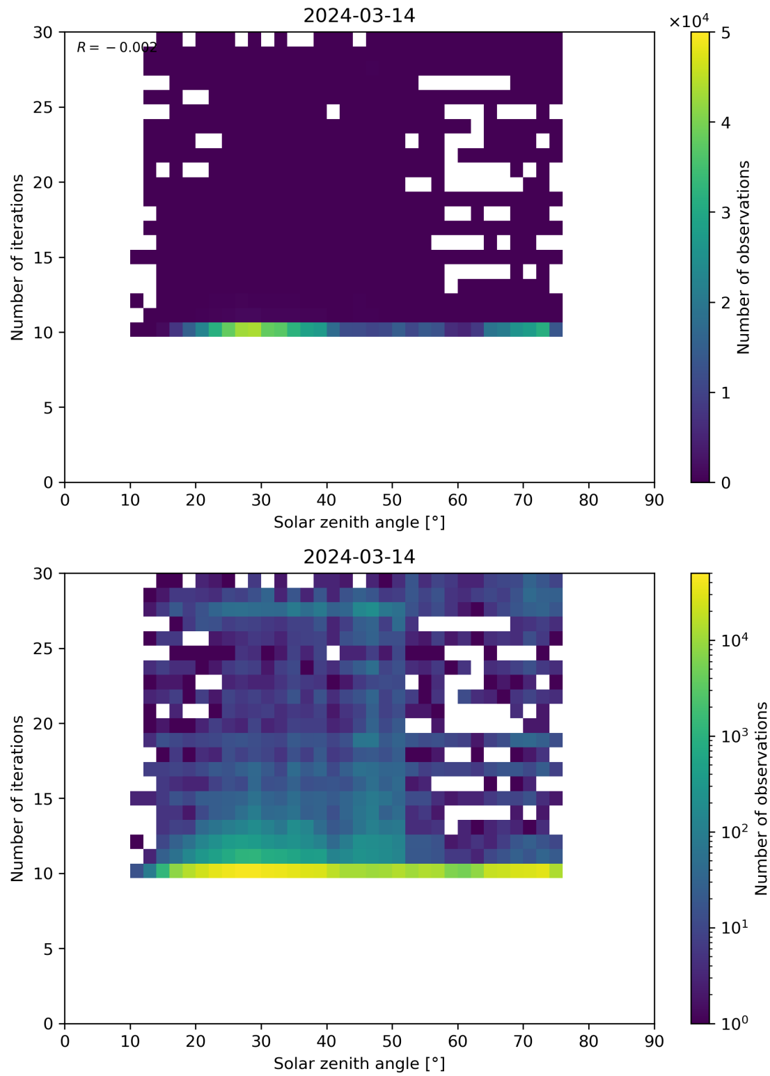
Figure 102: Scatter density plot of “Solar zenith angle” against “Number of iterations” for 2024-03-14 to 2024-03-15.
