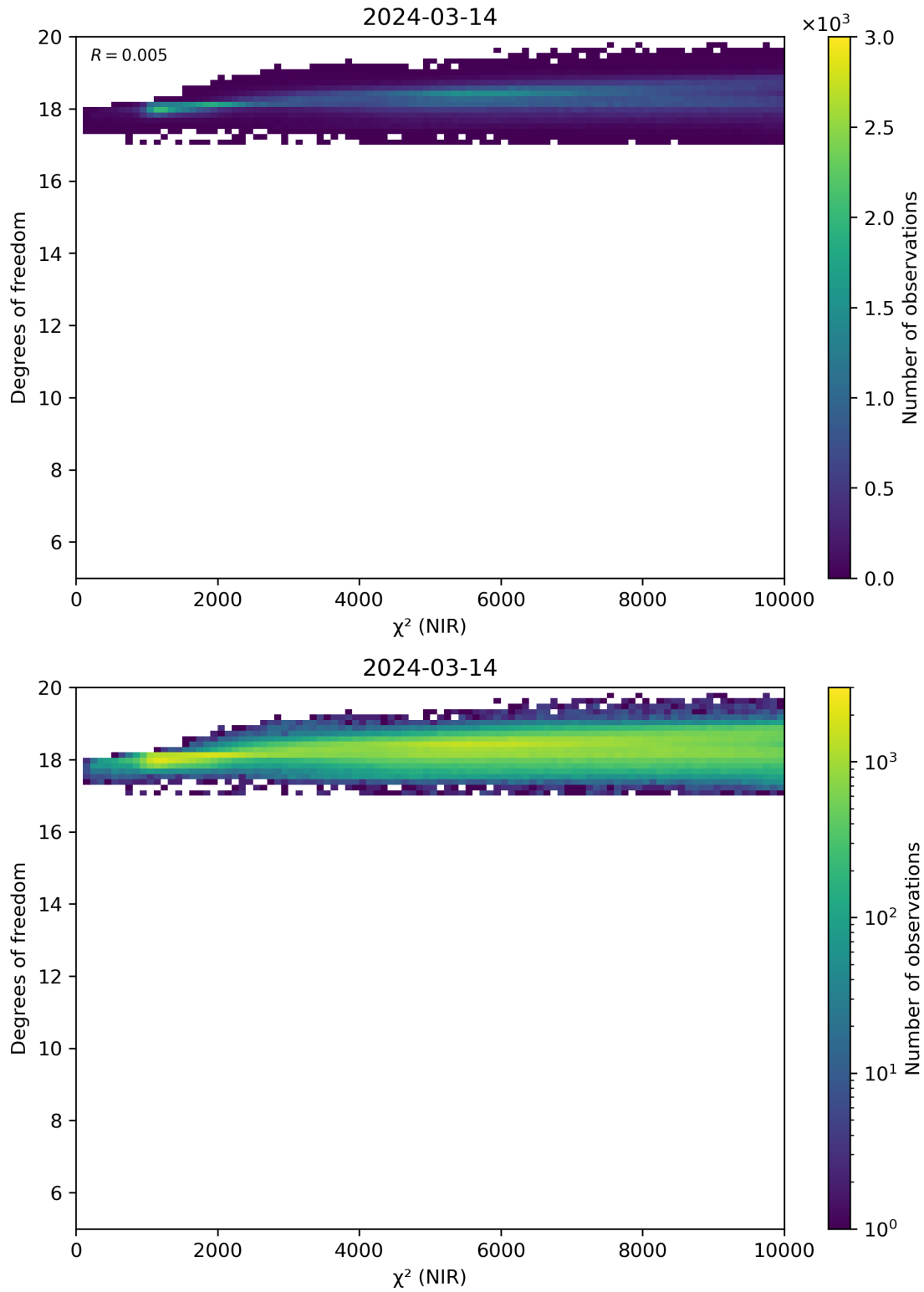
Figure 44: Scatter density plot of “ \chi^2 (NIR)” against “Degrees of freedom” for 2024-03-14 to 2024-03-15.
