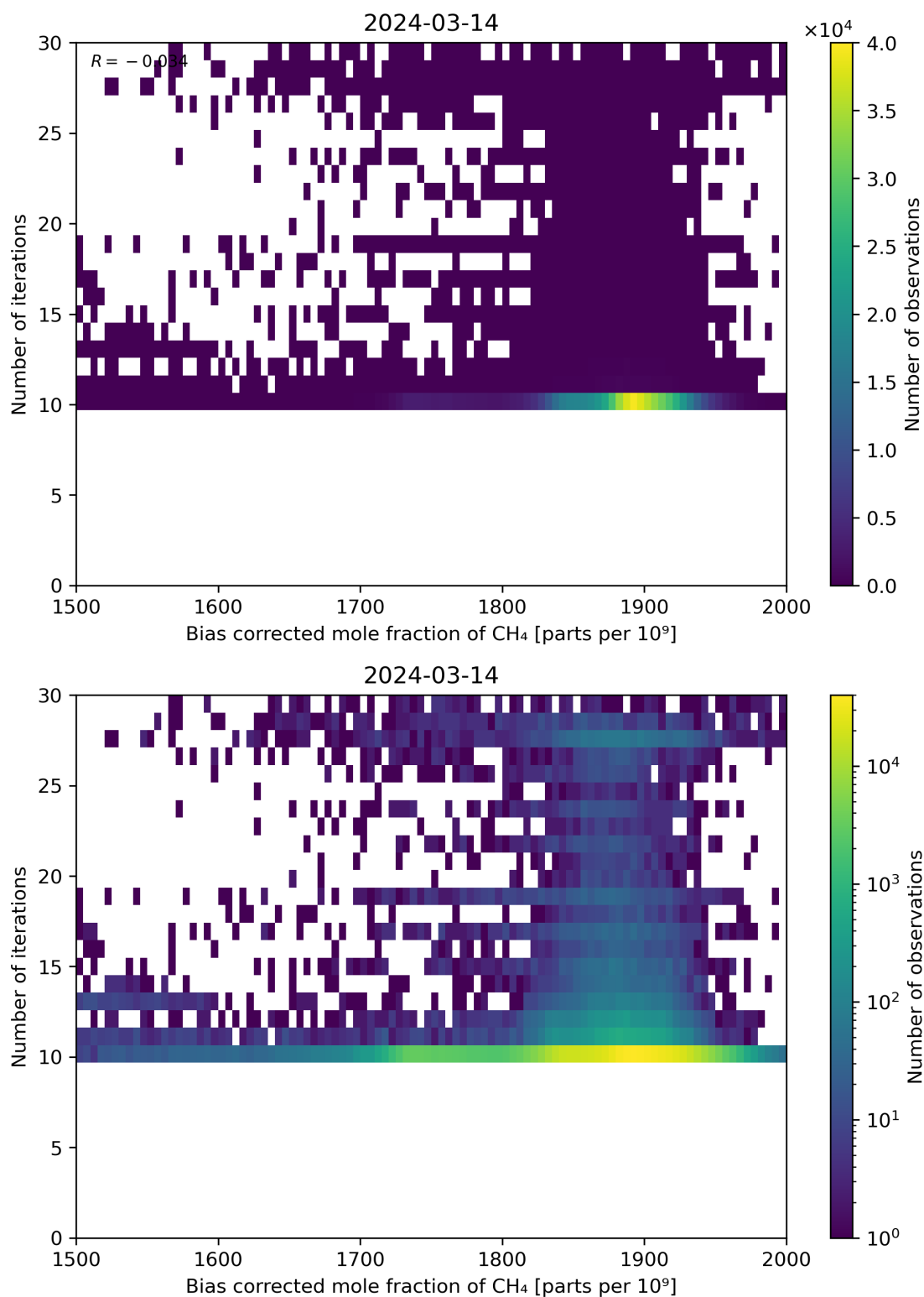
Figure 67: Scatter density plot of “Bias corrected mole fraction of CH 4 ” against “Number of iterations” for 2024-03-14 to 2024-03-15.
