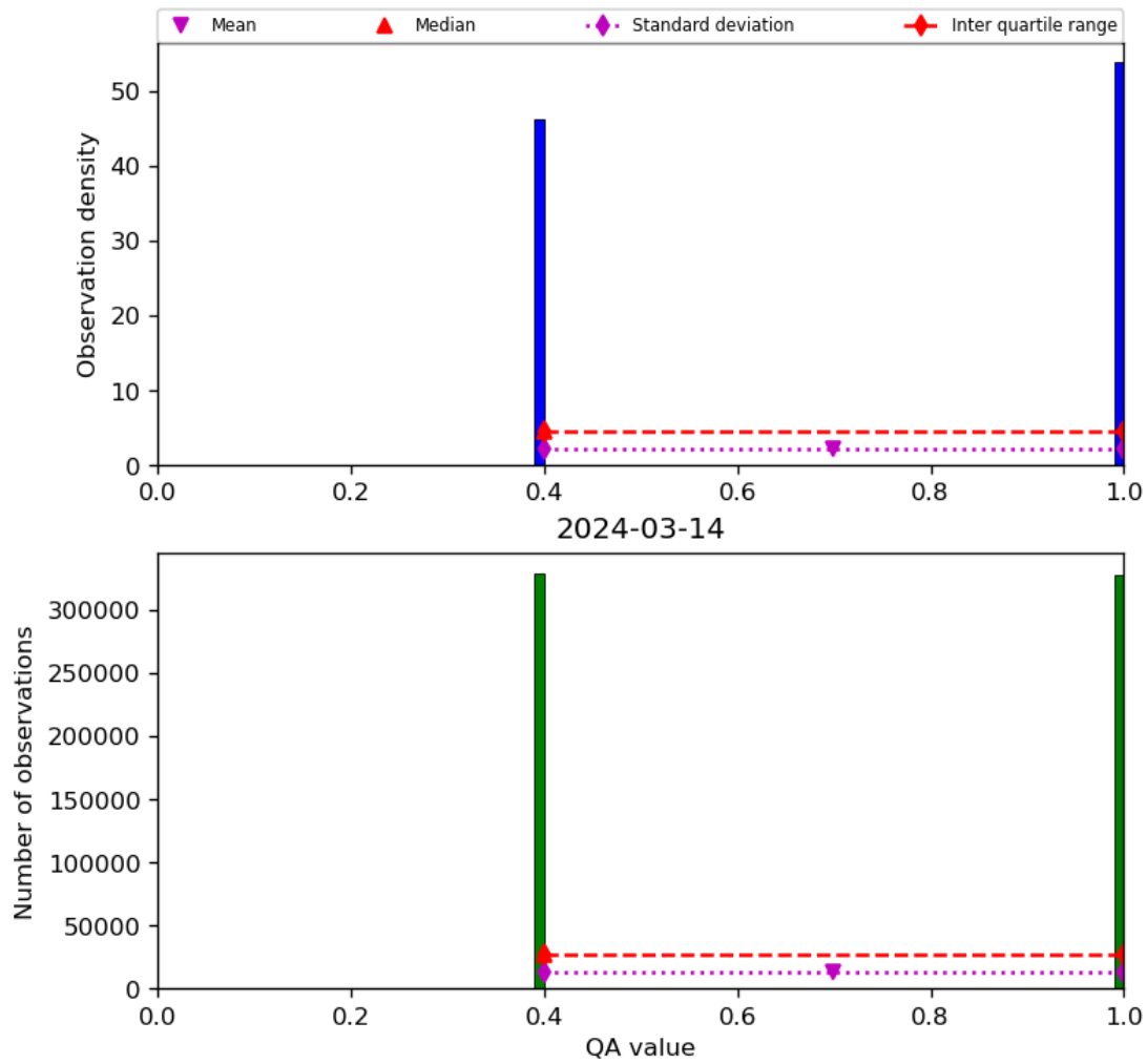
Figure 22: Histogram of “QA value” for 2024-03-14 to 2024-03-15
