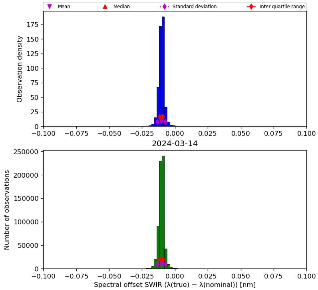
Figure 27: Histogram of “Spectral offset SWIR ( \lambda(\text{true}) - \lambda(\text{nominal}) )” for 2024-03-14 to 2024-03-15
