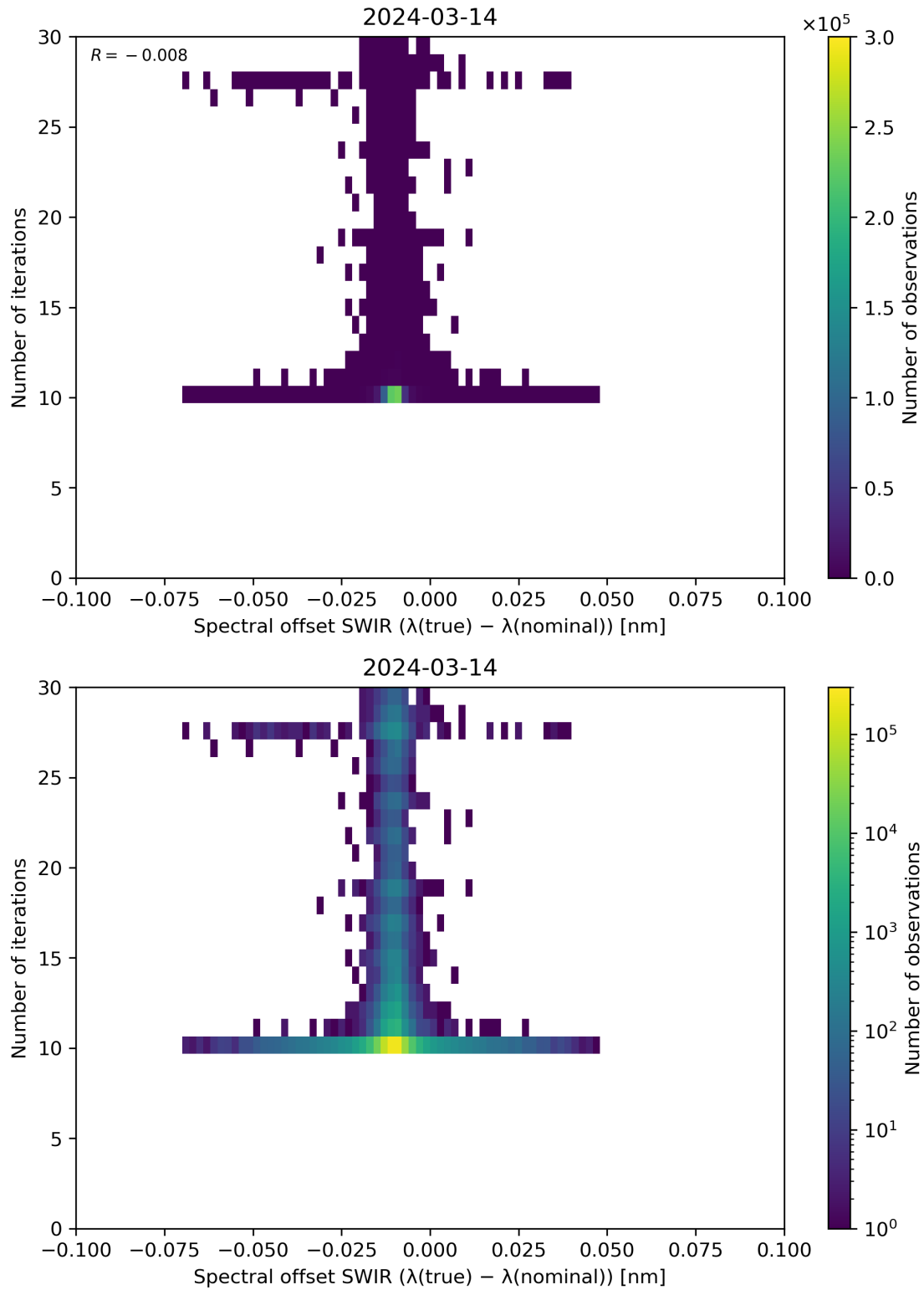
Figure 121: Scatter density plot of “Spectral offset SWIR ( \lambda(\text{true}) - \lambda(\text{nominal}) )” against “Number of iterations” for 2024-03-14 to 2024-03-15.
