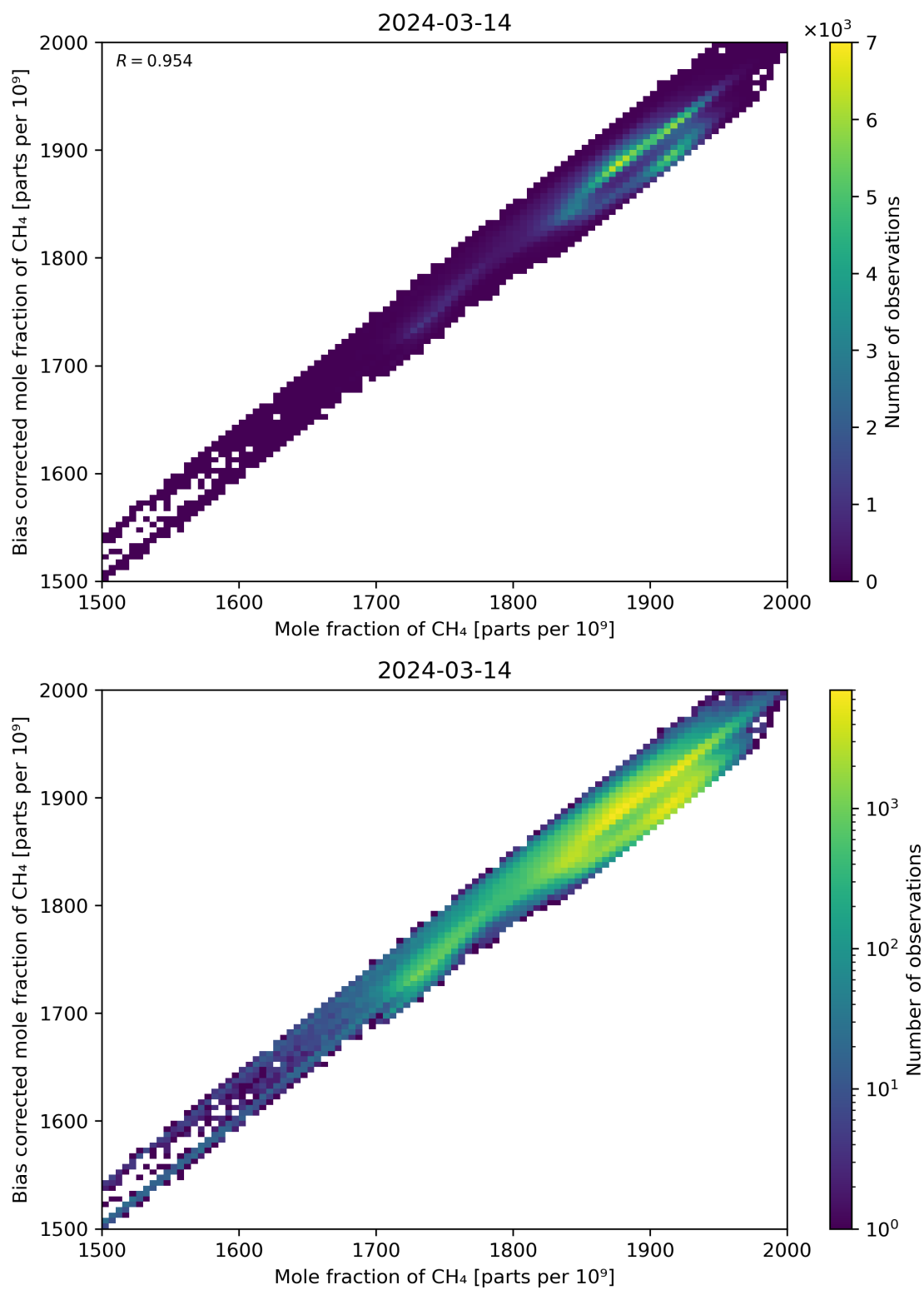
Figure 74: Scatter density plot of “Mole fraction of CH 4 ” against “Bias corrected mole fraction of CH 4 ” for 2024-03-14 to 2024-03-15.
