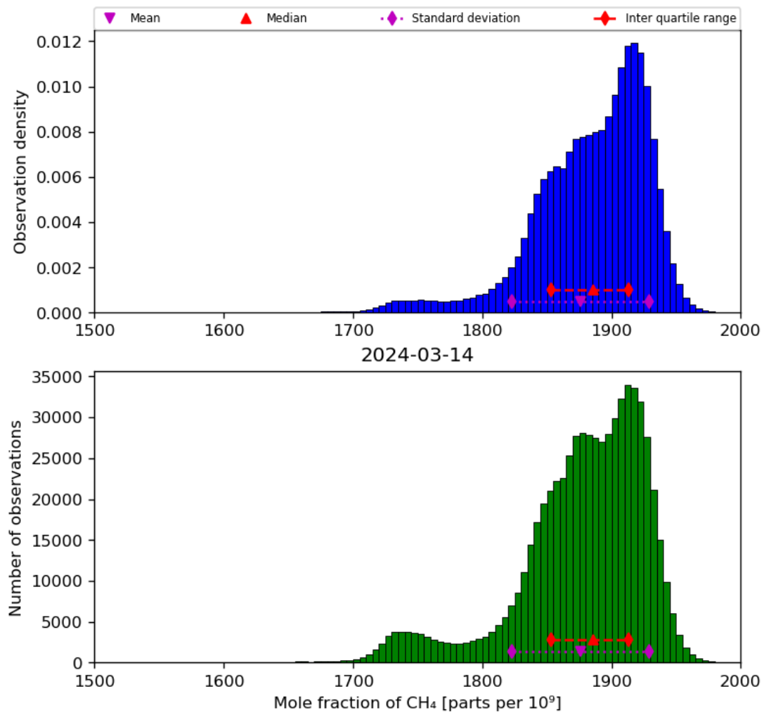
Figure 23: Histogram of “Mole fraction of CH 4 ” for 2024-03-14 to 2024-03-15
