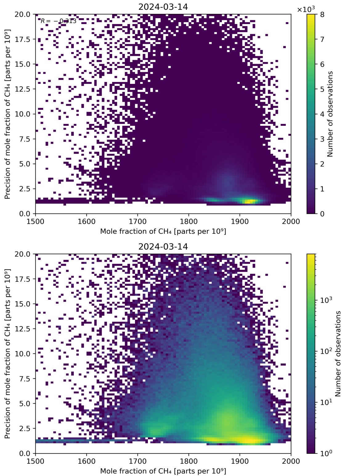
Figure 75: Scatter density plot of “Mole fraction of CH 4 ” against “Precision of mole fraction of CH 4 ” for 2024-03-14 to 2024-03-15.
