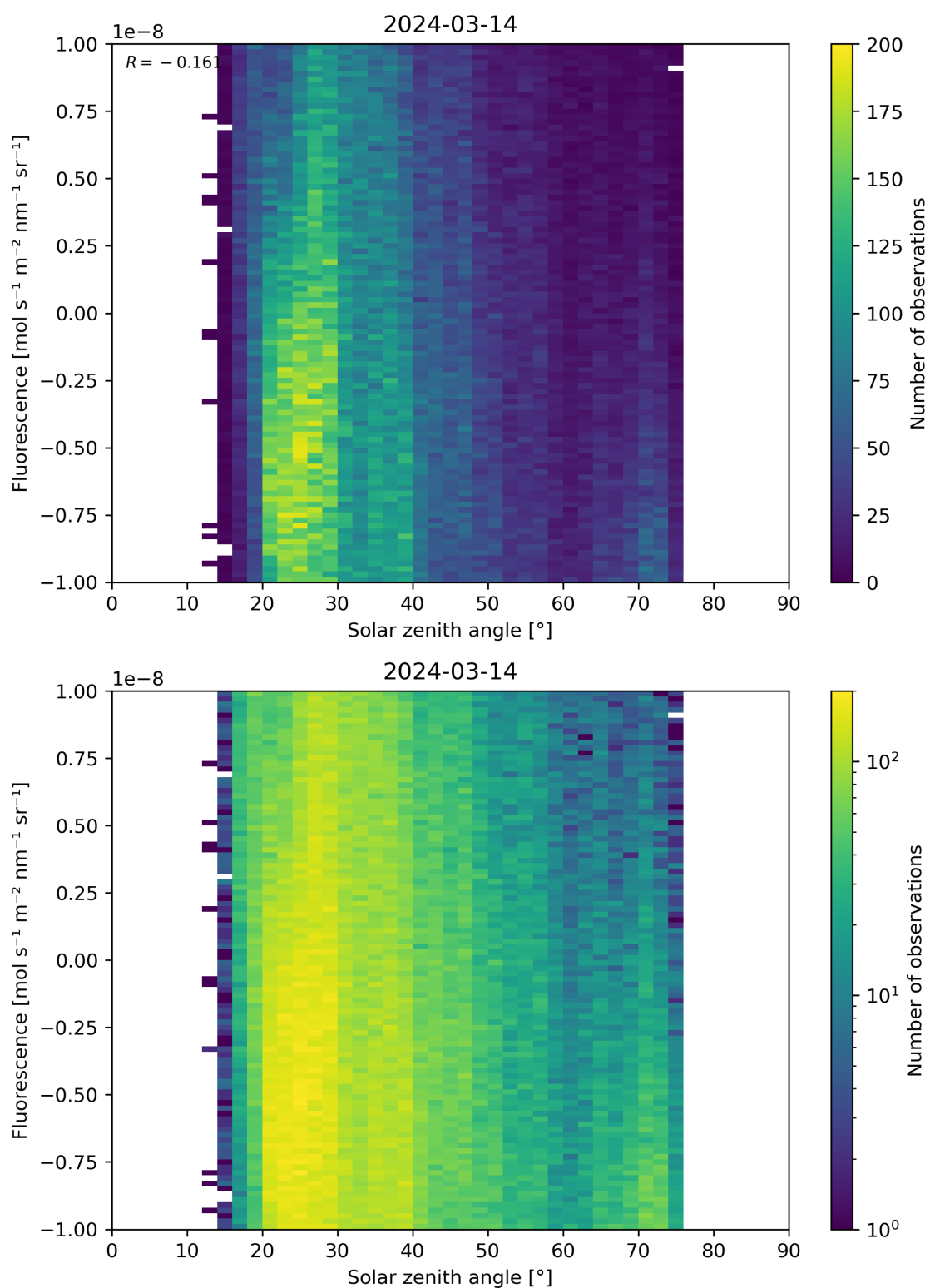
Figure 97: Scatter density plot of “Solar zenith angle” against “Fluorescence” for 2024-03-14 to 2024-03-15.
