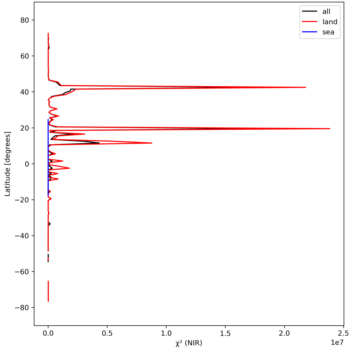
Figure 18: Zonal average of “ \chi^2 (NIR)” for 2024-03-14 to 2024-03-15.
