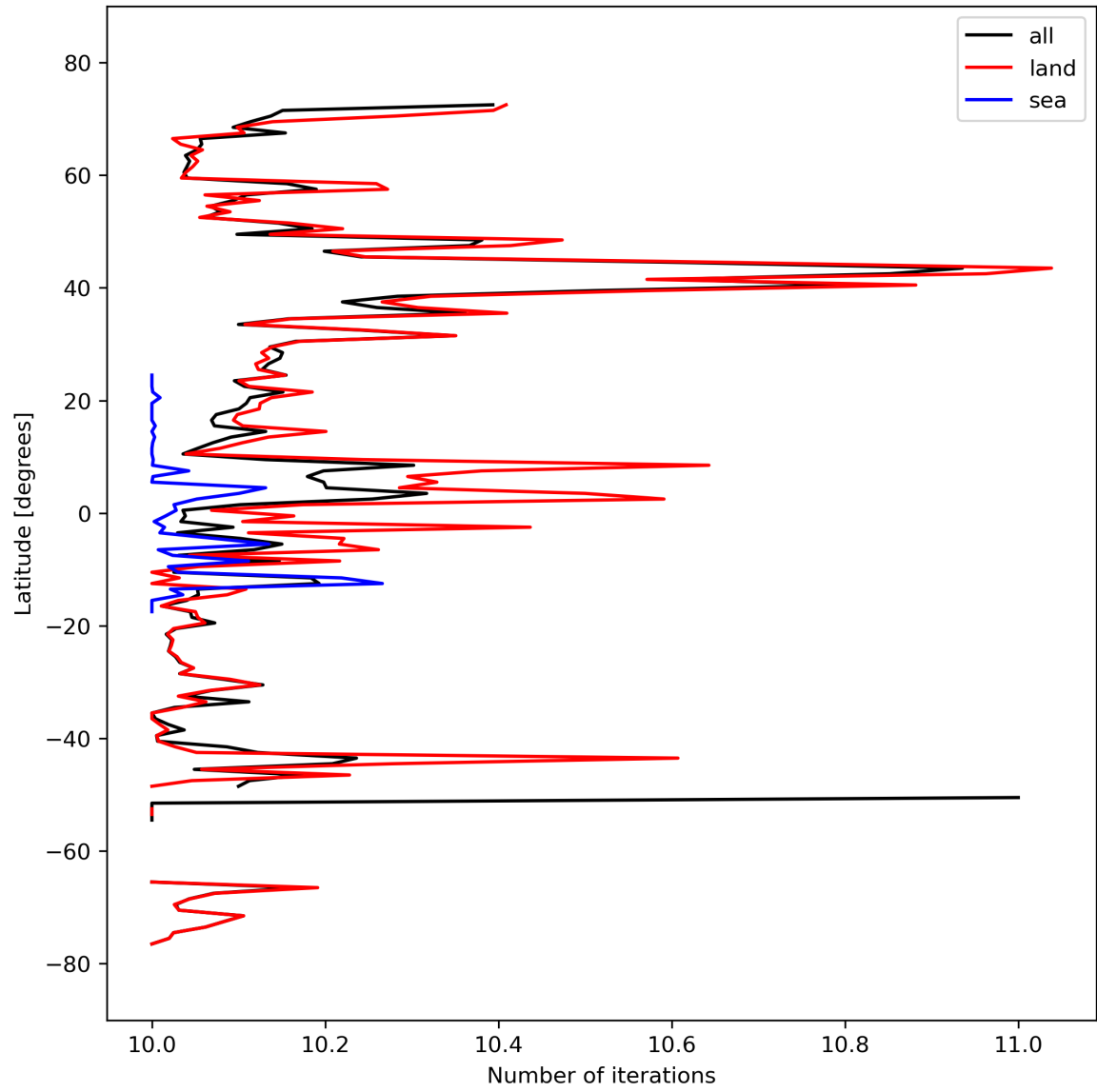
Figure 20: Zonal average of “Number of iterations” for 2024-03-14 to 2024-03-15.
