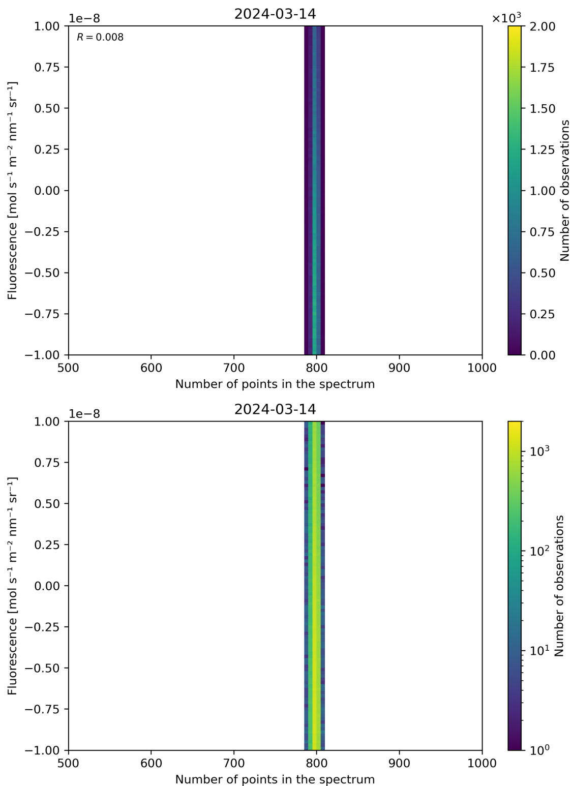
Figure 91: Scatter density plot of “Number of points in the spectrum” against “Fluorescence” for 2024-03-14 to 2024-03-15.
