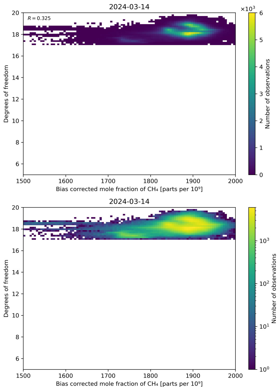
Figure 65: Scatter density plot of “Bias corrected mole fraction of CH 4 ” against “Degrees of freedom” for 2024-03-14 to 2024-03-15.
