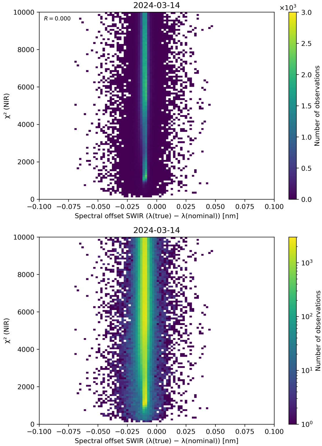
Figure 117: Scatter density plot of “Spectral offset SWIR ( \lambda(\text{true}) - \lambda(\text{nominal}) )” against “ \chi^2 (NIR)” for 2024-03-14 to 2024-03-15.
