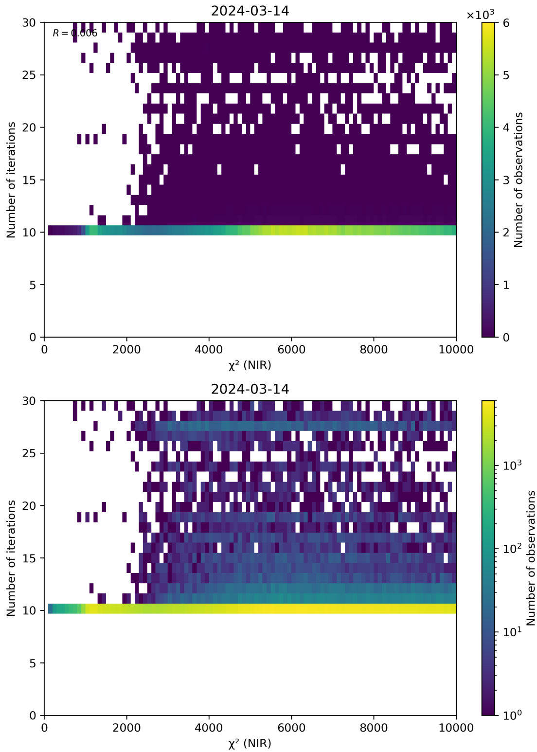
Figure 46: Scatter density plot of “ \chi^2 (NIR)” against “Number of iterations” for 2024-03-14 to 2024-03-15.
