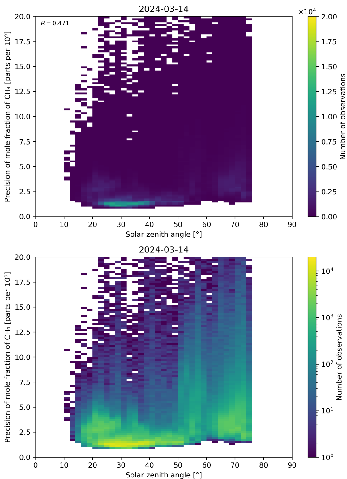
Figure 101: Scatter density plot of “Solar zenith angle” against “Precision of mole fraction of \text{CH}_4 ” for 2024-03-14 to 2024-03-15.
