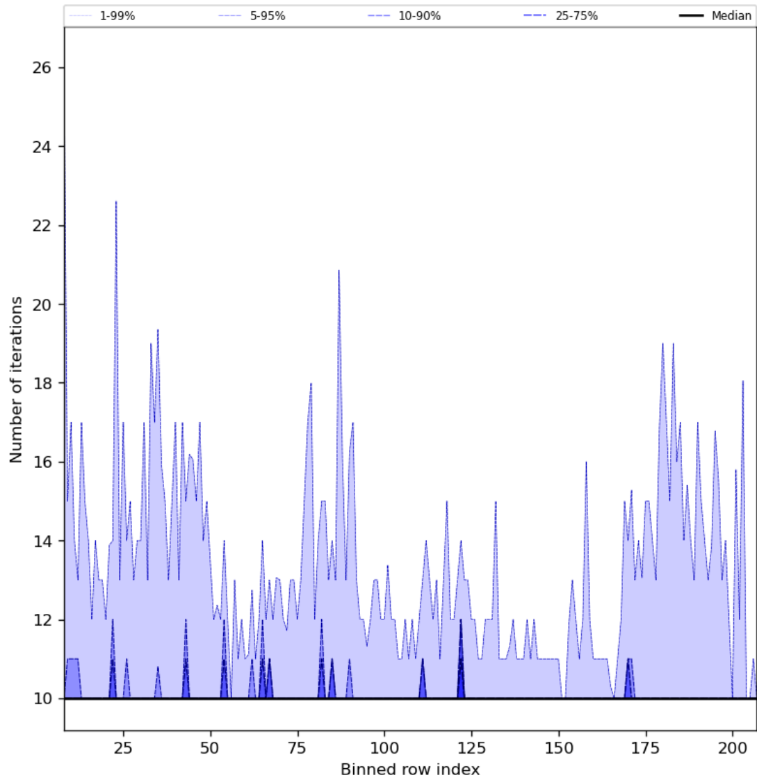
Figure 42: Along track statistics of “Number of iterations” for 2024-03-14 to 2024-03-15
