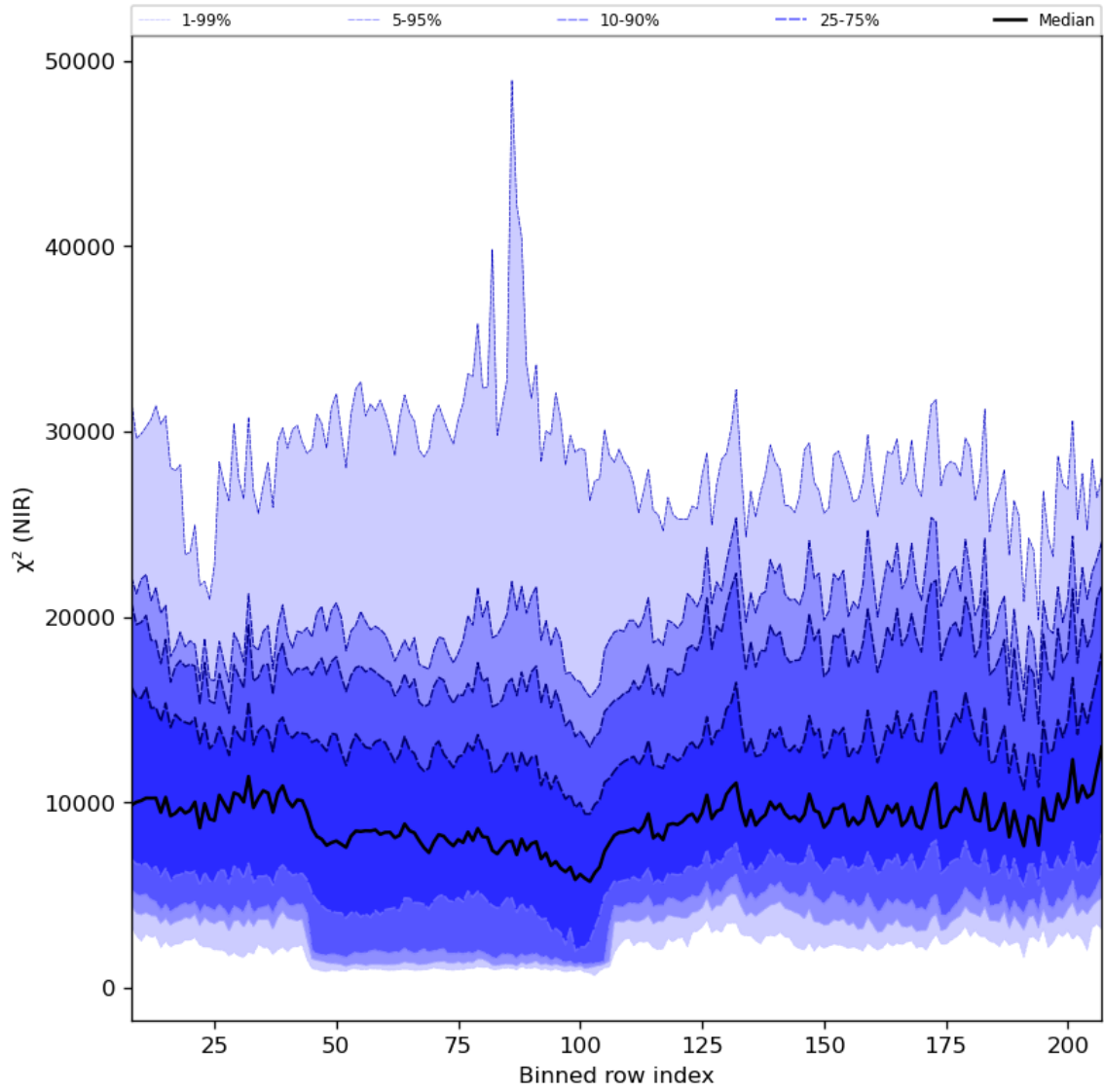
Figure 40: Along track statistics of “ \chi^2 (NIR)” for 2024-03-14 to 2024-03-15
