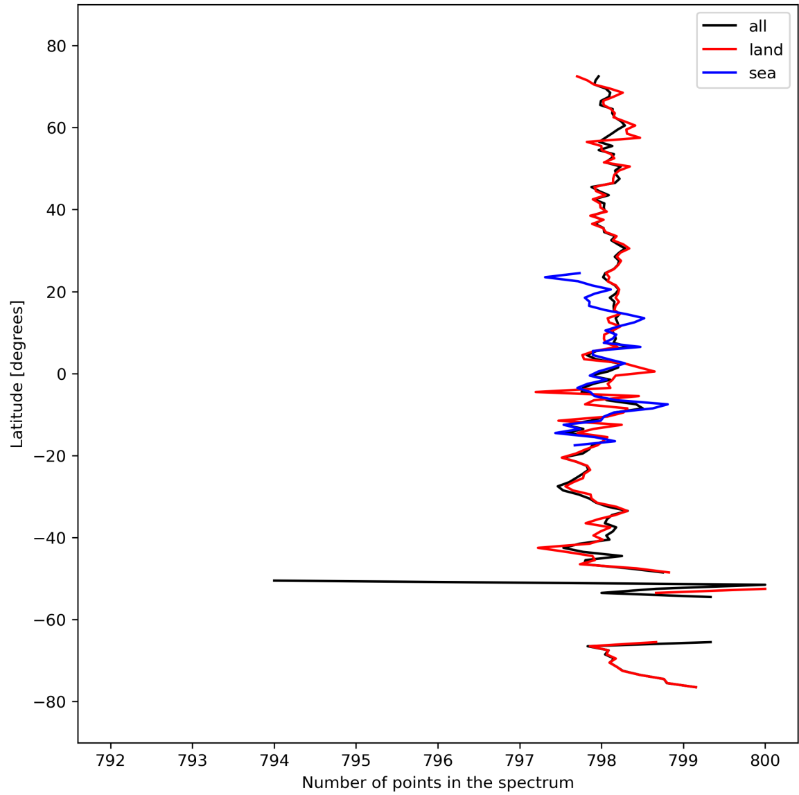
Figure 15: Zonal average of “Number of points in the spectrum” for 2024-03-14 to 2024-03-15.
