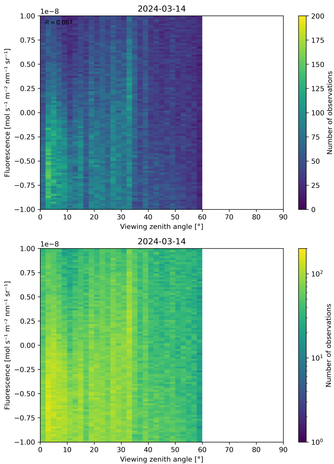
Figure 108: Scatter density plot of “Viewing zenith angle” against “Fluorescence” for 2024-03-14 to 2024-03-15.
