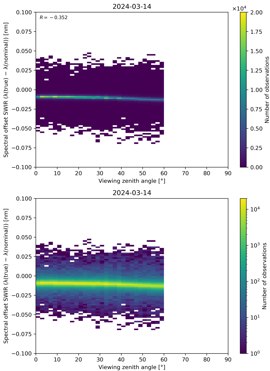
Figure 116: Scatter density plot of “Viewing zenith angle” against “Spectral offset SWIR ( \lambda(\text{true}) - \lambda(\text{nominal}) )” for 2024-03-14 to 2024-03-15.
