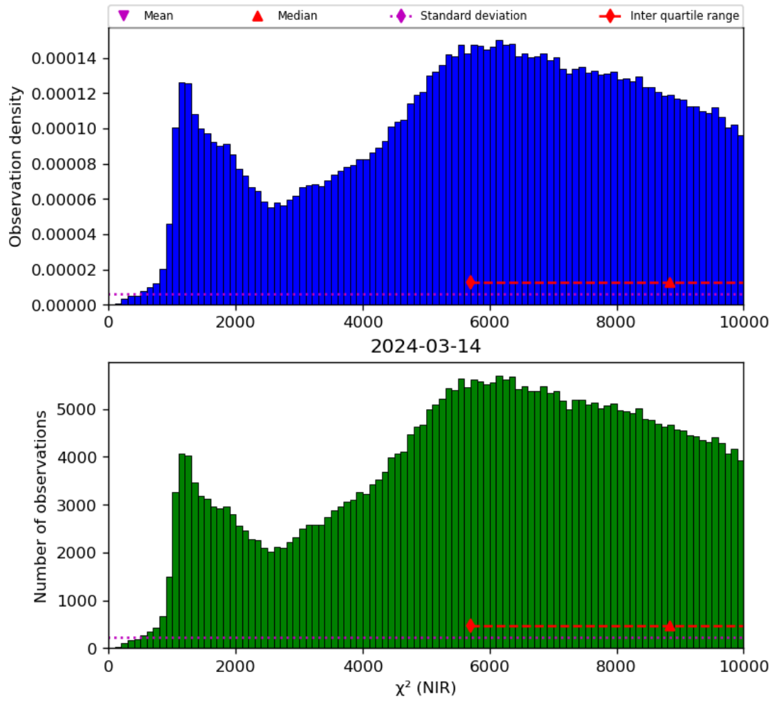
Figure 29: Histogram of “ \chi^2 (NIR)” for 2024-03-14 to 2024-03-15
