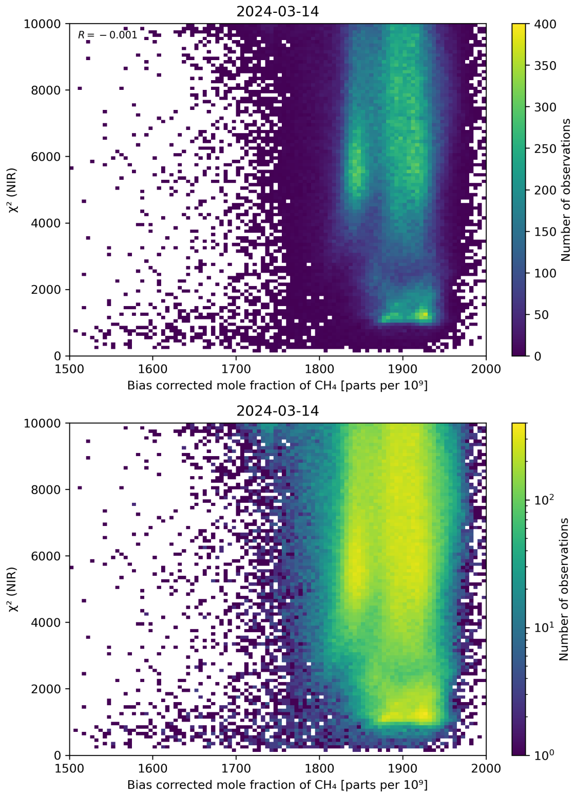
Figure 63: Scatter density plot of “Bias corrected mole fraction of CH 4 ” against “ \chi^2 (NIR)” for 2024-03-14 to 2024-03-15.
