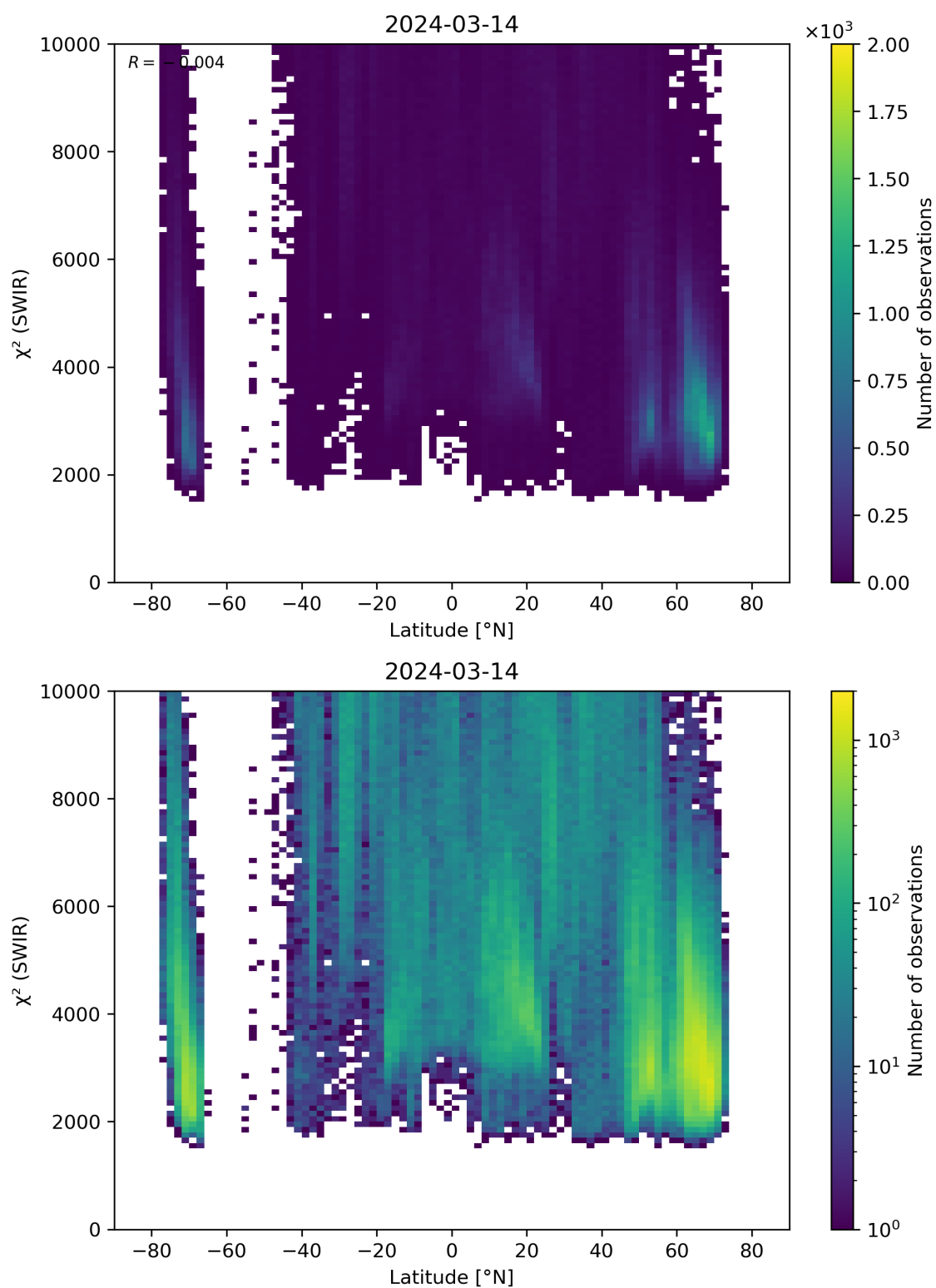
Figure 54: Scatter density plot of “Latitude” against “ \chi^2 (SWIR)” for 2024-03-14 to 2024-03-15.
