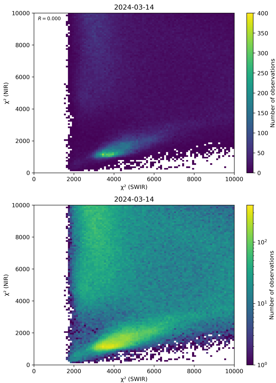
Figure 47: Scatter density plot of “ \chi^2 (SWIR)” against “ \chi^2 (NIR)” for 2024-03-14 to 2024-03-15.
