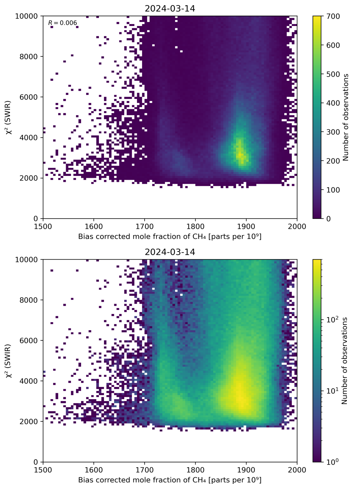
Figure 64: Scatter density plot of “Bias corrected mole fraction of CH 4 ” against “ \chi^2 (SWIR)” for 2024-03-14 to 2024-03-15.
