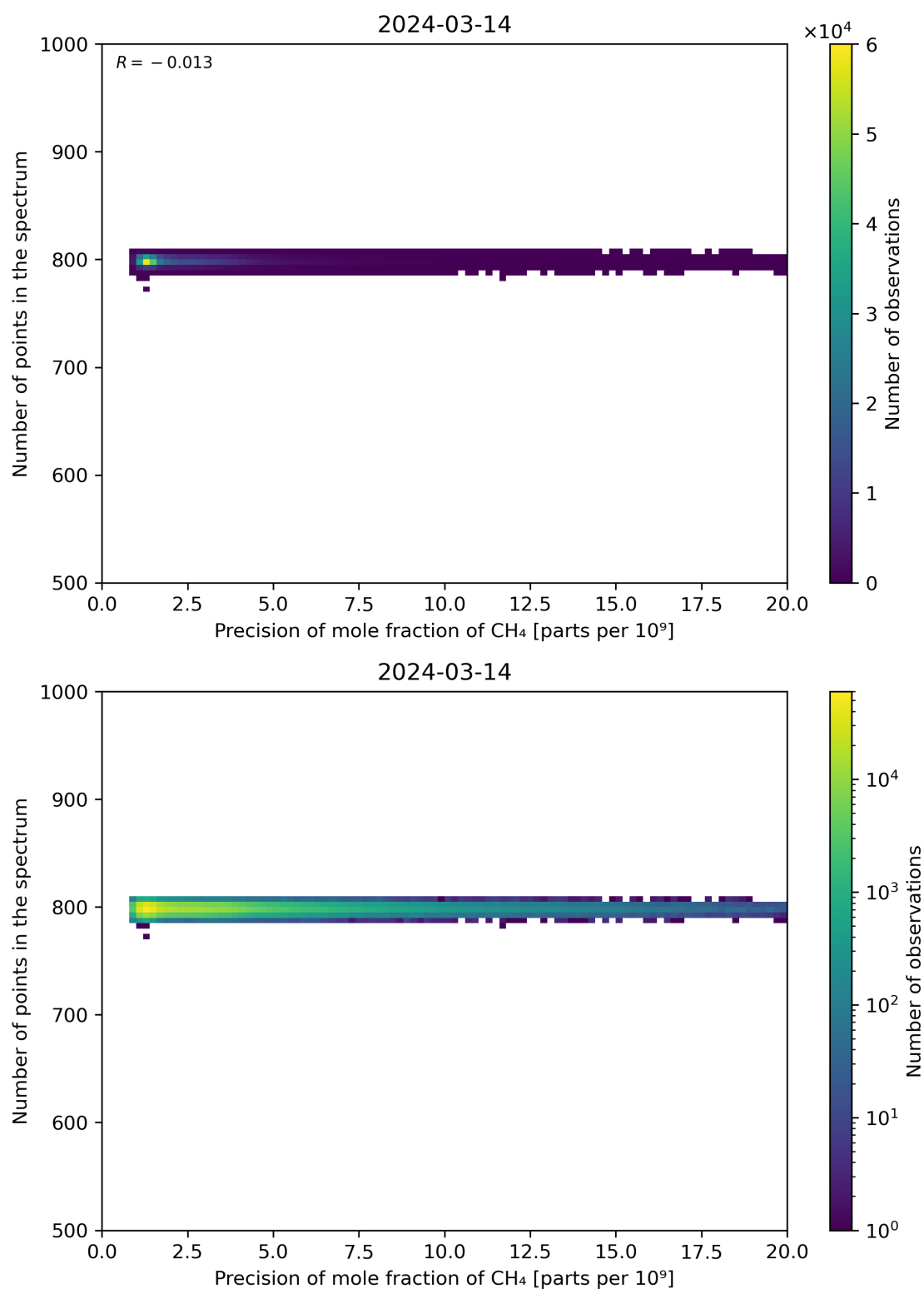
Figure 84: Scatter density plot of “Precision of mole fraction of CH 4 ” against “Number of points in the spectrum” for 2024-03-14 to 2024-03-15.
