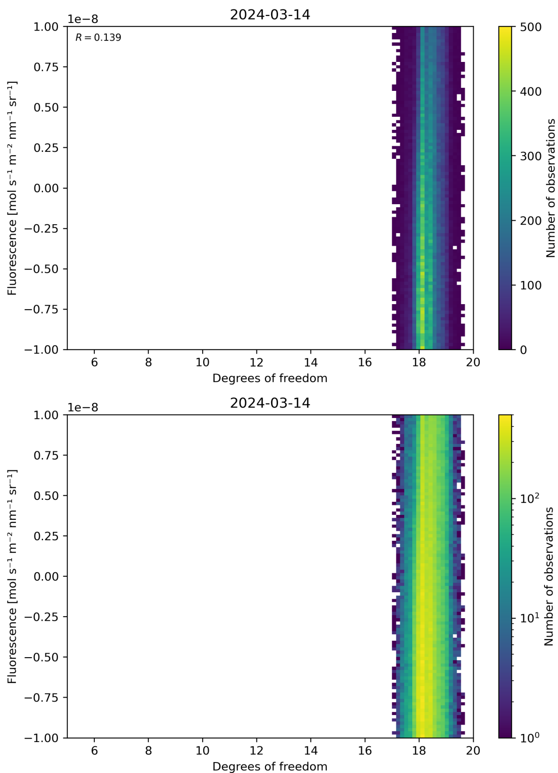
Figure 51: Scatter density plot of “Degrees of freedom” against “Fluorescence” for 2024-03-14 to 2024-03-15.
