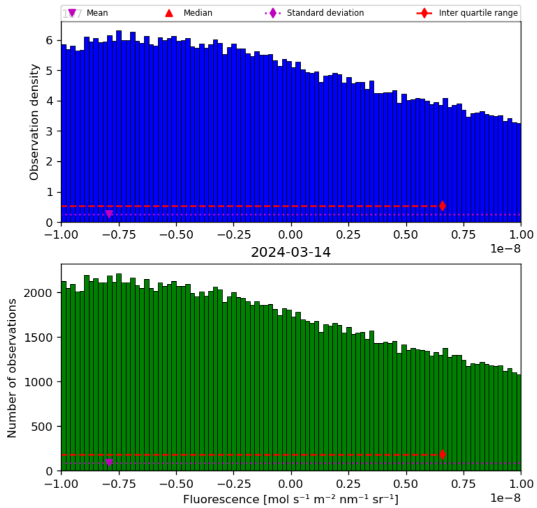
Figure 32: Histogram of “Fluorescence” for 2024-03-14 to 2024-03-15
