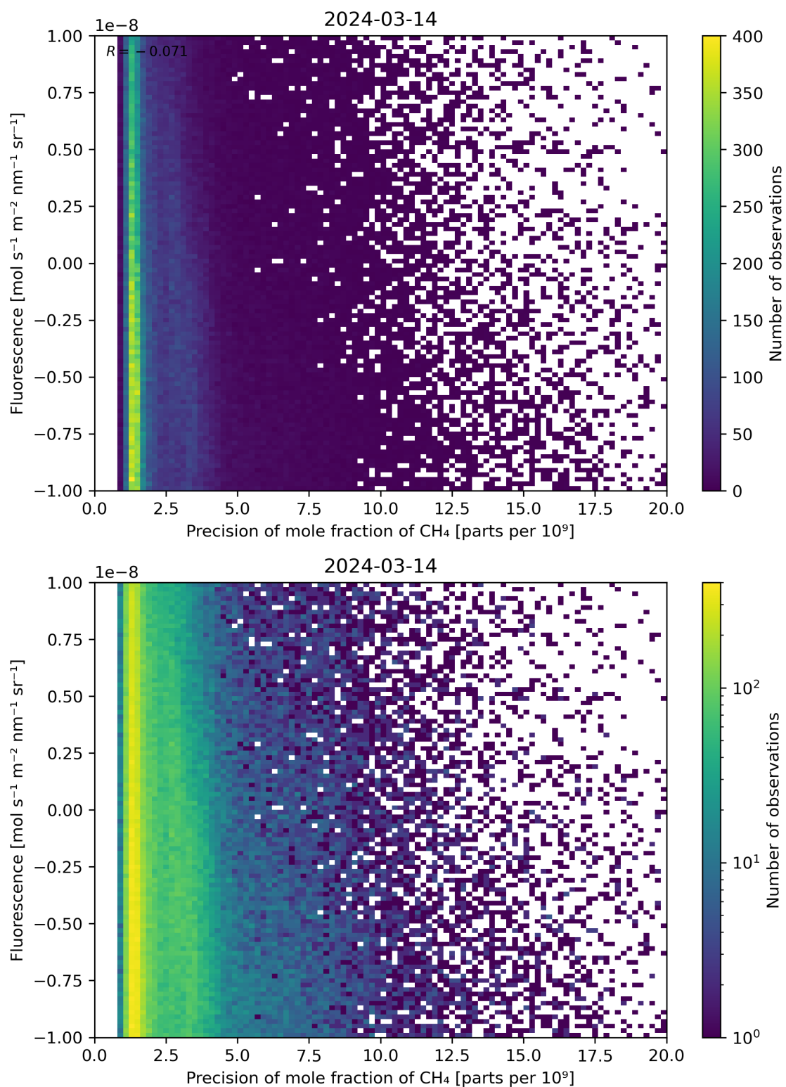
Figure 81: Scatter density plot of “Precision of mole fraction of \text{CH}_4 ” against “Fluorescence” for 2024-03-14 to 2024-03-15.
