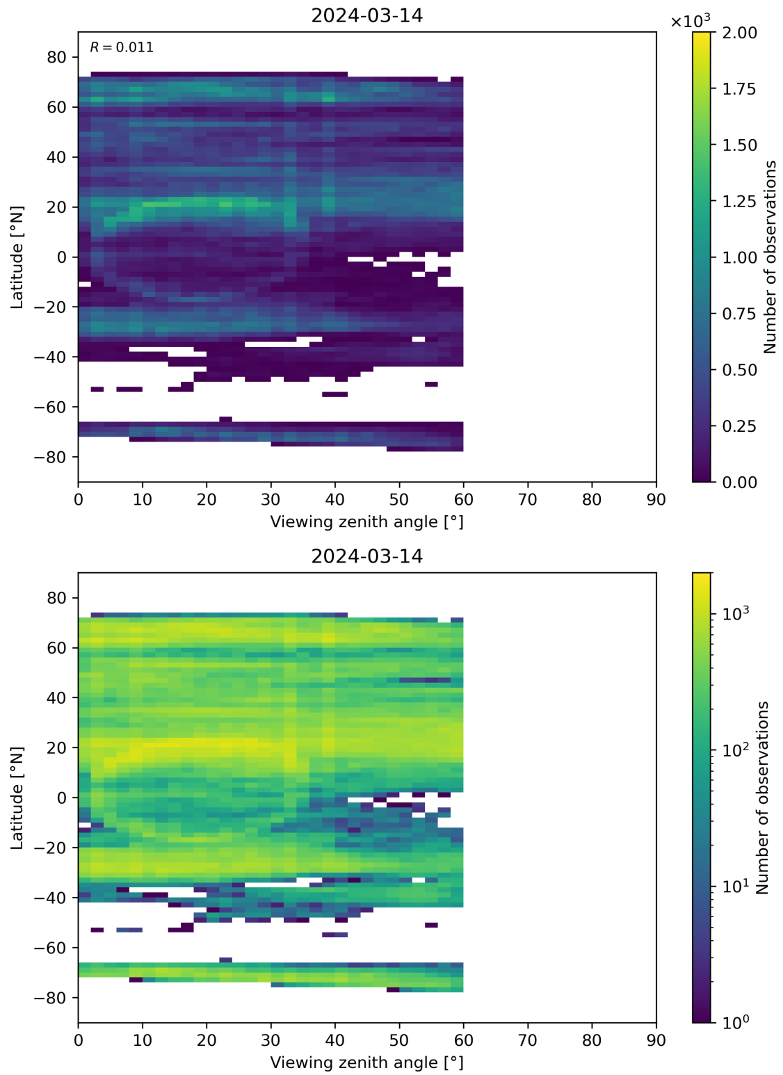
Figure 109: Scatter density plot of “Viewing zenith angle” against “Latitude” for 2024-03-14 to 2024-03-15.
