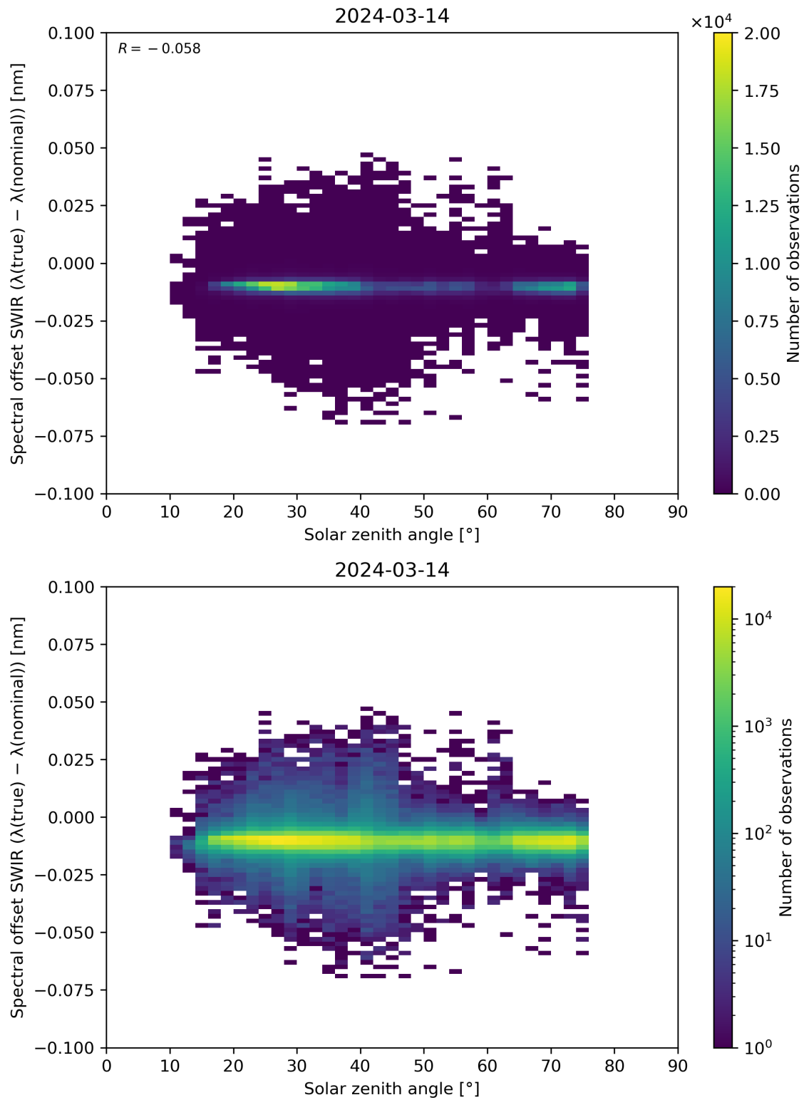
Figure 104: Scatter density plot of “Solar zenith angle” against “Spectral offset SWIR ( \lambda(\text{true}) - \lambda(\text{nominal}) )” for 2024-03-14 to 2024-03-15.
