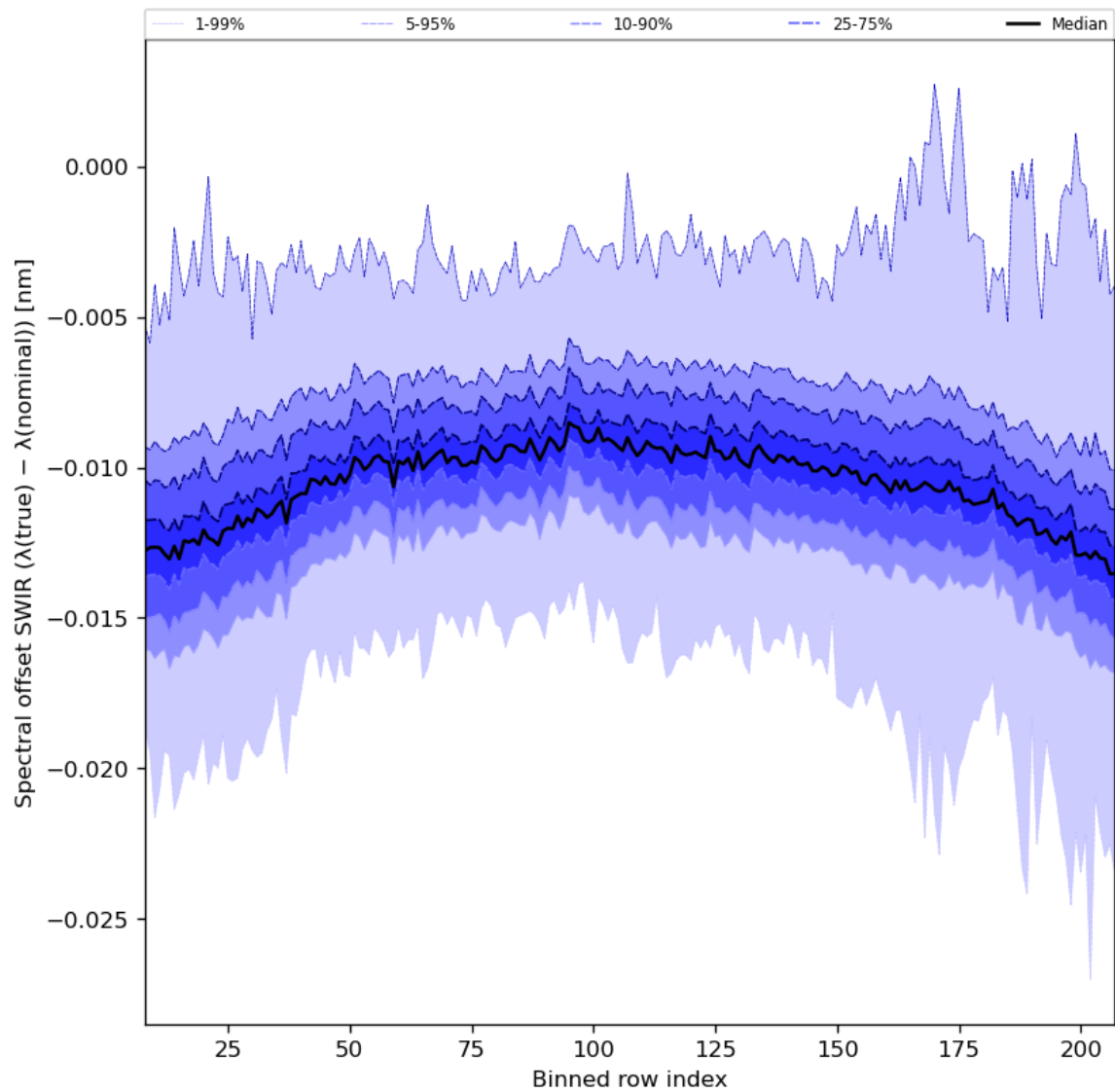
Figure 38: Along track statistics of “Spectral offset SWIR ( \lambda(\text{true}) - \lambda(\text{nominal}) )” for 2024-03-14 to 2024-03-15
