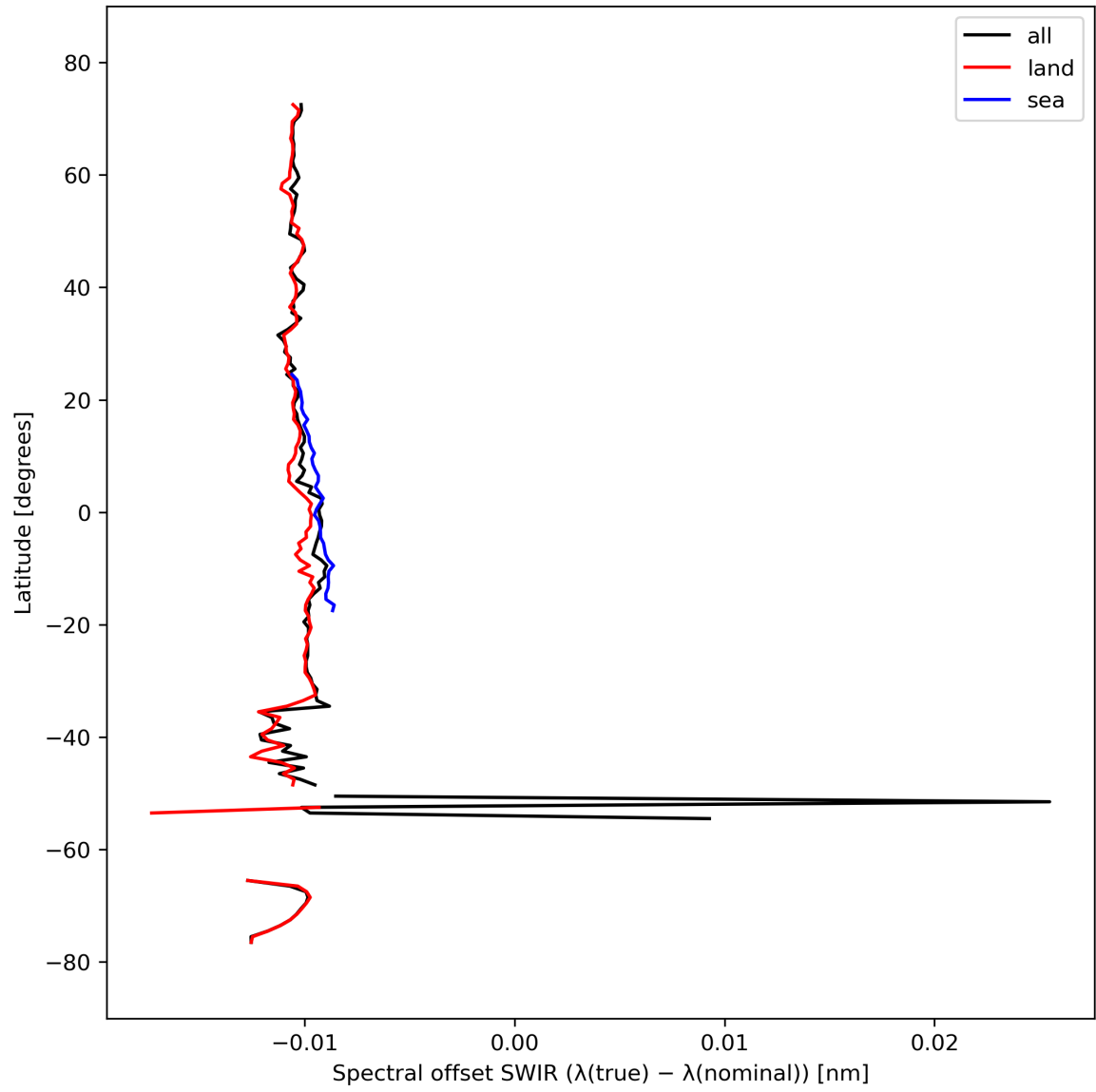
Figure 16: Zonal average of “Spectral offset SWIR ( \lambda(\text{true}) - \lambda(\text{nominal}) )” for 2024-03-14 to 2024-03-15.
