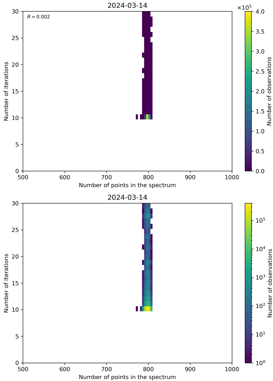
Figure 92: Scatter density plot of “Number of points in the spectrum” against “Number of iterations” for 2024-03-14 to 2024-03-15.
