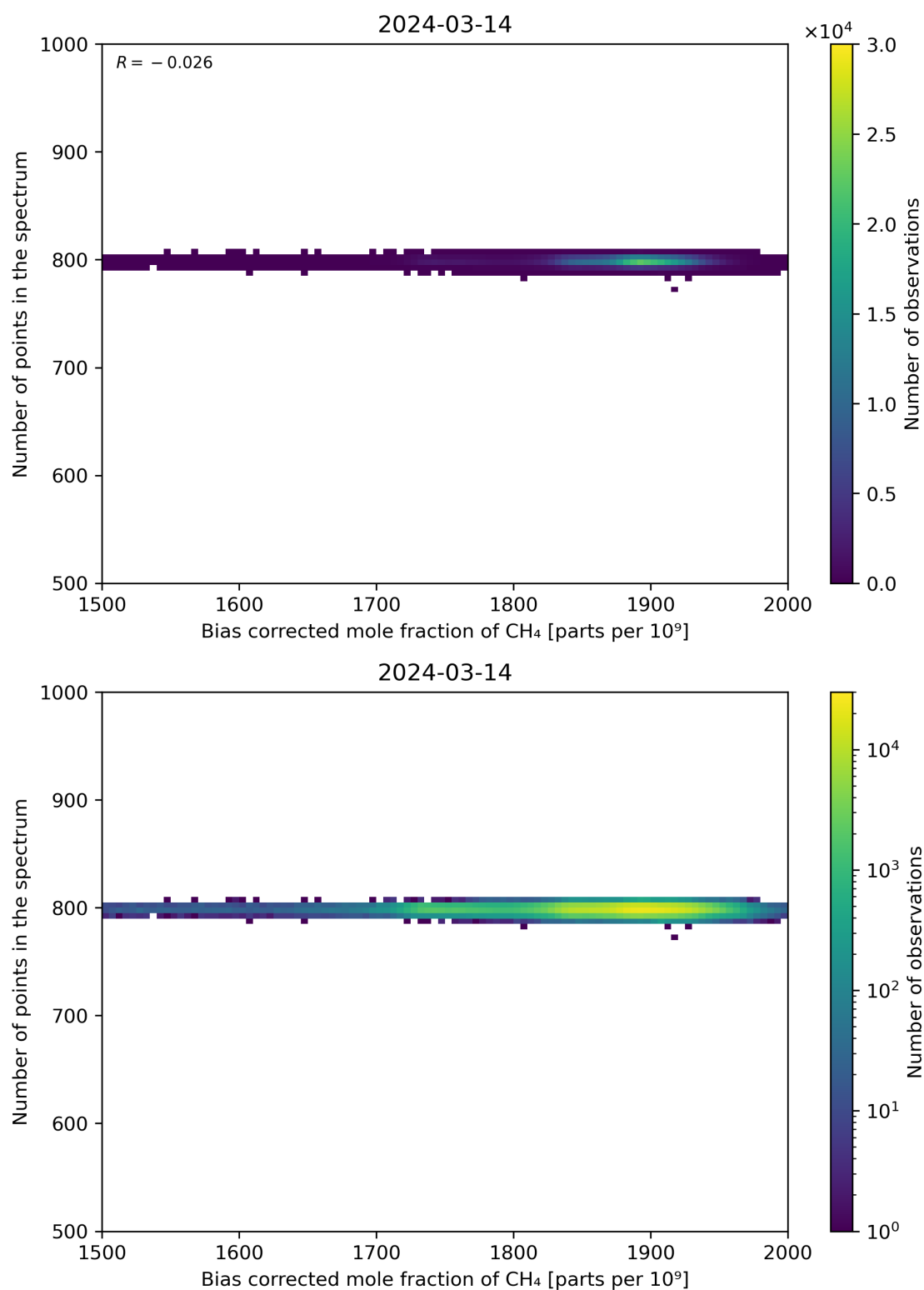
Figure 68: Scatter density plot of “Bias corrected mole fraction of CH 4 ” against “Number of points in the spectrum” for 2024-03-14 to 2024-03-15.
