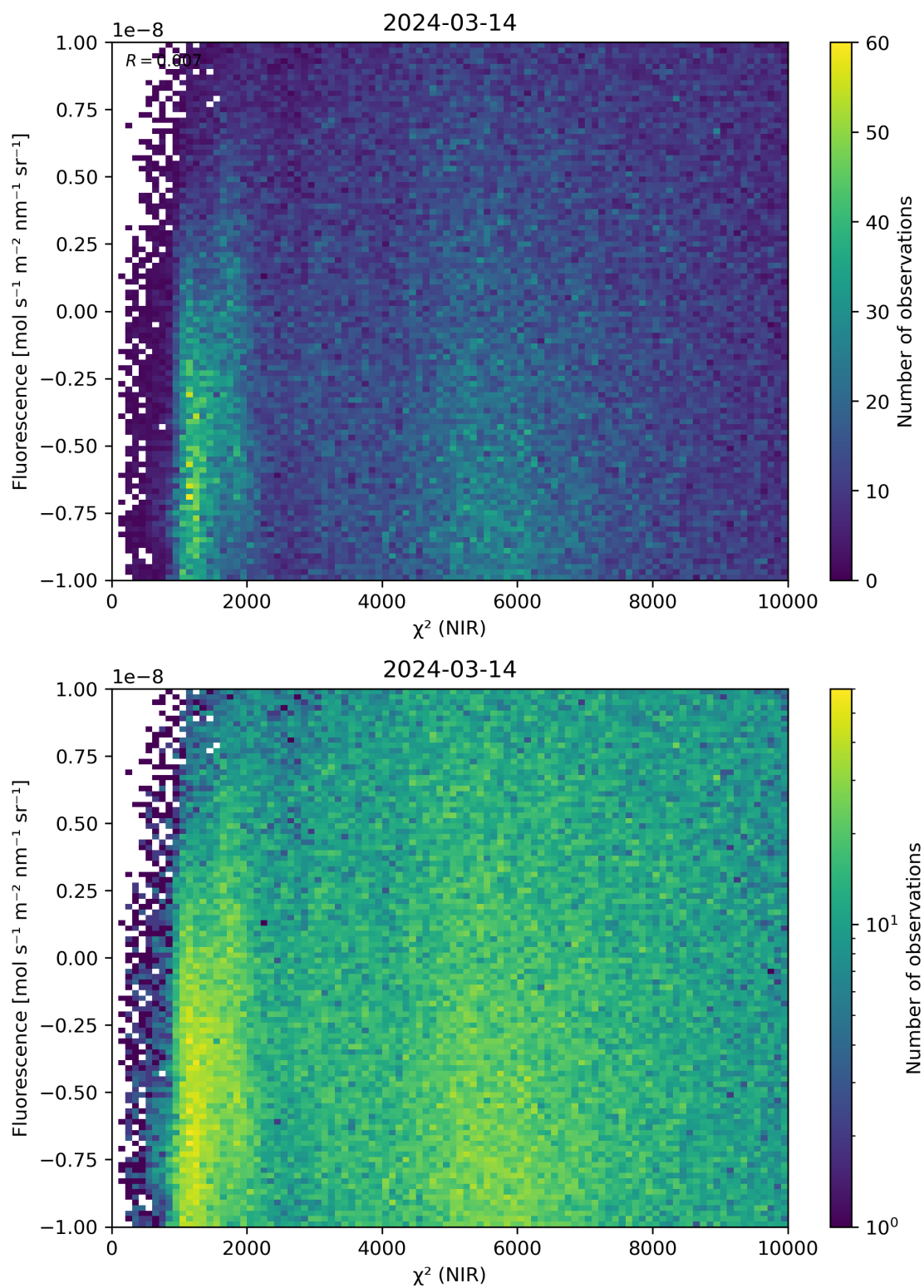
Figure 45: Scatter density plot of “ \chi^2 (NIR)” against “Fluorescence” for 2024-03-14 to 2024-03-15.
