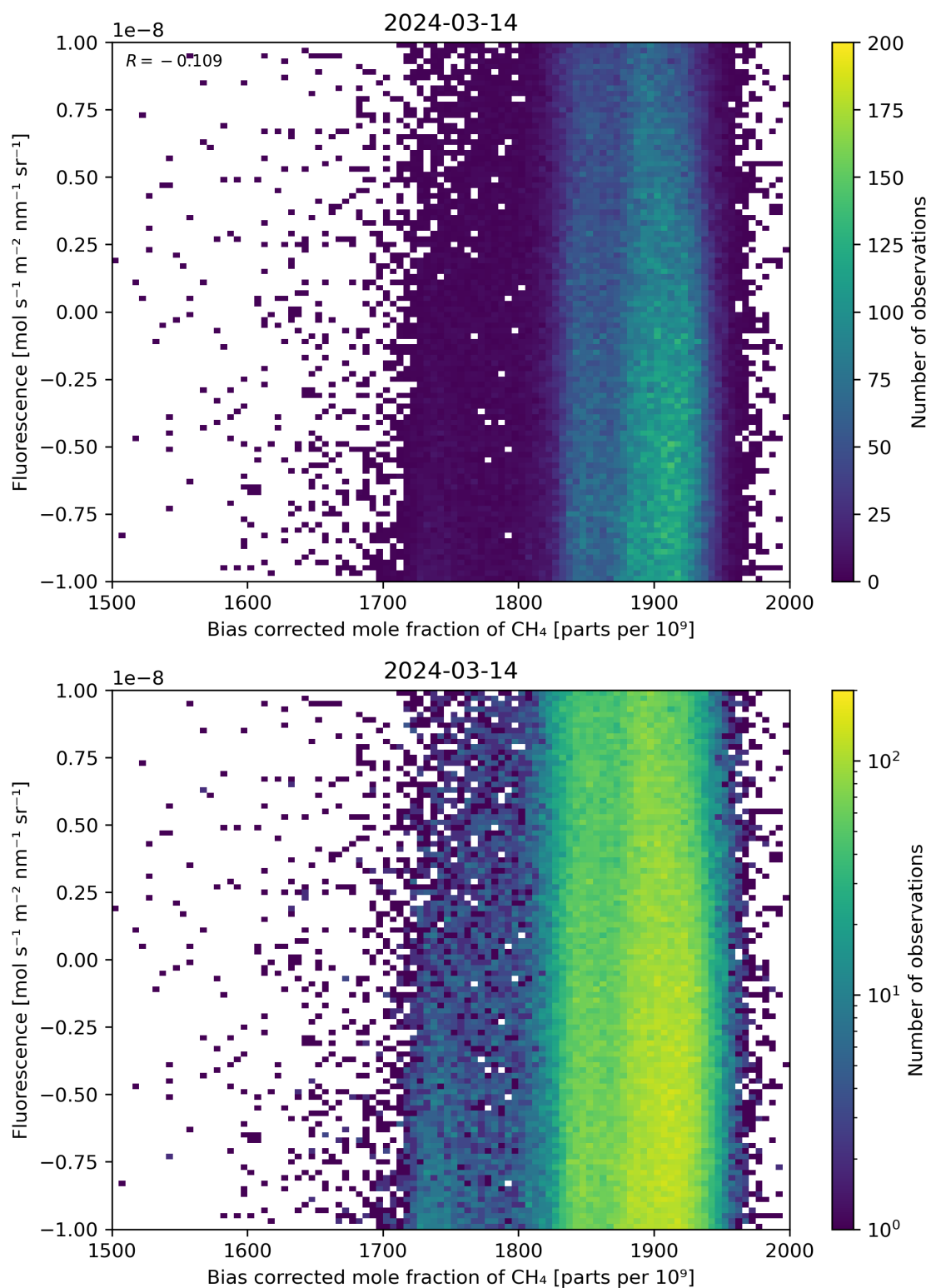
Figure 66: Scatter density plot of “Bias corrected mole fraction of \text{CH}_4 ” against “Fluorescence” for 2024-03-14 to 2024-03-15.
