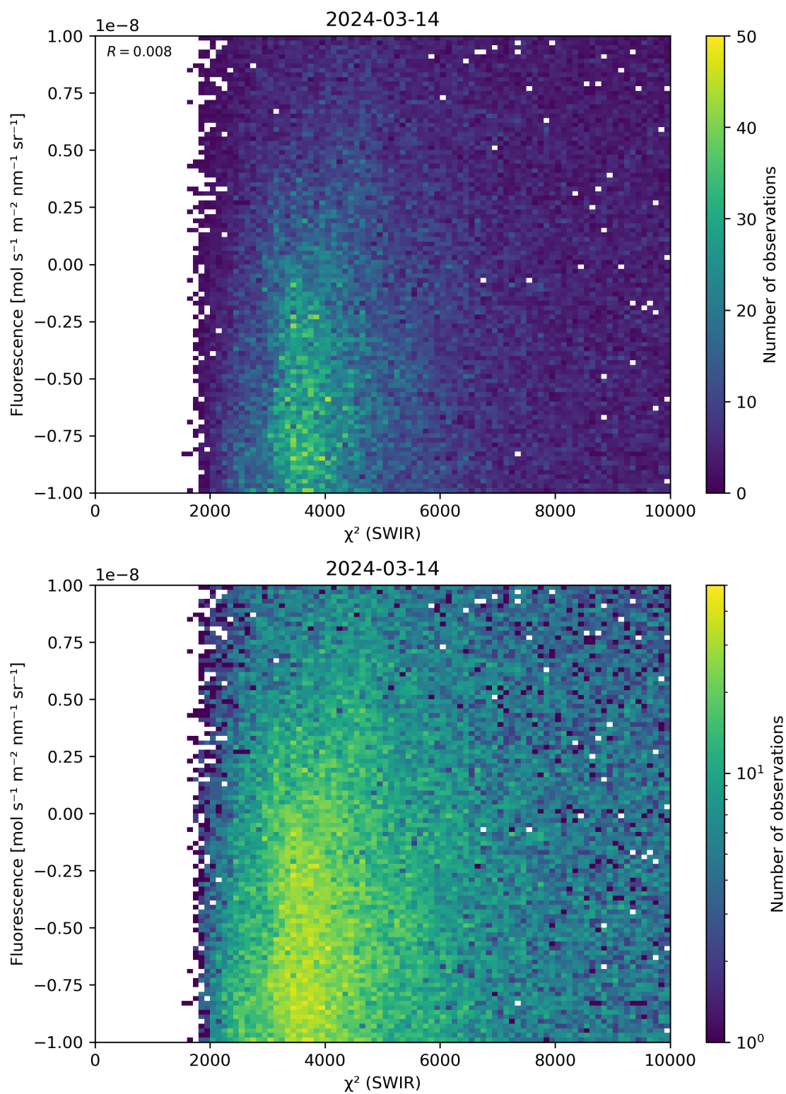
Figure 49: Scatter density plot of “ \chi^2 (SWIR)” against “Fluorescence” for 2024-03-14 to 2024-03-15.
