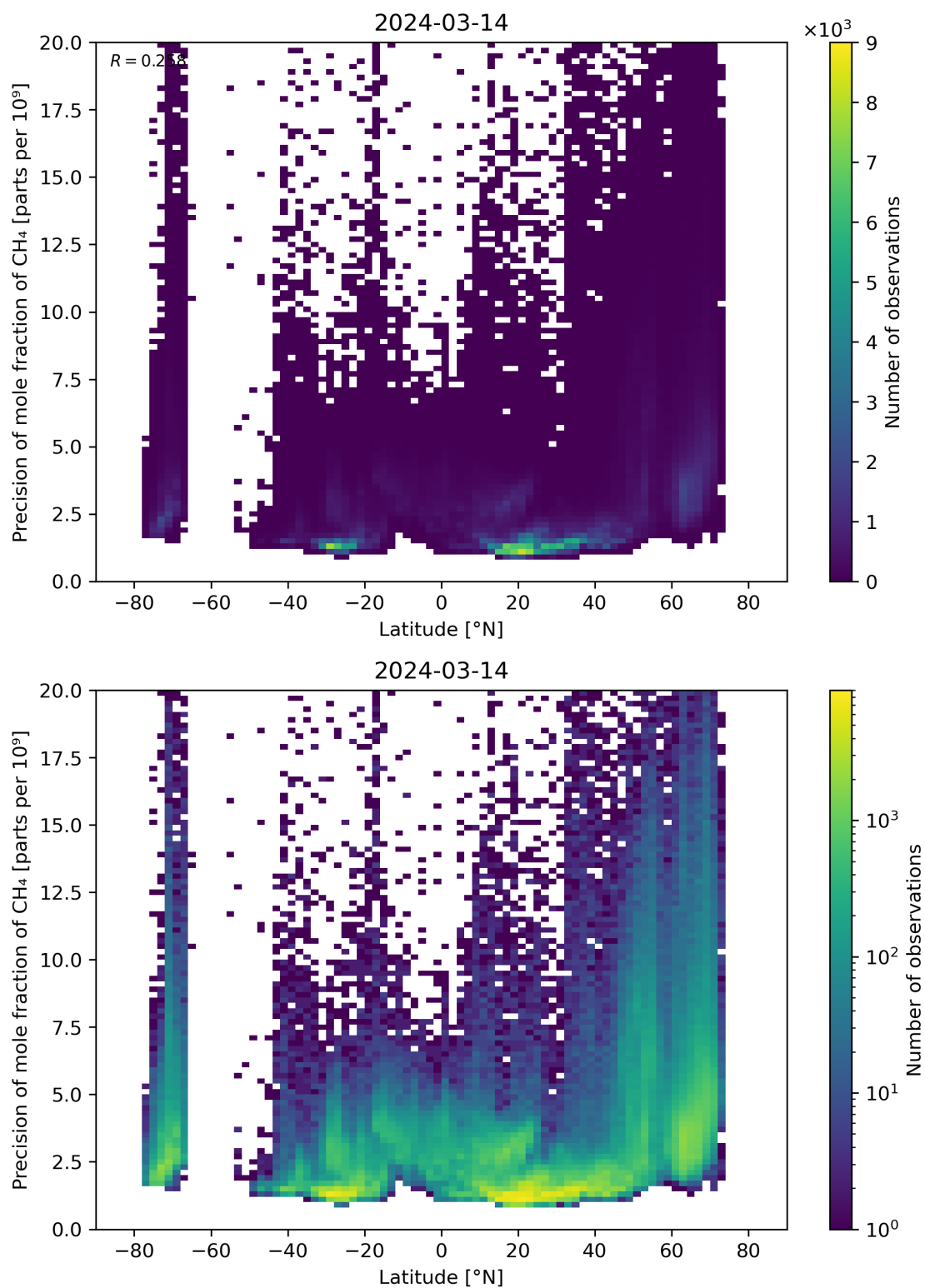
Figure 59: Scatter density plot of “Latitude” against “Precision of mole fraction of CH 4 ” for 2024-03-14 to 2024-03-15.
