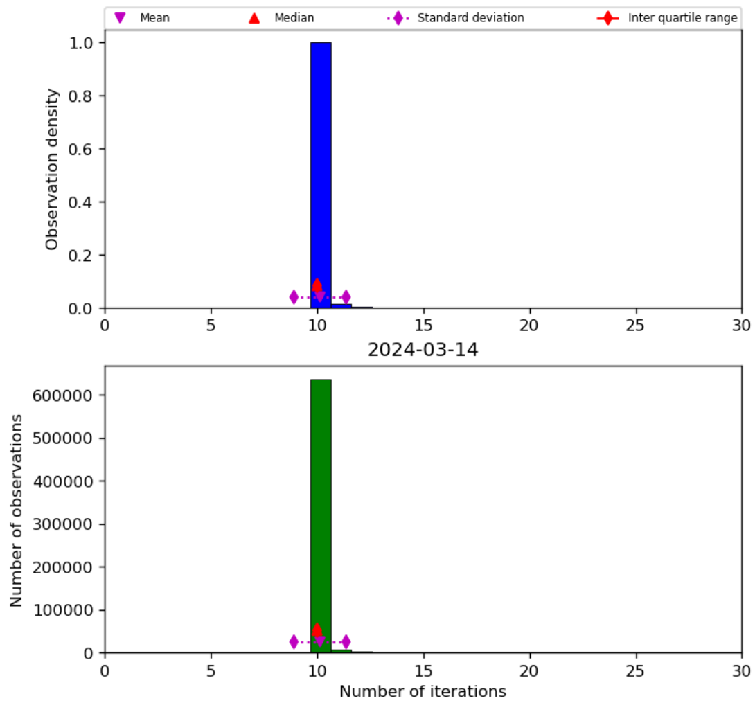
Figure 31: Histogram of “Number of iterations” for 2024-03-14 to 2024-03-15
