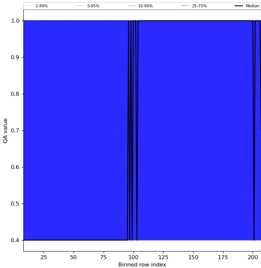
Figure 33: Along track statistics of “QA value” for 2024-03-14 to 2024-03-15
