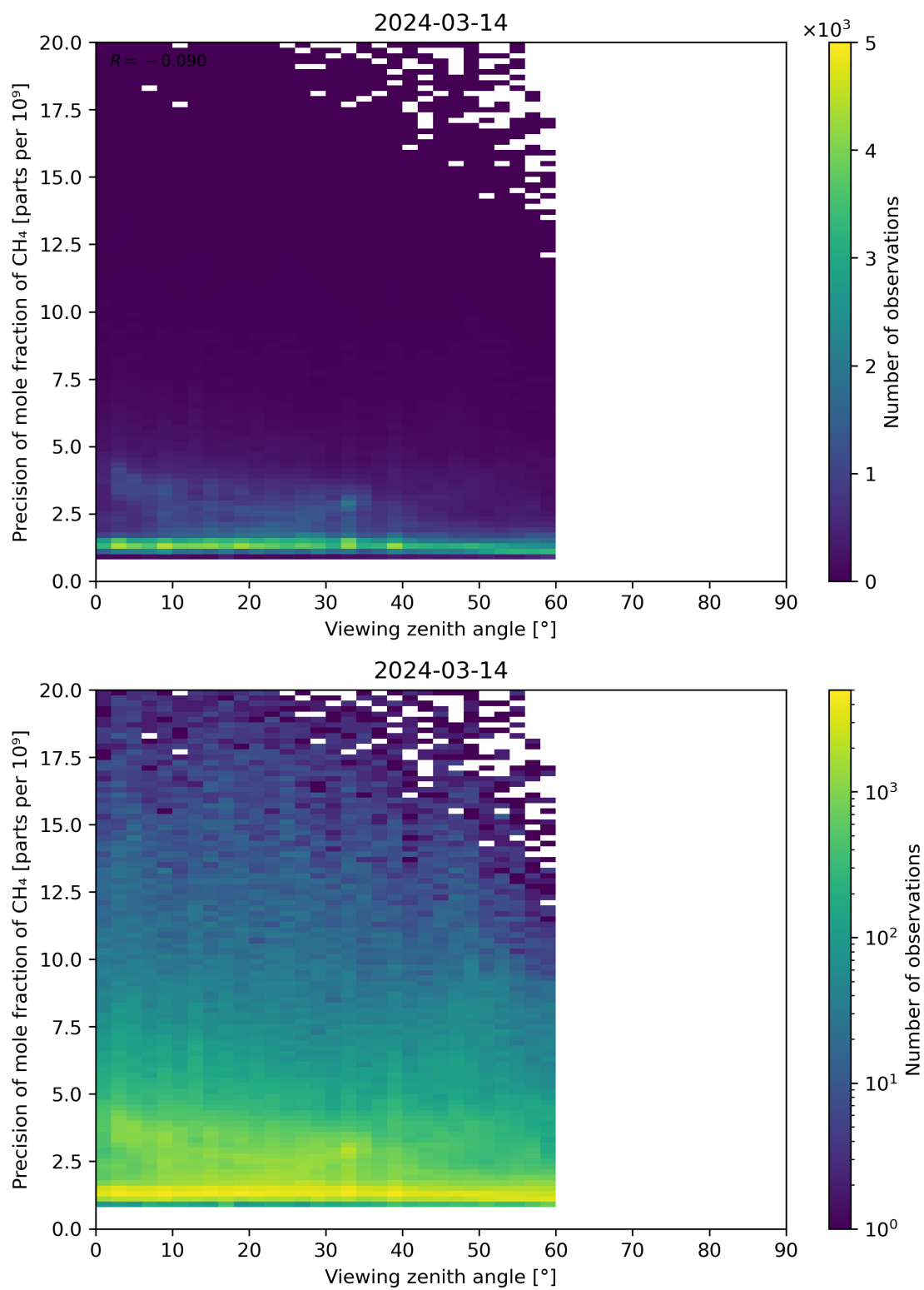
Figure 112: Scatter density plot of “Viewing zenith angle” against “Precision of mole fraction of CH 4 ” for 2024-03-14 to 2024-03-15.
