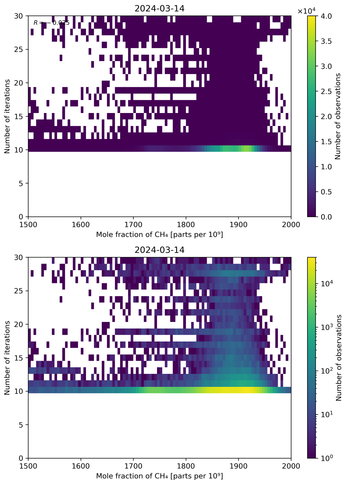
Figure 76: Scatter density plot of “Mole fraction of CH 4 ” against “Number of iterations” for 2024-03-14 to 2024-03-15.
