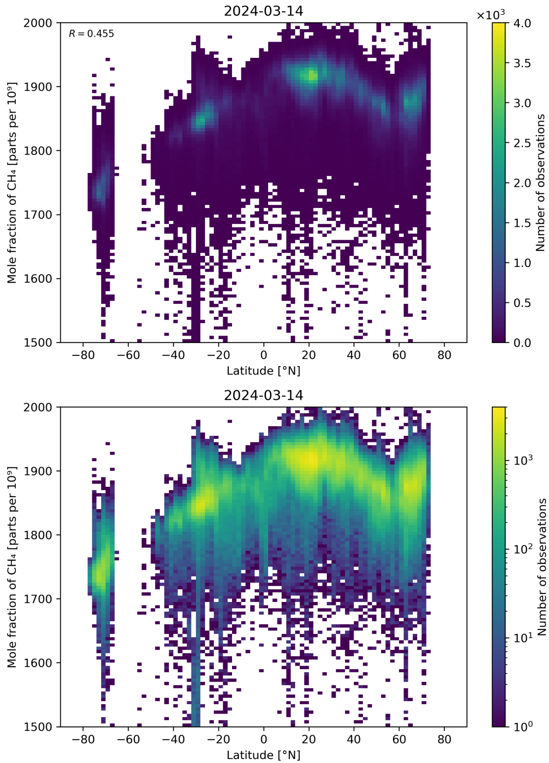
Figure 57: Scatter density plot of “Latitude” against “Mole fraction of CH 4 ” for 2024-03-14 to 2024-03-15.
