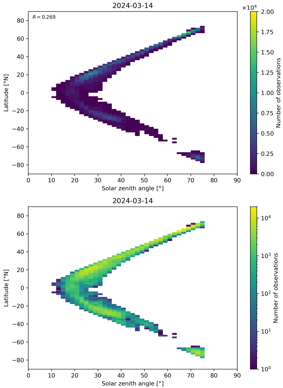
Figure 98: Scatter density plot of “Solar zenith angle” against “Latitude” for 2024-03-14 to 2024-03-15.
