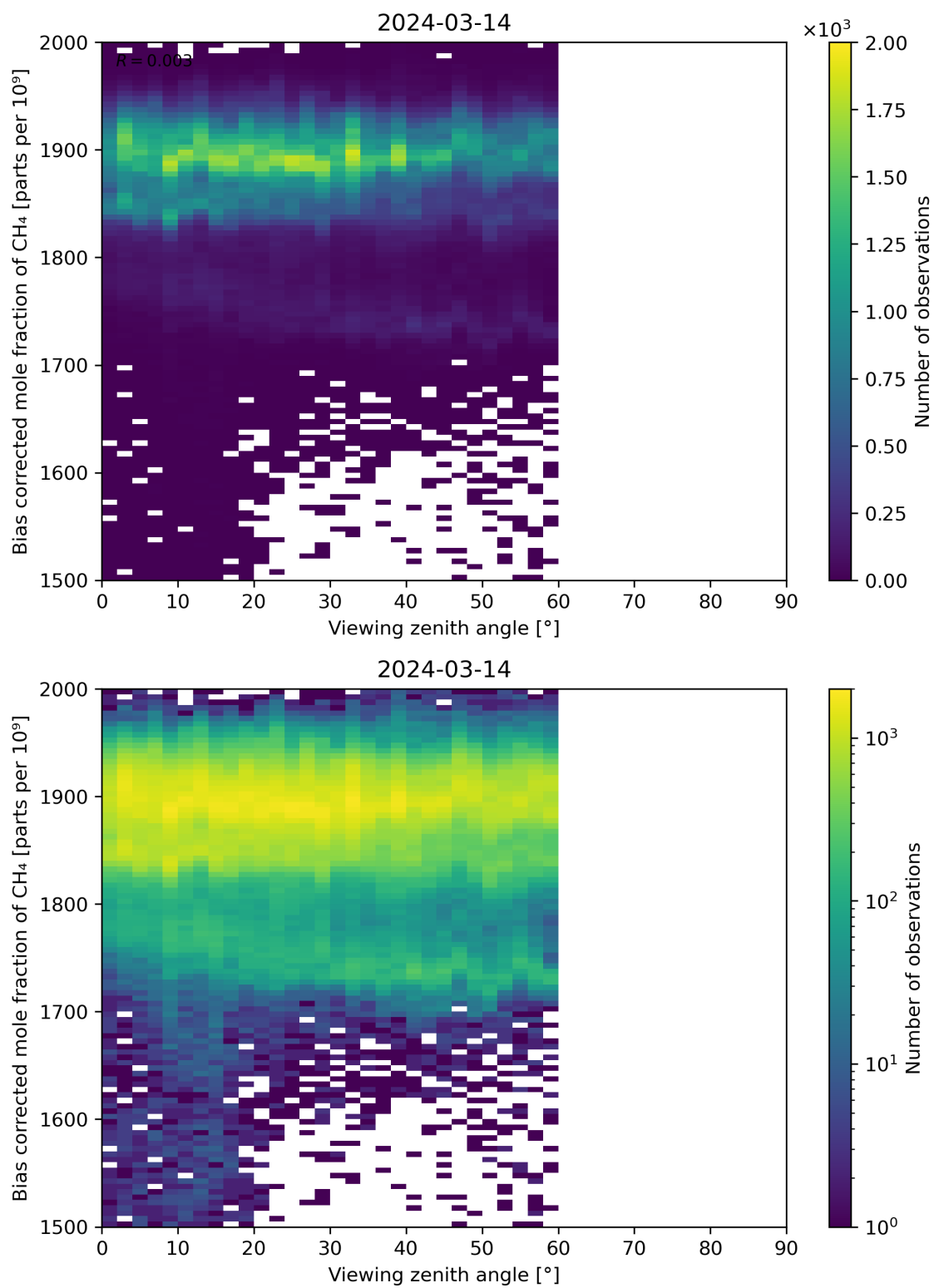
Figure 111: Scatter density plot of “Viewing zenith angle” against “Bias corrected mole fraction of CH 4 ” for 2024-03-14 to 2024-03-15.
