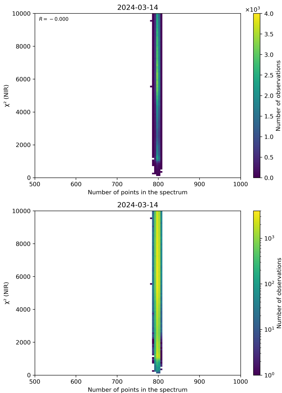
Figure 88: Scatter density plot of “Number of points in the spectrum” against “ \chi^2 (NIR)” for 2024-03-14 to 2024-03-15.
