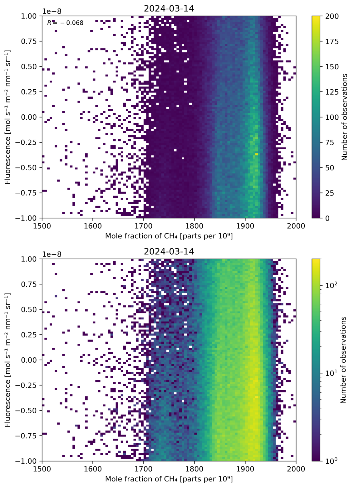
Figure 73: Scatter density plot of “Mole fraction of \text{CH}_4 ” against “Fluorescence” for 2024-03-14 to 2024-03-15.
