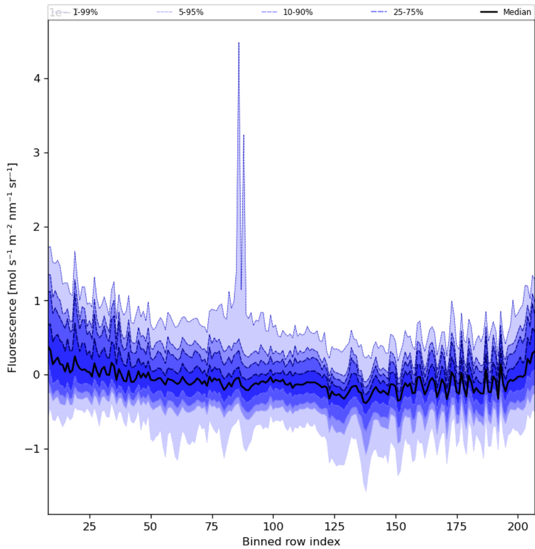
Figure 43: Along track statistics of “Fluorescence” for 2024-03-14 to 2024-03-15
