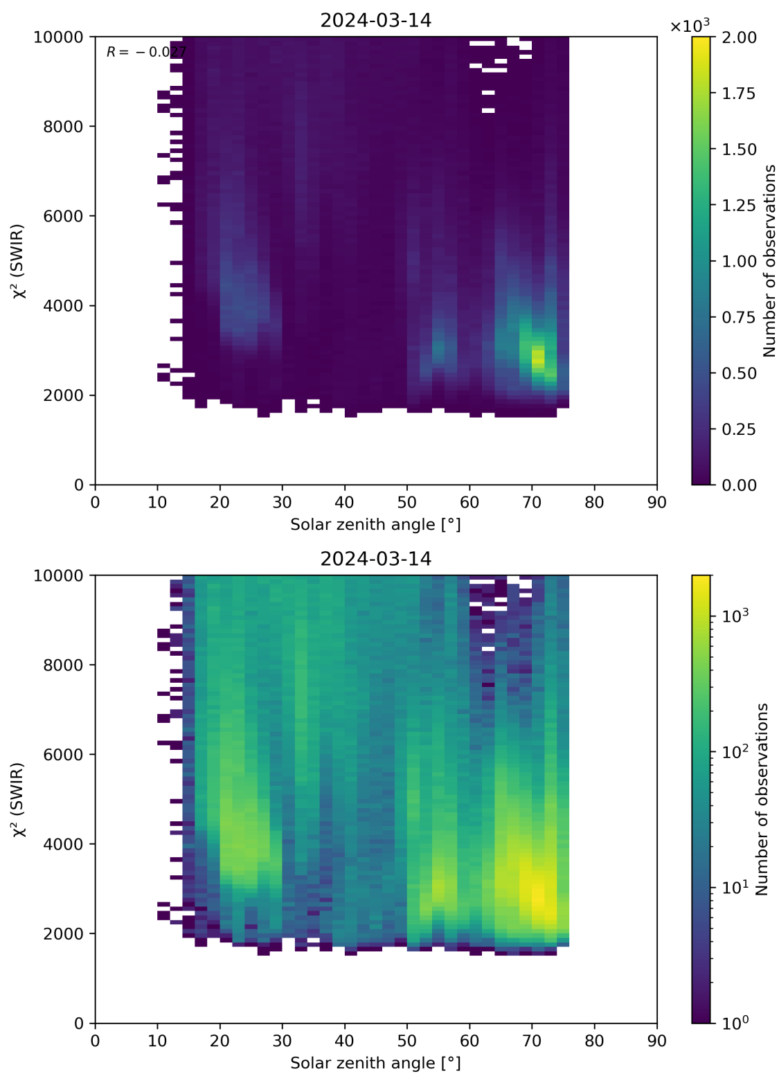
Figure 95: Scatter density plot of “Solar zenith angle” against “ \chi^2 (SWIR)” for 2024-03-14 to 2024-03-15.
