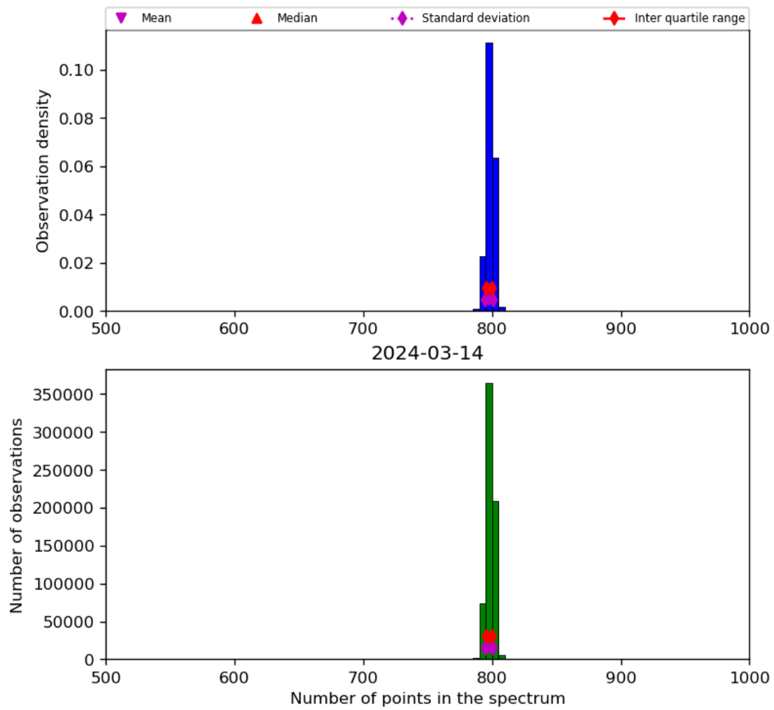
Figure 26: Histogram of “Number of points in the spectrum” for 2024-03-14 to 2024-03-15
