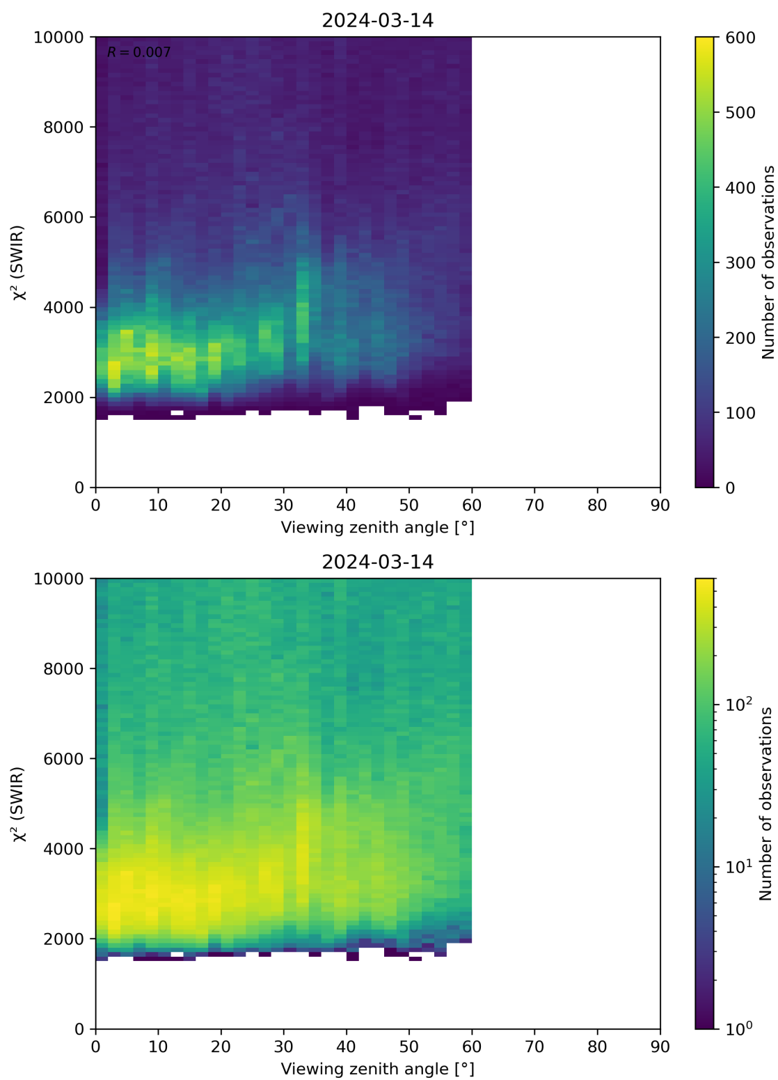
Figure 106: Scatter density plot of “Viewing zenith angle” against “ \chi^2 (SWIR)” for 2024-03-14 to 2024-03-15.
