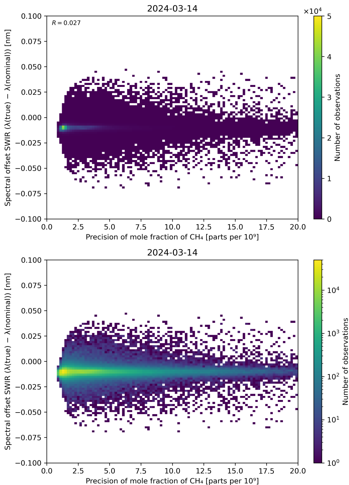
Figure 85: Scatter density plot of “Precision of mole fraction of \text{CH}_4 ” against “Spectral offset SWIR ( \lambda(\text{true}) - \lambda(\text{nominal}) )” for 2024-03-14 to 2024-03-15.
