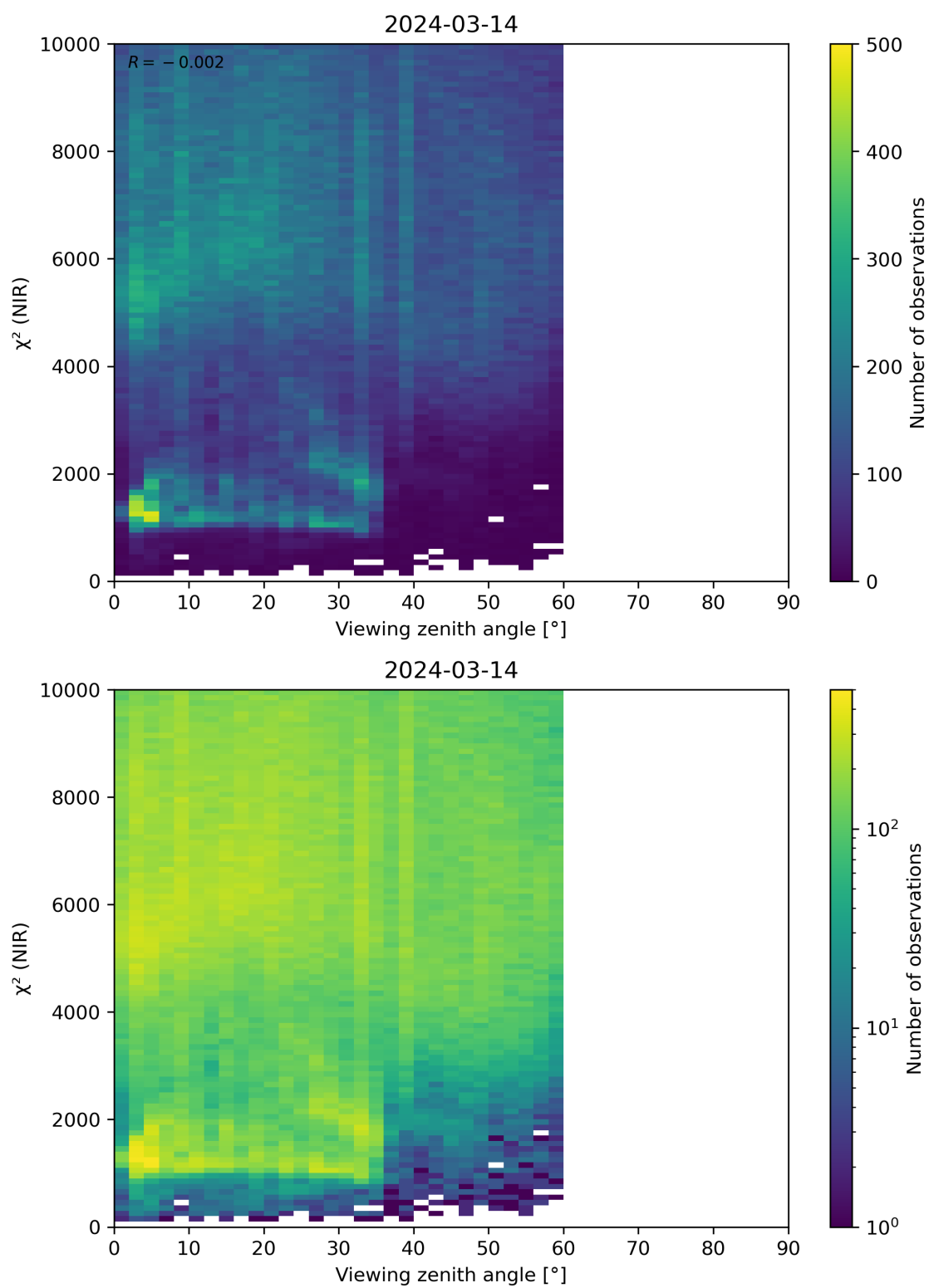
Figure 105: Scatter density plot of “Viewing zenith angle” against “ \chi^2 (NIR)” for 2024-03-14 to 2024-03-15.
