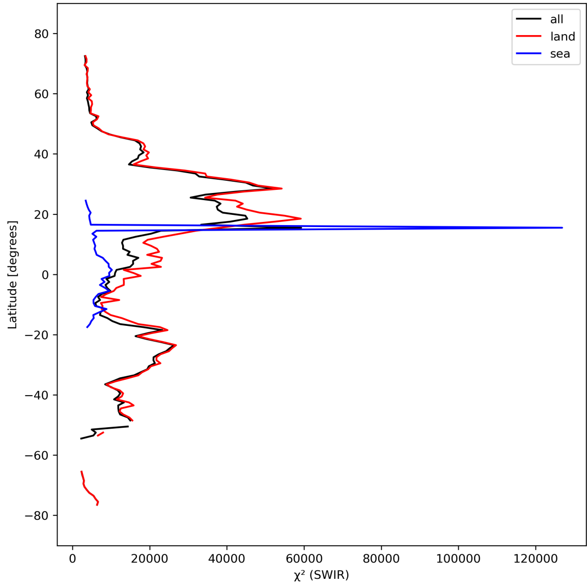
Figure 17: Zonal average of “ \chi^2 (SWIR)” for 2024-03-14 to 2024-03-15.
