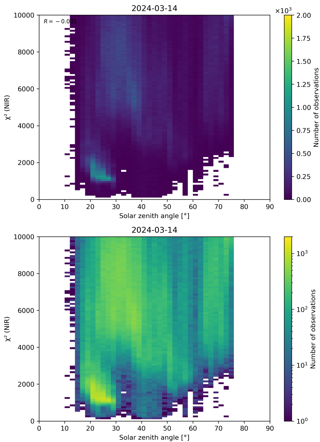
Figure 94: Scatter density plot of “Solar zenith angle” against “ \chi^2 (NIR)” for 2024-03-14 to 2024-03-15.
