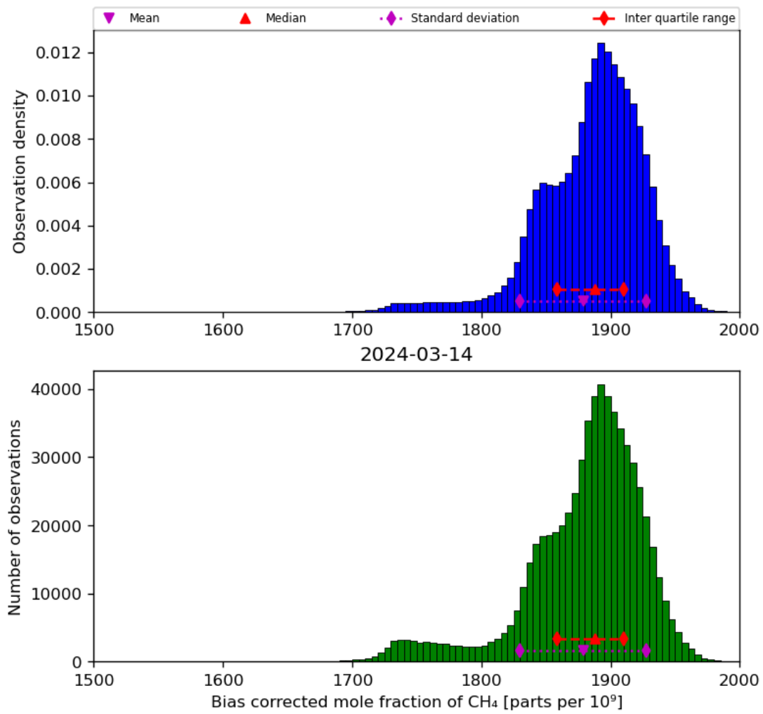
Figure 25: Histogram of “Bias corrected mole fraction of CH 4 ” for 2024-03-14 to 2024-03-15
