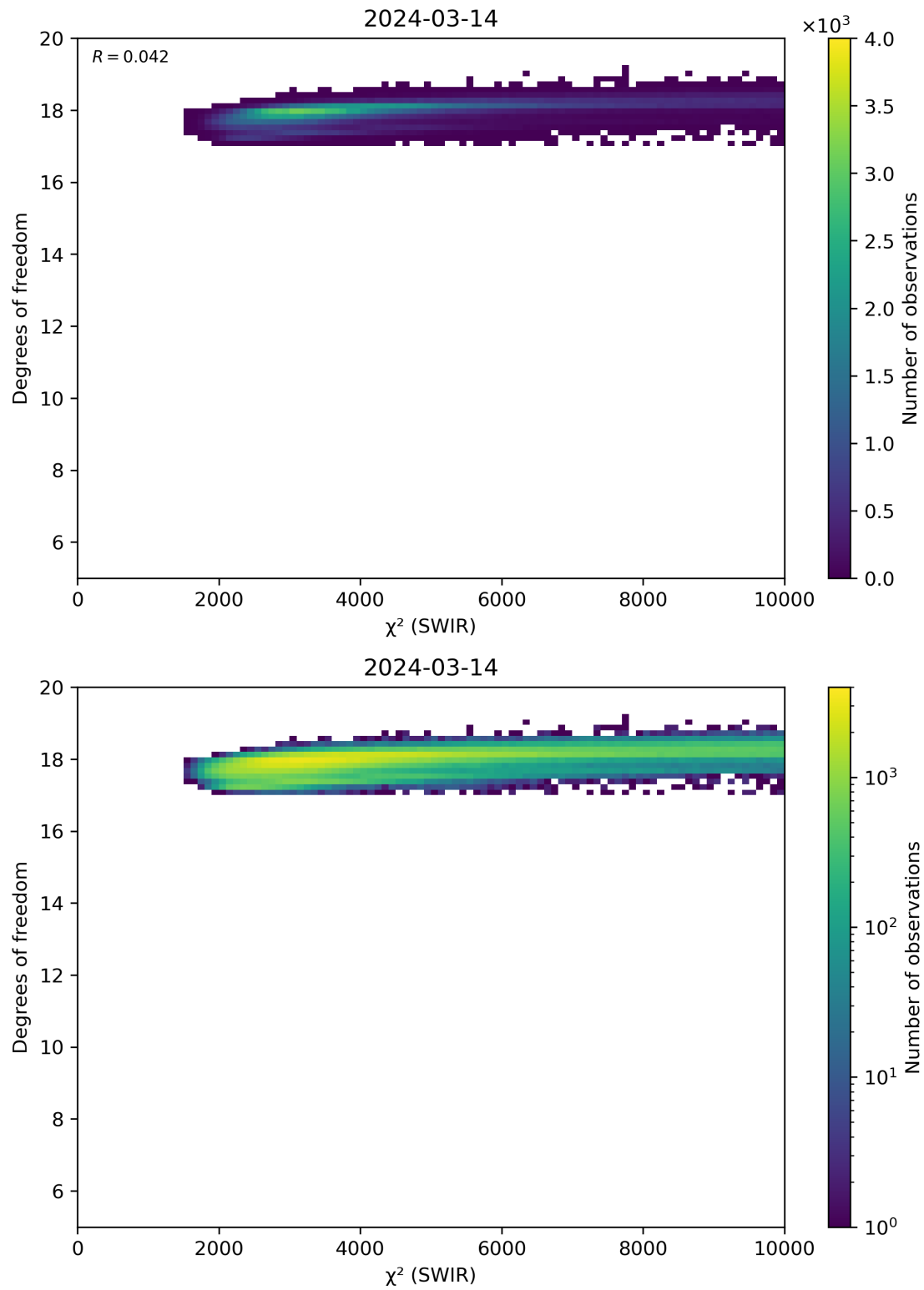
Figure 48: Scatter density plot of “ \chi^2 (SWIR)” against “Degrees of freedom” for 2024-03-14 to 2024-03-15.
