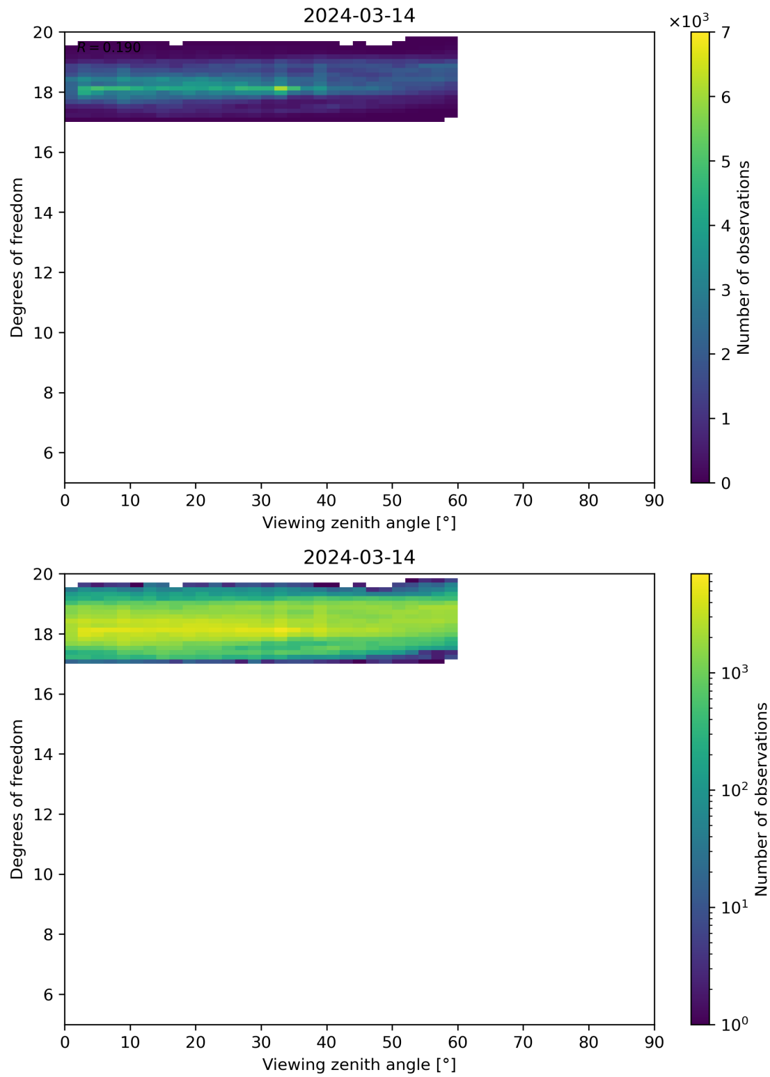
Figure 107: Scatter density plot of “Viewing zenith angle” against “Degrees of freedom” for 2024-03-14 to 2024-03-15.
