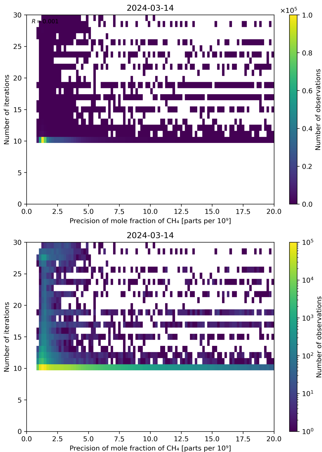
Figure 83: Scatter density plot of “Precision of mole fraction of CH 4 ” against “Number of iterations” for 2024-03-14 to 2024-03-15.
