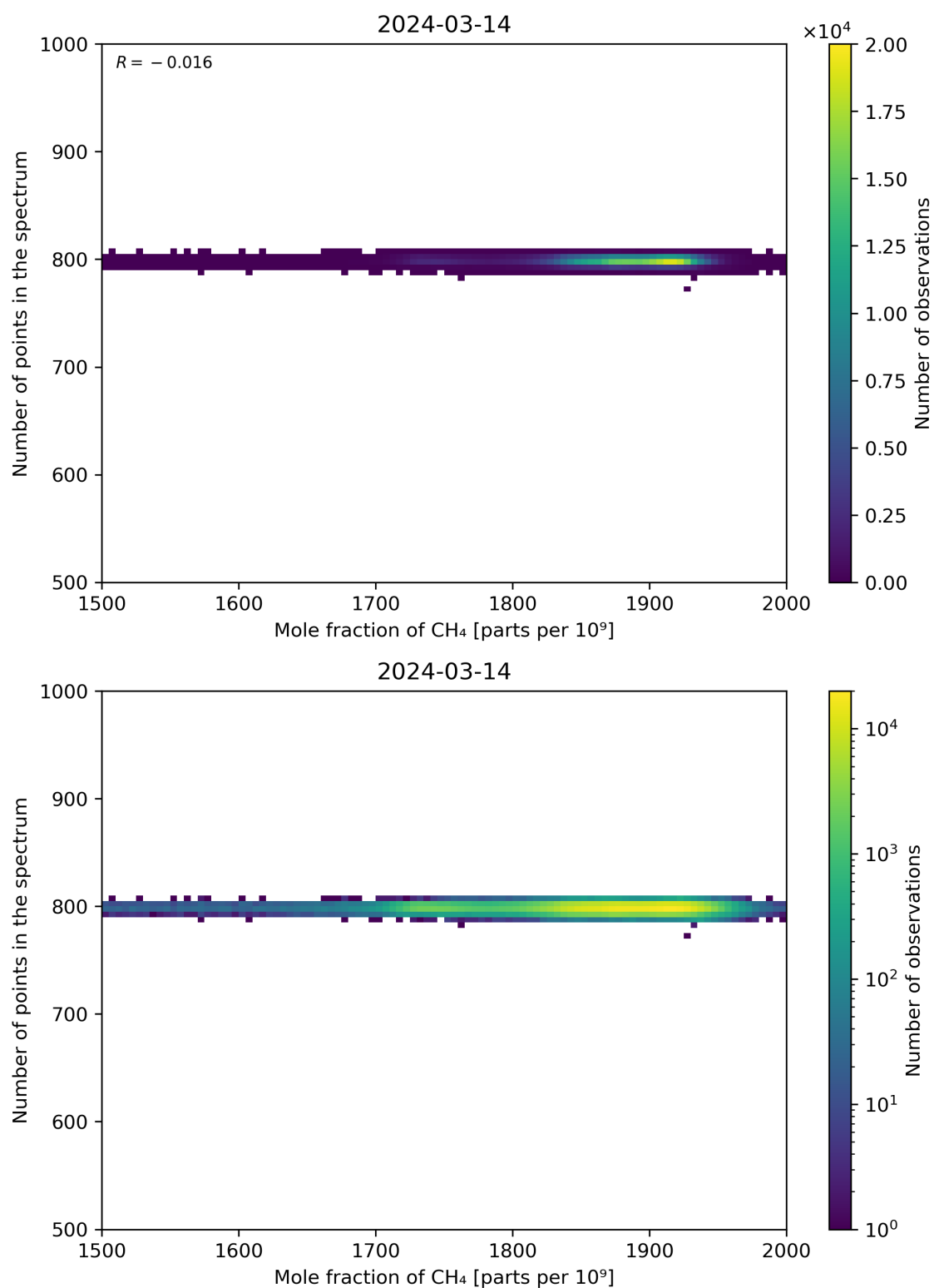
Figure 77: Scatter density plot of “Mole fraction of CH 4 ” against “Number of points in the spectrum” for 2024-03-14 to 2024-03-15.
