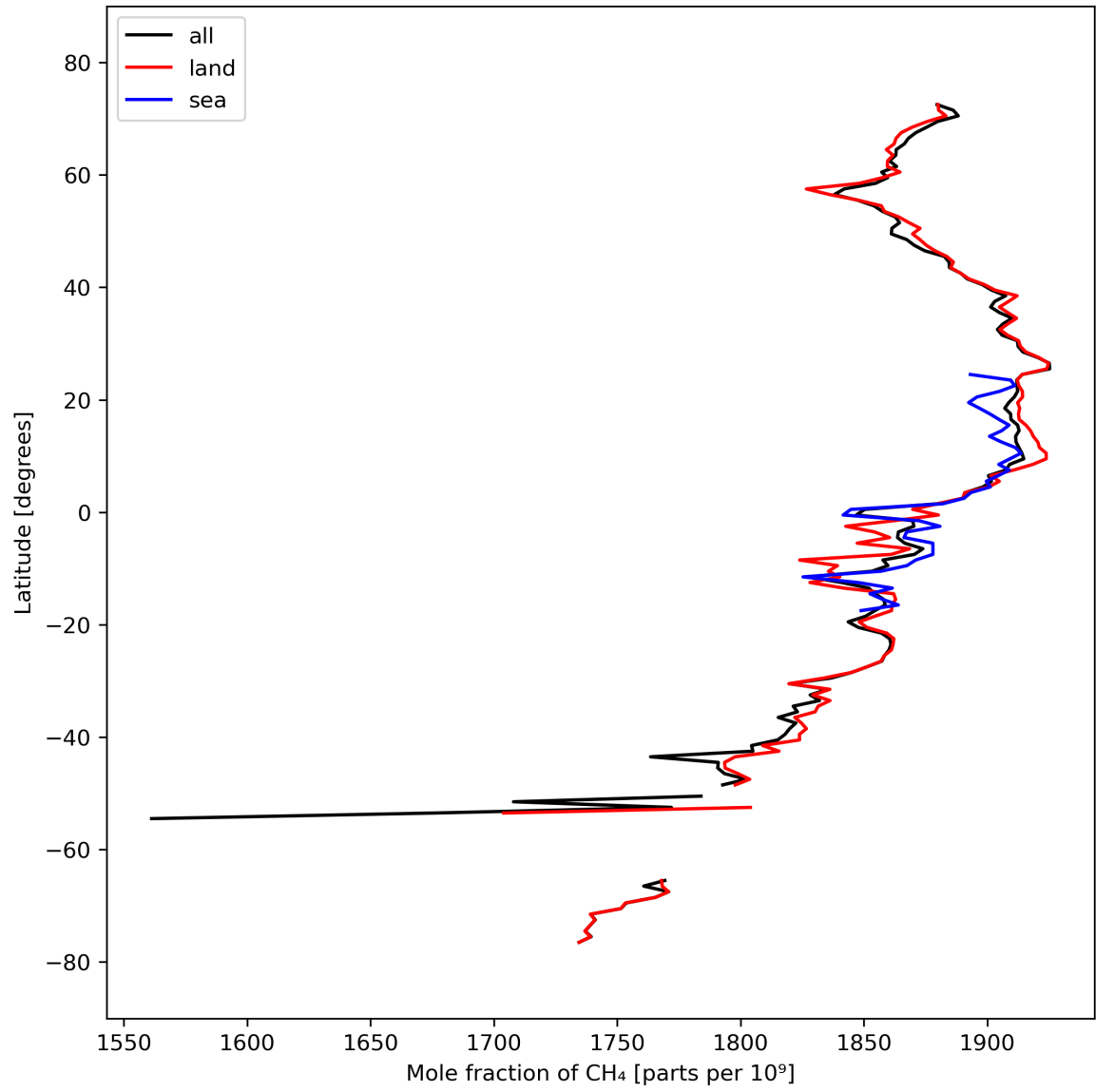
Figure 12: Zonal average of “Mole fraction of \text{CH}_4 ” for 2024-03-14 to 2024-03-15.
