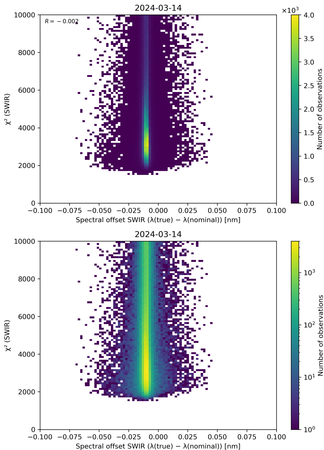
Figure 118: Scatter density plot of “Spectral offset SWIR ( \lambda(\text{true}) - \lambda(\text{nominal}) )” against “ \chi^2 (SWIR)” for 2024-03-14 to 2024-03-15.
