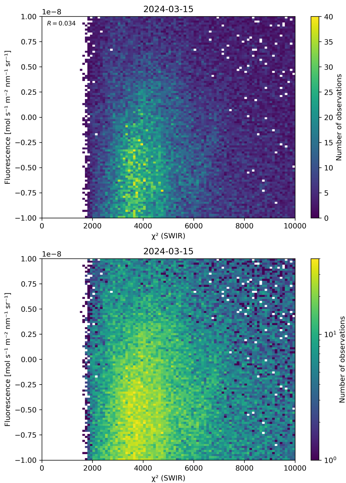
Figure 49: Scatter density plot of “ \chi^2 (SWIR)” against “Fluorescence” for 2024-03-14 to 2024-03-16.
