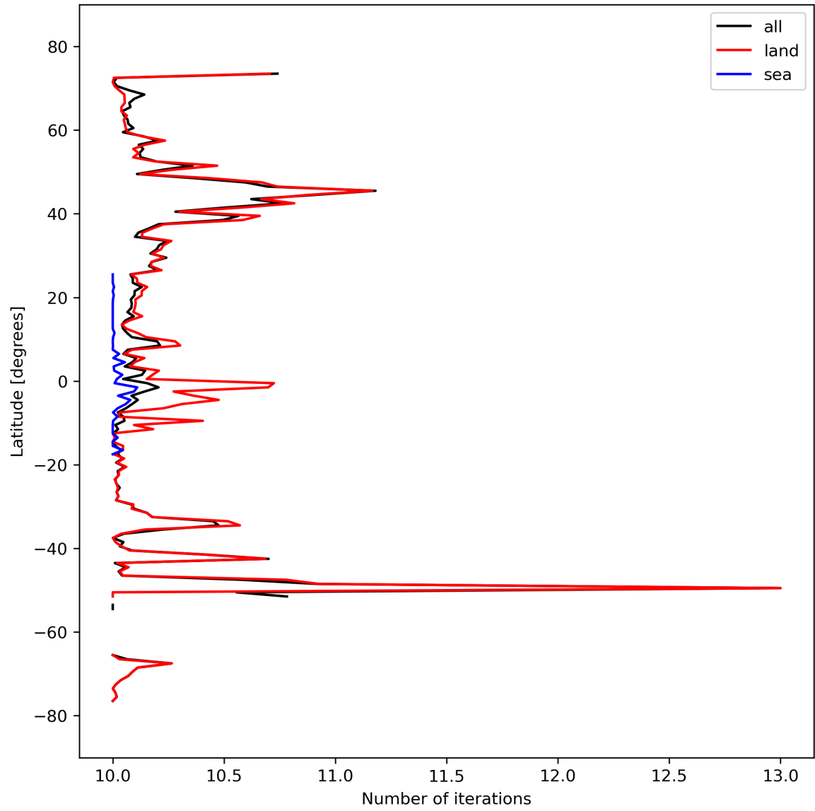
Figure 20: Zonal average of “Number of iterations” for 2024-03-14 to 2024-03-16.
