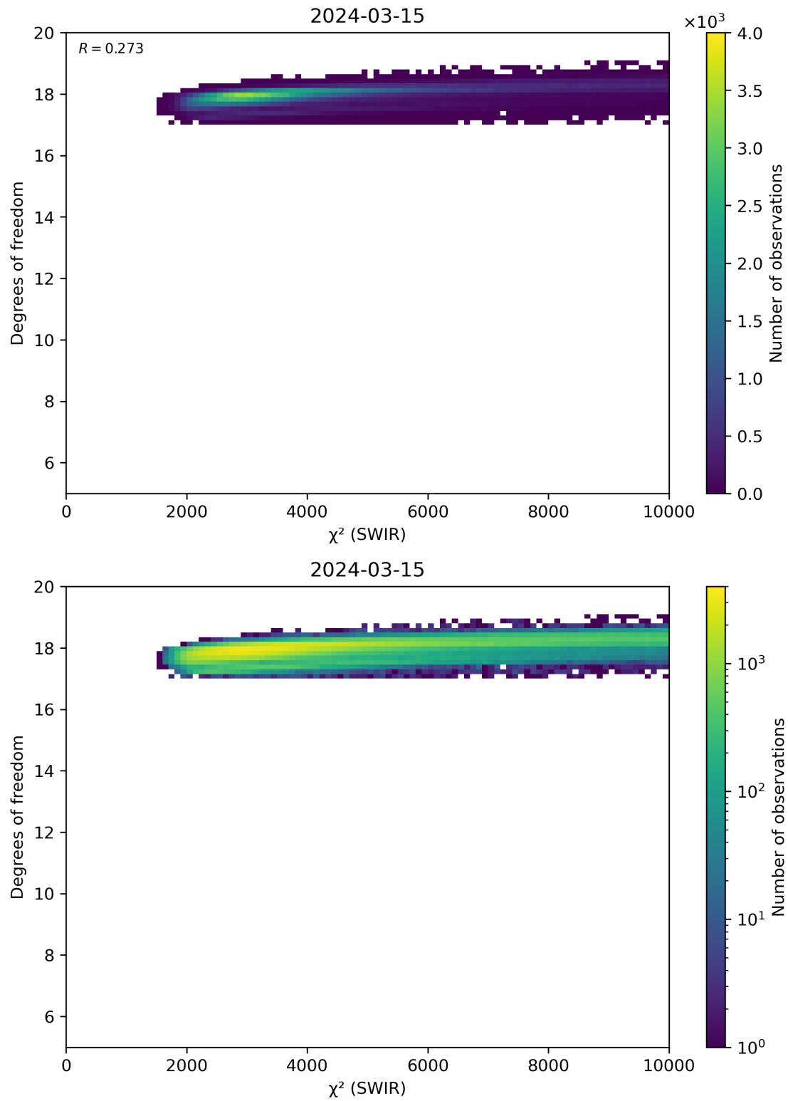
Figure 48: Scatter density plot of “ \chi^2 (SWIR)” against “Degrees of freedom” for 2024-03-14 to 2024-03-16.
