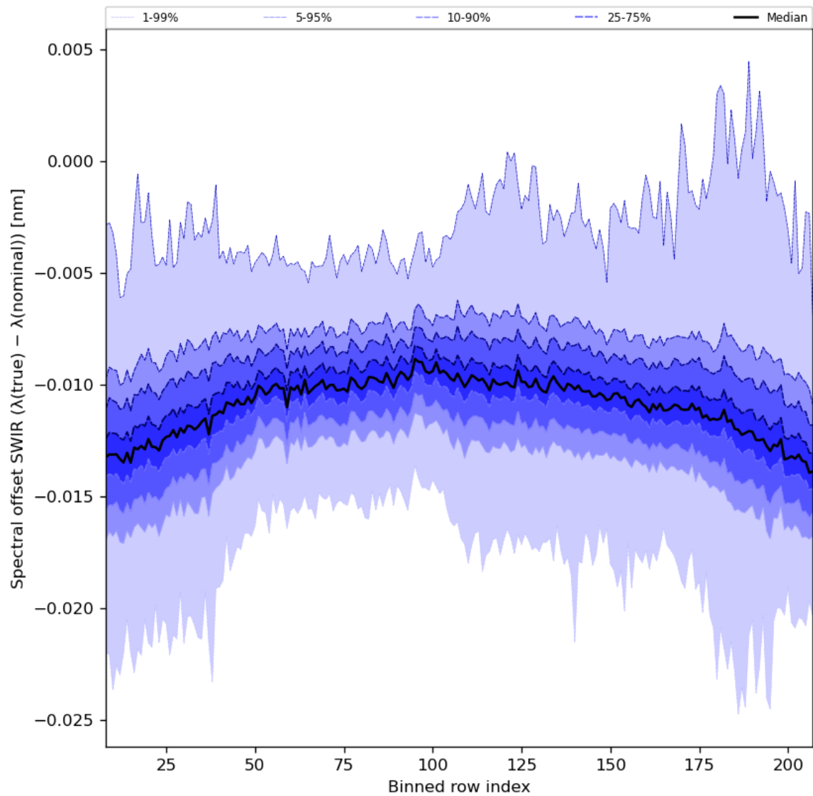
Figure 38: Along track statistics of “Spectral offset SWIR ( \lambda(\text{true}) - \lambda(\text{nominal}) )” for 2024-03-14 to 2024-03-16
