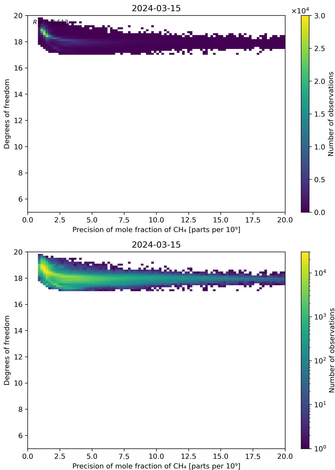
Figure 80: Scatter density plot of “Precision of mole fraction of CH 4 ” against “Degrees of freedom” for 2024-03-14 to 2024-03-16.
