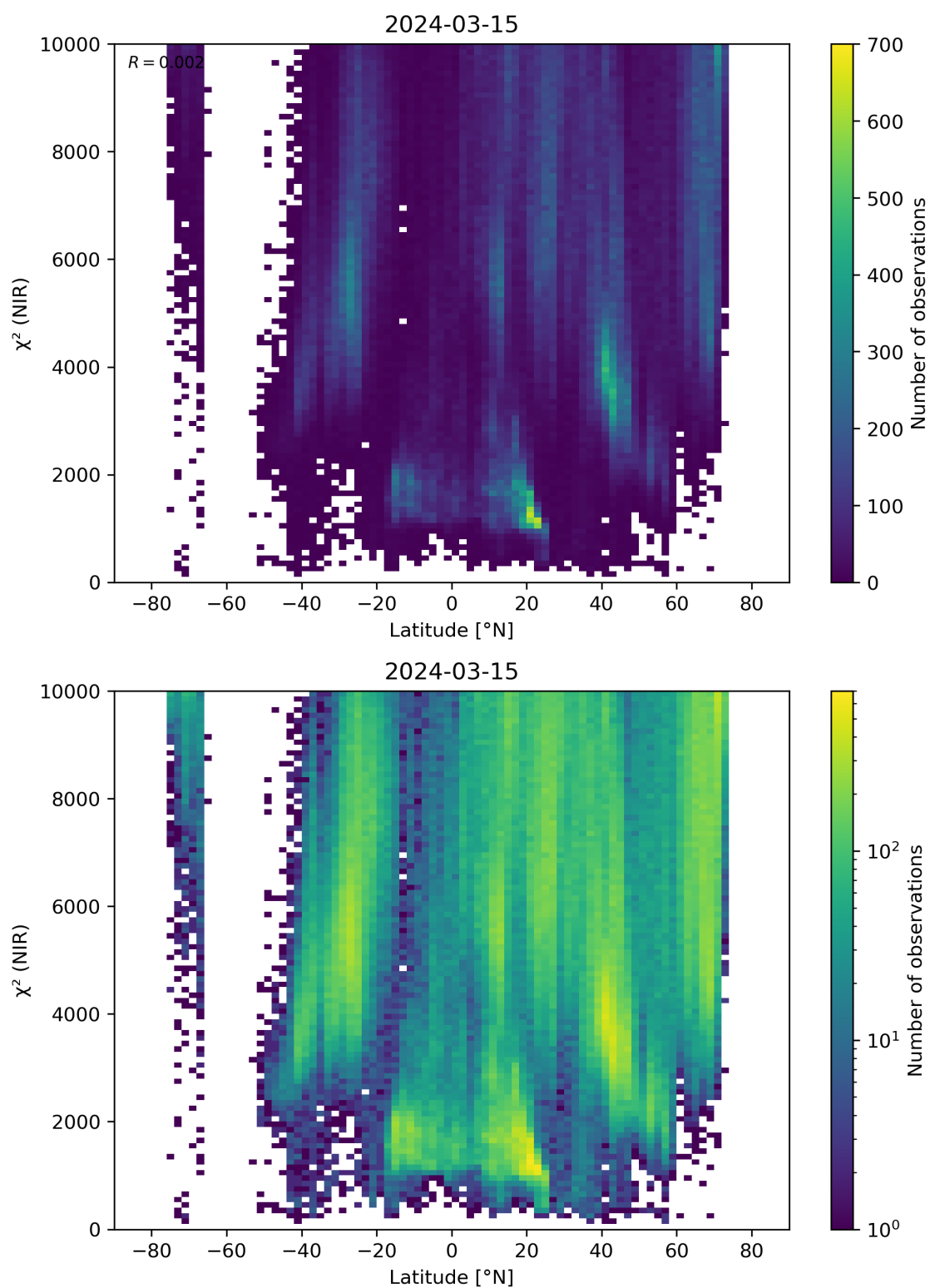
Figure 53: Scatter density plot of “Latitude” against “ \chi^2 (NIR)” for 2024-03-14 to 2024-03-16.
