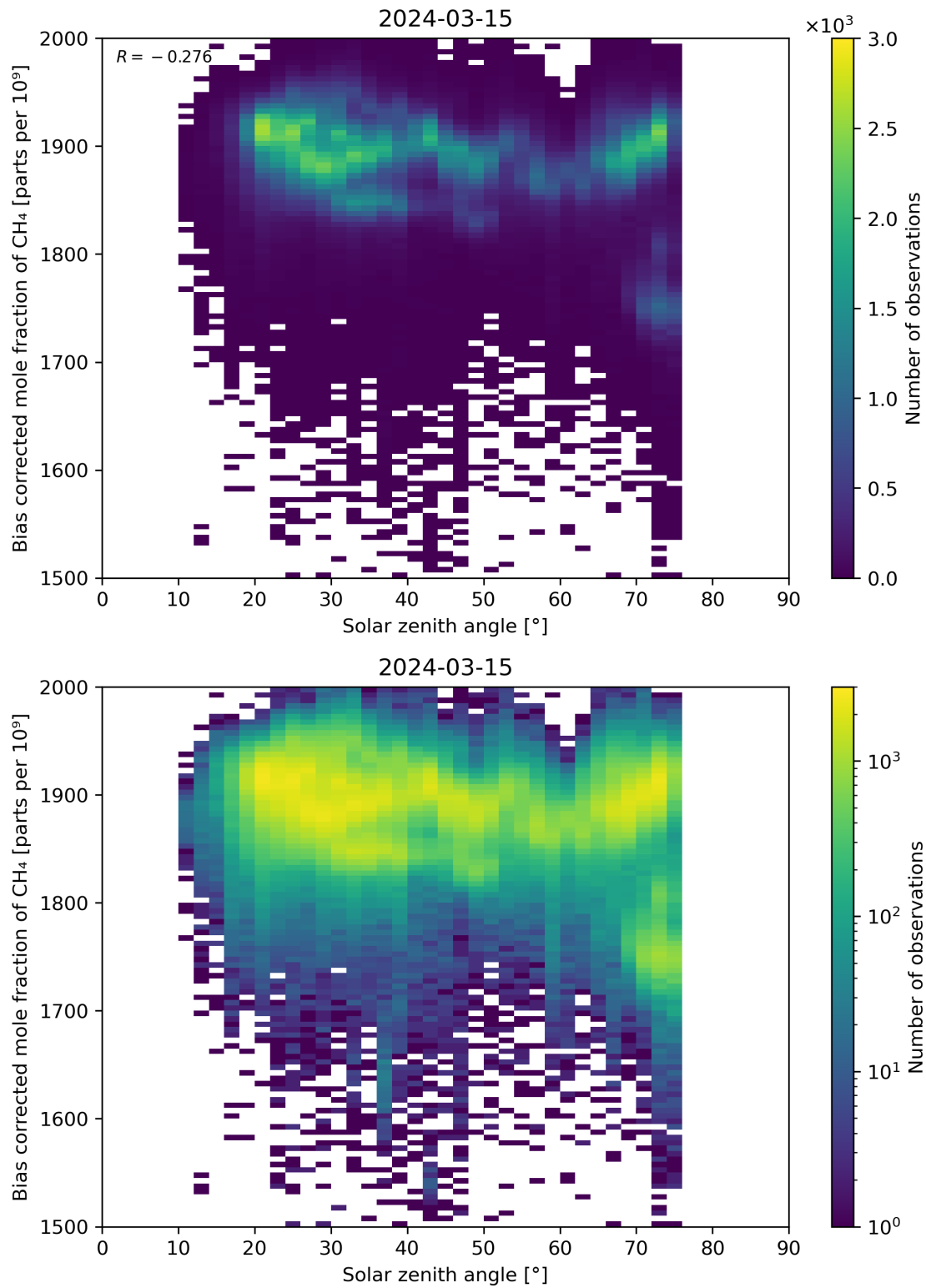
Figure 100: Scatter density plot of “Solar zenith angle” against “Bias corrected mole fraction of CH 4 ” for 2024-03-14 to 2024-03-16.
