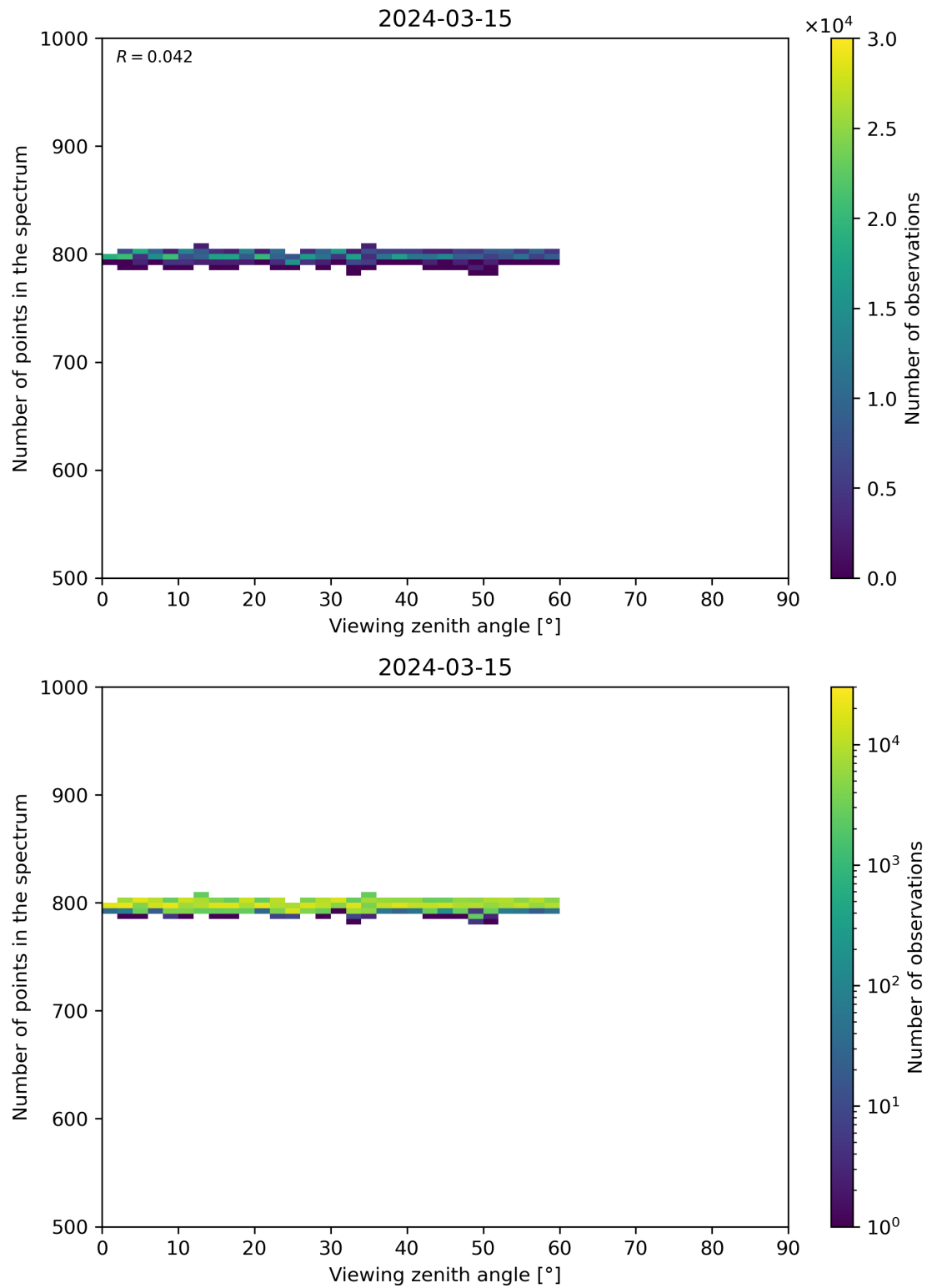
Figure 114: Scatter density plot of “Viewing zenith angle” against “Number of points in the spectrum” for 2024-03-14 to 2024-03-16.
