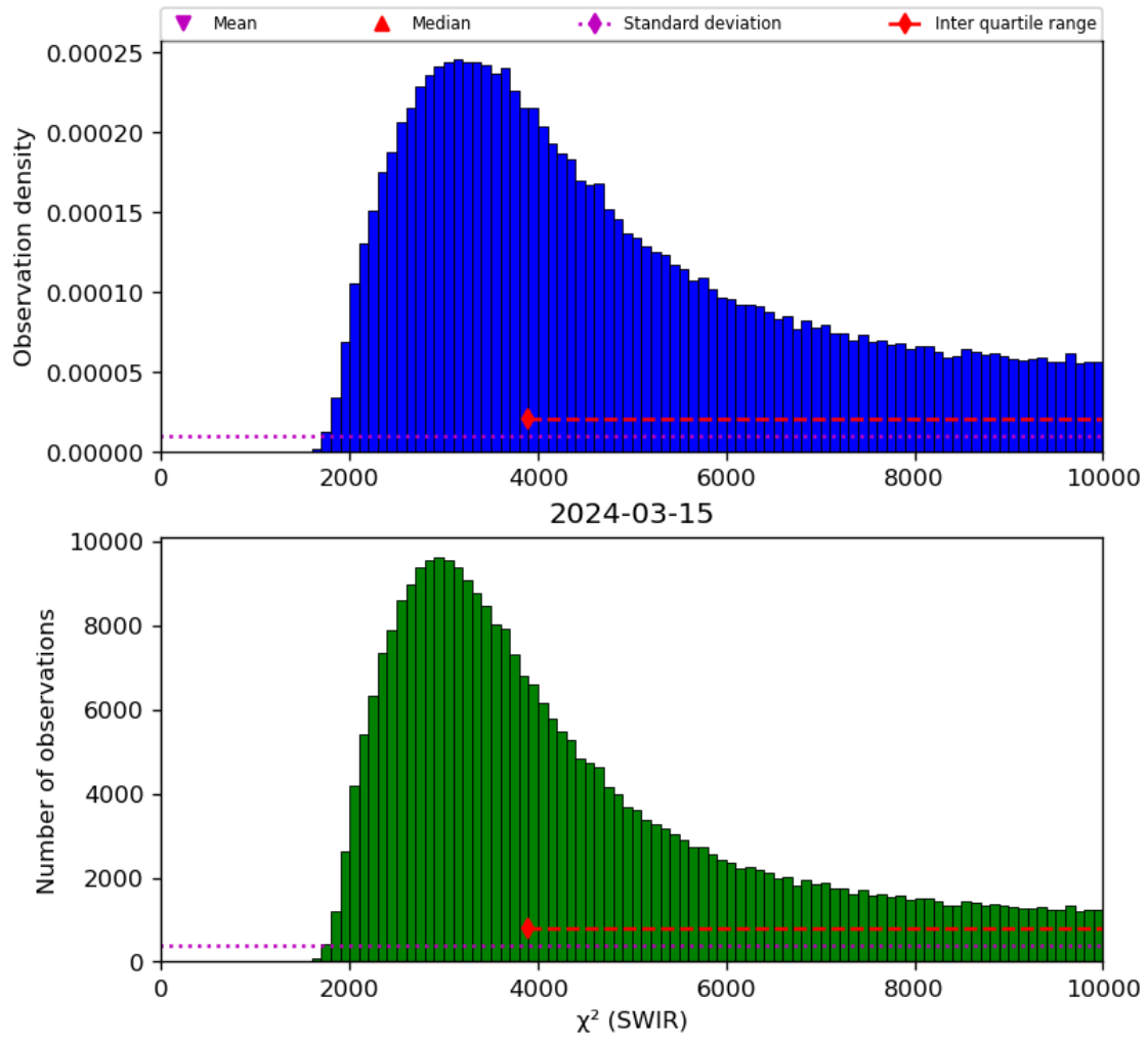
Figure 28: Histogram of “ \chi^2 (SWIR)” for 2024-03-14 to 2024-03-16
