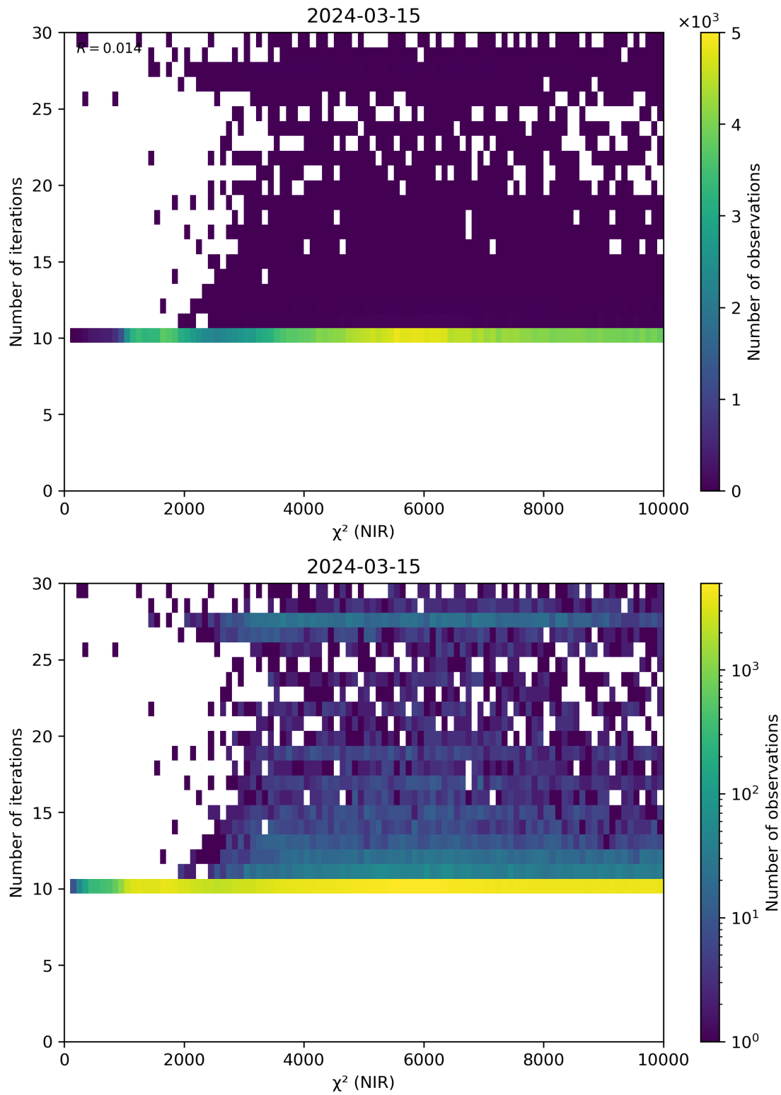
Figure 46: Scatter density plot of “ \chi^2 (NIR)” against “Number of iterations” for 2024-03-14 to 2024-03-16.
