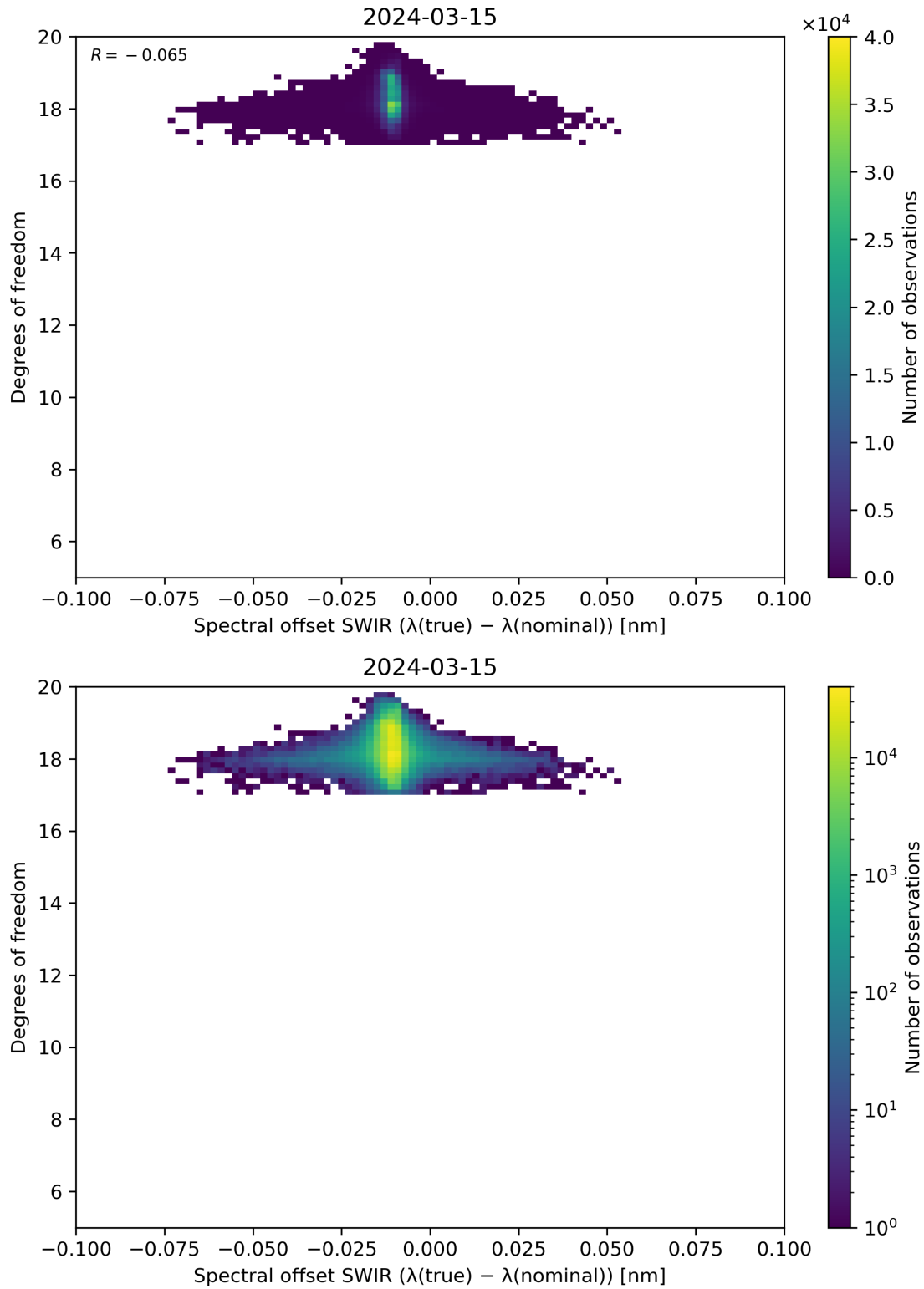
Figure 119: Scatter density plot of “Spectral offset SWIR ( \lambda(\text{true}) - \lambda(\text{nominal}) )” against “Degrees of freedom” for 2024-03-14 to 2024-03-16.
