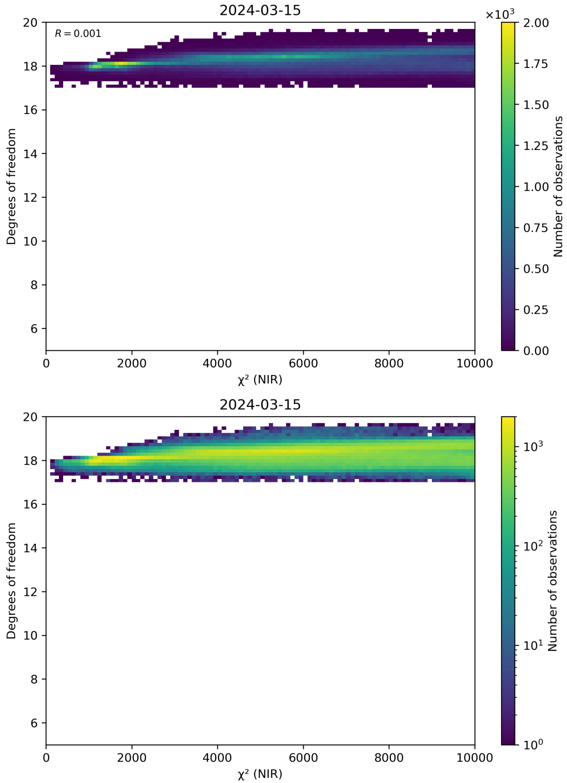
Figure 44: Scatter density plot of “ \chi^2 (NIR)” against “Degrees of freedom” for 2024-03-14 to 2024-03-16.
