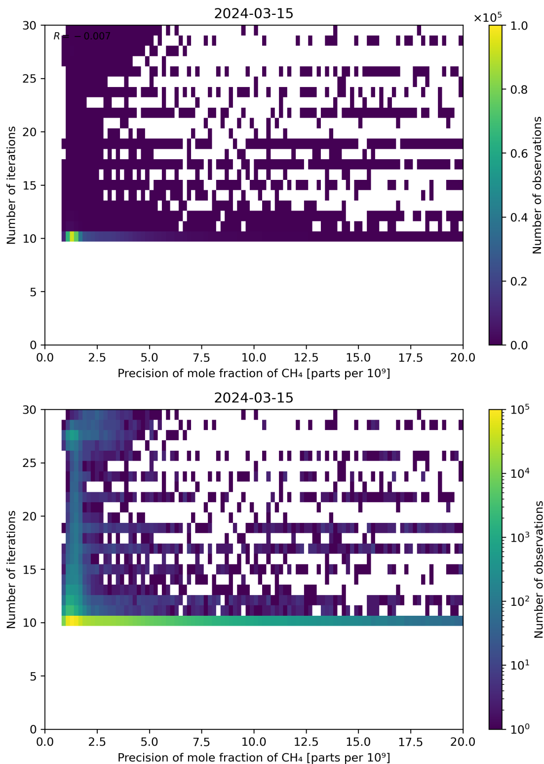
Figure 83: Scatter density plot of “Precision of mole fraction of CH 4 ” against “Number of iterations” for 2024-03-14 to 2024-03-16.
