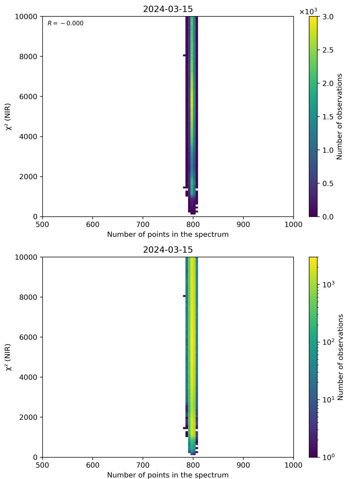
Figure 88: Scatter density plot of “Number of points in the spectrum” against “ \chi^2 (NIR)” for 2024-03-14 to 2024-03-16.
