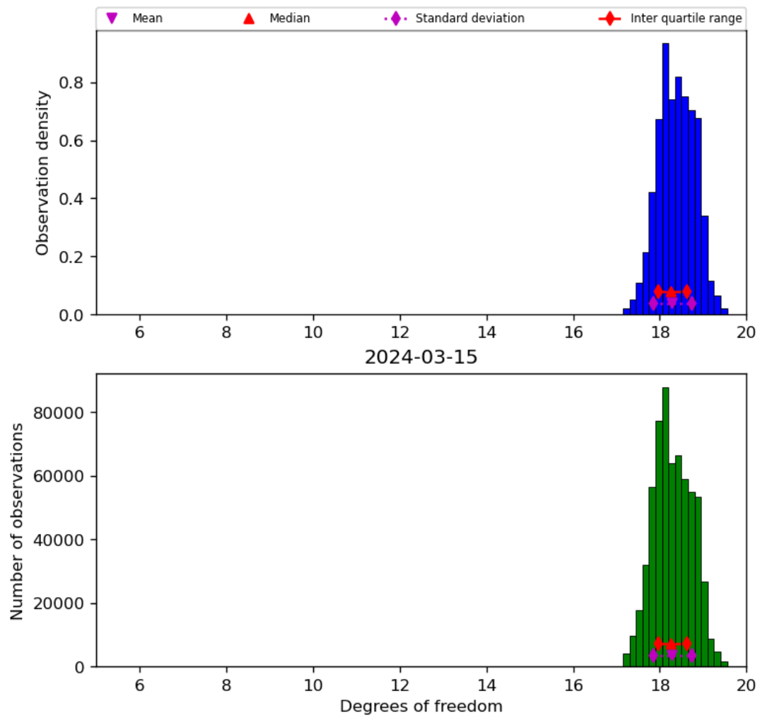
Figure 30: Histogram of "Degrees of freedom" for 2024-03-14 to 2024-03-16
