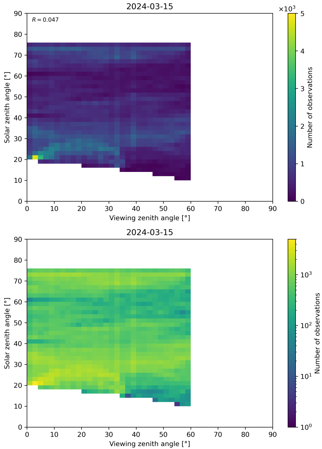
Figure 115: Scatter density plot of “Viewing zenith angle” against “Solar zenith angle” for 2024-03-14 to 2024-03-16.
