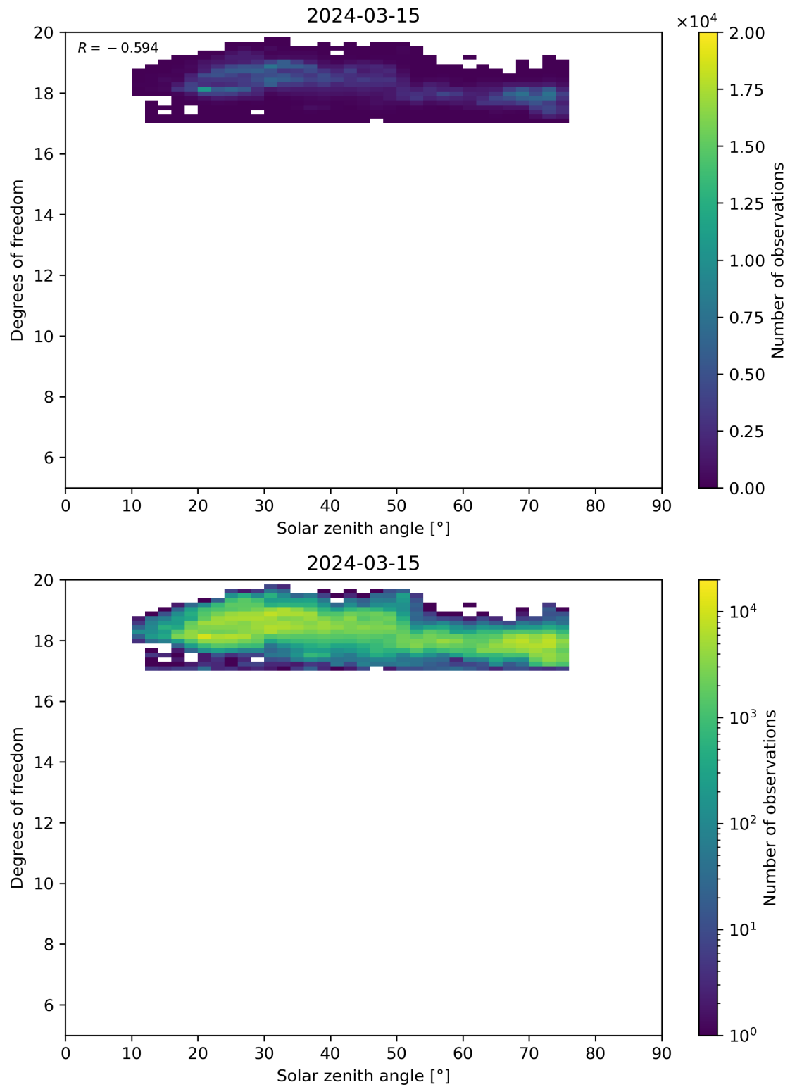
Figure 96: Scatter density plot of “Solar zenith angle” against “Degrees of freedom” for 2024-03-14 to 2024-03-16.
