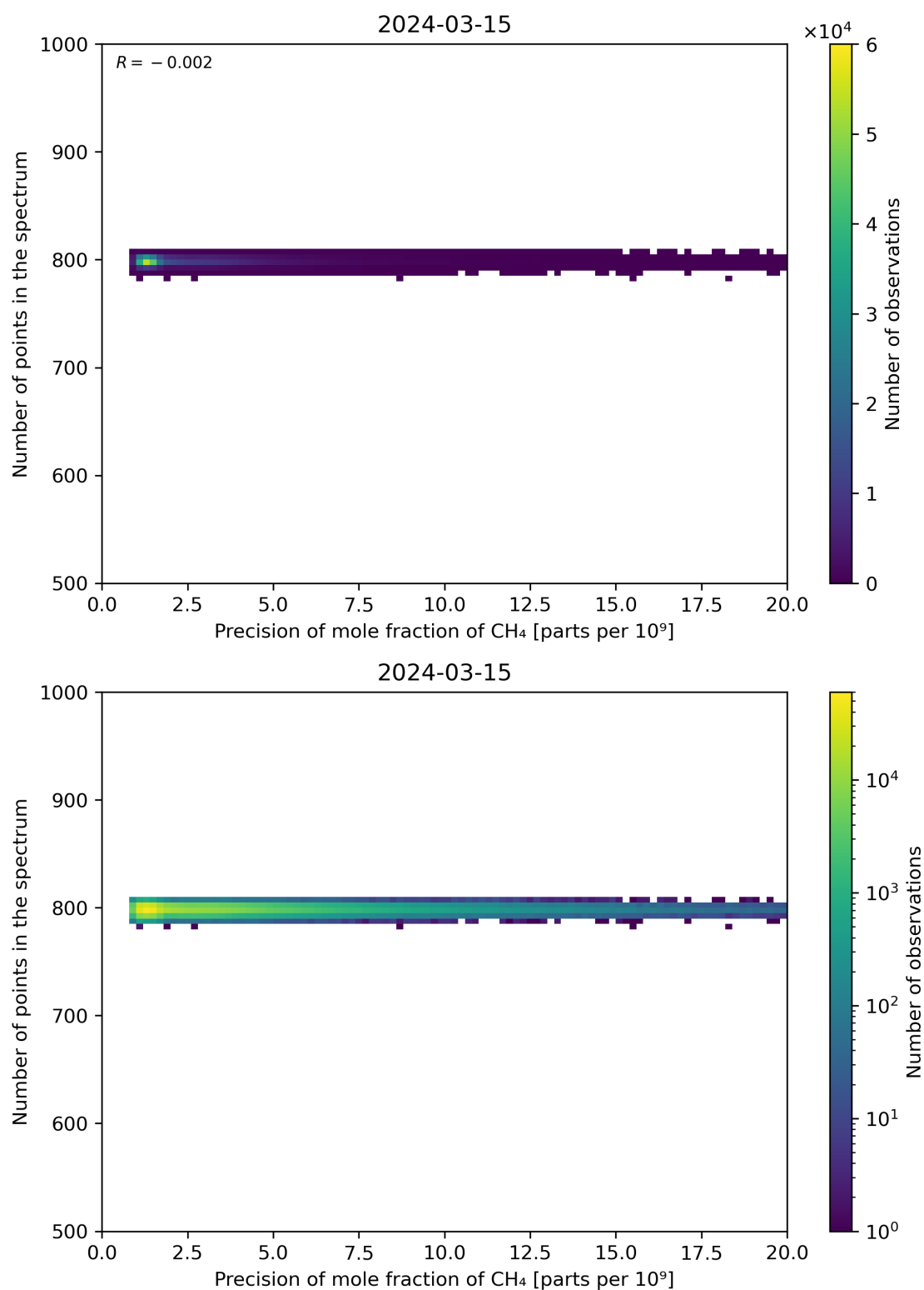
Figure 84: Scatter density plot of “Precision of mole fraction of CH 4 ” against “Number of points in the spectrum” for 2024-03-14 to 2024-03-16.
