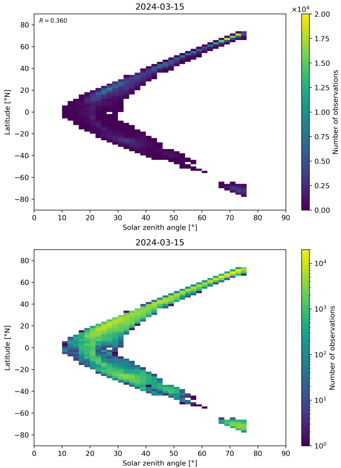
Figure 98: Scatter density plot of “Solar zenith angle” against “Latitude” for 2024-03-14 to 2024-03-16.
