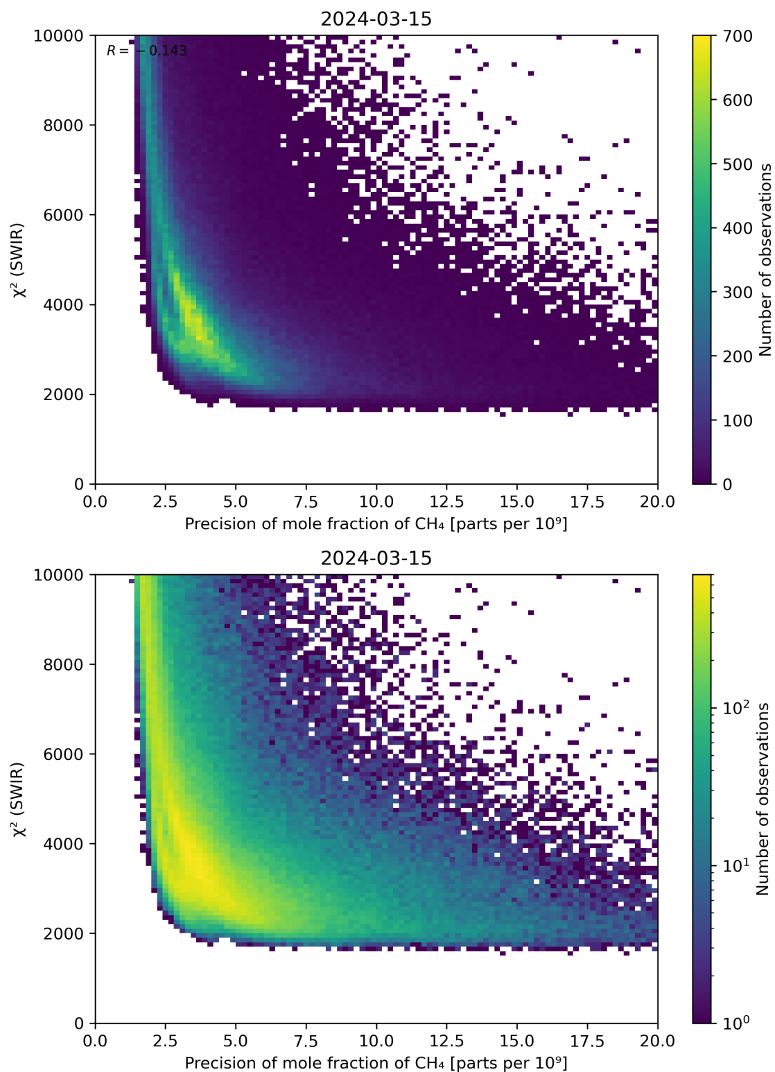
Figure 79: Scatter density plot of “Precision of mole fraction of CH 4 ” against “ \chi^2 (SWIR)” for 2024-03-14 to 2024-03-16.
