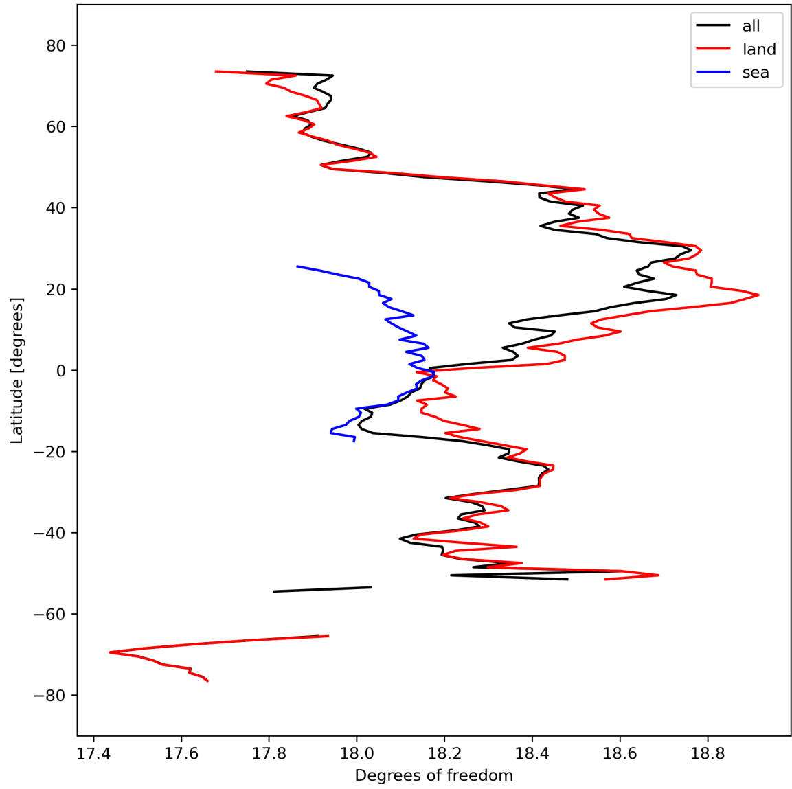
Figure 19: Zonal average of “Degrees of freedom” for 2024-03-14 to 2024-03-16.
