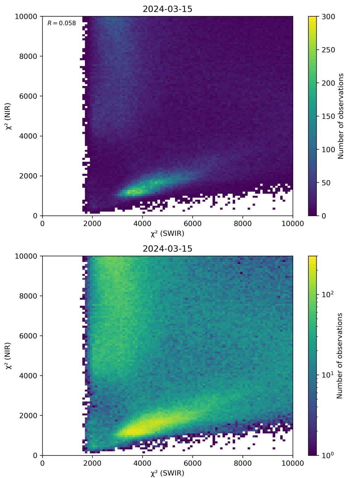
Figure 47: Scatter density plot of “ \chi^2 (SWIR)” against “ \chi^2 (NIR)” for 2024-03-14 to 2024-03-16.
