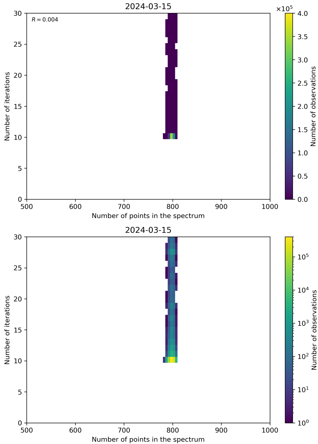
Figure 92: Scatter density plot of “Number of points in the spectrum” against “Number of iterations” for 2024-03-14 to 2024-03-16.
