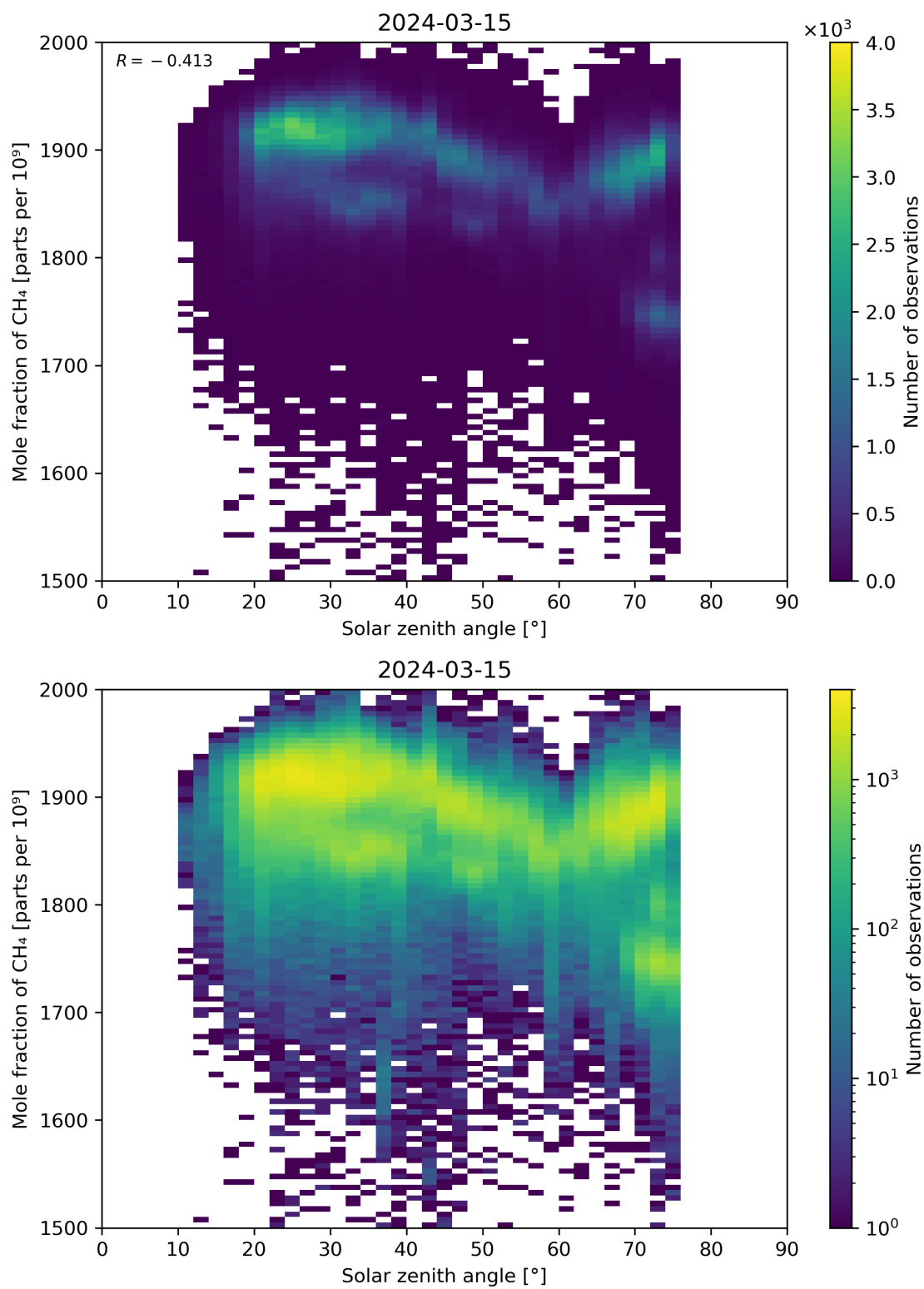
Figure 99: Scatter density plot of “Solar zenith angle” against “Mole fraction of CH 4 ” for 2024-03-14 to 2024-03-16.
