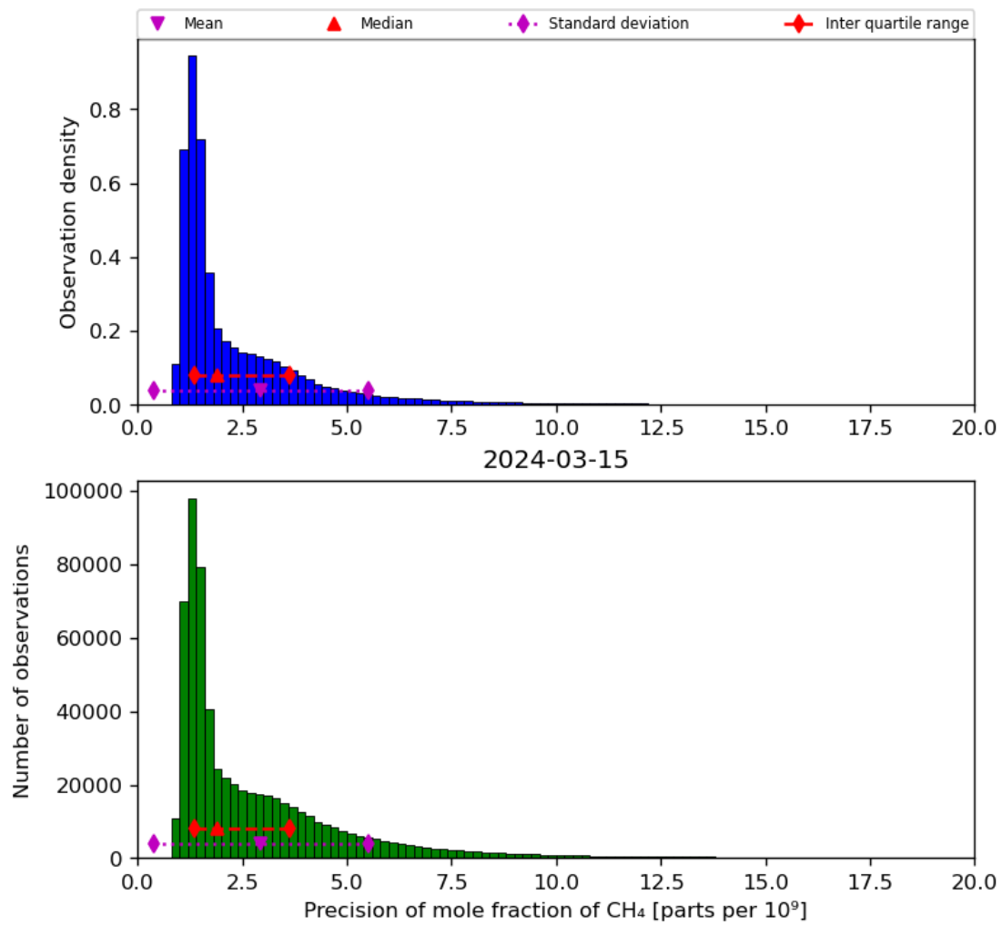
Figure 24: Histogram of “Precision of mole fraction of CH 4 ” for 2024-03-14 to 2024-03-16
