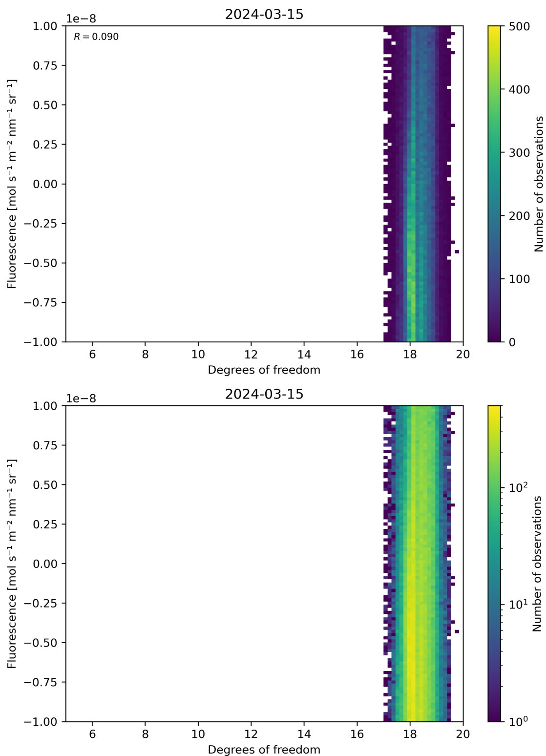
Figure 51: Scatter density plot of “Degrees of freedom” against “Fluorescence” for 2024-03-14 to 2024-03-16.
