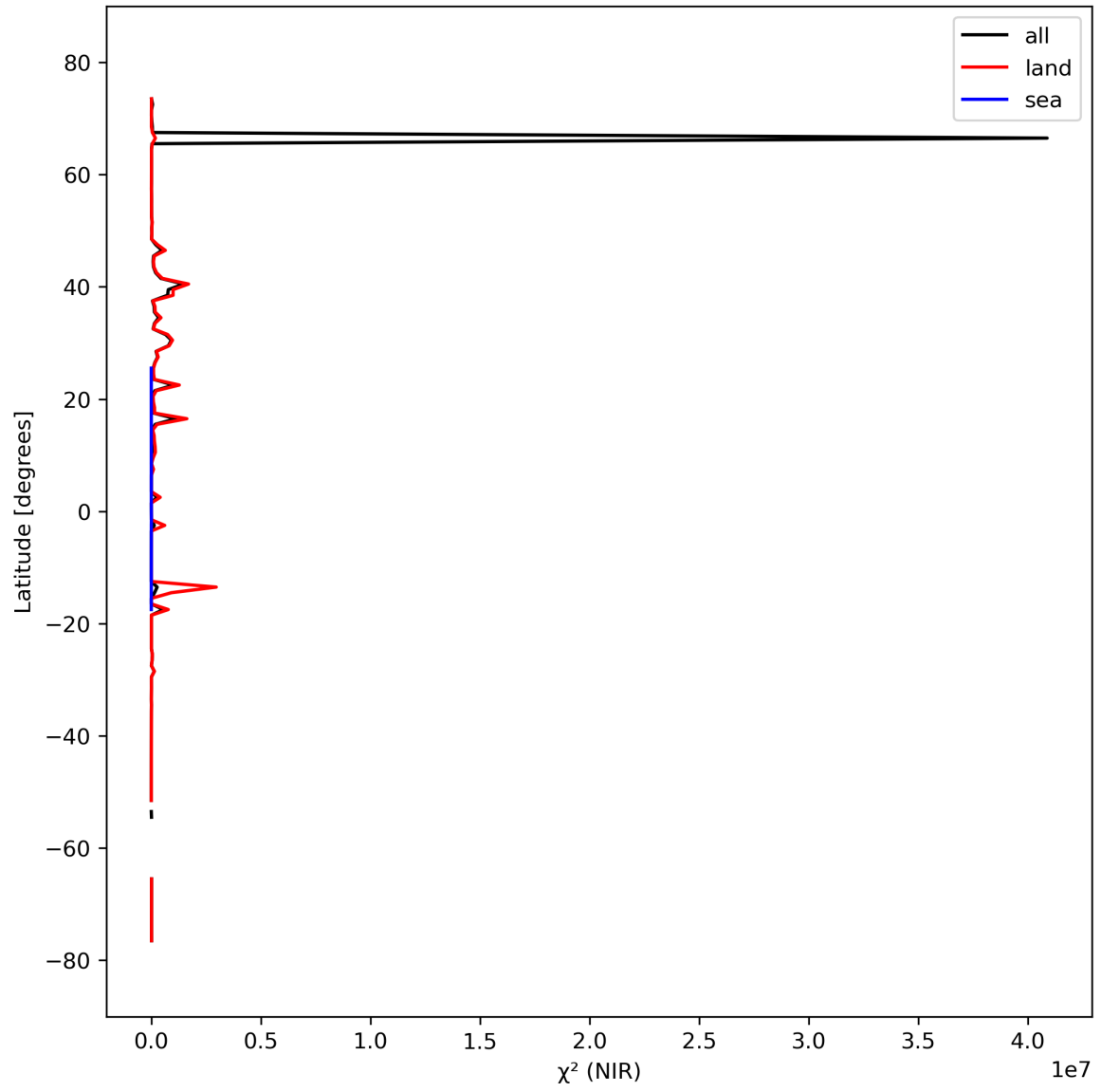
Figure 18: Zonal average of “ \chi^2 (NIR)” for 2024-03-14 to 2024-03-16.
