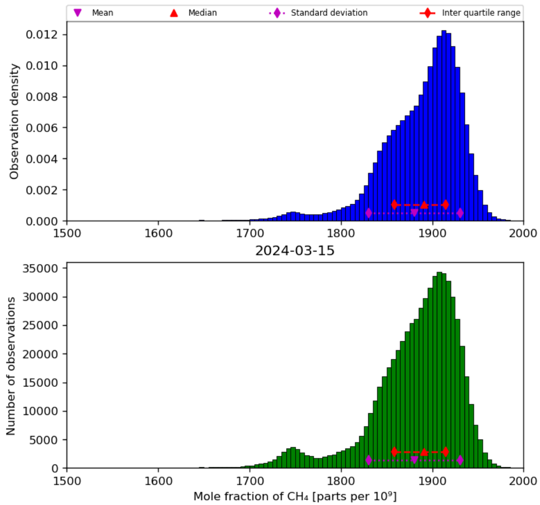
Figure 23: Histogram of “Mole fraction of CH 4 ” for 2024-03-14 to 2024-03-16
