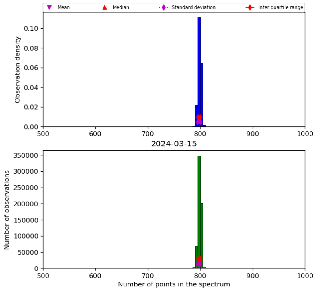
Figure 26: Histogram of “Number of points in the spectrum” for 2024-03-14 to 2024-03-16
