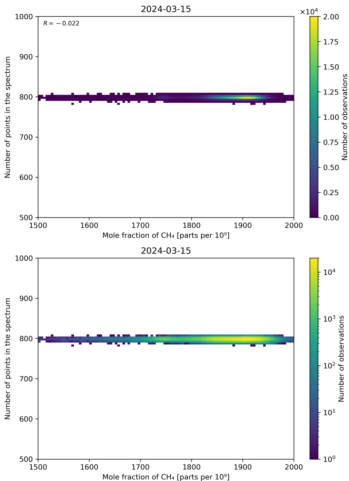
Figure 77: Scatter density plot of “Mole fraction of CH 4 ” against “Number of points in the spectrum” for 2024-03-14 to 2024-03-16.
