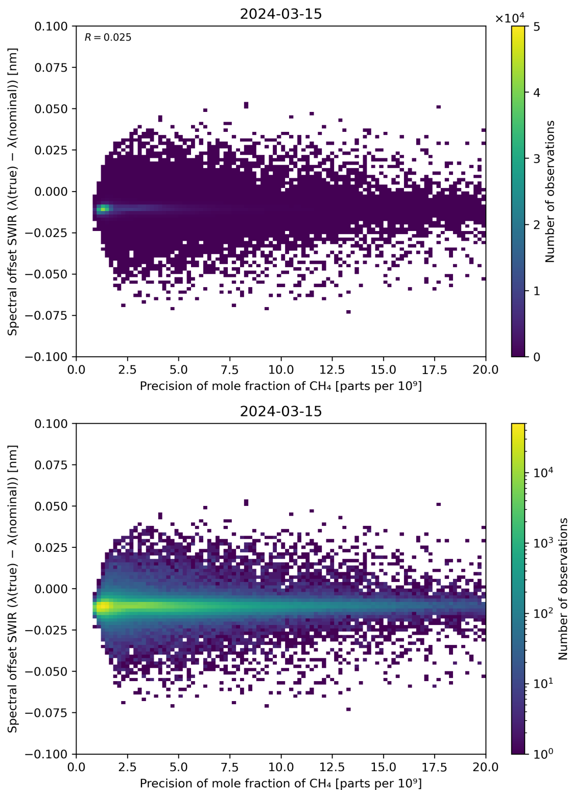
Figure 85: Scatter density plot of “Precision of mole fraction of \text{CH}_4 ” against “Spectral offset SWIR ( \lambda(\text{true}) - \lambda(\text{nominal}) )” for 2024-03-14 to 2024-03-16.
