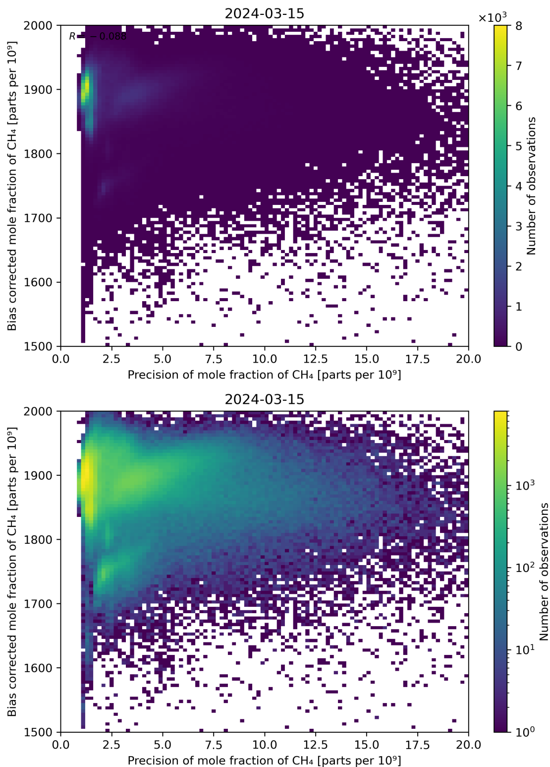
Figure 82: Scatter density plot of “Precision of mole fraction of CH 4 ” against “Bias corrected mole fraction of CH 4 ” for 2024-03-14 to 2024-03-16.
