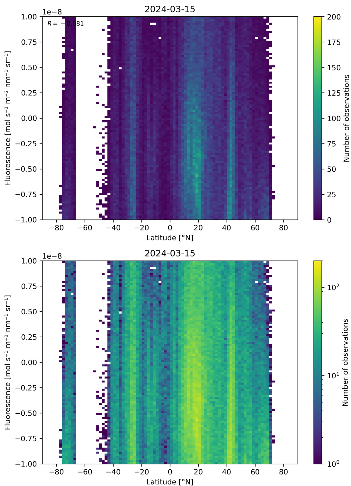
Figure 56: Scatter density plot of “Latitude” against “Fluorescence” for 2024-03-14 to 2024-03-16.
