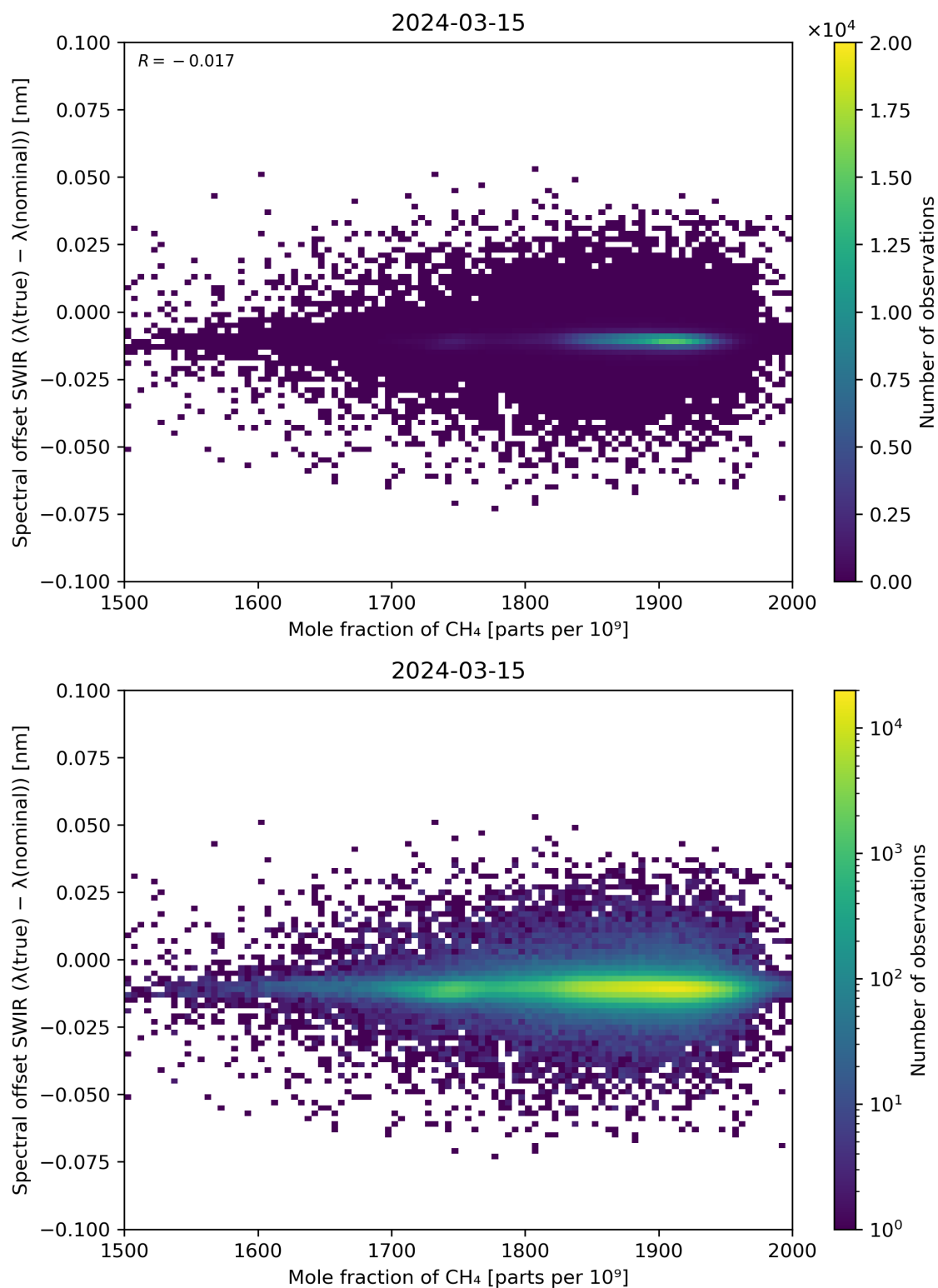
Figure 86: Scatter density plot of “Mole fraction of CH 4 ” against “Spectral offset SWIR ( \lambda(\text{true}) - \lambda(\text{nominal}) )” for 2024-03-14 to 2024-03-16.
