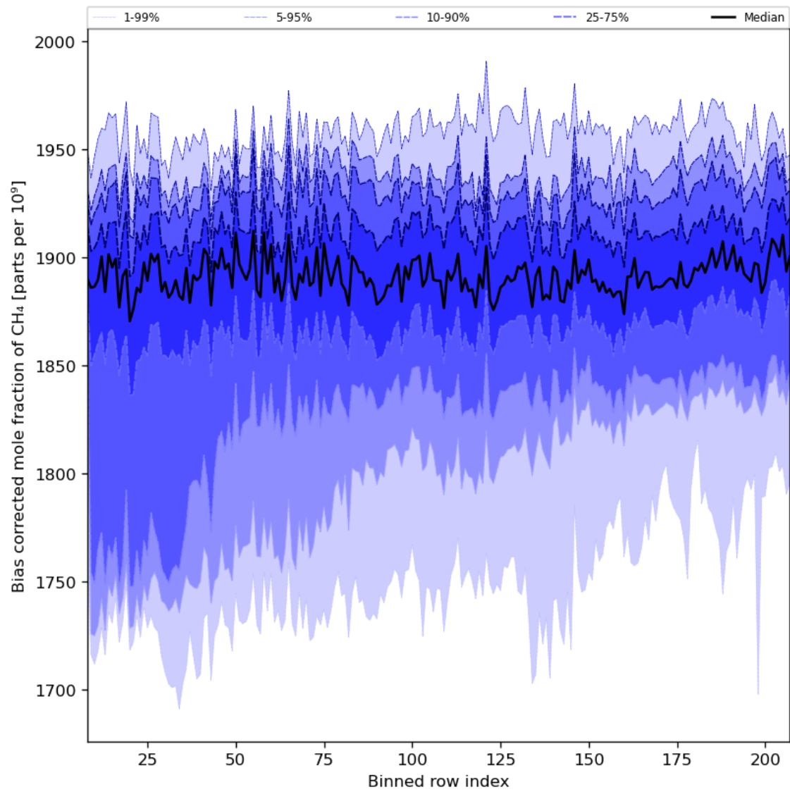
Figure 36: Along track statistics of “Bias corrected mole fraction of CH 4 ” for 2024-03-14 to 2024-03-16
