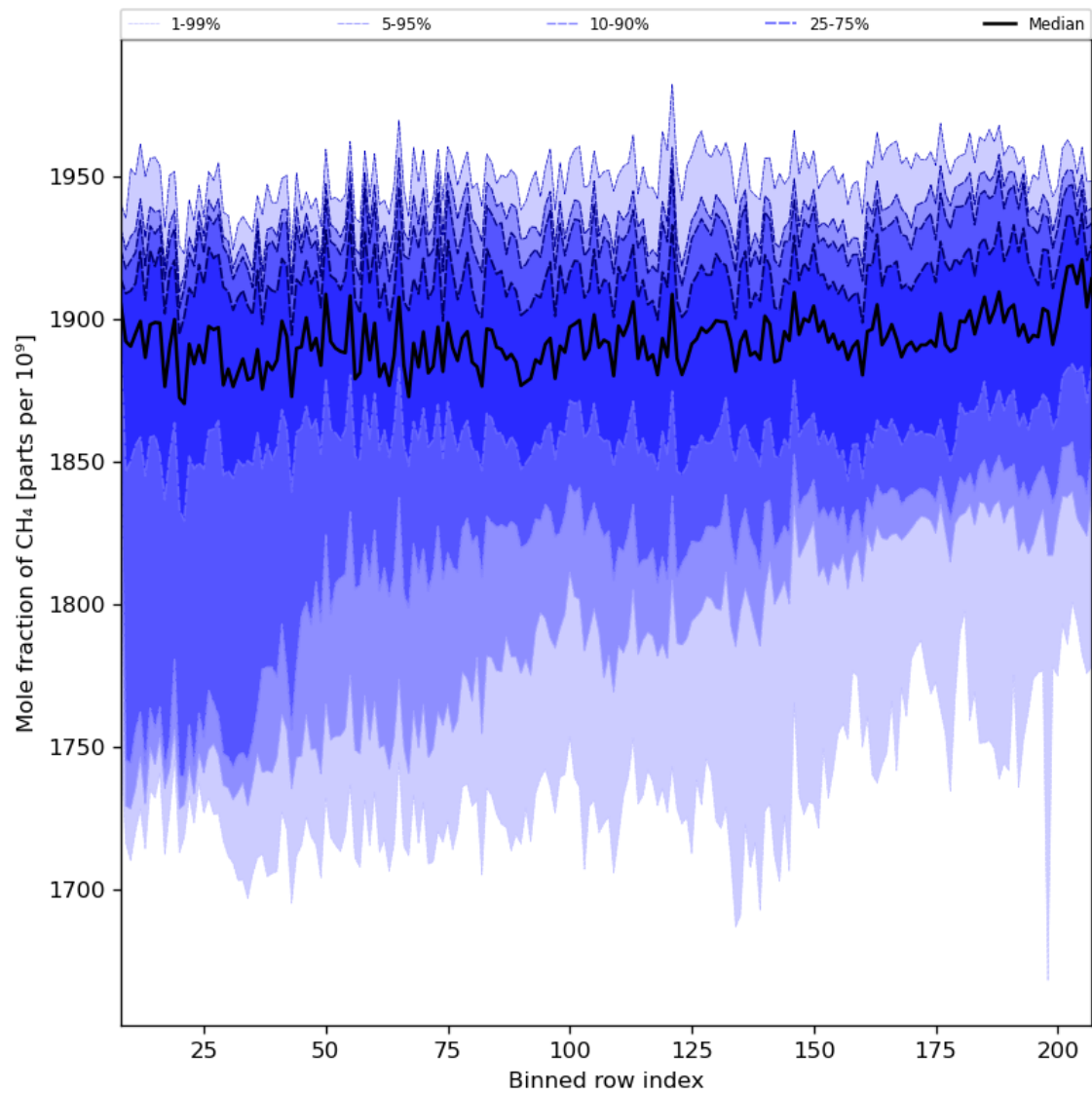
Figure 34: Along track statistics of “Mole fraction of CH 4 ” for 2024-03-14 to 2024-03-16
