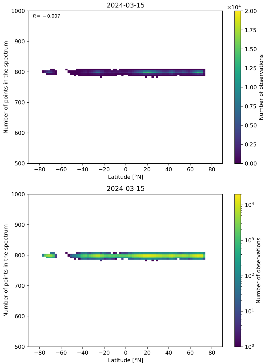
Figure 61: Scatter density plot of “Latitude” against “Number of points in the spectrum” for 2024-03-14 to 2024-03-16.
