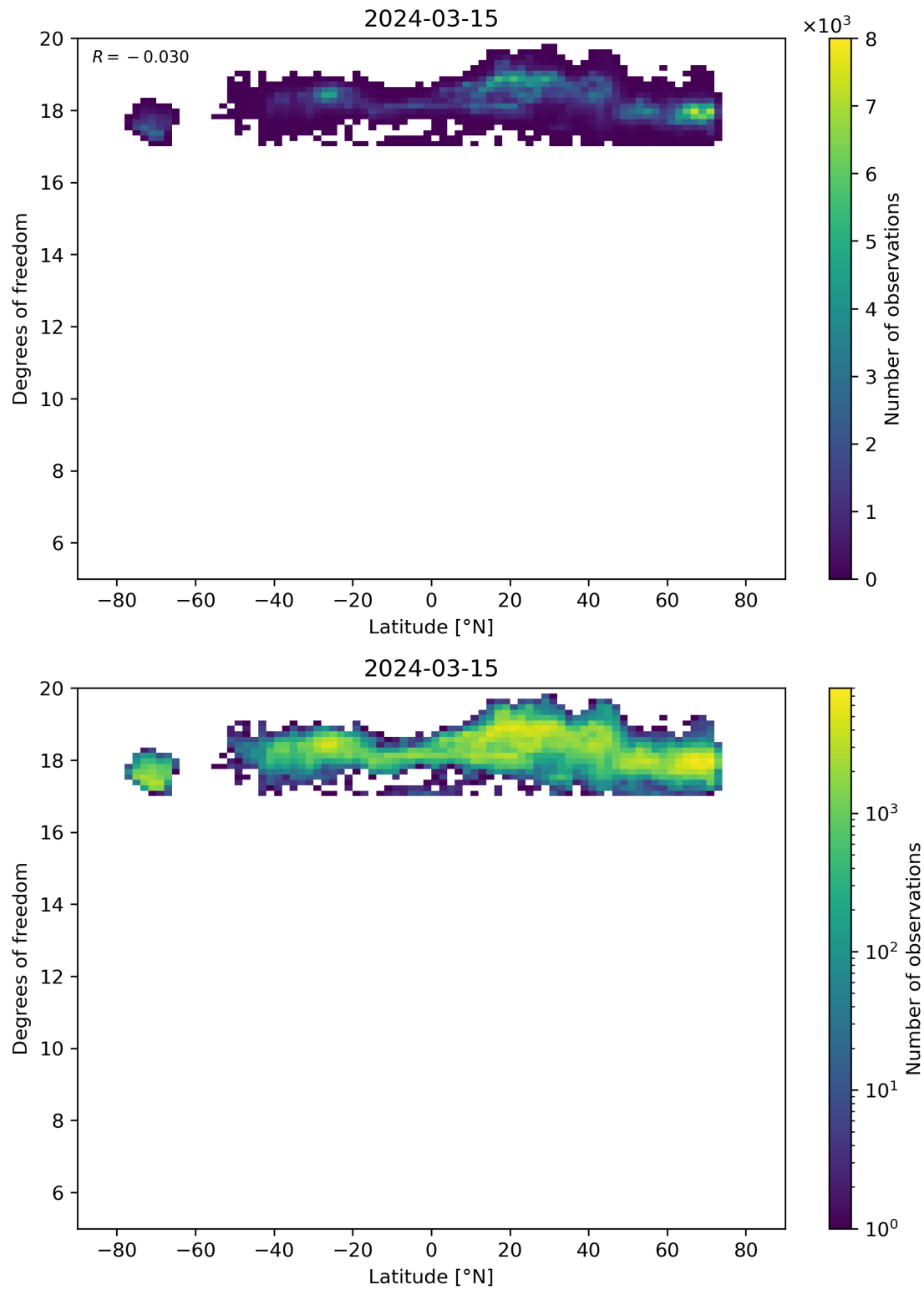
Figure 55: Scatter density plot of “Latitude” against “Degrees of freedom” for 2024-03-14 to 2024-03-16.
