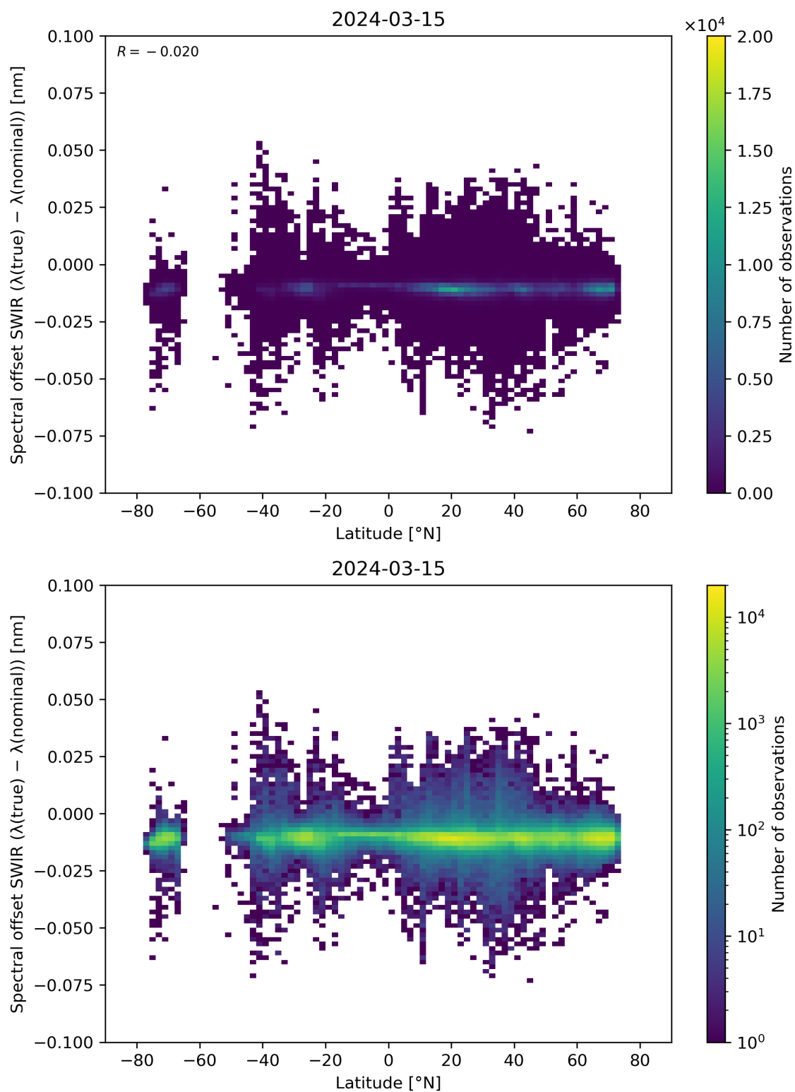
Figure 62: Scatter density plot of “Latitude” against “Spectral offset SWIR ( \lambda(\text{true}) - \lambda(\text{nominal}) )” for 2024-03-14 to 2024-03-16.
