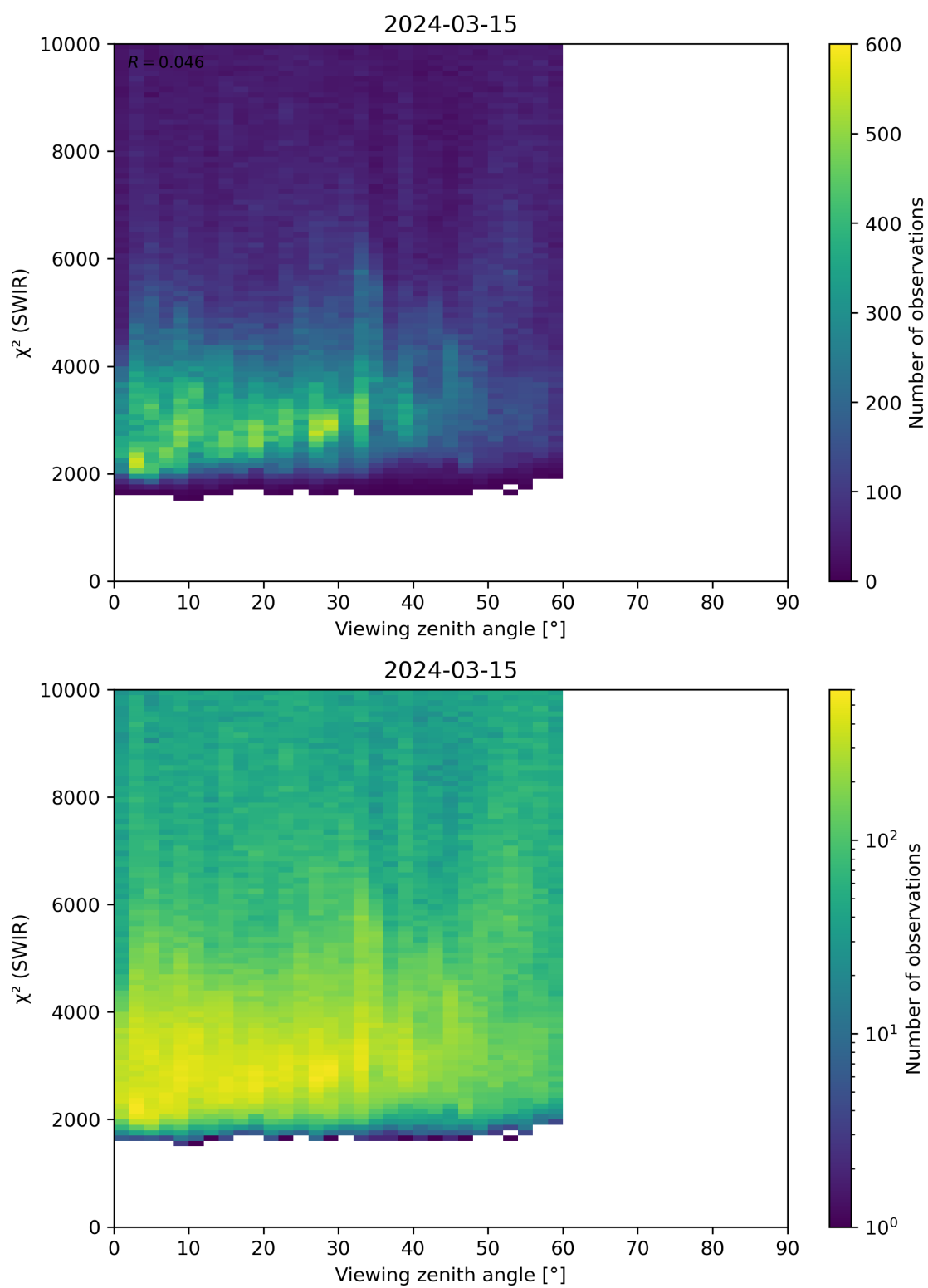
Figure 106: Scatter density plot of “Viewing zenith angle” against “ \chi^2 (SWIR)” for 2024-03-14 to 2024-03-16.
