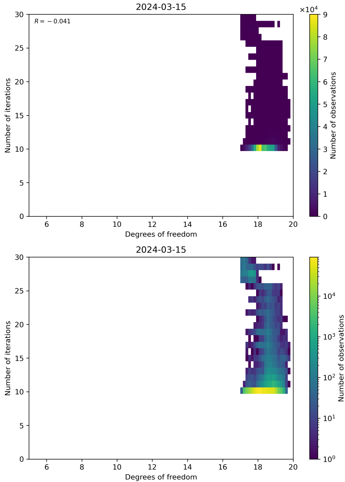
Figure 52: Scatter density plot of “Degrees of freedom” against “Number of iterations” for 2024-03-14 to 2024-03-16.
