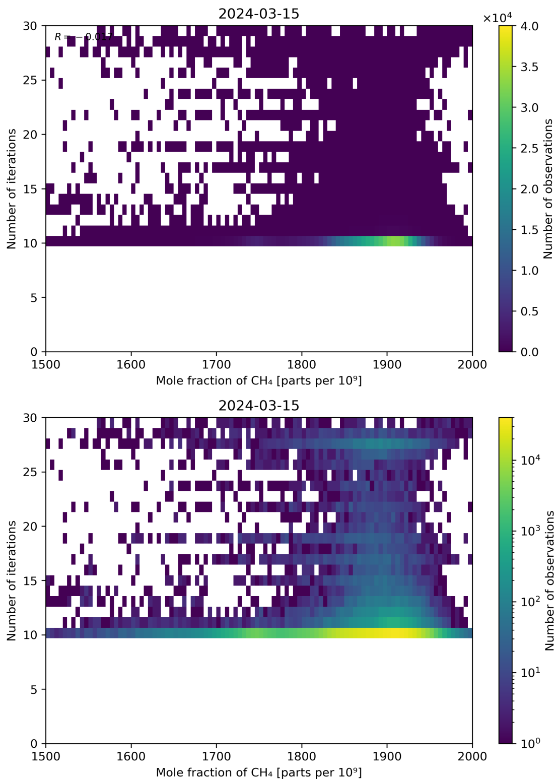
Figure 76: Scatter density plot of “Mole fraction of CH 4 ” against “Number of iterations” for 2024-03-14 to 2024-03-16.
