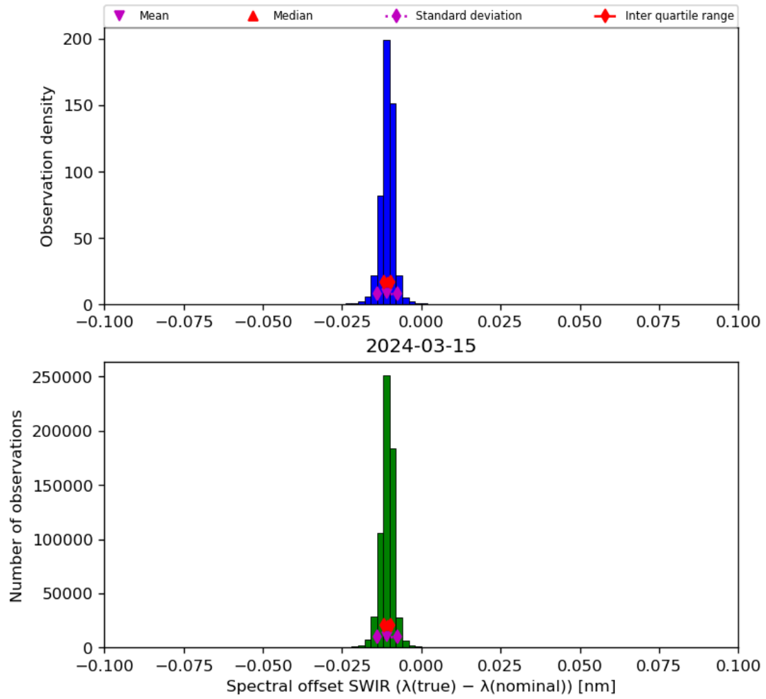
Figure 27: Histogram of “Spectral offset SWIR ( \lambda(\text{true}) - \lambda(\text{nominal}) )” for 2024-03-14 to 2024-03-16
