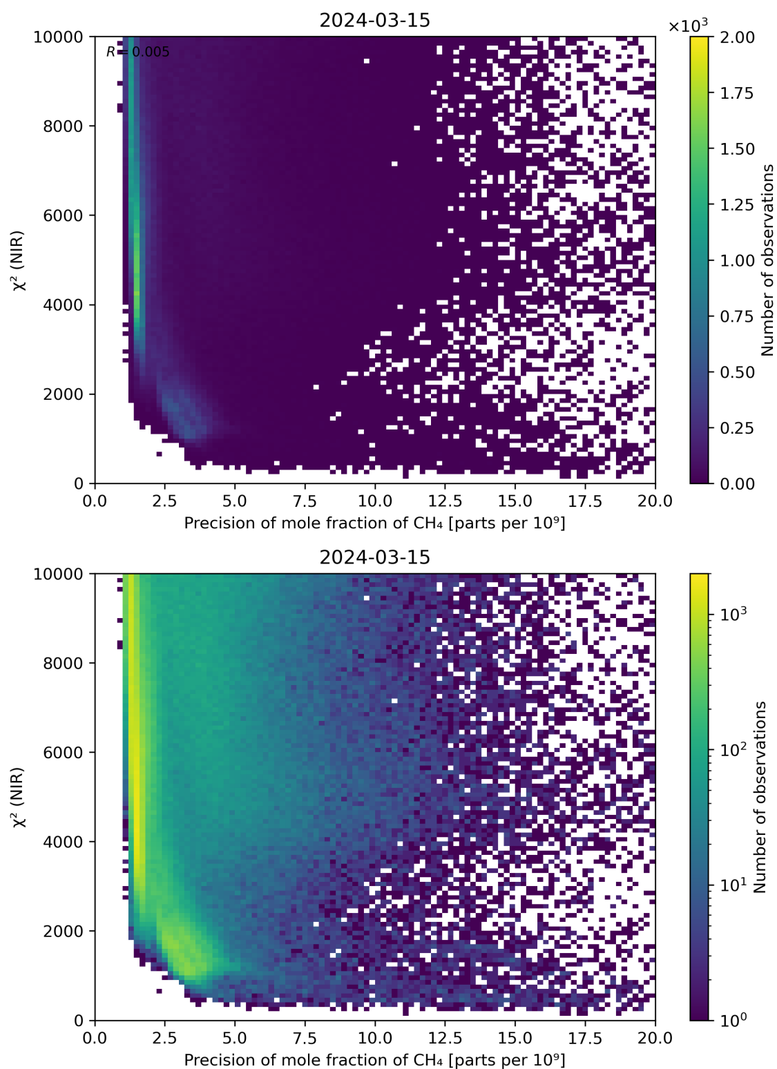
Figure 78: Scatter density plot of “Precision of mole fraction of CH 4 ” against “ \chi^2 (NIR)” for 2024-03-14 to 2024-03-16.
