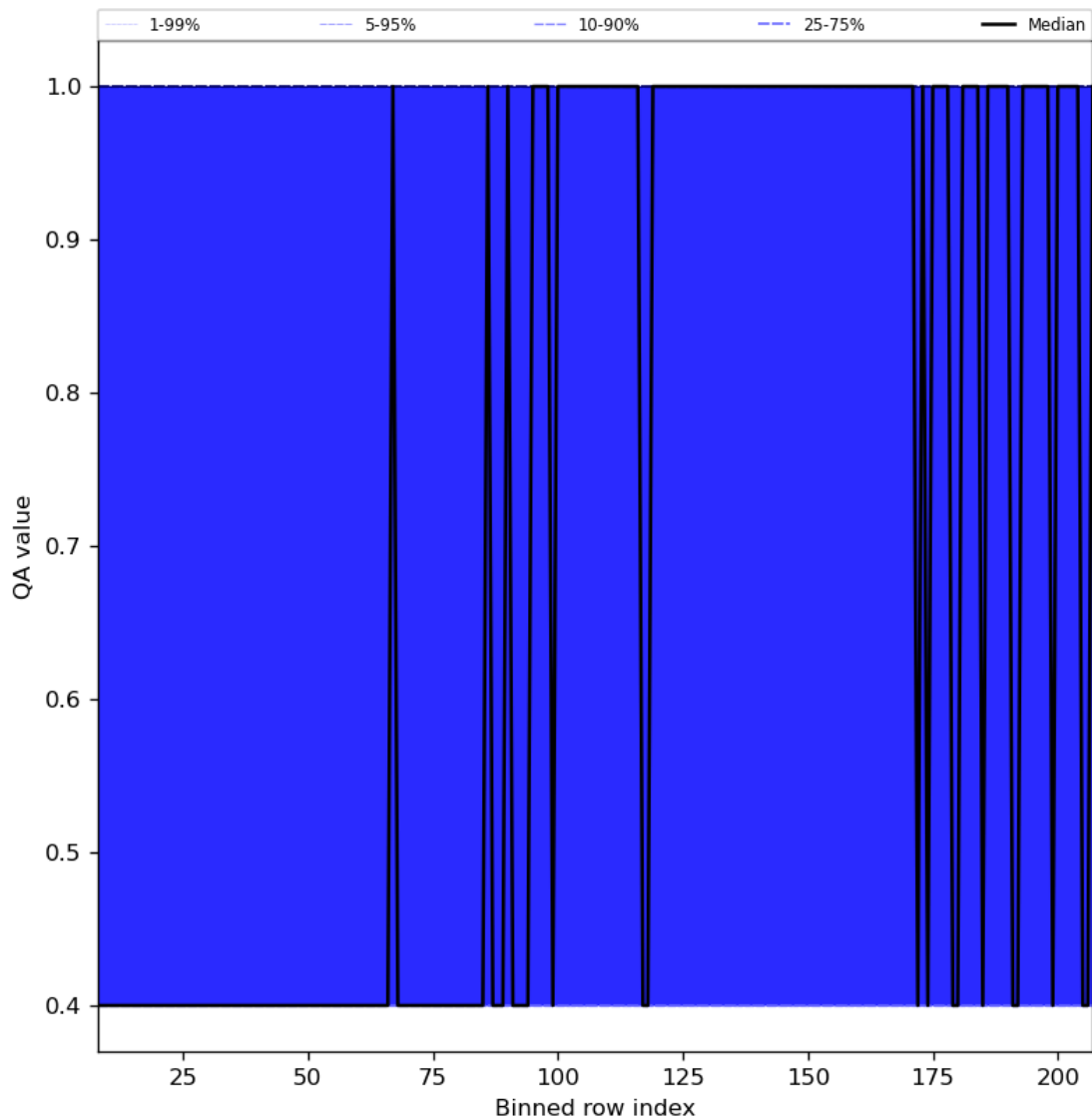
Figure 33: Along track statistics of “QA value” for 2024-03-14 to 2024-03-16
