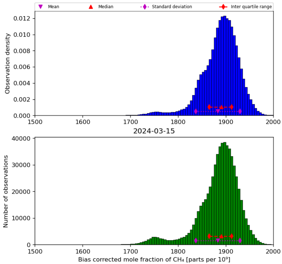
Figure 25: Histogram of “Bias corrected mole fraction of CH 4 ” for 2024-03-14 to 2024-03-16
