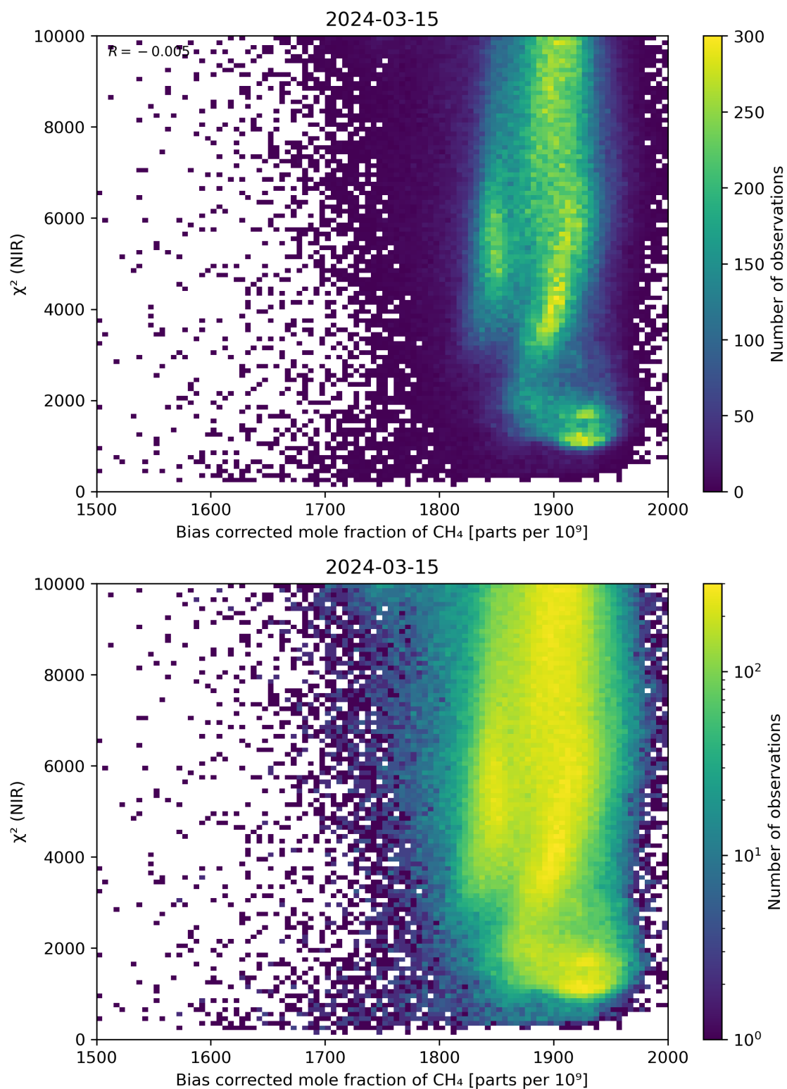
Figure 63: Scatter density plot of “Bias corrected mole fraction of \text{CH}_4 ” against “ \chi^2 (NIR)” for 2024-03-14 to 2024-03-16.
