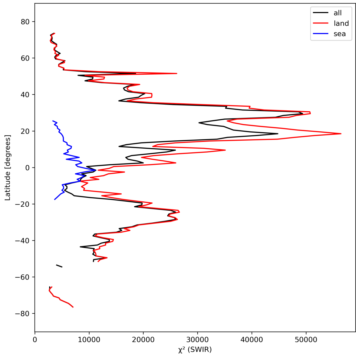
Figure 17: Zonal average of “ \chi^2 (SWIR)” for 2024-03-14 to 2024-03-16.
