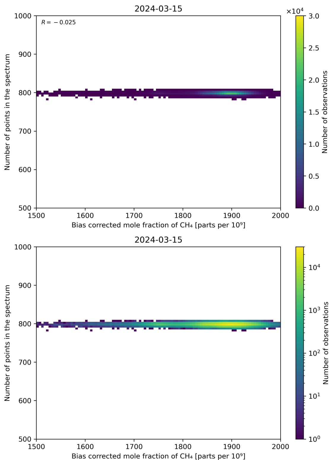
Figure 68: Scatter density plot of “Bias corrected mole fraction of CH 4 ” against “Number of points in the spectrum” for 2024-03-14 to 2024-03-16.
