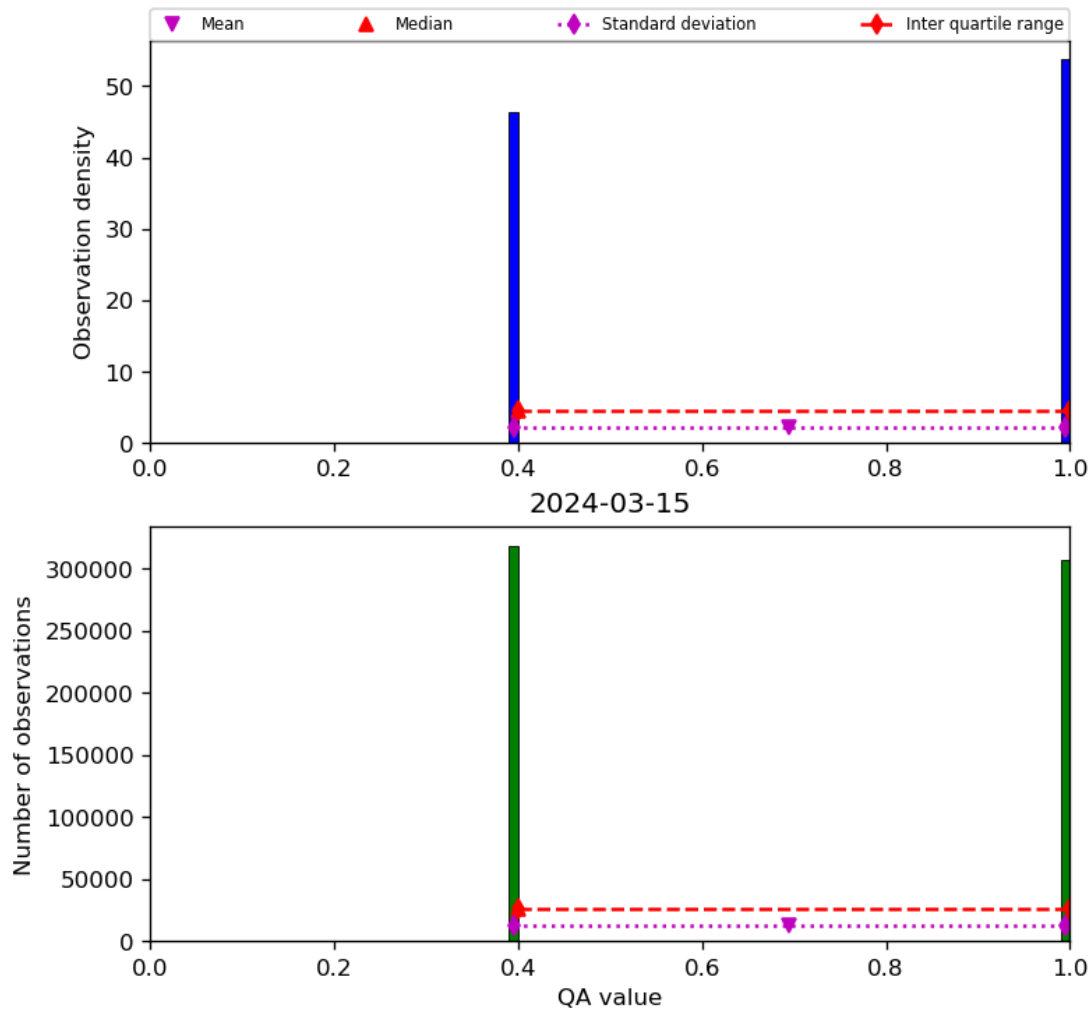
Figure 22: Histogram of “QA value” for 2024-03-14 to 2024-03-16
