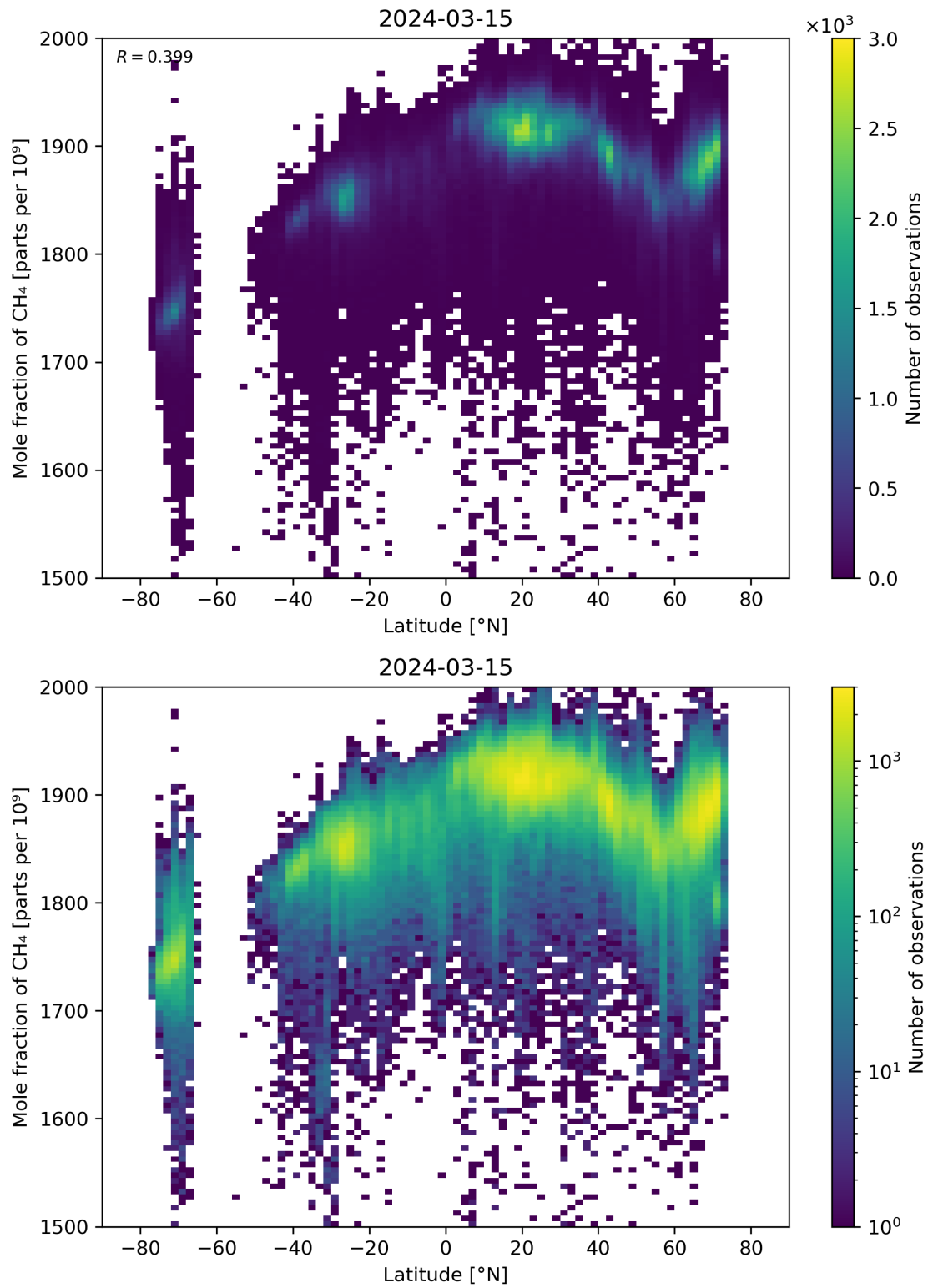
Figure 57: Scatter density plot of “Latitude” against “Mole fraction of \text{CH}_4 ” for 2024-03-14 to 2024-03-16.
