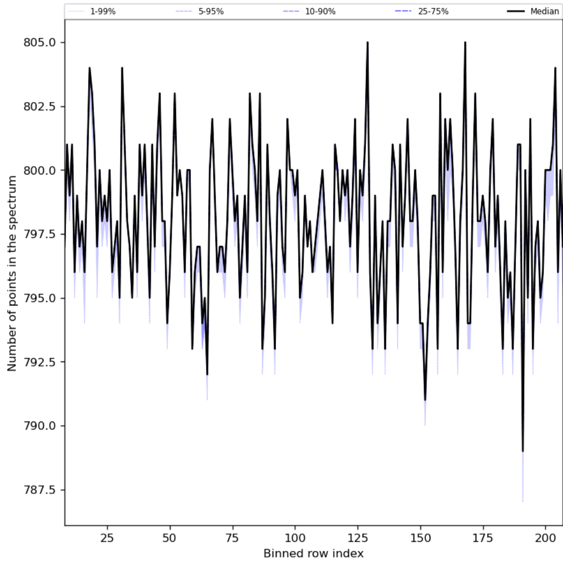
Figure 37: Along track statistics of “Number of points in the spectrum” for 2024-03-14 to 2024-03-16
