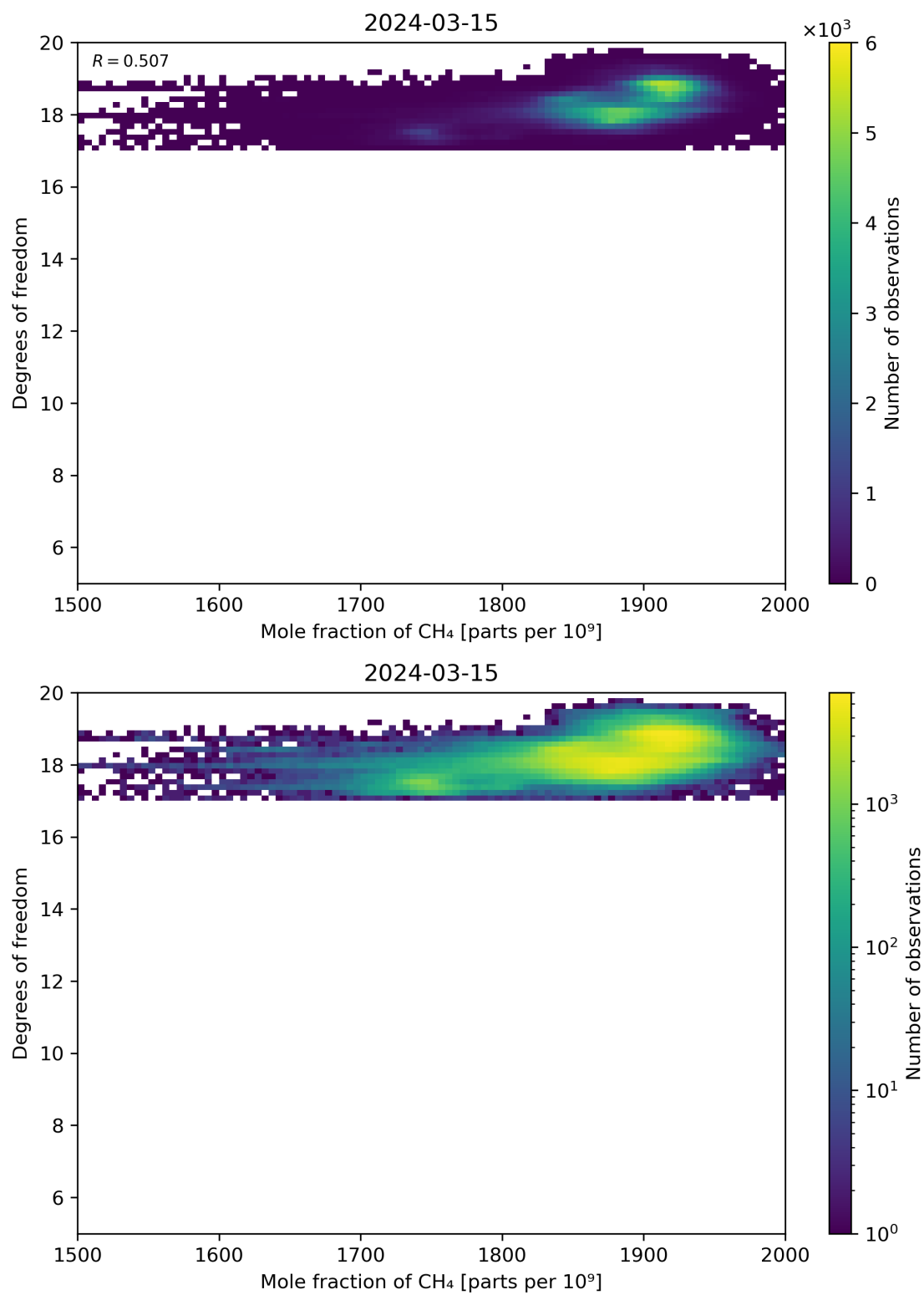
Figure 72: Scatter density plot of “Mole fraction of CH 4 ” against “Degrees of freedom” for 2024-03-14 to 2024-03-16.
