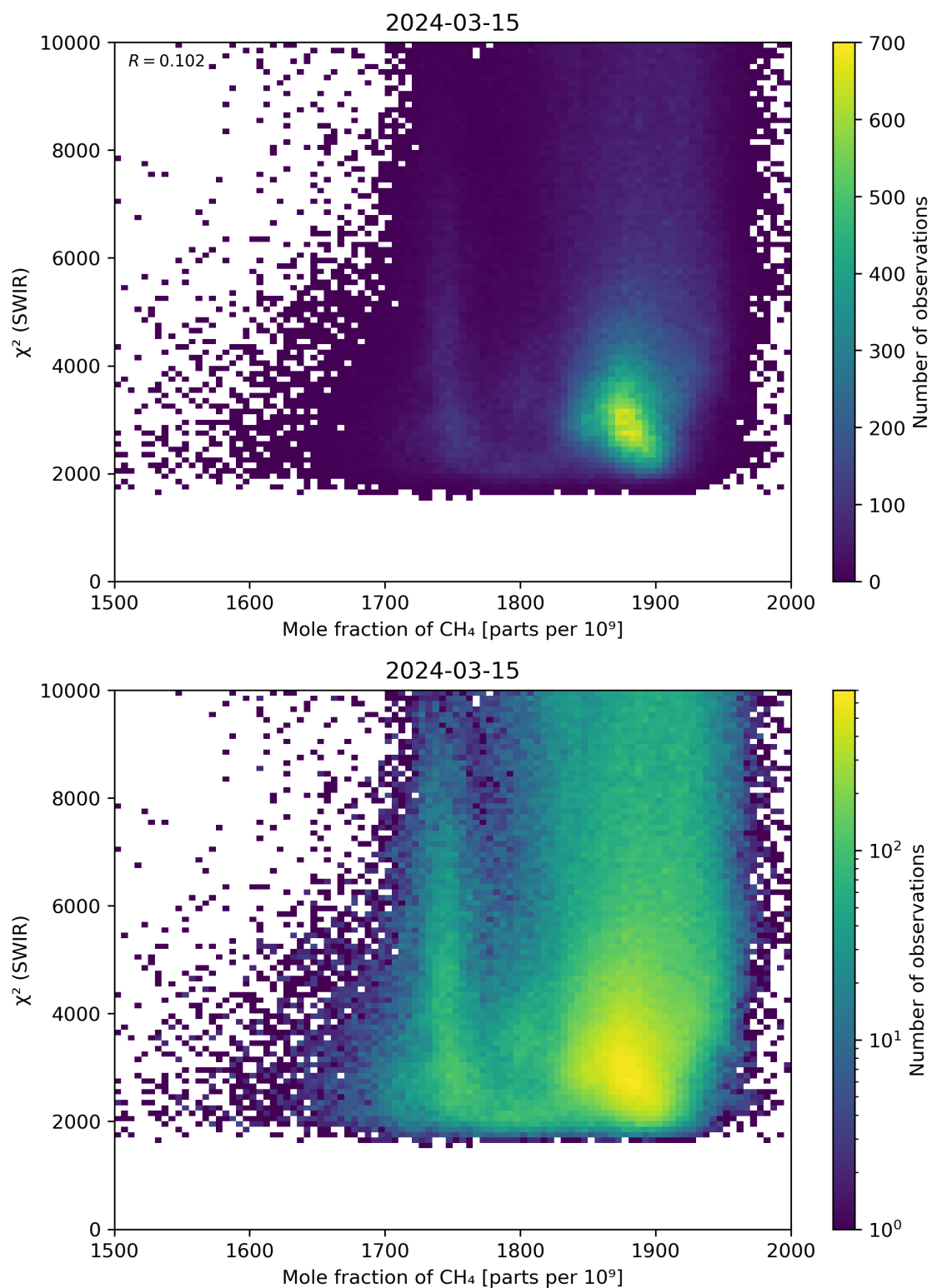
Figure 71: Scatter density plot of “Mole fraction of \text{CH}_4 ” against “ \chi^2 (SWIR)” for 2024-03-14 to 2024-03-16.
