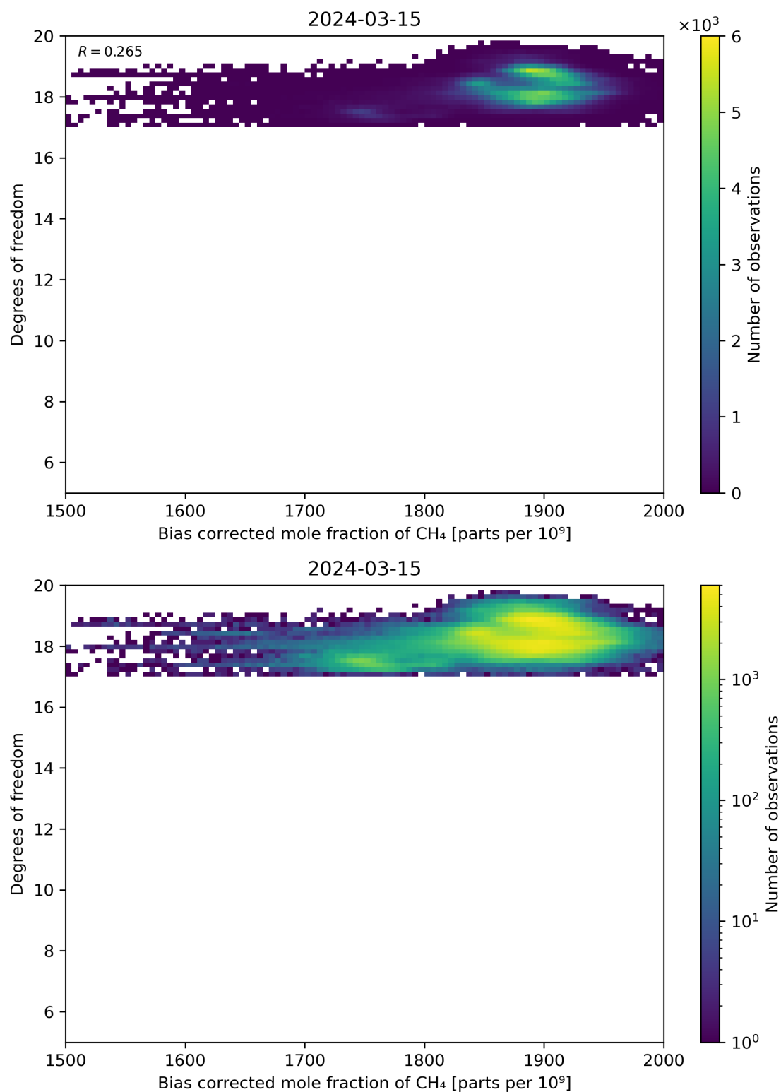
Figure 65: Scatter density plot of “Bias corrected mole fraction of CH 4 ” against “Degrees of freedom” for 2024-03-14 to 2024-03-16.
