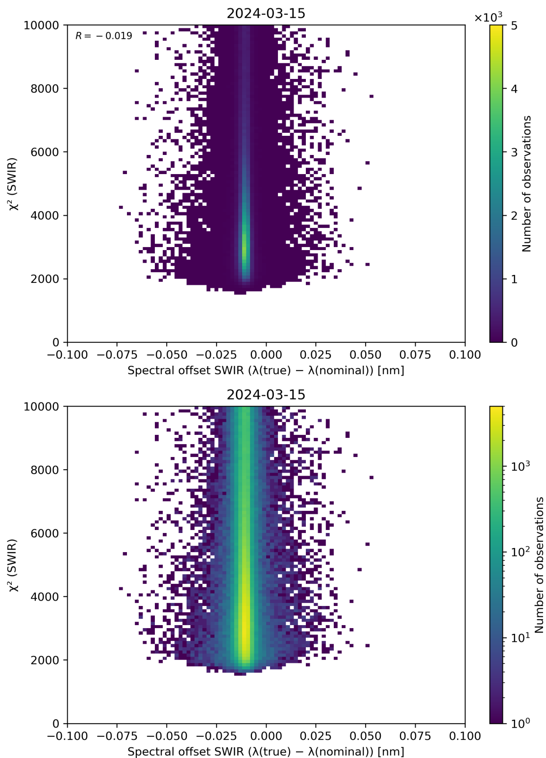
Figure 118: Scatter density plot of “Spectral offset SWIR ( \lambda(\text{true}) - \lambda(\text{nominal}) )” against “ \chi^2 (SWIR)” for 2024-03-14 to 2024-03-16.
