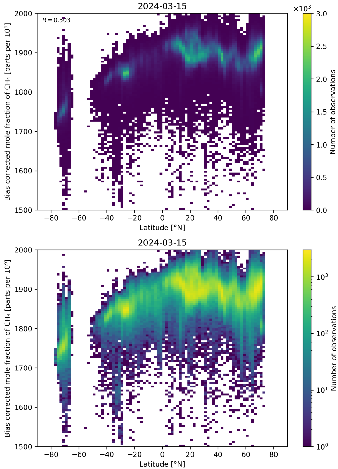
Figure 58: Scatter density plot of “Latitude” against “Bias corrected mole fraction of CH 4 ” for 2024-03-14 to 2024-03-16.
