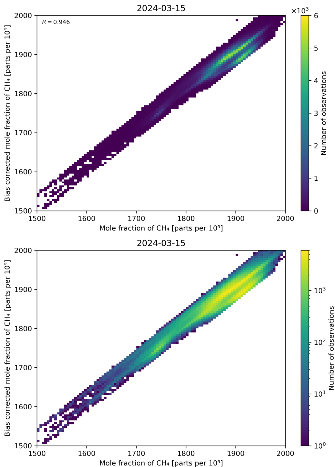
Figure 74: Scatter density plot of “Mole fraction of CH 4 ” against “Bias corrected mole fraction of CH 4 ” for 2024-03-14 to 2024-03-16.
