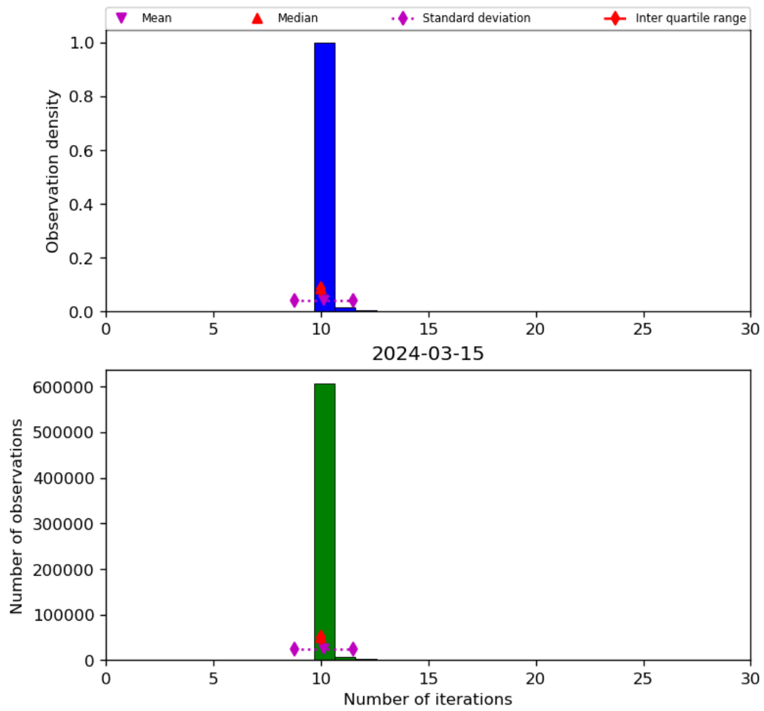
Figure 31: Histogram of “Number of iterations” for 2024-03-14 to 2024-03-16
