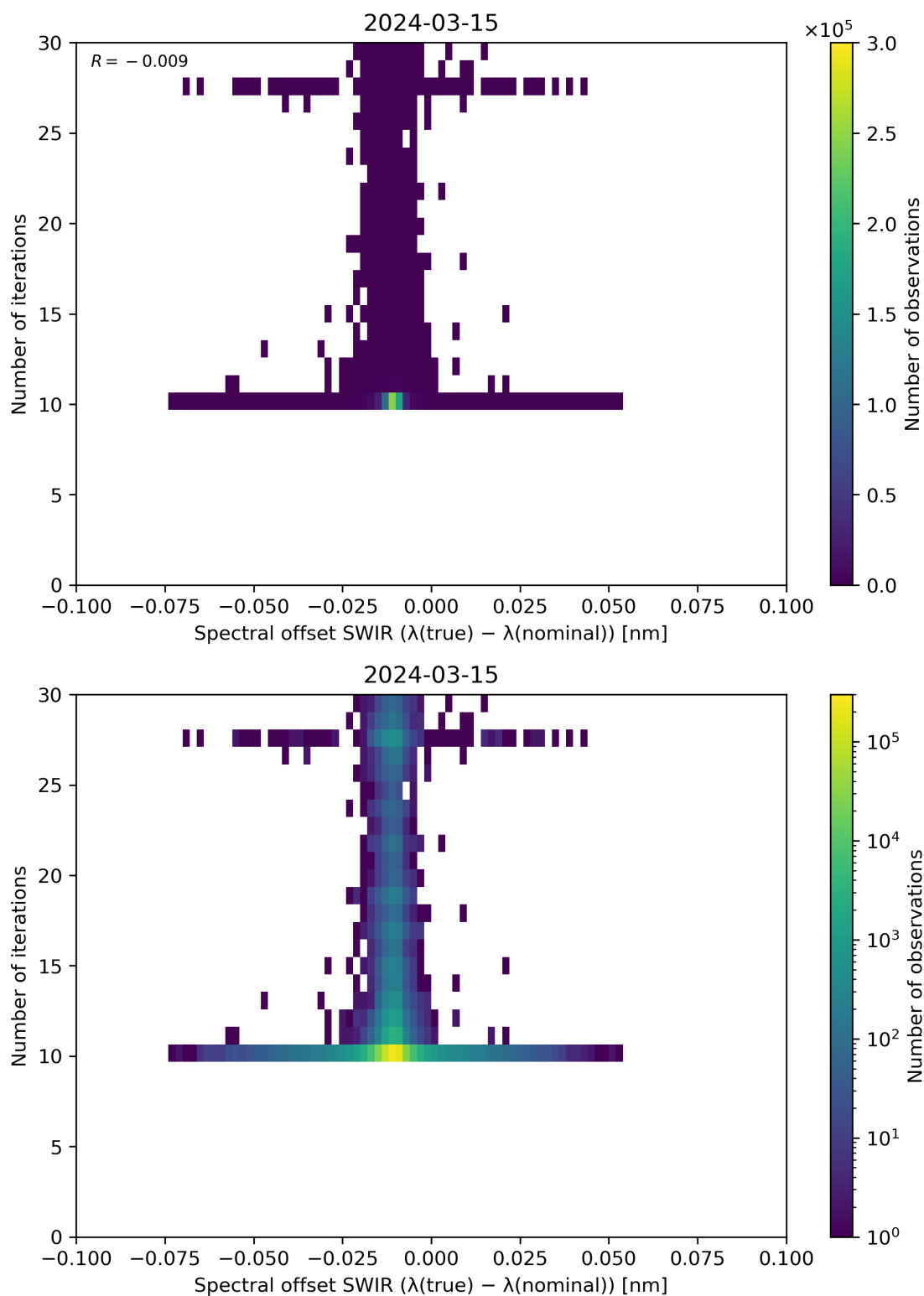
Figure 121: Scatter density plot of “Spectral offset SWIR ( \lambda(\text{true}) - \lambda(\text{nominal}) )” against “Number of iterations” for 2024-03-14 to 2024-03-16.
