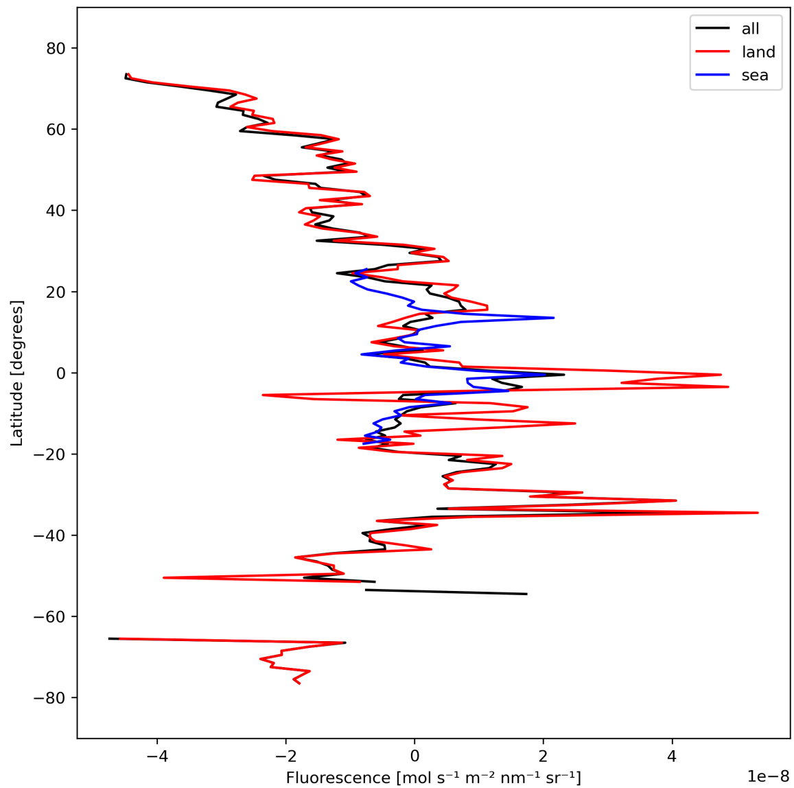
Figure 21: Zonal average of “Fluorescence” for 2024-03-14 to 2024-03-16.
