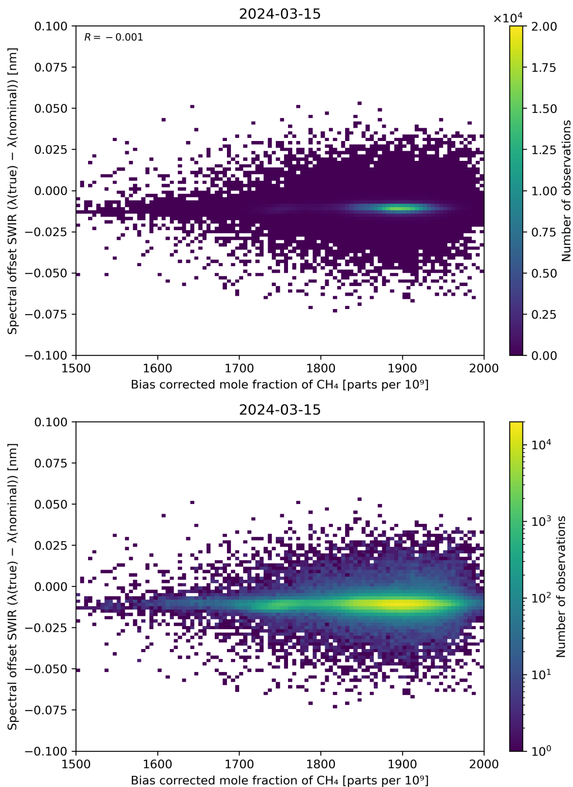
Figure 69: Scatter density plot of “Bias corrected mole fraction of \text{CH}_4 ” against “Spectral offset SWIR ( \lambda(\text{true}) - \lambda(\text{nominal}) )” for 2024-03-14 to 2024-03-16.
