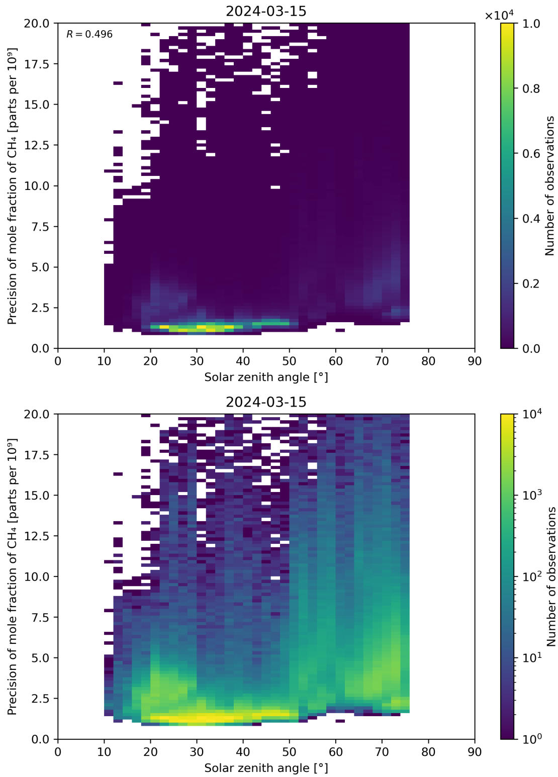
Figure 101: Scatter density plot of “Solar zenith angle” against “Precision of mole fraction of CH 4 ” for 2024-03-14 to 2024-03-16.
