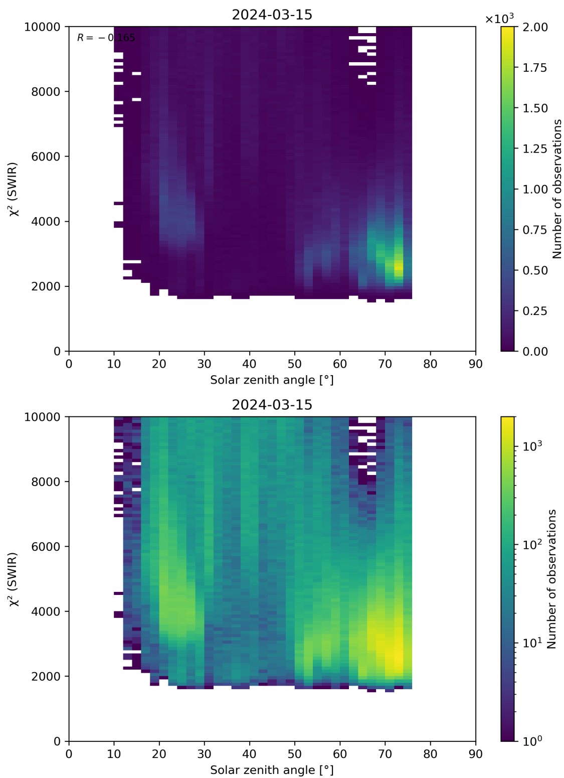
Figure 95: Scatter density plot of “Solar zenith angle” against “ \chi^2 (SWIR)” for 2024-03-14 to 2024-03-16.
