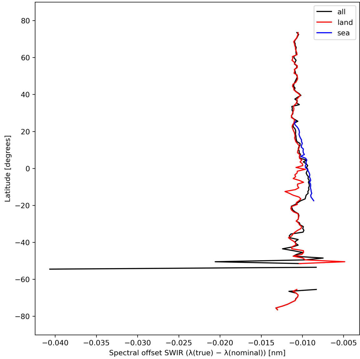
Figure 16: Zonal average of “Spectral offset SWIR ( \lambda(\text{true}) - \lambda(\text{nominal}) )” for 2024-03-14 to 2024-03-16.
