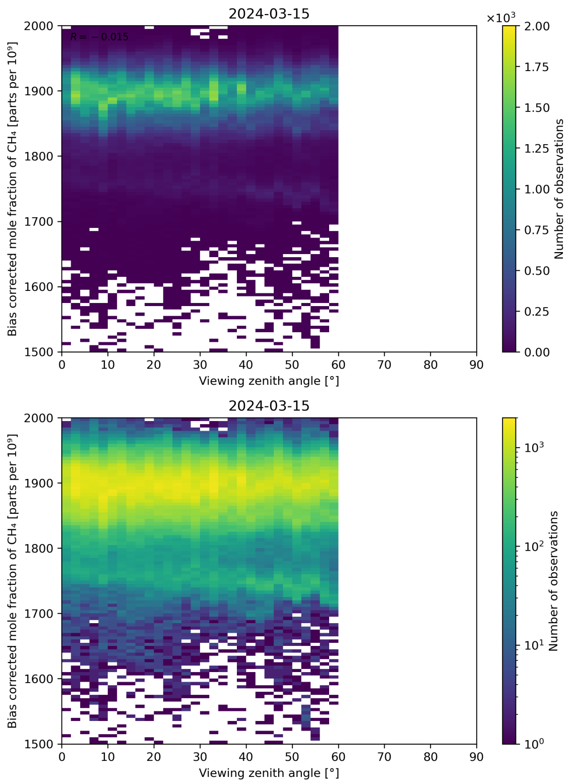
Figure 111: Scatter density plot of “Viewing zenith angle” against “Bias corrected mole fraction of CH 4 ” for 2024-03-14 to 2024-03-16.
