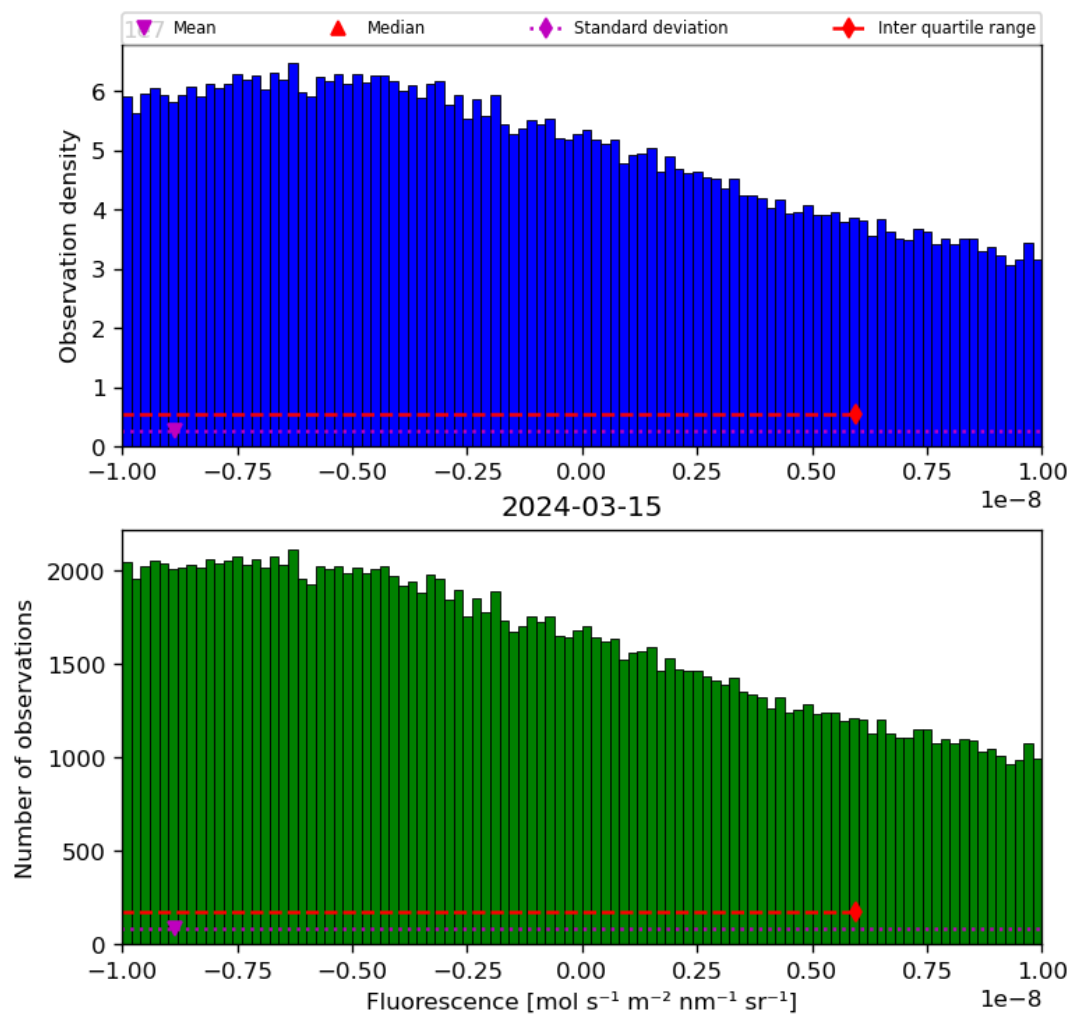
Figure 32: Histogram of “Fluorescence” for 2024-03-14 to 2024-03-16
