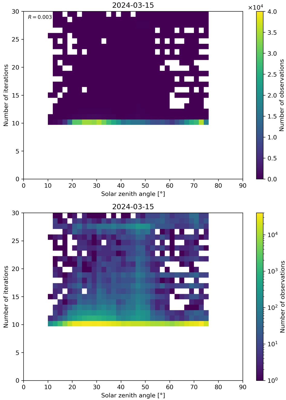
Figure 102: Scatter density plot of “Solar zenith angle” against “Number of iterations” for 2024-03-14 to 2024-03-16.
