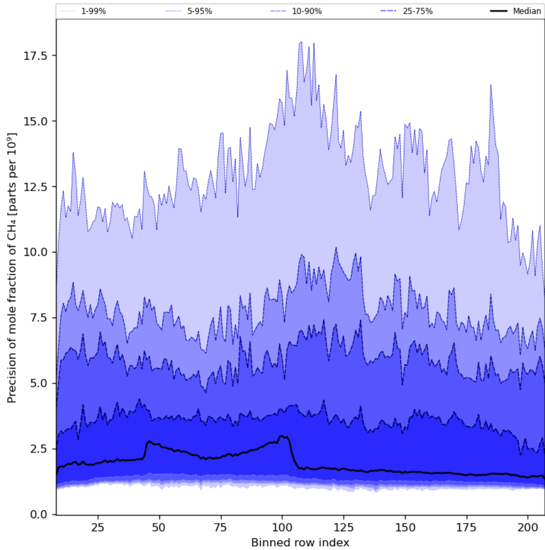
Figure 35: Along track statistics of “Precision of mole fraction of CH 4 ” for 2024-03-14 to 2024-03-16
