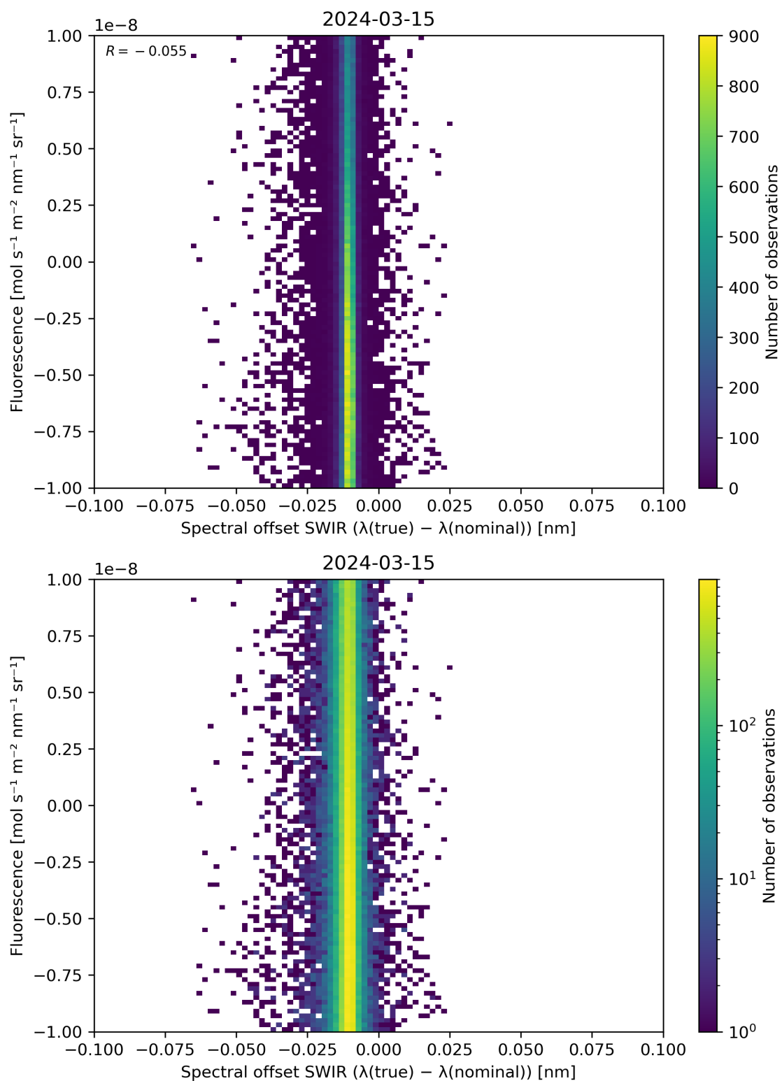
Figure 120: Scatter density plot of “Spectral offset SWIR ( \lambda(\text{true}) - \lambda(\text{nominal}) )” against “Fluorescence” for 2024-03-14 to 2024-03-16.
