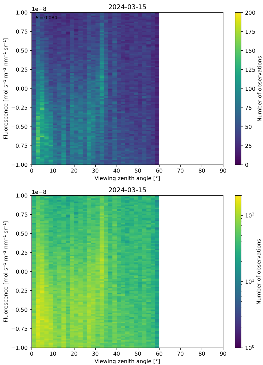
Figure 108: Scatter density plot of “Viewing zenith angle” against “Fluorescence” for 2024-03-14 to 2024-03-16.
