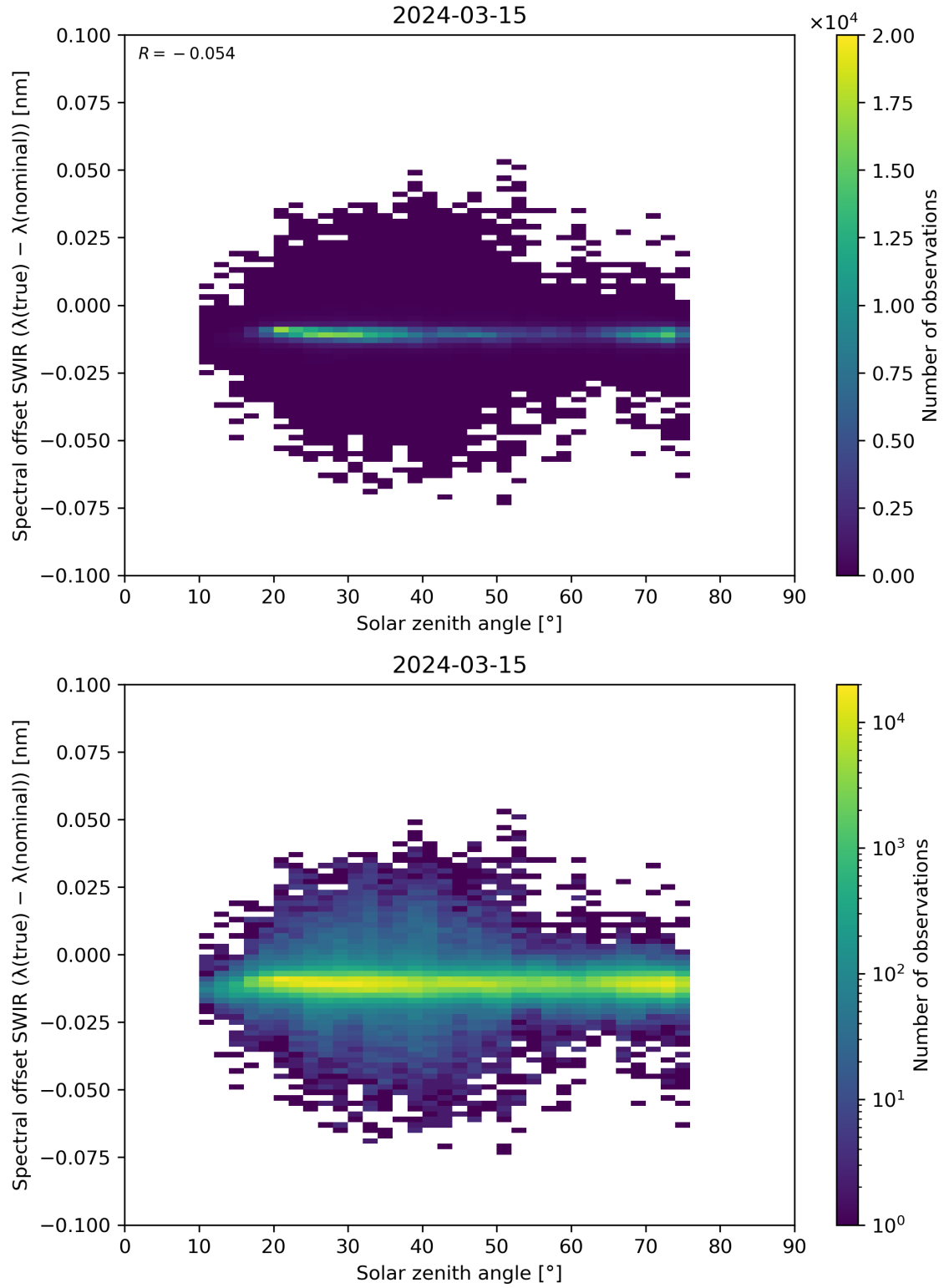
Figure 104: Scatter density plot of “Solar zenith angle” against “Spectral offset SWIR ( \lambda(\text{true}) - \lambda(\text{nominal}) )” for 2024-03-14 to 2024-03-16.
