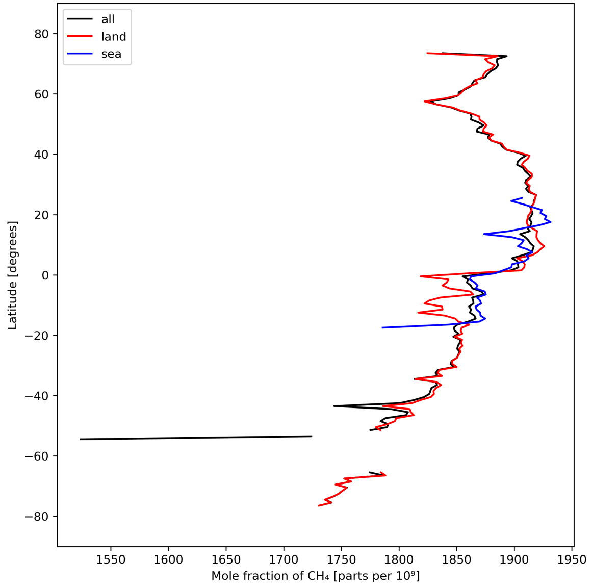
Figure 12: Zonal average of “Mole fraction of \text{CH}_4 ” for 2024-03-14 to 2024-03-16.
