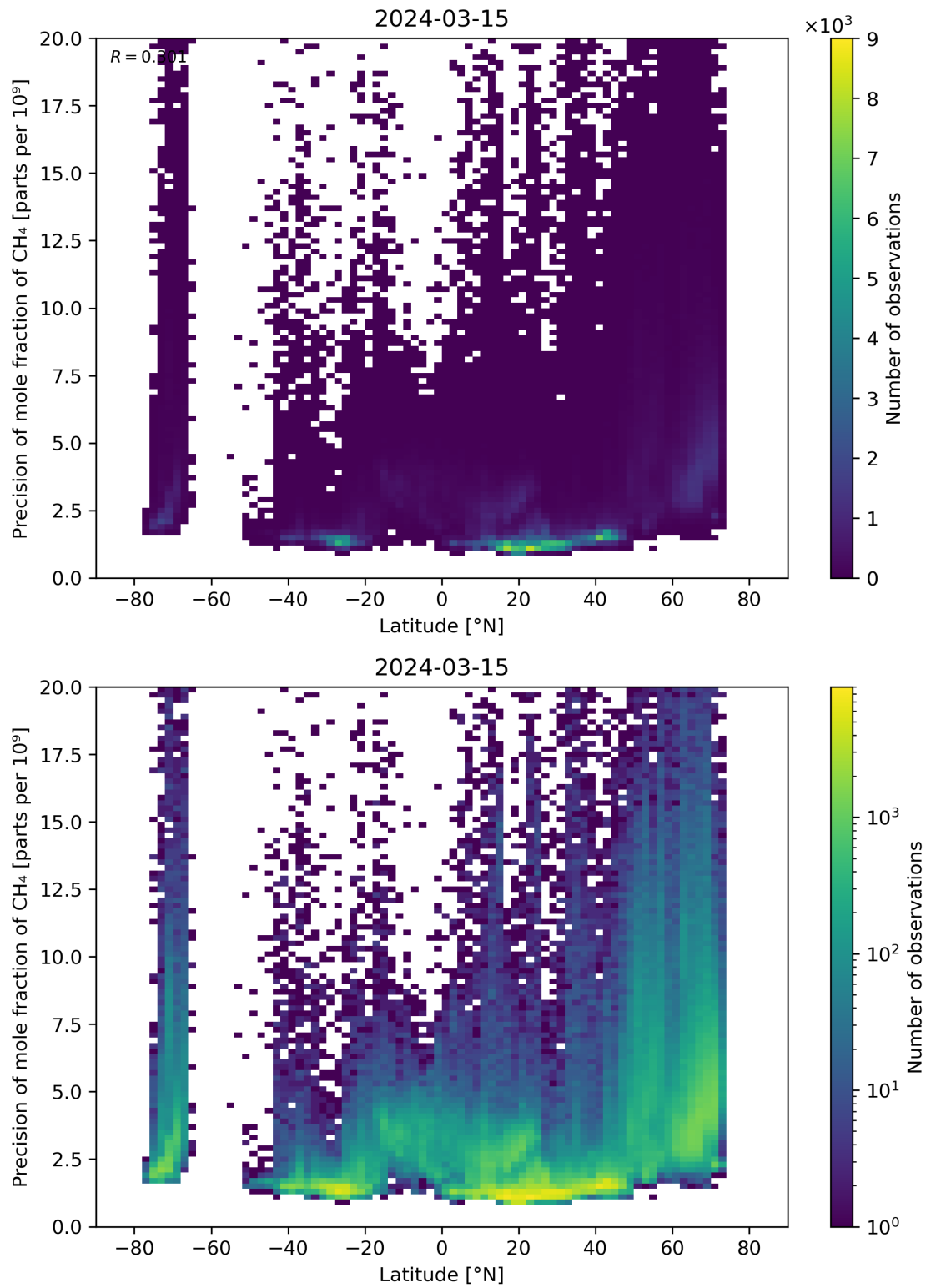
Figure 59: Scatter density plot of “Latitude” against “Precision of mole fraction of CH 4 ” for 2024-03-14 to 2024-03-16.
