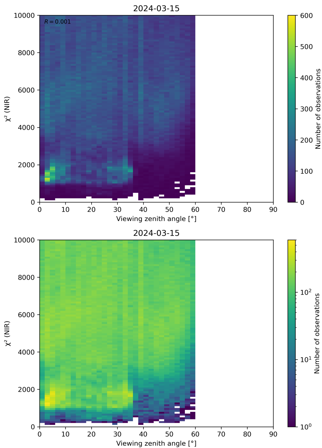
Figure 105: Scatter density plot of “Viewing zenith angle” against “ \chi^2 (NIR)” for 2024-03-14 to 2024-03-16.
