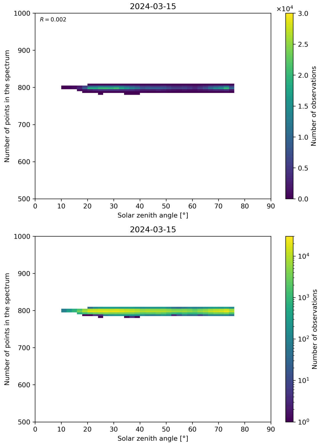
Figure 103: Scatter density plot of “Solar zenith angle” against “Number of points in the spectrum” for 2024-03-14 to 2024-03-16.
