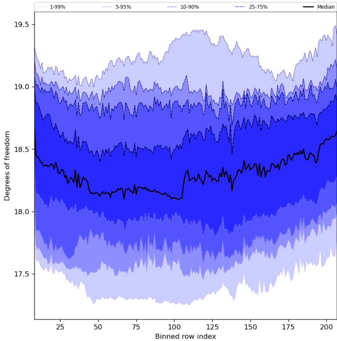
Figure 41: Along track statistics of “Degrees of freedom” for 2024-03-14 to 2024-03-16
