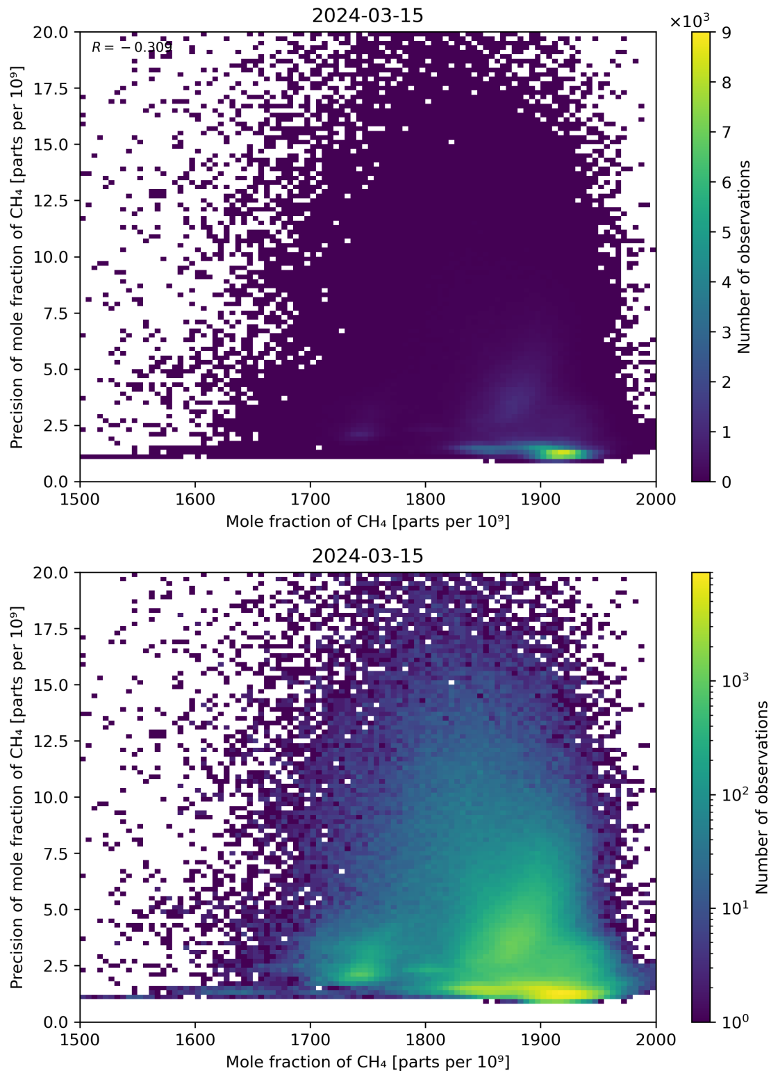
Figure 75: Scatter density plot of “Mole fraction of CH 4 ” against “Precision of mole fraction of CH 4 ” for 2024-03-14 to 2024-03-16.
