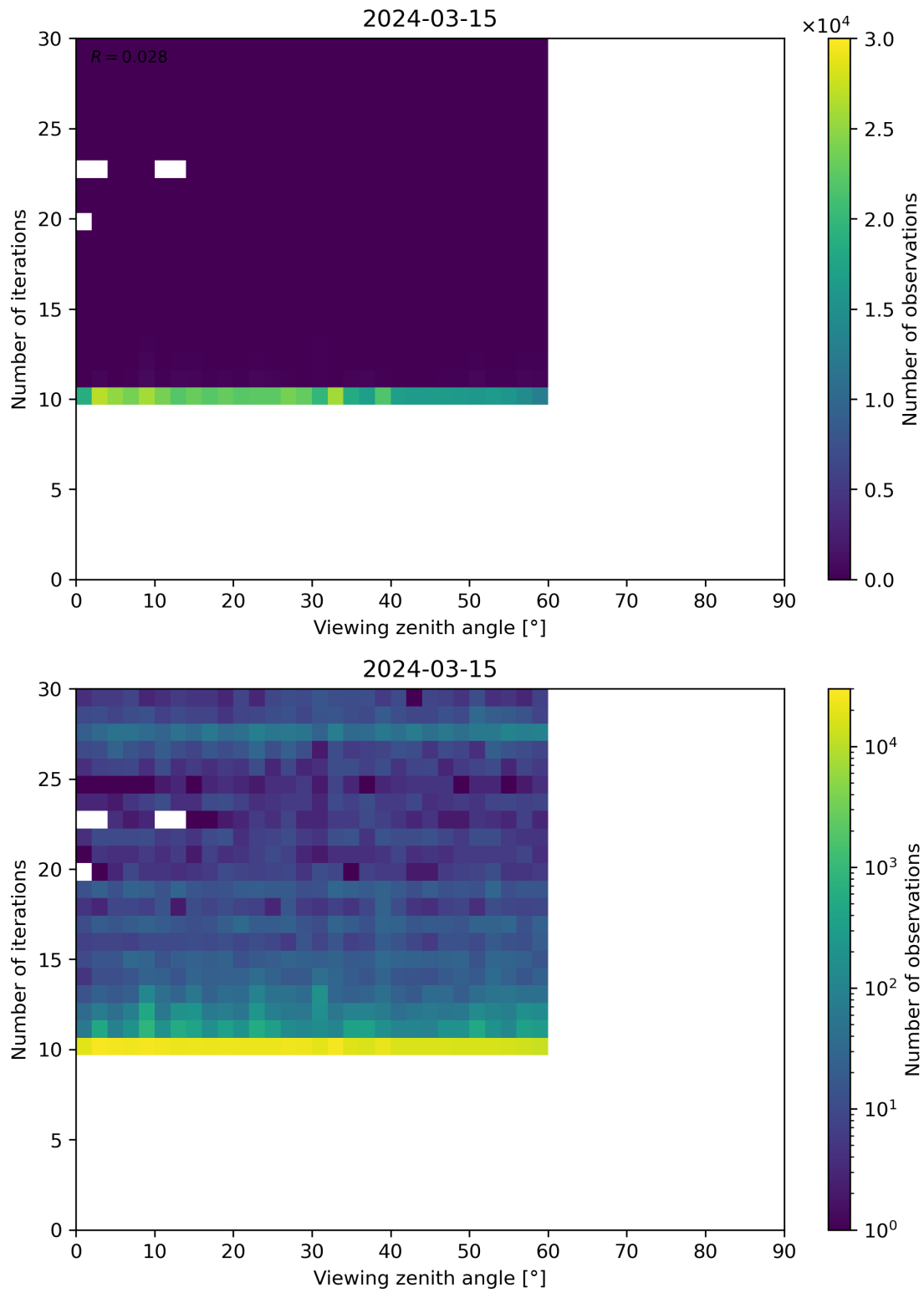
Figure 113: Scatter density plot of “Viewing zenith angle” against “Number of iterations” for 2024-03-14 to 2024-03-16.
