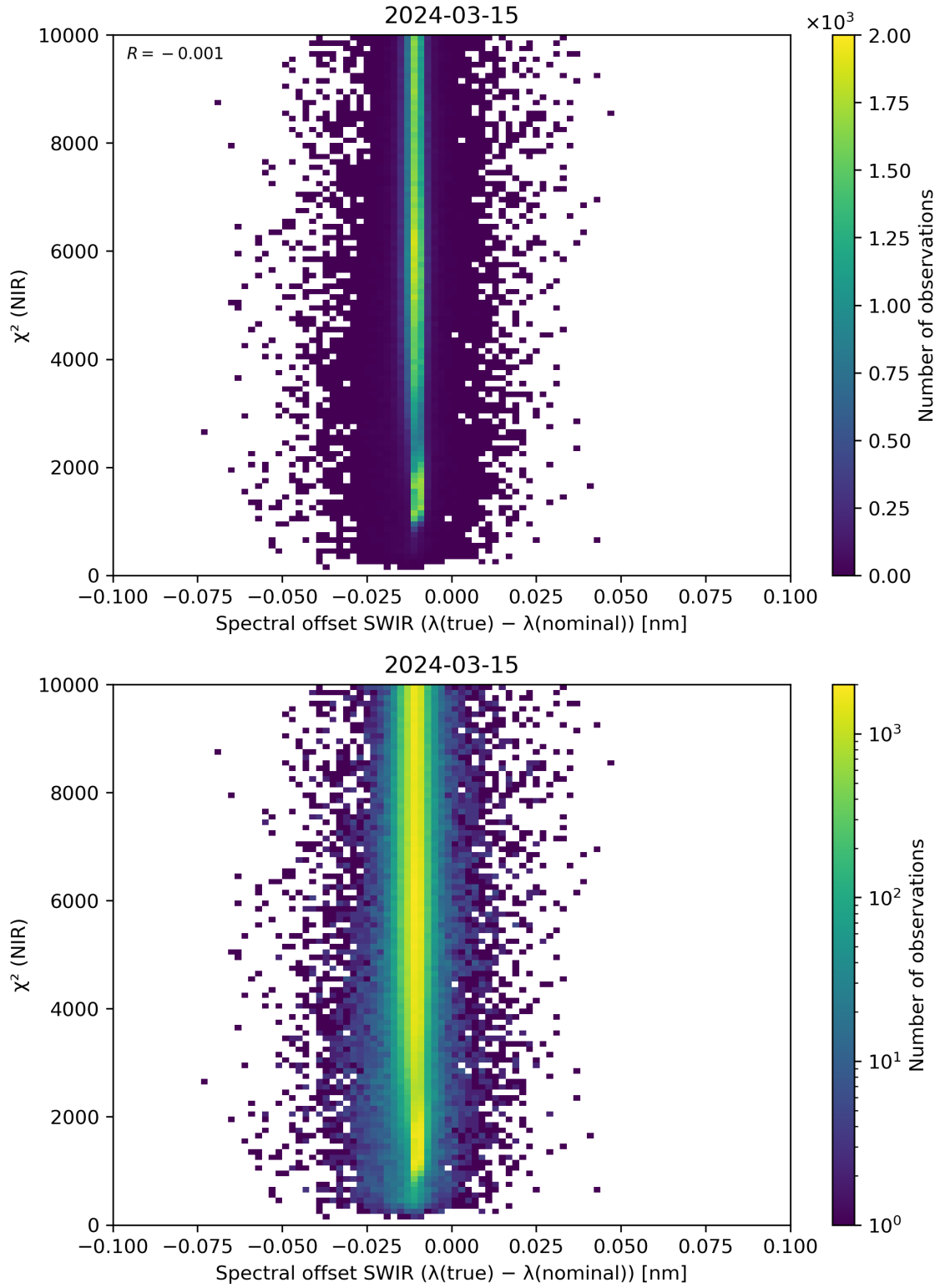
Figure 117: Scatter density plot of “Spectral offset SWIR ( \lambda(\text{true}) - \lambda(\text{nominal}) )” against “ \chi^2 (NIR)” for 2024-03-14 to 2024-03-16.
