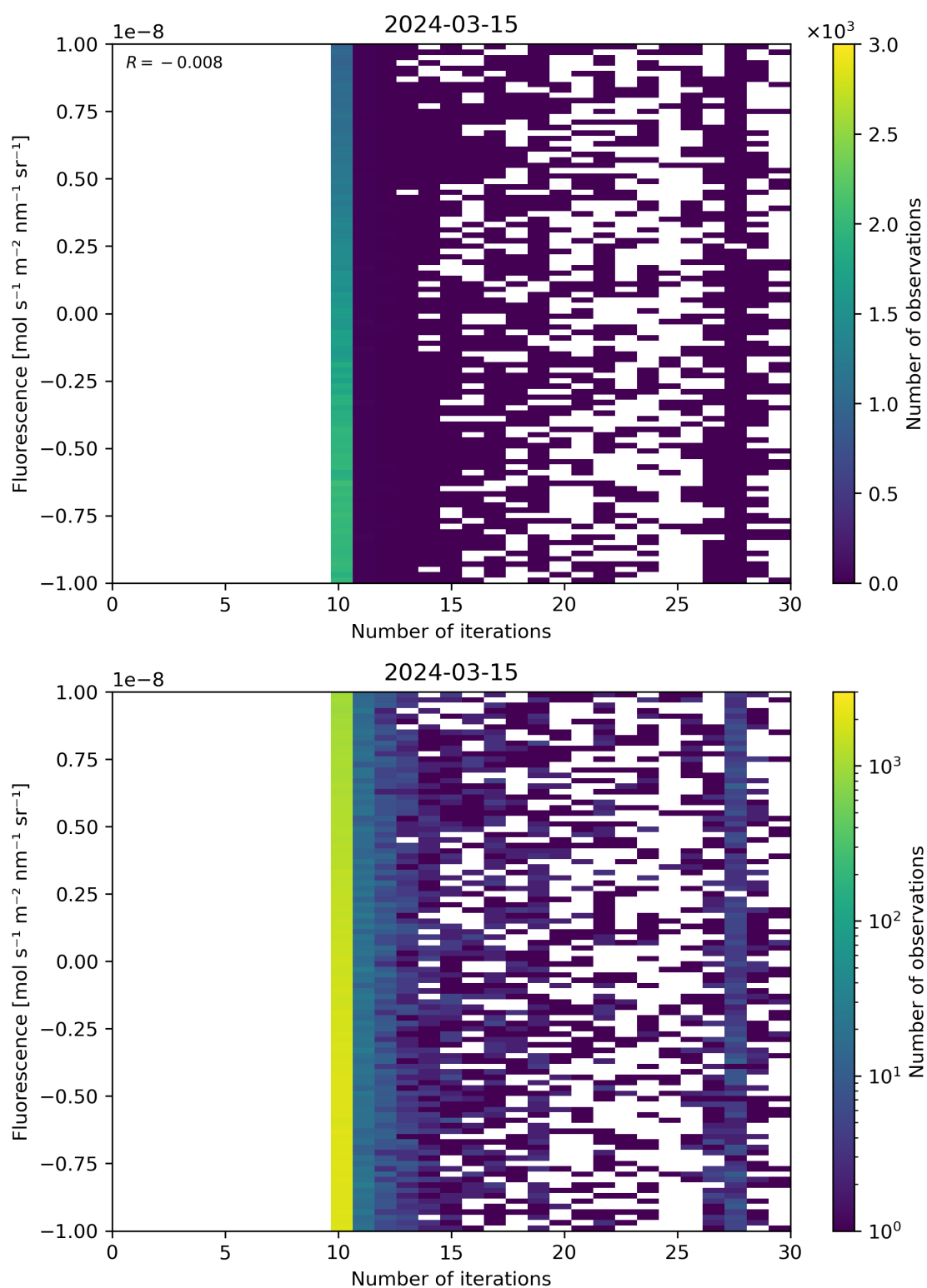
Figure 87: Scatter density plot of “Number of iterations” against “Fluorescence” for 2024-03-14 to 2024-03-16.
