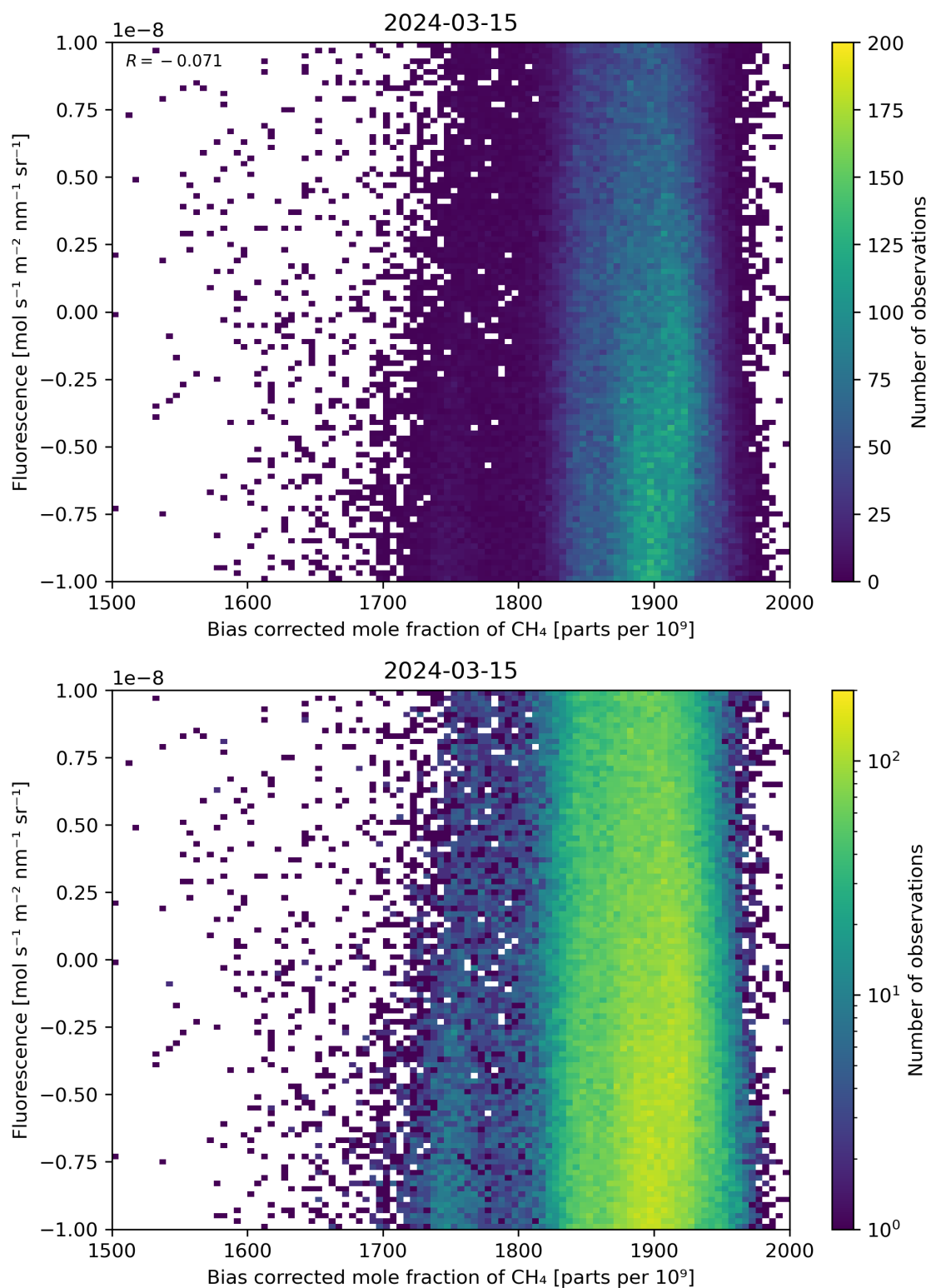
Figure 66: Scatter density plot of “Bias corrected mole fraction of \text{CH}_4 ” against “Fluorescence” for 2024-03-14 to 2024-03-16.
