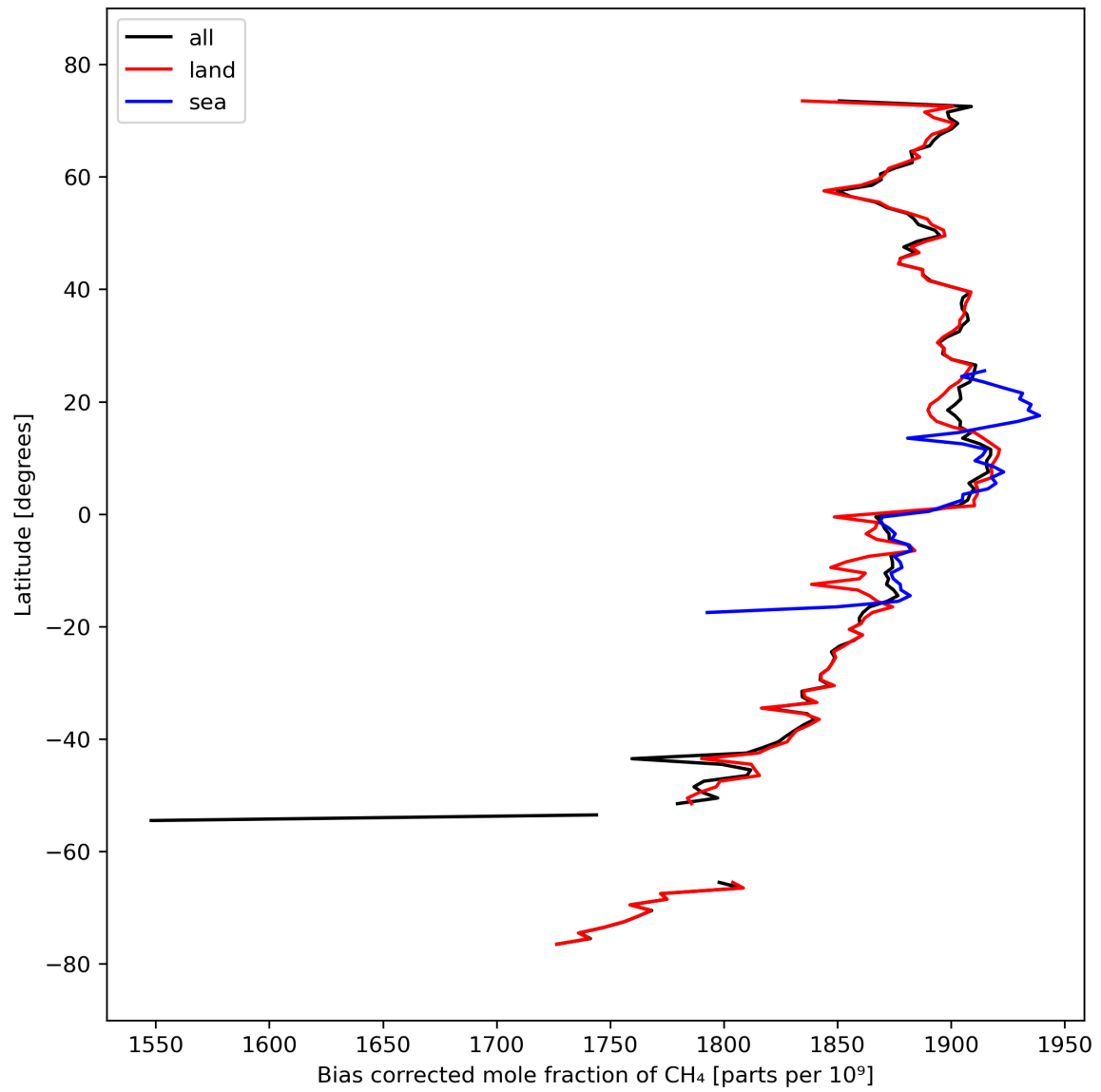
Figure 14: Zonal average of “Bias corrected mole fraction of CH 4 ” for 2024-03-14 to 2024-03-16.
