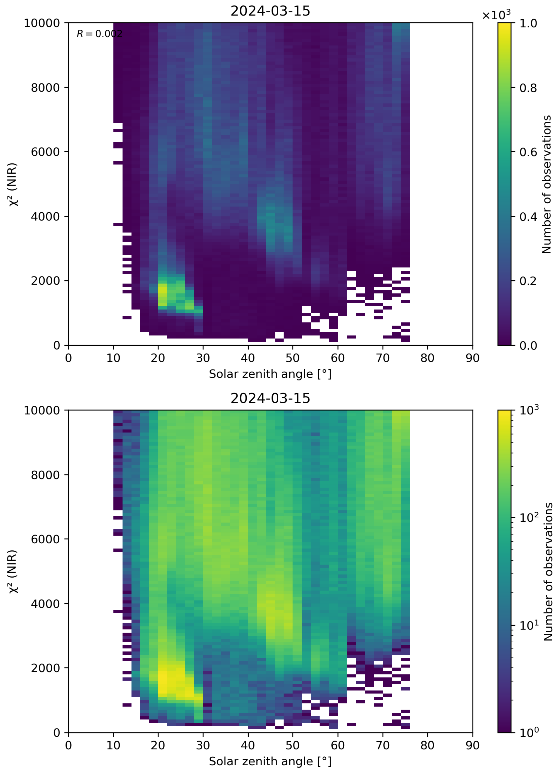
Figure 94: Scatter density plot of “Solar zenith angle” against “ \chi^2 (NIR)” for 2024-03-14 to 2024-03-16.
