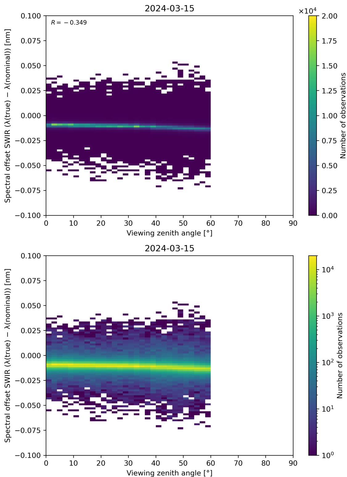
Figure 116: Scatter density plot of “Viewing zenith angle” against “Spectral offset SWIR ( \lambda(\text{true}) - \lambda(\text{nominal}) )” for 2024-03-14 to 2024-03-16.
