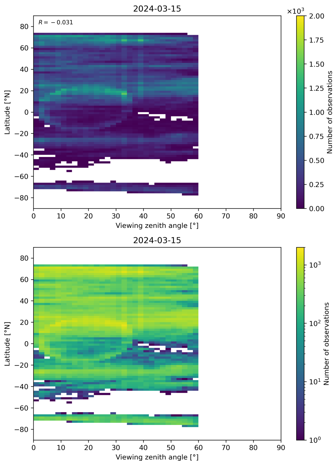
Figure 109: Scatter density plot of “Viewing zenith angle” against “Latitude” for 2024-03-14 to 2024-03-16.
