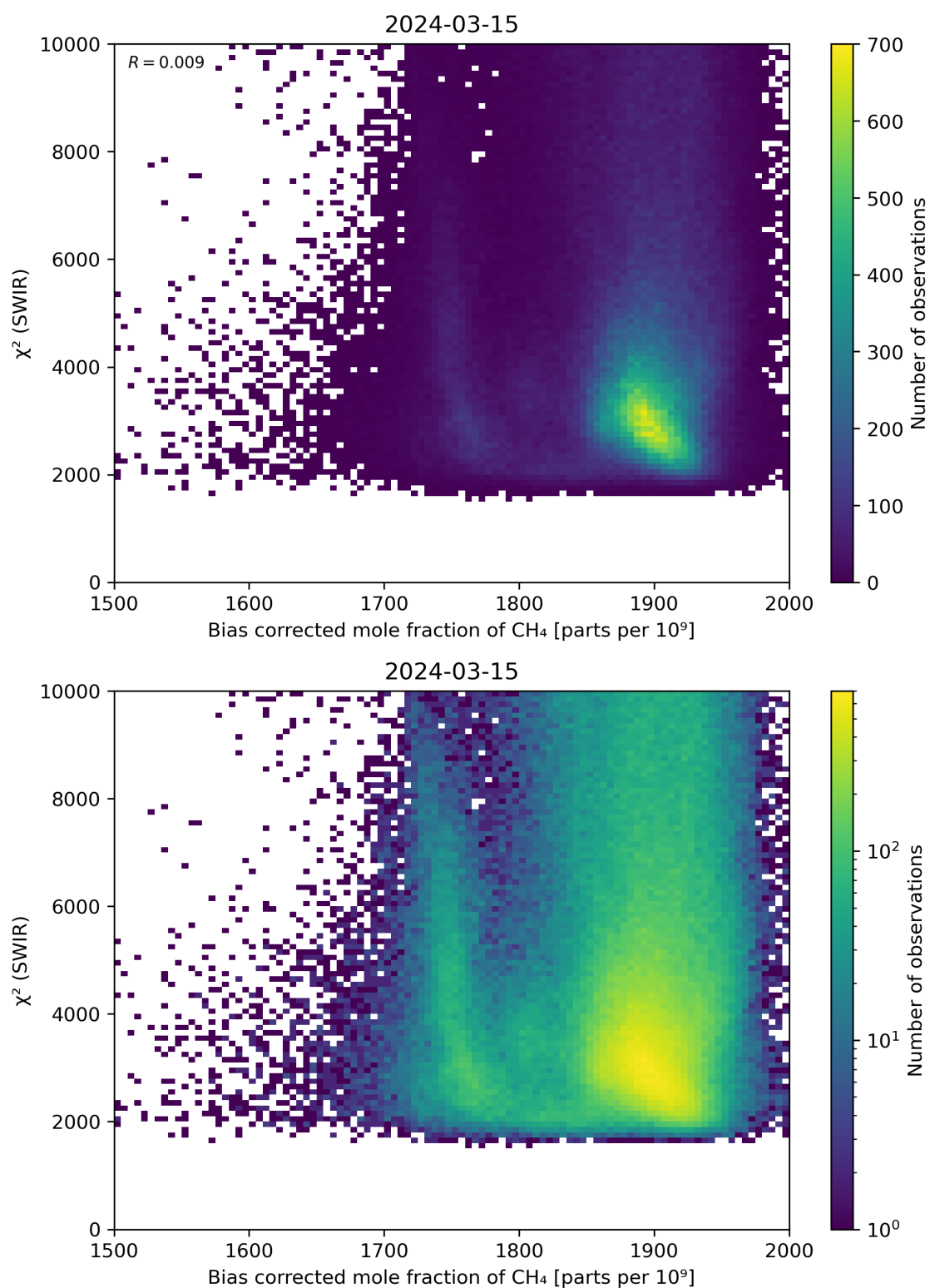
Figure 64: Scatter density plot of “Bias corrected mole fraction of \text{CH}_4 ” against “ \chi^2 (SWIR)” for 2024-03-14 to 2024-03-16.
