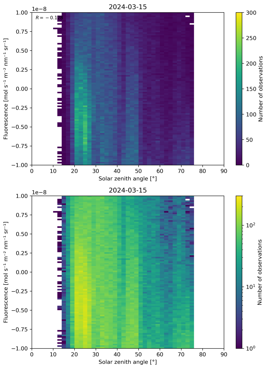
Figure 97: Scatter density plot of “Solar zenith angle” against “Fluorescence” for 2024-03-14 to 2024-03-16.
