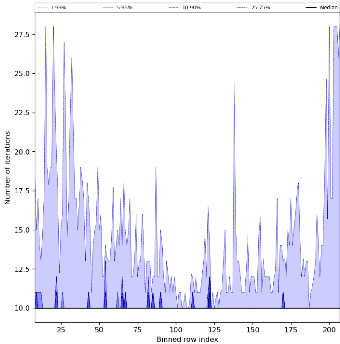
Figure 42: Along track statistics of “Number of iterations” for 2024-03-14 to 2024-03-16
