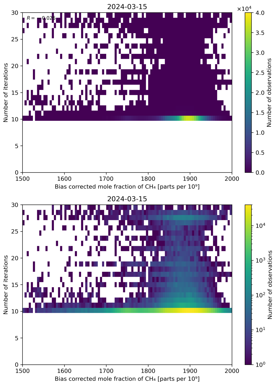
Figure 67: Scatter density plot of “Bias corrected mole fraction of \text{CH}_4 ” against “Number of iterations” for 2024-03-14 to 2024-03-16.
