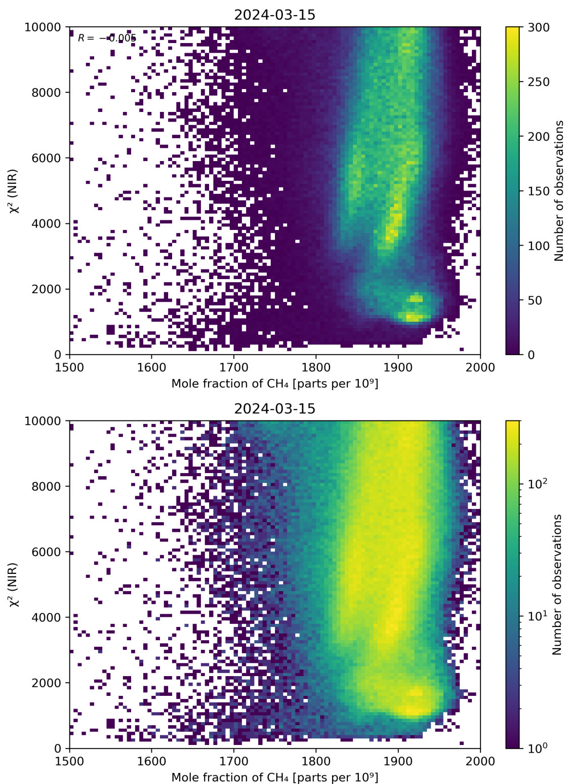
Figure 70: Scatter density plot of “Mole fraction of \text{CH}_4 ” against “ \chi^2 (NIR)” for 2024-03-14 to 2024-03-16.
