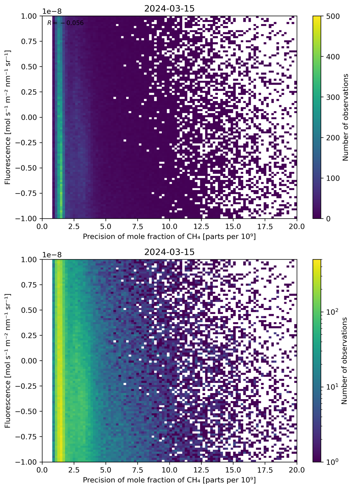
Figure 81: Scatter density plot of “Precision of mole fraction of \text{CH}_4 ” against “Fluorescence” for 2024-03-14 to 2024-03-16.
