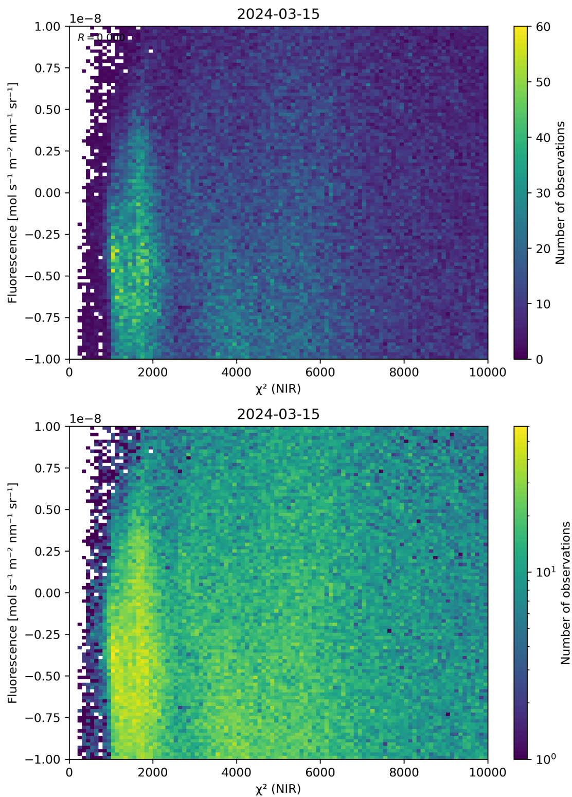
Figure 45: Scatter density plot of “ \chi^2 (NIR)” against “Fluorescence” for 2024-03-14 to 2024-03-16.
