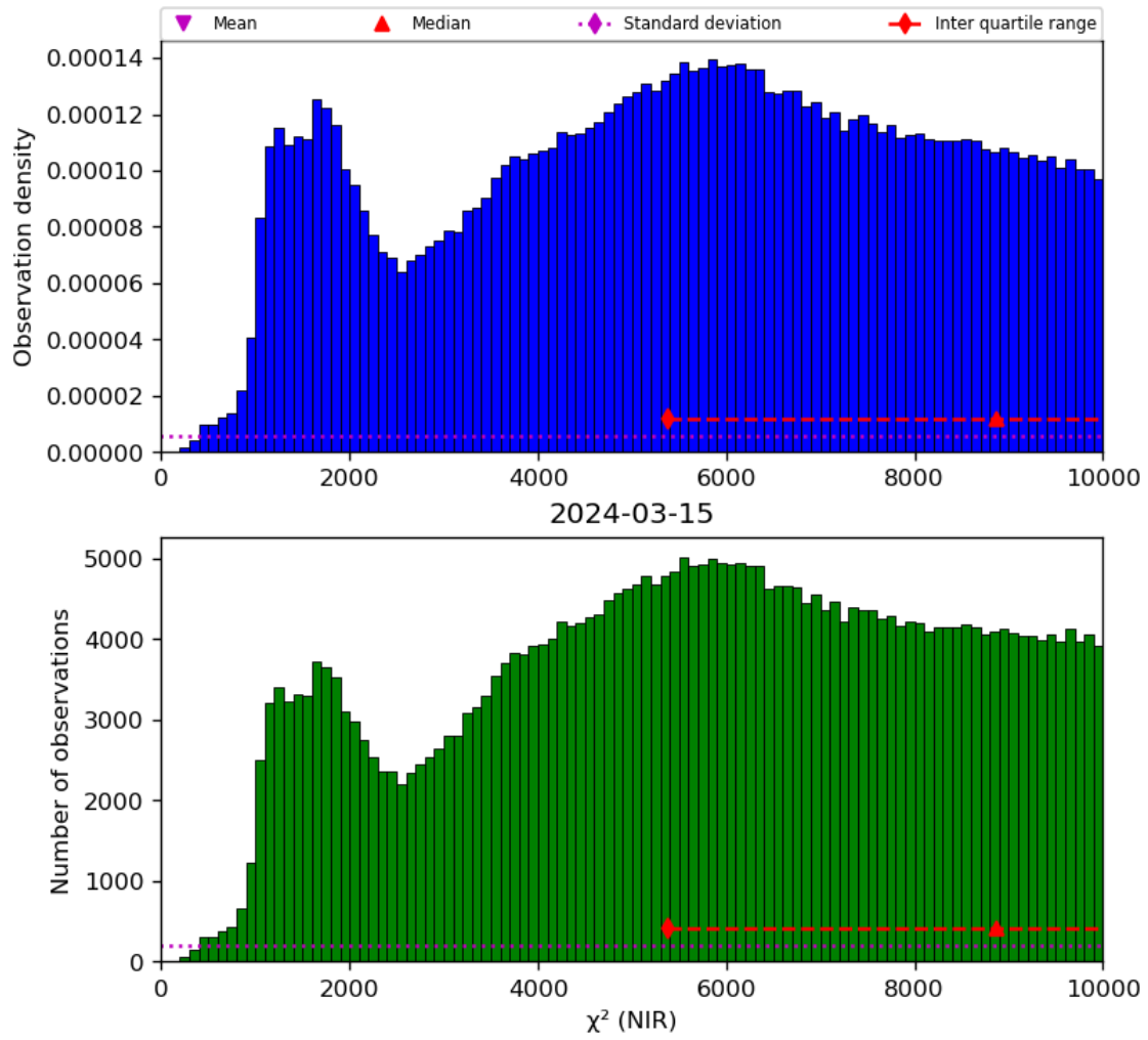
Figure 29: Histogram of “ \chi^2 (NIR)” for 2024-03-14 to 2024-03-16
