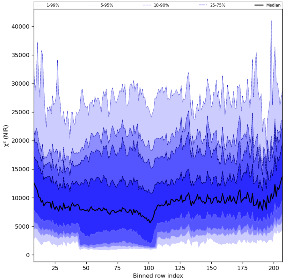
Figure 40: Along track statistics of " \chi^2 (NIR)" for 2024-03-14 to 2024-03-16
