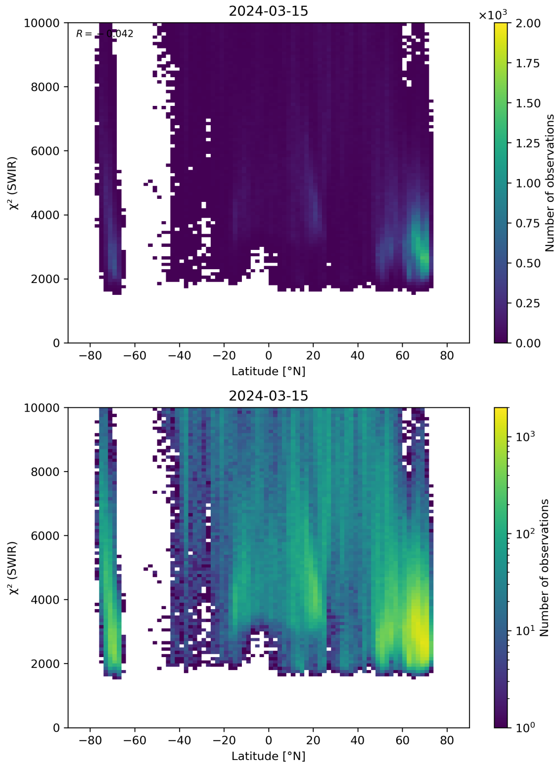
Figure 54: Scatter density plot of “Latitude” against “ \chi^2 (SWIR)” for 2024-03-14 to 2024-03-16.
