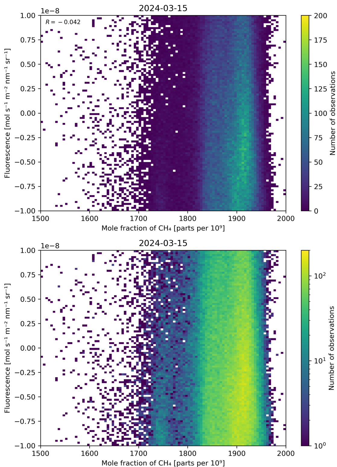
Figure 73: Scatter density plot of “Mole fraction of \text{CH}_4 ” against “Fluorescence” for 2024-03-14 to 2024-03-16.
