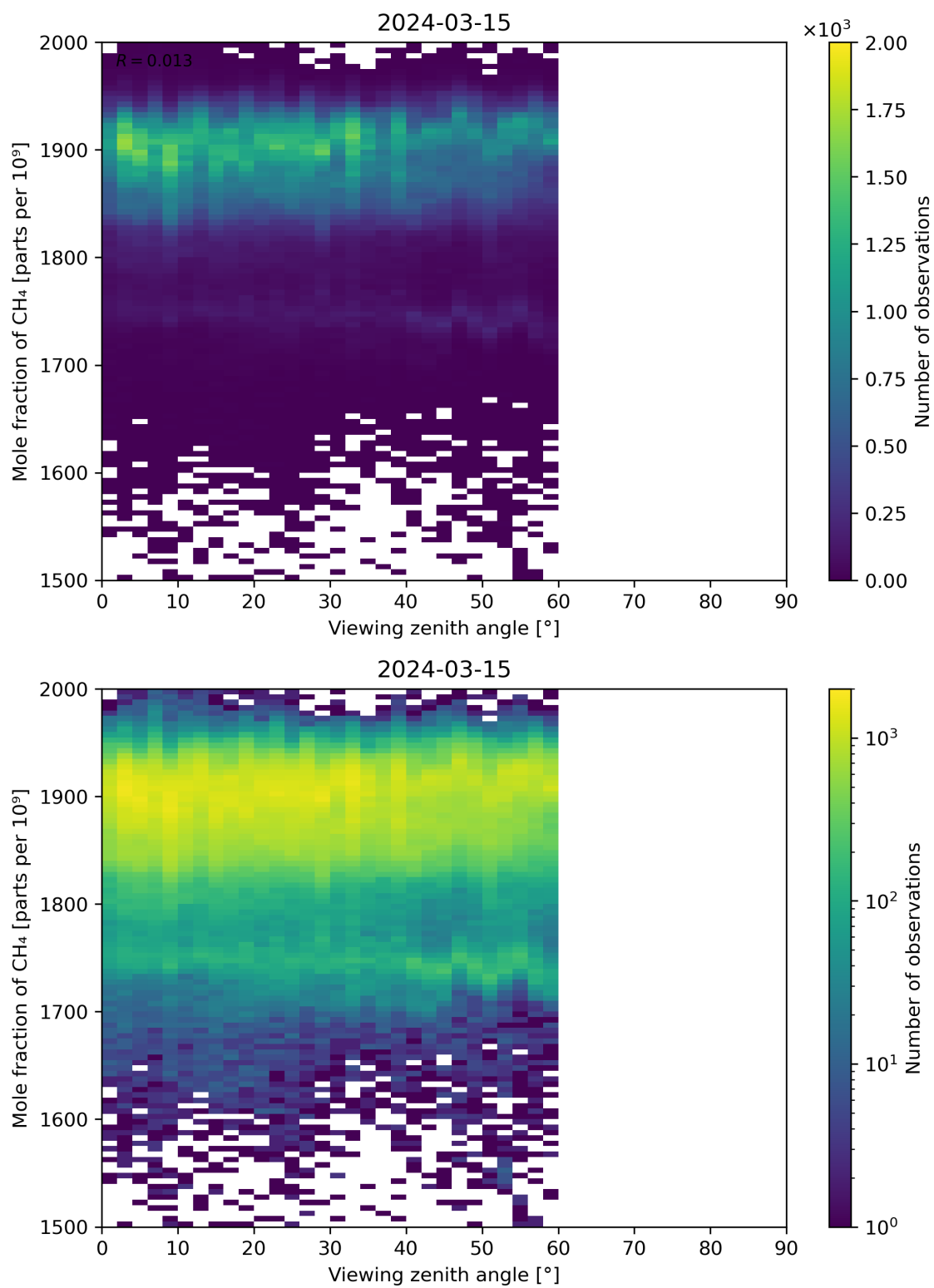
Figure 110: Scatter density plot of “Viewing zenith angle” against “Mole fraction of CH 4 ” for 2024-03-14 to 2024-03-16.
