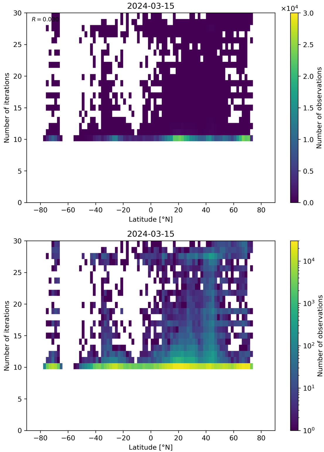
Figure 60: Scatter density plot of “Latitude” against “Number of iterations” for 2024-03-14 to 2024-03-16.
