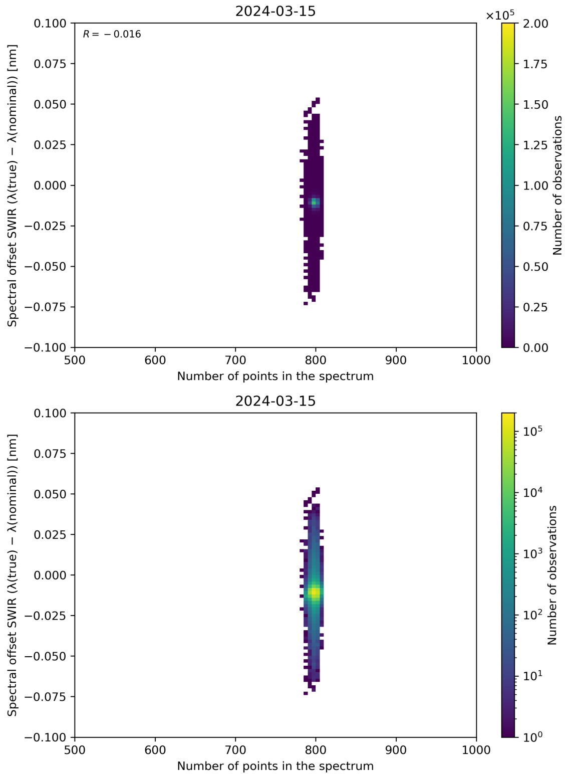
Figure 93: Scatter density plot of “Number of points in the spectrum” against “Spectral offset SWIR ( \lambda(\text{true}) - \lambda(\text{nominal}) )” for 2024-03-14 to 2024-03-16.
