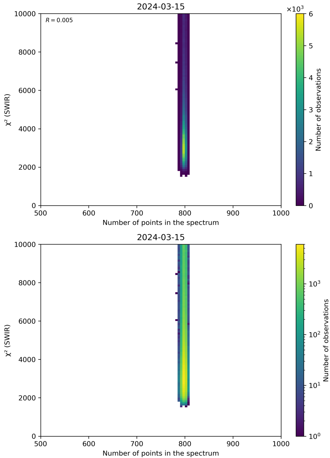
Figure 89: Scatter density plot of “Number of points in the spectrum” against “ \chi^2 (SWIR)” for 2024-03-14 to 2024-03-16.
