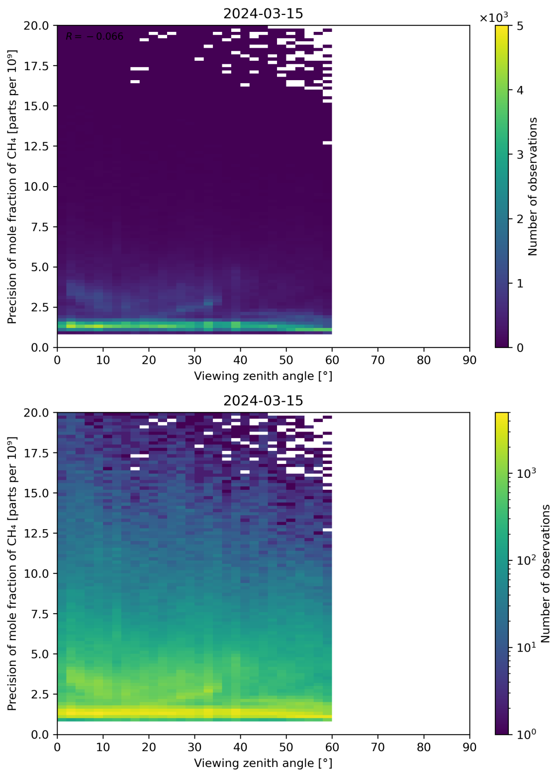
Figure 112: Scatter density plot of “Viewing zenith angle” against “Precision of mole fraction of \text{CH}_4 ” for 2024-03-14 to 2024-03-16.
