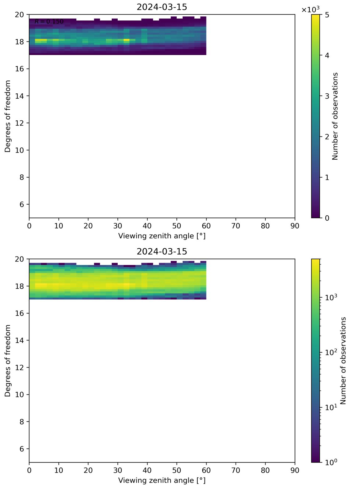
Figure 107: Scatter density plot of “Viewing zenith angle” against “Degrees of freedom” for 2024-03-14 to 2024-03-16.
