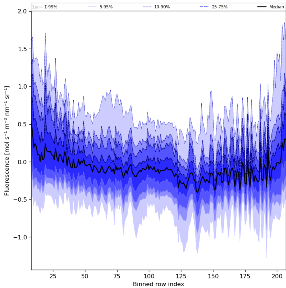
Figure 43: Along track statistics of “Fluorescence” for 2024-03-14 to 2024-03-16
