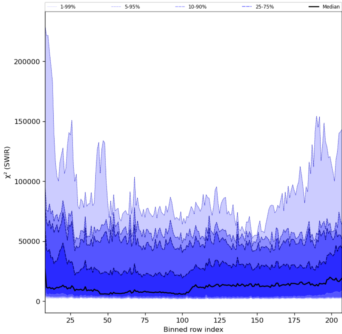
Figure 39: Along track statistics of “ \chi^2 (SWIR)” for 2024-03-14 to 2024-03-16
