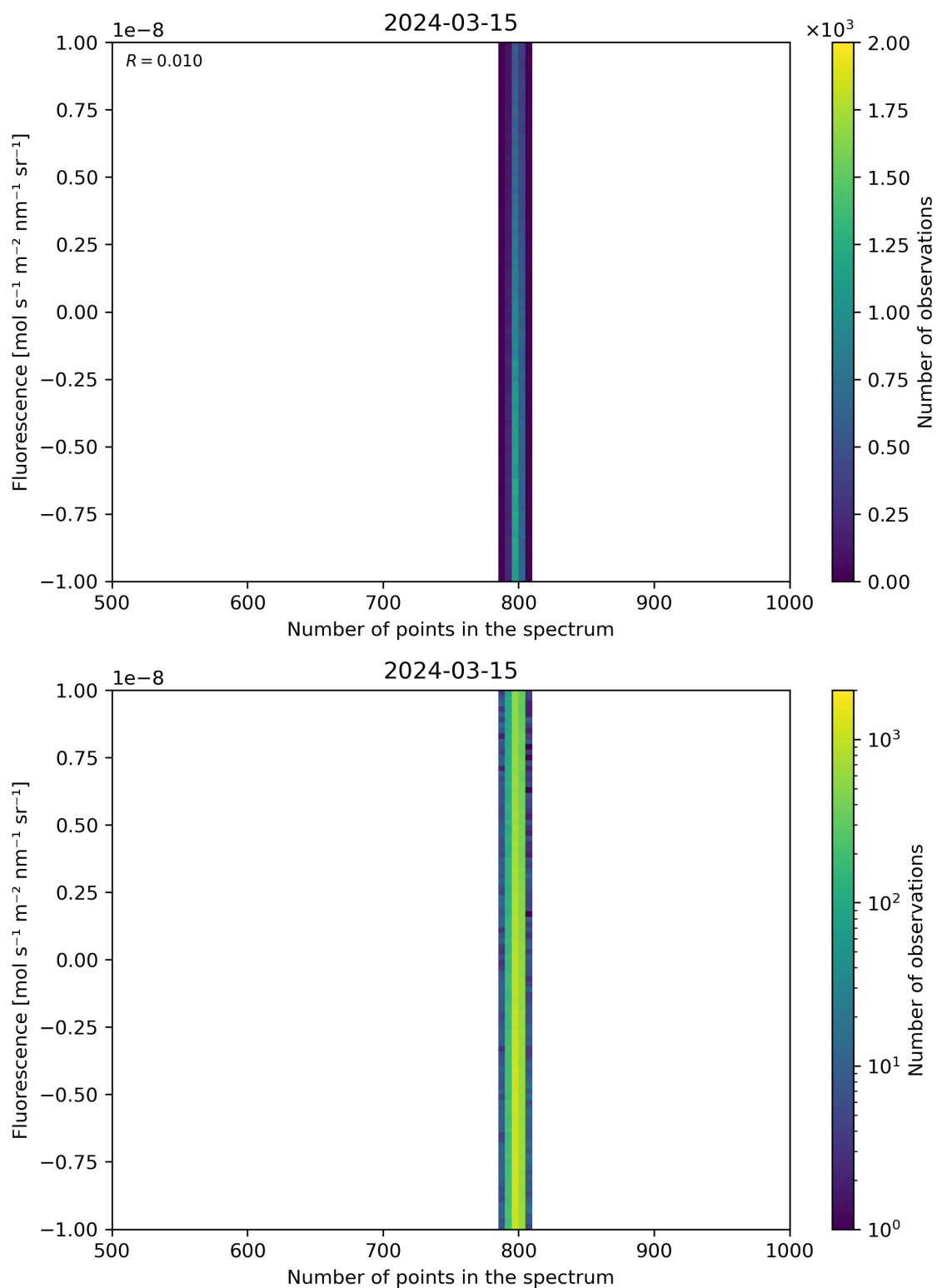
Figure 91: Scatter density plot of “Number of points in the spectrum” against “Fluorescence” for 2024-03-14 to 2024-03-16.
