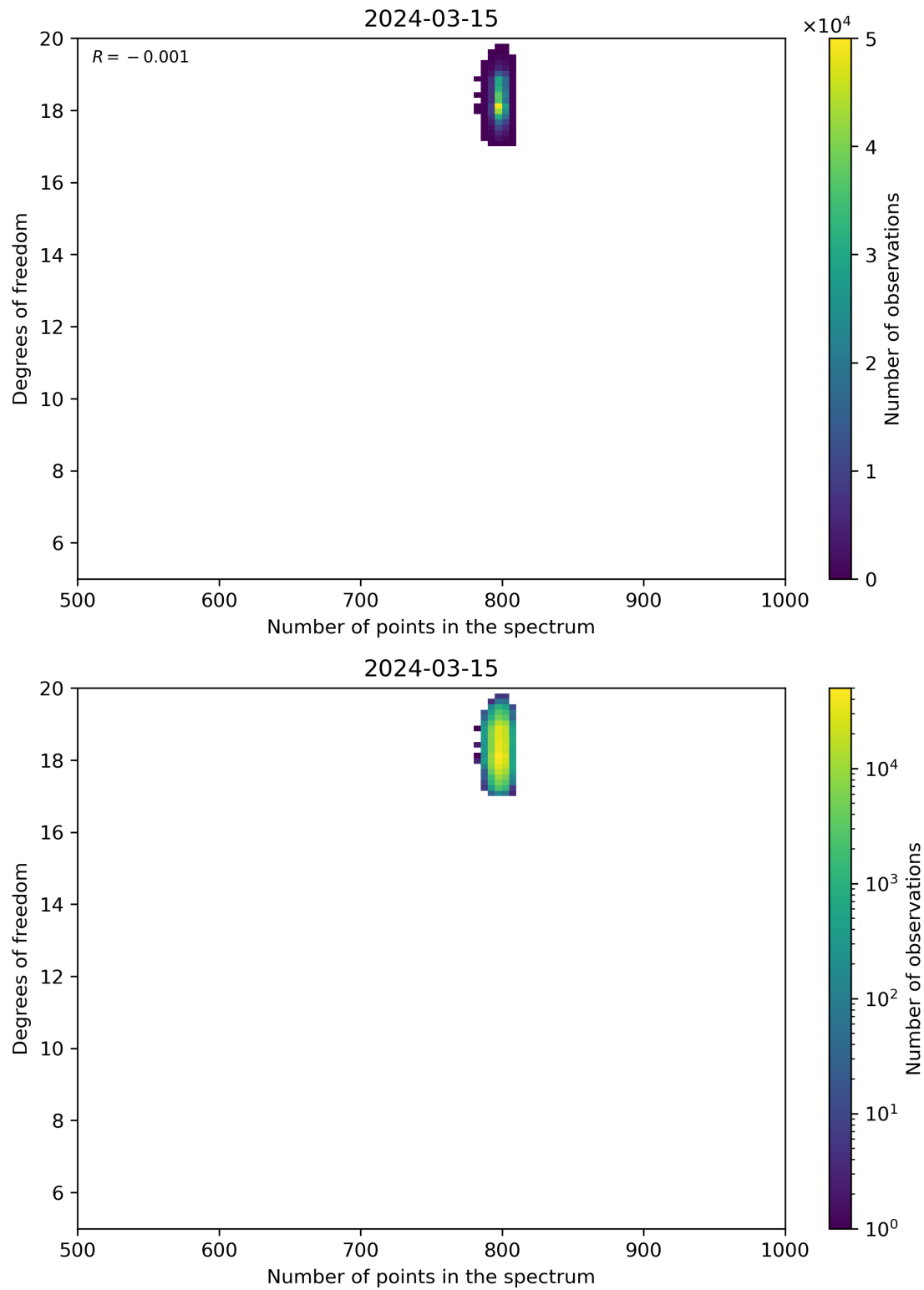
Figure 90: Scatter density plot of “Number of points in the spectrum” against “Degrees of freedom” for 2024-03-14 to 2024-03-16.
