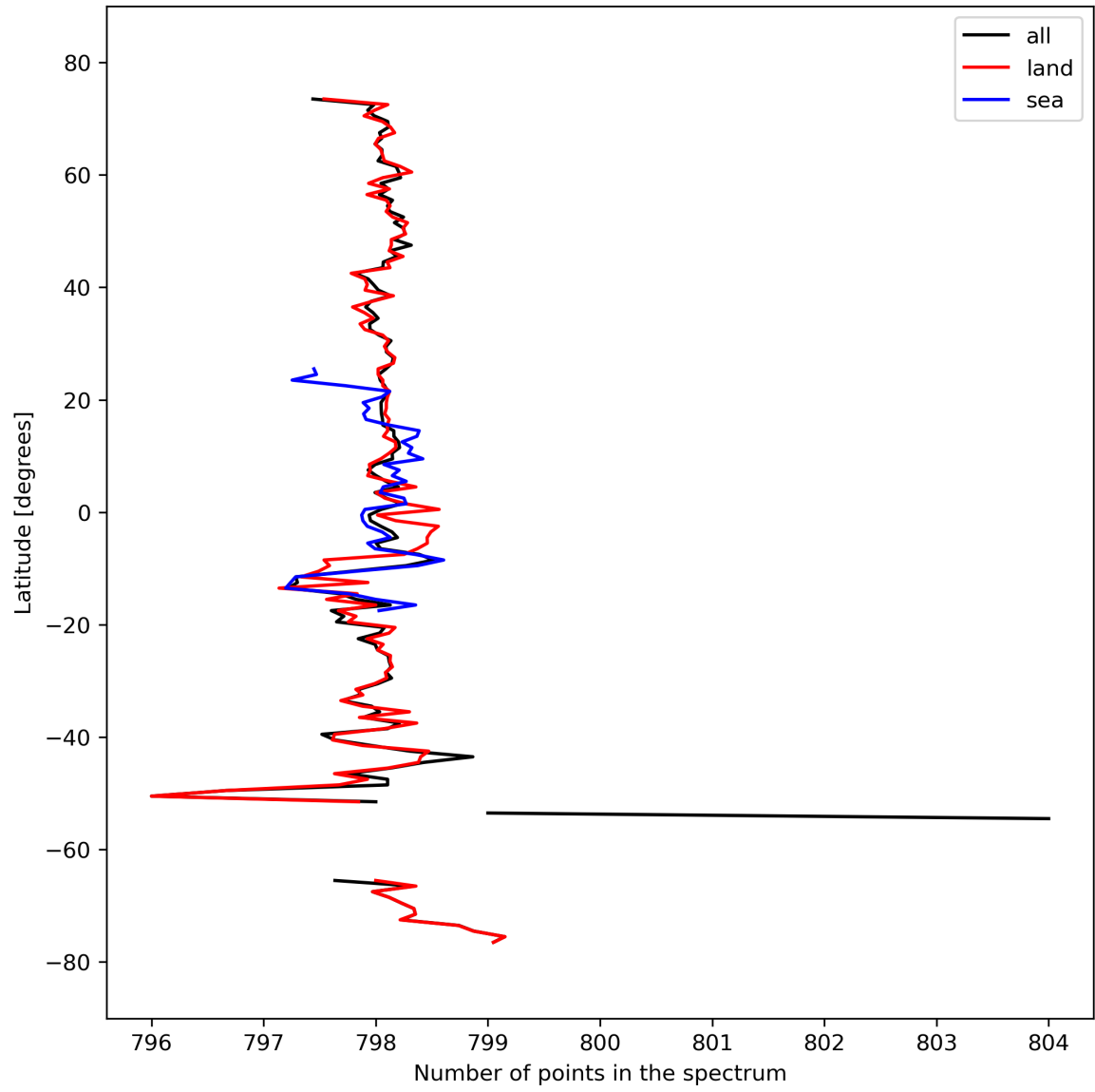
Figure 15: Zonal average of “Number of points in the spectrum” for 2024-03-14 to 2024-03-16.
