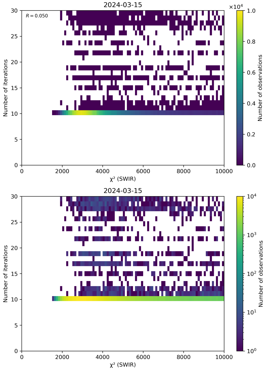
Figure 50: Scatter density plot of “ \chi^2 (SWIR)” against “Number of iterations” for 2024-03-14 to 2024-03-16.
