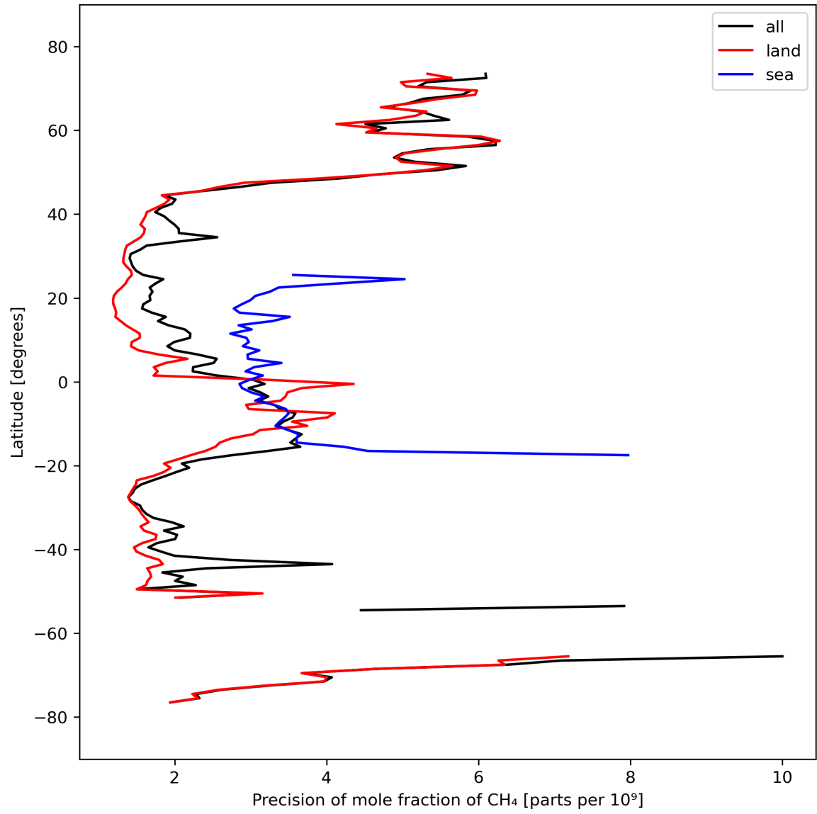
Figure 13: Zonal average of “Precision of mole fraction of CH 4 ” for 2024-03-14 to 2024-03-16.
