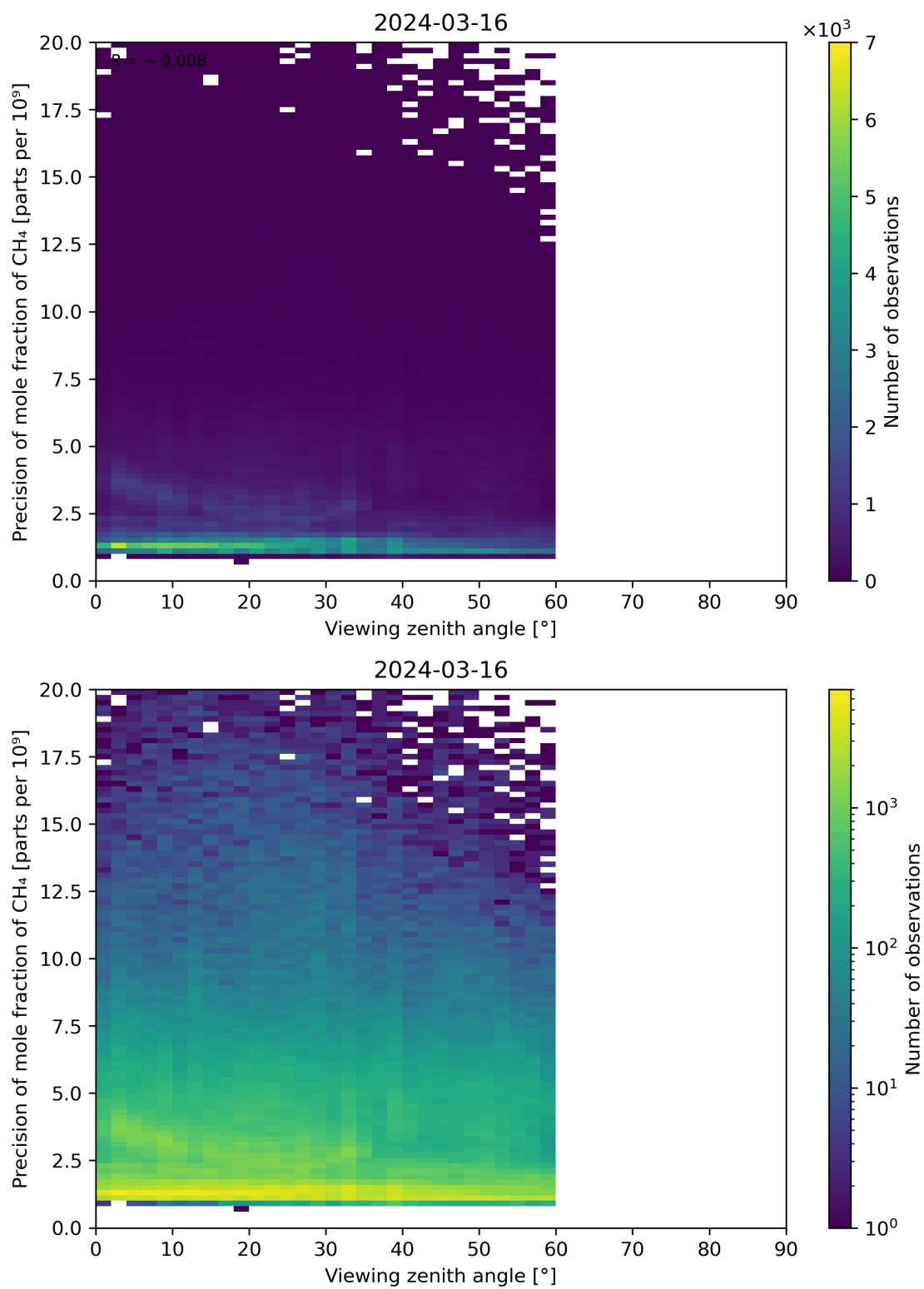
Figure 112: Scatter density plot of “Viewing zenith angle” against “Precision of mole fraction of CH 4 ” for 2024-03-15 to 2024-03-17.
