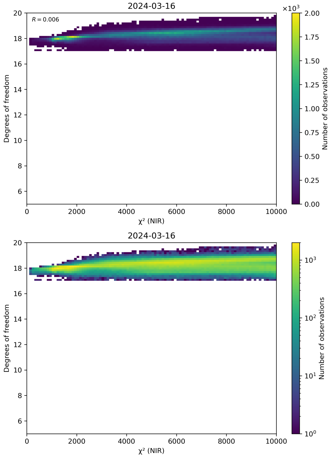
Figure 44: Scatter density plot of “ \chi^2 (NIR)” against “Degrees of freedom” for 2024-03-15 to 2024-03-17.
