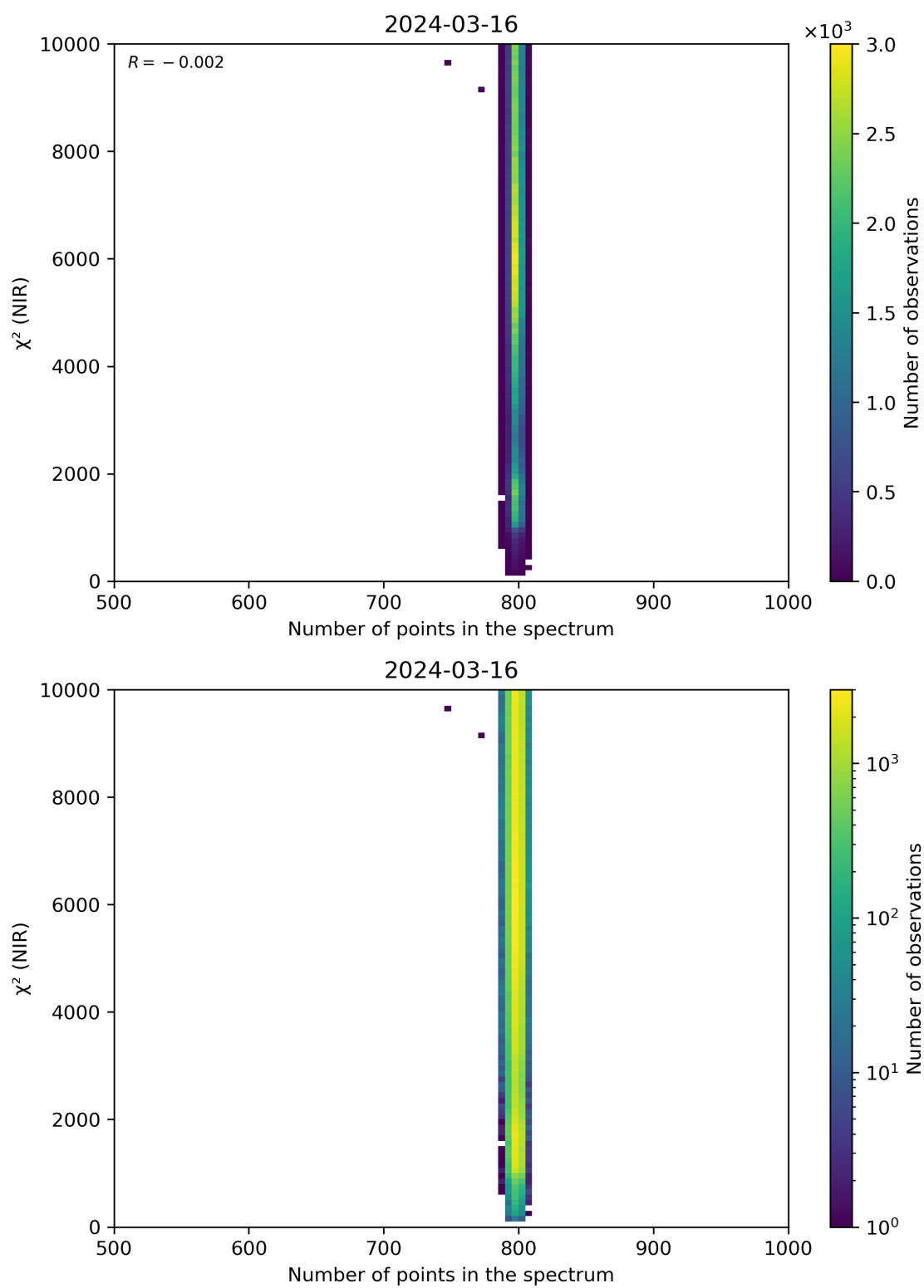
Figure 88: Scatter density plot of “Number of points in the spectrum” against “ \chi^2 (NIR)” for 2024-03-15 to 2024-03-17.
