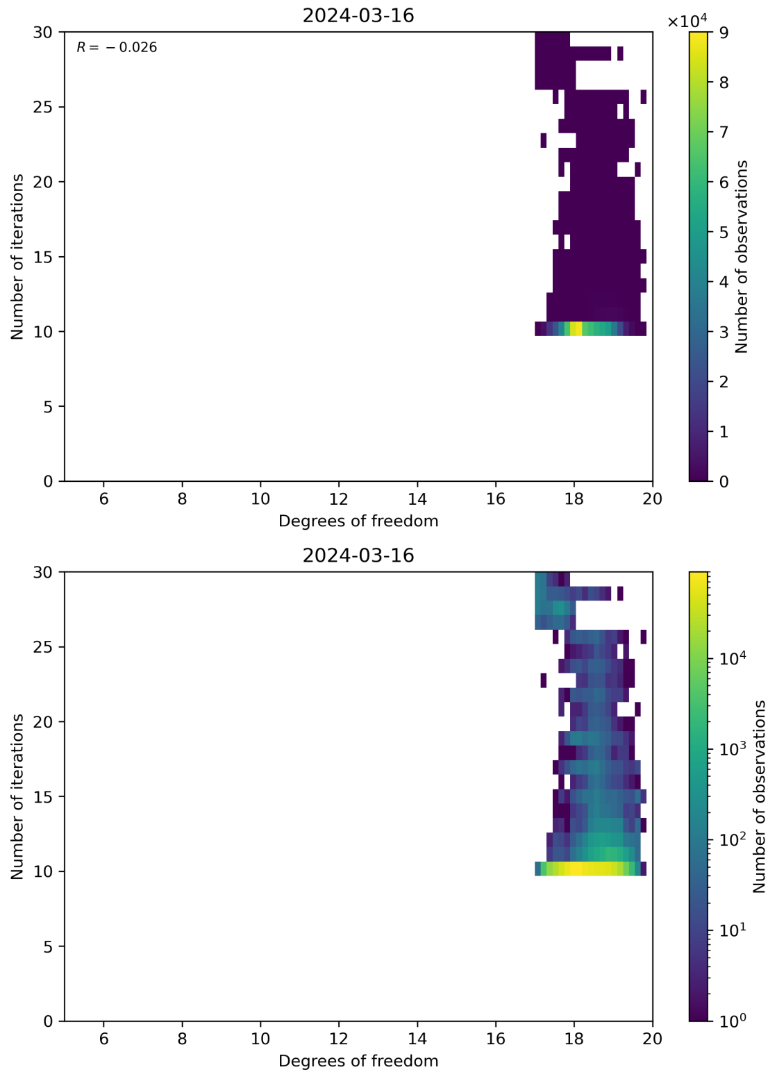
Figure 52: Scatter density plot of “Degrees of freedom” against “Number of iterations” for 2024-03-15 to 2024-03-17.
