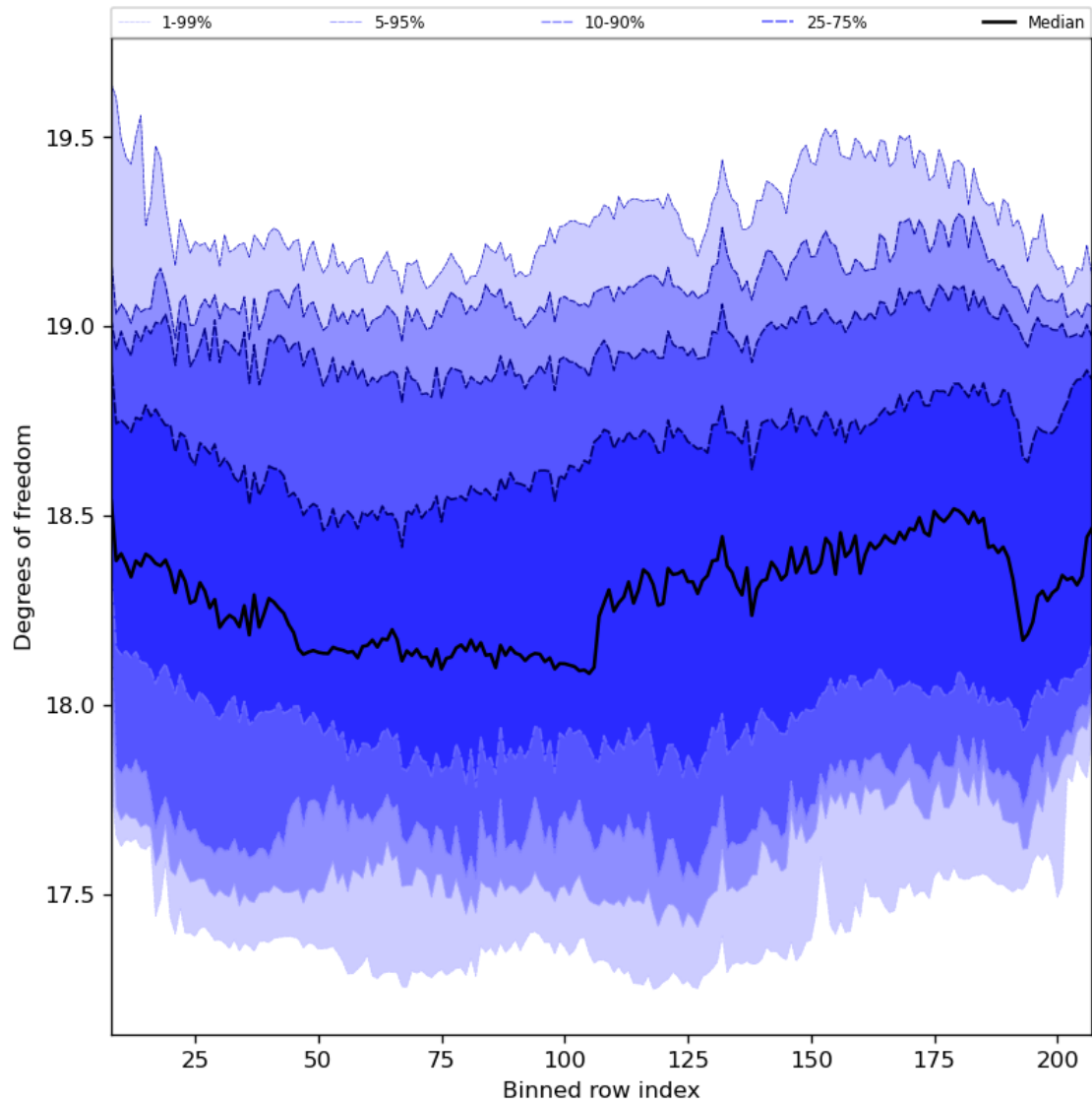
Figure 41: Along track statistics of “Degrees of freedom” for 2024-03-15 to 2024-03-17
