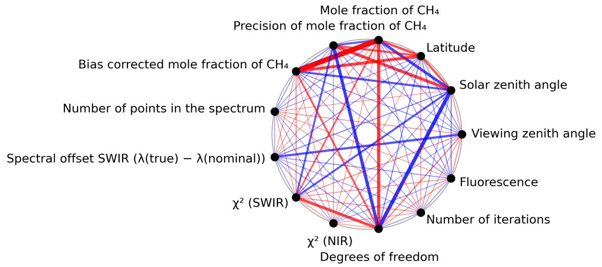
Figure 1: Map of correlation graph for 2024-03-15 to 2024-03-17.
