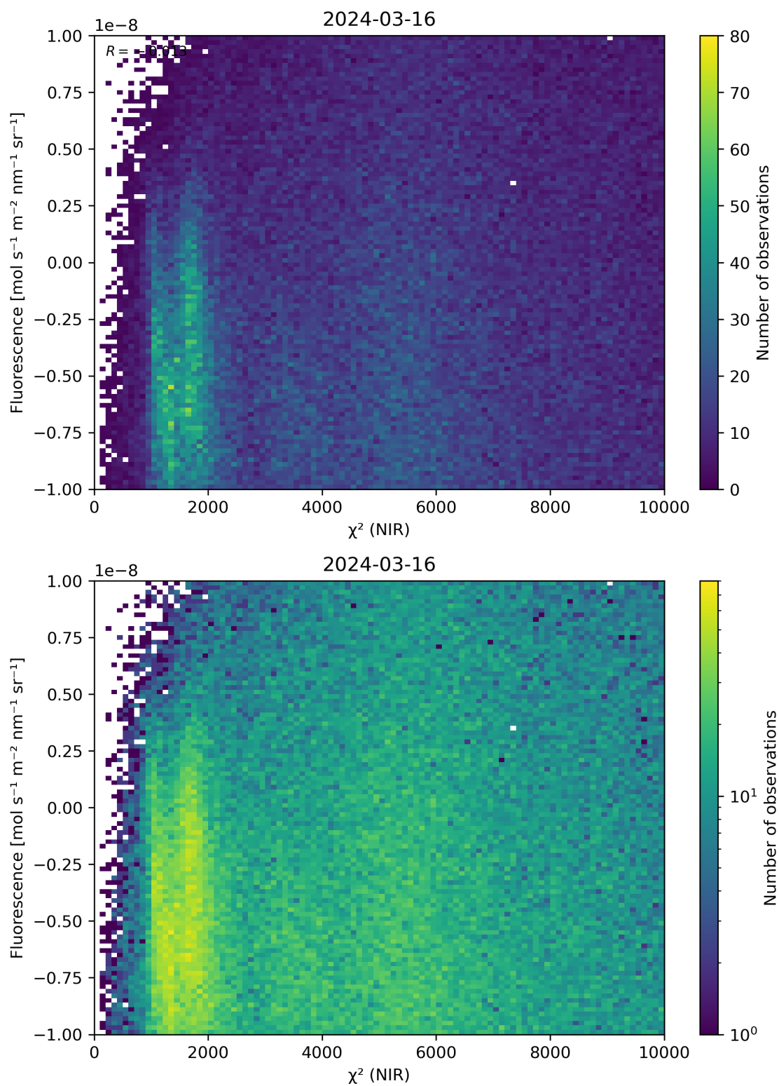
Figure 45: Scatter density plot of “ \chi^2 (NIR)” against “Fluorescence” for 2024-03-15 to 2024-03-17.
