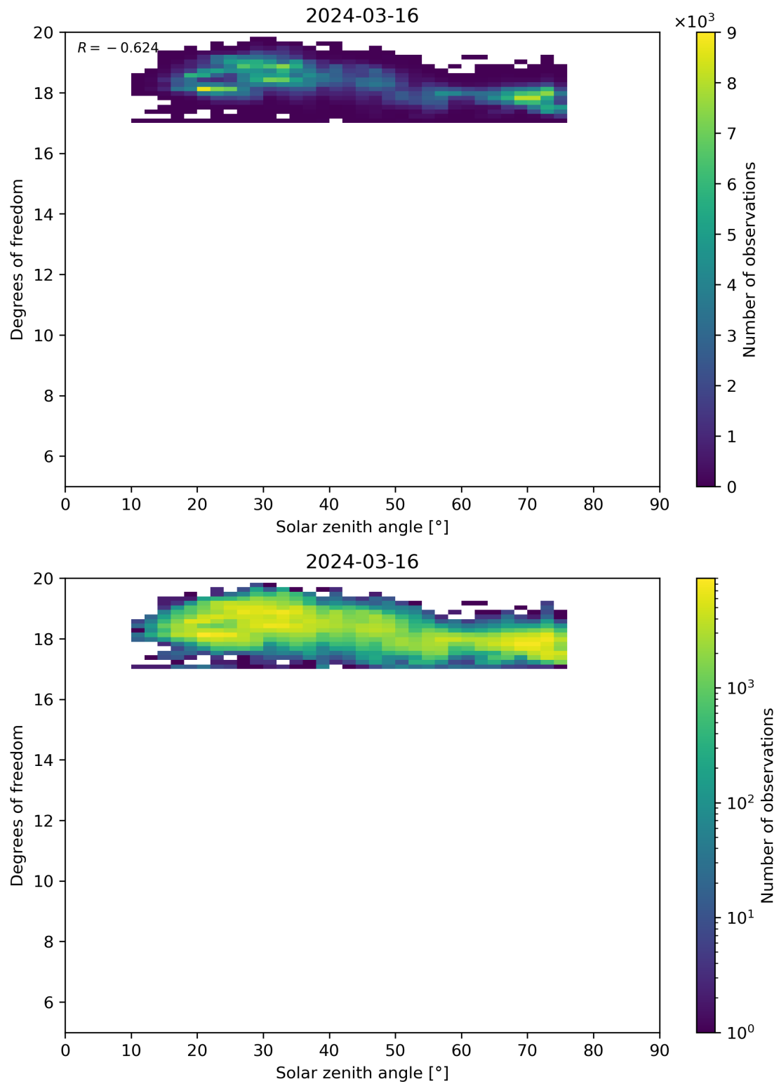
Figure 96: Scatter density plot of “Solar zenith angle” against “Degrees of freedom” for 2024-03-15 to 2024-03-17.
