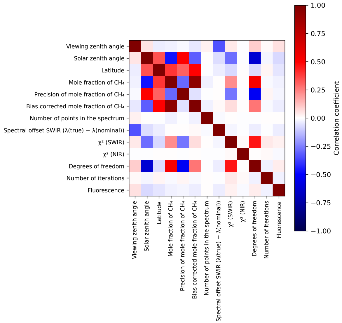
Figure 2: Map of correlation matrix for 2024-03-15 to 2024-03-17.
