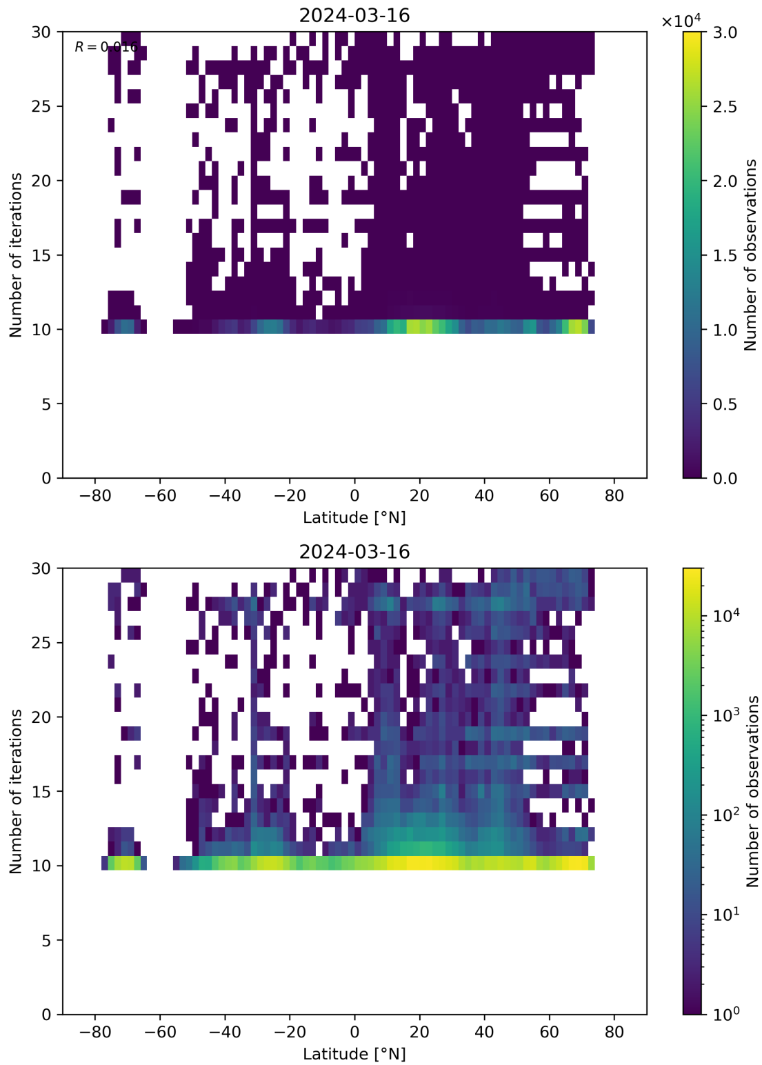
Figure 60: Scatter density plot of “Latitude” against “Number of iterations” for 2024-03-15 to 2024-03-17.
