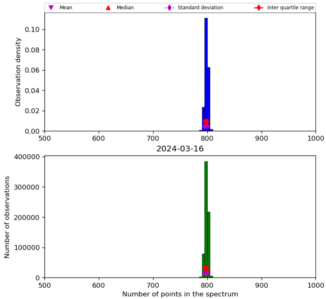
Figure 26: Histogram of “Number of points in the spectrum” for 2024-03-15 to 2024-03-17
