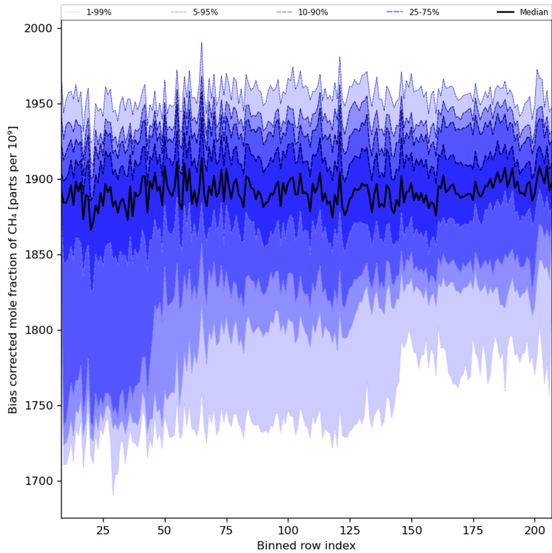
Figure 36: Along track statistics of “Bias corrected mole fraction of CH 4 ” for 2024-03-15 to 2024-03-17
