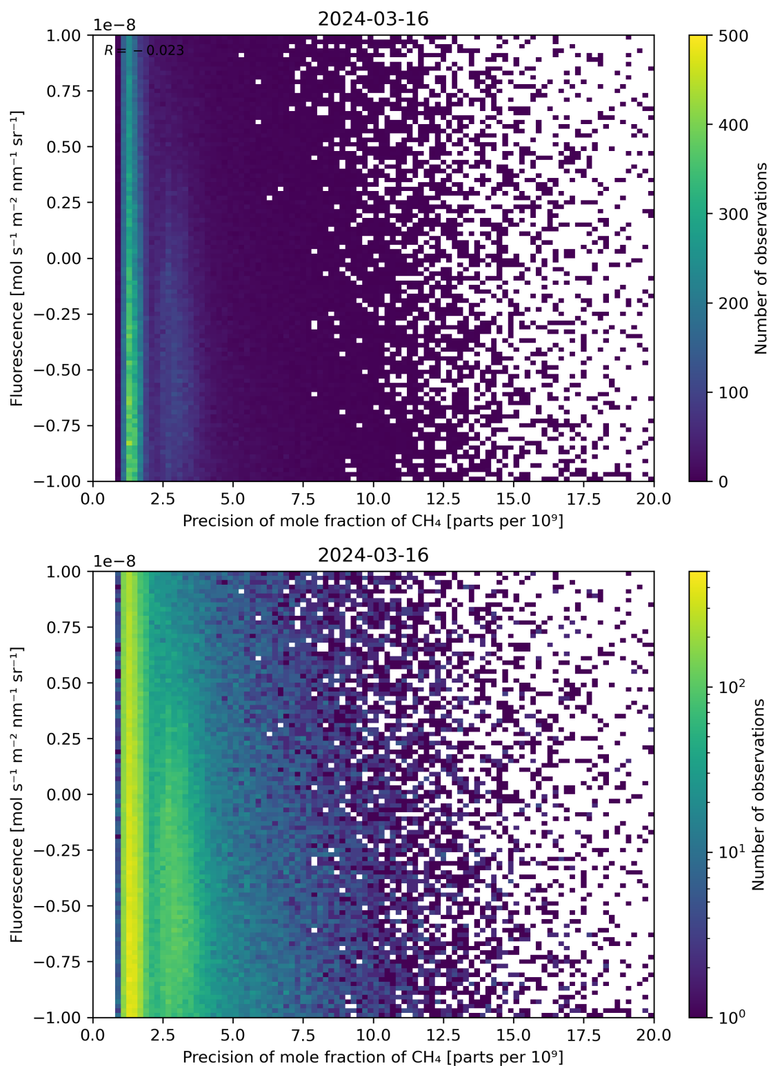
Figure 81: Scatter density plot of “Precision of mole fraction of CH 4 ” against “Fluorescence” for 2024-03-15 to 2024-03-17.
