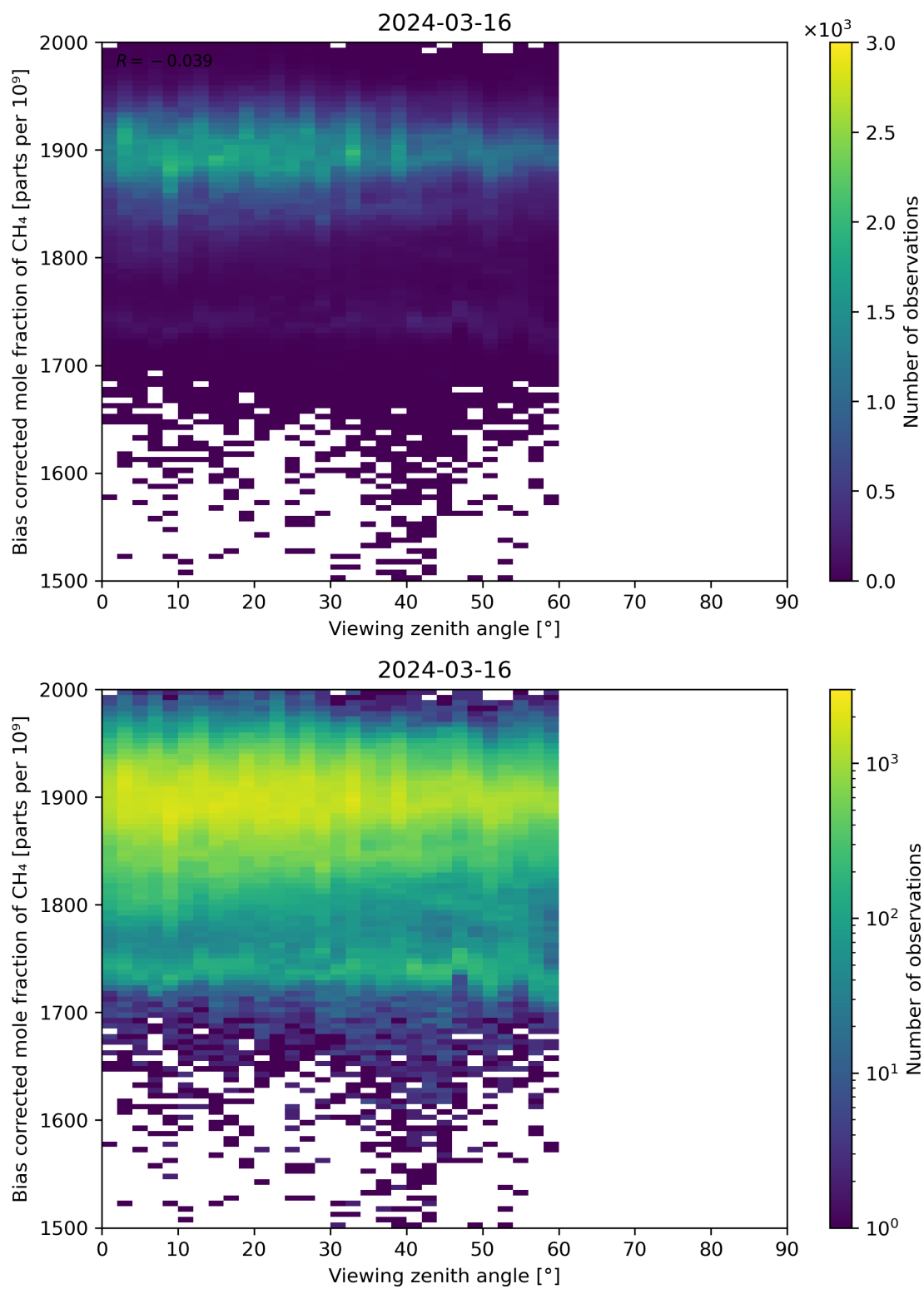
Figure 111: Scatter density plot of “Viewing zenith angle” against “Bias corrected mole fraction of CH 4 ” for 2024-03-15 to 2024-03-17.
