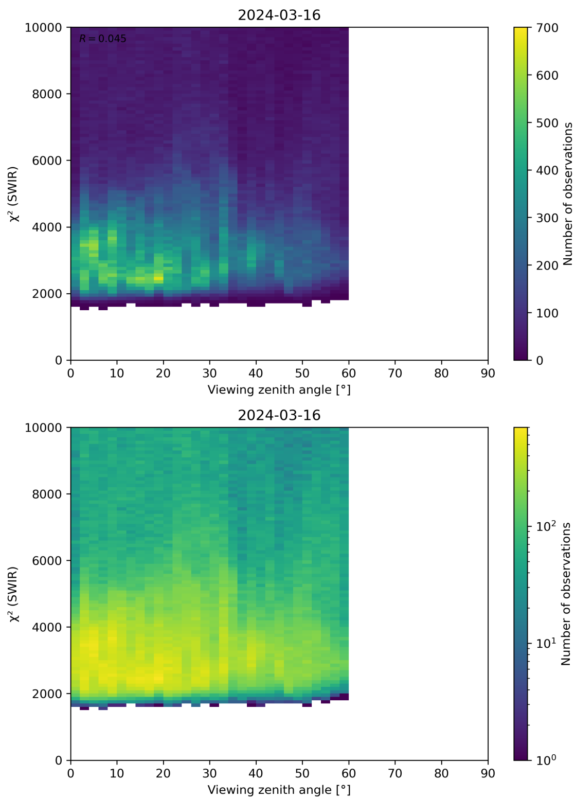
Figure 106: Scatter density plot of “Viewing zenith angle” against “ \chi^2 (SWIR)” for 2024-03-15 to 2024-03-17.
