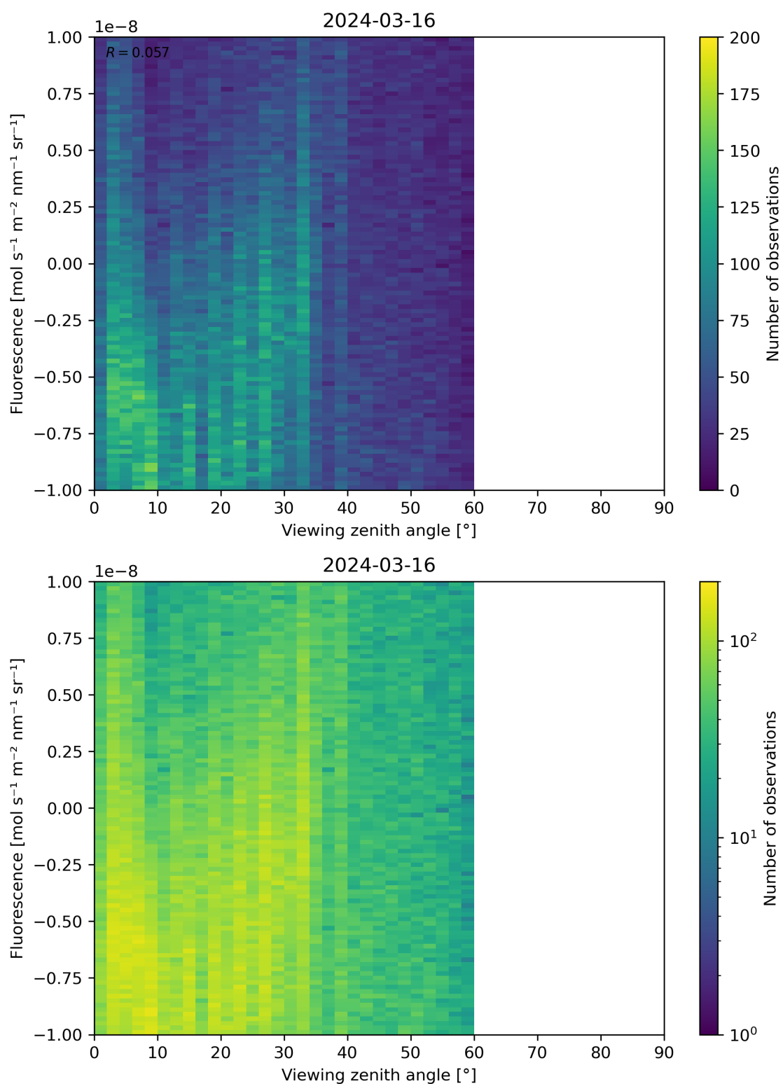
Figure 108: Scatter density plot of “Viewing zenith angle” against “Fluorescence” for 2024-03-15 to 2024-03-17.
