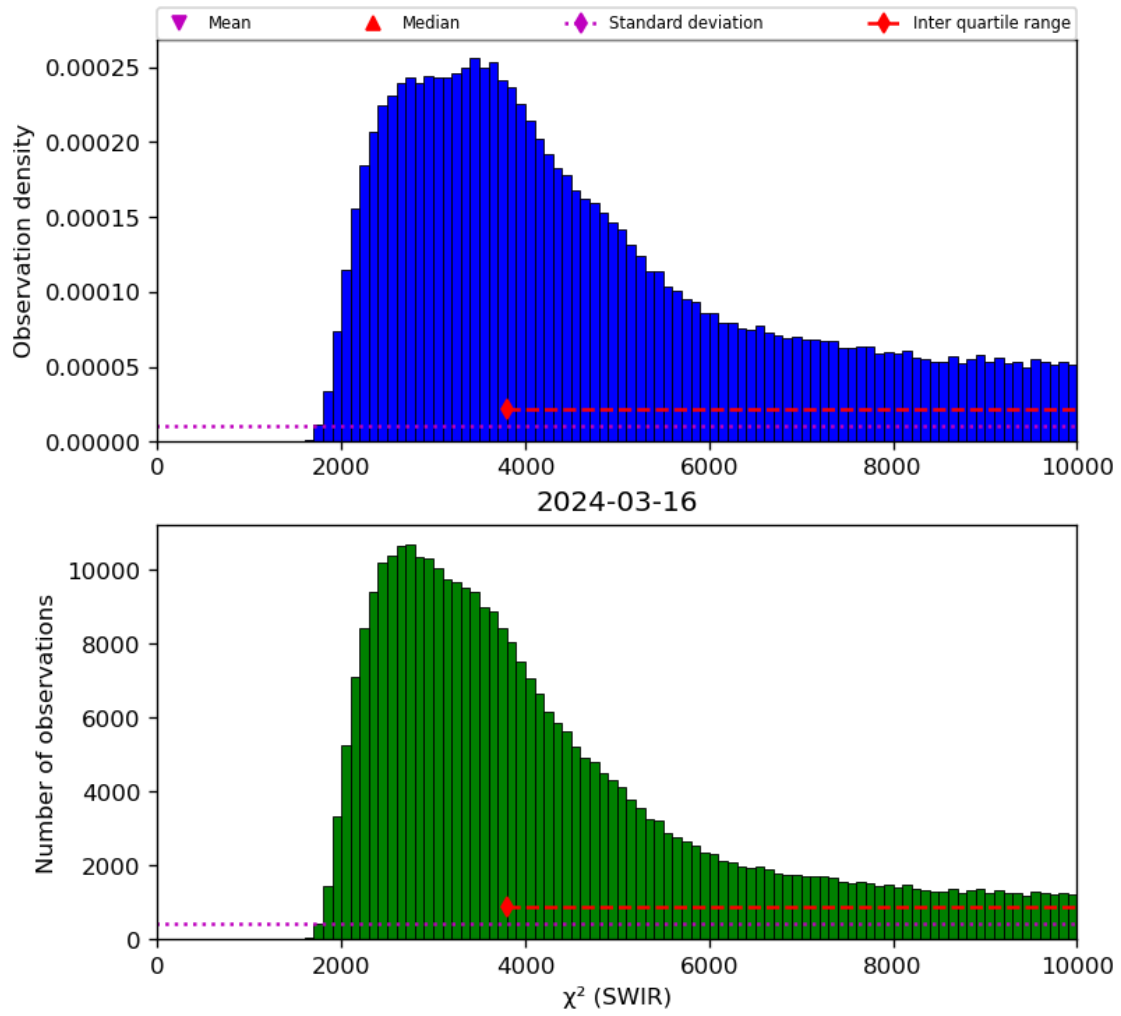
Figure 28: Histogram of “ \chi^2 (SWIR)” for 2024-03-15 to 2024-03-17
