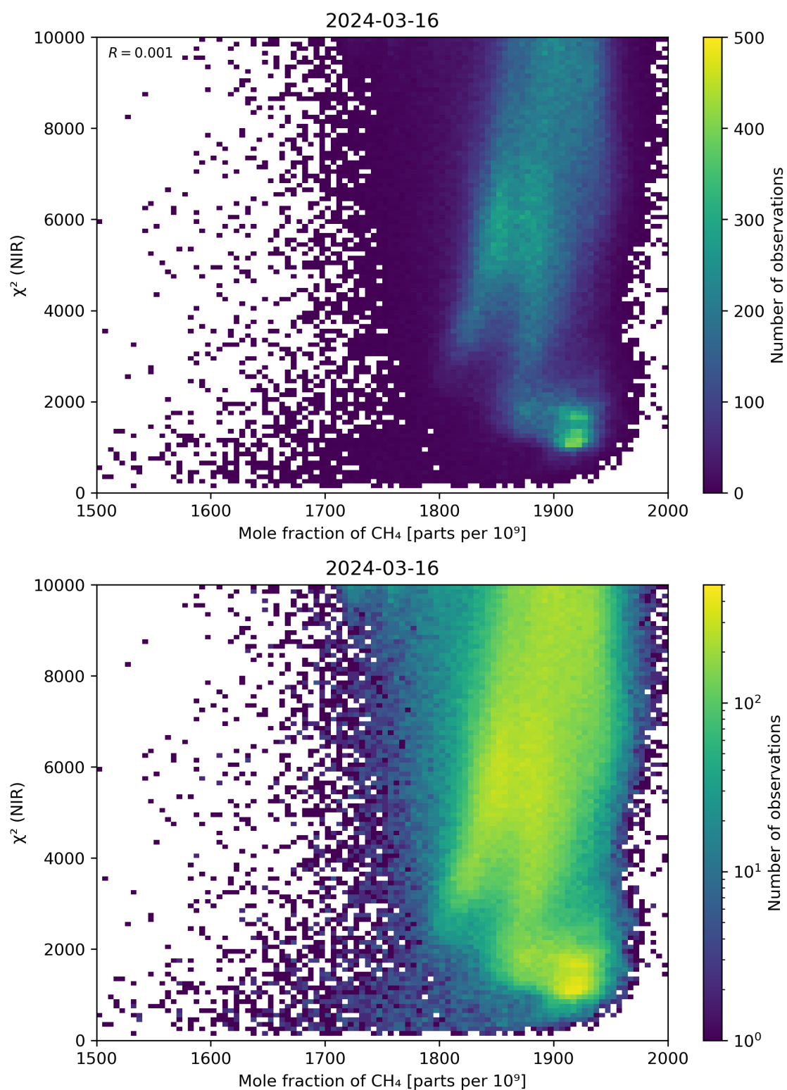
Figure 70: Scatter density plot of “Mole fraction of CH 4 ” against “ \chi^2 (NIR)” for 2024-03-15 to 2024-03-17.
