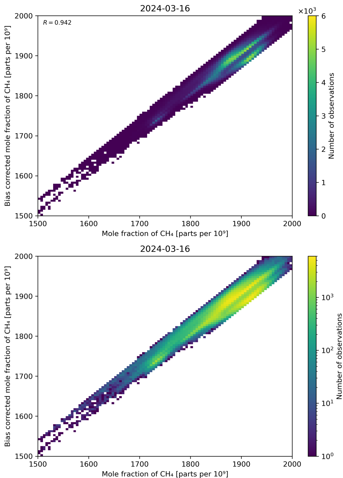
Figure 74: Scatter density plot of “Mole fraction of CH 4 ” against “Bias corrected mole fraction of CH 4 ” for 2024-03-15 to 2024-03-17.
