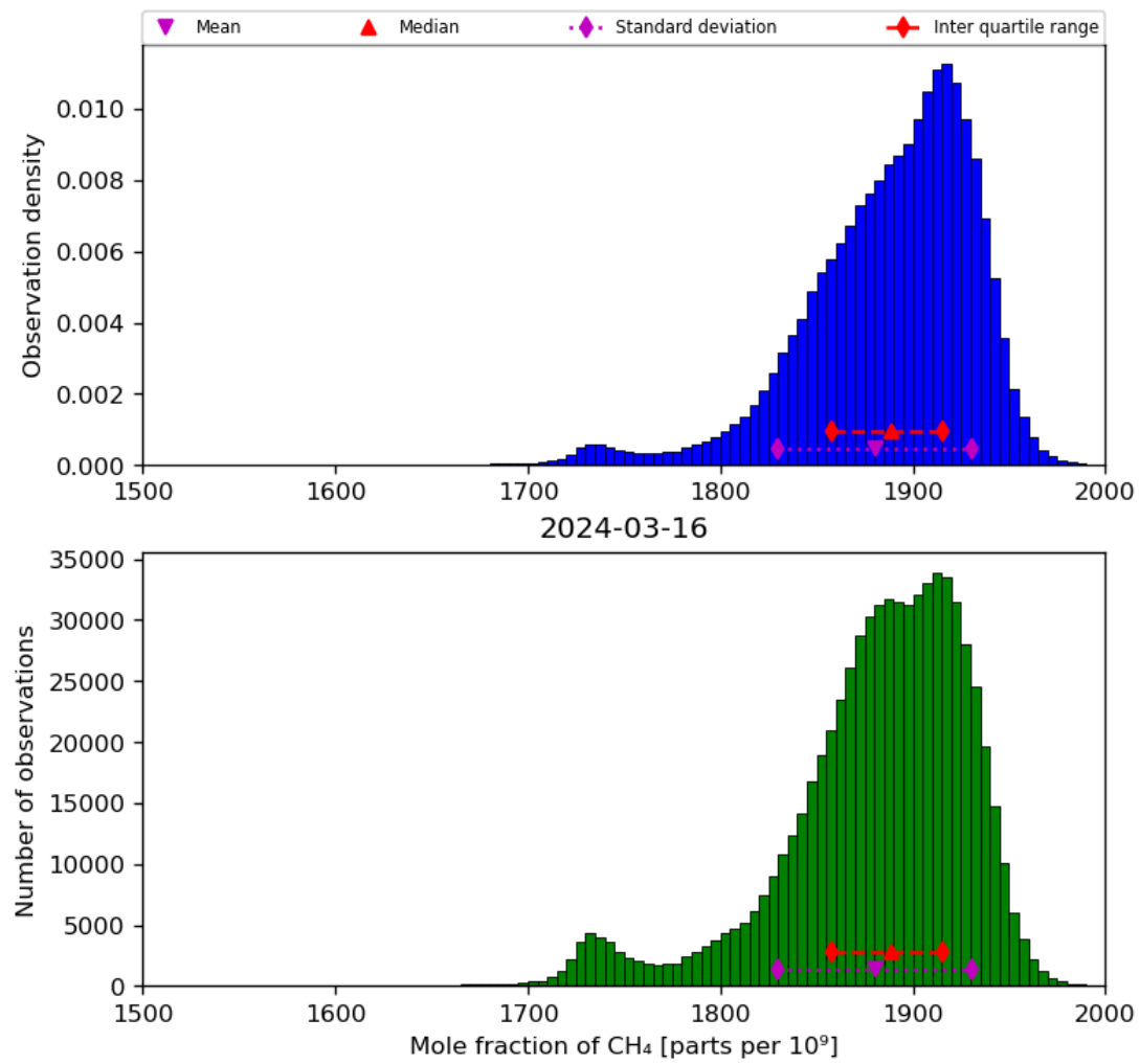
Figure 23: Histogram of “Mole fraction of CH 4 ” for 2024-03-15 to 2024-03-17
