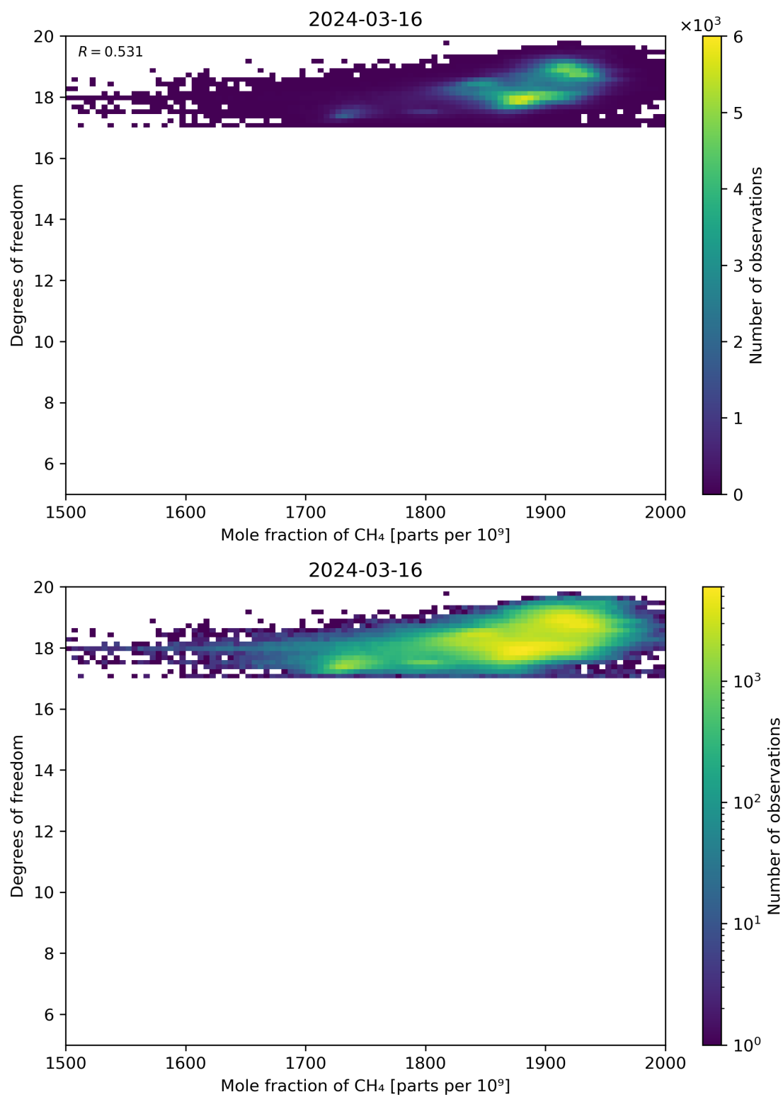
Figure 72: Scatter density plot of “Mole fraction of CH 4 ” against “Degrees of freedom” for 2024-03-15 to 2024-03-17.
