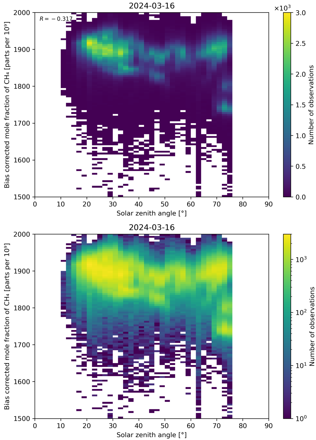
Figure 100: Scatter density plot of “Solar zenith angle” against “Bias corrected mole fraction of \text{CH}_4 ” for 2024-03-15 to 2024-03-17.
