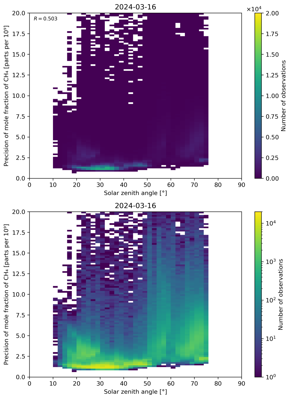
Figure 101: Scatter density plot of “Solar zenith angle” against “Precision of mole fraction of CH 4 ” for 2024-03-15 to 2024-03-17.
