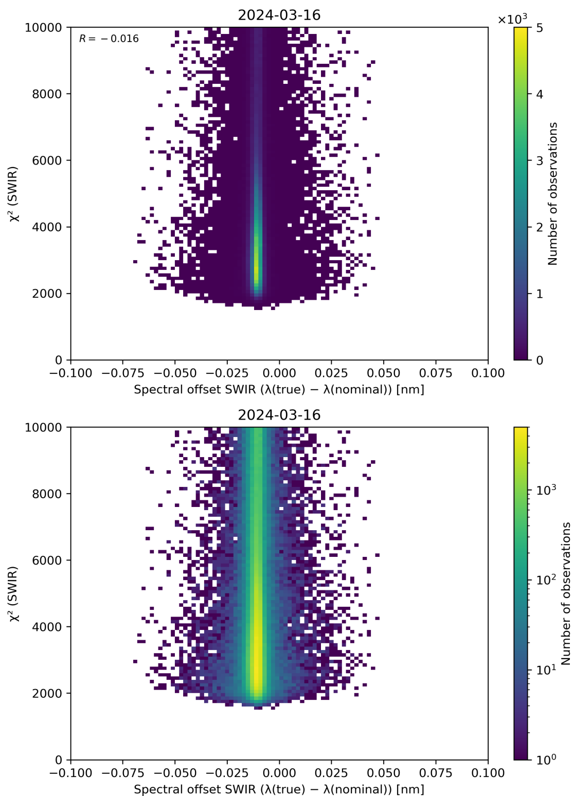
Figure 118: Scatter density plot of “Spectral offset SWIR ( \lambda(\text{true}) - \lambda(\text{nominal}) )” against “ \chi^2 (SWIR)” for 2024-03-15 to 2024-03-17.
