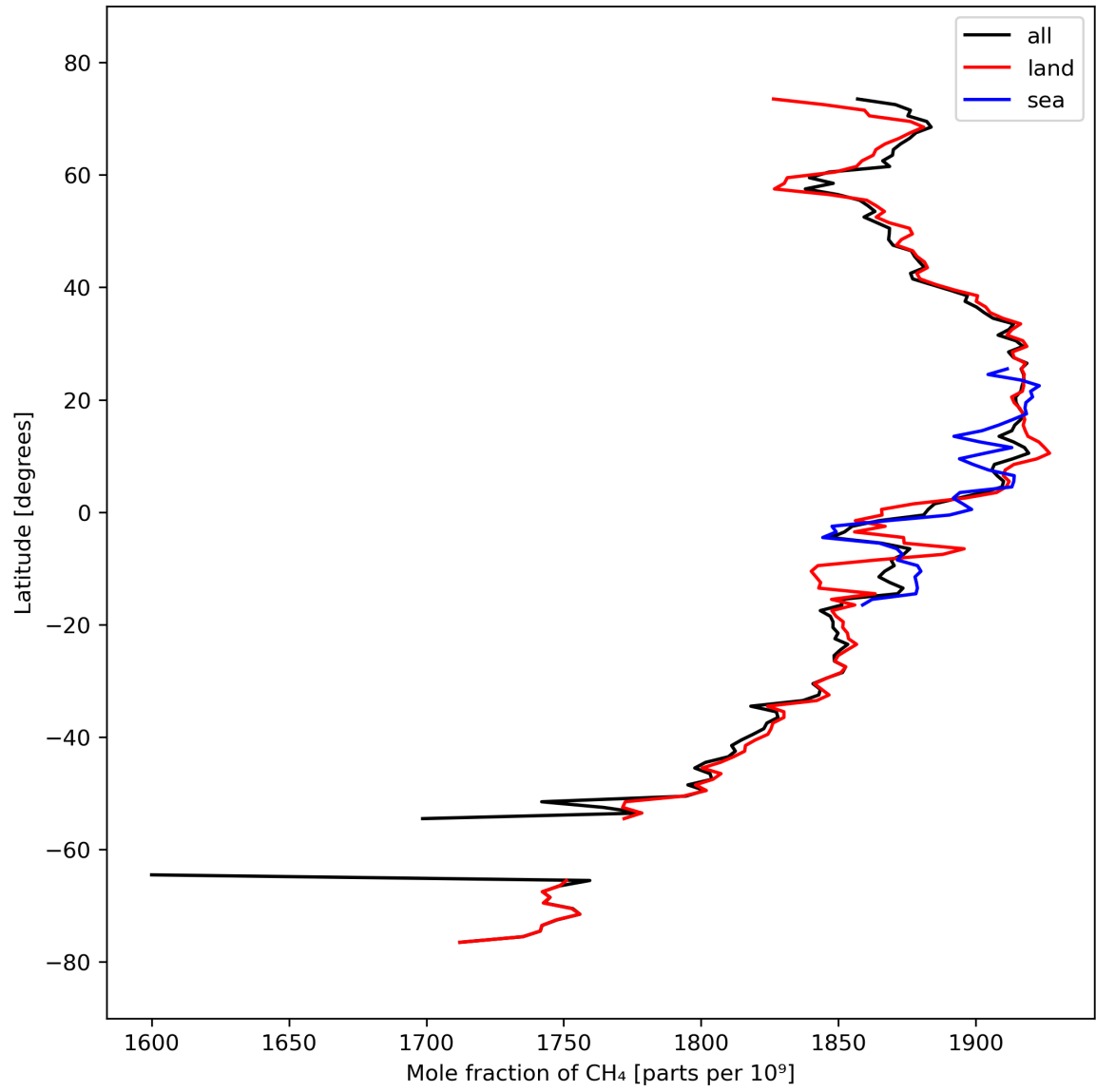
Figure 12: Zonal average of “Mole fraction of \text{CH}_4 ” for 2024-03-15 to 2024-03-17.
