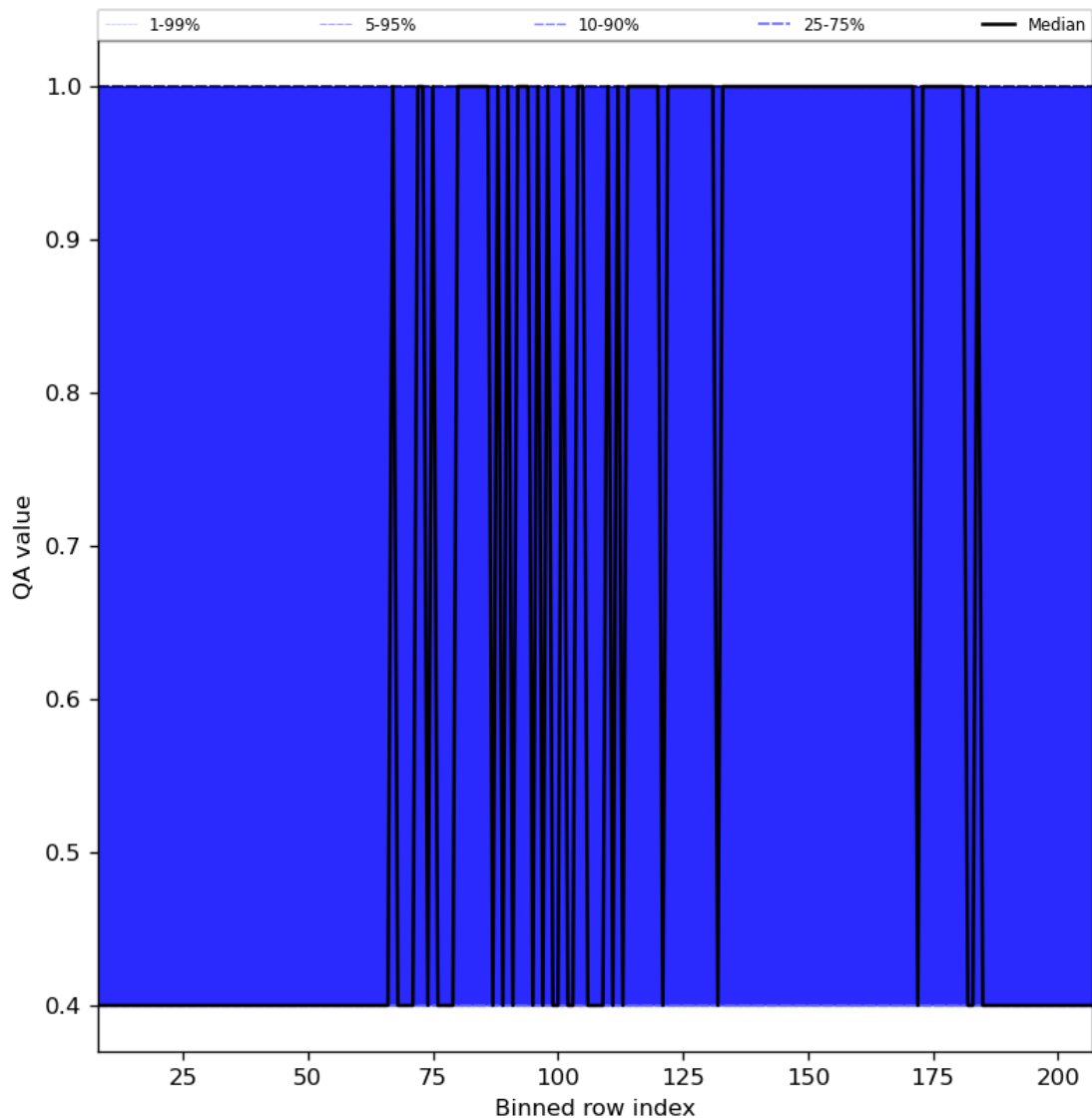
Figure 33: Along track statistics of “QA value” for 2024-03-15 to 2024-03-17
