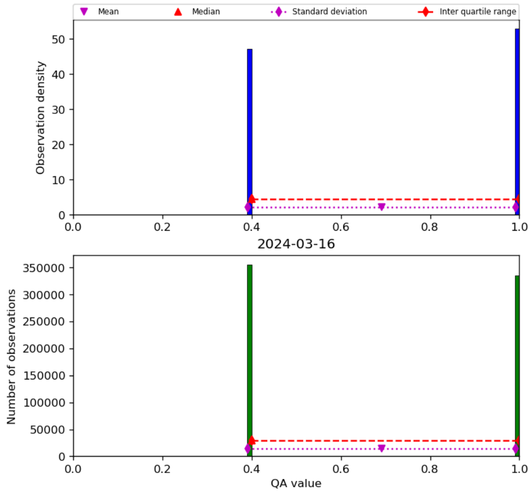
Figure 22: Histogram of “QA value” for 2024-03-15 to 2024-03-17
