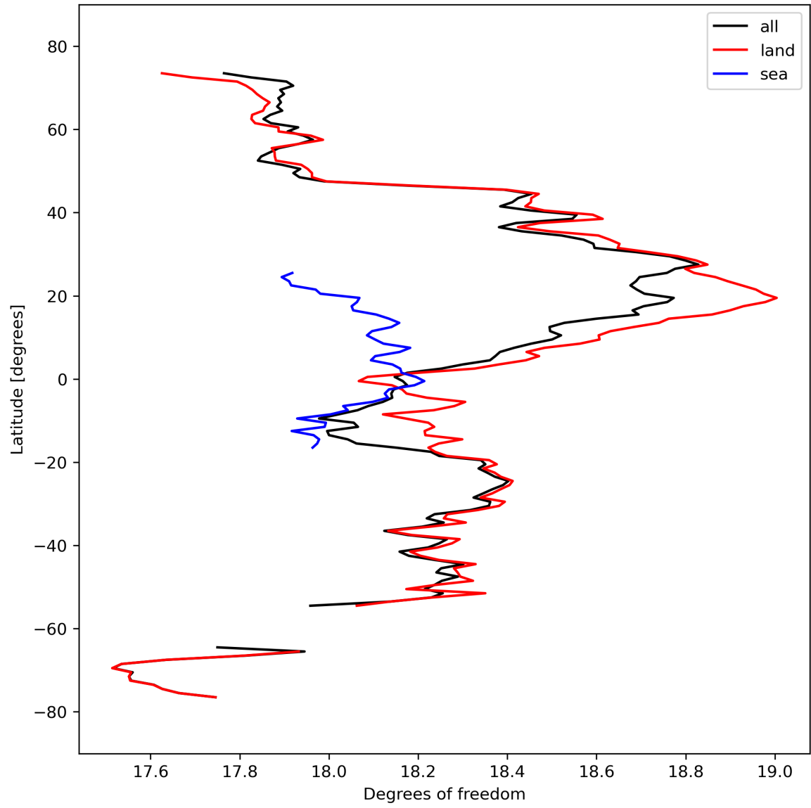
Figure 19: Zonal average of “Degrees of freedom” for 2024-03-15 to 2024-03-17.
