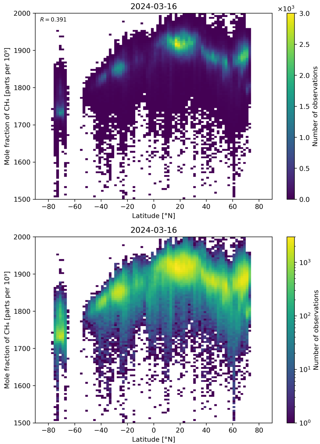
Figure 57: Scatter density plot of “Latitude” against “Mole fraction of CH 4 ” for 2024-03-15 to 2024-03-17.
