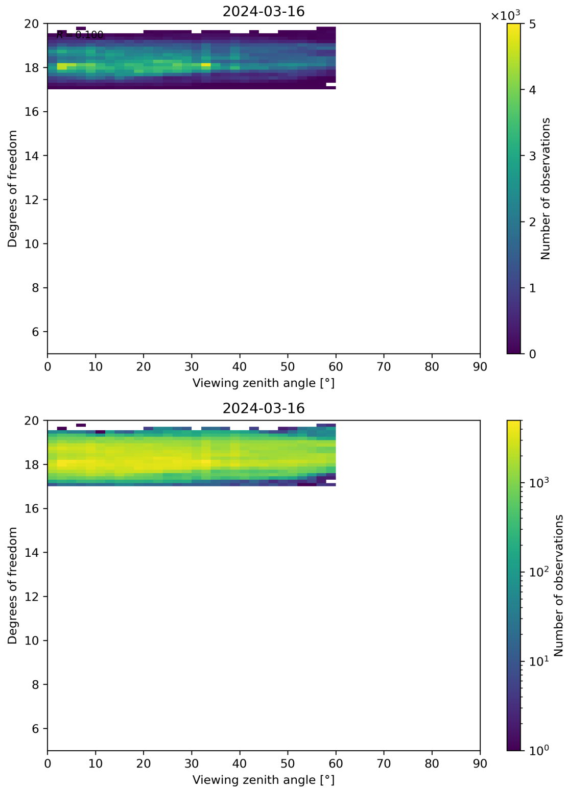
Figure 107: Scatter density plot of “Viewing zenith angle” against “Degrees of freedom” for 2024-03-15 to 2024-03-17.
