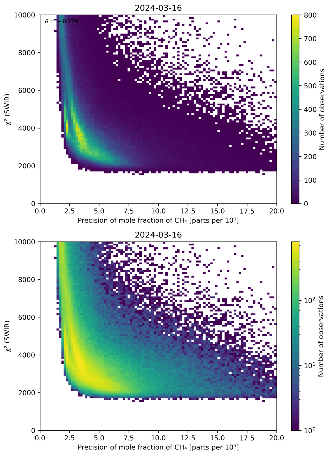
Figure 79: Scatter density plot of “Precision of mole fraction of CH 4 ” against “ \chi^2 (SWIR)” for 2024-03-15 to 2024-03-17.
