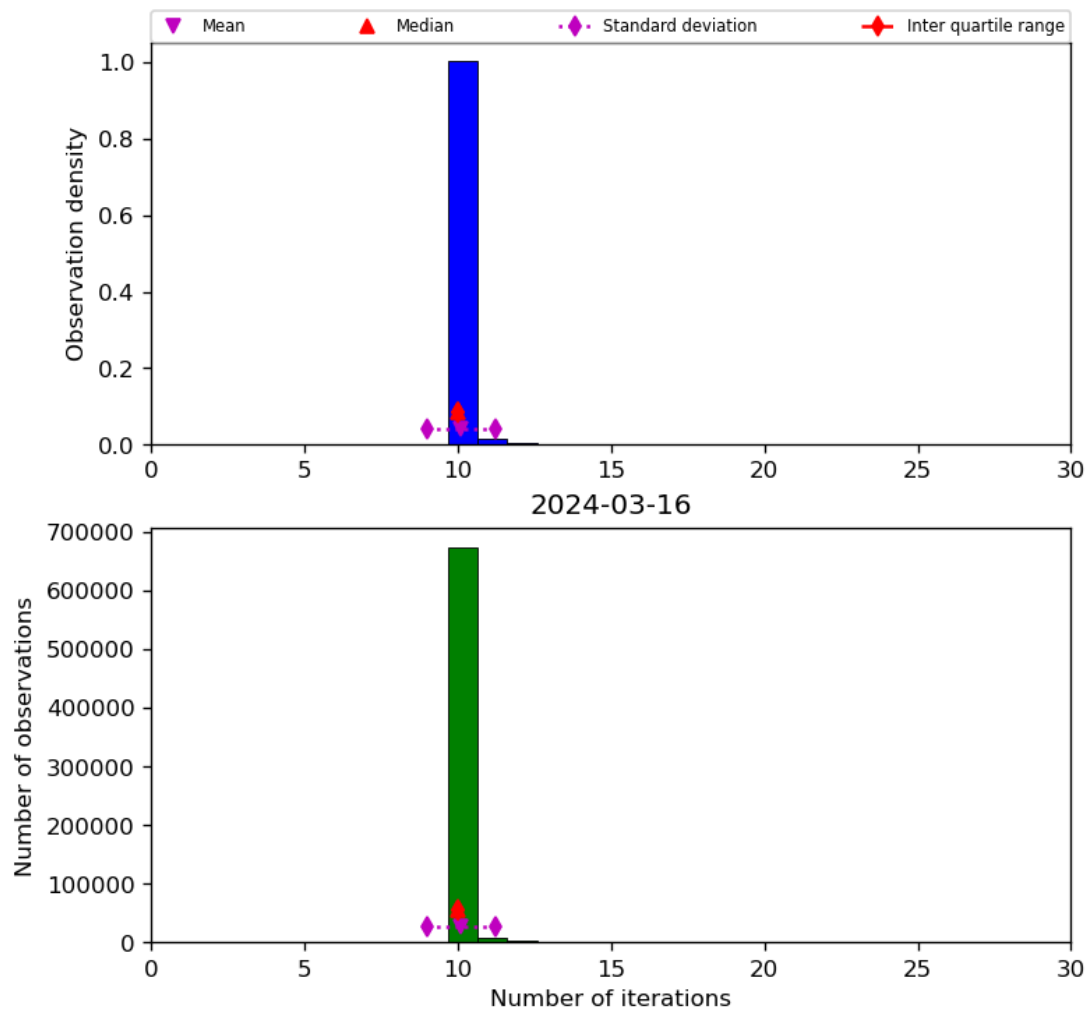
Figure 31: Histogram of “Number of iterations” for 2024-03-15 to 2024-03-17
