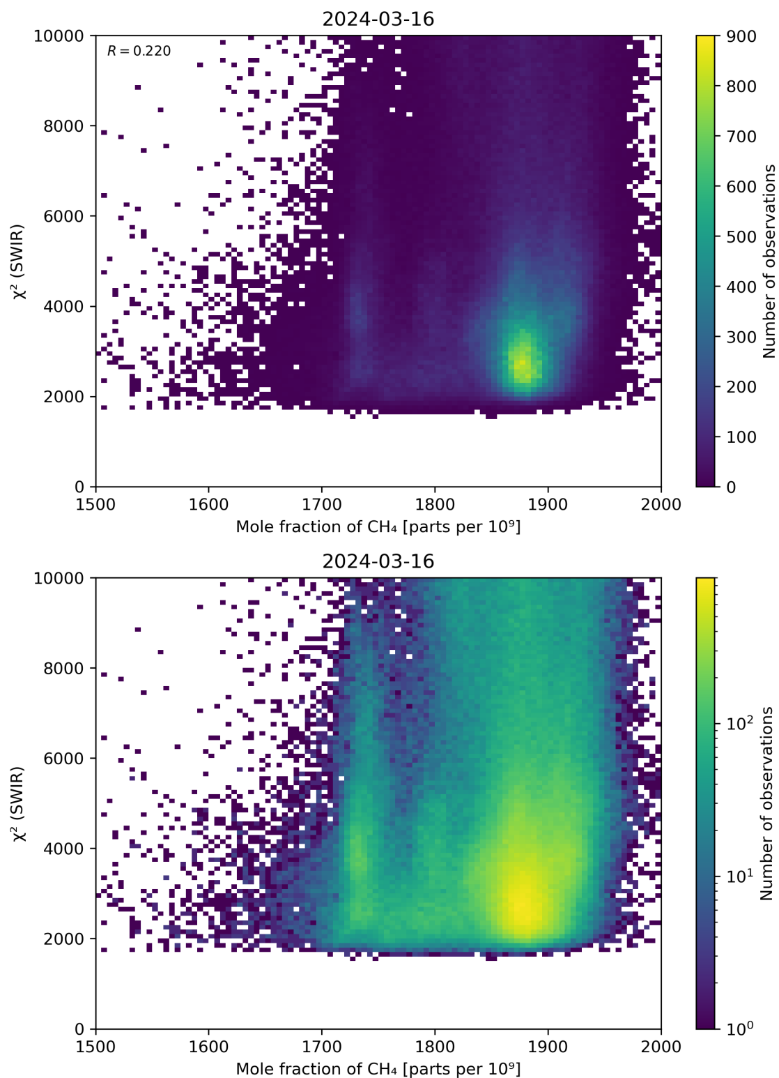
Figure 71: Scatter density plot of “Mole fraction of \text{CH}_4 ” against “ \chi^2 (SWIR)” for 2024-03-15 to 2024-03-17.
