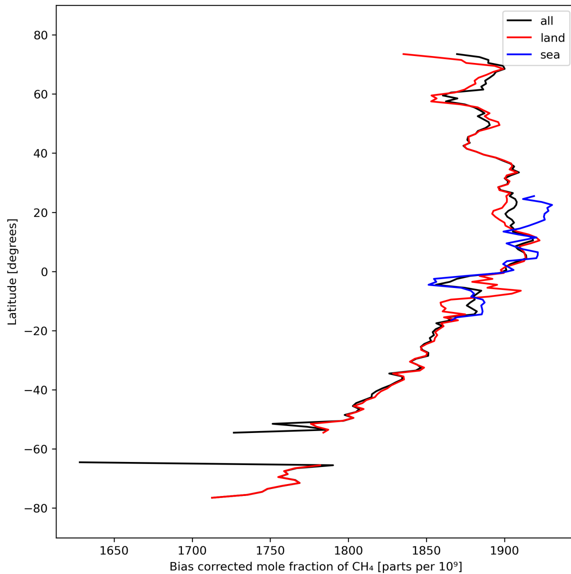
Figure 14: Zonal average of “Bias corrected mole fraction of CH 4 ” for 2024-03-15 to 2024-03-17.
