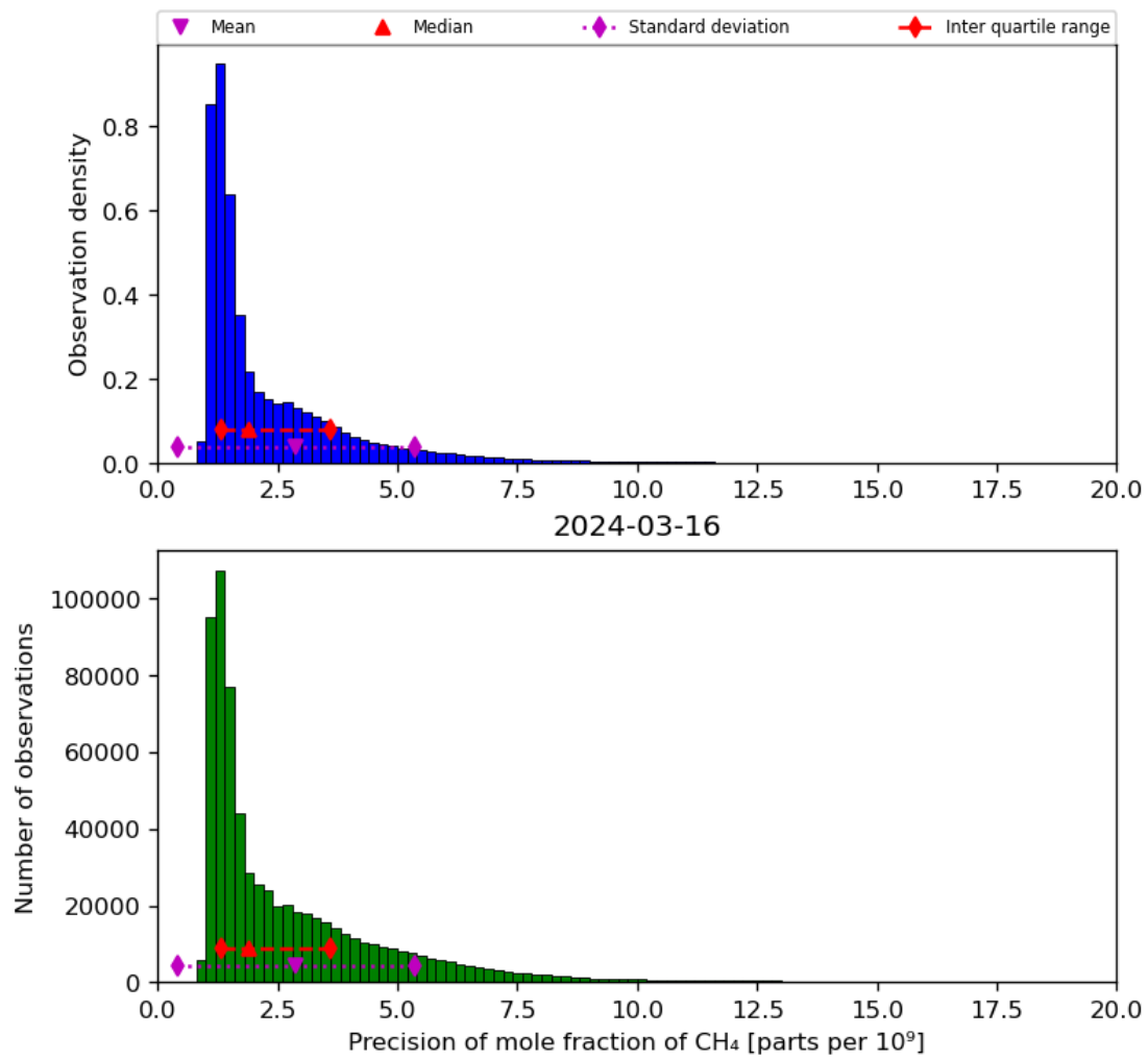
Figure 24: Histogram of “Precision of mole fraction of CH 4 ” for 2024-03-15 to 2024-03-17
