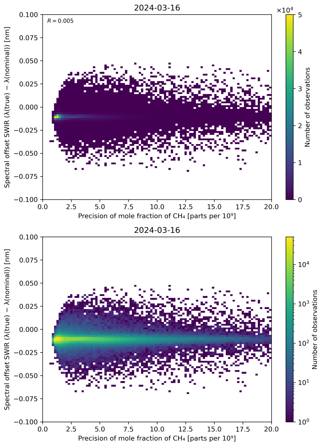
Figure 85: Scatter density plot of “Precision of mole fraction of CH 4 ” against “Spectral offset SWIR ( \lambda(\text{true}) - \lambda(\text{nominal}) )” for 2024-03-15 to 2024-03-17.
