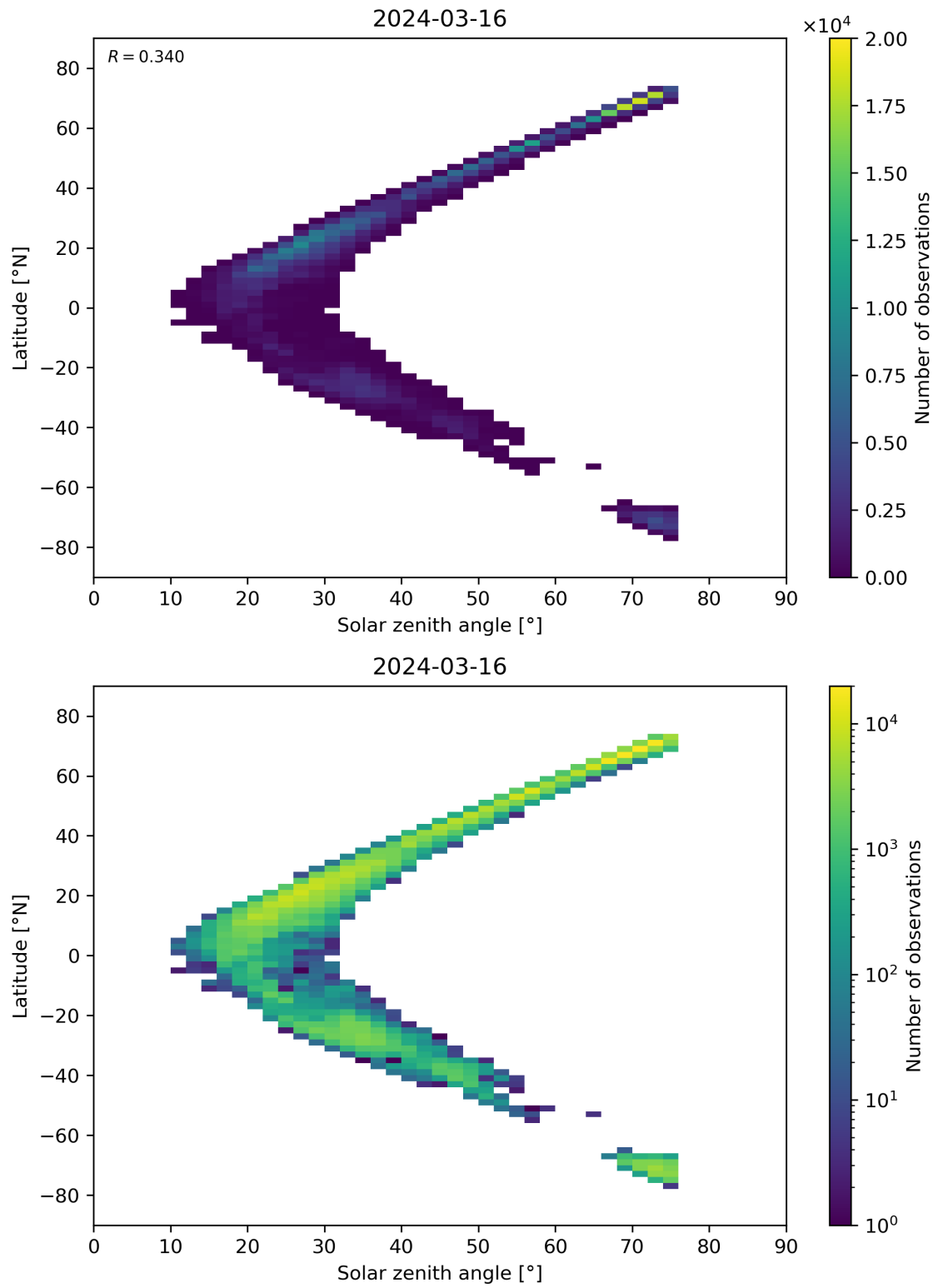
Figure 98: Scatter density plot of “Solar zenith angle” against “Latitude” for 2024-03-15 to 2024-03-17.
