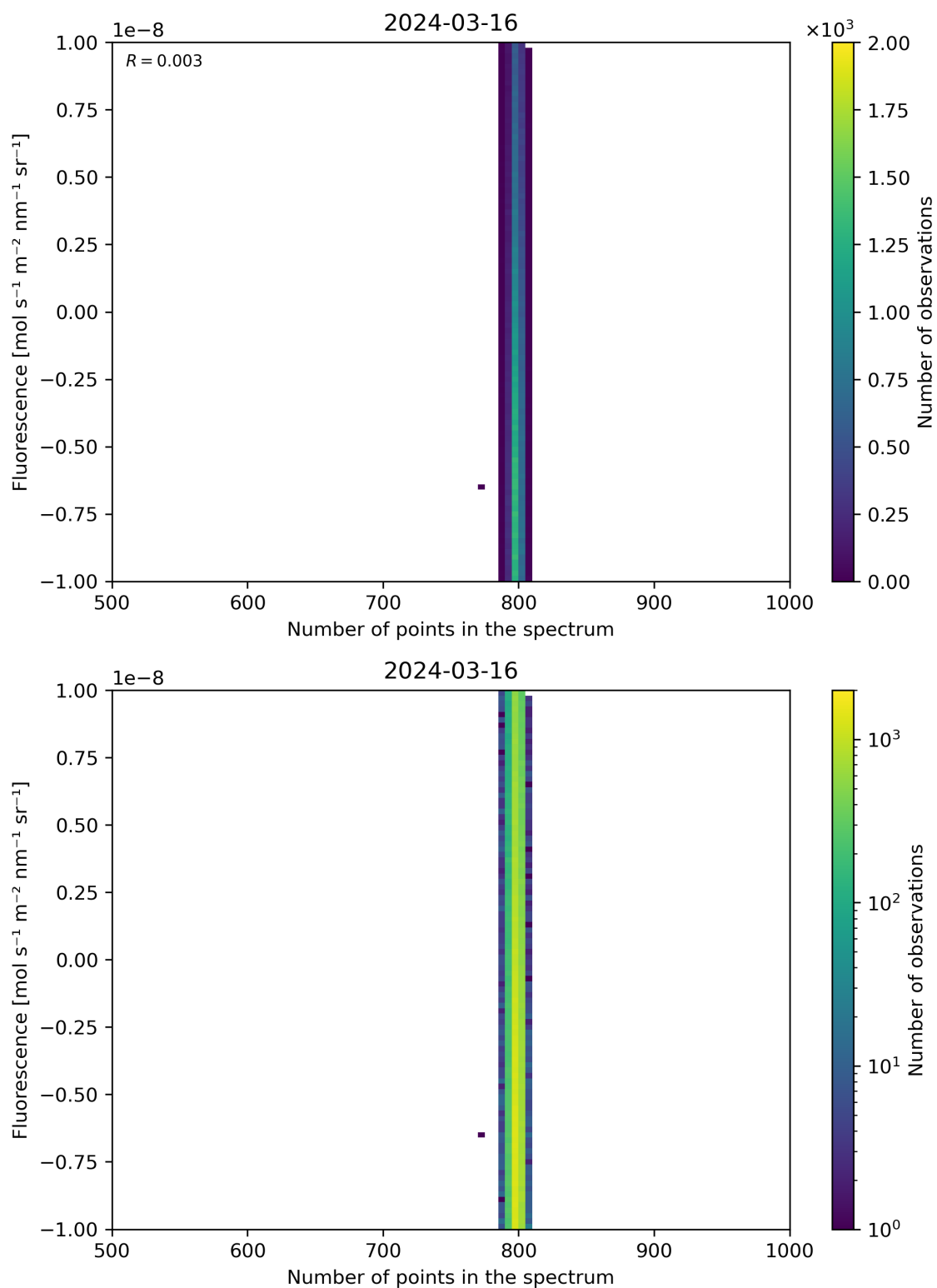
Figure 91: Scatter density plot of “Number of points in the spectrum” against “Fluorescence” for 2024-03-15 to 2024-03-17.
