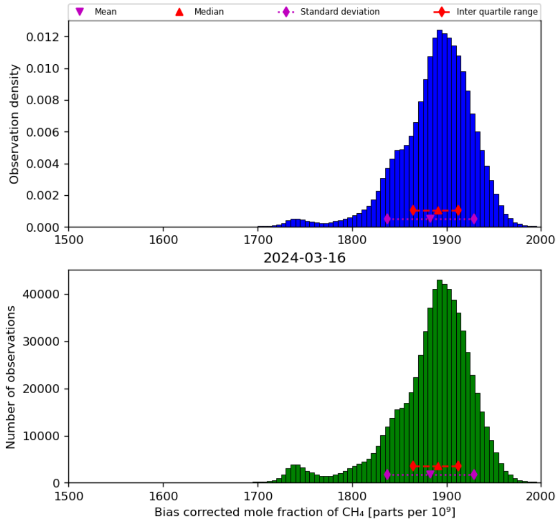
Figure 25: Histogram of “Bias corrected mole fraction of CH 4 ” for 2024-03-15 to 2024-03-17
