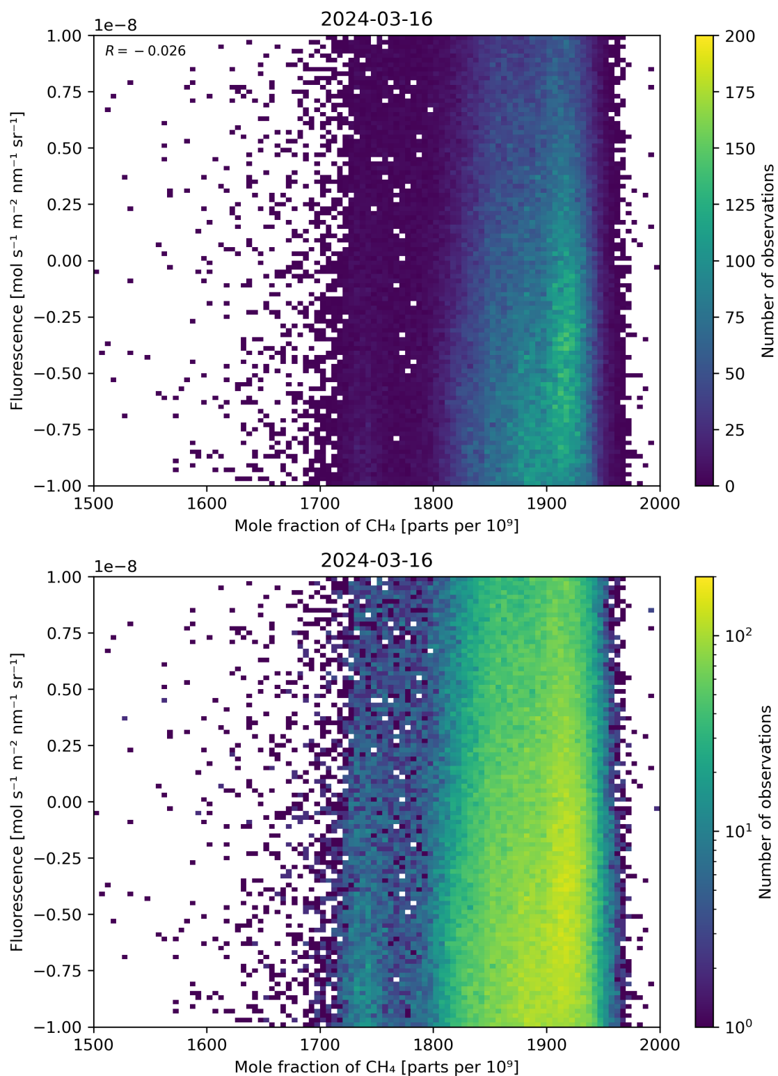
Figure 73: Scatter density plot of “Mole fraction of \text{CH}_4 ” against “Fluorescence” for 2024-03-15 to 2024-03-17.
