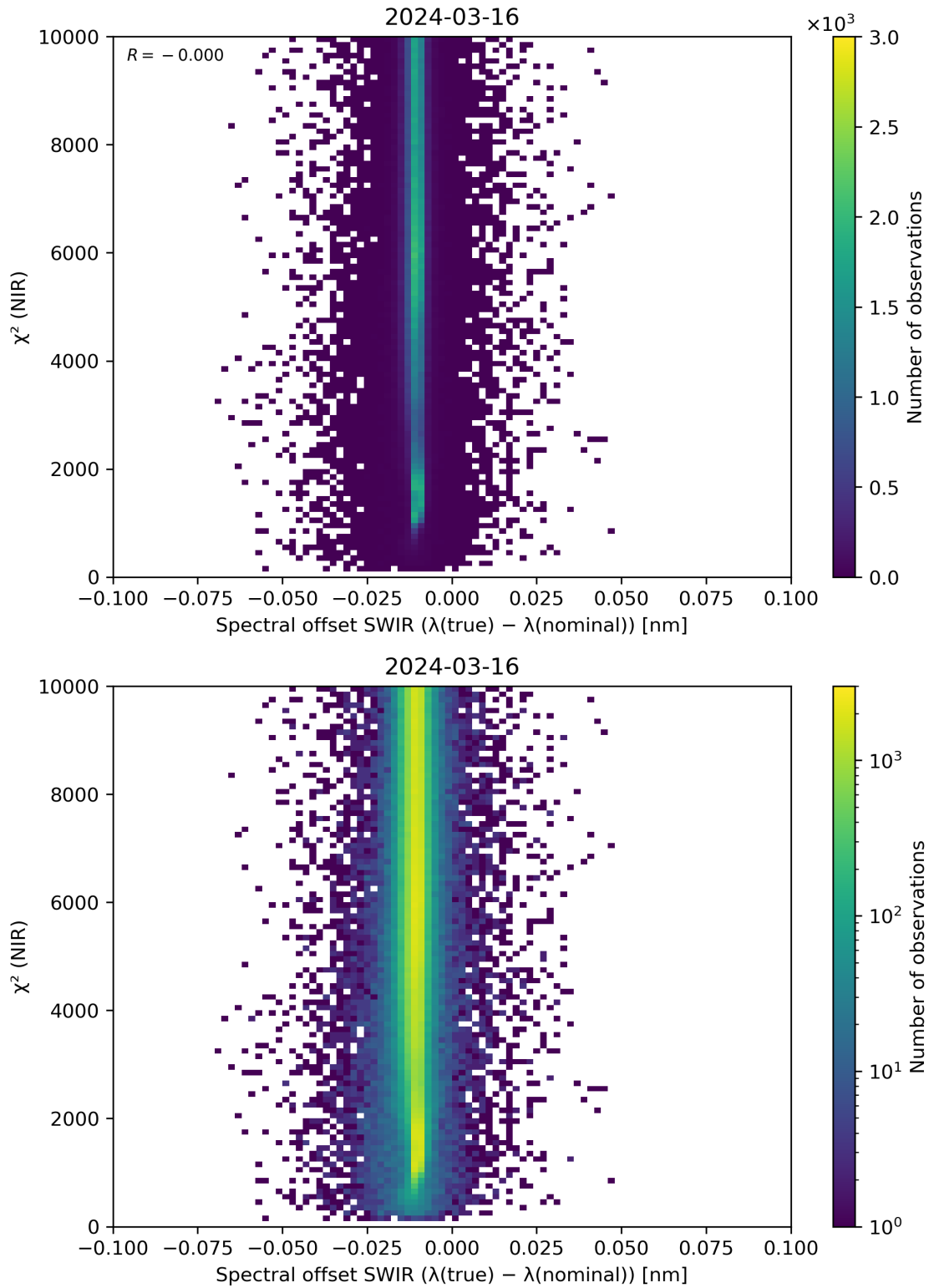
Figure 117: Scatter density plot of “Spectral offset SWIR ( \lambda(\text{true}) - \lambda(\text{nominal}) )” against “ \chi^2 (NIR)” for 2024-03-15 to 2024-03-17.
