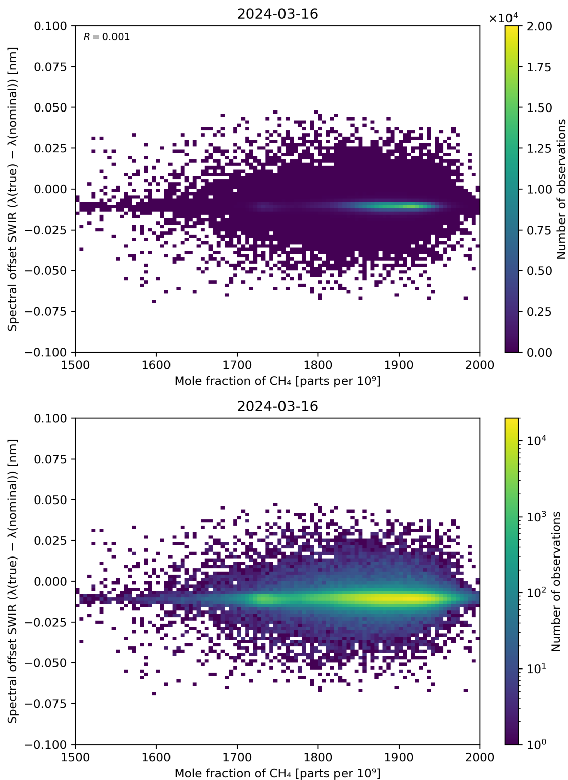
Figure 86: Scatter density plot of “Mole fraction of CH 4 ” against “Spectral offset SWIR ( \lambda(\text{true}) - \lambda(\text{nominal}) )” for 2024-03-15 to 2024-03-17.
