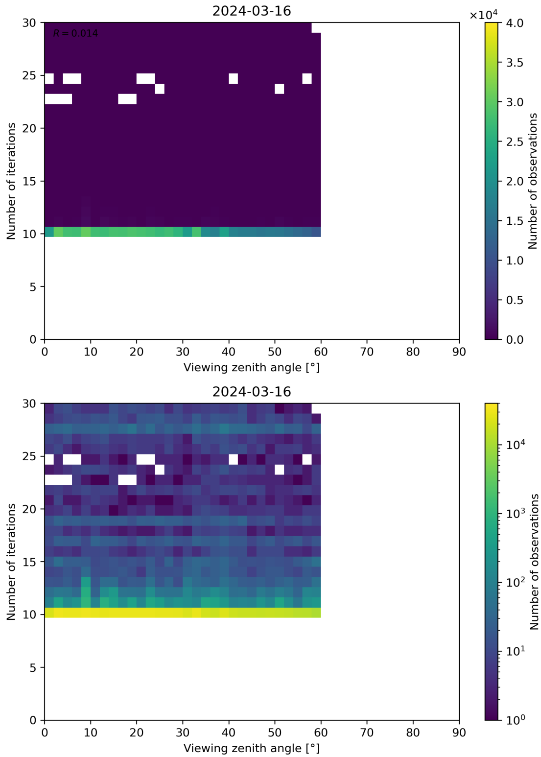
Figure 113: Scatter density plot of “Viewing zenith angle” against “Number of iterations” for 2024-03-15 to 2024-03-17.
