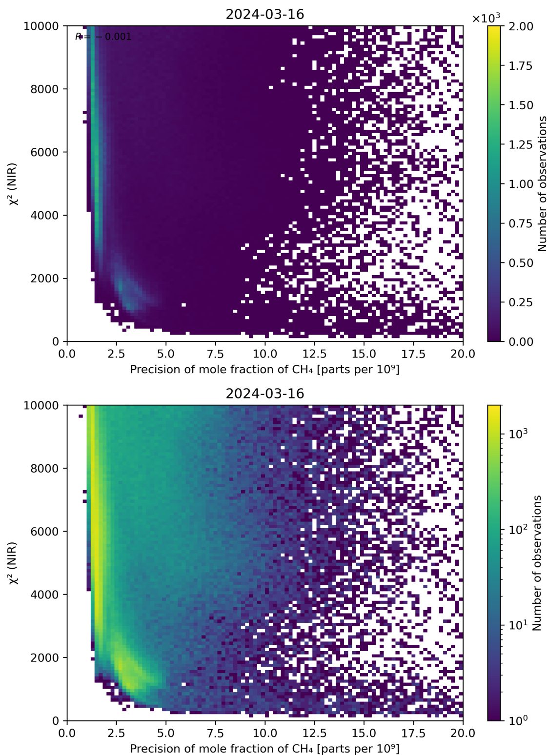
Figure 78: Scatter density plot of “Precision of mole fraction of CH 4 ” against “ \chi^2 (NIR)” for 2024-03-15 to 2024-03-17.
