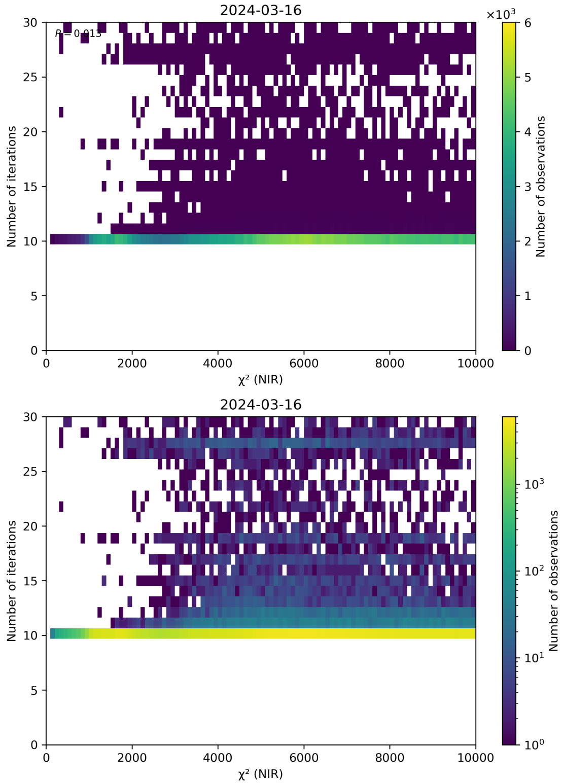
Figure 46: Scatter density plot of “ \chi^2 (NIR)” against “Number of iterations” for 2024-03-15 to 2024-03-17.
