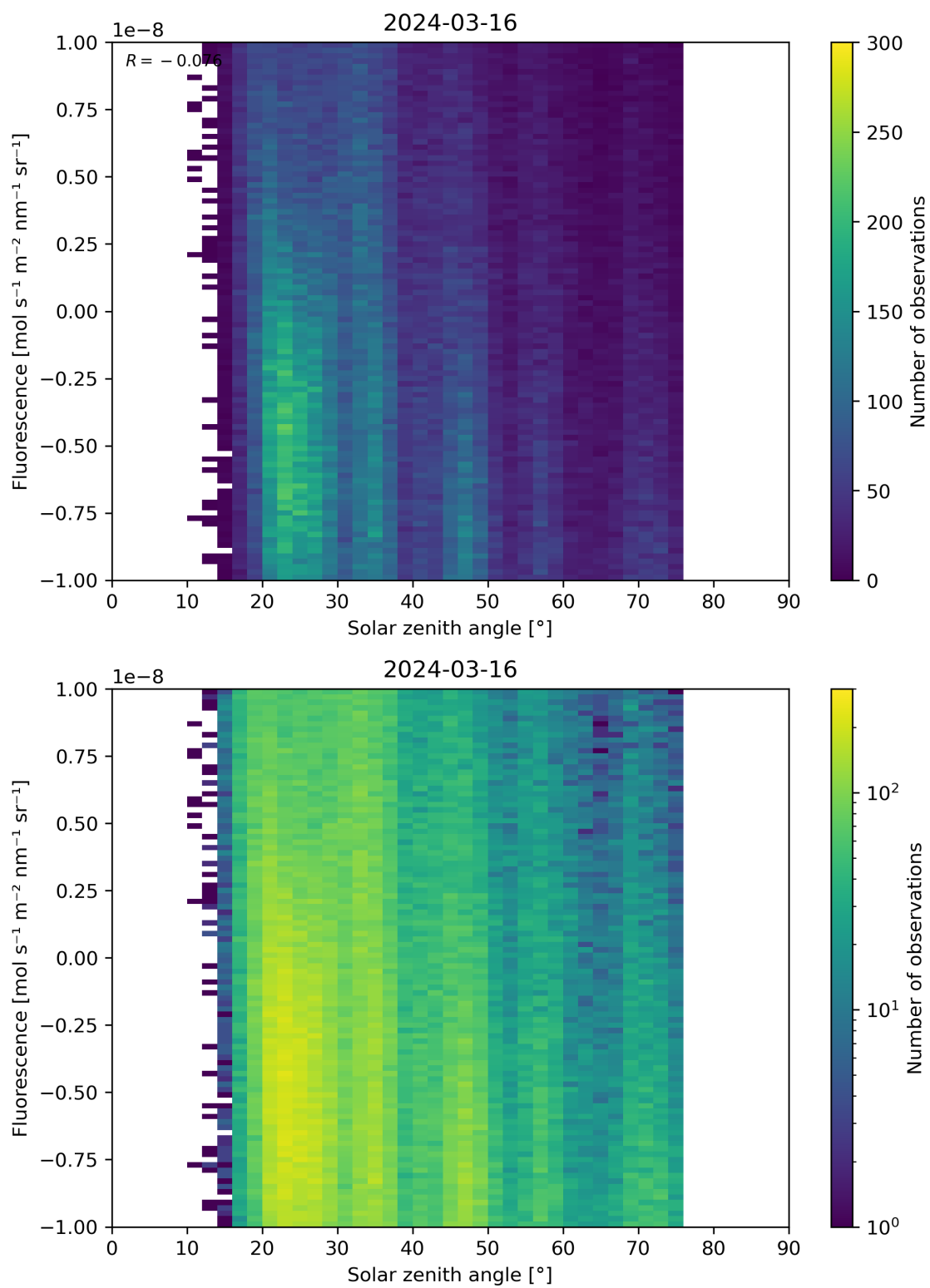
Figure 97: Scatter density plot of “Solar zenith angle” against “Fluorescence” for 2024-03-15 to 2024-03-17.
