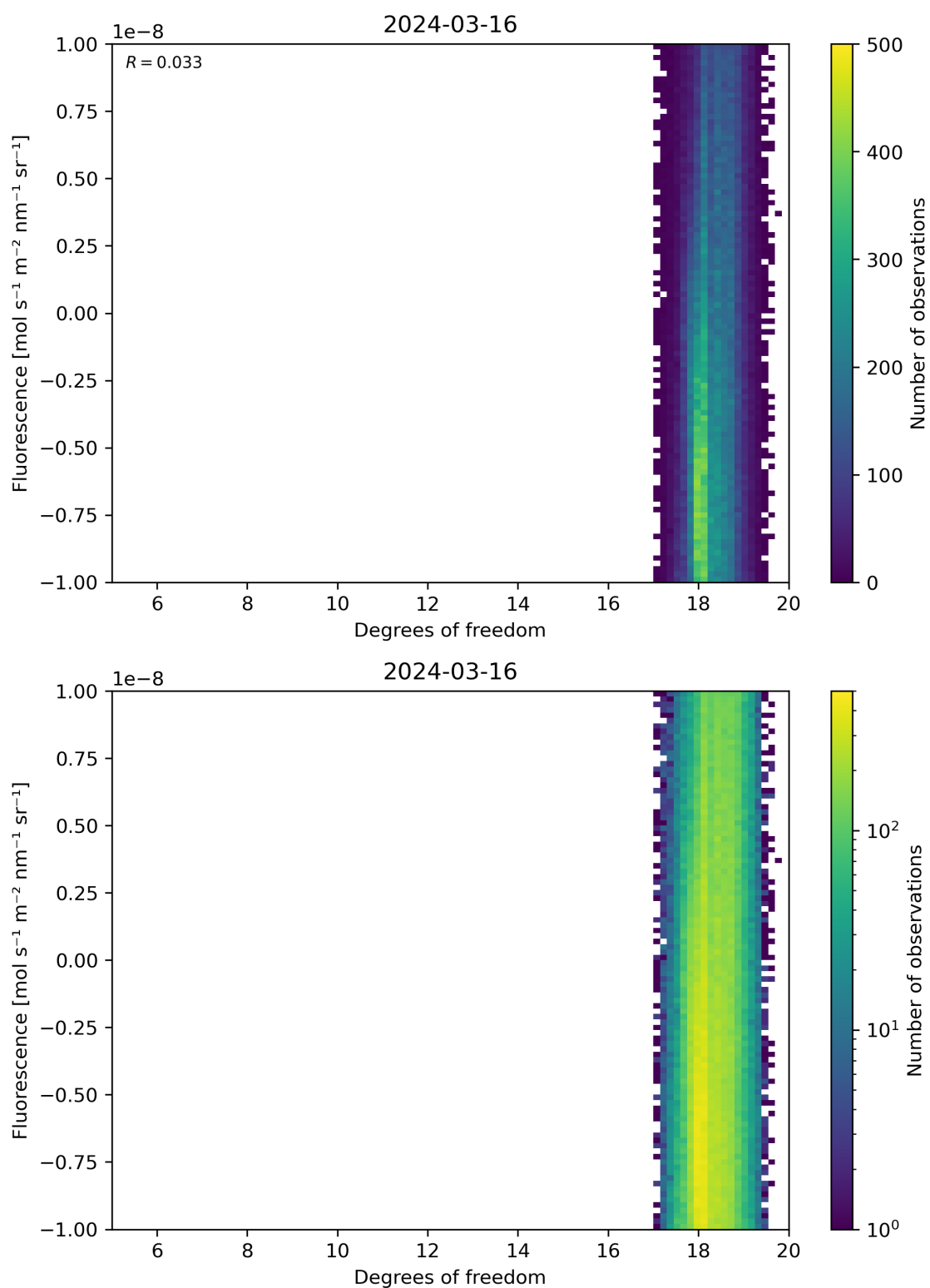
Figure 51: Scatter density plot of “Degrees of freedom” against “Fluorescence” for 2024-03-15 to 2024-03-17.
