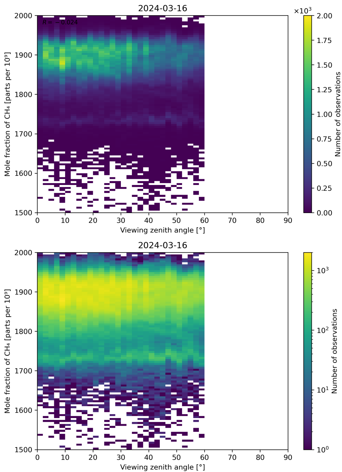
Figure 110: Scatter density plot of “Viewing zenith angle” against “Mole fraction of CH 4 ” for 2024-03-15 to 2024-03-17.
