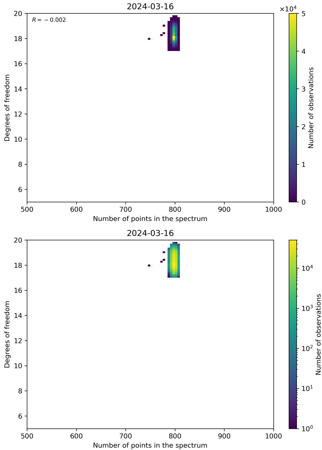
Figure 90: Scatter density plot of “Number of points in the spectrum” against “Degrees of freedom” for 2024-03-15 to 2024-03-17.
