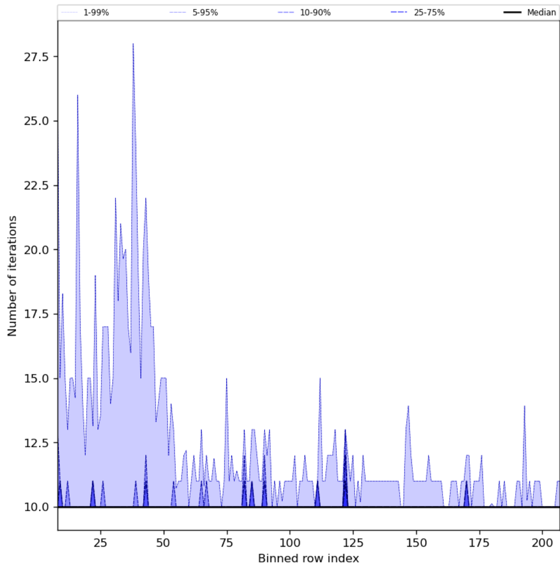
Figure 42: Along track statistics of “Number of iterations” for 2024-03-15 to 2024-03-17
