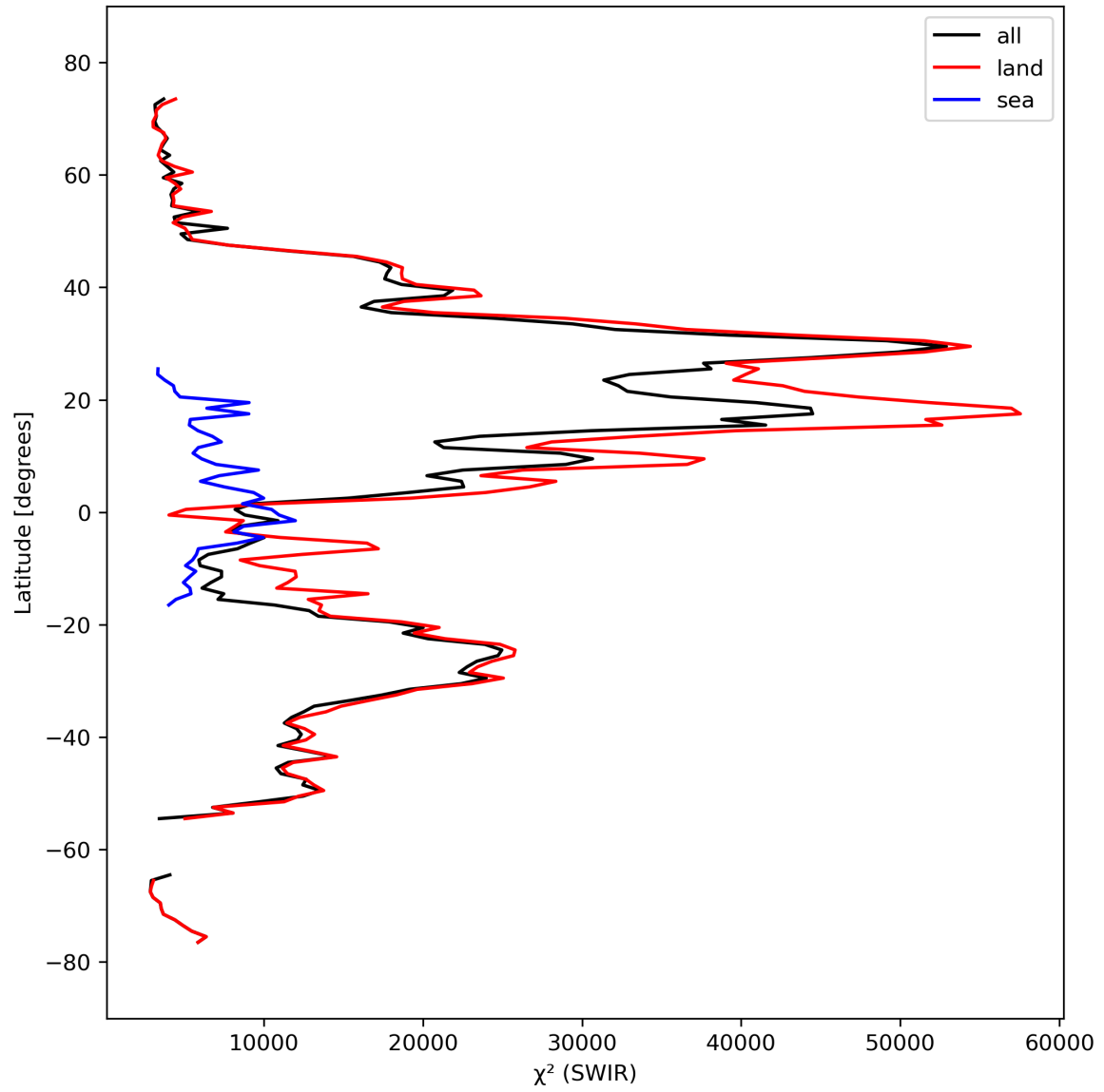
Figure 17: Zonal average of “ \chi^2 (SWIR)” for 2024-03-15 to 2024-03-17.
