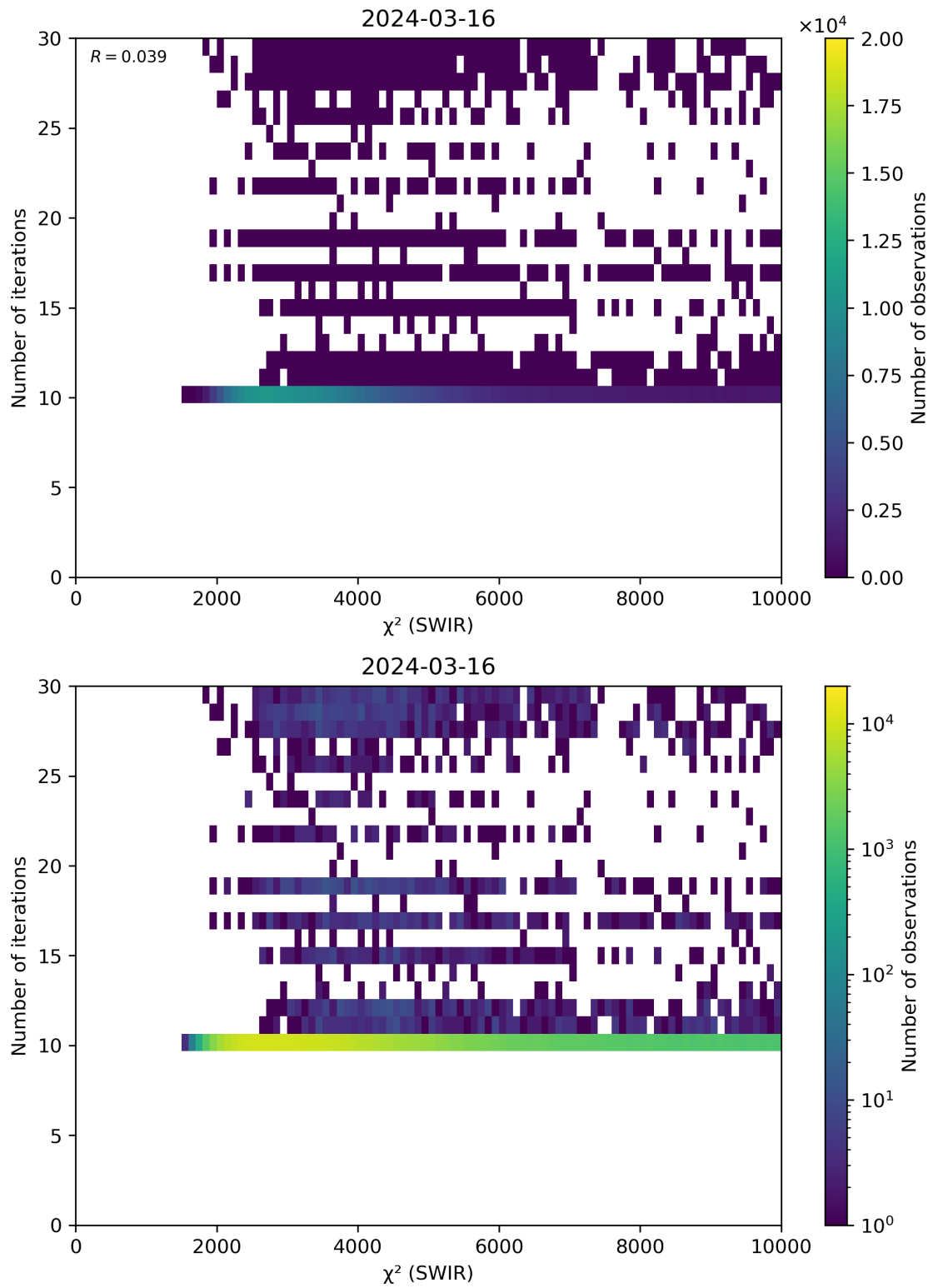
Figure 50: Scatter density plot of “ \chi^2 (SWIR)” against “Number of iterations” for 2024-03-15 to 2024-03-17.
