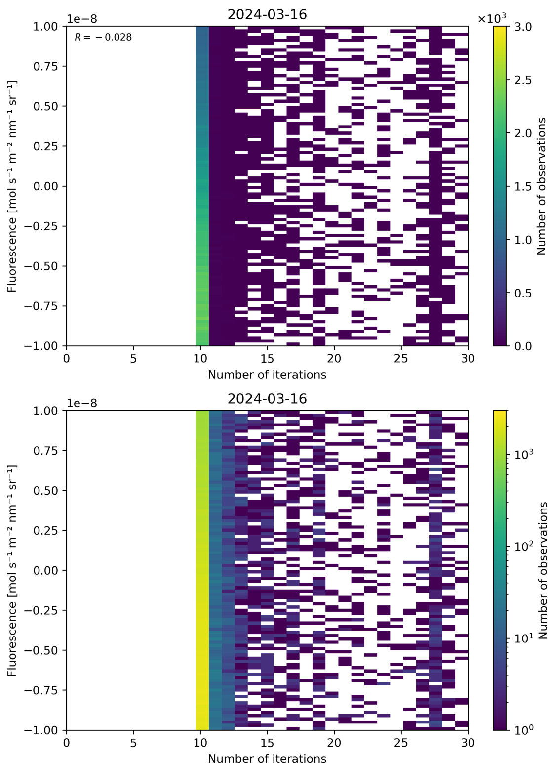
Figure 87: Scatter density plot of “Number of iterations” against “Fluorescence” for 2024-03-15 to 2024-03-17.
