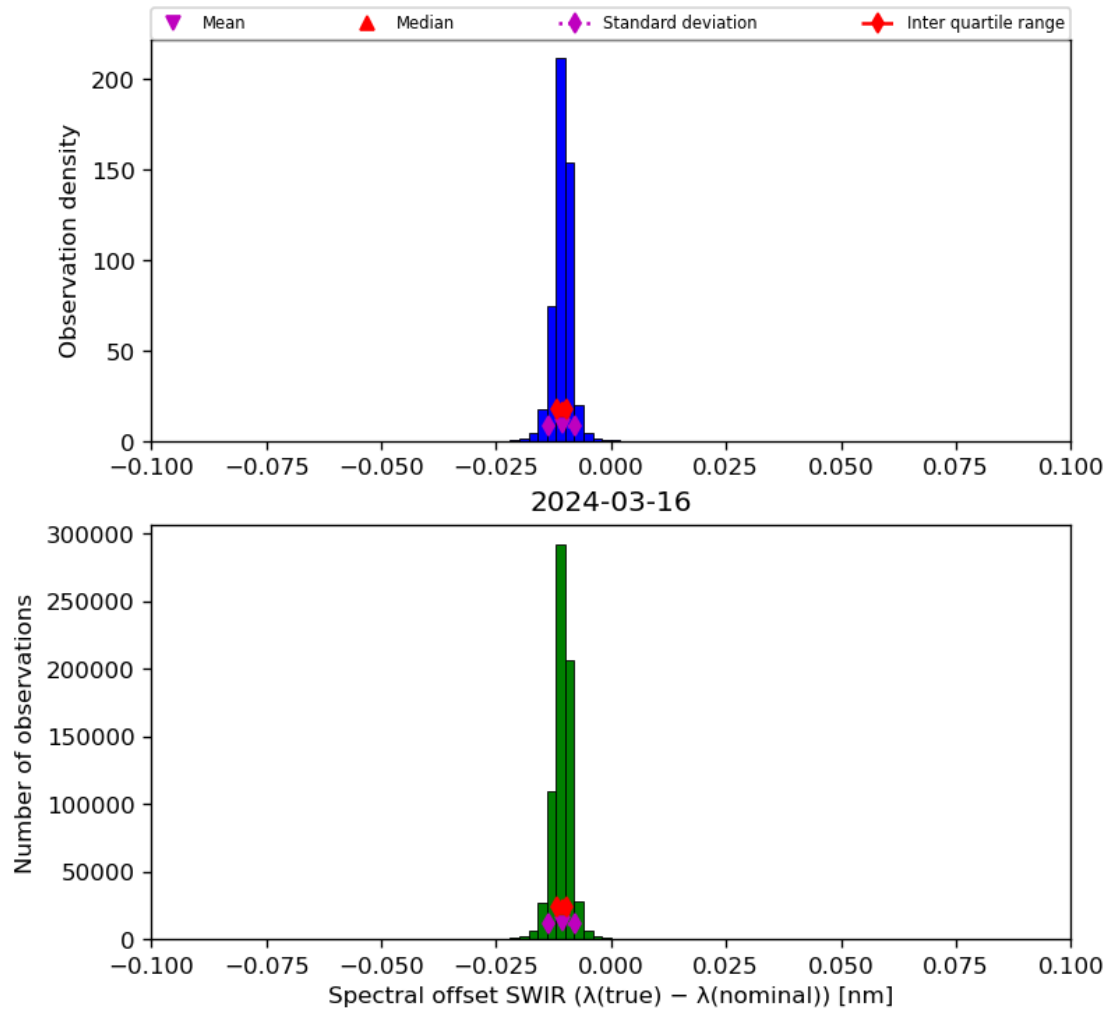
Figure 27: Histogram of “Spectral offset SWIR ( \lambda(\text{true}) - \lambda(\text{nominal}) )” for 2024-03-15 to 2024-03-17
