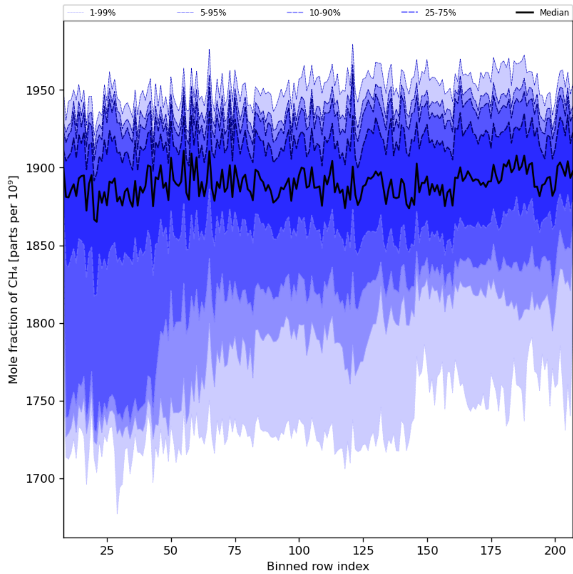
Figure 34: Along track statistics of “Mole fraction of CH 4 ” for 2024-03-15 to 2024-03-17
