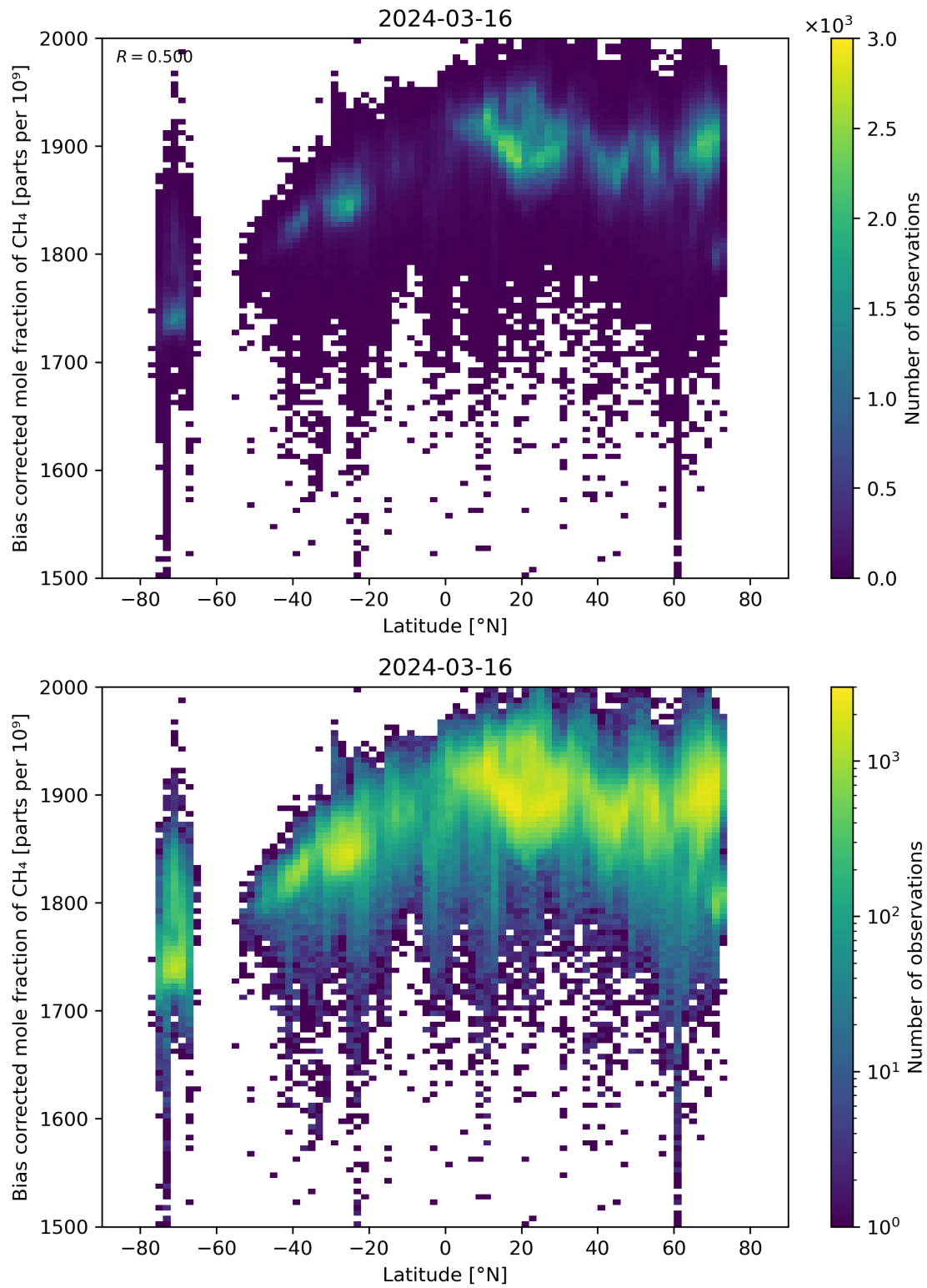
Figure 58: Scatter density plot of “Latitude” against “Bias corrected mole fraction of \text{CH}_4 ” for 2024-03-15 to 2024-03-17.
