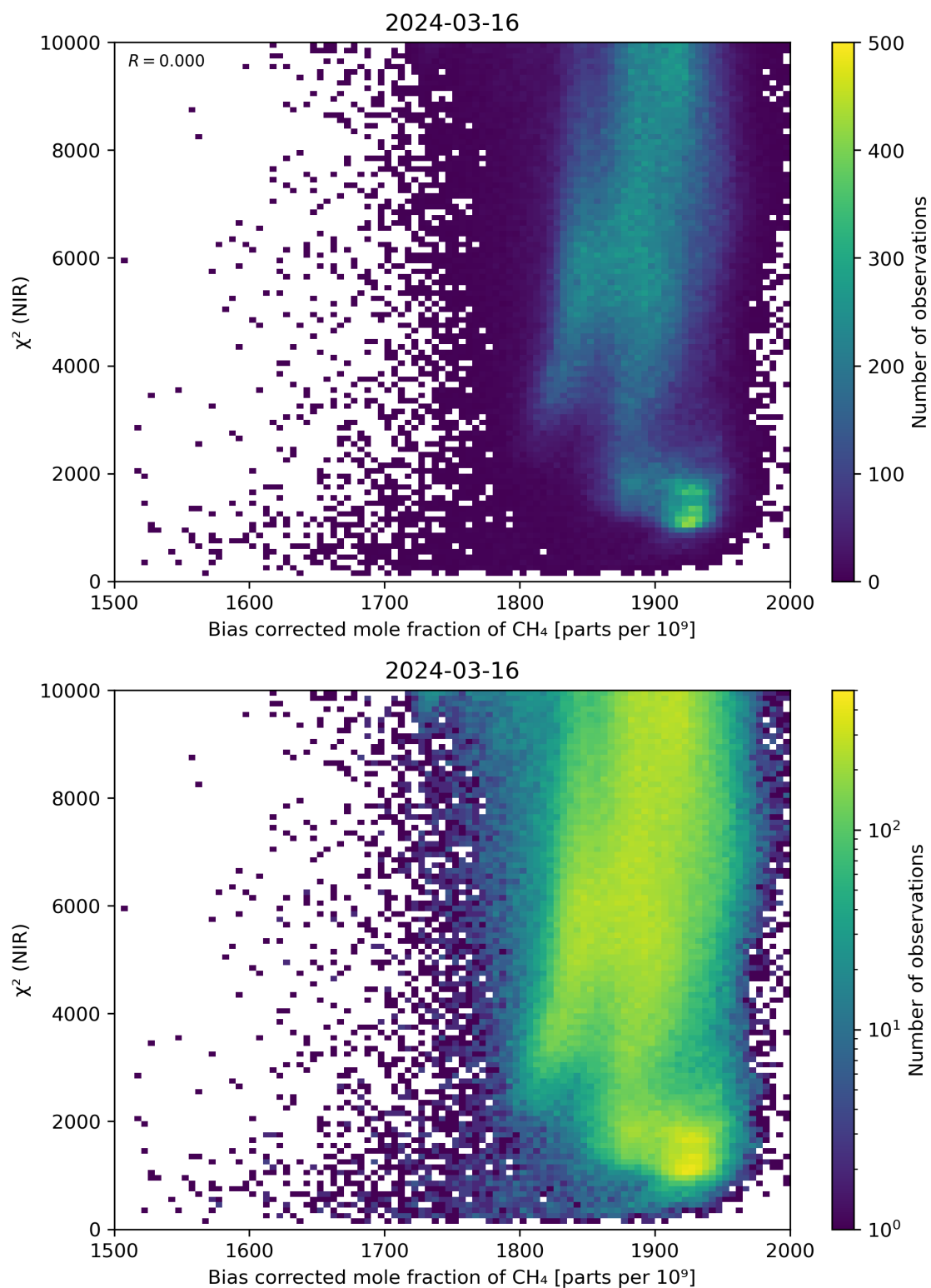
Figure 63: Scatter density plot of “Bias corrected mole fraction of \text{CH}_4 ” against “ \chi^2 (NIR)” for 2024-03-15 to 2024-03-17.
