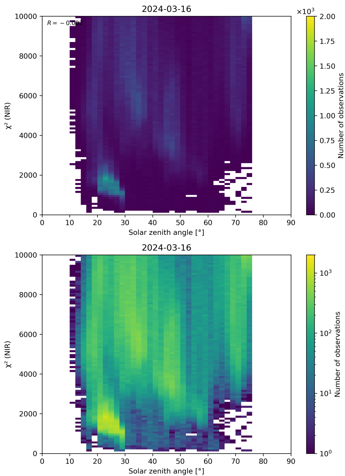
Figure 94: Scatter density plot of “Solar zenith angle” against “ \chi^2 (NIR)” for 2024-03-15 to 2024-03-17.
