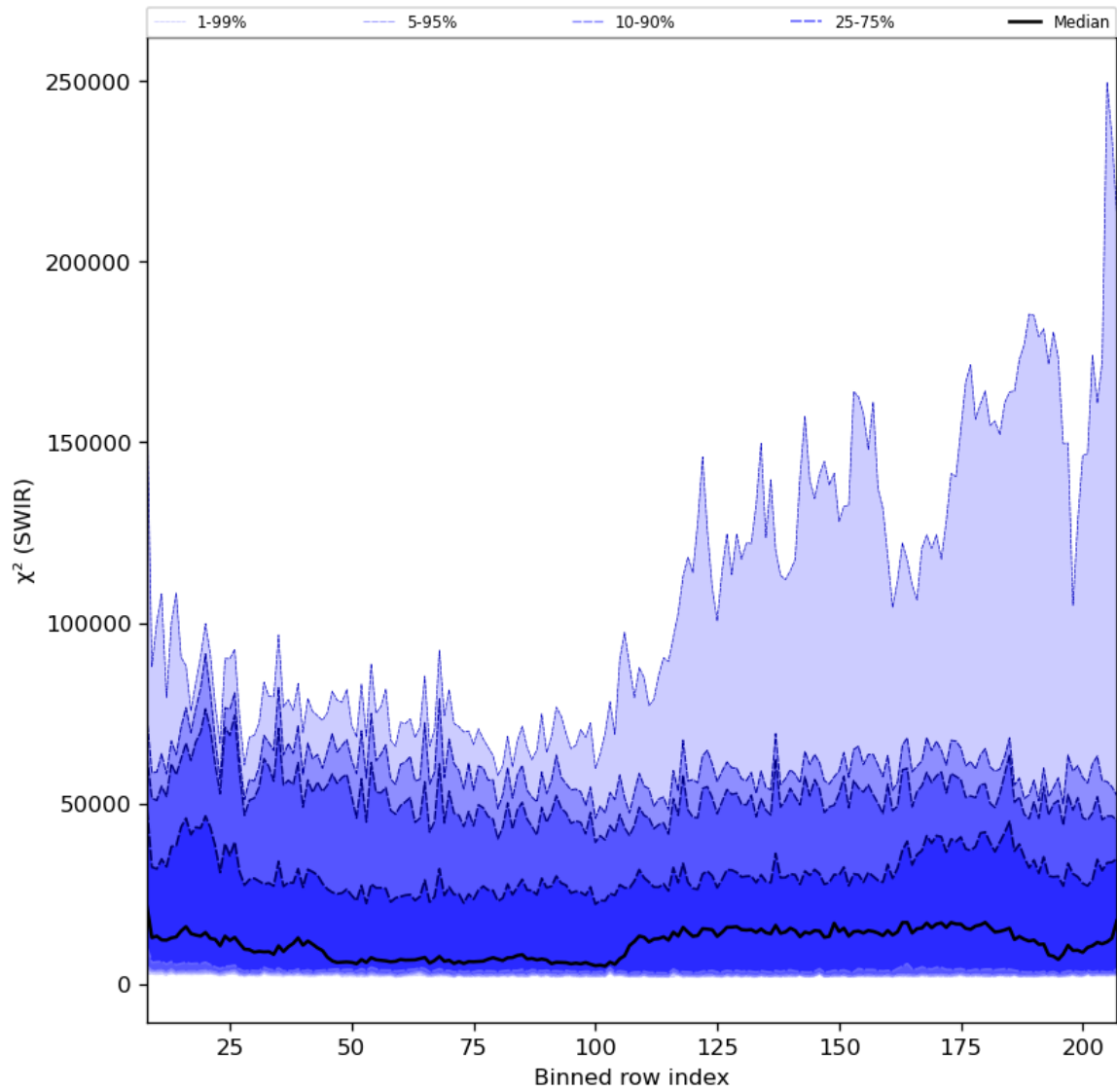
Figure 39: Along track statistics of “ \chi^2 (SWIR)” for 2024-03-15 to 2024-03-17
