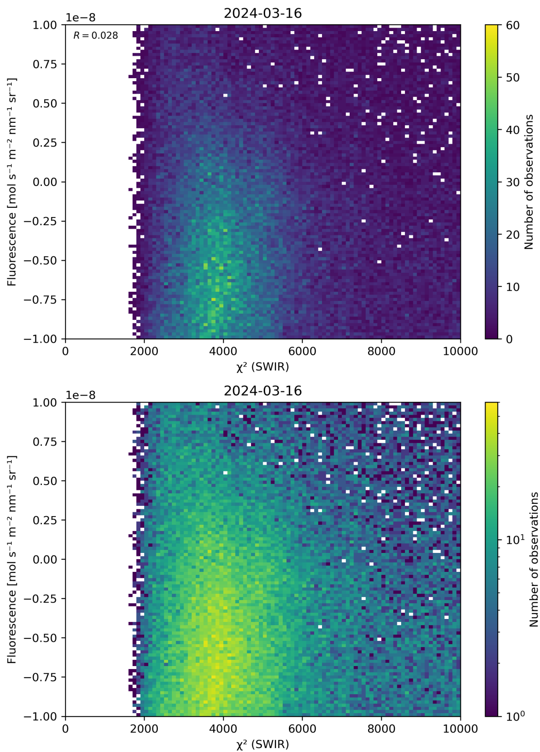
Figure 49: Scatter density plot of “ \chi^2 (SWIR)” against “Fluorescence” for 2024-03-15 to 2024-03-17.
