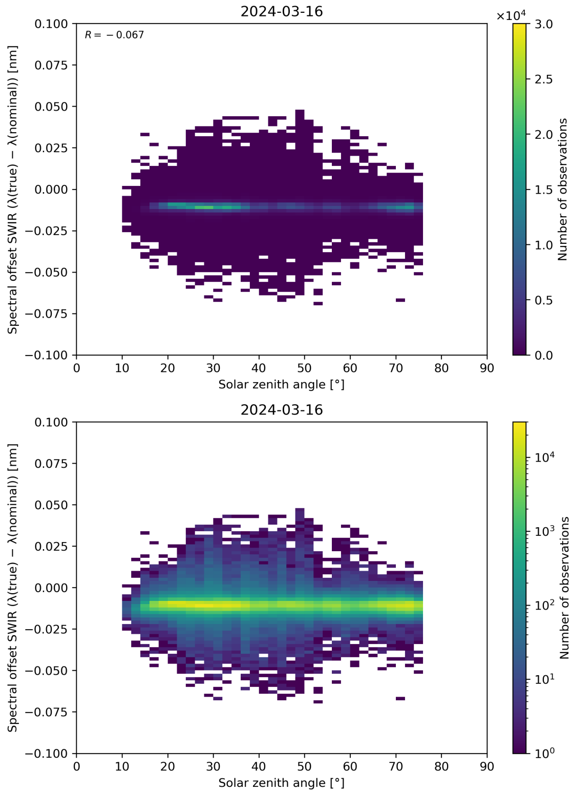
Figure 104: Scatter density plot of “Solar zenith angle” against “Spectral offset SWIR ( \lambda(\text{true}) - \lambda(\text{nominal}) )” for 2024-03-15 to 2024-03-17.
