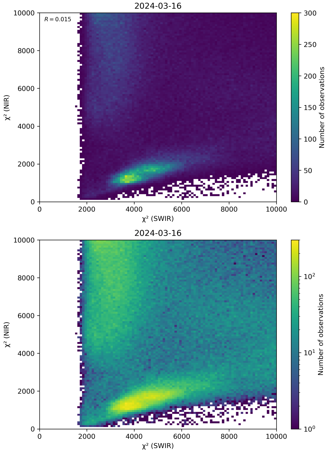
Figure 47: Scatter density plot of “ \chi^2 (SWIR)” against “ \chi^2 (NIR)” for 2024-03-15 to 2024-03-17.
