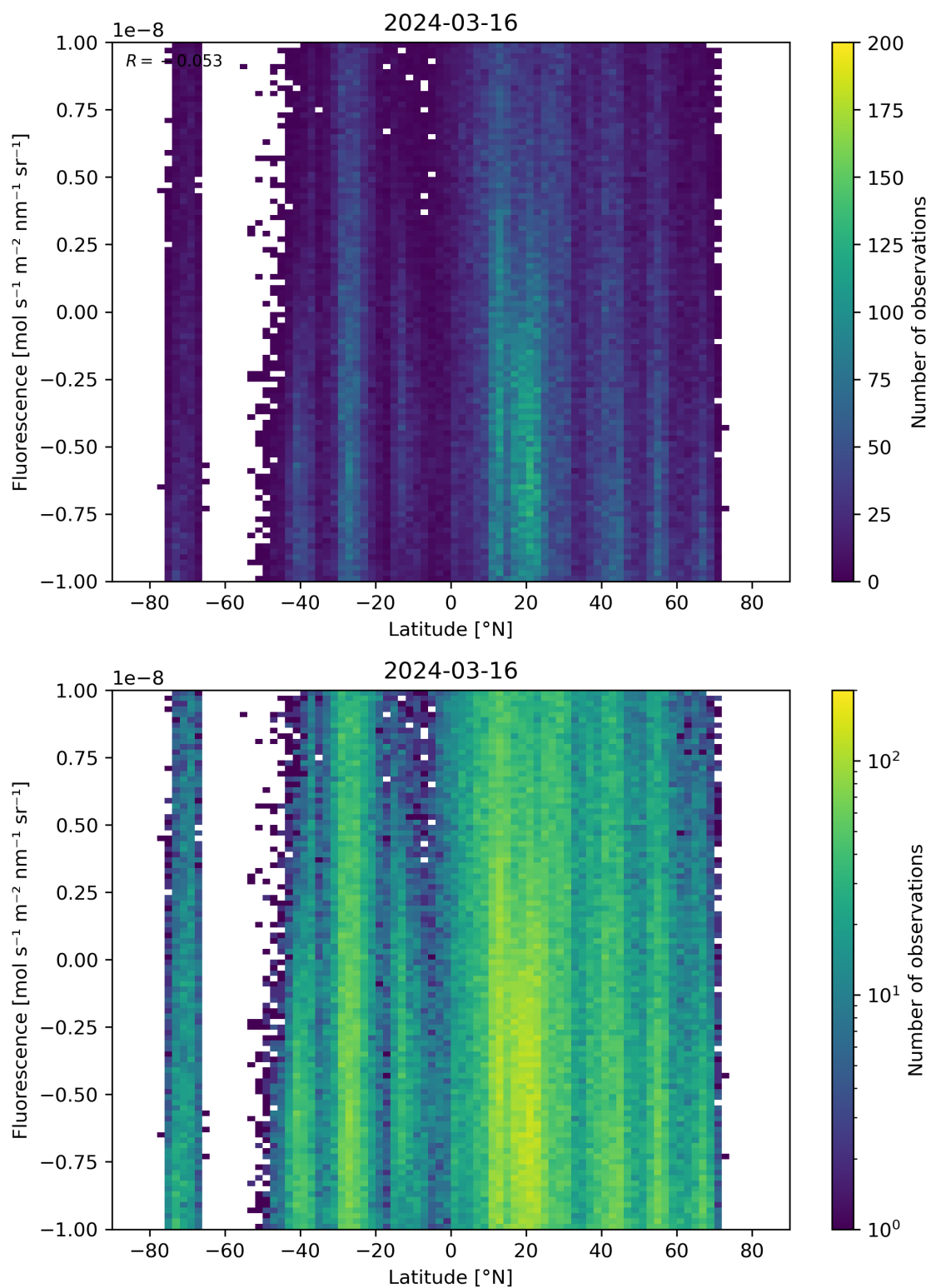
Figure 56: Scatter density plot of “Latitude” against “Fluorescence” for 2024-03-15 to 2024-03-17.
