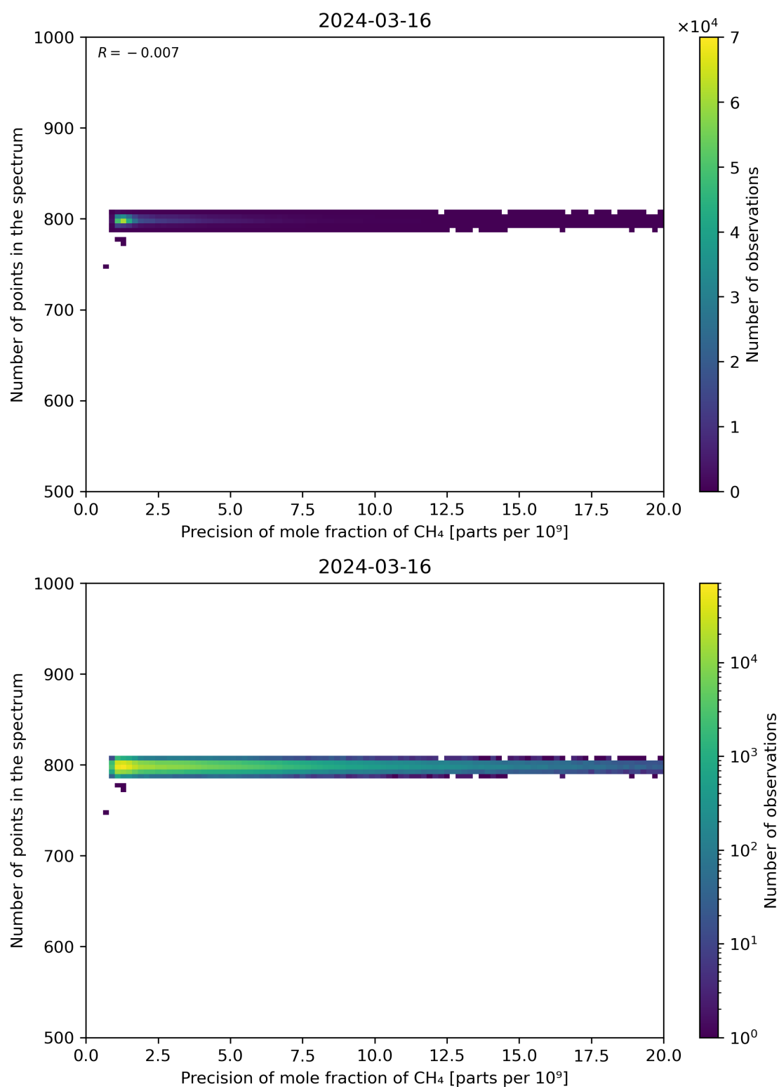
Figure 84: Scatter density plot of “Precision of mole fraction of CH 4 ” against “Number of points in the spectrum” for 2024-03-15 to 2024-03-17.
