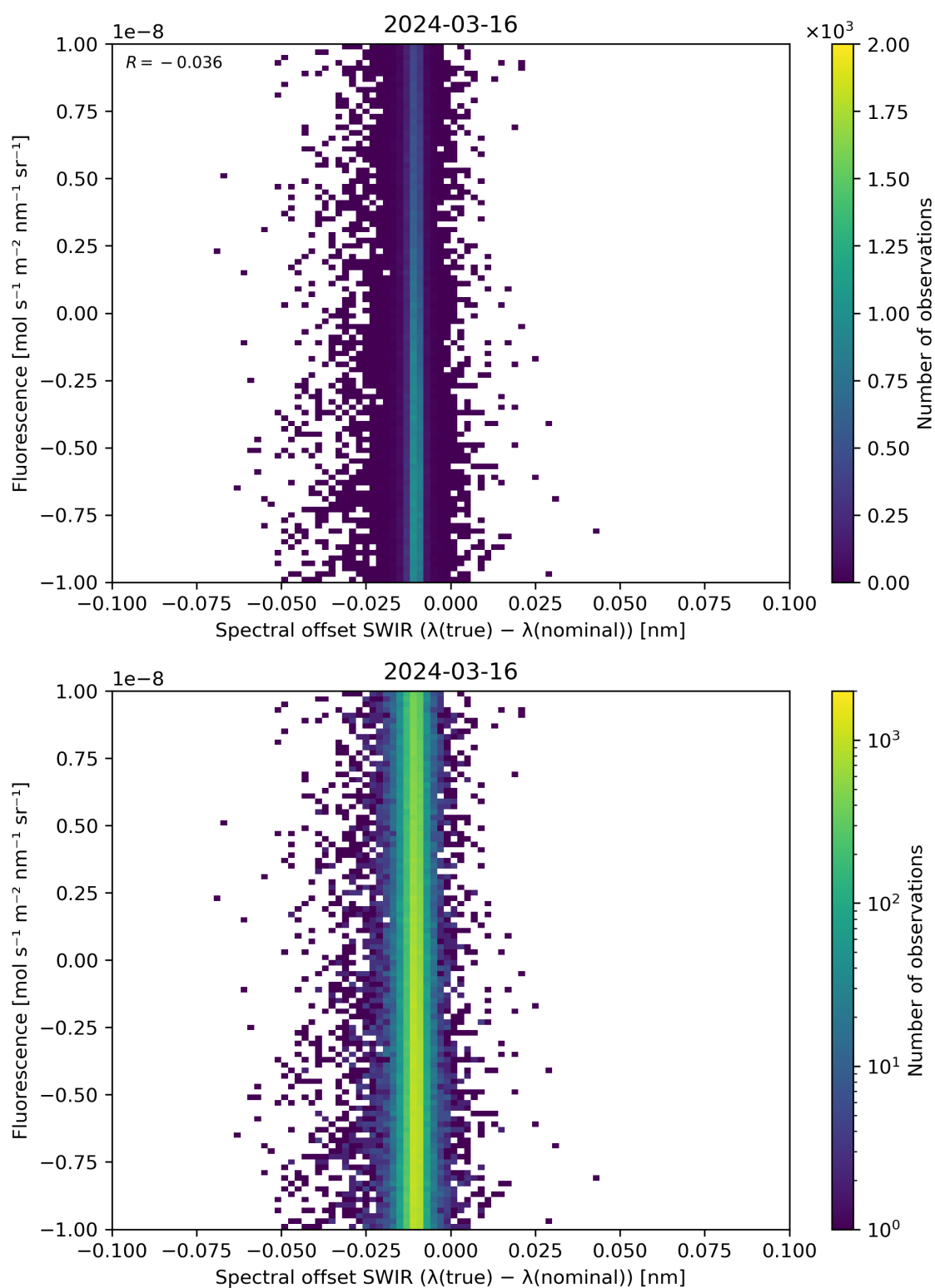
Figure 120: Scatter density plot of “Spectral offset SWIR ( \lambda(\text{true}) - \lambda(\text{nominal}) )” against “Fluorescence” for 2024-03-15 to 2024-03-17.
