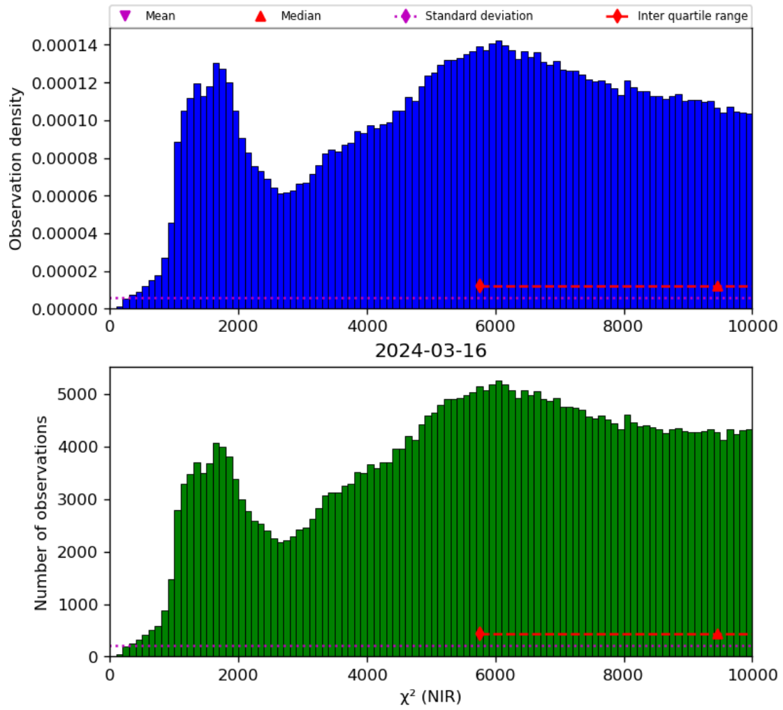
Figure 29: Histogram of " \chi^2 (NIR)" for 2024-03-15 to 2024-03-17
