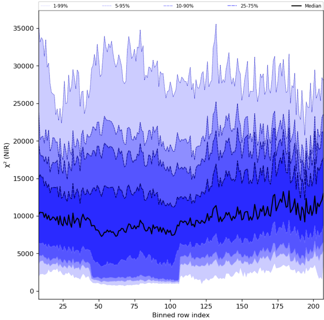
Figure 40: Along track statistics of “ \chi^2 (NIR)” for 2024-03-15 to 2024-03-17
