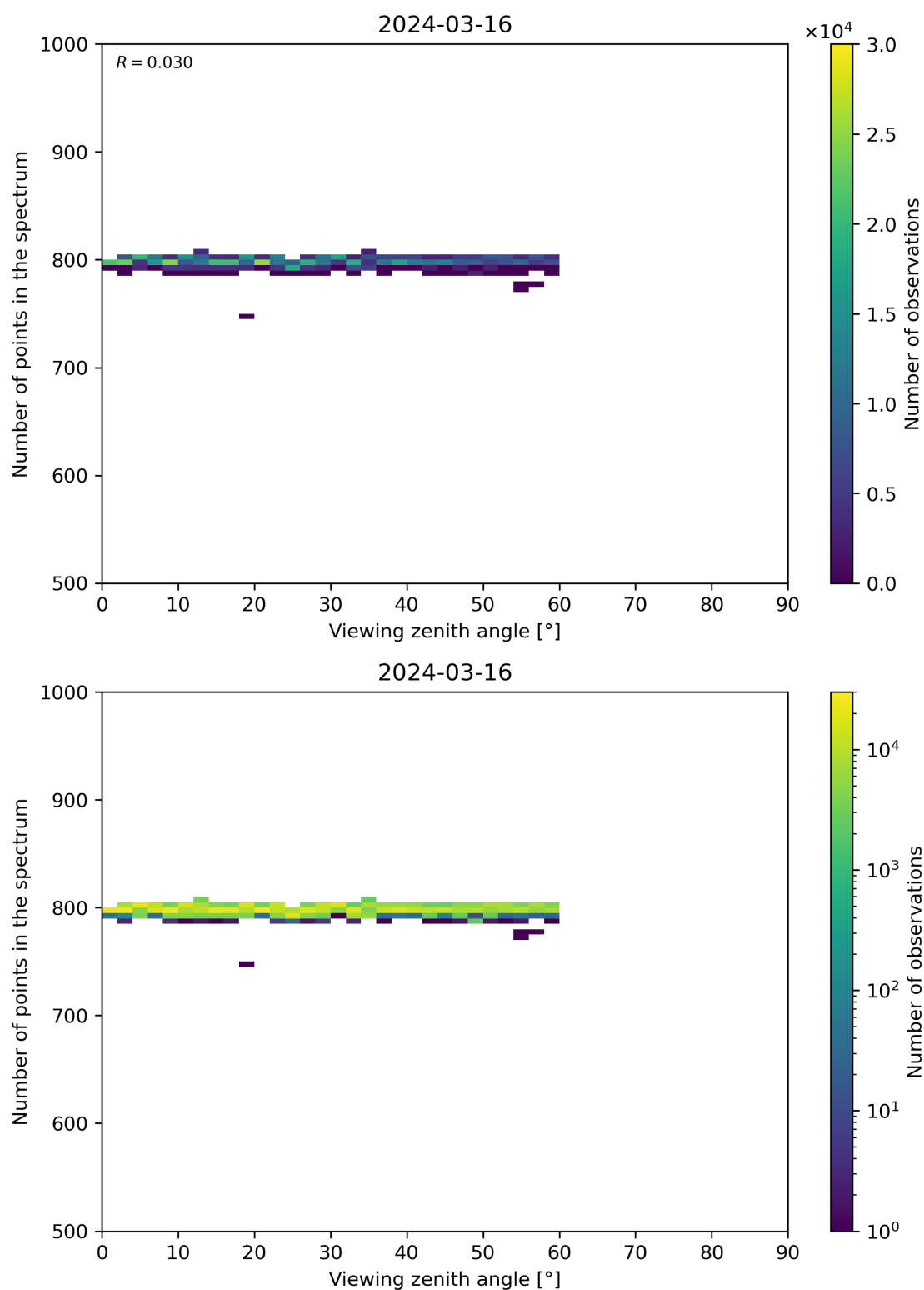
Figure 114: Scatter density plot of “Viewing zenith angle” against “Number of points in the spectrum” for 2024-03-15 to 2024-03-17.
