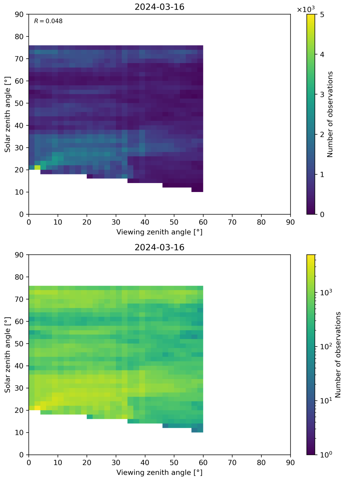
Figure 115: Scatter density plot of “Viewing zenith angle” against “Solar zenith angle” for 2024-03-15 to 2024-03-17.
