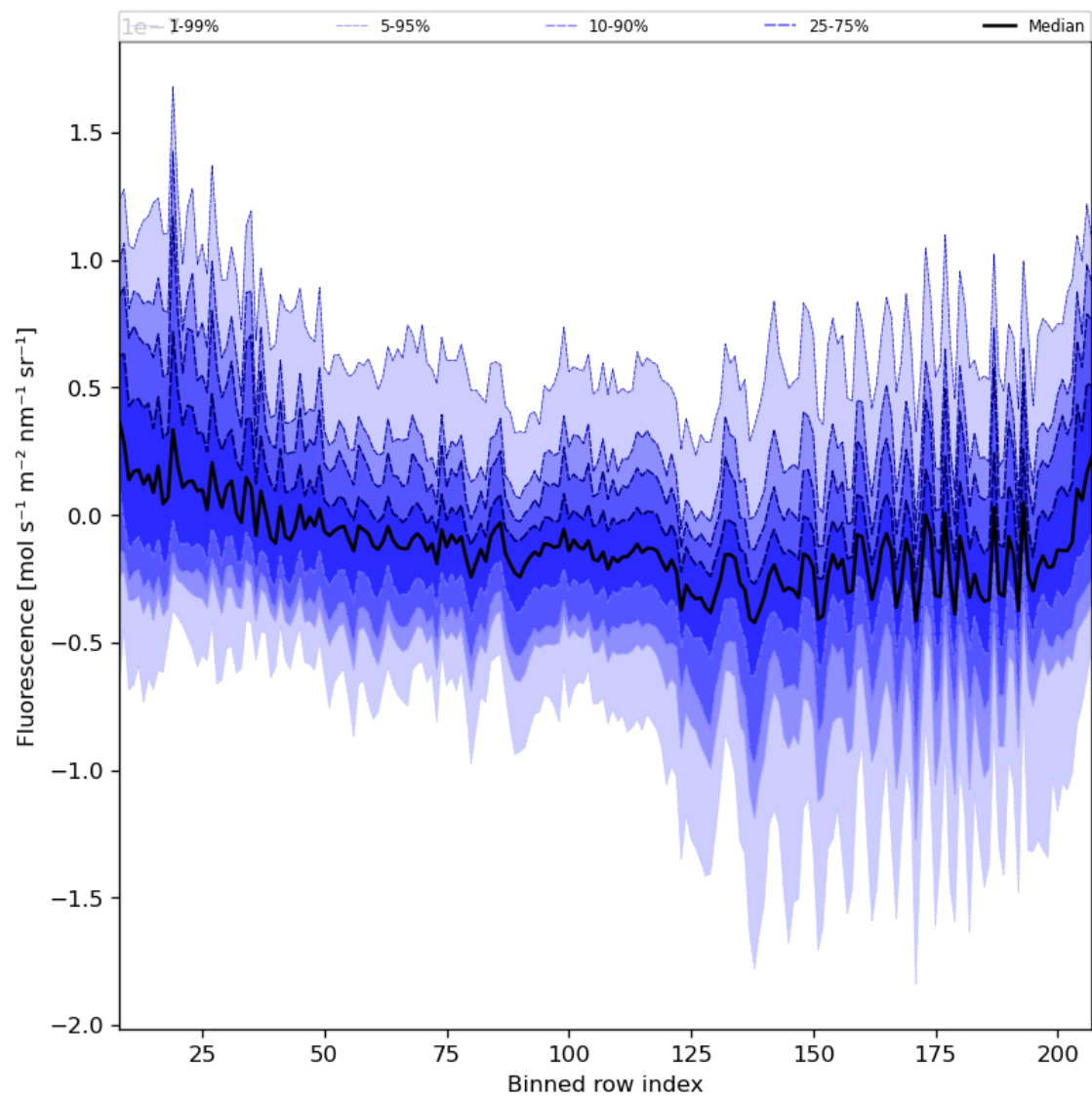
Figure 43: Along track statistics of “Fluorescence” for 2024-03-15 to 2024-03-17
