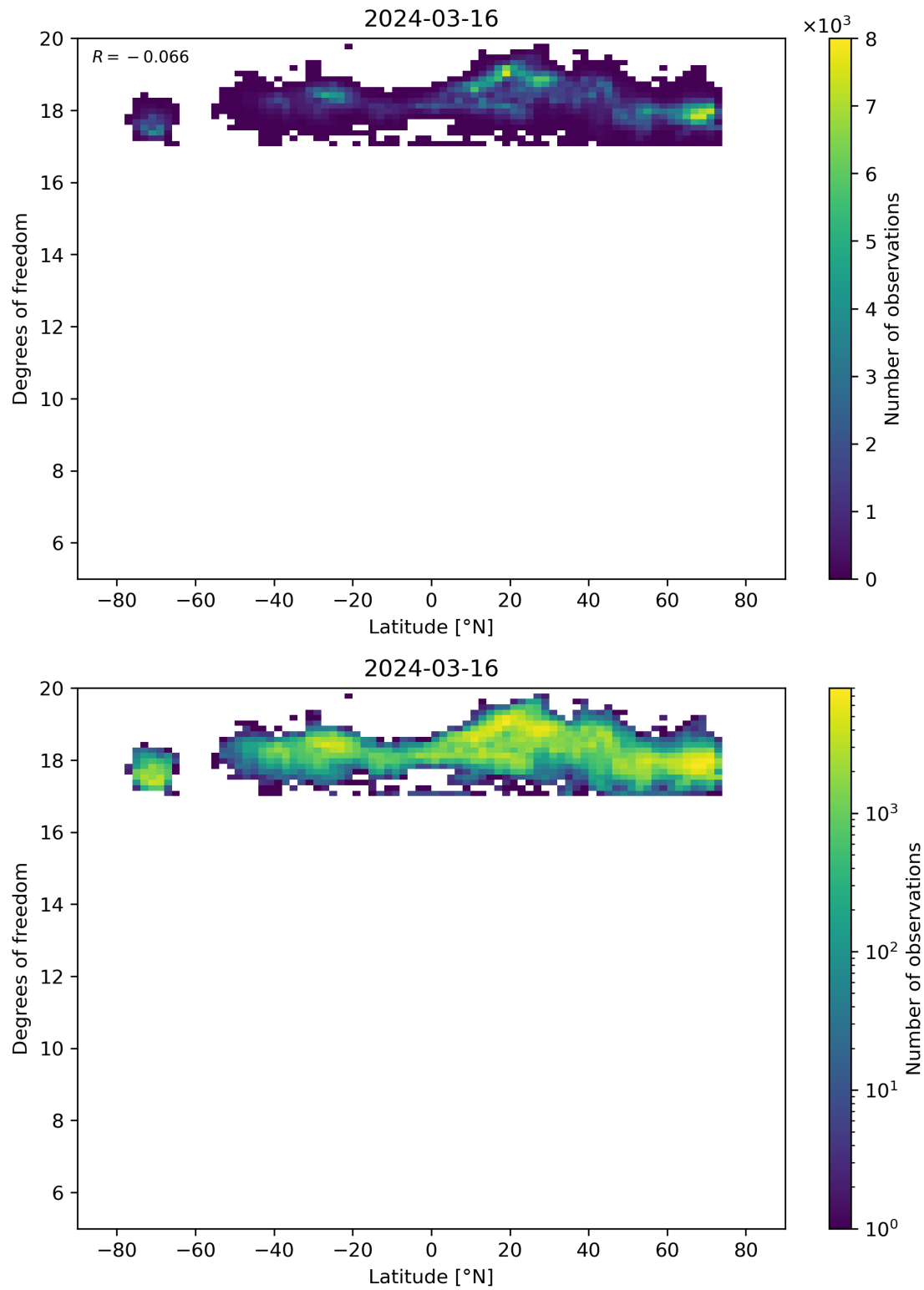
Figure 55: Scatter density plot of “Latitude” against “Degrees of freedom” for 2024-03-15 to 2024-03-17.
