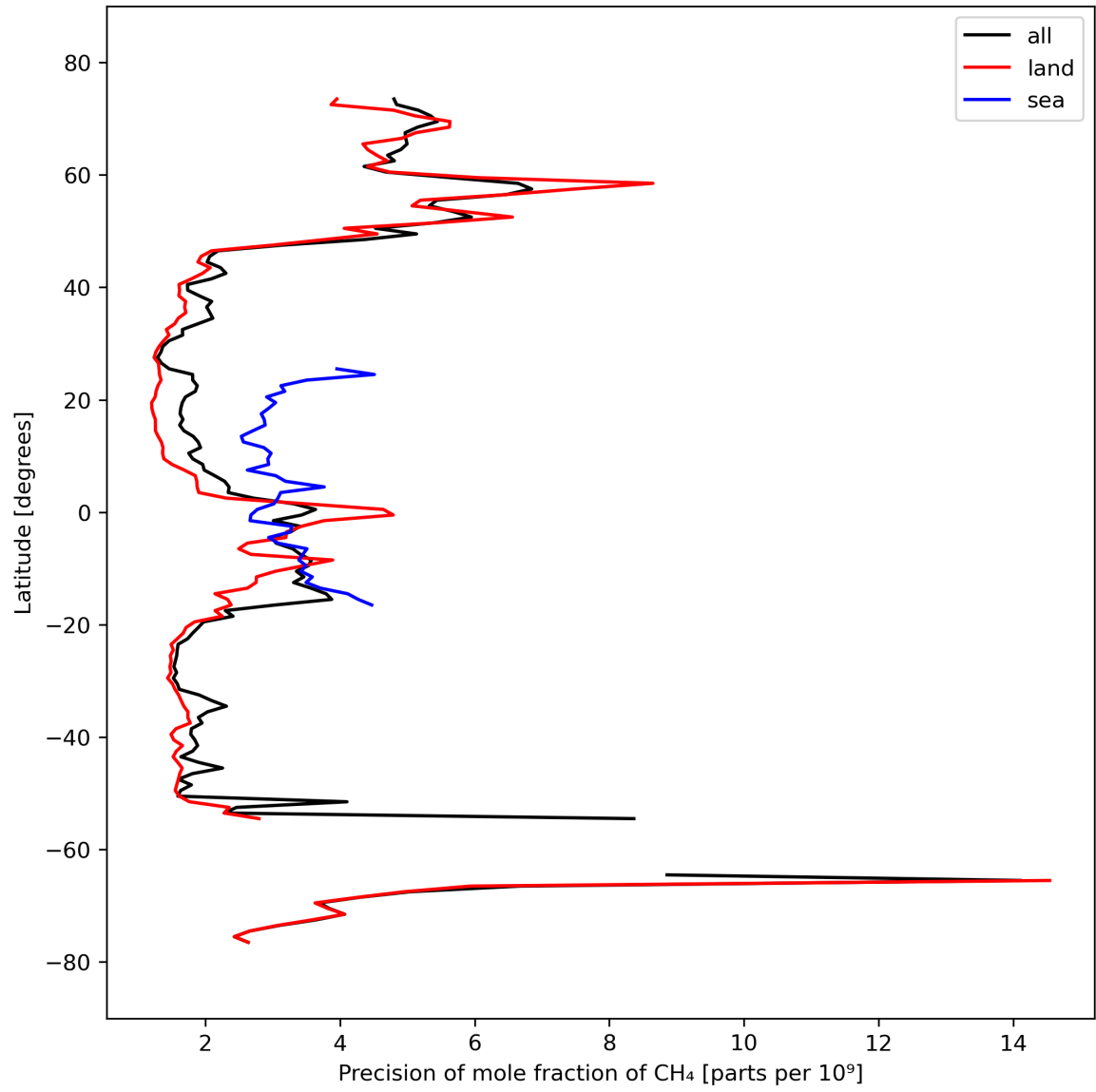
Figure 13: Zonal average of “Precision of mole fraction of CH 4 ” for 2024-03-15 to 2024-03-17.
