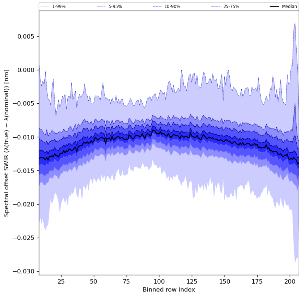
Figure 38: Along track statistics of “Spectral offset SWIR ( \lambda(\text{true}) - \lambda(\text{nominal}) )” for 2024-03-15 to 2024-03-17
