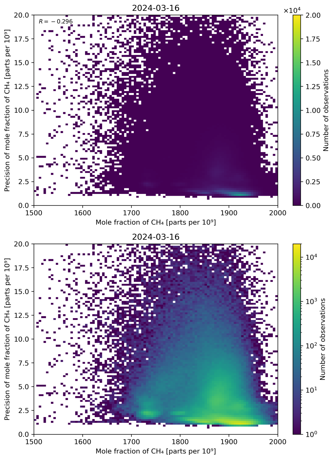
Figure 75: Scatter density plot of “Mole fraction of CH 4 ” against “Precision of mole fraction of CH 4 ” for 2024-03-15 to 2024-03-17.
