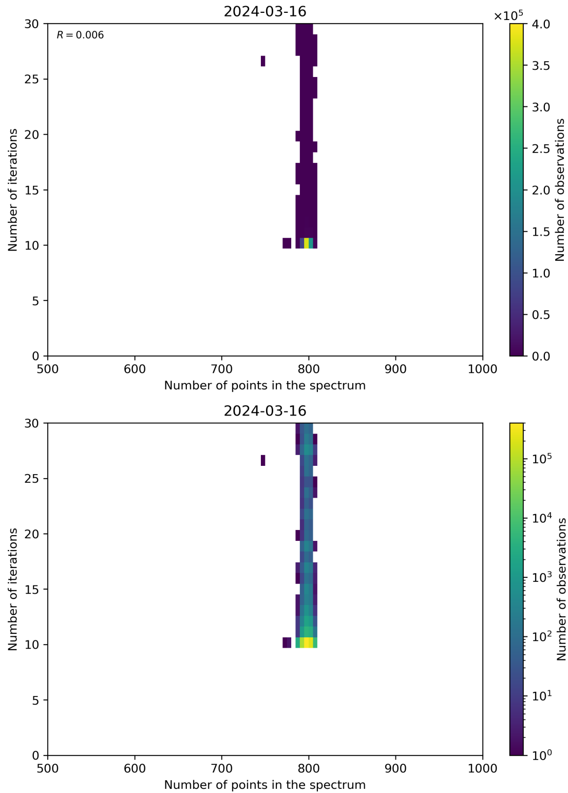
Figure 92: Scatter density plot of “Number of points in the spectrum” against “Number of iterations” for 2024-03-15 to 2024-03-17.
