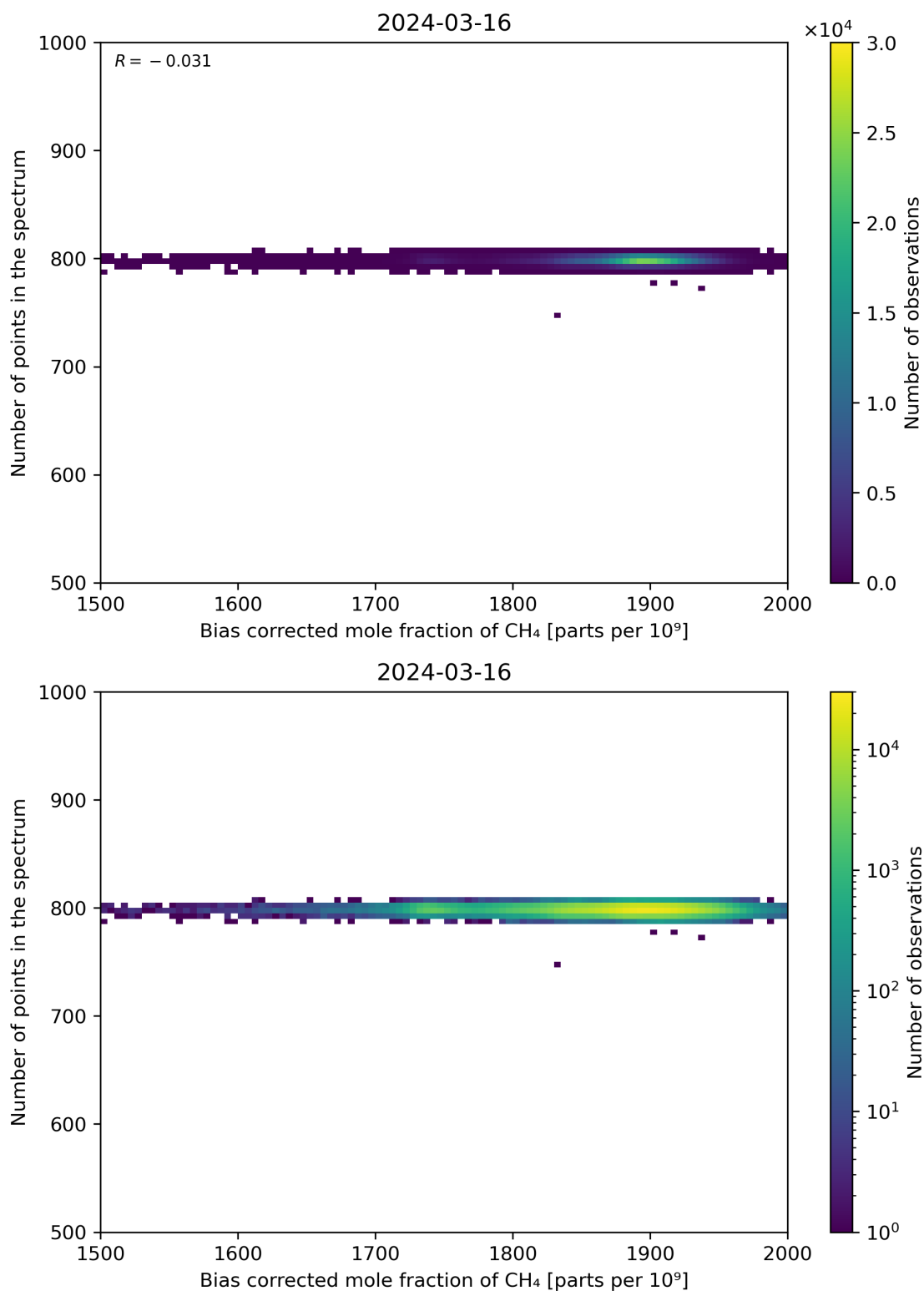
Figure 68: Scatter density plot of “Bias corrected mole fraction of CH 4 ” against “Number of points in the spectrum” for 2024-03-15 to 2024-03-17.
