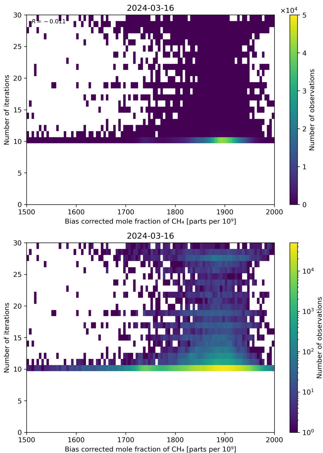
Figure 67: Scatter density plot of “Bias corrected mole fraction of CH 4 ” against “Number of iterations” for 2024-03-15 to 2024-03-17.
