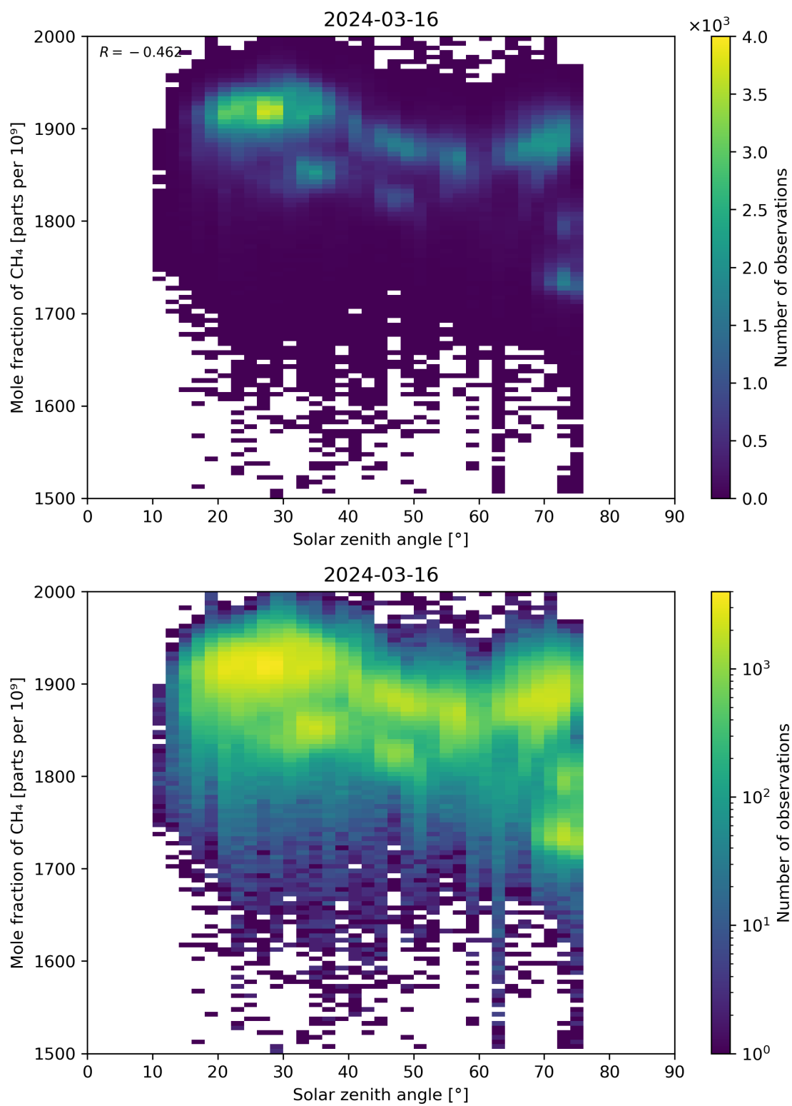
Figure 99: Scatter density plot of “Solar zenith angle” against “Mole fraction of \text{CH}_4 ” for 2024-03-15 to 2024-03-17.
