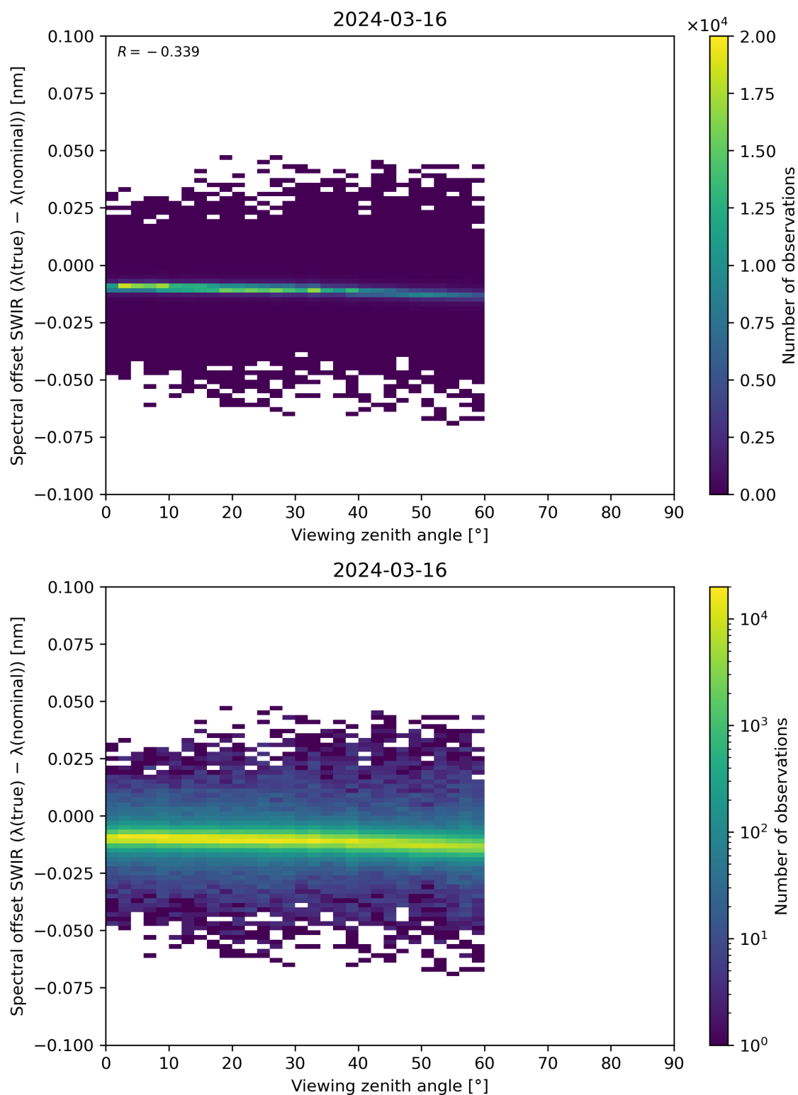
Figure 116: Scatter density plot of “Viewing zenith angle” against “Spectral offset SWIR ( \lambda(\text{true}) - \lambda(\text{nominal}) )” for 2024-03-15 to 2024-03-17.
