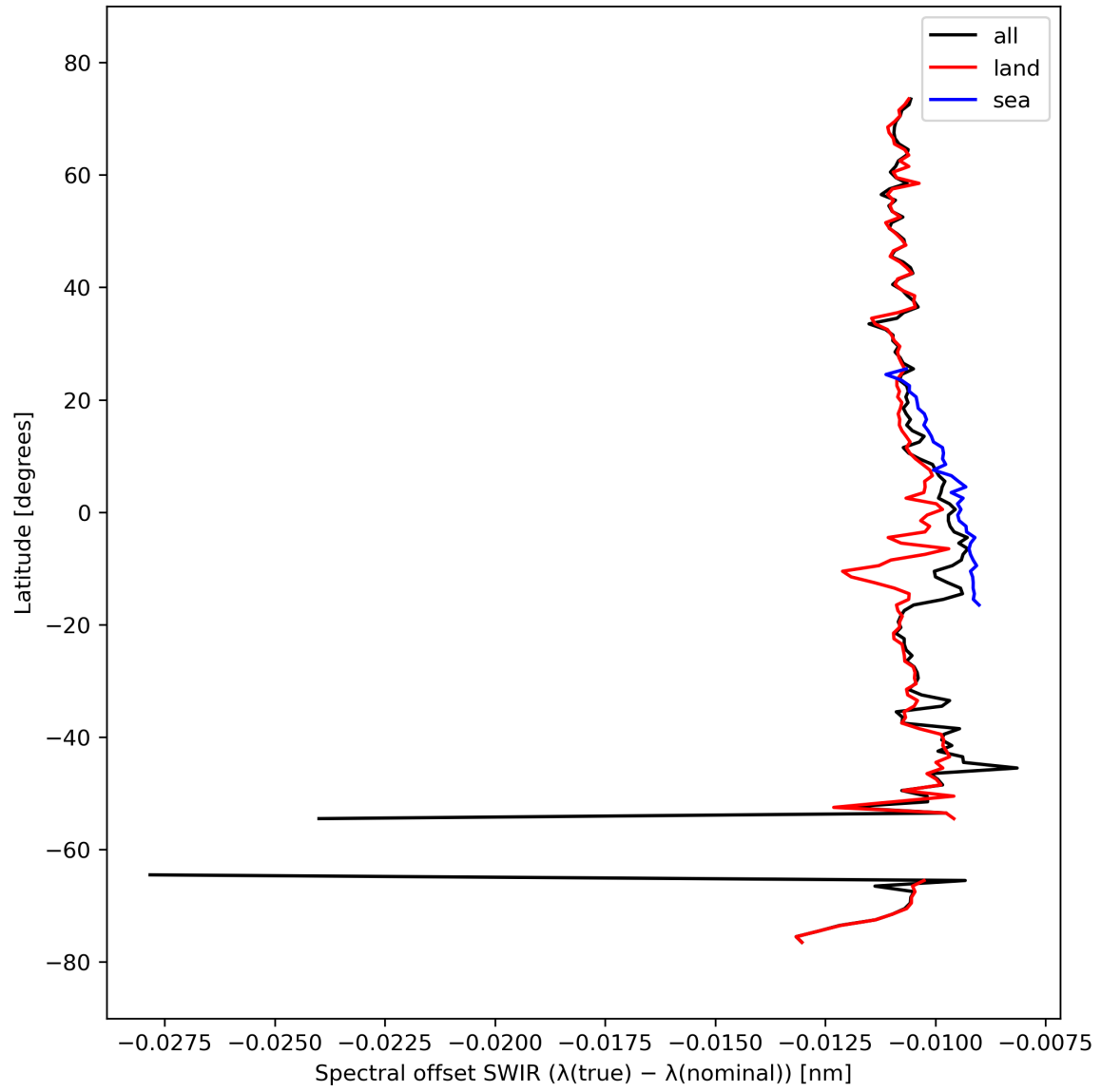
Figure 16: Zonal average of “Spectral offset SWIR ( \lambda(\text{true}) - \lambda(\text{nominal}) )” for 2024-03-15 to 2024-03-17.
