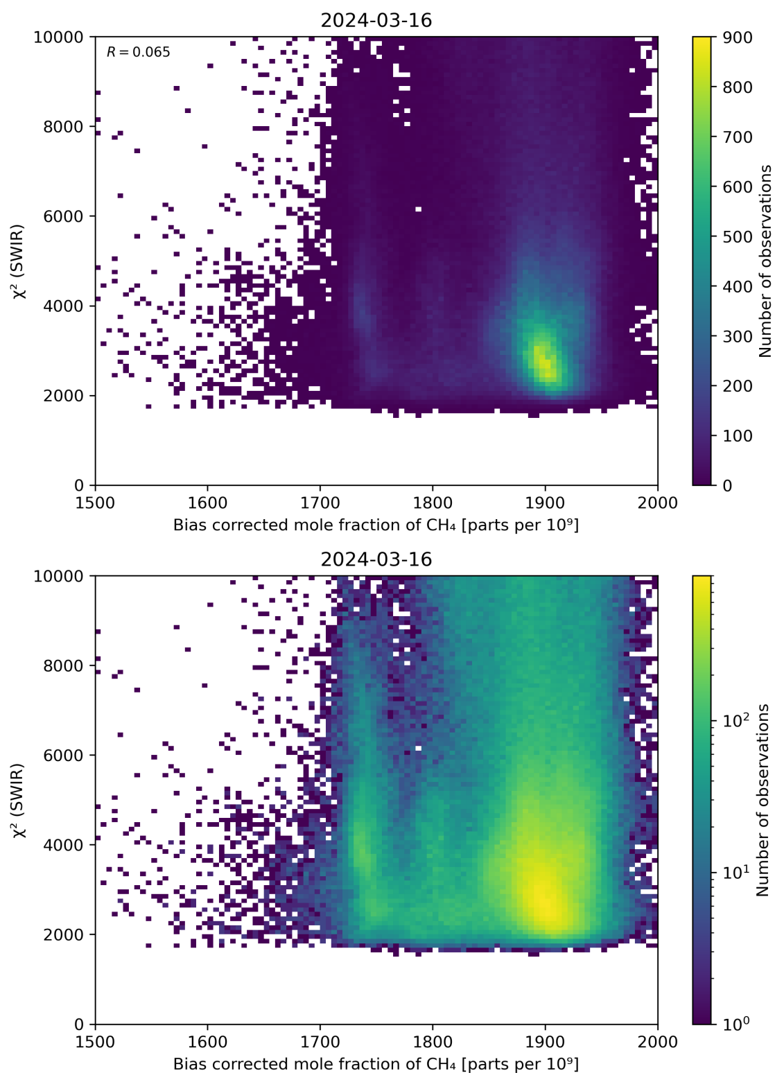
Figure 64: Scatter density plot of “Bias corrected mole fraction of CH 4 ” against “ \chi^2 (SWIR)” for 2024-03-15 to 2024-03-17.
