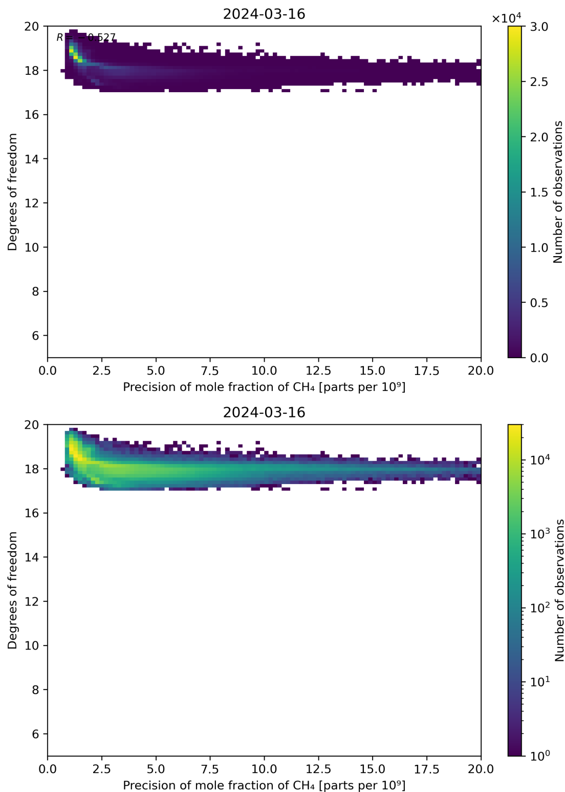
Figure 80: Scatter density plot of “Precision of mole fraction of CH 4 ” against “Degrees of freedom” for 2024-03-15 to 2024-03-17.
