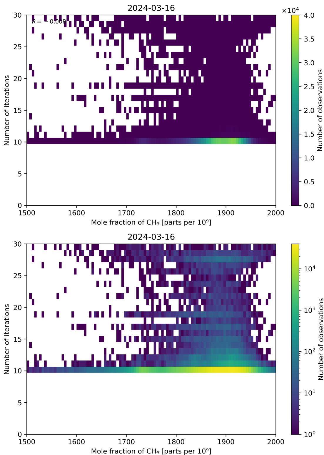
Figure 76: Scatter density plot of “Mole fraction of CH 4 ” against “Number of iterations” for 2024-03-15 to 2024-03-17.
