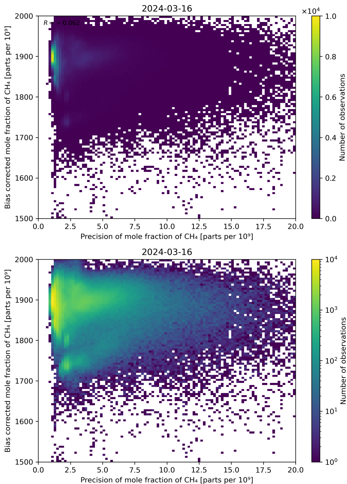
Figure 82: Scatter density plot of “Precision of mole fraction of CH 4 ” against “Bias corrected mole fraction of CH 4 ” for 2024-03-15 to 2024-03-17.
