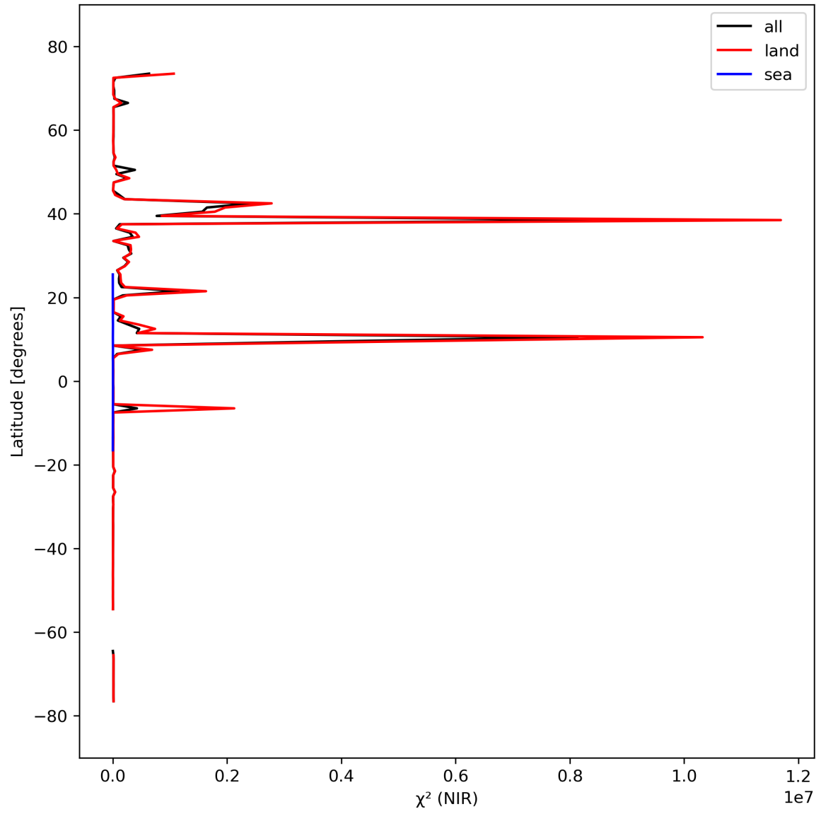
Figure 18: Zonal average of “ \chi^2 (NIR)” for 2024-03-15 to 2024-03-17.
