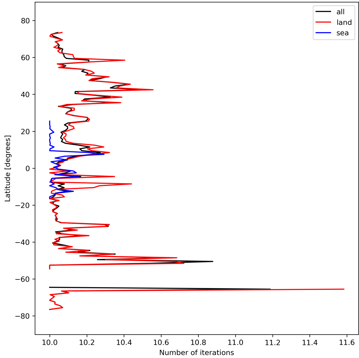
Figure 20: Zonal average of “Number of iterations” for 2024-03-15 to 2024-03-17.
