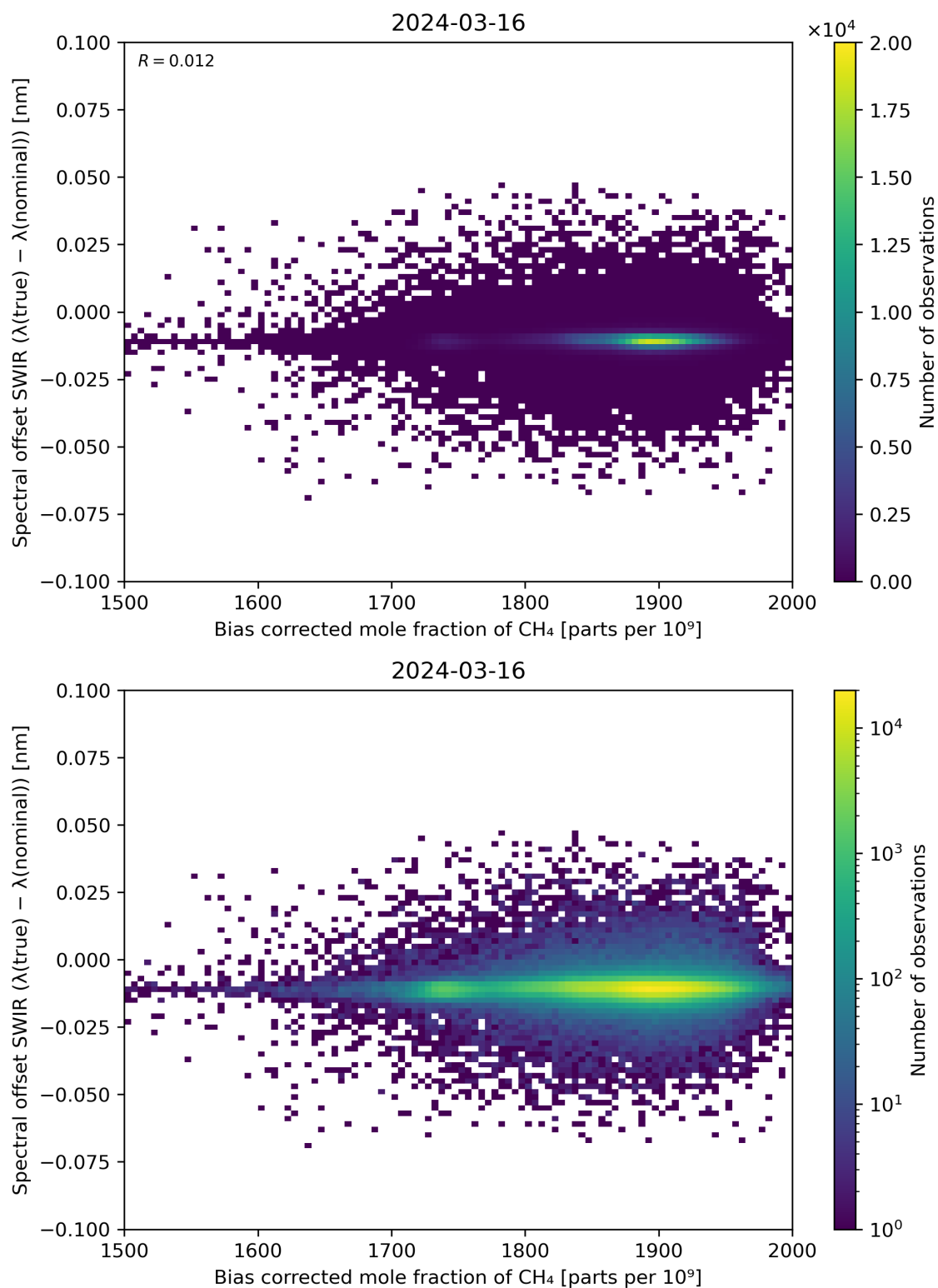
Figure 69: Scatter density plot of “Bias corrected mole fraction of \text{CH}_4 ” against “Spectral offset SWIR ( \lambda(\text{true}) - \lambda(\text{nominal}) )” for 2024-03-15 to 2024-03-17.
