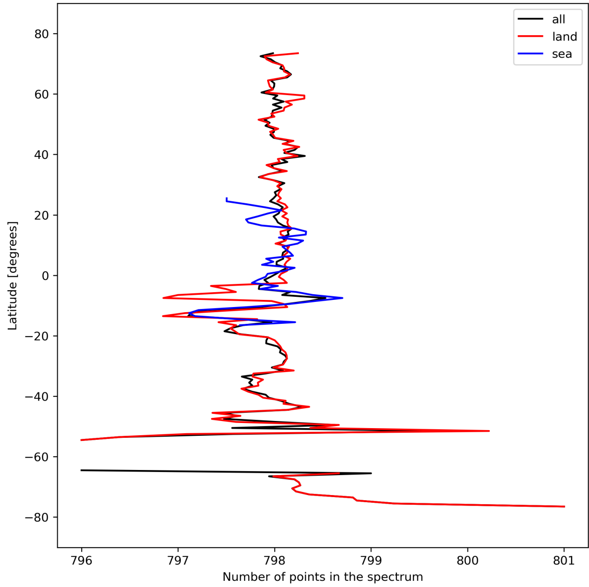
Figure 15: Zonal average of “Number of points in the spectrum” for 2024-03-15 to 2024-03-17.
