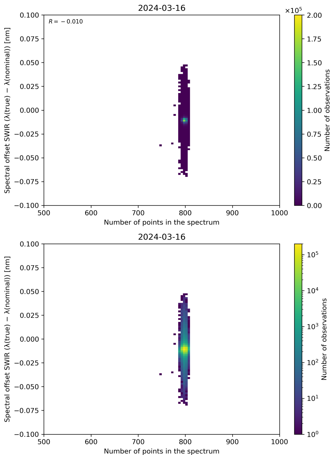
Figure 93: Scatter density plot of “Number of points in the spectrum” against “Spectral offset SWIR ( \lambda(\text{true}) - \lambda(\text{nominal}) )” for 2024-03-15 to 2024-03-17.
