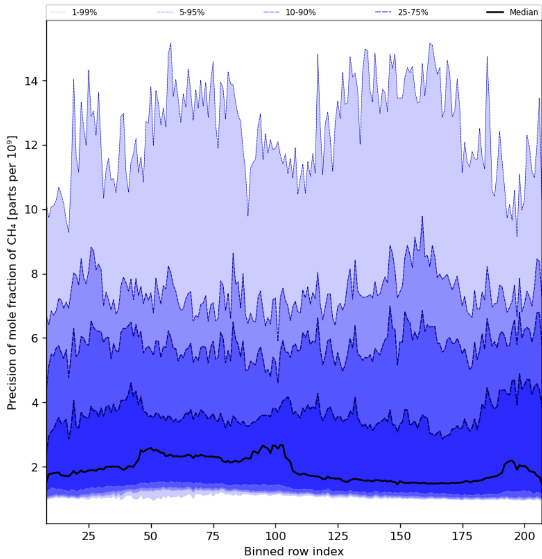
Figure 35: Along track statistics of “Precision of mole fraction of CH 4 ” for 2024-03-15 to 2024-03-17
