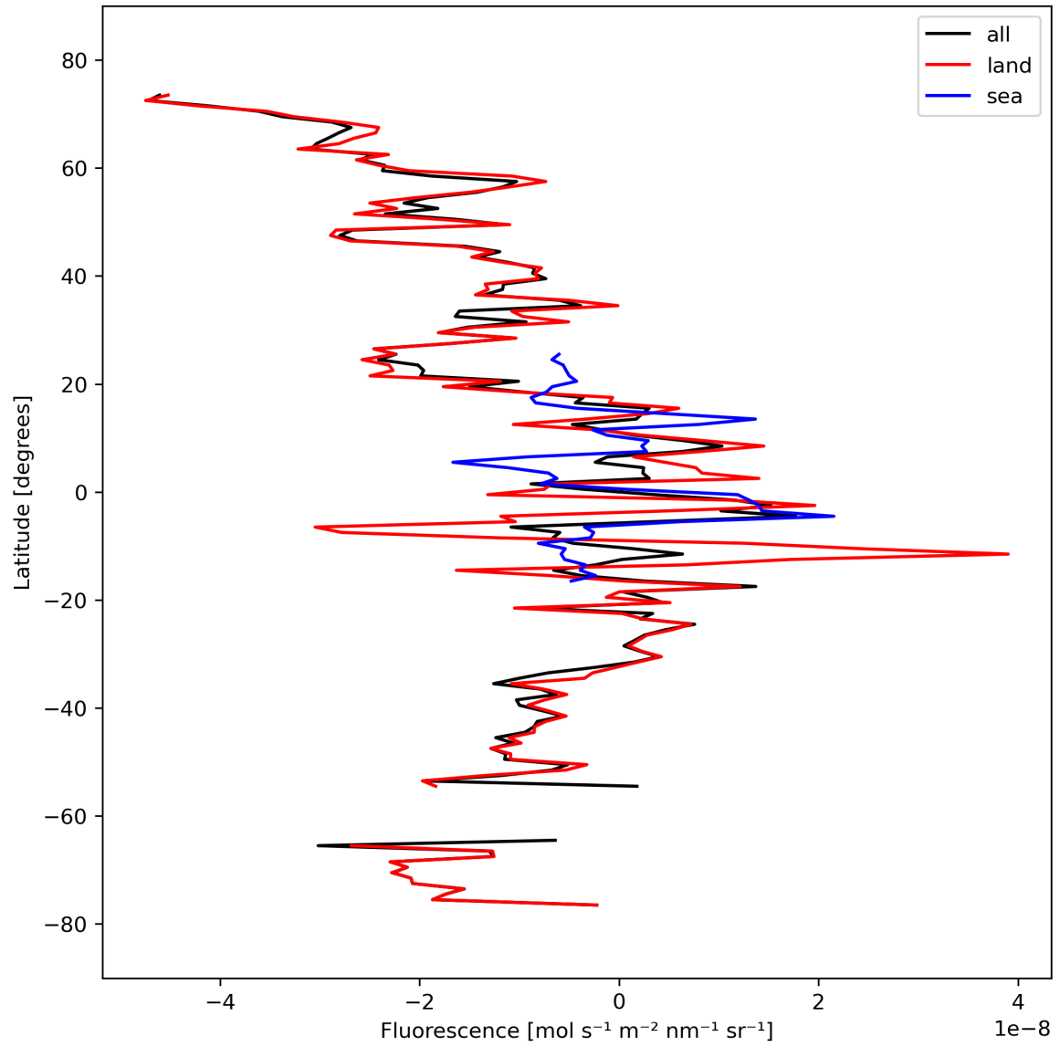
Figure 21: Zonal average of “Fluorescence” for 2024-03-15 to 2024-03-17.
