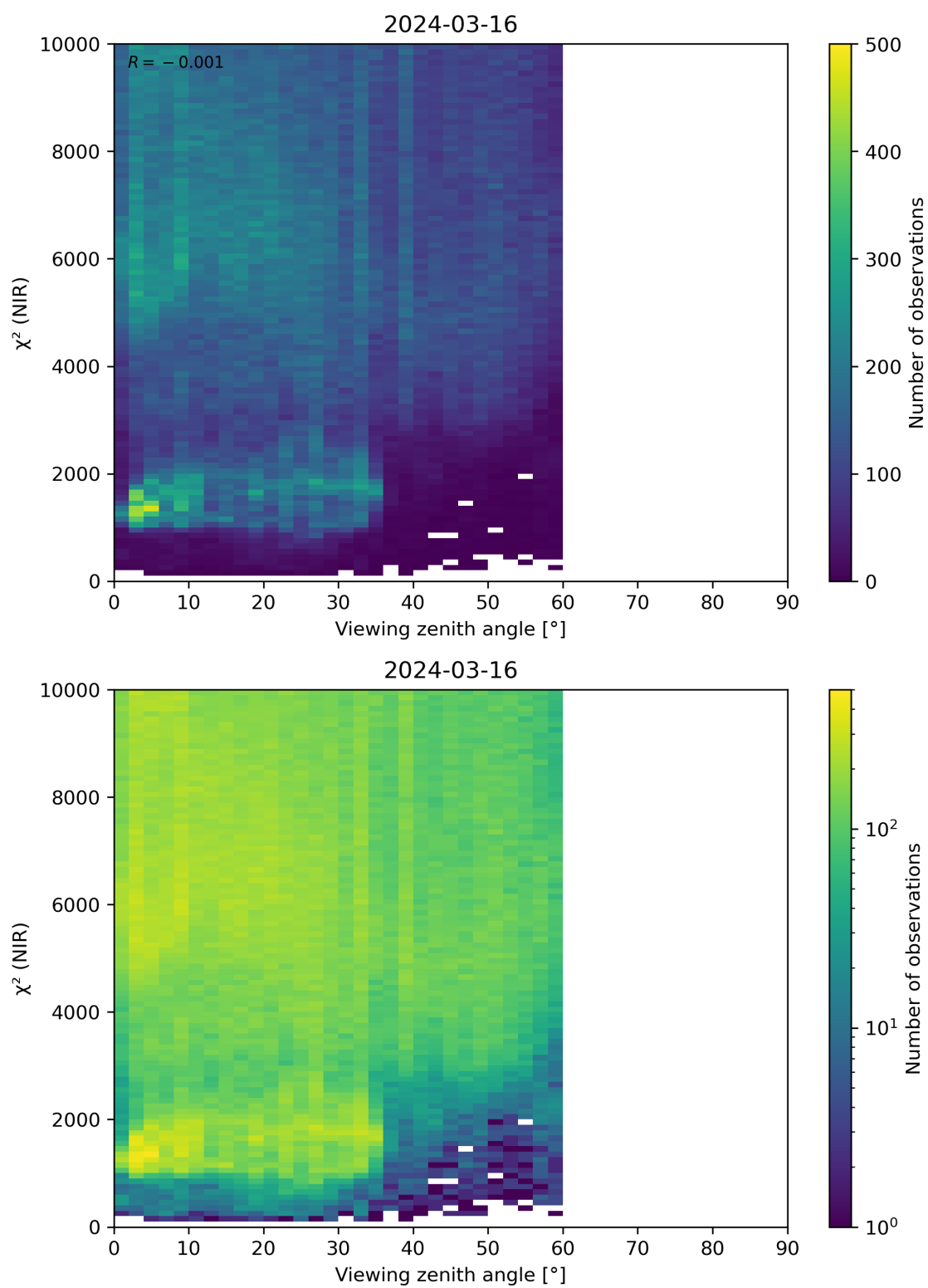
Figure 105: Scatter density plot of “Viewing zenith angle” against “ \chi^2 (NIR)” for 2024-03-15 to 2024-03-17.
