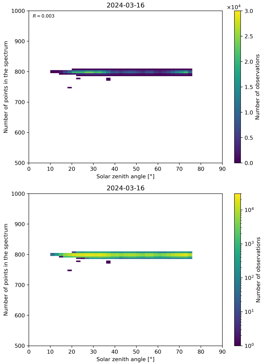
Figure 103: Scatter density plot of “Solar zenith angle” against “Number of points in the spectrum” for 2024-03-15 to 2024-03-17.
