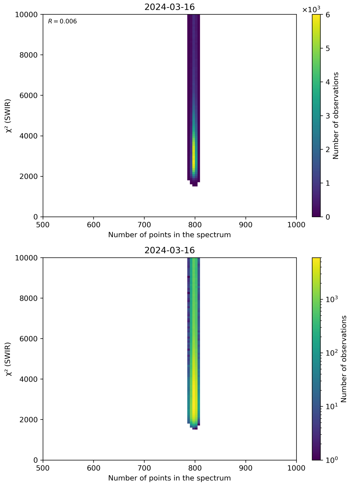
Figure 89: Scatter density plot of “Number of points in the spectrum” against “ \chi^2 (SWIR)” for 2024-03-15 to 2024-03-17.
