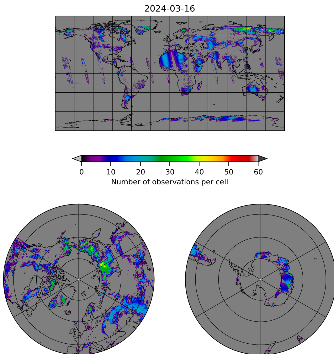
Figure 10: Map of the number of observations for 2024-03-15 to 2024-03-17
