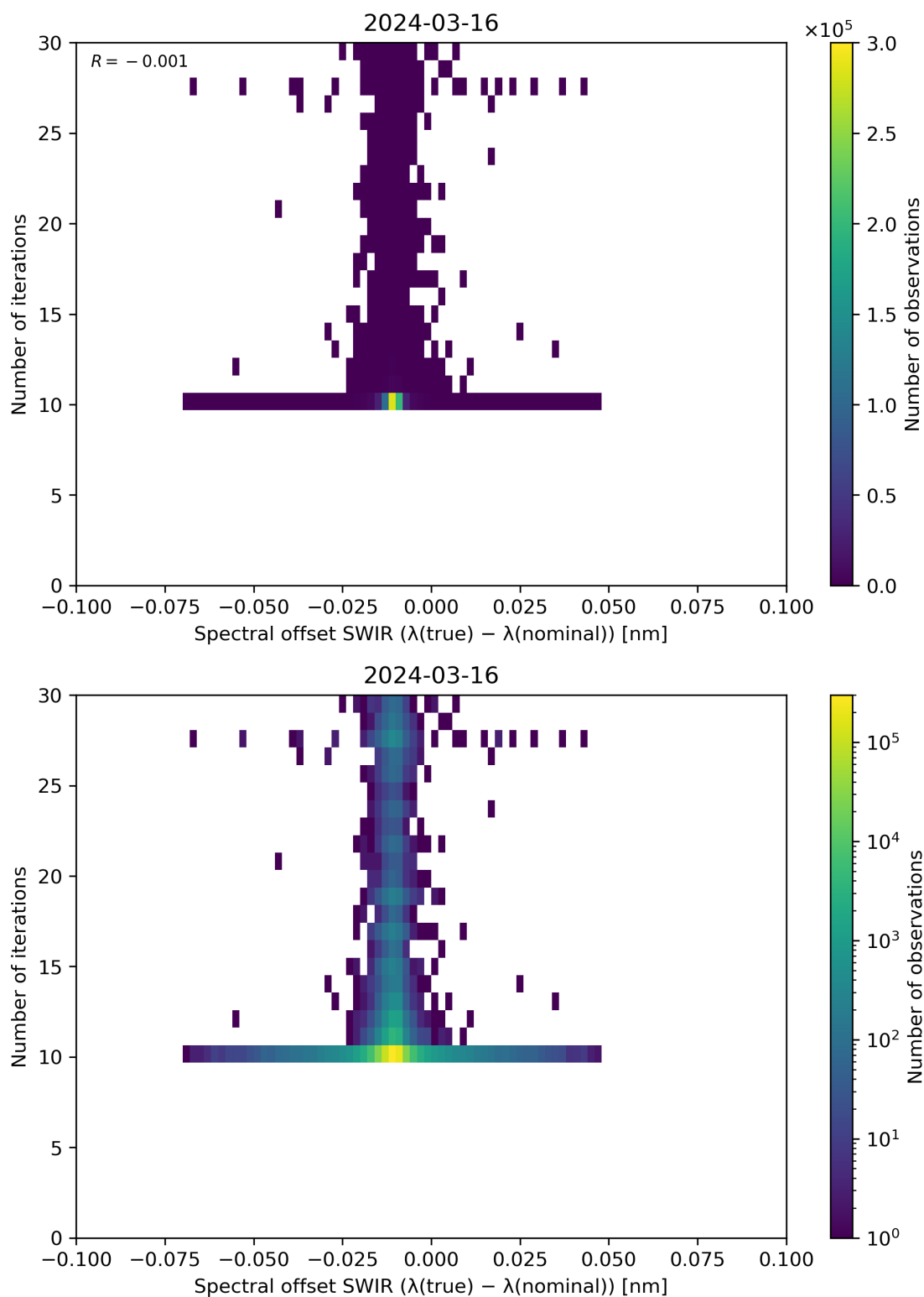
Figure 121: Scatter density plot of “Spectral offset SWIR ( \lambda(\text{true}) - \lambda(\text{nominal}) )” against “Number of iterations” for 2024-03-15 to 2024-03-17.
