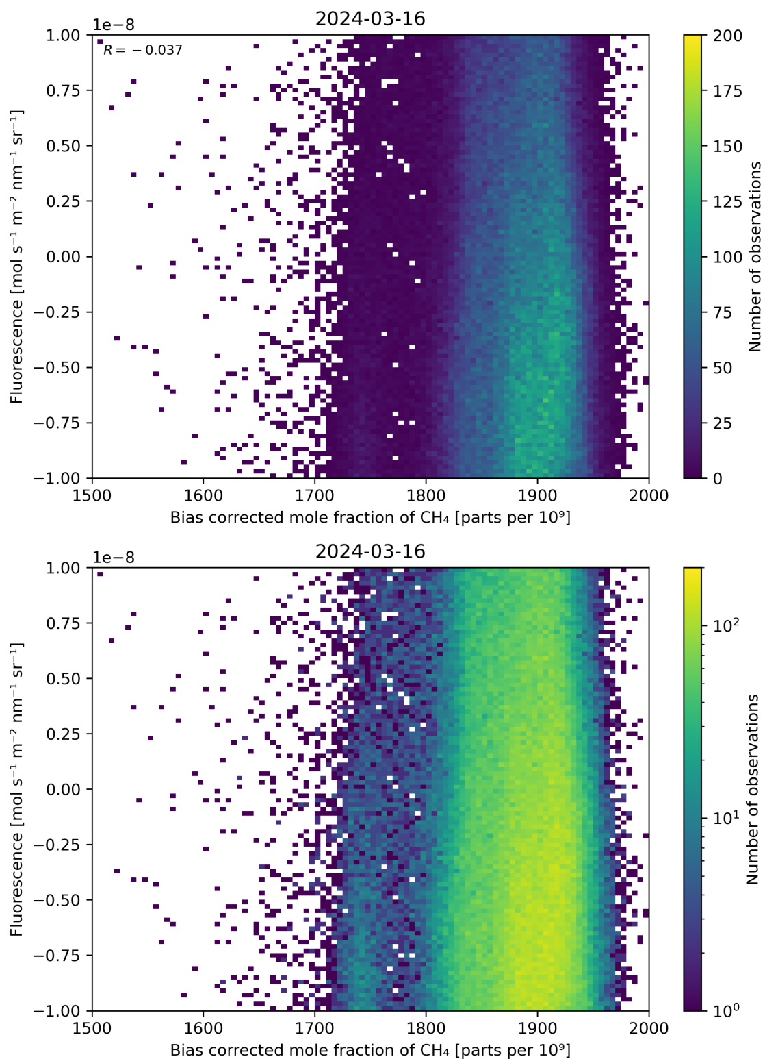
Figure 66: Scatter density plot of “Bias corrected mole fraction of \text{CH}_4 ” against “Fluorescence” for 2024-03-15 to 2024-03-17.
