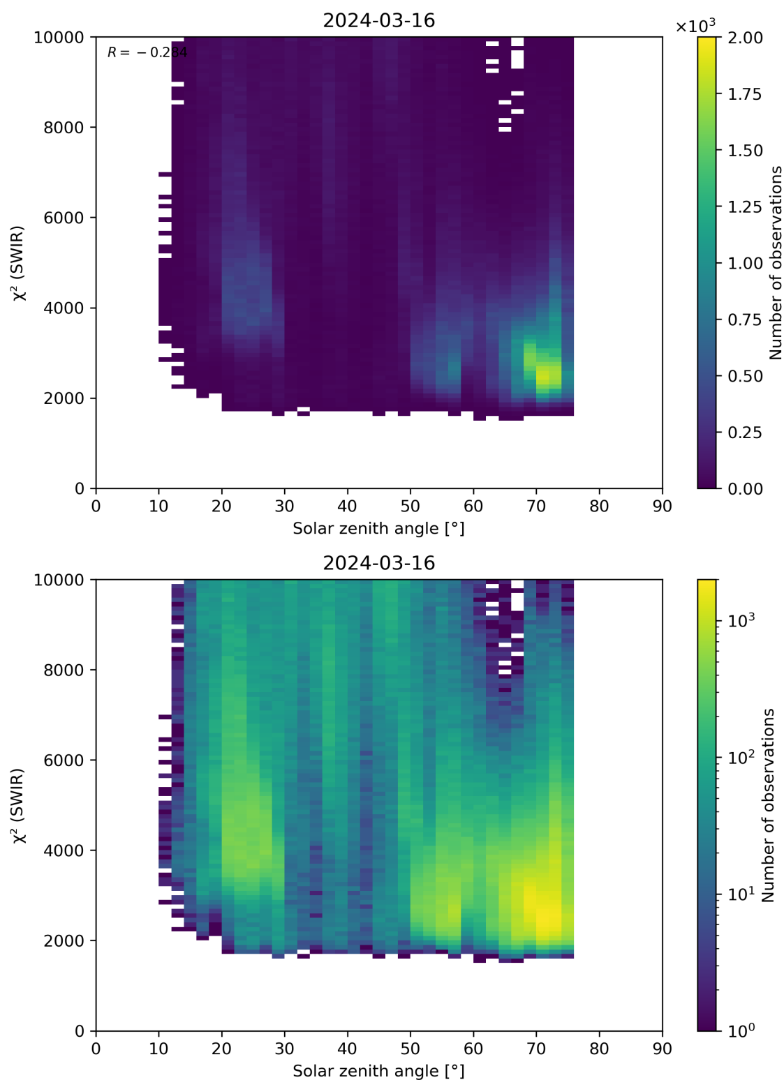
Figure 95: Scatter density plot of “Solar zenith angle” against “ \chi^2 (SWIR)” for 2024-03-15 to 2024-03-17.
