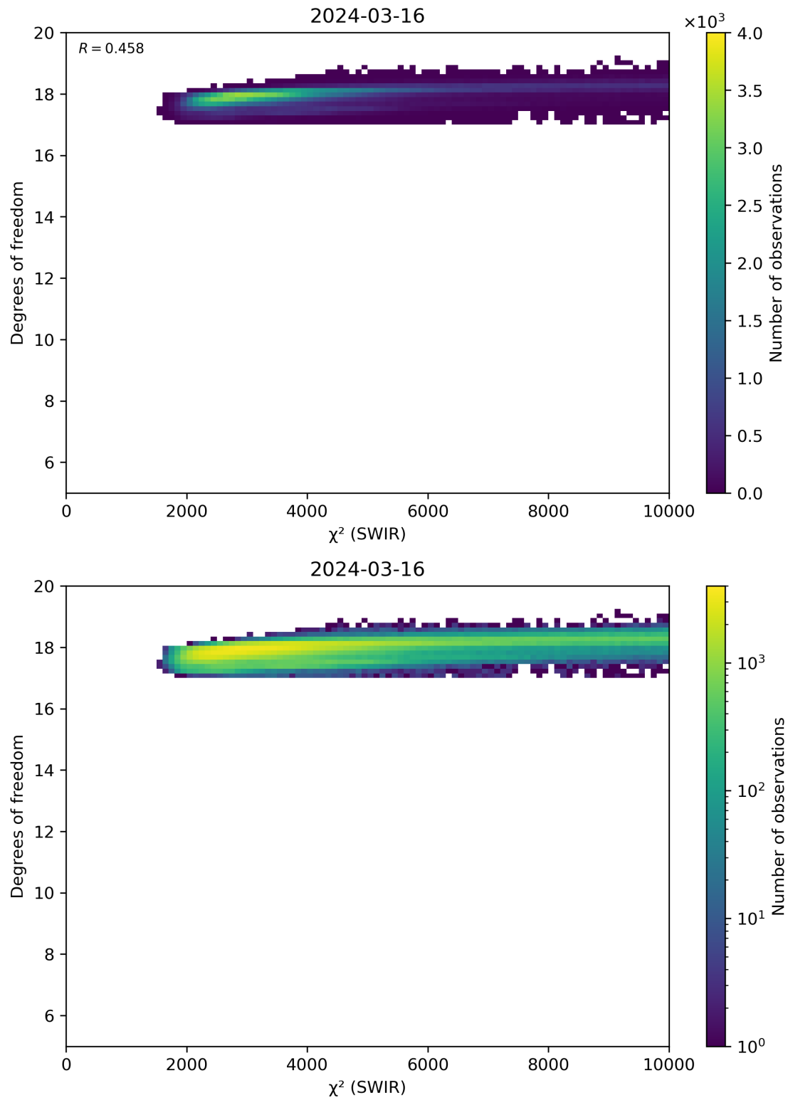
Figure 48: Scatter density plot of “ \chi^2 (SWIR)” against “Degrees of freedom” for 2024-03-15 to 2024-03-17.
