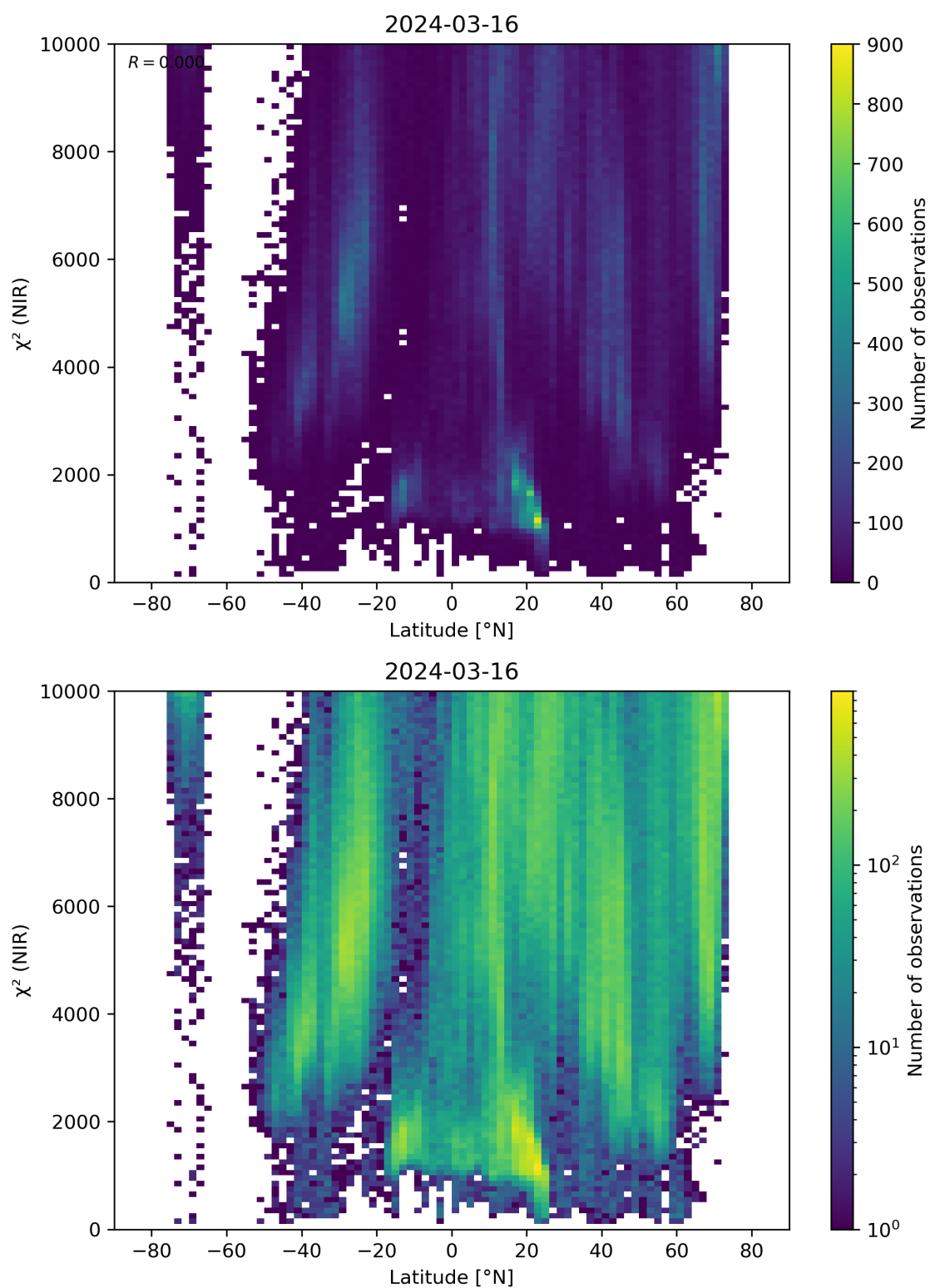
Figure 53: Scatter density plot of “Latitude” against “ \chi^2 (NIR)” for 2024-03-15 to 2024-03-17.
