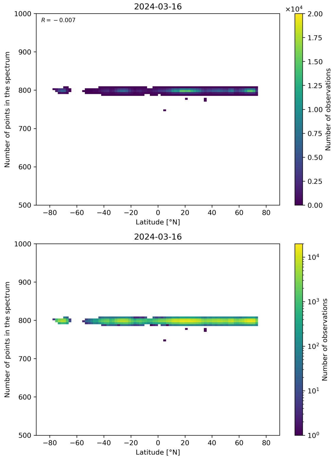
Figure 61: Scatter density plot of “Latitude” against “Number of points in the spectrum” for 2024-03-15 to 2024-03-17.
