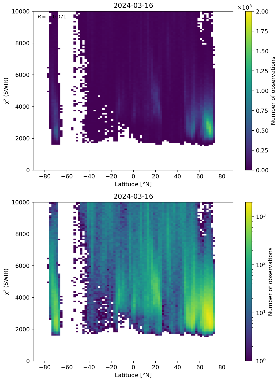
Figure 54: Scatter density plot of “Latitude” against “ \chi^2 (SWIR)” for 2024-03-15 to 2024-03-17.
