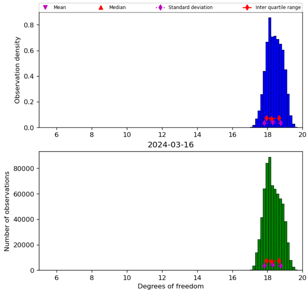
Figure 30: Histogram of “Degrees of freedom” for 2024-03-15 to 2024-03-17
