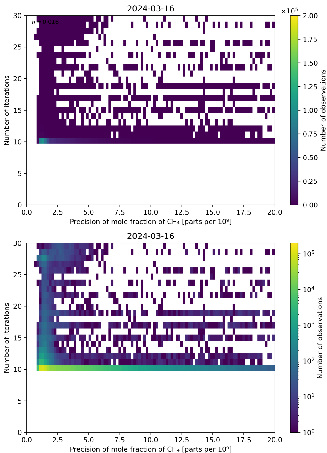
Figure 83: Scatter density plot of “Precision of mole fraction of CH 4 ” against “Number of iterations” for 2024-03-15 to 2024-03-17.
