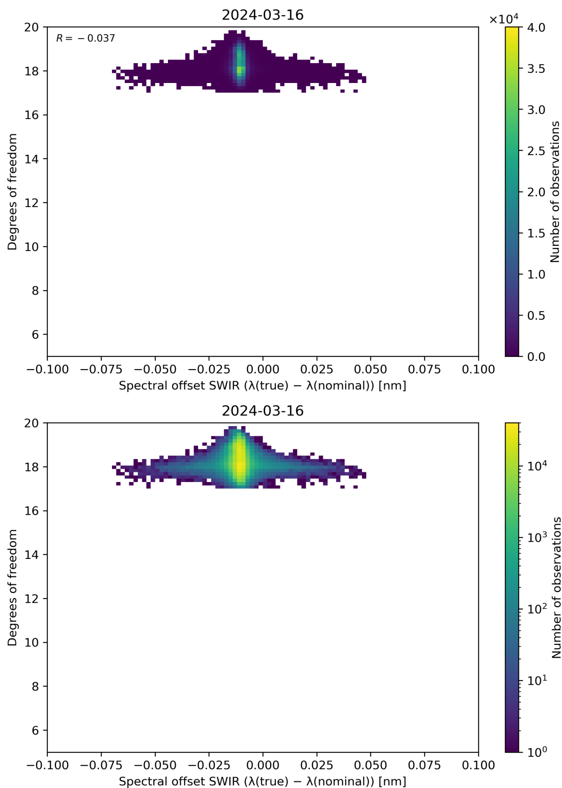
Figure 119: Scatter density plot of “Spectral offset SWIR ( \lambda(\text{true}) - \lambda(\text{nominal}) )” against “Degrees of freedom” for 2024-03-15 to 2024-03-17.
