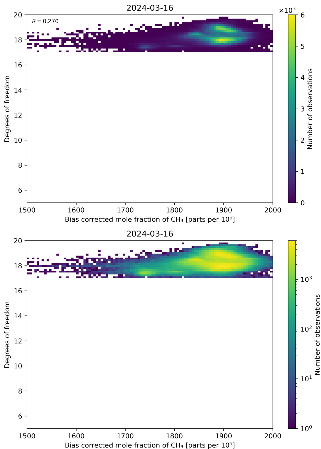
Figure 65: Scatter density plot of “Bias corrected mole fraction of CH 4 ” against “Degrees of freedom” for 2024-03-15 to 2024-03-17.
