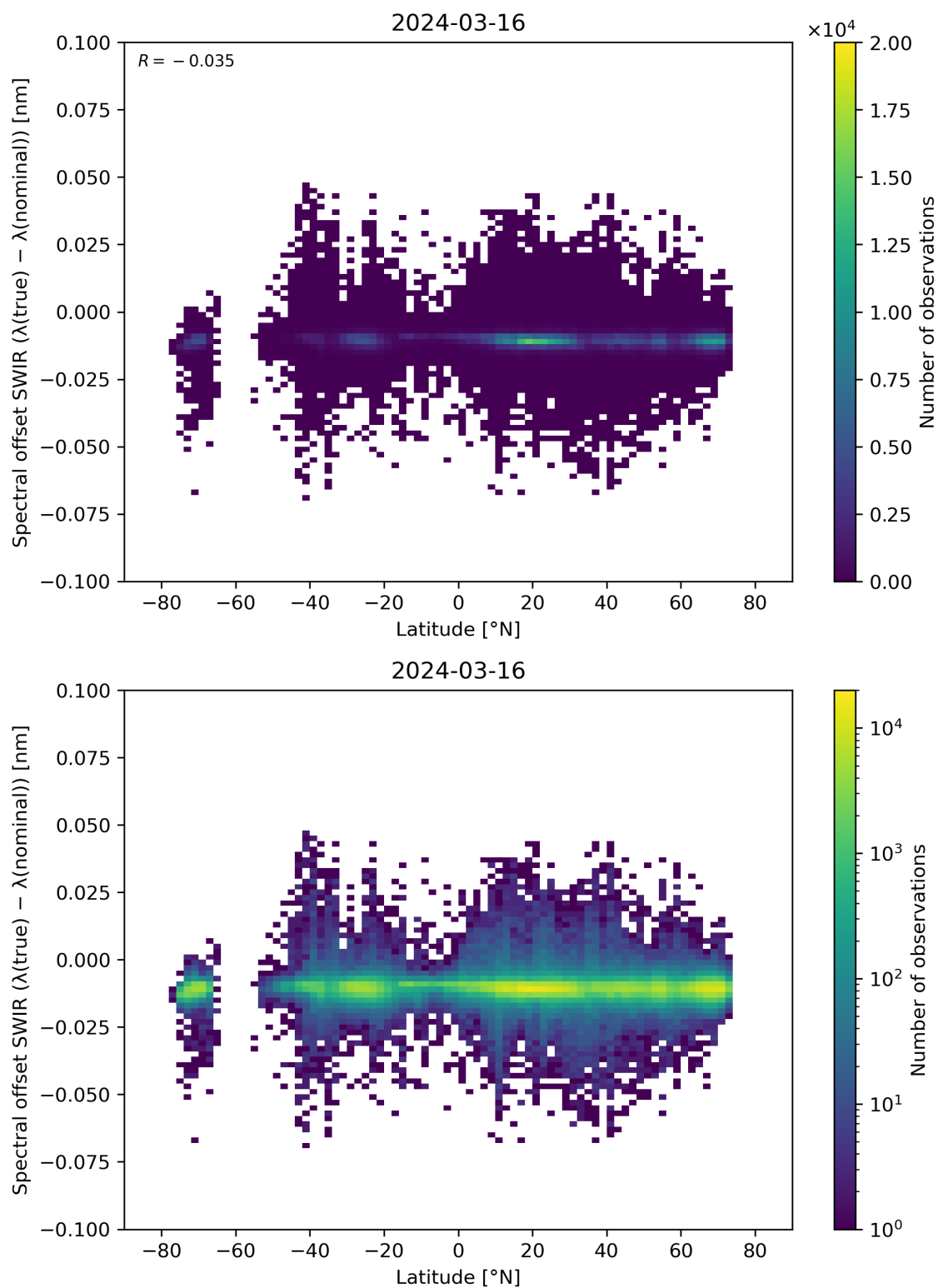
Figure 62: Scatter density plot of “Latitude” against “Spectral offset SWIR ( \lambda(\text{true}) - \lambda(\text{nominal}) )” for 2024-03-15 to 2024-03-17.
