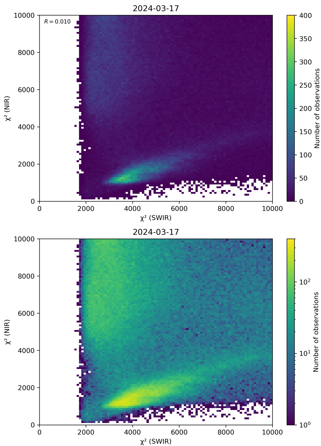
Figure 47: Scatter density plot of “ \chi^2 (SWIR)” against “ \chi^2 (NIR)” for 2024-03-16 to 2024-03-18.
