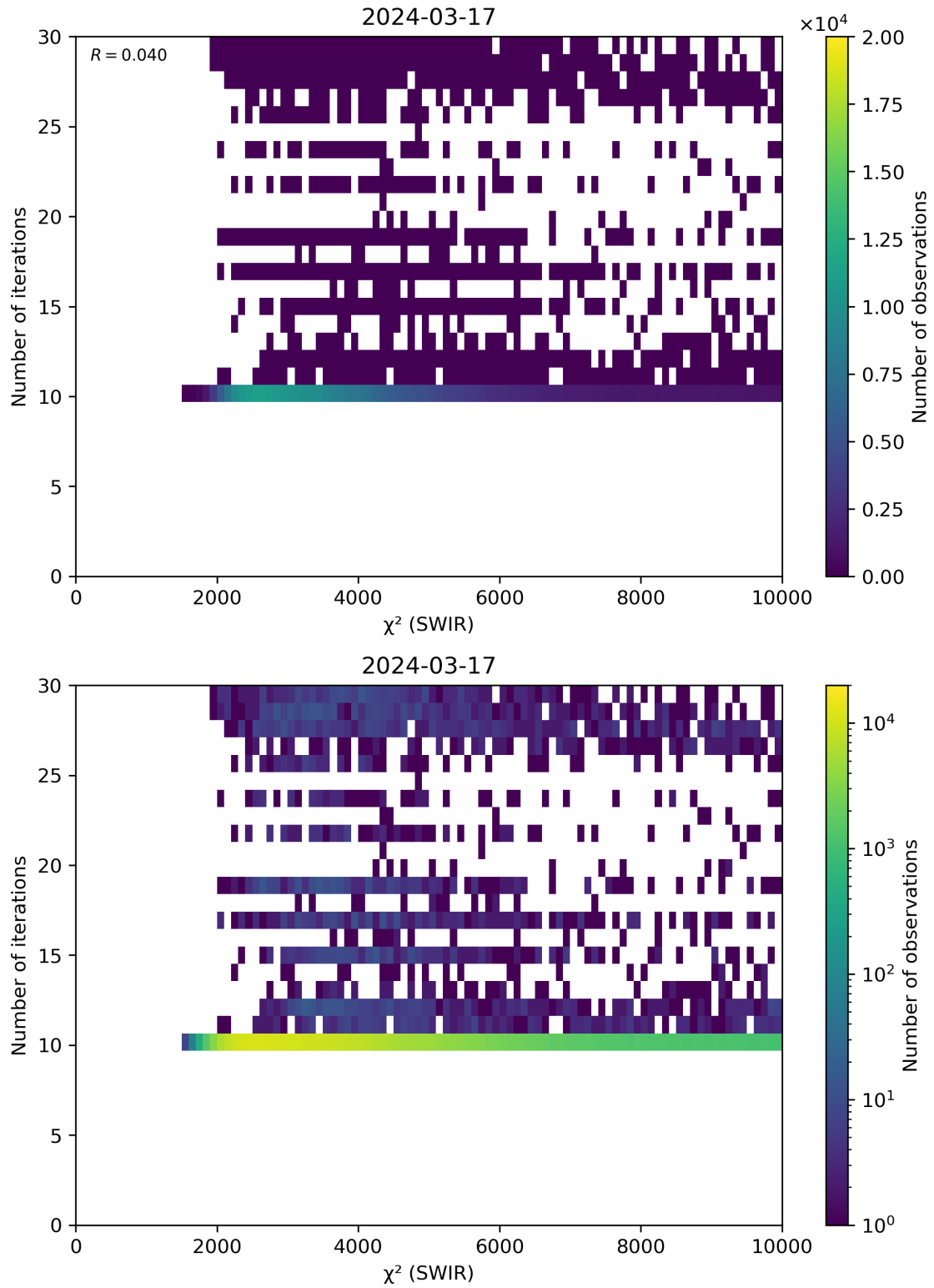
Figure 50: Scatter density plot of " \chi^2 (SWIR)" against "Number of iterations" for 2024-03-16 to 2024-03-18.
