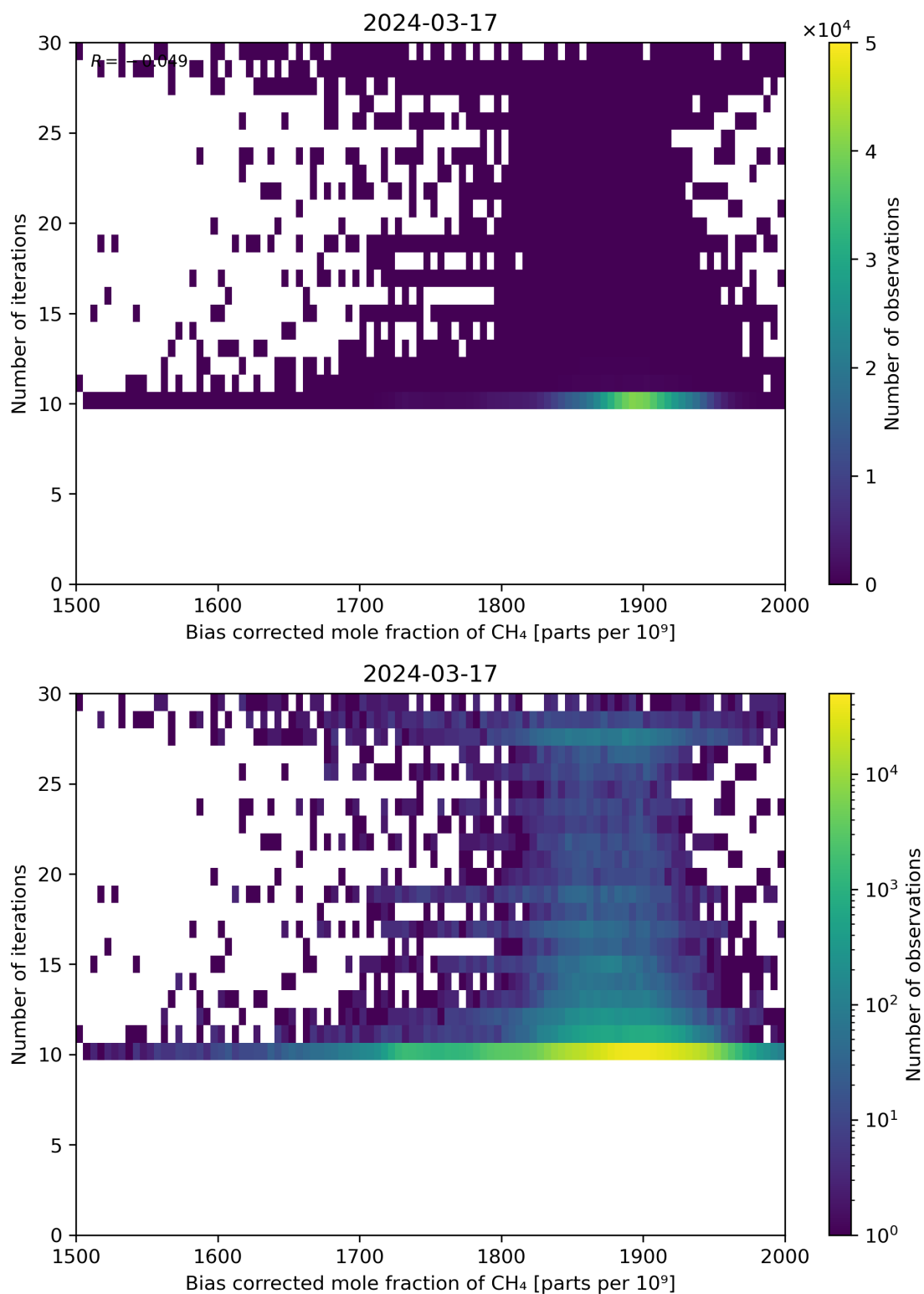
Figure 67: Scatter density plot of “Bias corrected mole fraction of CH 4 ” against “Number of iterations” for 2024-03-16 to 2024-03-18.
