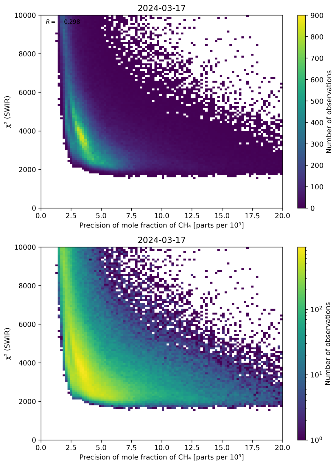
Figure 79: Scatter density plot of “Precision of mole fraction of \text{CH}_4 ” against “ \chi^2 (SWIR)” for 2024-03-16 to 2024-03-18.
