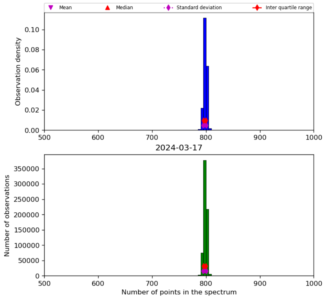
Figure 26: Histogram of “Number of points in the spectrum” for 2024-03-16 to 2024-03-18
