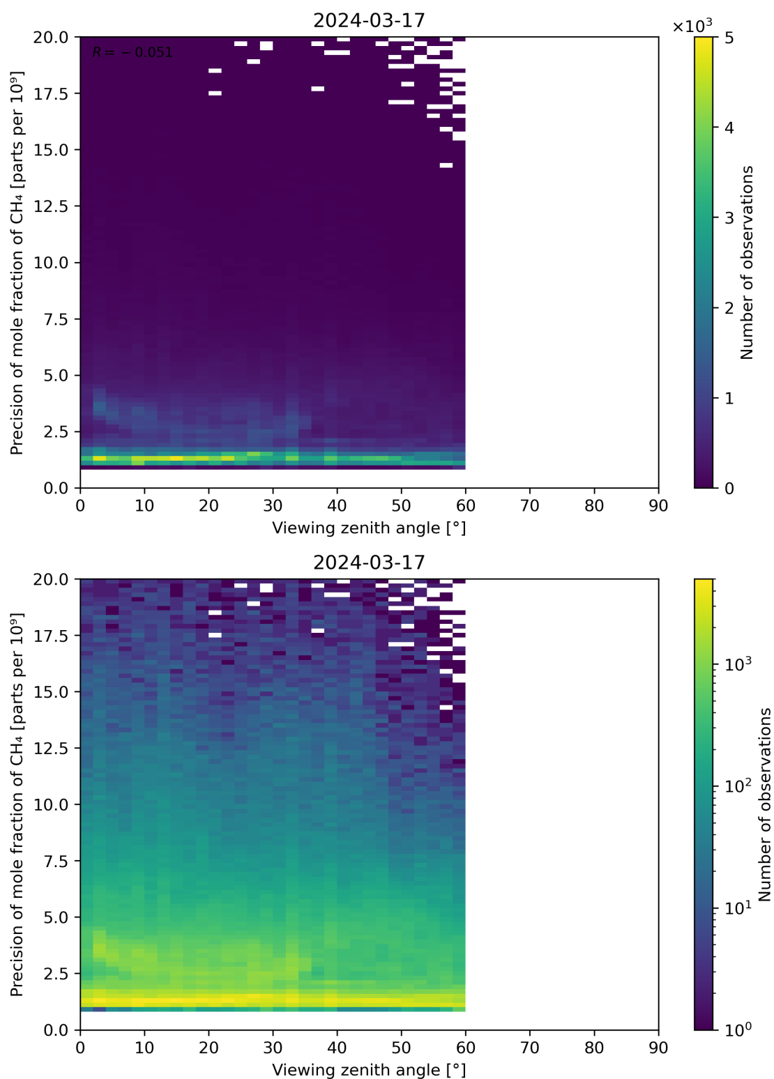
Figure 112: Scatter density plot of “Viewing zenith angle” against “Precision of mole fraction of CH 4 ” for 2024-03-16 to 2024-03-18.
