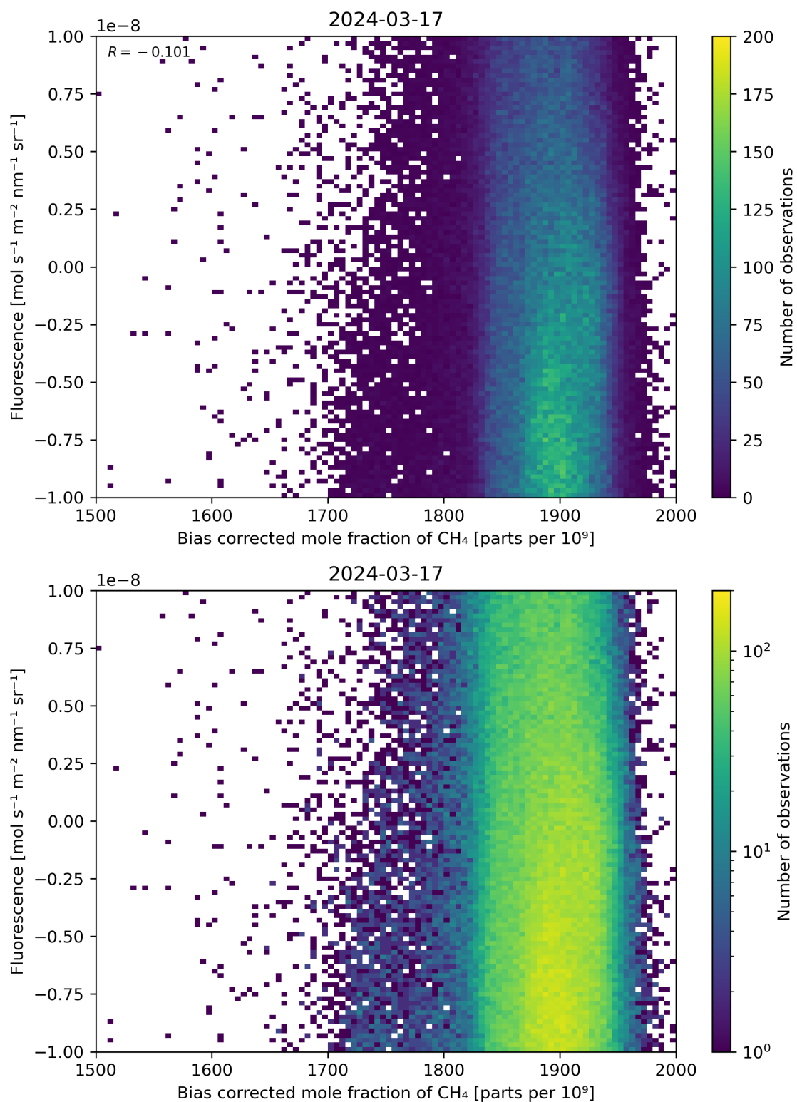
Figure 66: Scatter density plot of “Bias corrected mole fraction of \text{CH}_4 ” against “Fluorescence” for 2024-03-16 to 2024-03-18.
