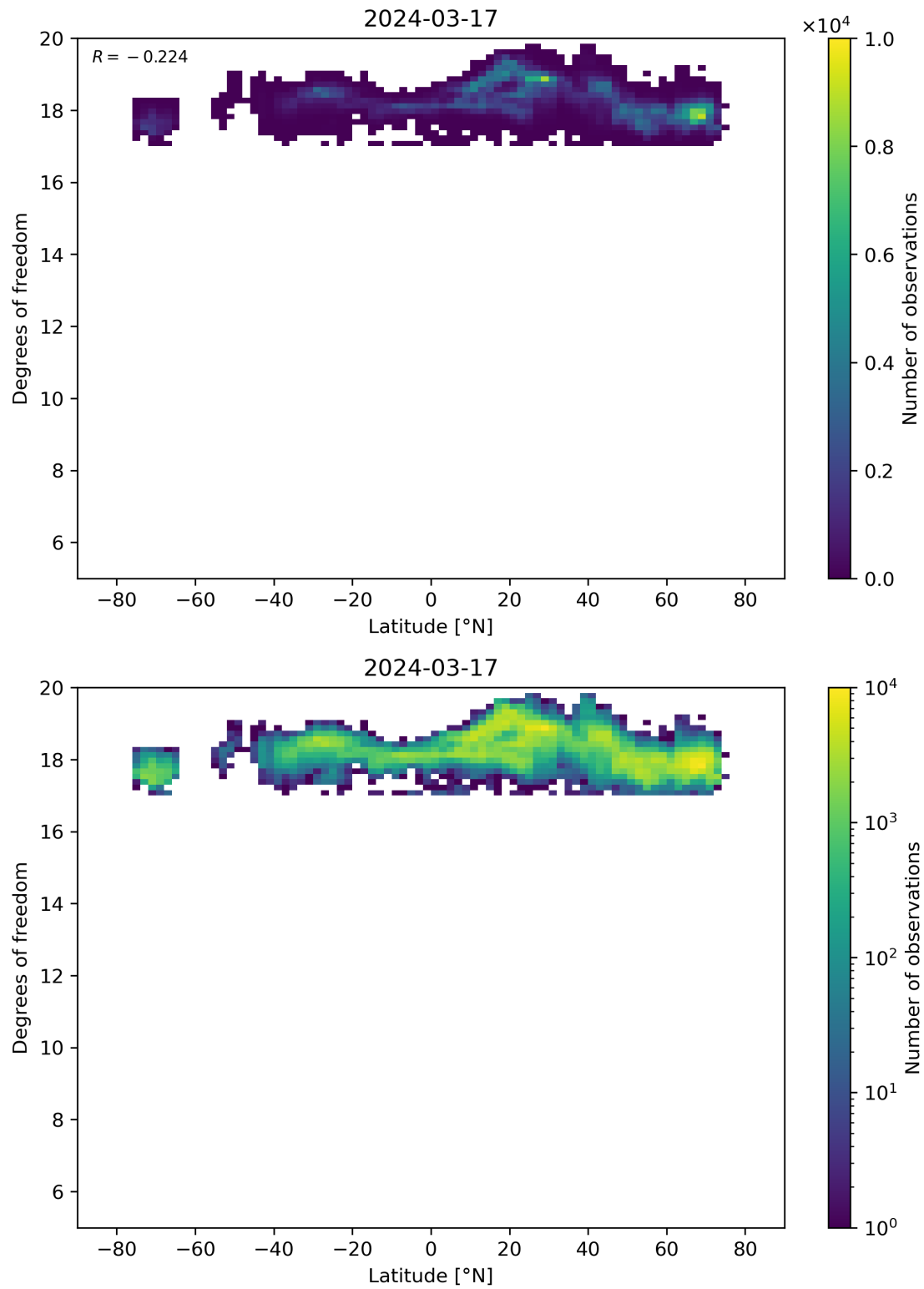
Figure 55: Scatter density plot of “Latitude” against “Degrees of freedom” for 2024-03-16 to 2024-03-18.
