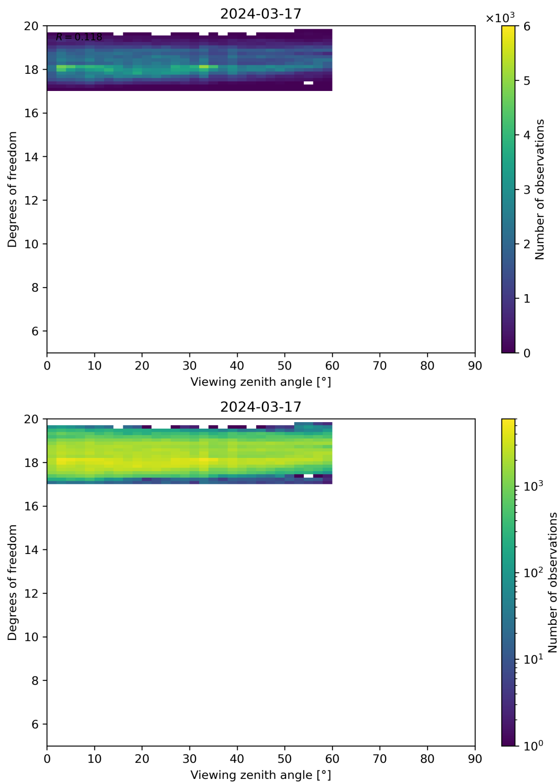
Figure 107: Scatter density plot of “Viewing zenith angle” against “Degrees of freedom” for 2024-03-16 to 2024-03-18.
