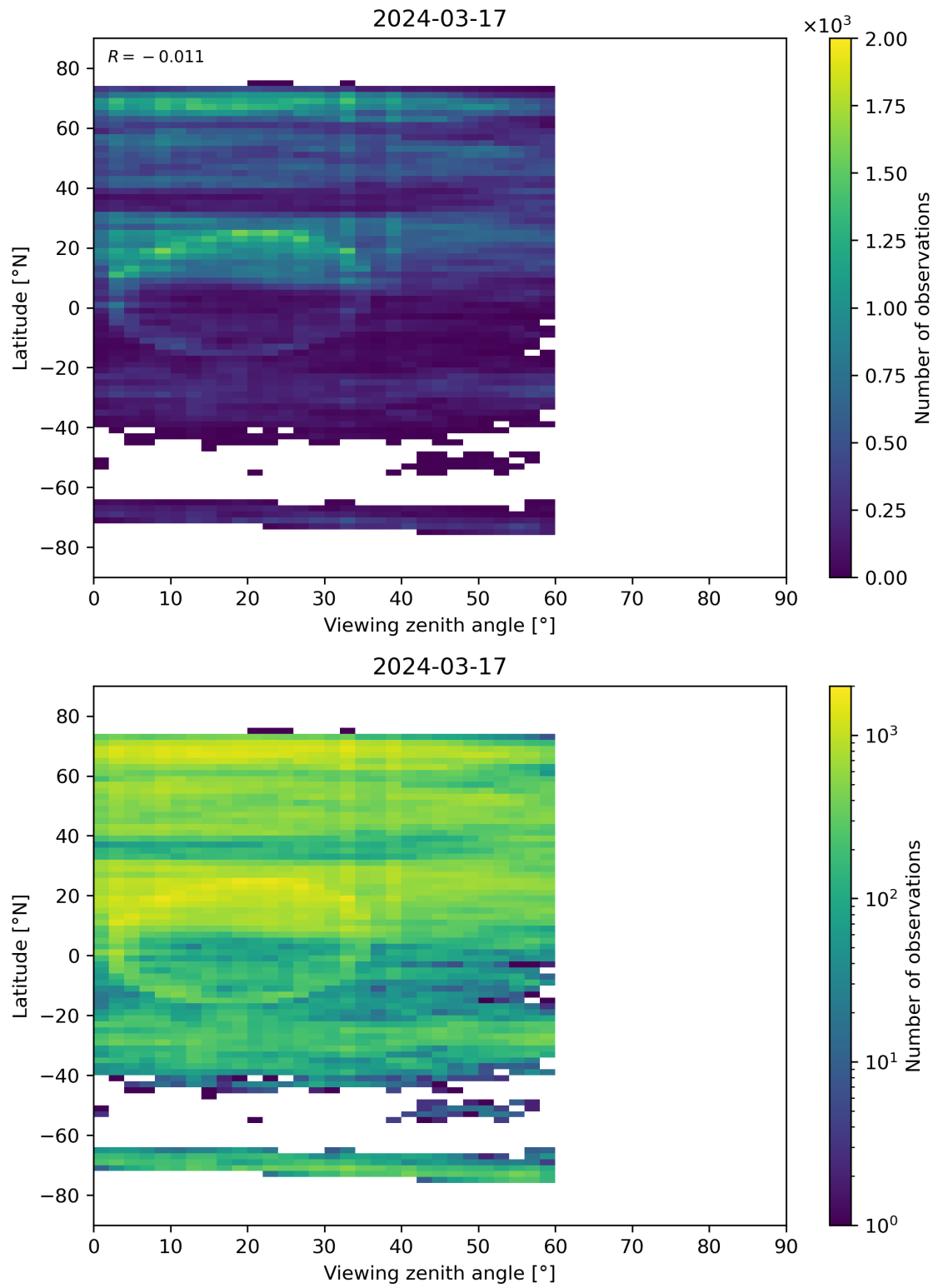
Figure 109: Scatter density plot of “Viewing zenith angle” against “Latitude” for 2024-03-16 to 2024-03-18.
