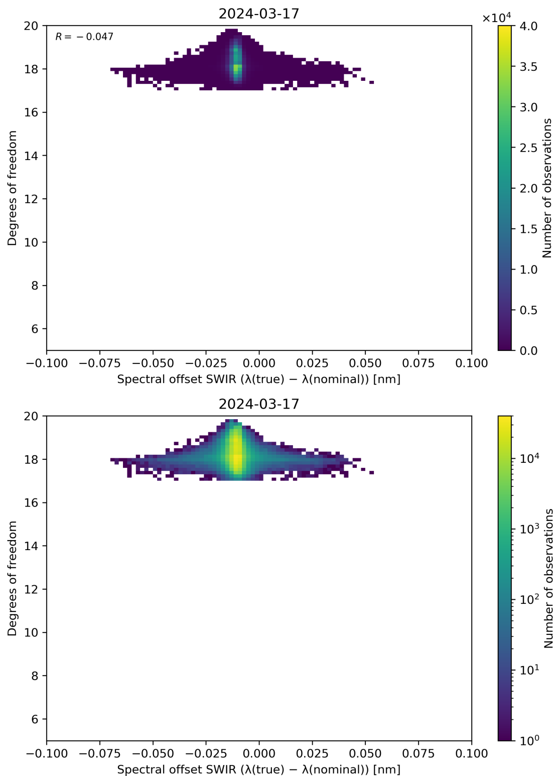
Figure 119: Scatter density plot of “Spectral offset SWIR ( \lambda(\text{true}) - \lambda(\text{nominal}) )” against “Degrees of freedom” for 2024-03-16 to 2024-03-18.
