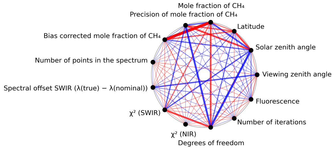
Figure 1: Map of correlation graph for 2024-03-16 to 2024-03-18.
