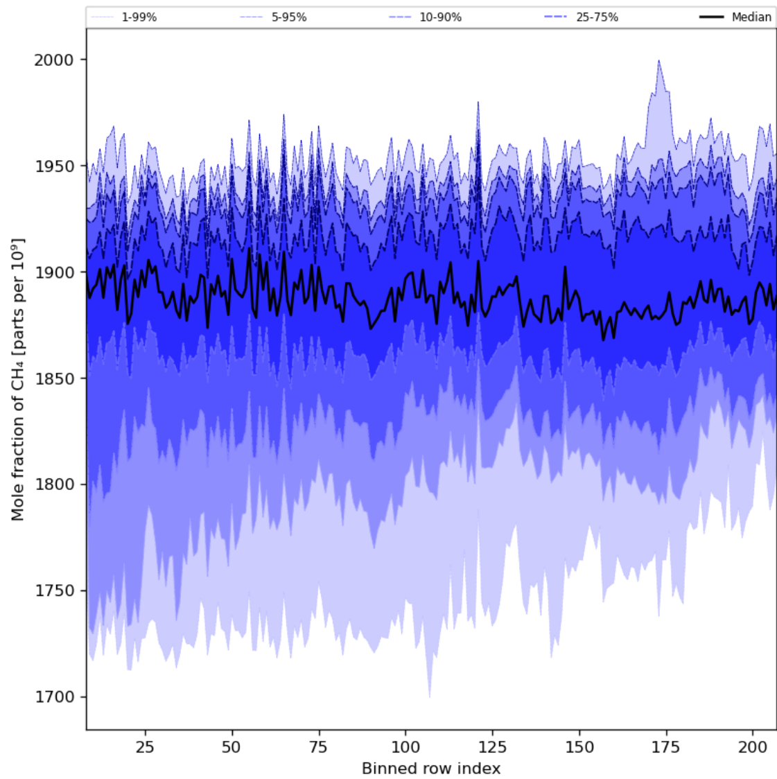
Figure 34: Along track statistics of “Mole fraction of CH 4 ” for 2024-03-16 to 2024-03-18
