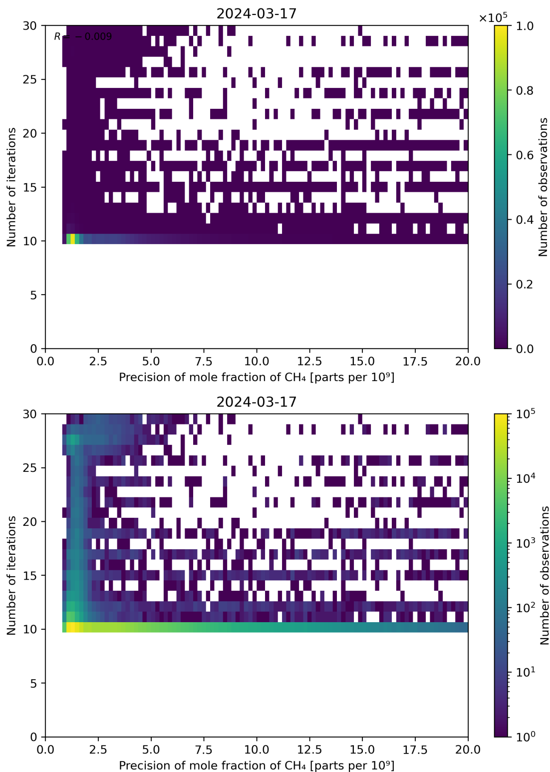
Figure 83: Scatter density plot of “Precision of mole fraction of CH 4 ” against “Number of iterations” for 2024-03-16 to 2024-03-18.
