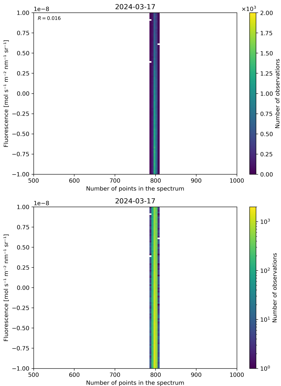
Figure 91: Scatter density plot of “Number of points in the spectrum” against “Fluorescence” for 2024-03-16 to 2024-03-18.
