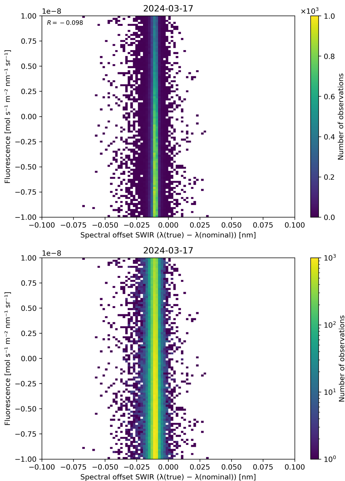
Figure 120: Scatter density plot of “Spectral offset SWIR ( \lambda(\text{true}) - \lambda(\text{nominal}) )” against “Fluorescence” for 2024-03-16 to 2024-03-18.
