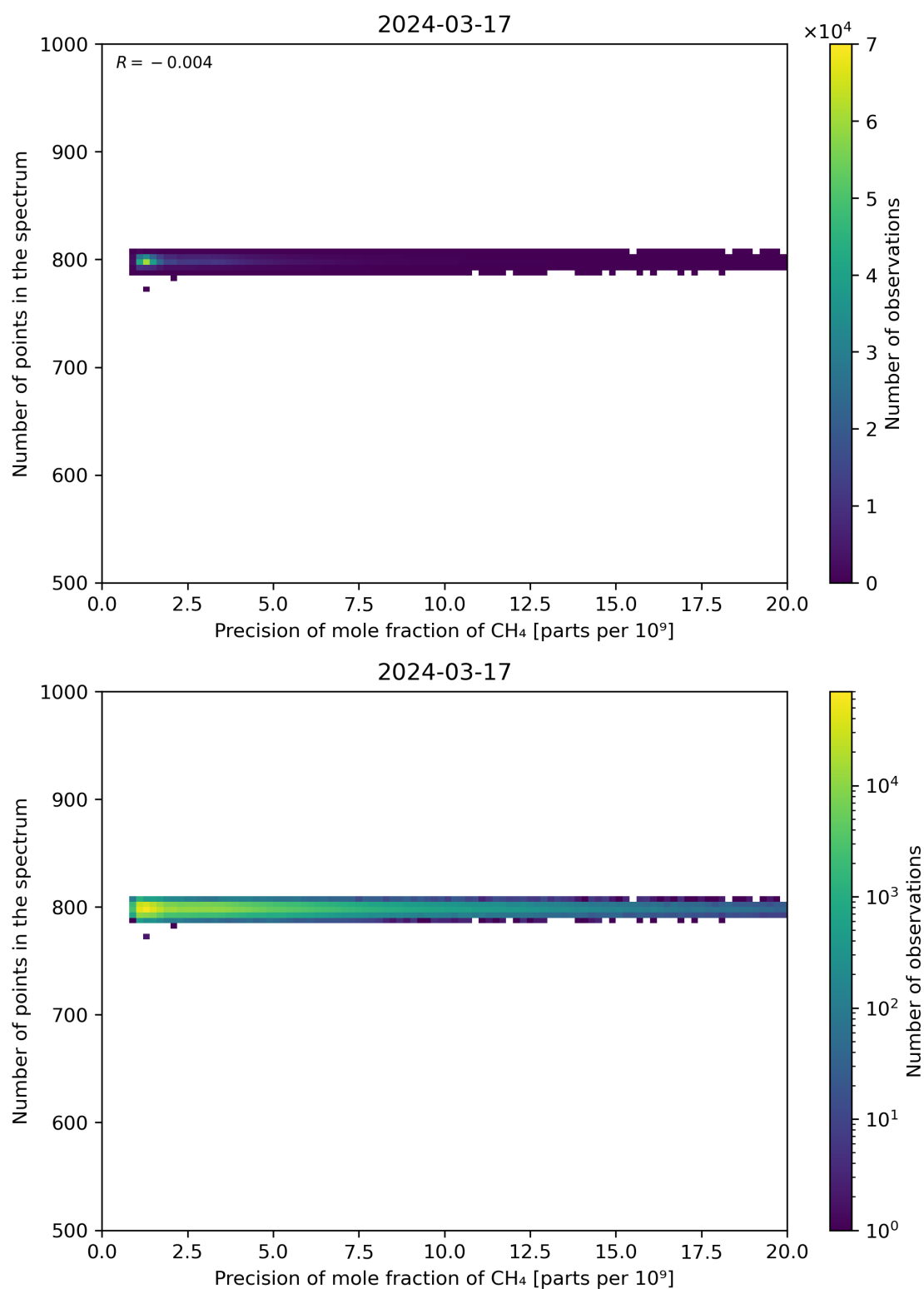
Figure 84: Scatter density plot of “Precision of mole fraction of CH 4 ” against “Number of points in the spectrum” for 2024-03-16 to 2024-03-18.
