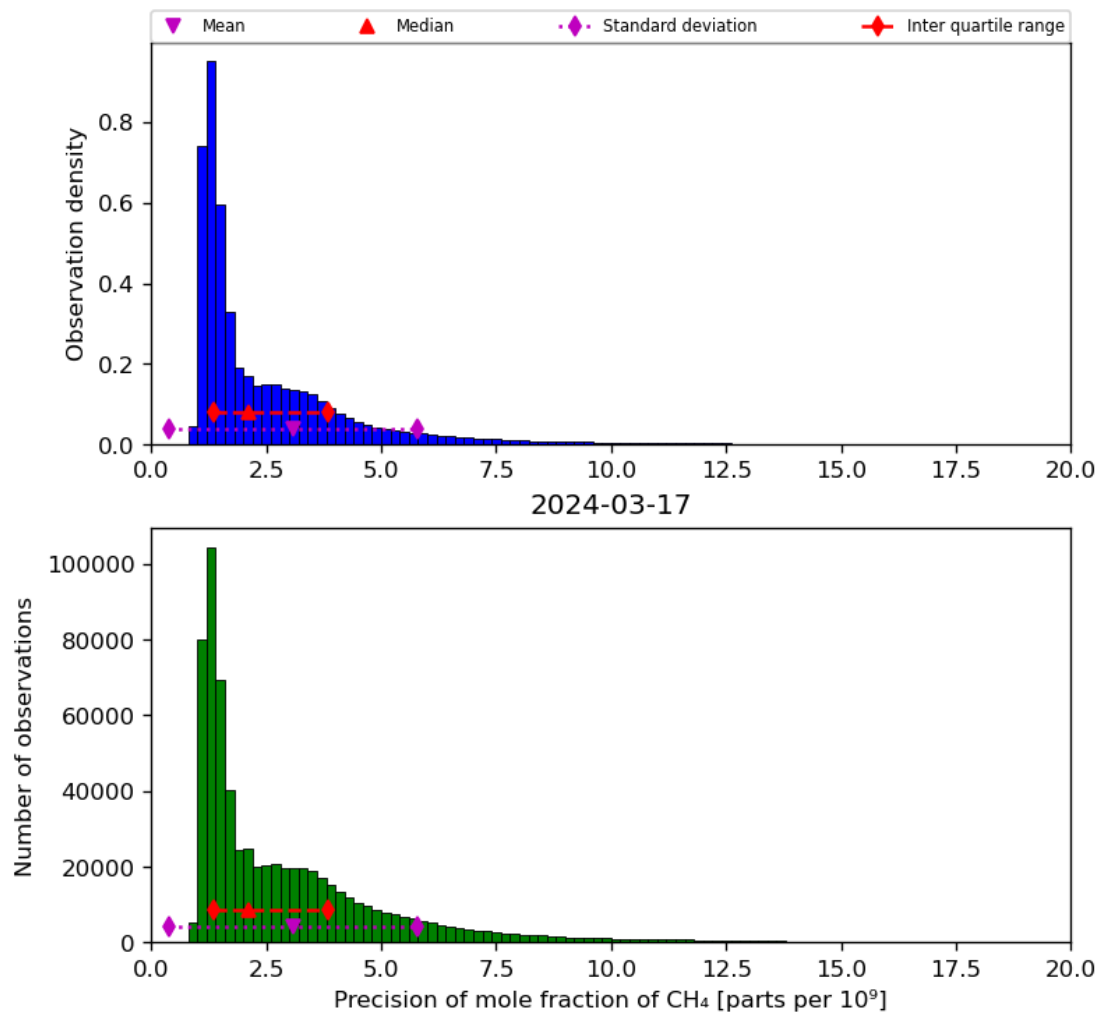
Figure 24: Histogram of “Precision of mole fraction of CH 4 ” for 2024-03-16 to 2024-03-18
