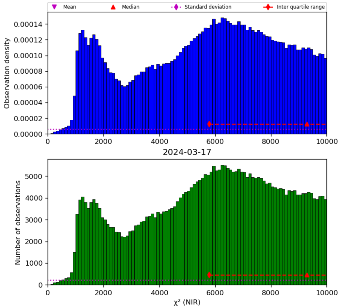
Figure 29: Histogram of " \chi^2 (NIR)" for 2024-03-16 to 2024-03-18
