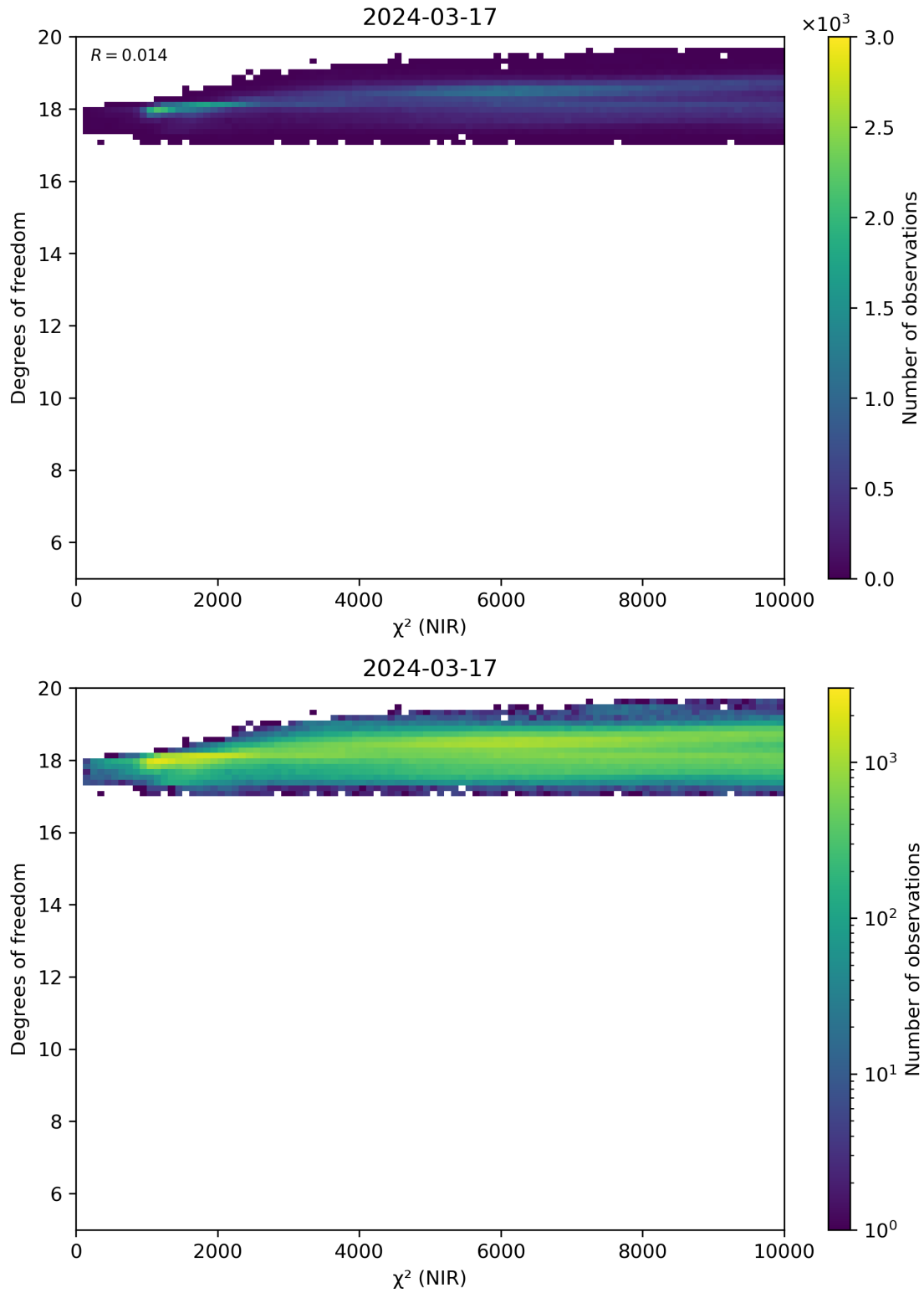
Figure 44: Scatter density plot of “ \chi^2 (NIR)” against “Degrees of freedom” for 2024-03-16 to 2024-03-18.
