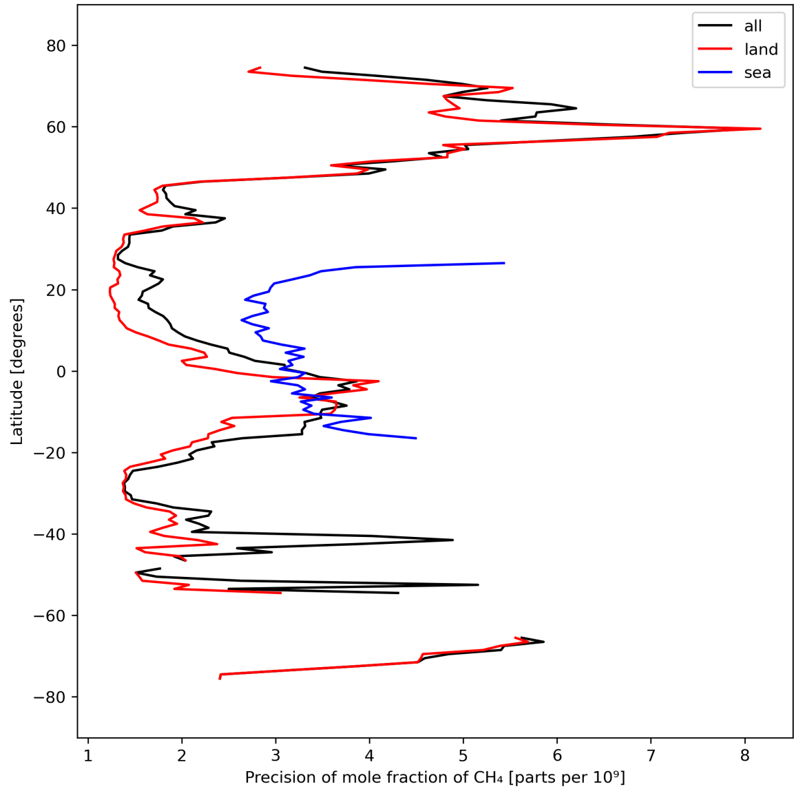
Figure 13: Zonal average of “Precision of mole fraction of CH 4 ” for 2024-03-16 to 2024-03-18.
