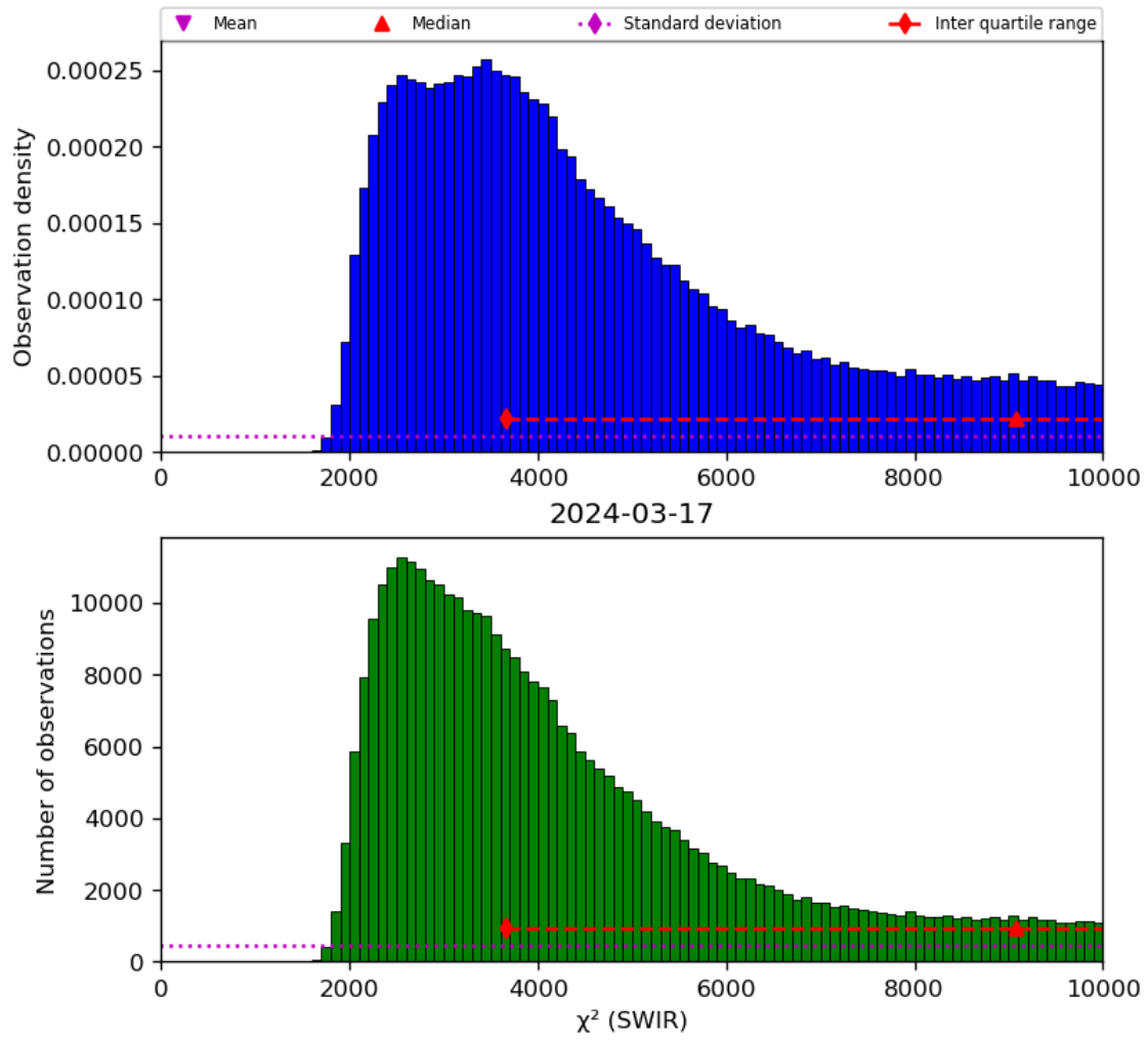
Figure 28: Histogram of “ \chi^2 (SWIR)” for 2024-03-16 to 2024-03-18
