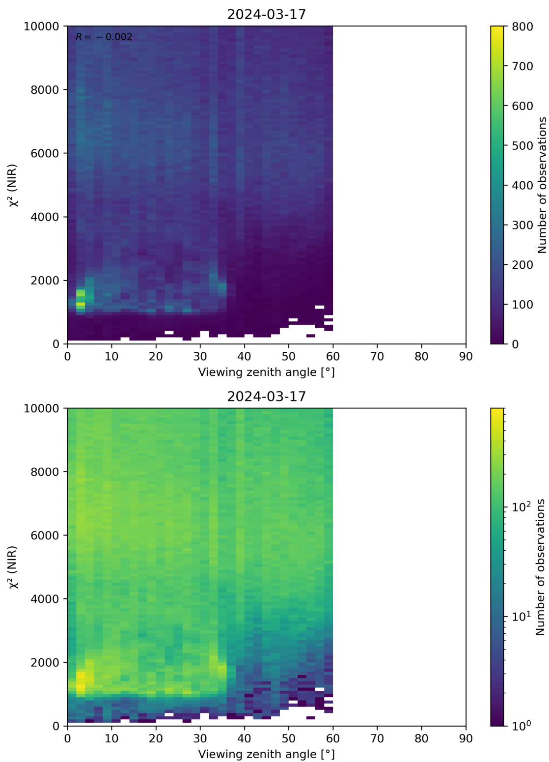
Figure 105: Scatter density plot of “Viewing zenith angle” against “ \chi^2 (NIR)” for 2024-03-16 to 2024-03-18.
