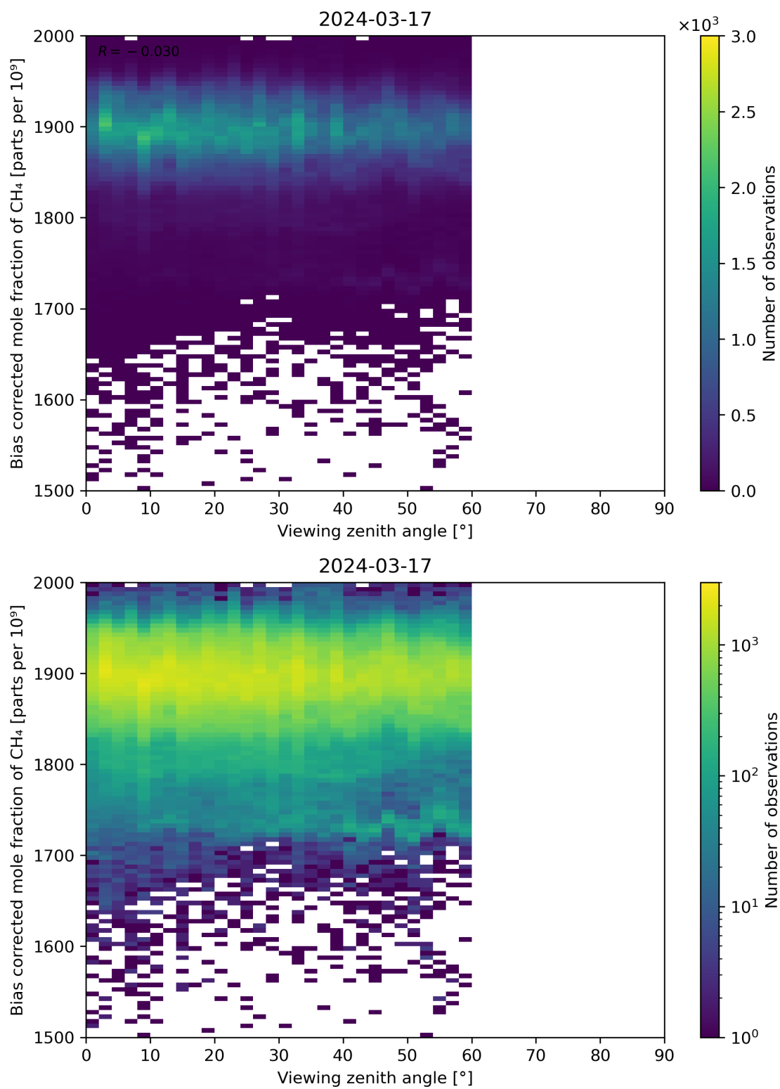
Figure 111: Scatter density plot of “Viewing zenith angle” against “Bias corrected mole fraction of CH 4 ” for 2024-03-16 to 2024-03-18.
