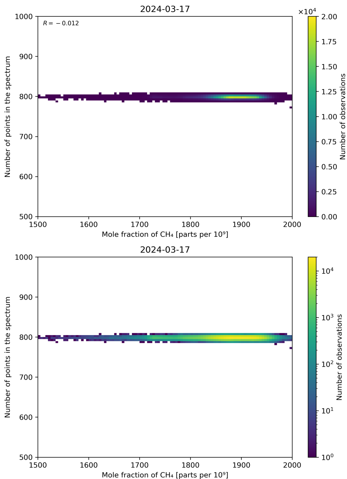
Figure 77: Scatter density plot of “Mole fraction of CH 4 ” against “Number of points in the spectrum” for 2024-03-16 to 2024-03-18.
