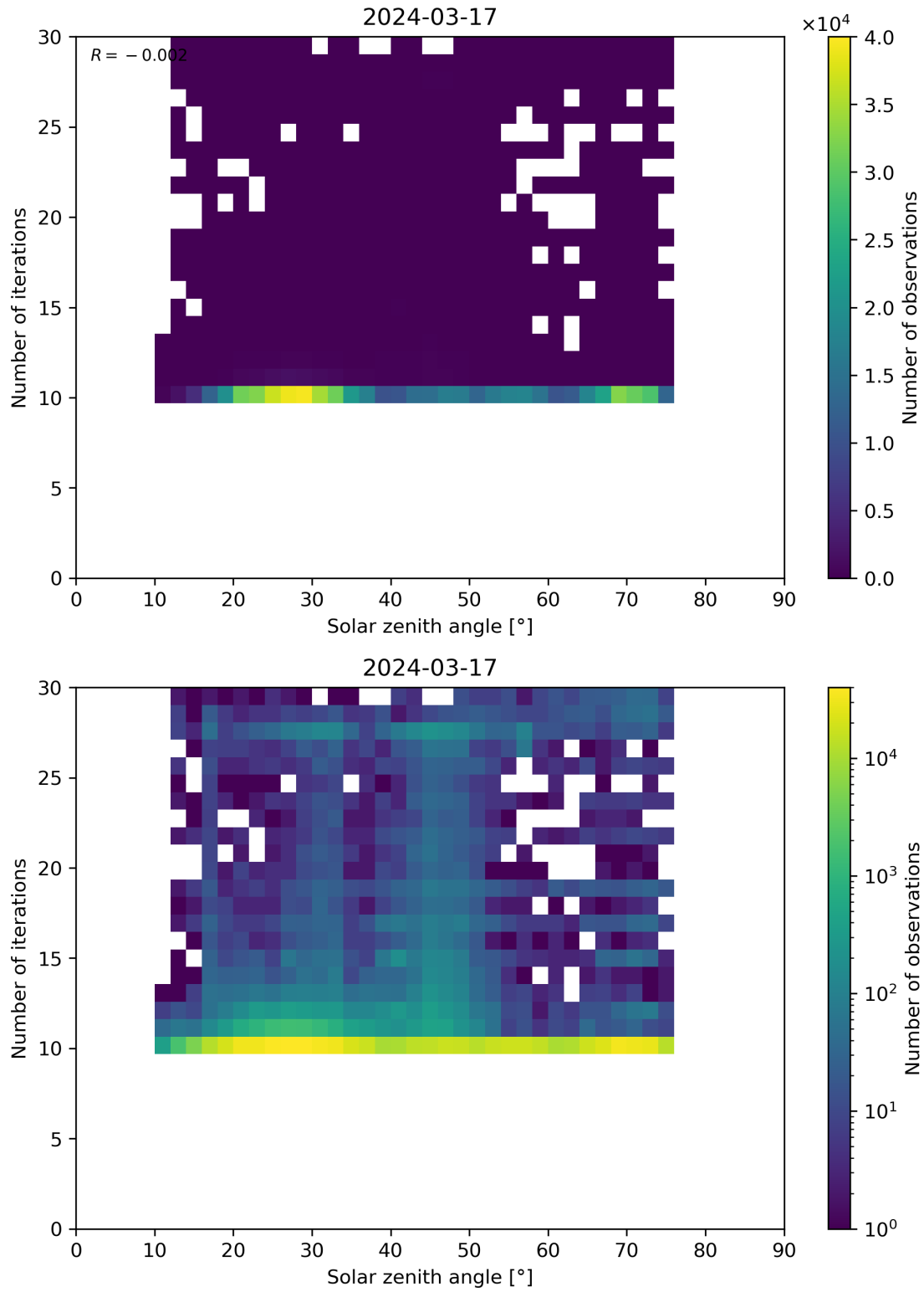
Figure 102: Scatter density plot of “Solar zenith angle” against “Number of iterations” for 2024-03-16 to 2024-03-18.
