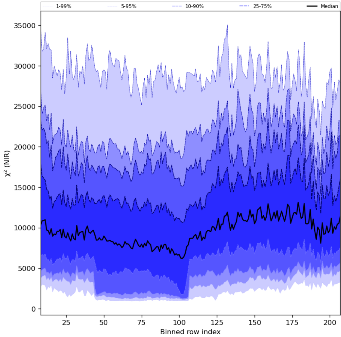
Figure 40: Along track statistics of “ \chi^2 (NIR)” for 2024-03-16 to 2024-03-18
