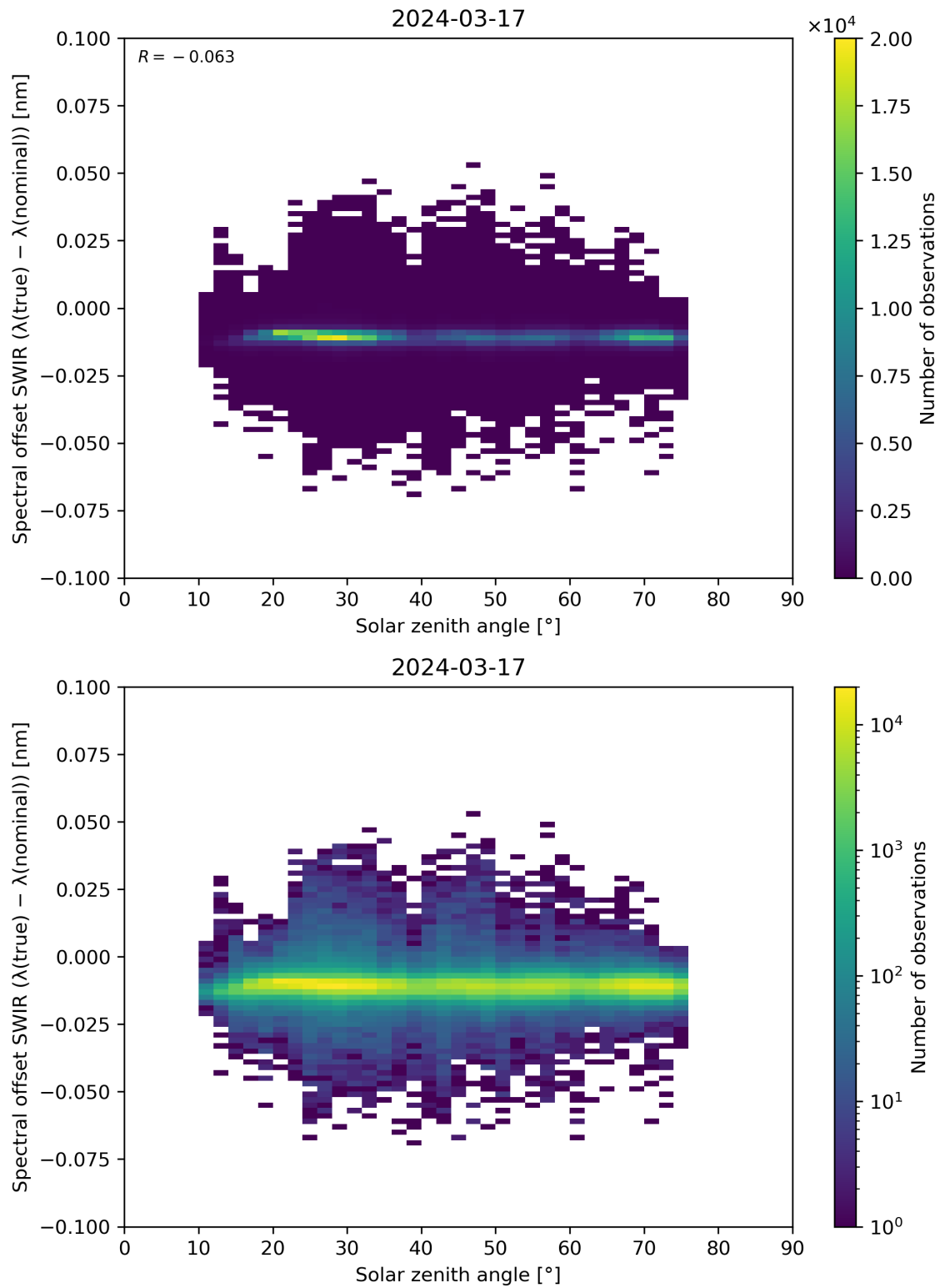
Figure 104: Scatter density plot of “Solar zenith angle” against “Spectral offset SWIR ( \lambda(\text{true}) - \lambda(\text{nominal}) )” for 2024-03-16 to 2024-03-18.
