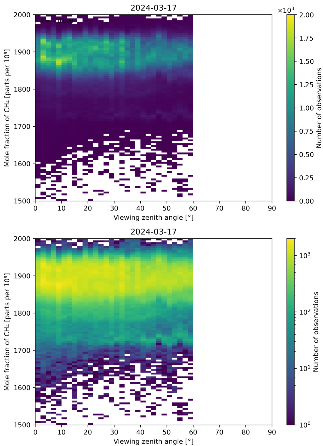
Figure 110: Scatter density plot of “Viewing zenith angle” against “Mole fraction of CH 4 ” for 2024-03-16 to 2024-03-18.
