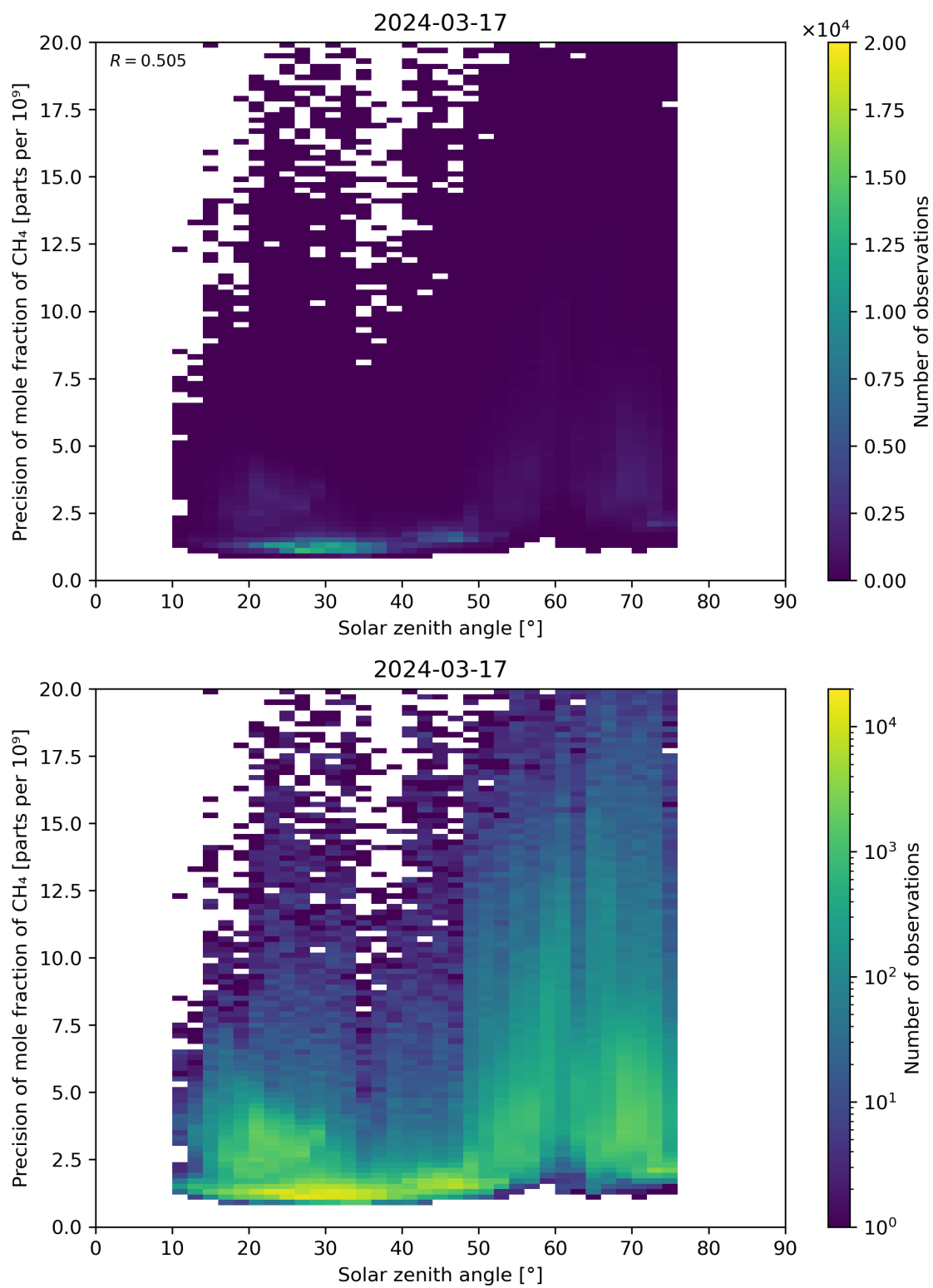
Figure 101: Scatter density plot of “Solar zenith angle” against “Precision of mole fraction of CH 4 ” for 2024-03-16 to 2024-03-18.
