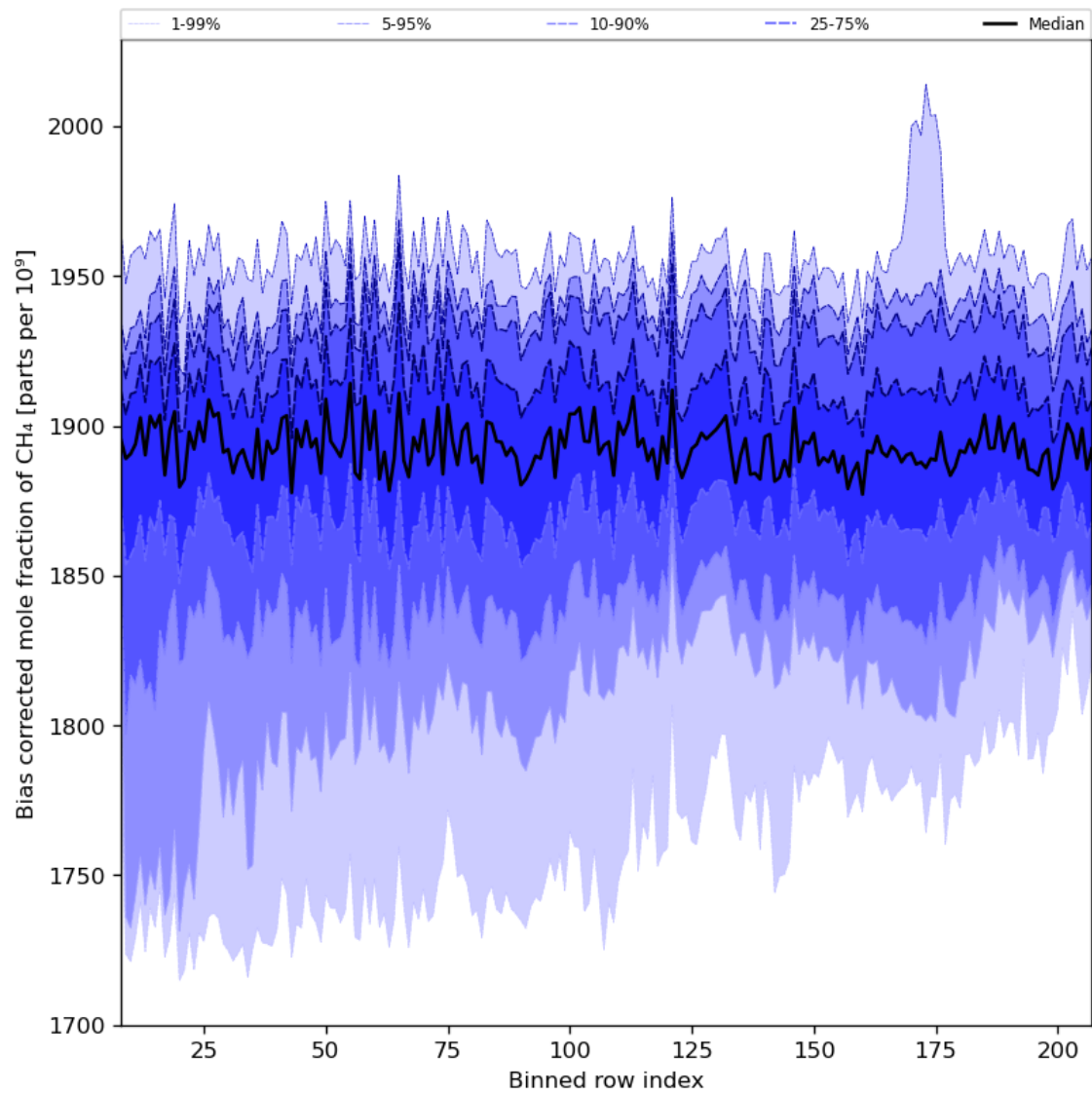
Figure 36: Along track statistics of “Bias corrected mole fraction of CH 4 ” for 2024-03-16 to 2024-03-18
