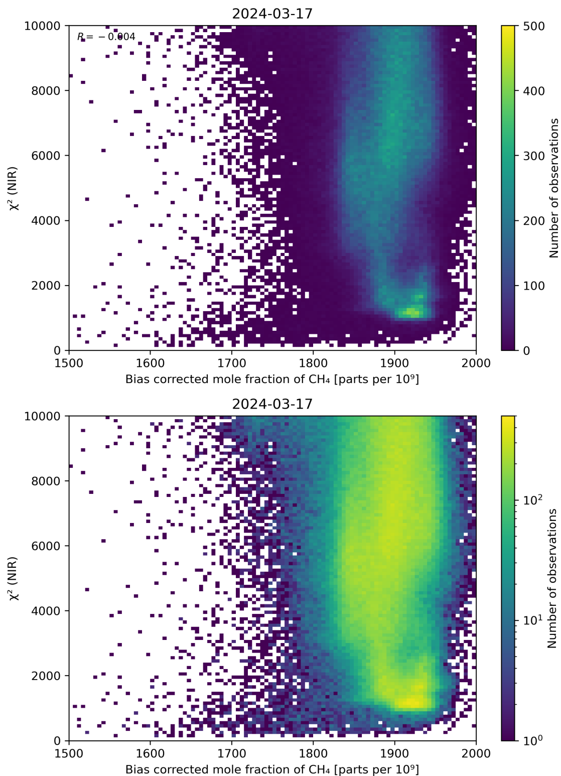
Figure 63: Scatter density plot of “Bias corrected mole fraction of CH 4 ” against “ \chi^2 (NIR)” for 2024-03-16 to 2024-03-18.
