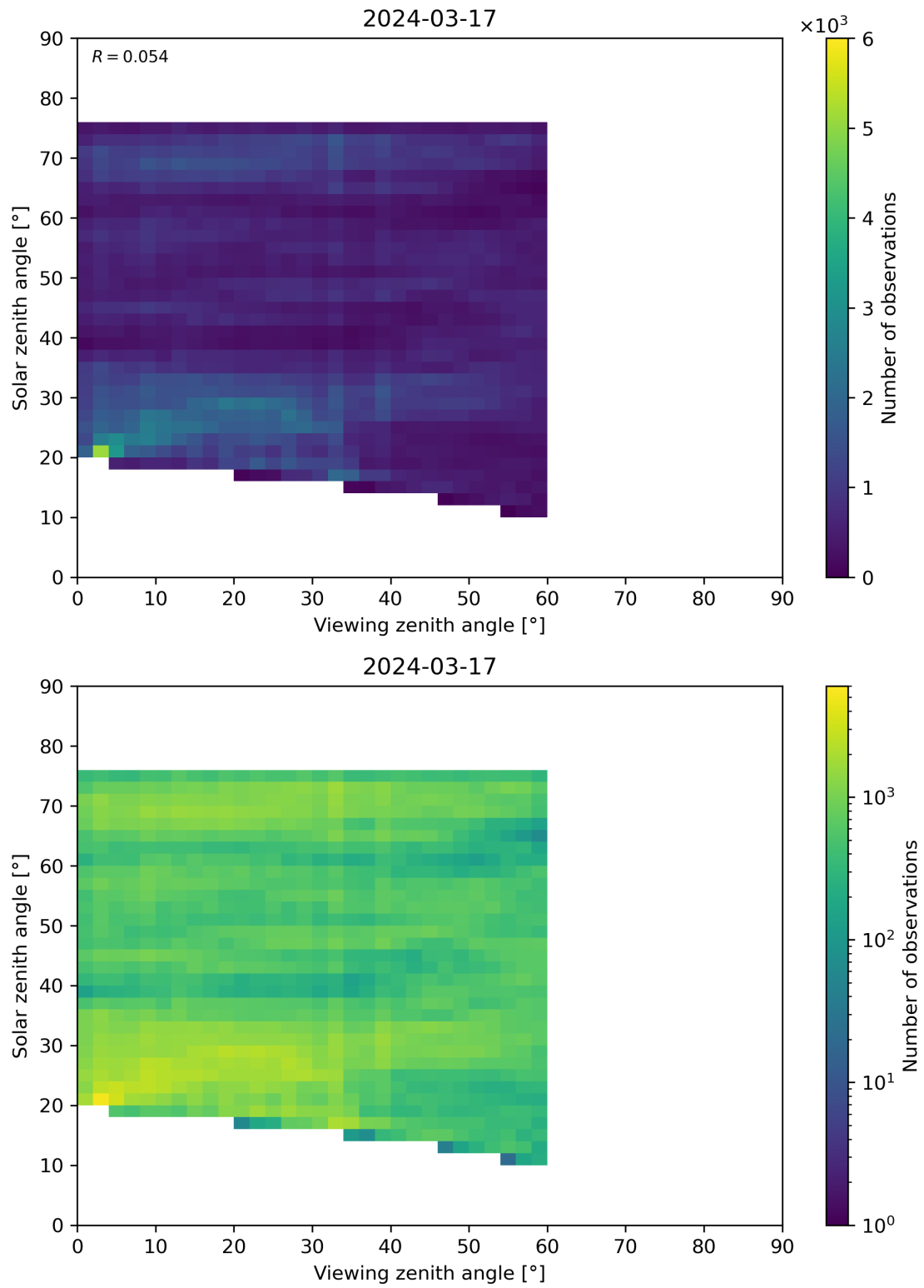
Figure 115: Scatter density plot of “Viewing zenith angle” against “Solar zenith angle” for 2024-03-16 to 2024-03-18.
