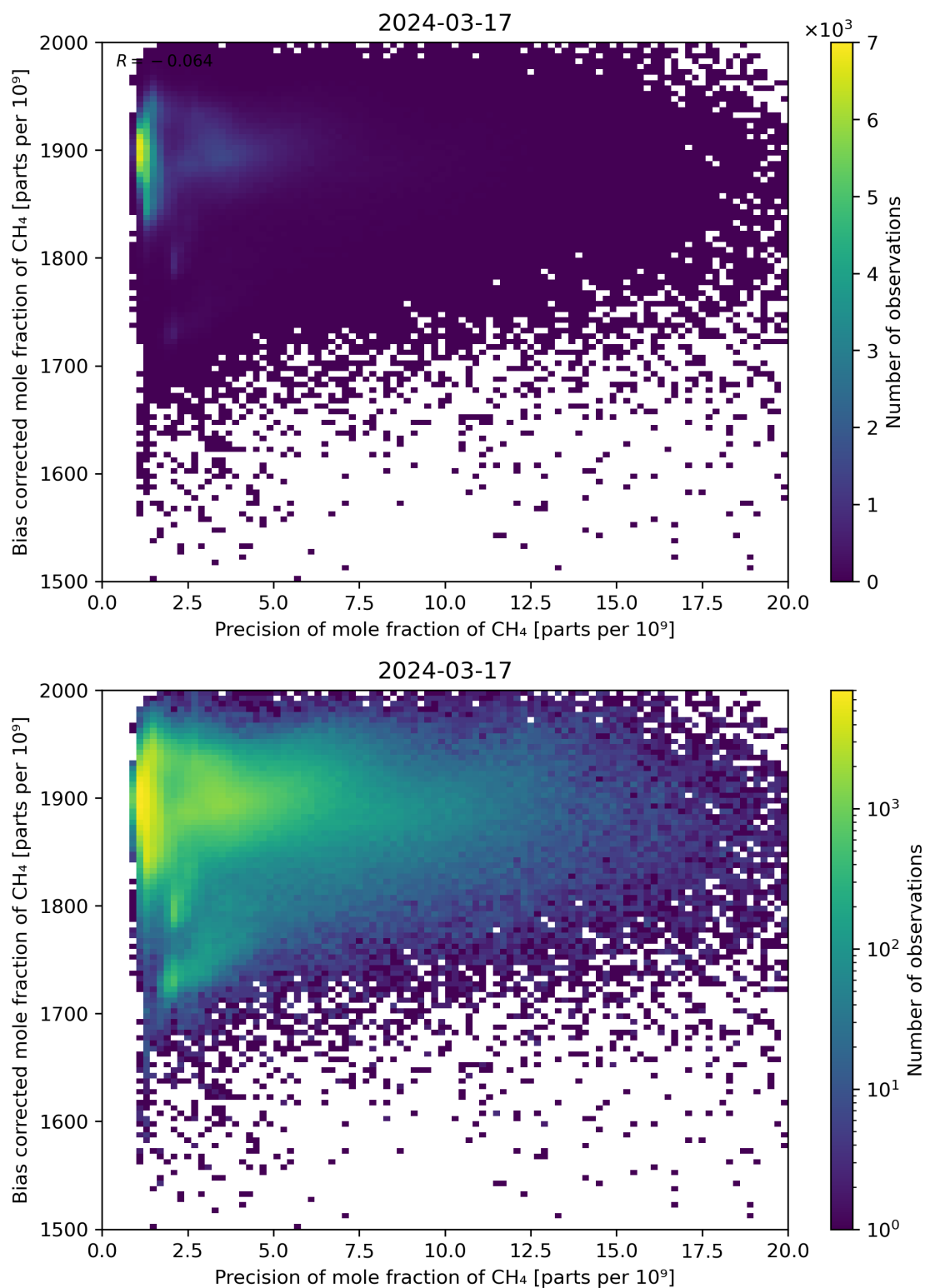
Figure 82: Scatter density plot of “Precision of mole fraction of CH 4 ” against “Bias corrected mole fraction of CH 4 ” for 2024-03-16 to 2024-03-18.
