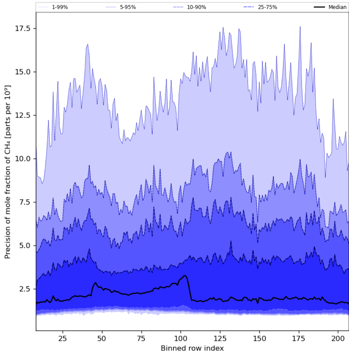
Figure 35: Along track statistics of “Precision of mole fraction of CH 4 ” for 2024-03-16 to 2024-03-18
