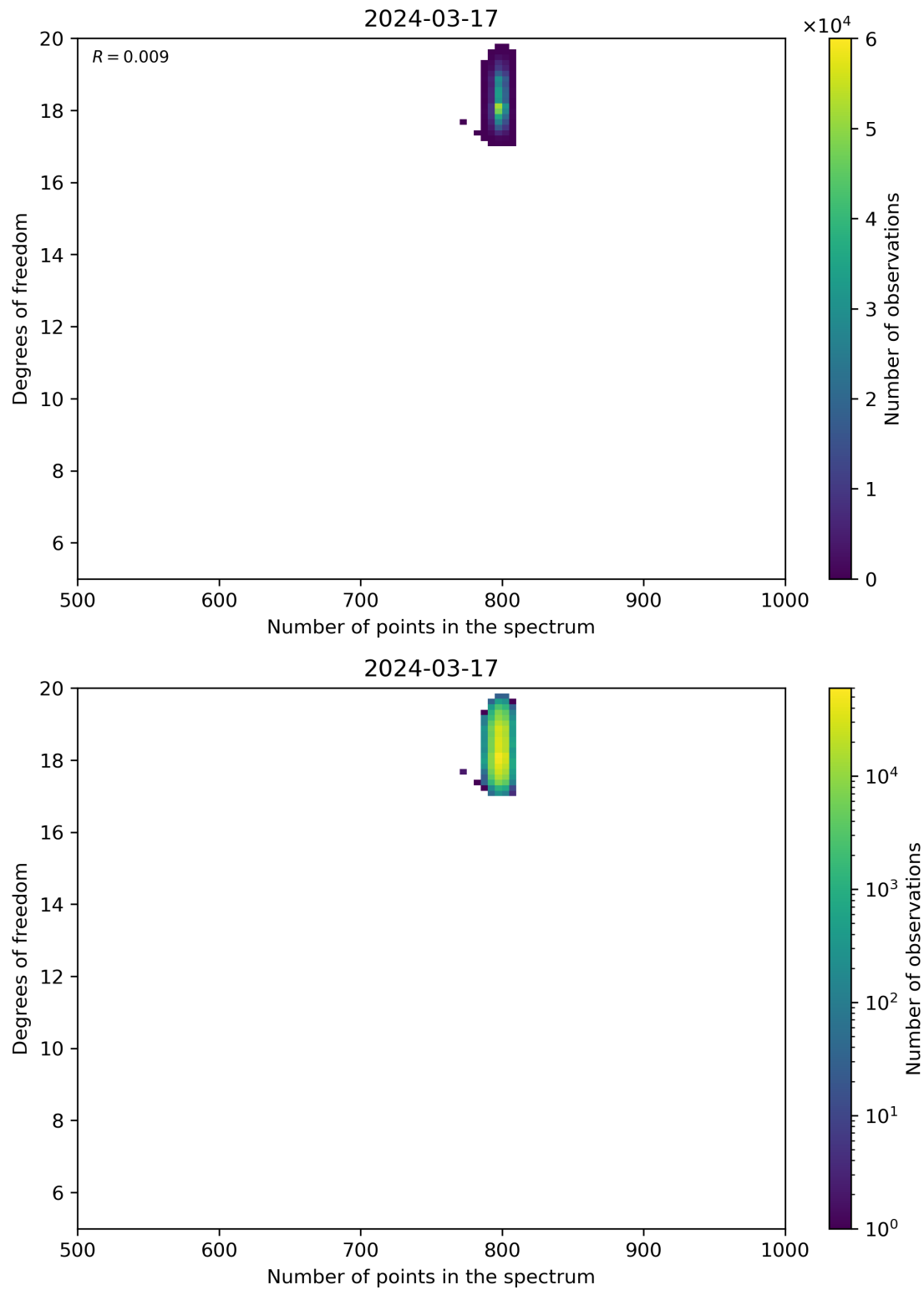
Figure 90: Scatter density plot of “Number of points in the spectrum” against “Degrees of freedom” for 2024-03-16 to 2024-03-18.
