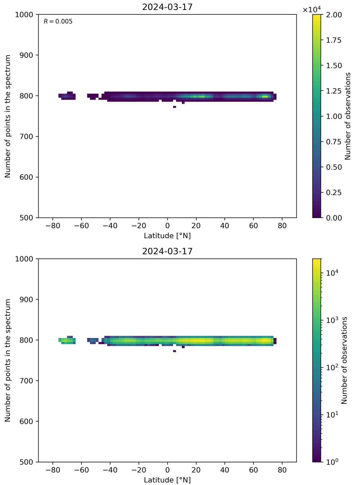
Figure 61: Scatter density plot of “Latitude” against “Number of points in the spectrum” for 2024-03-16 to 2024-03-18.
