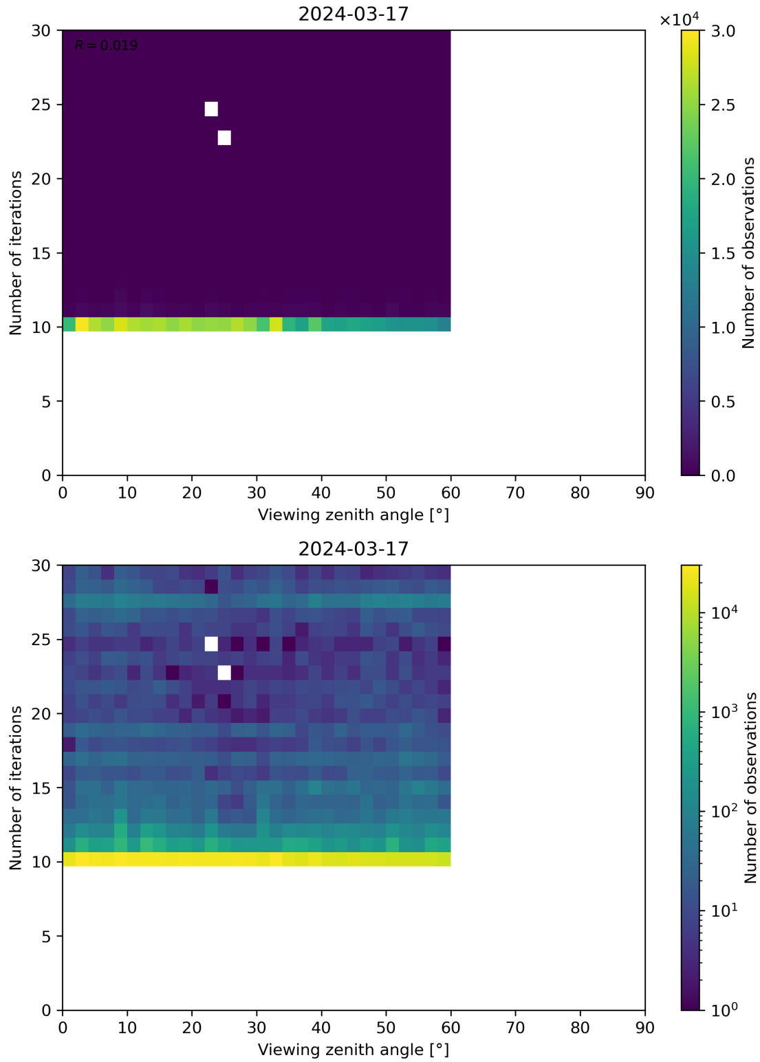
Figure 113: Scatter density plot of “Viewing zenith angle” against “Number of iterations” for 2024-03-16 to 2024-03-18.
