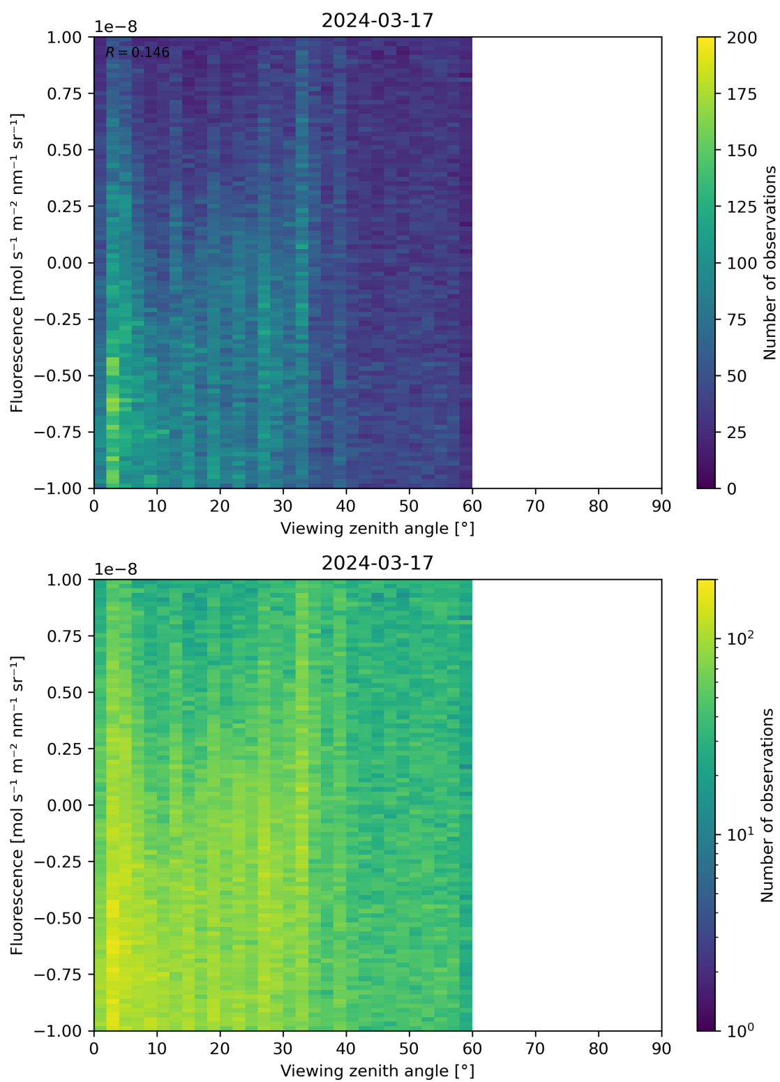
Figure 108: Scatter density plot of “Viewing zenith angle” against “Fluorescence” for 2024-03-16 to 2024-03-18.
