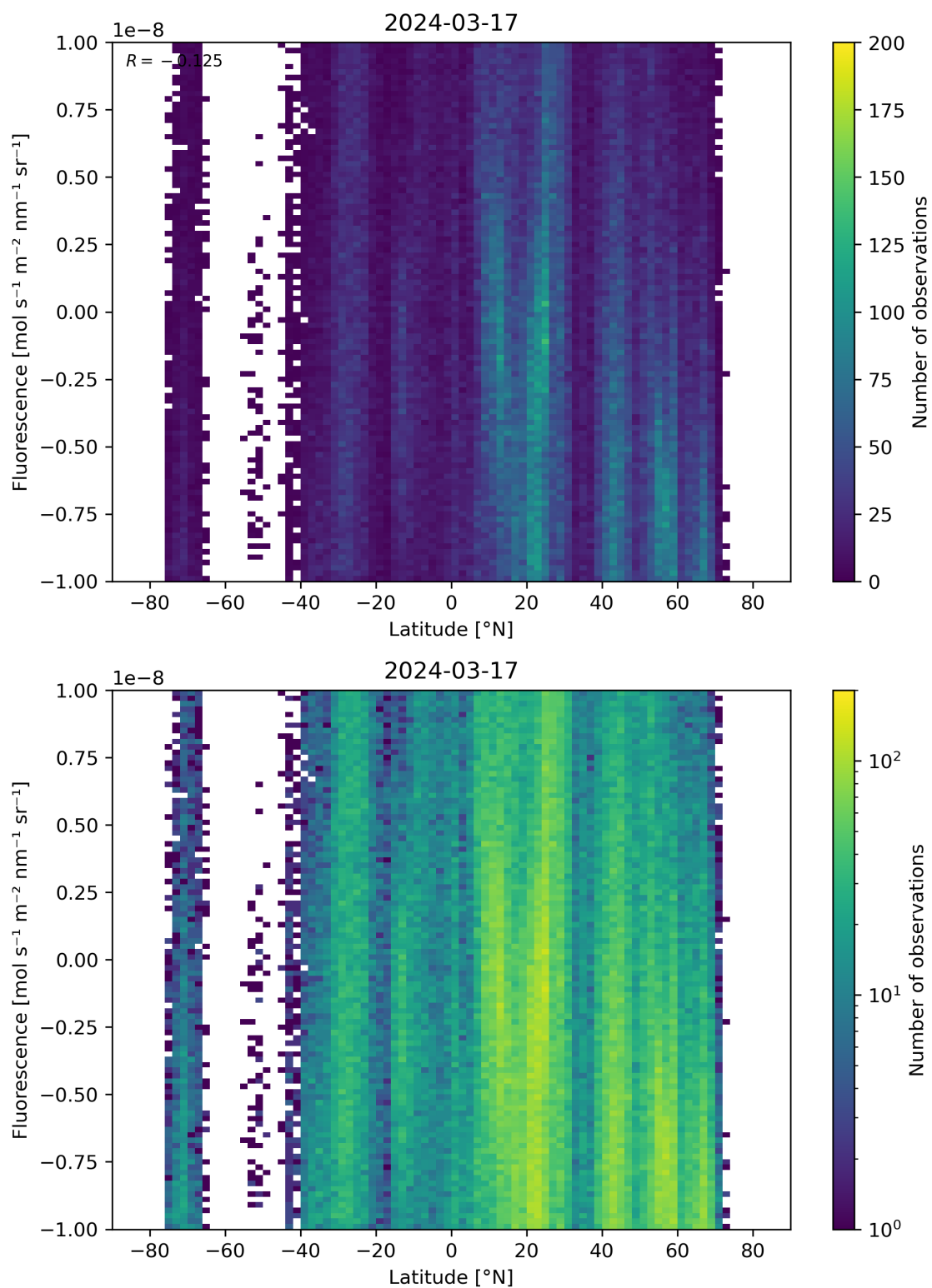
Figure 56: Scatter density plot of “Latitude” against “Fluorescence” for 2024-03-16 to 2024-03-18.
