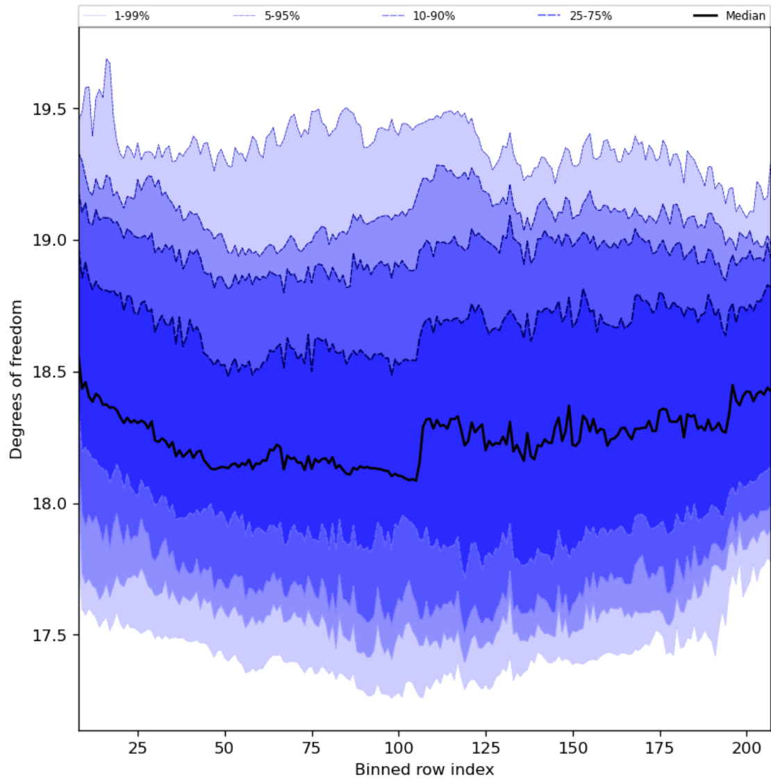
Figure 41: Along track statistics of “Degrees of freedom” for 2024-03-16 to 2024-03-18
