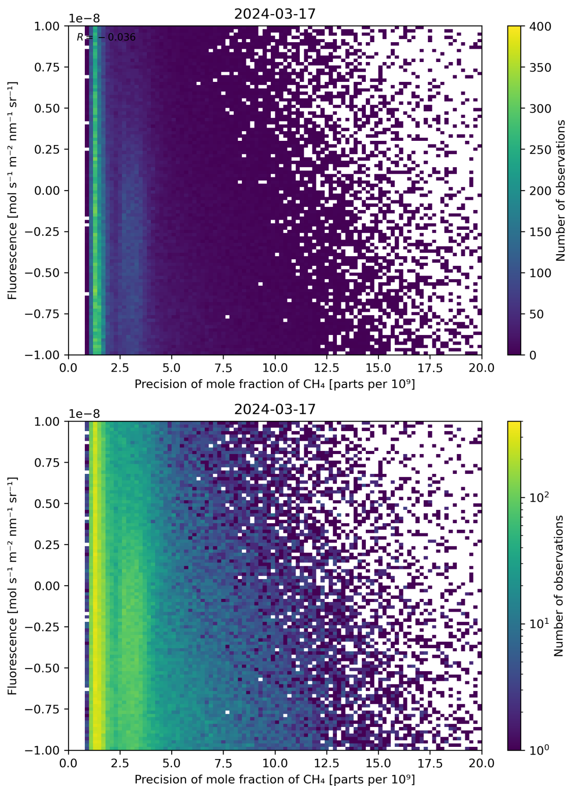
Figure 81: Scatter density plot of “Precision of mole fraction of \text{CH}_4 ” against “Fluorescence” for 2024-03-16 to 2024-03-18.
