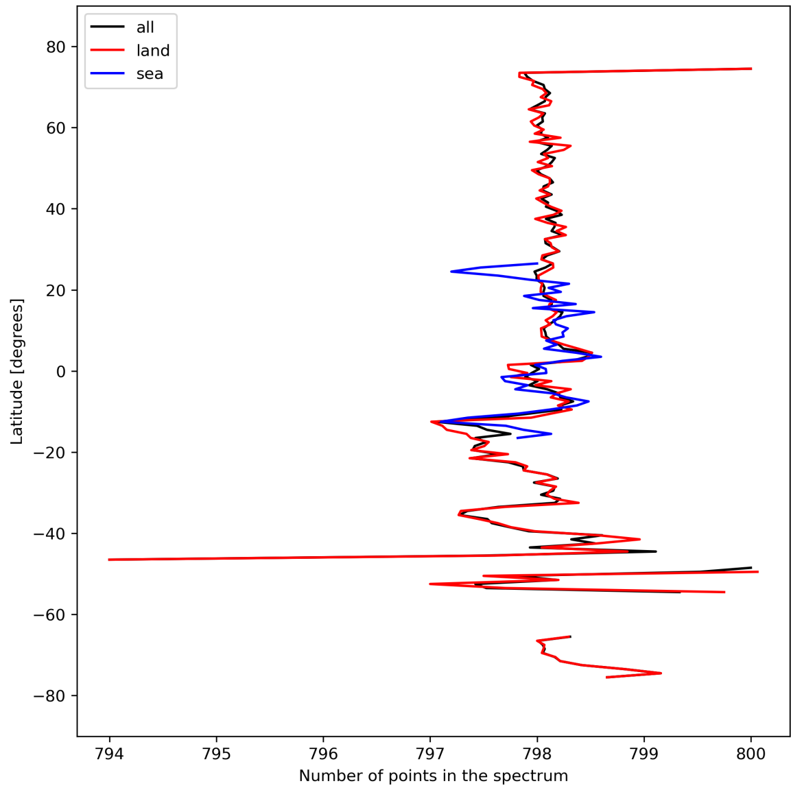
Figure 15: Zonal average of “Number of points in the spectrum” for 2024-03-16 to 2024-03-18.
