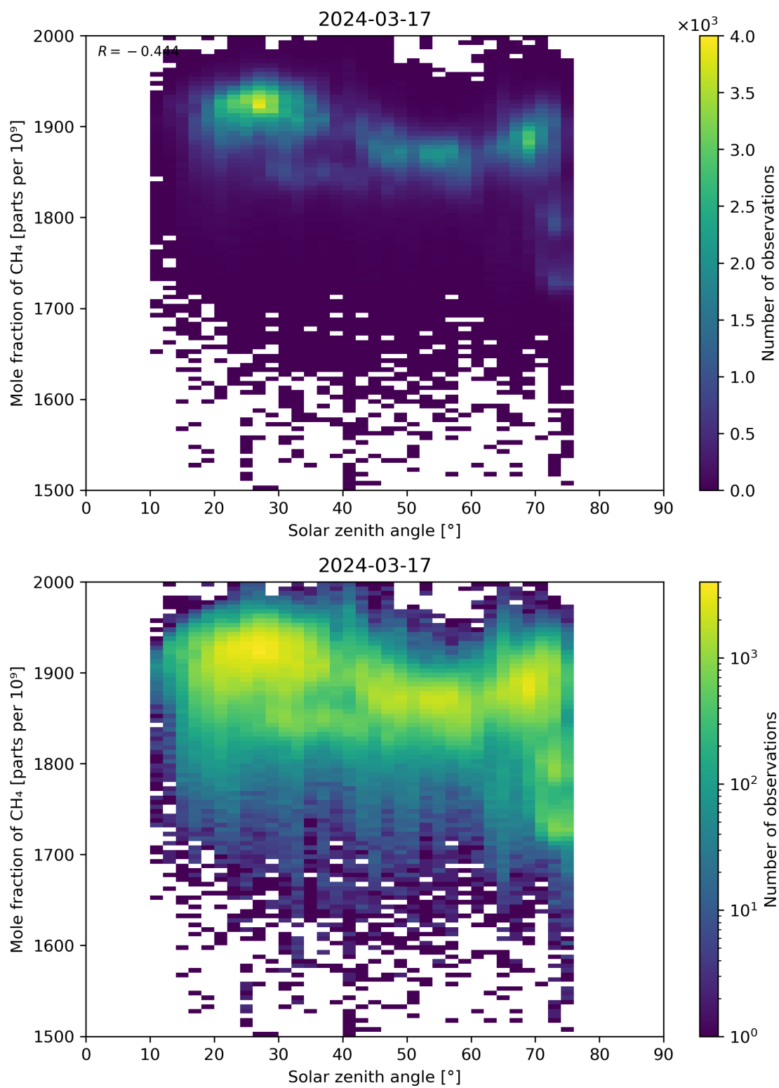
Figure 99: Scatter density plot of “Solar zenith angle” against “Mole fraction of CH 4 ” for 2024-03-16 to 2024-03-18.
