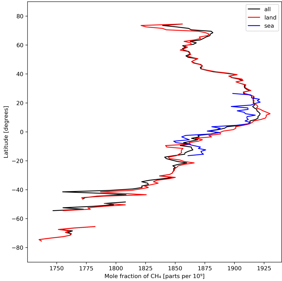
Figure 12: Zonal average of “Mole fraction of \text{CH}_4 ” for 2024-03-16 to 2024-03-18.
