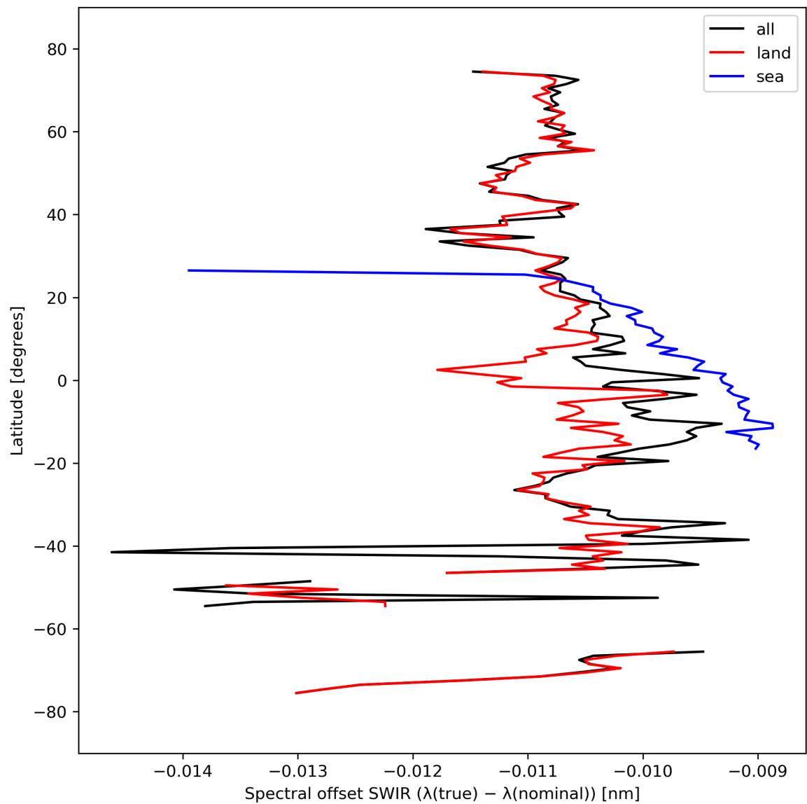
Figure 16: Zonal average of “Spectral offset SWIR ( \lambda(\text{true}) - \lambda(\text{nominal}) )” for 2024-03-16 to 2024-03-18.
