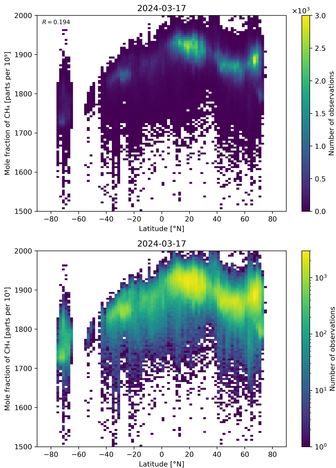
Figure 57: Scatter density plot of “Latitude” against “Mole fraction of CH 4 ” for 2024-03-16 to 2024-03-18.
