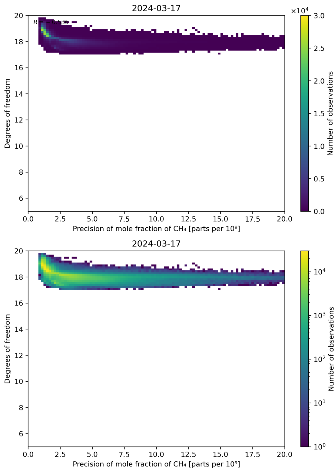
Figure 80: Scatter density plot of “Precision of mole fraction of CH 4 ” against “Degrees of freedom” for 2024-03-16 to 2024-03-18.
