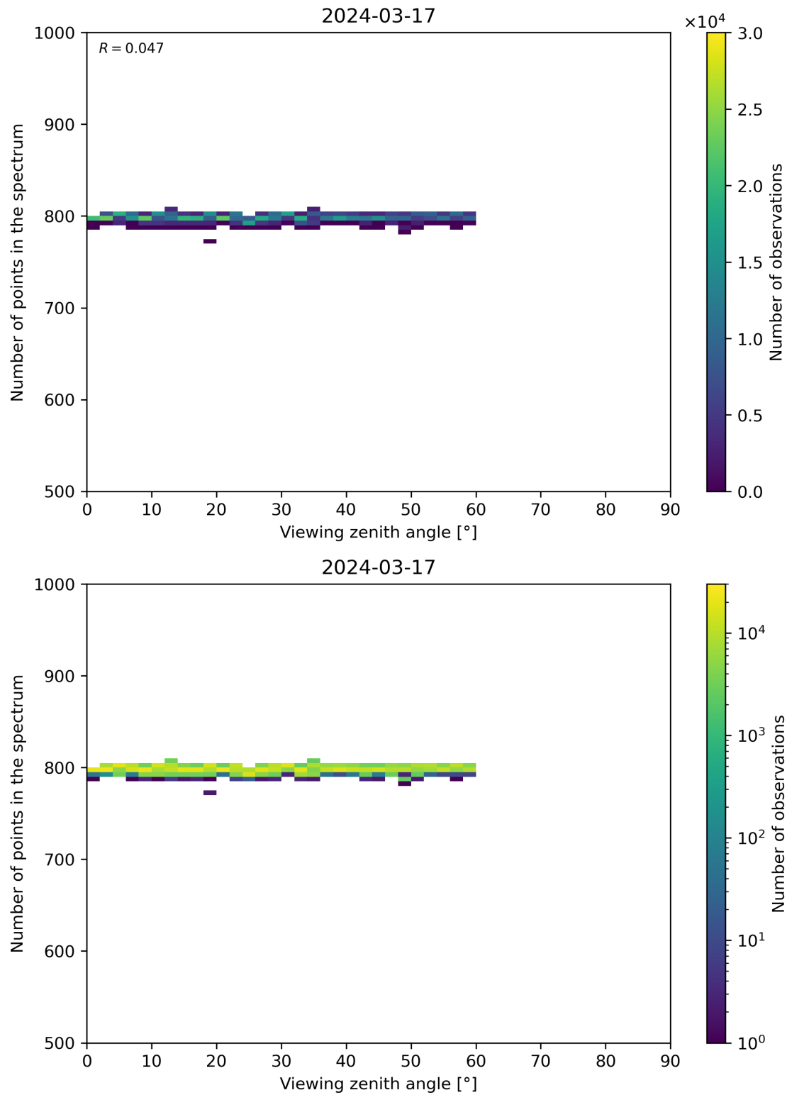
Figure 114: Scatter density plot of “Viewing zenith angle” against “Number of points in the spectrum” for 2024-03-16 to 2024-03-18.
