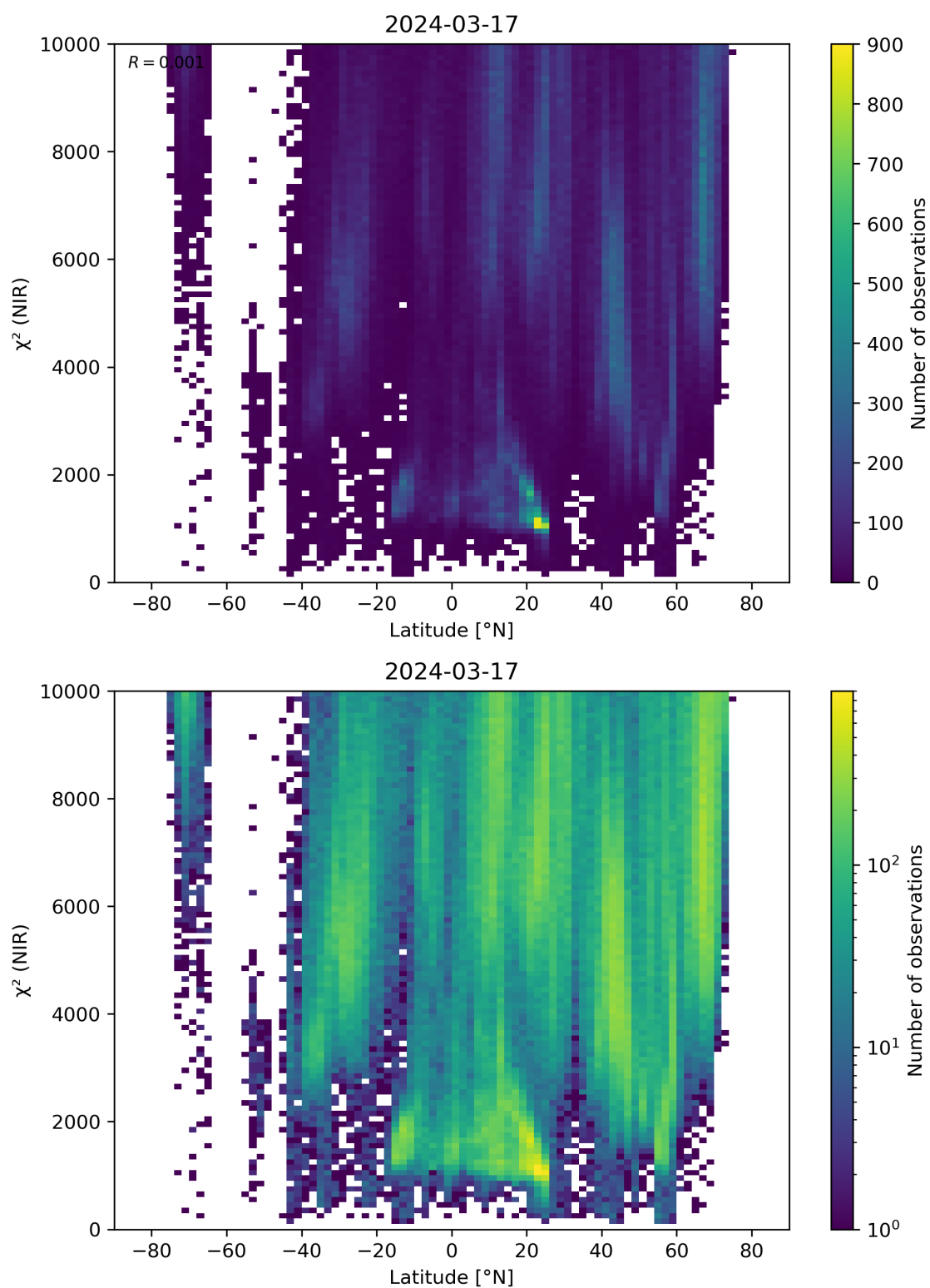
Figure 53: Scatter density plot of “Latitude” against “ \chi^2 (NIR)” for 2024-03-16 to 2024-03-18.
