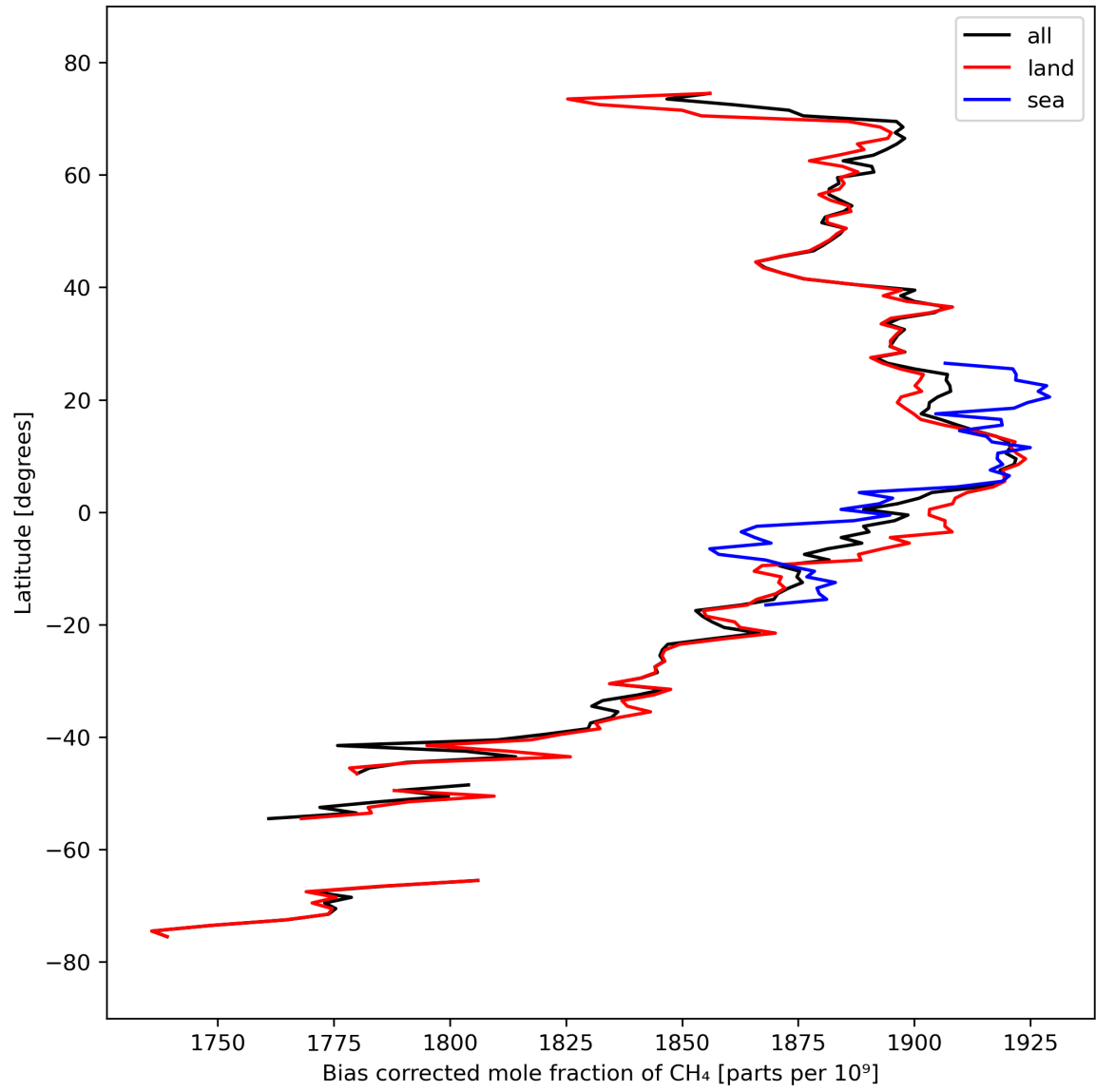
Figure 14: Zonal average of “Bias corrected mole fraction of \text{CH}_4 ” for 2024-03-16 to 2024-03-18.
