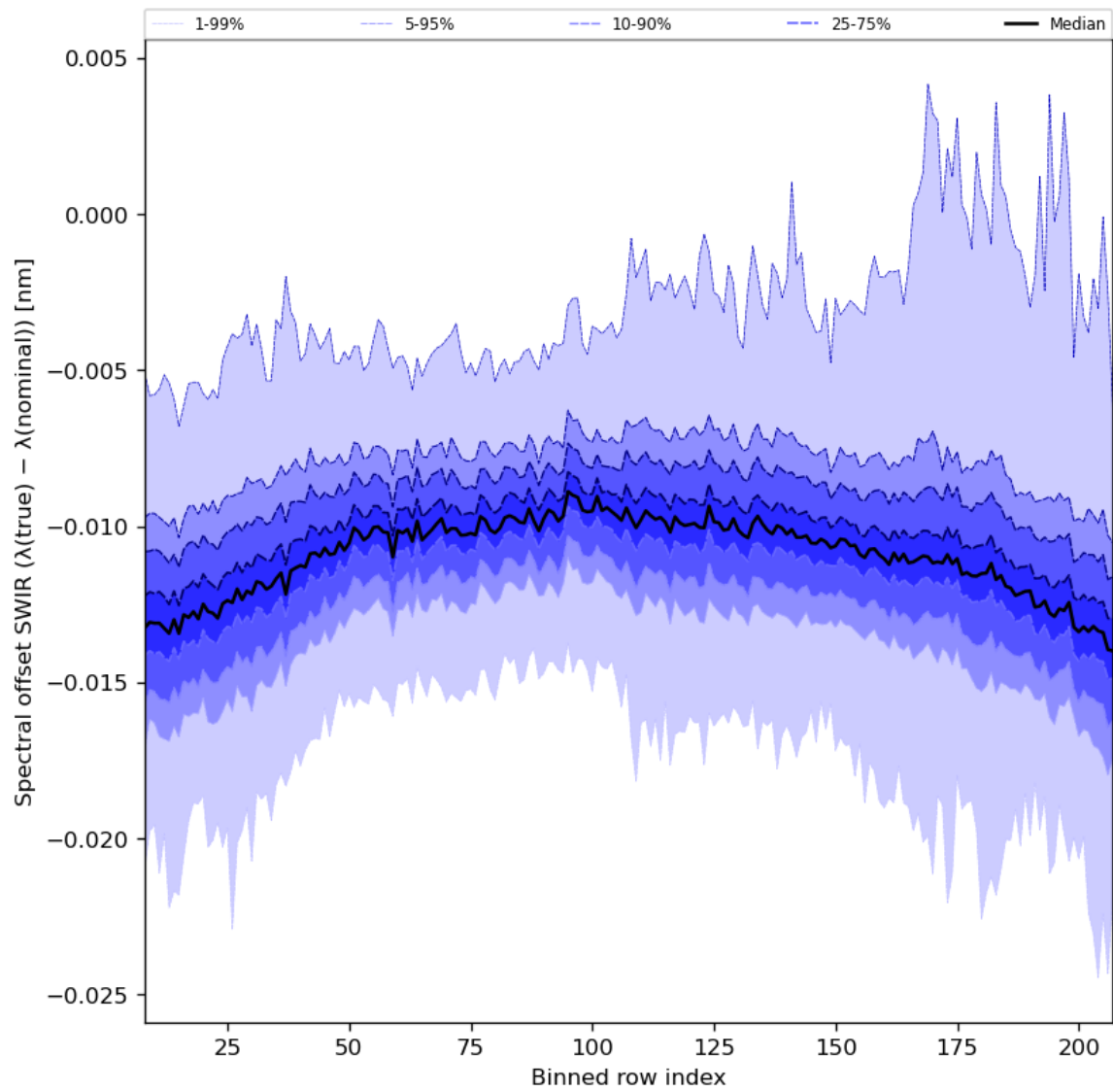
Figure 38: Along track statistics of “Spectral offset SWIR ( \lambda(\text{true}) - \lambda(\text{nominal}) )” for 2024-03-16 to 2024-03-18
