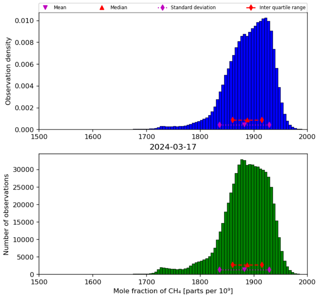
Figure 23: Histogram of "Mole fraction of CH 4 " for 2024-03-16 to 2024-03-18
