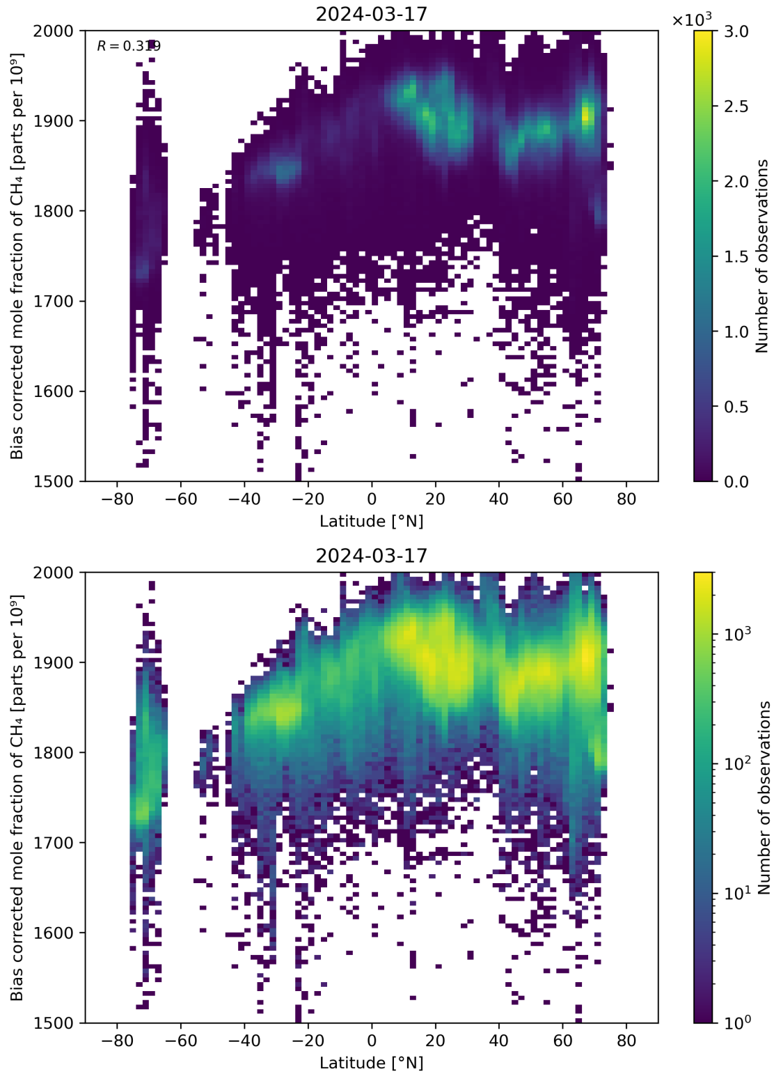
Figure 58: Scatter density plot of “Latitude” against “Bias corrected mole fraction of \text{CH}_4 ” for 2024-03-16 to 2024-03-18.
