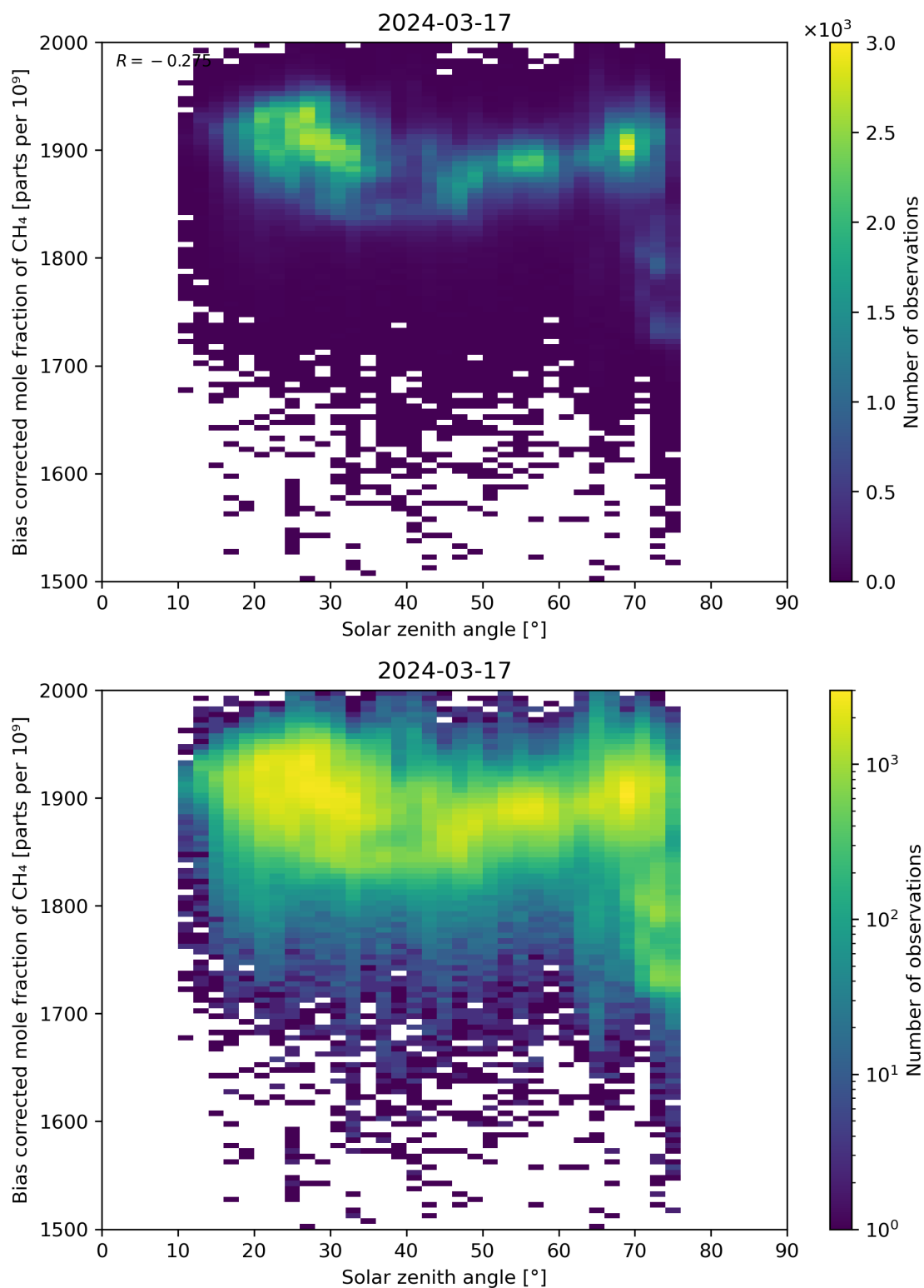
Figure 100: Scatter density plot of “Solar zenith angle” against “Bias corrected mole fraction of CH 4 ” for 2024-03-16 to 2024-03-18.
