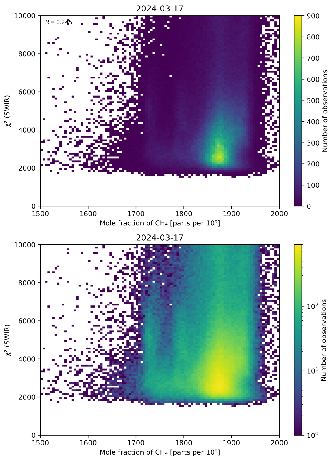
Figure 71: Scatter density plot of “Mole fraction of CH 4 ” against “ \chi^2 (SWIR)” for 2024-03-16 to 2024-03-18.
