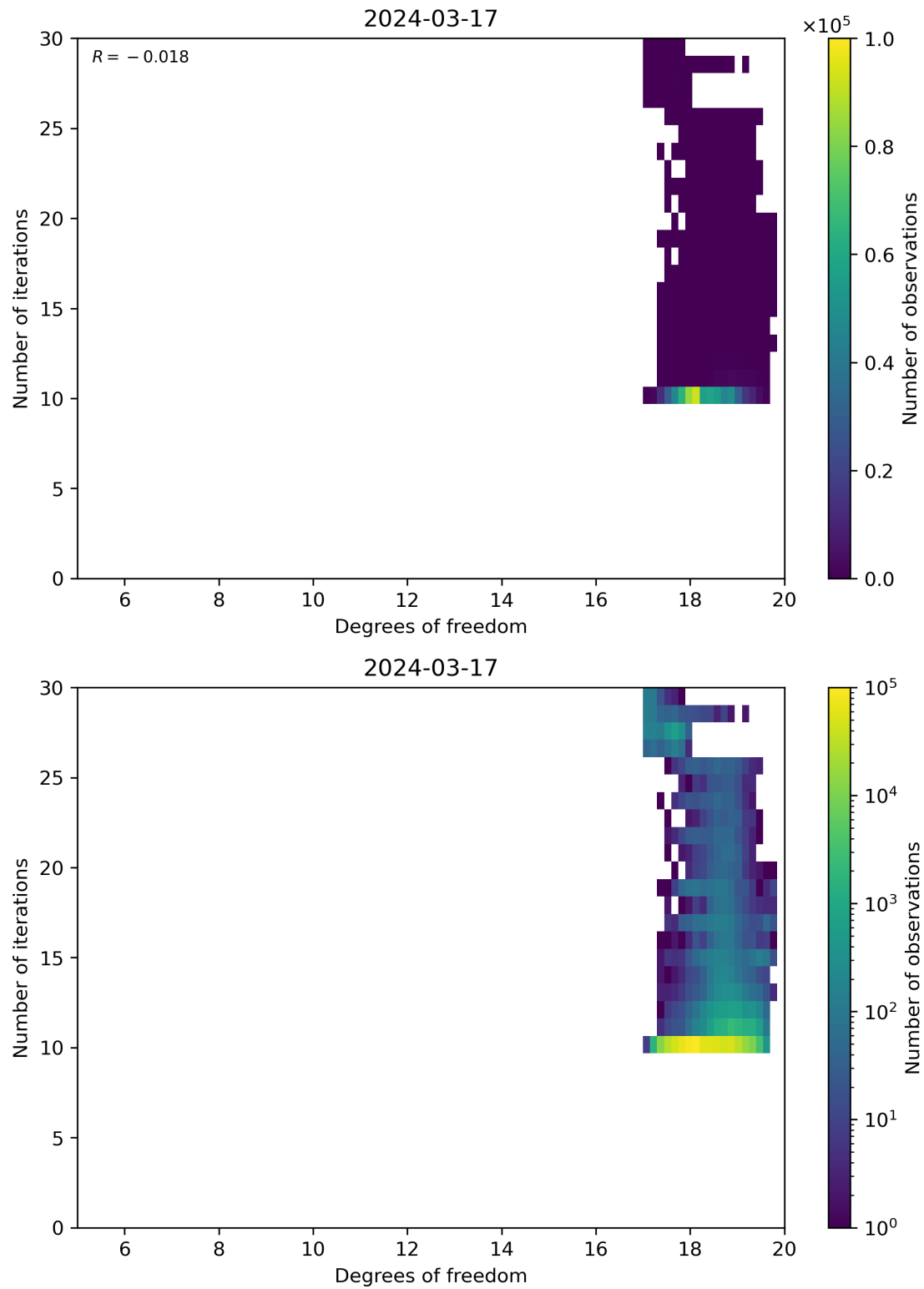
Figure 52: Scatter density plot of “Degrees of freedom” against “Number of iterations” for 2024-03-16 to 2024-03-18.
