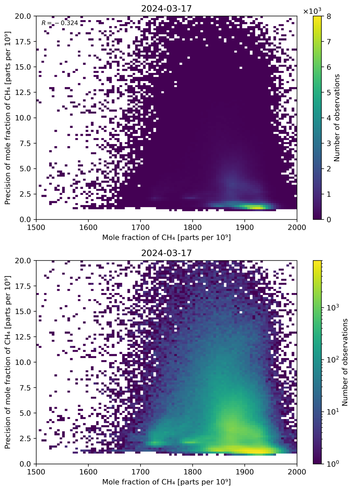
Figure 75: Scatter density plot of “Mole fraction of CH 4 ” against “Precision of mole fraction of CH 4 ” for 2024-03-16 to 2024-03-18.
