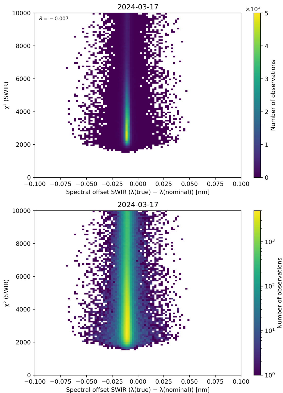
Figure 118: Scatter density plot of “Spectral offset SWIR ( \lambda(\text{true}) - \lambda(\text{nominal}) )” against “ \chi^2 (SWIR)” for 2024-03-16 to 2024-03-18.
