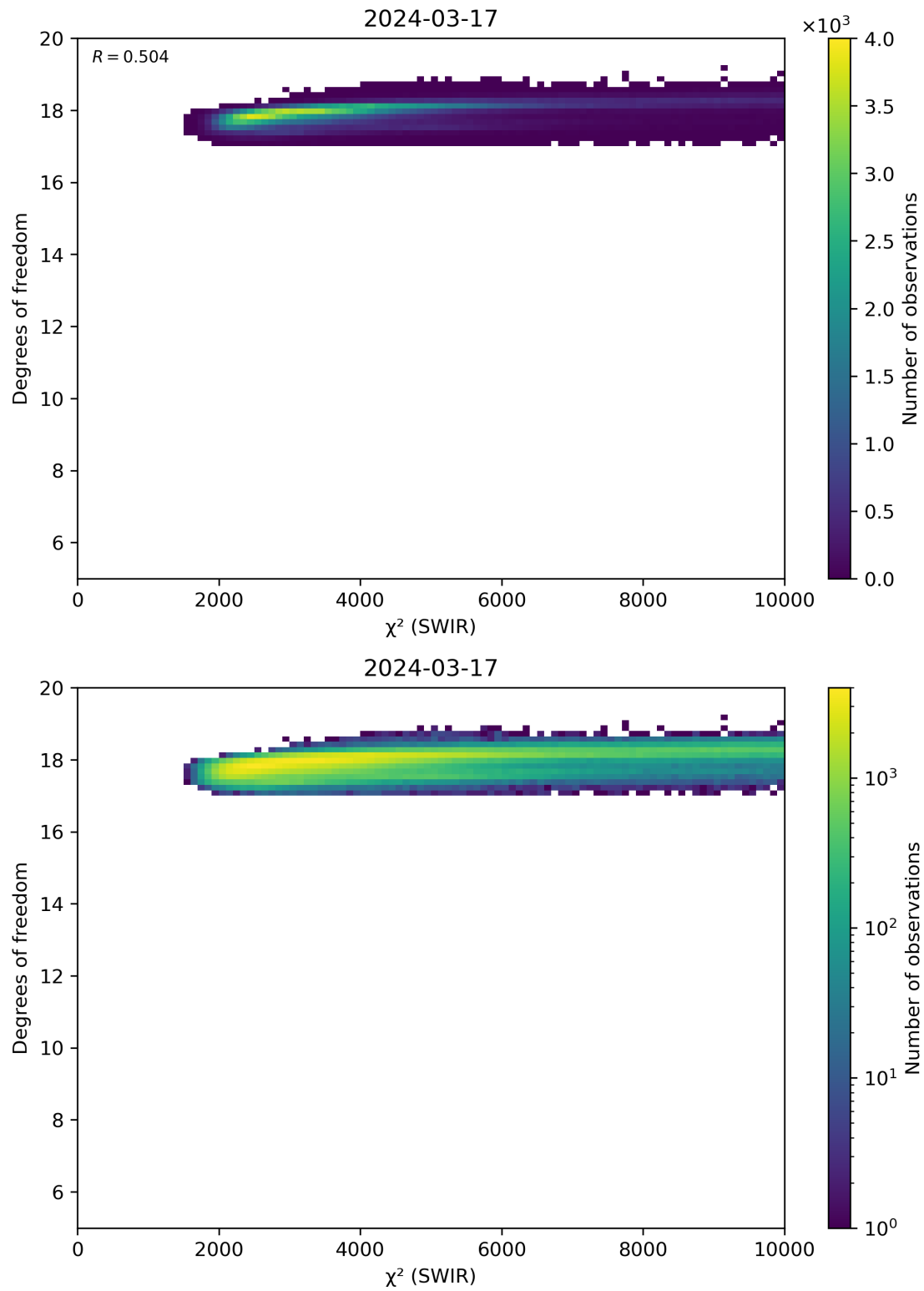
Figure 48: Scatter density plot of “ \chi^2 (SWIR)” against “Degrees of freedom” for 2024-03-16 to 2024-03-18.
