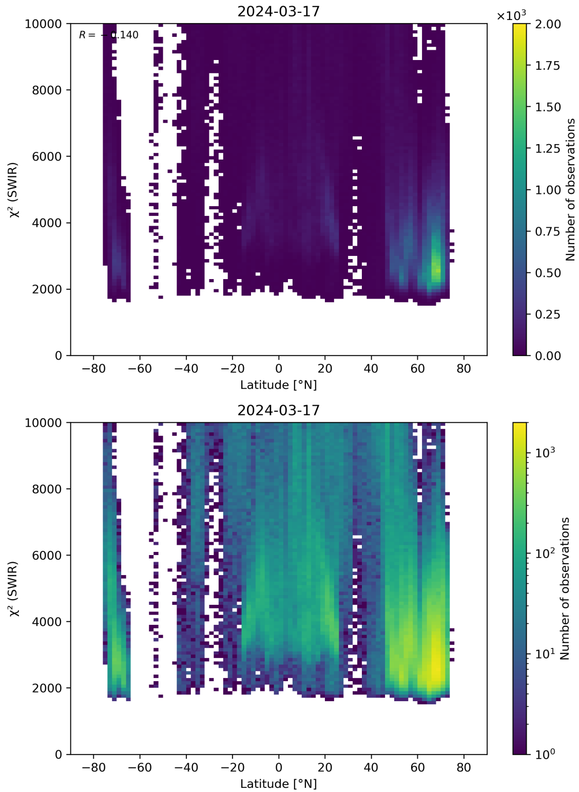
Figure 54: Scatter density plot of “Latitude” against “ \chi^2 (SWIR)” for 2024-03-16 to 2024-03-18.
