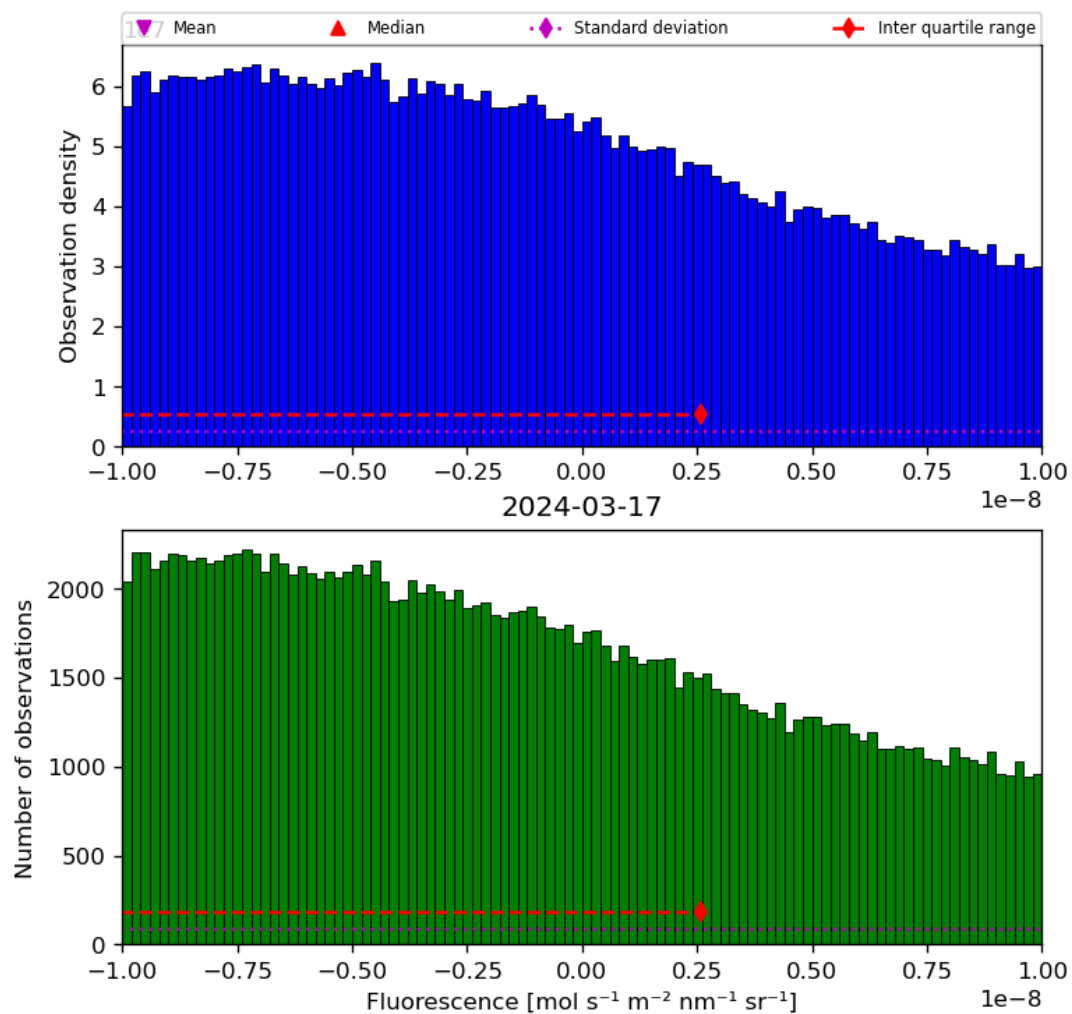
Figure 32: Histogram of “Fluorescence” for 2024-03-16 to 2024-03-18
