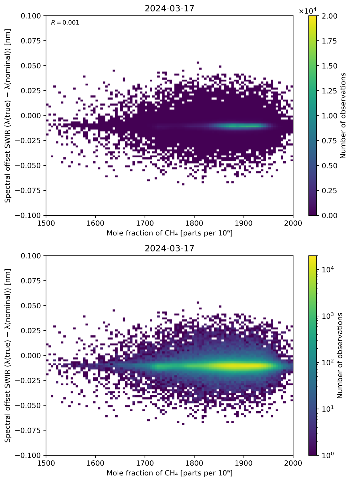
Figure 86: Scatter density plot of “Mole fraction of CH 4 ” against “Spectral offset SWIR ( \lambda(\text{true}) - \lambda(\text{nominal}) )” for 2024-03-16 to 2024-03-18.
