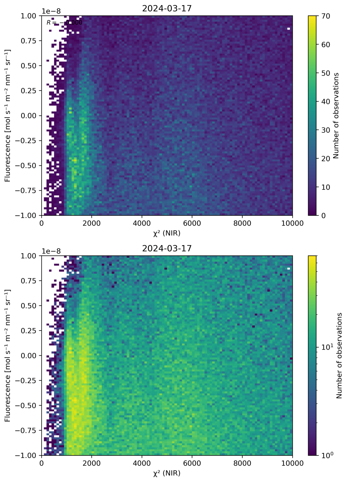
Figure 45: Scatter density plot of “ \chi^2 (NIR)” against “Fluorescence” for 2024-03-16 to 2024-03-18.
