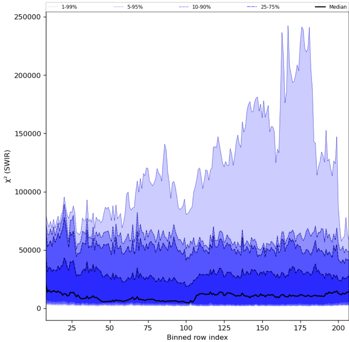
Figure 39: Along track statistics of " \chi^2 (SWIR)" for 2024-03-16 to 2024-03-18
