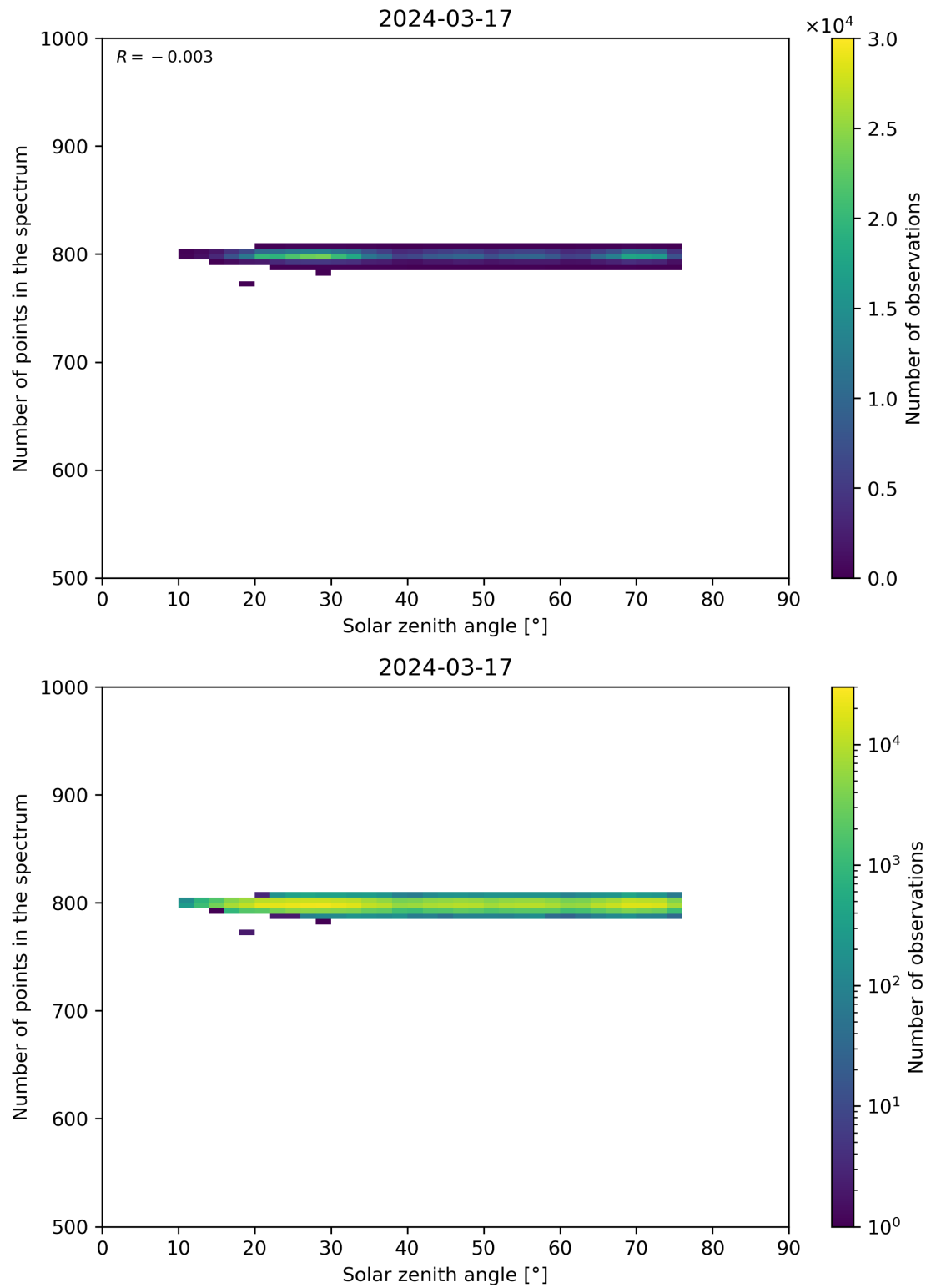
Figure 103: Scatter density plot of “Solar zenith angle” against “Number of points in the spectrum” for 2024-03-16 to 2024-03-18.
