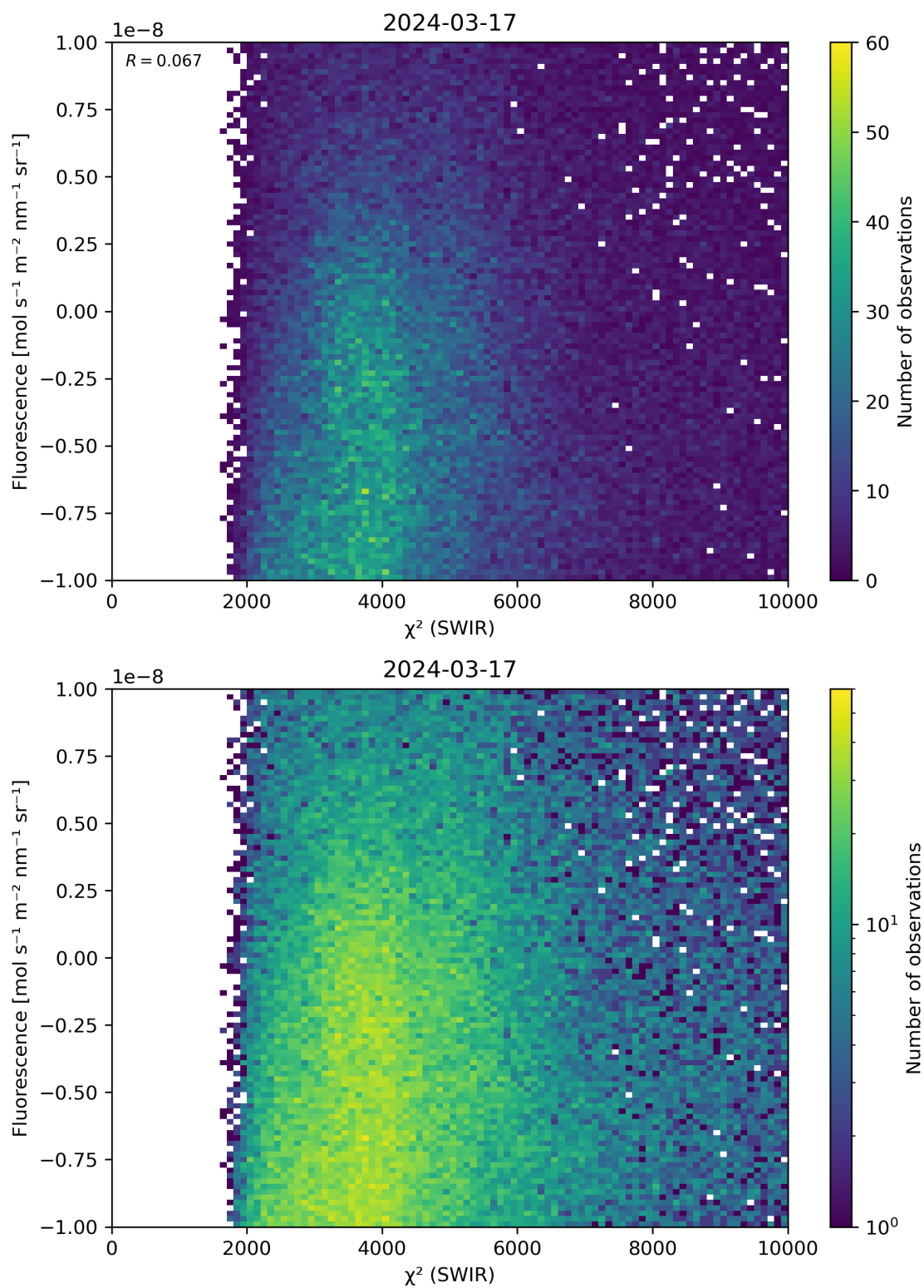
Figure 49: Scatter density plot of “ \chi^2 (SWIR)” against “Fluorescence” for 2024-03-16 to 2024-03-18.
