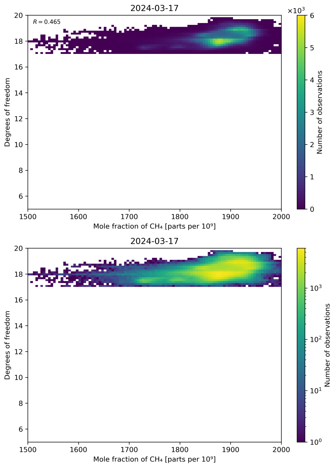
Figure 72: Scatter density plot of “Mole fraction of CH 4 ” against “Degrees of freedom” for 2024-03-16 to 2024-03-18.
