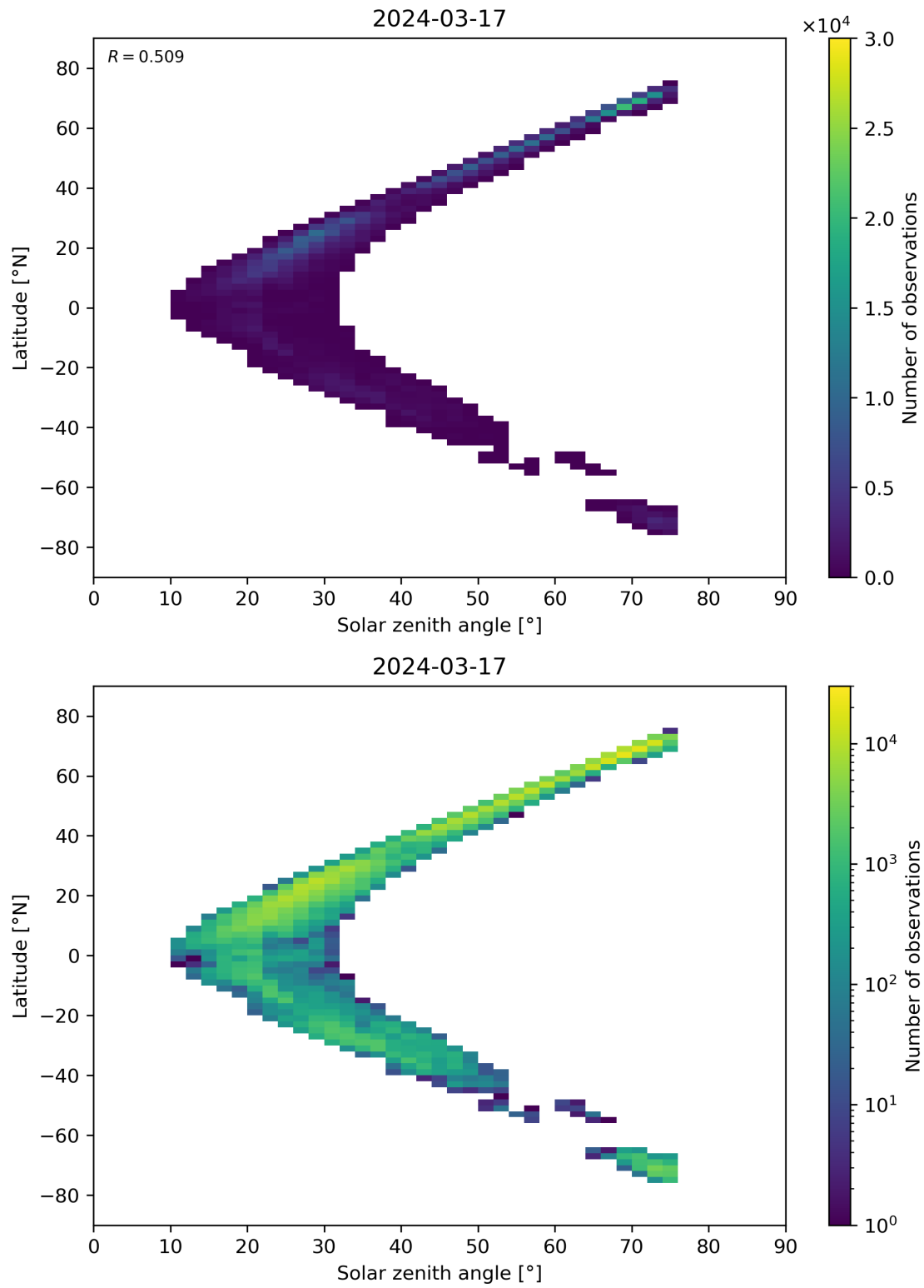
Figure 98: Scatter density plot of “Solar zenith angle” against “Latitude” for 2024-03-16 to 2024-03-18.
