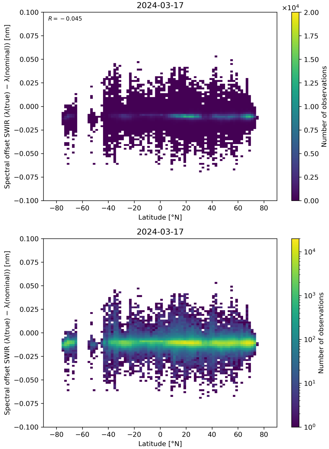
Figure 62: Scatter density plot of “Latitude” against “Spectral offset SWIR ( \lambda(\text{true}) - \lambda(\text{nominal}) )” for 2024-03-16 to 2024-03-18.
