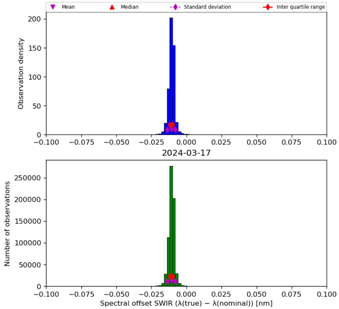
Figure 27: Histogram of “Spectral offset SWIR ( \lambda(\text{true}) - \lambda(\text{nominal}) )” for 2024-03-16 to 2024-03-18
