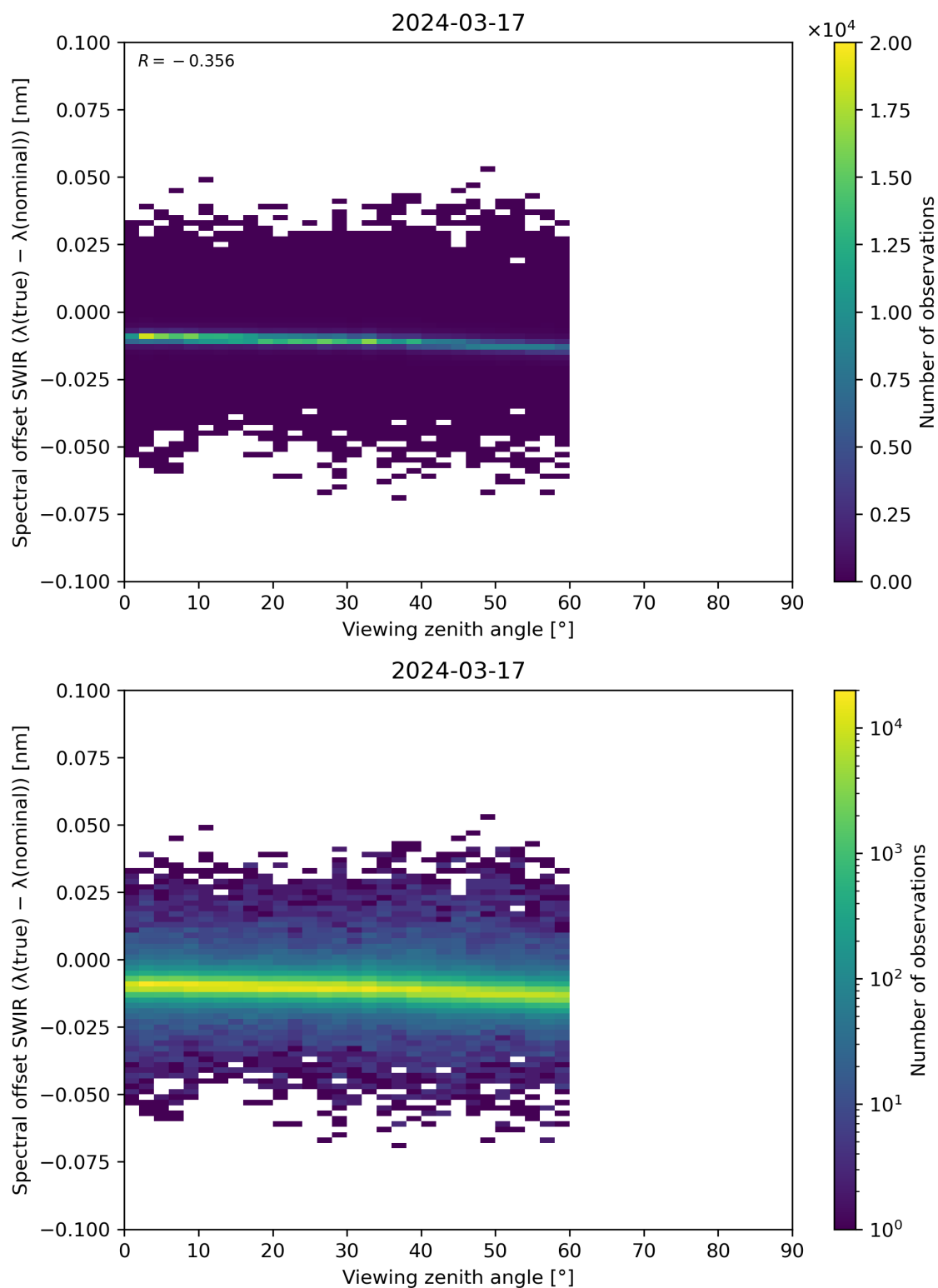
Figure 116: Scatter density plot of “Viewing zenith angle” against “Spectral offset SWIR ( \lambda(\text{true}) - \lambda(\text{nominal}) )” for 2024-03-16 to 2024-03-18.
