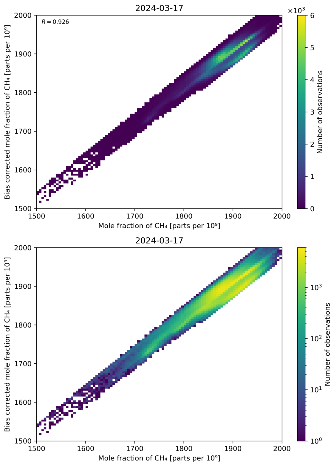
Figure 74: Scatter density plot of “Mole fraction of CH 4 ” against “Bias corrected mole fraction of CH 4 ” for 2024-03-16 to 2024-03-18.
