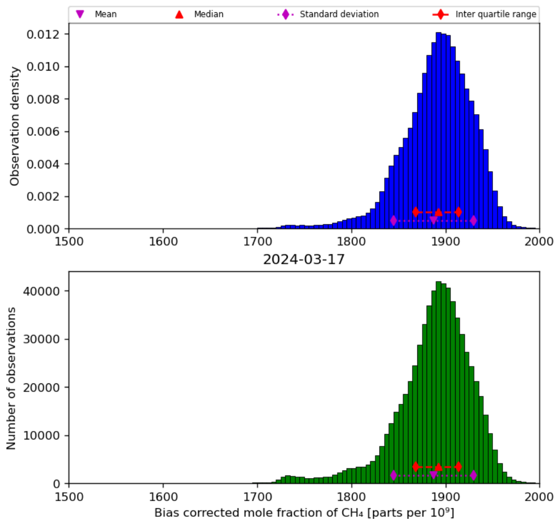
Figure 25: Histogram of “Bias corrected mole fraction of CH 4 ” for 2024-03-16 to 2024-03-18
