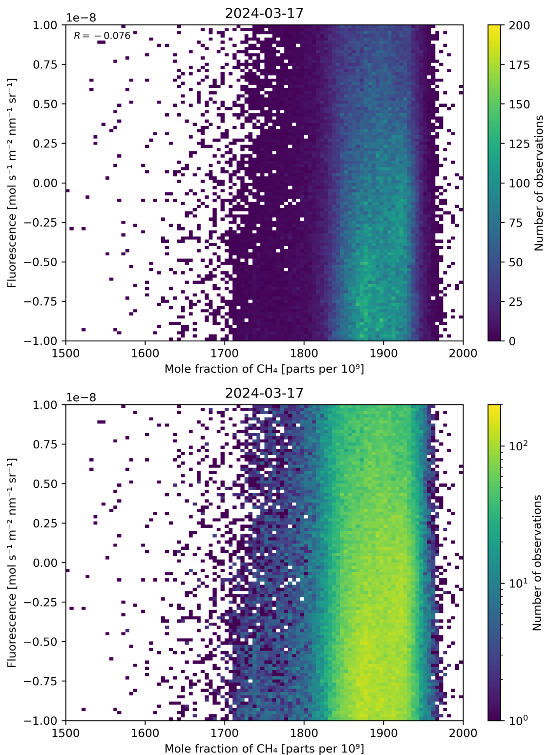
Figure 73: Scatter density plot of “Mole fraction of \text{CH}_4 ” against “Fluorescence” for 2024-03-16 to 2024-03-18.
