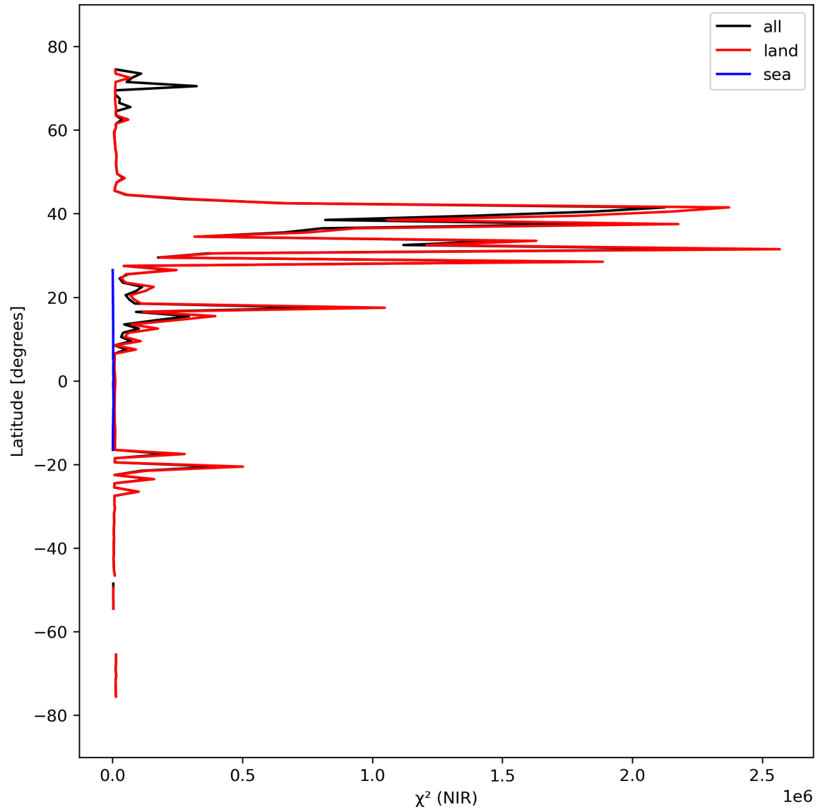
Figure 18: Zonal average of “ \chi^2 (NIR)” for 2024-03-16 to 2024-03-18.
