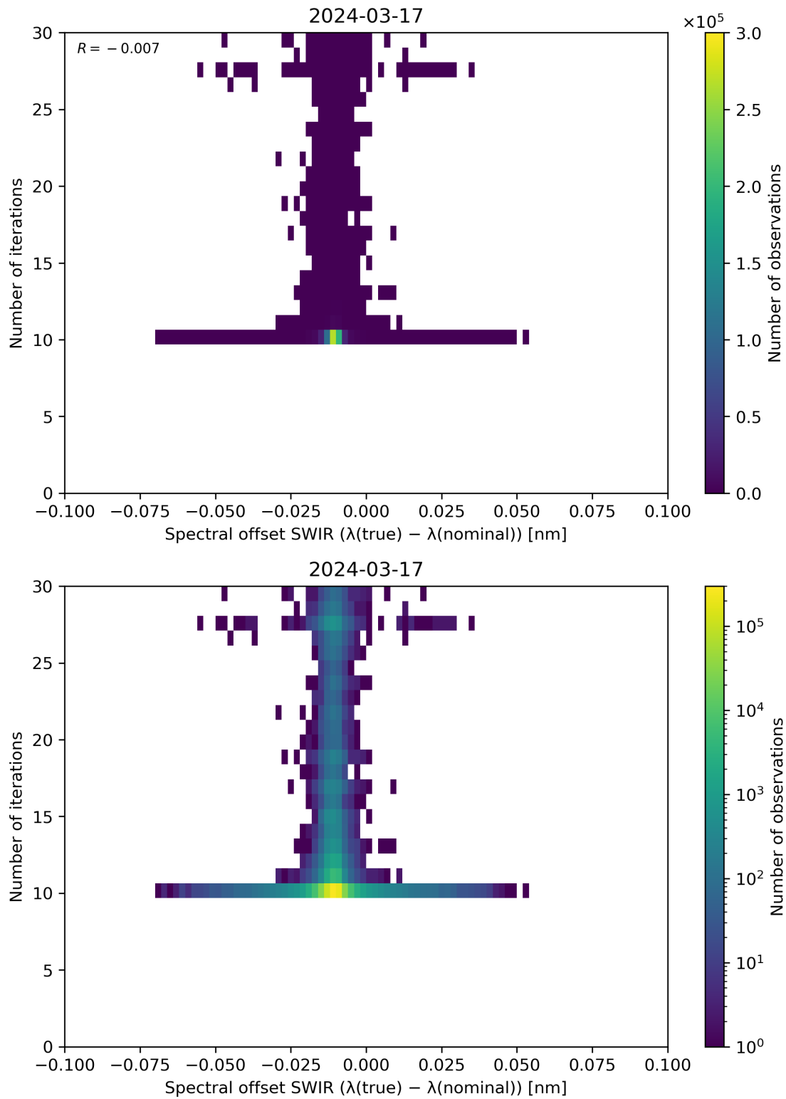
Figure 121: Scatter density plot of “Spectral offset SWIR ( \lambda(\text{true}) - \lambda(\text{nominal}) )” against “Number of iterations” for 2024-03-16 to 2024-03-18.
