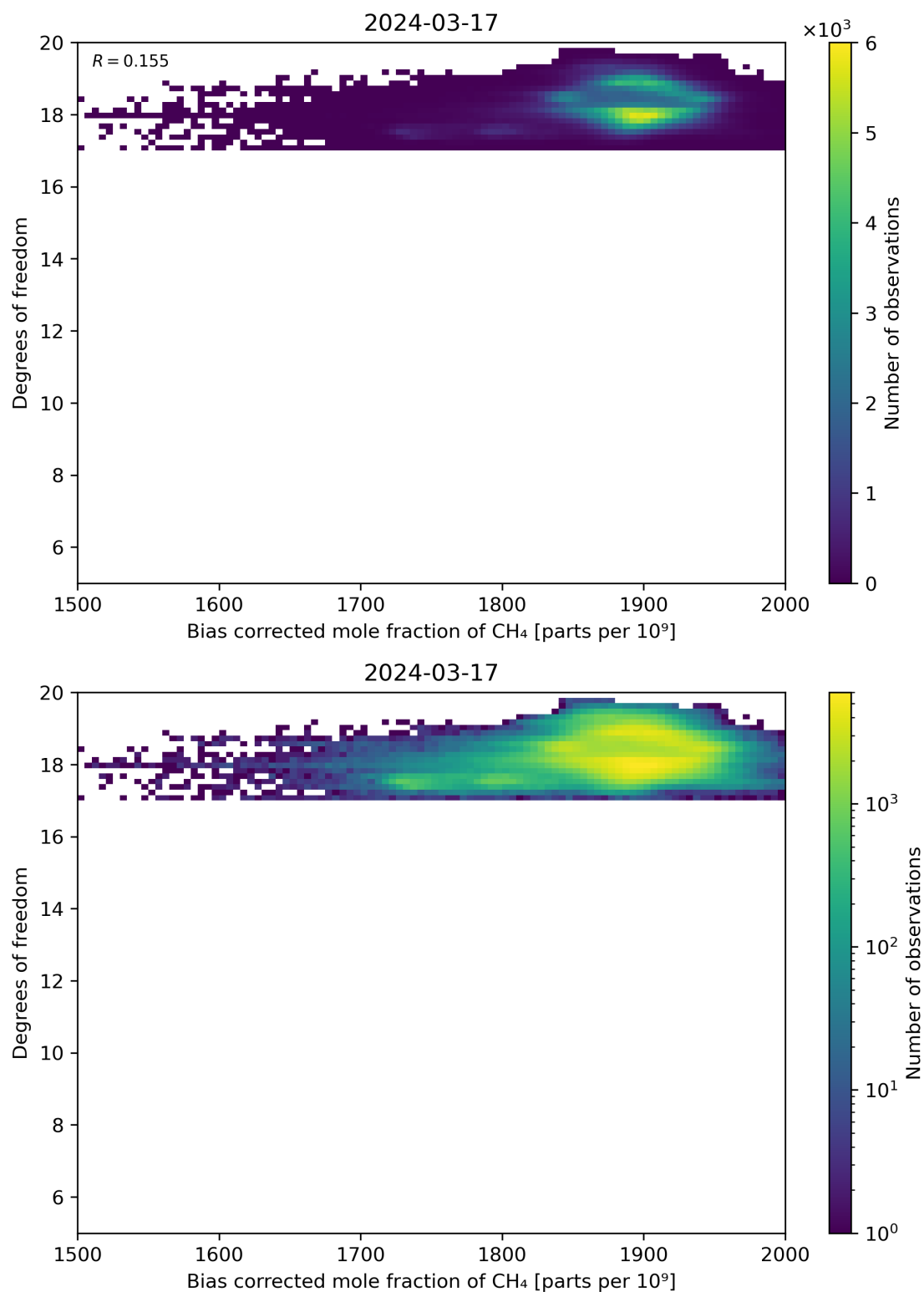
Figure 65: Scatter density plot of “Bias corrected mole fraction of CH 4 ” against “Degrees of freedom” for 2024-03-16 to 2024-03-18.
