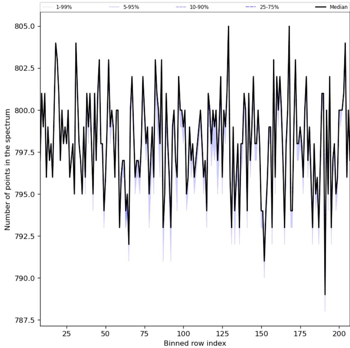
Figure 37: Along track statistics of “Number of points in the spectrum” for 2024-03-16 to 2024-03-18
