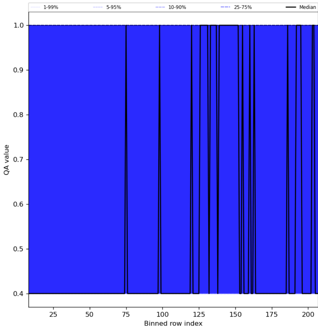
Figure 33: Along track statistics of “QA value” for 2024-03-16 to 2024-03-18
