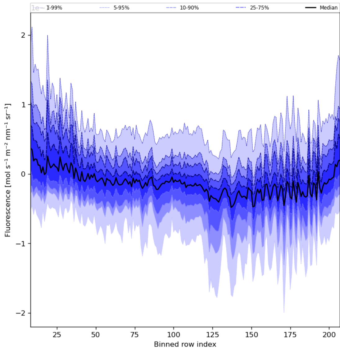
Figure 43: Along track statistics of “Fluorescence” for 2024-03-16 to 2024-03-18
