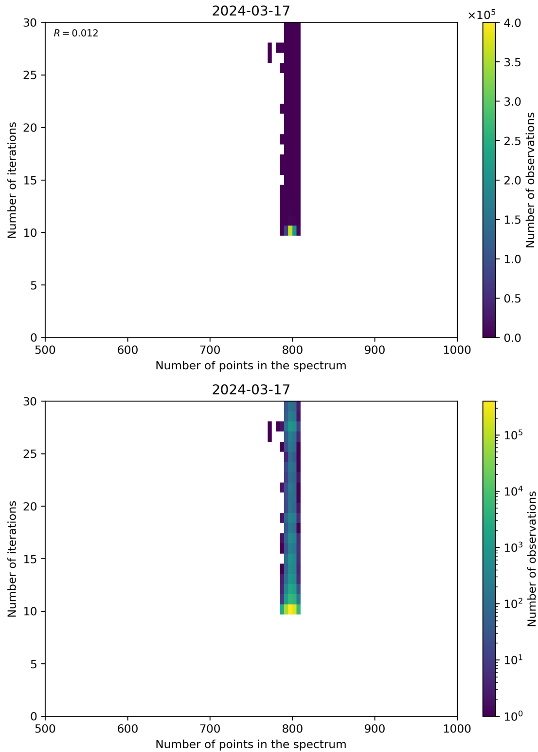
Figure 92: Scatter density plot of “Number of points in the spectrum” against “Number of iterations” for 2024-03-16 to 2024-03-18.
