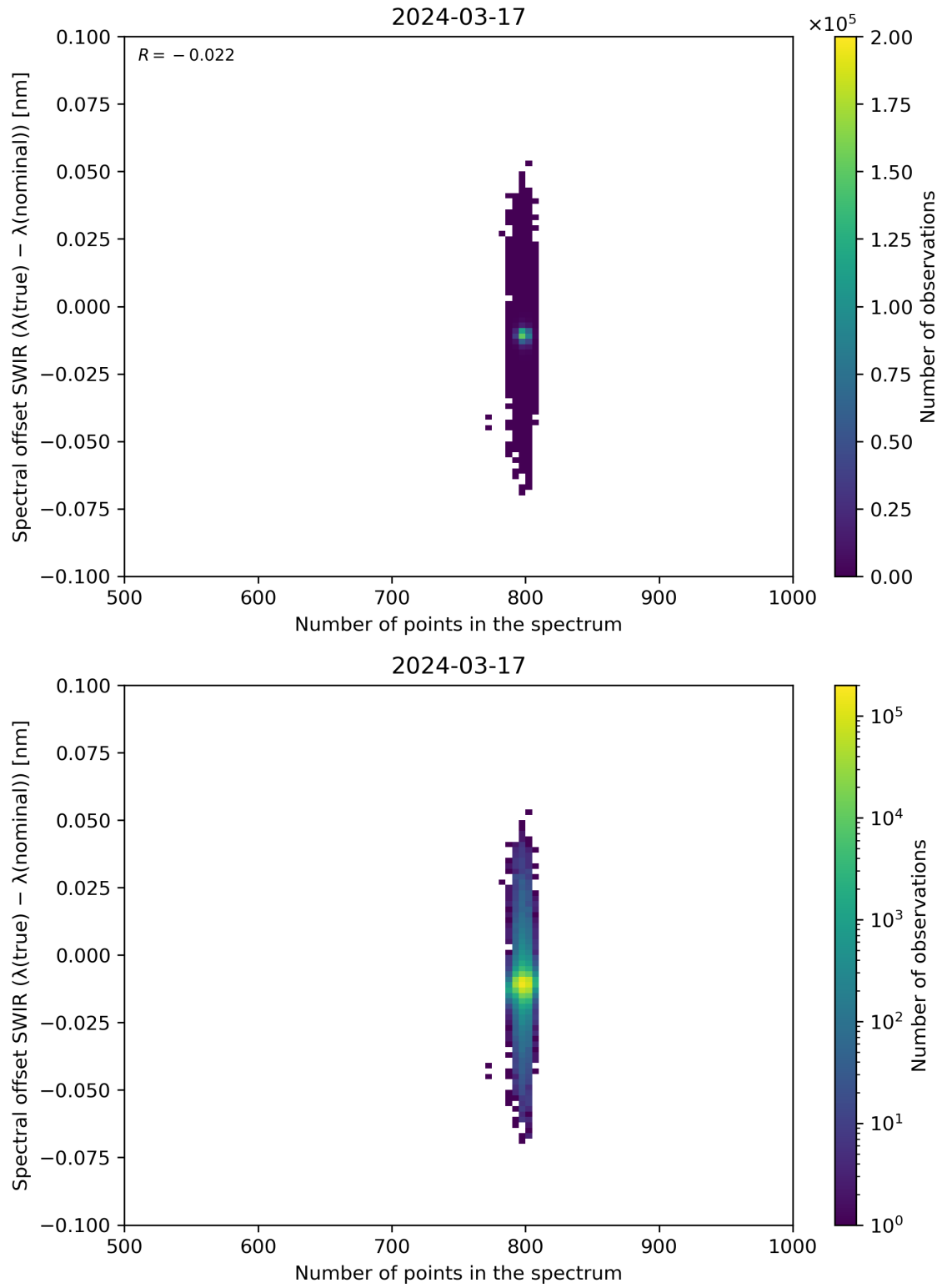
Figure 93: Scatter density plot of “Number of points in the spectrum” against “Spectral offset SWIR ( \lambda(\text{true}) - \lambda(\text{nominal}) )” for 2024-03-16 to 2024-03-18.
