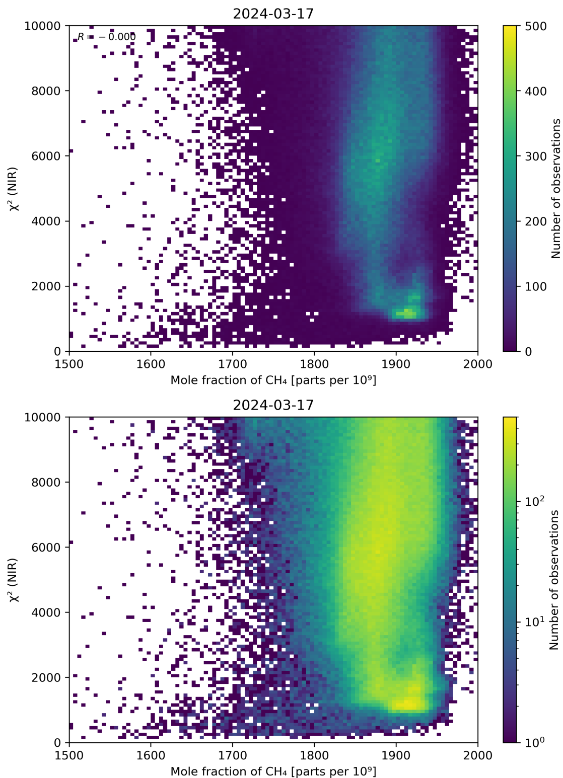
Figure 70: Scatter density plot of “Mole fraction of \text{CH}_4 ” against “ \chi^2 (NIR)” for 2024-03-16 to 2024-03-18.
