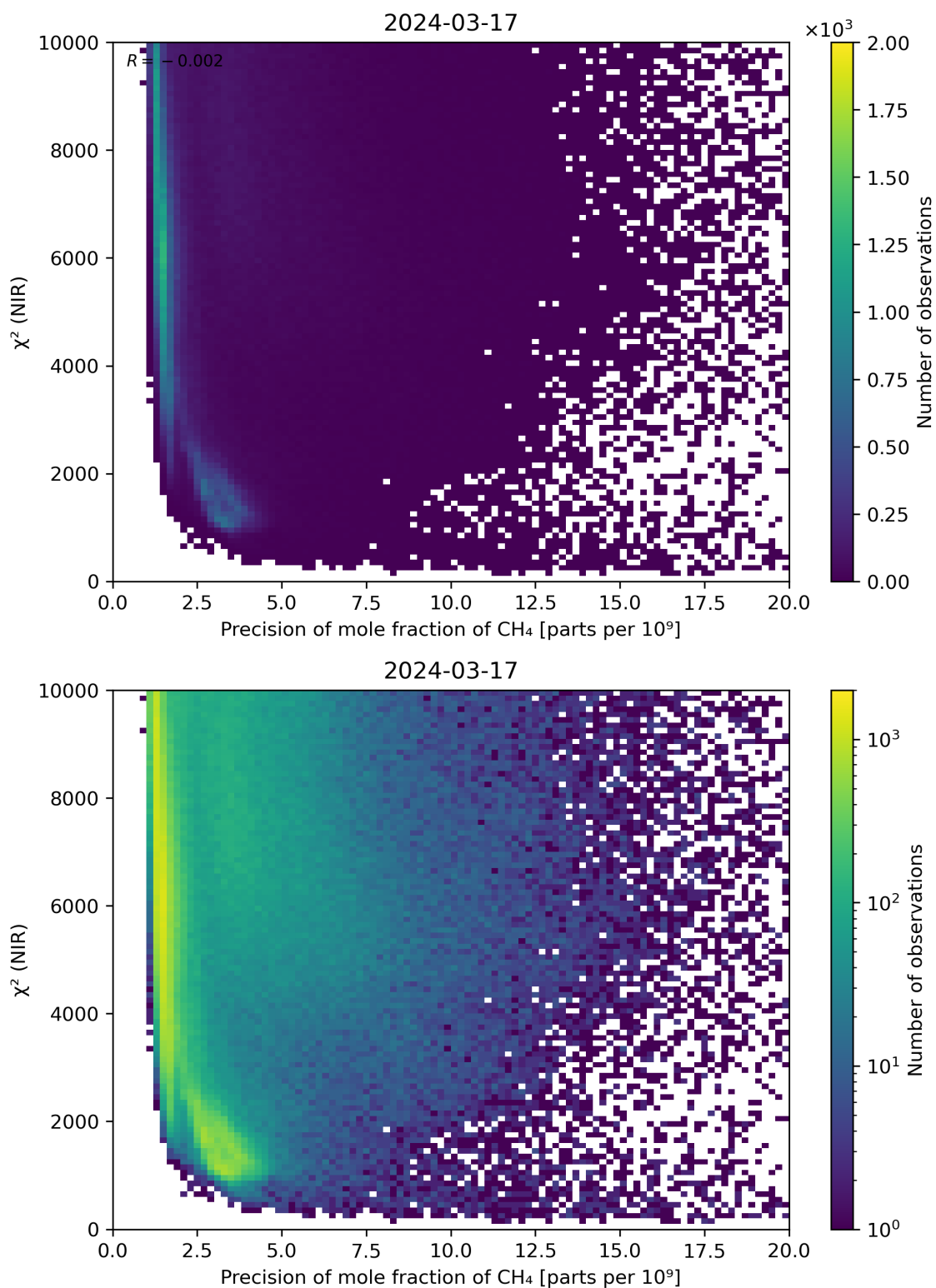
Figure 78: Scatter density plot of “Precision of mole fraction of CH 4 ” against “ \chi^2 (NIR)” for 2024-03-16 to 2024-03-18.
