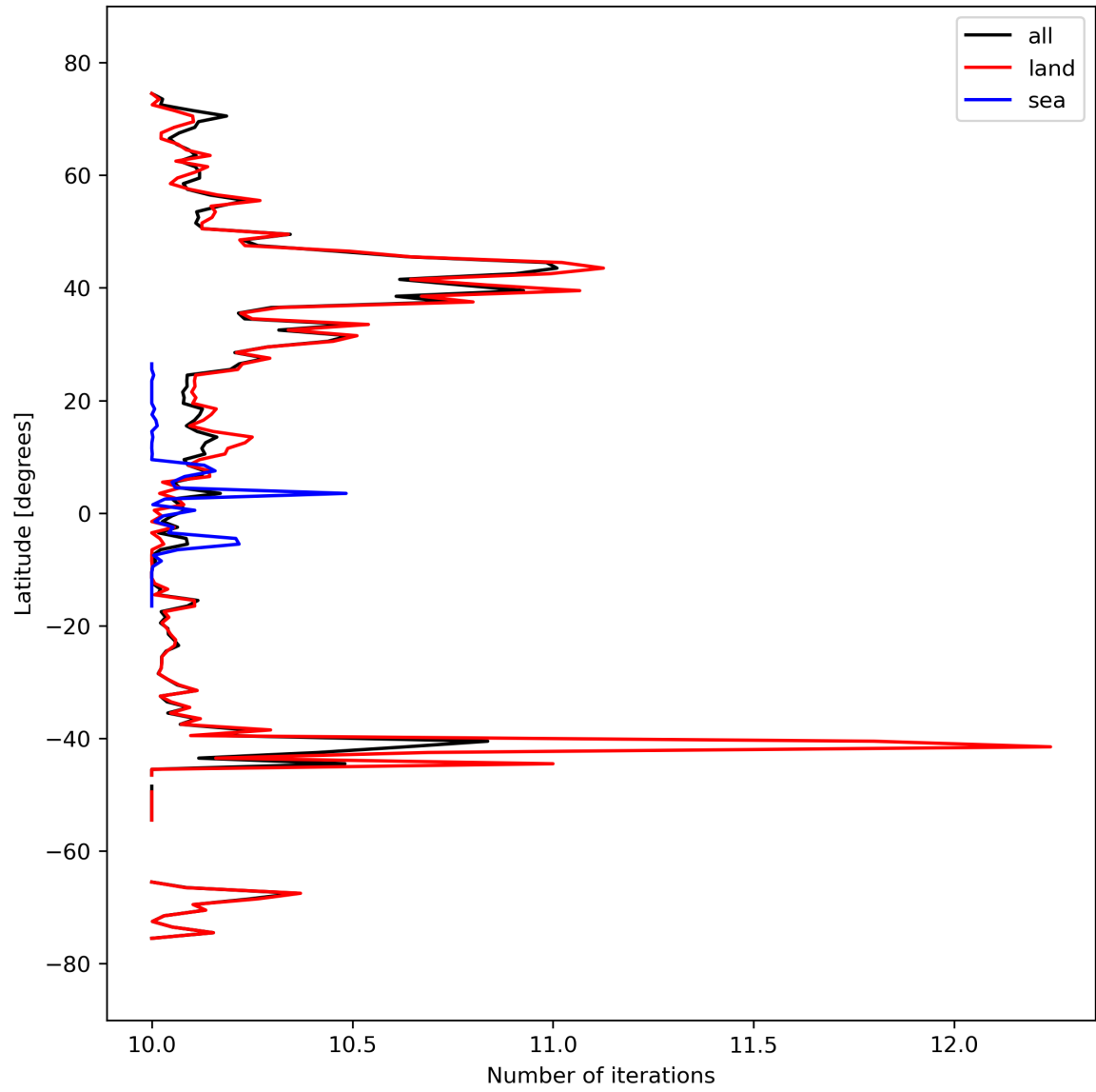
Figure 20: Zonal average of “Number of iterations” for 2024-03-16 to 2024-03-18.
