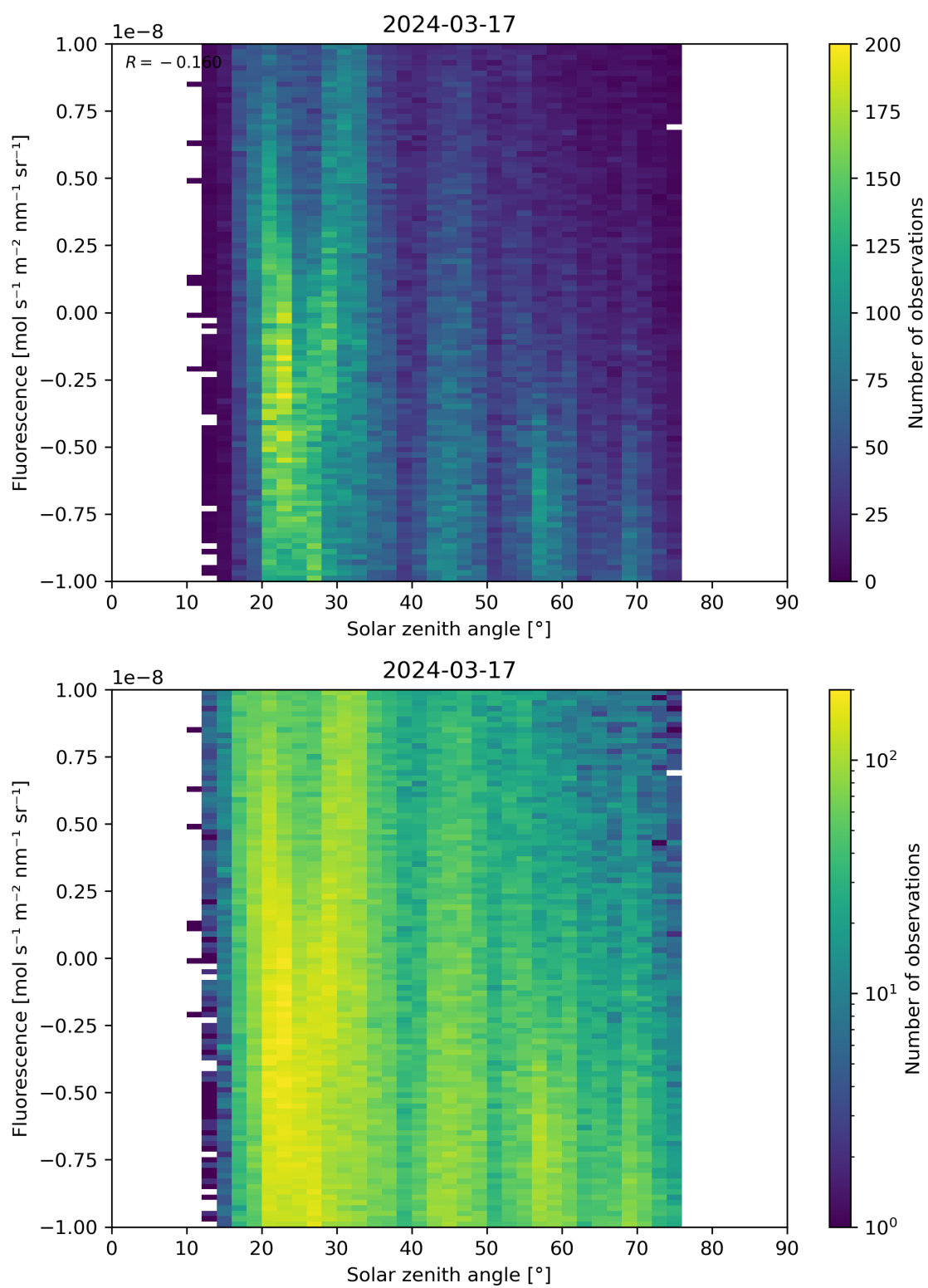
Figure 97: Scatter density plot of “Solar zenith angle” against “Fluorescence” for 2024-03-16 to 2024-03-18.
