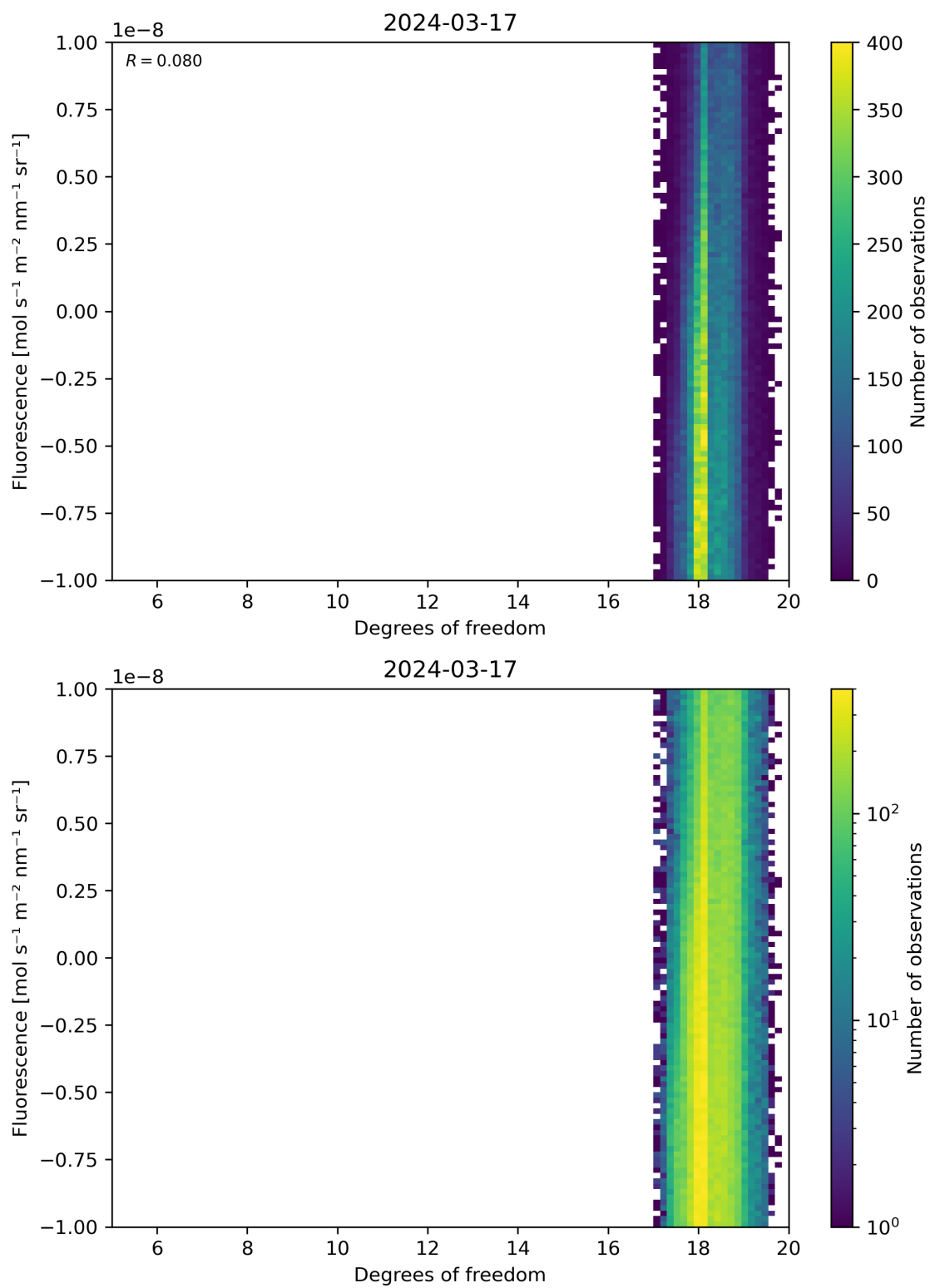
Figure 51: Scatter density plot of “Degrees of freedom” against “Fluorescence” for 2024-03-16 to 2024-03-18.
