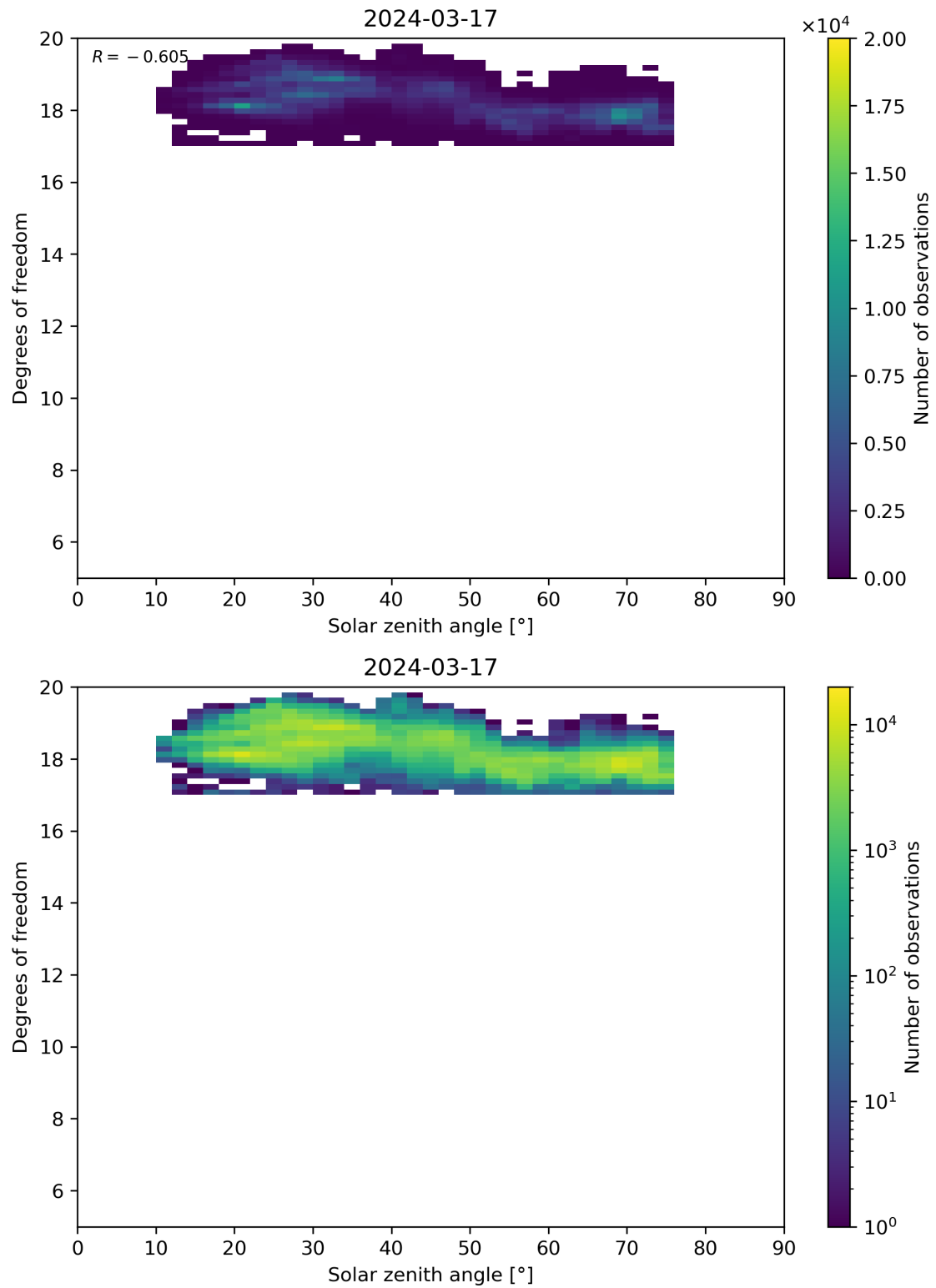
Figure 96: Scatter density plot of “Solar zenith angle” against “Degrees of freedom” for 2024-03-16 to 2024-03-18.
