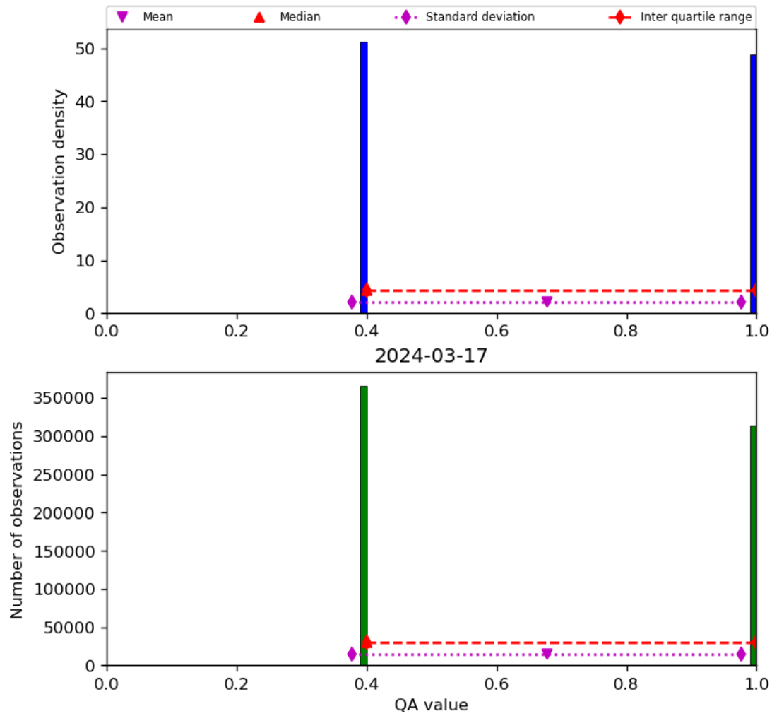
Figure 22: Histogram of “QA value” for 2024-03-16 to 2024-03-18
