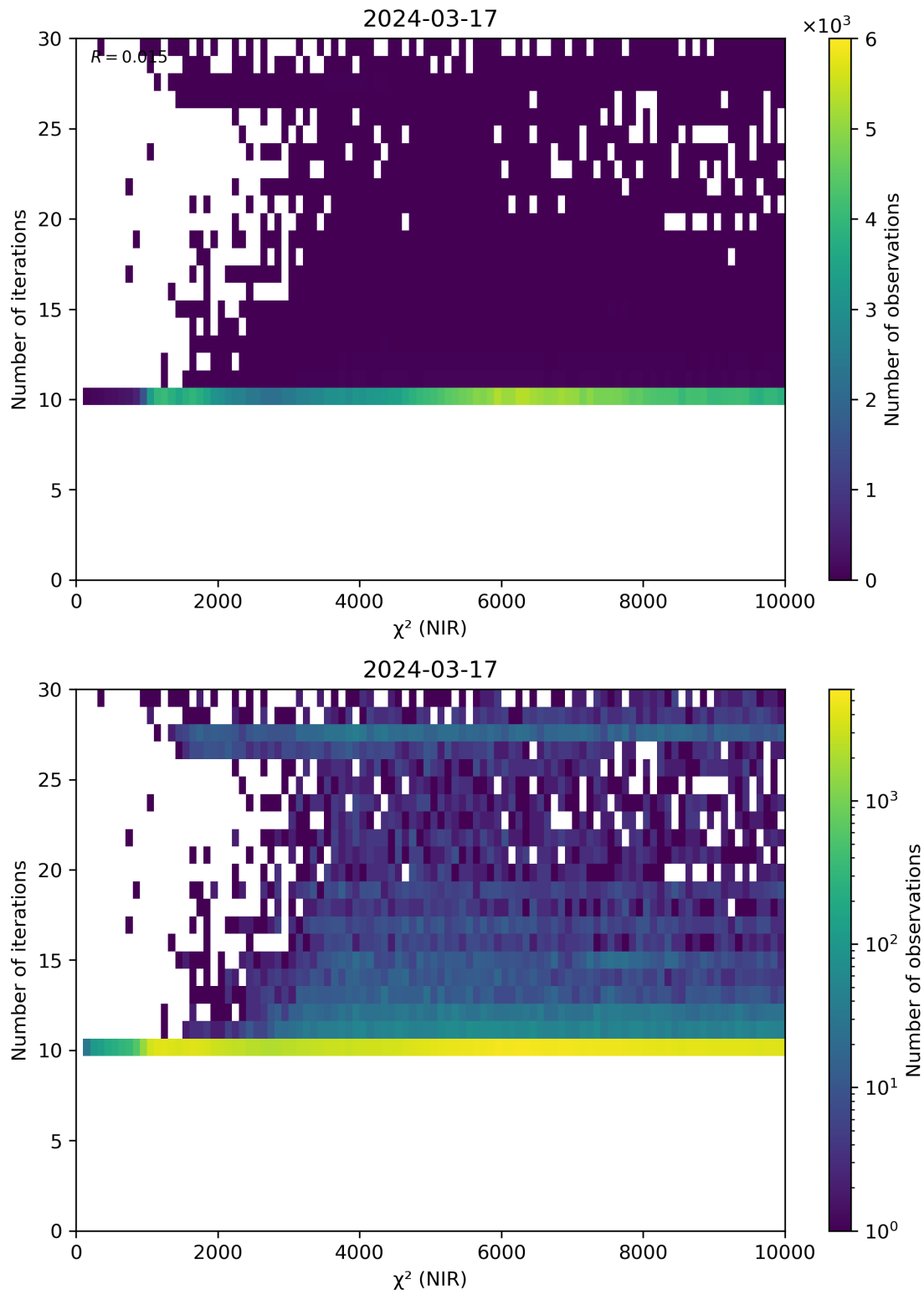
Figure 46: Scatter density plot of “ \chi^2 (NIR)” against “Number of iterations” for 2024-03-16 to 2024-03-18.
