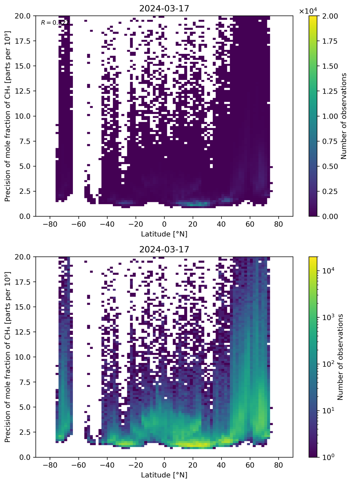
Figure 59: Scatter density plot of “Latitude” against “Precision of mole fraction of \text{CH}_4 ” for 2024-03-16 to 2024-03-18.
