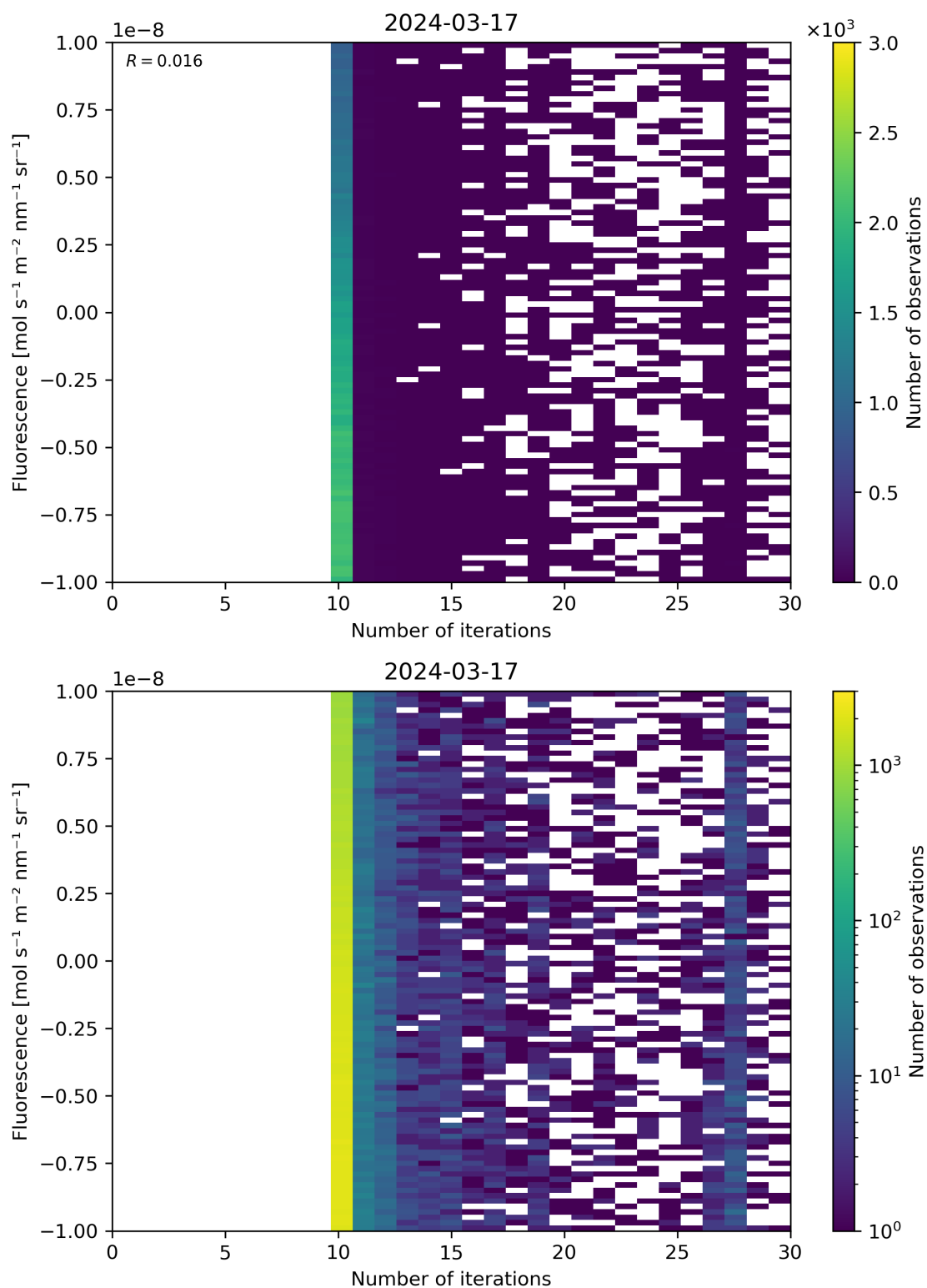
Figure 87: Scatter density plot of “Number of iterations” against “Fluorescence” for 2024-03-16 to 2024-03-18.
