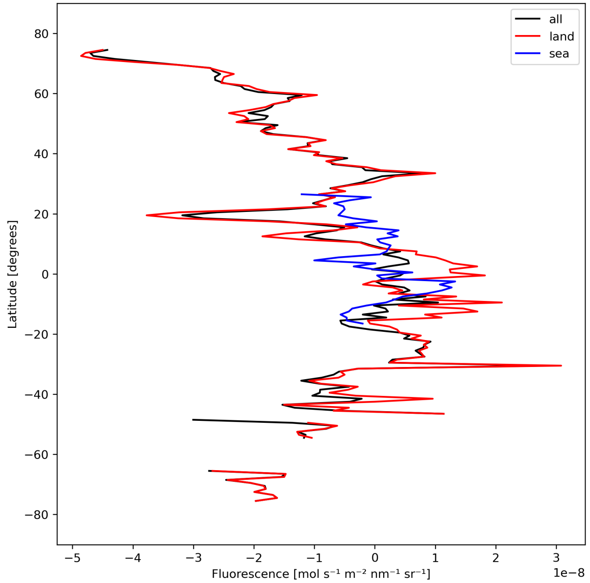
Figure 21: Zonal average of “Fluorescence” for 2024-03-16 to 2024-03-18.
