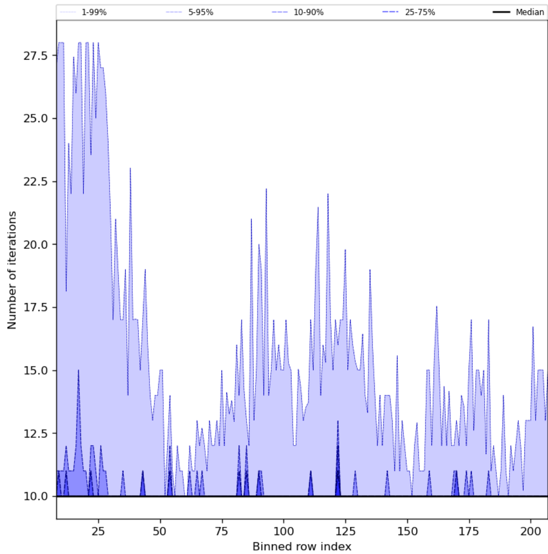
Figure 42: Along track statistics of “Number of iterations” for 2024-03-16 to 2024-03-18
