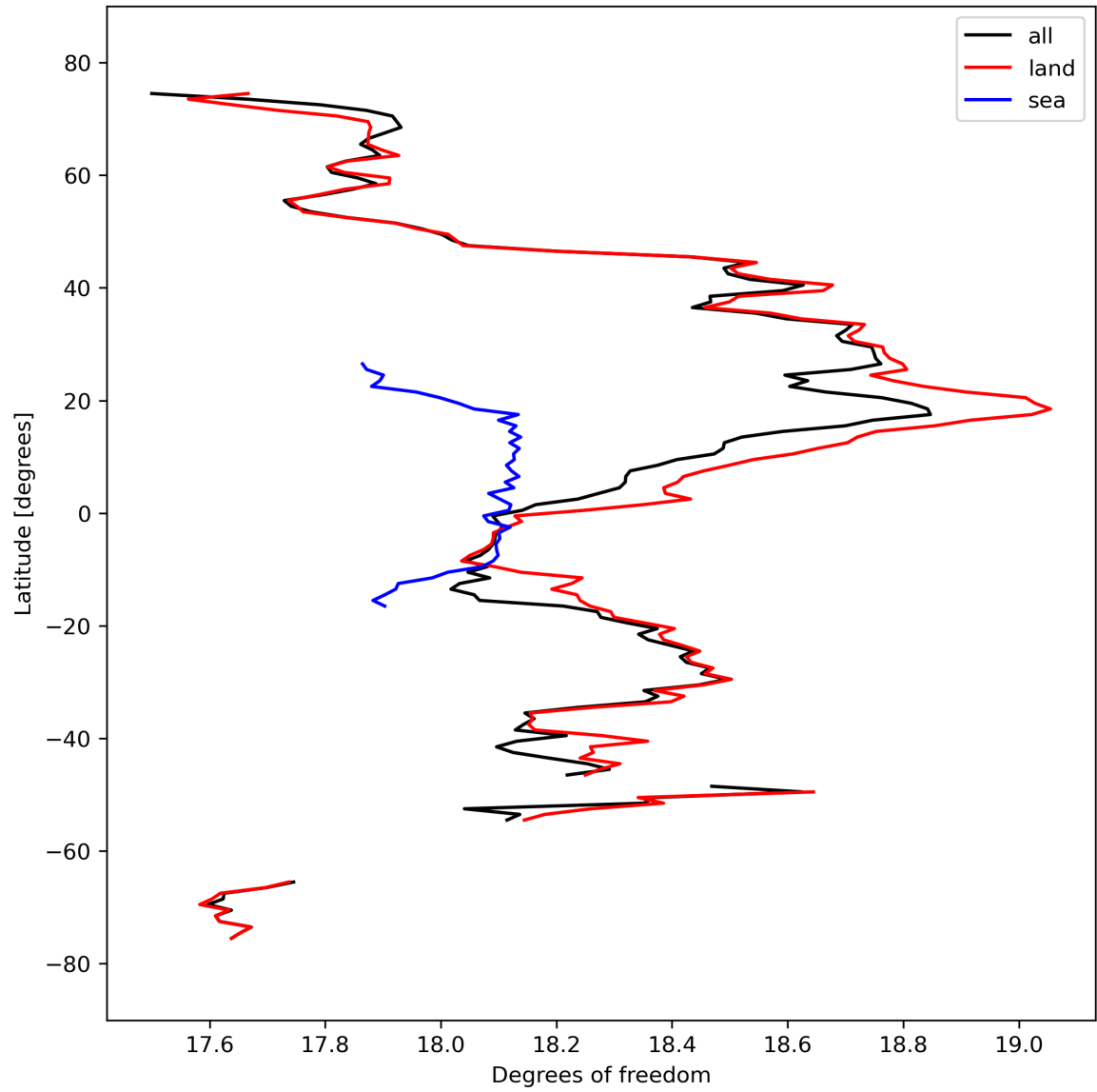
Figure 19: Zonal average of “Degrees of freedom” for 2024-03-16 to 2024-03-18.
