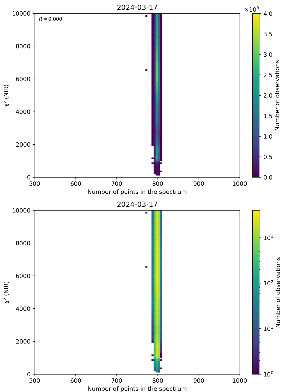
Figure 88: Scatter density plot of “Number of points in the spectrum” against “ \chi^2 (NIR)” for 2024-03-16 to 2024-03-18.
