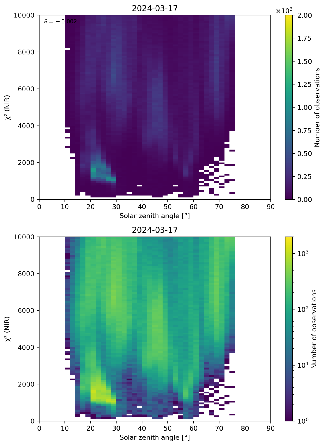
Figure 94: Scatter density plot of “Solar zenith angle” against “ \chi^2 (NIR)” for 2024-03-16 to 2024-03-18.
