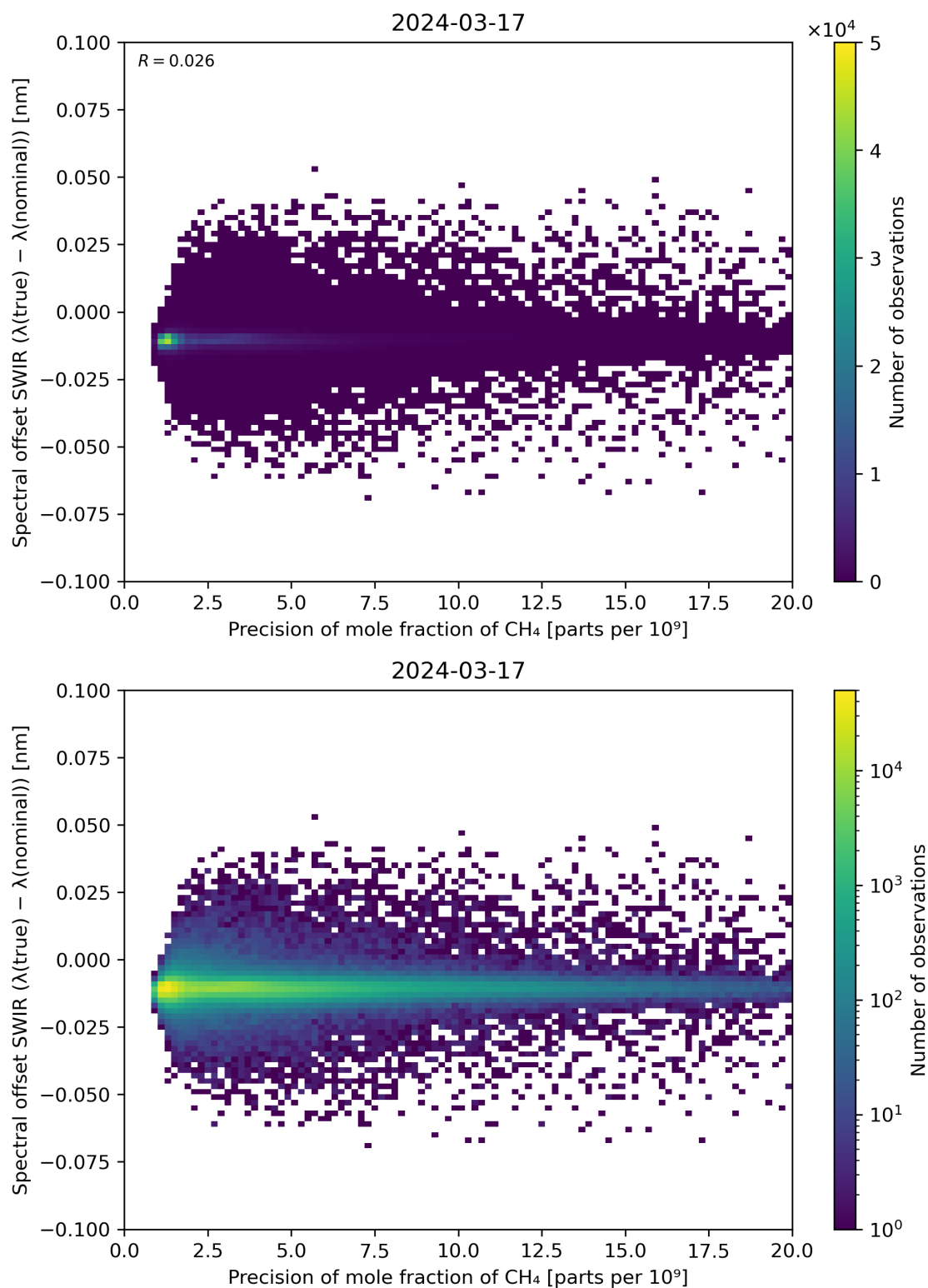
Figure 85: Scatter density plot of “Precision of mole fraction of CH 4 ” against “Spectral offset SWIR ( \lambda(\text{true}) - \lambda(\text{nominal}) )” for 2024-03-16 to 2024-03-18.
