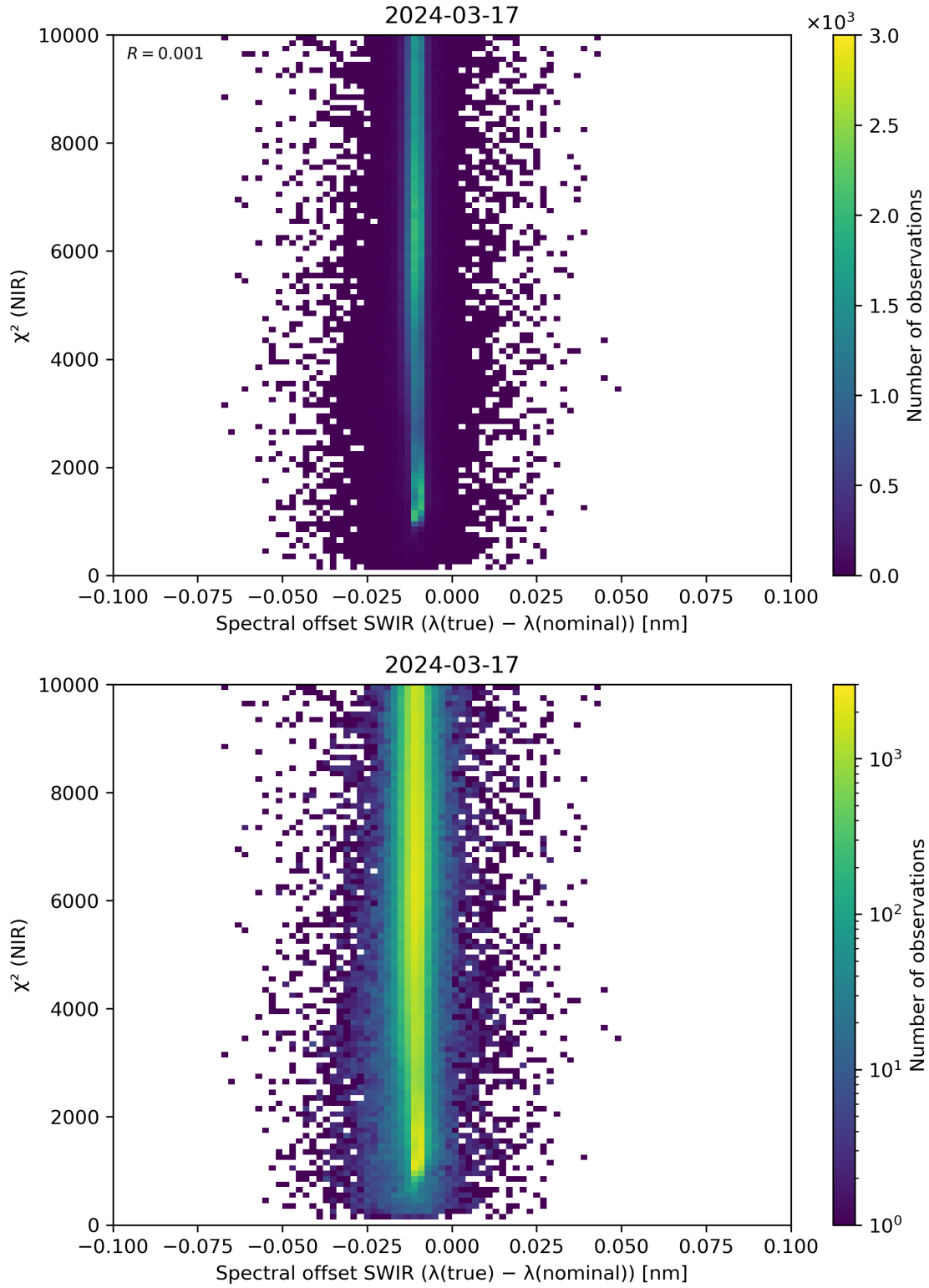
Figure 117: Scatter density plot of “Spectral offset SWIR ( \lambda(\text{true}) - \lambda(\text{nominal}) )” against “ \chi^2 (NIR)” for 2024-03-16 to 2024-03-18.
