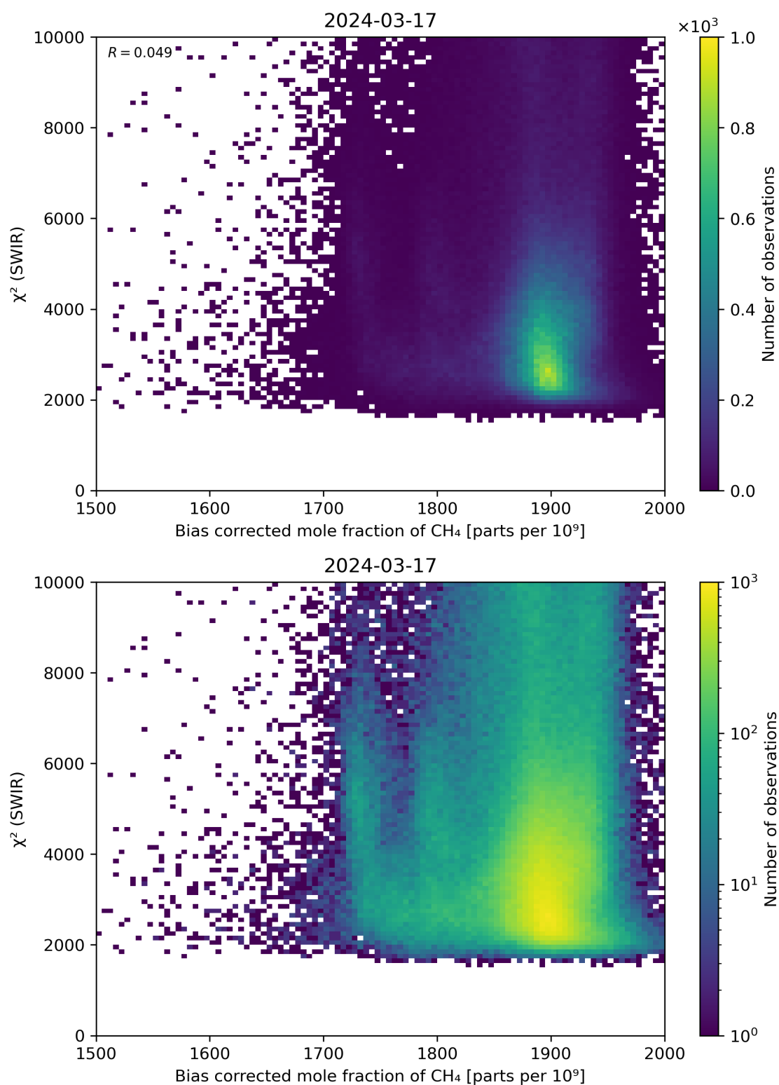
Figure 64: Scatter density plot of “Bias corrected mole fraction of \text{CH}_4 ” against “ \chi^2 (SWIR)” for 2024-03-16 to 2024-03-18.
