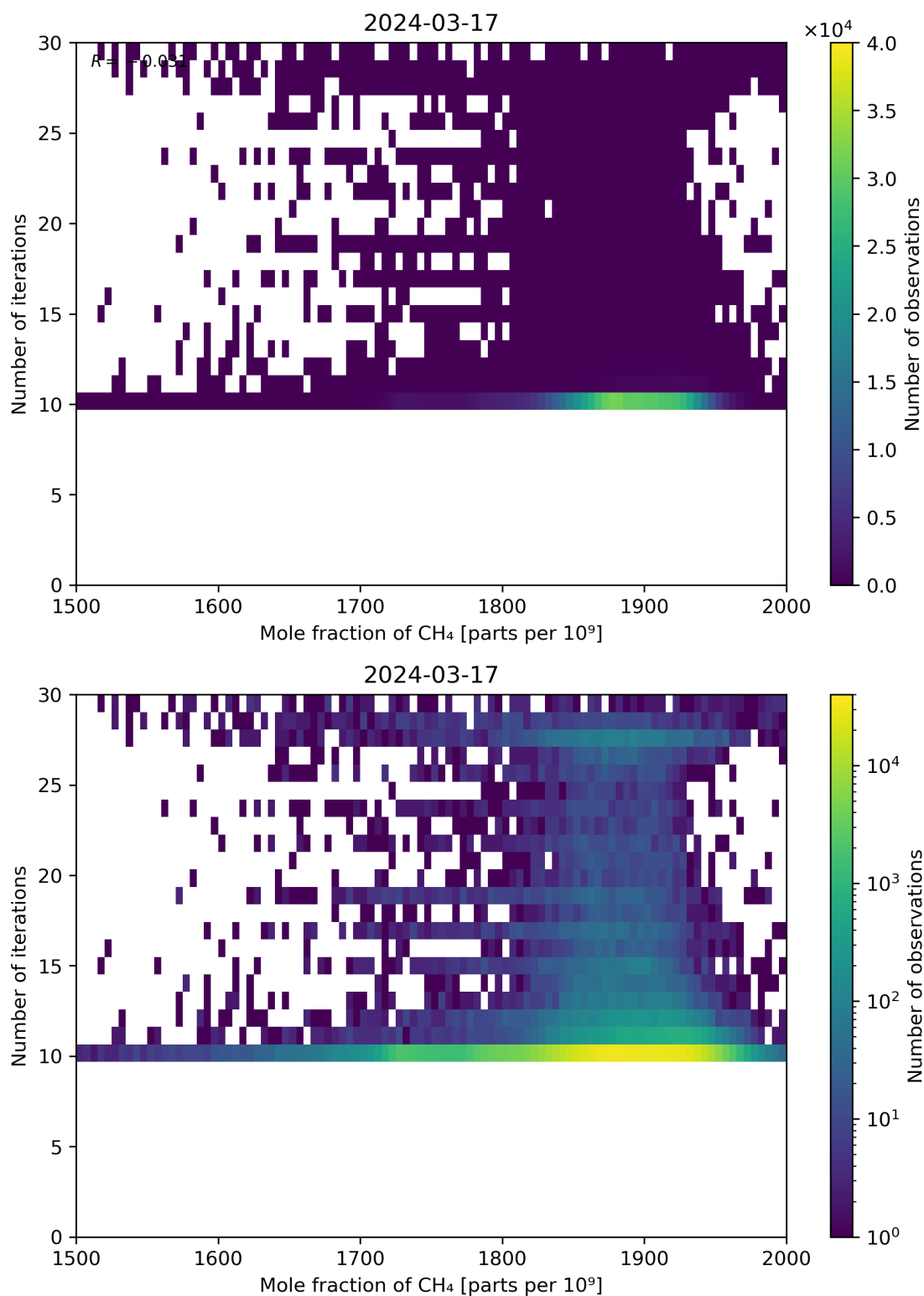
Figure 76: Scatter density plot of “Mole fraction of CH 4 ” against “Number of iterations” for 2024-03-16 to 2024-03-18.
