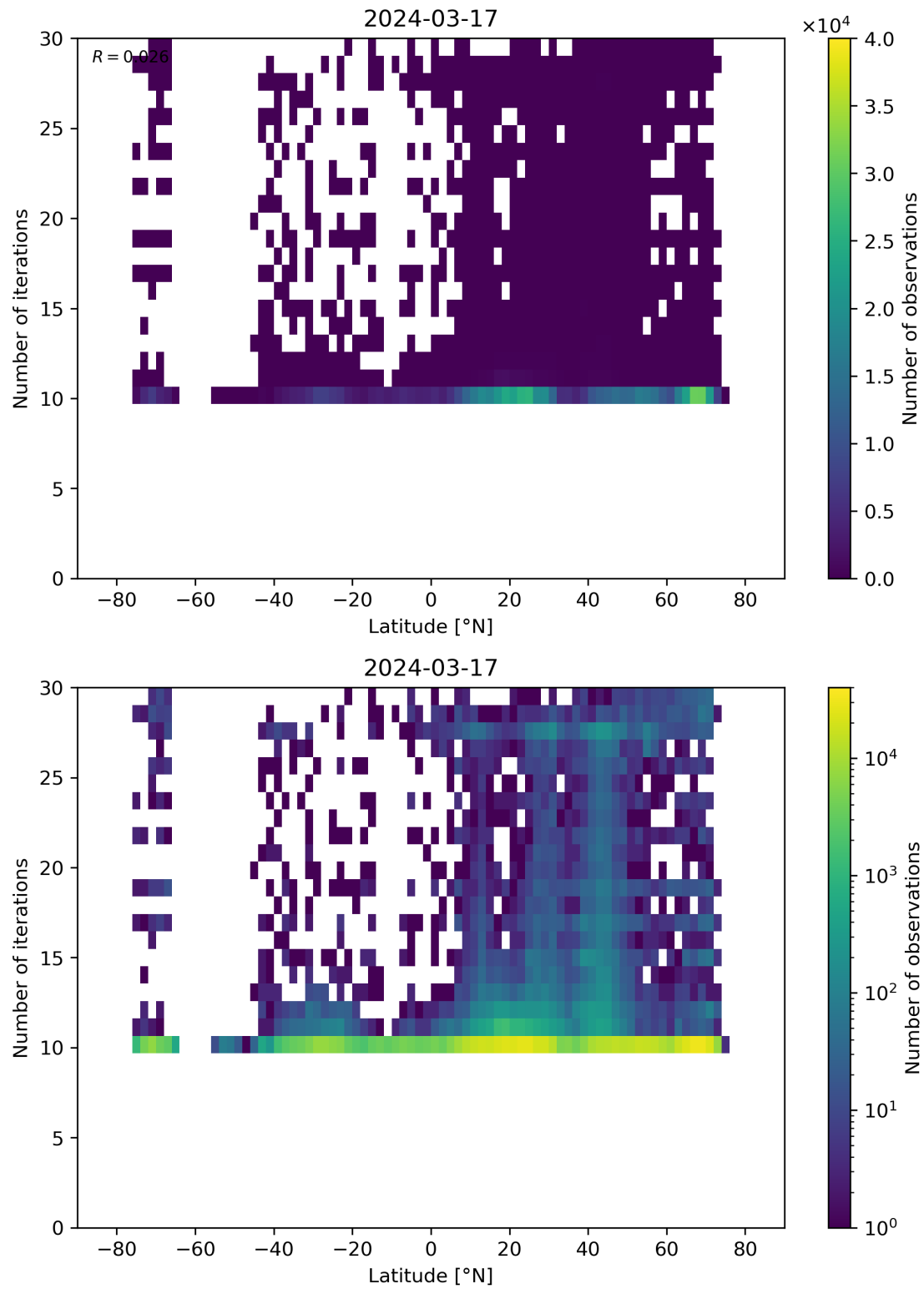
Figure 60: Scatter density plot of “Latitude” against “Number of iterations” for 2024-03-16 to 2024-03-18.
