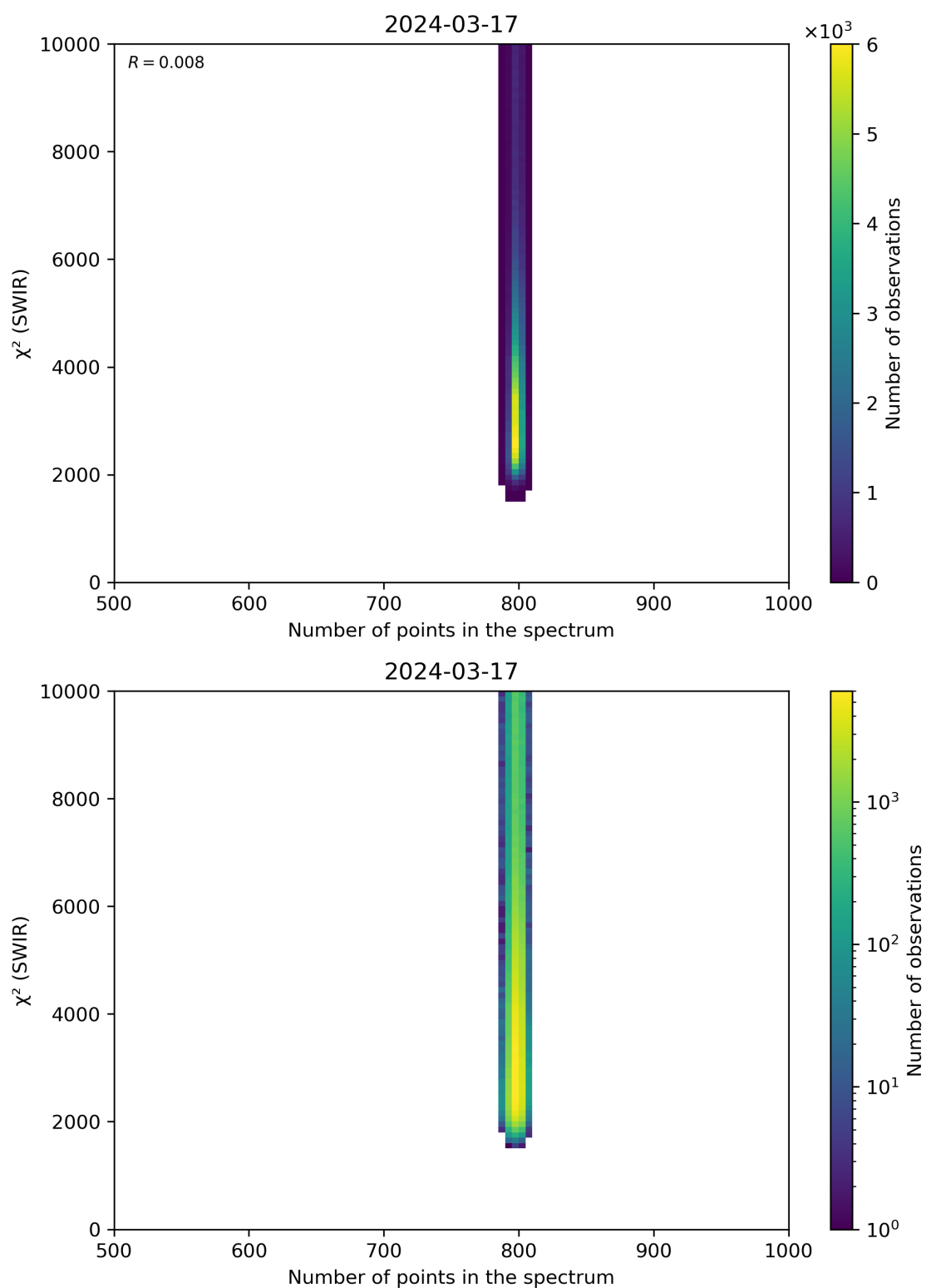
Figure 89: Scatter density plot of “Number of points in the spectrum” against “ \chi^2 (SWIR)” for 2024-03-16 to 2024-03-18.
