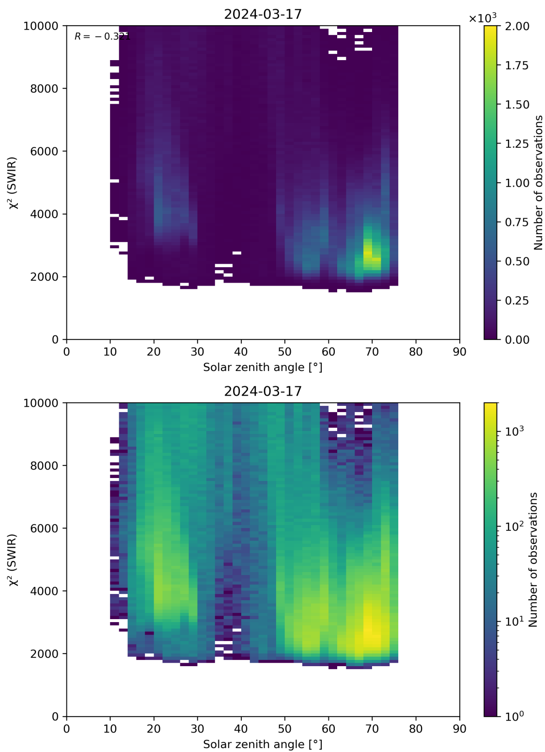
Figure 95: Scatter density plot of “Solar zenith angle” against “ \chi^2 (SWIR)” for 2024-03-16 to 2024-03-18.
