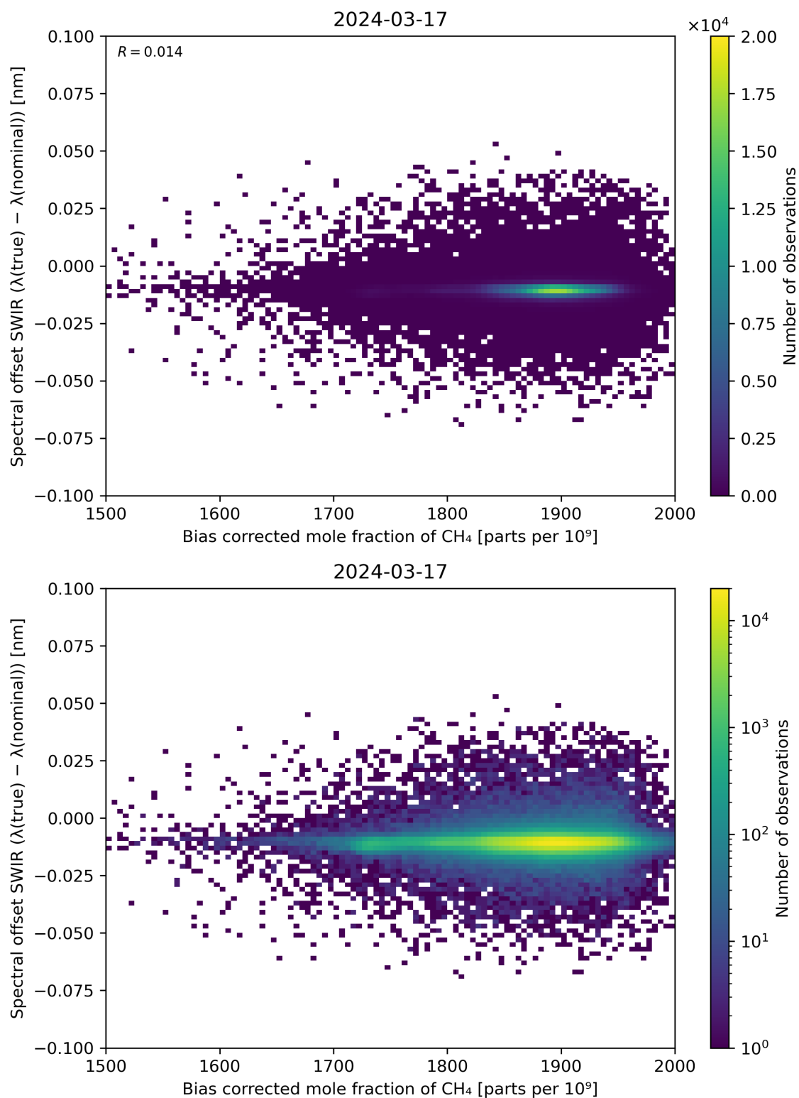
Figure 69: Scatter density plot of “Bias corrected mole fraction of \text{CH}_4 ” against “Spectral offset SWIR ( \lambda(\text{true}) - \lambda(\text{nominal}) )” for 2024-03-16 to 2024-03-18.
