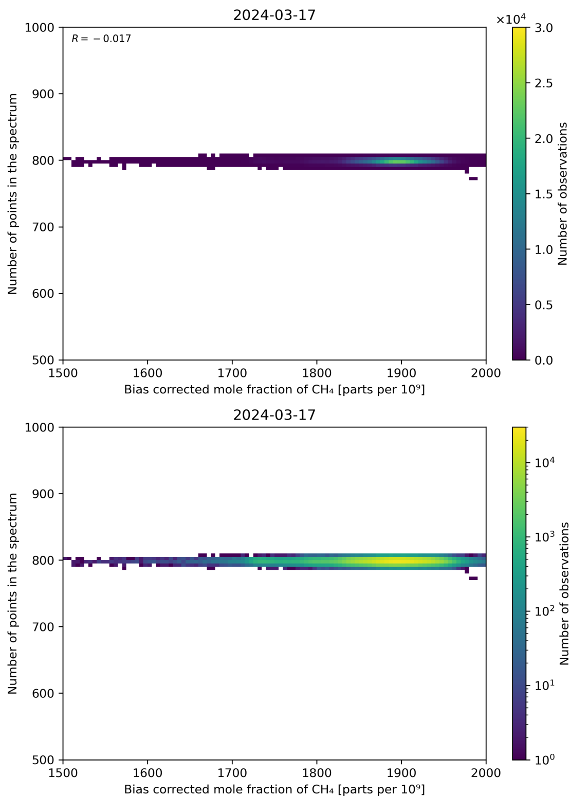
Figure 68: Scatter density plot of “Bias corrected mole fraction of CH 4 ” against “Number of points in the spectrum” for 2024-03-16 to 2024-03-18.
