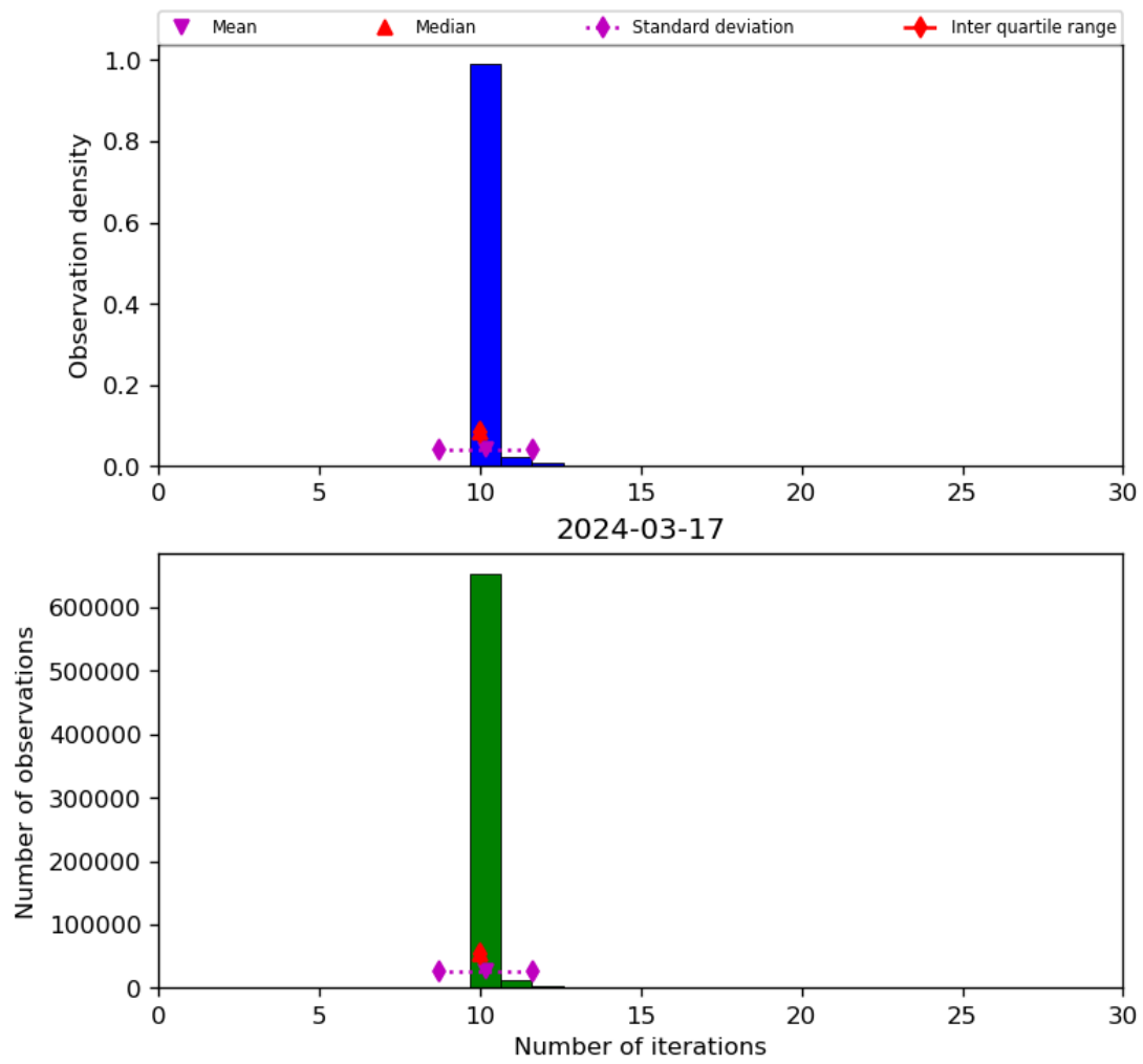
Figure 31: Histogram of “Number of iterations” for 2024-03-16 to 2024-03-18
