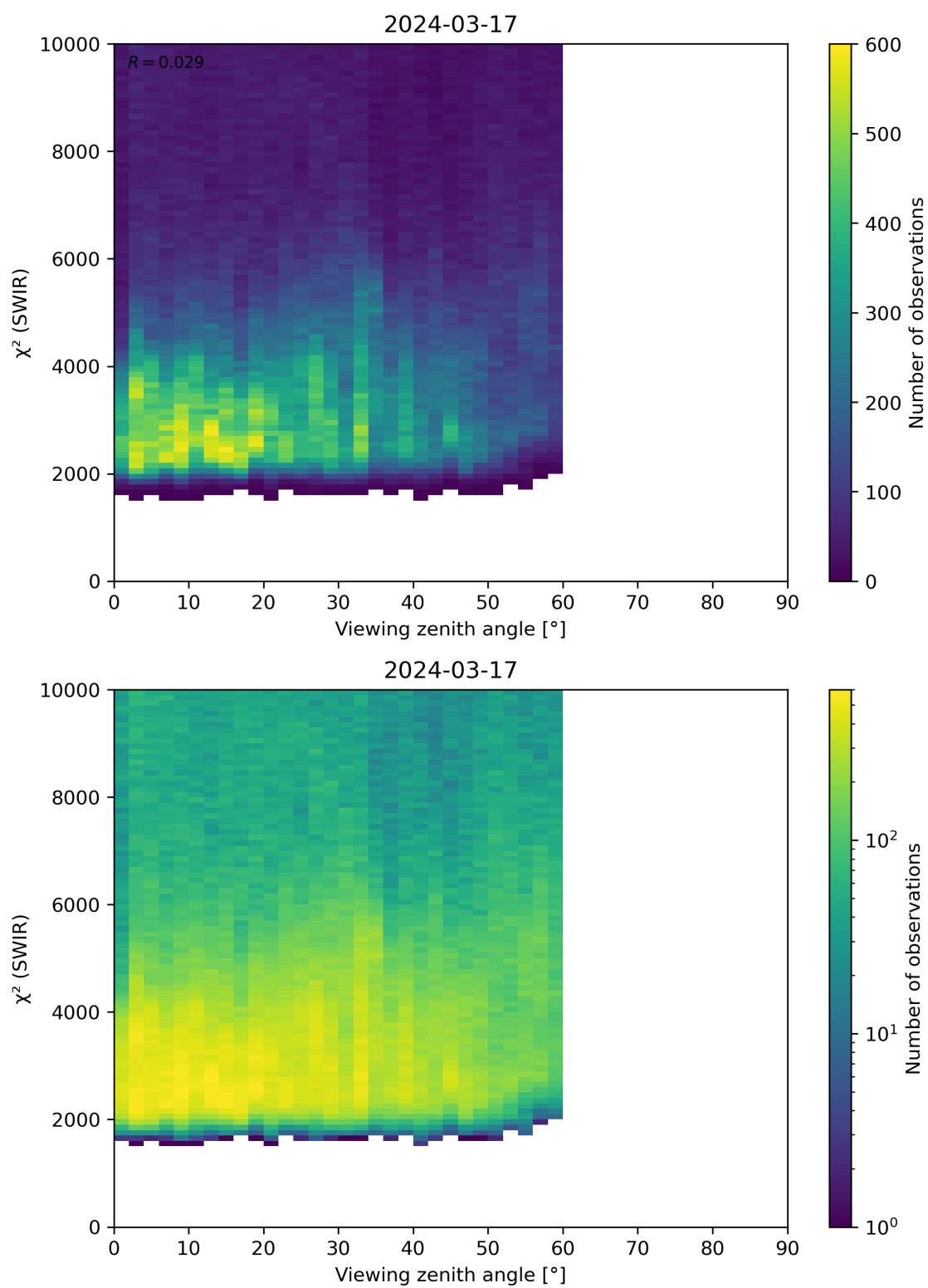
Figure 106: Scatter density plot of “Viewing zenith angle” against “ \chi^2 (SWIR)” for 2024-03-16 to 2024-03-18.
