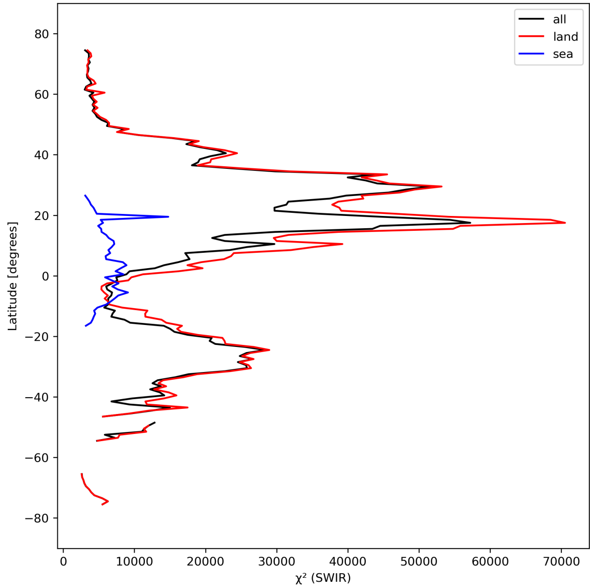
Figure 17: Zonal average of “ \chi^2 (SWIR)” for 2024-03-16 to 2024-03-18.
