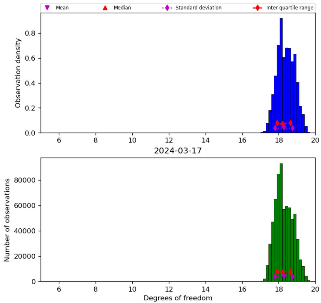
Figure 30: Histogram of “Degrees of freedom” for 2024-03-16 to 2024-03-18
