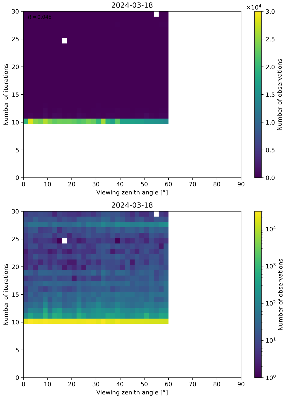
Figure 113: Scatter density plot of “Viewing zenith angle” against “Number of iterations” for 2024-03-17 to 2024-03-19.
