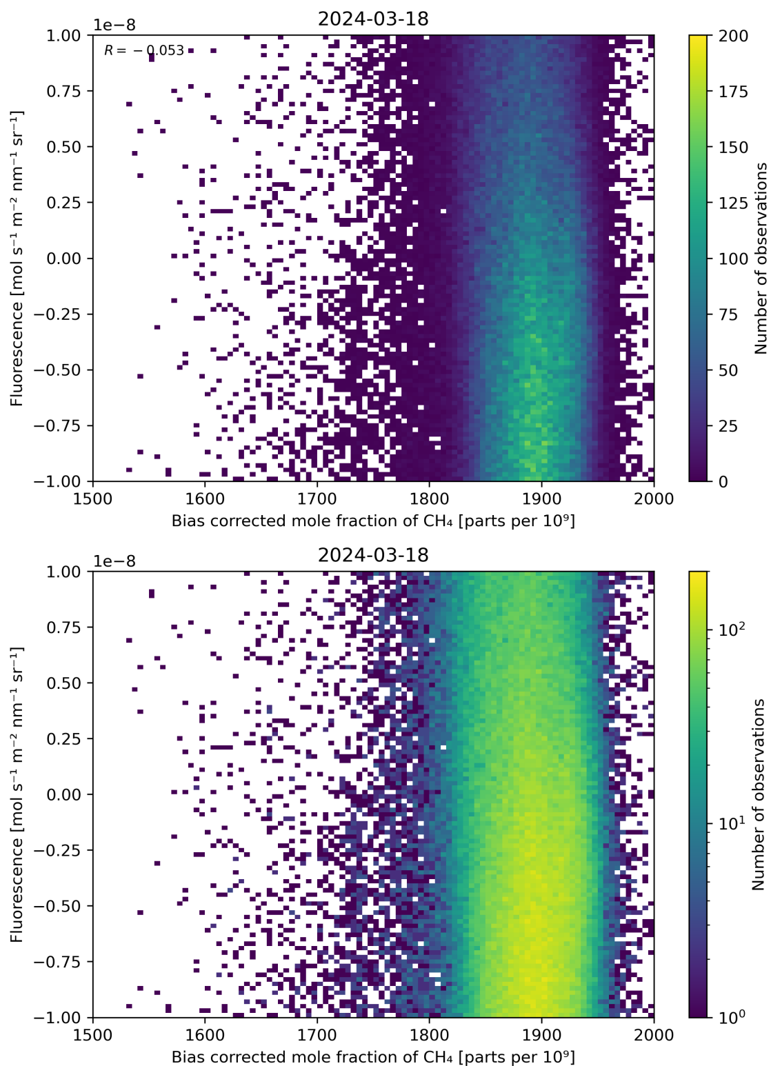
Figure 66: Scatter density plot of “Bias corrected mole fraction of \text{CH}_4 ” against “Fluorescence” for 2024-03-17 to 2024-03-19.
