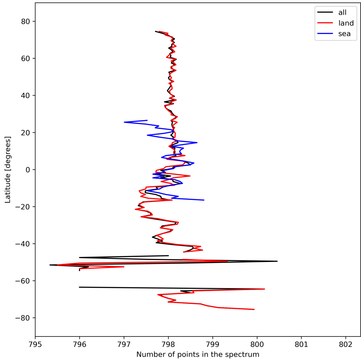
Figure 15: Zonal average of “Number of points in the spectrum” for 2024-03-17 to 2024-03-19.
