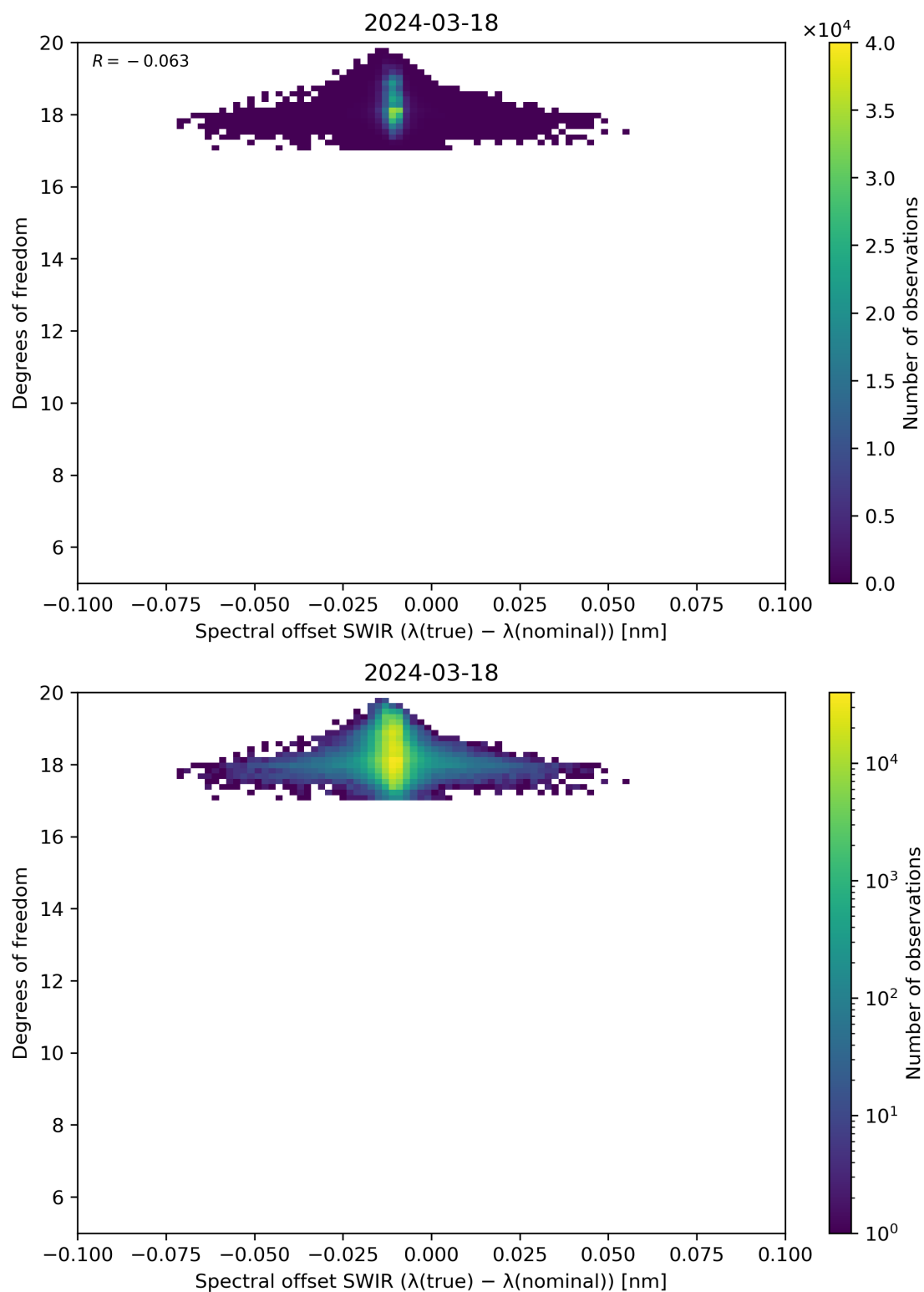
Figure 119: Scatter density plot of “Spectral offset SWIR ( \lambda(\text{true}) - \lambda(\text{nominal}) )” against “Degrees of freedom” for 2024-03-17 to 2024-03-19.
