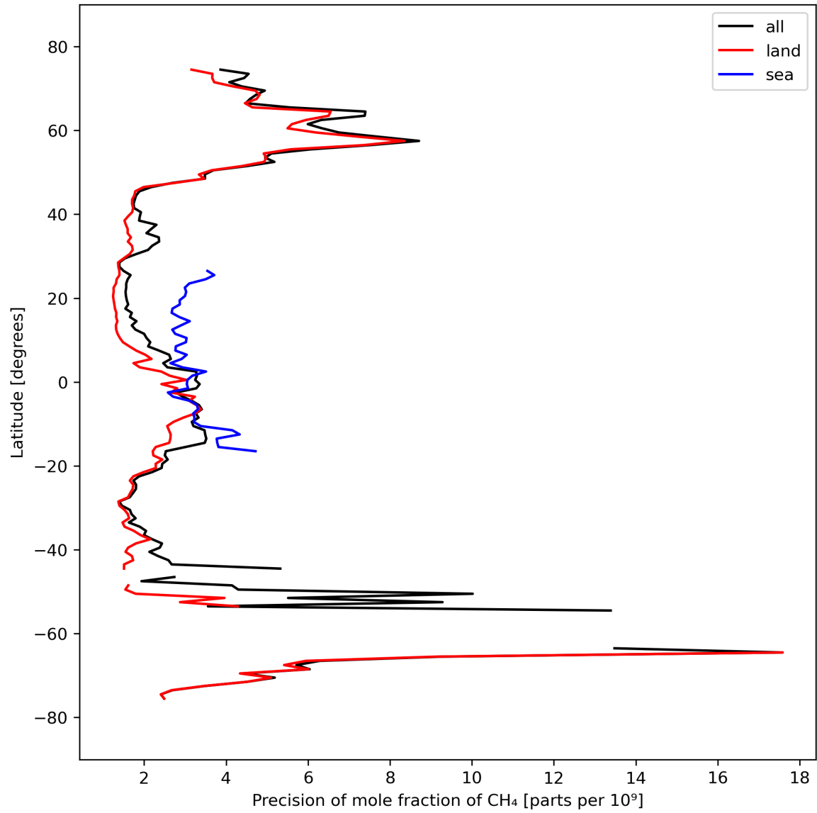
Figure 13: Zonal average of “Precision of mole fraction of CH 4 ” for 2024-03-17 to 2024-03-19.
