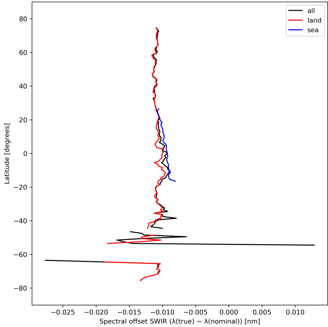
Figure 16: Zonal average of “Spectral offset SWIR ( \lambda(\text{true}) - \lambda(\text{nominal}) )” for 2024-03-17 to 2024-03-19.
