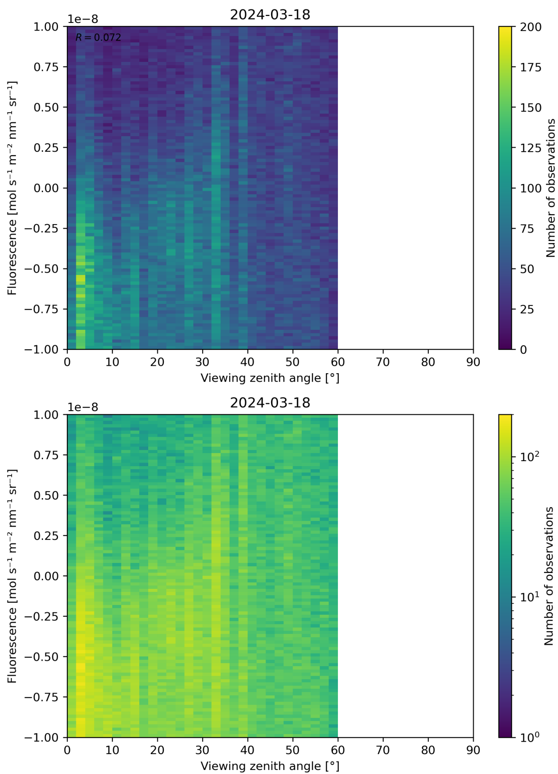
Figure 108: Scatter density plot of “Viewing zenith angle” against “Fluorescence” for 2024-03-17 to 2024-03-19.
