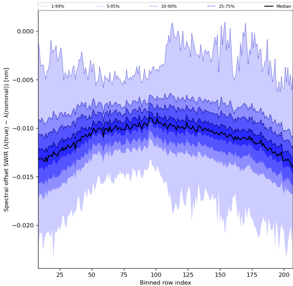
Figure 38: Along track statistics of “Spectral offset SWIR ( \lambda(\text{true}) - \lambda(\text{nominal}) )” for 2024-03-17 to 2024-03-19
