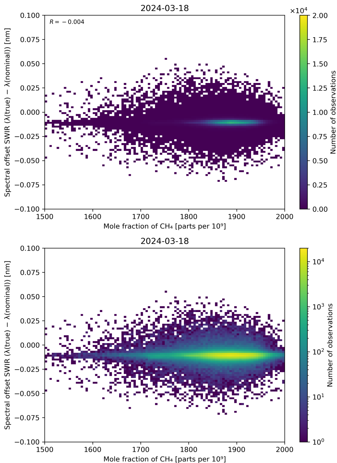
Figure 86: Scatter density plot of “Mole fraction of CH 4 ” against “Spectral offset SWIR ( \lambda(\text{true}) - \lambda(\text{nominal}) )” for 2024-03-17 to 2024-03-19.
