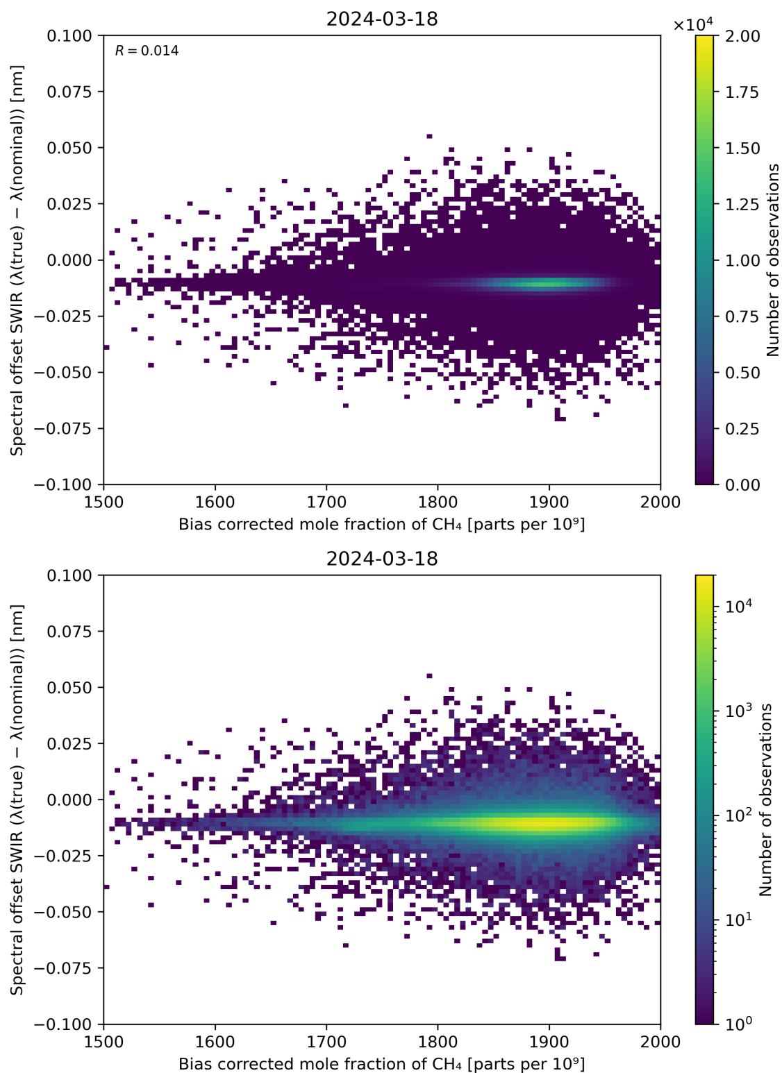
Figure 69: Scatter density plot of “Bias corrected mole fraction of \text{CH}_4 ” against “Spectral offset SWIR ( \lambda(\text{true}) - \lambda(\text{nominal}) )” for 2024-03-17 to 2024-03-19.
