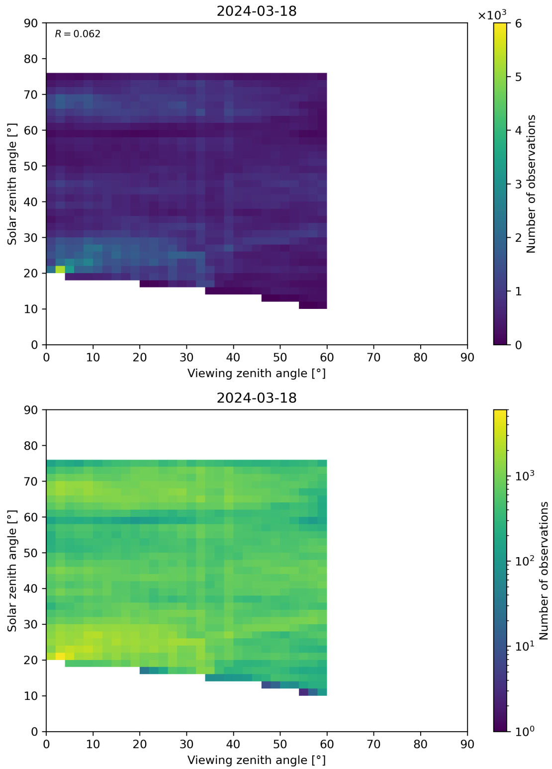
Figure 115: Scatter density plot of “Viewing zenith angle” against “Solar zenith angle” for 2024-03-17 to 2024-03-19.
