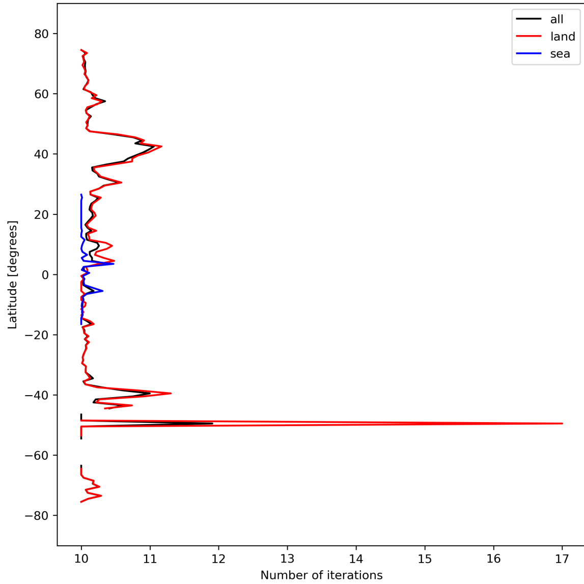
Figure 20: Zonal average of “Number of iterations” for 2024-03-17 to 2024-03-19.
