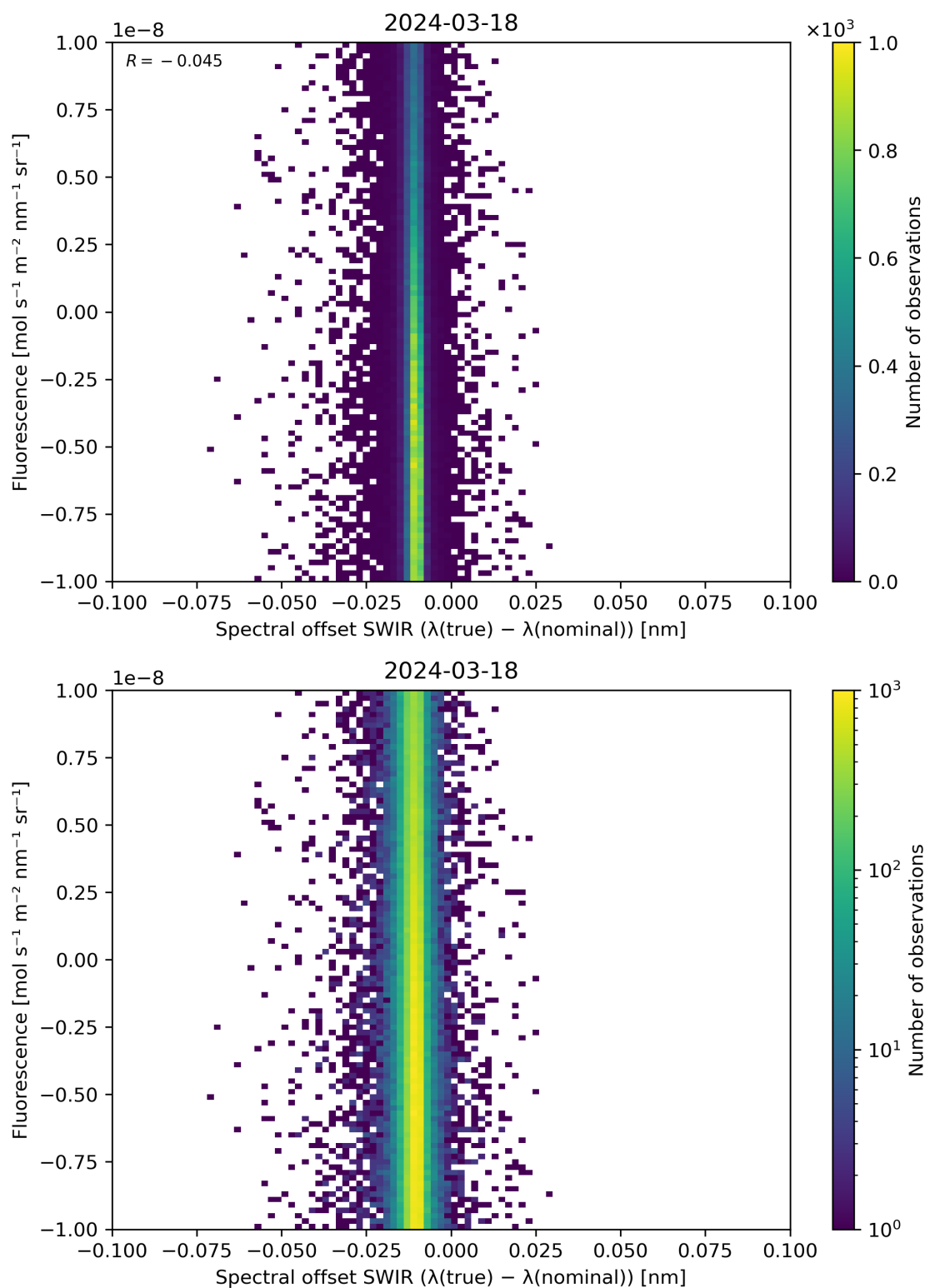
Figure 120: Scatter density plot of “Spectral offset SWIR ( \lambda(\text{true}) - \lambda(\text{nominal}) )” against “Fluorescence” for 2024-03-17 to 2024-03-19.
