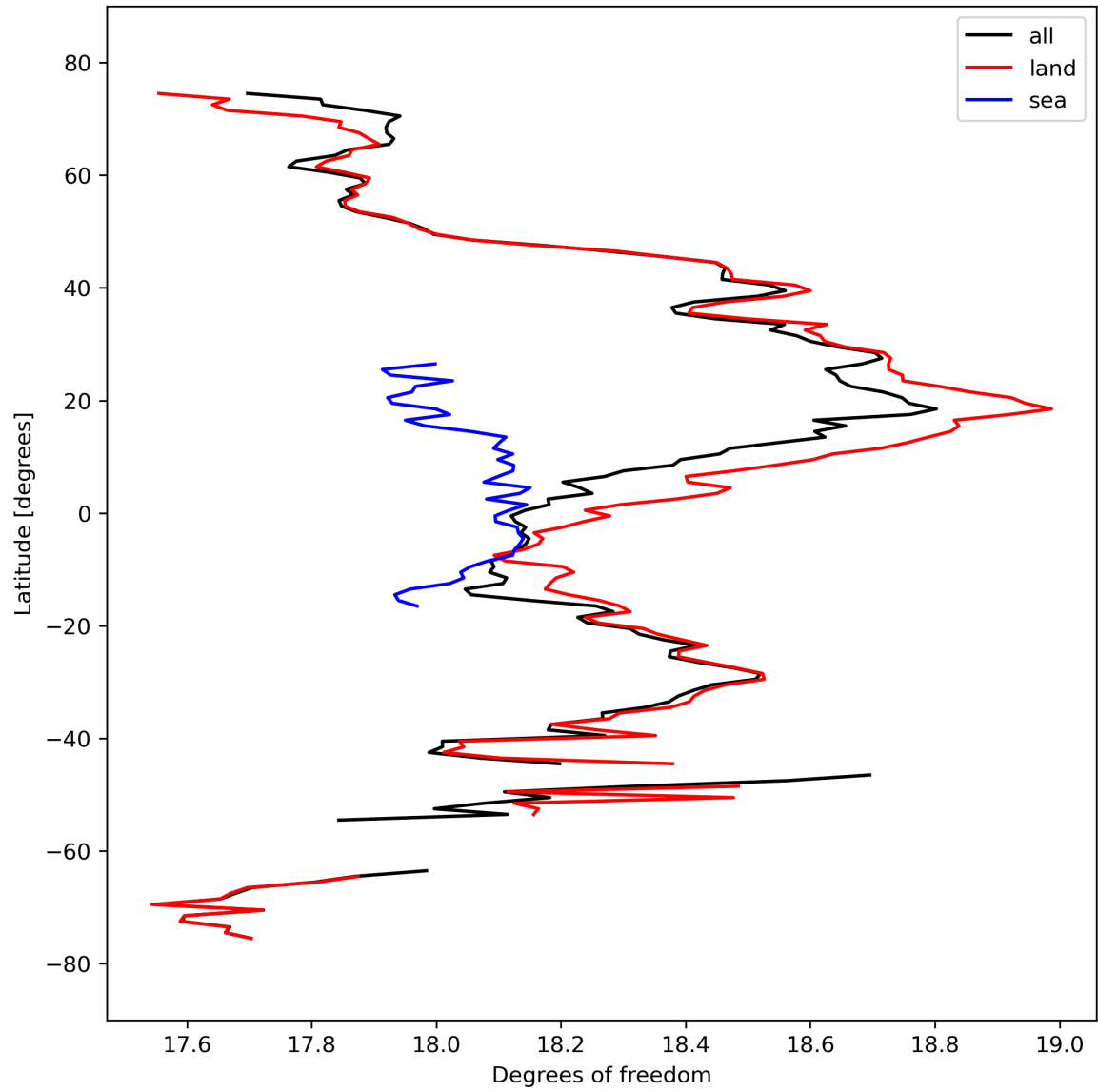
Figure 19: Zonal average of “Degrees of freedom” for 2024-03-17 to 2024-03-19.
