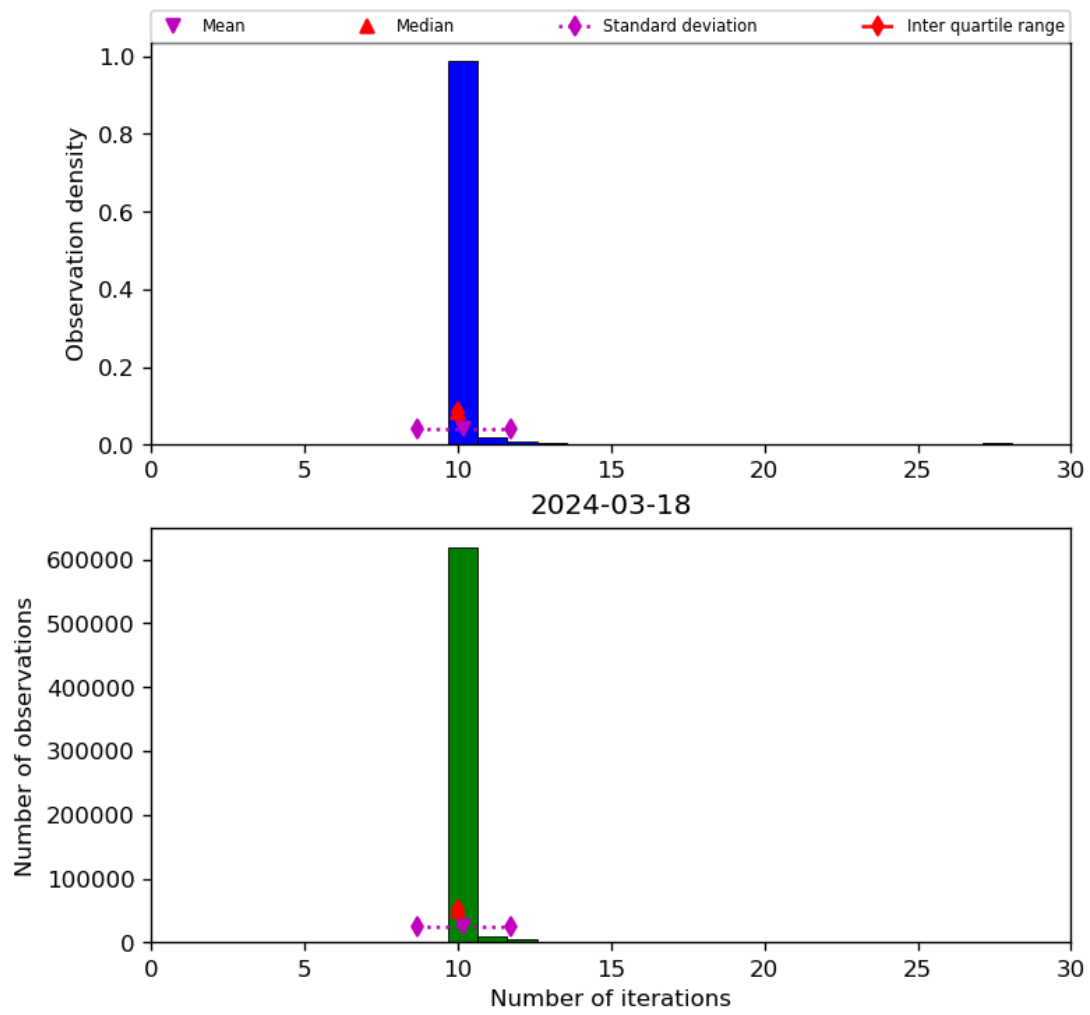
Figure 31: Histogram of “Number of iterations” for 2024-03-17 to 2024-03-19
