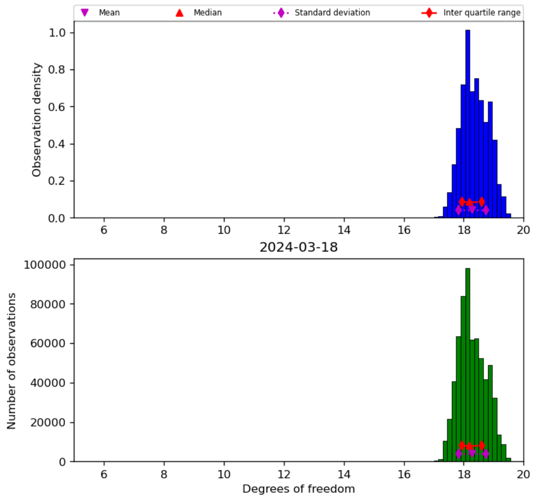
Figure 30: Histogram of “Degrees of freedom” for 2024-03-17 to 2024-03-19
