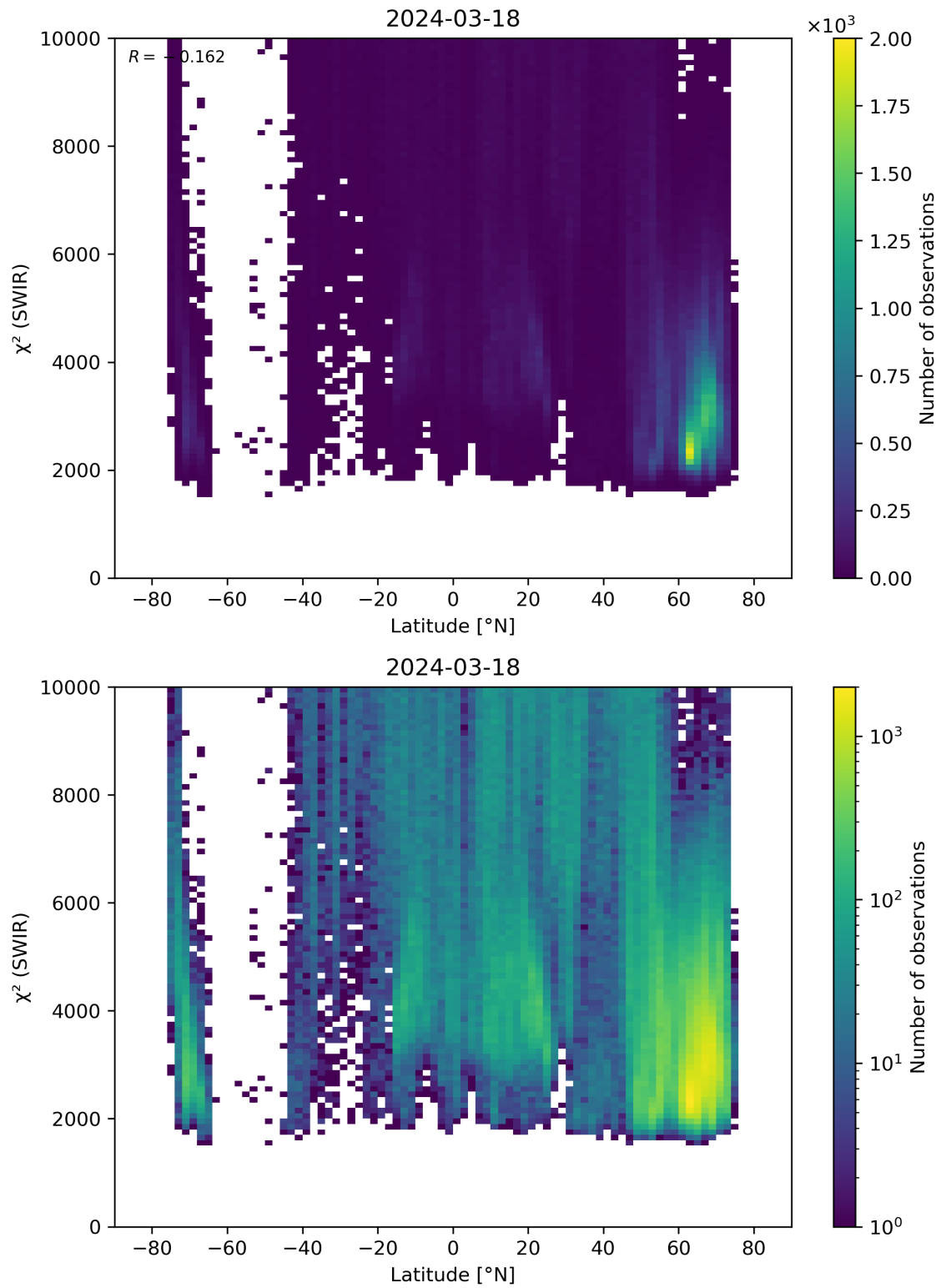
Figure 54: Scatter density plot of “Latitude” against “ \chi^2 (SWIR)” for 2024-03-17 to 2024-03-19.
