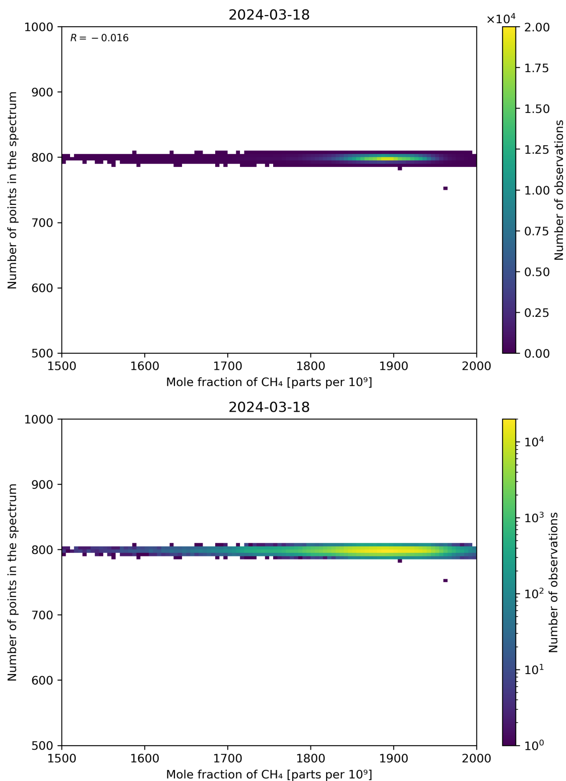
Figure 77: Scatter density plot of “Mole fraction of CH 4 ” against “Number of points in the spectrum” for 2024-03-17 to 2024-03-19.
