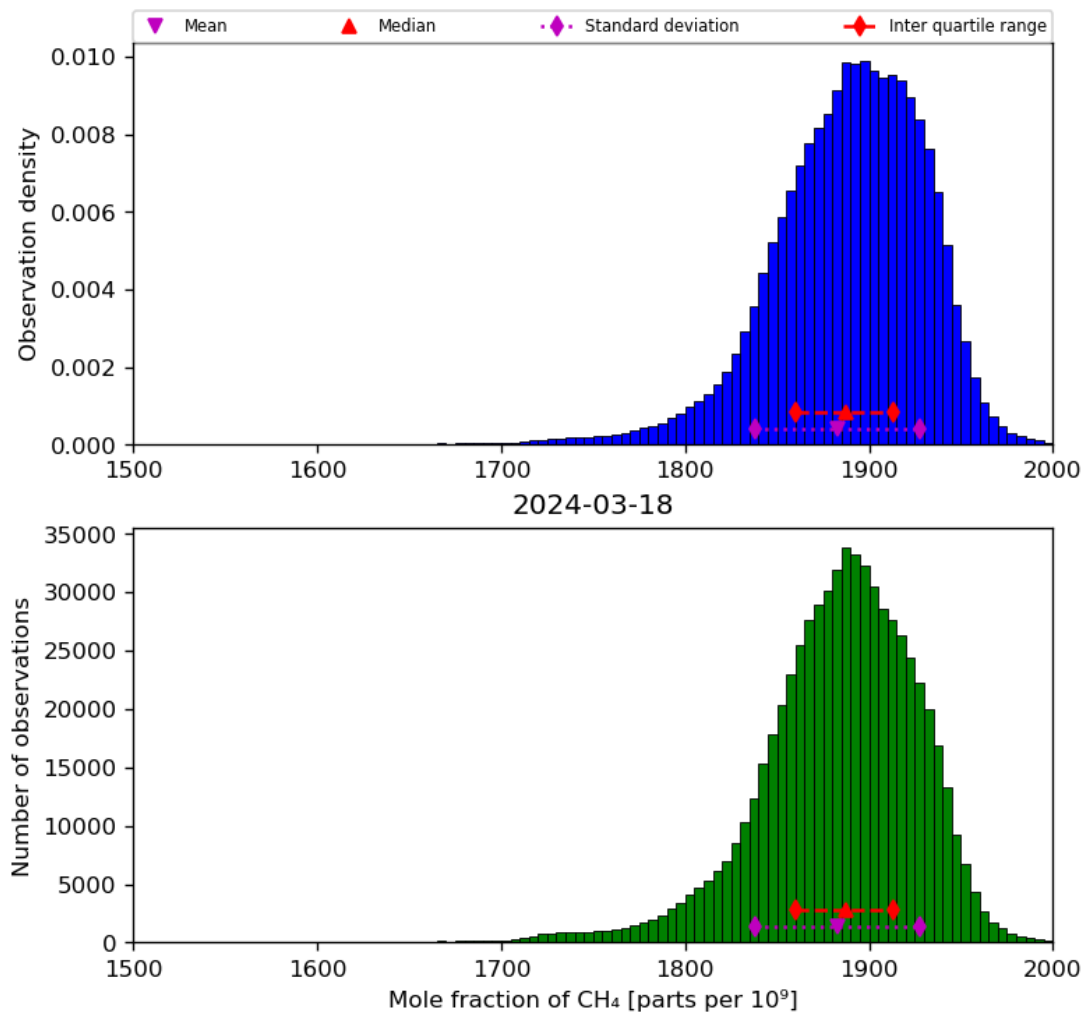
Figure 23: Histogram of “Mole fraction of CH 4 ” for 2024-03-17 to 2024-03-19
