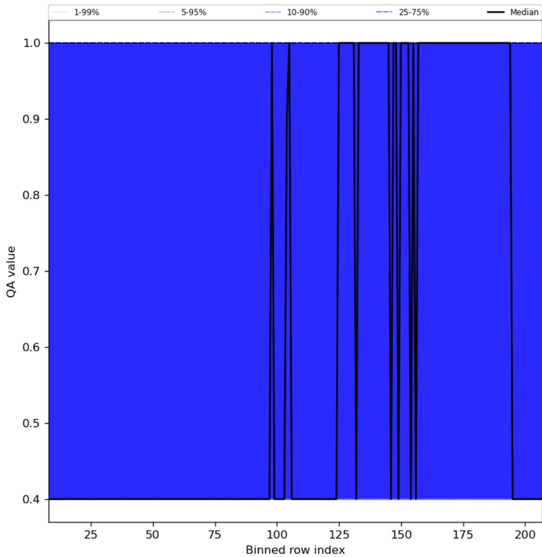
Figure 33: Along track statistics of “QA value” for 2024-03-17 to 2024-03-19
