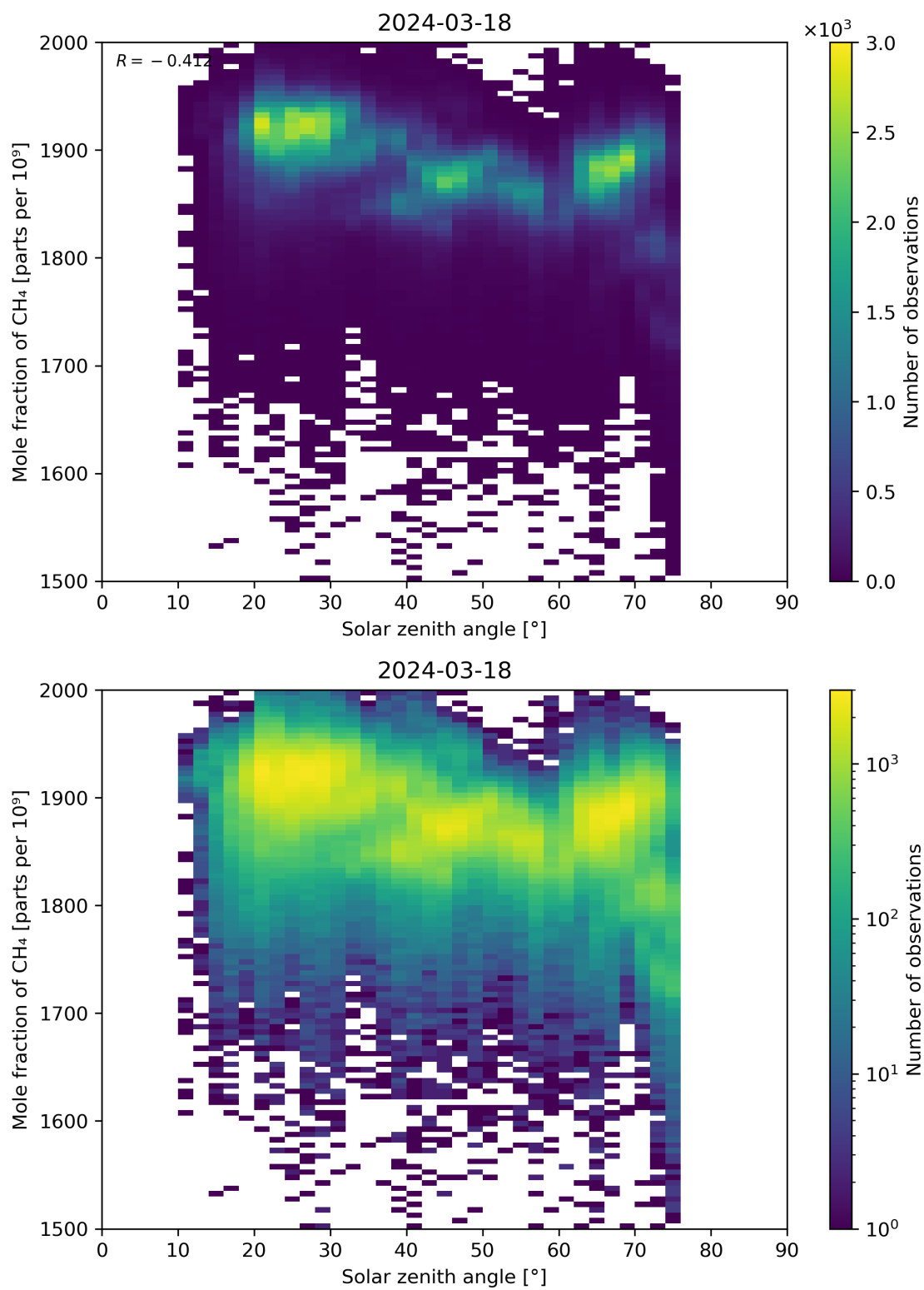
Figure 99: Scatter density plot of “Solar zenith angle” against “Mole fraction of \text{CH}_4 ” for 2024-03-17 to 2024-03-19.
