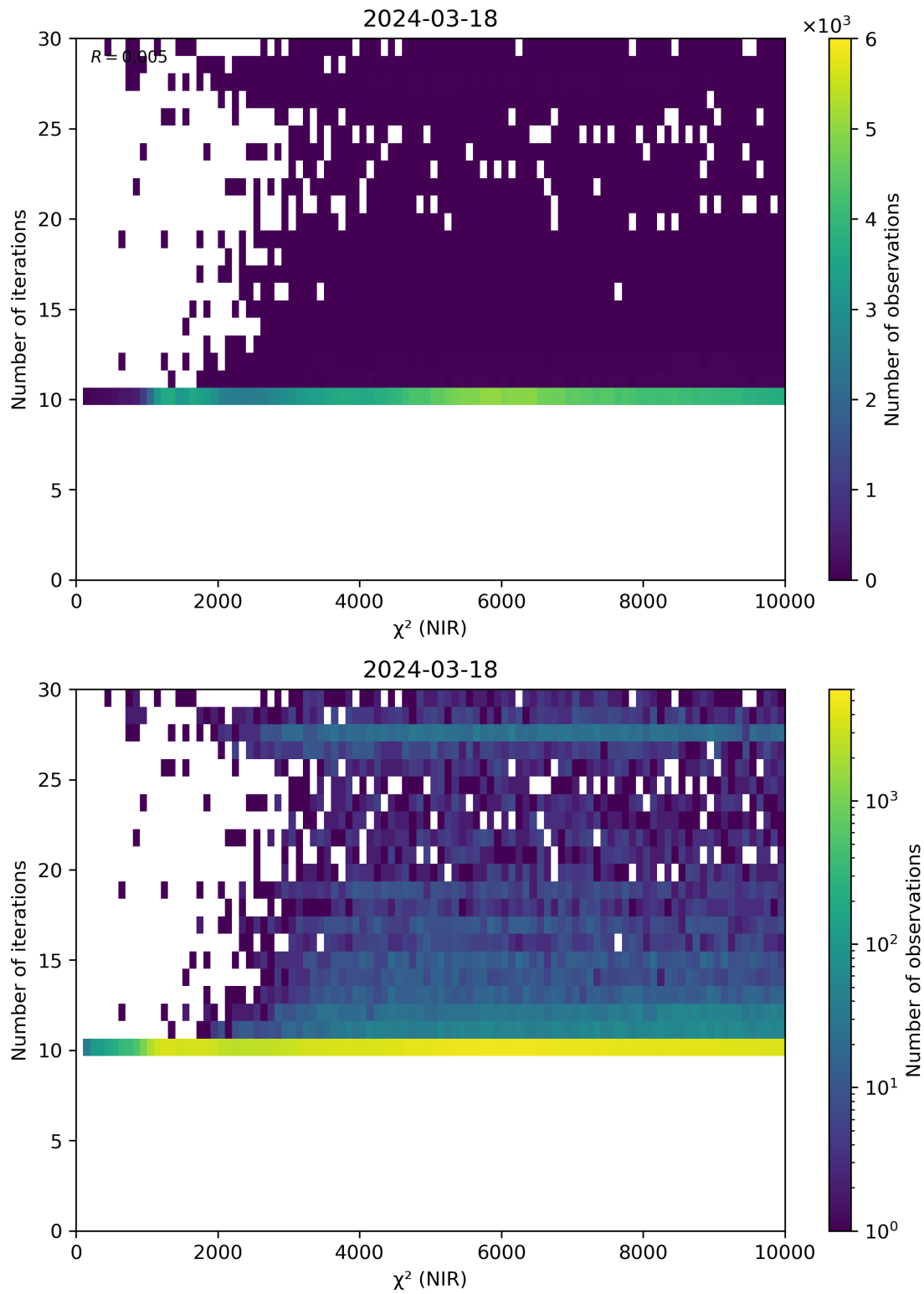
Figure 46: Scatter density plot of “ \chi^2 (NIR)” against “Number of iterations” for 2024-03-17 to 2024-03-19.
