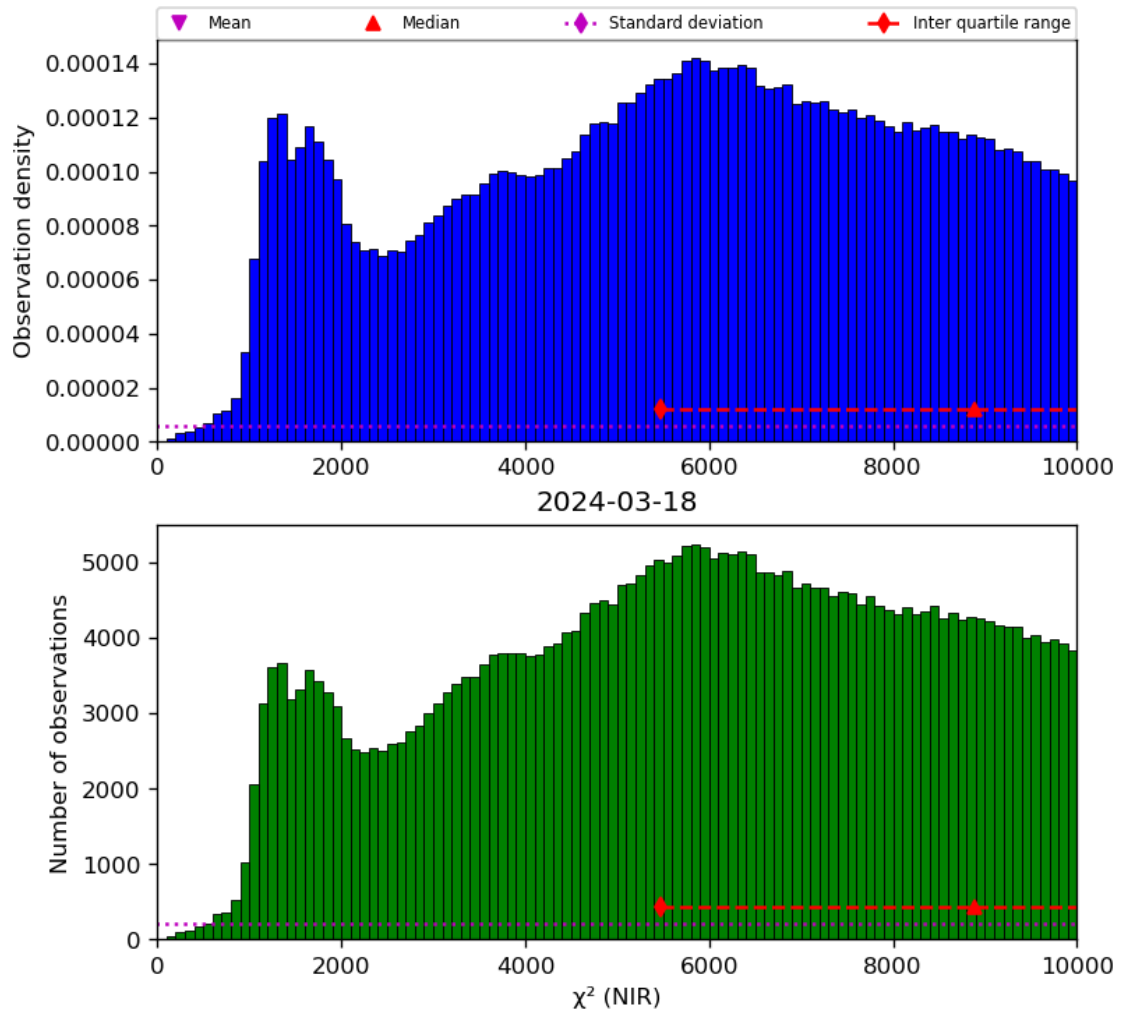
Figure 29: Histogram of " \chi^2 (NIR)" for 2024-03-17 to 2024-03-19
