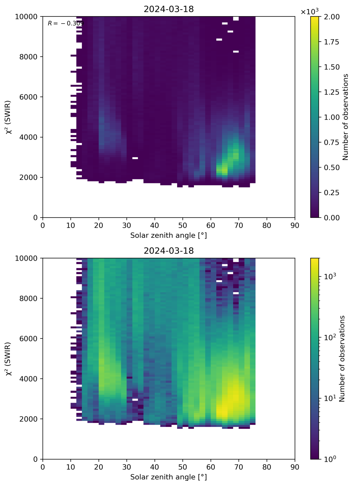
Figure 95: Scatter density plot of “Solar zenith angle” against “ \chi^2 (SWIR)” for 2024-03-17 to 2024-03-19.
