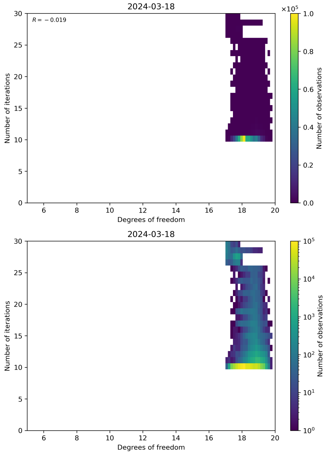
Figure 52: Scatter density plot of “Degrees of freedom” against “Number of iterations” for 2024-03-17 to 2024-03-19.
