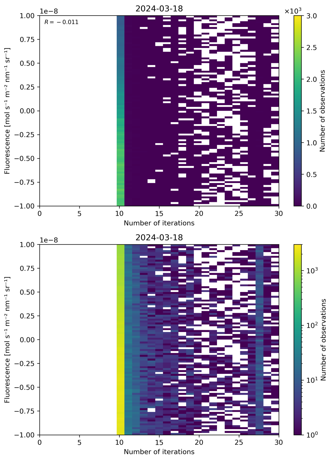
Figure 87: Scatter density plot of “Number of iterations” against “Fluorescence” for 2024-03-17 to 2024-03-19.
