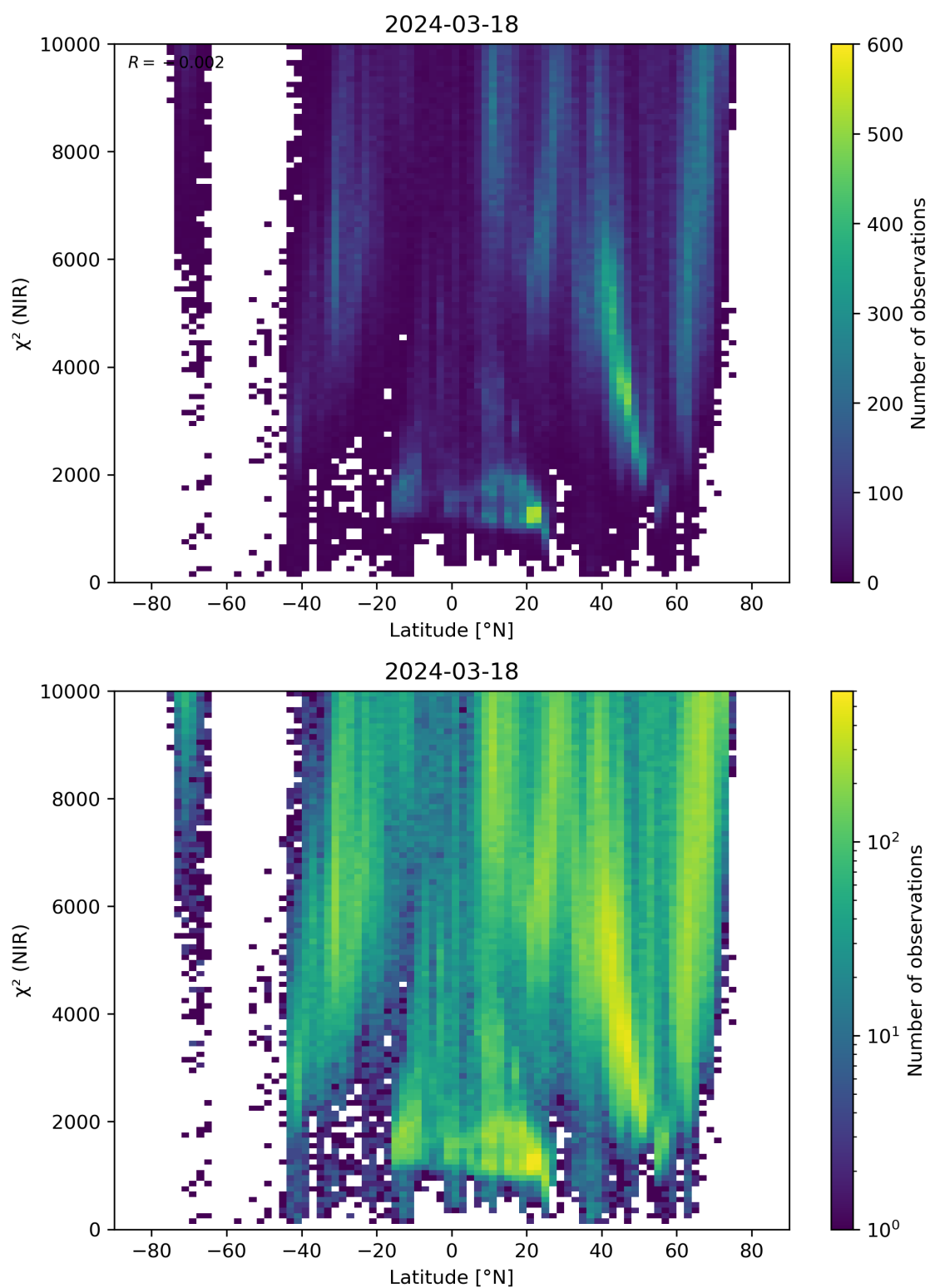
Figure 53: Scatter density plot of “Latitude” against “ \chi^2 (NIR)” for 2024-03-17 to 2024-03-19.
