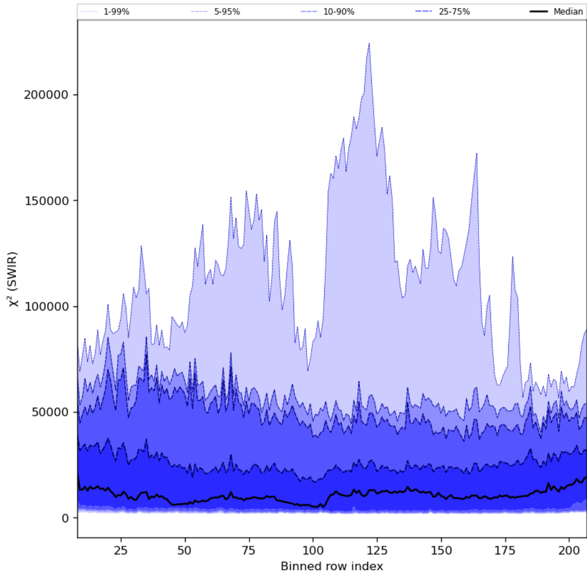
Figure 39: Along track statistics of “ \chi^2 (SWIR)” for 2024-03-17 to 2024-03-19
