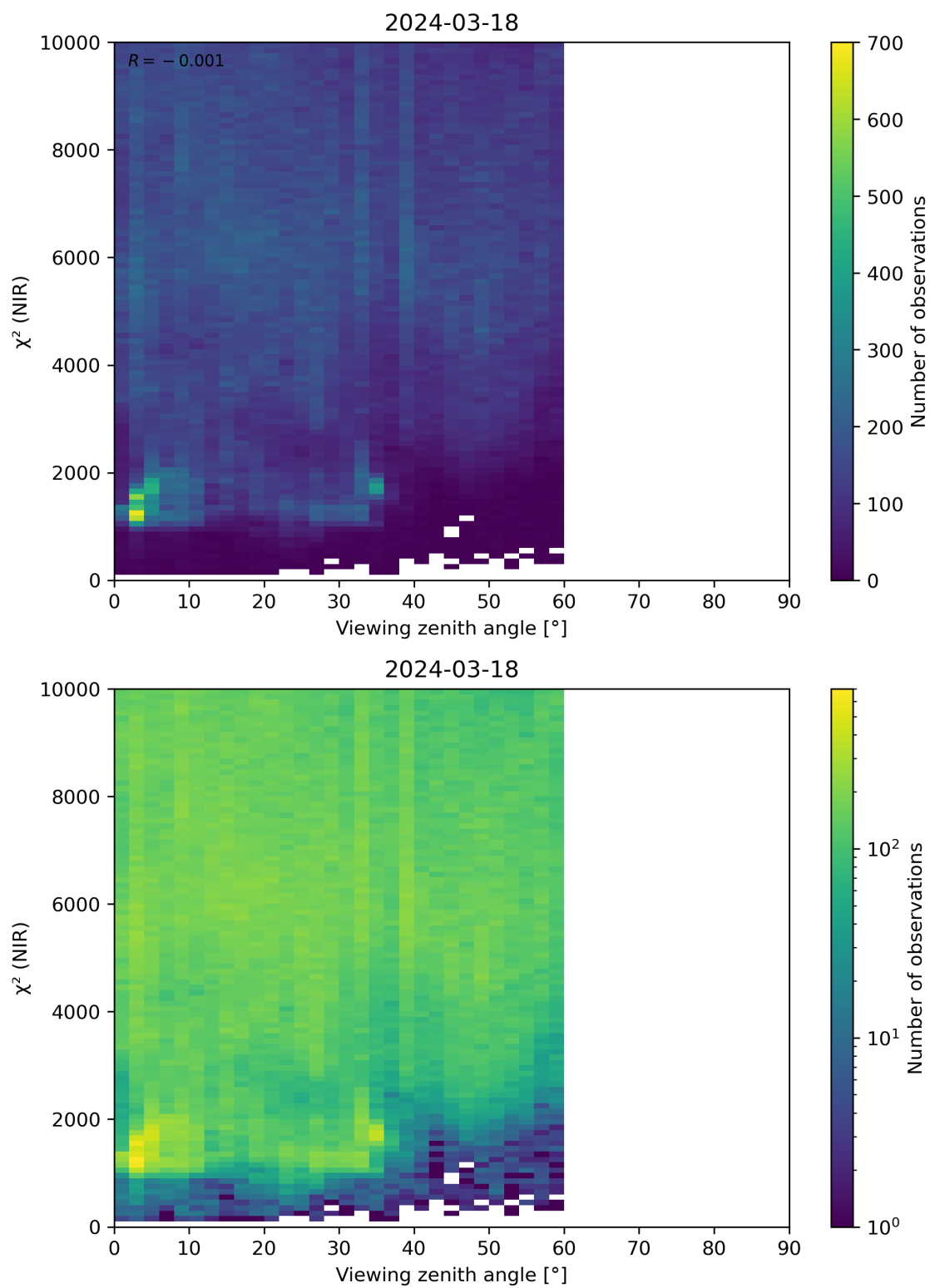
Figure 105: Scatter density plot of “Viewing zenith angle” against “ \chi^2 (NIR)” for 2024-03-17 to 2024-03-19.
