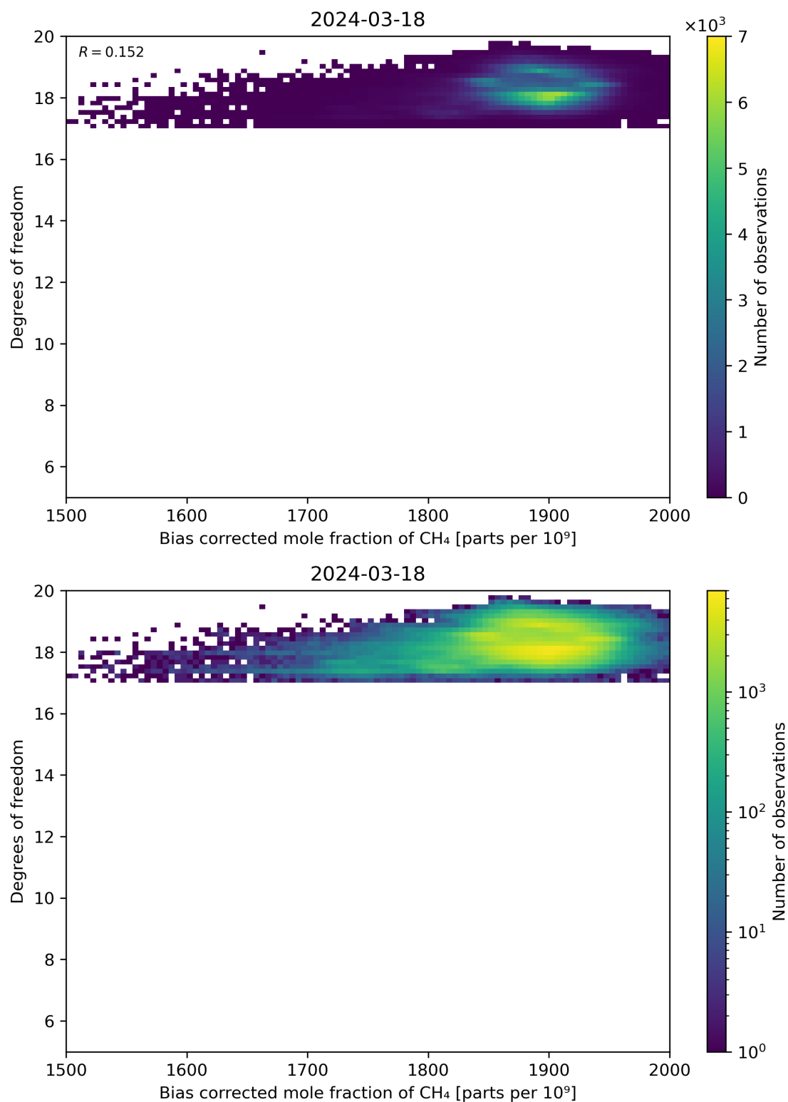
Figure 65: Scatter density plot of “Bias corrected mole fraction of CH 4 ” against “Degrees of freedom” for 2024-03-17 to 2024-03-19.
