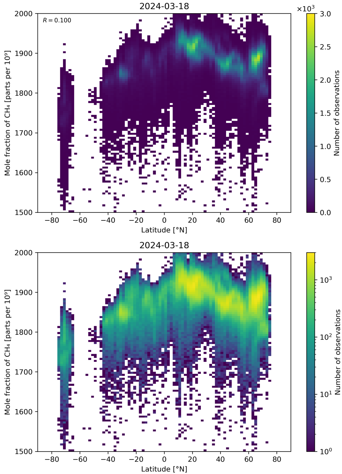
Figure 57: Scatter density plot of “Latitude” against “Mole fraction of CH 4 ” for 2024-03-17 to 2024-03-19.
