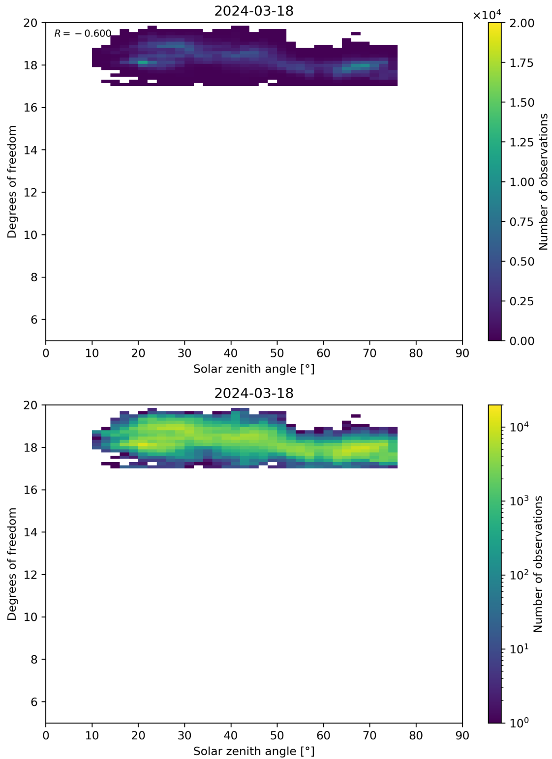
Figure 96: Scatter density plot of “Solar zenith angle” against “Degrees of freedom” for 2024-03-17 to 2024-03-19.
