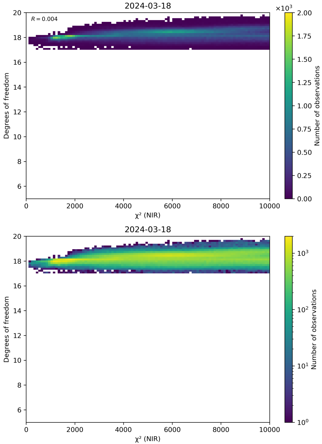
Figure 44: Scatter density plot of “ \chi^2 (NIR)” against “Degrees of freedom” for 2024-03-17 to 2024-03-19.
