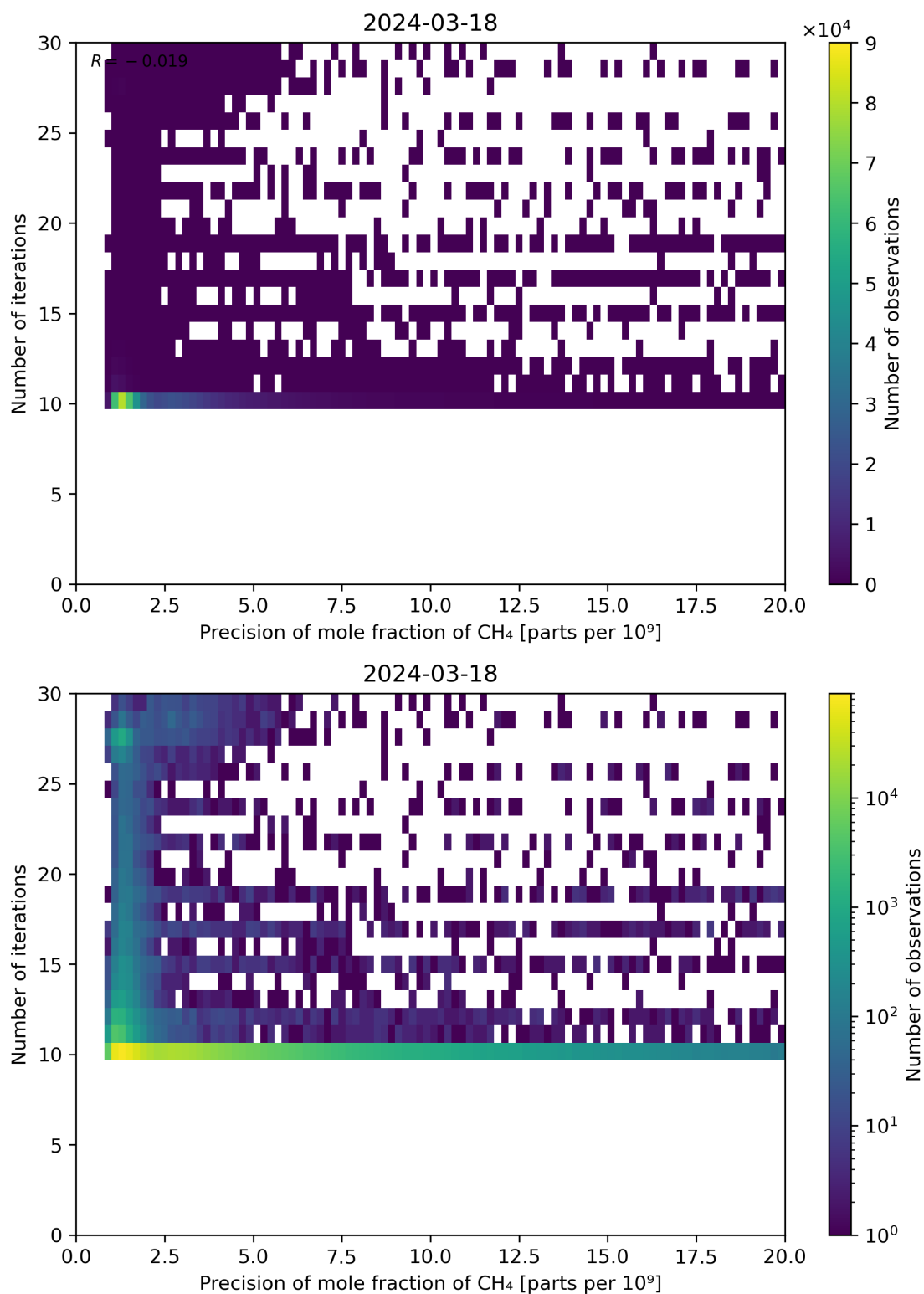
Figure 83: Scatter density plot of “Precision of mole fraction of CH 4 ” against “Number of iterations” for 2024-03-17 to 2024-03-19.
