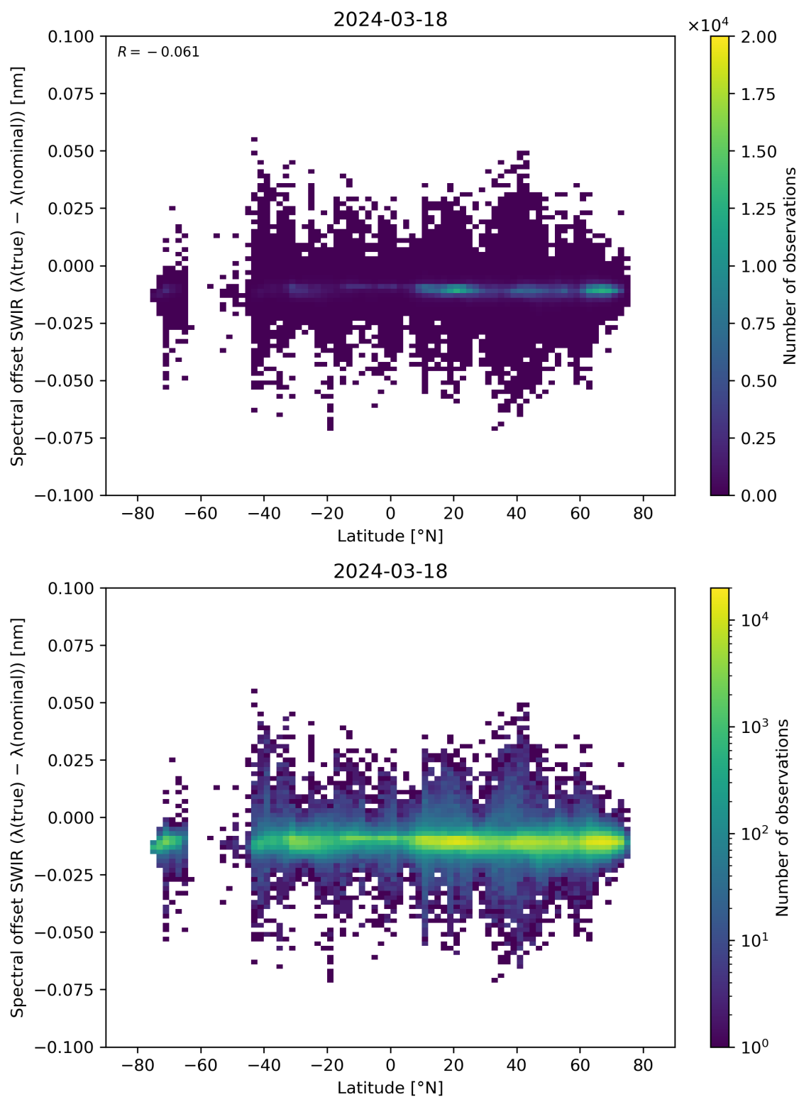
Figure 62: Scatter density plot of “Latitude” against “Spectral offset SWIR ( \lambda(\text{true}) - \lambda(\text{nominal}) )” for 2024-03-17 to 2024-03-19.
