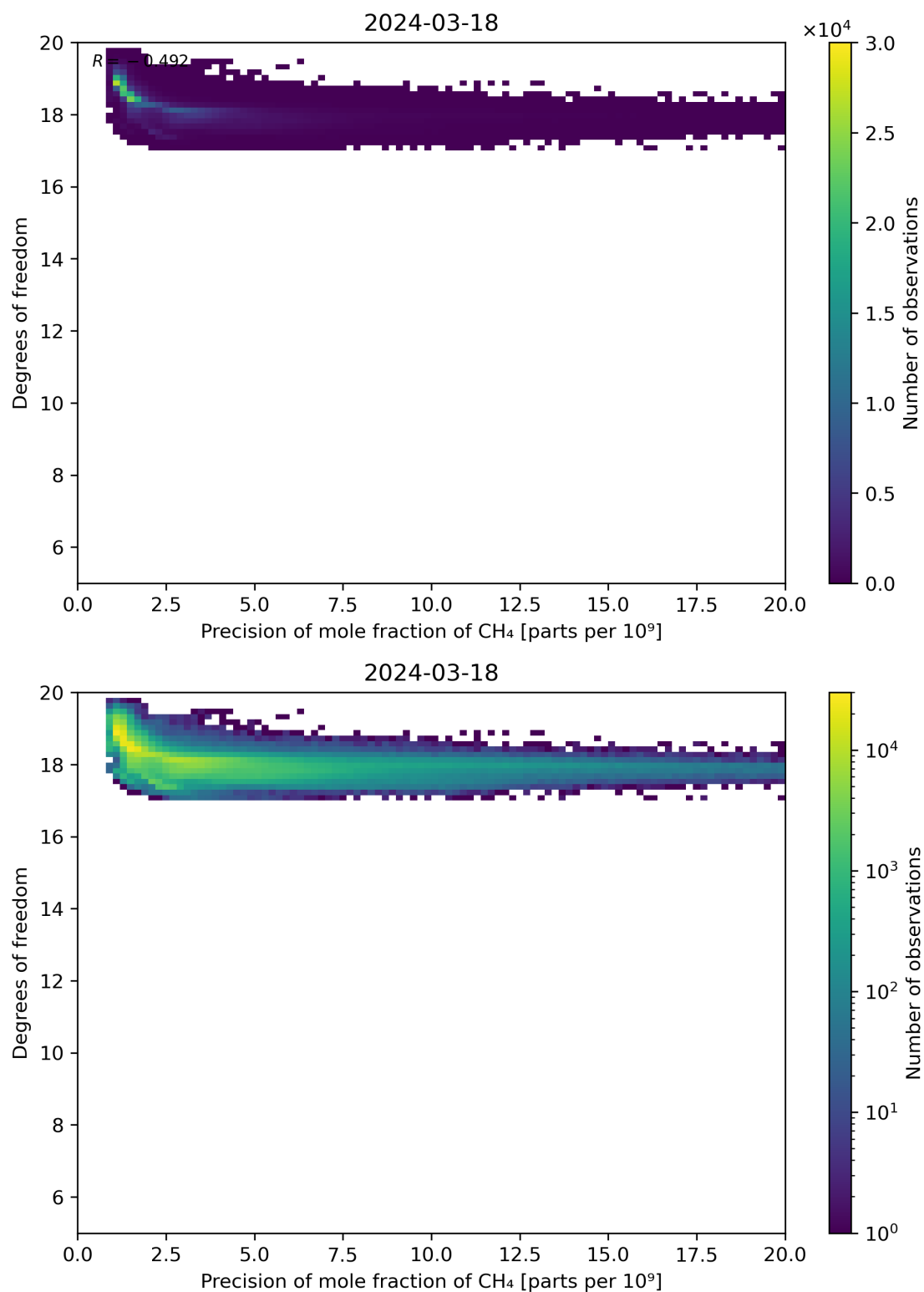
Figure 80: Scatter density plot of “Precision of mole fraction of CH 4 ” against “Degrees of freedom” for 2024-03-17 to 2024-03-19.
