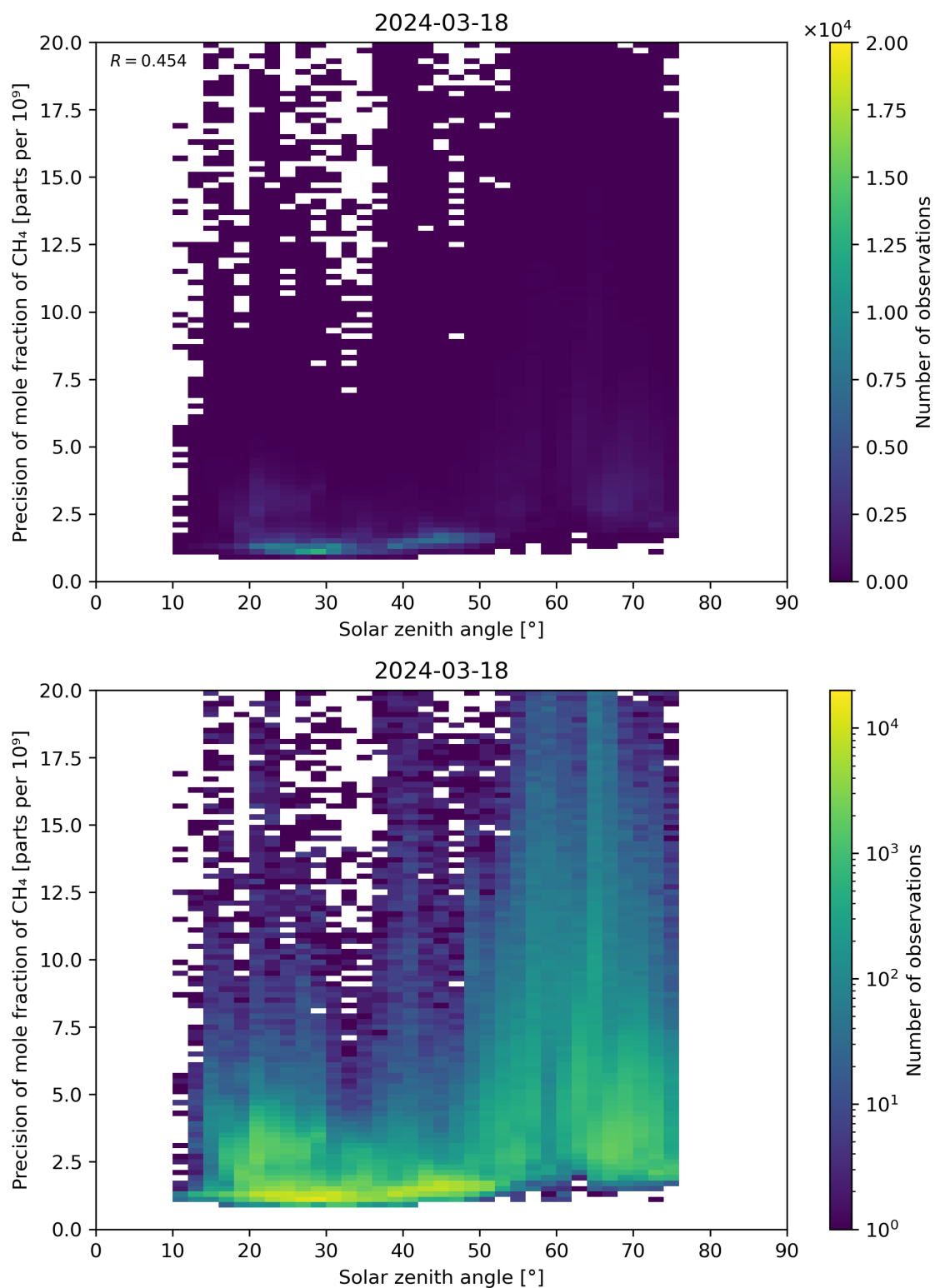
Figure 101: Scatter density plot of “Solar zenith angle” against “Precision of mole fraction of CH 4 ” for 2024-03-17 to 2024-03-19.
