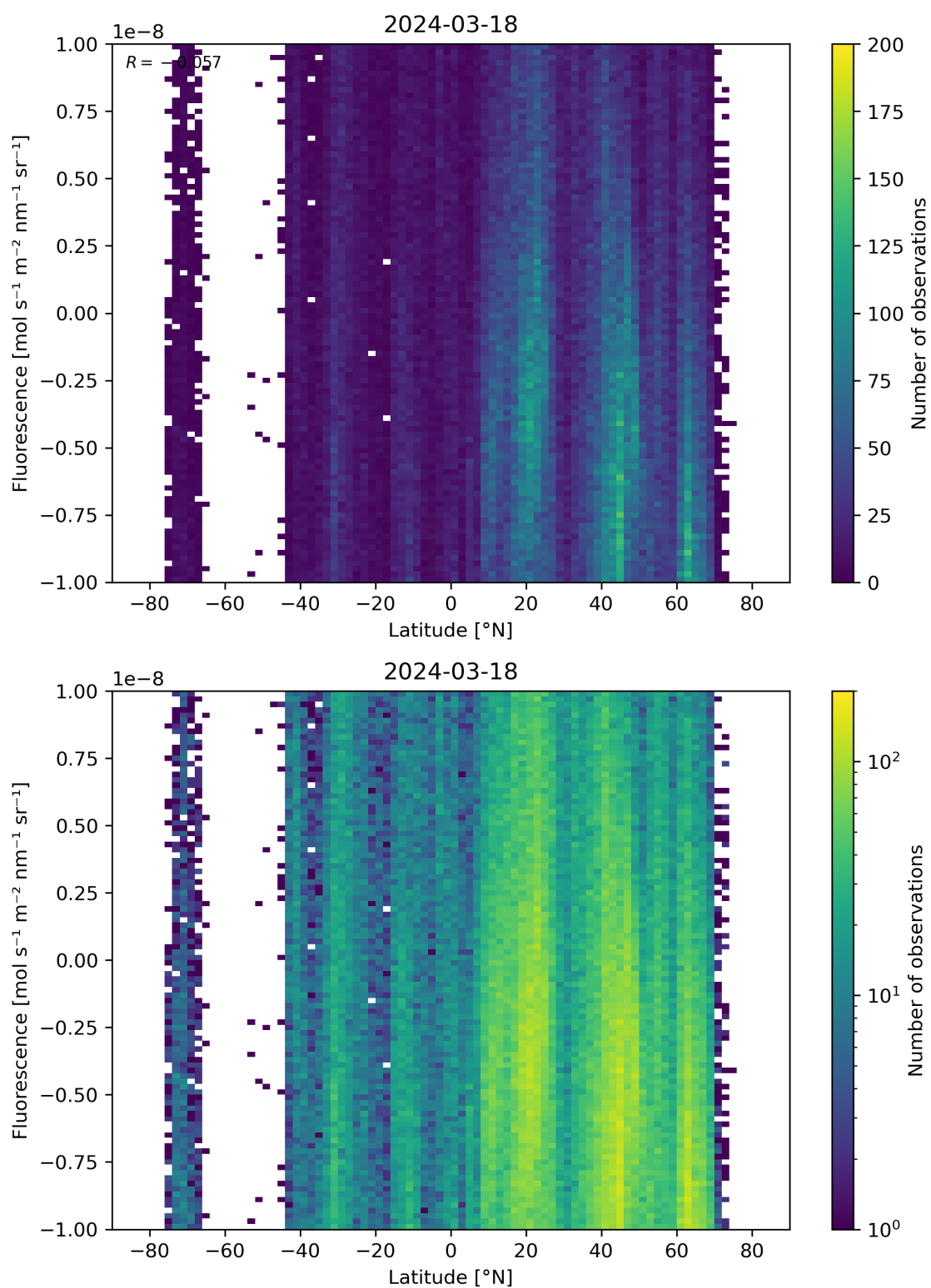
Figure 56: Scatter density plot of “Latitude” against “Fluorescence” for 2024-03-17 to 2024-03-19.
