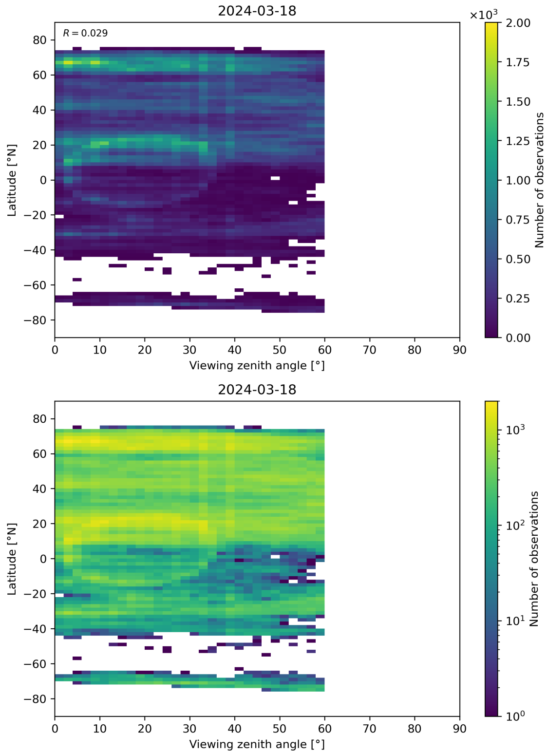
Figure 109: Scatter density plot of “Viewing zenith angle” against “Latitude” for 2024-03-17 to 2024-03-19.
