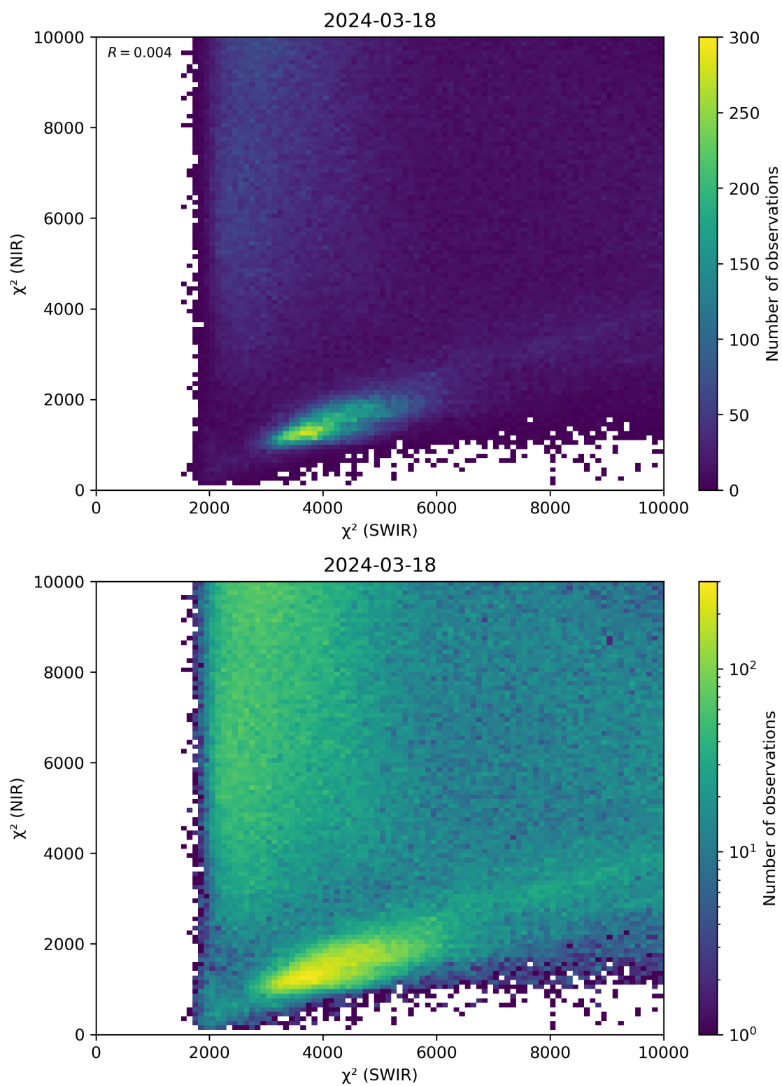
Figure 47: Scatter density plot of “ \chi^2 (SWIR)” against “ \chi^2 (NIR)” for 2024-03-17 to 2024-03-19.
