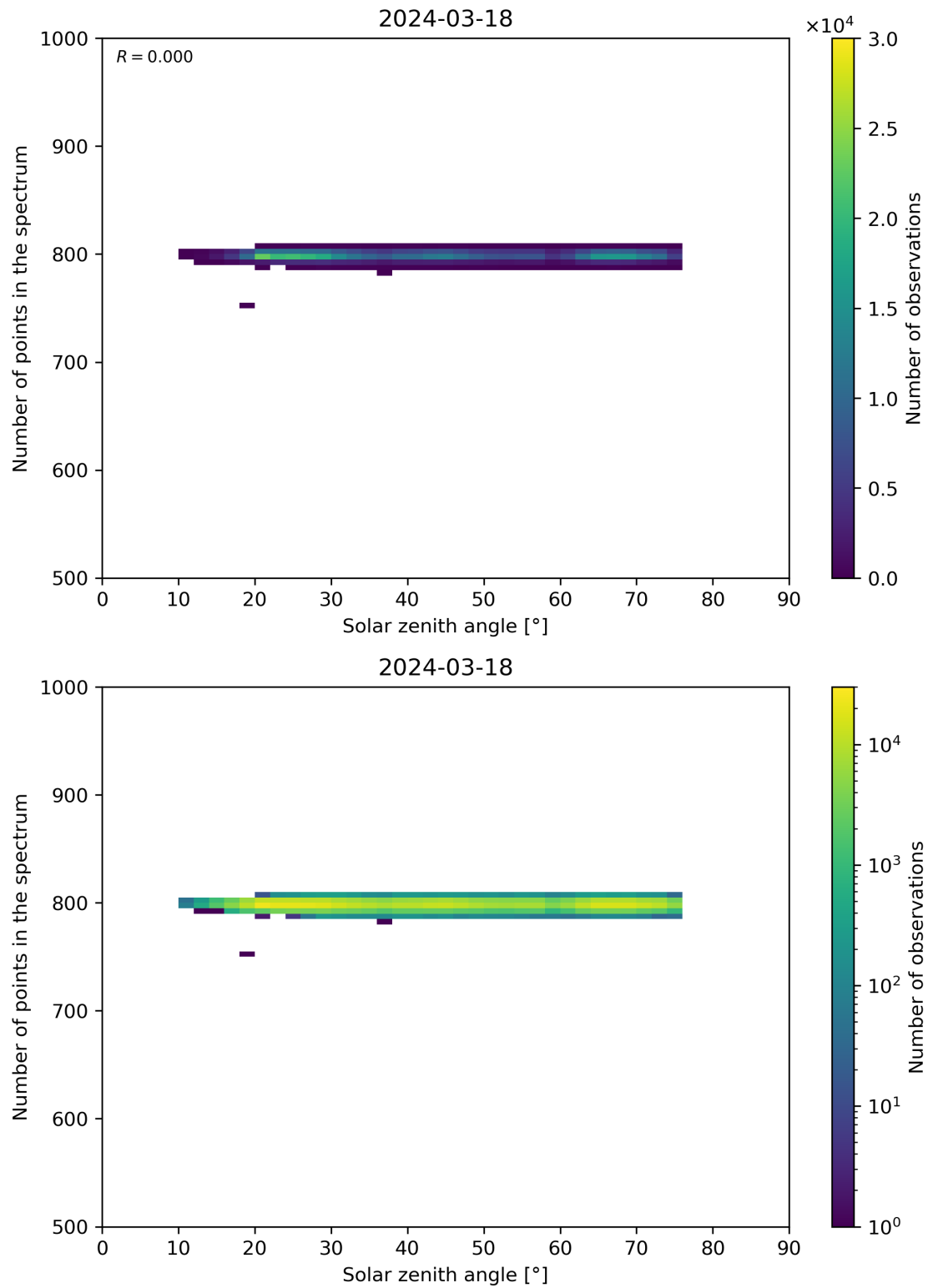
Figure 103: Scatter density plot of “Solar zenith angle” against “Number of points in the spectrum” for 2024-03-17 to 2024-03-19.
