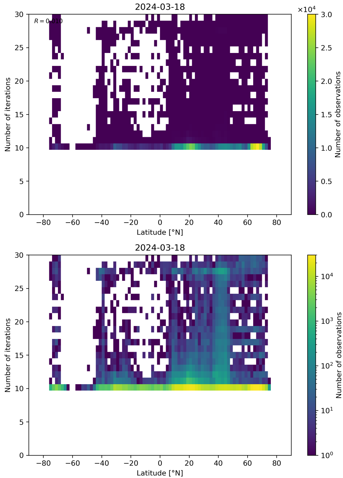
Figure 60: Scatter density plot of “Latitude” against “Number of iterations” for 2024-03-17 to 2024-03-19.
