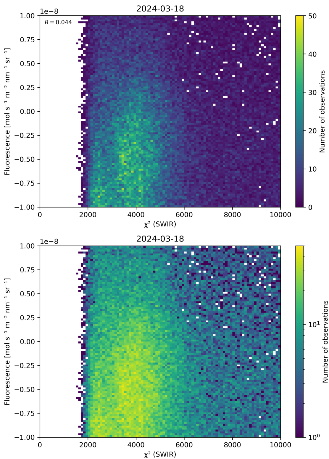
Figure 49: Scatter density plot of “ \chi^2 (SWIR)” against “Fluorescence” for 2024-03-17 to 2024-03-19.
