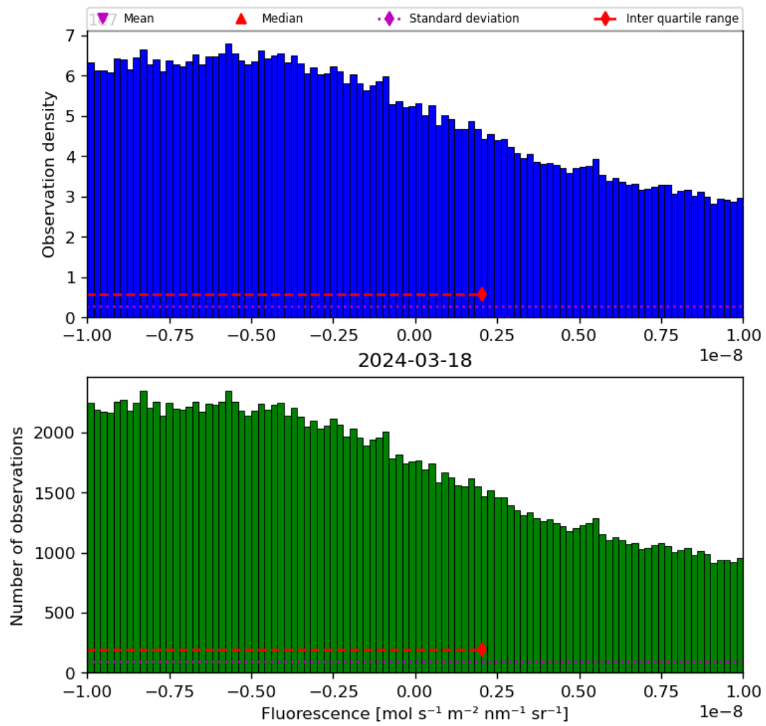
Figure 32: Histogram of “Fluorescence” for 2024-03-17 to 2024-03-19
