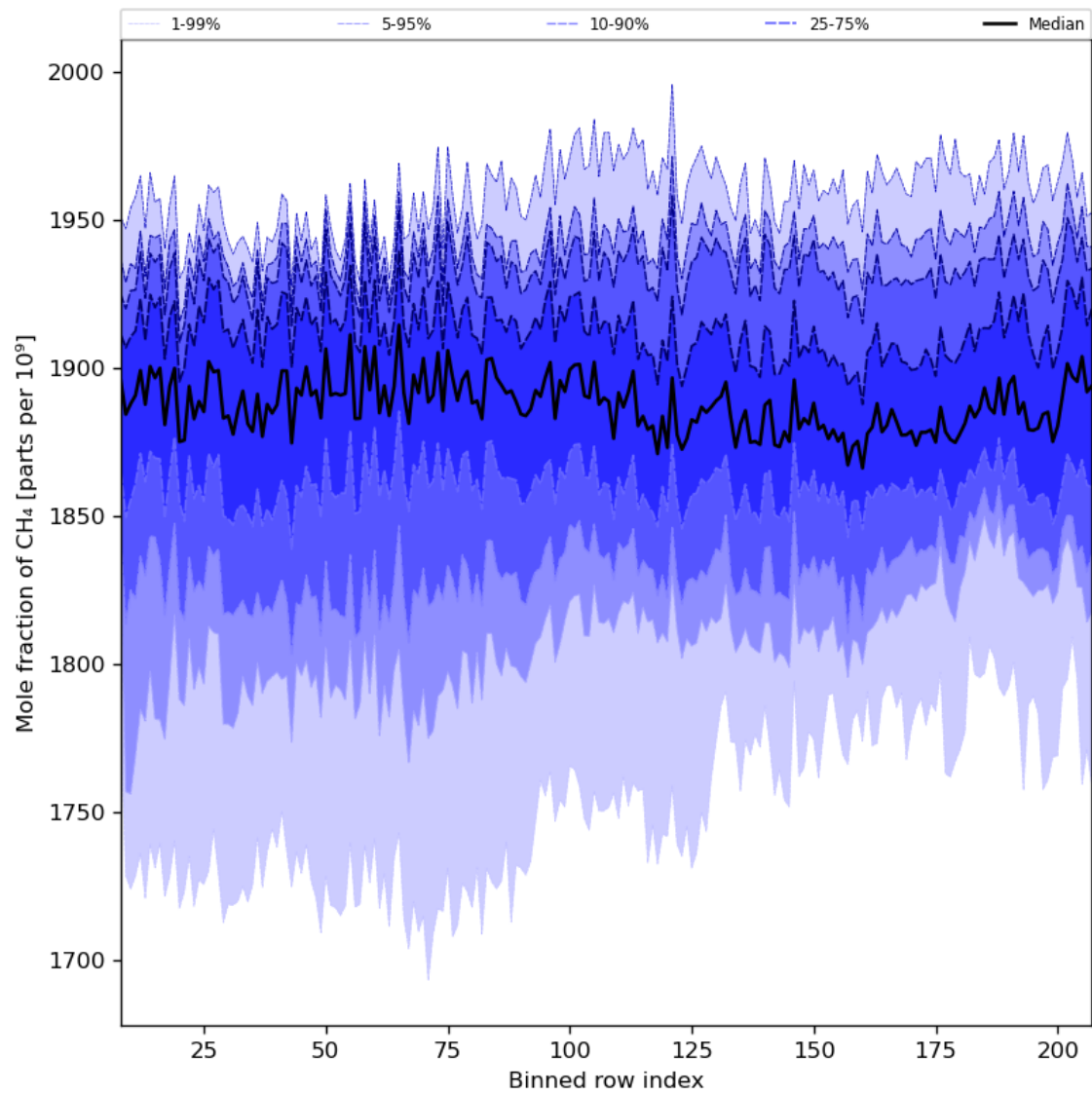
Figure 34: Along track statistics of “Mole fraction of CH 4 ” for 2024-03-17 to 2024-03-19
