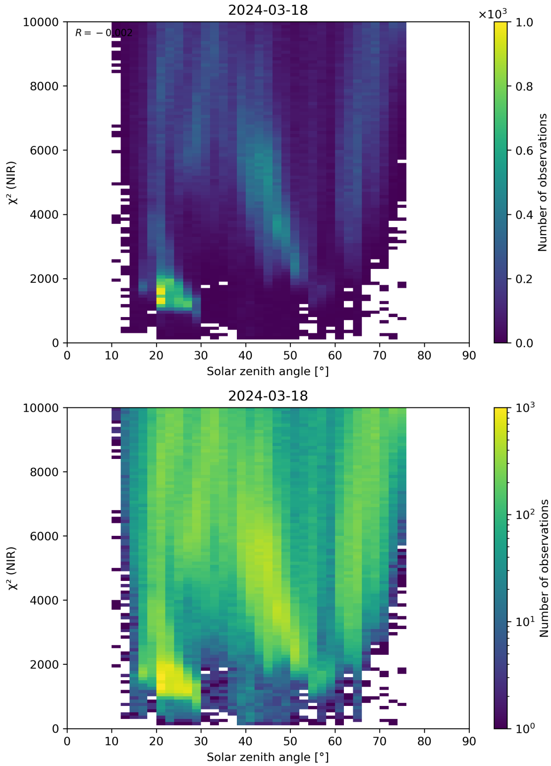
Figure 94: Scatter density plot of “Solar zenith angle” against “ \chi^2 (NIR)” for 2024-03-17 to 2024-03-19.
