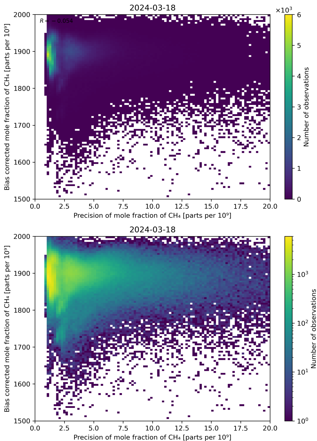
Figure 82: Scatter density plot of “Precision of mole fraction of CH 4 ” against “Bias corrected mole fraction of CH 4 ” for 2024-03-17 to 2024-03-19.
