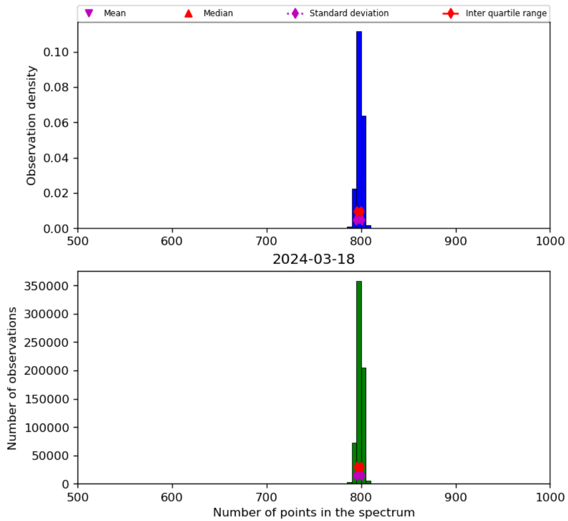
Figure 26: Histogram of “Number of points in the spectrum” for 2024-03-17 to 2024-03-19
