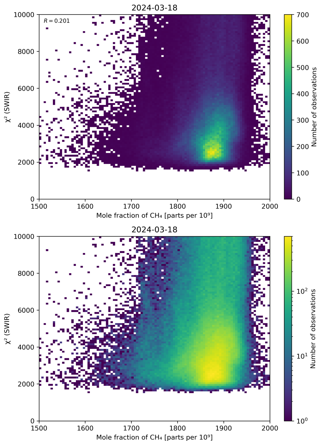
Figure 71: Scatter density plot of “Mole fraction of CH 4 ” against “ \chi^2 (SWIR)” for 2024-03-17 to 2024-03-19.
