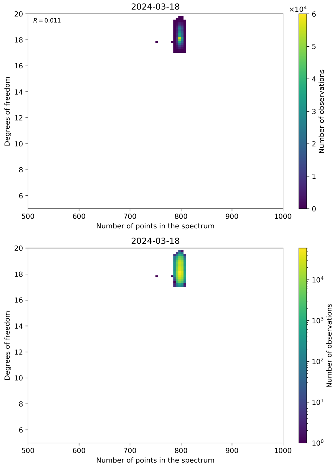
Figure 90: Scatter density plot of “Number of points in the spectrum” against “Degrees of freedom” for 2024-03-17 to 2024-03-19.
