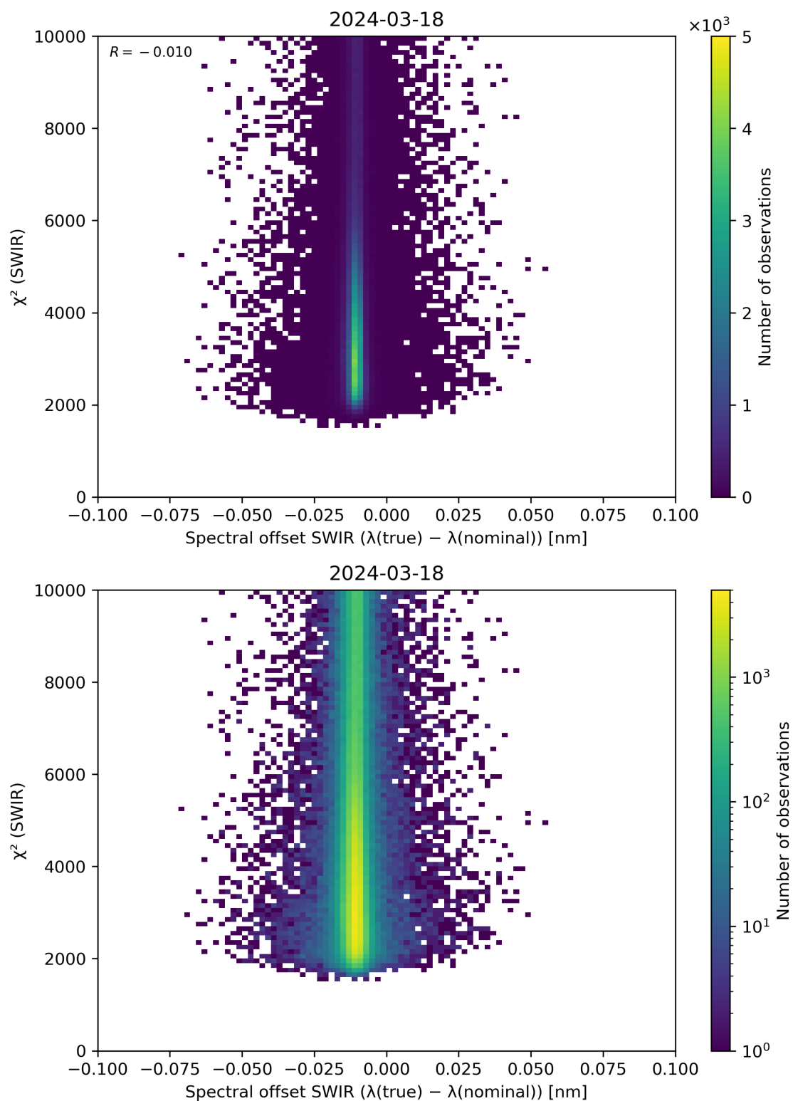
Figure 118: Scatter density plot of “Spectral offset SWIR ( \lambda(\text{true}) - \lambda(\text{nominal}) )” against “ \chi^2 (SWIR)” for 2024-03-17 to 2024-03-19.
