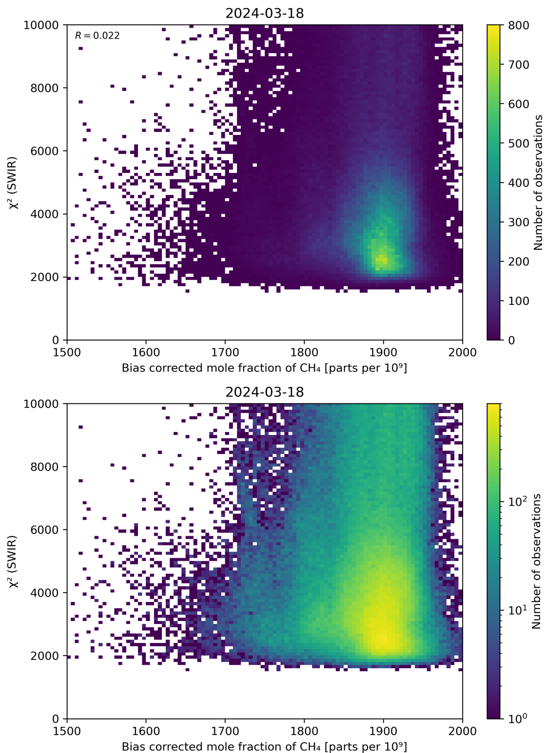
Figure 64: Scatter density plot of “Bias corrected mole fraction of CH 4 ” against “ \chi^2 (SWIR)” for 2024-03-17 to 2024-03-19.
