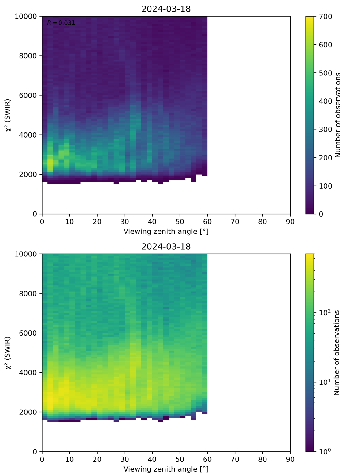
Figure 106: Scatter density plot of “Viewing zenith angle” against “ \chi^2 (SWIR)” for 2024-03-17 to 2024-03-19.
