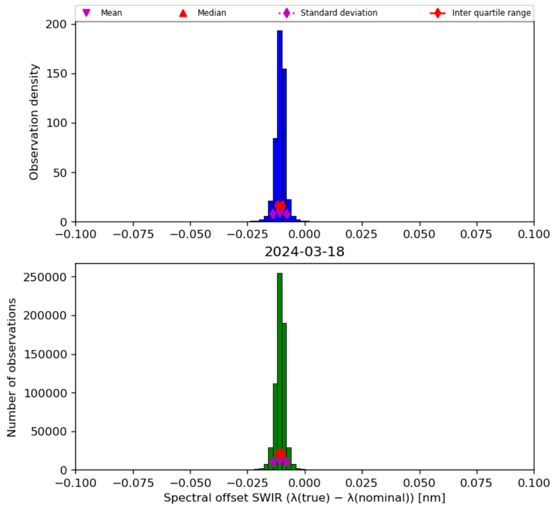
Figure 27: Histogram of “Spectral offset SWIR ( \lambda(\text{true}) - \lambda(\text{nominal}) )” for 2024-03-17 to 2024-03-19
