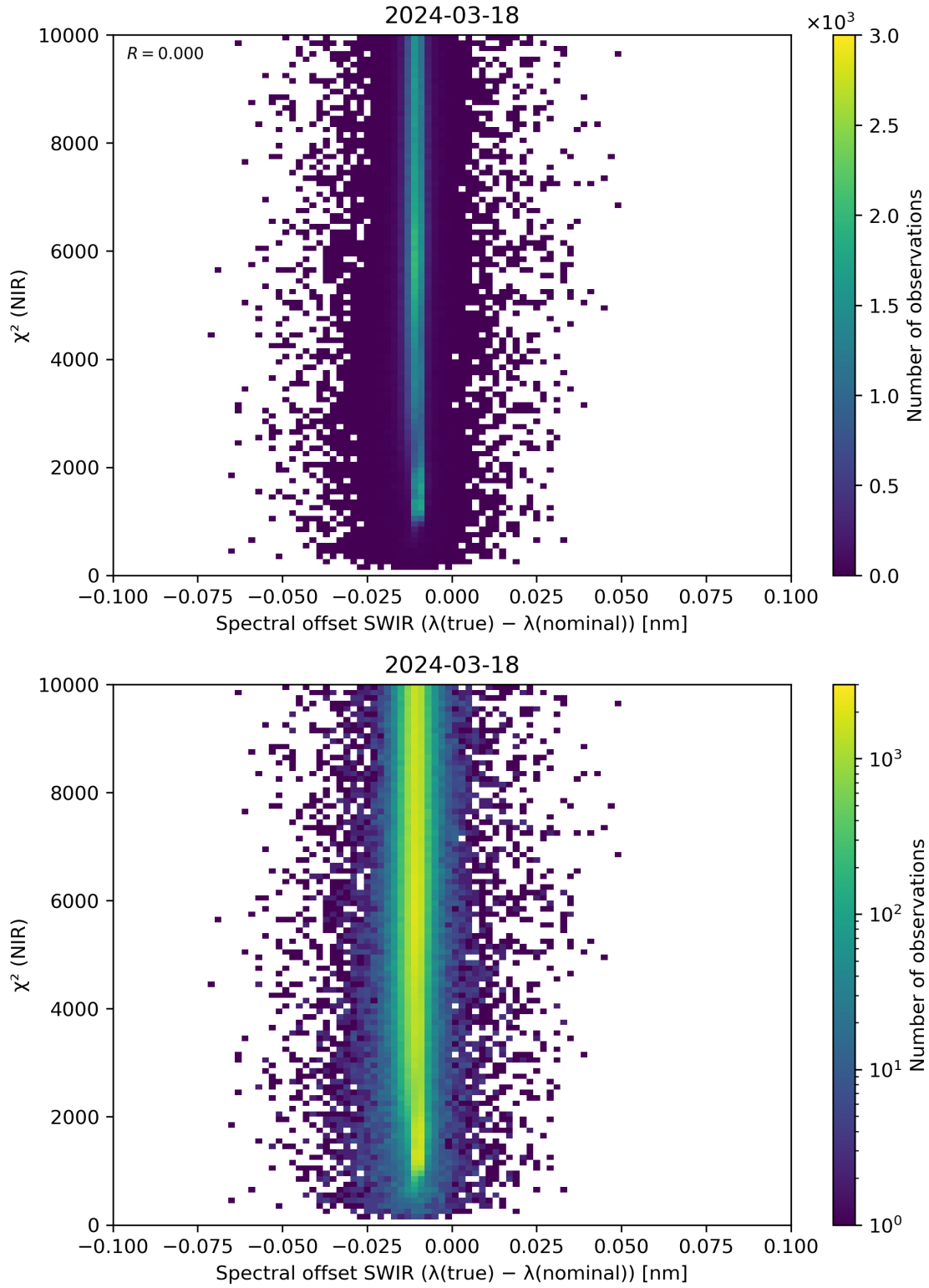
Figure 117: Scatter density plot of “Spectral offset SWIR ( \lambda(\text{true}) - \lambda(\text{nominal}) )” against “ \chi^2 (NIR)” for 2024-03-17 to 2024-03-19.
