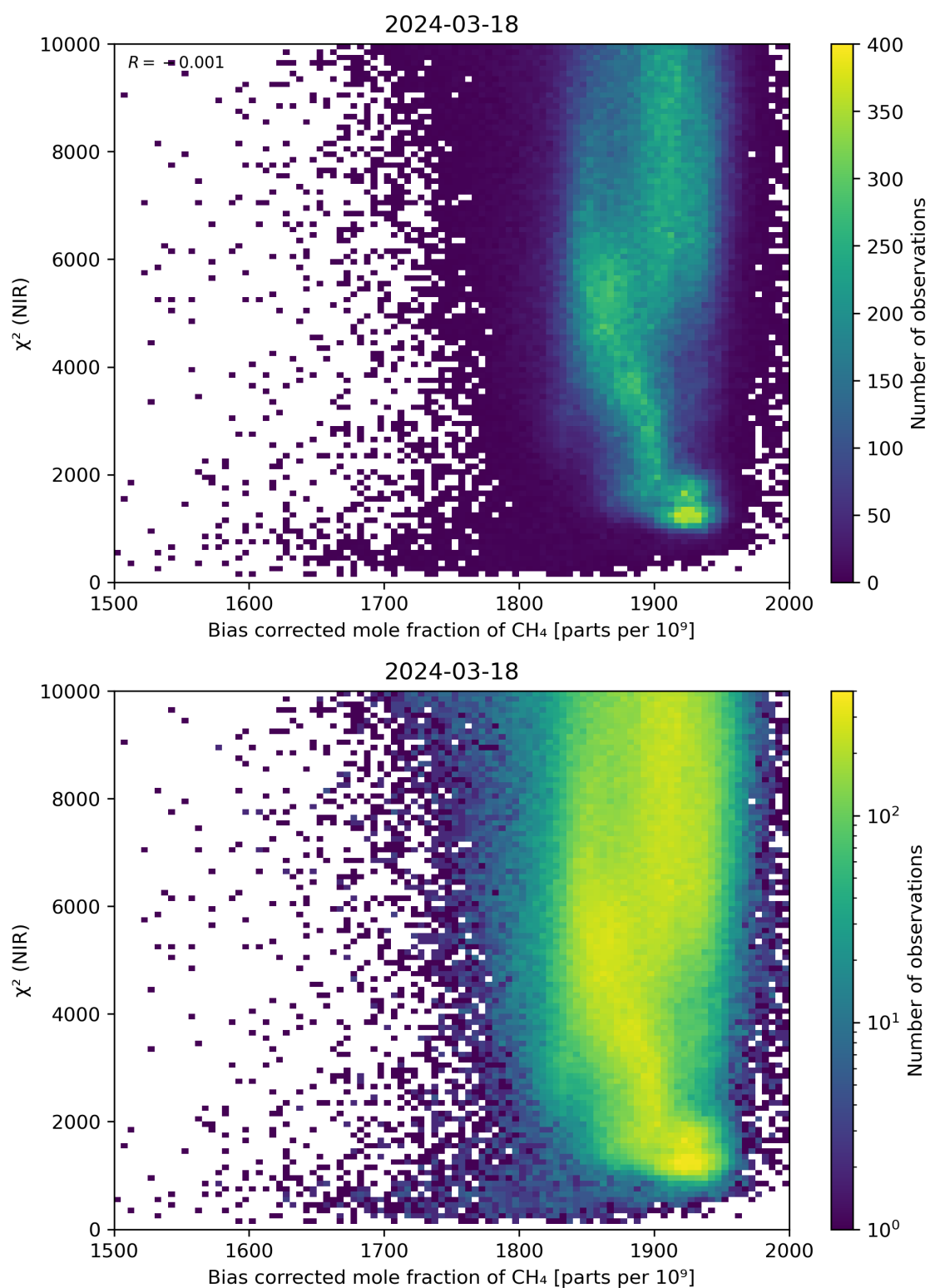
Figure 63: Scatter density plot of “Bias corrected mole fraction of CH 4 ” against “ \chi^2 (NIR)” for 2024-03-17 to 2024-03-19.
