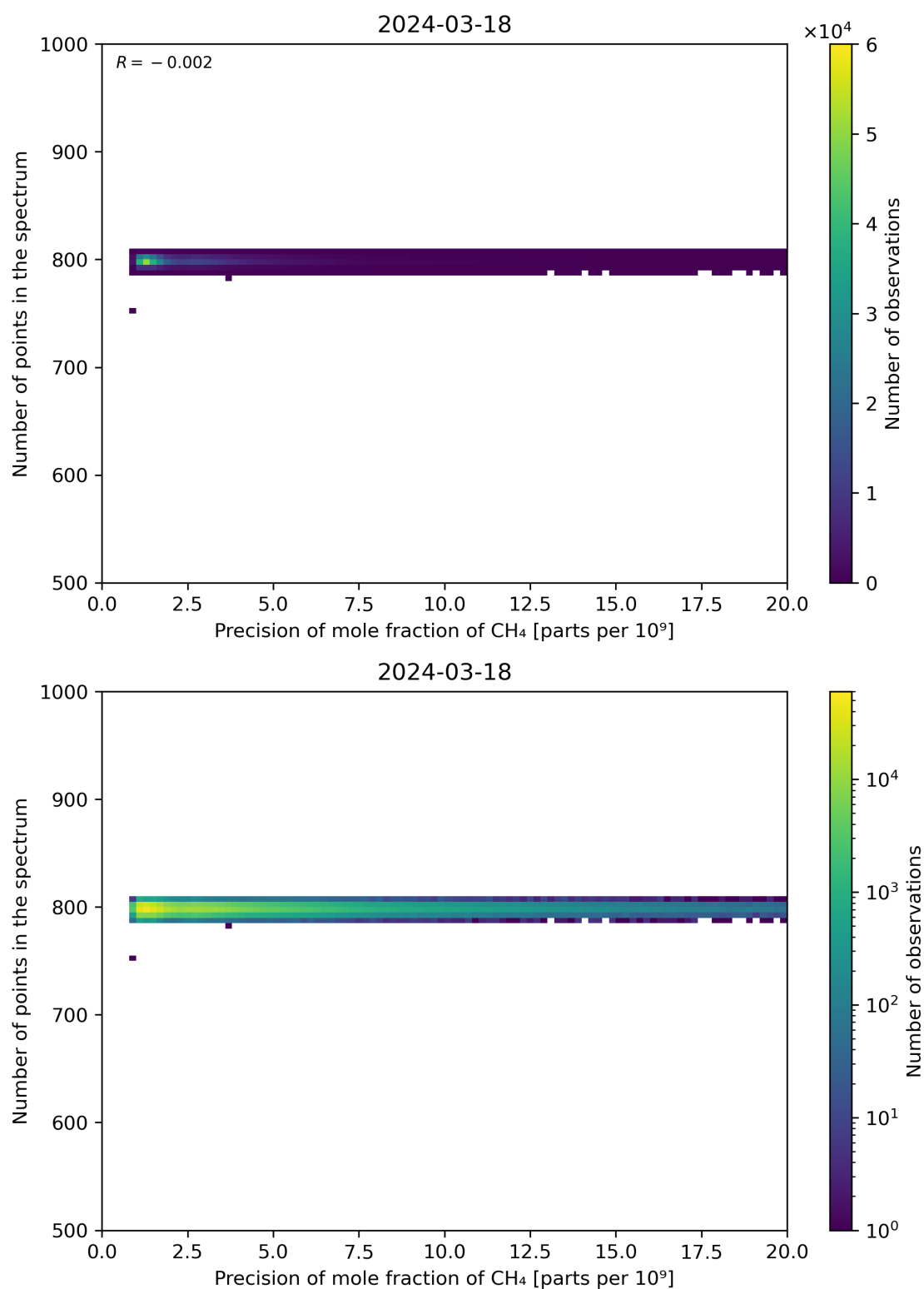
Figure 84: Scatter density plot of “Precision of mole fraction of CH 4 ” against “Number of points in the spectrum” for 2024-03-17 to 2024-03-19.
