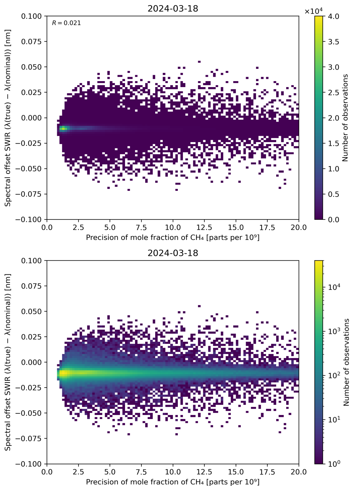
Figure 85: Scatter density plot of “Precision of mole fraction of CH 4 ” against “Spectral offset SWIR ( \lambda(\text{true}) - \lambda(\text{nominal}) )” for 2024-03-17 to 2024-03-19.
