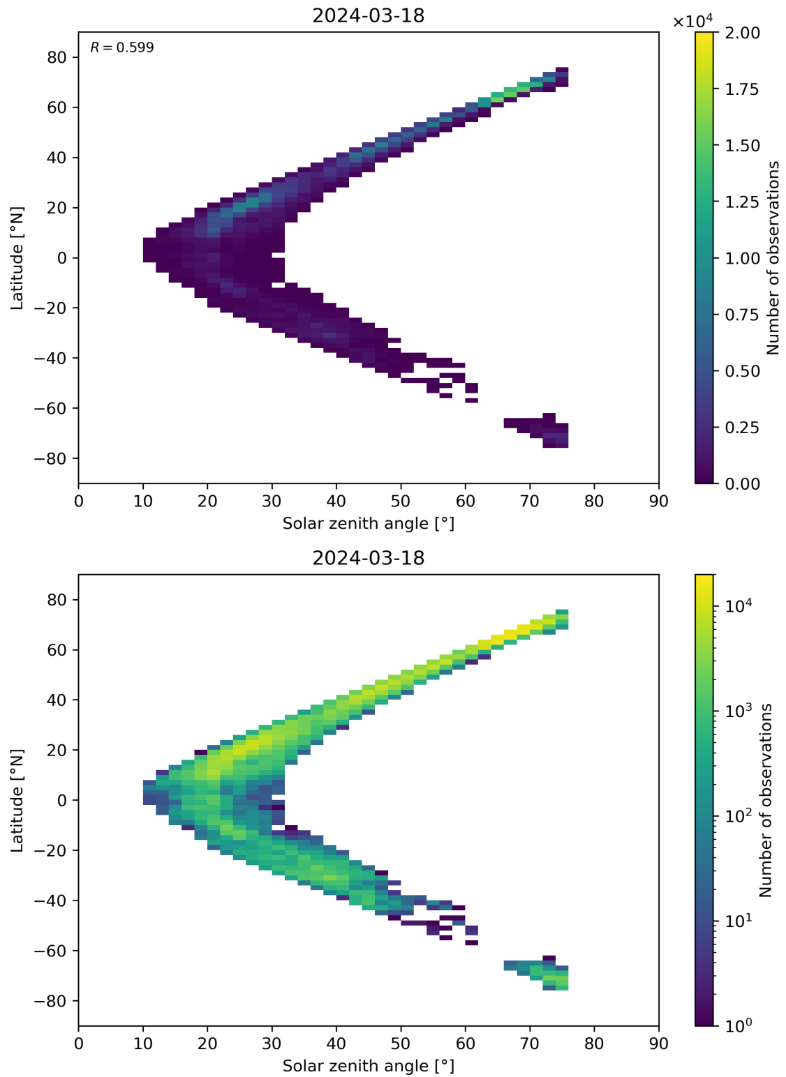
Figure 98: Scatter density plot of “Solar zenith angle” against “Latitude” for 2024-03-17 to 2024-03-19.
