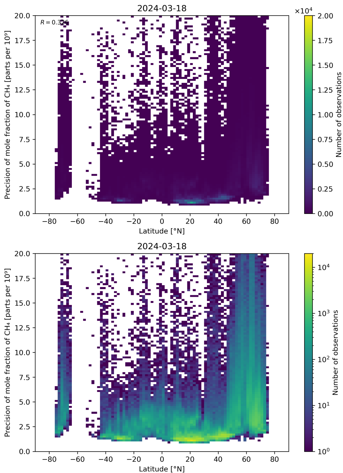
Figure 59: Scatter density plot of “Latitude” against “Precision of mole fraction of CH 4 ” for 2024-03-17 to 2024-03-19.
