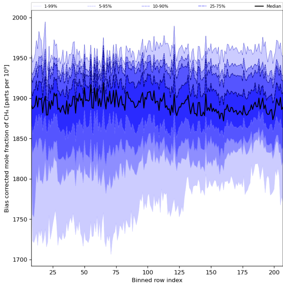
Figure 36: Along track statistics of “Bias corrected mole fraction of CH 4 ” for 2024-03-17 to 2024-03-19
