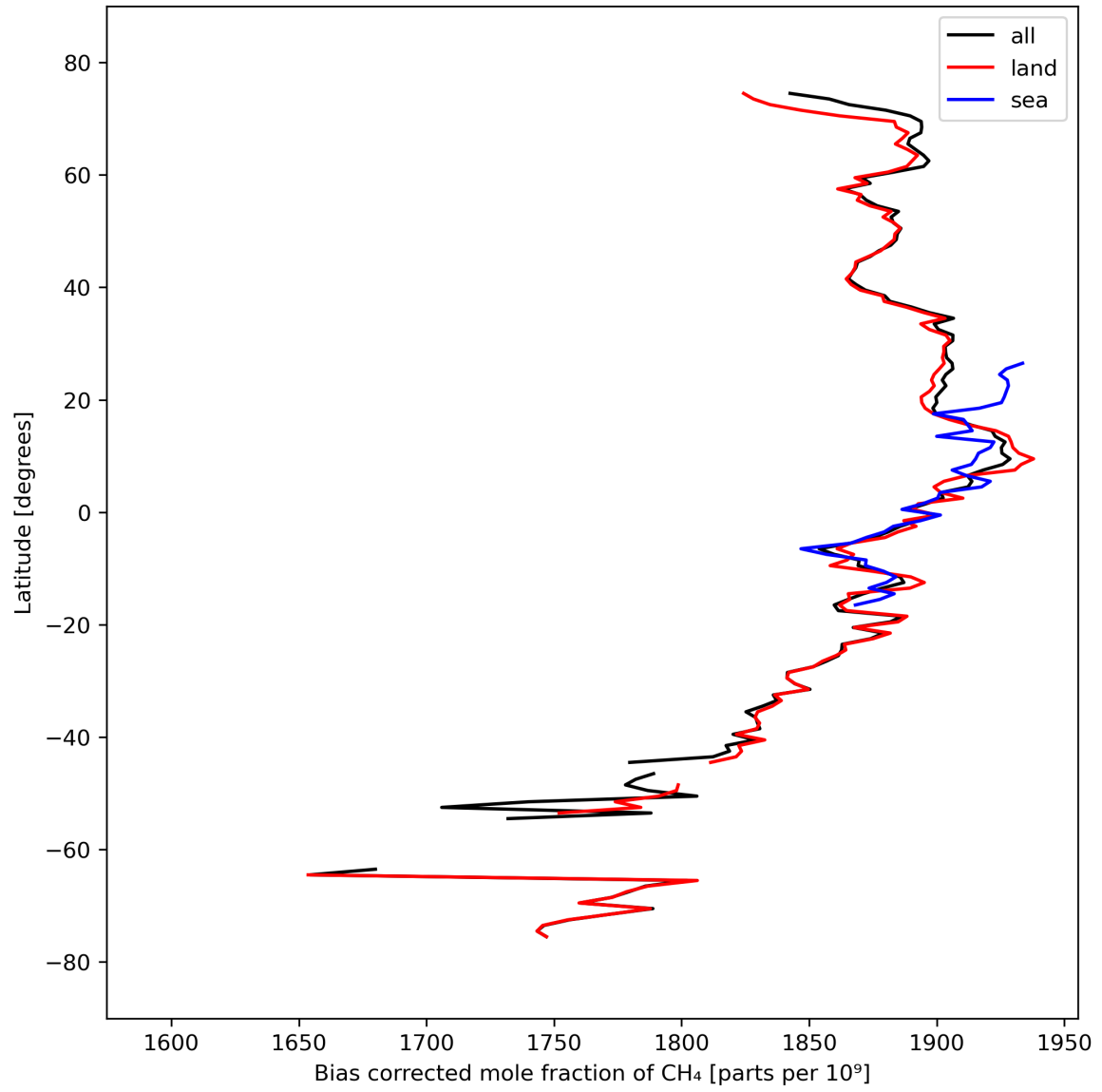
Figure 14: Zonal average of “Bias corrected mole fraction of \text{CH}_4 ” for 2024-03-17 to 2024-03-19.
