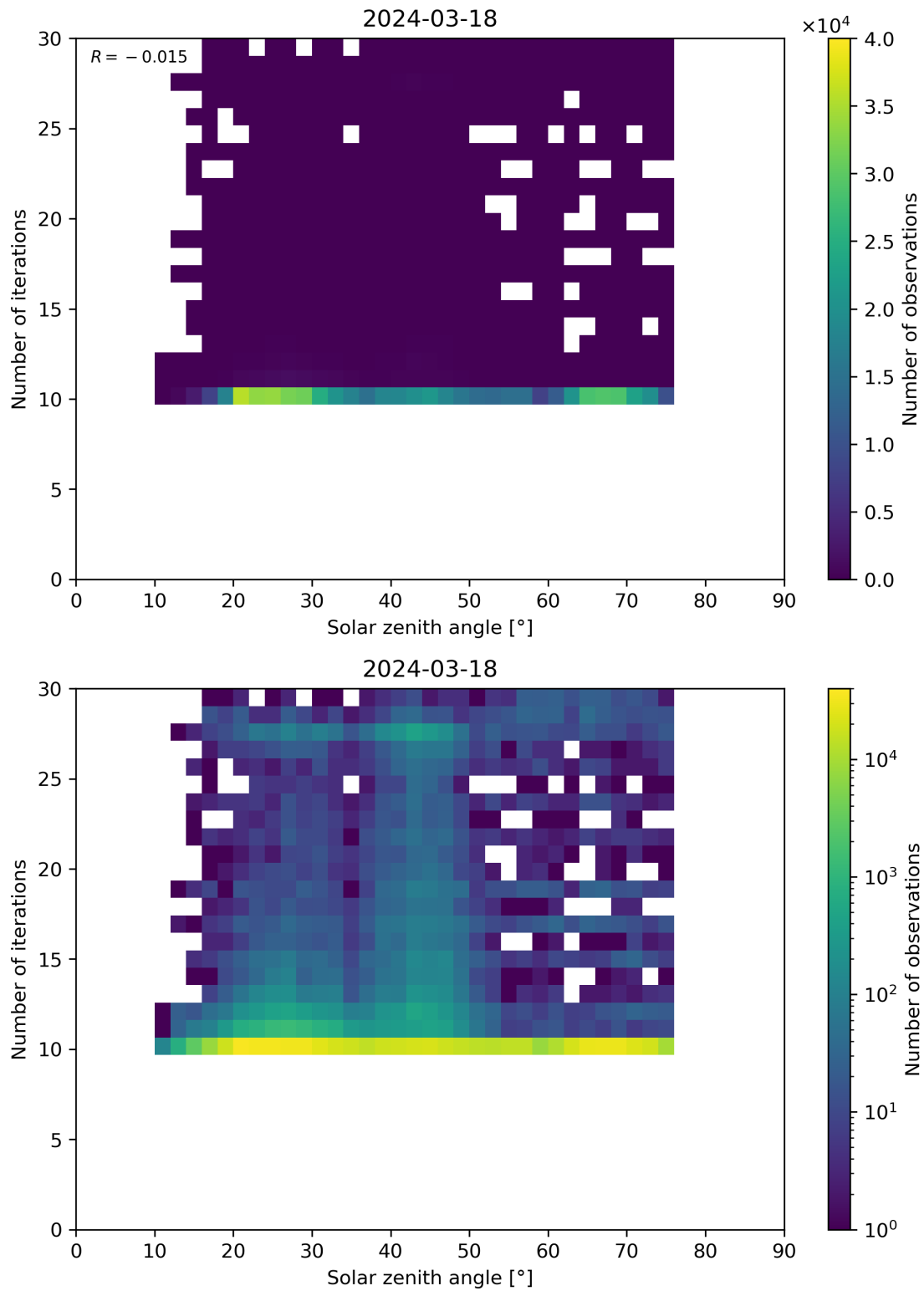
Figure 102: Scatter density plot of “Solar zenith angle” against “Number of iterations” for 2024-03-17 to 2024-03-19.
