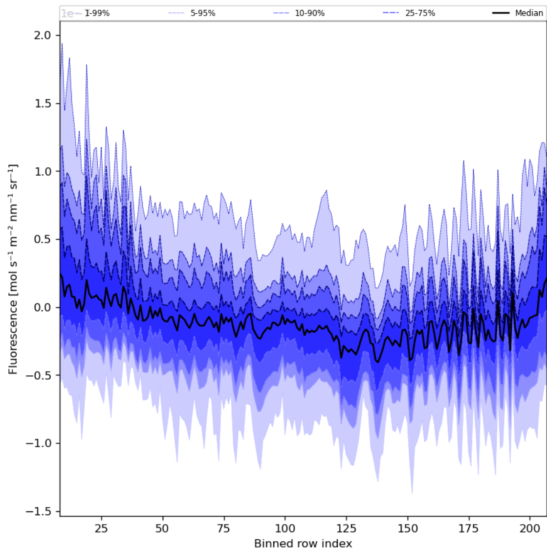
Figure 43: Along track statistics of “Fluorescence” for 2024-03-17 to 2024-03-19
