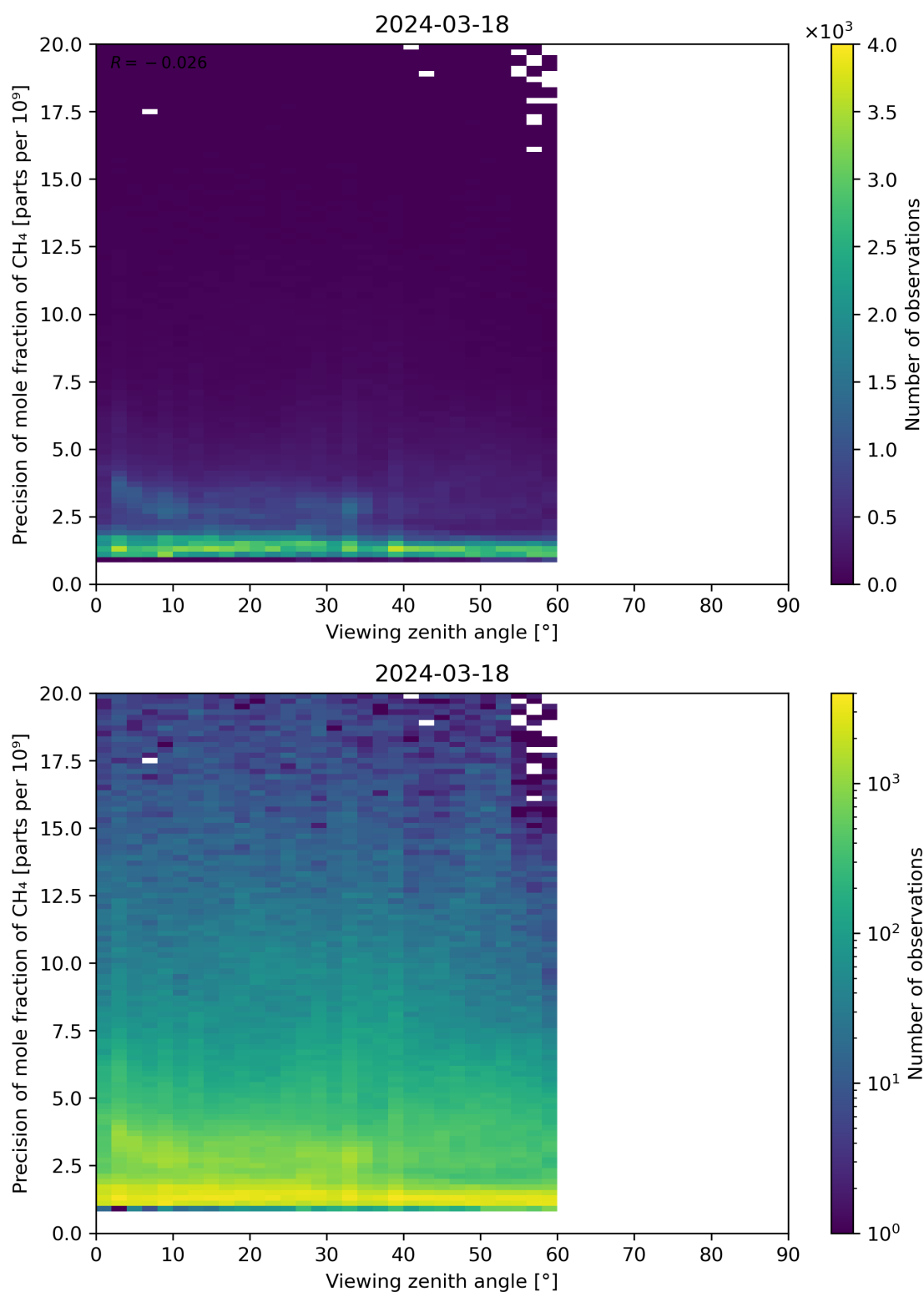
Figure 112: Scatter density plot of “Viewing zenith angle” against “Precision of mole fraction of CH 4 ” for 2024-03-17 to 2024-03-19.
