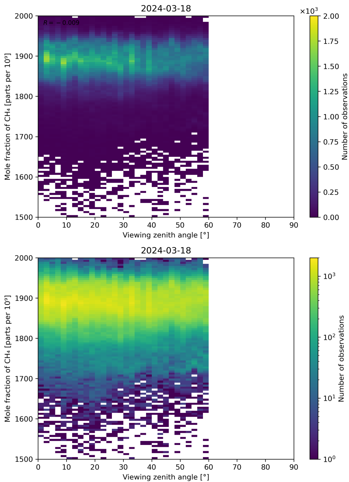
Figure 110: Scatter density plot of “Viewing zenith angle” against “Mole fraction of CH 4 ” for 2024-03-17 to 2024-03-19.
