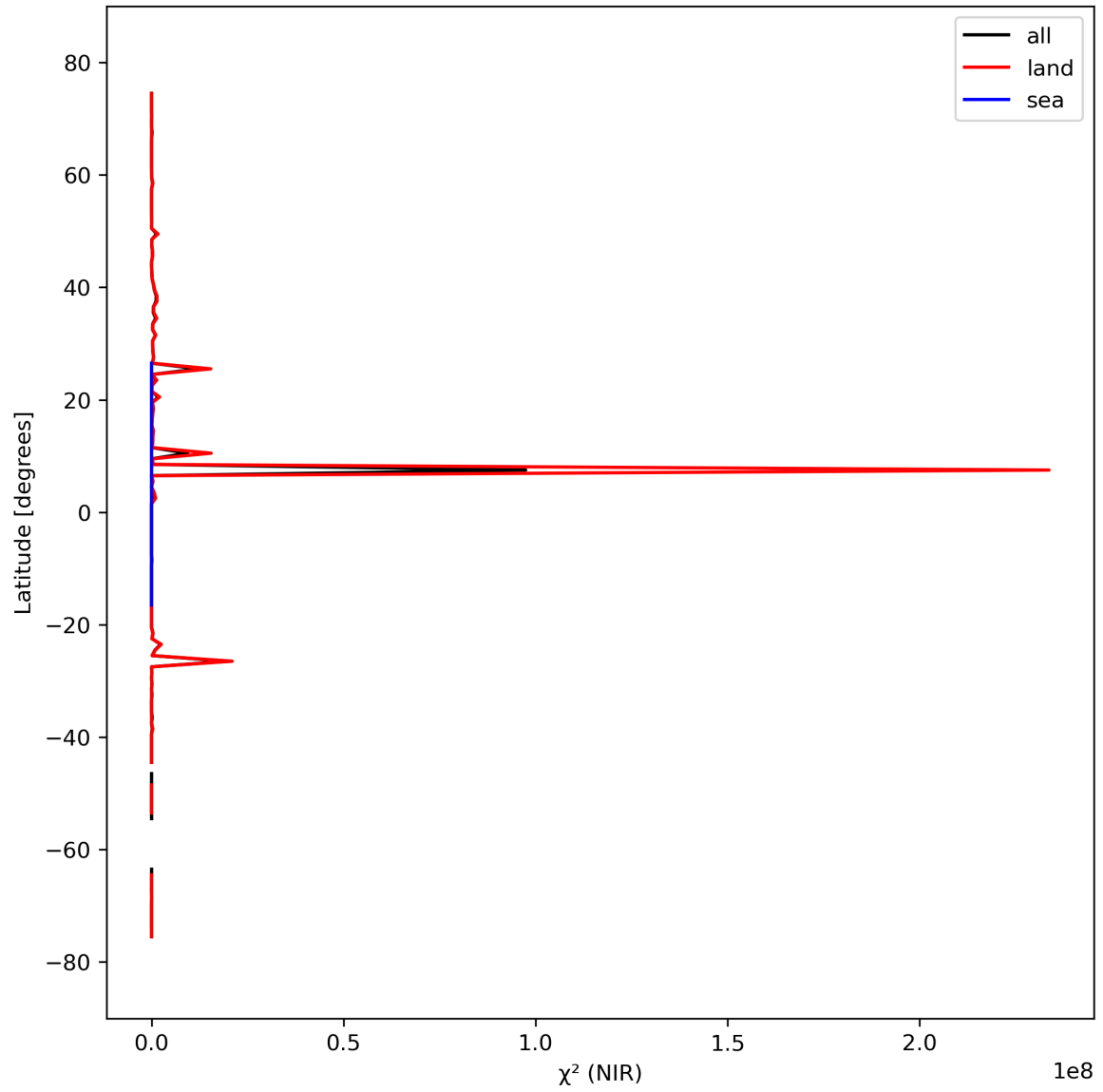
Figure 18: Zonal average of “ \chi^2 (NIR)” for 2024-03-17 to 2024-03-19.
