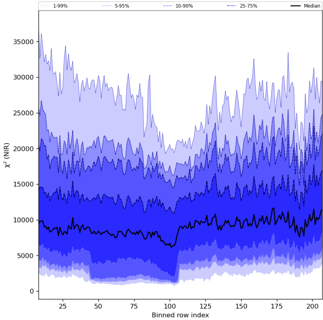
Figure 40: Along track statistics of “ \chi^2 (NIR)” for 2024-03-17 to 2024-03-19
