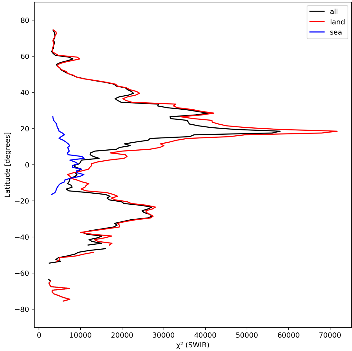
Figure 17: Zonal average of “ \chi^2 (SWIR)” for 2024-03-17 to 2024-03-19.
