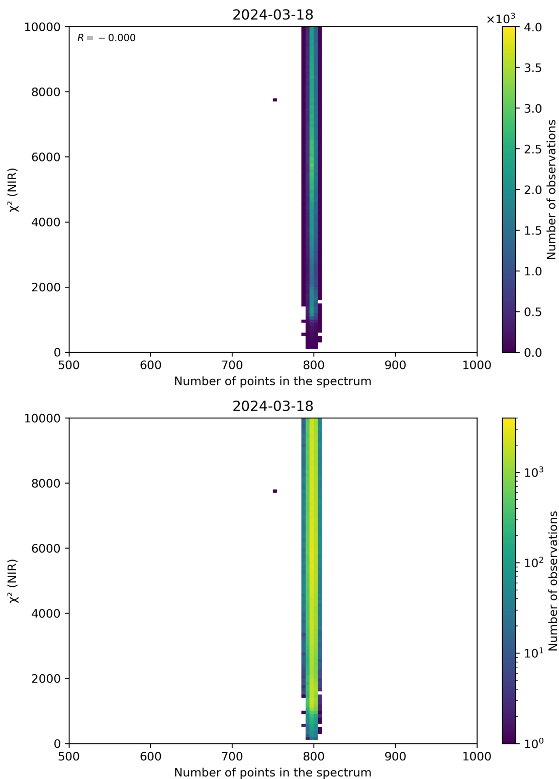
Figure 88: Scatter density plot of “Number of points in the spectrum” against “ \chi^2 (NIR)” for 2024-03-17 to 2024-03-19.
