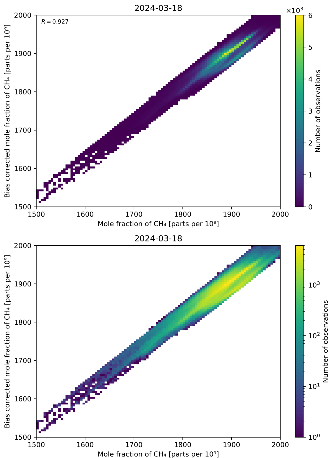
Figure 74: Scatter density plot of “Mole fraction of CH 4 ” against “Bias corrected mole fraction of CH 4 ” for 2024-03-17 to 2024-03-19.
