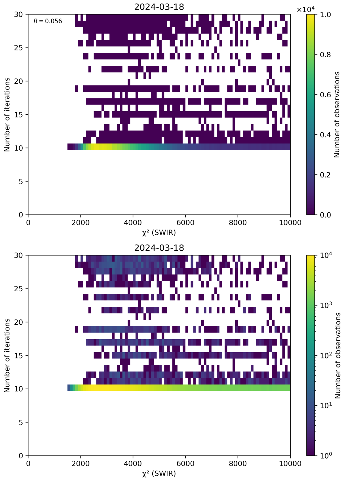
Figure 50: Scatter density plot of “ \chi^2 (SWIR)” against “Number of iterations” for 2024-03-17 to 2024-03-19.
