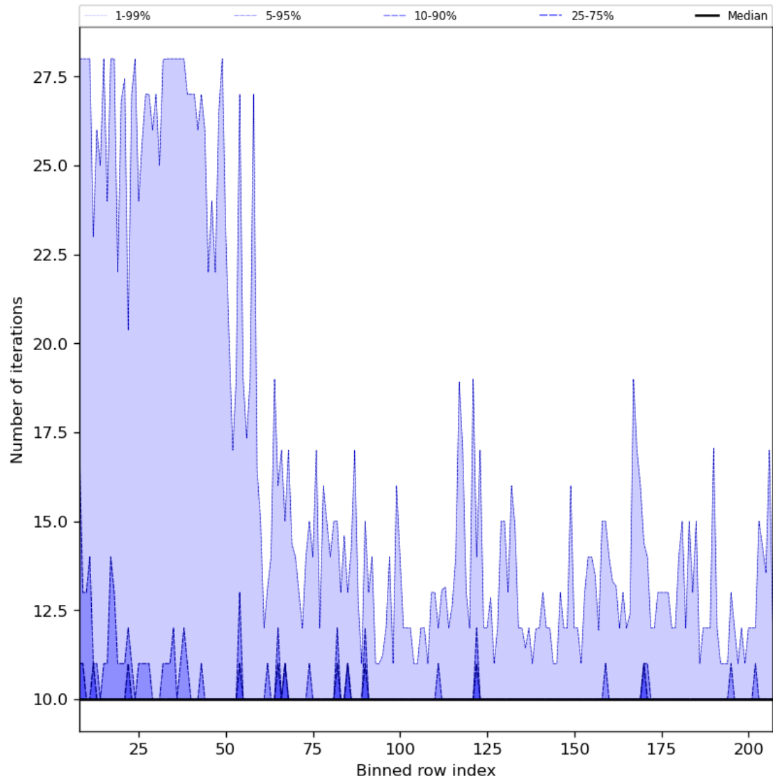
Figure 42: Along track statistics of “Number of iterations” for 2024-03-17 to 2024-03-19
