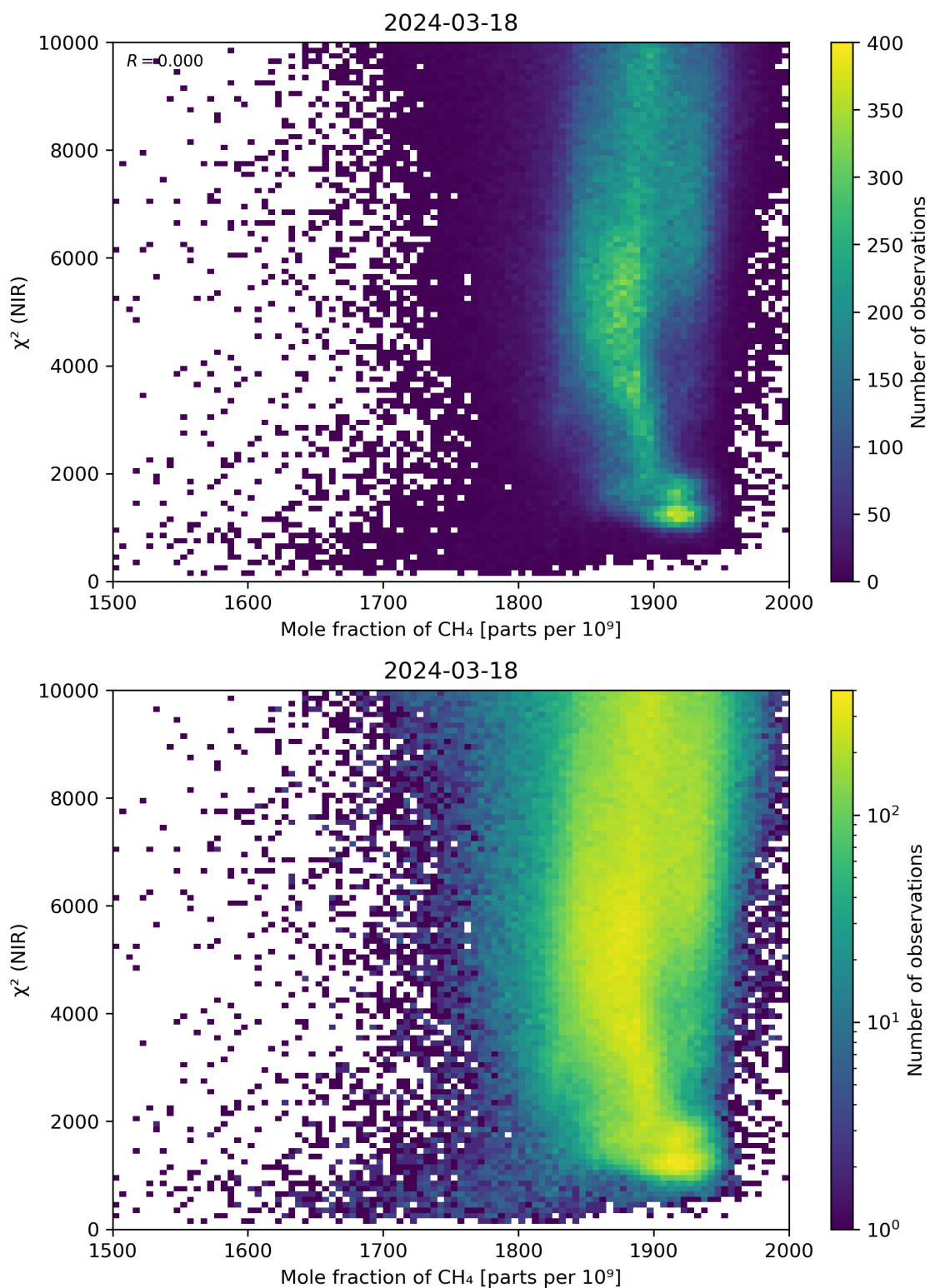
Figure 70: Scatter density plot of “Mole fraction of CH 4 ” against “ \chi^2 (NIR)” for 2024-03-17 to 2024-03-19.
