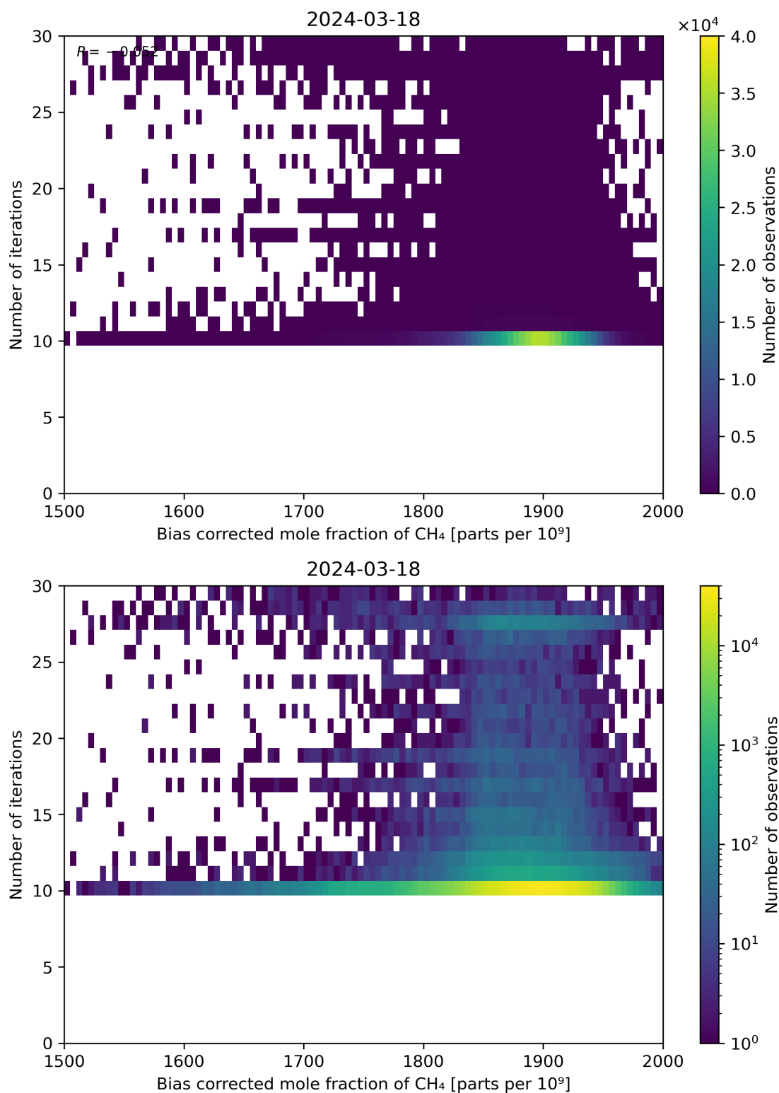
Figure 67: Scatter density plot of “Bias corrected mole fraction of CH 4 ” against “Number of iterations” for 2024-03-17 to 2024-03-19.
