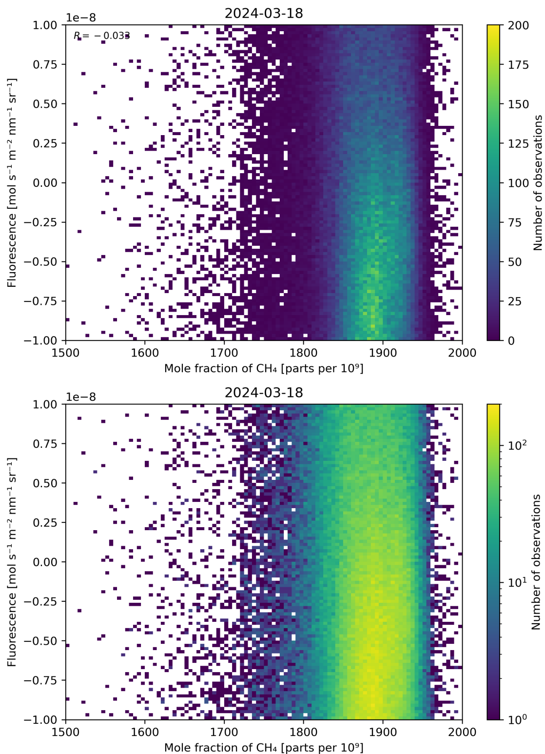
Figure 73: Scatter density plot of “Mole fraction of \text{CH}_4 ” against “Fluorescence” for 2024-03-17 to 2024-03-19.
