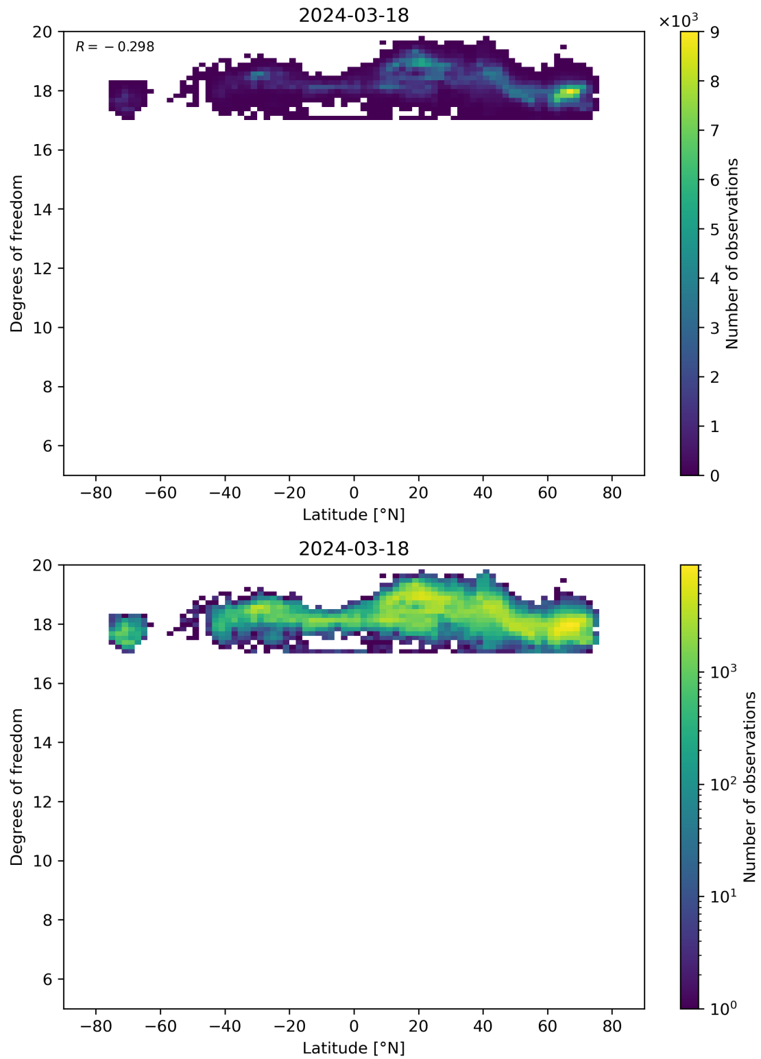
Figure 55: Scatter density plot of “Latitude” against “Degrees of freedom” for 2024-03-17 to 2024-03-19.
