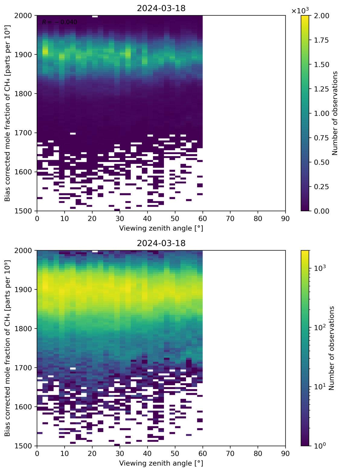
Figure 111: Scatter density plot of “Viewing zenith angle” against “Bias corrected mole fraction of CH 4 ” for 2024-03-17 to 2024-03-19.
