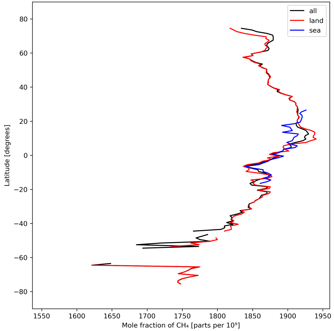
Figure 12: Zonal average of “Mole fraction of \text{CH}_4 ” for 2024-03-17 to 2024-03-19.
