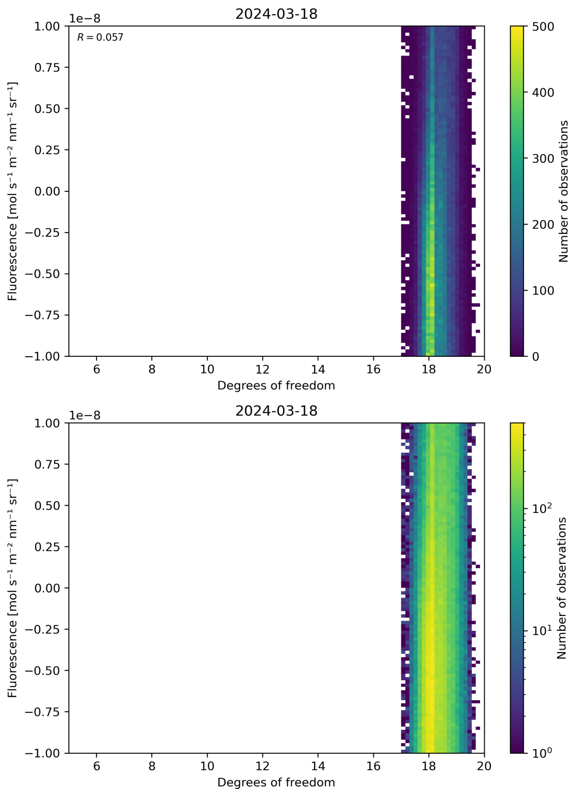
Figure 51: Scatter density plot of “Degrees of freedom” against “Fluorescence” for 2024-03-17 to 2024-03-19.
