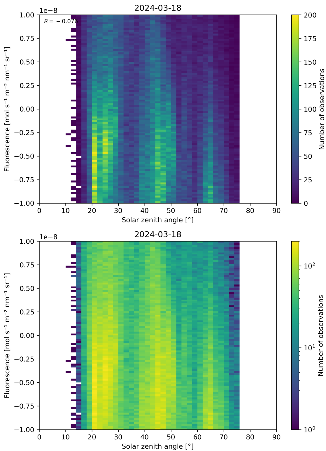
Figure 97: Scatter density plot of “Solar zenith angle” against “Fluorescence” for 2024-03-17 to 2024-03-19.
