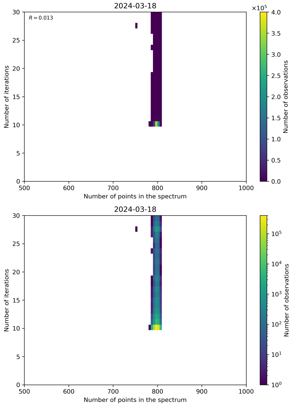
Figure 92: Scatter density plot of “Number of points in the spectrum” against “Number of iterations” for 2024-03-17 to 2024-03-19.
