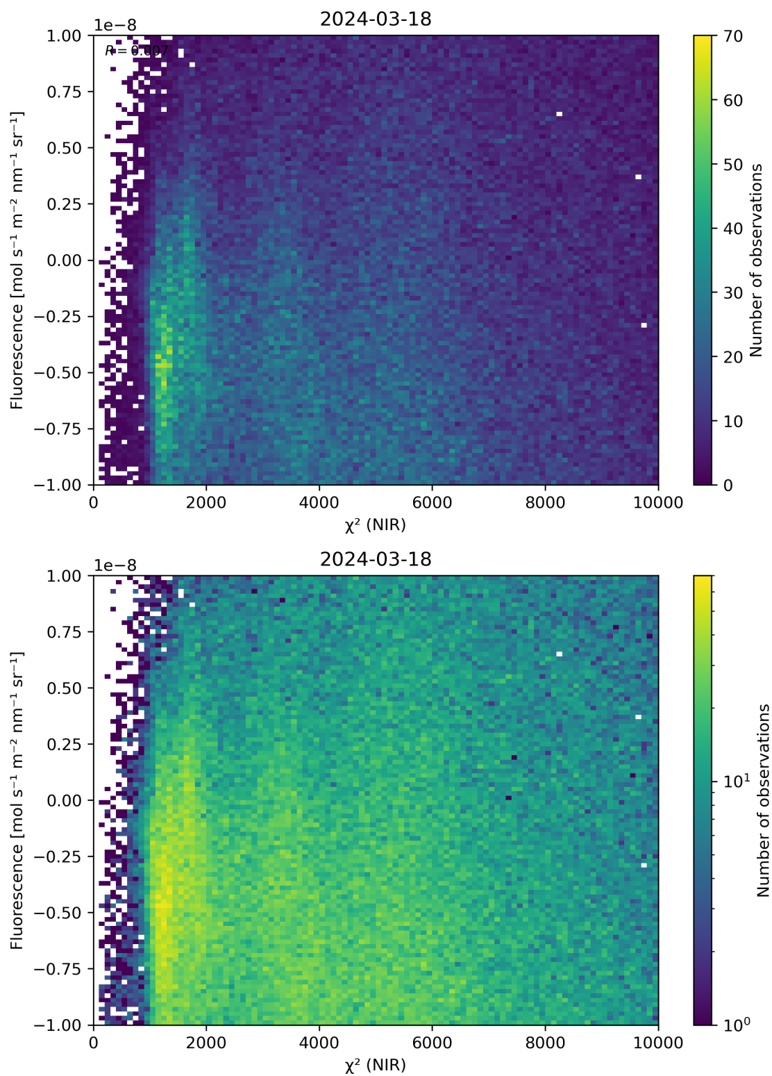
Figure 45: Scatter density plot of “ \chi^2 (NIR)” against “Fluorescence” for 2024-03-17 to 2024-03-19.
