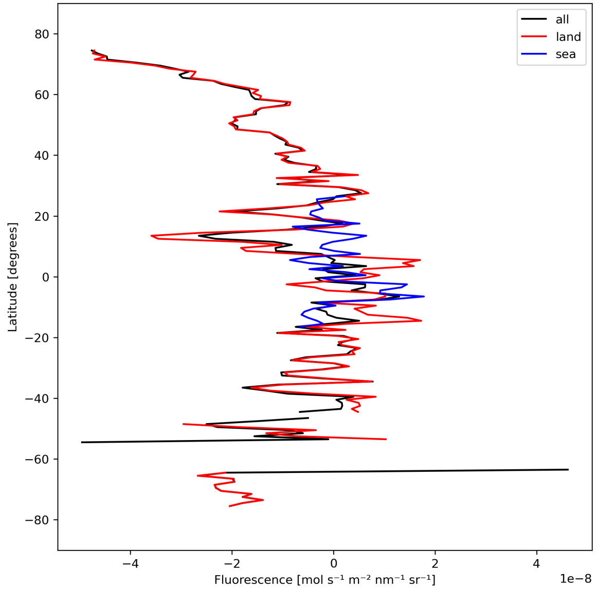
Figure 21: Zonal average of “Fluorescence” for 2024-03-17 to 2024-03-19.
