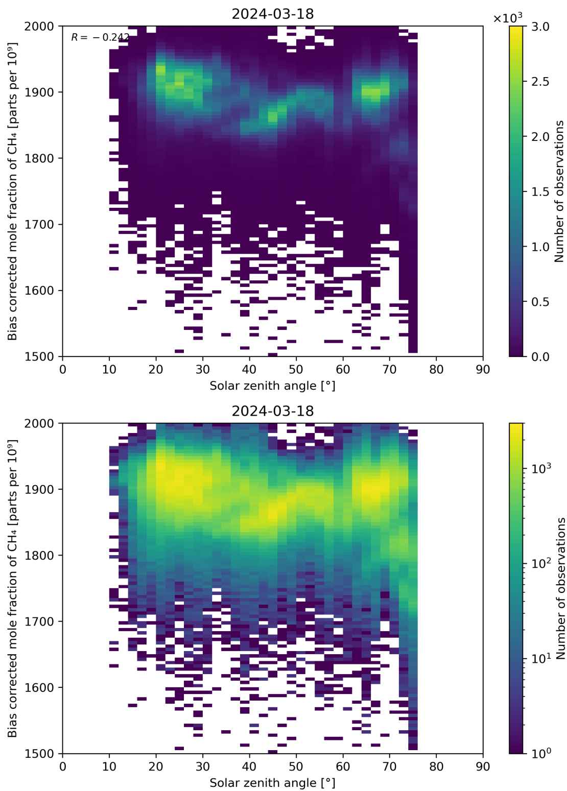
Figure 100: Scatter density plot of “Solar zenith angle” against “Bias corrected mole fraction of CH 4 ” for 2024-03-17 to 2024-03-19.
