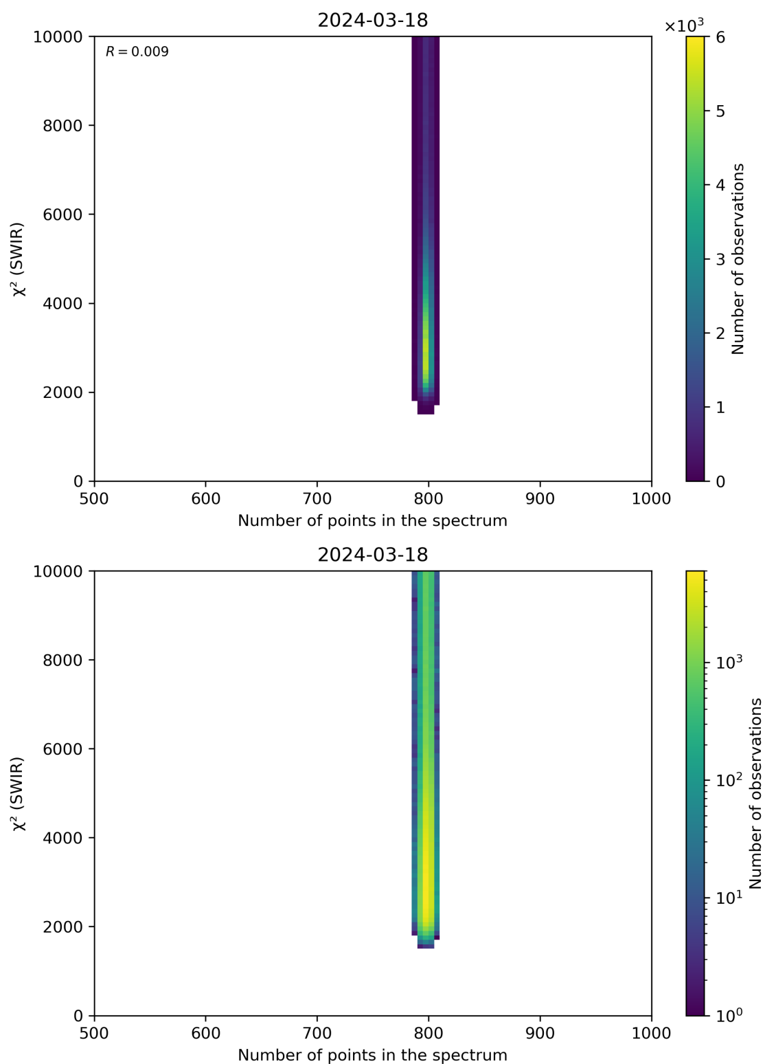
Figure 89: Scatter density plot of “Number of points in the spectrum” against “ \chi^2 (SWIR)” for 2024-03-17 to 2024-03-19.
