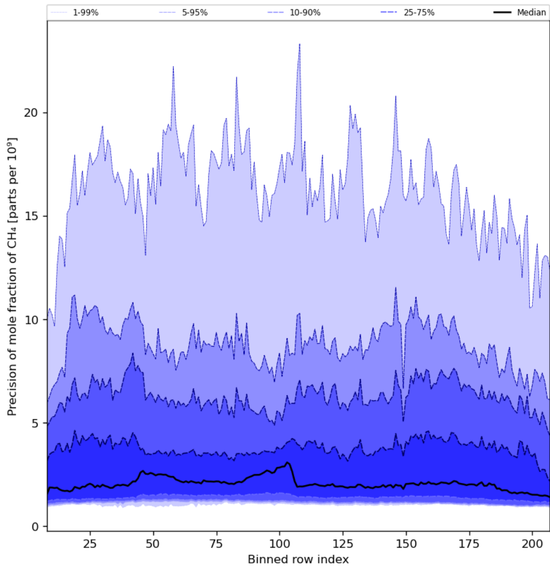
Figure 35: Along track statistics of “Precision of mole fraction of CH 4 ” for 2024-03-17 to 2024-03-19
