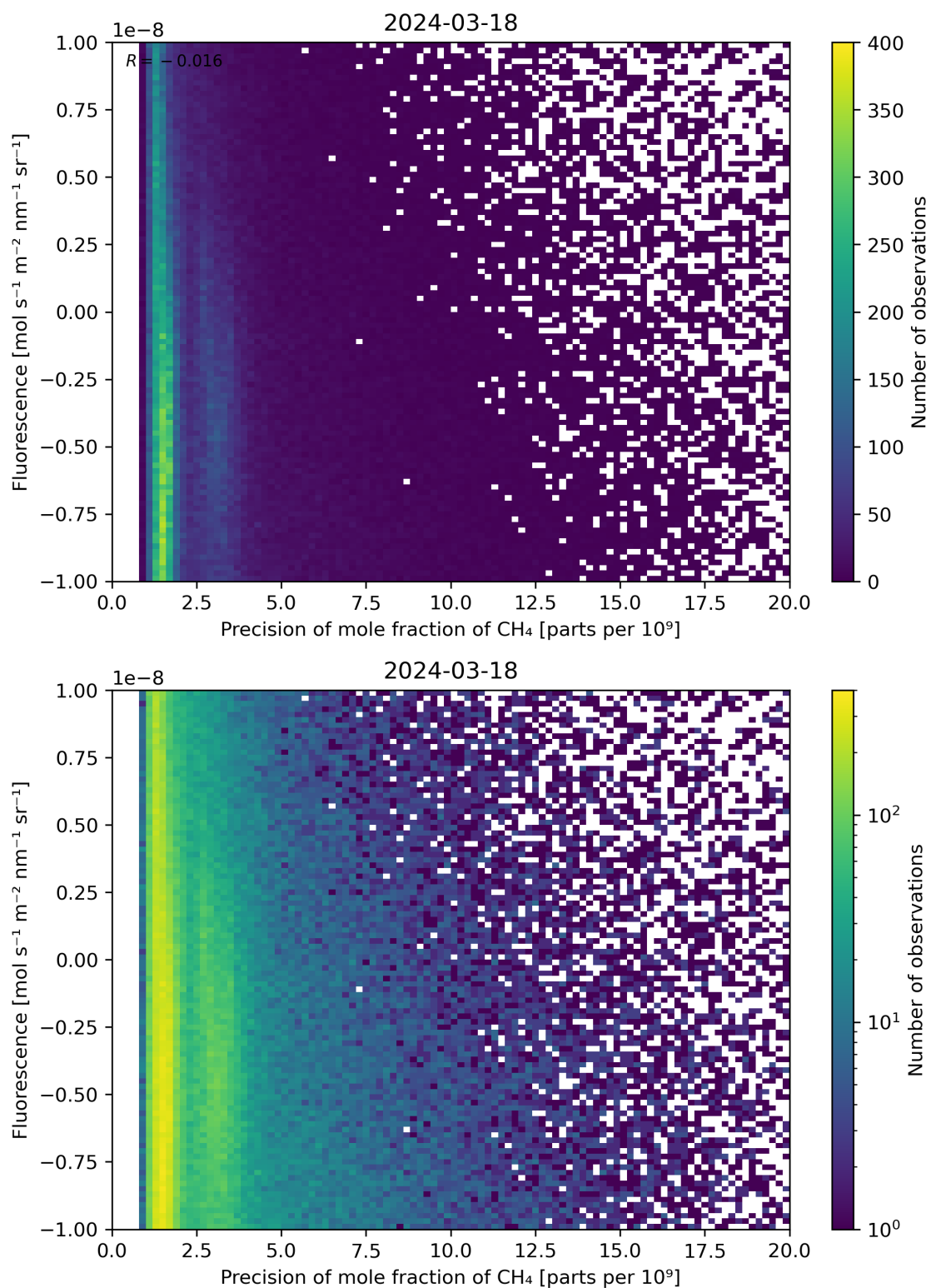
Figure 81: Scatter density plot of “Precision of mole fraction of \text{CH}_4 ” against “Fluorescence” for 2024-03-17 to 2024-03-19.
