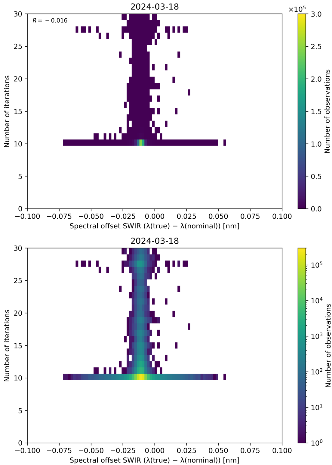
Figure 121: Scatter density plot of “Spectral offset SWIR ( \lambda(\text{true}) - \lambda(\text{nominal}) )” against “Number of iterations” for 2024-03-17 to 2024-03-19.
