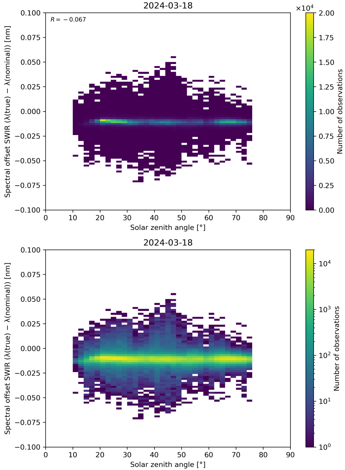
Figure 104: Scatter density plot of “Solar zenith angle” against “Spectral offset SWIR ( \lambda(\text{true}) - \lambda(\text{nominal}) )” for 2024-03-17 to 2024-03-19.
