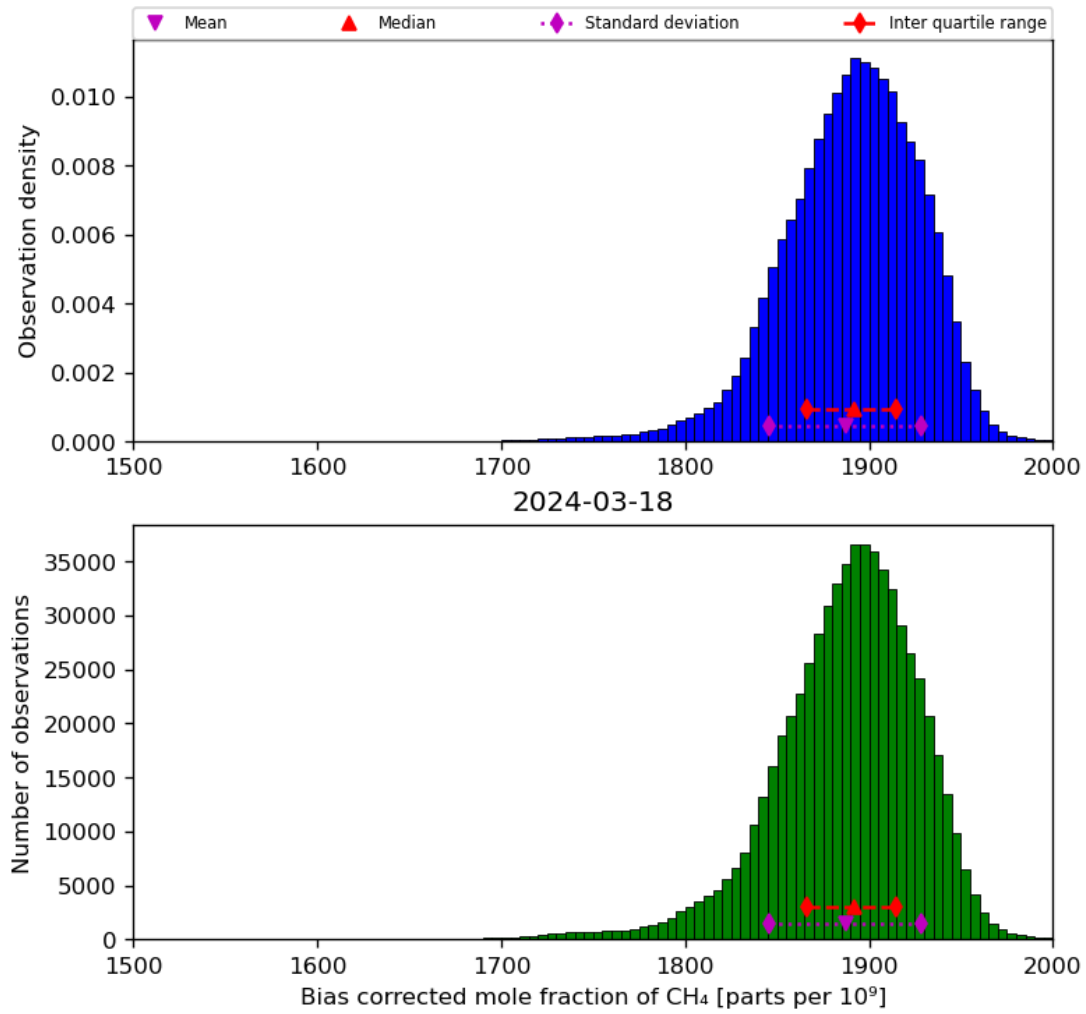
Figure 25: Histogram of “Bias corrected mole fraction of CH 4 ” for 2024-03-17 to 2024-03-19
