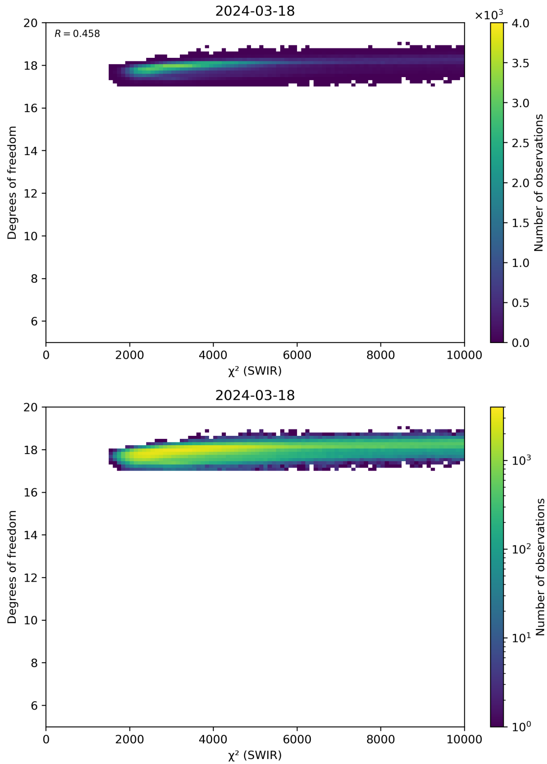
Figure 48: Scatter density plot of “ \chi^2 (SWIR)” against “Degrees of freedom” for 2024-03-17 to 2024-03-19.
