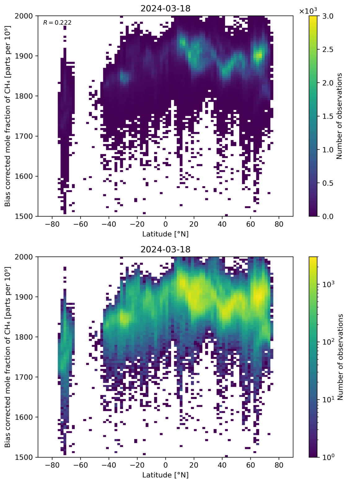
Figure 58: Scatter density plot of “Latitude” against “Bias corrected mole fraction of \text{CH}_4 ” for 2024-03-17 to 2024-03-19.
