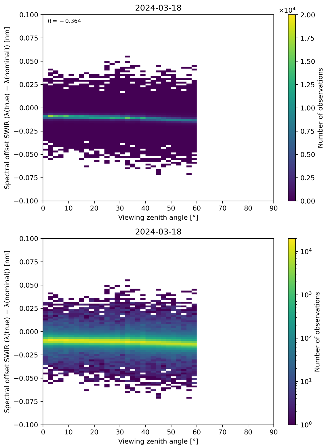
Figure 116: Scatter density plot of “Viewing zenith angle” against “Spectral offset SWIR ( \lambda(\text{true}) - \lambda(\text{nominal}) )” for 2024-03-17 to 2024-03-19.
