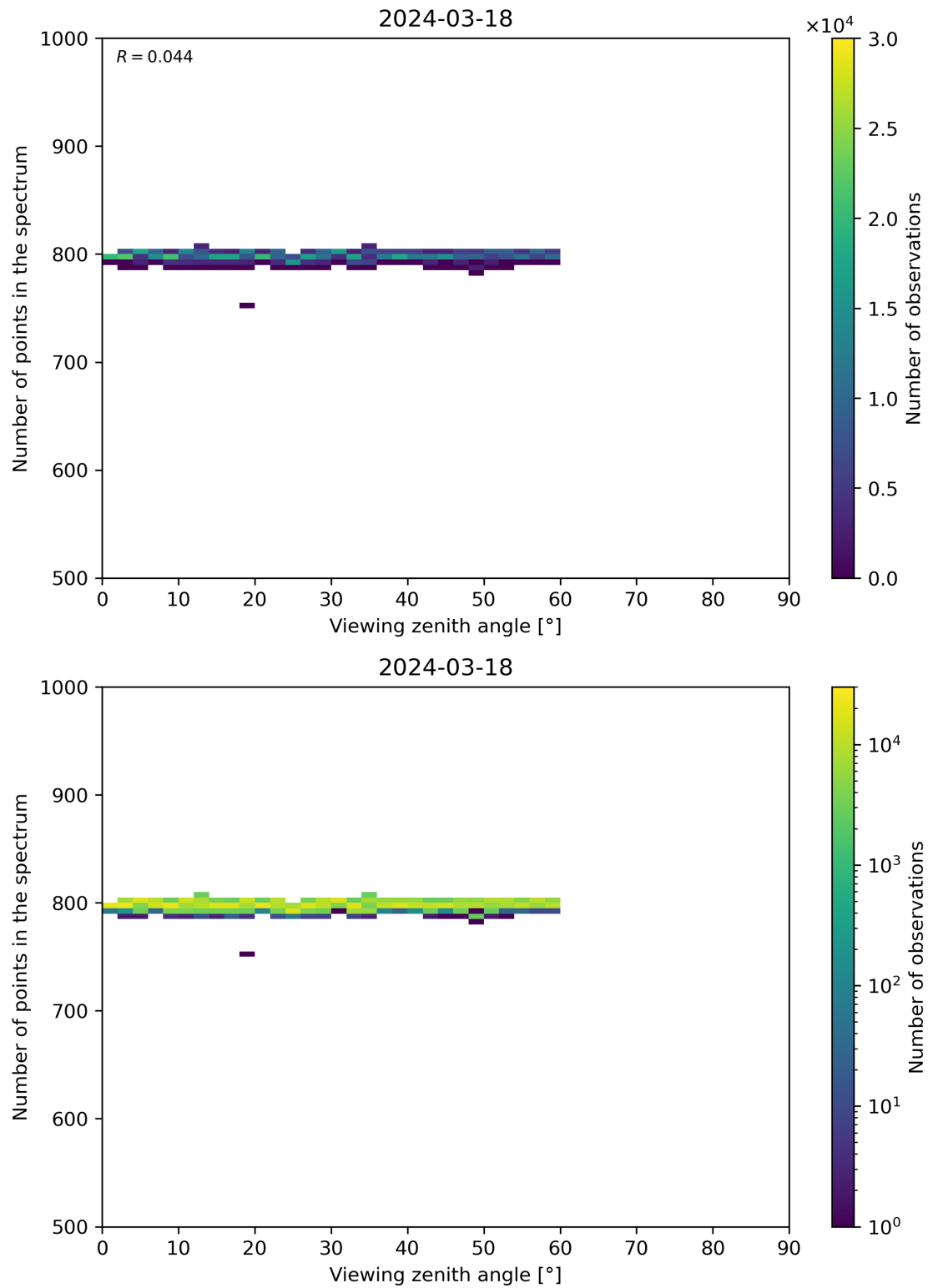
Figure 114: Scatter density plot of “Viewing zenith angle” against “Number of points in the spectrum” for 2024-03-17 to 2024-03-19.
