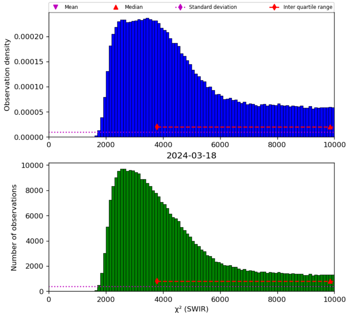
Figure 28: Histogram of “ \chi^2 (SWIR)” for 2024-03-17 to 2024-03-19
