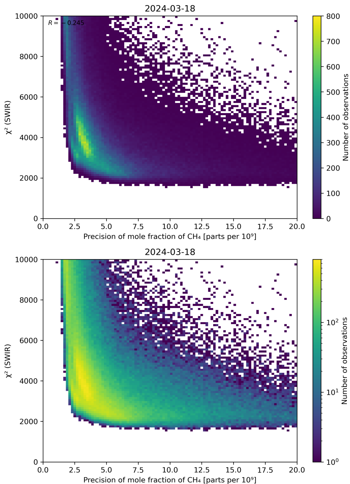
Figure 79: Scatter density plot of “Precision of mole fraction of CH 4 ” against “ \chi^2 (SWIR)” for 2024-03-17 to 2024-03-19.
