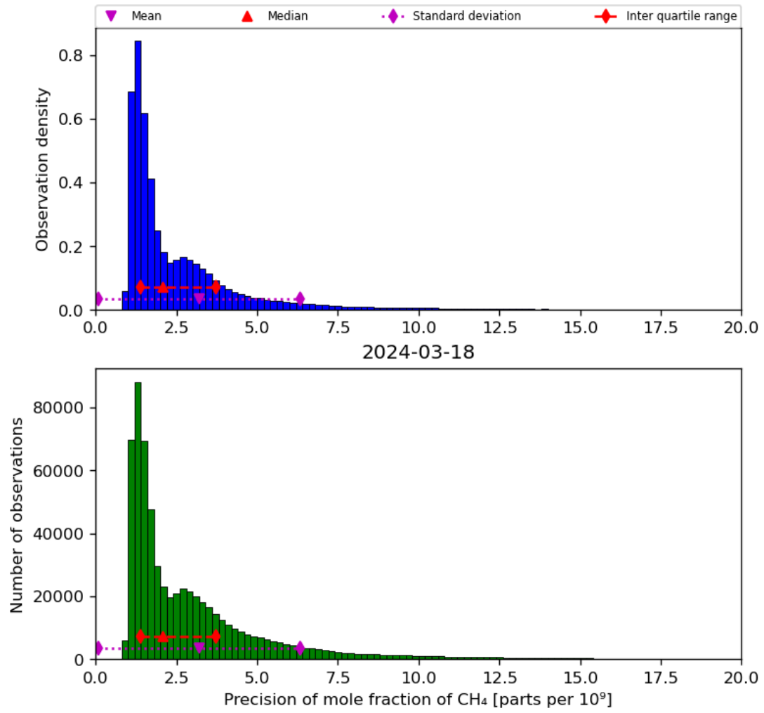
Figure 24: Histogram of “Precision of mole fraction of CH 4 ” for 2024-03-17 to 2024-03-19
