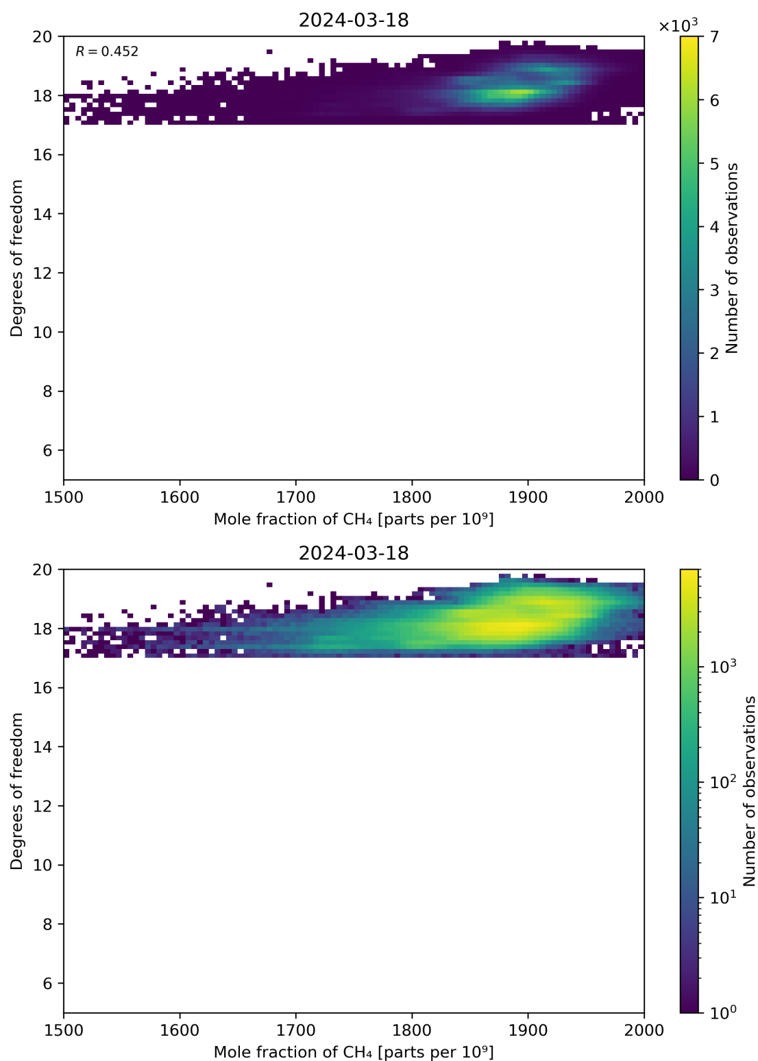
Figure 72: Scatter density plot of “Mole fraction of CH 4 ” against “Degrees of freedom” for 2024-03-17 to 2024-03-19.
