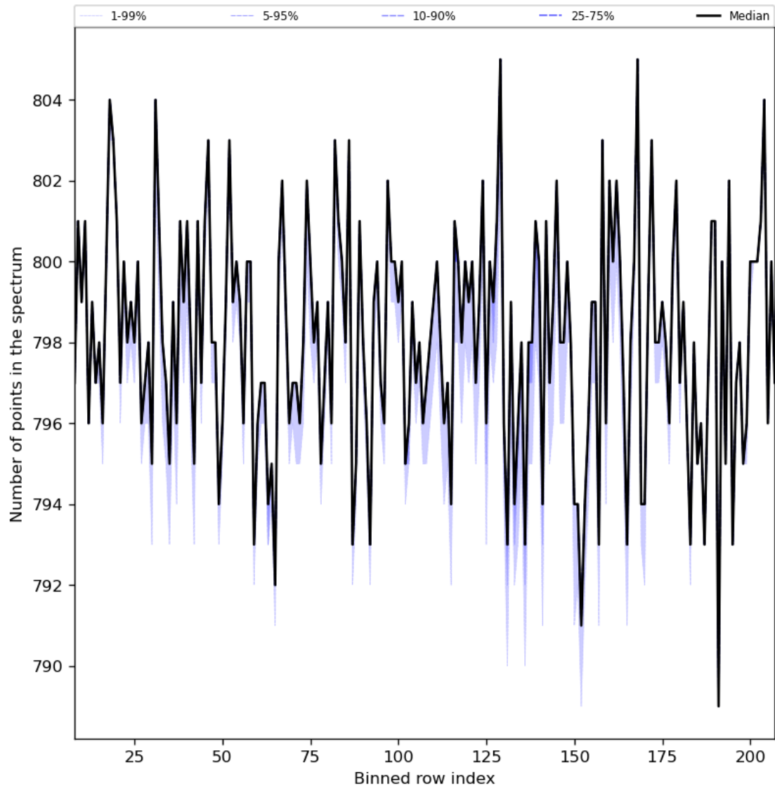
Figure 37: Along track statistics of “Number of points in the spectrum” for 2024-03-17 to 2024-03-19
