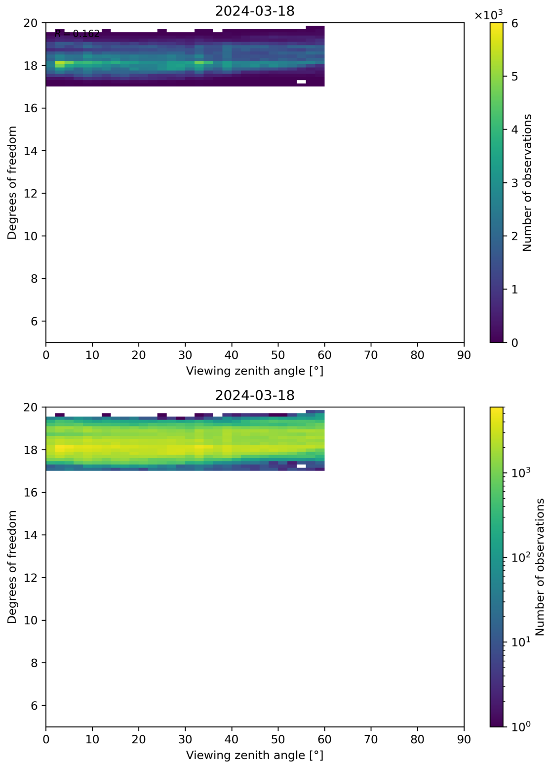
Figure 107: Scatter density plot of “Viewing zenith angle” against “Degrees of freedom” for 2024-03-17 to 2024-03-19.
