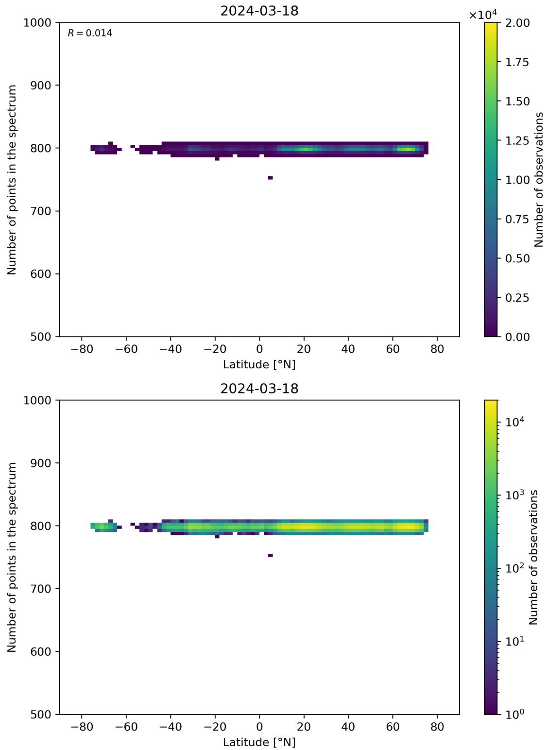
Figure 61: Scatter density plot of “Latitude” against “Number of points in the spectrum” for 2024-03-17 to 2024-03-19.
