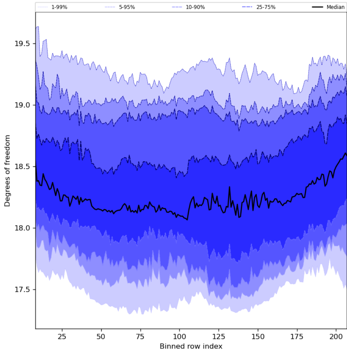
Figure 41: Along track statistics of “Degrees of freedom” for 2024-03-17 to 2024-03-19
