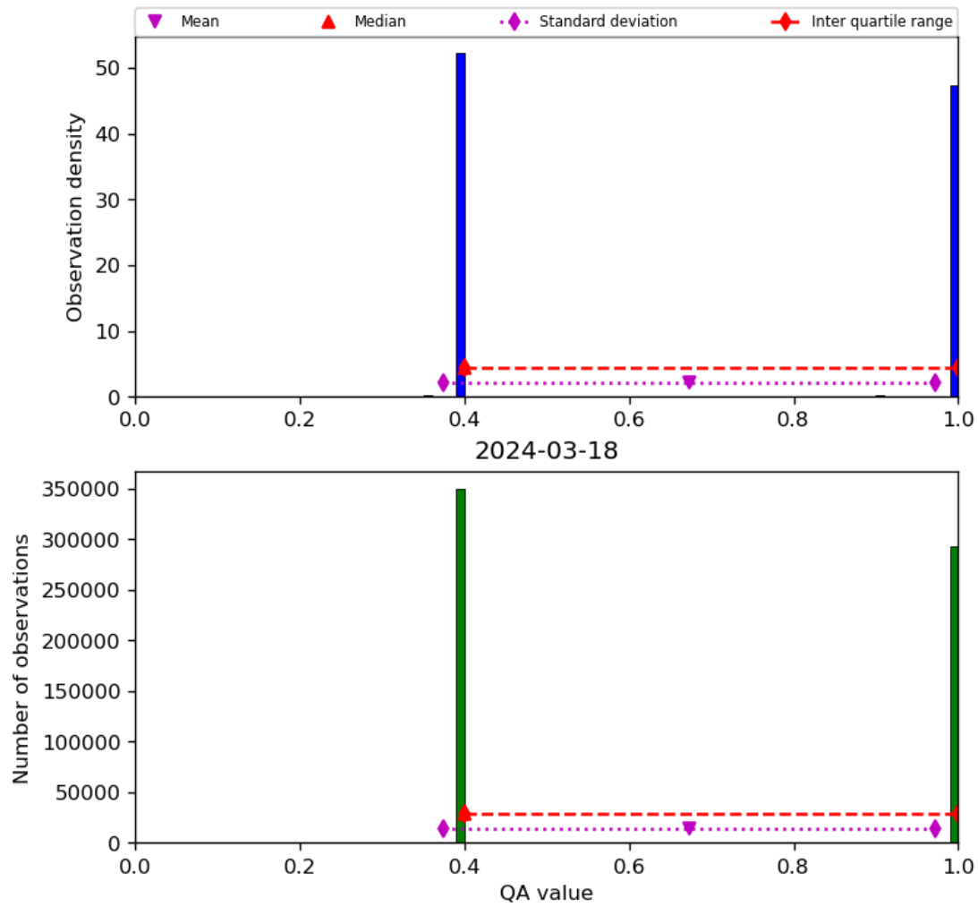
Figure 22: Histogram of “QA value” for 2024-03-17 to 2024-03-19
