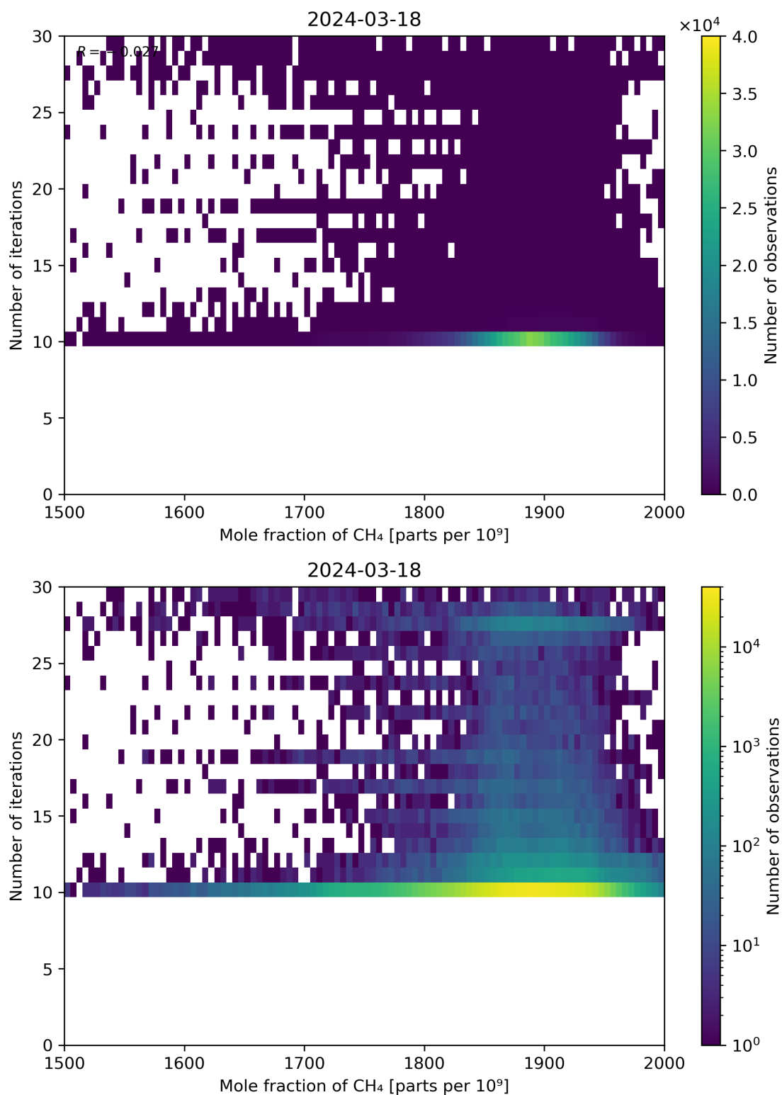
Figure 76: Scatter density plot of “Mole fraction of CH 4 ” against “Number of iterations” for 2024-03-17 to 2024-03-19.
