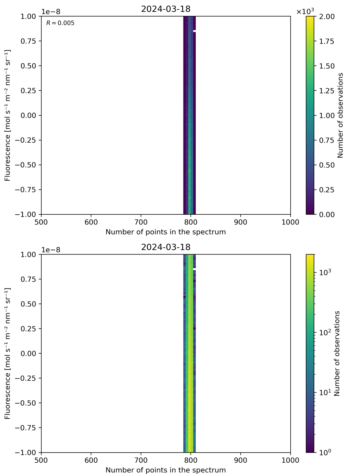
Figure 91: Scatter density plot of “Number of points in the spectrum” against “Fluorescence” for 2024-03-17 to 2024-03-19.
