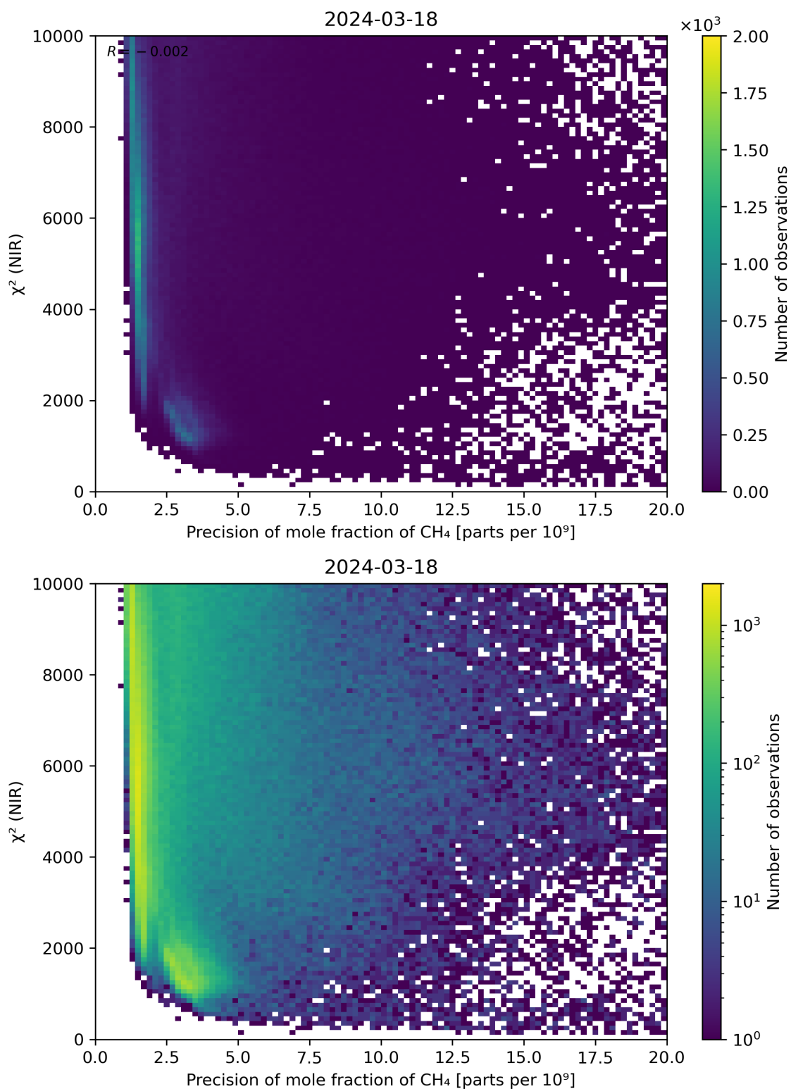
Figure 78: Scatter density plot of “Precision of mole fraction of CH 4 ” against “ \chi^2 (NIR)” for 2024-03-17 to 2024-03-19.
