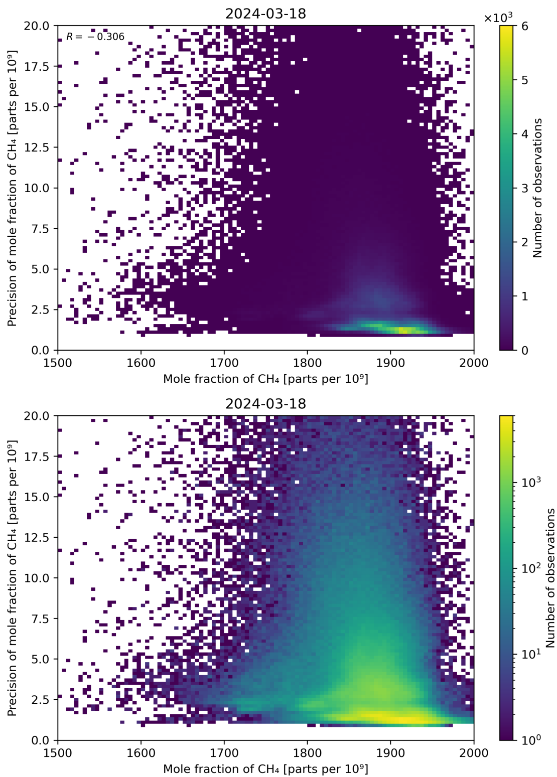
Figure 75: Scatter density plot of “Mole fraction of CH 4 ” against “Precision of mole fraction of CH 4 ” for 2024-03-17 to 2024-03-19.
