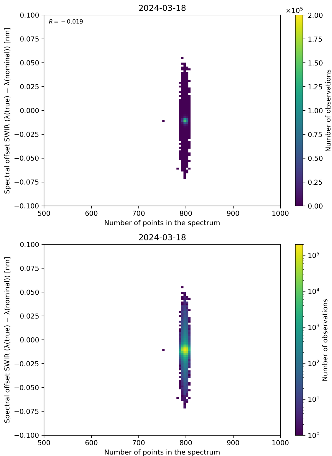
Figure 93: Scatter density plot of “Number of points in the spectrum” against “Spectral offset SWIR ( \lambda(\text{true}) - \lambda(\text{nominal}) )” for 2024-03-17 to 2024-03-19.
