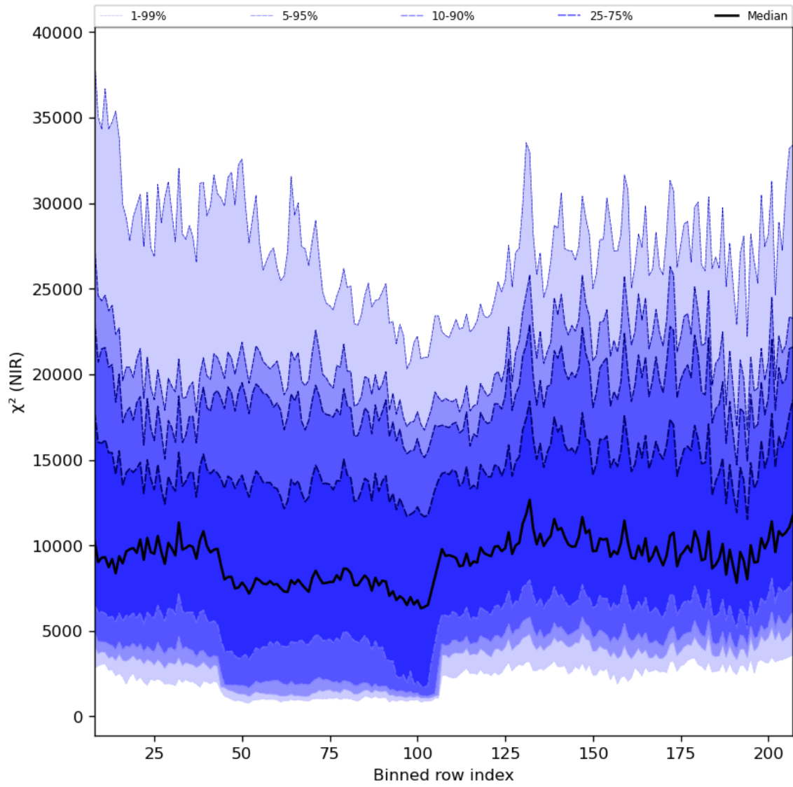
Figure 40: Along track statistics of " \chi^2 (NIR)" for 2024-03-18 to 2024-03-20
