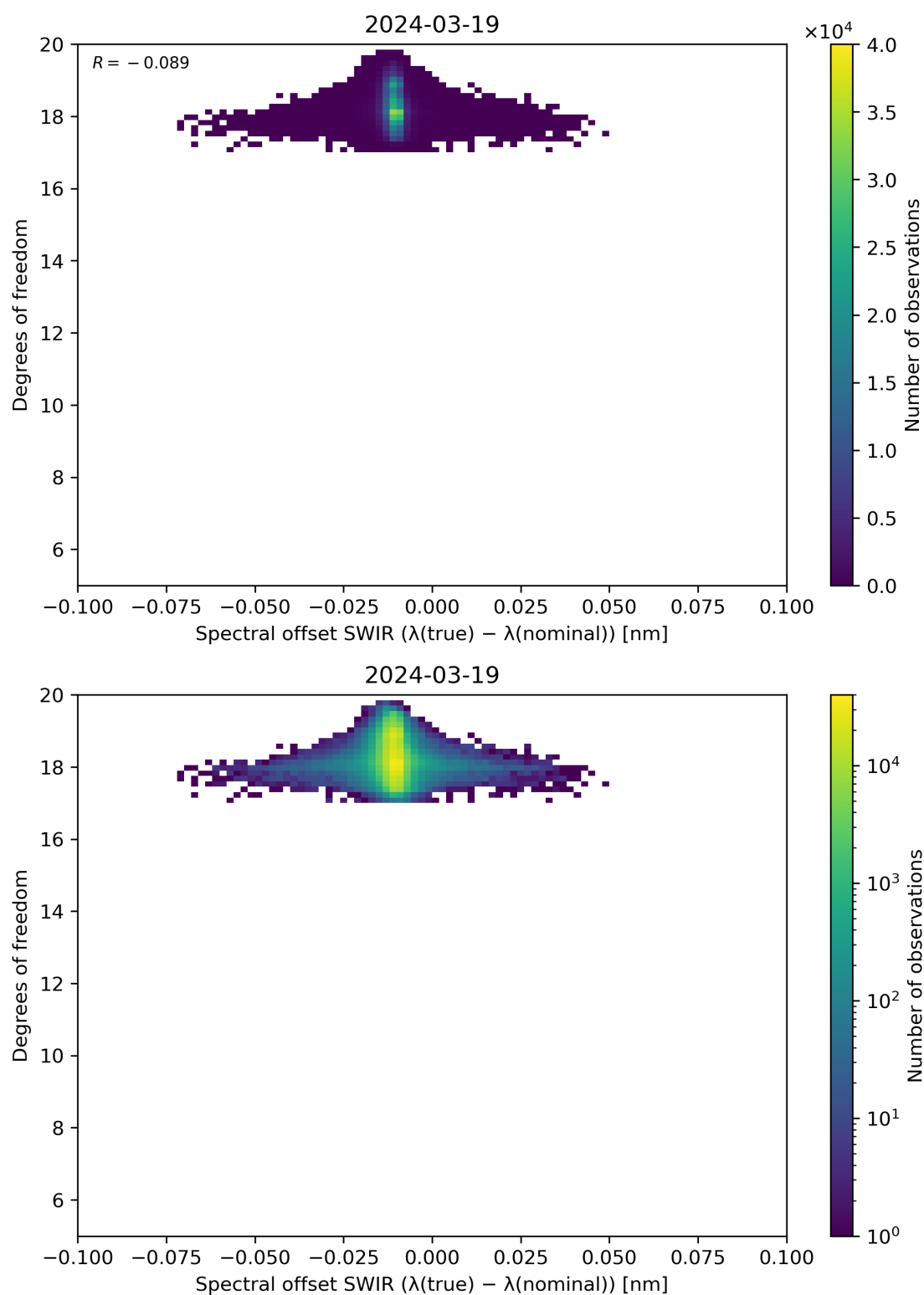
Figure 119: Scatter density plot of “Spectral offset SWIR ( \lambda(\text{true}) - \lambda(\text{nominal}) )” against “Degrees of freedom” for 2024-03-18 to 2024-03-20.
