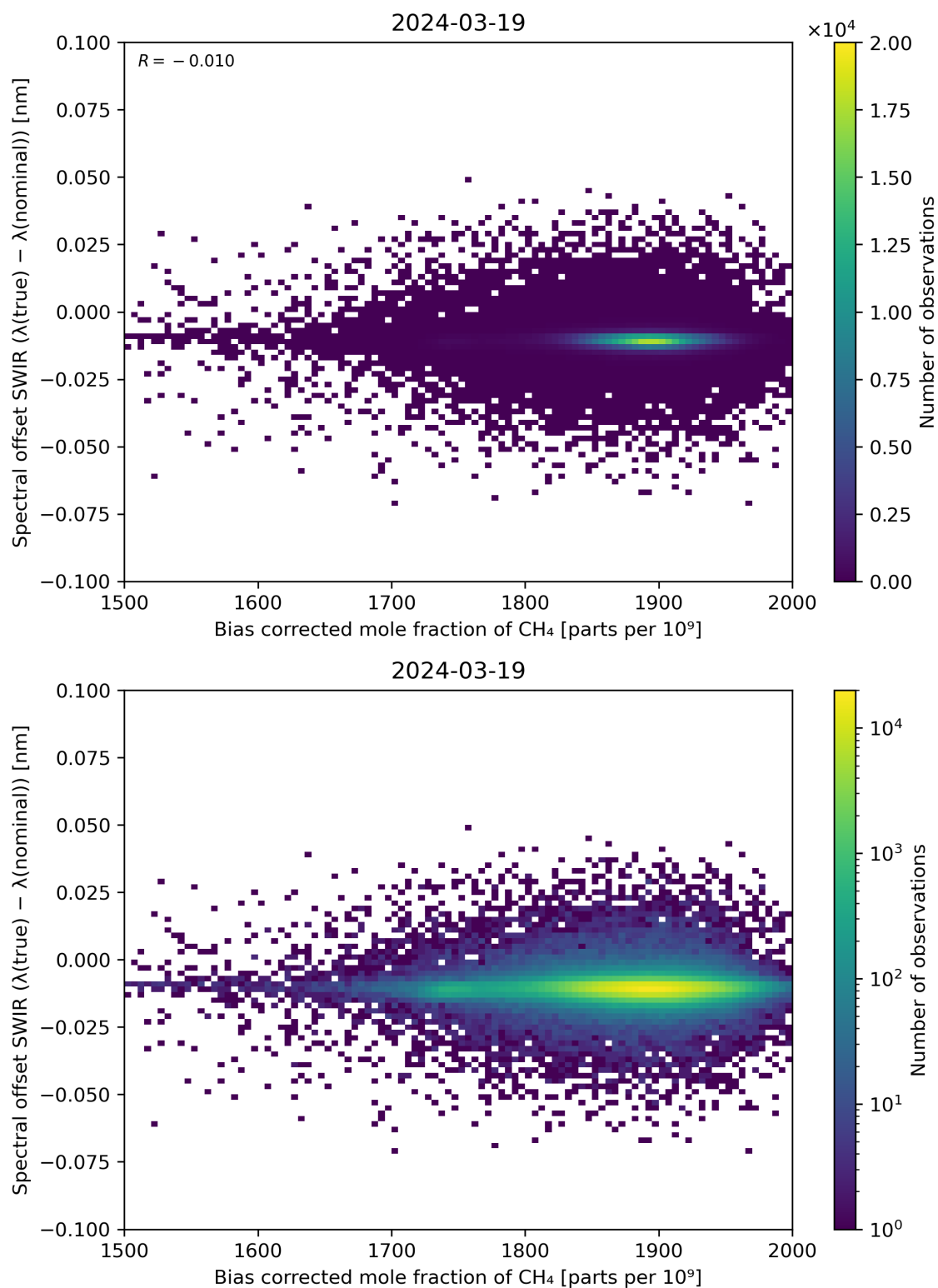
Figure 69: Scatter density plot of “Bias corrected mole fraction of \text{CH}_4 ” against “Spectral offset SWIR ( \lambda(\text{true}) - \lambda(\text{nominal}) )” for 2024-03-18 to 2024-03-20.
