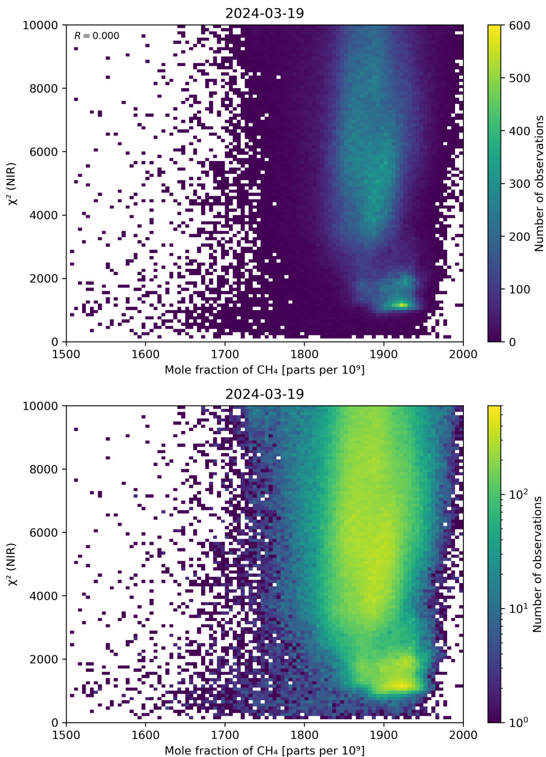
Figure 70: Scatter density plot of “Mole fraction of CH 4 ” against “ \chi^2 (NIR)” for 2024-03-18 to 2024-03-20.
