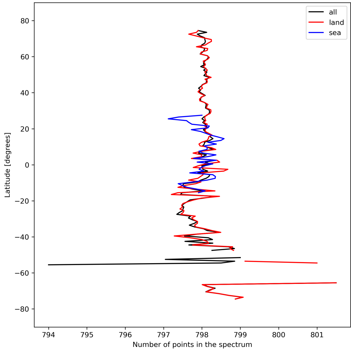
Figure 15: Zonal average of “Number of points in the spectrum” for 2024-03-18 to 2024-03-20.
