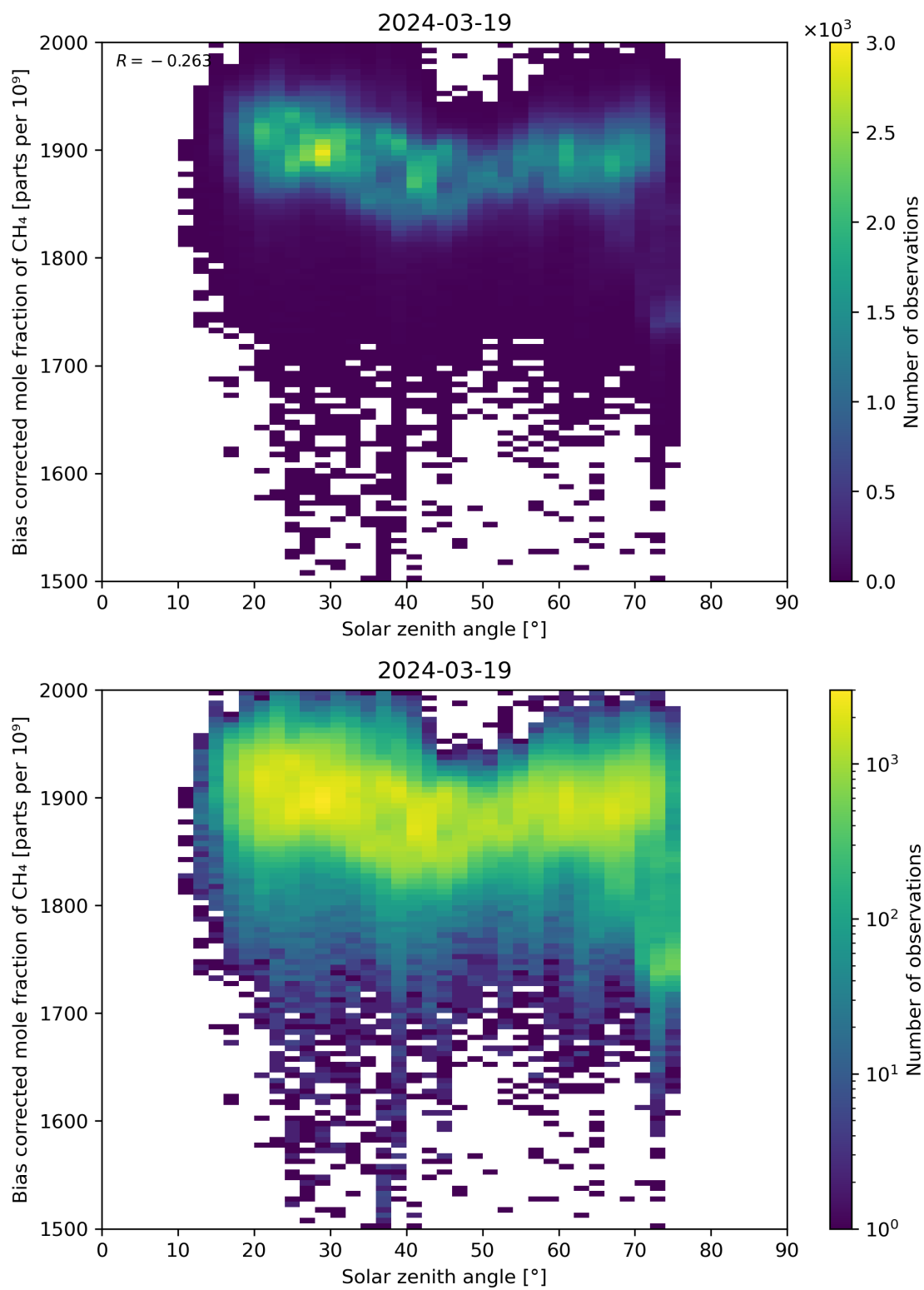
Figure 100: Scatter density plot of “Solar zenith angle” against “Bias corrected mole fraction of CH 4 ” for 2024-03-18 to 2024-03-20.
