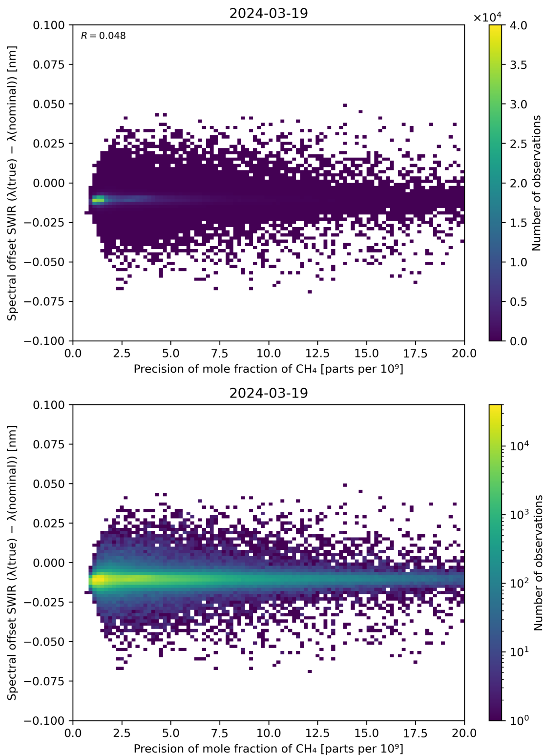
Figure 85: Scatter density plot of “Precision of mole fraction of \text{CH}_4 ” against “Spectral offset SWIR ( \lambda(\text{true}) - \lambda(\text{nominal}) )” for 2024-03-18 to 2024-03-20.
