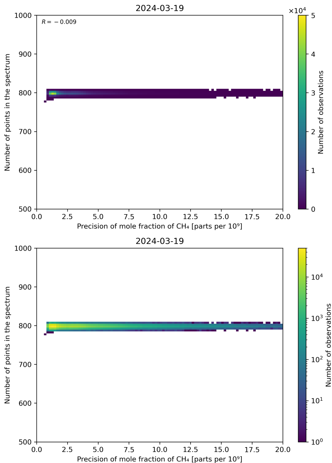
Figure 84: Scatter density plot of “Precision of mole fraction of CH 4 ” against “Number of points in the spectrum” for 2024-03-18 to 2024-03-20.
