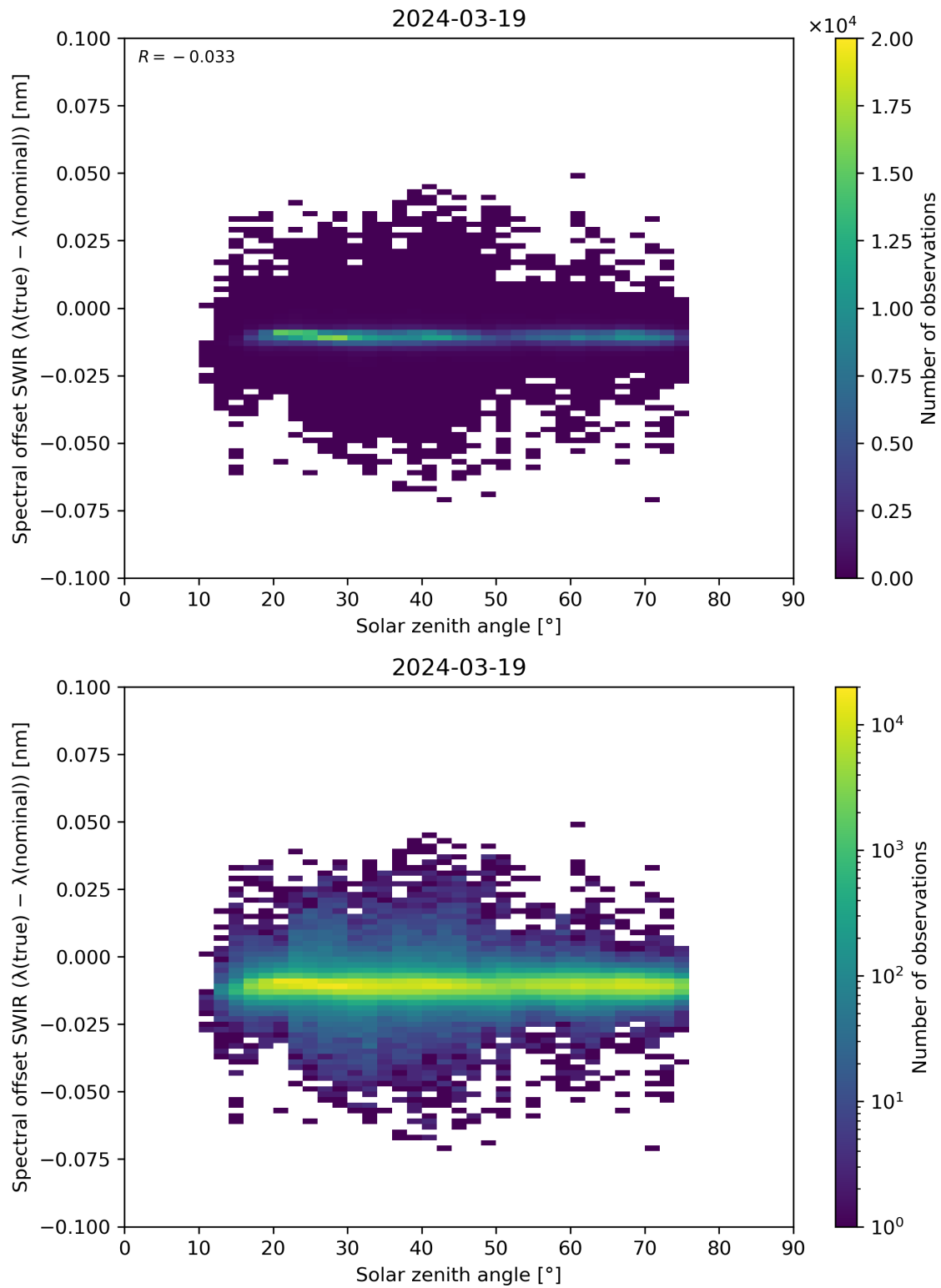
Figure 104: Scatter density plot of “Solar zenith angle” against “Spectral offset SWIR ( \lambda(\text{true}) - \lambda(\text{nominal}) )” for 2024-03-18 to 2024-03-20.
