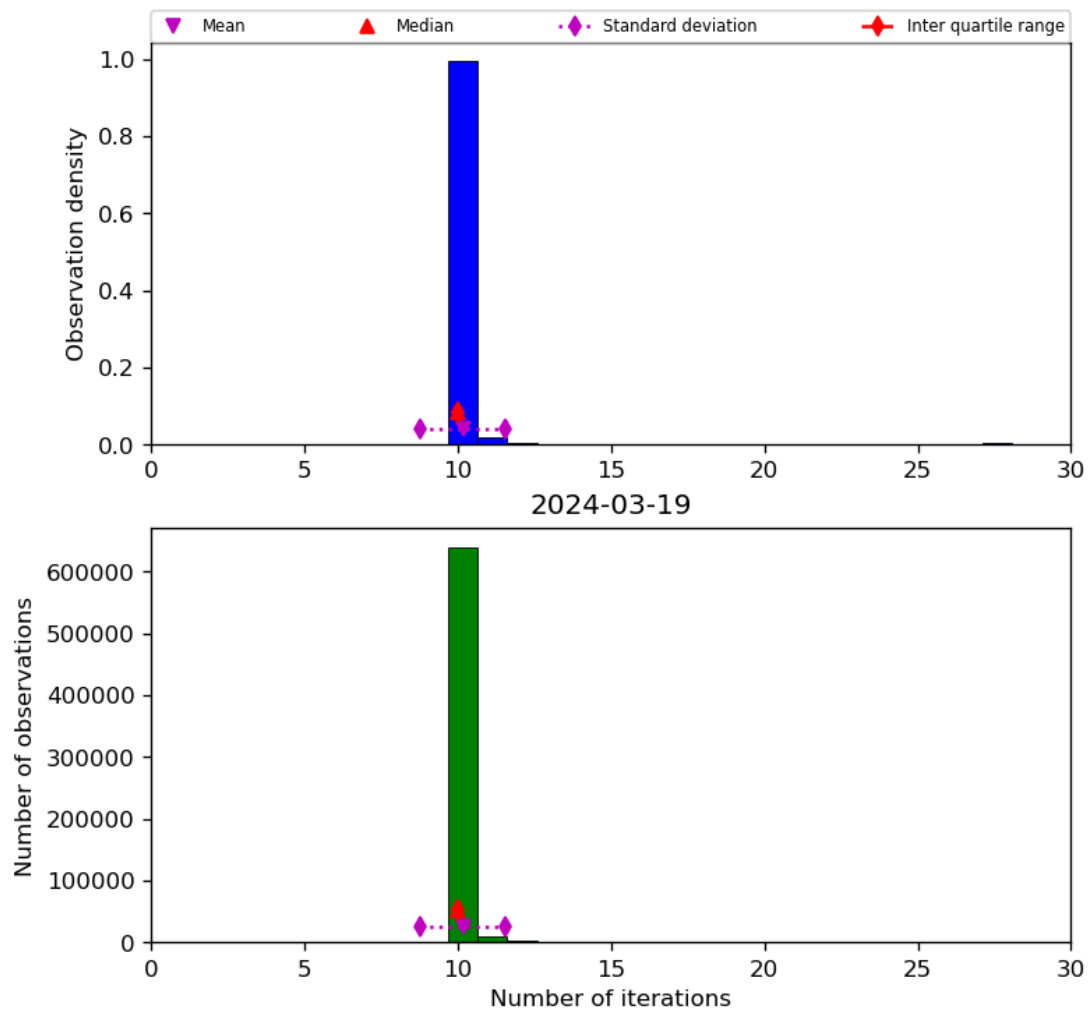
Figure 31: Histogram of “Number of iterations” for 2024-03-18 to 2024-03-20
