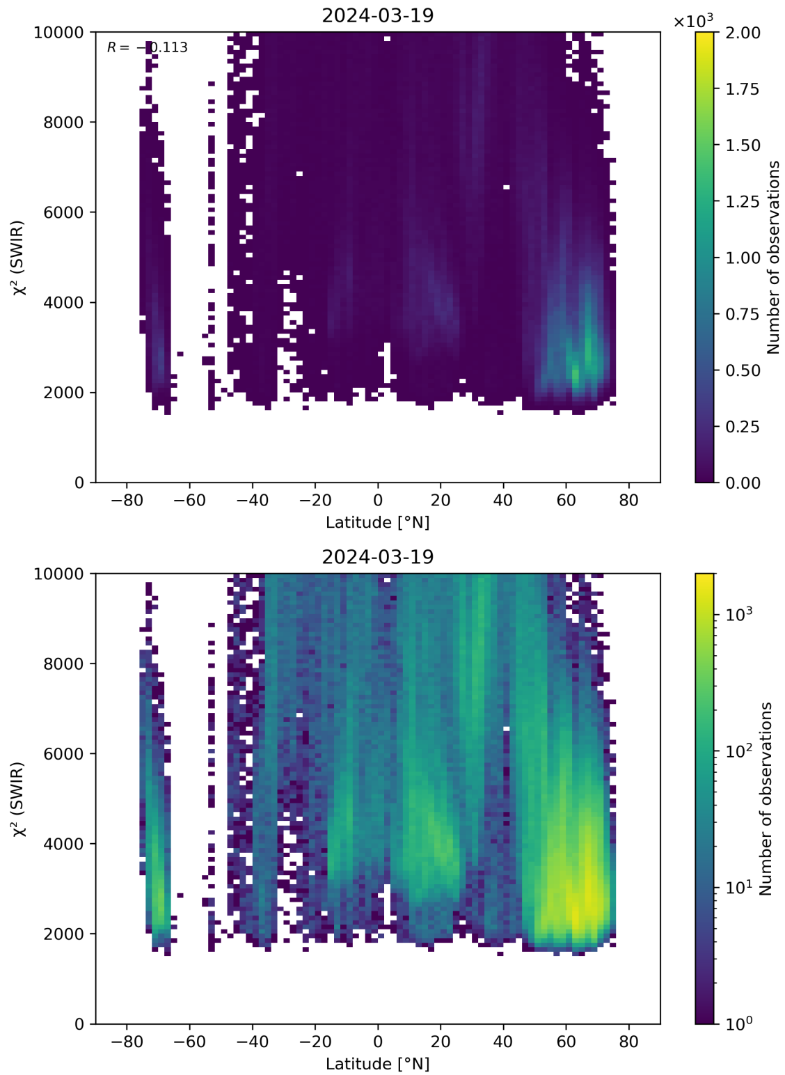
Figure 54: Scatter density plot of “Latitude” against “ \chi^2 (SWIR)” for 2024-03-18 to 2024-03-20.
