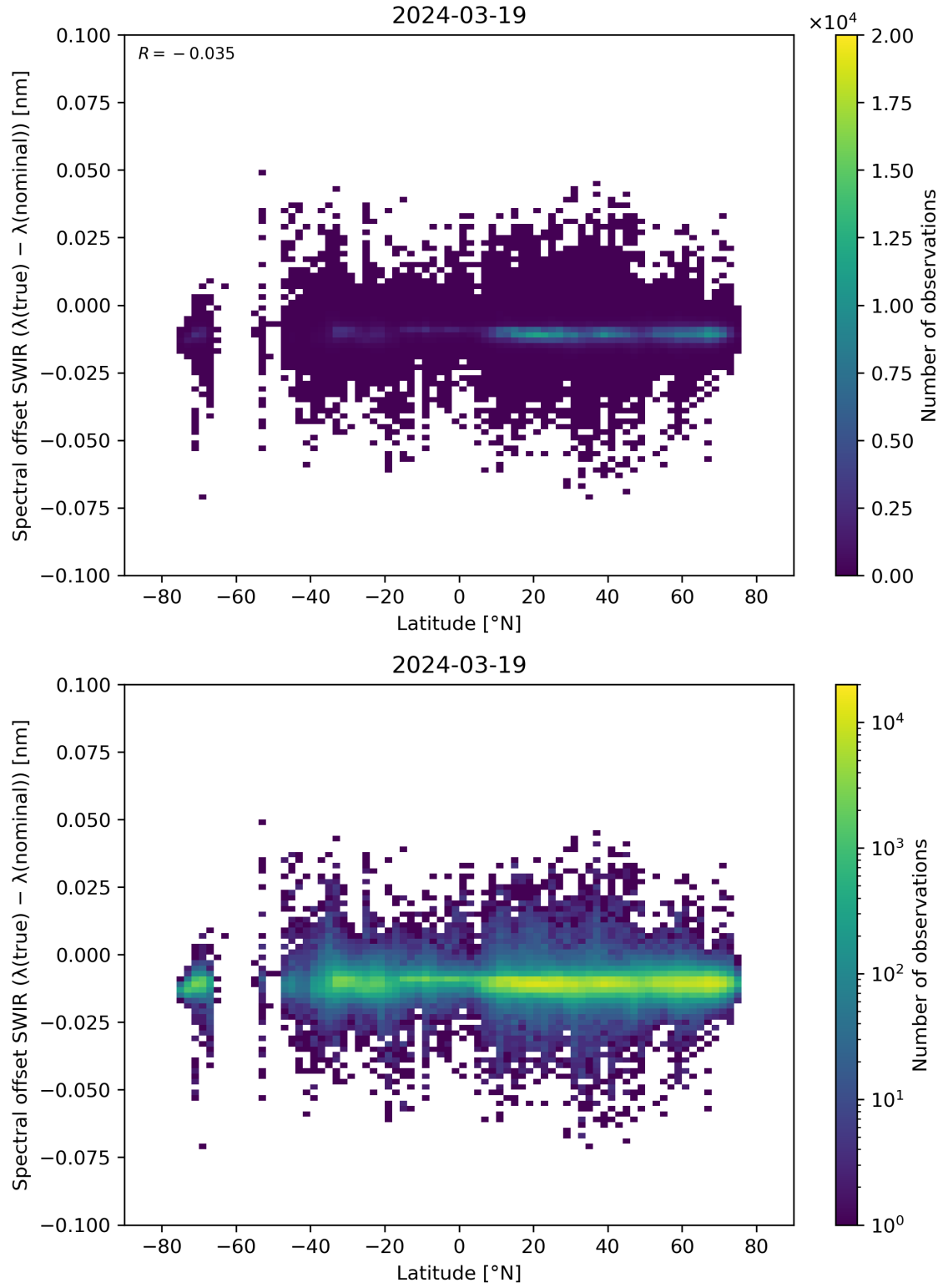
Figure 62: Scatter density plot of “Latitude” against “Spectral offset SWIR ( \lambda(\text{true}) - \lambda(\text{nominal}) )” for 2024-03-18 to 2024-03-20.
