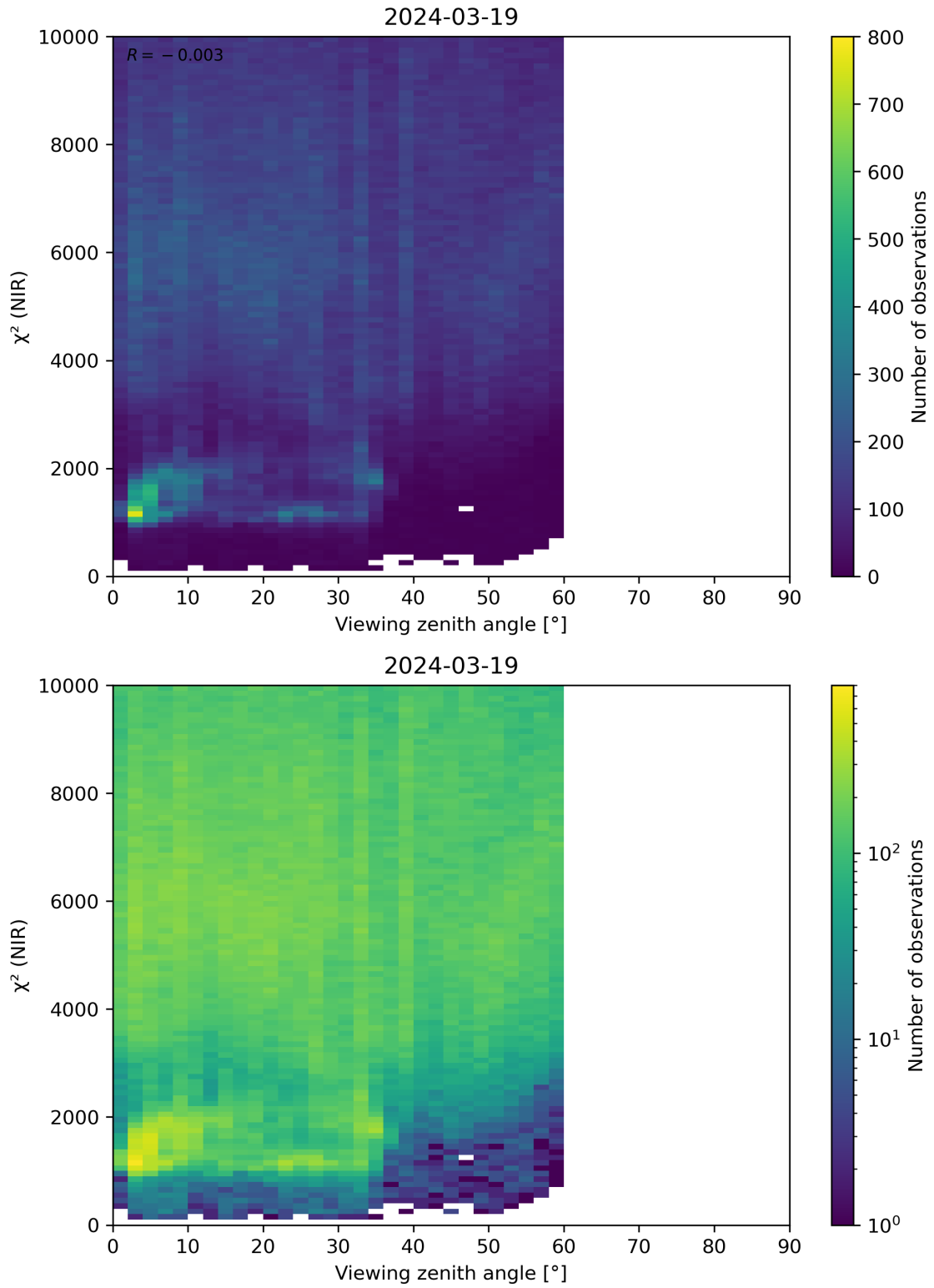
Figure 105: Scatter density plot of “Viewing zenith angle” against “ \chi^2 (NIR)” for 2024-03-18 to 2024-03-20.
