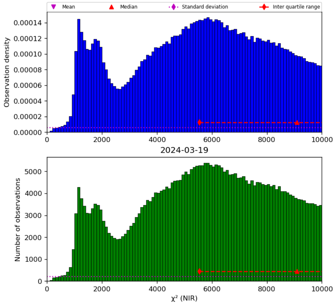
Figure 29: Histogram of “ \chi^2 (NIR)” for 2024-03-18 to 2024-03-20
