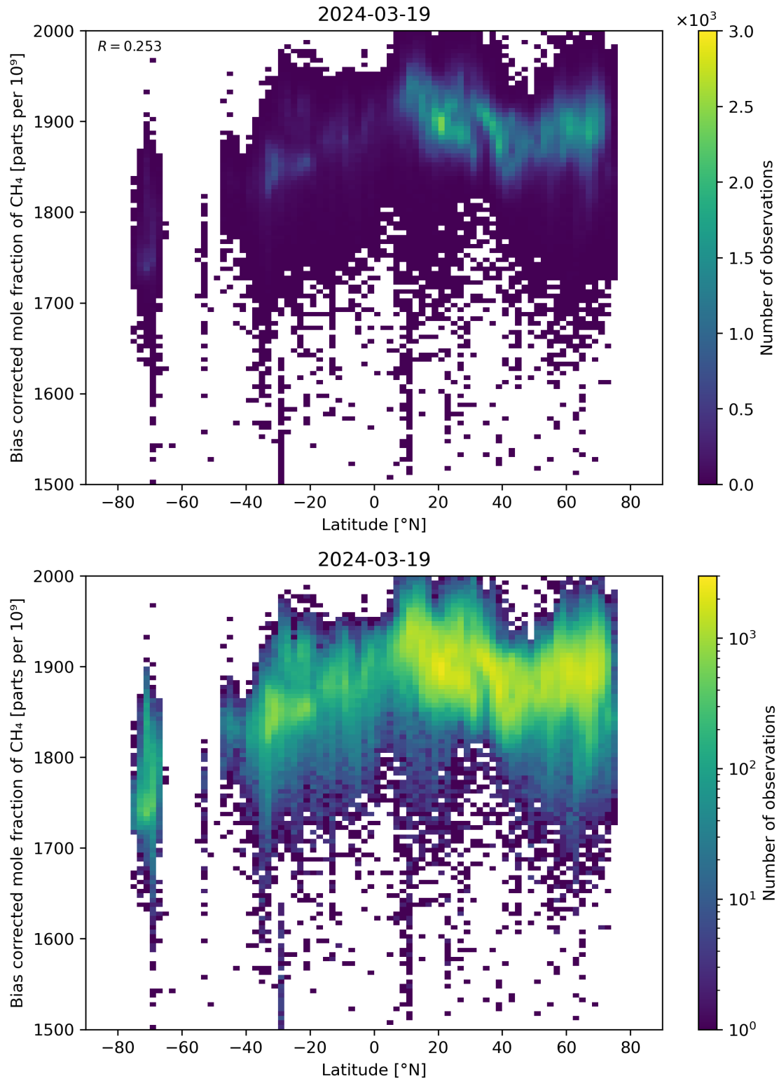
Figure 58: Scatter density plot of “Latitude” against “Bias corrected mole fraction of CH 4 ” for 2024-03-18 to 2024-03-20.
