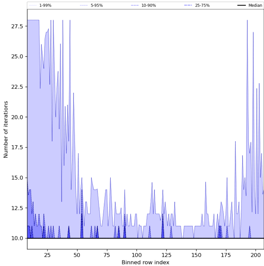
Figure 42: Along track statistics of “Number of iterations” for 2024-03-18 to 2024-03-20
