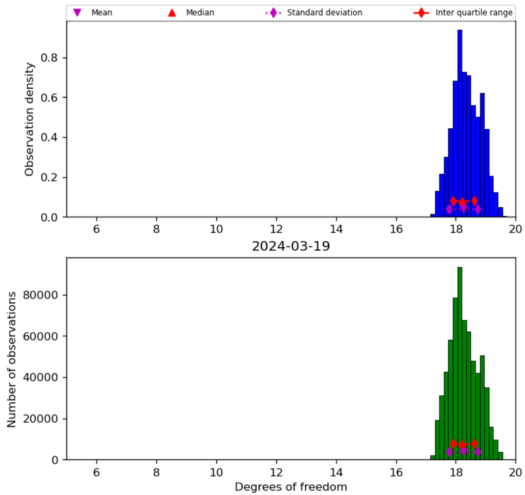
Figure 30: Histogram of “Degrees of freedom” for 2024-03-18 to 2024-03-20
