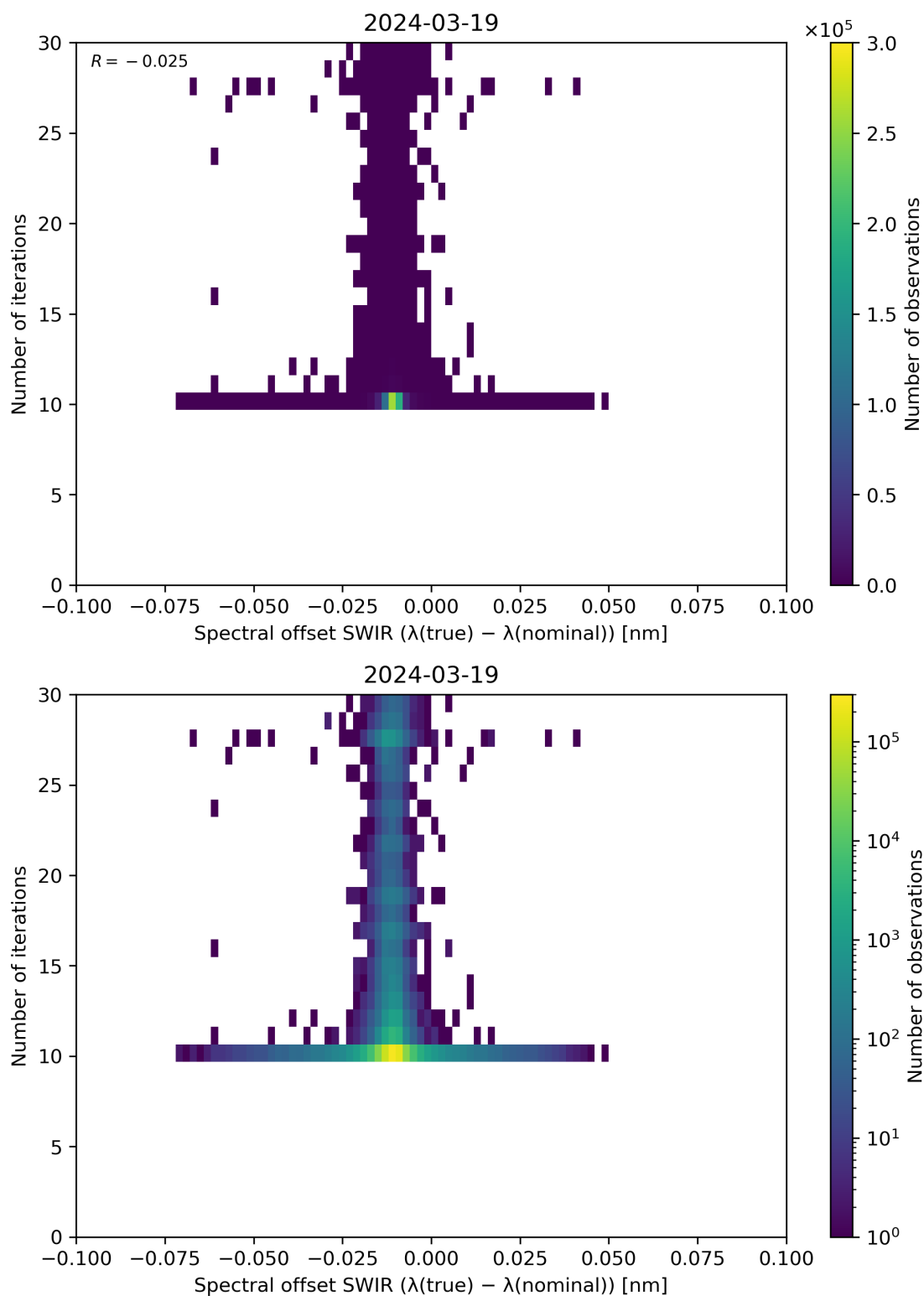
Figure 121: Scatter density plot of “Spectral offset SWIR ( \lambda(\text{true}) - \lambda(\text{nominal}) )” against “Number of iterations” for 2024-03-18 to 2024-03-20.
