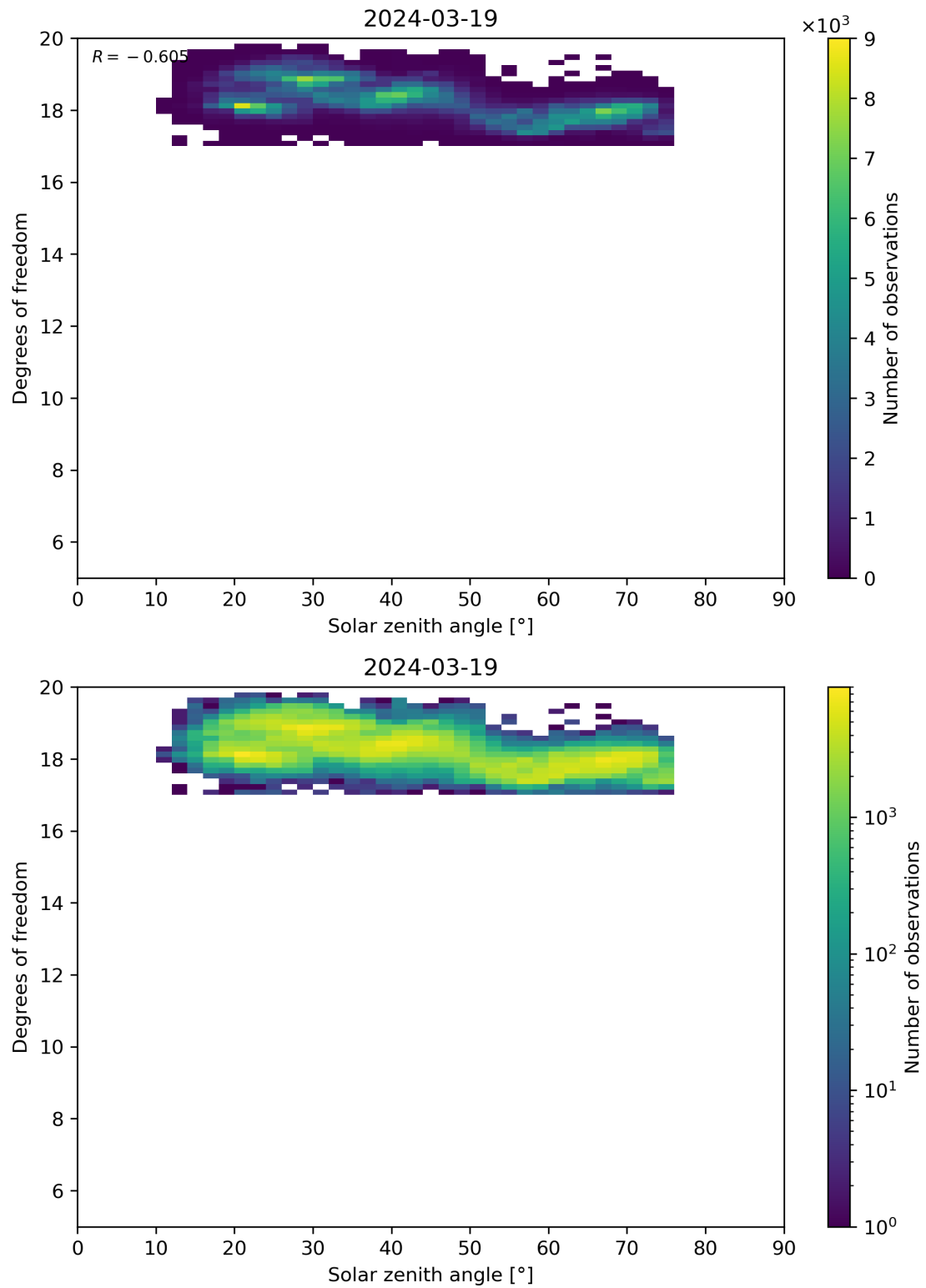
Figure 96: Scatter density plot of “Solar zenith angle” against “Degrees of freedom” for 2024-03-18 to 2024-03-20.
