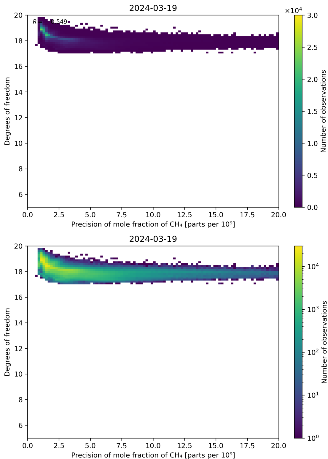
Figure 80: Scatter density plot of “Precision of mole fraction of CH 4 ” against “Degrees of freedom” for 2024-03-18 to 2024-03-20.
