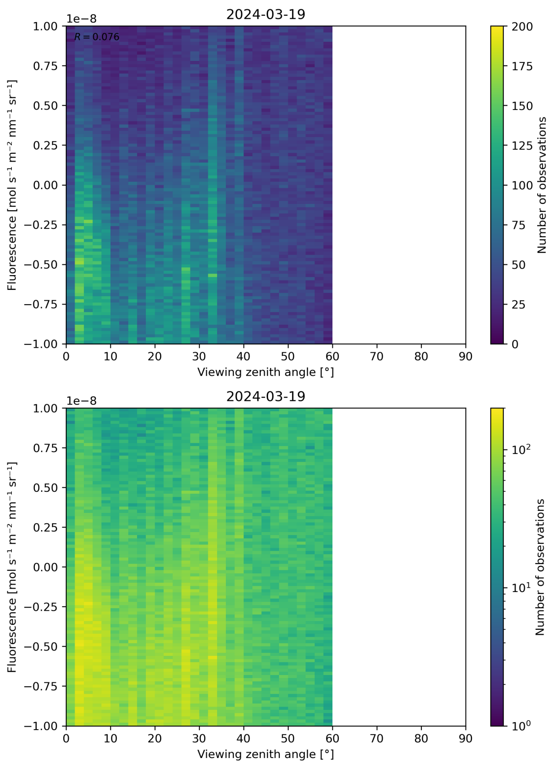
Figure 108: Scatter density plot of “Viewing zenith angle” against “Fluorescence” for 2024-03-18 to 2024-03-20.
