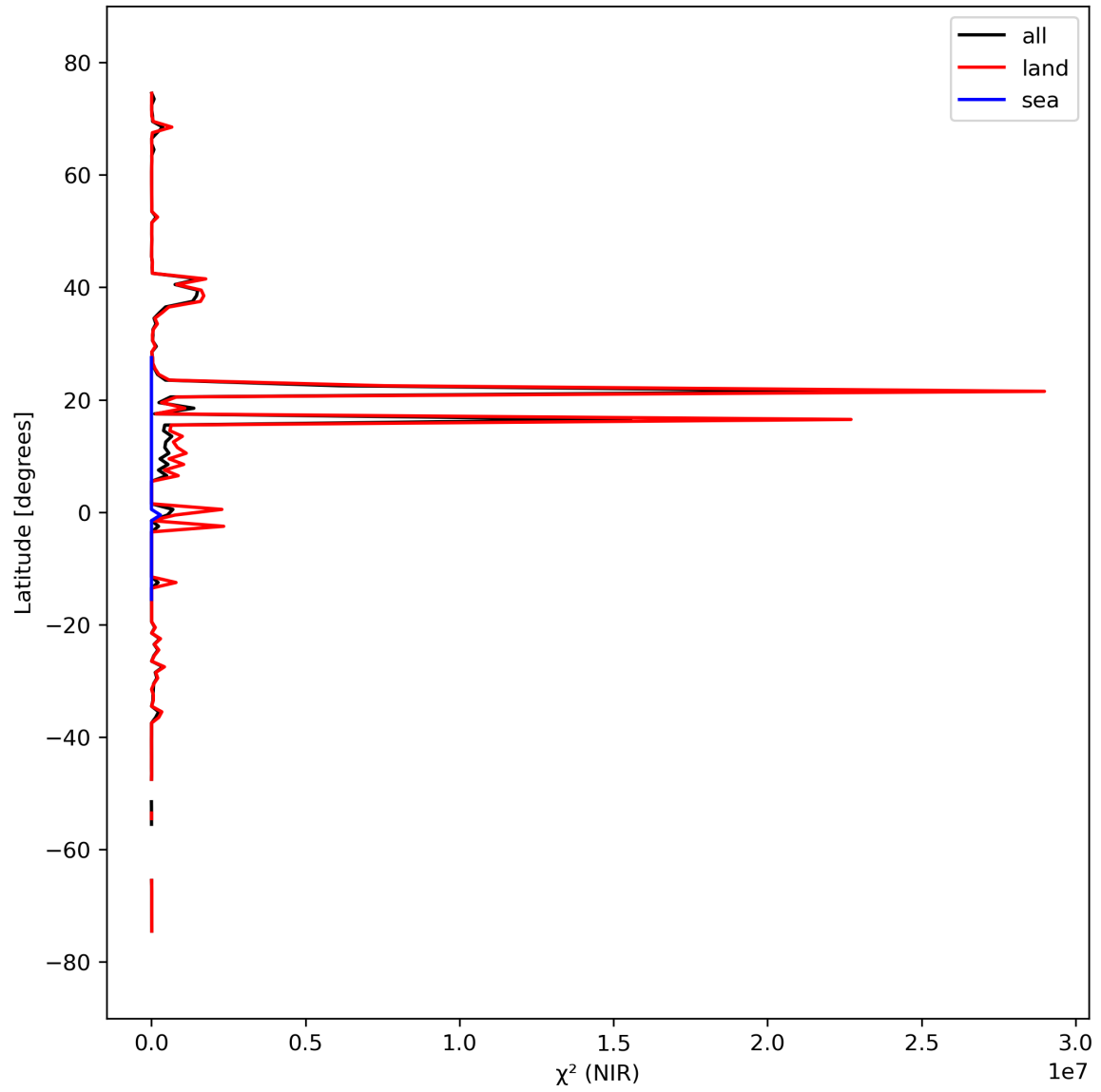
Figure 18: Zonal average of “ \chi^2 (NIR)” for 2024-03-18 to 2024-03-20.
