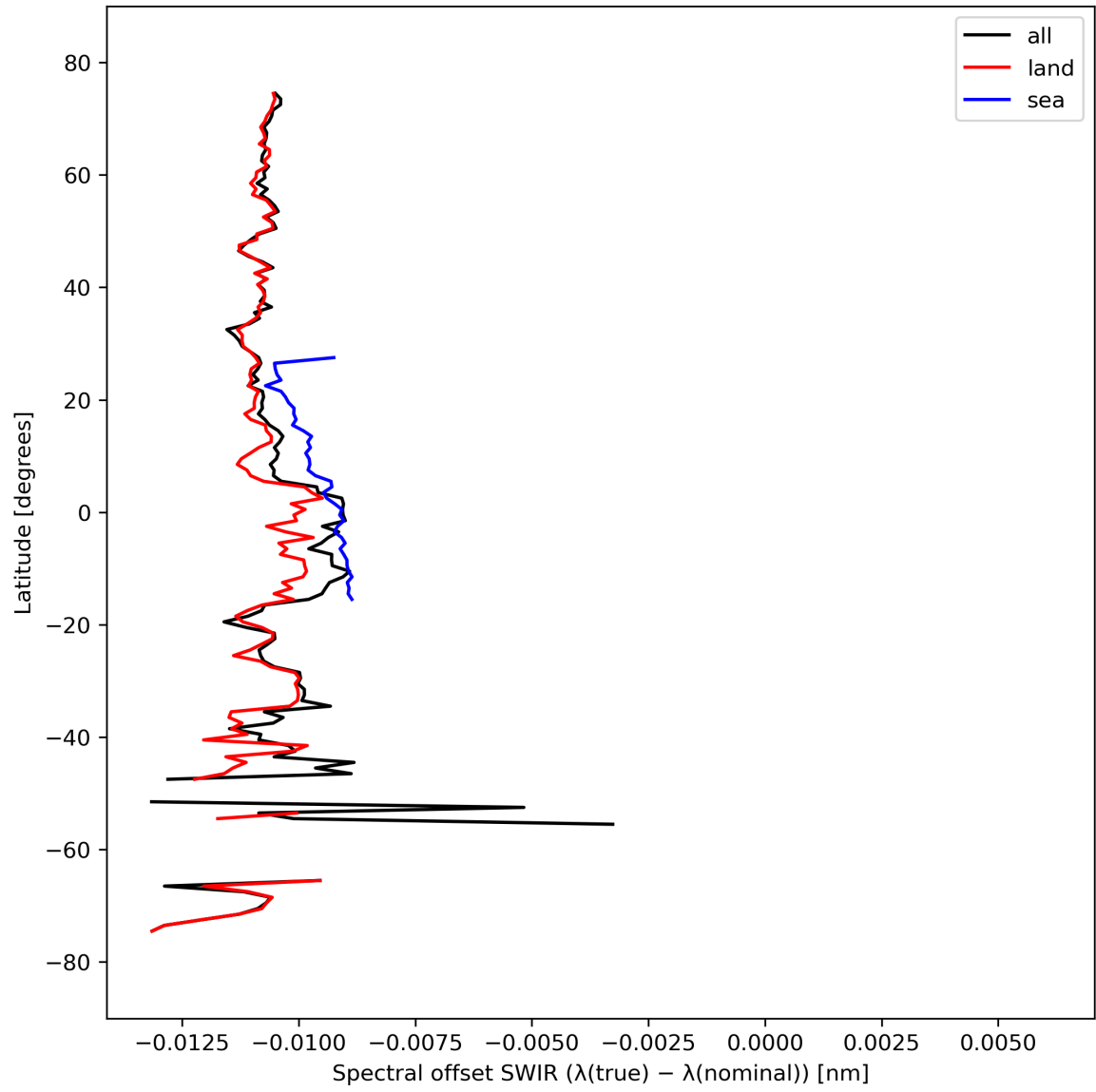
Figure 16: Zonal average of “Spectral offset SWIR ( \lambda(\text{true}) - \lambda(\text{nominal}) )” for 2024-03-18 to 2024-03-20.
