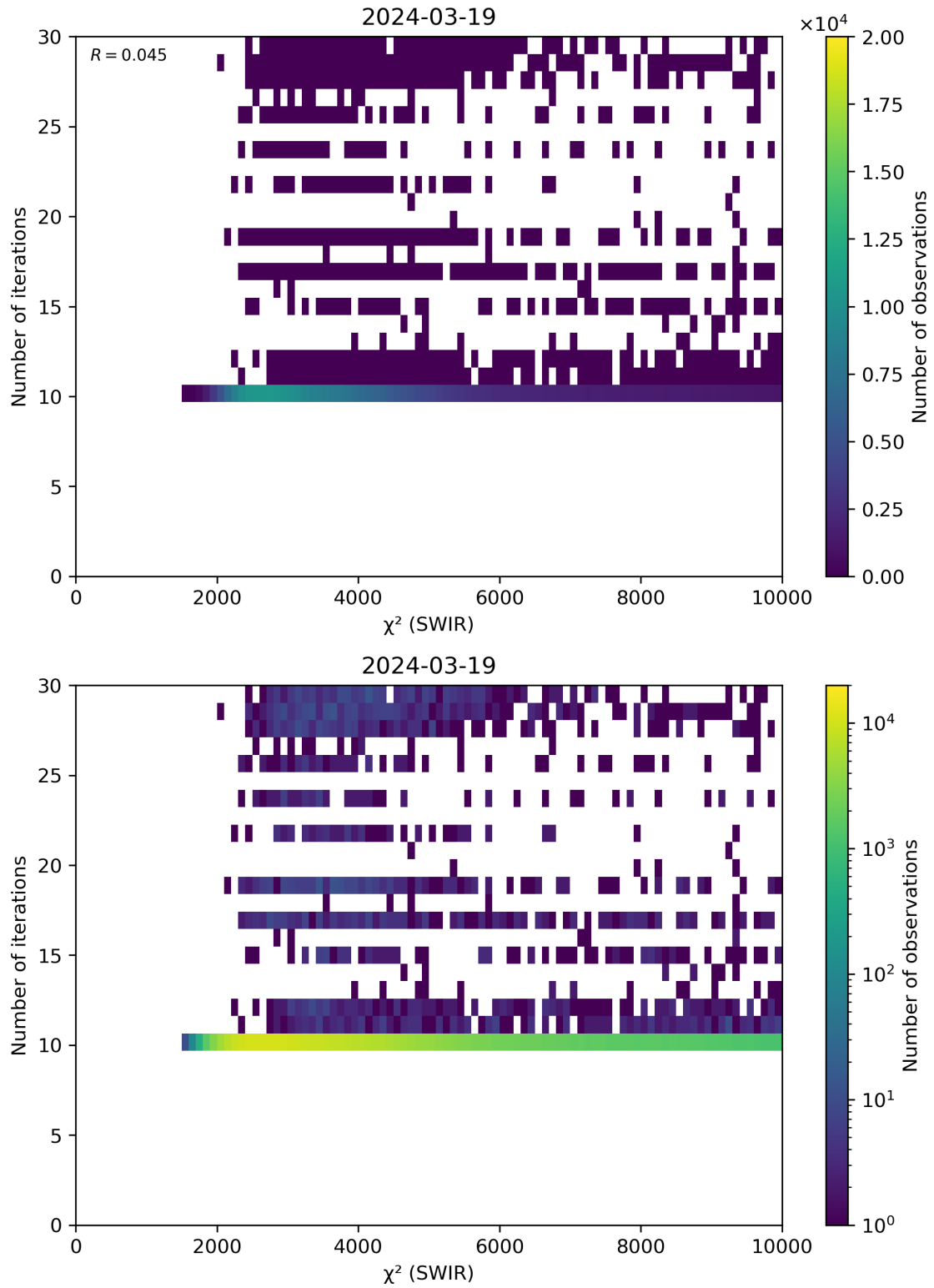
Figure 50: Scatter density plot of “ \chi^2 (SWIR)” against “Number of iterations” for 2024-03-18 to 2024-03-20.
