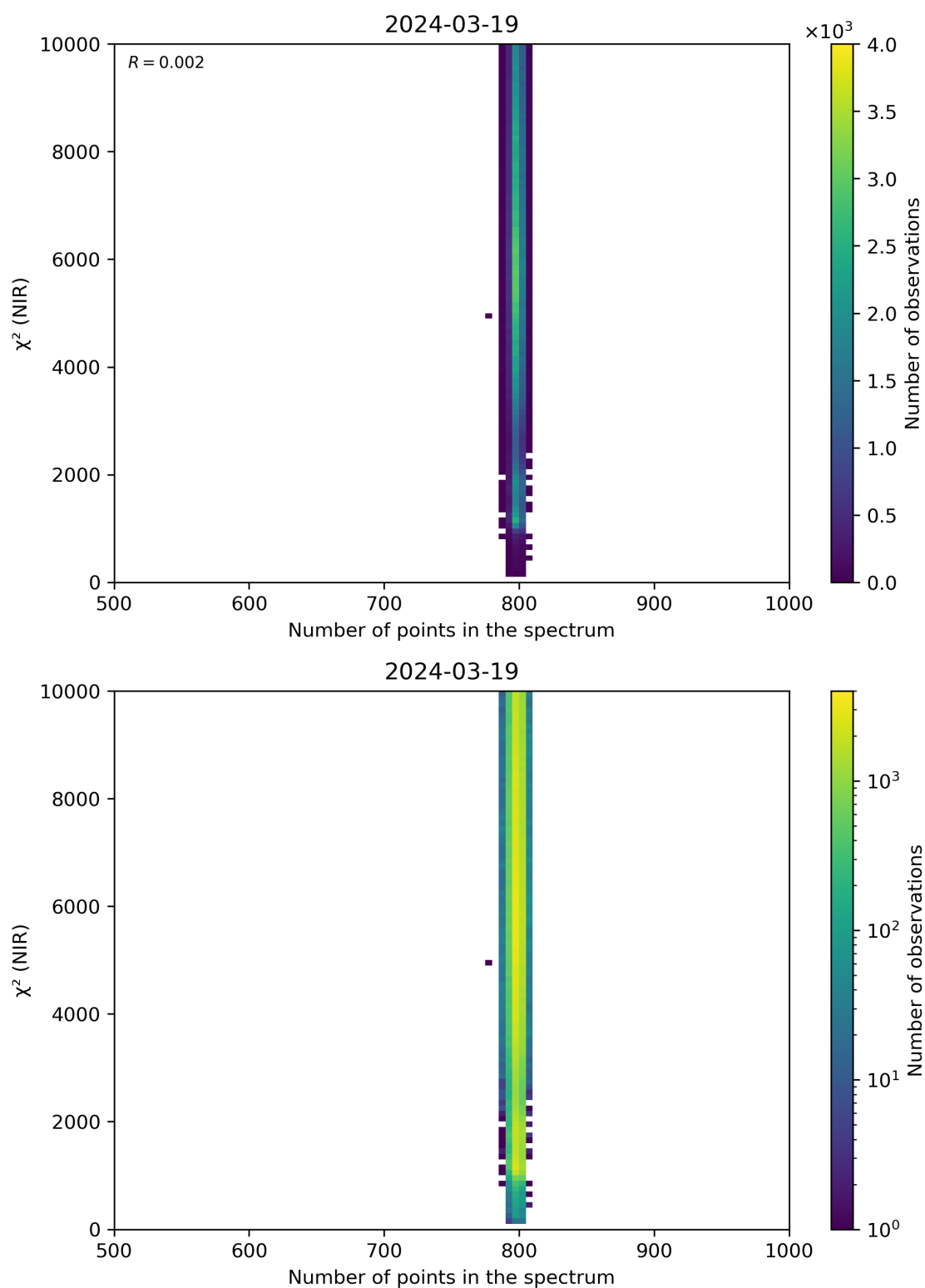
Figure 88: Scatter density plot of “Number of points in the spectrum” against “ \chi^2 (NIR)” for 2024-03-18 to 2024-03-20.
