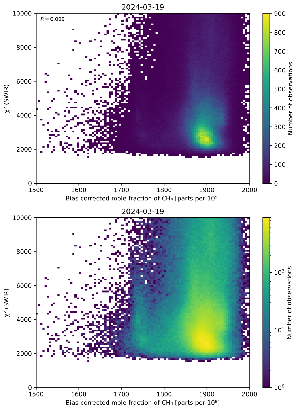
Figure 64: Scatter density plot of “Bias corrected mole fraction of CH 4 ” against “ \chi^2 (SWIR)” for 2024-03-18 to 2024-03-20.
