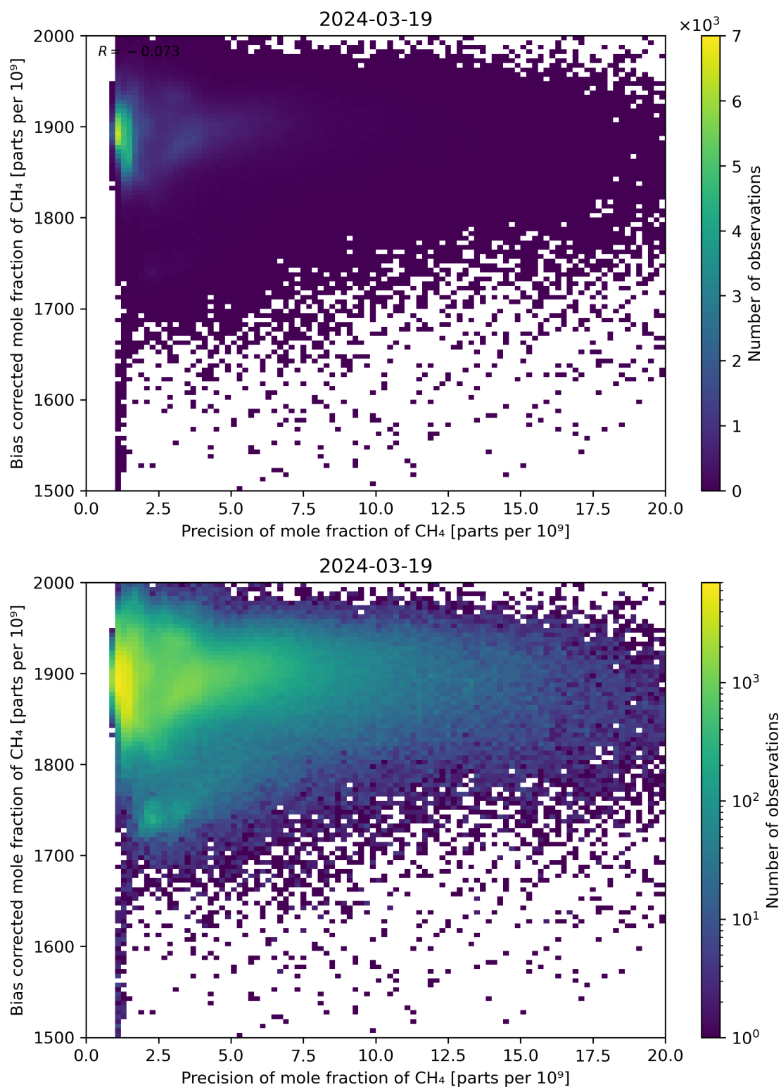
Figure 82: Scatter density plot of “Precision of mole fraction of CH 4 ” against “Bias corrected mole fraction of CH 4 ” for 2024-03-18 to 2024-03-20.
