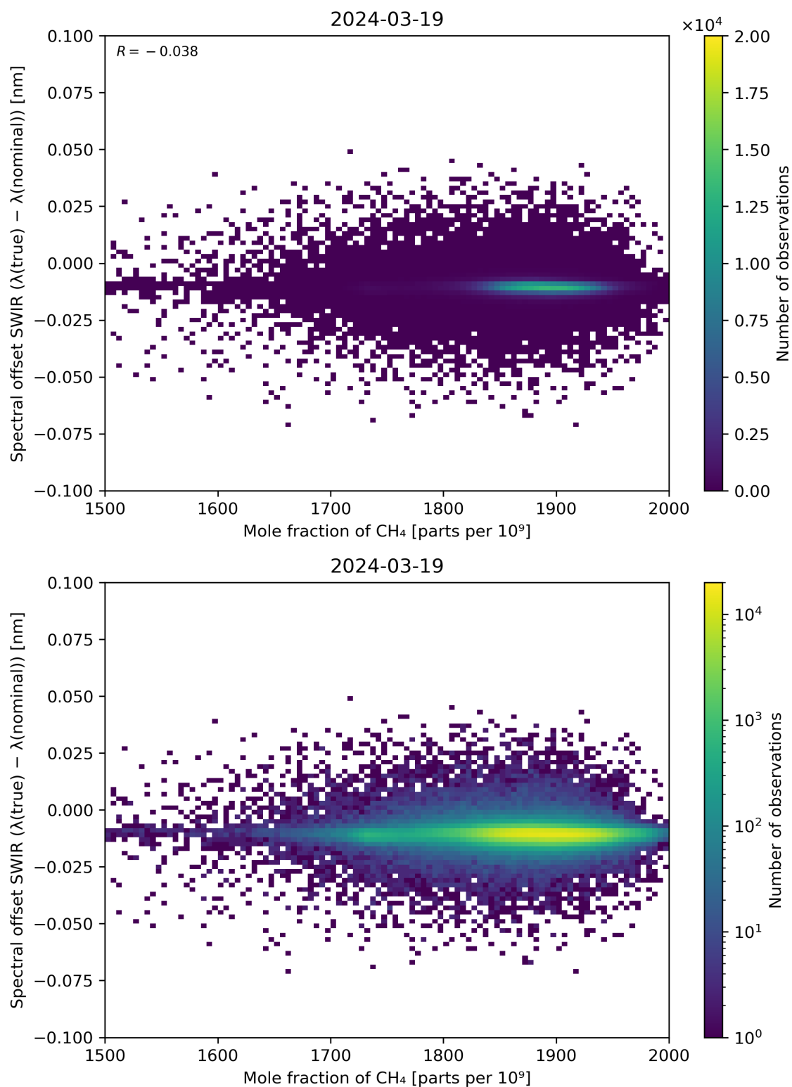
Figure 86: Scatter density plot of “Mole fraction of CH 4 ” against “Spectral offset SWIR ( \lambda(\text{true}) - \lambda(\text{nominal}) )” for 2024-03-18 to 2024-03-20.
