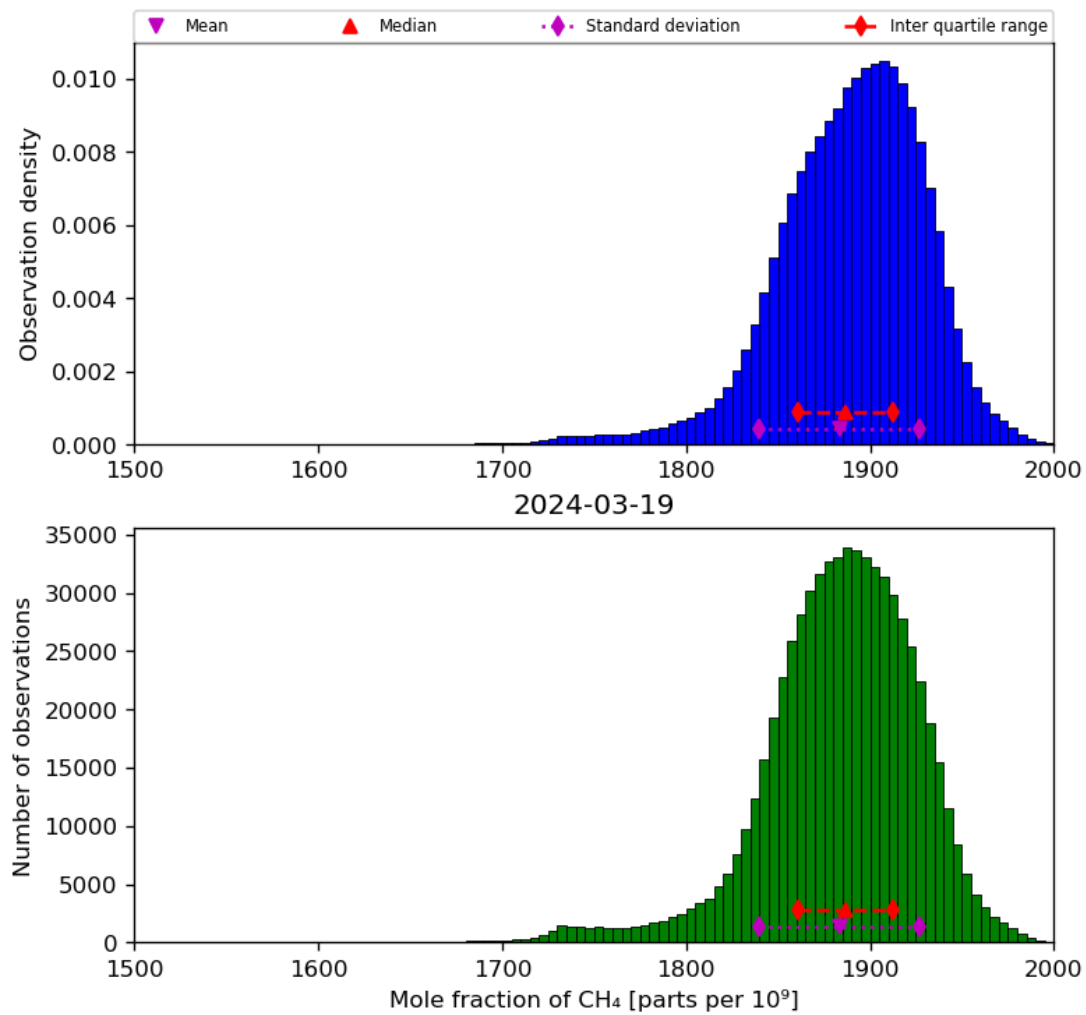
Figure 23: Histogram of “Mole fraction of CH 4 ” for 2024-03-18 to 2024-03-20
