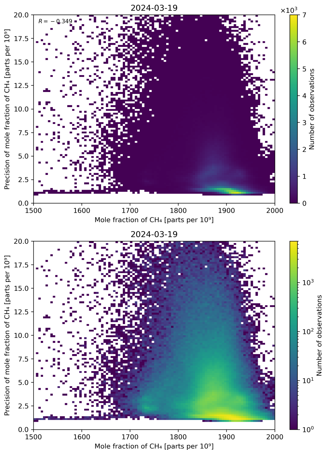
Figure 75: Scatter density plot of “Mole fraction of CH 4 ” against “Precision of mole fraction of CH 4 ” for 2024-03-18 to 2024-03-20.
