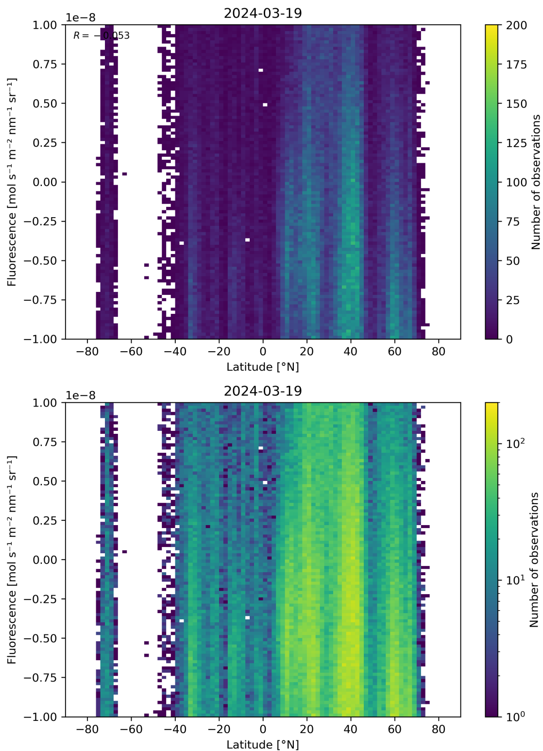
Figure 56: Scatter density plot of “Latitude” against “Fluorescence” for 2024-03-18 to 2024-03-20.
