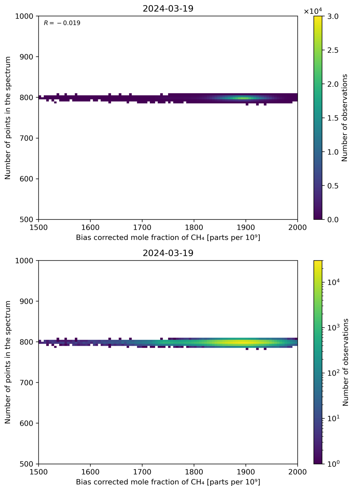
Figure 68: Scatter density plot of “Bias corrected mole fraction of CH 4 ” against “Number of points in the spectrum” for 2024-03-18 to 2024-03-20.
