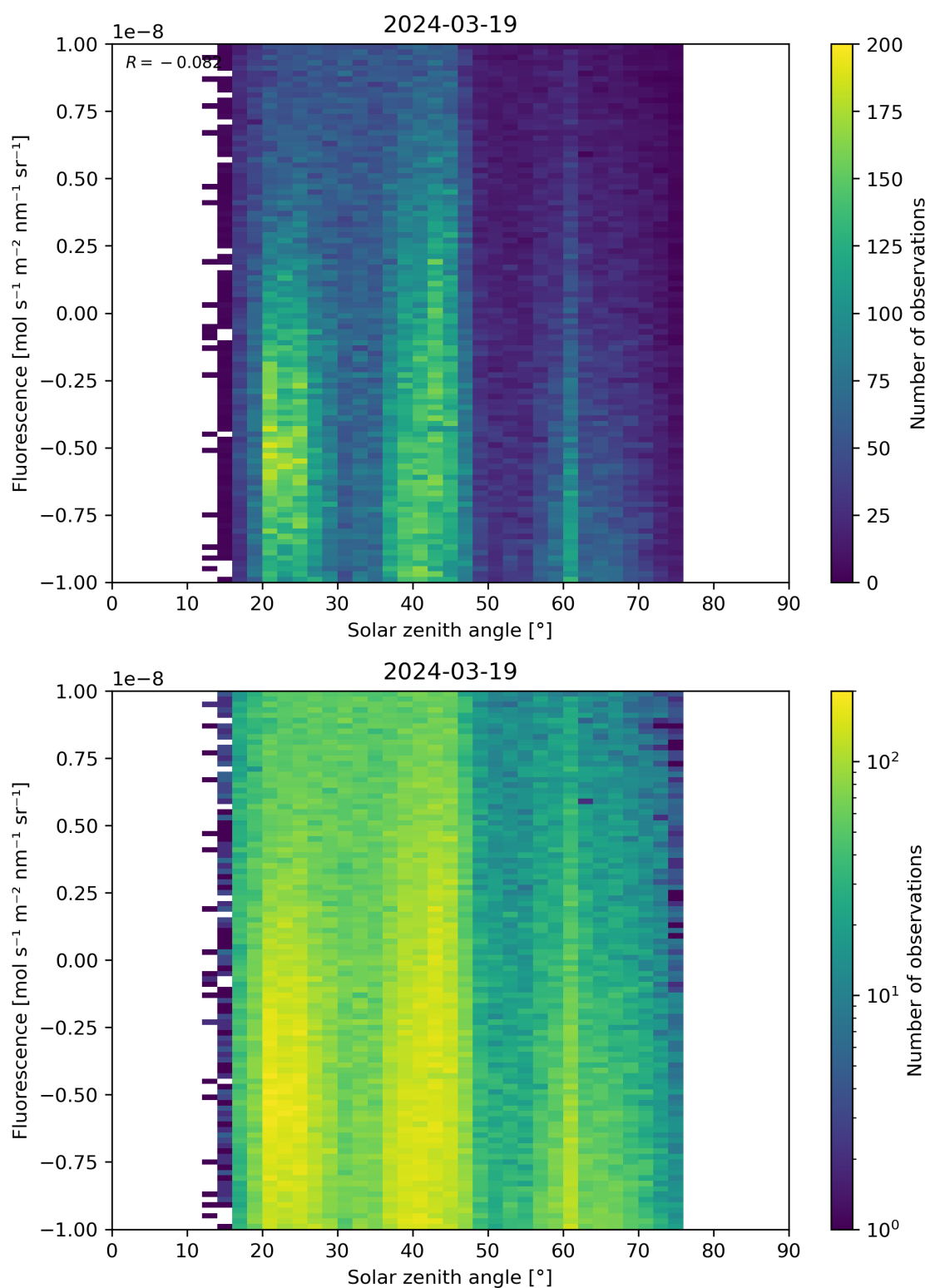
Figure 97: Scatter density plot of “Solar zenith angle” against “Fluorescence” for 2024-03-18 to 2024-03-20.
