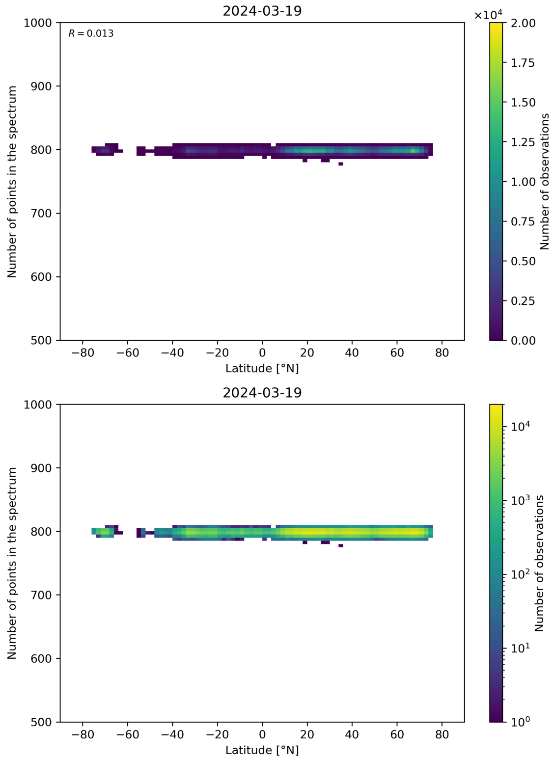
Figure 61: Scatter density plot of “Latitude” against “Number of points in the spectrum” for 2024-03-18 to 2024-03-20.
