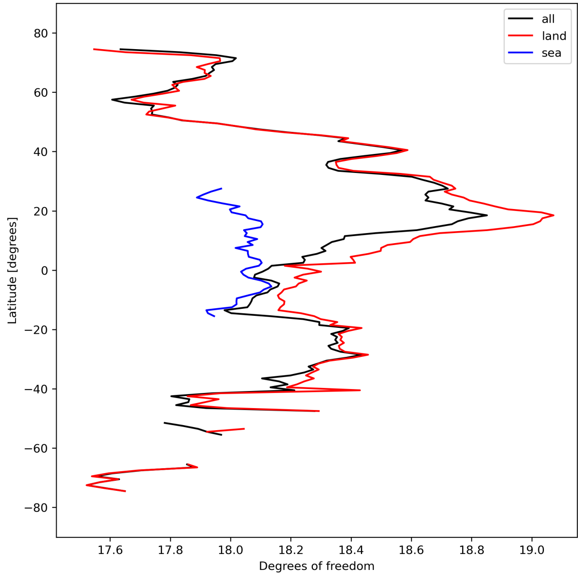
Figure 19: Zonal average of “Degrees of freedom” for 2024-03-18 to 2024-03-20.
