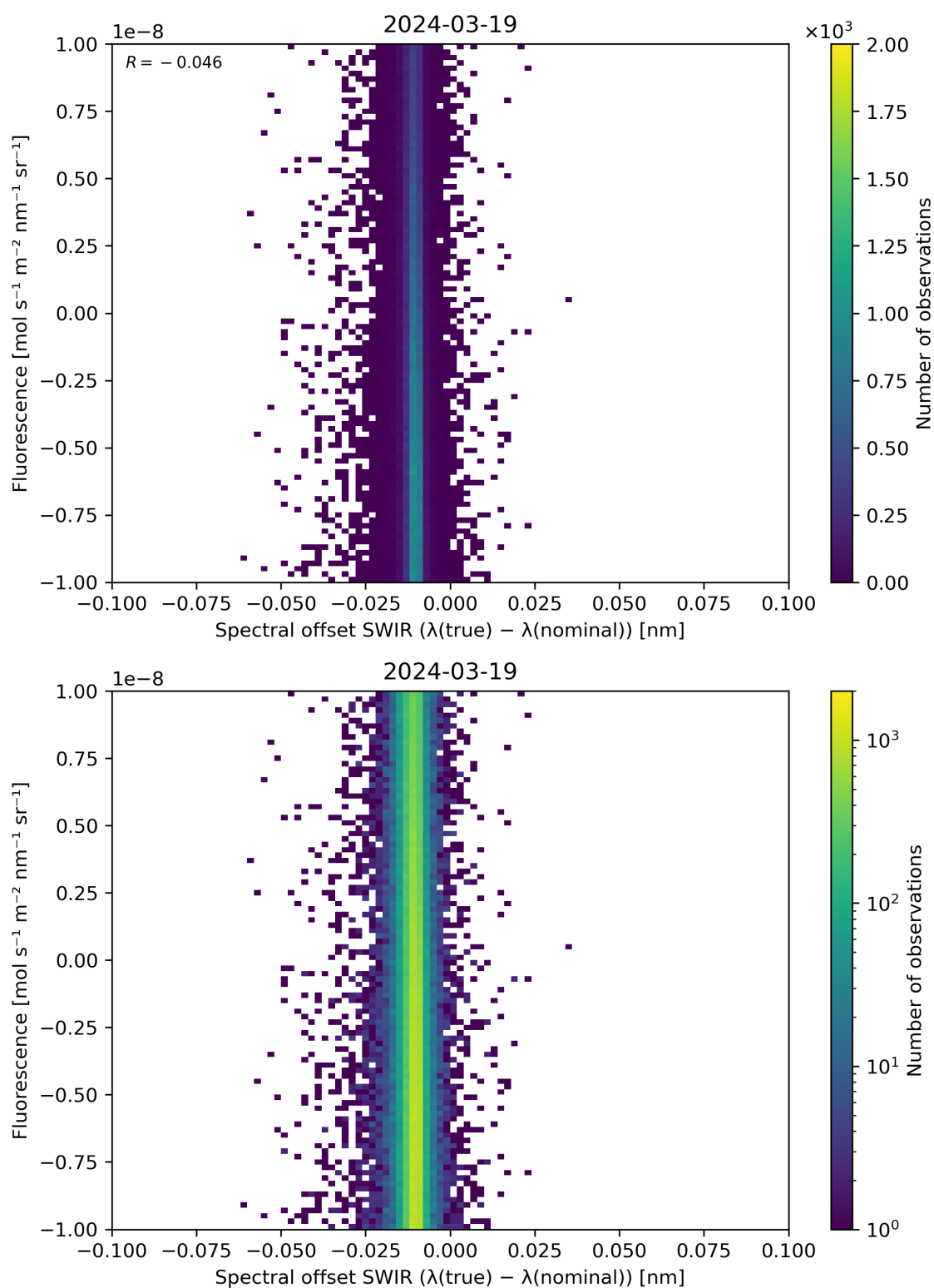
Figure 120: Scatter density plot of “Spectral offset SWIR ( \lambda(\text{true}) - \lambda(\text{nominal}) )” against “Fluorescence” for 2024-03-18 to 2024-03-20.
