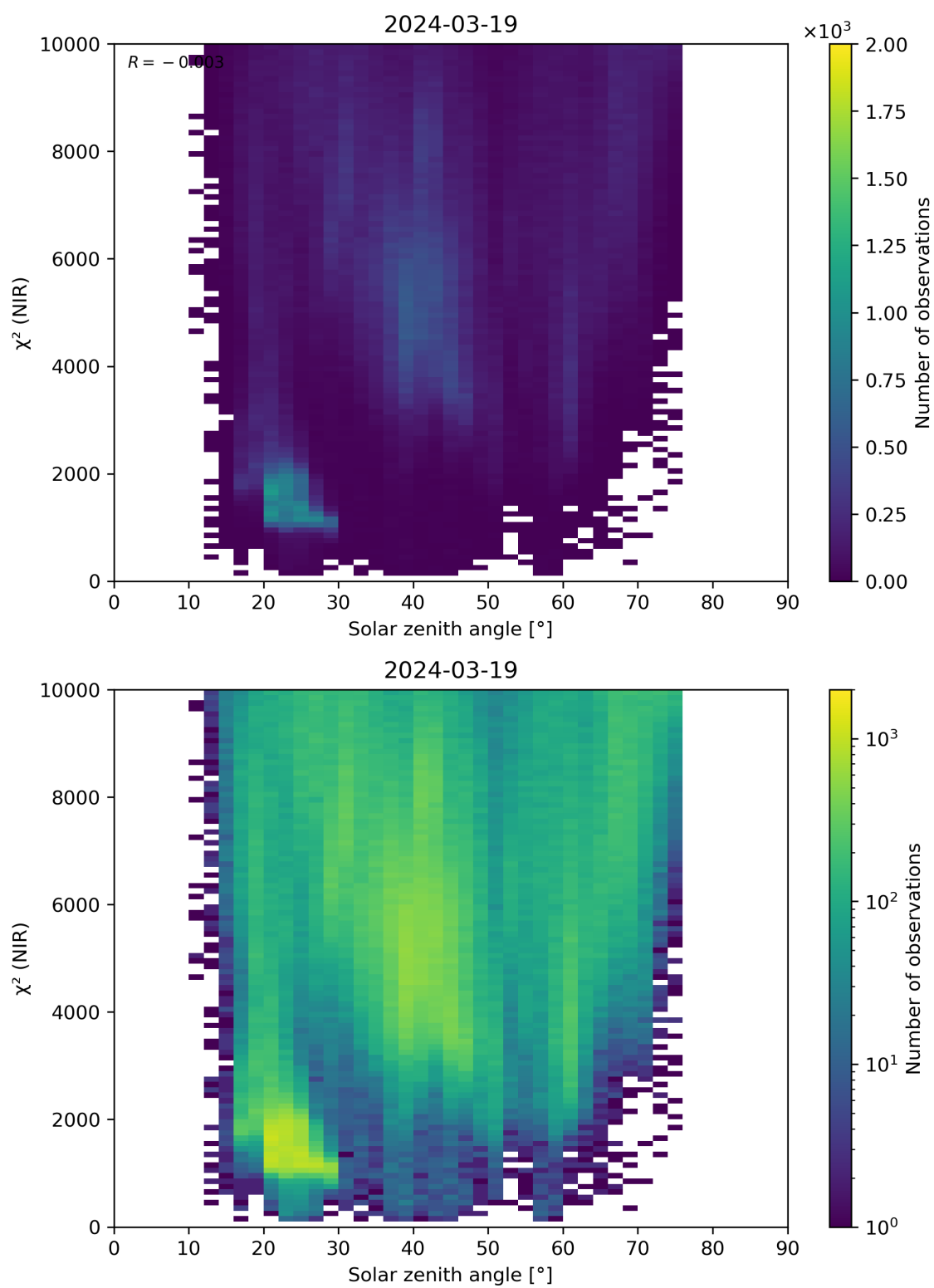
Figure 94: Scatter density plot of “Solar zenith angle” against “ \chi^2 (NIR)” for 2024-03-18 to 2024-03-20.
