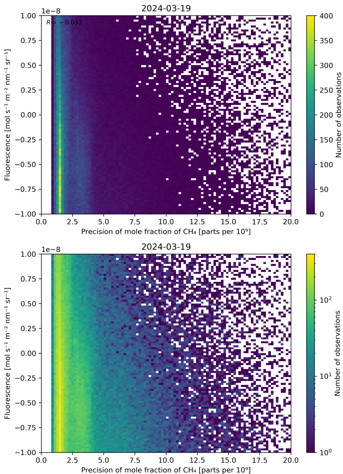
Figure 81: Scatter density plot of “Precision of mole fraction of CH 4 ” against “Fluorescence” for 2024-03-18 to 2024-03-20.
