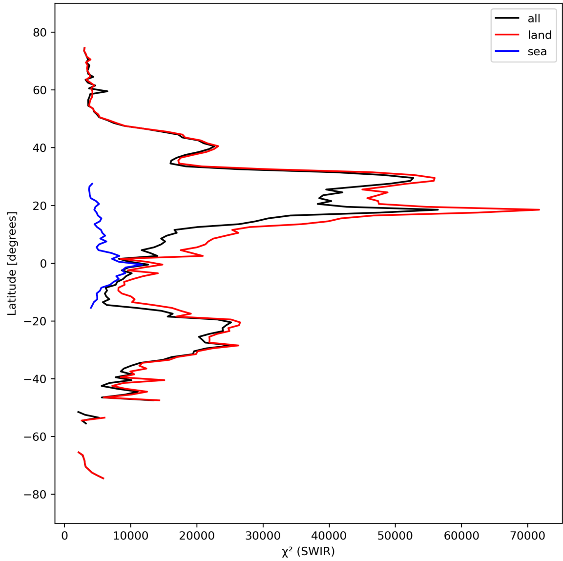
Figure 17: Zonal average of “ \chi^2 (SWIR)” for 2024-03-18 to 2024-03-20.
