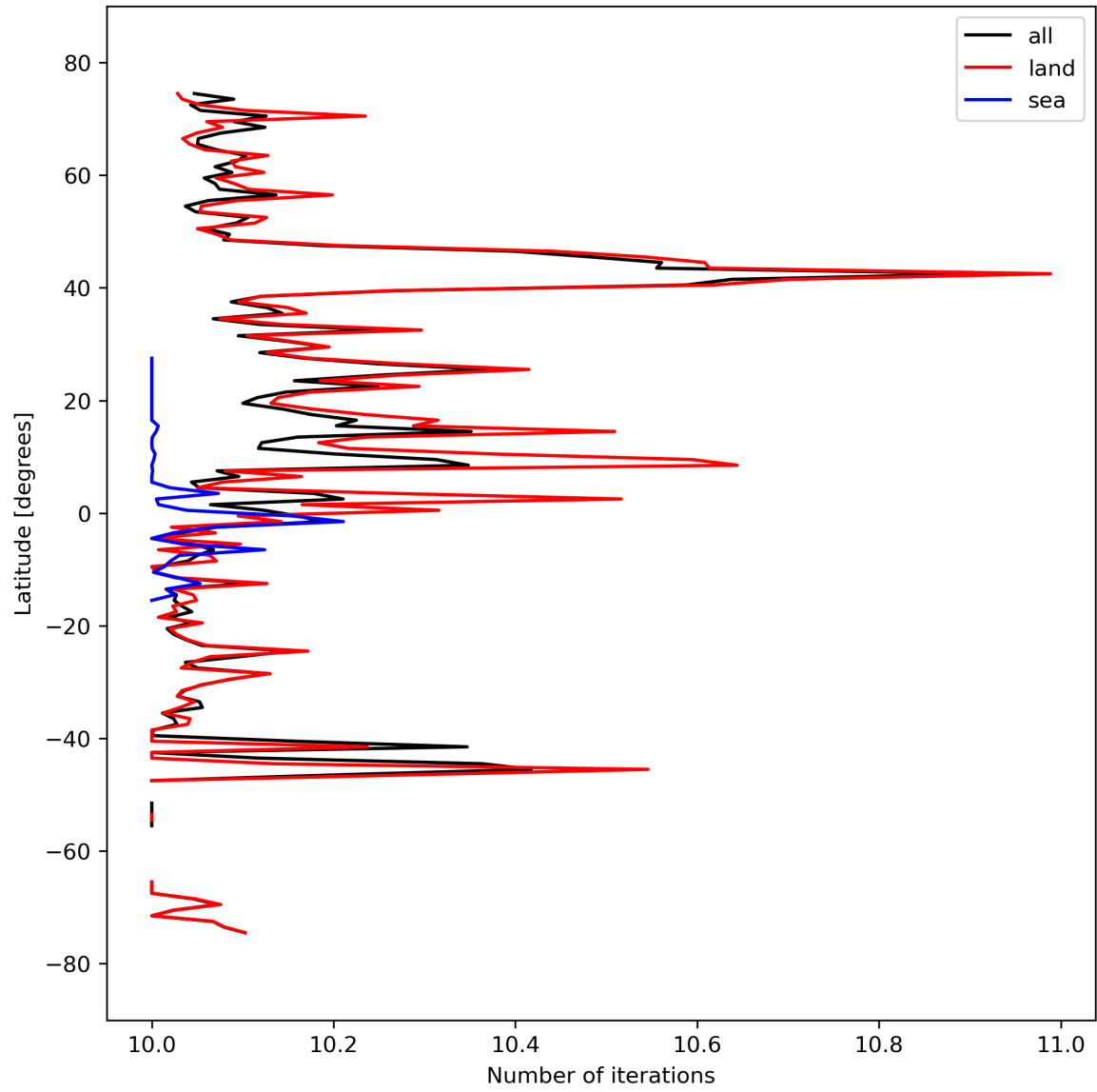
Figure 20: Zonal average of “Number of iterations” for 2024-03-18 to 2024-03-20.
