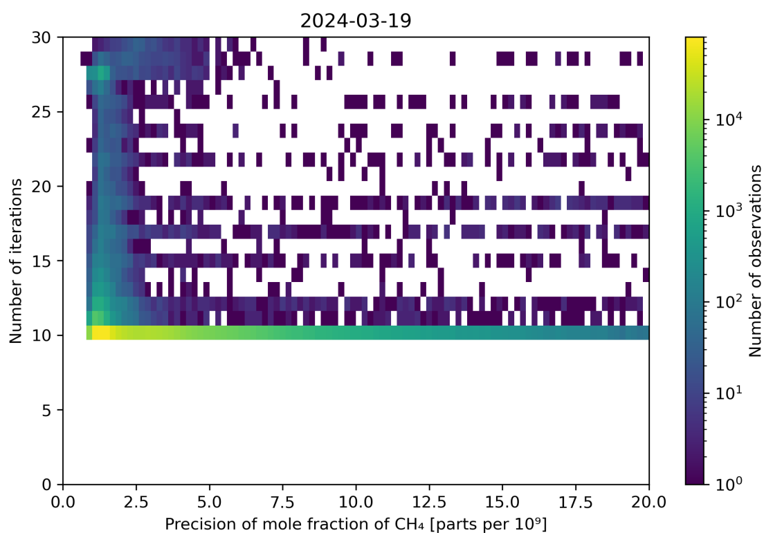
Figure 83: Scatter density plot of “Precision of mole fraction of CH 4 ” against “Number of iterations” for 2024-03-18 to 2024-03-20.
