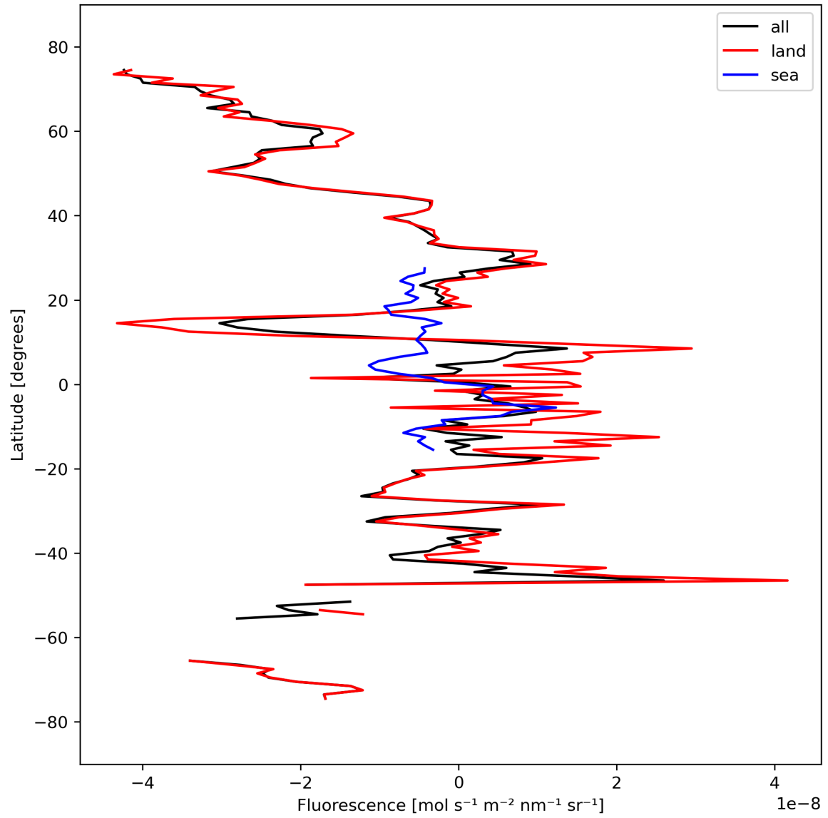
Figure 21: Zonal average of “Fluorescence” for 2024-03-18 to 2024-03-20.
