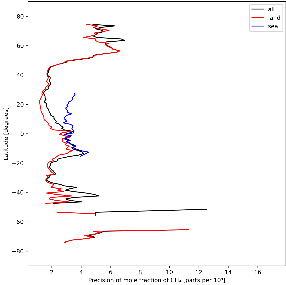
Figure 13: Zonal average of “Precision of mole fraction of CH 4 ” for 2024-03-18 to 2024-03-20.
