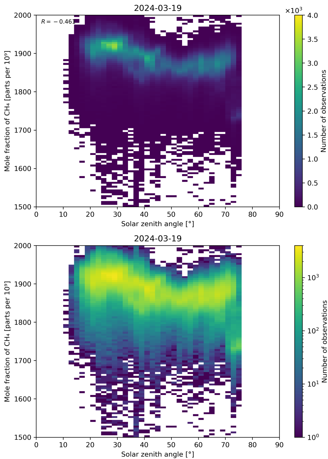
Figure 99: Scatter density plot of “Solar zenith angle” against “Mole fraction of CH 4 ” for 2024-03-18 to 2024-03-20.
