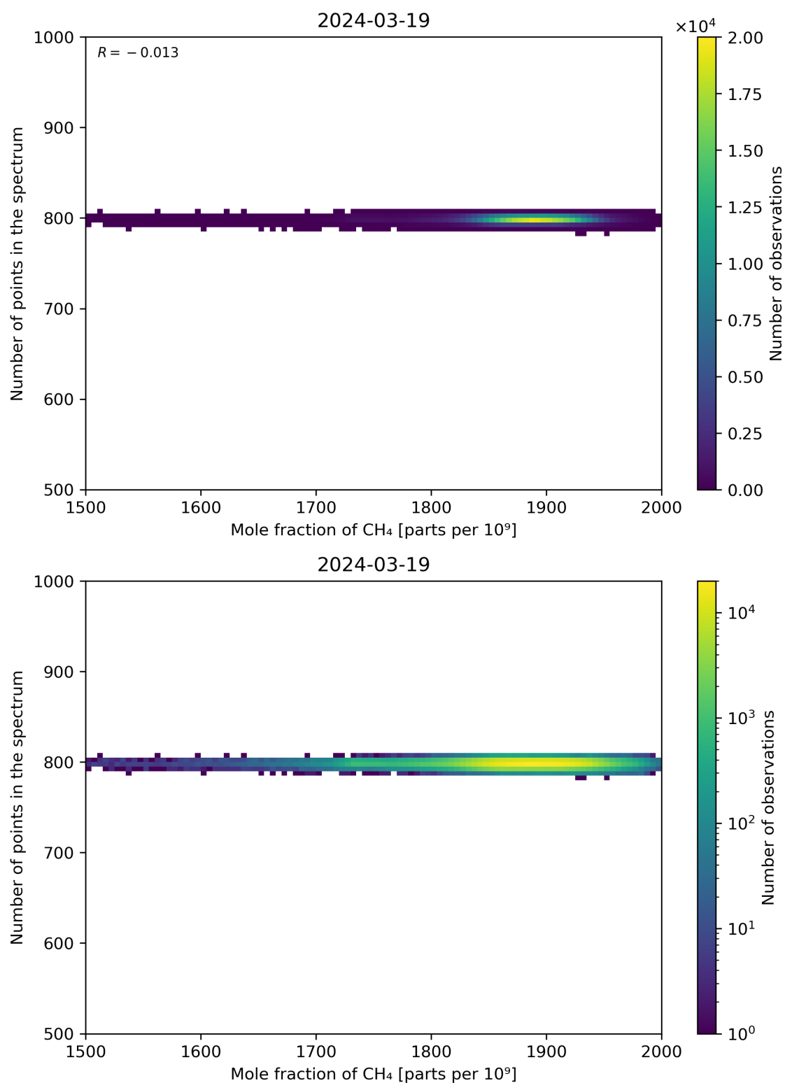
Figure 77: Scatter density plot of “Mole fraction of CH 4 ” against “Number of points in the spectrum” for 2024-03-18 to 2024-03-20.
