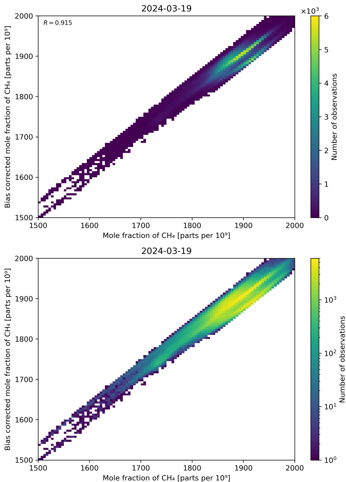
Figure 74: Scatter density plot of “Mole fraction of CH 4 ” against “Bias corrected mole fraction of CH 4 ” for 2024-03-18 to 2024-03-20.
