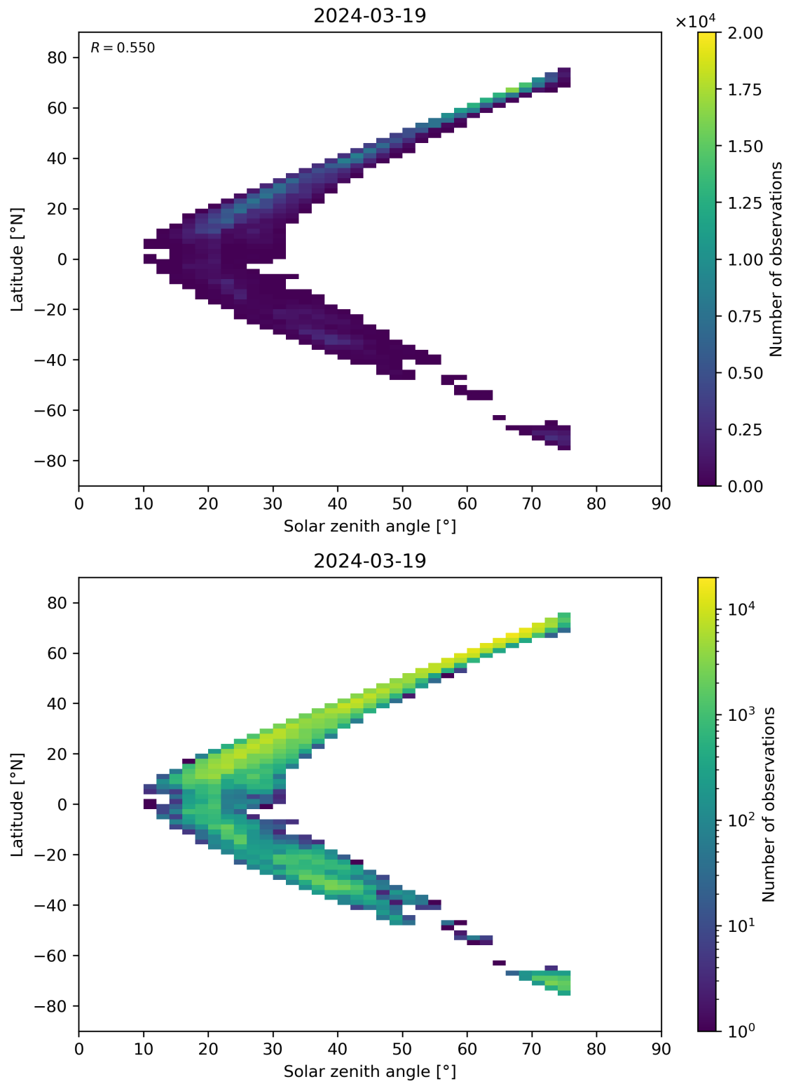
Figure 98: Scatter density plot of “Solar zenith angle” against “Latitude” for 2024-03-18 to 2024-03-20.
