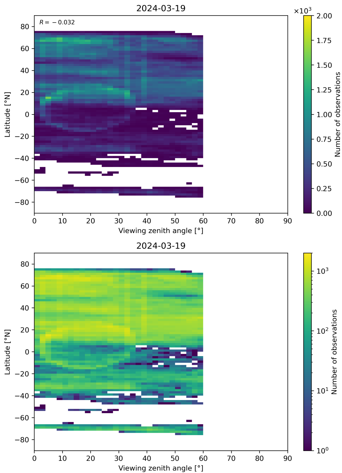
Figure 109: Scatter density plot of “Viewing zenith angle” against “Latitude” for 2024-03-18 to 2024-03-20.
