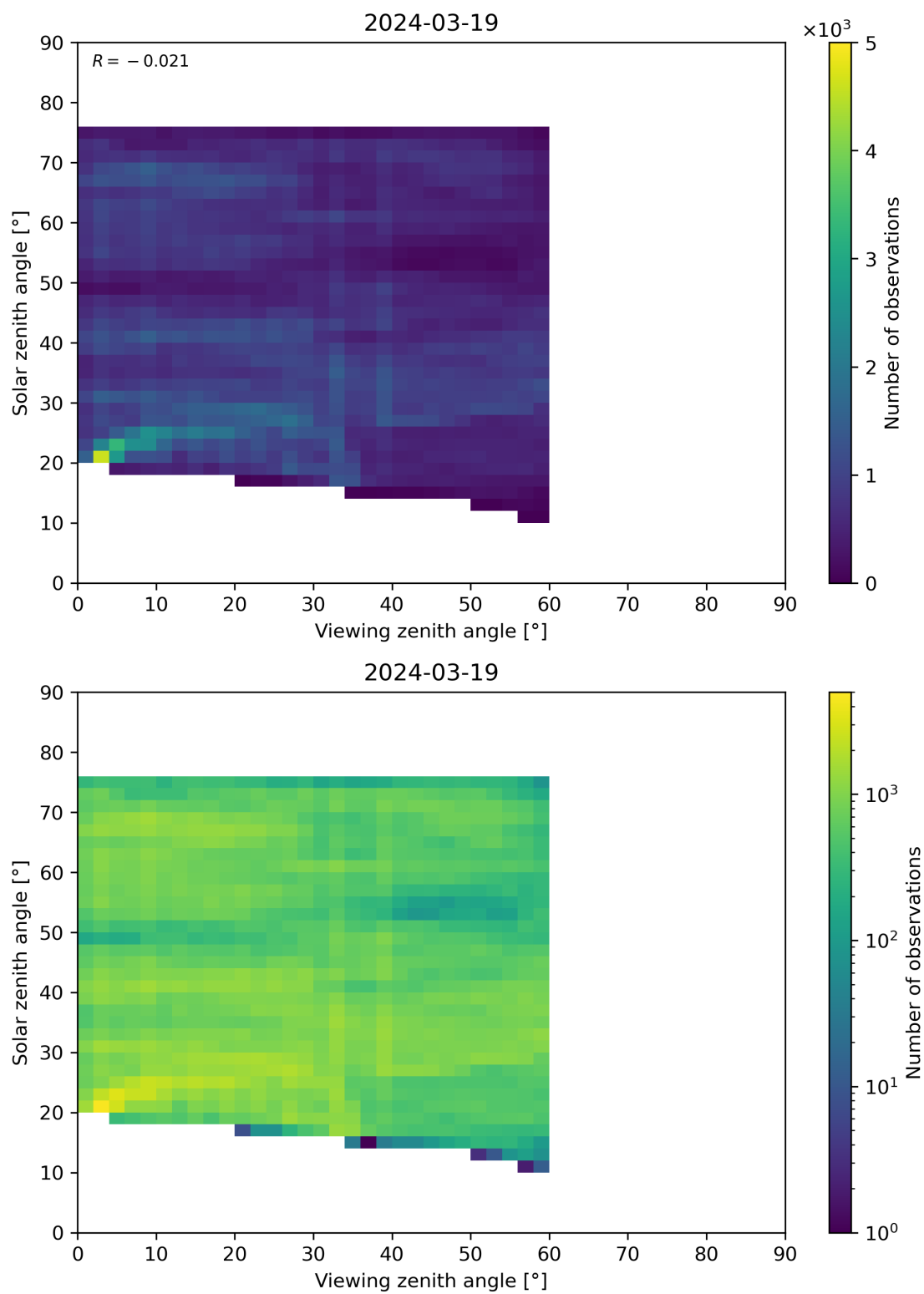
Figure 115: Scatter density plot of “Viewing zenith angle” against “Solar zenith angle” for 2024-03-18 to 2024-03-20.
