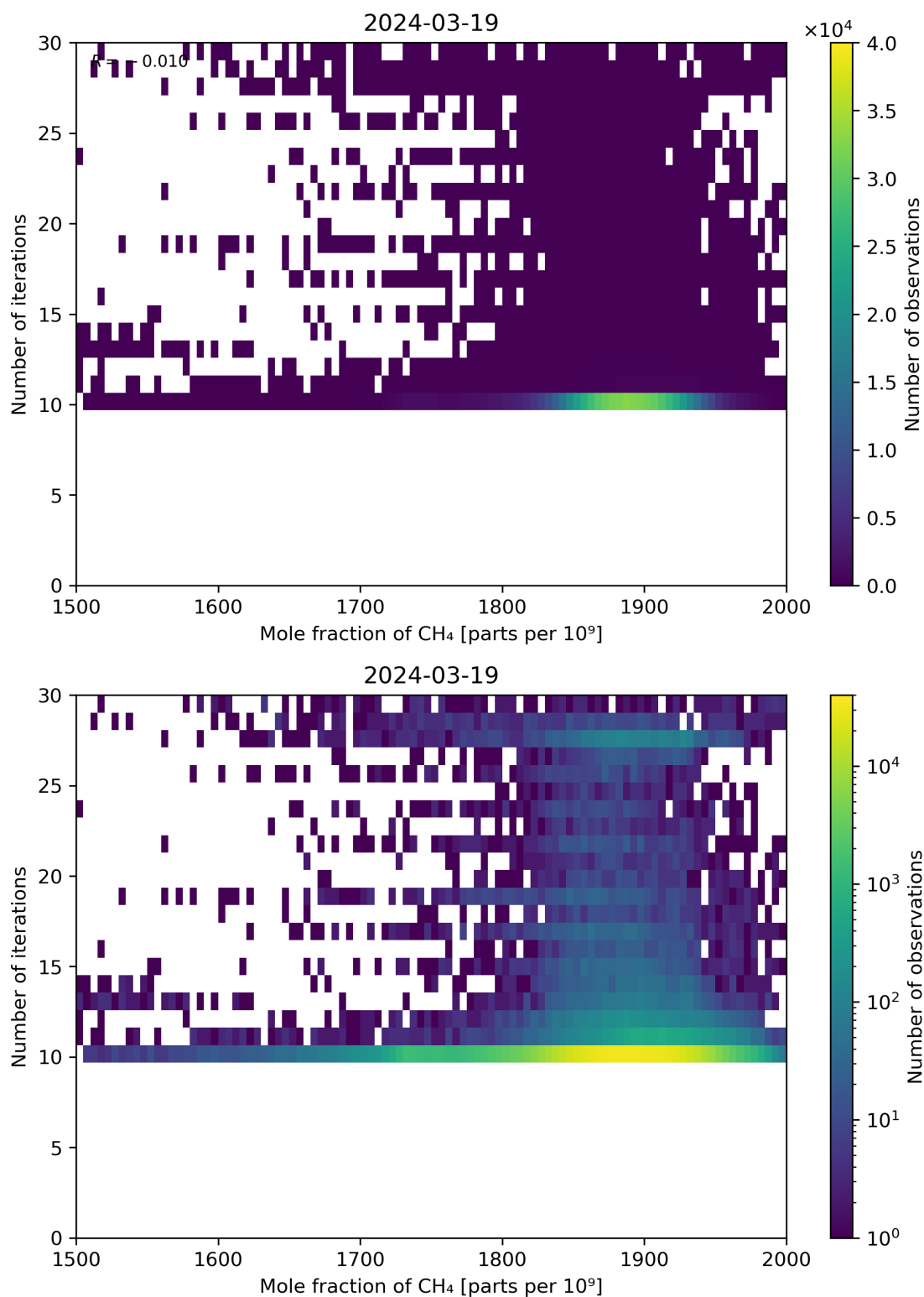
Figure 76: Scatter density plot of “Mole fraction of CH 4 ” against “Number of iterations” for 2024-03-18 to 2024-03-20.
