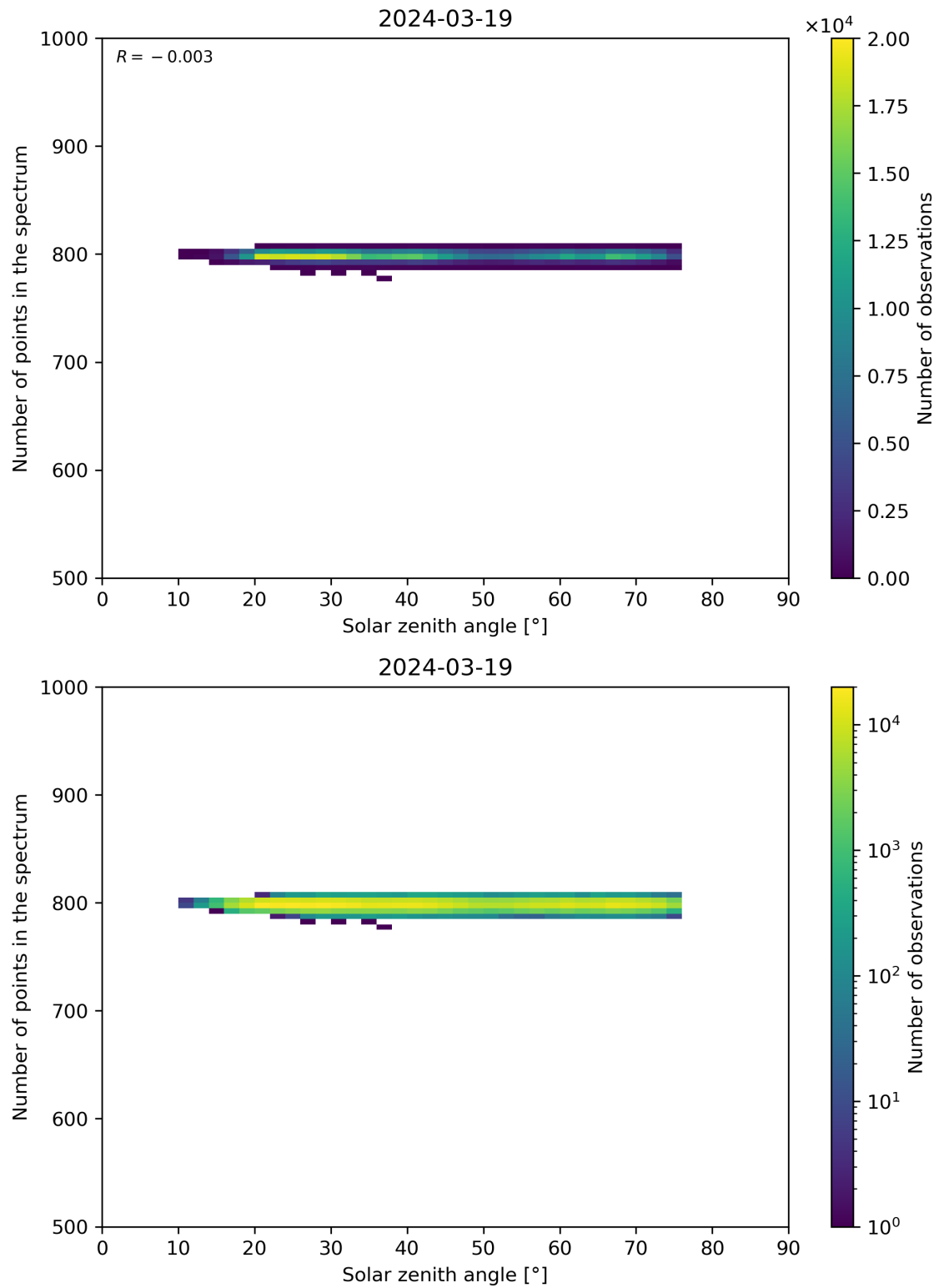
Figure 103: Scatter density plot of “Solar zenith angle” against “Number of points in the spectrum” for 2024-03-18 to 2024-03-20.
