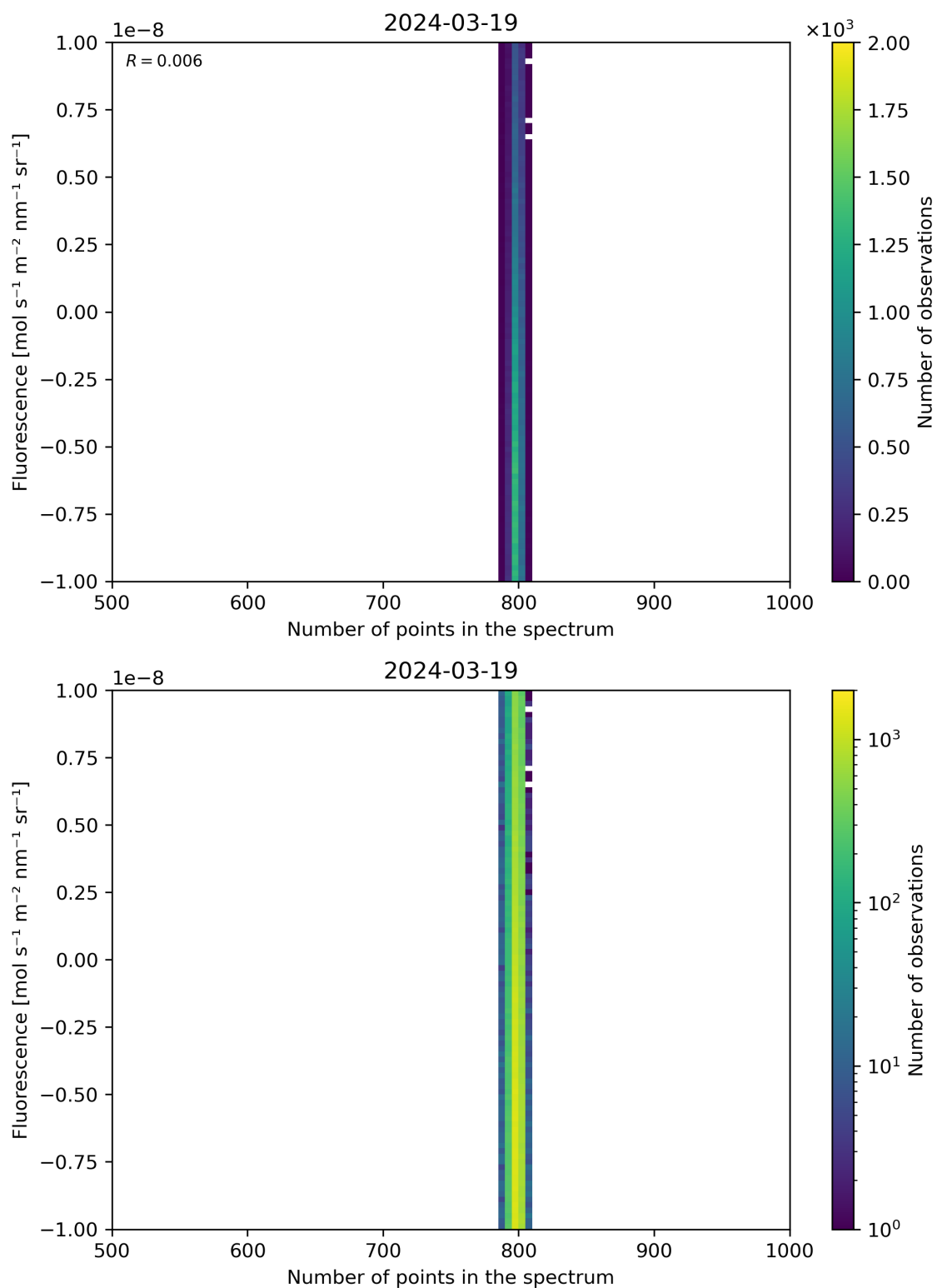
Figure 91: Scatter density plot of “Number of points in the spectrum” against “Fluorescence” for 2024-03-18 to 2024-03-20.
