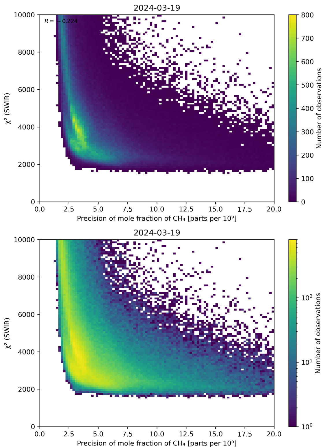
Figure 79: Scatter density plot of “Precision of mole fraction of CH 4 ” against “ \chi^2 (SWIR)” for 2024-03-18 to 2024-03-20.
