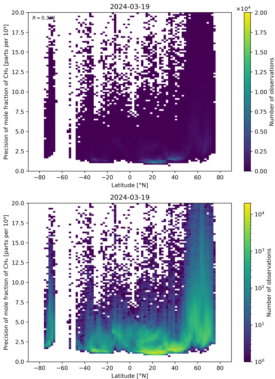
Figure 59: Scatter density plot of “Latitude” against “Precision of mole fraction of CH 4 ” for 2024-03-18 to 2024-03-20.
