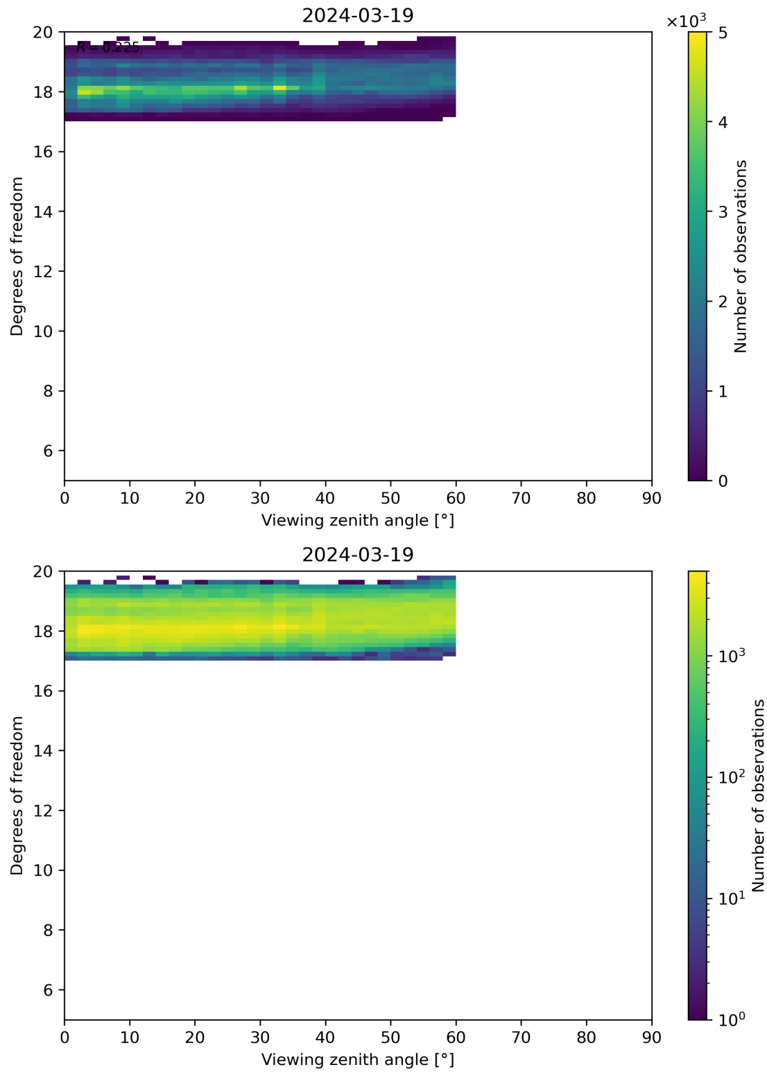
Figure 107: Scatter density plot of “Viewing zenith angle” against “Degrees of freedom” for 2024-03-18 to 2024-03-20.
