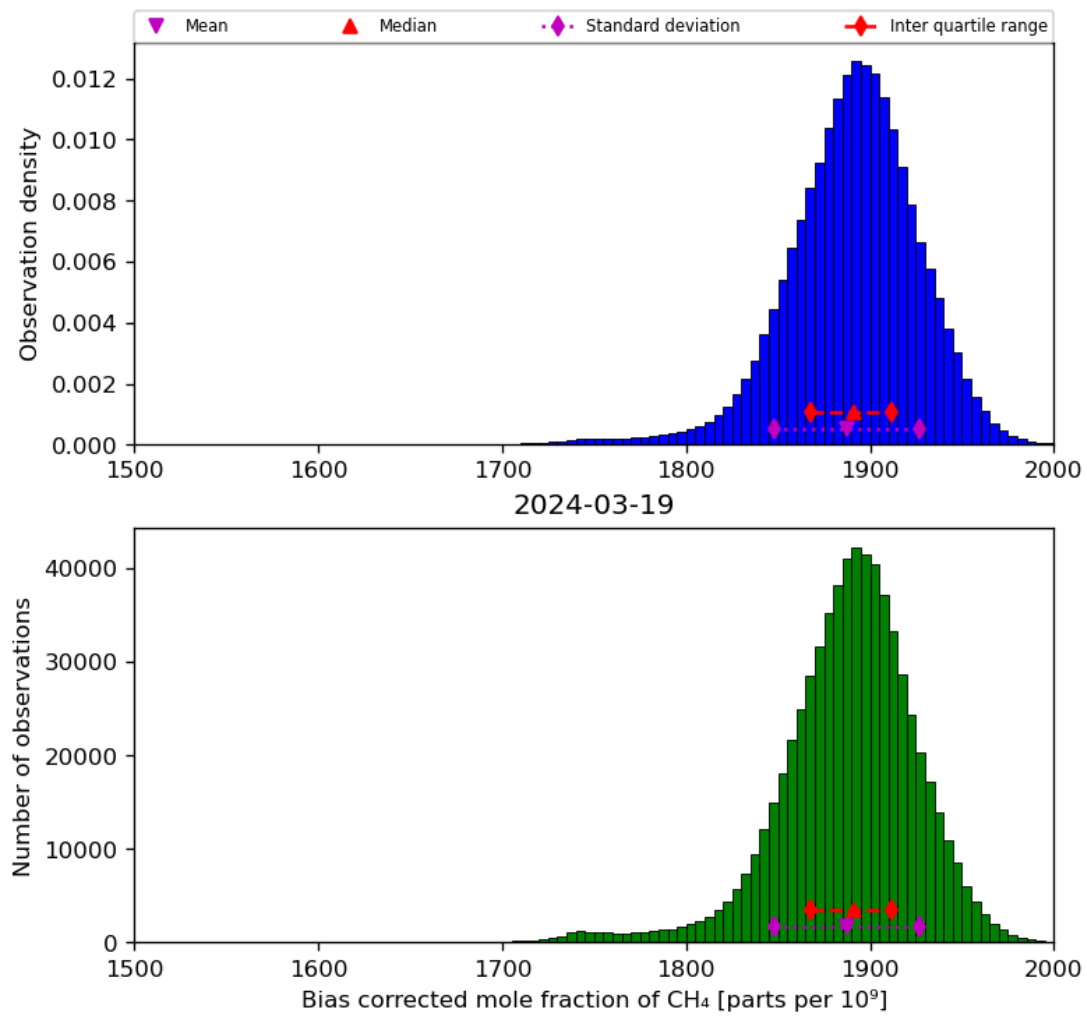
Figure 25: Histogram of “Bias corrected mole fraction of CH 4 ” for 2024-03-18 to 2024-03-20
