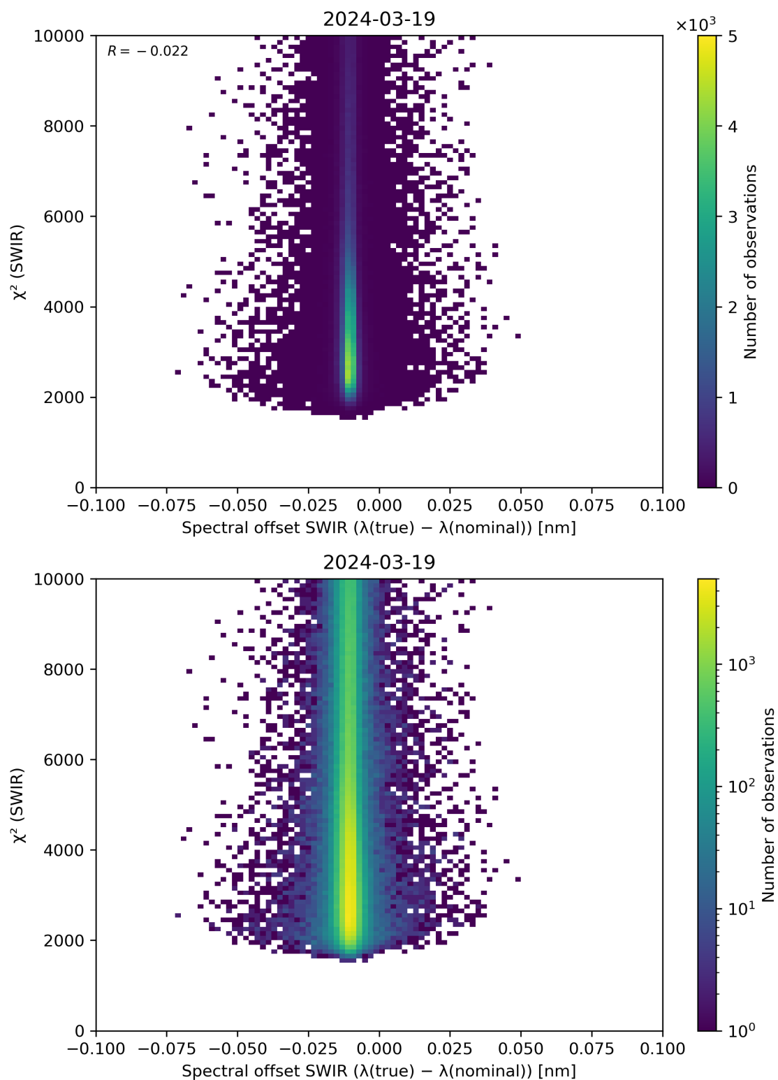
Figure 118: Scatter density plot of “Spectral offset SWIR ( \lambda(\text{true}) - \lambda(\text{nominal}) )” against “ \chi^2 (SWIR)” for 2024-03-18 to 2024-03-20.
