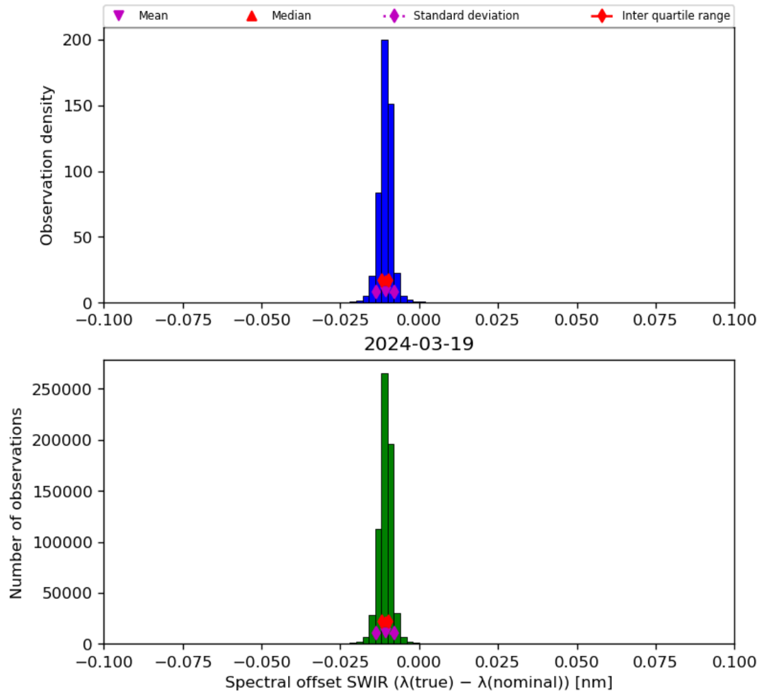
Figure 27: Histogram of “Spectral offset SWIR ( \lambda(\text{true}) - \lambda(\text{nominal}) )” for 2024-03-18 to 2024-03-20
