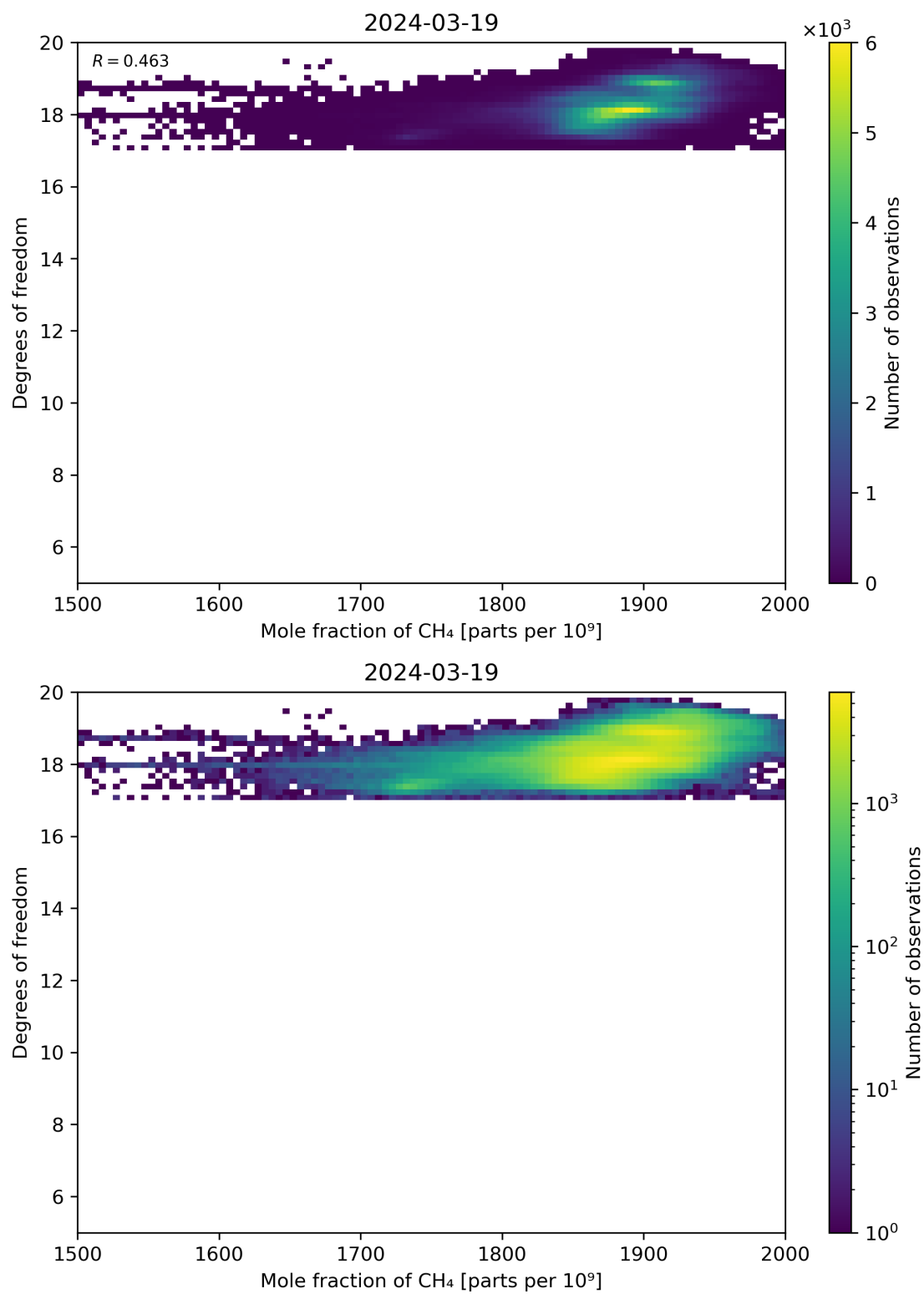
Figure 72: Scatter density plot of “Mole fraction of CH 4 ” against “Degrees of freedom” for 2024-03-18 to 2024-03-20.
