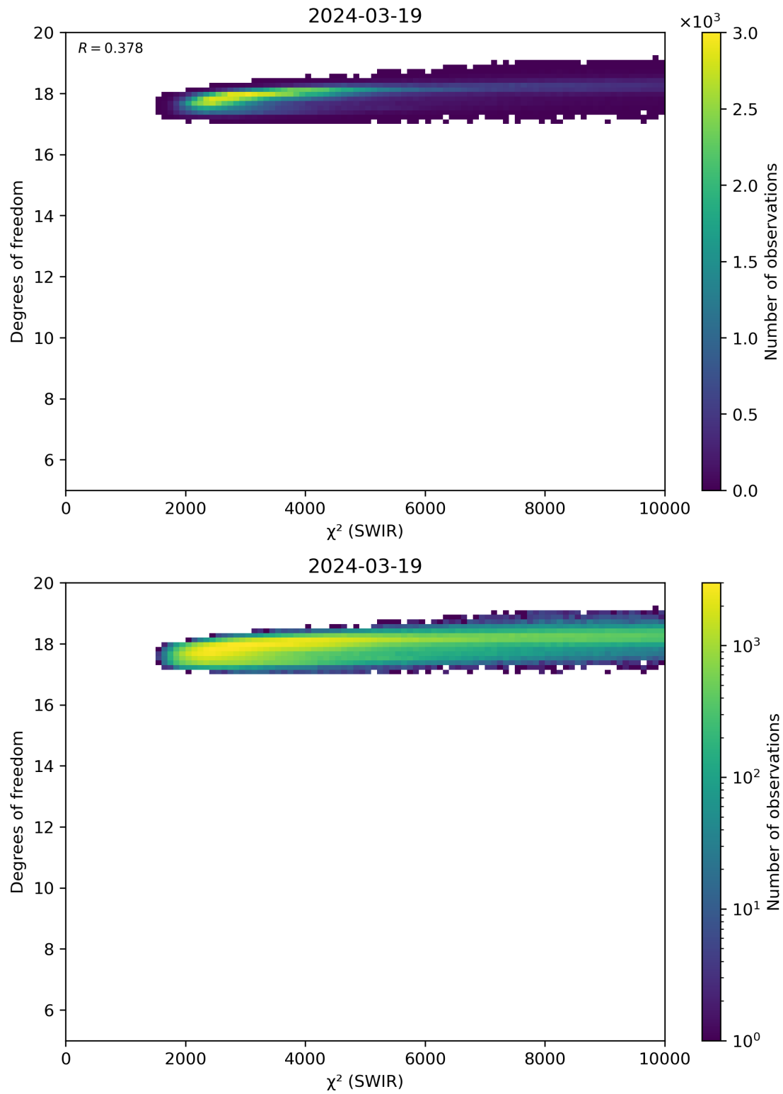
Figure 48: Scatter density plot of “ \chi^2 (SWIR)” against “Degrees of freedom” for 2024-03-18 to 2024-03-20.
