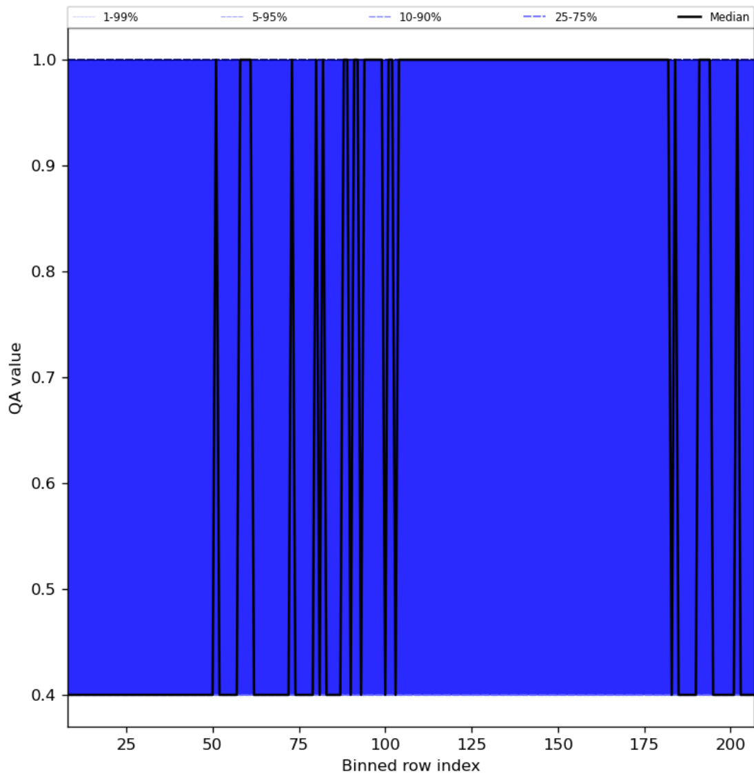
Figure 33: Along track statistics of “QA value” for 2024-03-18 to 2024-03-20
