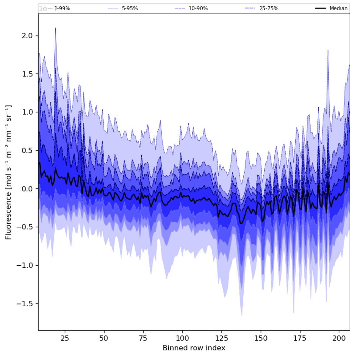
Figure 43: Along track statistics of “Fluorescence” for 2024-03-18 to 2024-03-20
