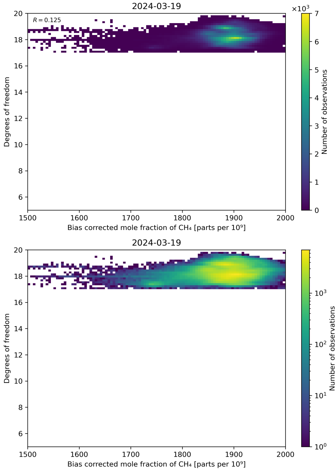
Figure 65: Scatter density plot of “Bias corrected mole fraction of CH 4 ” against “Degrees of freedom” for 2024-03-18 to 2024-03-20.
