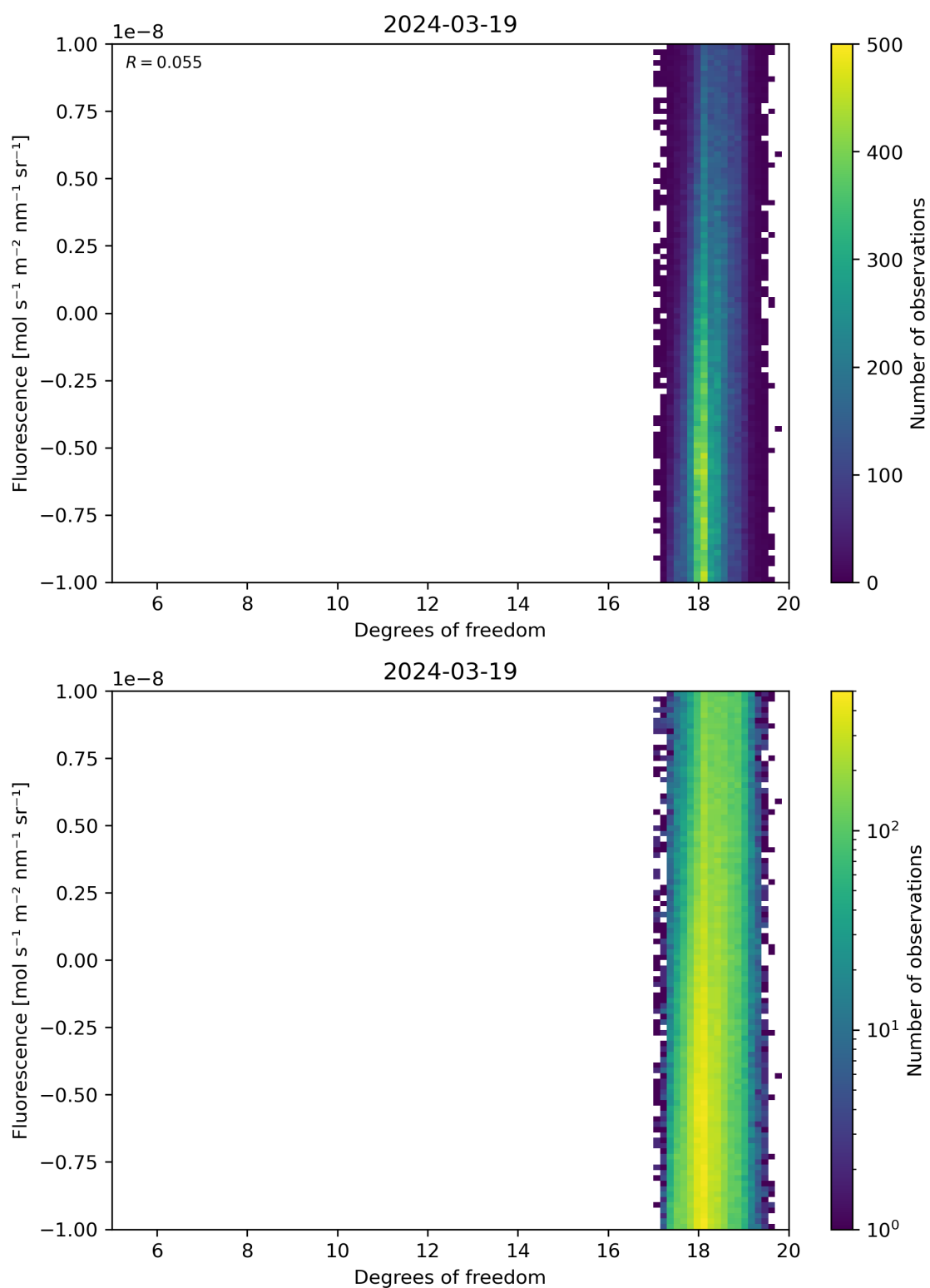
Figure 51: Scatter density plot of “Degrees of freedom” against “Fluorescence” for 2024-03-18 to 2024-03-20.
