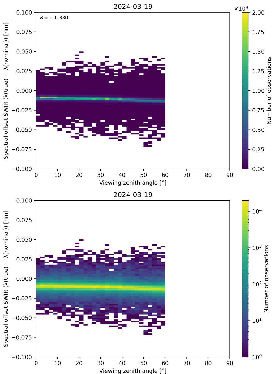
Figure 116: Scatter density plot of “Viewing zenith angle” against “Spectral offset SWIR ( \lambda(\text{true}) - \lambda(\text{nominal}) )” for 2024-03-18 to 2024-03-20.
