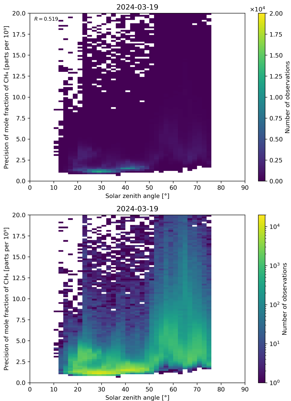
Figure 101: Scatter density plot of “Solar zenith angle” against “Precision of mole fraction of CH 4 ” for 2024-03-18 to 2024-03-20.
