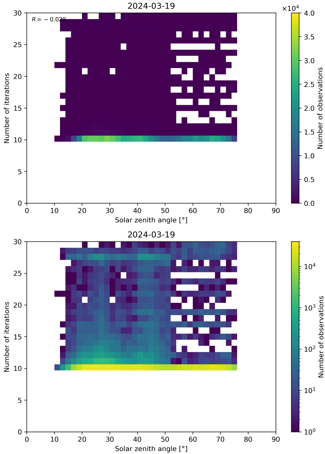
Figure 102: Scatter density plot of “Solar zenith angle” against “Number of iterations” for 2024-03-18 to 2024-03-20.
