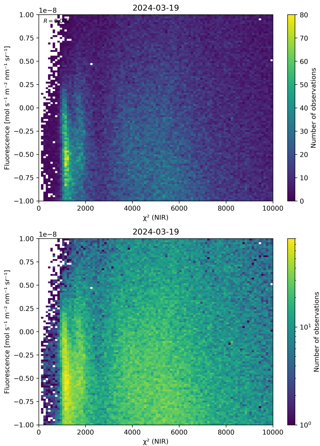
Figure 45: Scatter density plot of “ \chi^2 (NIR)” against “Fluorescence” for 2024-03-18 to 2024-03-20.
