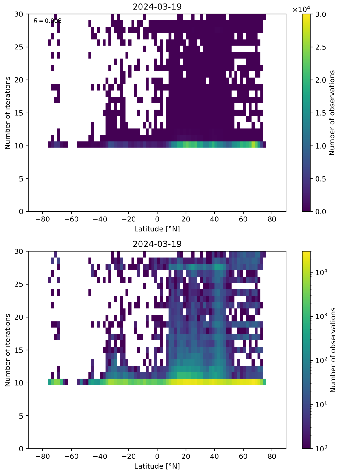
Figure 60: Scatter density plot of “Latitude” against “Number of iterations” for 2024-03-18 to 2024-03-20.
