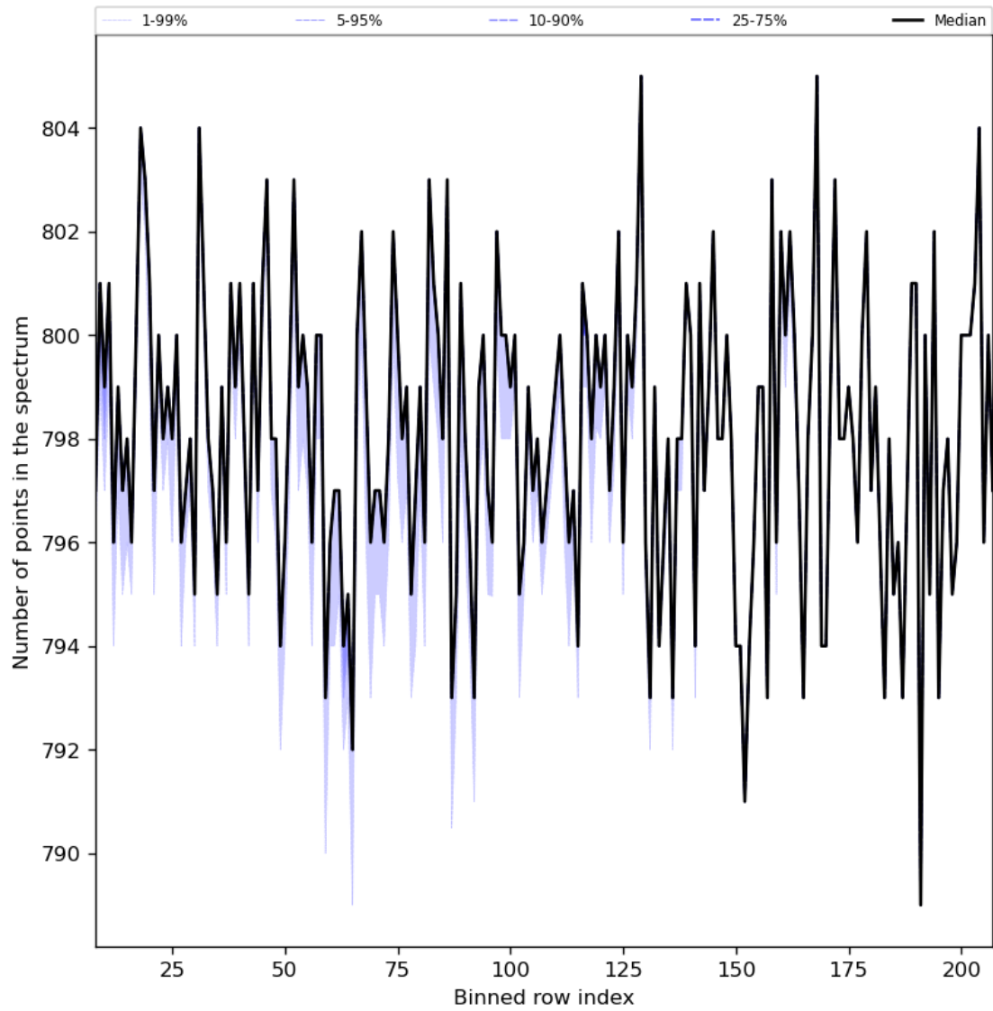
Figure 37: Along track statistics of “Number of points in the spectrum” for 2024-03-18 to 2024-03-20
