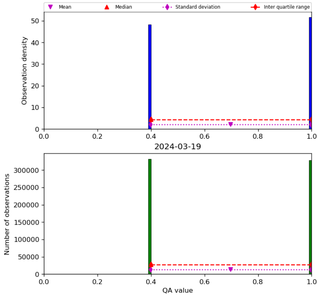
Figure 22: Histogram of “QA value” for 2024-03-18 to 2024-03-20
