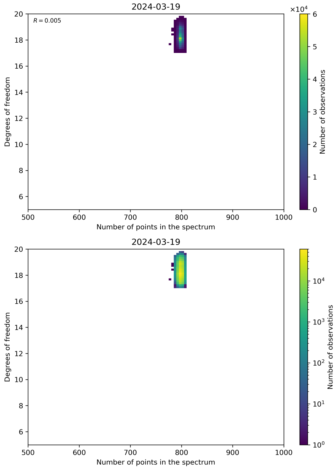
Figure 90: Scatter density plot of “Number of points in the spectrum” against “Degrees of freedom” for 2024-03-18 to 2024-03-20.
