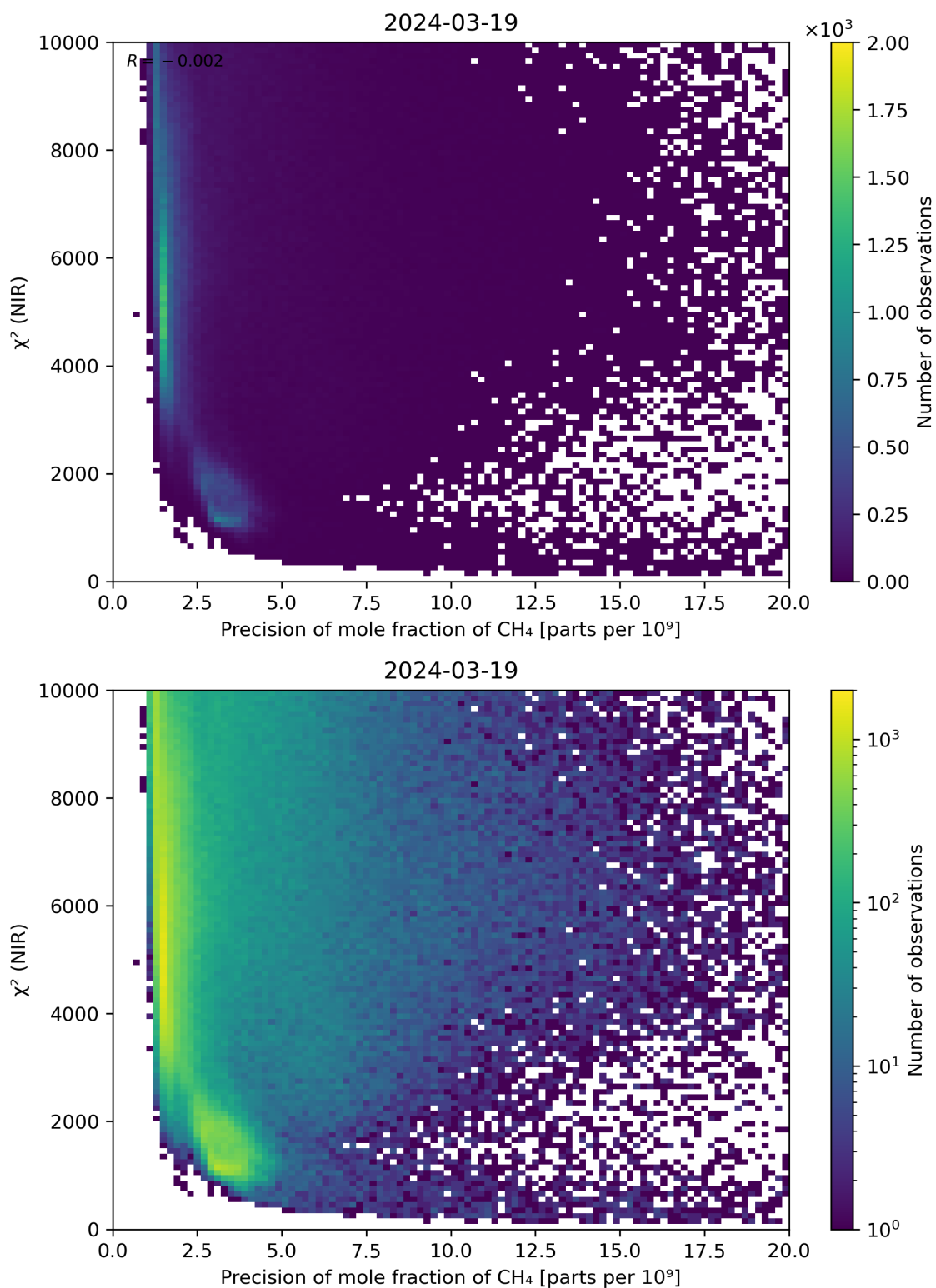
Figure 78: Scatter density plot of “Precision of mole fraction of \text{CH}_4 ” against “ \chi^2 (NIR)” for 2024-03-18 to 2024-03-20.
