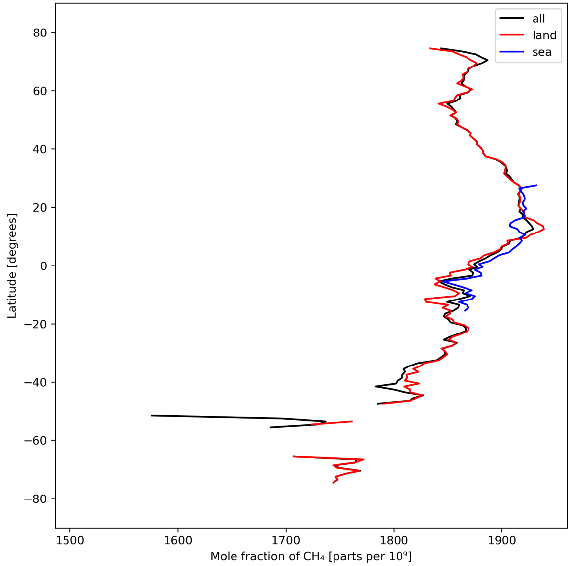
Figure 12: Zonal average of “Mole fraction of \text{CH}_4 ” for 2024-03-18 to 2024-03-20.
