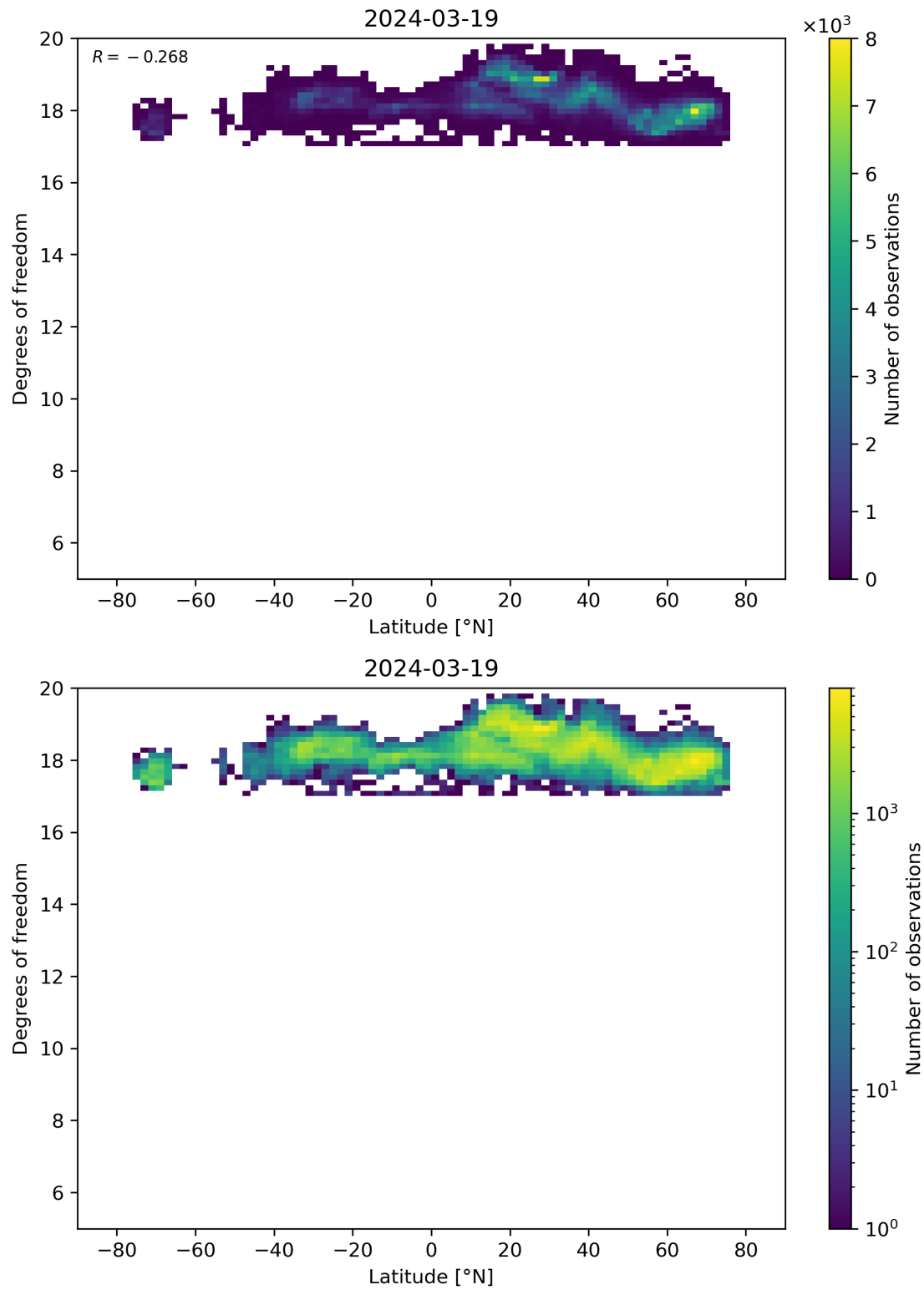
Figure 55: Scatter density plot of “Latitude” against “Degrees of freedom” for 2024-03-18 to 2024-03-20.
