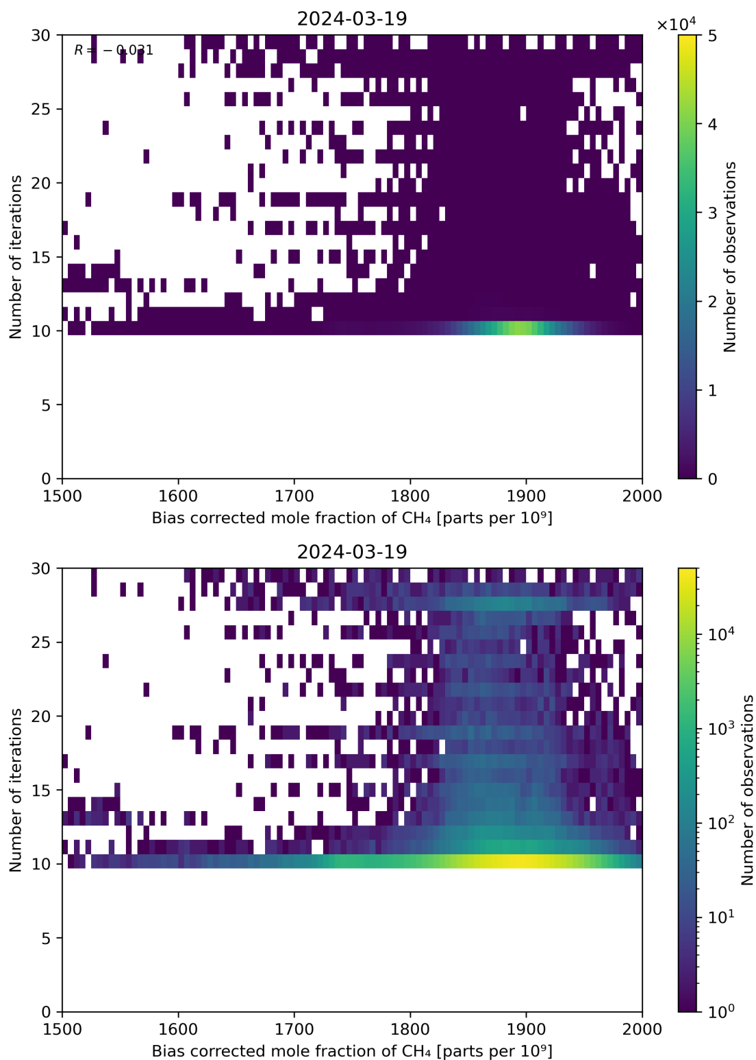
Figure 67: Scatter density plot of “Bias corrected mole fraction of \text{CH}_4 ” against “Number of iterations” for 2024-03-18 to 2024-03-20.
