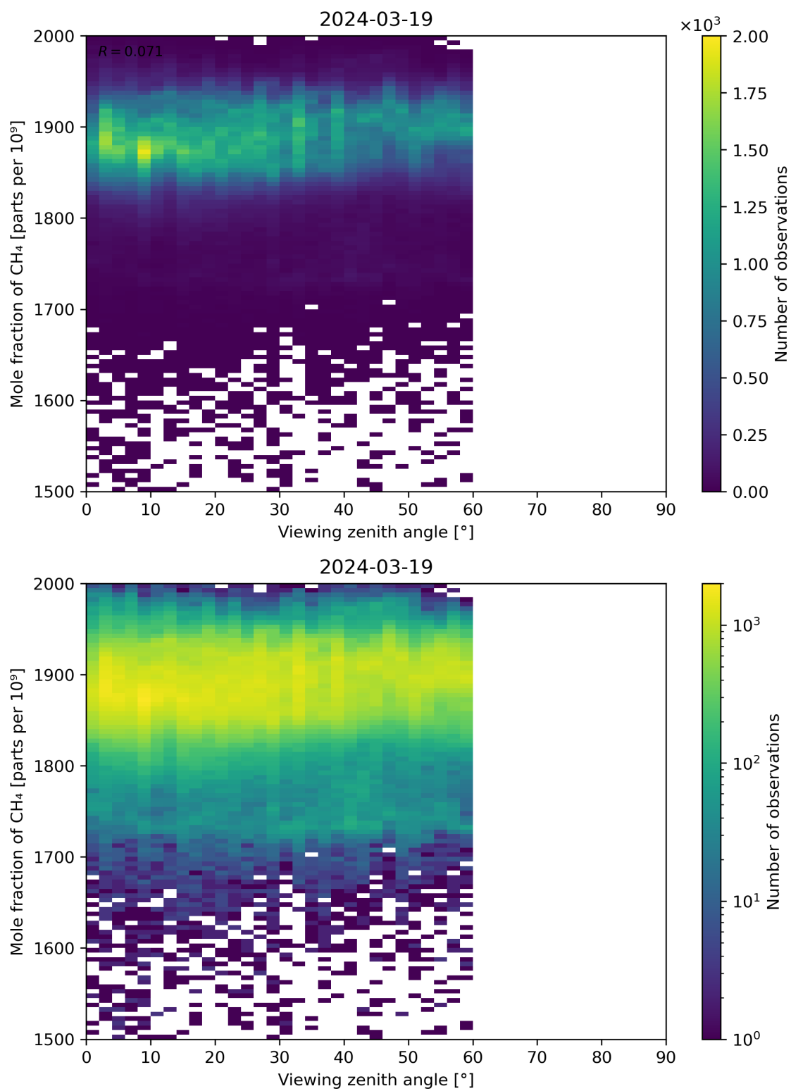
Figure 110: Scatter density plot of “Viewing zenith angle” against “Mole fraction of CH 4 ” for 2024-03-18 to 2024-03-20.
