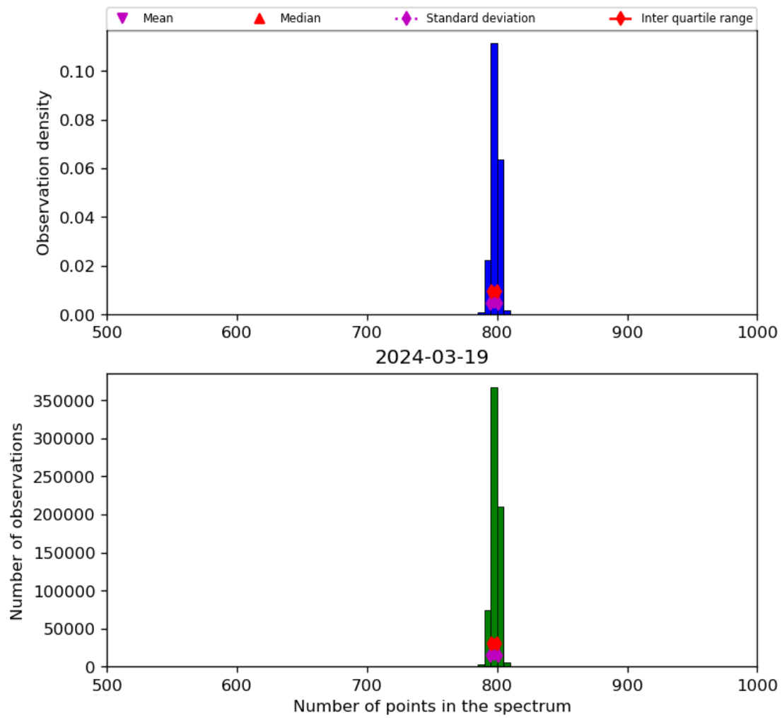
Figure 26: Histogram of “Number of points in the spectrum” for 2024-03-18 to 2024-03-20
