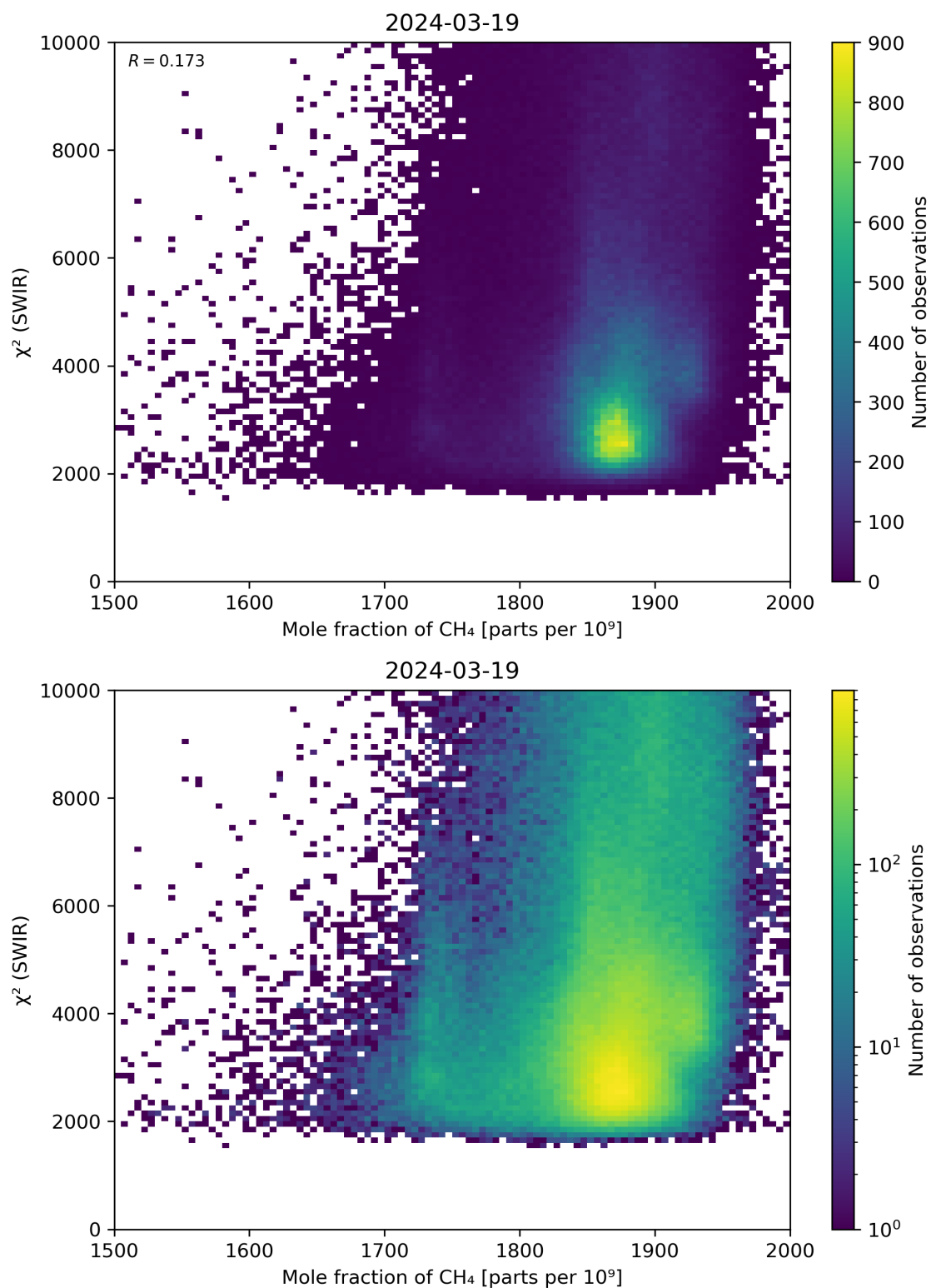
Figure 71: Scatter density plot of “Mole fraction of CH 4 ” against “ \chi^2 (SWIR)” for 2024-03-18 to 2024-03-20.
