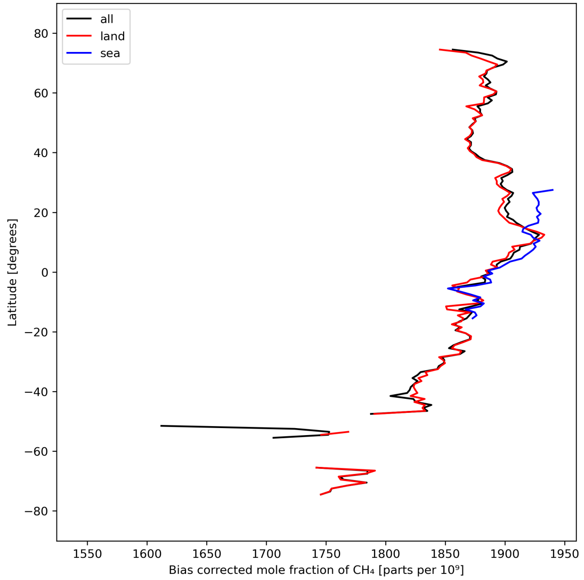
Figure 14: Zonal average of “Bias corrected mole fraction of CH 4 ” for 2024-03-18 to 2024-03-20.
