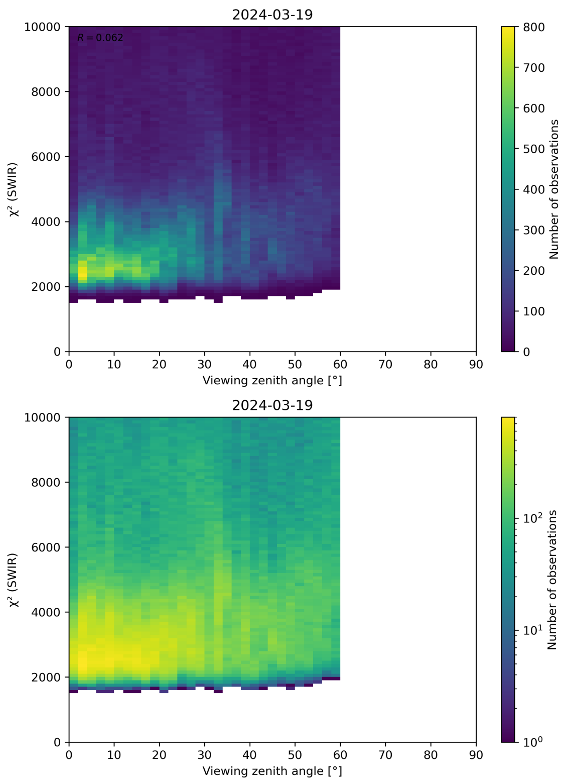
Figure 106: Scatter density plot of “Viewing zenith angle” against “ \chi^2 (SWIR)” for 2024-03-18 to 2024-03-20.
