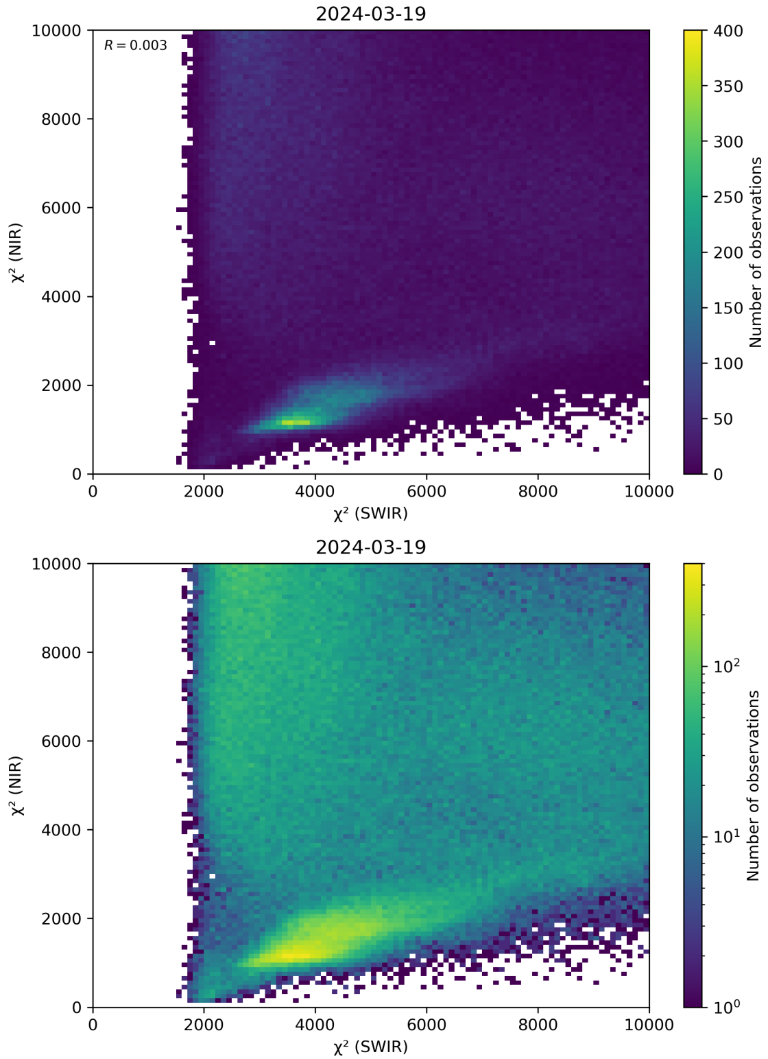
Figure 47: Scatter density plot of “ \chi^2 (SWIR)” against “ \chi^2 (NIR)” for 2024-03-18 to 2024-03-20.
