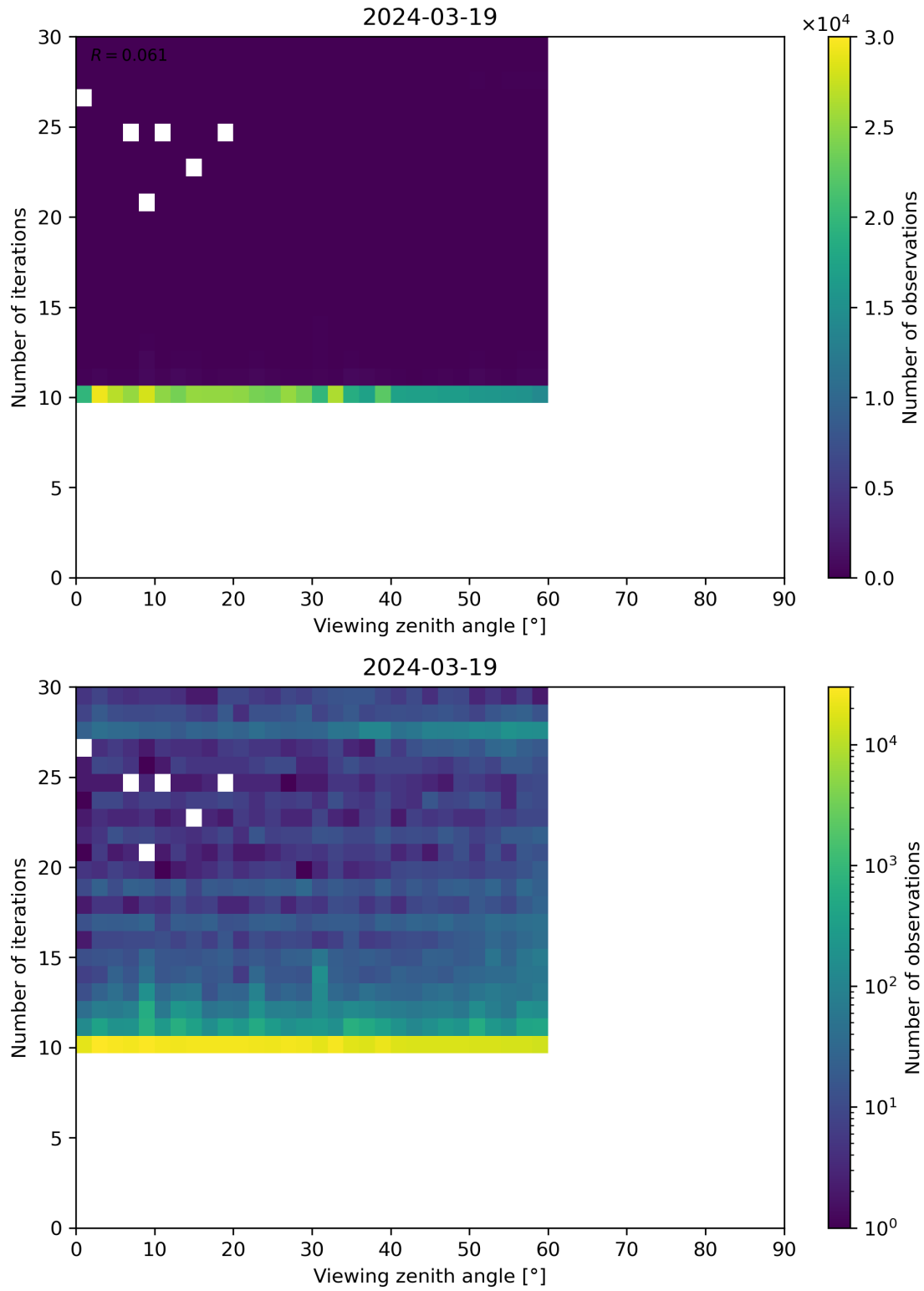
Figure 113: Scatter density plot of “Viewing zenith angle” against “Number of iterations” for 2024-03-18 to 2024-03-20.
