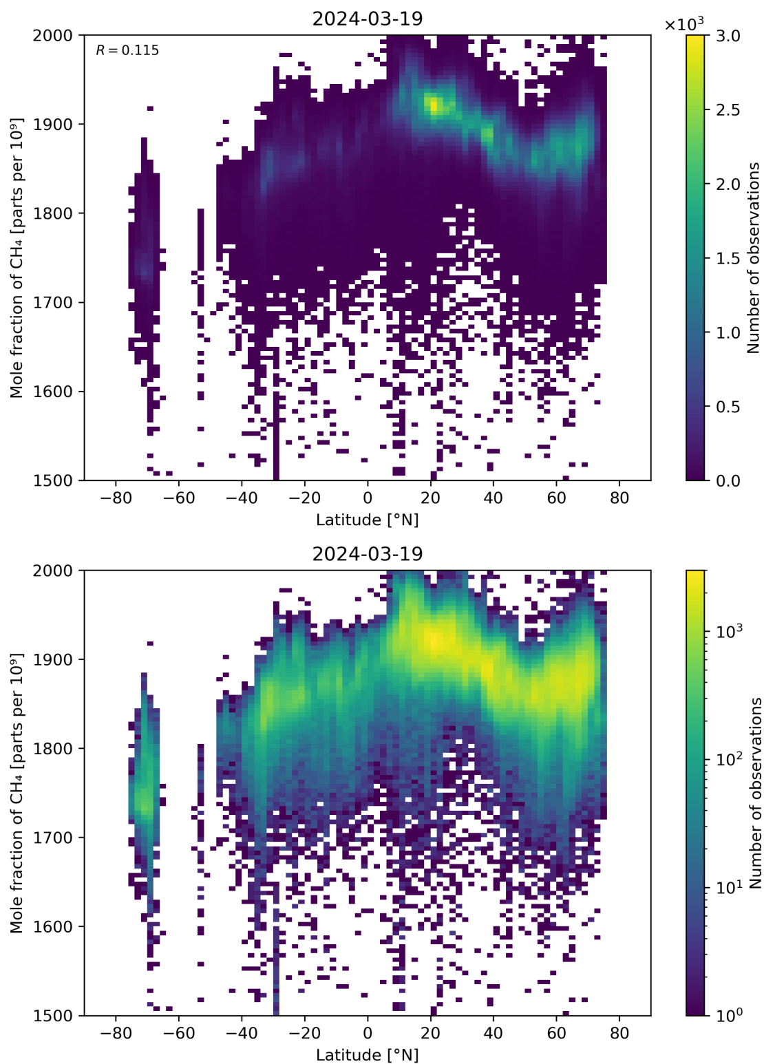
Figure 57: Scatter density plot of “Latitude” against “Mole fraction of \text{CH}_4 ” for 2024-03-18 to 2024-03-20.
