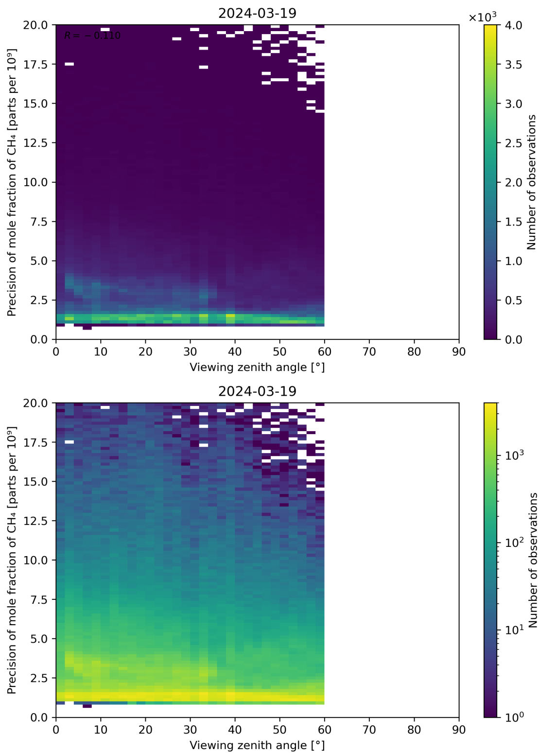
Figure 112: Scatter density plot of “Viewing zenith angle” against “Precision of mole fraction of CH 4 ” for 2024-03-18 to 2024-03-20.
