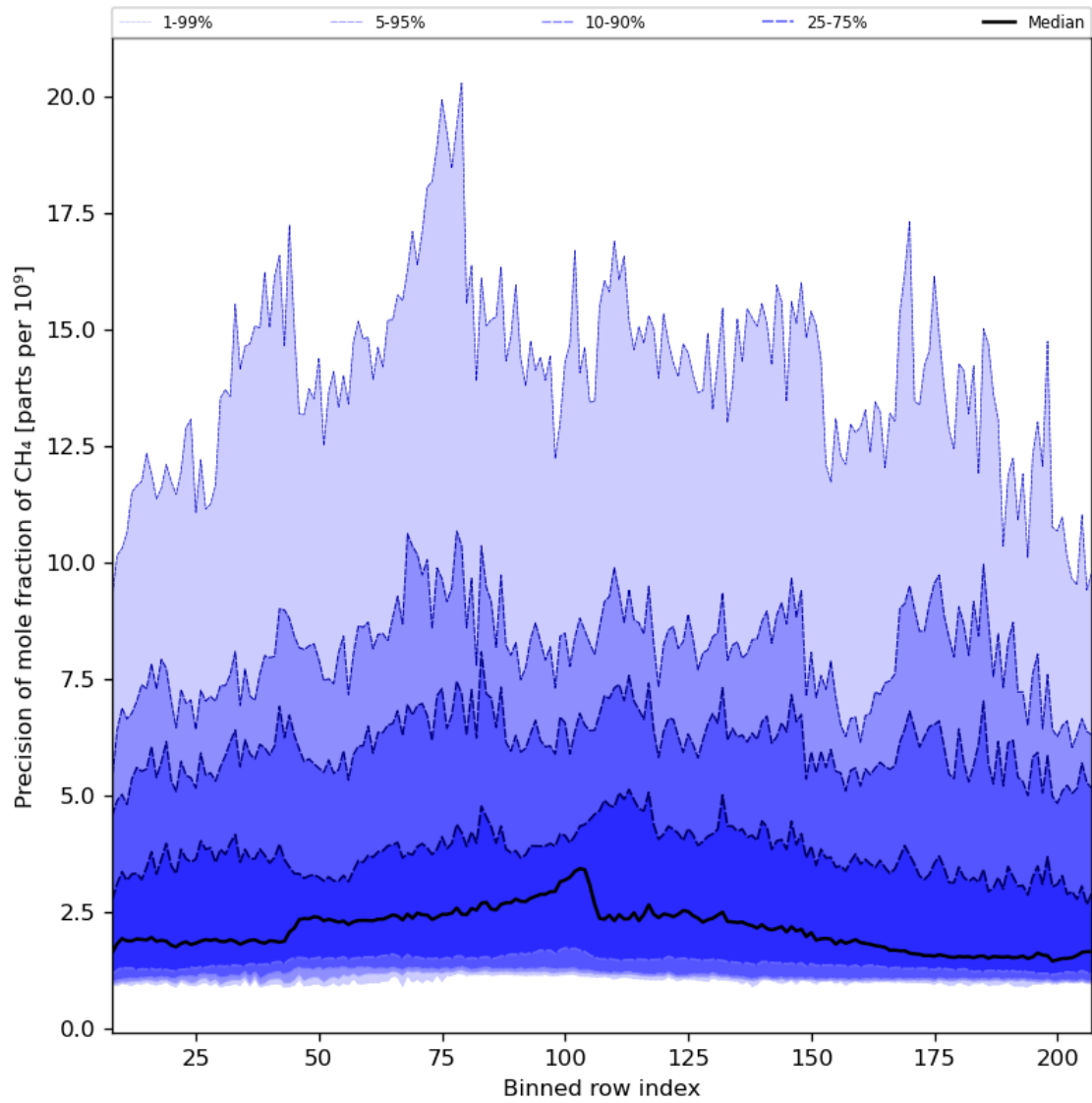
Figure 35: Along track statistics of “Precision of mole fraction of CH 4 ” for 2024-03-18 to 2024-03-20
