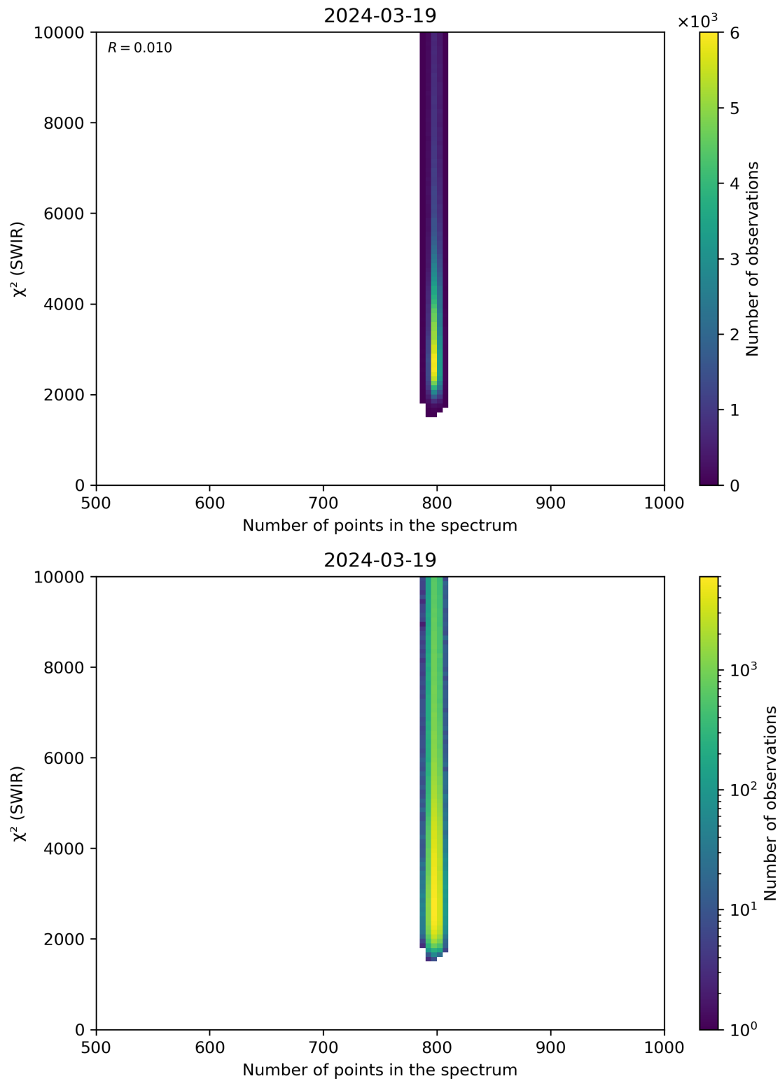
Figure 89: Scatter density plot of “Number of points in the spectrum” against “ \chi^2 (SWIR)” for 2024-03-18 to 2024-03-20.
