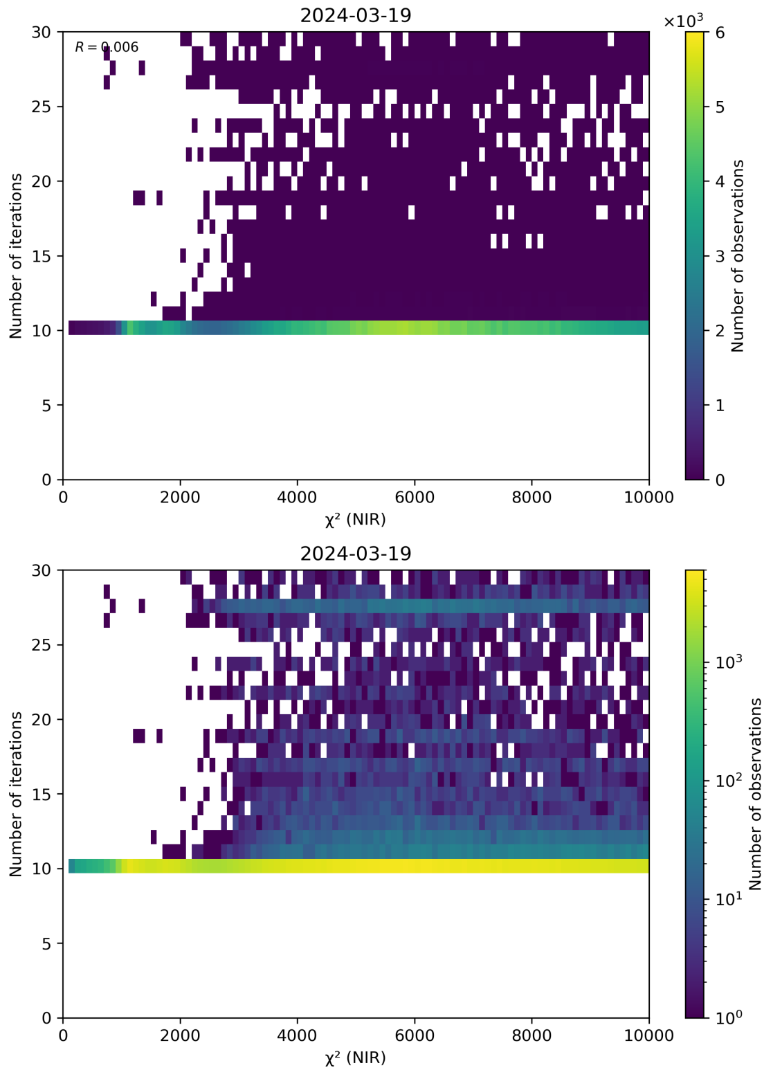
Figure 46: Scatter density plot of “ \chi^2 (NIR)” against “Number of iterations” for 2024-03-18 to 2024-03-20.
