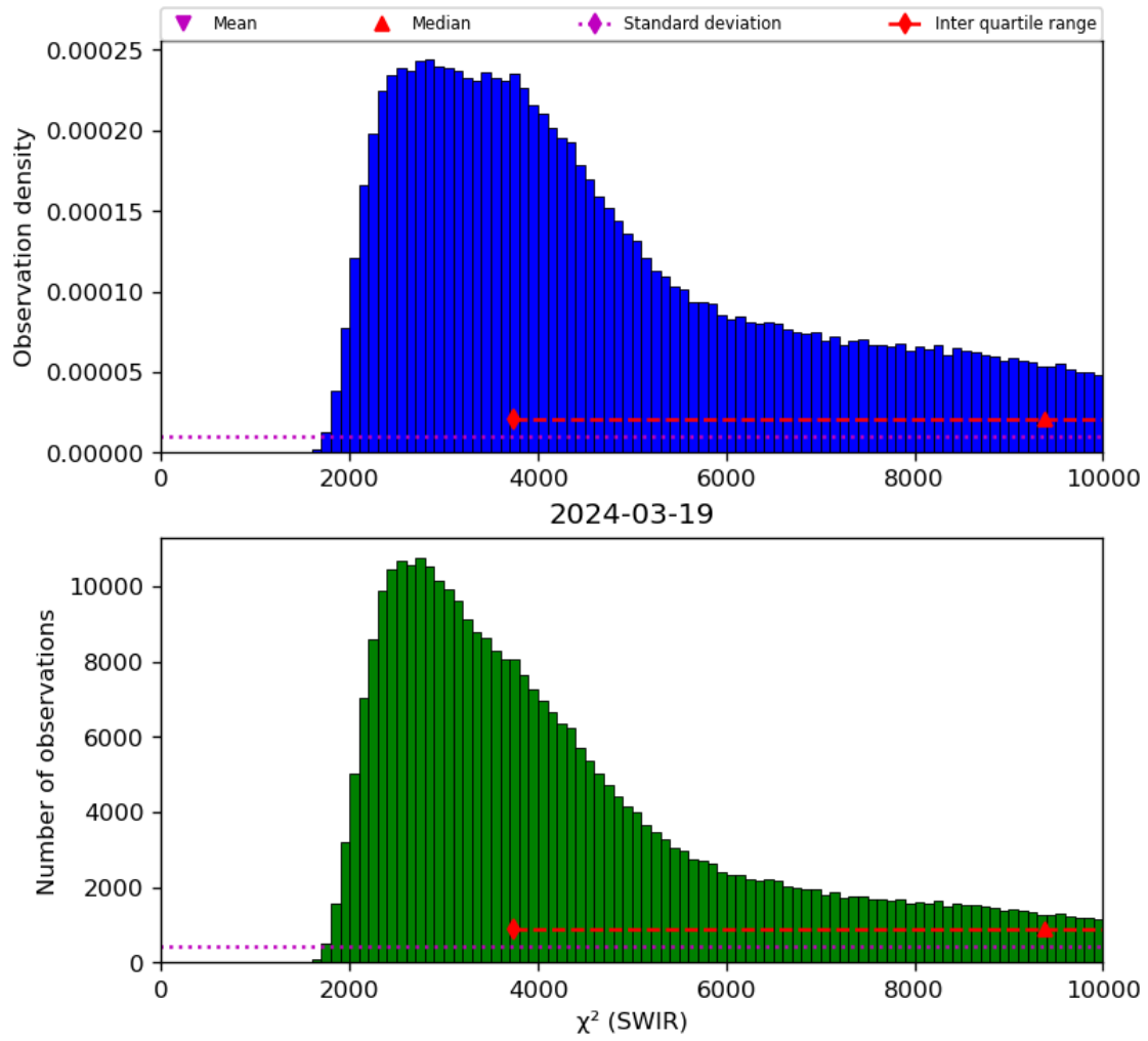
Figure 28: Histogram of “ \chi^2 (SWIR)” for 2024-03-18 to 2024-03-20
