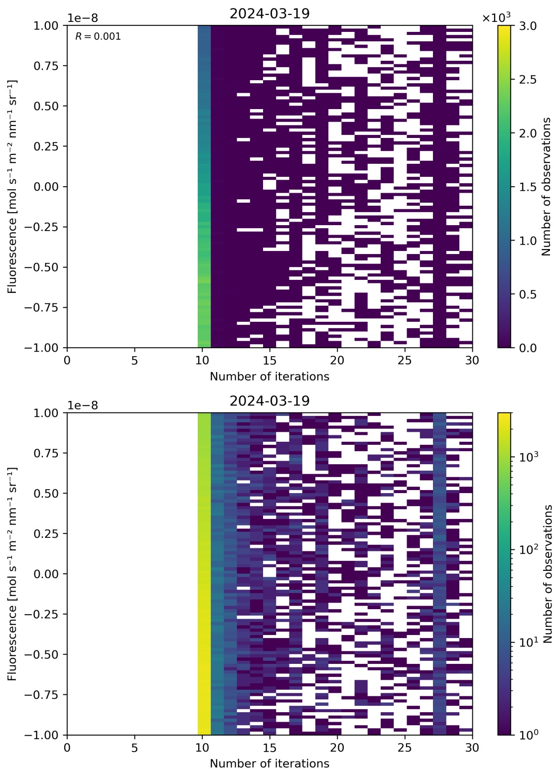
Figure 87: Scatter density plot of “Number of iterations” against “Fluorescence” for 2024-03-18 to 2024-03-20.
