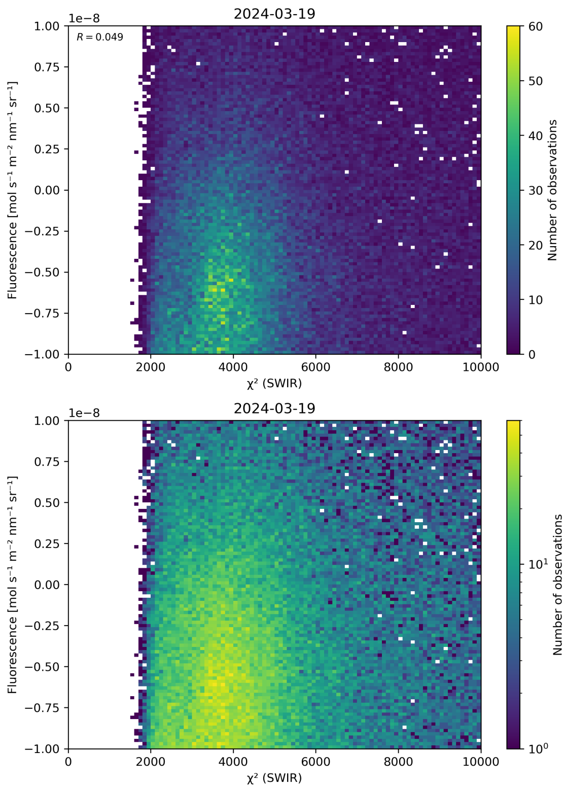
Figure 49: Scatter density plot of “ \chi^2 (SWIR)” against “Fluorescence” for 2024-03-18 to 2024-03-20.
