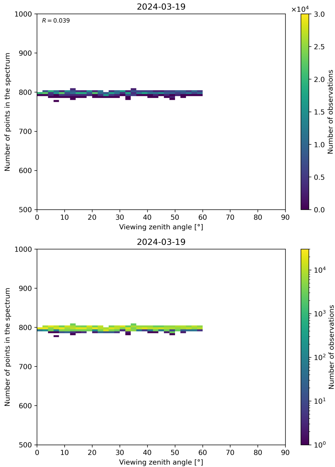
Figure 114: Scatter density plot of “Viewing zenith angle” against “Number of points in the spectrum” for 2024-03-18 to 2024-03-20.
