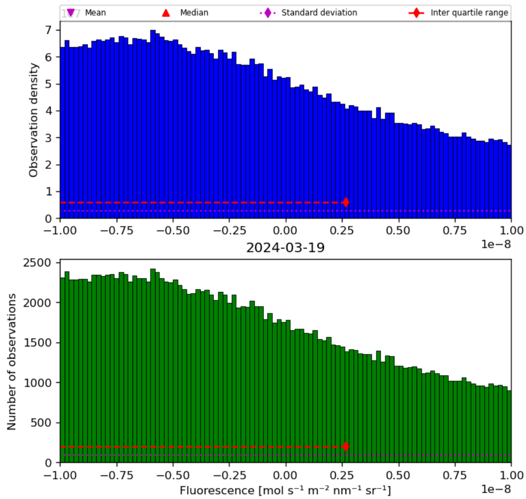
Figure 32: Histogram of “Fluorescence” for 2024-03-18 to 2024-03-20
