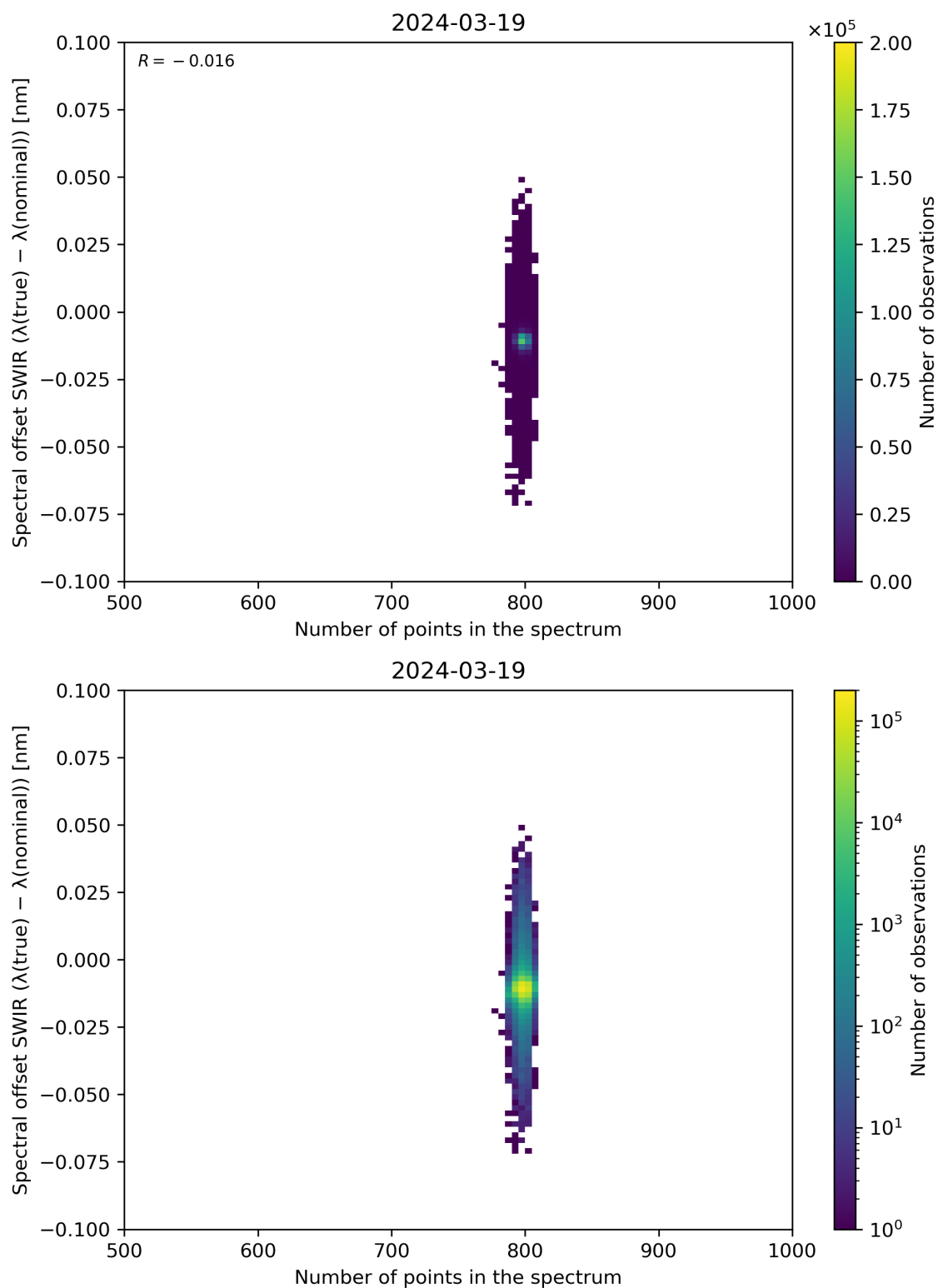
Figure 93: Scatter density plot of “Number of points in the spectrum” against “Spectral offset SWIR ( \lambda(\text{true}) - \lambda(\text{nominal}) )” for 2024-03-18 to 2024-03-20.
