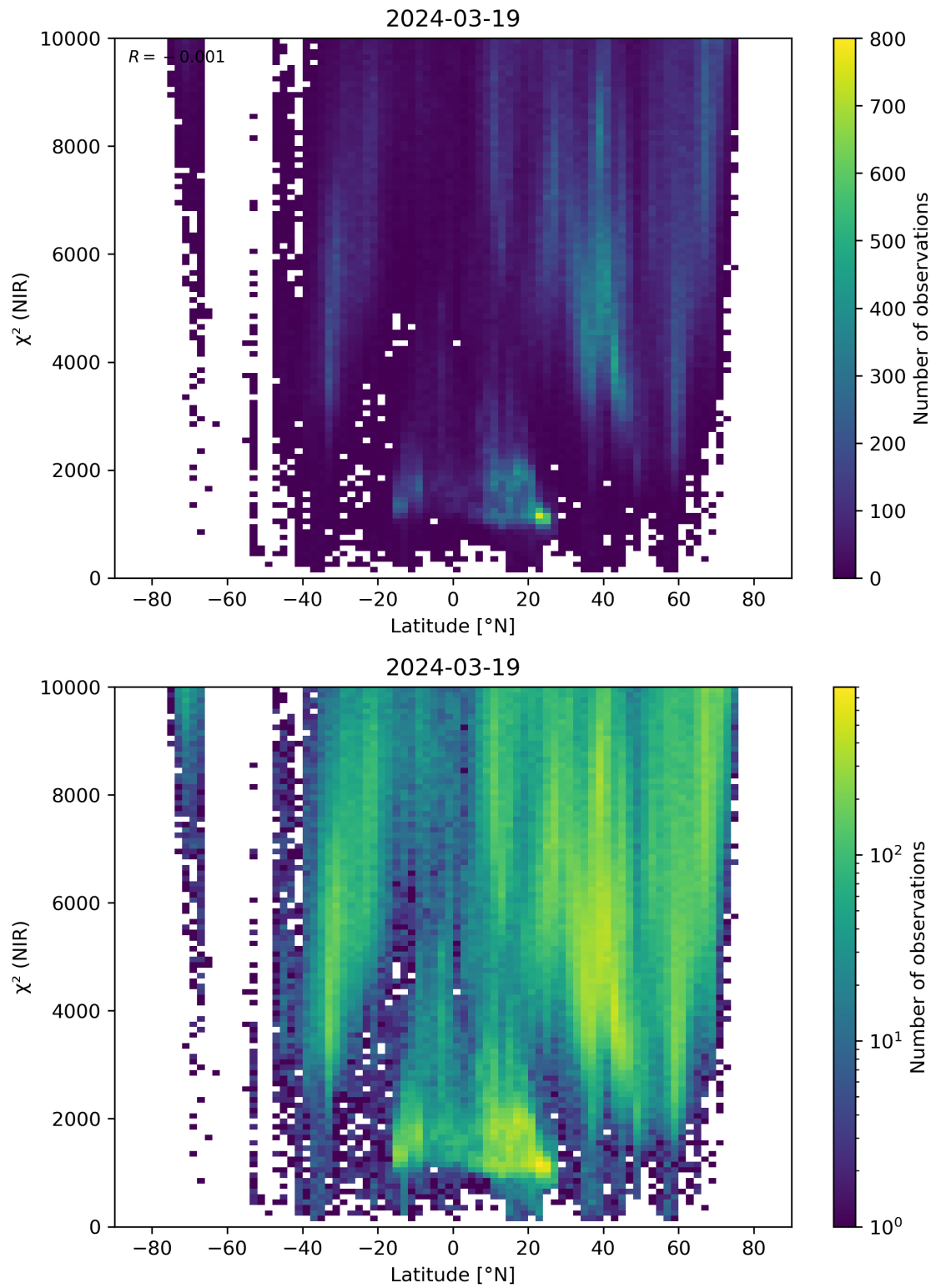
Figure 53: Scatter density plot of “Latitude” against “ \chi^2 (NIR)” for 2024-03-18 to 2024-03-20.
