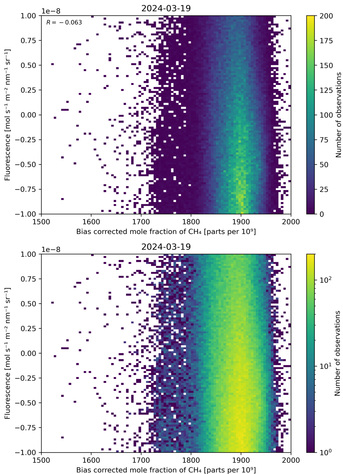
Figure 66: Scatter density plot of “Bias corrected mole fraction of \text{CH}_4 ” against “Fluorescence” for 2024-03-18 to 2024-03-20.
