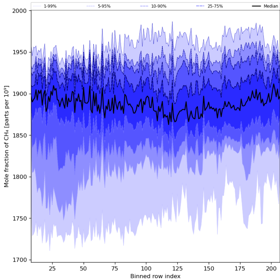
Figure 34: Along track statistics of “Mole fraction of CH 4 ” for 2024-03-18 to 2024-03-20
