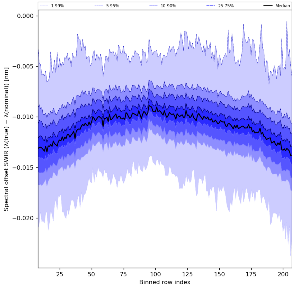
Figure 38: Along track statistics of “Spectral offset SWIR ( \lambda(\text{true}) - \lambda(\text{nominal}) )” for 2024-03-18 to 2024-03-20
