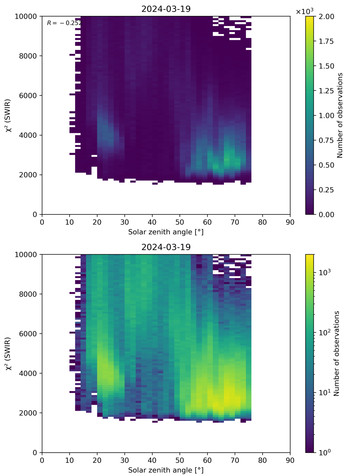
Figure 95: Scatter density plot of “Solar zenith angle” against “ \chi^2 (SWIR)” for 2024-03-18 to 2024-03-20.
