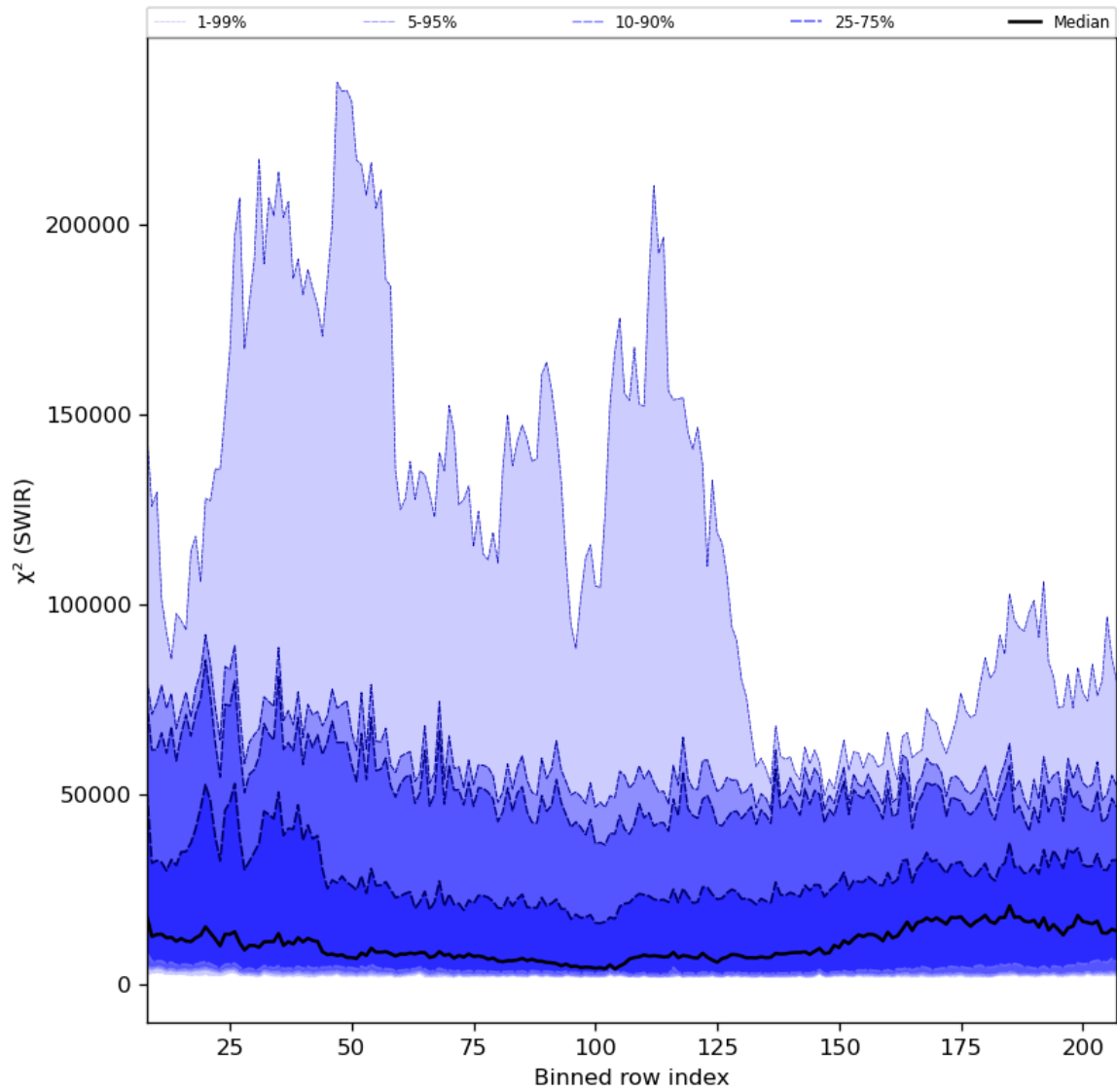
Figure 39: Along track statistics of “ \chi^2 (SWIR)” for 2024-03-18 to 2024-03-20
