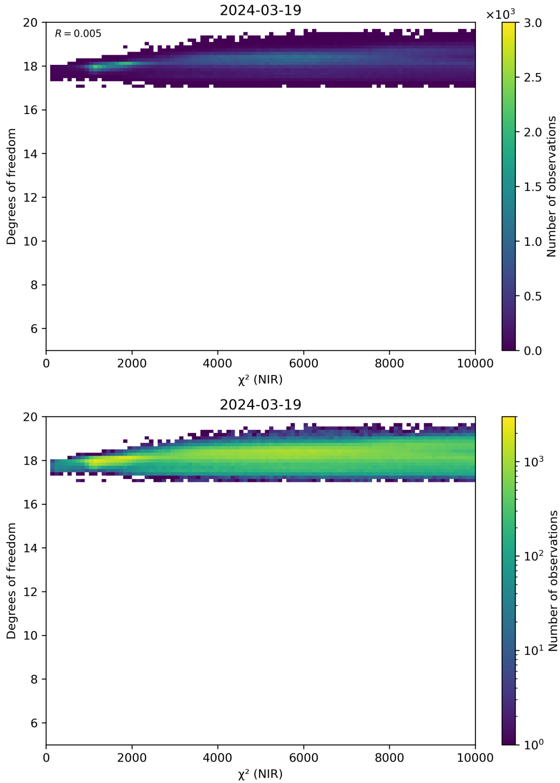
Figure 44: Scatter density plot of “ \chi^2 (NIR)” against “Degrees of freedom” for 2024-03-18 to 2024-03-20.
