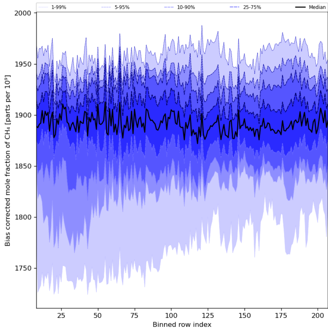
Figure 36: Along track statistics of “Bias corrected mole fraction of CH 4 ” for 2024-03-18 to 2024-03-20
