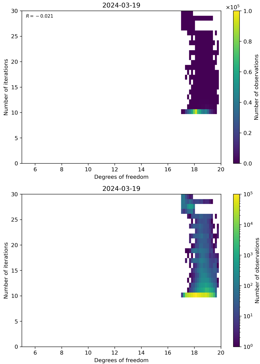
Figure 52: Scatter density plot of “Degrees of freedom” against “Number of iterations” for 2024-03-18 to 2024-03-20.
