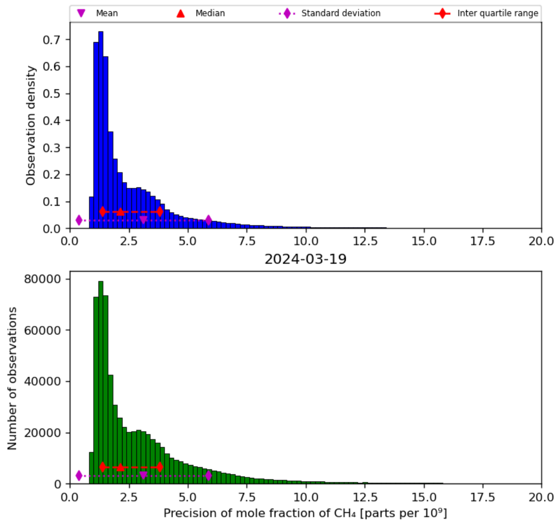
Figure 24: Histogram of “Precision of mole fraction of CH 4 ” for 2024-03-18 to 2024-03-20
