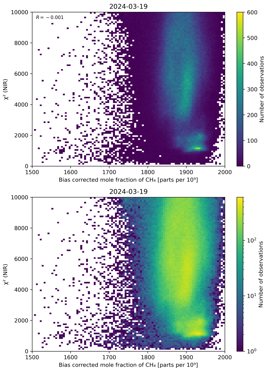
Figure 63: Scatter density plot of “Bias corrected mole fraction of CH 4 ” against “ \chi^2 (NIR)” for 2024-03-18 to 2024-03-20.
