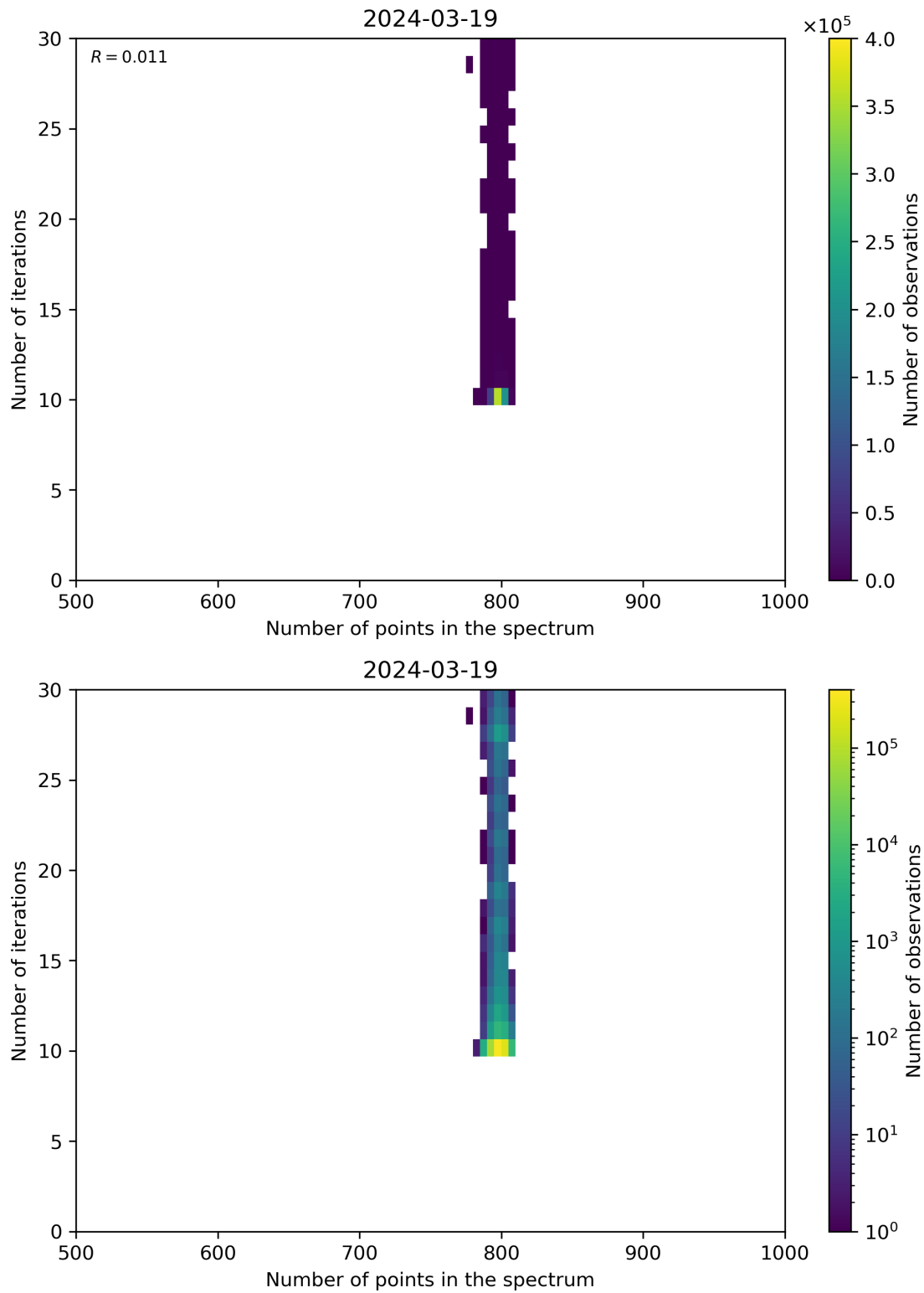
Figure 92: Scatter density plot of “Number of points in the spectrum” against “Number of iterations” for 2024-03-18 to 2024-03-20.
