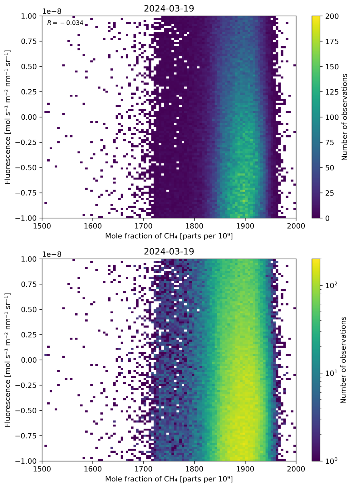
Figure 73: Scatter density plot of “Mole fraction of \text{CH}_4 ” against “Fluorescence” for 2024-03-18 to 2024-03-20.
