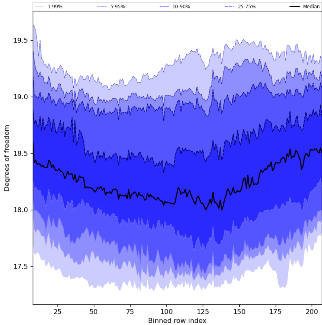
Figure 41: Along track statistics of “Degrees of freedom” for 2024-03-18 to 2024-03-20
