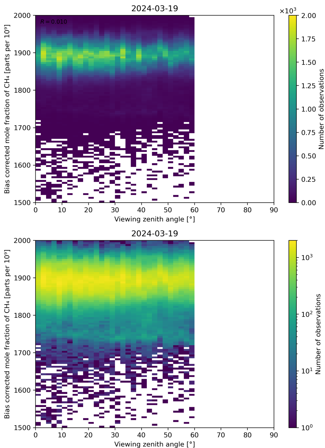
Figure 111: Scatter density plot of “Viewing zenith angle” against “Bias corrected mole fraction of CH 4 ” for 2024-03-18 to 2024-03-20.
