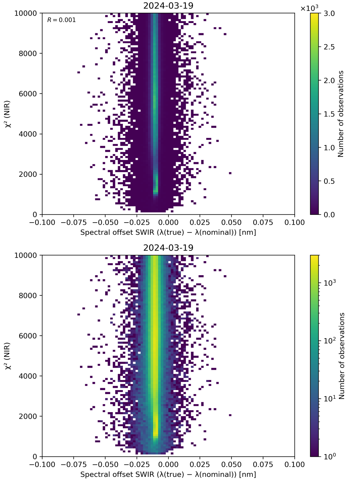
Figure 117: Scatter density plot of “Spectral offset SWIR ( \lambda(\text{true}) - \lambda(\text{nominal}) )” against “ \chi^2 (NIR)” for 2024-03-18 to 2024-03-20.
