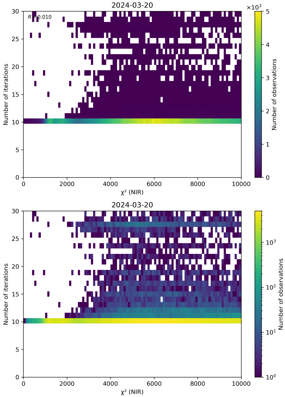
Figure 46: Scatter density plot of “ \chi^2 (NIR)” against “Number of iterations” for 2024-03-20 to 2024-03-21.
