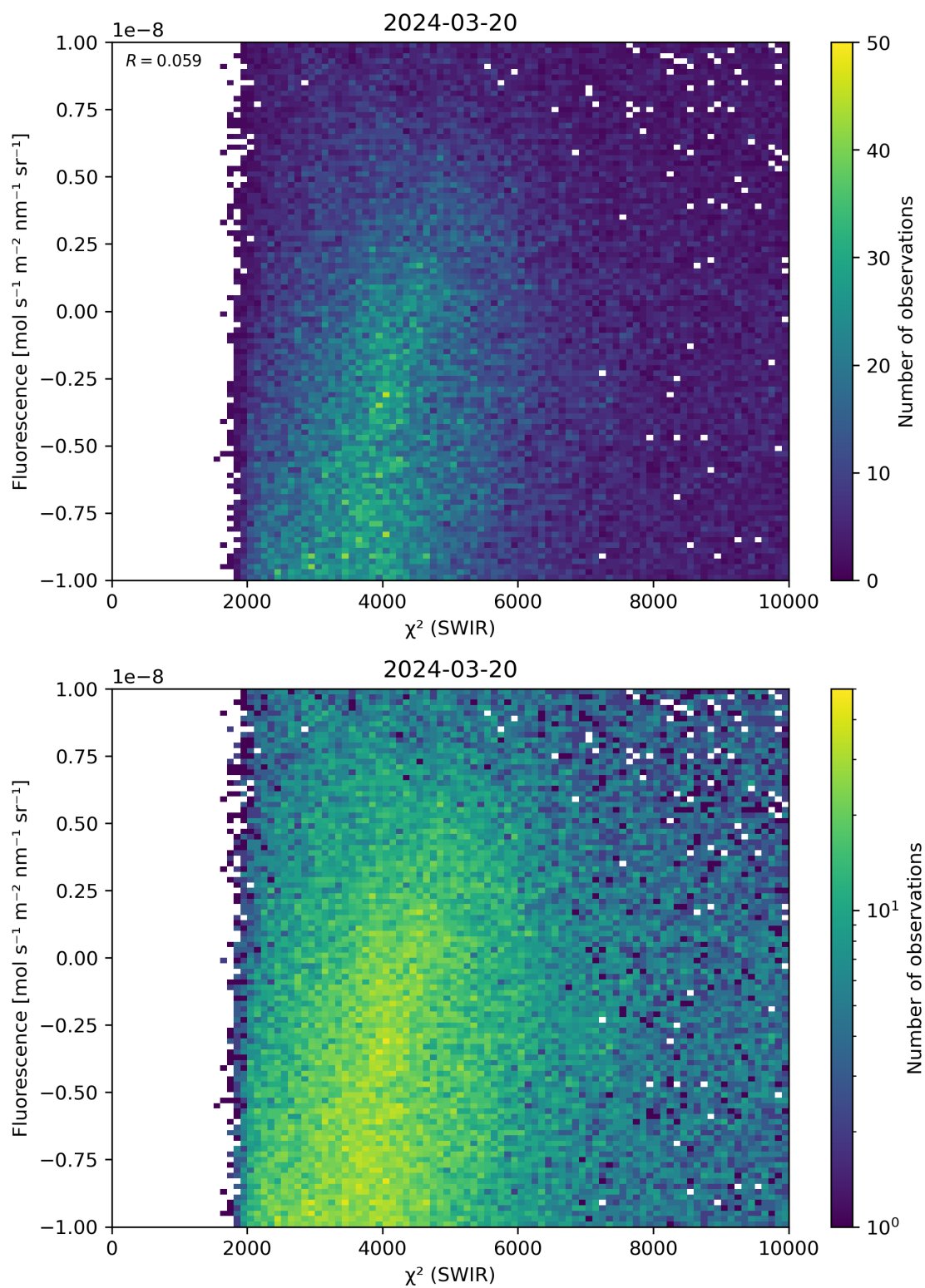
Figure 49: Scatter density plot of “ \chi^2 (SWIR)” against “Fluorescence” for 2024-03-20 to 2024-03-21.
