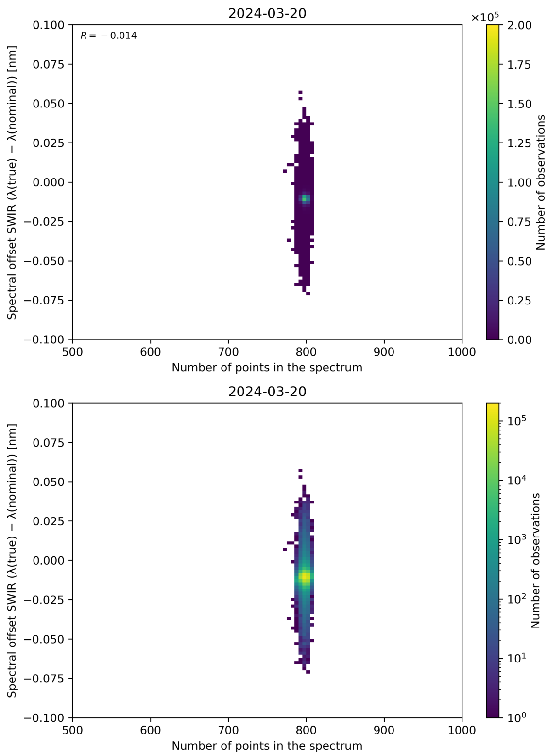
Figure 93: Scatter density plot of “Number of points in the spectrum” against “Spectral offset SWIR ( \lambda(\text{true}) - \lambda(\text{nominal}) )” for 2024-03-20 to 2024-03-21.
