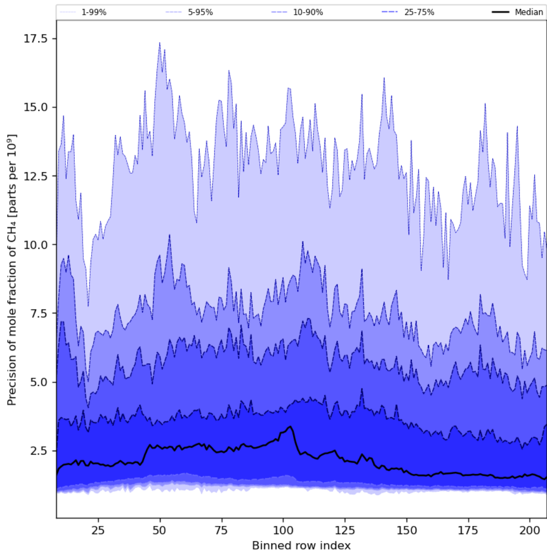
Figure 35: Along track statistics of “Precision of mole fraction of CH 4 ” for 2024-03-20 to 2024-03-21
