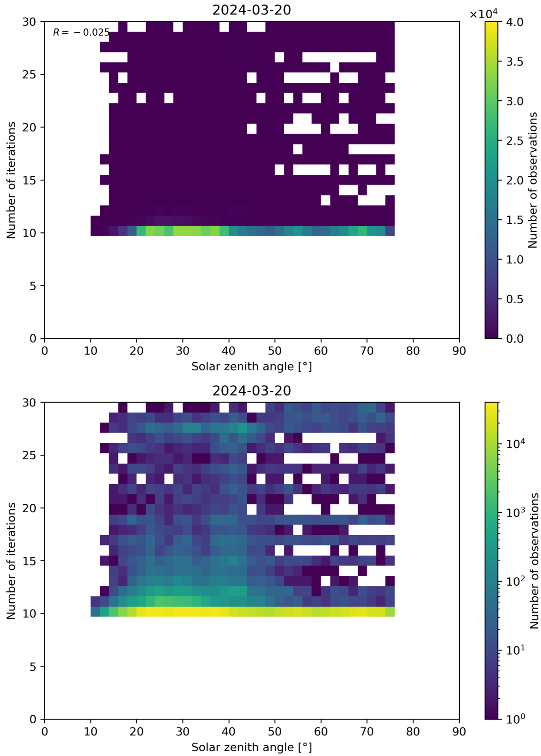
Figure 102: Scatter density plot of “Solar zenith angle” against “Number of iterations” for 2024-03-20 to 2024-03-21.
