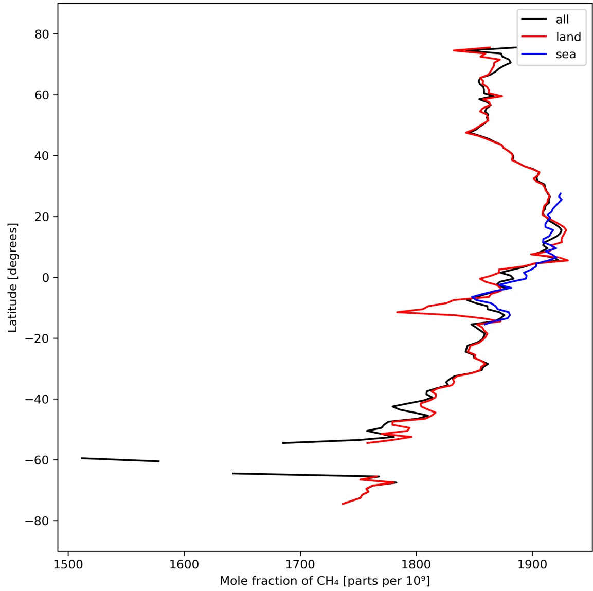
Figure 12: Zonal average of “Mole fraction of \text{CH}_4 ” for 2024-03-20 to 2024-03-21.
