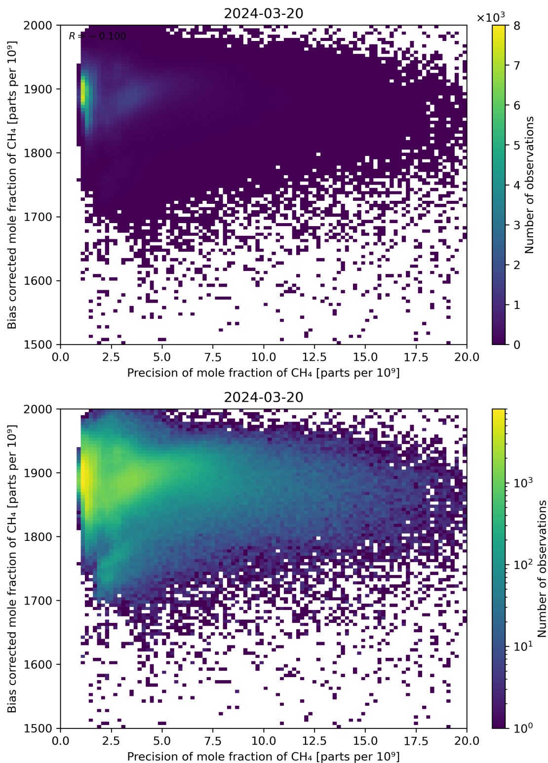
Figure 82: Scatter density plot of “Precision of mole fraction of CH 4 ” against “Bias corrected mole fraction of CH 4 ” for 2024-03-20 to 2024-03-21.
