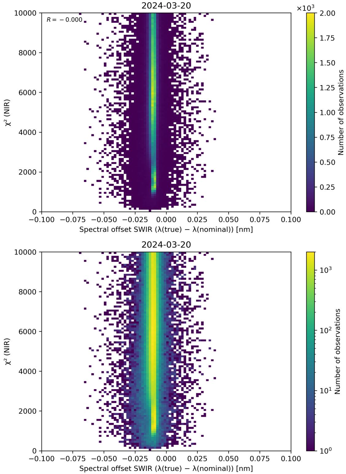
Figure 117: Scatter density plot of “Spectral offset SWIR ( \lambda(\text{true}) - \lambda(\text{nominal}) )” against “ \chi^2 (NIR)” for 2024-03-20 to 2024-03-21.
