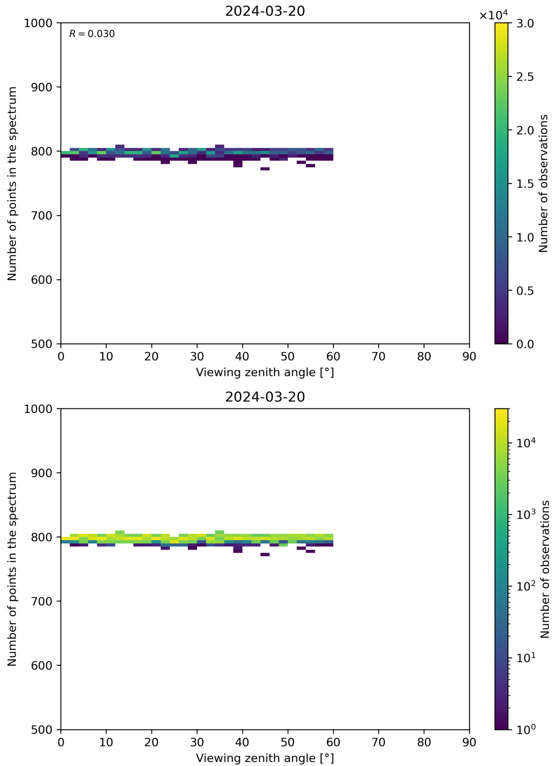
Figure 114: Scatter density plot of “Viewing zenith angle” against “Number of points in the spectrum” for 2024-03-20 to 2024-03-21.
