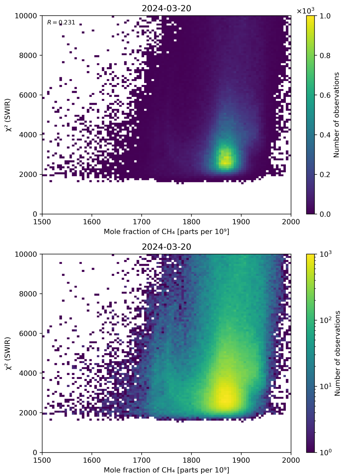
Figure 71: Scatter density plot of “Mole fraction of \text{CH}_4 ” against “ \chi^2 (SWIR)” for 2024-03-20 to 2024-03-21.
