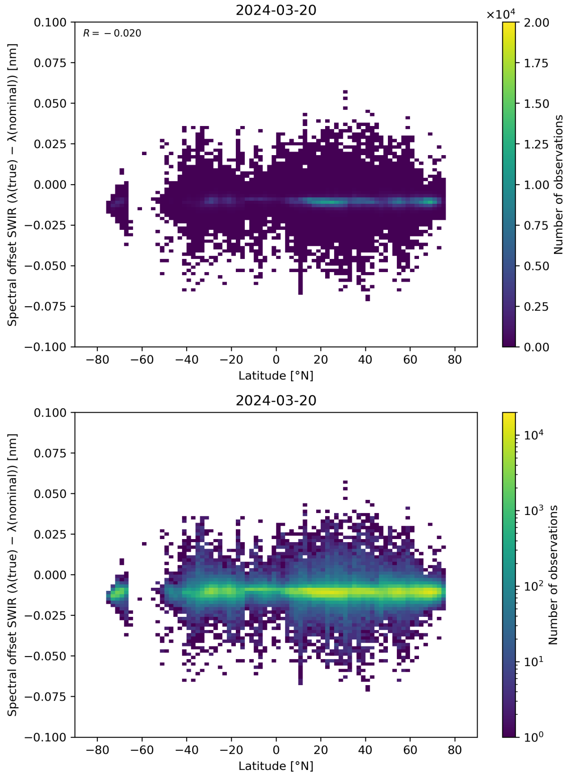
Figure 62: Scatter density plot of “Latitude” against “Spectral offset SWIR ( \lambda(\text{true}) - \lambda(\text{nominal}) )” for 2024-03-20 to 2024-03-21.
