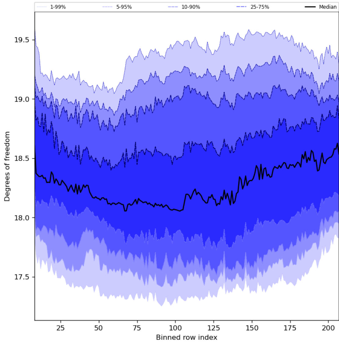
Figure 41: Along track statistics of “Degrees of freedom” for 2024-03-20 to 2024-03-21
