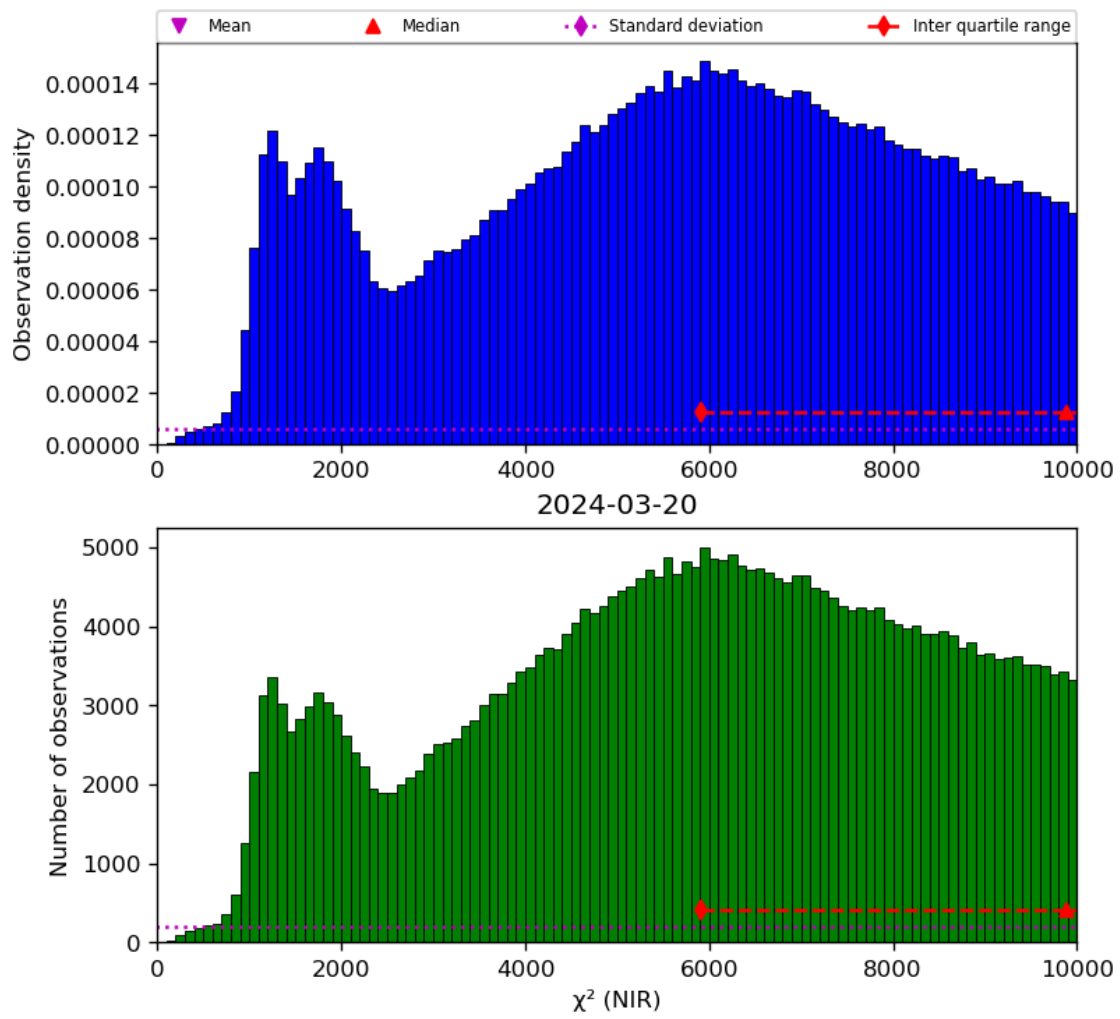
Figure 29: Histogram of “ \chi^2 (NIR)” for 2024-03-20 to 2024-03-21
