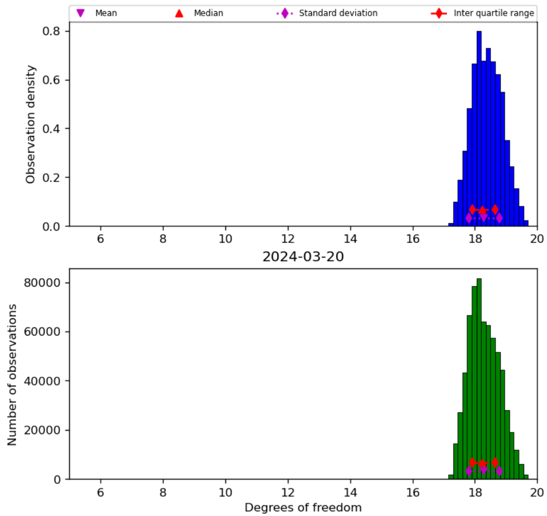
Figure 30: Histogram of “Degrees of freedom” for 2024-03-20 to 2024-03-21
