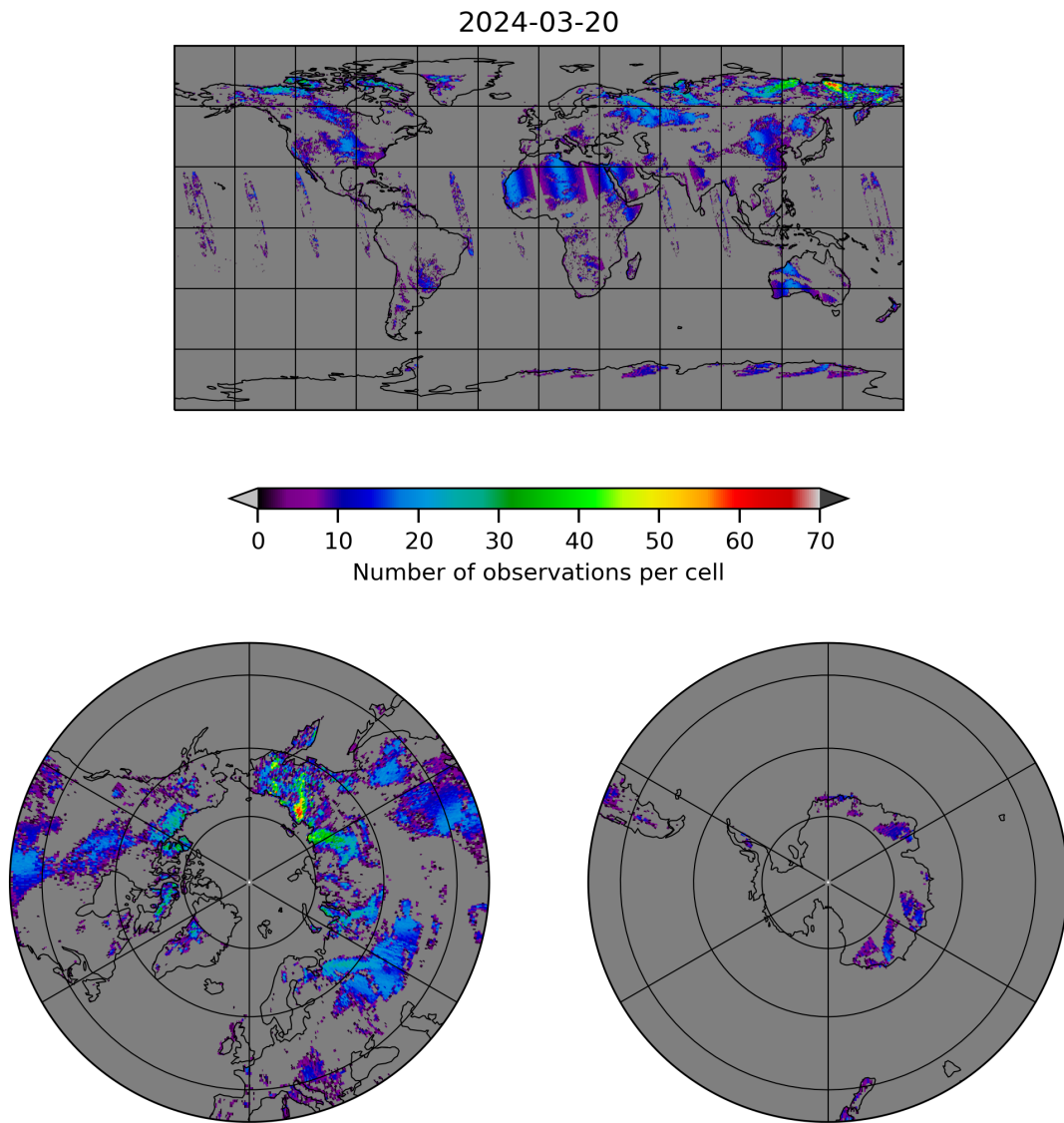
Figure 10: Map of the number of observations for 2024-03-20 to 2024-03-21
