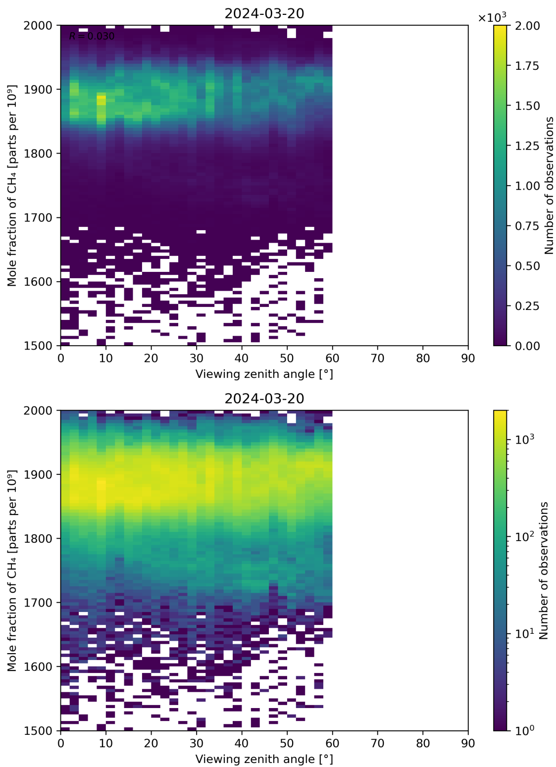
Figure 110: Scatter density plot of “Viewing zenith angle” against “Mole fraction of CH 4 ” for 2024-03-20 to 2024-03-21.
