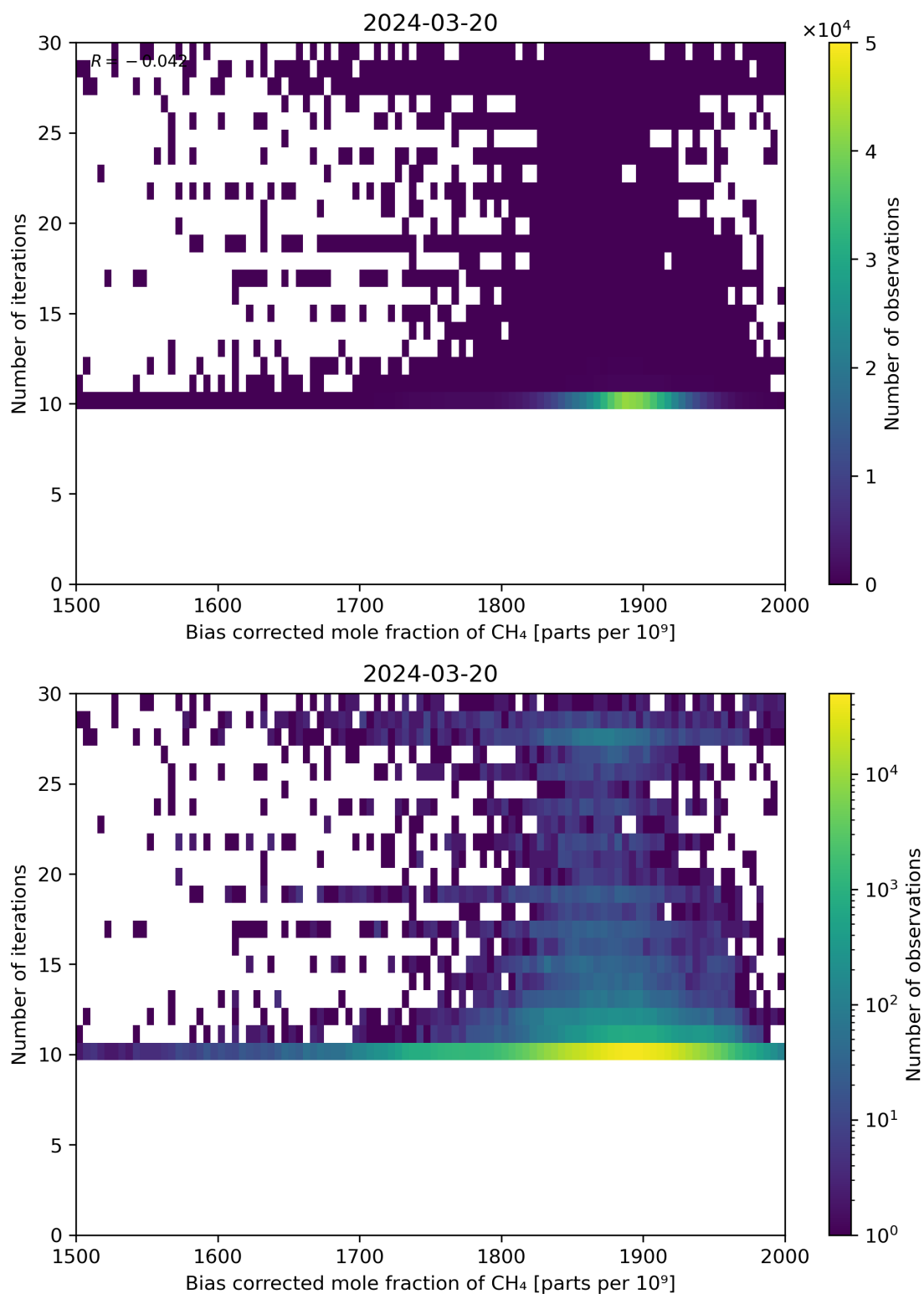
Figure 67: Scatter density plot of “Bias corrected mole fraction of CH 4 ” against “Number of iterations” for 2024-03-20 to 2024-03-21.
