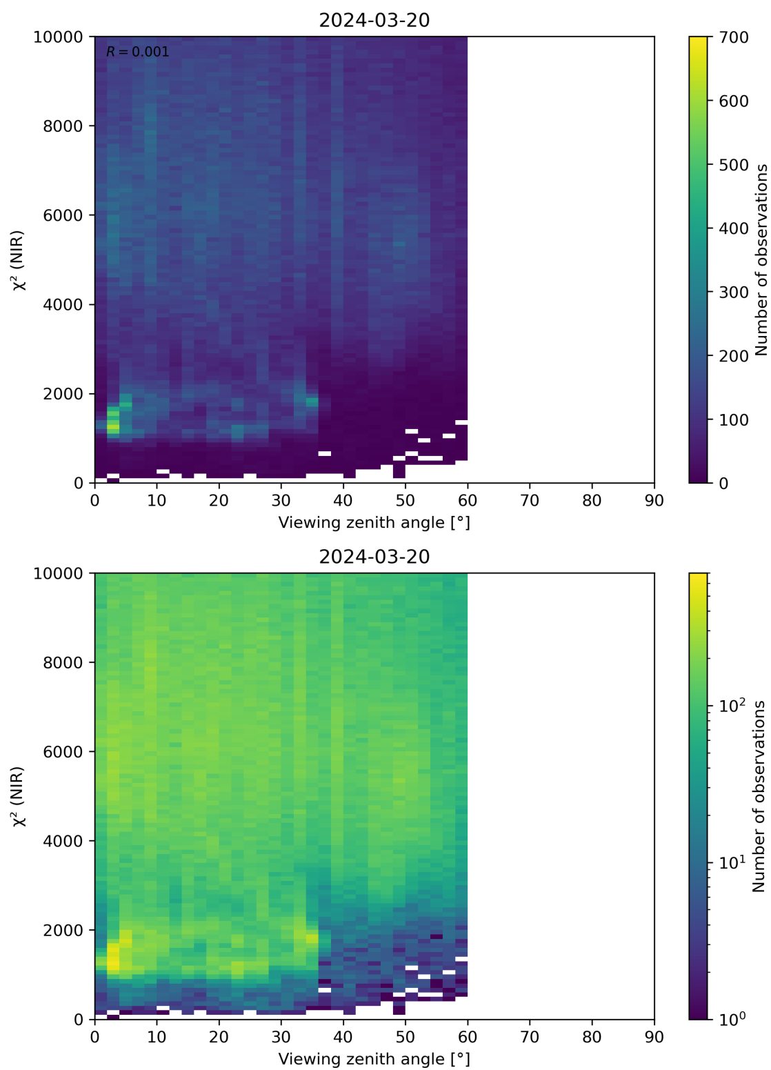
Figure 105: Scatter density plot of “Viewing zenith angle” against “ \chi^2 (NIR)” for 2024-03-20 to 2024-03-21.
