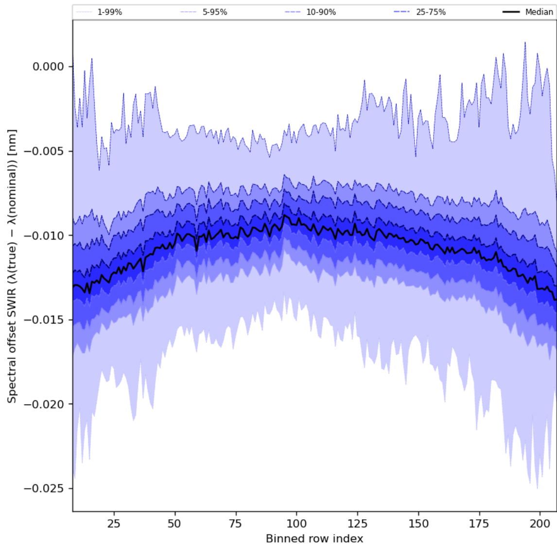
Figure 38: Along track statistics of “Spectral offset SWIR ( \lambda(\text{true}) - \lambda(\text{nominal}) )” for 2024-03-20 to 2024-03-21
