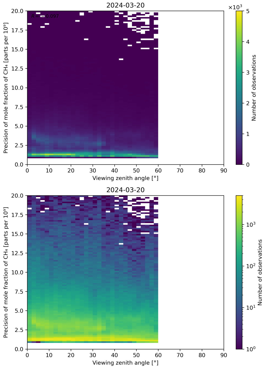
Figure 112: Scatter density plot of “Viewing zenith angle” against “Precision of mole fraction of CH 4 ” for 2024-03-20 to 2024-03-21.
