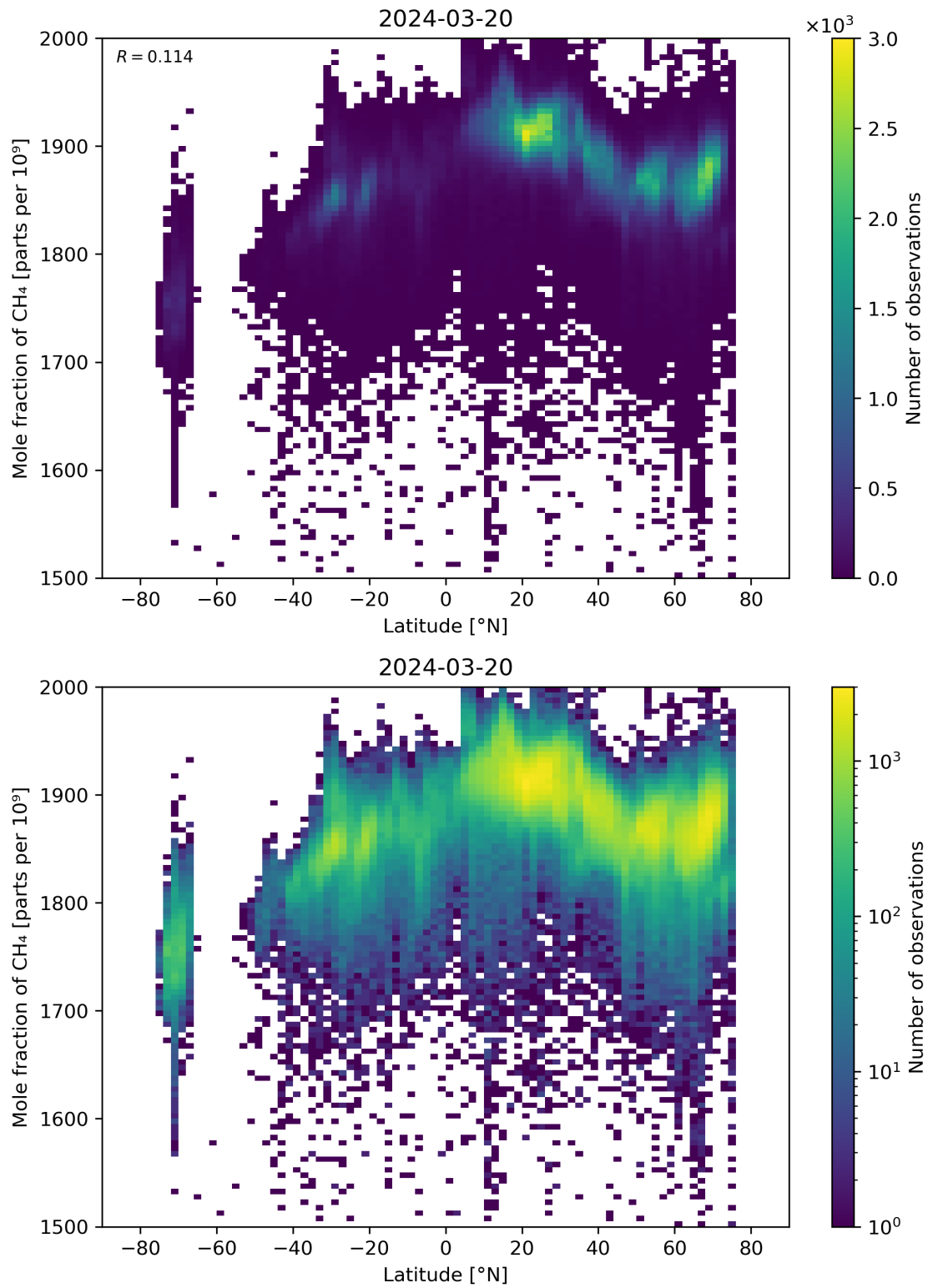
Figure 57: Scatter density plot of “Latitude” against “Mole fraction of \text{CH}_4 ” for 2024-03-20 to 2024-03-21.
