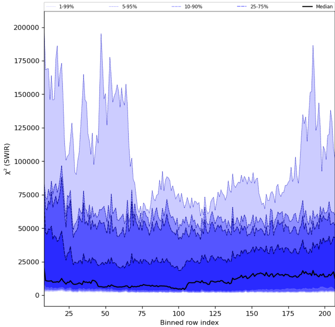
Figure 39: Along track statistics of “ \chi^2 (SWIR)” for 2024-03-20 to 2024-03-21
