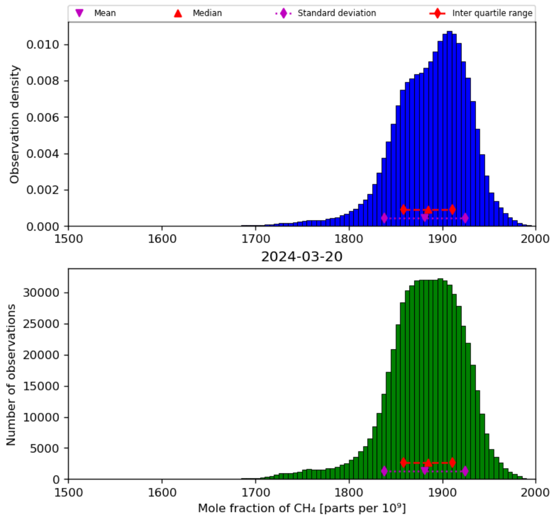
Figure 23: Histogram of “Mole fraction of CH 4 ” for 2024-03-20 to 2024-03-21
