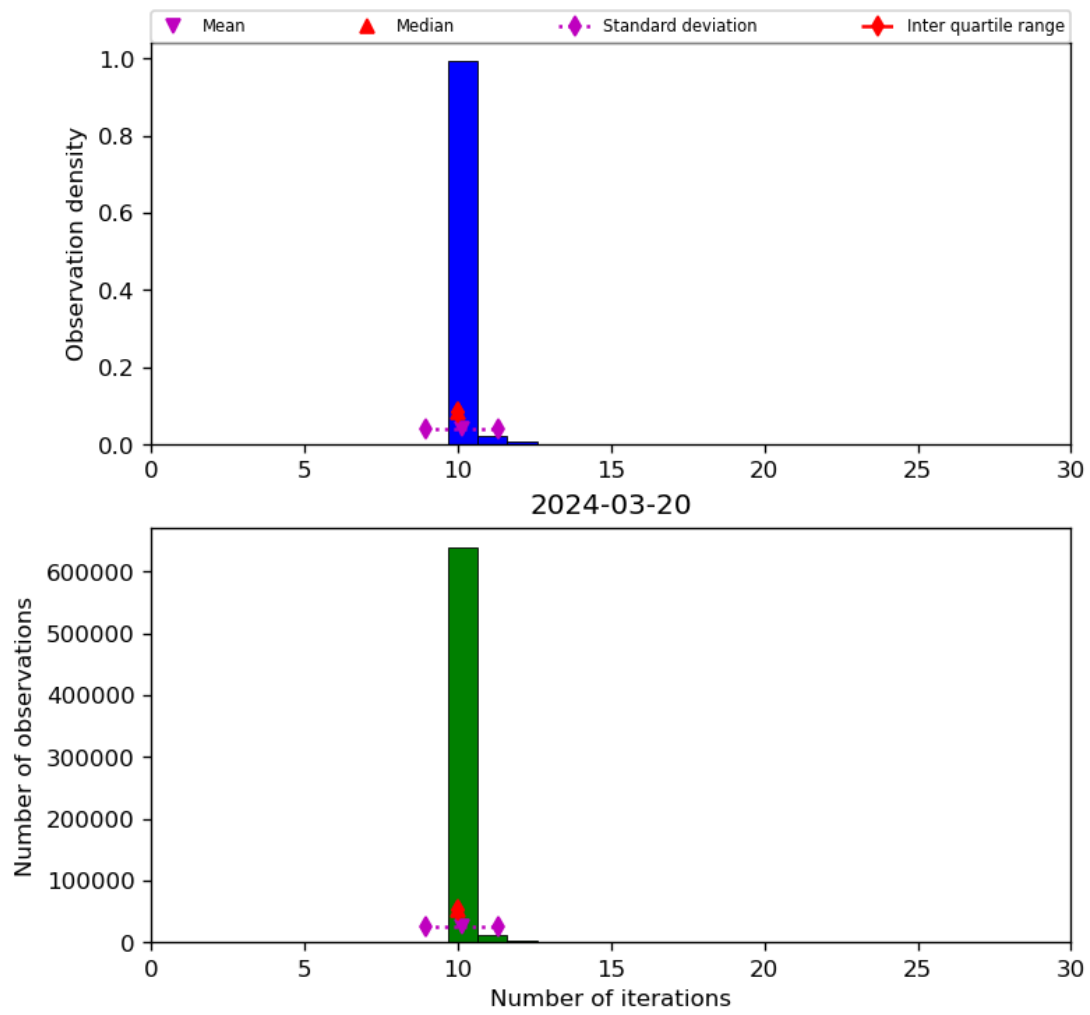
Figure 31: Histogram of “Number of iterations” for 2024-03-20 to 2024-03-21
