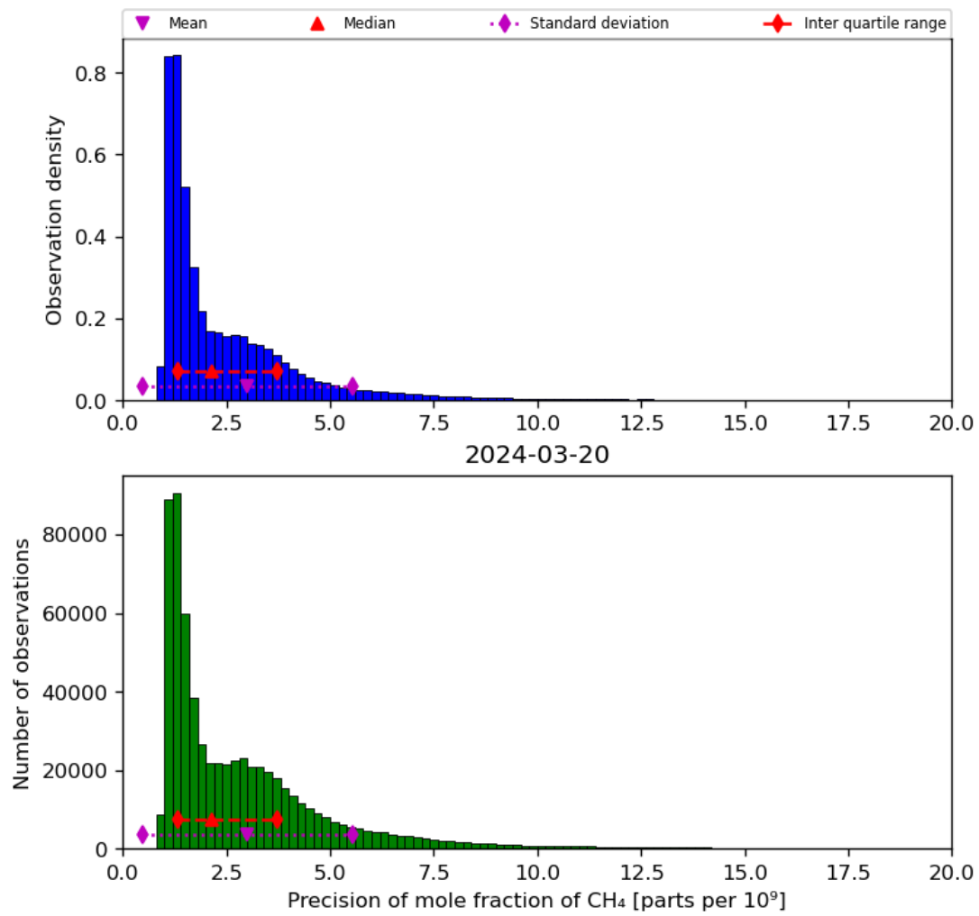
Figure 24: Histogram of “Precision of mole fraction of CH 4 ” for 2024-03-20 to 2024-03-21
