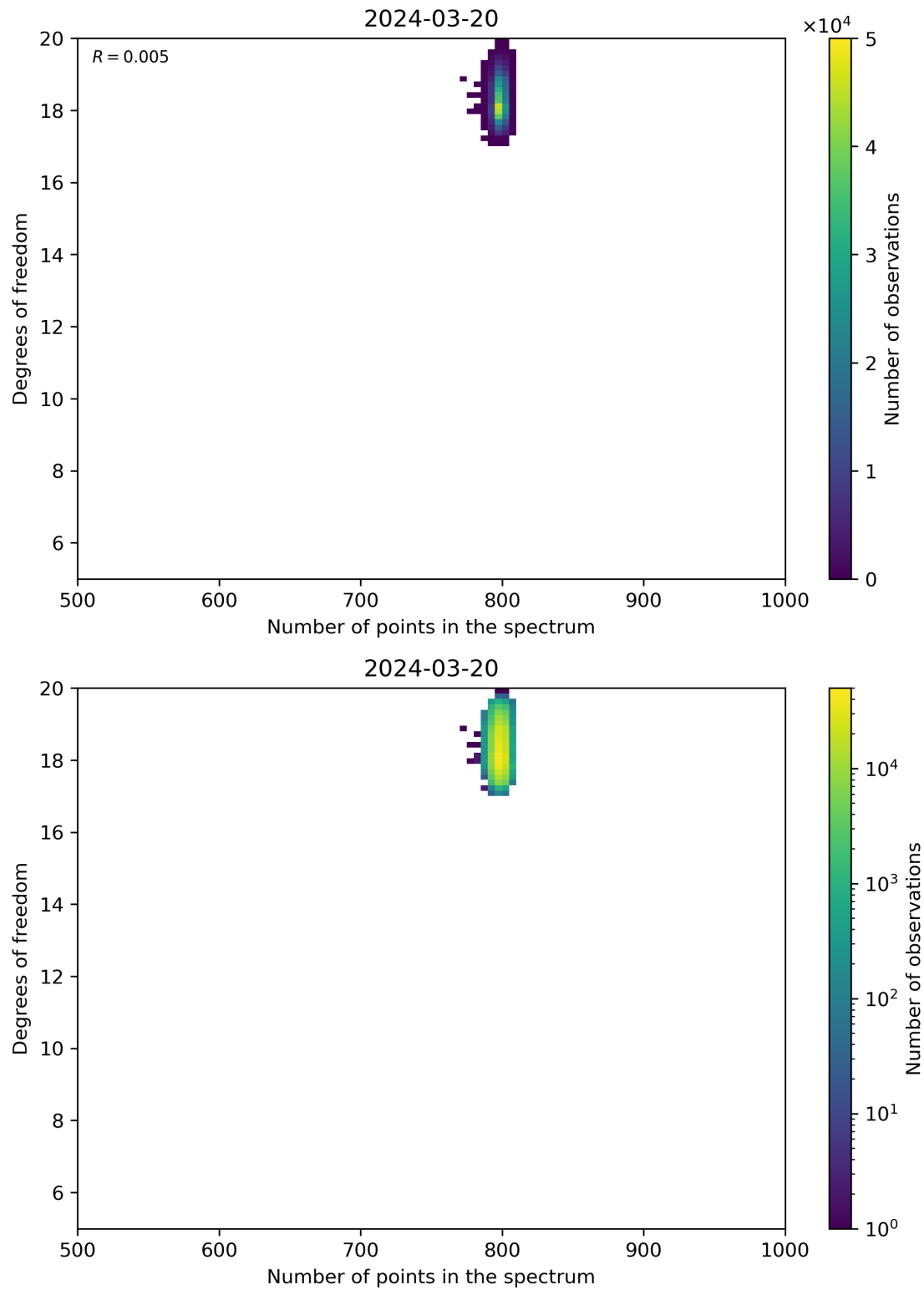
Figure 90: Scatter density plot of “Number of points in the spectrum” against “Degrees of freedom” for 2024-03-20 to 2024-03-21.
