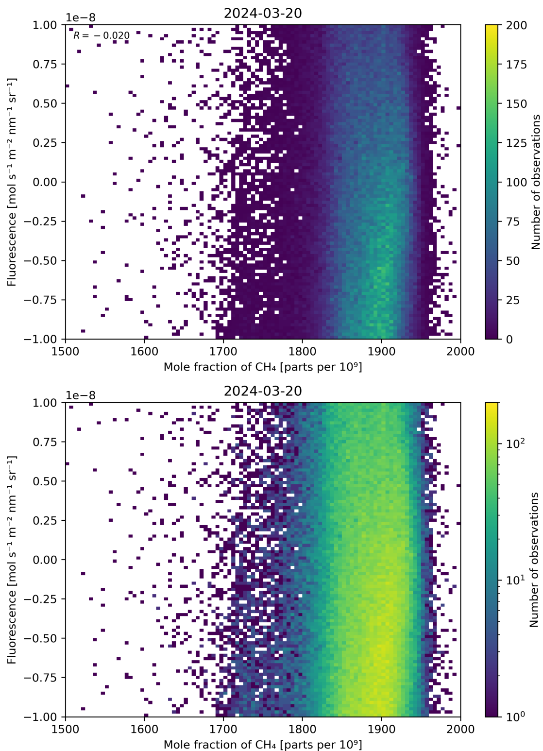
Figure 73: Scatter density plot of “Mole fraction of \text{CH}_4 ” against “Fluorescence” for 2024-03-20 to 2024-03-21.
