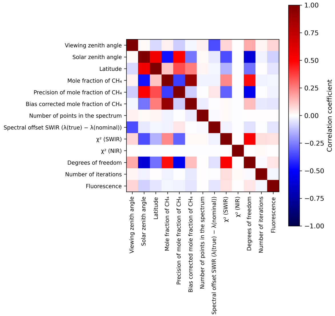
Figure 2: Map of correlation matrix for 2024-03-20 to 2024-03-21.
