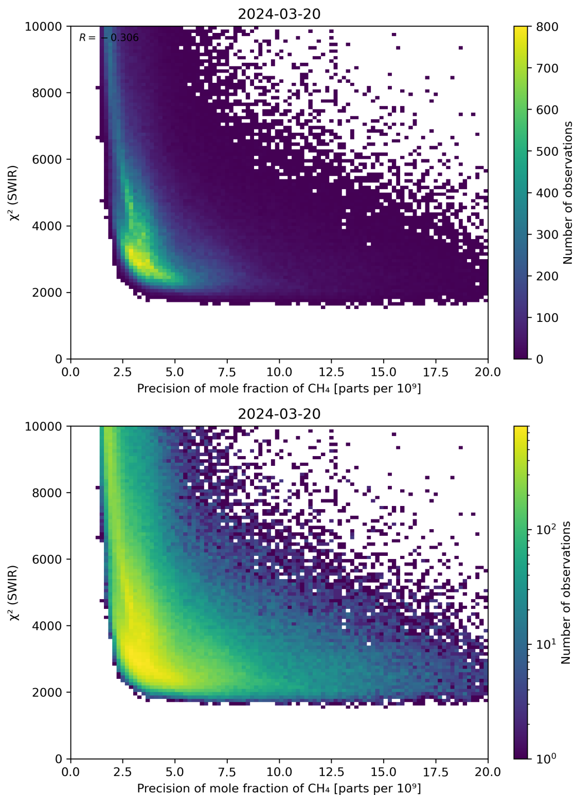
Figure 79: Scatter density plot of “Precision of mole fraction of CH 4 ” against “ \chi^2 (SWIR)” for 2024-03-20 to 2024-03-21.
