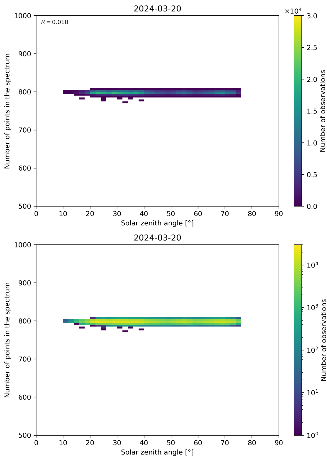
Figure 103: Scatter density plot of “Solar zenith angle” against “Number of points in the spectrum” for 2024-03-20 to 2024-03-21.
