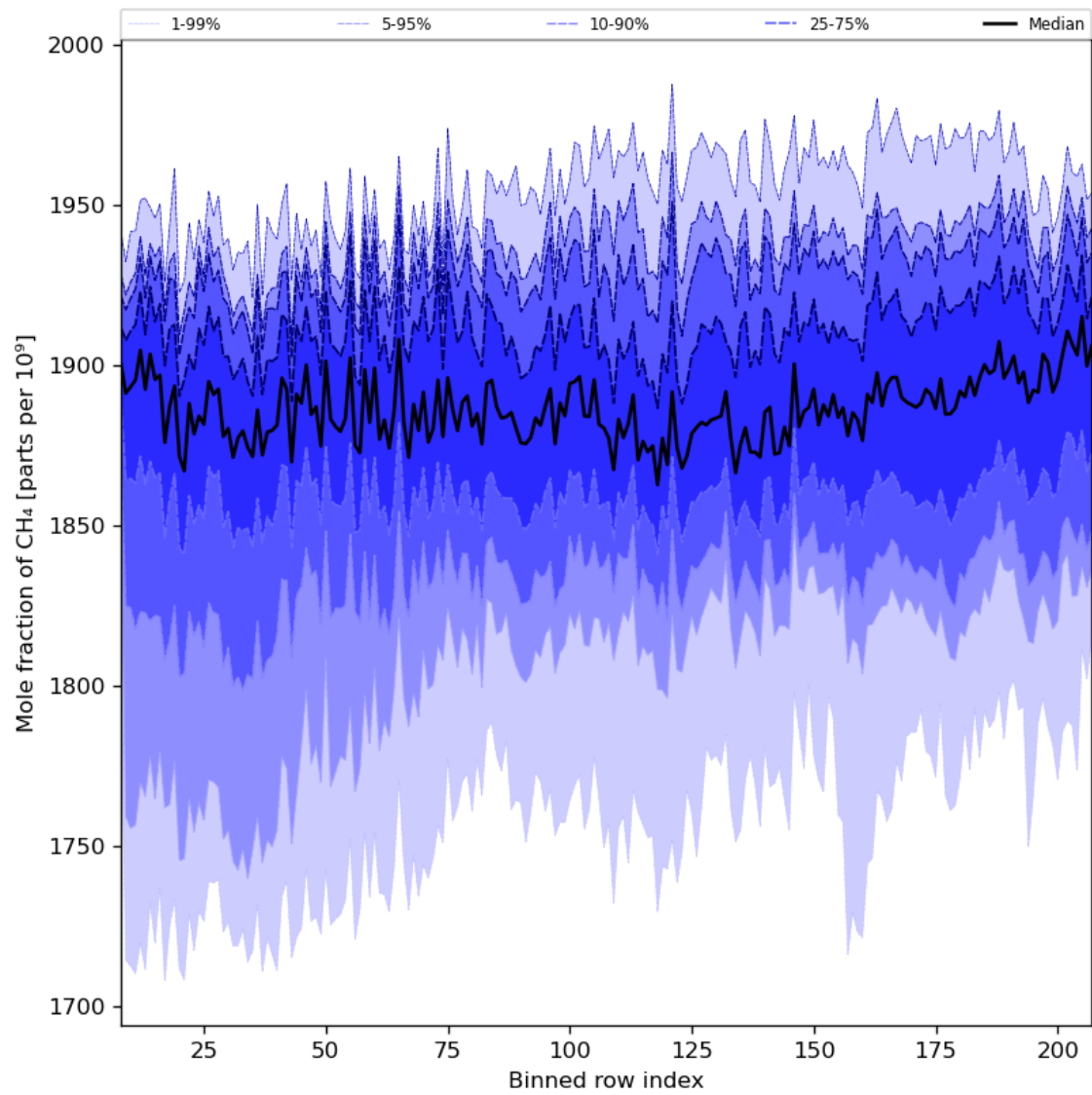
Figure 34: Along track statistics of “Mole fraction of CH 4 ” for 2024-03-20 to 2024-03-21
