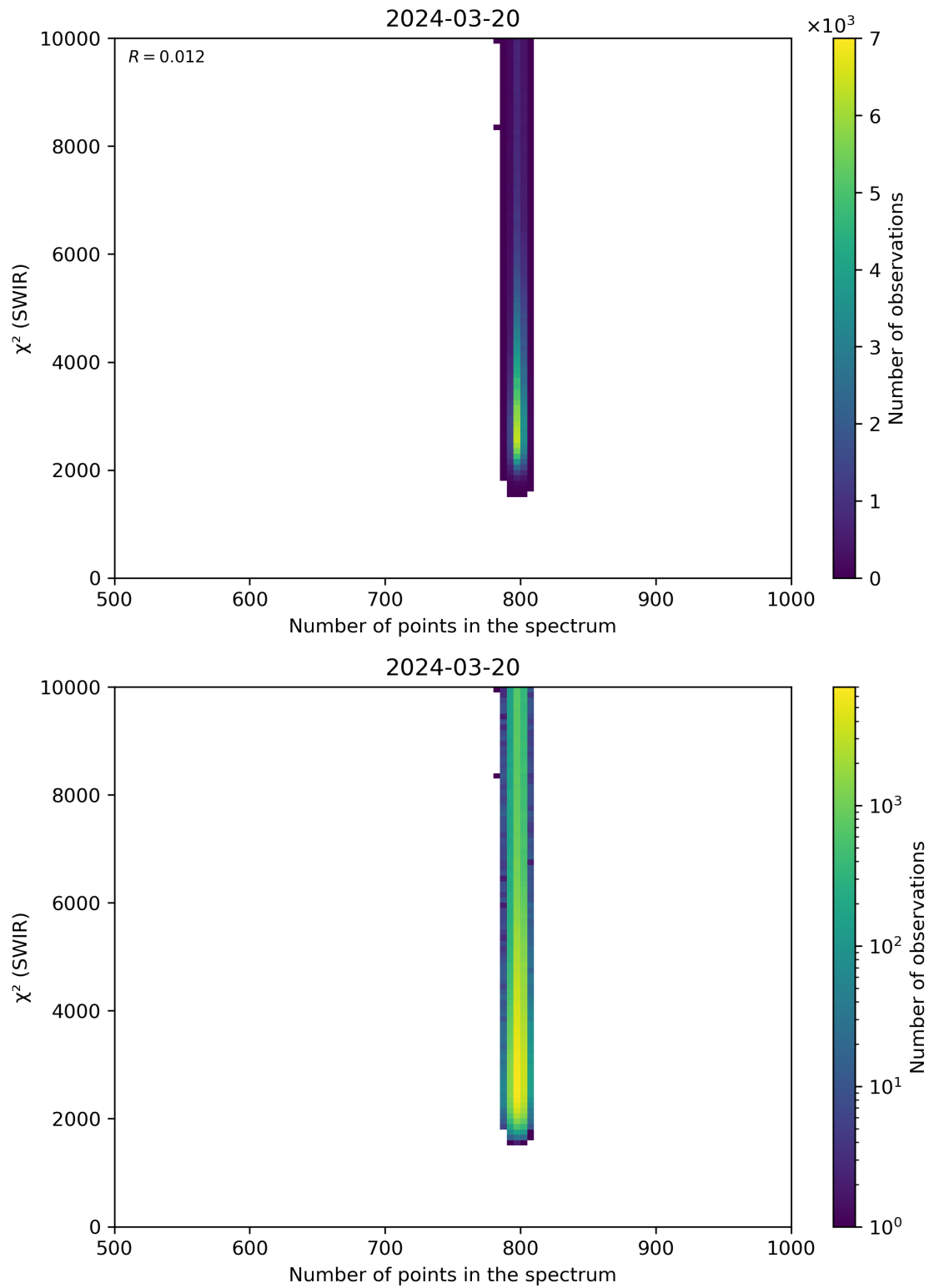
Figure 89: Scatter density plot of “Number of points in the spectrum” against “ \chi^2 (SWIR)” for 2024-03-20 to 2024-03-21.
