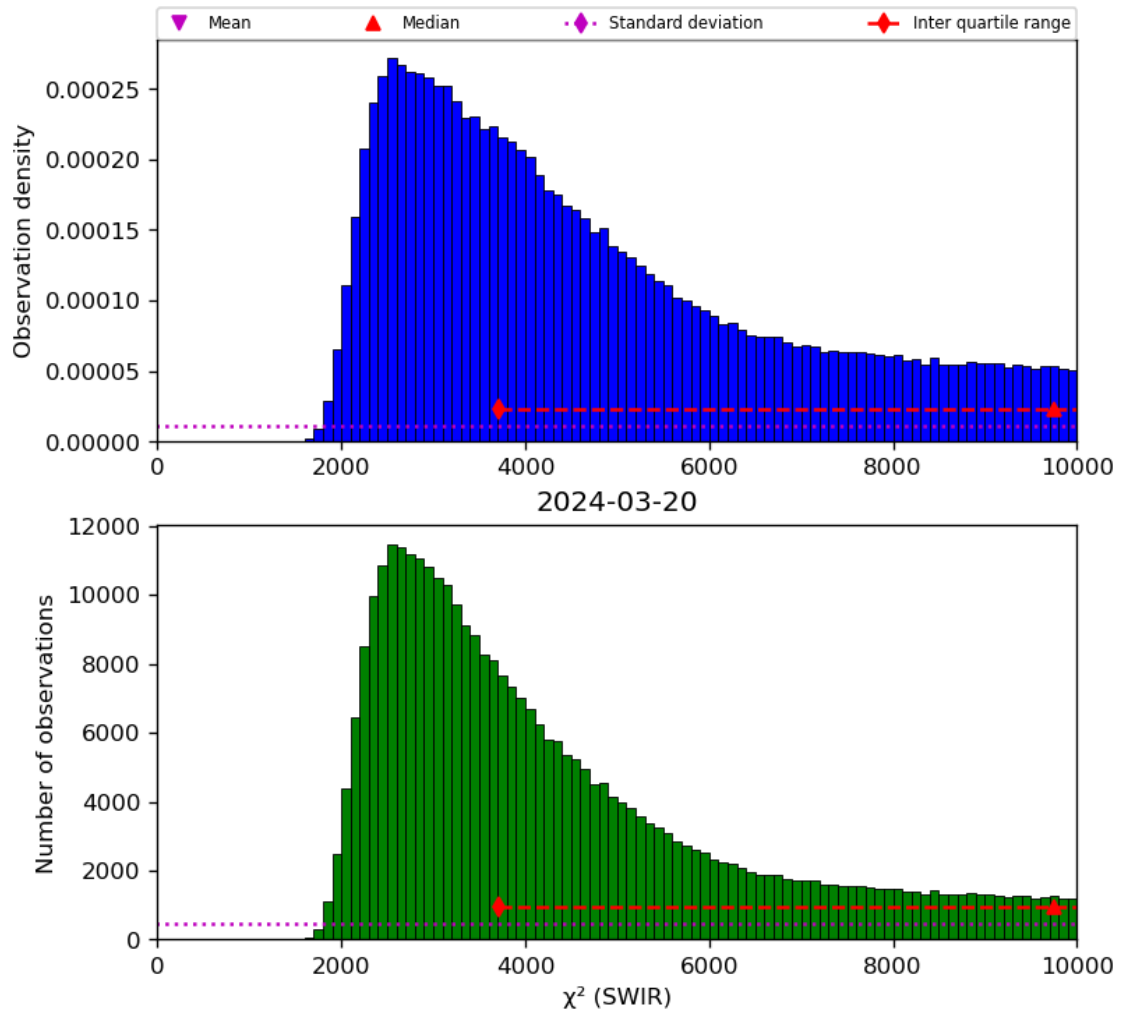
Figure 28: Histogram of “ \chi^2 (SWIR)” for 2024-03-20 to 2024-03-21
