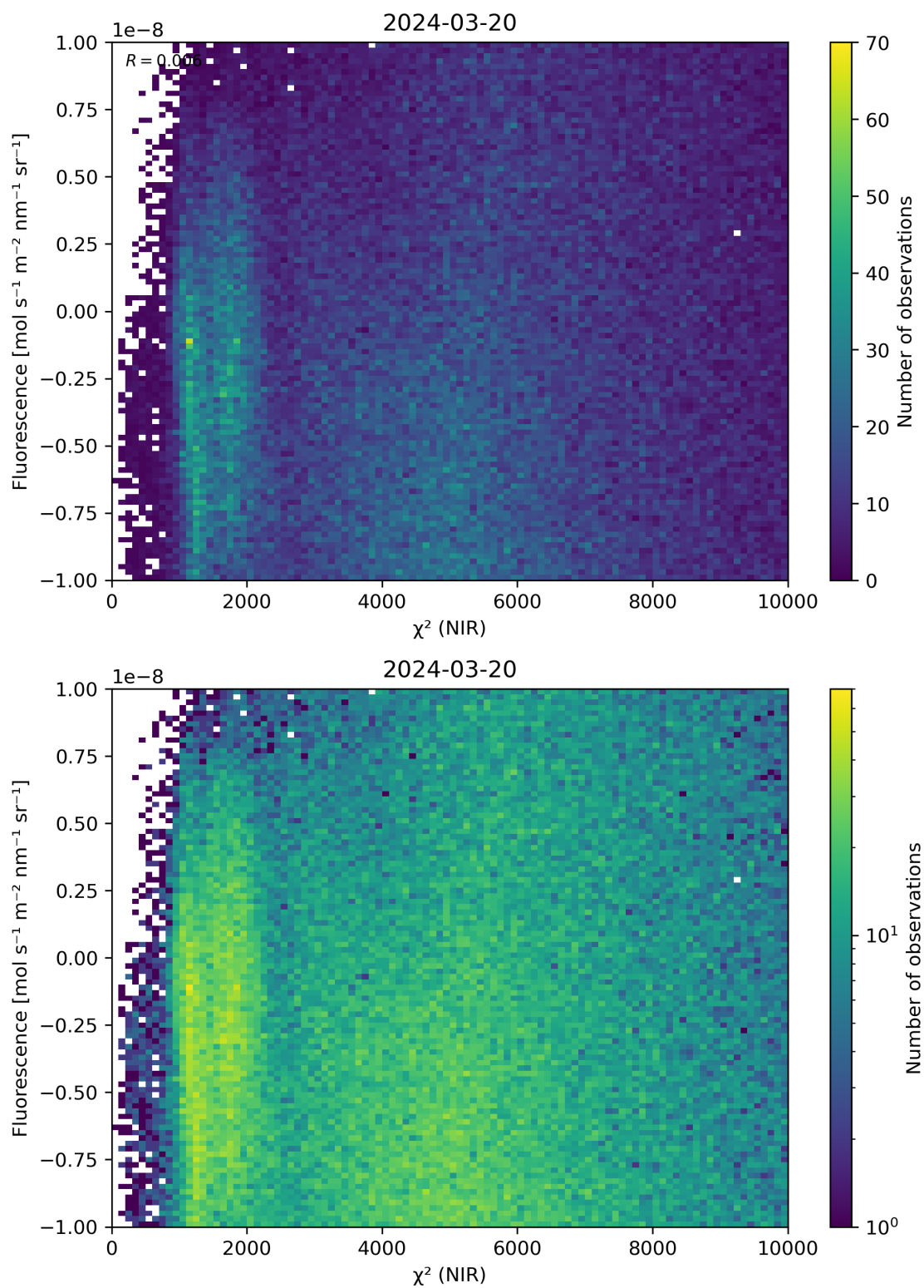
Figure 45: Scatter density plot of “ \chi^2 (NIR)” against “Fluorescence” for 2024-03-20 to 2024-03-21.
