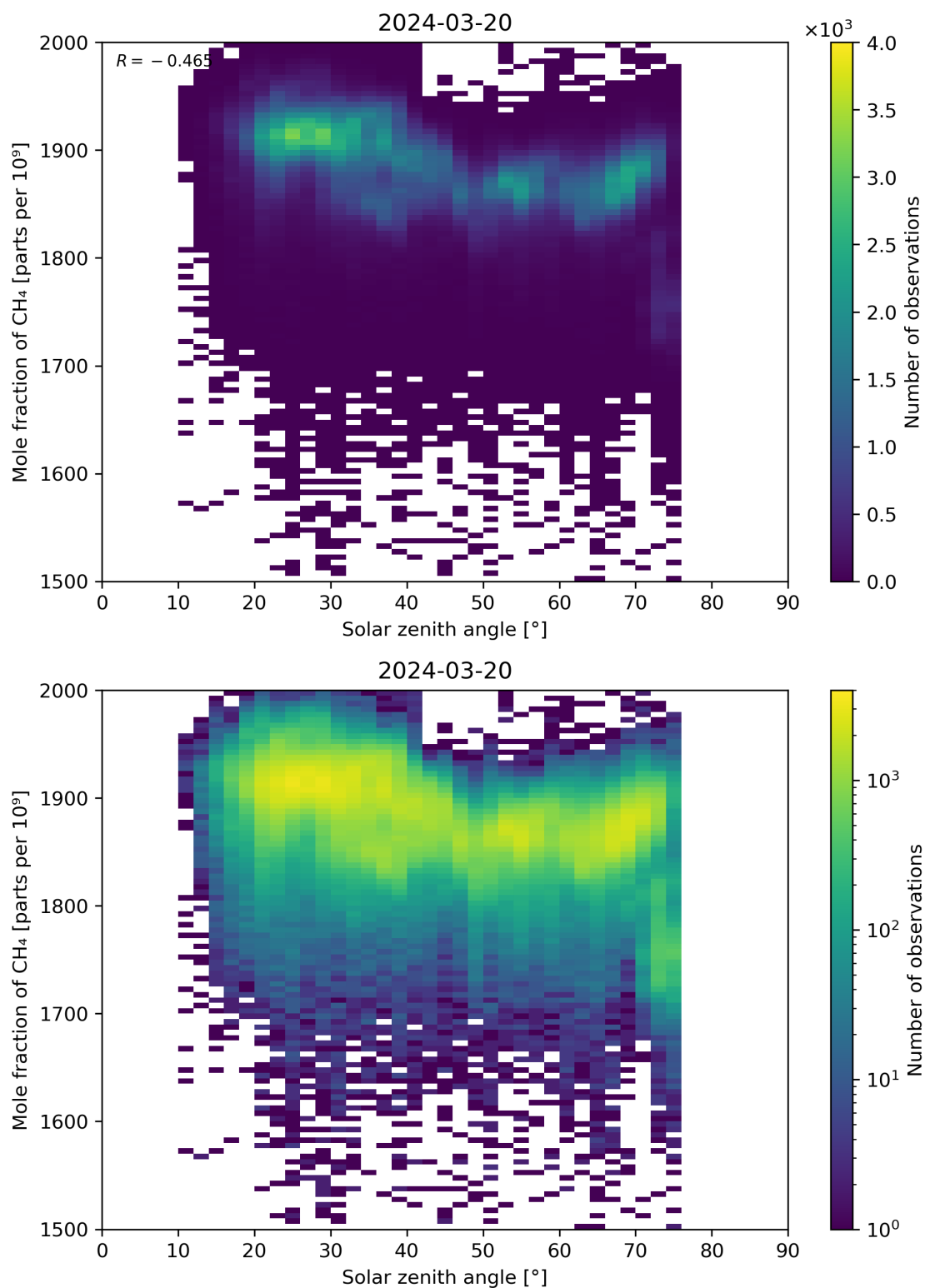
Figure 99: Scatter density plot of “Solar zenith angle” against “Mole fraction of CH 4 ” for 2024-03-20 to 2024-03-21.
