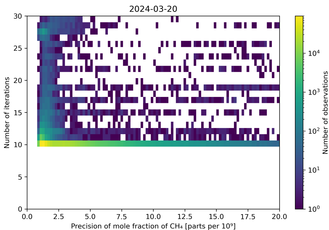
Figure 83: Scatter density plot of “Precision of mole fraction of CH 4 ” against “Number of iterations” for 2024-03-20 to 2024-03-21.
