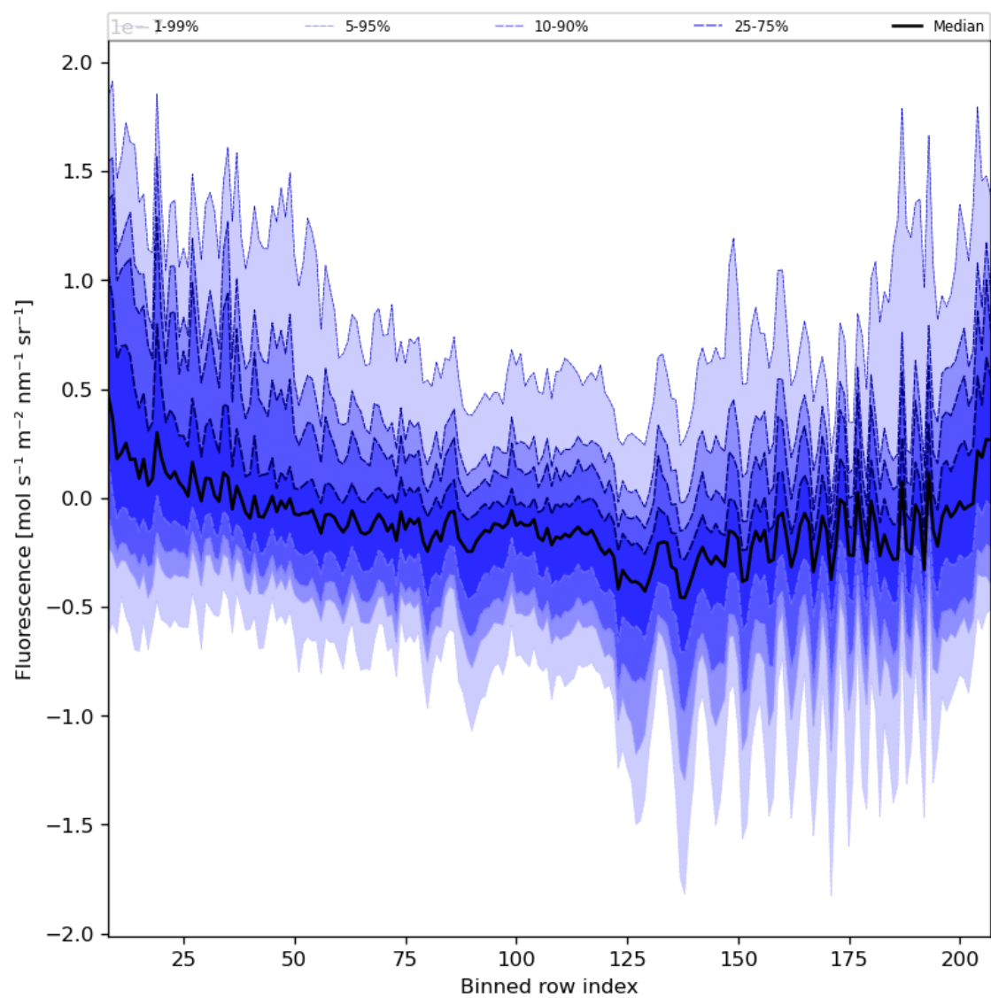
Figure 43: Along track statistics of “Fluorescence” for 2024-03-20 to 2024-03-21
