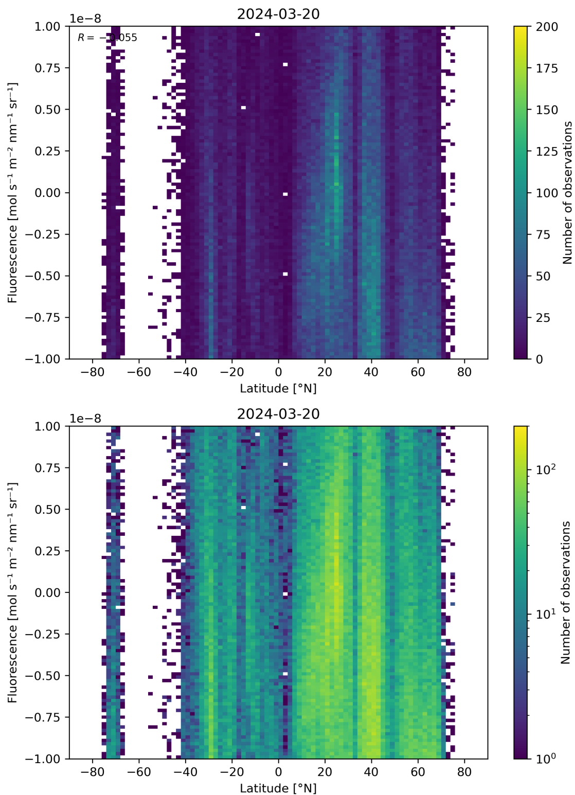
Figure 56: Scatter density plot of “Latitude” against “Fluorescence” for 2024-03-20 to 2024-03-21.
