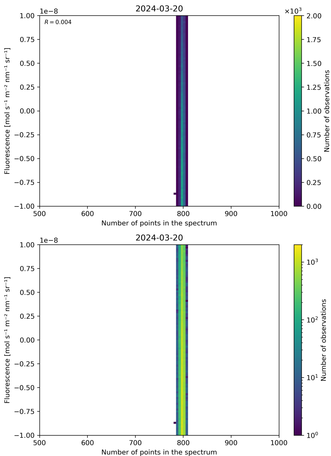
Figure 91: Scatter density plot of “Number of points in the spectrum” against “Fluorescence” for 2024-03-20 to 2024-03-21.
