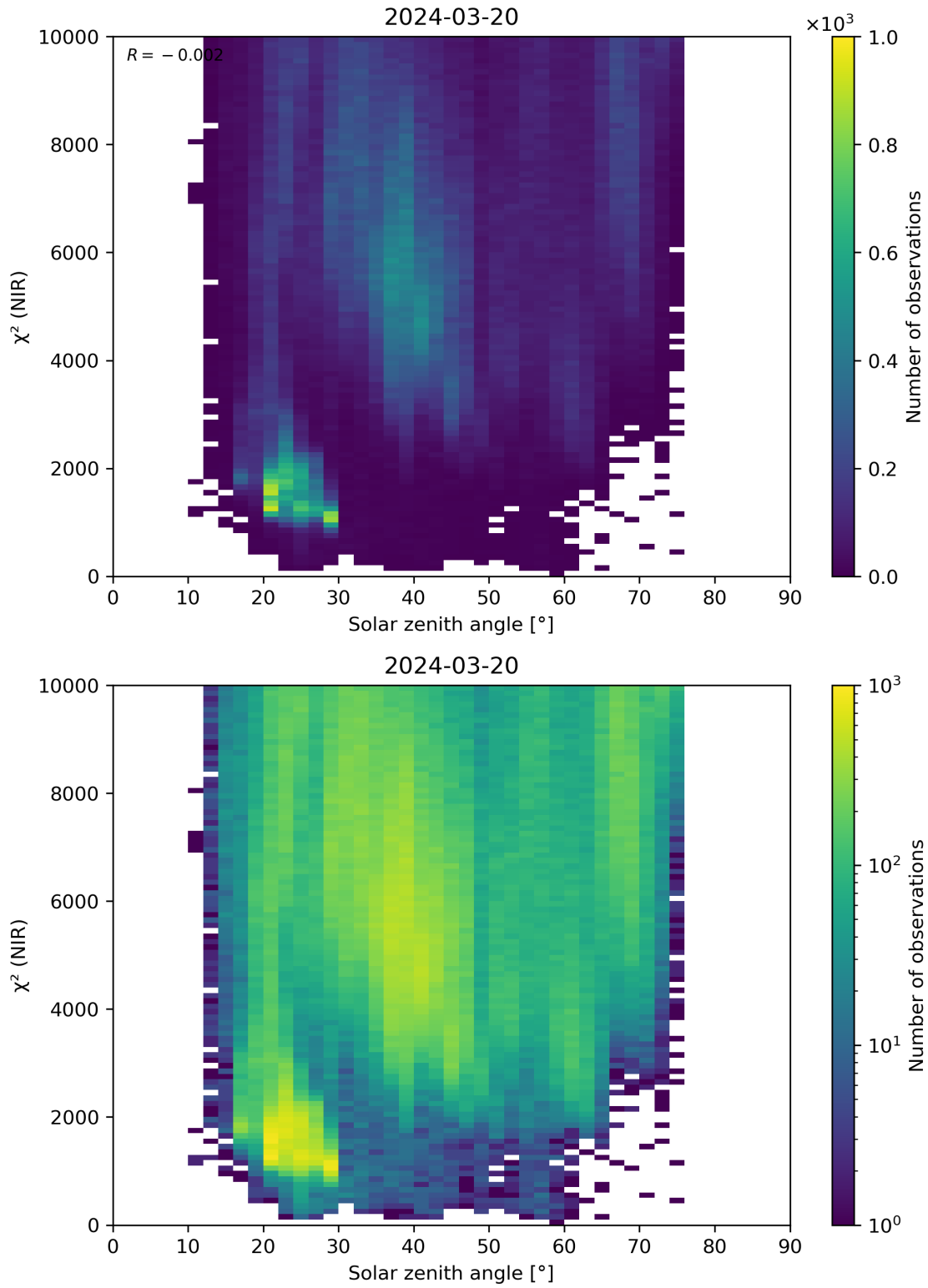
Figure 94: Scatter density plot of “Solar zenith angle” against “ \chi^2 (NIR)” for 2024-03-20 to 2024-03-21.
