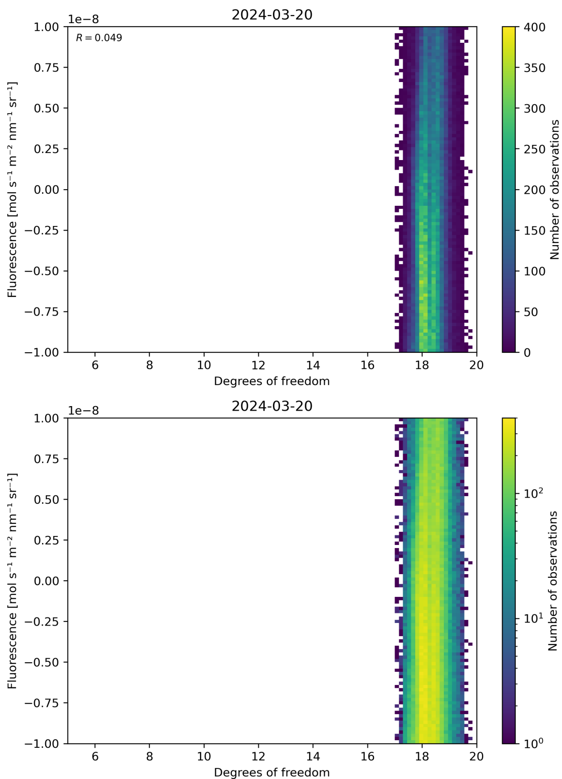
Figure 51: Scatter density plot of “Degrees of freedom” against “Fluorescence” for 2024-03-20 to 2024-03-21.
