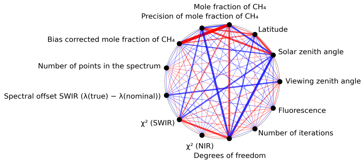
Figure 1: Map of correlation graph for 2024-03-20 to 2024-03-21.
