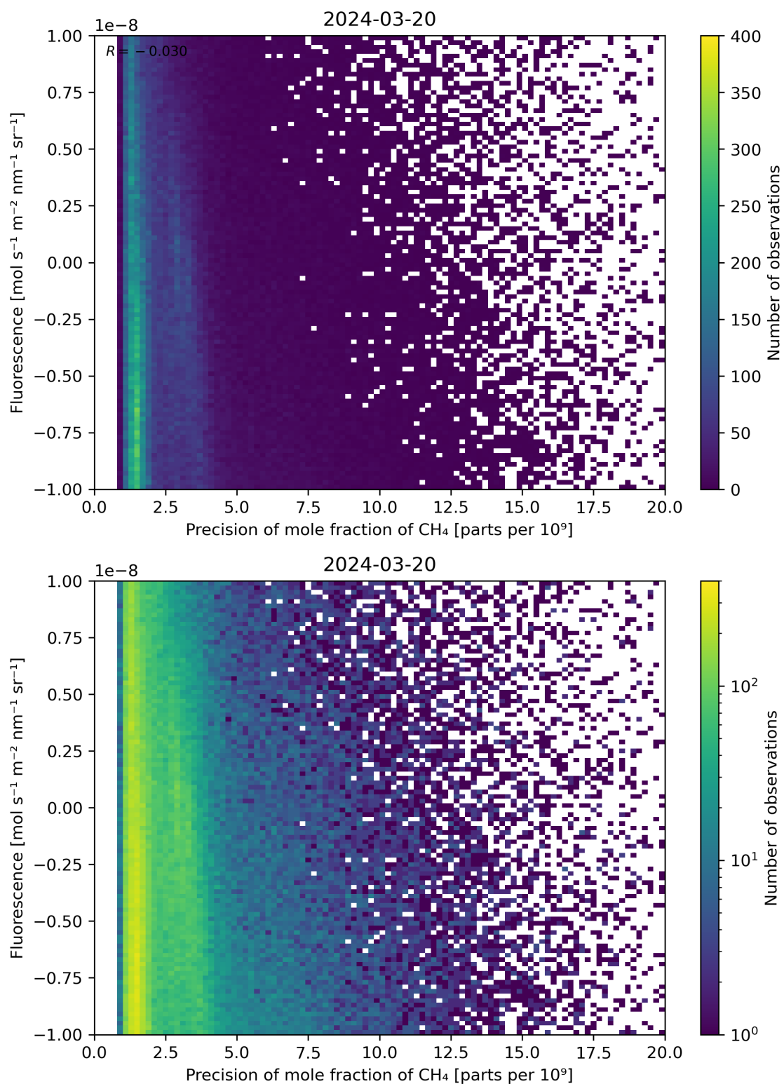
Figure 81: Scatter density plot of “Precision of mole fraction of \text{CH}_4 ” against “Fluorescence” for 2024-03-20 to 2024-03-21.
