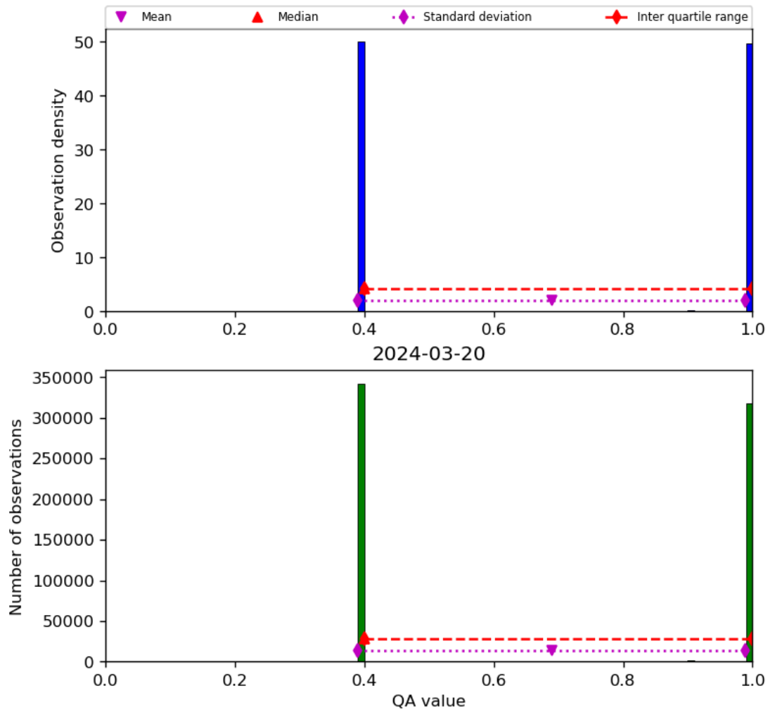
Figure 22: Histogram of “QA value” for 2024-03-20 to 2024-03-21
