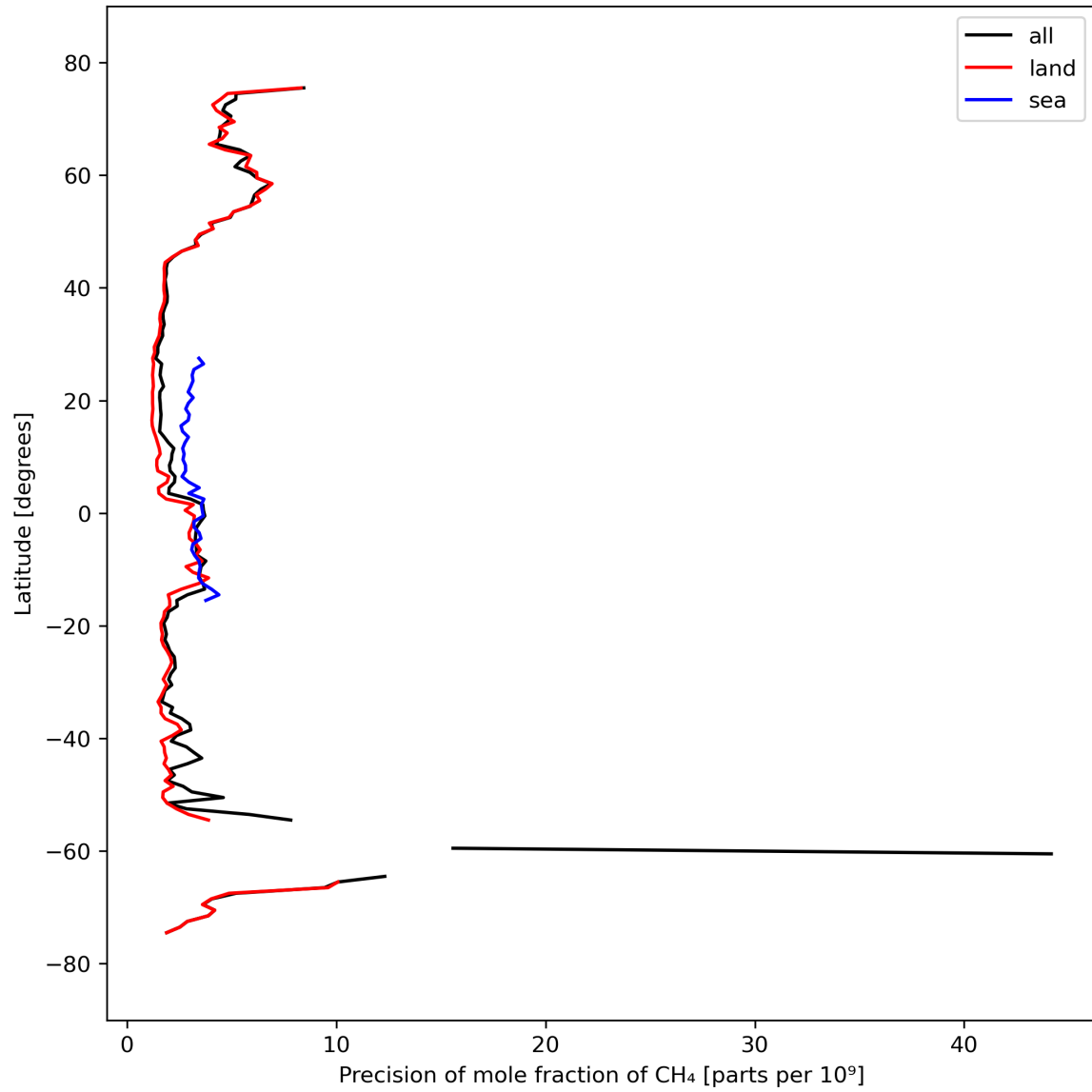
Figure 13: Zonal average of “Precision of mole fraction of CH 4 ” for 2024-03-20 to 2024-03-21.
