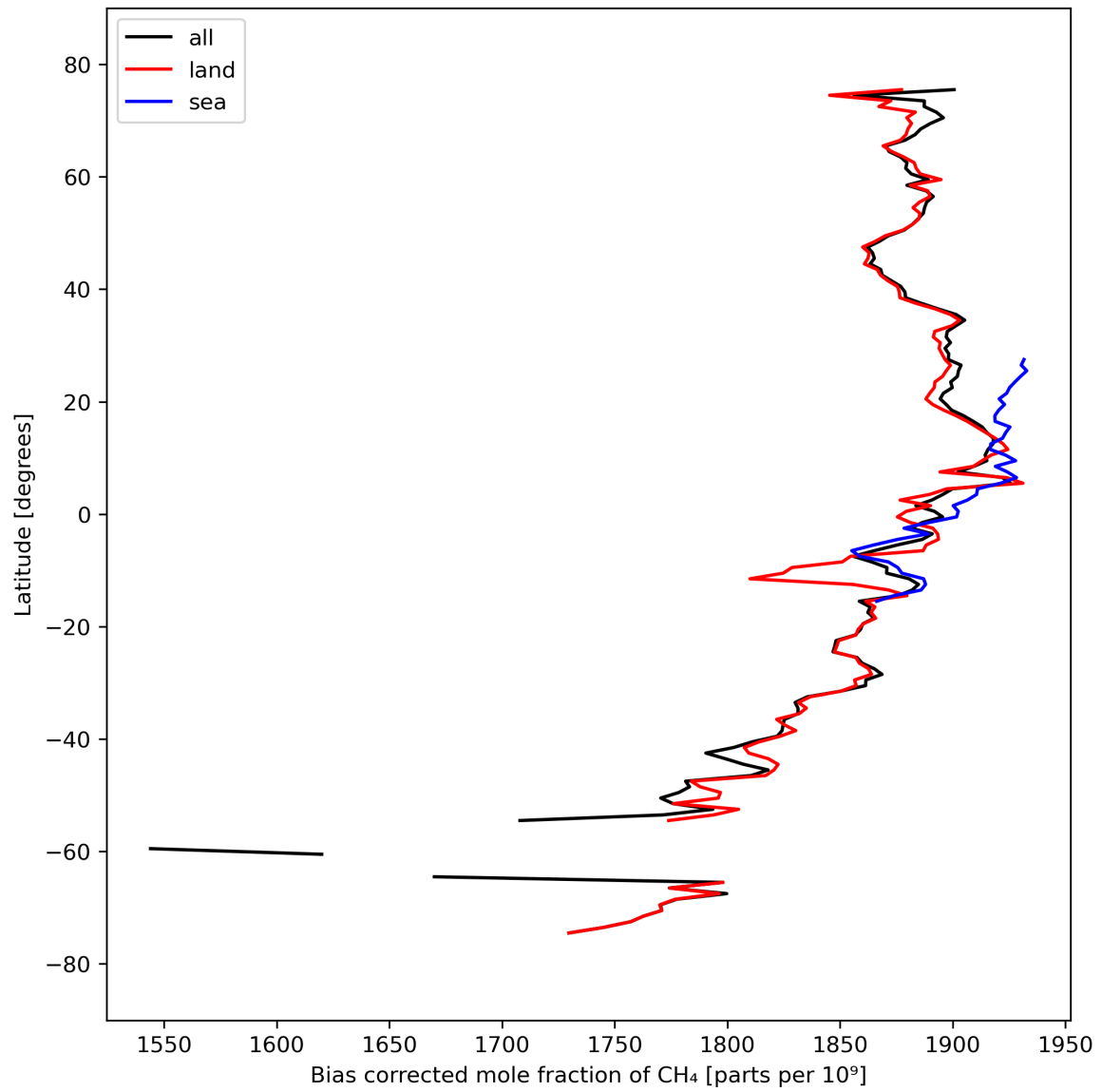
Figure 14: Zonal average of “Bias corrected mole fraction of CH 4 ” for 2024-03-20 to 2024-03-21.
