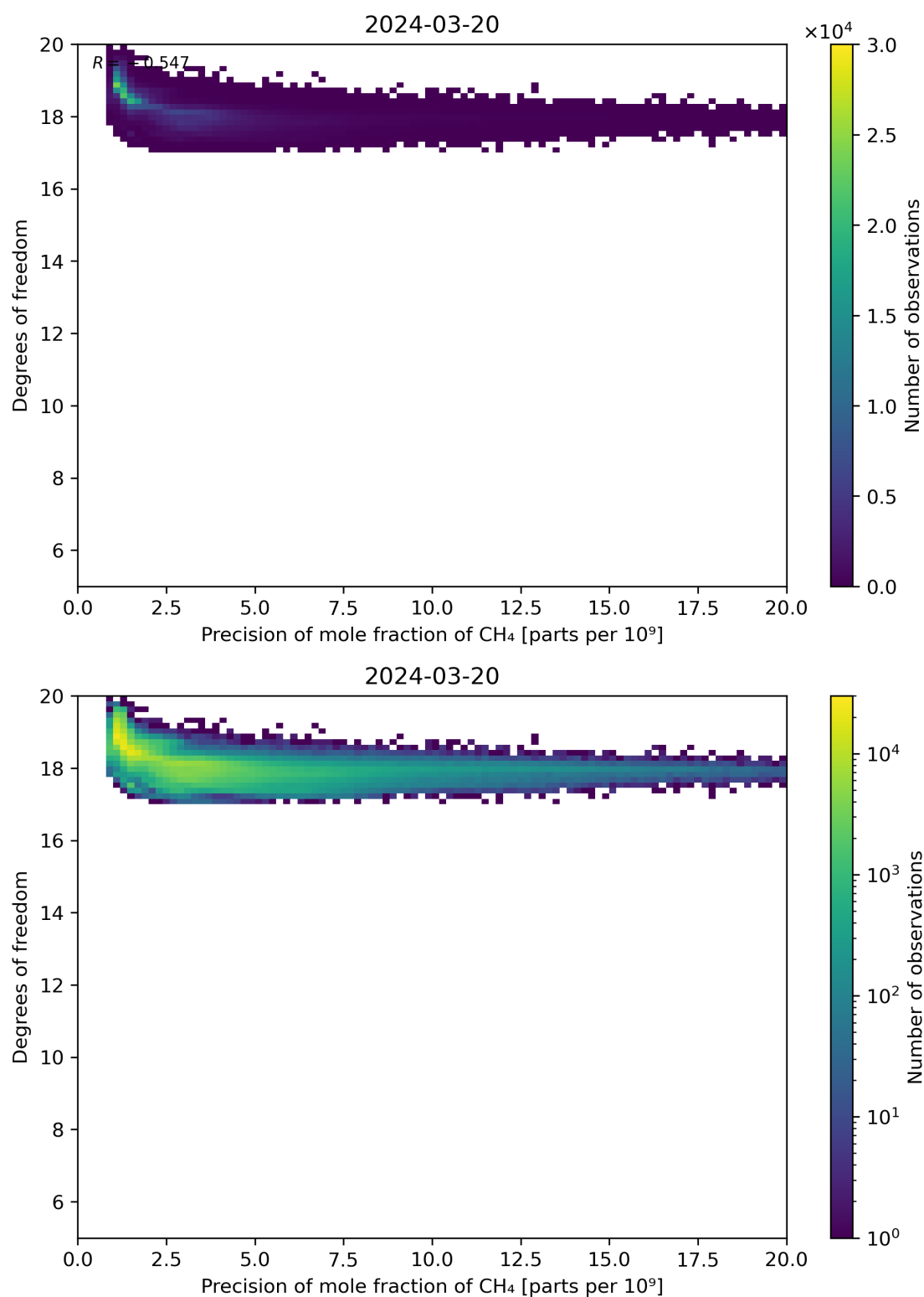
Figure 80: Scatter density plot of “Precision of mole fraction of CH 4 ” against “Degrees of freedom” for 2024-03-20 to 2024-03-21.
