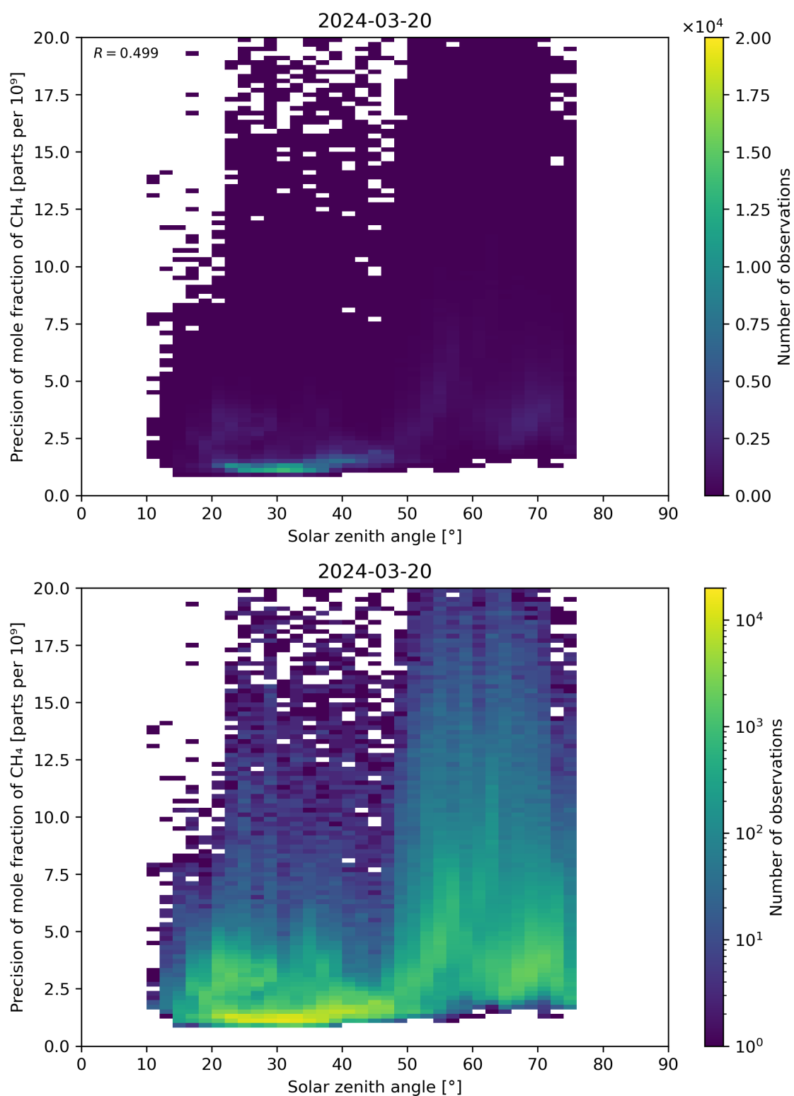
Figure 101: Scatter density plot of “Solar zenith angle” against “Precision of mole fraction of \text{CH}_4 ” for 2024-03-20 to 2024-03-21.
