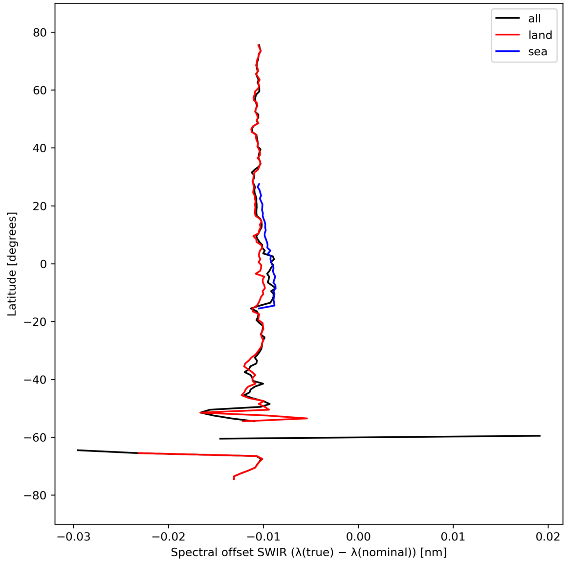
Figure 16: Zonal average of “Spectral offset SWIR ( \lambda(\text{true}) - \lambda(\text{nominal}) )” for 2024-03-20 to 2024-03-21.
