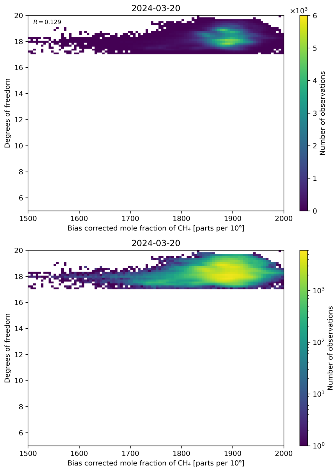
Figure 65: Scatter density plot of “Bias corrected mole fraction of CH 4 ” against “Degrees of freedom” for 2024-03-20 to 2024-03-21.
