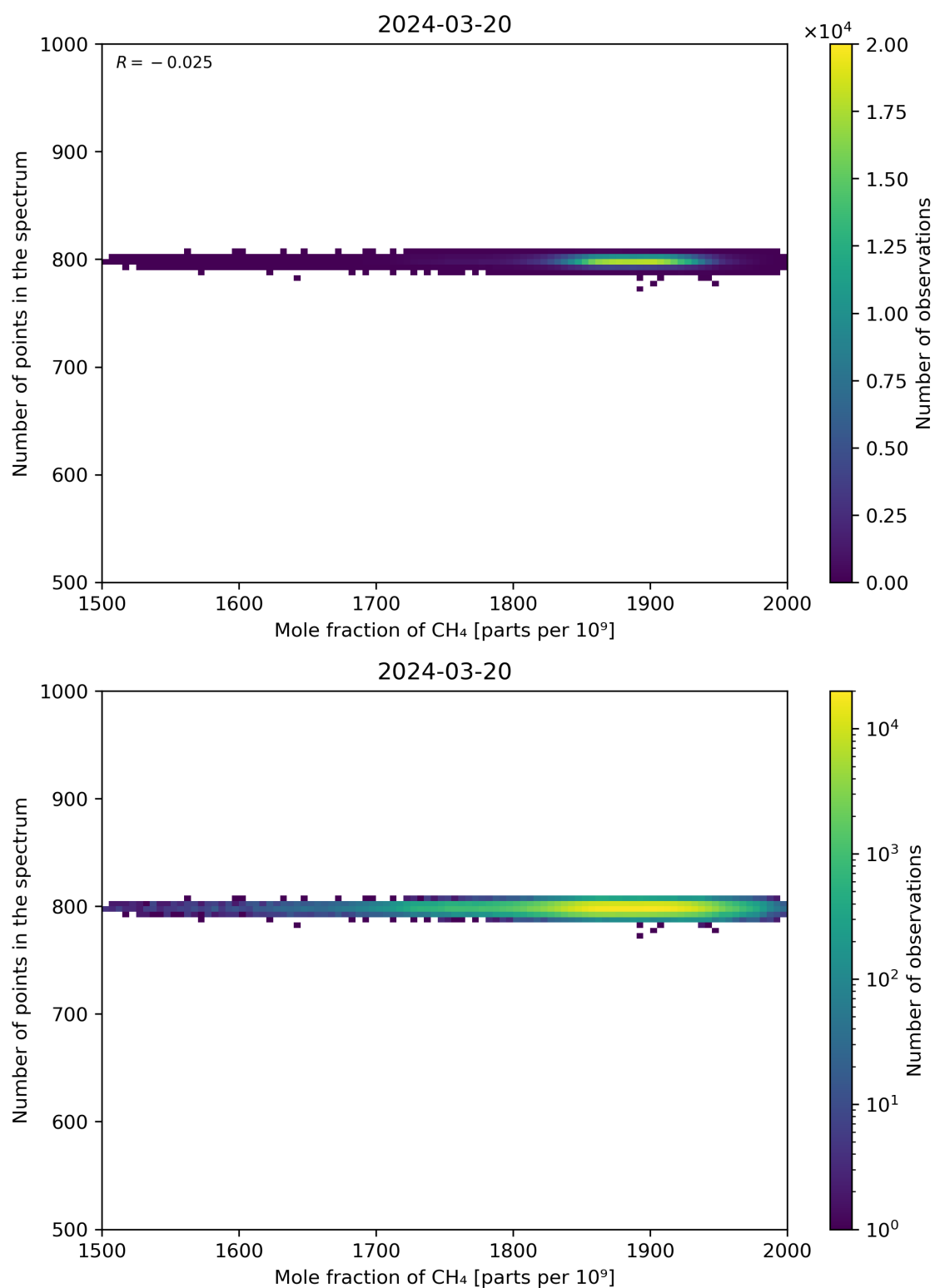
Figure 77: Scatter density plot of “Mole fraction of CH 4 ” against “Number of points in the spectrum” for 2024-03-20 to 2024-03-21.
