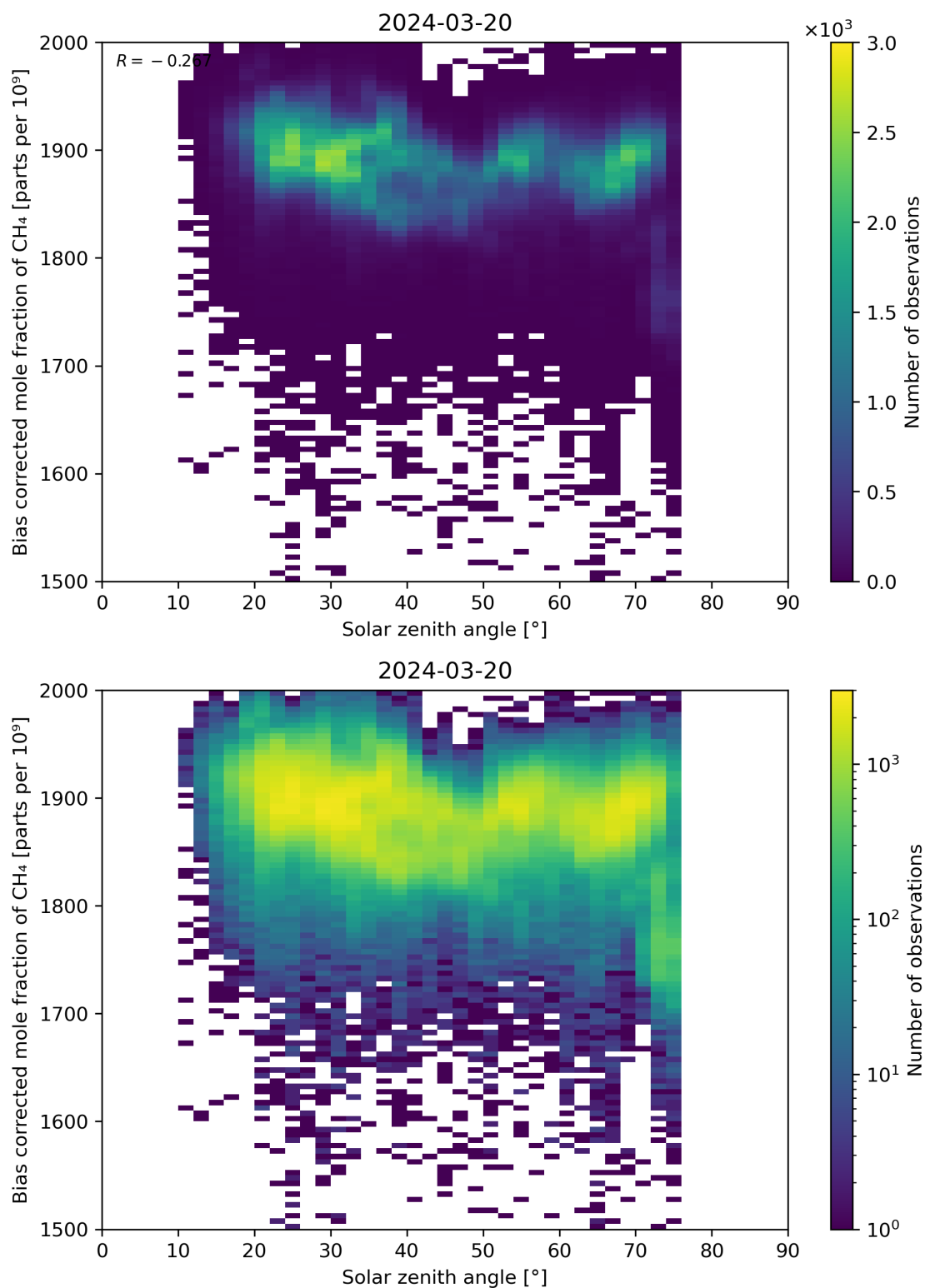
Figure 100: Scatter density plot of “Solar zenith angle” against “Bias corrected mole fraction of CH 4 ” for 2024-03-20 to 2024-03-21.
