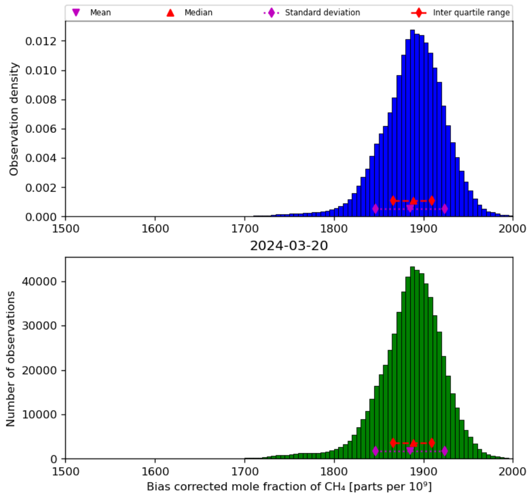
Figure 25: Histogram of “Bias corrected mole fraction of CH 4 ” for 2024-03-20 to 2024-03-21
