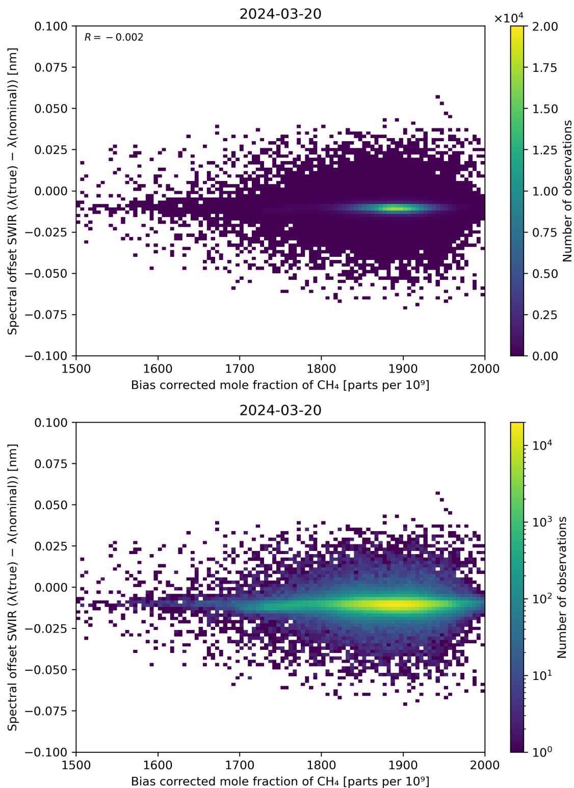
Figure 69: Scatter density plot of “Bias corrected mole fraction of \text{CH}_4 ” against “Spectral offset SWIR ( \lambda(\text{true}) - \lambda(\text{nominal}) )” for 2024-03-20 to 2024-03-21.
