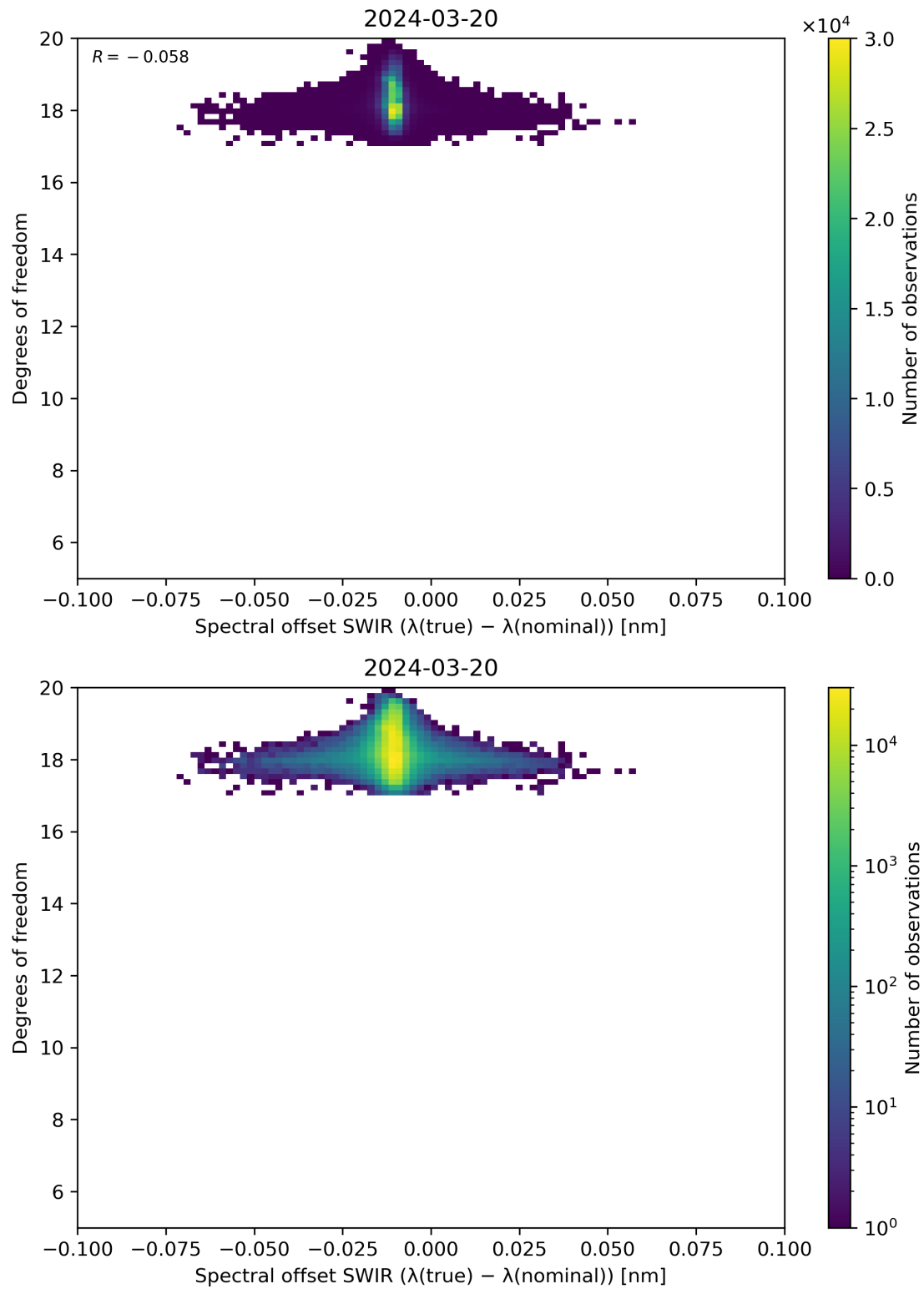
Figure 119: Scatter density plot of “Spectral offset SWIR ( \lambda(\text{true}) - \lambda(\text{nominal}) )” against “Degrees of freedom” for 2024-03-20 to 2024-03-21.
