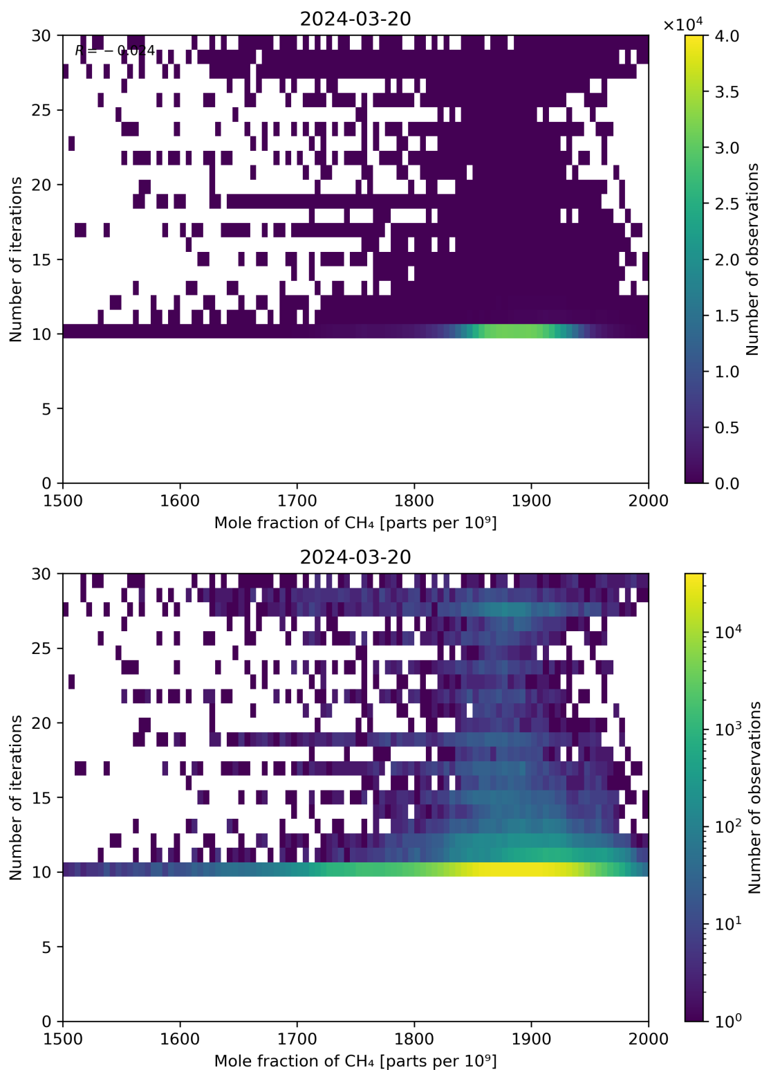
Figure 76: Scatter density plot of “Mole fraction of CH 4 ” against “Number of iterations” for 2024-03-20 to 2024-03-21.
