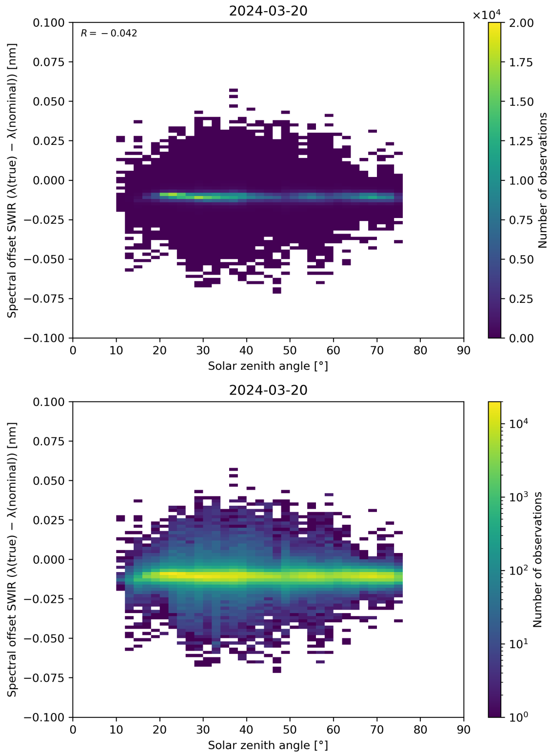
Figure 104: Scatter density plot of “Solar zenith angle” against “Spectral offset SWIR ( \lambda(\text{true}) - \lambda(\text{nominal}) )” for 2024-03-20 to 2024-03-21.
