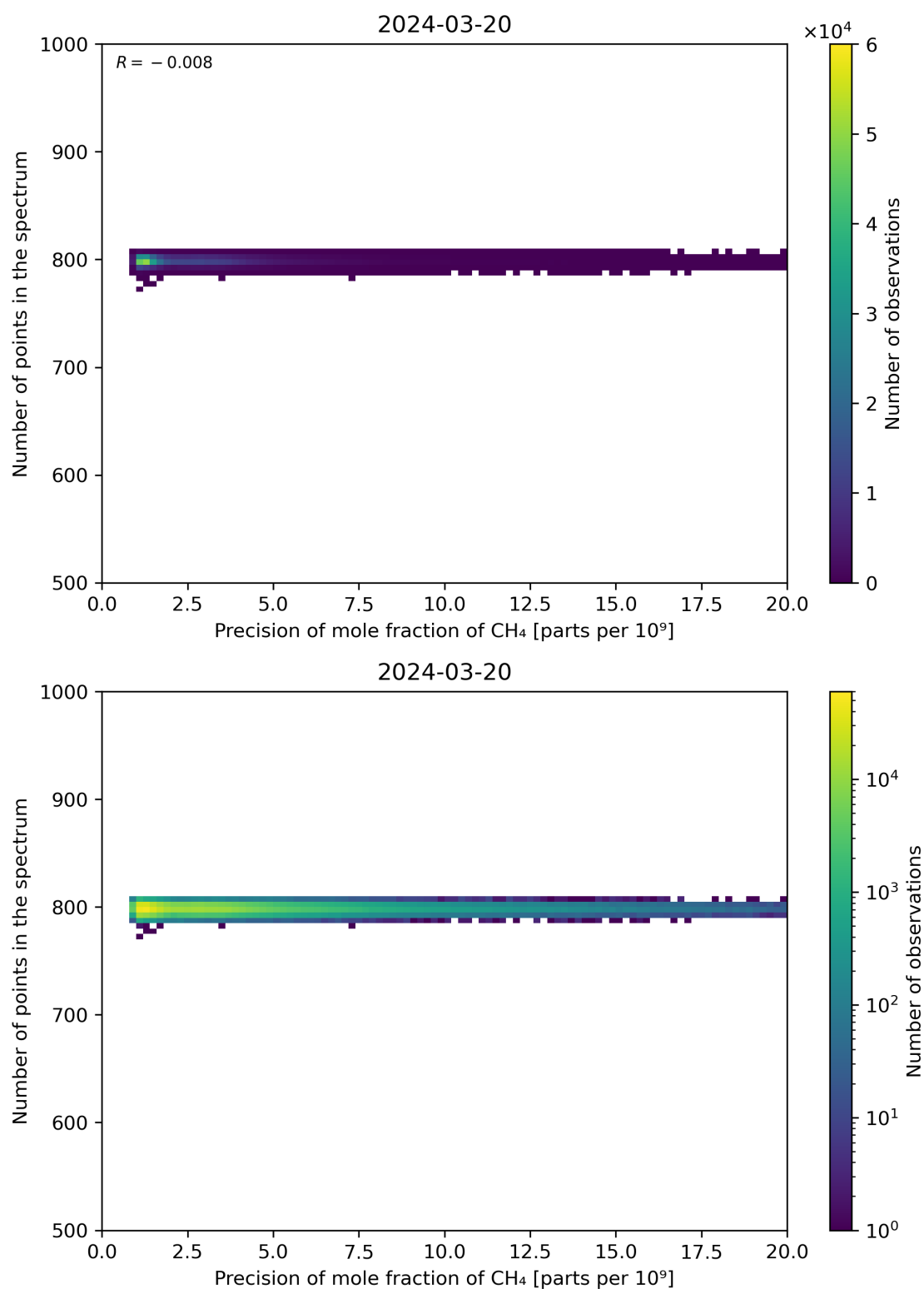
Figure 84: Scatter density plot of “Precision of mole fraction of CH 4 ” against “Number of points in the spectrum” for 2024-03-20 to 2024-03-21.
