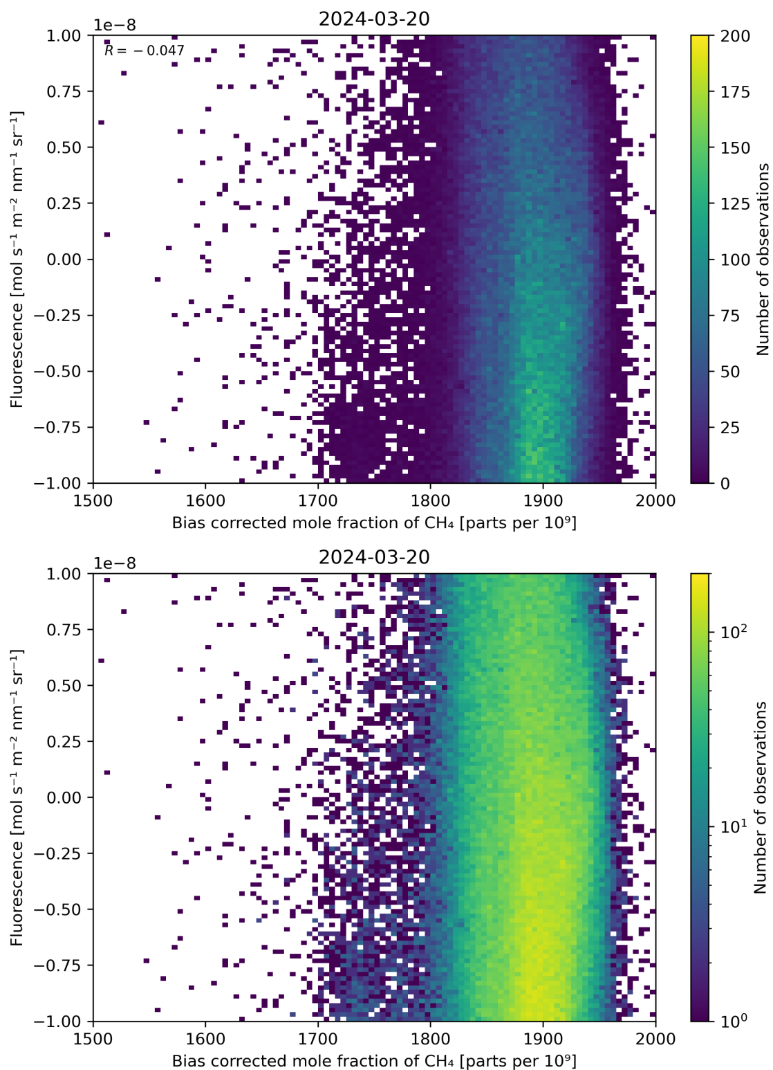
Figure 66: Scatter density plot of “Bias corrected mole fraction of CH 4 ” against “Fluorescence” for 2024-03-20 to 2024-03-21.
