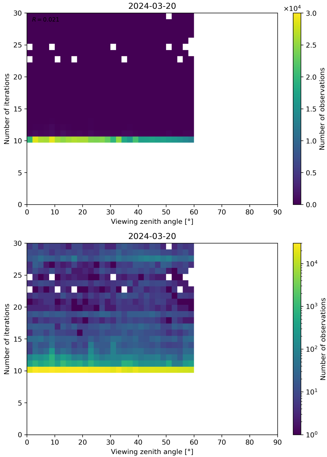
Figure 113: Scatter density plot of “Viewing zenith angle” against “Number of iterations” for 2024-03-20 to 2024-03-21.
