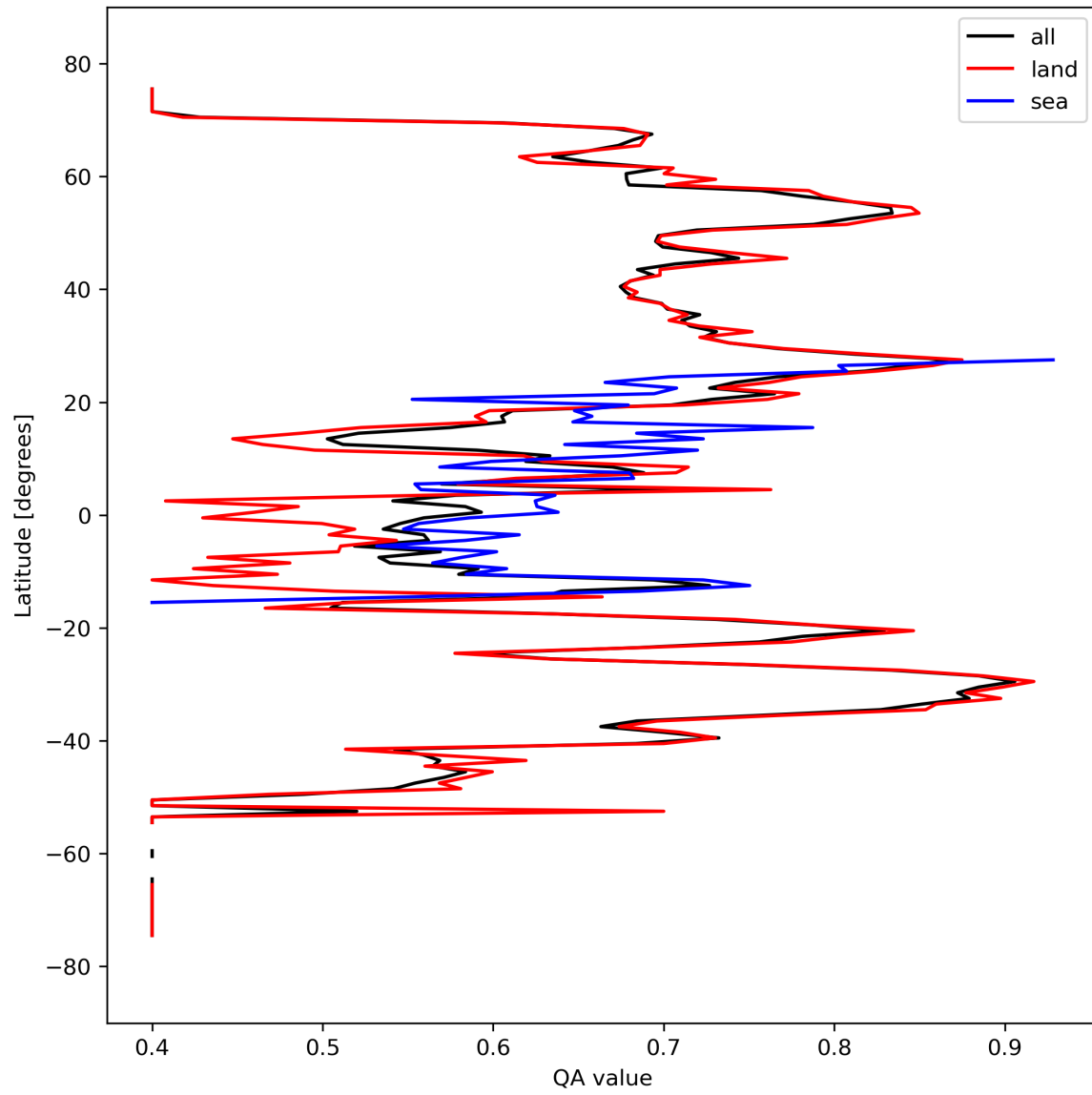
Figure 11: Zonal average of “QA value” for 2024-03-20 to 2024-03-21.
