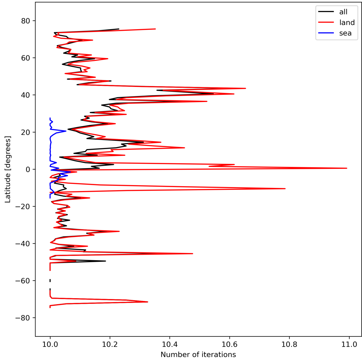
Figure 20: Zonal average of “Number of iterations” for 2024-03-20 to 2024-03-21.
