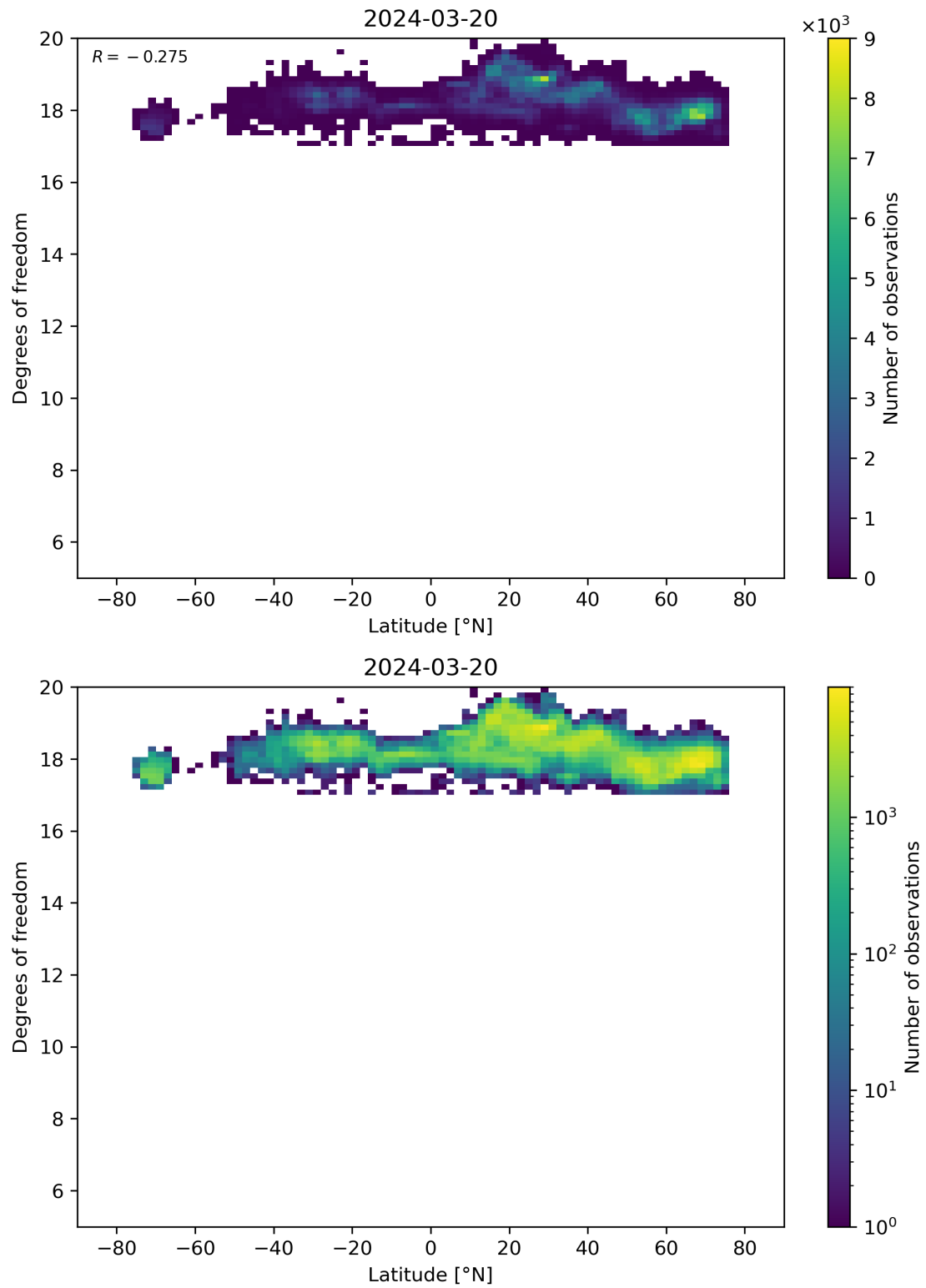
Figure 55: Scatter density plot of “Latitude” against “Degrees of freedom” for 2024-03-20 to 2024-03-21.
