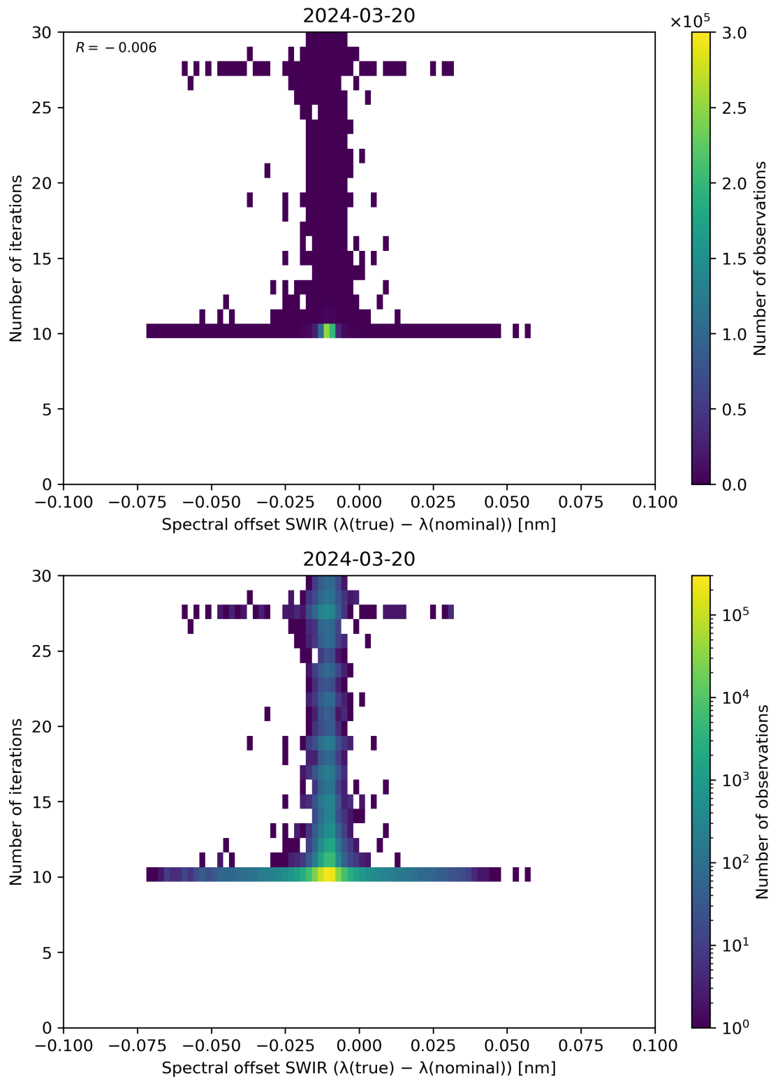
Figure 121: Scatter density plot of “Spectral offset SWIR ( \lambda(\text{true}) - \lambda(\text{nominal}) )” against “Number of iterations” for 2024-03-20 to 2024-03-21.
