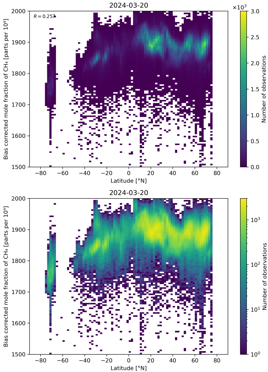
Figure 58: Scatter density plot of “Latitude” against “Bias corrected mole fraction of CH 4 ” for 2024-03-20 to 2024-03-21.
