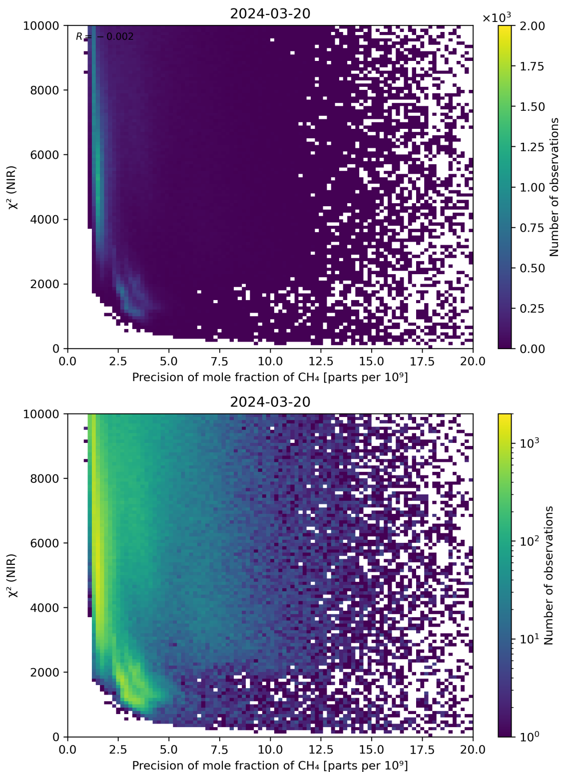
Figure 78: Scatter density plot of “Precision of mole fraction of CH 4 ” against “ \chi^2 (NIR)” for 2024-03-20 to 2024-03-21.
