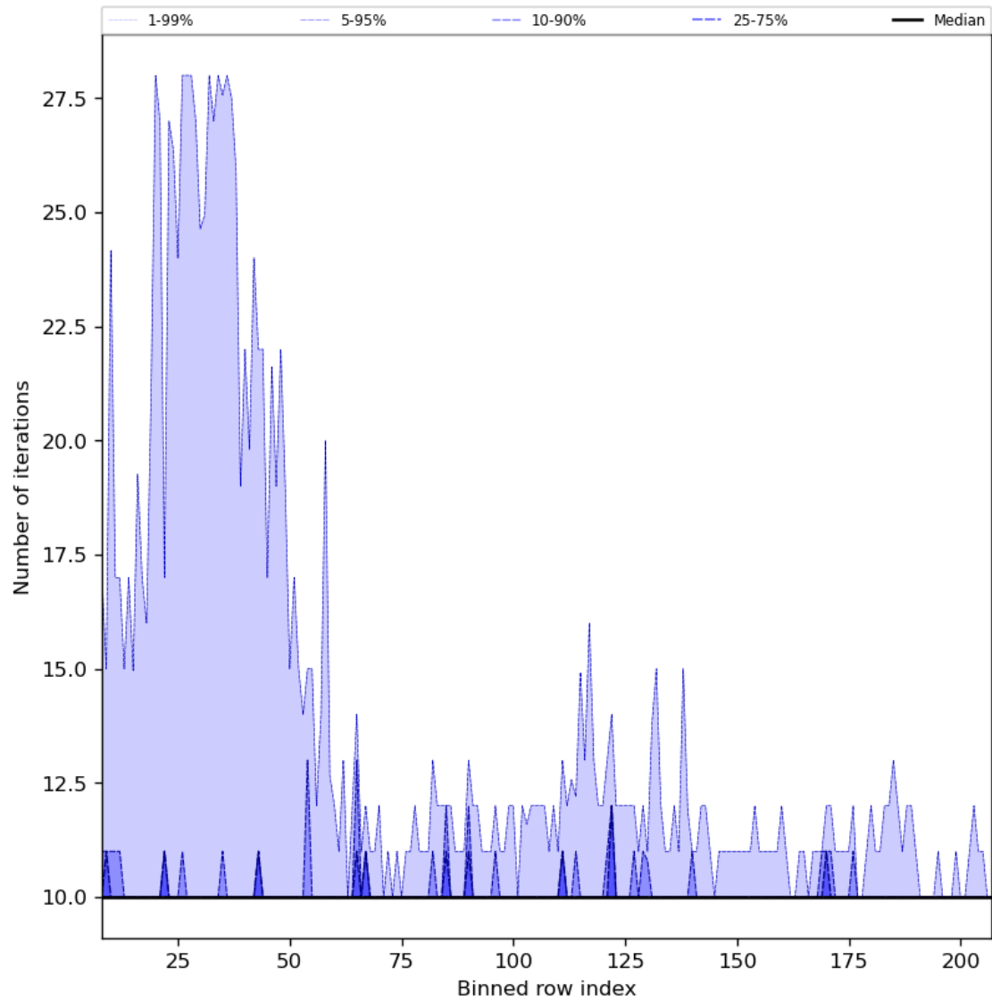
Figure 42: Along track statistics of “Number of iterations” for 2024-03-20 to 2024-03-21
