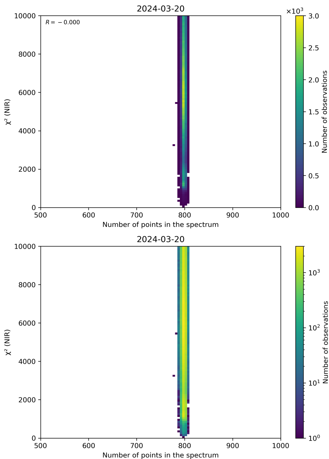
Figure 88: Scatter density plot of “Number of points in the spectrum” against “ \chi^2 (NIR)” for 2024-03-20 to 2024-03-21.
