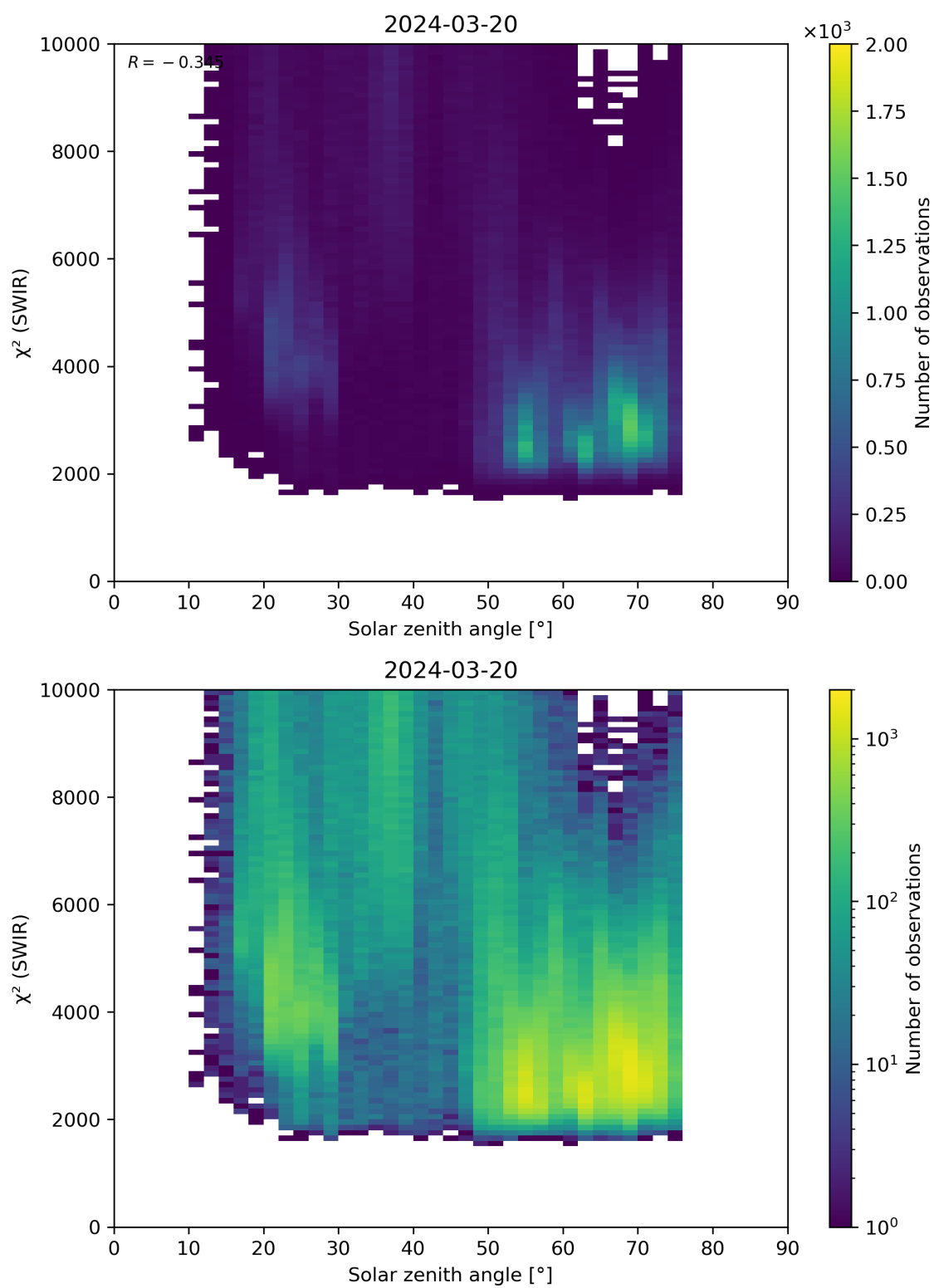
Figure 95: Scatter density plot of “Solar zenith angle” against “ \chi^2 (SWIR)” for 2024-03-20 to 2024-03-21.
