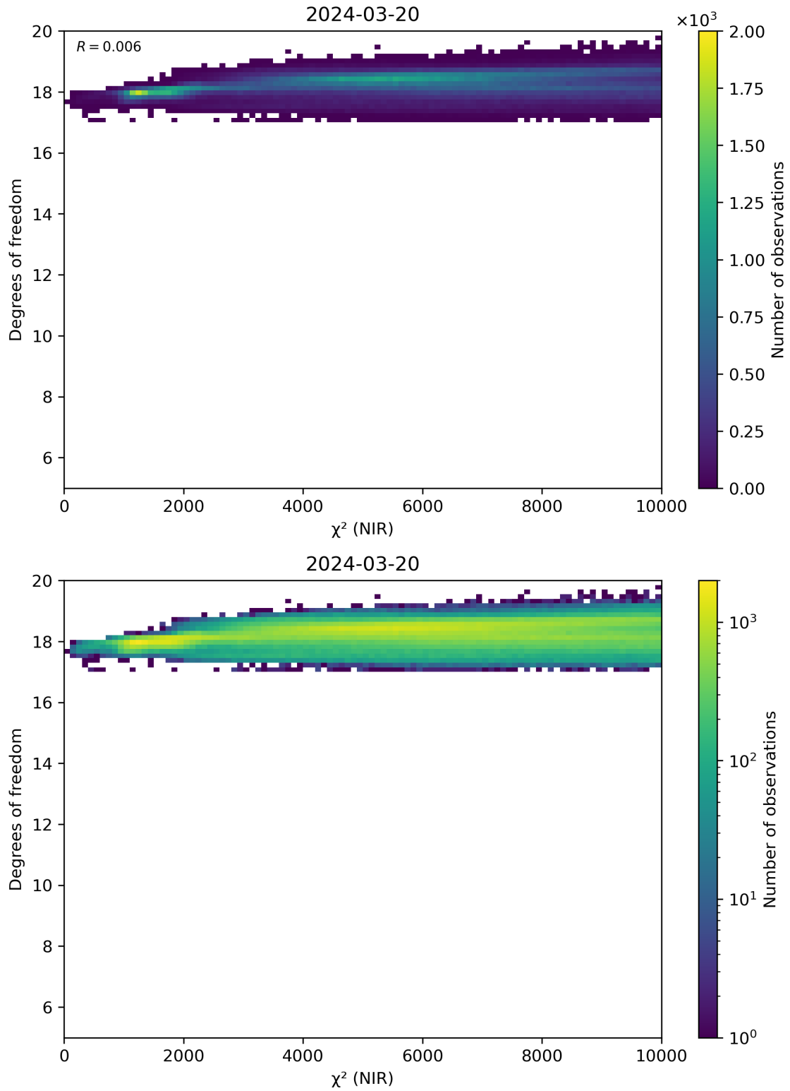
Figure 44: Scatter density plot of “ \chi^2 (NIR)” against “Degrees of freedom” for 2024-03-20 to 2024-03-21.
