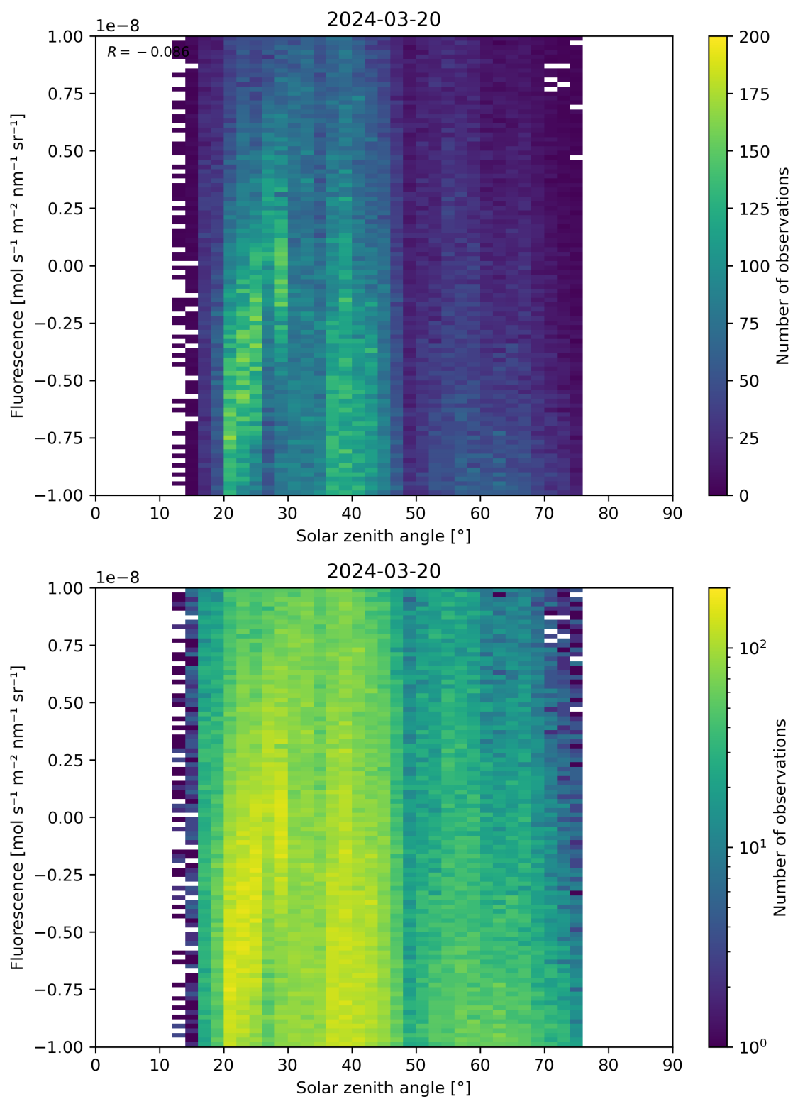
Figure 97: Scatter density plot of “Solar zenith angle” against “Fluorescence” for 2024-03-20 to 2024-03-21.
