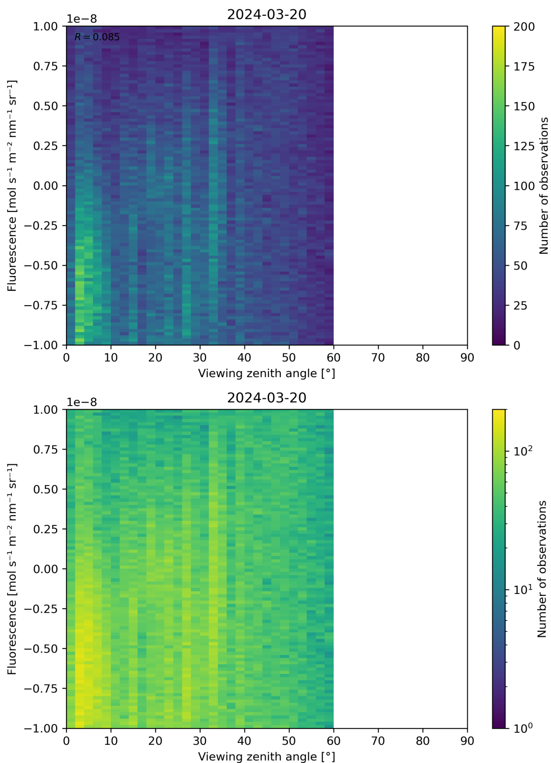
Figure 108: Scatter density plot of “Viewing zenith angle” against “Fluorescence” for 2024-03-20 to 2024-03-21.
