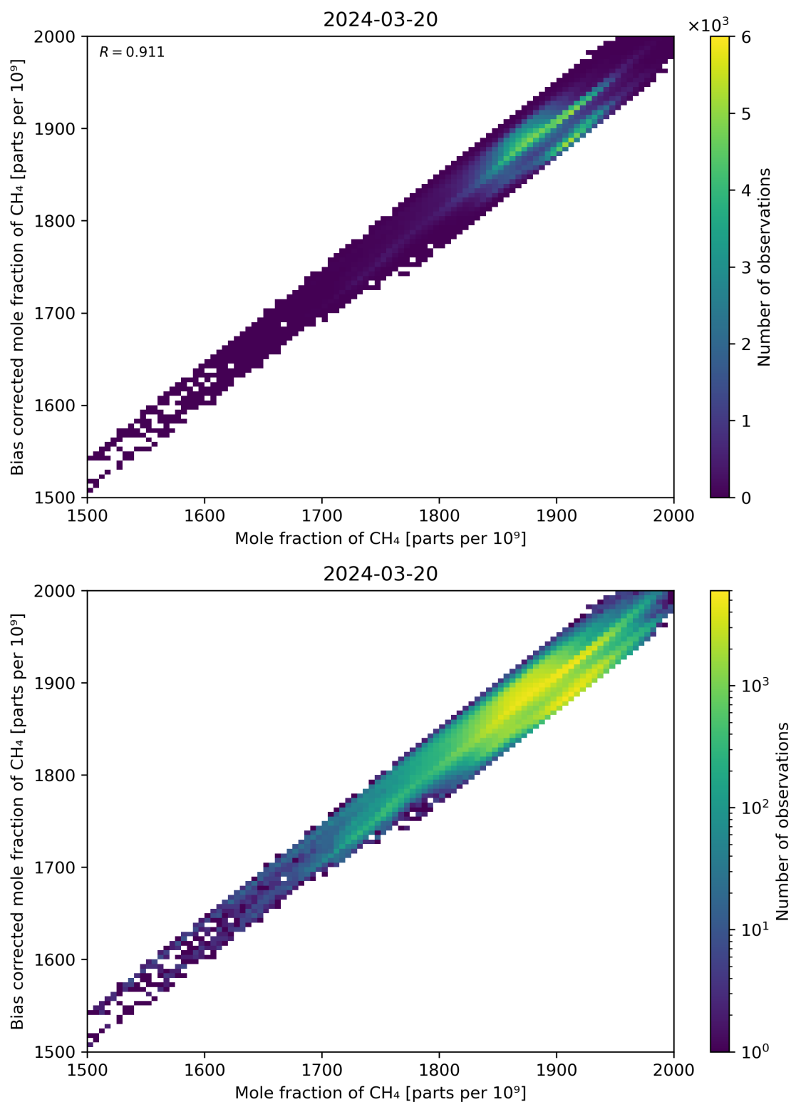
Figure 74: Scatter density plot of “Mole fraction of CH 4 ” against “Bias corrected mole fraction of CH 4 ” for 2024-03-20 to 2024-03-21.
