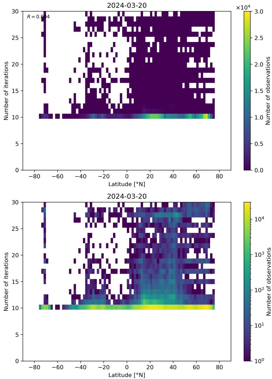
Figure 60: Scatter density plot of “Latitude” against “Number of iterations” for 2024-03-20 to 2024-03-21.
