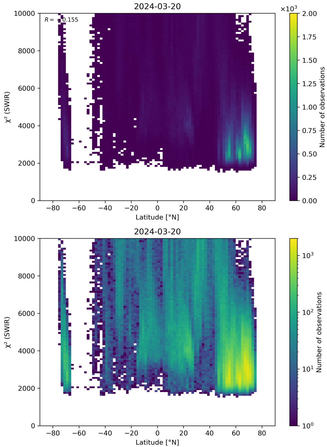
Figure 54: Scatter density plot of “Latitude” against “ \chi^2 (SWIR)” for 2024-03-20 to 2024-03-21.
