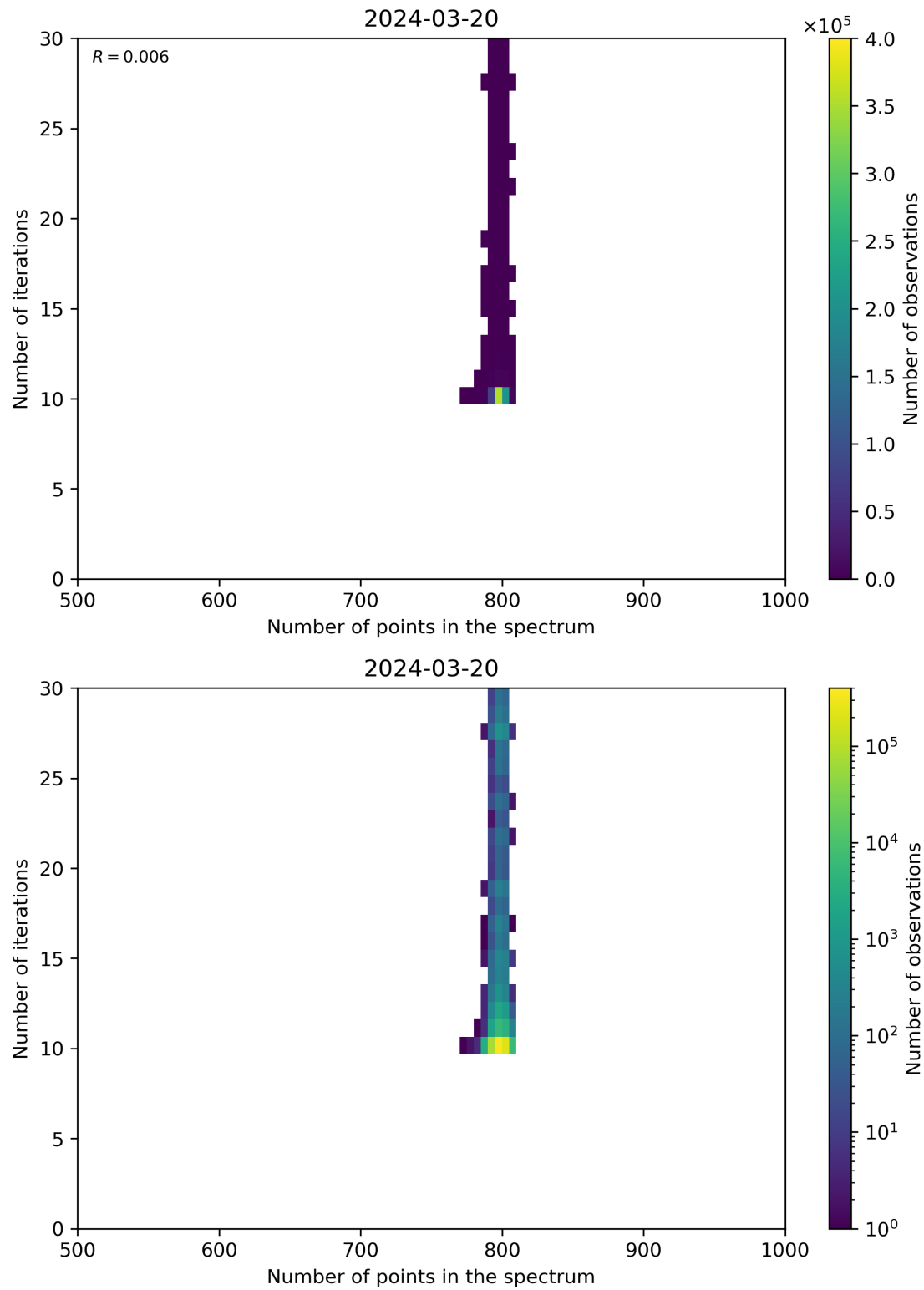
Figure 92: Scatter density plot of “Number of points in the spectrum” against “Number of iterations” for 2024-03-20 to 2024-03-21.
