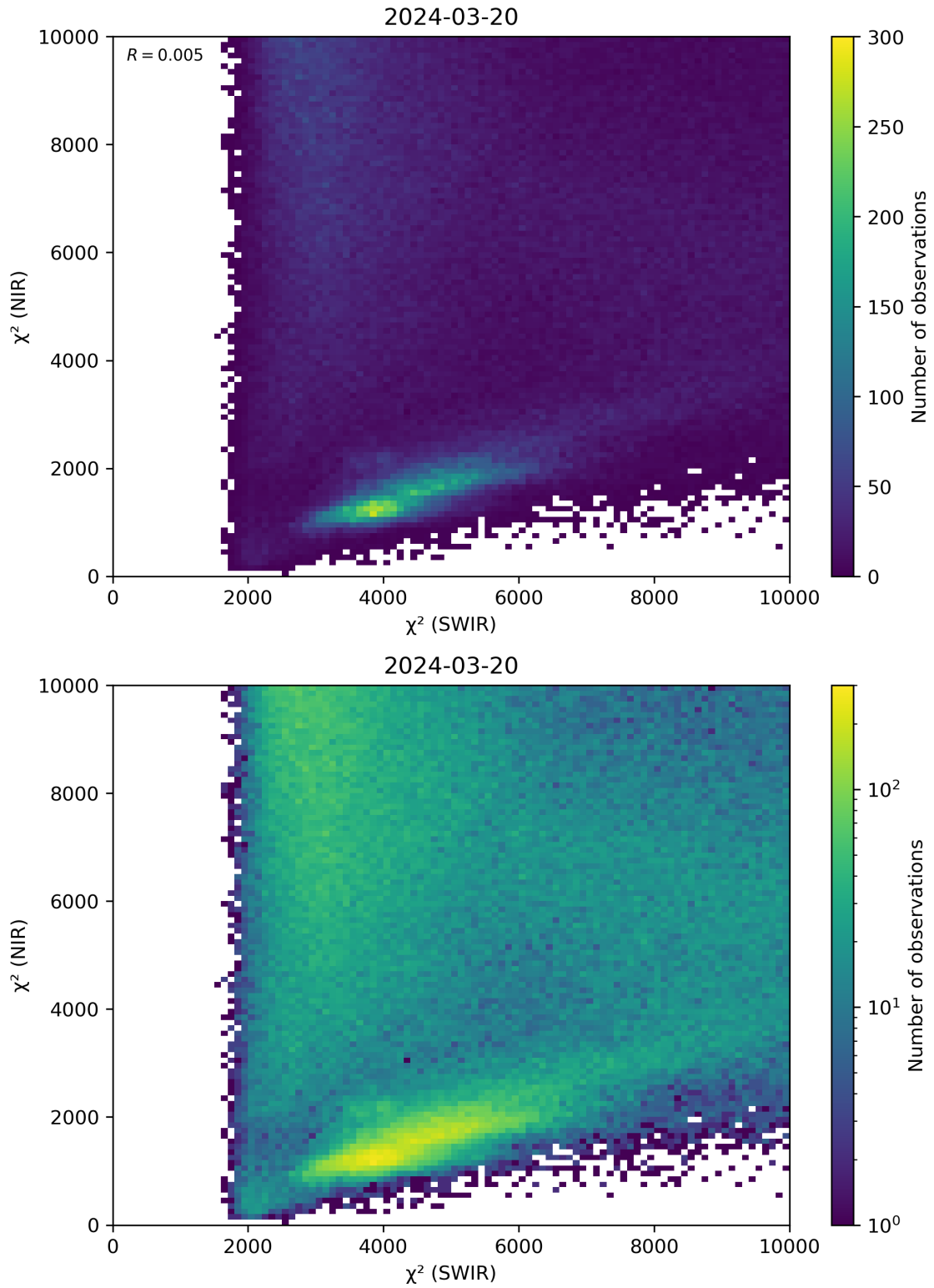
Figure 47: Scatter density plot of “ \chi^2 (SWIR)” against “ \chi^2 (NIR)” for 2024-03-20 to 2024-03-21.
