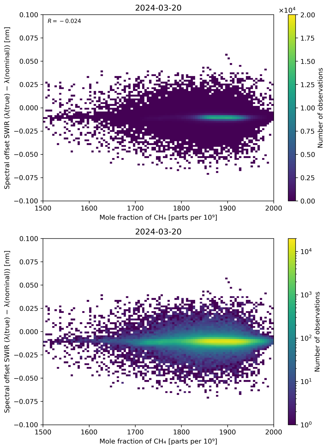
Figure 86: Scatter density plot of “Mole fraction of CH 4 ” against “Spectral offset SWIR ( \lambda(\text{true}) - \lambda(\text{nominal}) )” for 2024-03-20 to 2024-03-21.
