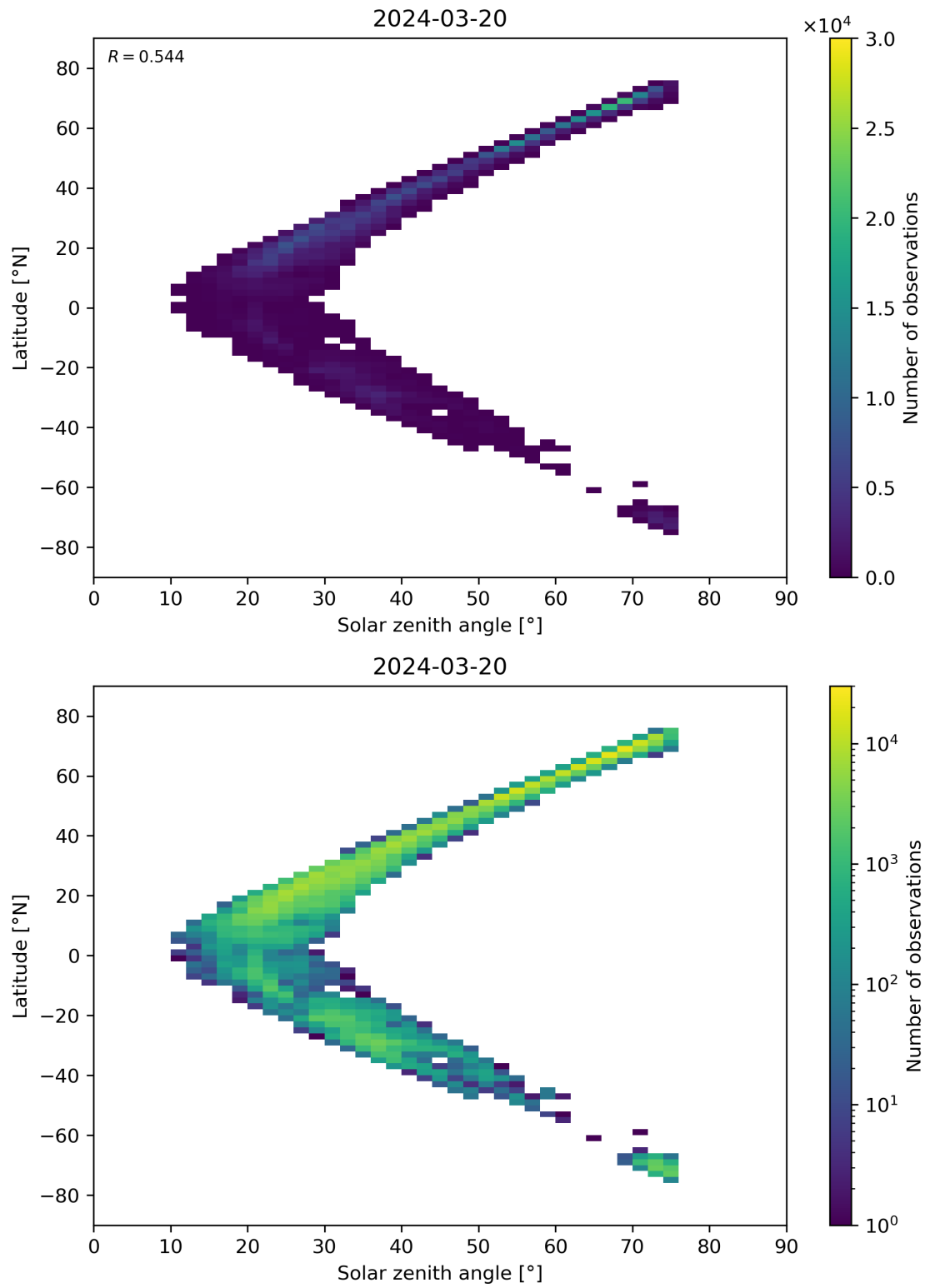
Figure 98: Scatter density plot of “Solar zenith angle” against “Latitude” for 2024-03-20 to 2024-03-21.
