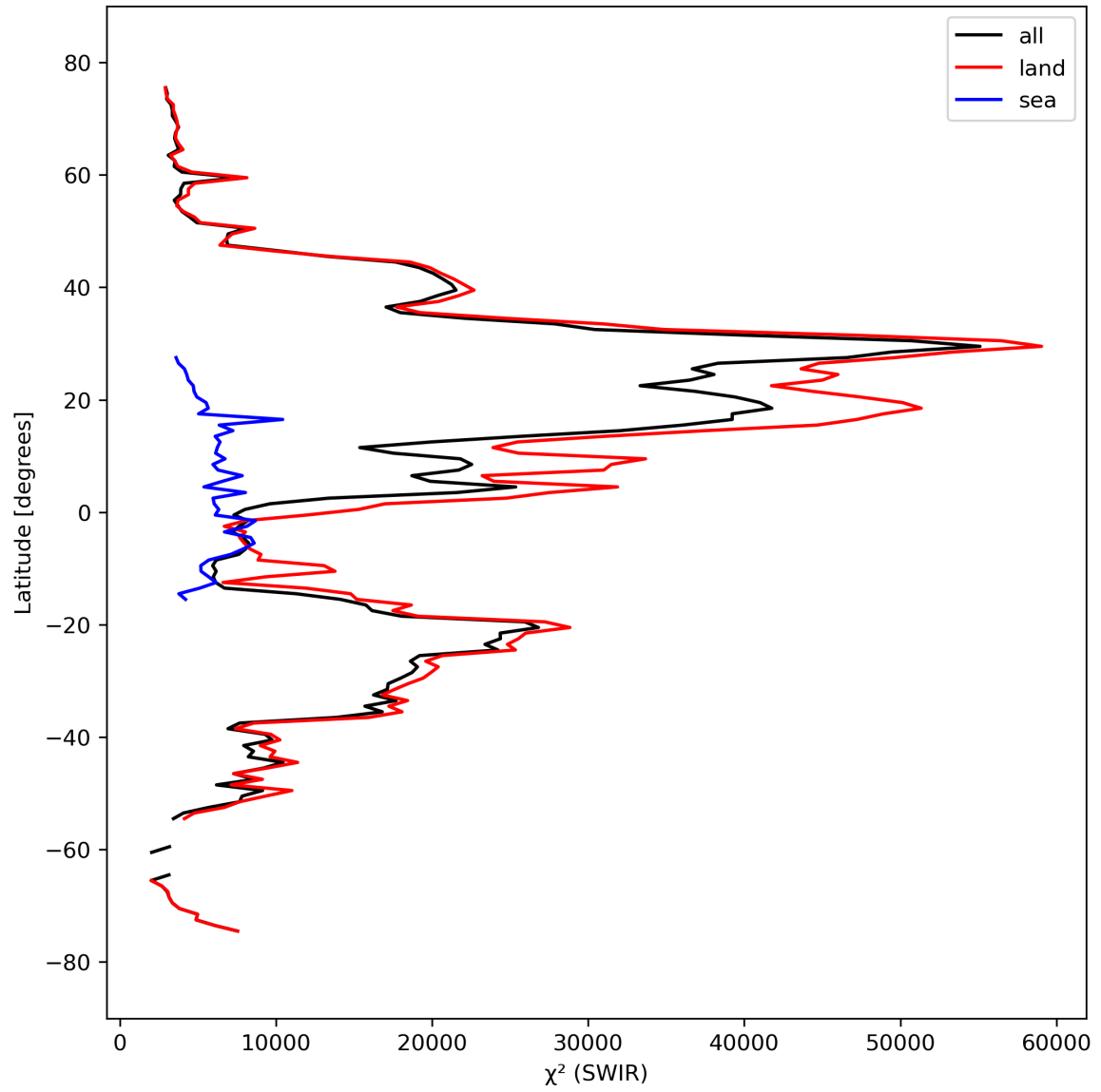
Figure 17: Zonal average of “ \chi^2 (SWIR)” for 2024-03-20 to 2024-03-21.
