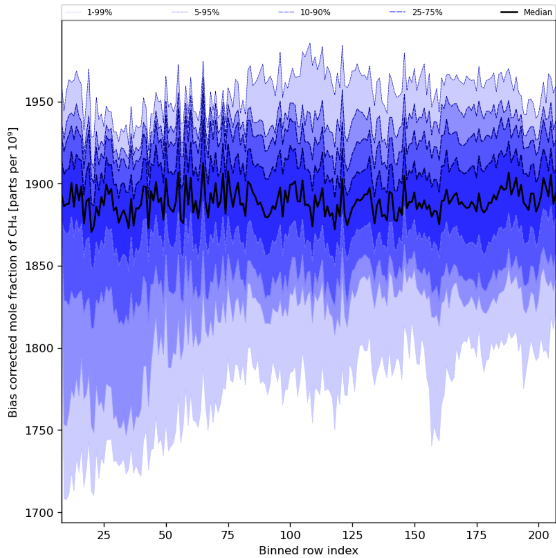
Figure 36: Along track statistics of “Bias corrected mole fraction of CH 4 ” for 2024-03-20 to 2024-03-21
