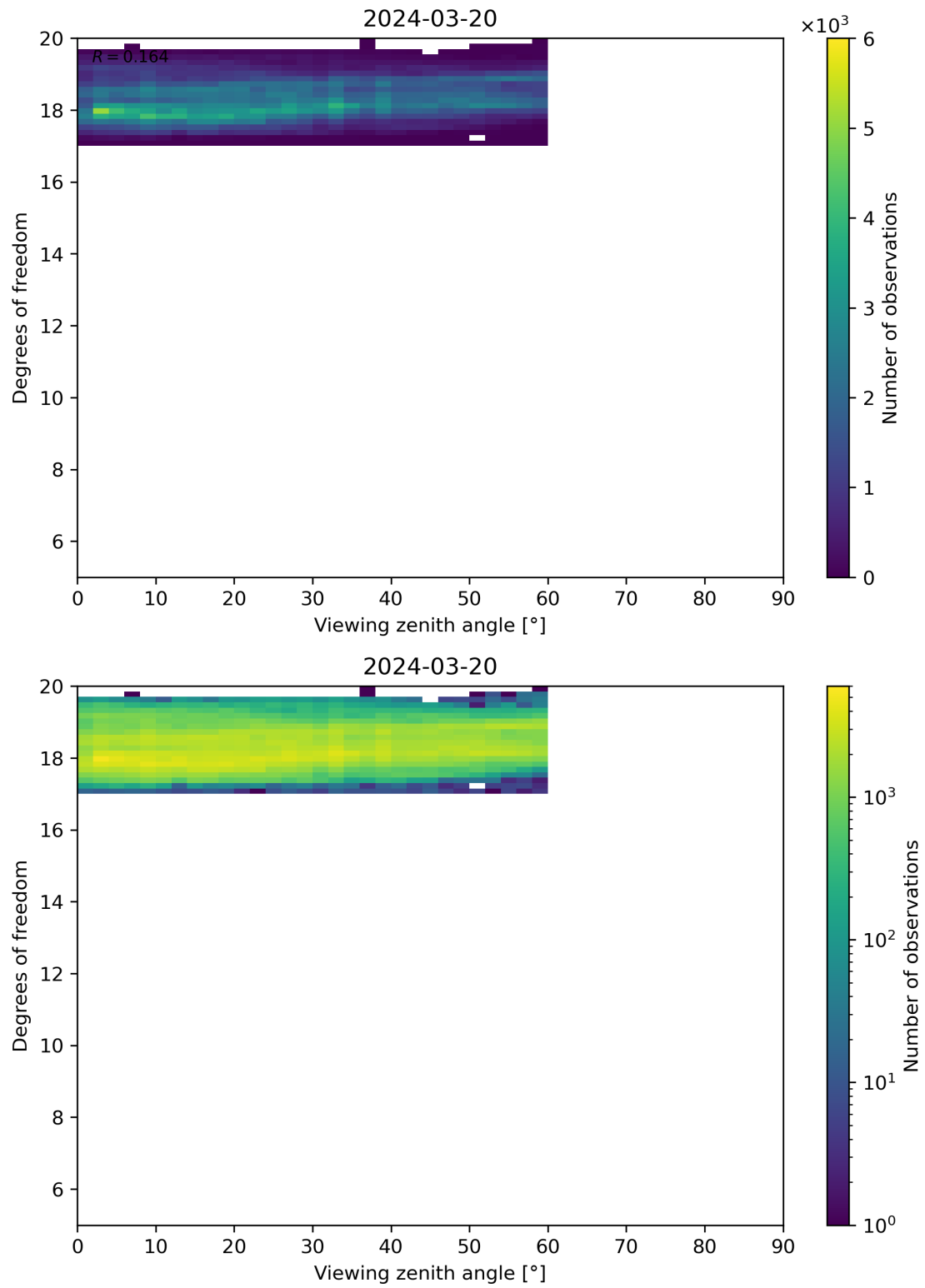
Figure 107: Scatter density plot of “Viewing zenith angle” against “Degrees of freedom” for 2024-03-20 to 2024-03-21.
