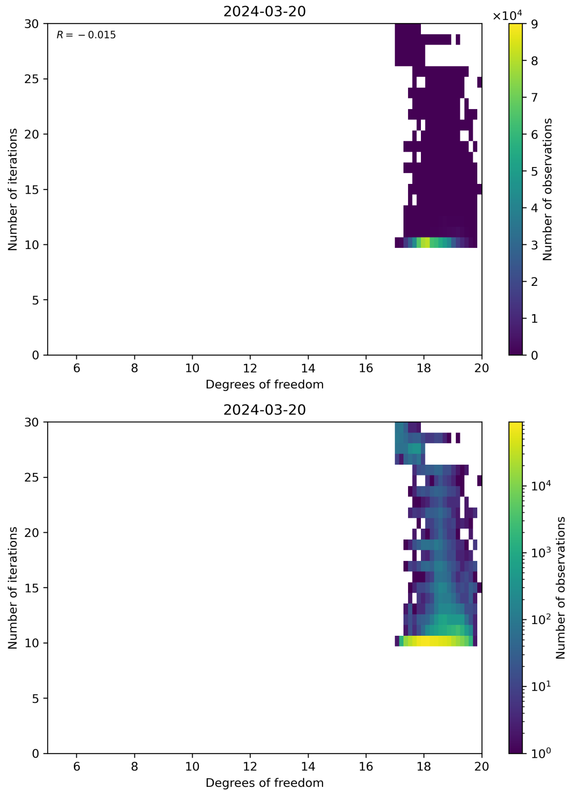
Figure 52: Scatter density plot of “Degrees of freedom” against “Number of iterations” for 2024-03-20 to 2024-03-21.
