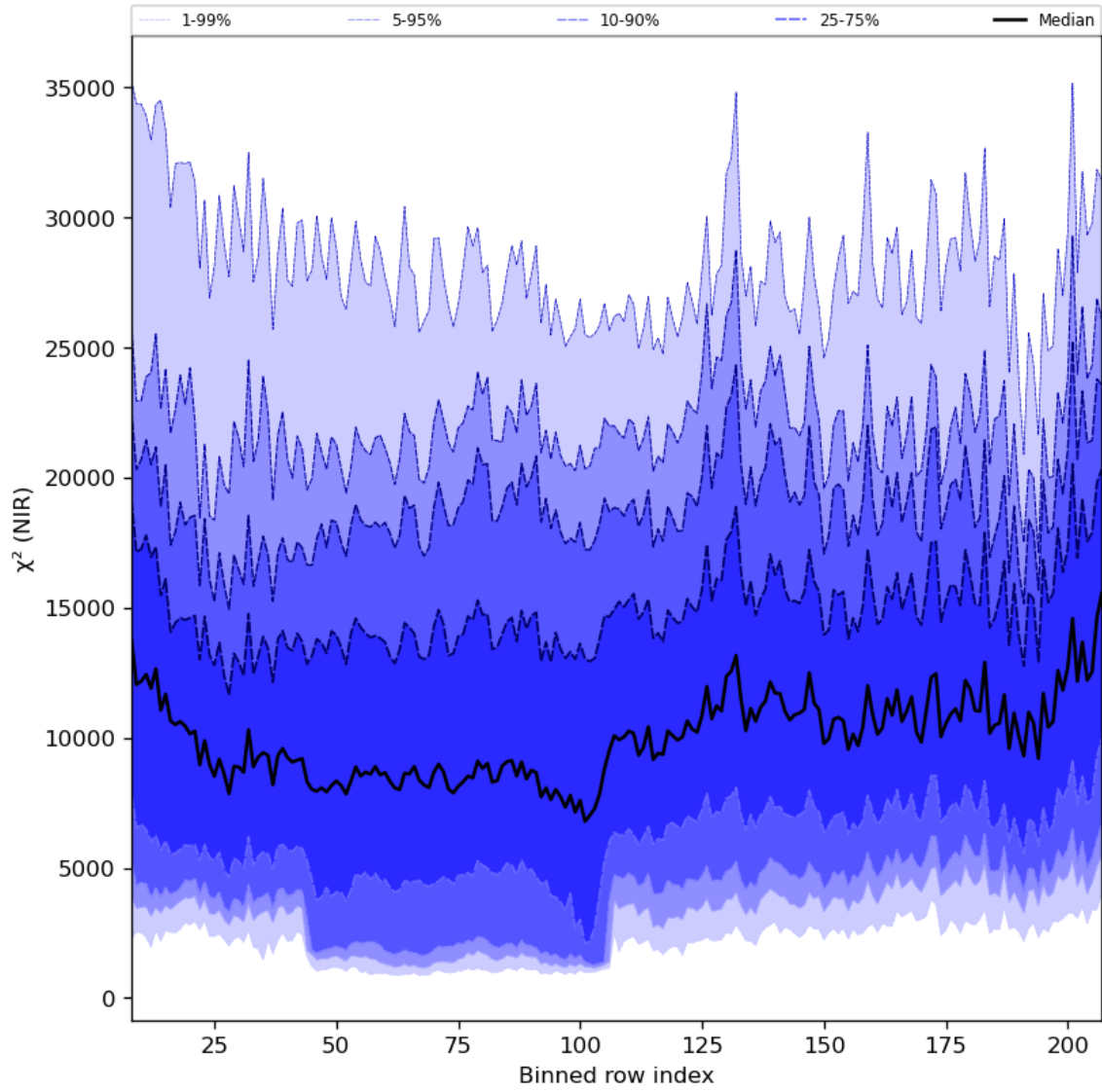
Figure 40: Along track statistics of “ \chi^2 (NIR)” for 2024-03-20 to 2024-03-21
