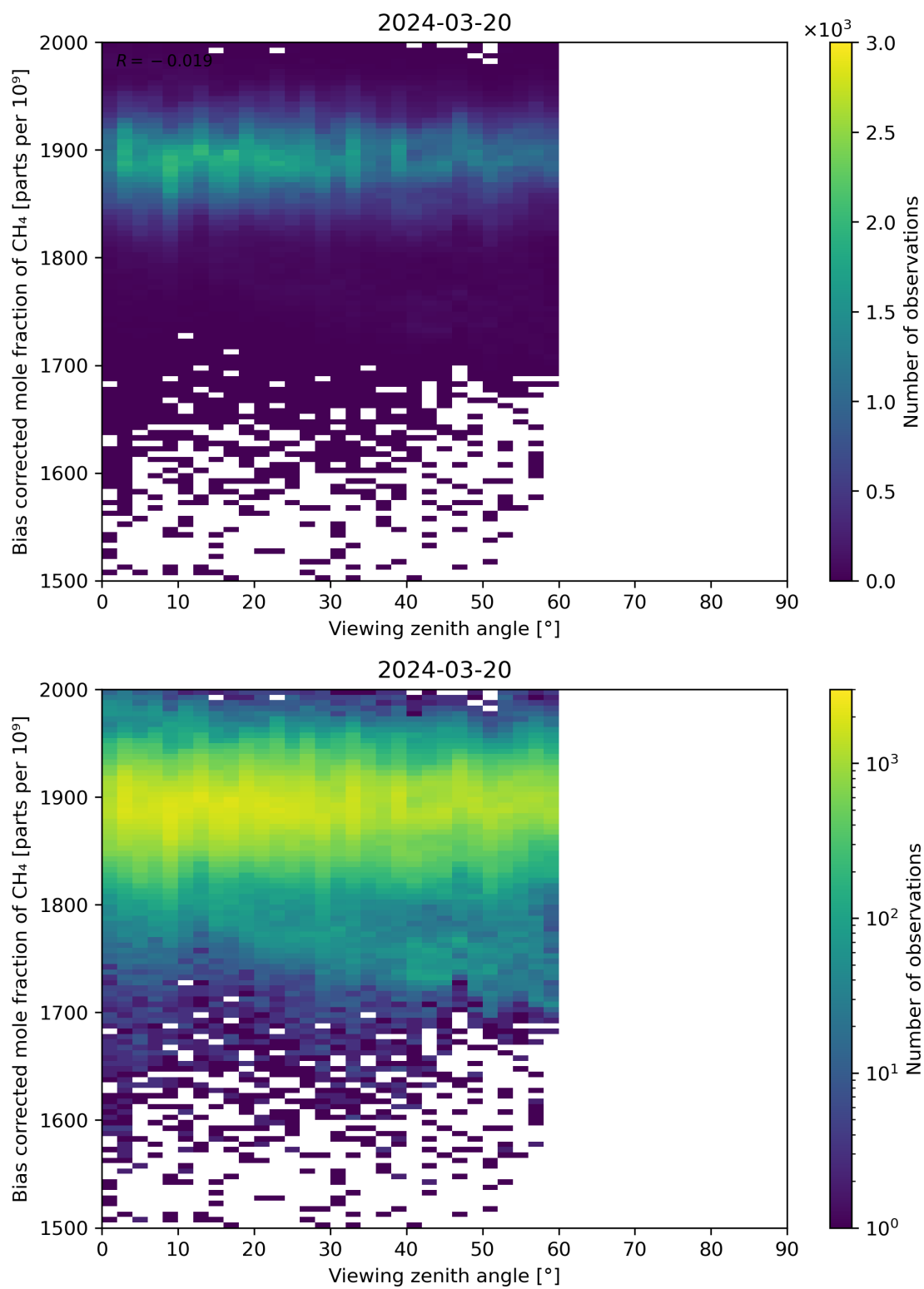
Figure 111: Scatter density plot of “Viewing zenith angle” against “Bias corrected mole fraction of CH 4 ” for 2024-03-20 to 2024-03-21.
