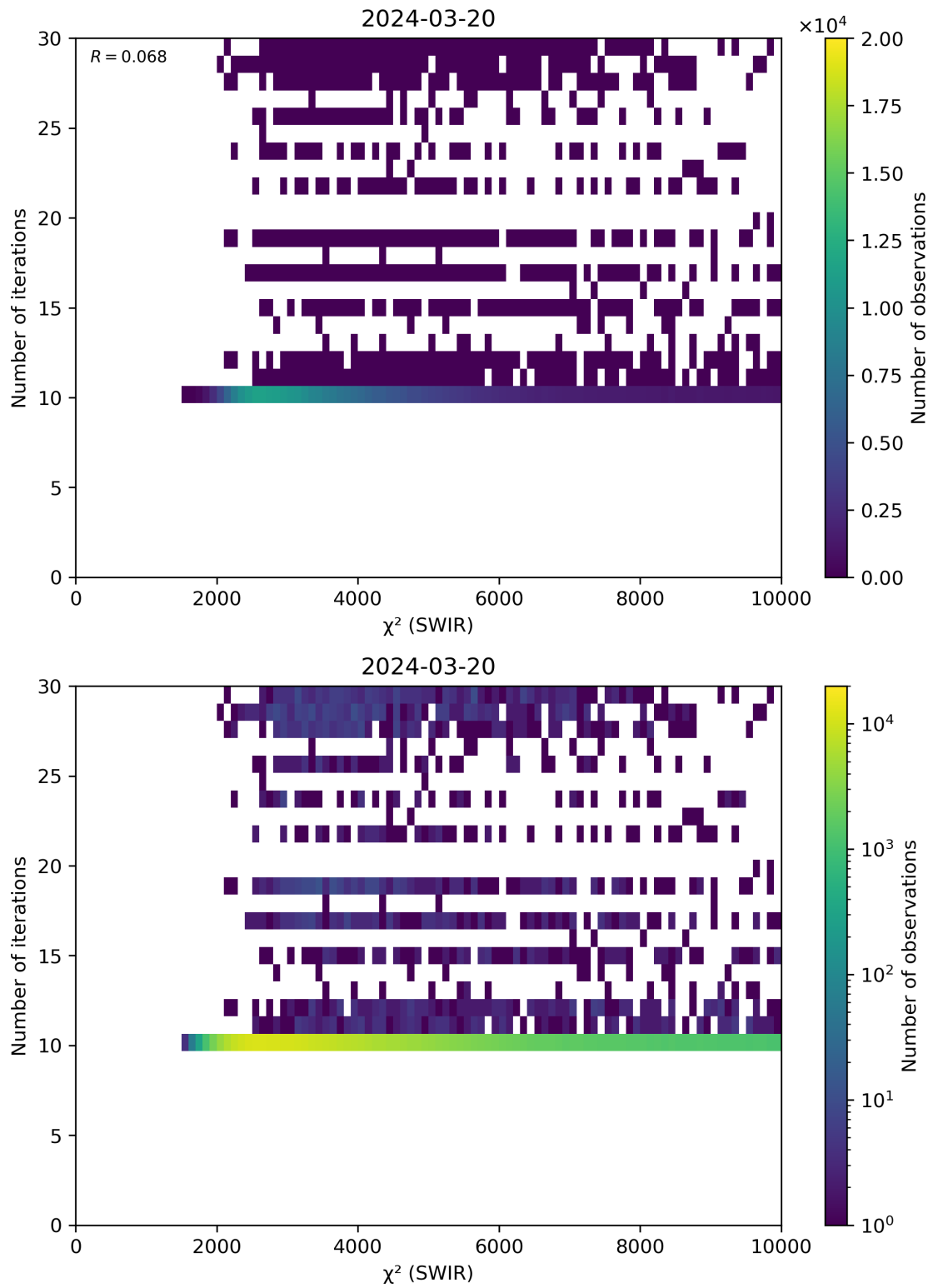
Figure 50: Scatter density plot of “ \chi^2 (SWIR)” against “Number of iterations” for 2024-03-20 to 2024-03-21.
