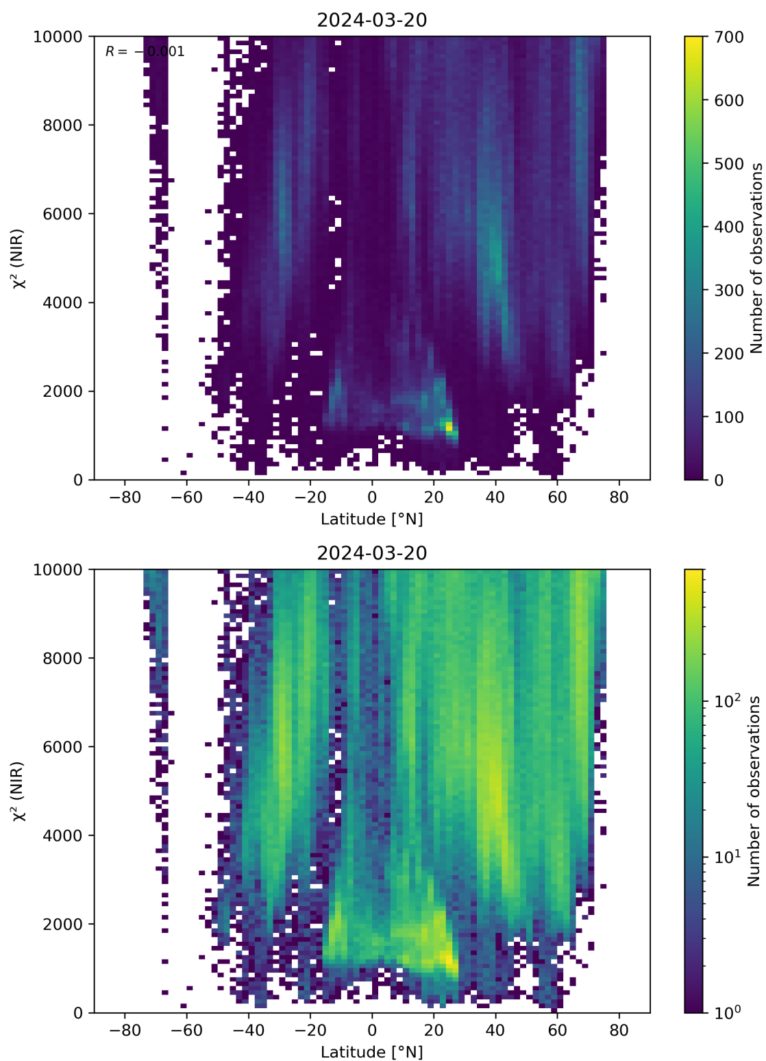
Figure 53: Scatter density plot of “Latitude” against “ \chi^2 (NIR)” for 2024-03-20 to 2024-03-21.
