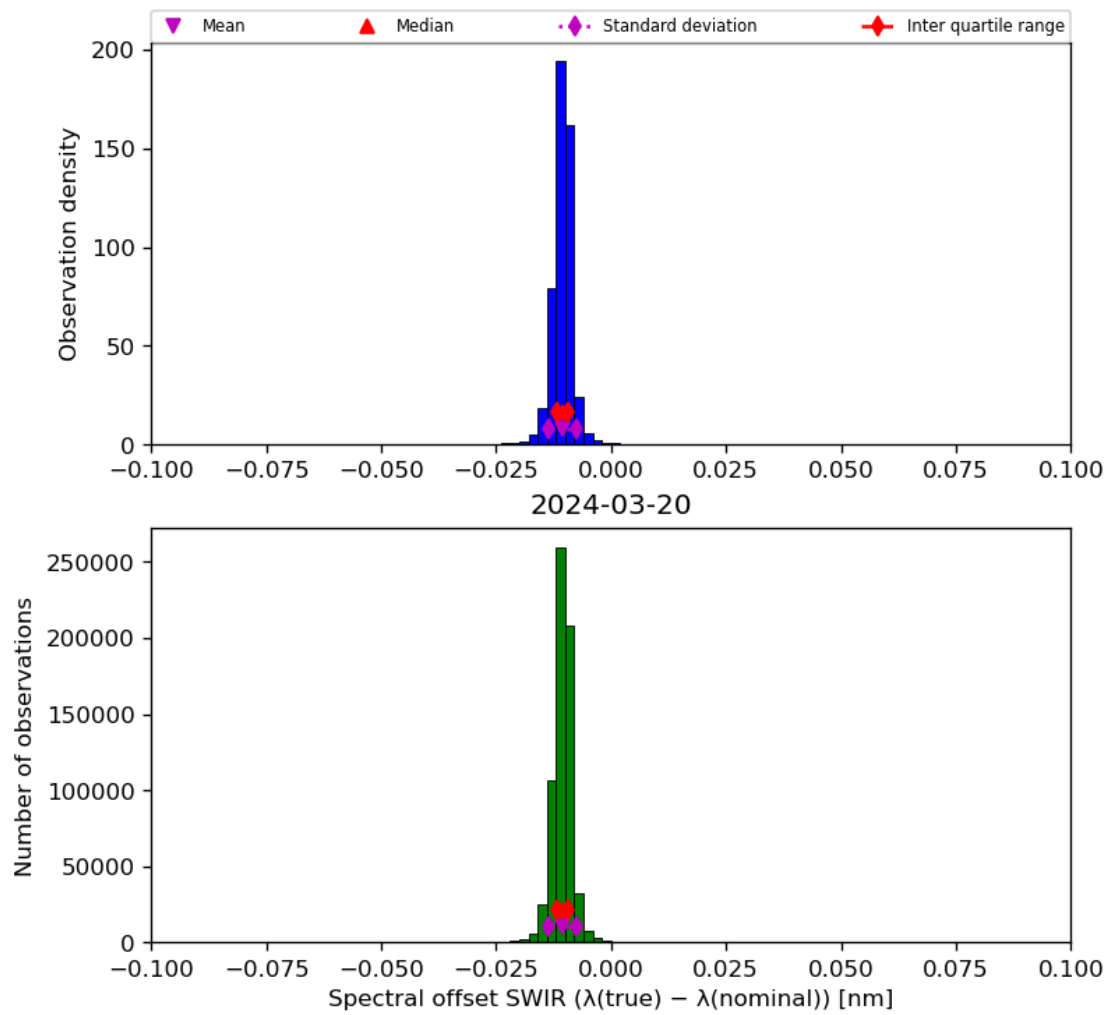
Figure 27: Histogram of “Spectral offset SWIR ( \lambda(\text{true}) - \lambda(\text{nominal}) )” for 2024-03-20 to 2024-03-21
