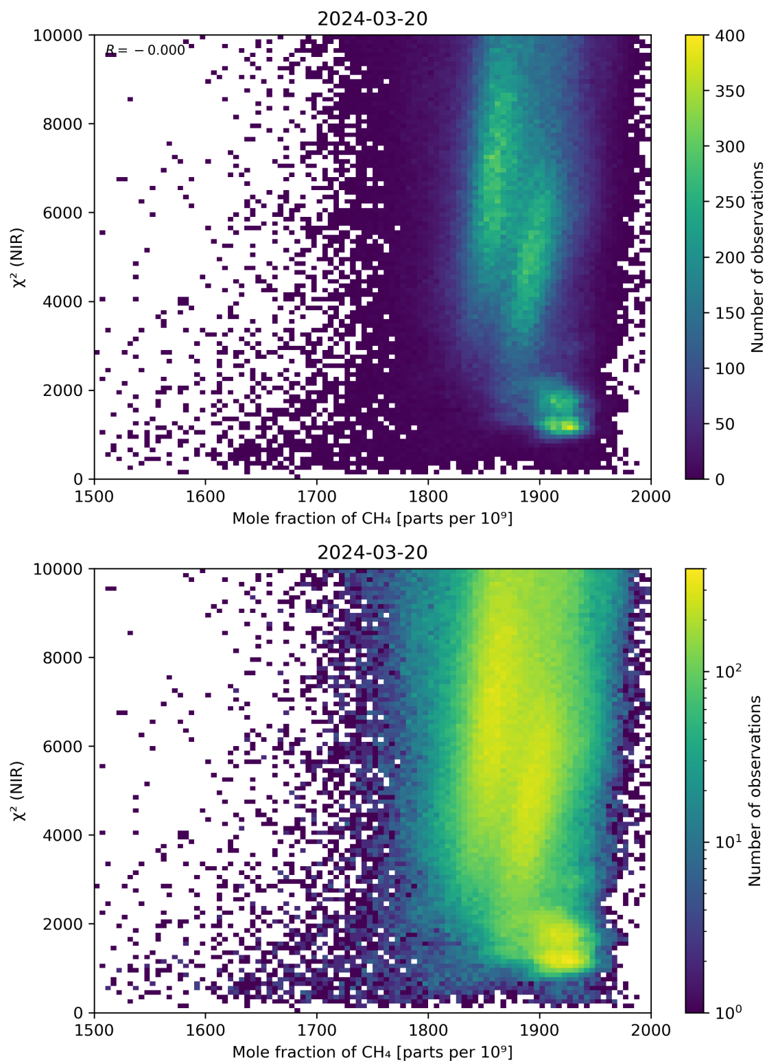
Figure 70: Scatter density plot of “Mole fraction of \text{CH}_4 ” against “ \chi^2 (NIR)” for 2024-03-20 to 2024-03-21.
