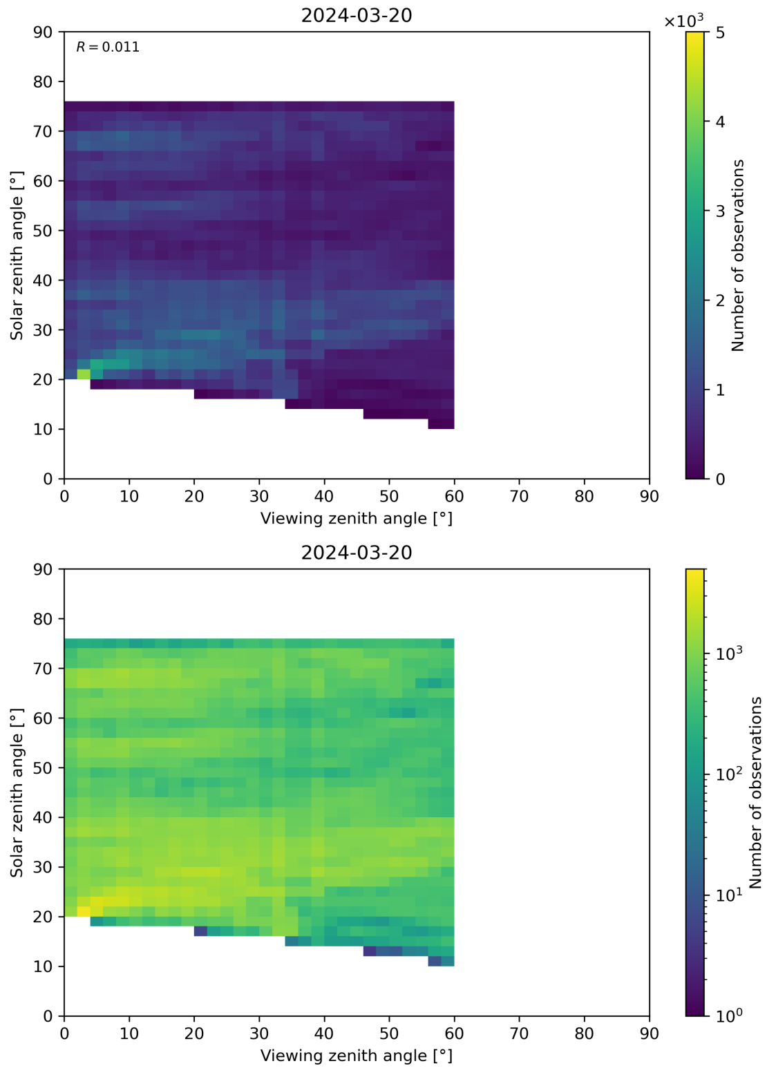
Figure 115: Scatter density plot of “Viewing zenith angle” against “Solar zenith angle” for 2024-03-20 to 2024-03-21.
