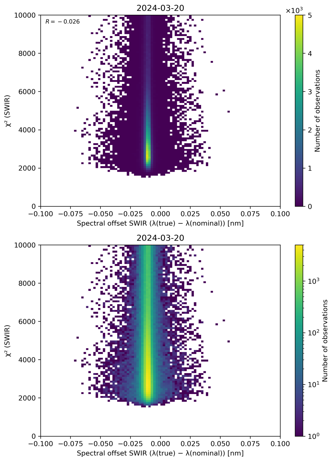
Figure 118: Scatter density plot of “Spectral offset SWIR ( \lambda(\text{true}) - \lambda(\text{nominal}) )” against “ \chi^2 (SWIR)” for 2024-03-20 to 2024-03-21.
