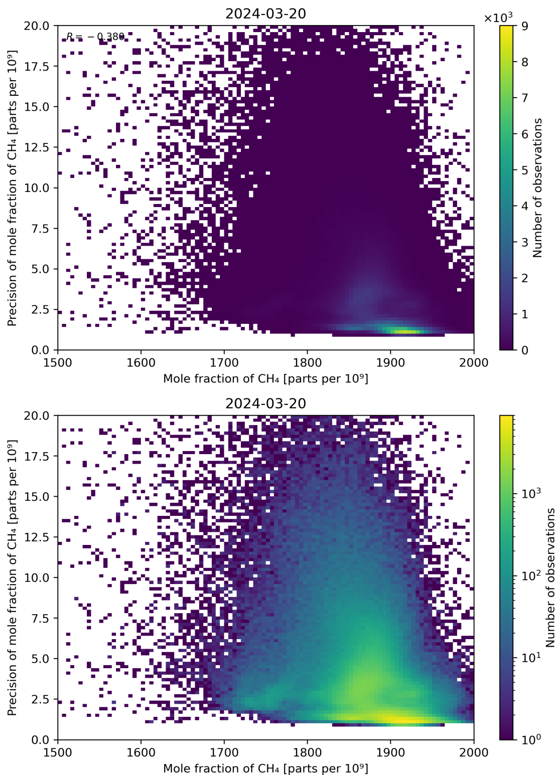
Figure 75: Scatter density plot of “Mole fraction of CH 4 ” against “Precision of mole fraction of CH 4 ” for 2024-03-20 to 2024-03-21.
