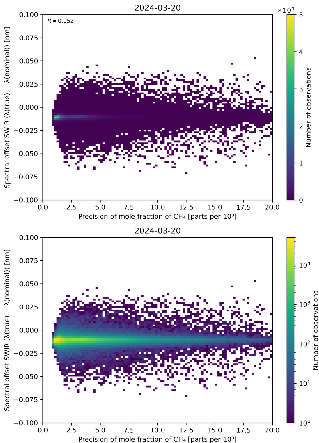
Figure 85: Scatter density plot of “Precision of mole fraction of CH 4 ” against “Spectral offset SWIR ( \lambda(\text{true}) - \lambda(\text{nominal}) )” for 2024-03-20 to 2024-03-21.
