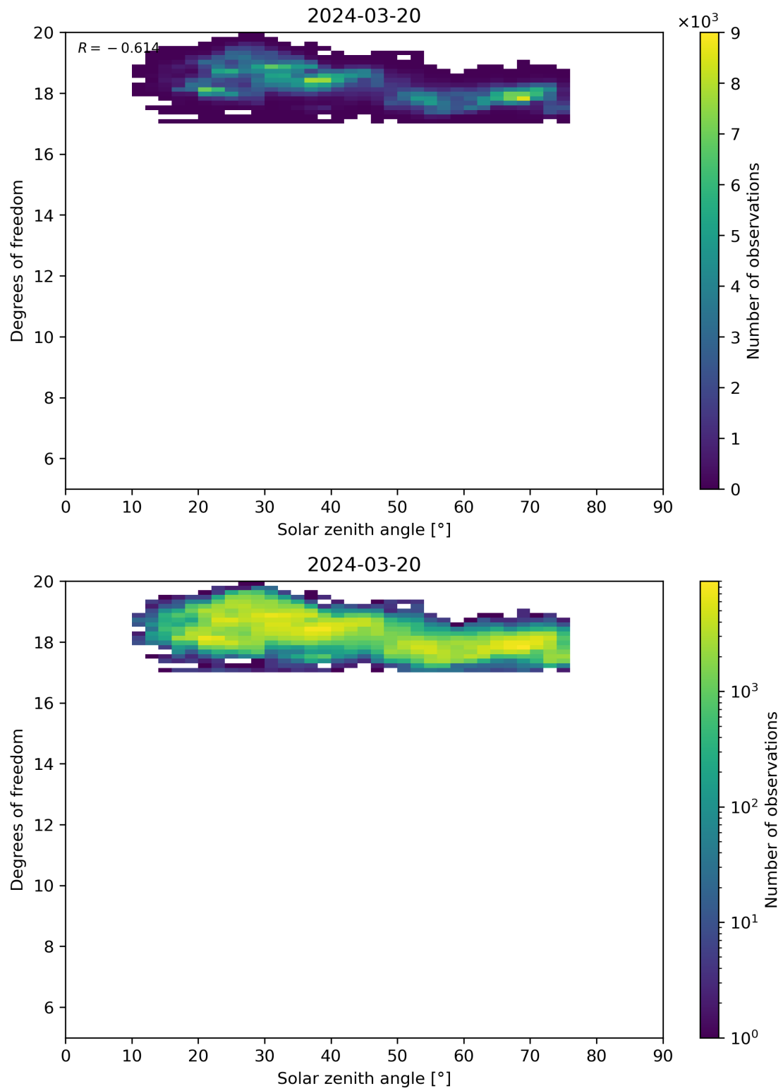
Figure 96: Scatter density plot of “Solar zenith angle” against “Degrees of freedom” for 2024-03-20 to 2024-03-21.
