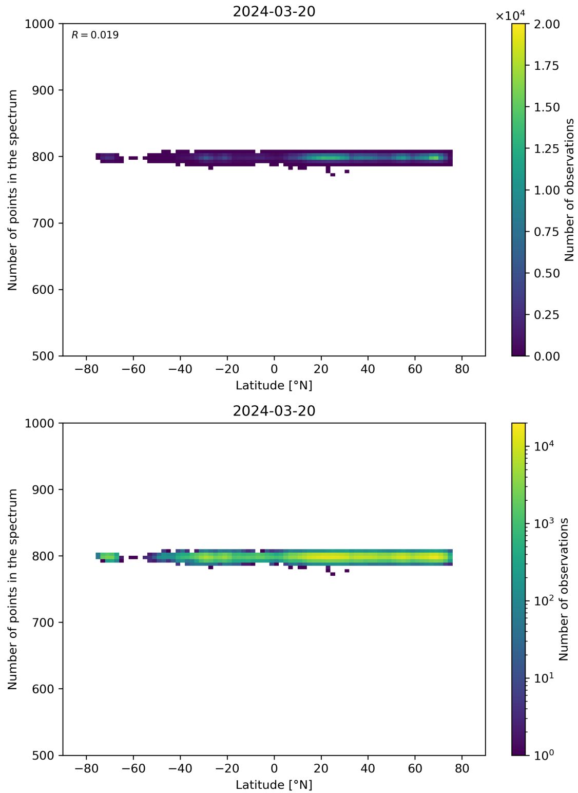
Figure 61: Scatter density plot of “Latitude” against “Number of points in the spectrum” for 2024-03-20 to 2024-03-21.
