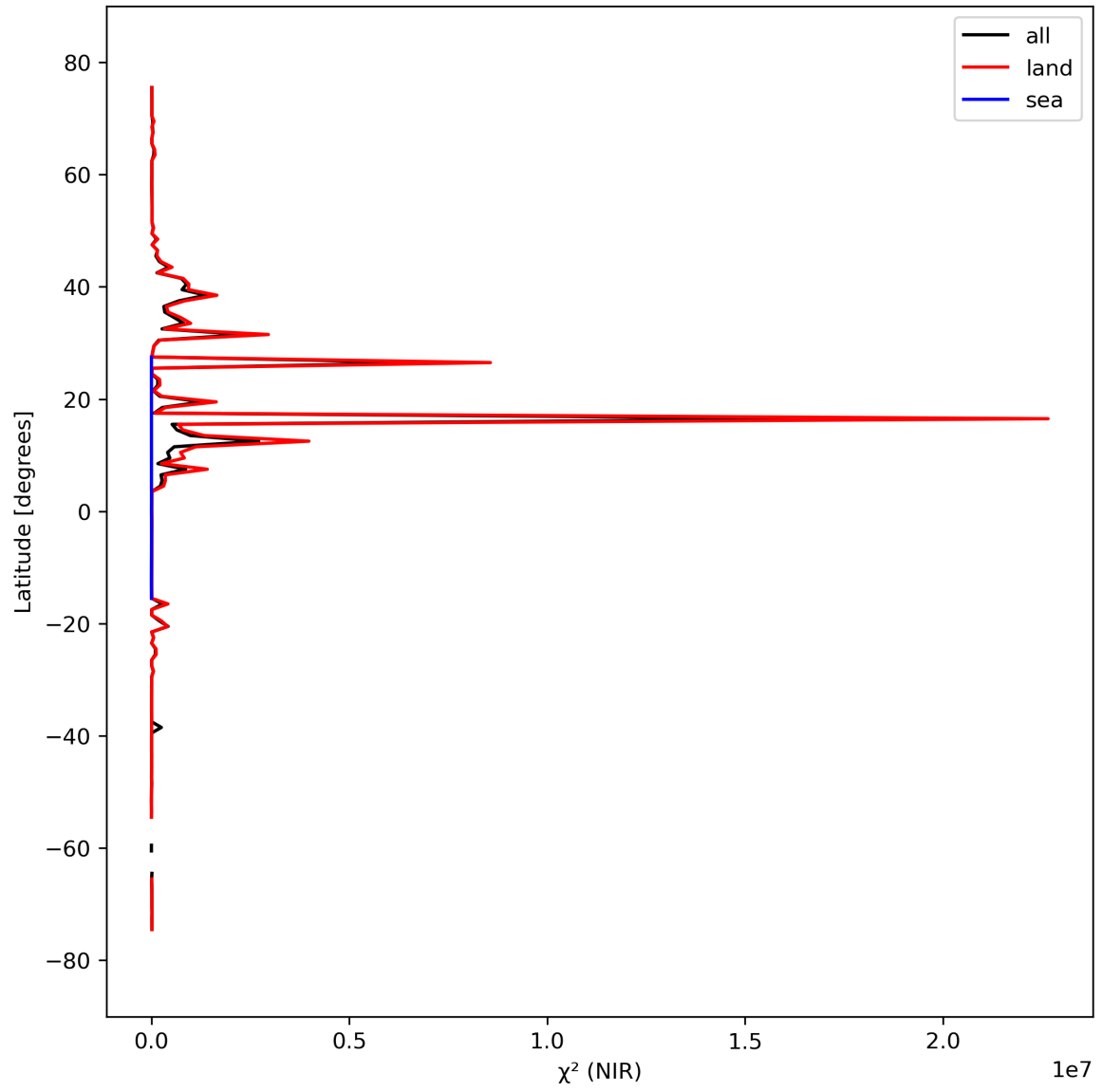
Figure 18: Zonal average of “ \chi^2 (NIR)” for 2024-03-20 to 2024-03-21.
