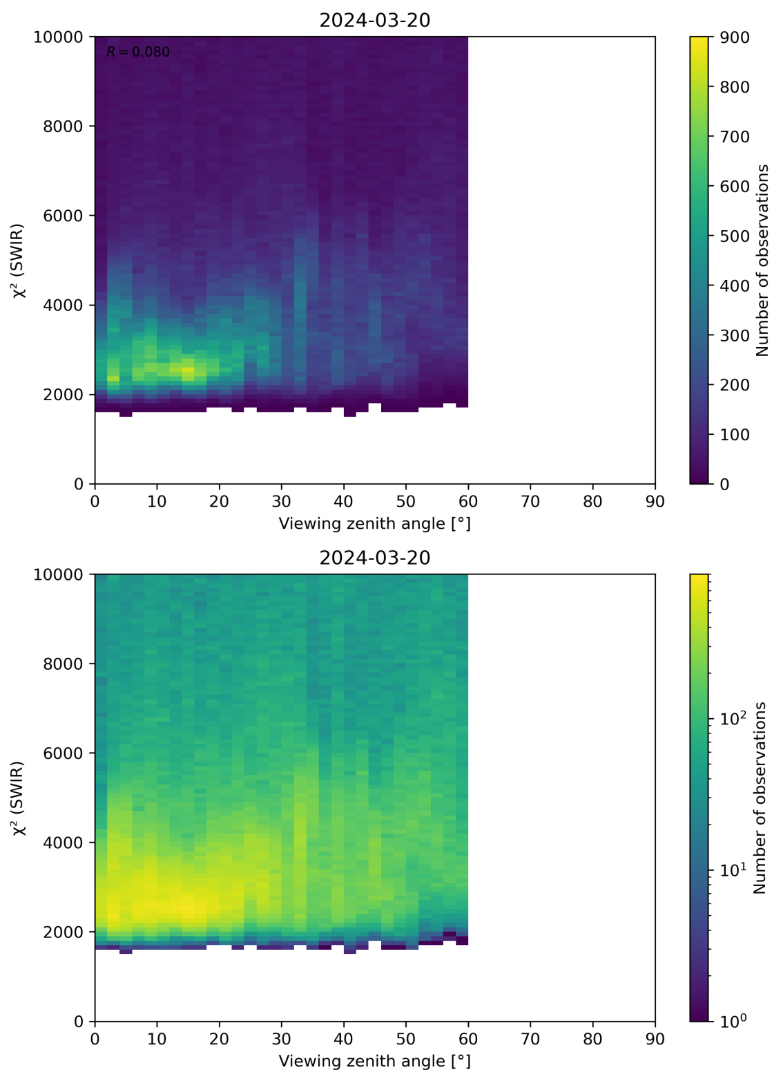
Figure 106: Scatter density plot of “Viewing zenith angle” against “ \chi^2 (SWIR)” for 2024-03-20 to 2024-03-21.
