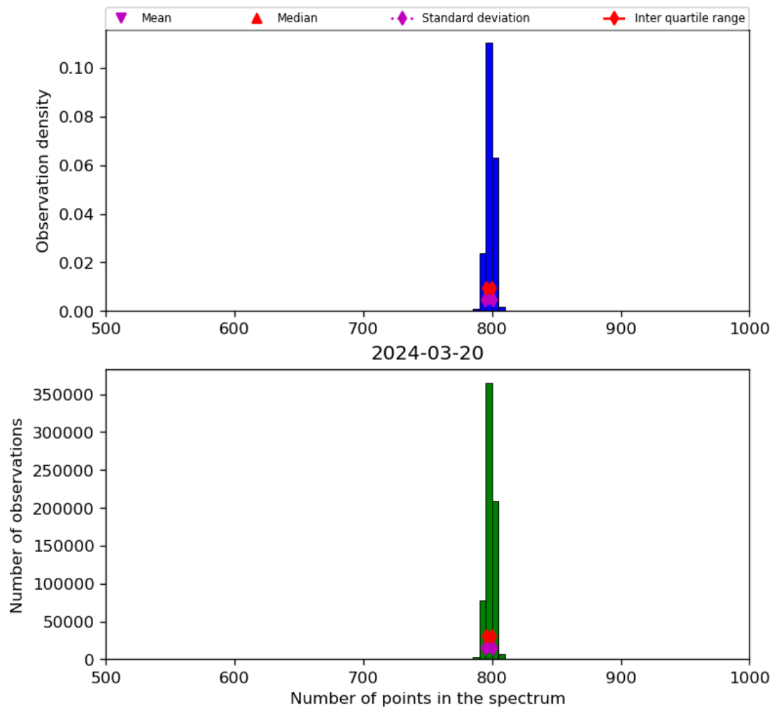
Figure 26: Histogram of “Number of points in the spectrum” for 2024-03-20 to 2024-03-21
