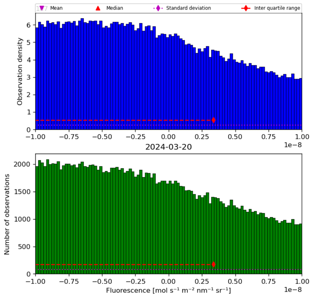
Figure 32: Histogram of “Fluorescence” for 2024-03-20 to 2024-03-21
