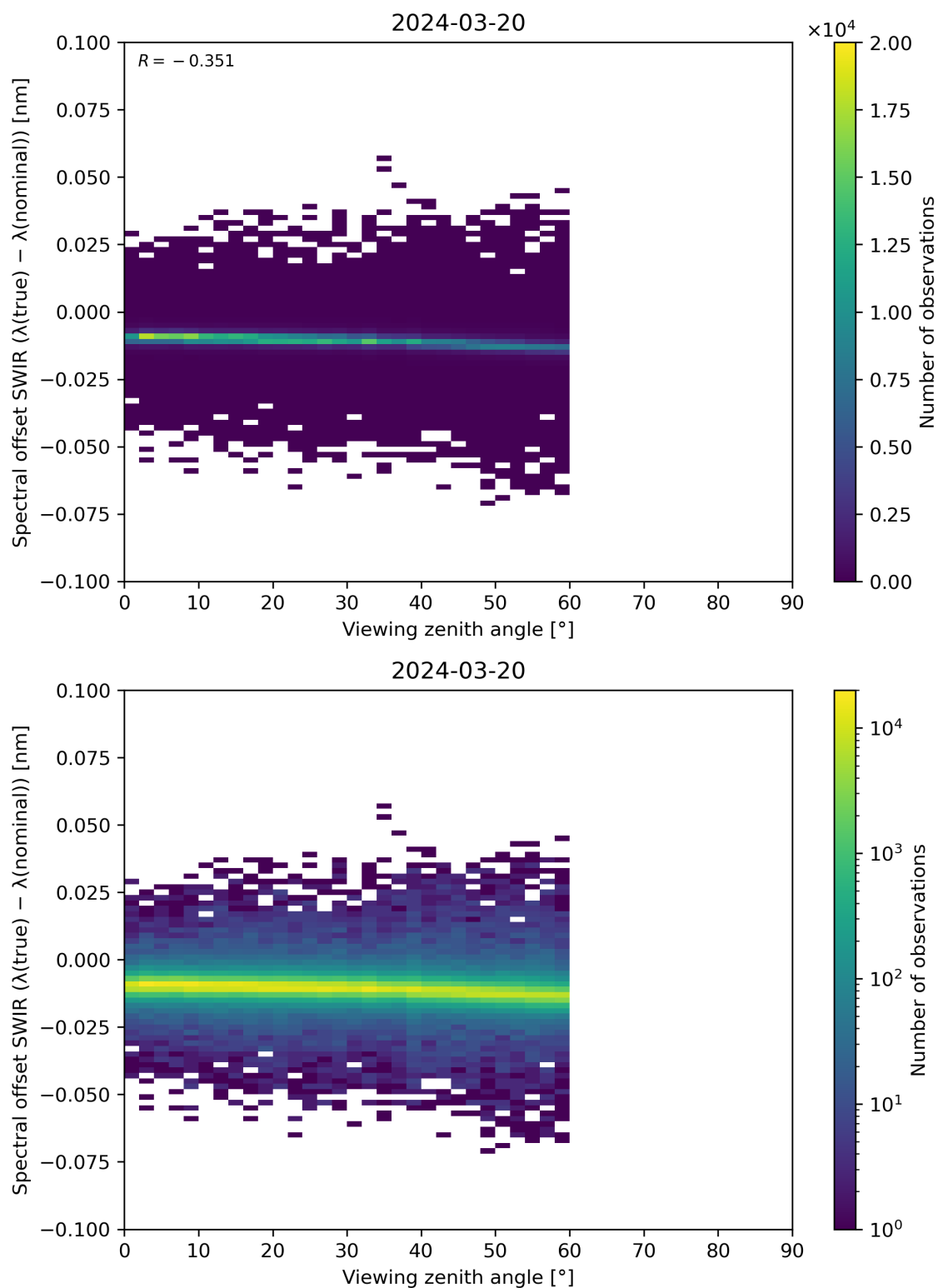
Figure 116: Scatter density plot of “Viewing zenith angle” against “Spectral offset SWIR ( \lambda(\text{true}) - \lambda(\text{nominal}) )” for 2024-03-20 to 2024-03-21.
