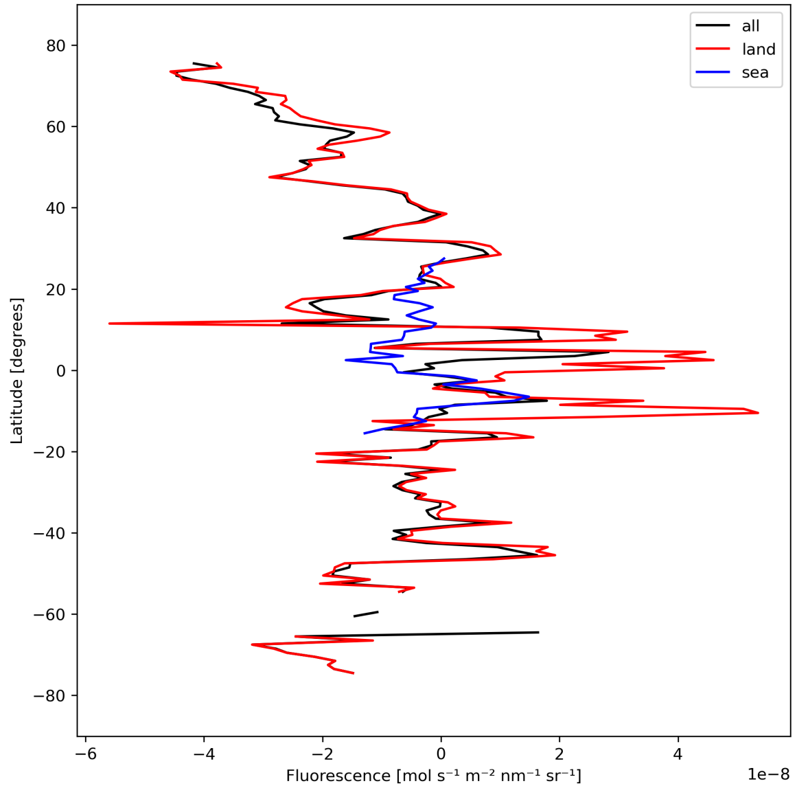
Figure 21: Zonal average of “Fluorescence” for 2024-03-20 to 2024-03-21.
