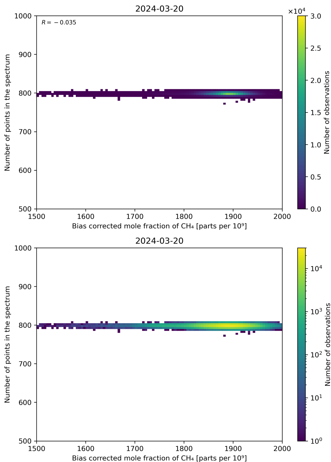
Figure 68: Scatter density plot of “Bias corrected mole fraction of CH 4 ” against “Number of points in the spectrum” for 2024-03-20 to 2024-03-21.
