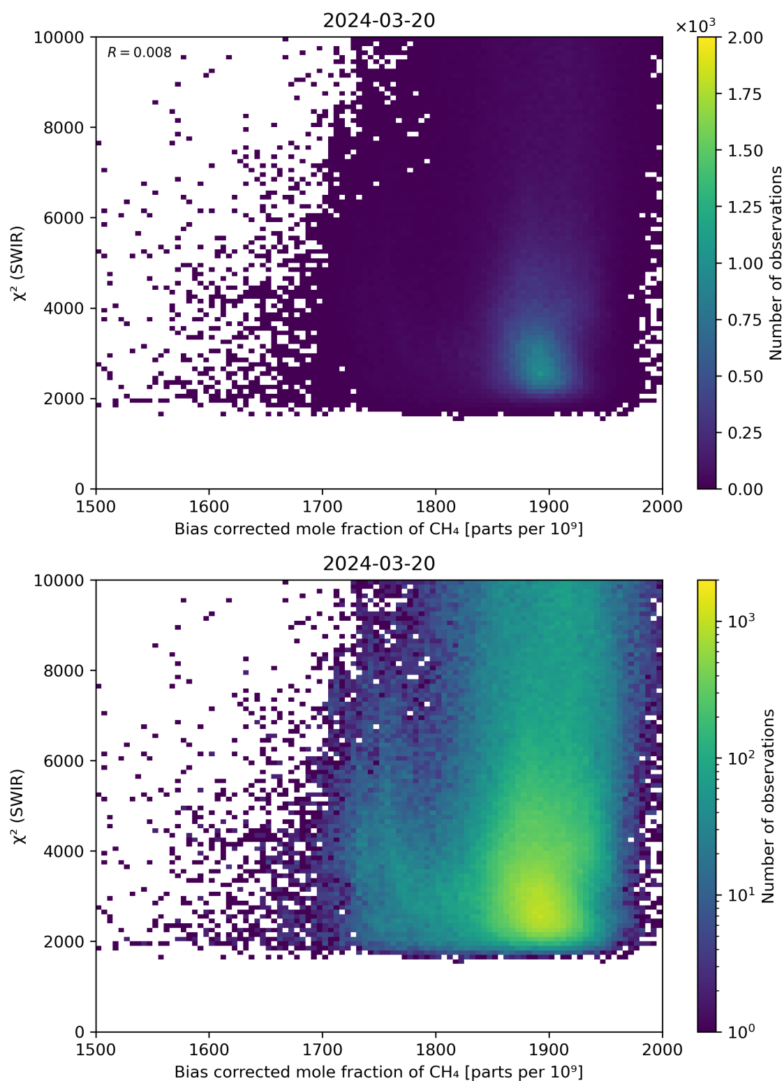
Figure 64: Scatter density plot of “Bias corrected mole fraction of \text{CH}_4 ” against “ \chi^2 (SWIR)” for 2024-03-20 to 2024-03-21.
