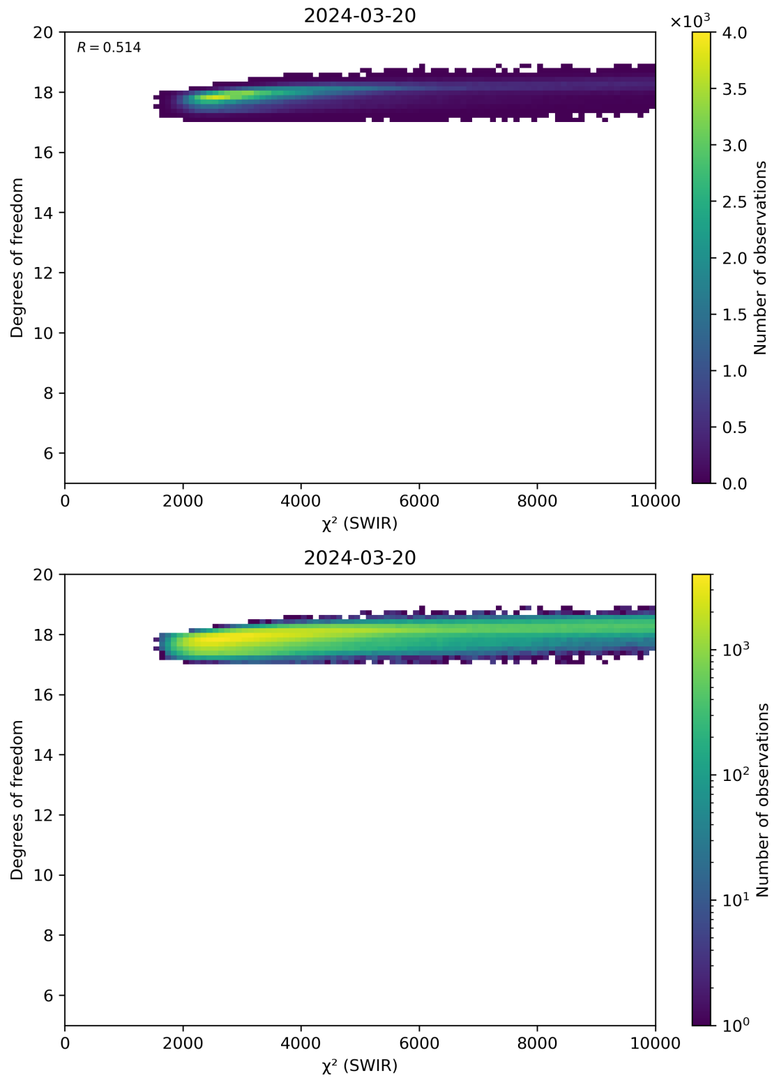
Figure 48: Scatter density plot of “ \chi^2 (SWIR)” against “Degrees of freedom” for 2024-03-20 to 2024-03-21.
