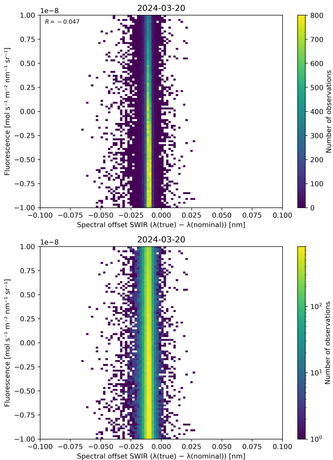
Figure 120: Scatter density plot of “Spectral offset SWIR ( \lambda(\text{true}) - \lambda(\text{nominal}) )” against “Fluorescence” for 2024-03-20 to 2024-03-21.
