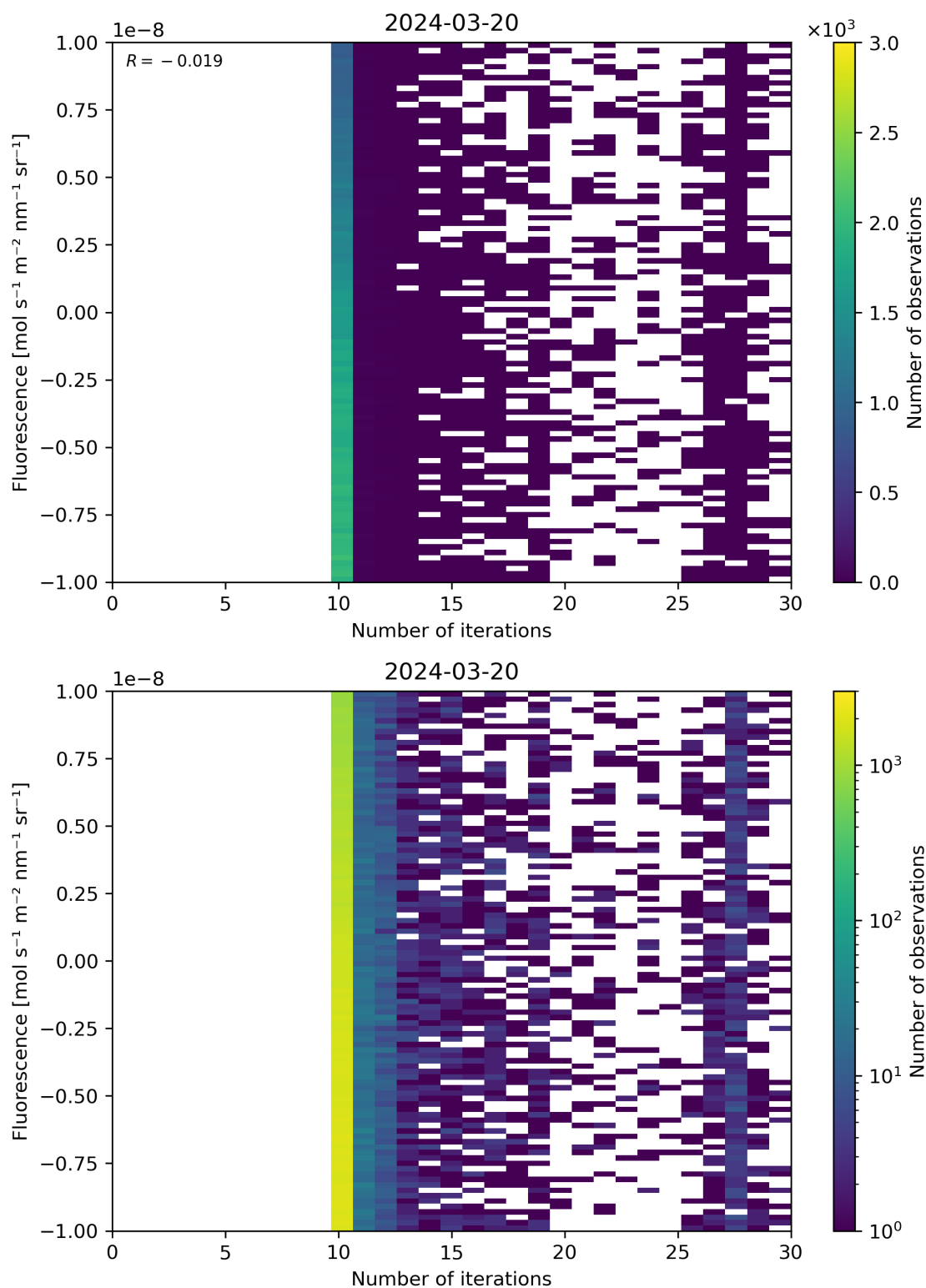
Figure 87: Scatter density plot of “Number of iterations” against “Fluorescence” for 2024-03-20 to 2024-03-21.
