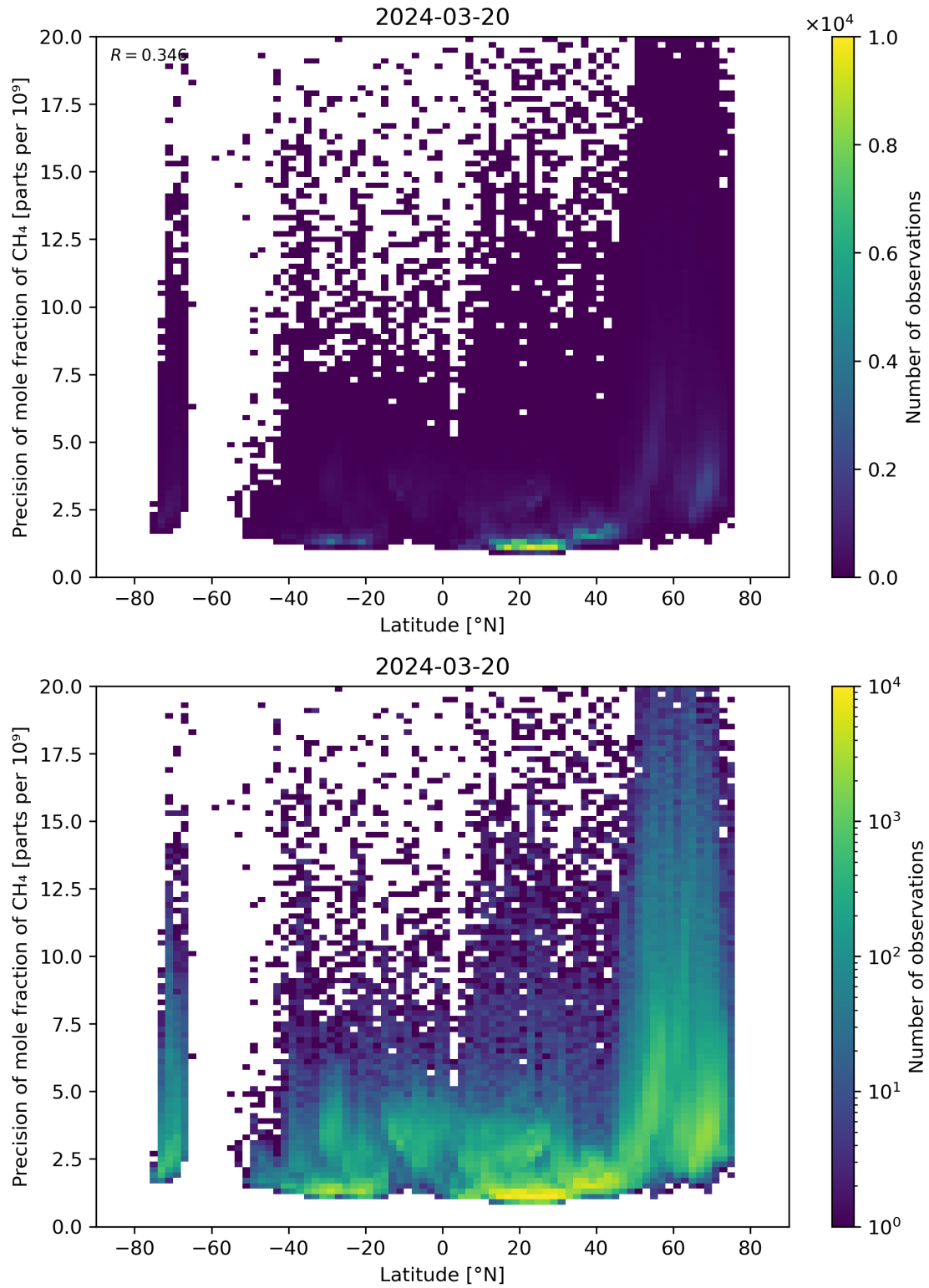
Figure 59: Scatter density plot of “Latitude” against “Precision of mole fraction of \text{CH}_4 ” for 2024-03-20 to 2024-03-21.
