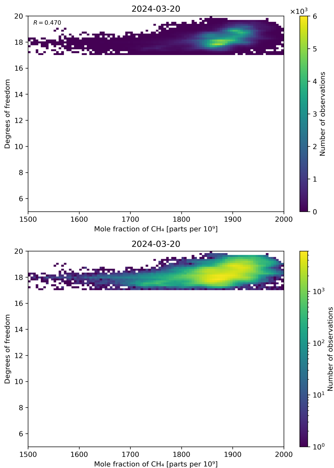
Figure 72: Scatter density plot of “Mole fraction of CH 4 ” against “Degrees of freedom” for 2024-03-20 to 2024-03-21.
