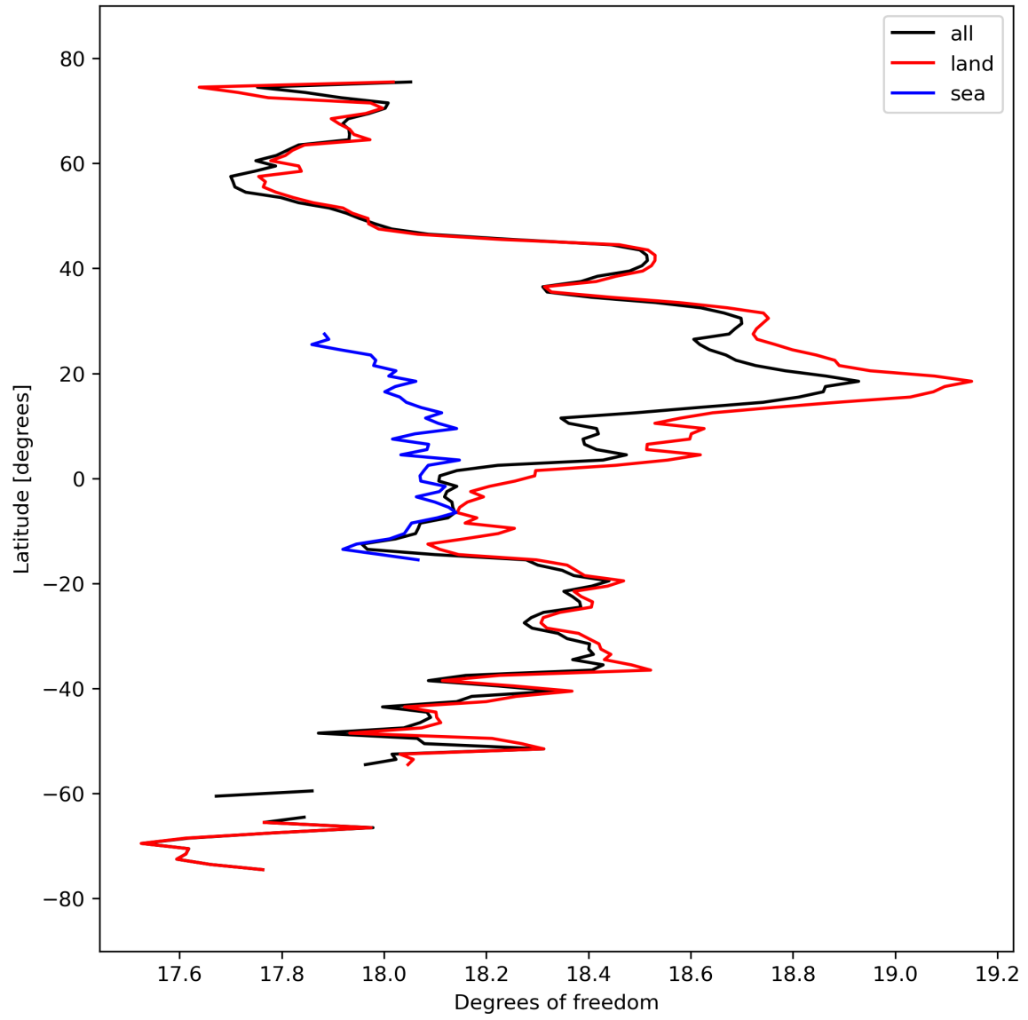
Figure 19: Zonal average of “Degrees of freedom” for 2024-03-20 to 2024-03-21.
