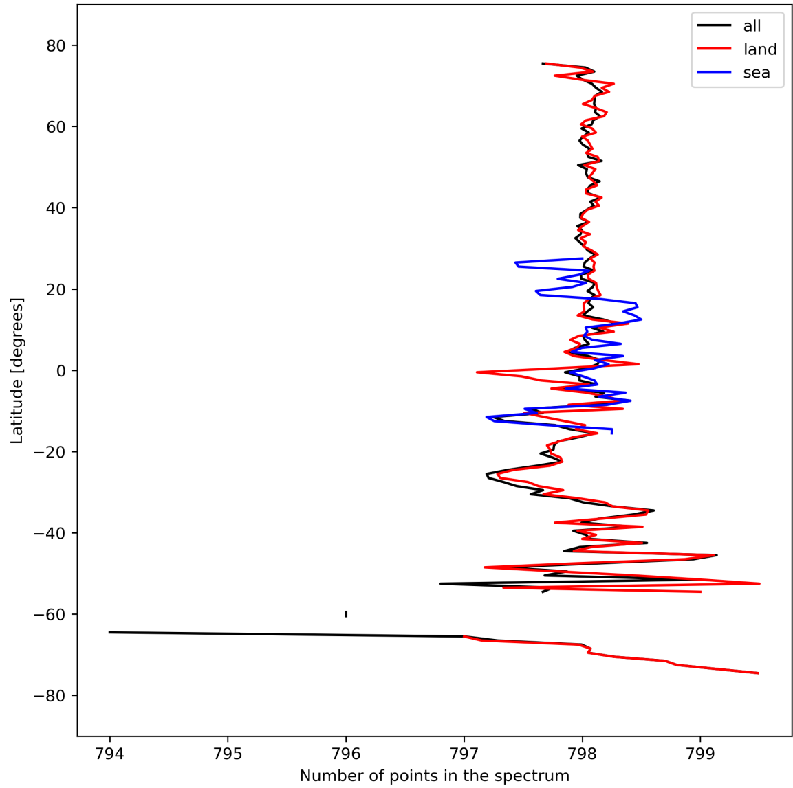
Figure 15: Zonal average of “Number of points in the spectrum” for 2024-03-20 to 2024-03-21.
