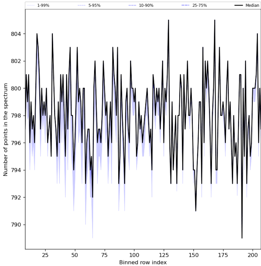
Figure 37: Along track statistics of “Number of points in the spectrum” for 2024-03-20 to 2024-03-21
