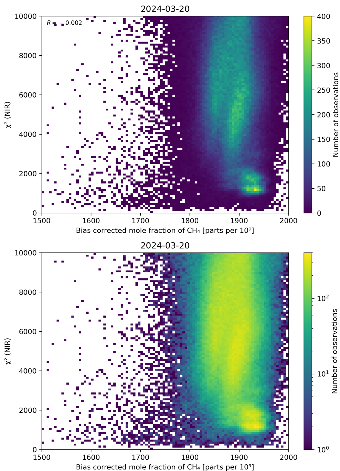
Figure 63: Scatter density plot of “Bias corrected mole fraction of CH 4 ” against “ \chi^2 (NIR)” for 2024-03-20 to 2024-03-21.
