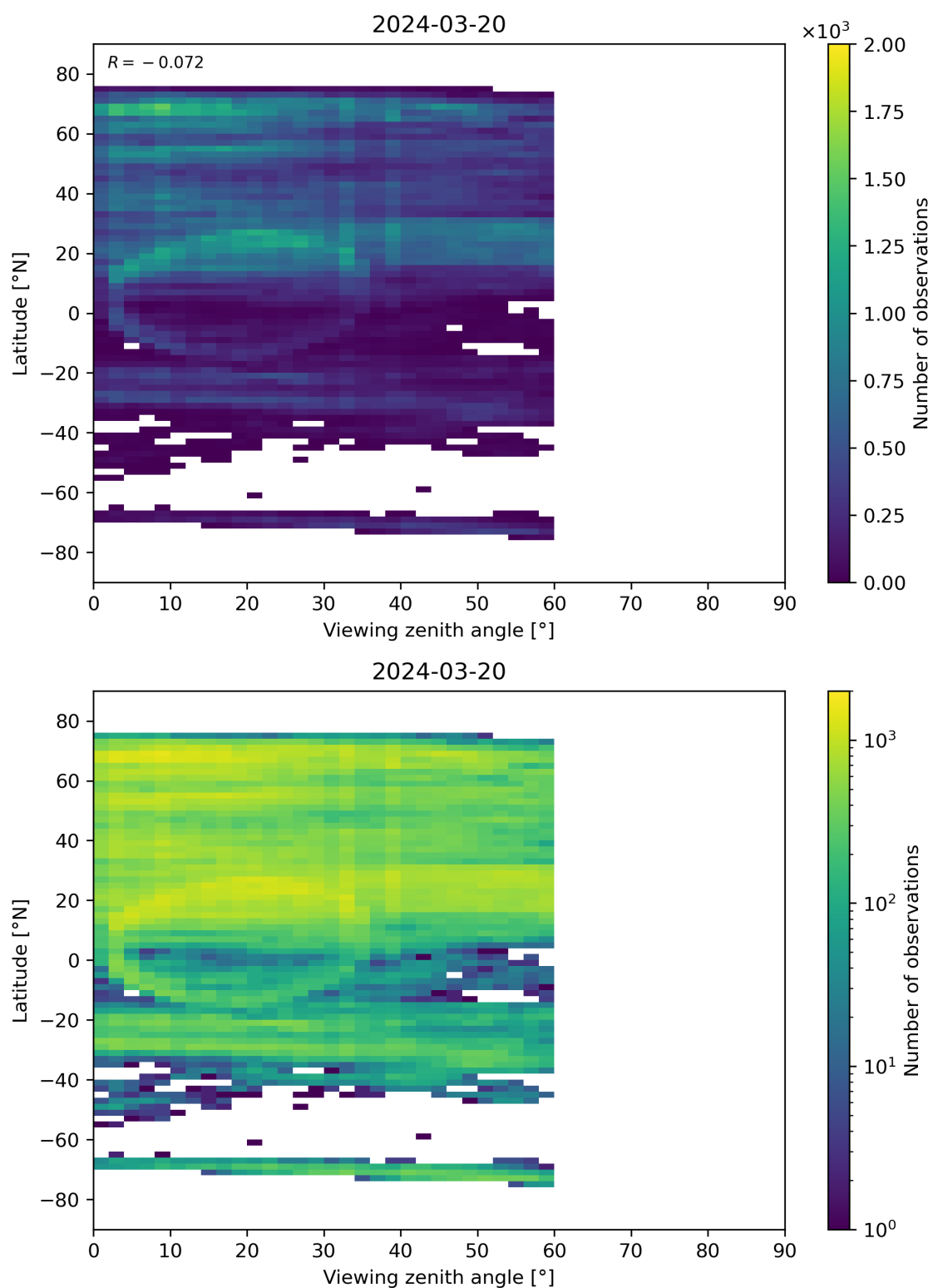
Figure 109: Scatter density plot of “Viewing zenith angle” against “Latitude” for 2024-03-20 to 2024-03-21.
