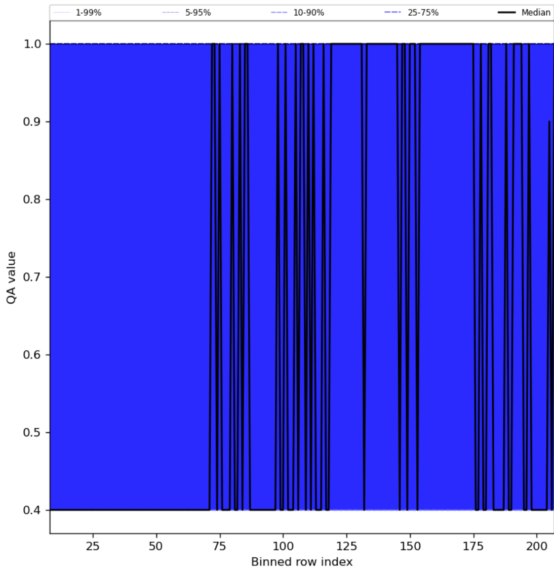
Figure 33: Along track statistics of “QA value” for 2024-03-20 to 2024-03-21
